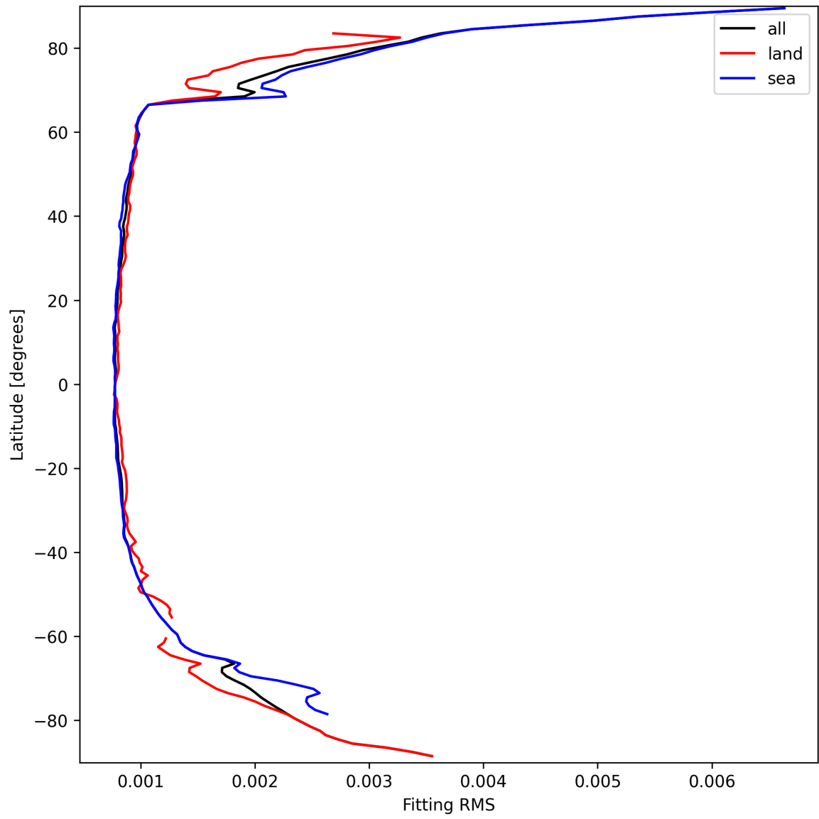
Figure 22: Zonal average of “Fitting RMS” for 2025-09-21 to 2025-09-22.
