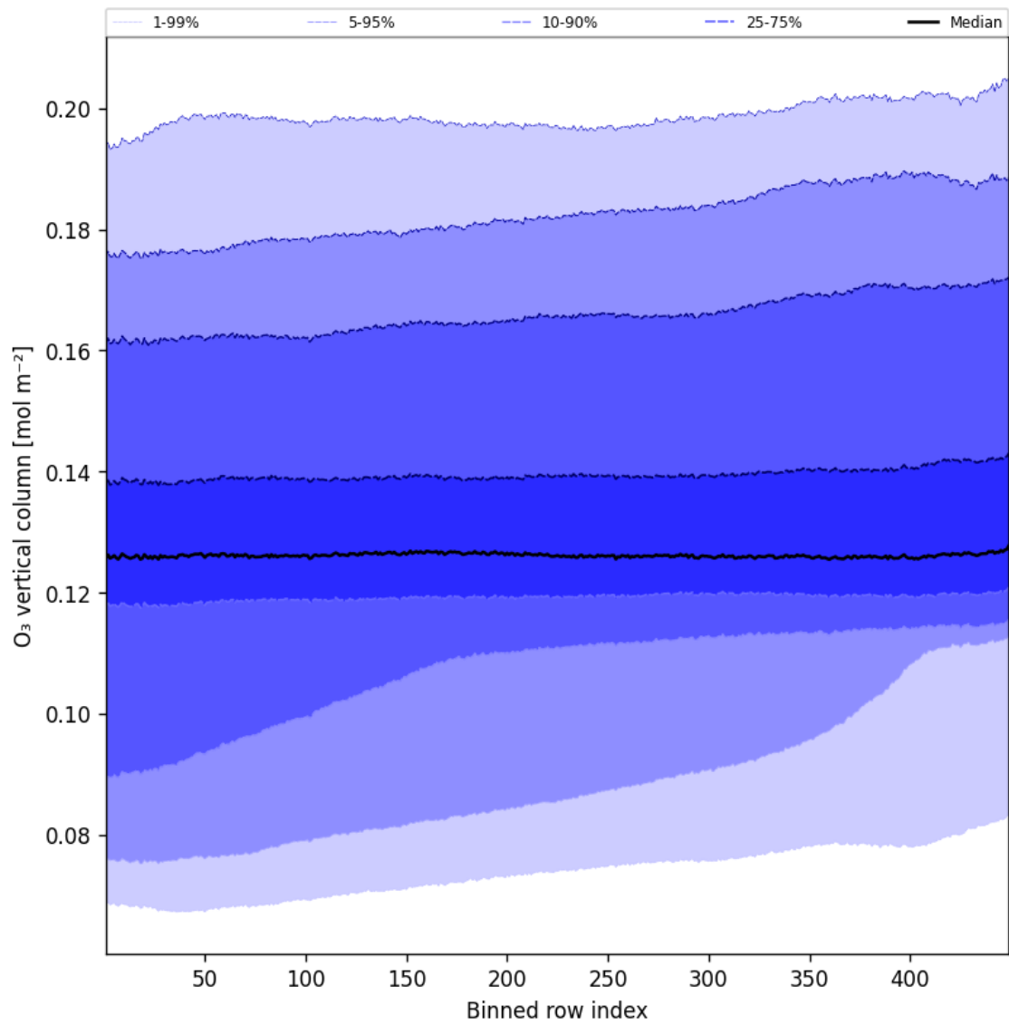
Figure 41: Along track statistics of “O 3 vertical column” for 2025-09-21 to 2025-09-22
