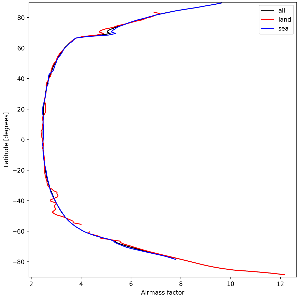
Figure 25: Zonal average of “Airmass factor” for 2025-09-21 to 2025-09-22.
