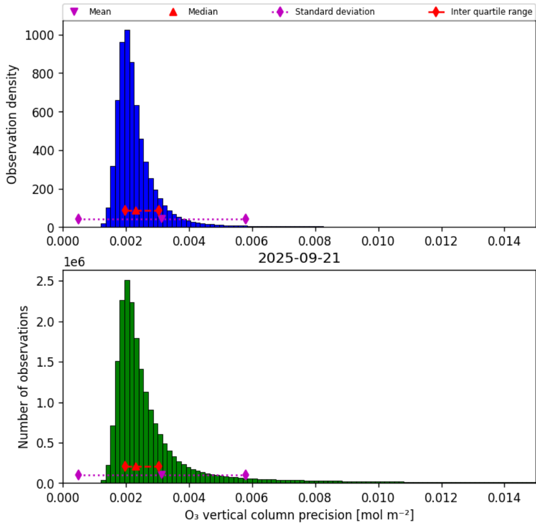
Figure 30: Histogram of “O 3 vertical column precision” for 2025-09-21 to 2025-09-22
