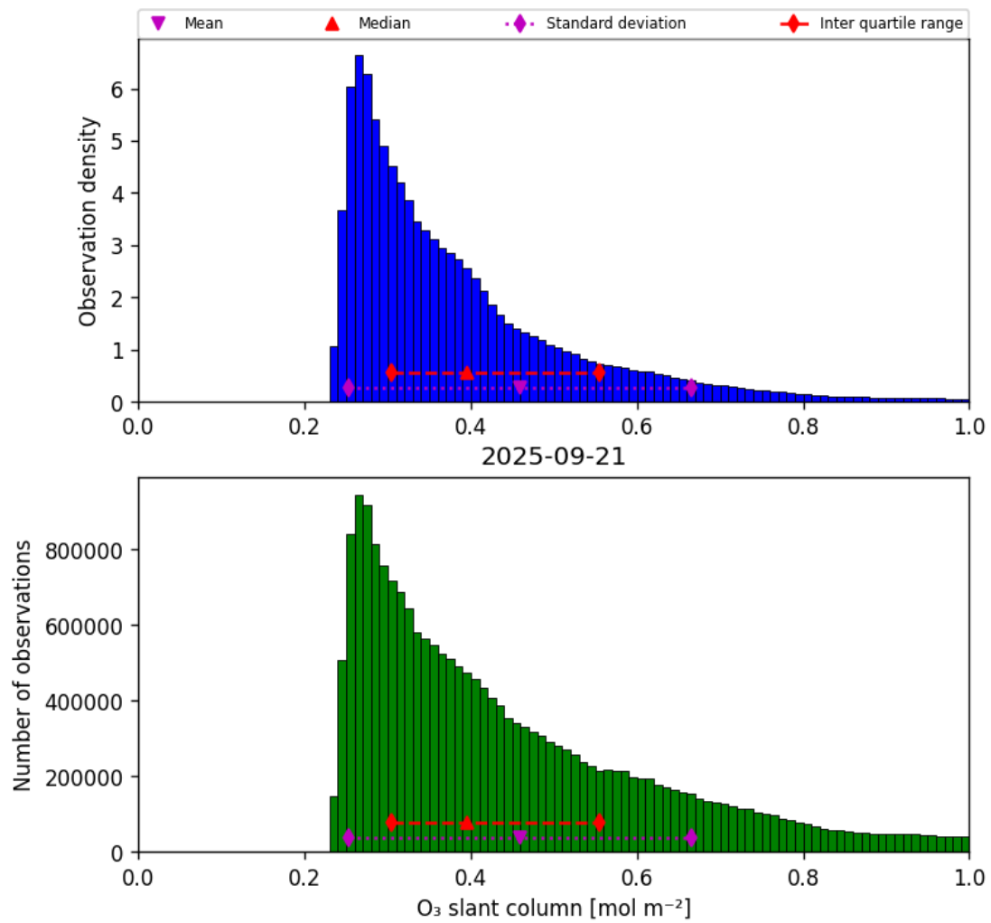
Figure 31: Histogram of “O 3 slant column” for 2025-09-21 to 2025-09-22
