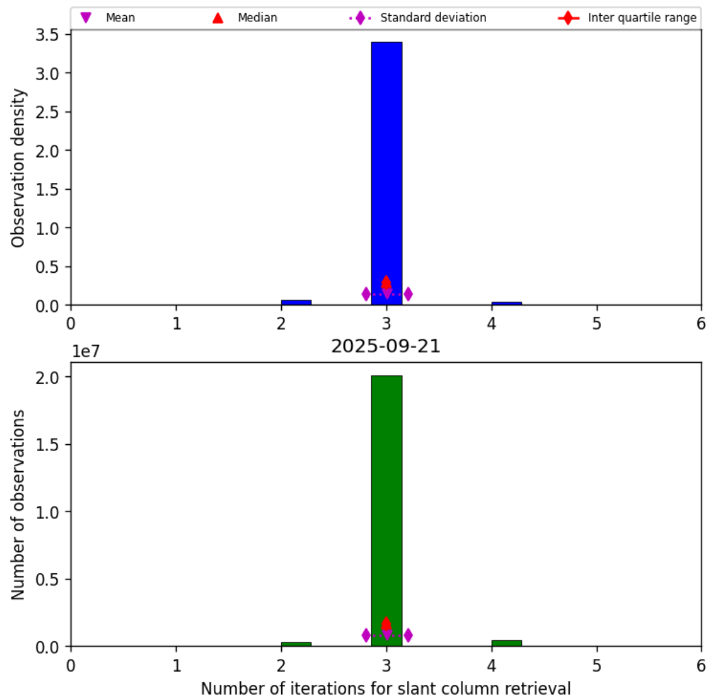
Figure 33: Histogram of “Number of iterations for slant column retrieval” for 2025-09-21 to 2025-09-22
