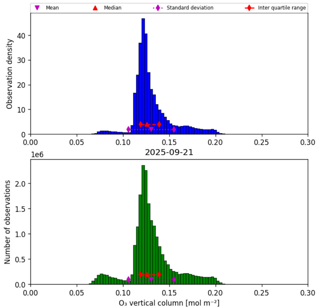
Figure 29: Histogram of “O 3 vertical column” for 2025-09-21 to 2025-09-22
