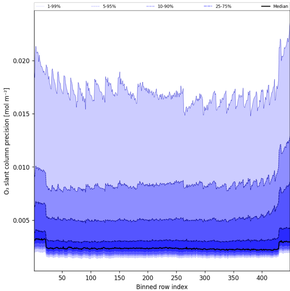
Figure 44: Along track statistics of “O 3 slant column precision” for 2025-09-21 to 2025-09-22
