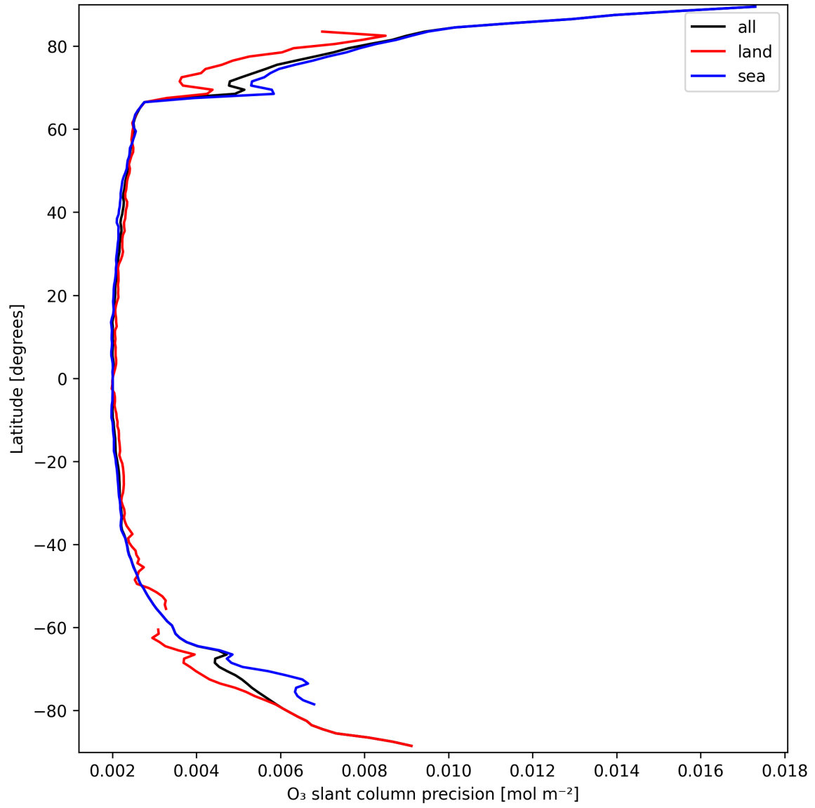
Figure 20: Zonal average of “O 3 slant column precision” for 2025-09-21 to 2025-09-22.
