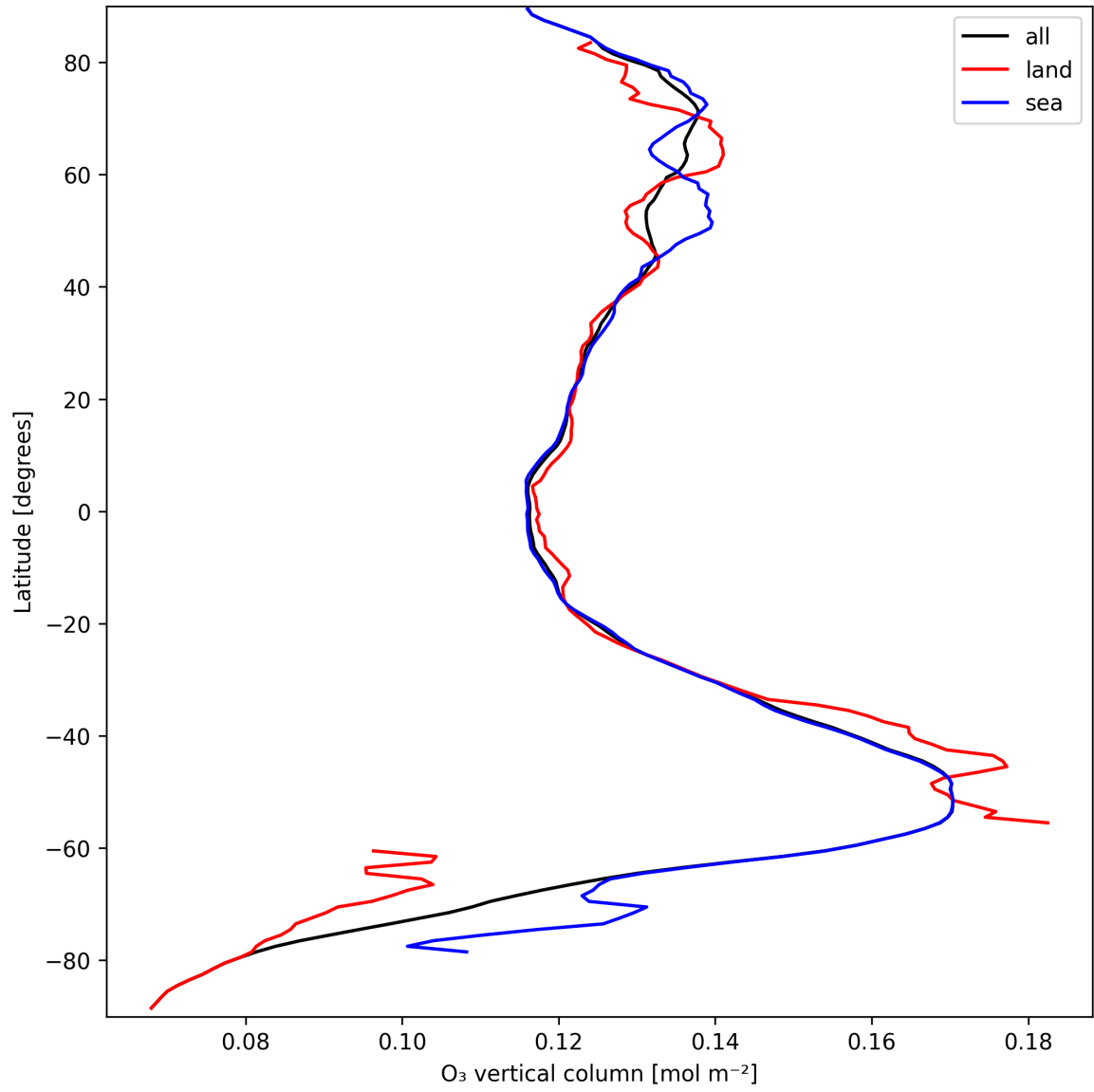
Figure 17: Zonal average of “O 3 vertical column” for 2025-09-21 to 2025-09-22.
