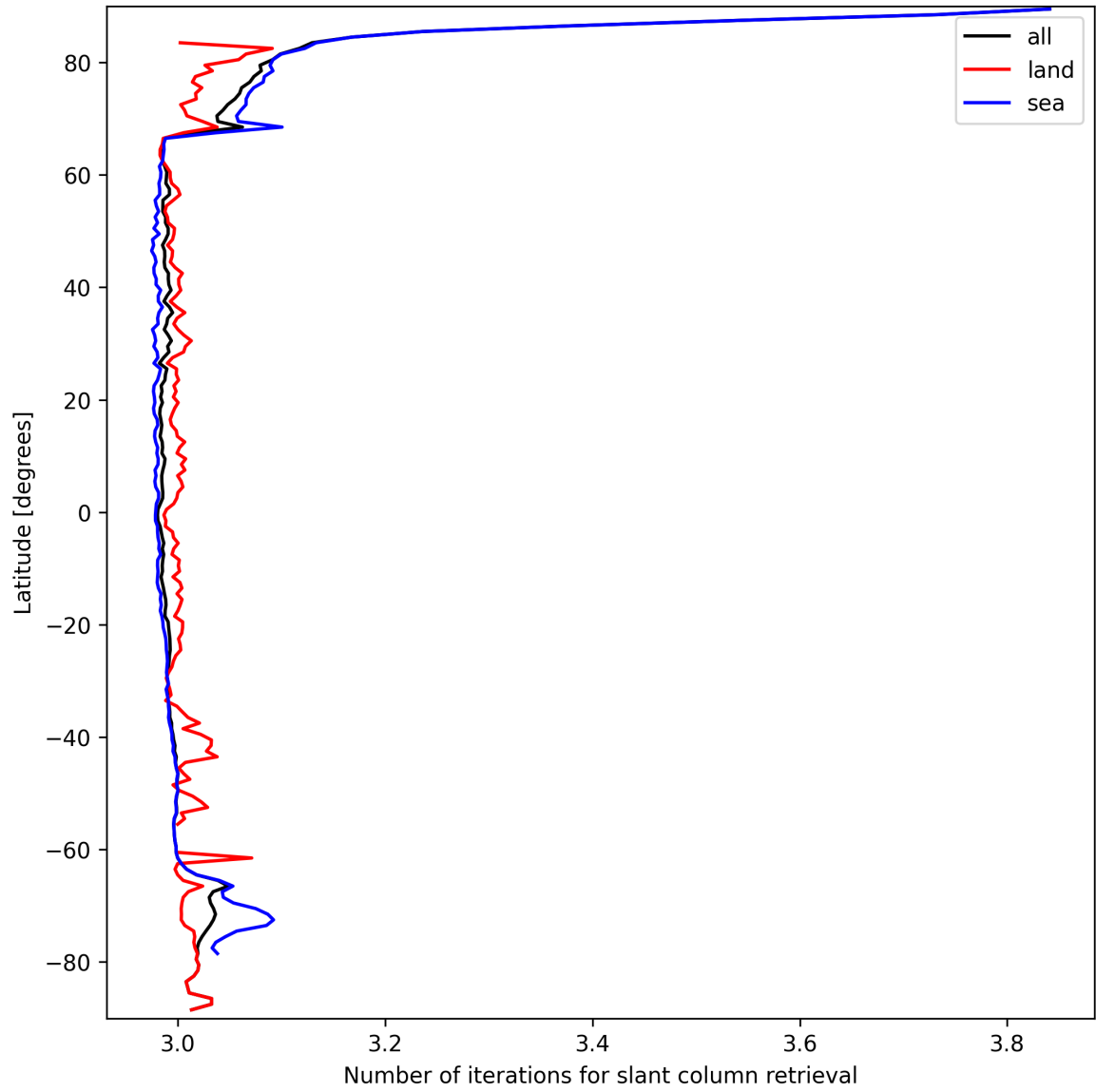
Figure 21: Zonal average of “Number of iterations for slant column retrieval” for 2025-09-21 to 2025-09-22.
