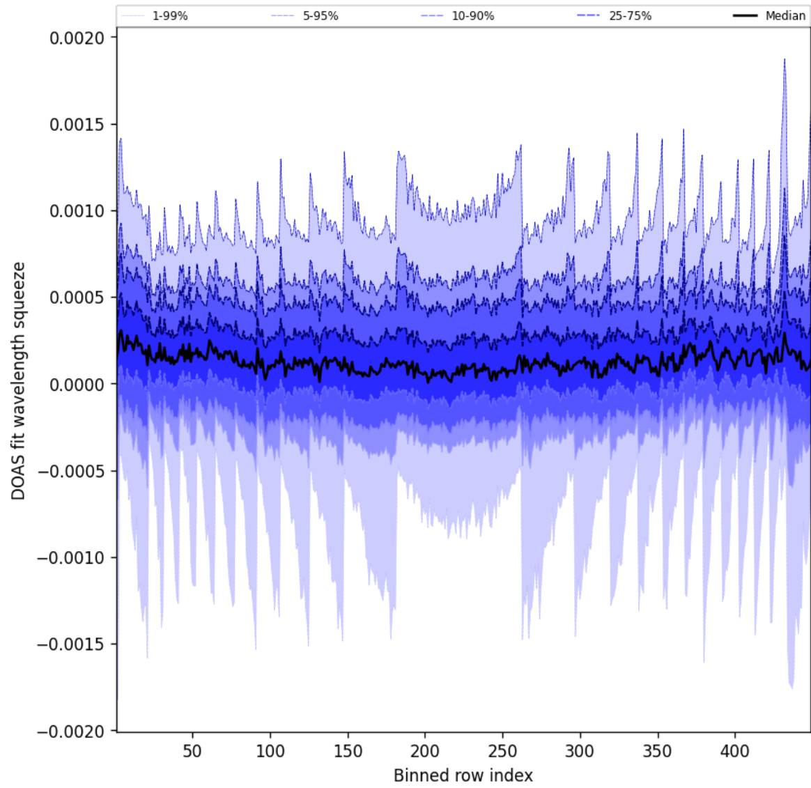
Figure 48: Along track statistics of “DOAS fit wavelength squeeze” for 2025-09-21 to 2025-09-22
