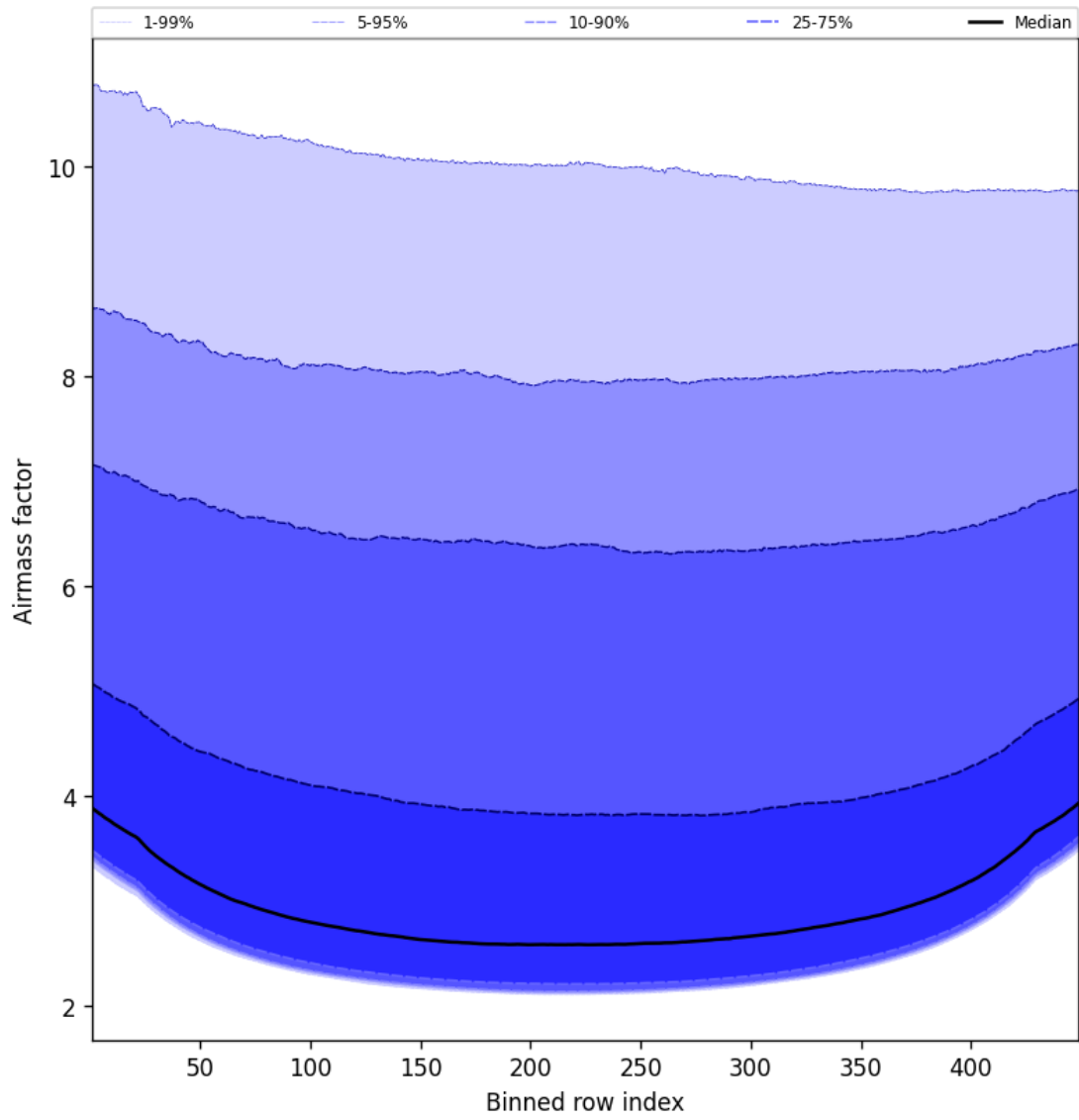
Figure 49: Along track statistics of “Airmass factor” for 2025-09-21 to 2025-09-22
