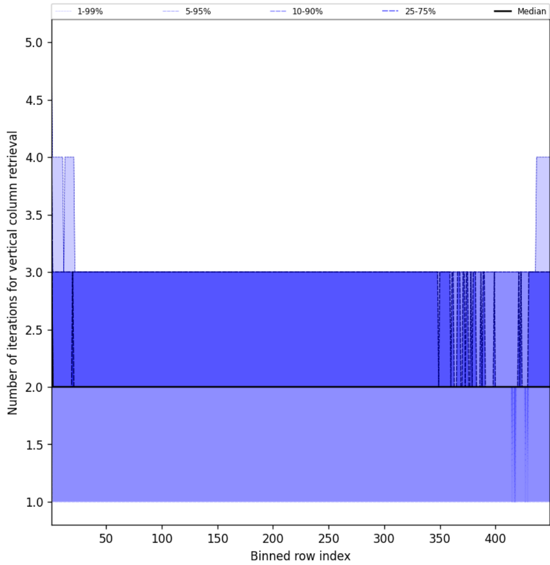
Figure 51: Along track statistics of “Number of iterations for vertical column retrieval” for 2025-09-21 to 2025-09-22
