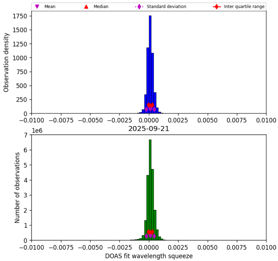
Figure 36: Histogram of “DOAS fit wavelength squeeze” for 2025-09-21 to 2025-09-22
