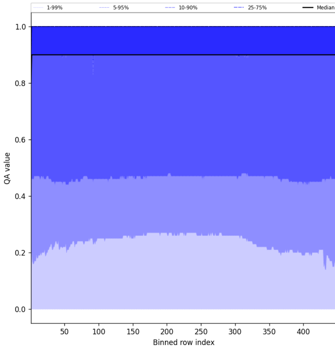
Figure 40: Along track statistics of “QA value” for 2025-09-21 to 2025-09-22
