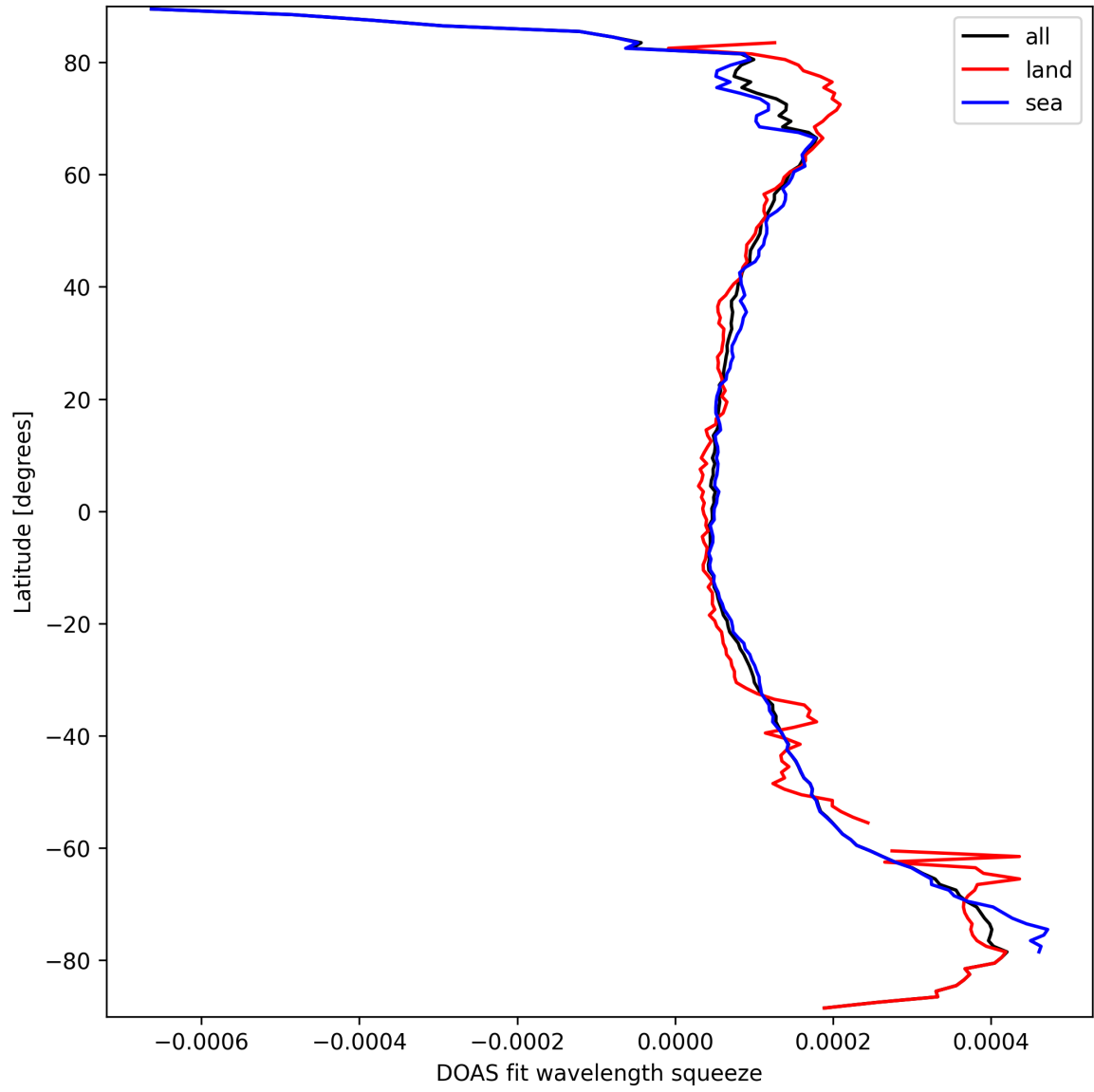
Figure 24: Zonal average of “DOAS fit wavelength squeeze” for 2025-09-21 to 2025-09-22.
