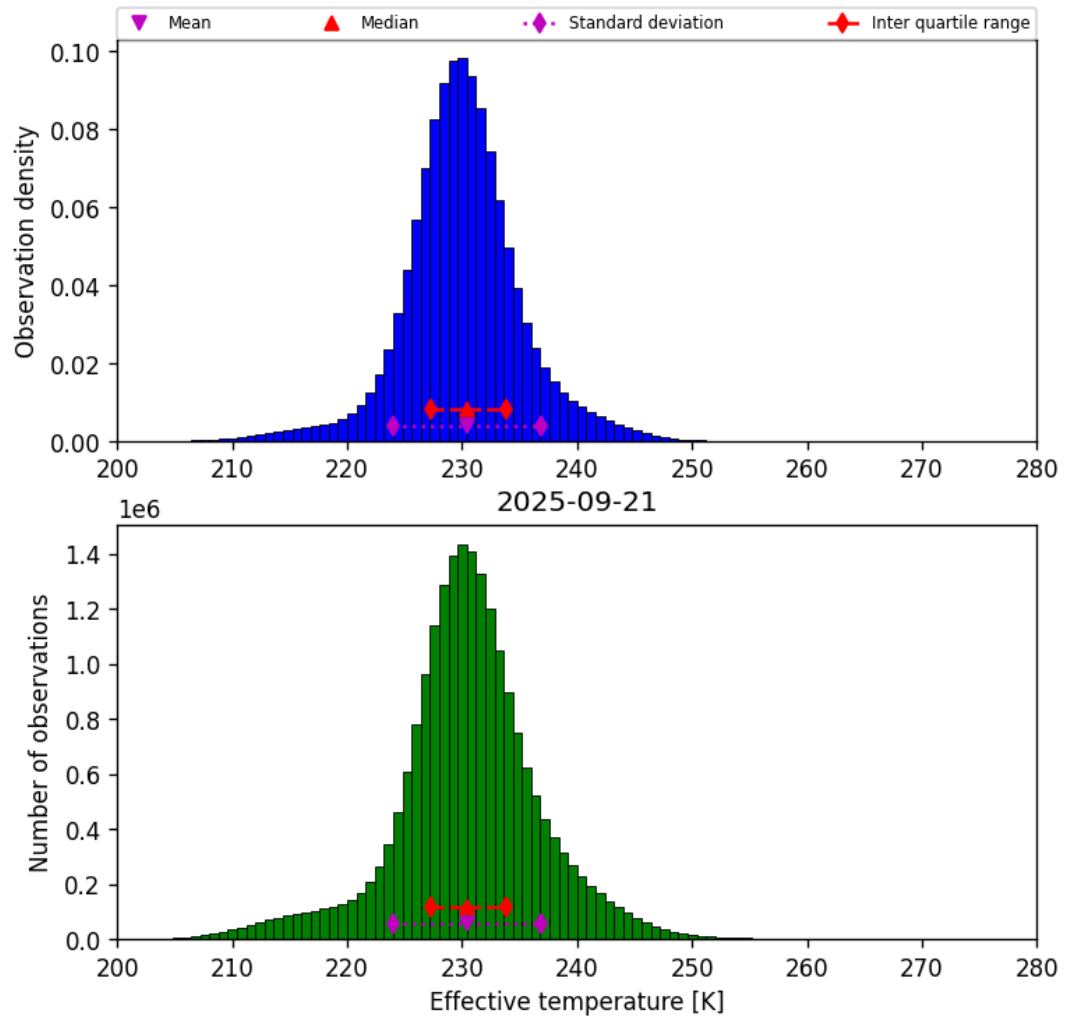
Figure 38: Histogram of “Effective temperature” for 2025-09-21 to 2025-09-22
