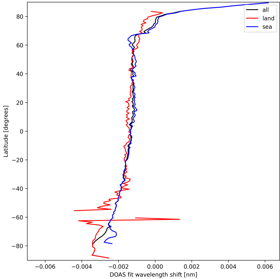
Figure 23: Zonal average of “DOAS fit wavelength shift” for 2025-09-21 to 2025-09-22.
