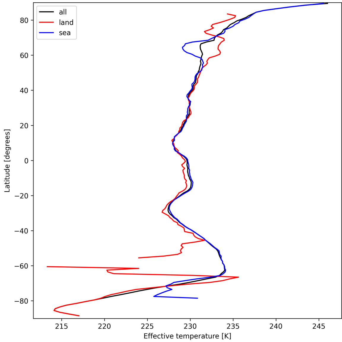
Figure 26: Zonal average of “Effective temperature” for 2025-09-21 to 2025-09-22.
