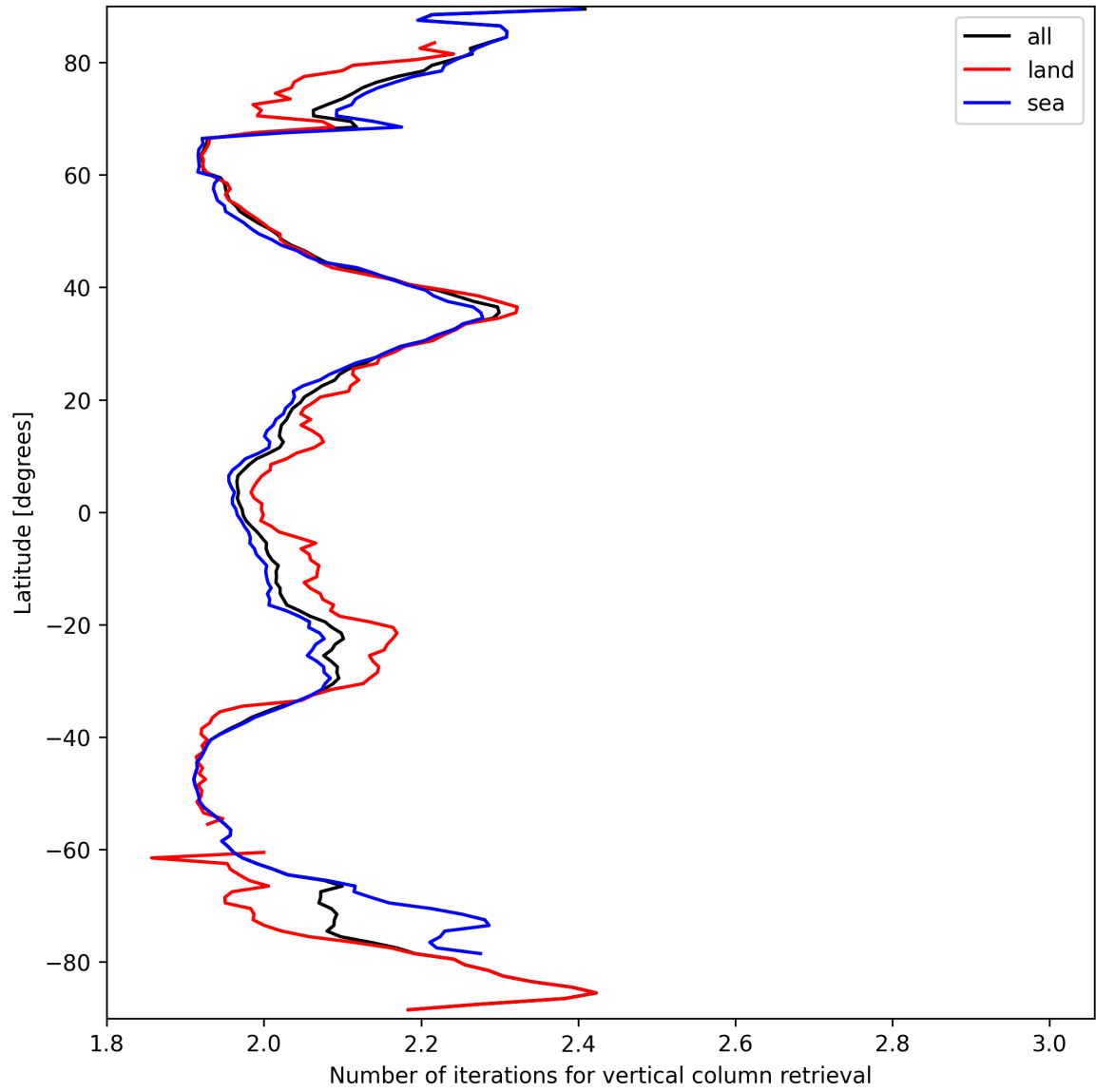
Figure 27: Zonal average of “Number of iterations for vertical column retrieval” for 2025-09-21 to 2025-09-22.
