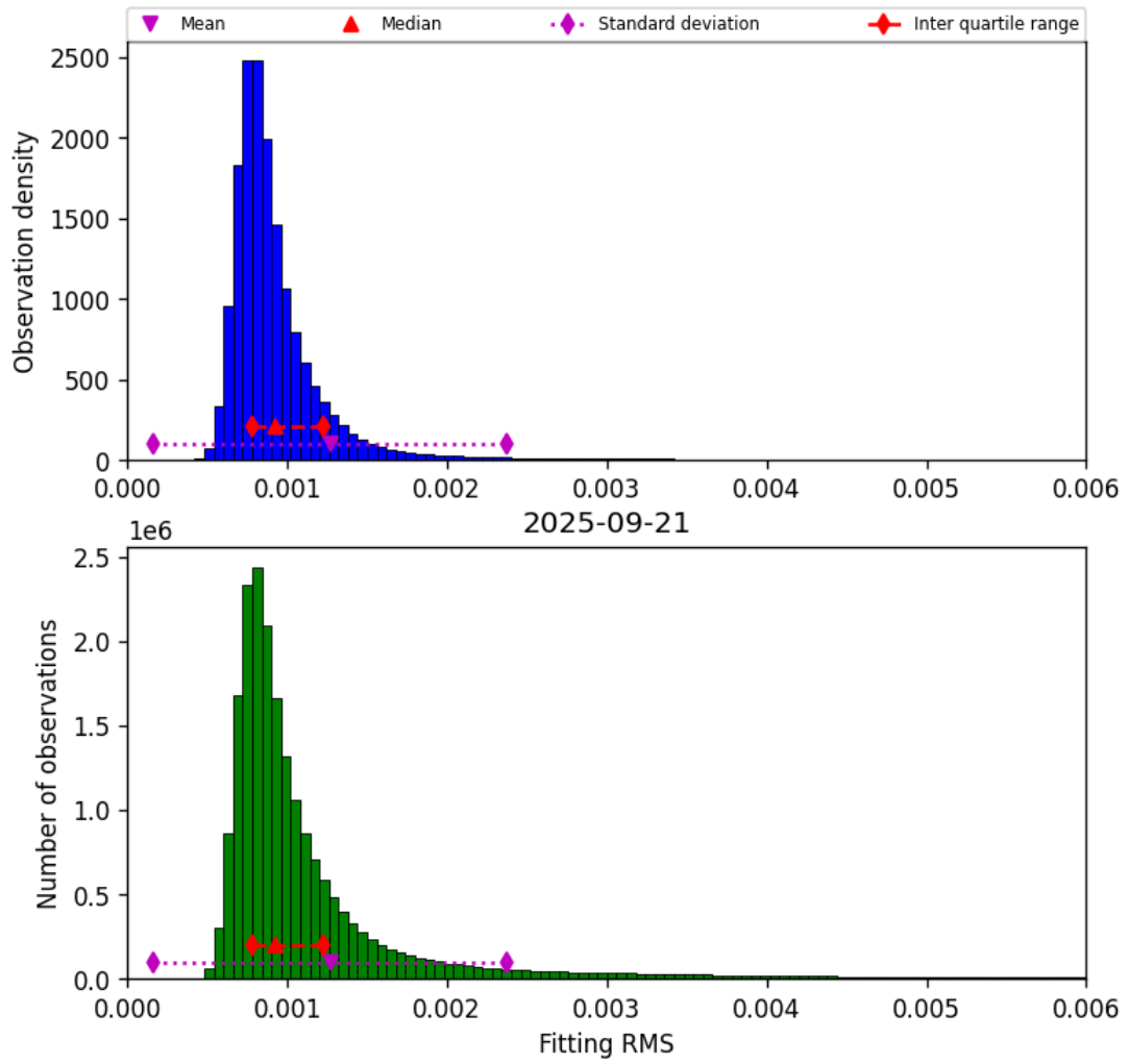
Figure 34: Histogram of “Fitting RMS” for 2025-09-21 to 2025-09-22
