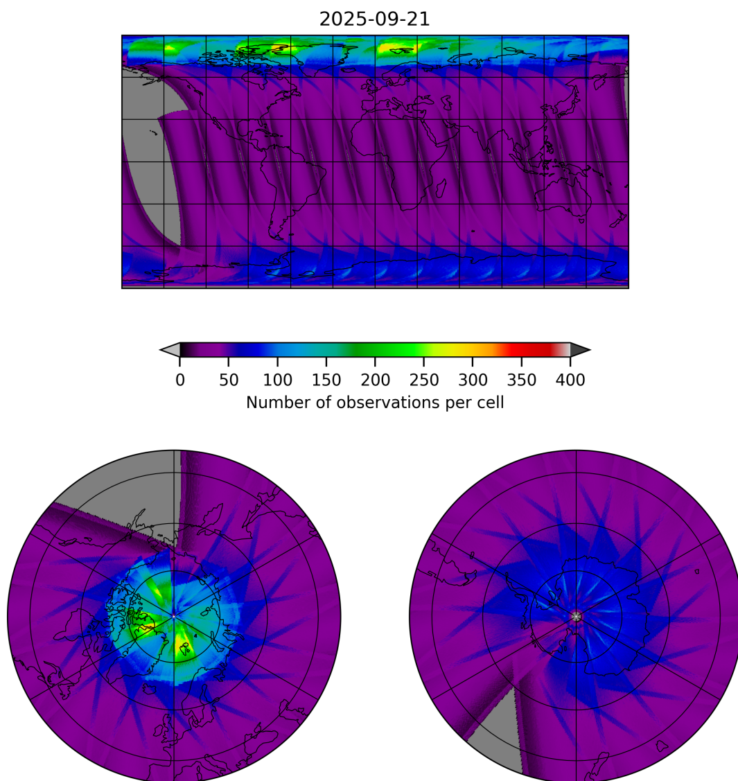
Figure 15: Map of the number of observations for 2025-09-21 to 2025-09-22
