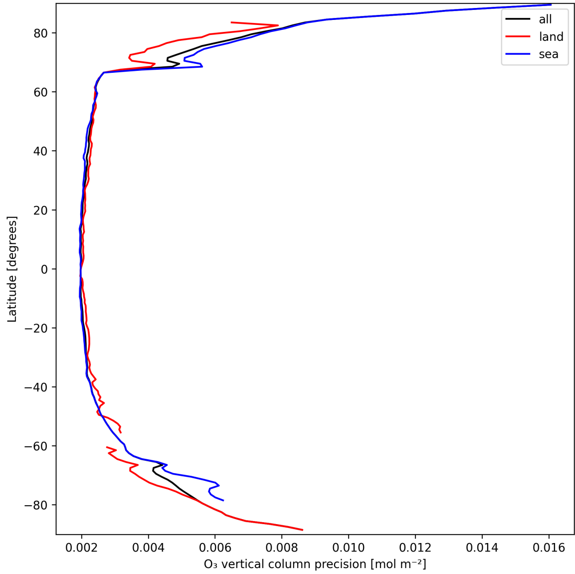
Figure 18: Zonal average of “O 3 vertical column precision” for 2025-09-21 to 2025-09-22.
