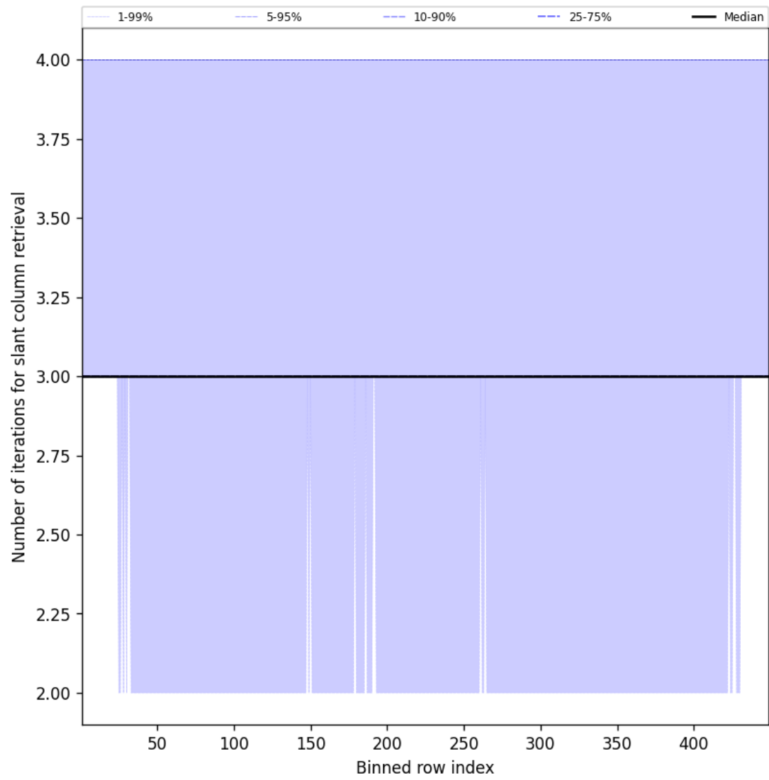
Figure 45: Along track statistics of “Number of iterations for slant column retrieval” for 2025-09-21 to 2025-09-22
