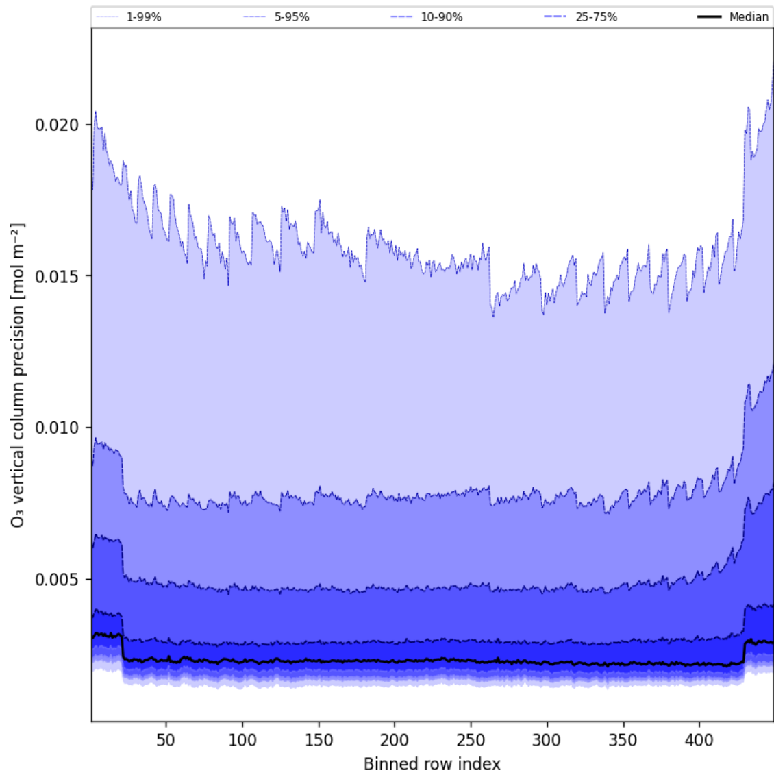
Figure 42: Along track statistics of “O 3 vertical column precision” for 2025-09-21 to 2025-09-22
