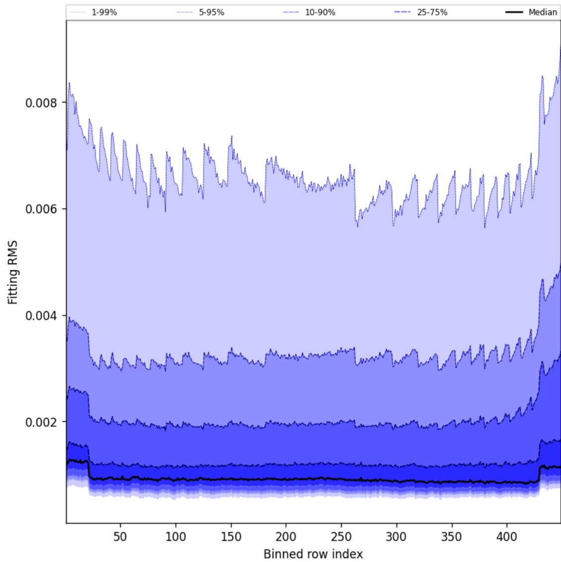
Figure 46: Along track statistics of “Fitting RMS” for 2025-09-21 to 2025-09-22
