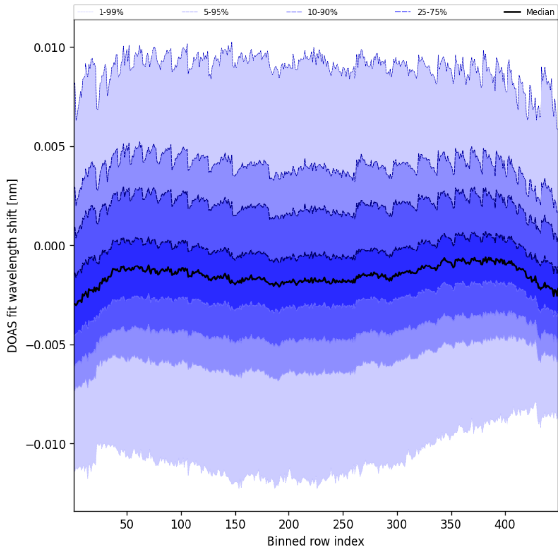
Figure 47: Along track statistics of “DOAS fit wavelength shift” for 2025-09-21 to 2025-09-22
