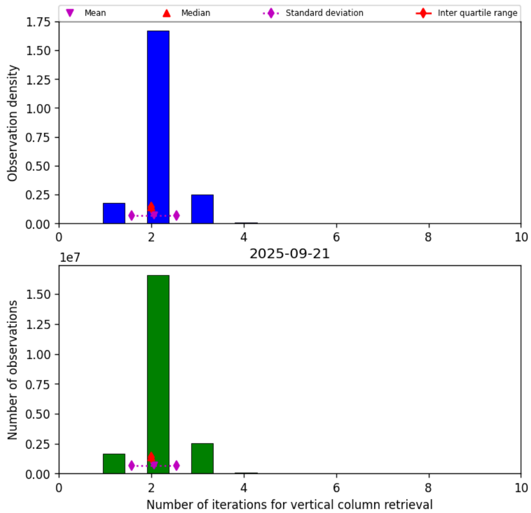
Figure 39: Histogram of “Number of iterations for vertical column retrieval” for 2025-09-21 to 2025-09-22
