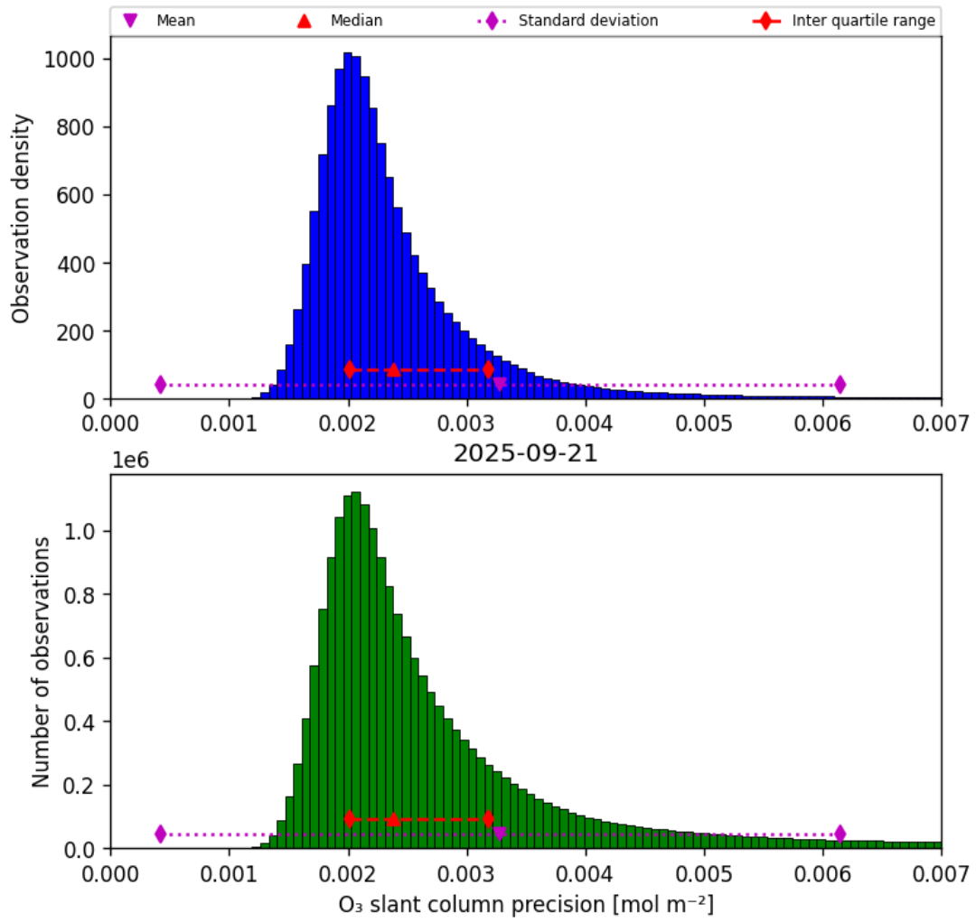
Figure 32: Histogram of “O 3 slant column precision” for 2025-09-21 to 2025-09-22
