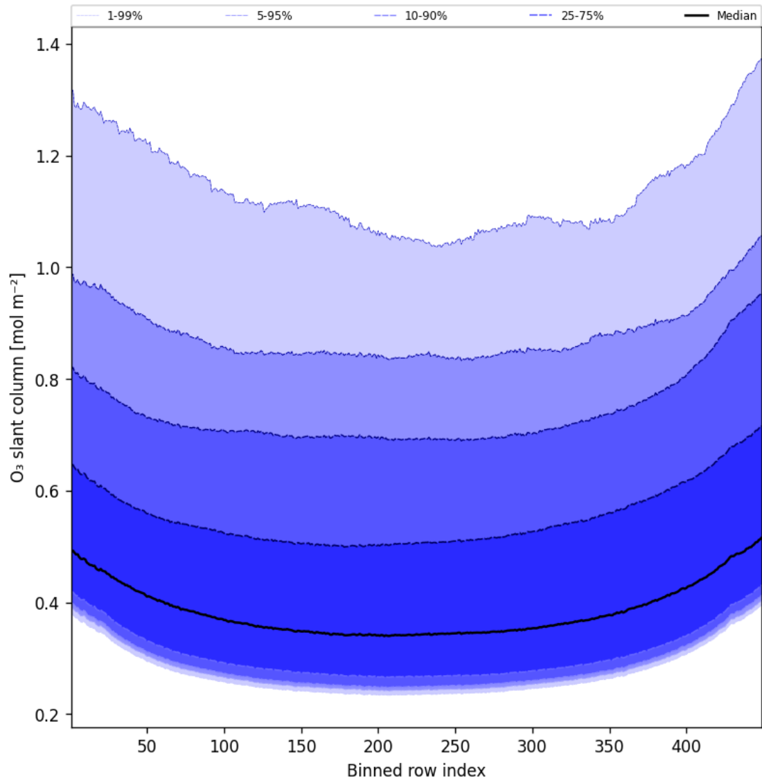
Figure 43: Along track statistics of “O 3 slant column” for 2025-09-21 to 2025-09-22
