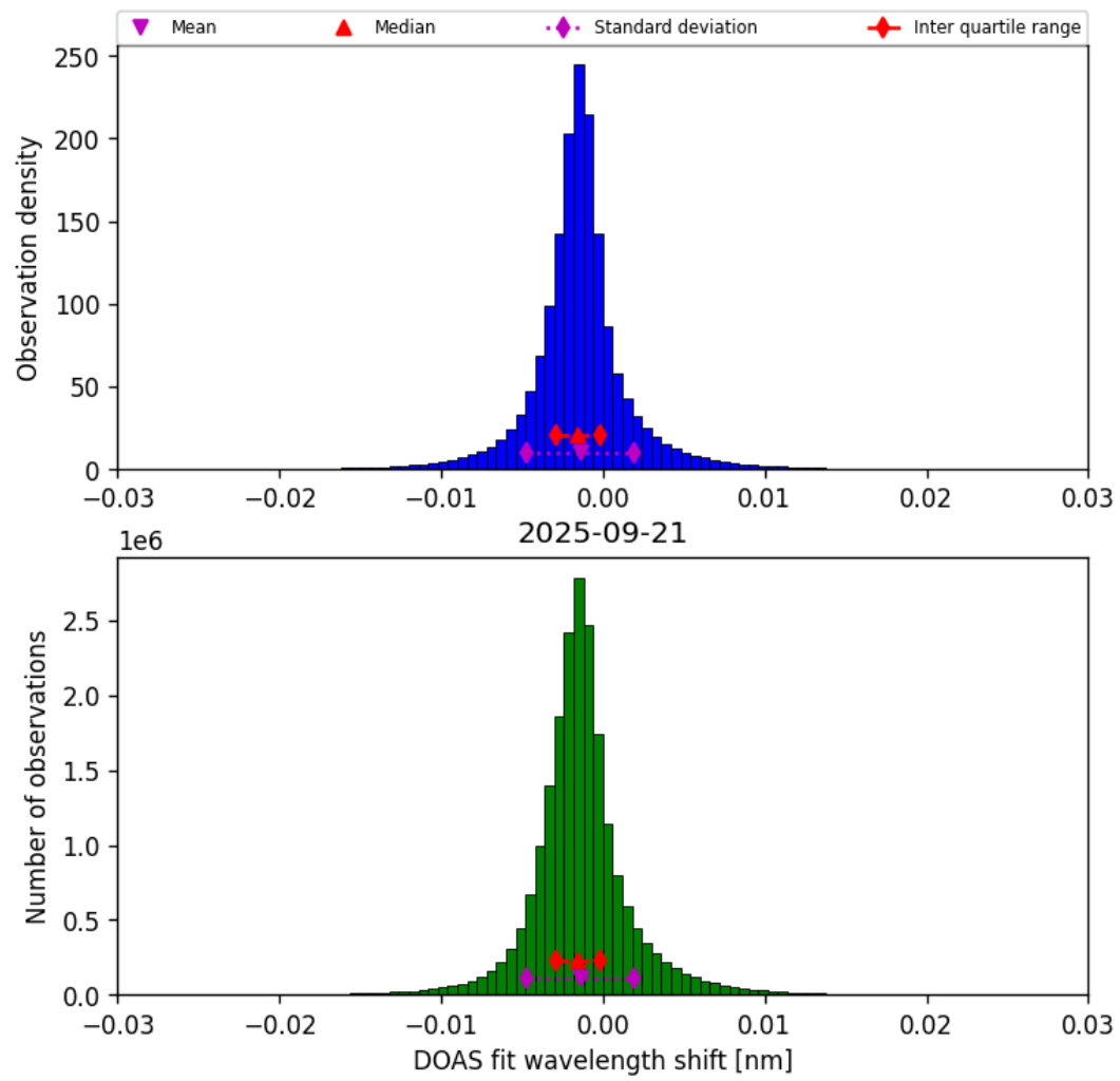
Figure 35: Histogram of “DOAS fit wavelength shift” for 2025-09-21 to 2025-09-22
