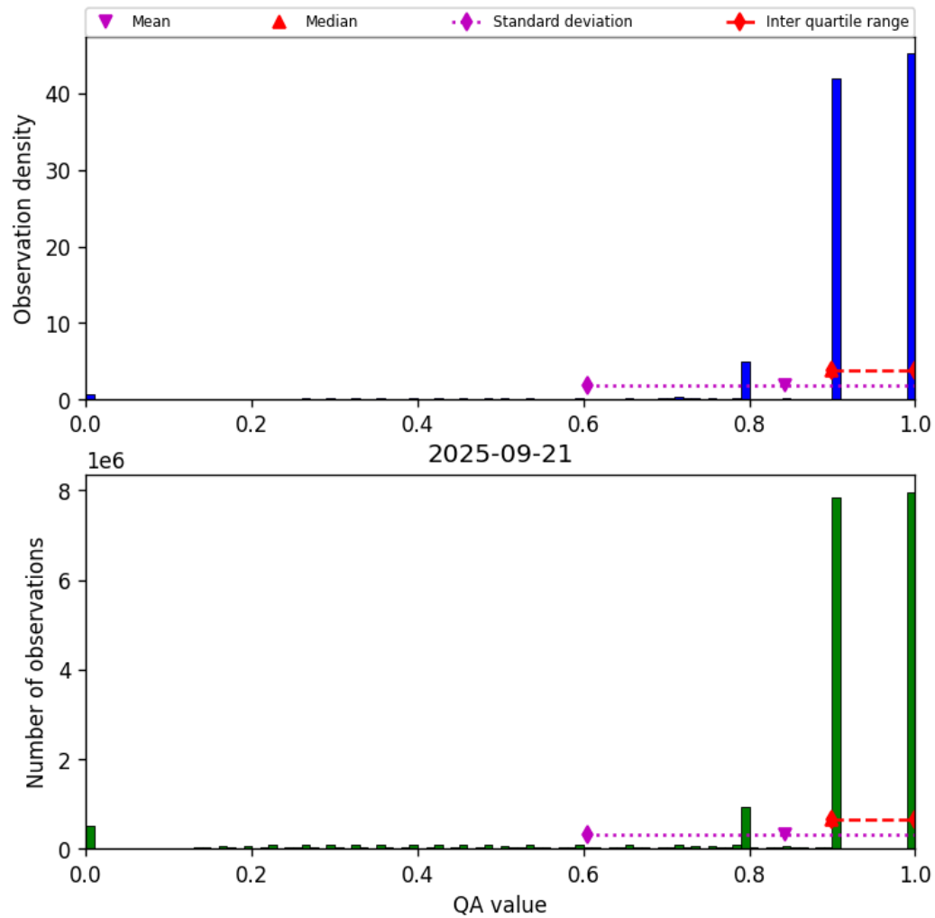
Figure 28: Histogram of “QA value” for 2025-09-21 to 2025-09-22
