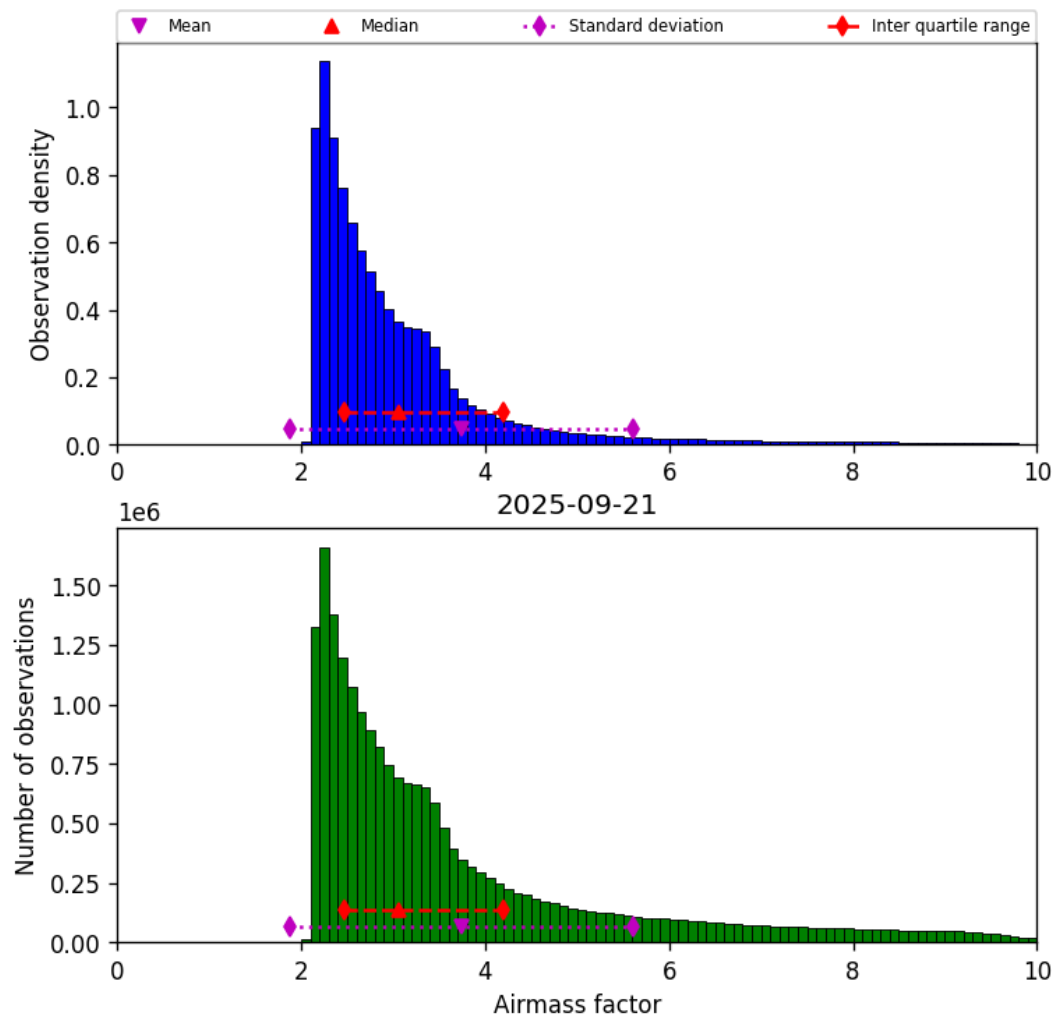
Figure 37: Histogram of “Airmass factor” for 2025-09-21 to 2025-09-22
