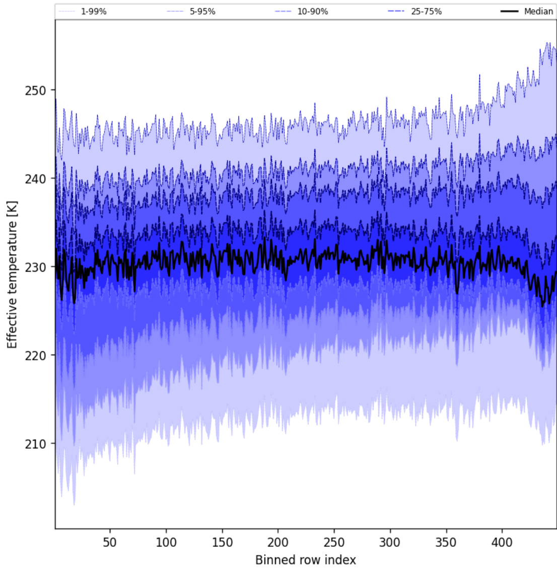
Figure 50: Along track statistics of “Effective temperature” for 2025-09-21 to 2025-09-22
