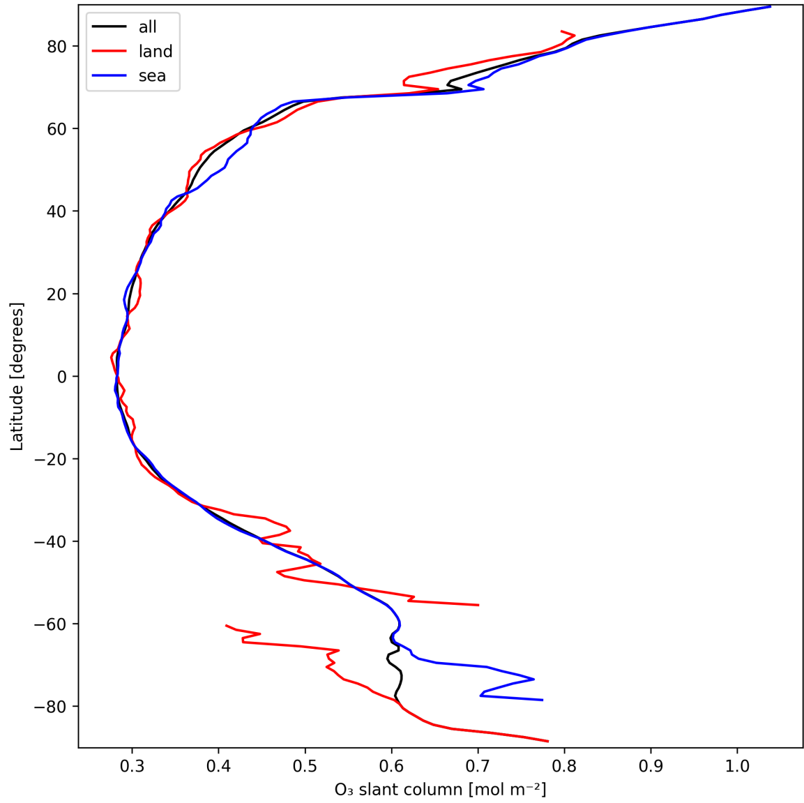
Figure 19: Zonal average of “O 3 slant column” for 2025-09-21 to 2025-09-22.
