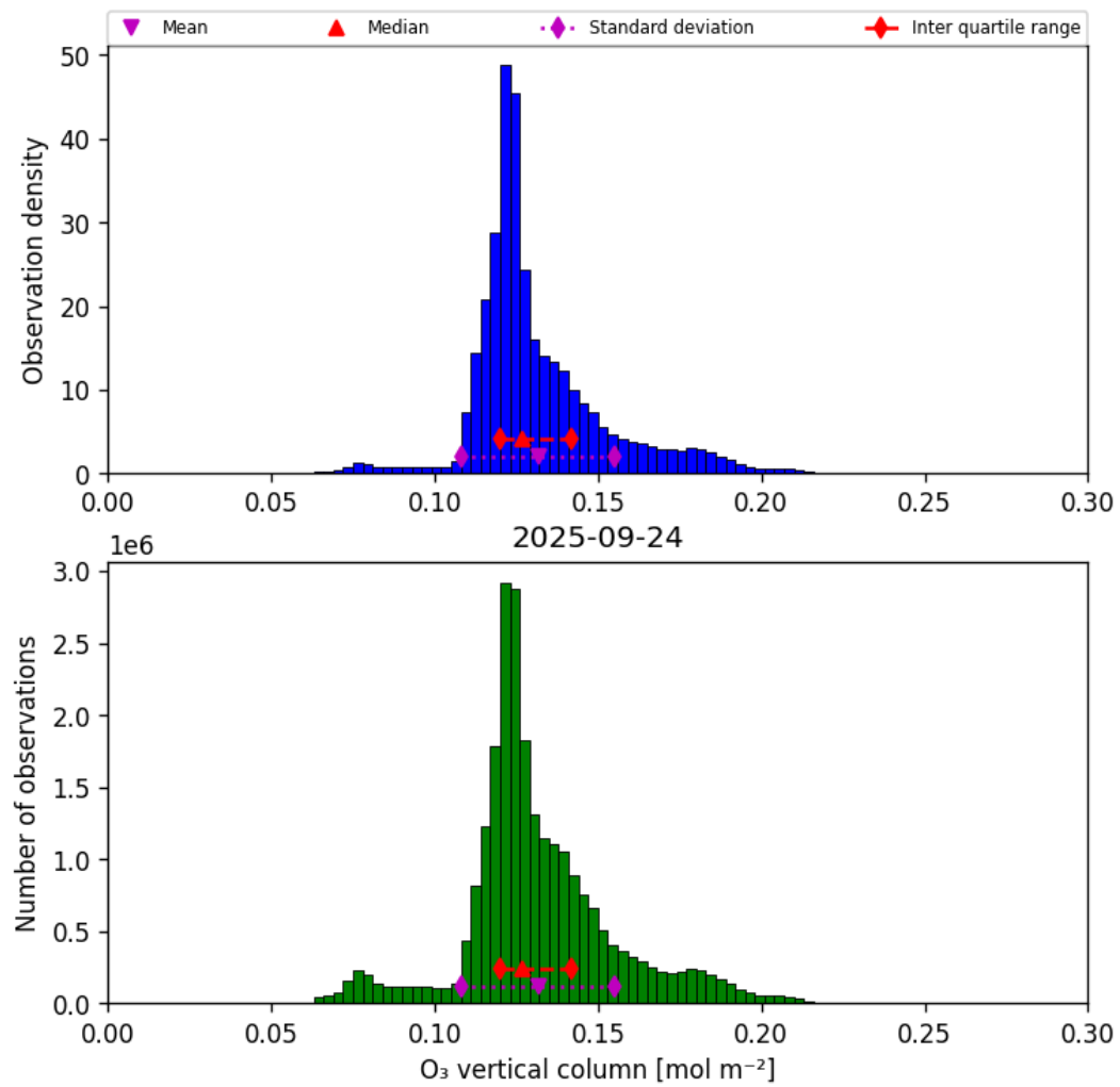
Figure 29: Histogram of “O 3 vertical column” for 2025-09-24 to 2025-09-25
