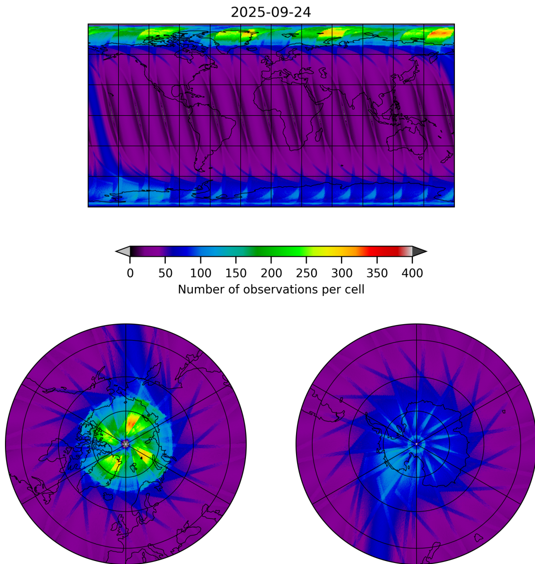
Figure 15: Map of the number of observations for 2025-09-24 to 2025-09-25
