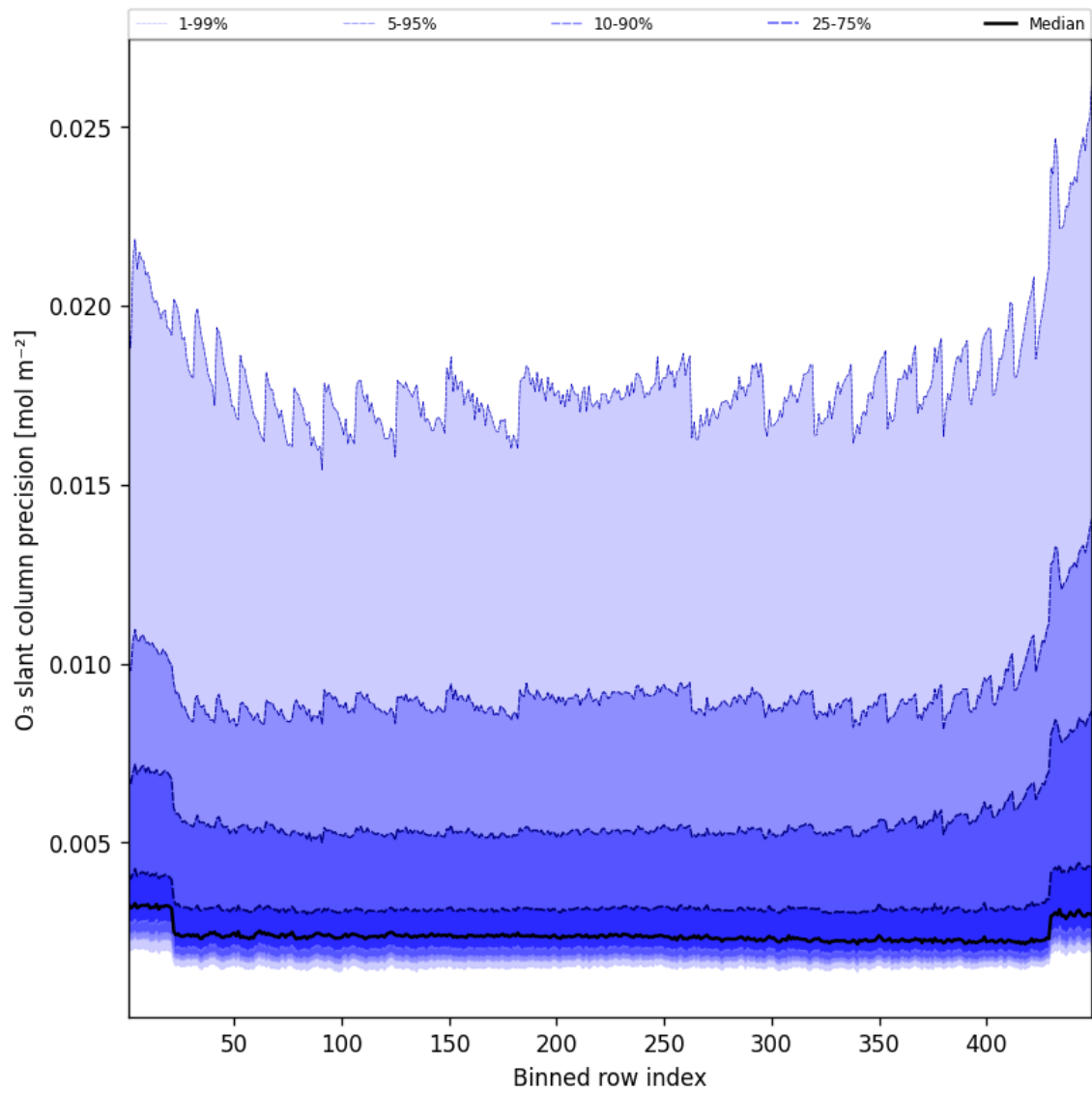
Figure 44: Along track statistics of “O 3 slant column precision” for 2025-09-24 to 2025-09-25
