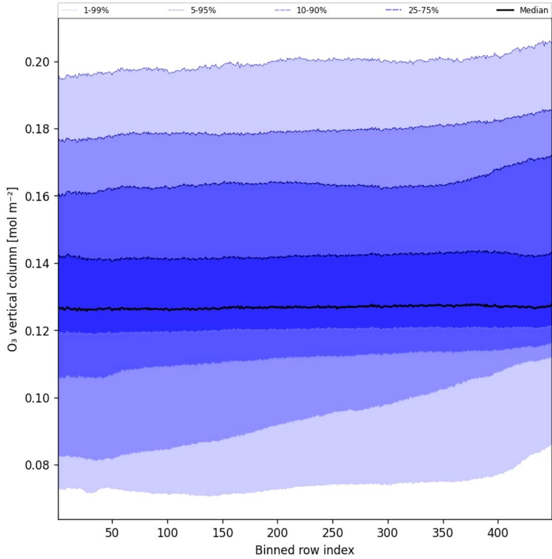
Figure 41: Along track statistics of “O 3 vertical column” for 2025-09-24 to 2025-09-25
