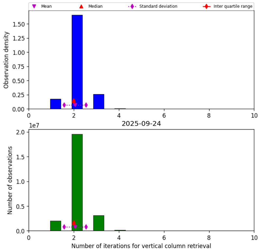
Figure 39: Histogram of “Number of iterations for vertical column retrieval” for 2025-09-24 to 2025-09-25
