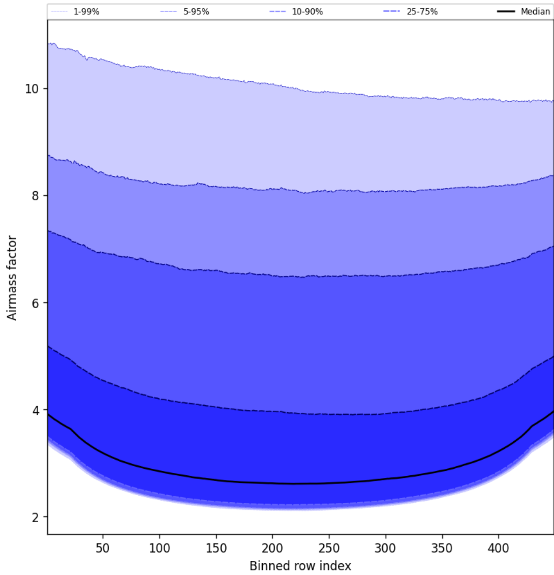
Figure 49: Along track statistics of “Airmass factor” for 2025-09-24 to 2025-09-25
