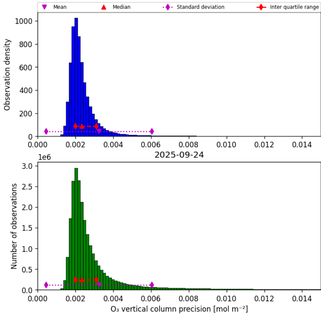
Figure 30: Histogram of “O 3 vertical column precision” for 2025-09-24 to 2025-09-25
