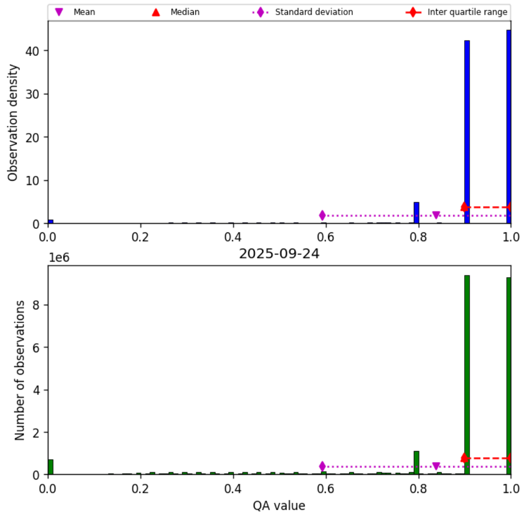
Figure 28: Histogram of “QA value” for 2025-09-24 to 2025-09-25
