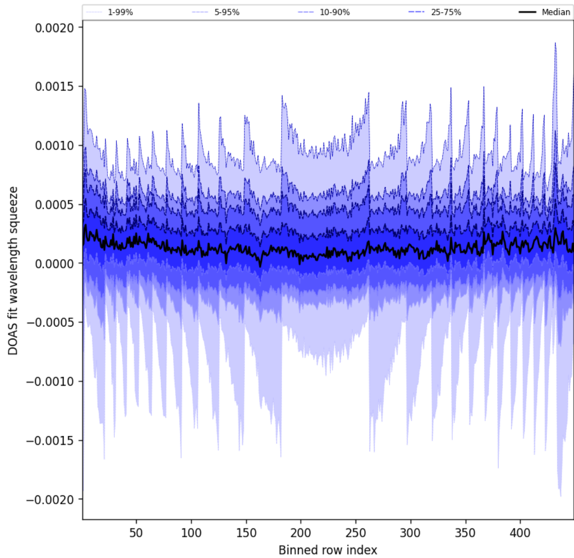
Figure 48: Along track statistics of “DOAS fit wavelength squeeze” for 2025-09-24 to 2025-09-25
