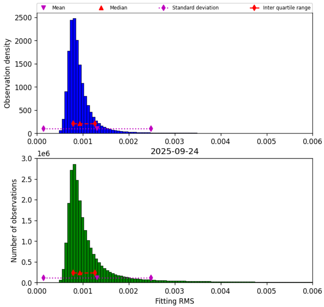
Figure 34: Histogram of “Fitting RMS” for 2025-09-24 to 2025-09-25
