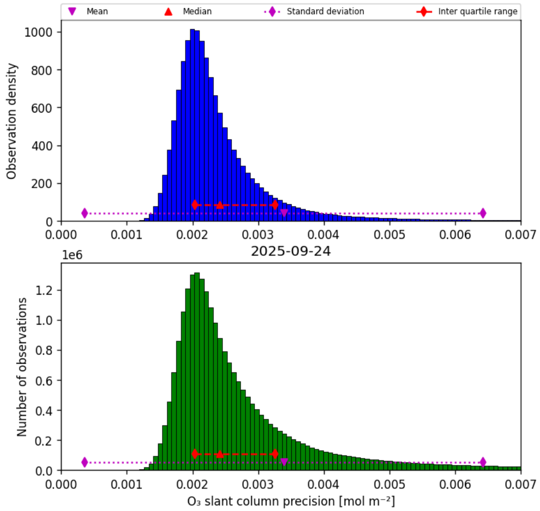
Figure 32: Histogram of “O 3 slant column precision” for 2025-09-24 to 2025-09-25
