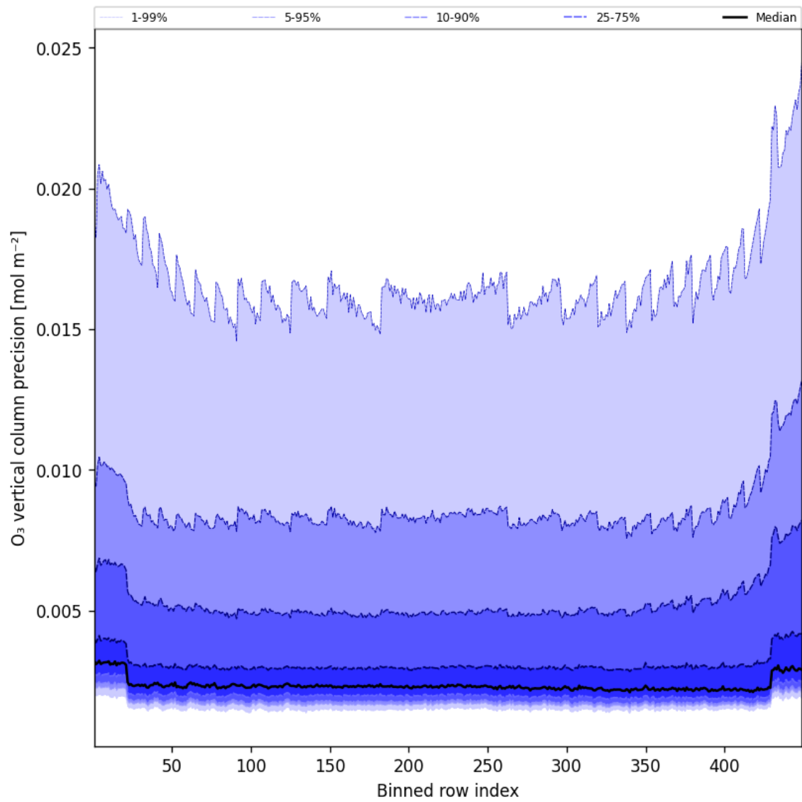
Figure 42: Along track statistics of “O 3 vertical column precision” for 2025-09-24 to 2025-09-25
