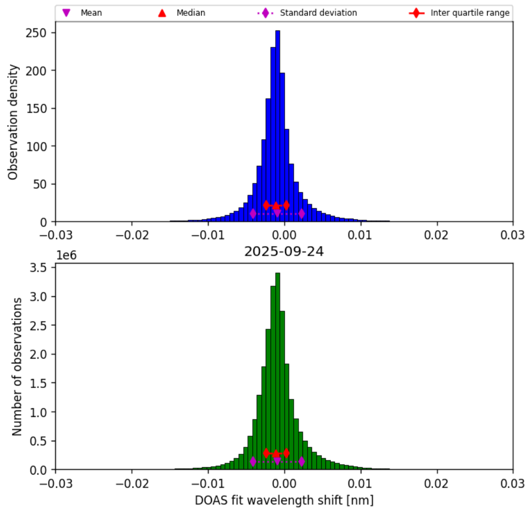
Figure 35: Histogram of “DOAS fit wavelength shift” for 2025-09-24 to 2025-09-25
