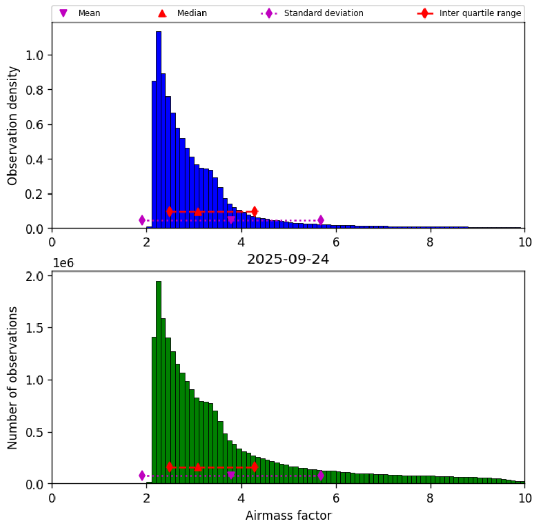
Figure 37: Histogram of “Airmass factor” for 2025-09-24 to 2025-09-25
