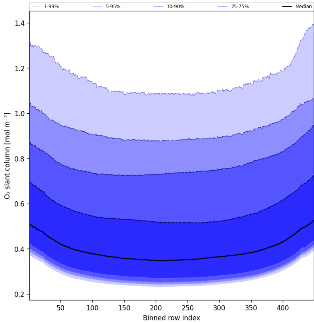
Figure 43: Along track statistics of “O 3 slant column” for 2025-09-24 to 2025-09-25
