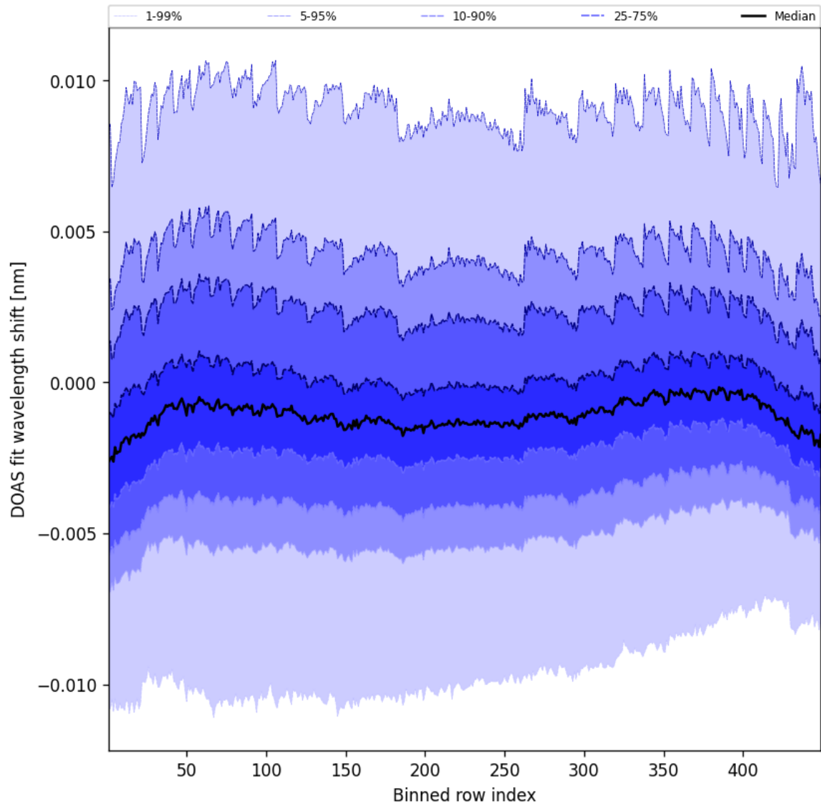
Figure 47: Along track statistics of “DOAS fit wavelength shift” for 2025-09-24 to 2025-09-25
