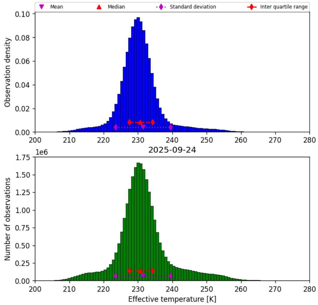
Figure 38: Histogram of “Effective temperature” for 2025-09-24 to 2025-09-25
