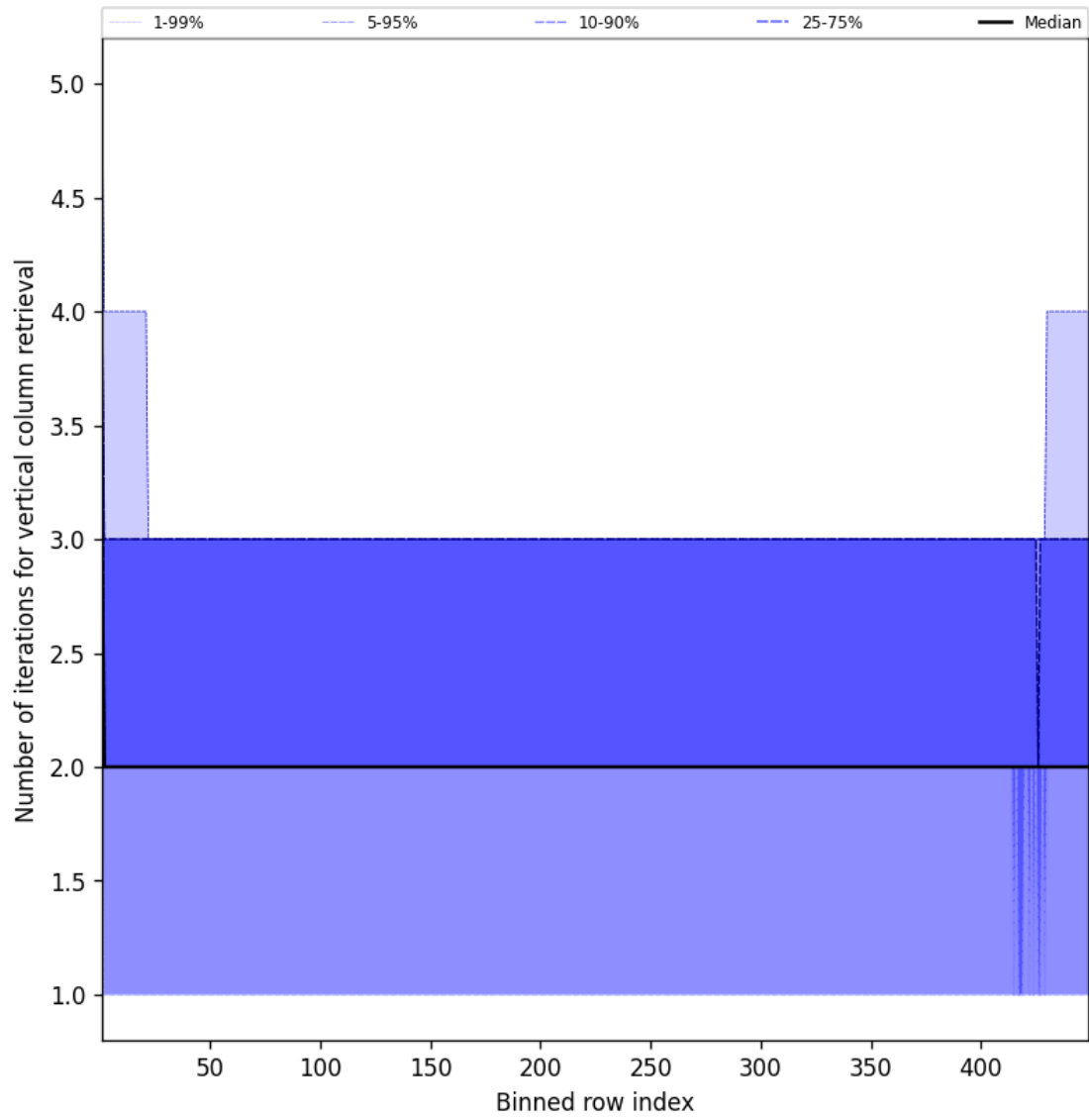
Figure 51: Along track statistics of “Number of iterations for vertical column retrieval” for 2025-09-24 to 2025-09-25
