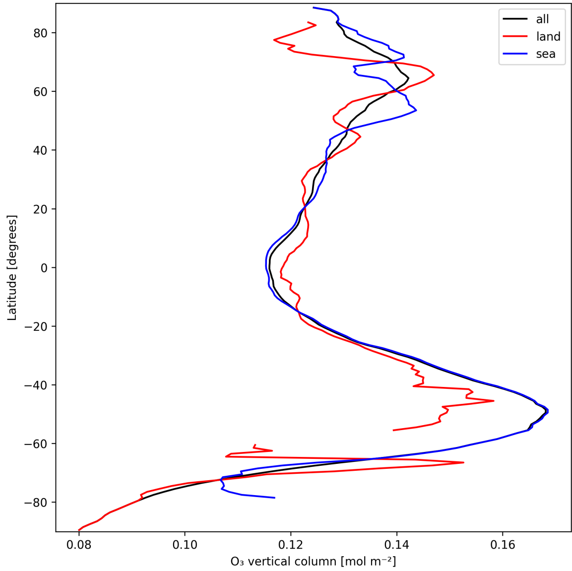
Figure 17: Zonal average of “O 3 vertical column” for 2025-09-24 to 2025-09-25.
