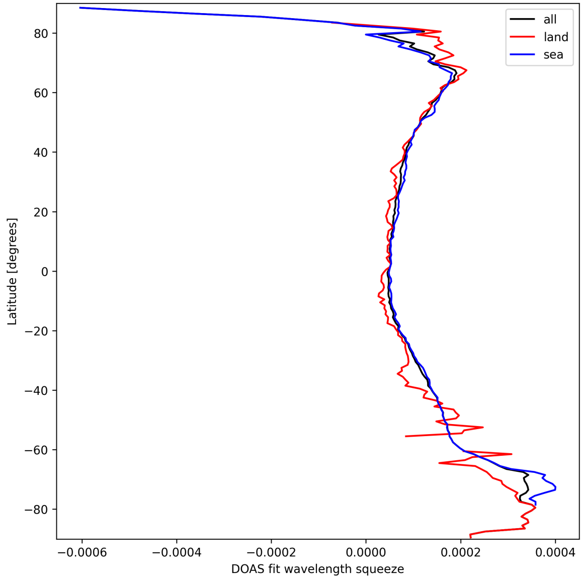
Figure 24: Zonal average of “DOAS fit wavelength squeeze” for 2025-09-24 to 2025-09-25.
