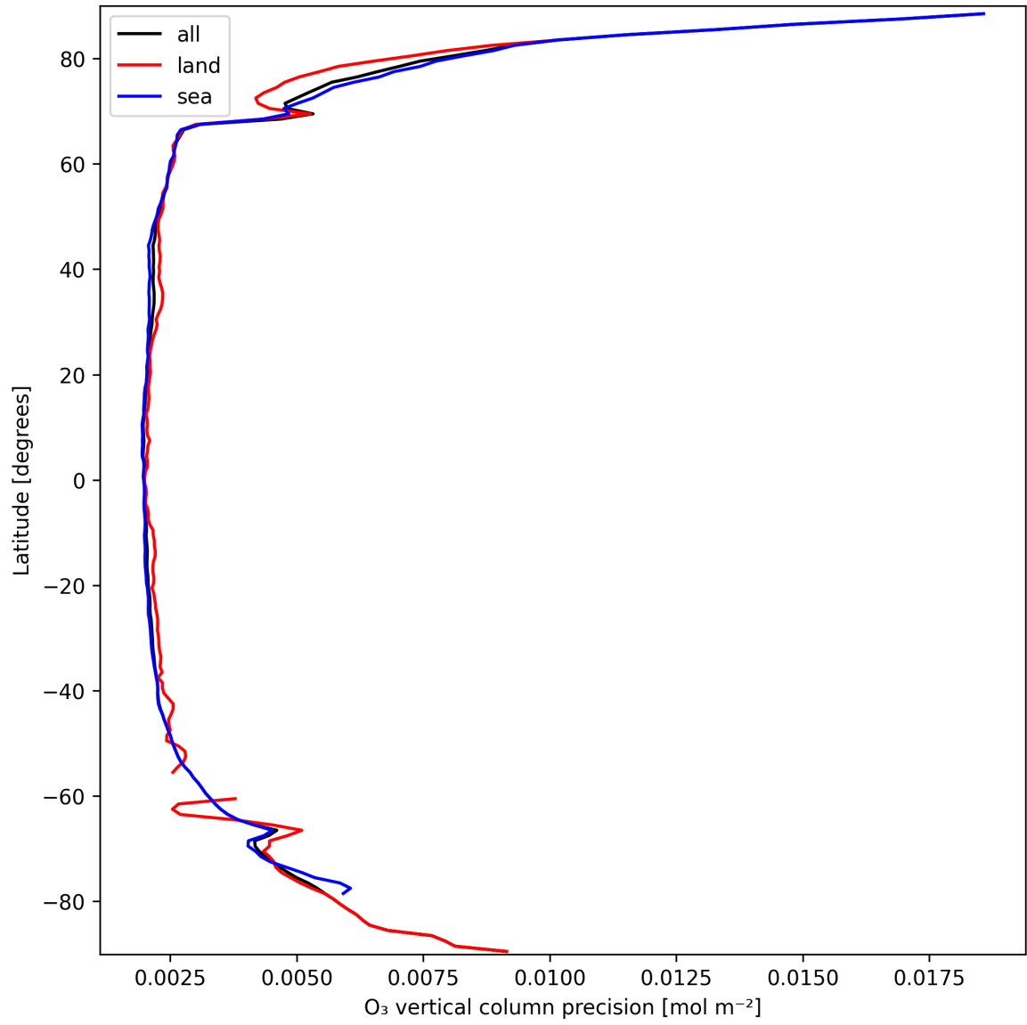
Figure 18: Zonal average of “O 3 vertical column precision” for 2025-09-24 to 2025-09-25.
