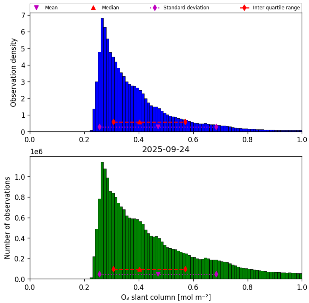
Figure 31: Histogram of “O 3 slant column” for 2025-09-24 to 2025-09-25
