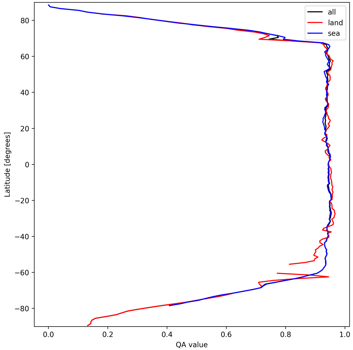
Figure 16: Zonal average of “QA value” for 2025-09-24 to 2025-09-25.
