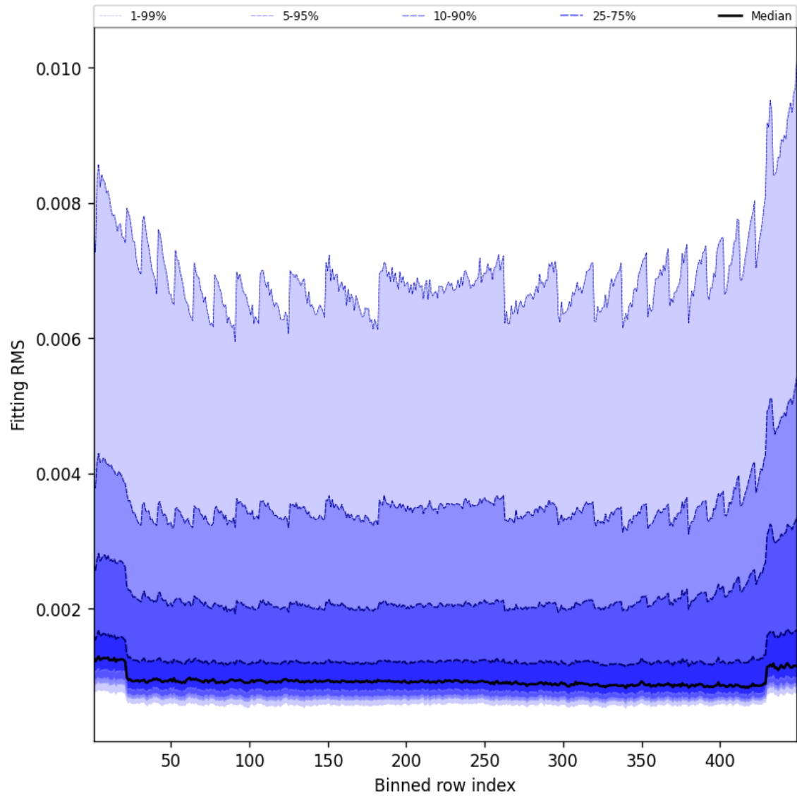
Figure 46: Along track statistics of “Fitting RMS” for 2025-09-24 to 2025-09-25
