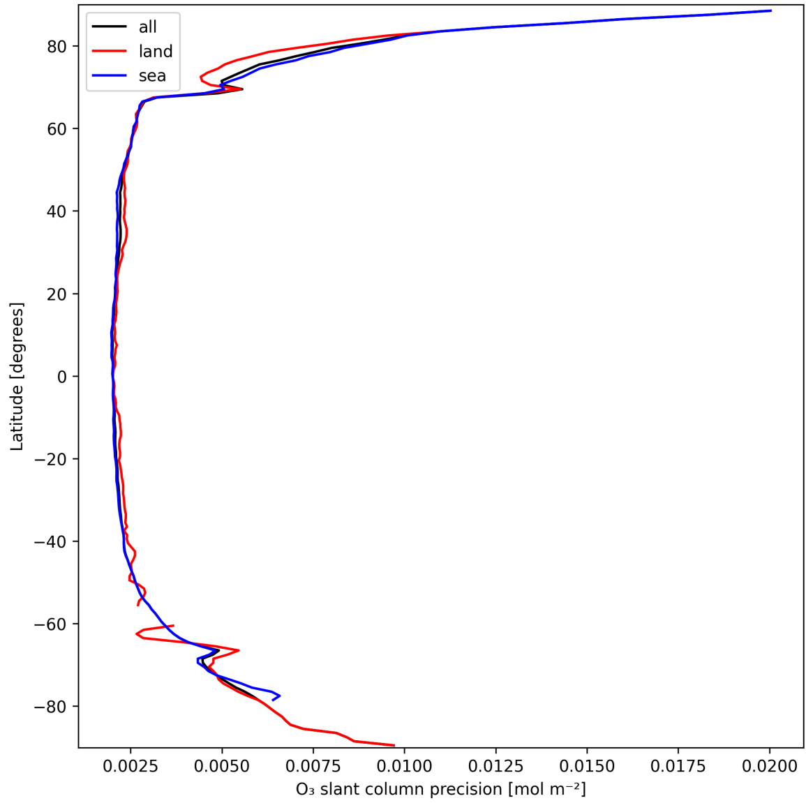
Figure 20: Zonal average of “O 3 slant column precision” for 2025-09-24 to 2025-09-25.
