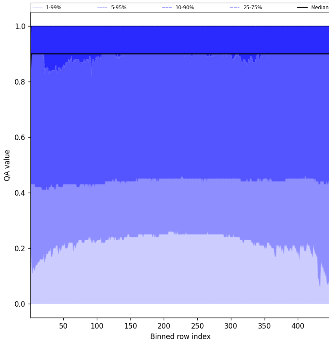
Figure 40: Along track statistics of “QA value” for 2025-09-24 to 2025-09-25
