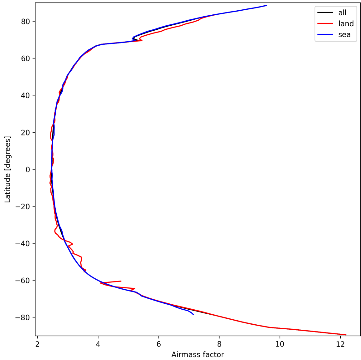
Figure 25: Zonal average of “Airmass factor” for 2025-09-24 to 2025-09-25.
