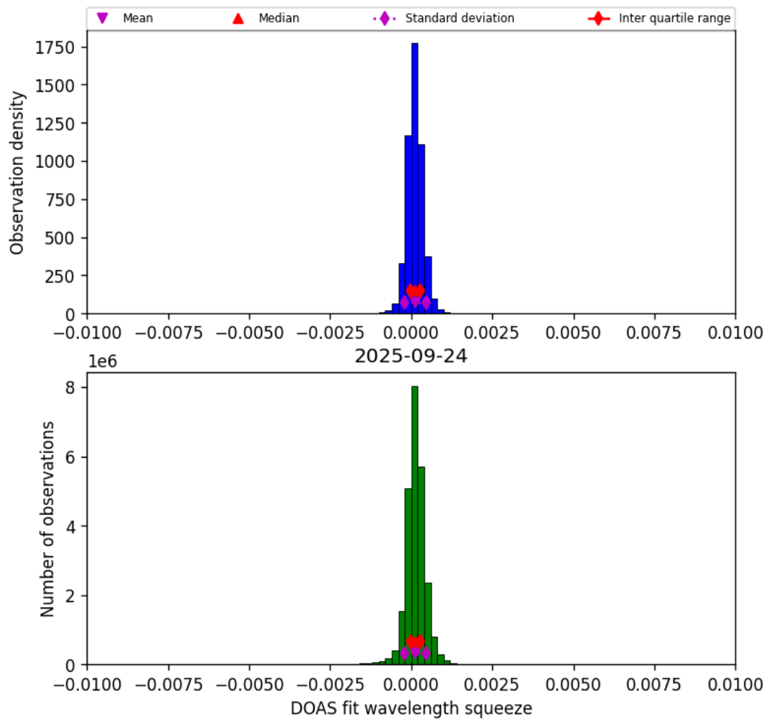
Figure 36: Histogram of “DOAS fit wavelength squeeze” for 2025-09-24 to 2025-09-25
