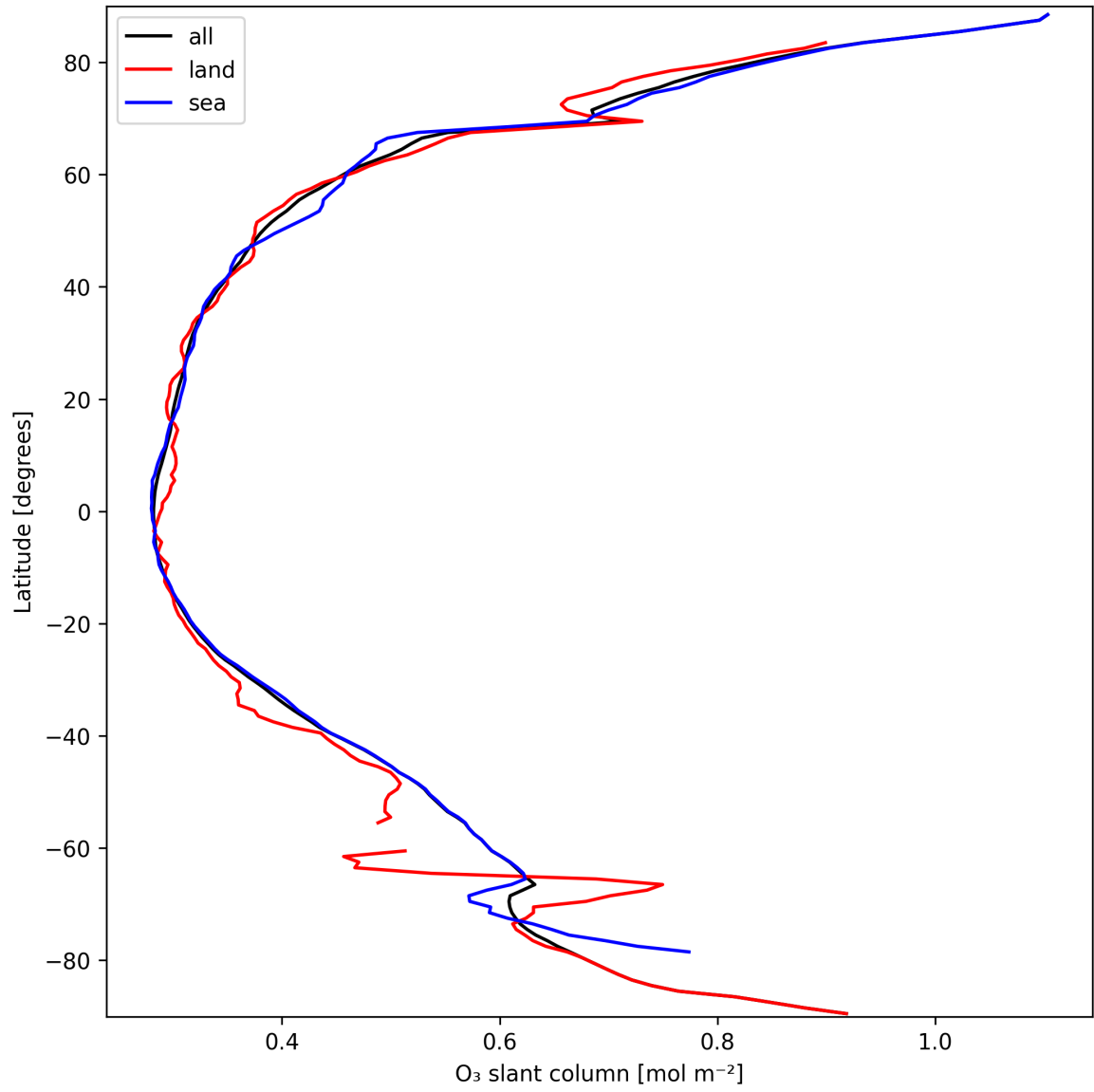
Figure 19: Zonal average of “O 3 slant column” for 2025-09-24 to 2025-09-25.
