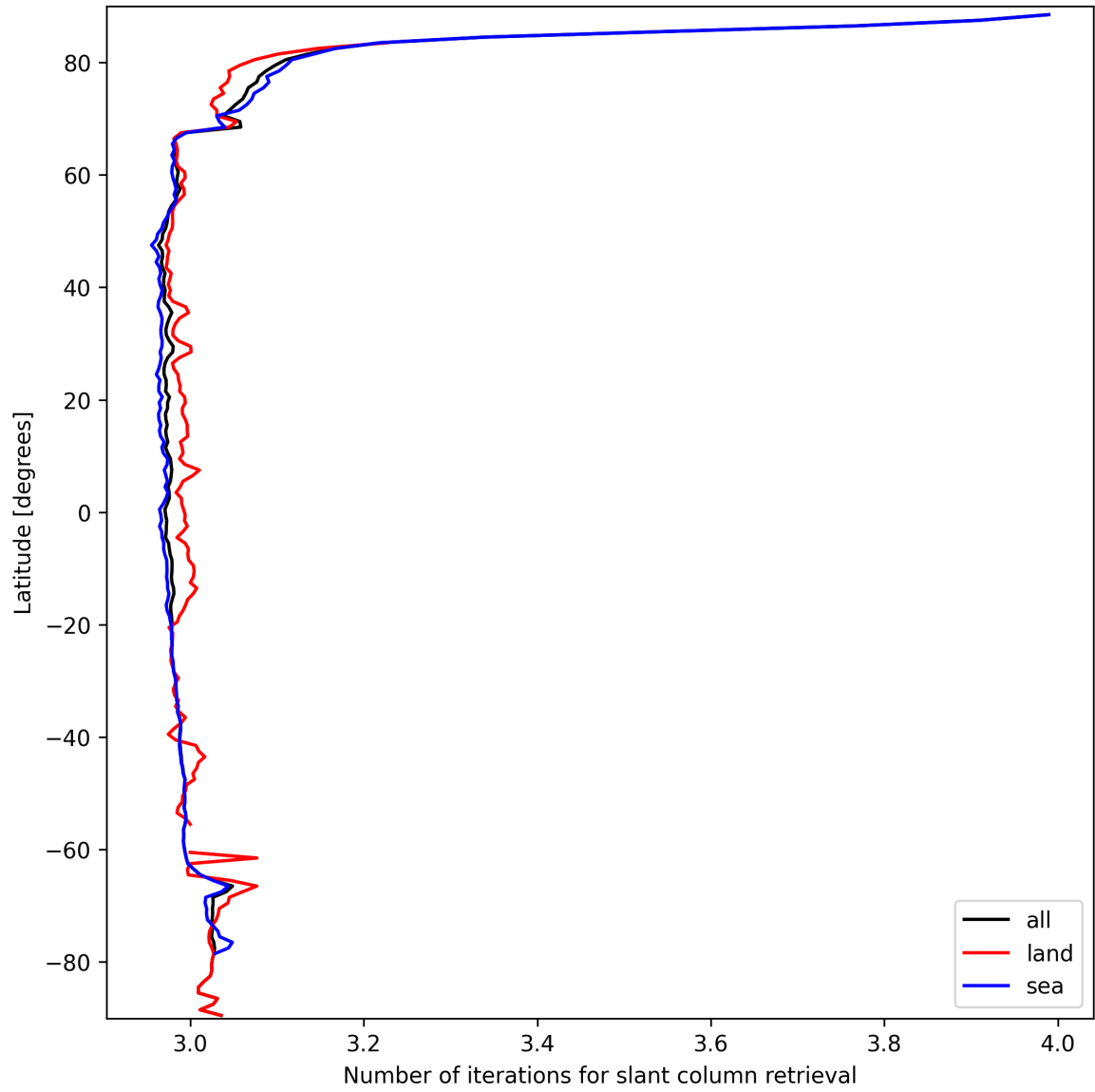
Figure 21: Zonal average of “Number of iterations for slant column retrieval” for 2025-09-24 to 2025-09-25.
