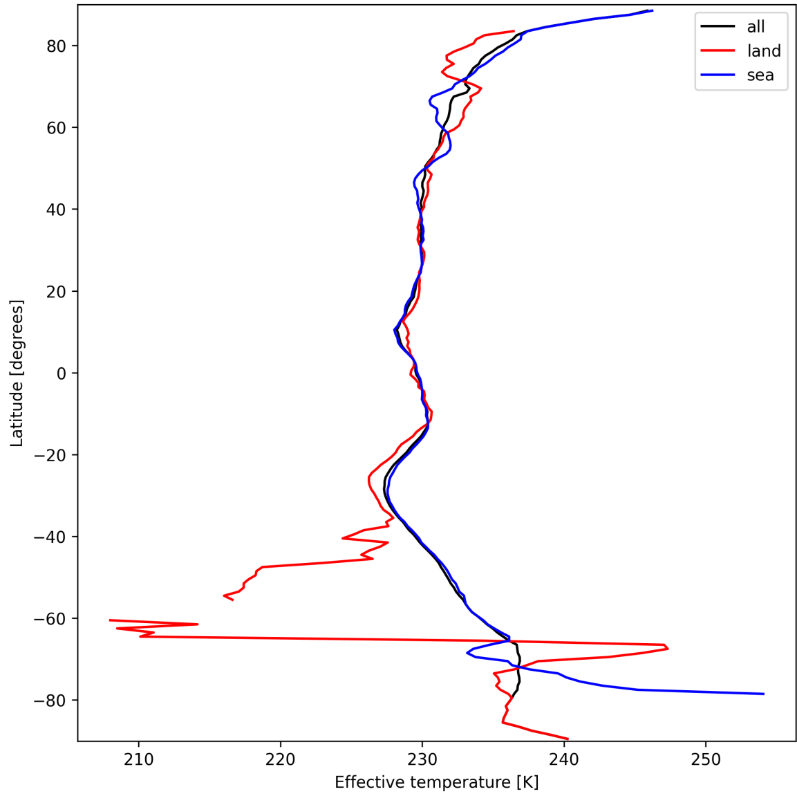
Figure 26: Zonal average of “Effective temperature” for 2025-09-24 to 2025-09-25.
