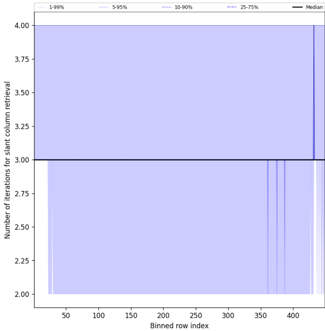
Figure 45: Along track statistics of “Number of iterations for slant column retrieval” for 2025-09-24 to 2025-09-25
