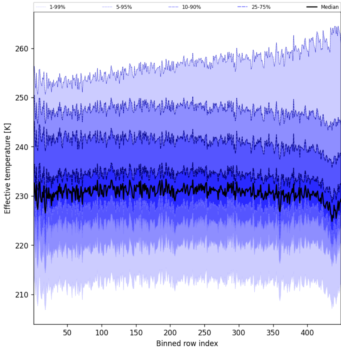
Figure 50: Along track statistics of “Effective temperature” for 2025-09-24 to 2025-09-25
