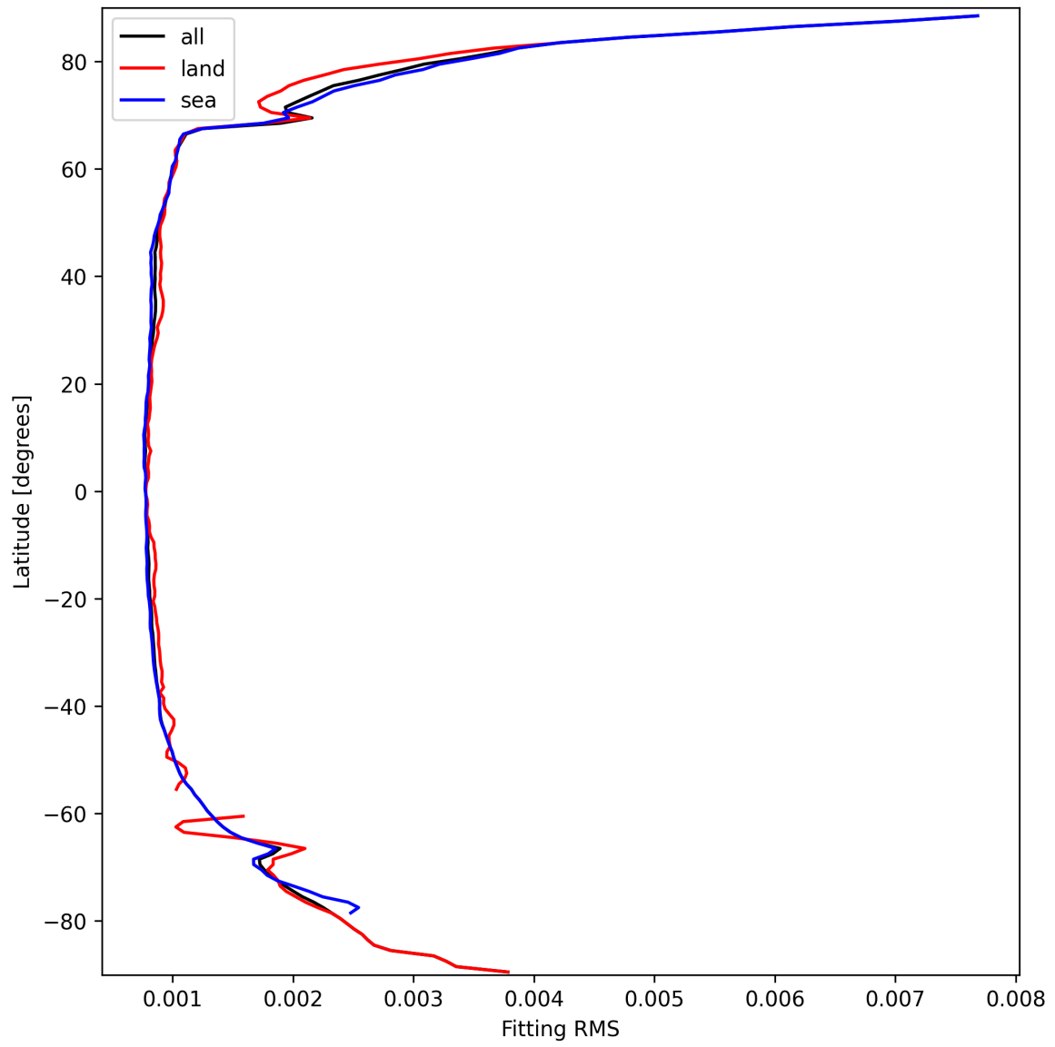
Figure 22: Zonal average of “Fitting RMS” for 2025-09-24 to 2025-09-25.
