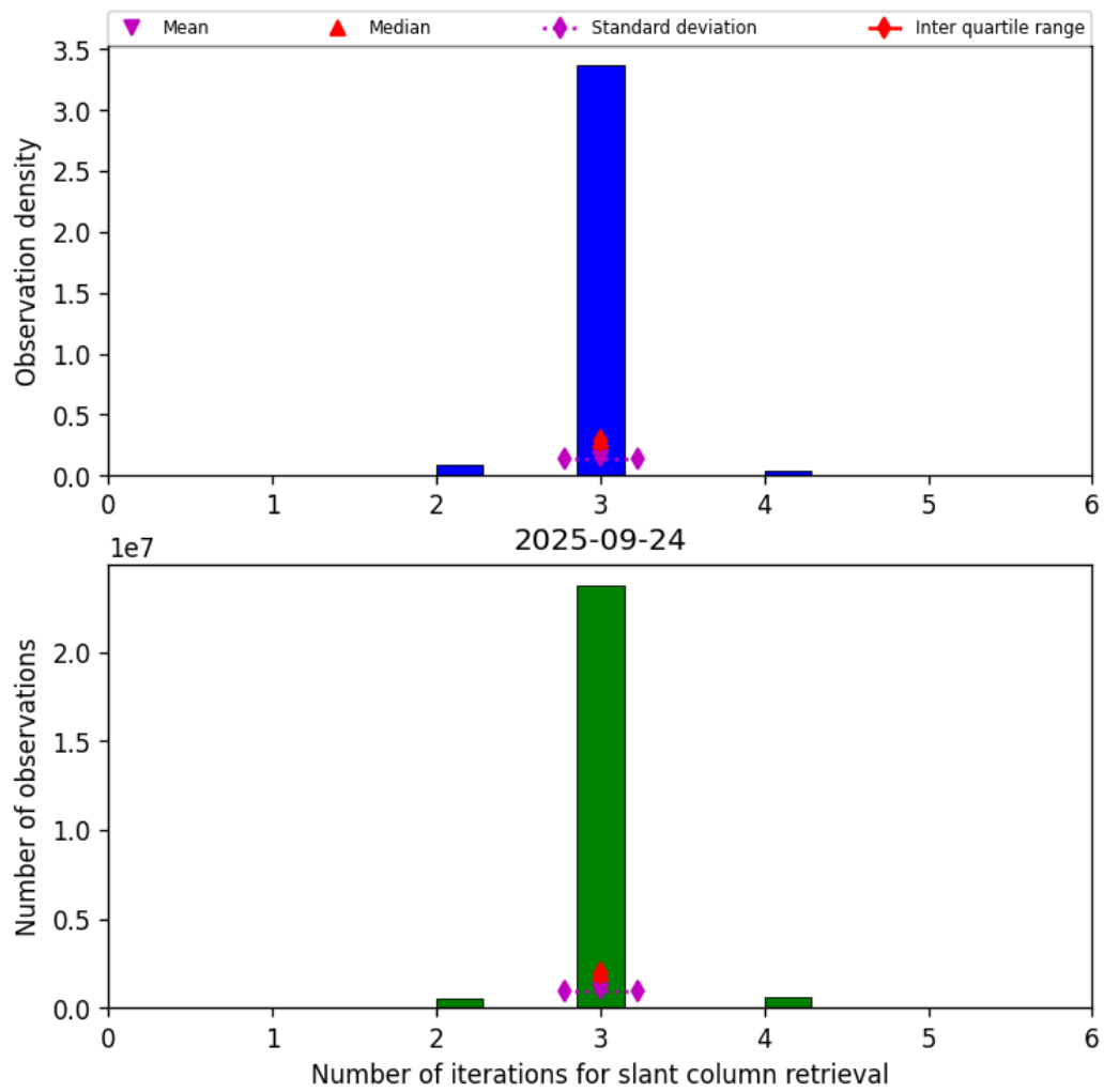
Figure 33: Histogram of “Number of iterations for slant column retrieval” for 2025-09-24 to 2025-09-25
