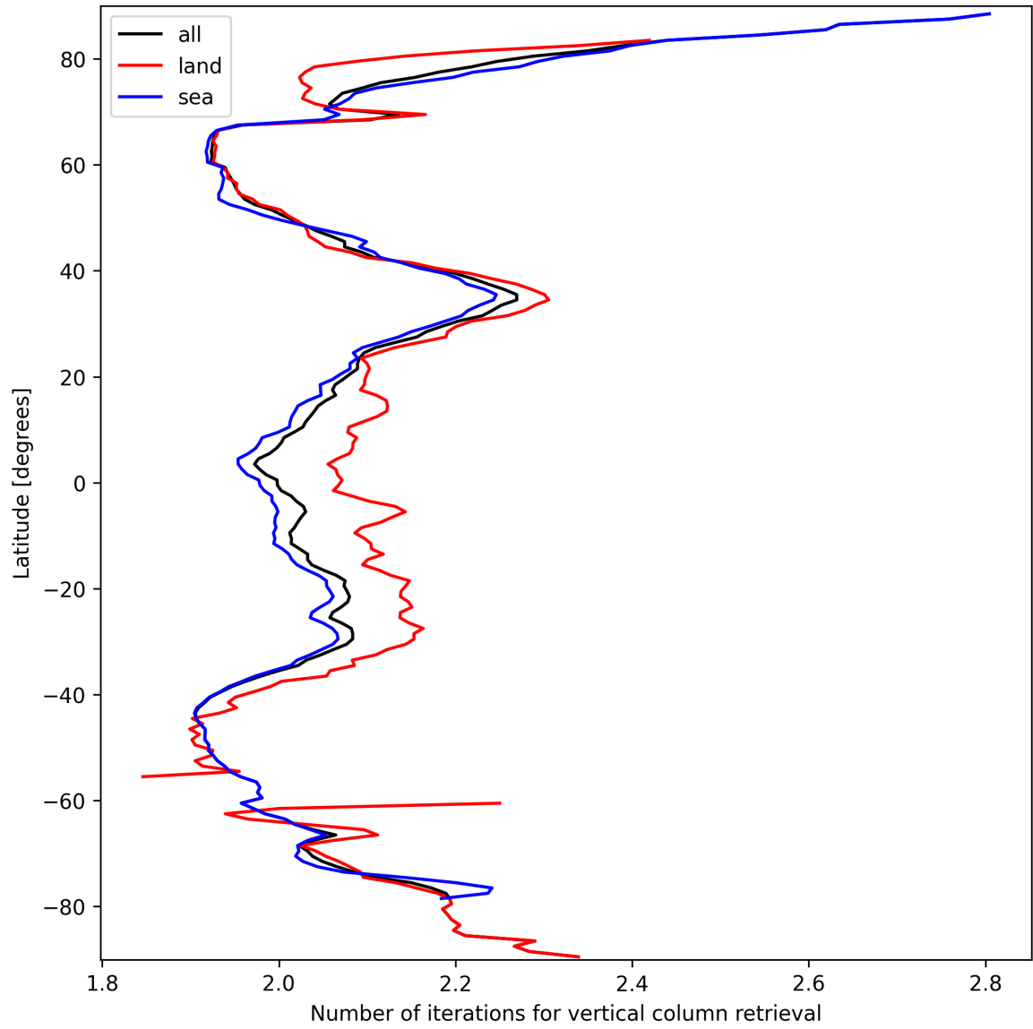
Figure 27: Zonal average of “Number of iterations for vertical column retrieval” for 2025-09-24 to 2025-09-25.
