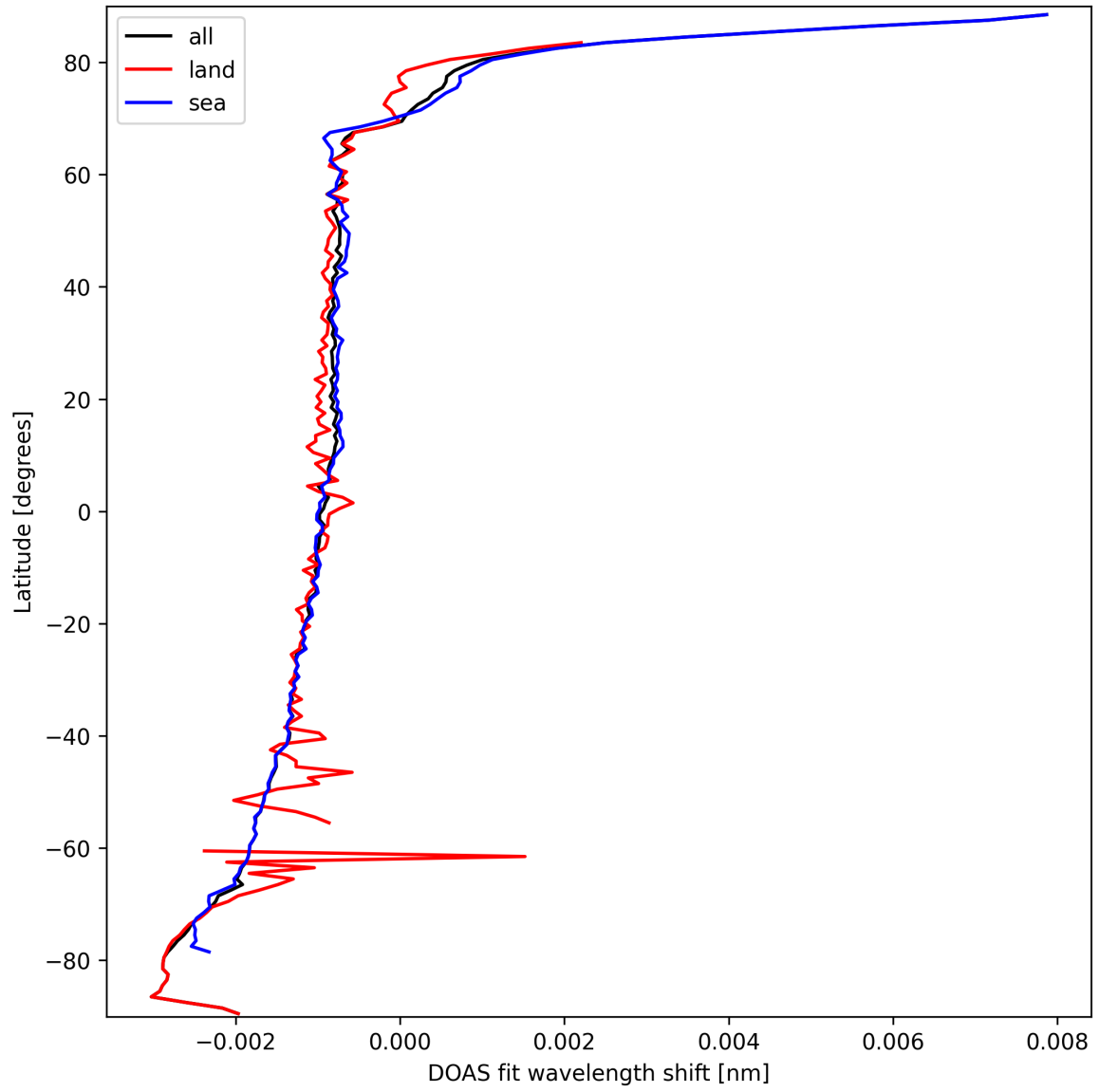
Figure 23: Zonal average of “DOAS fit wavelength shift” for 2025-09-24 to 2025-09-25.
