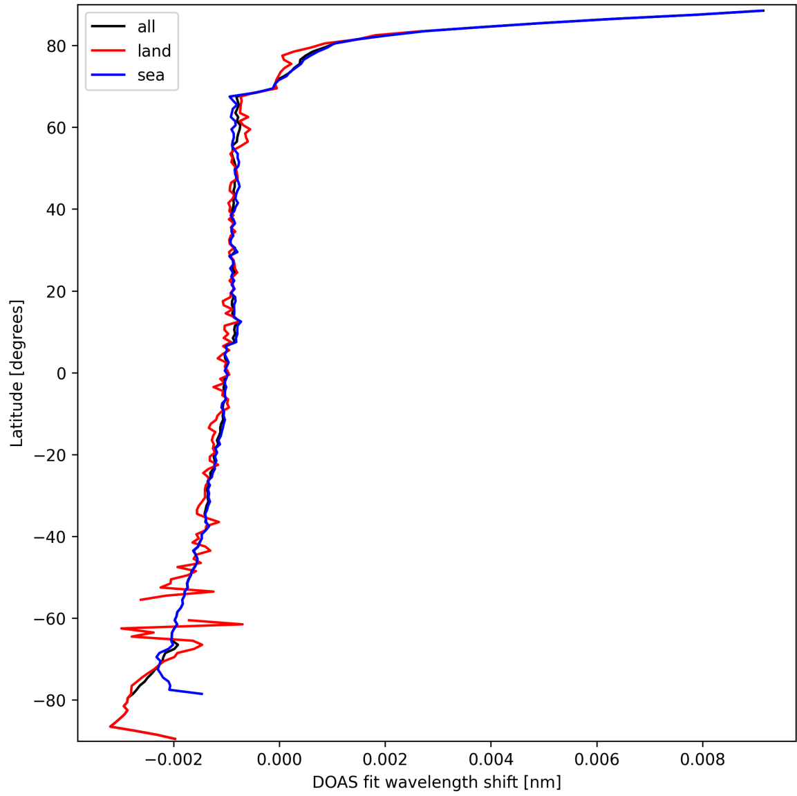
Figure 23: Zonal average of “DOAS fit wavelength shift” for 2025-09-25 to 2025-09-26.
