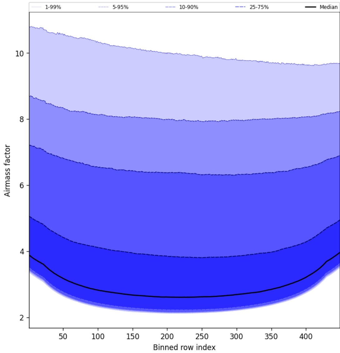
Figure 49: Along track statistics of “Airmass factor” for 2025-09-25 to 2025-09-26
