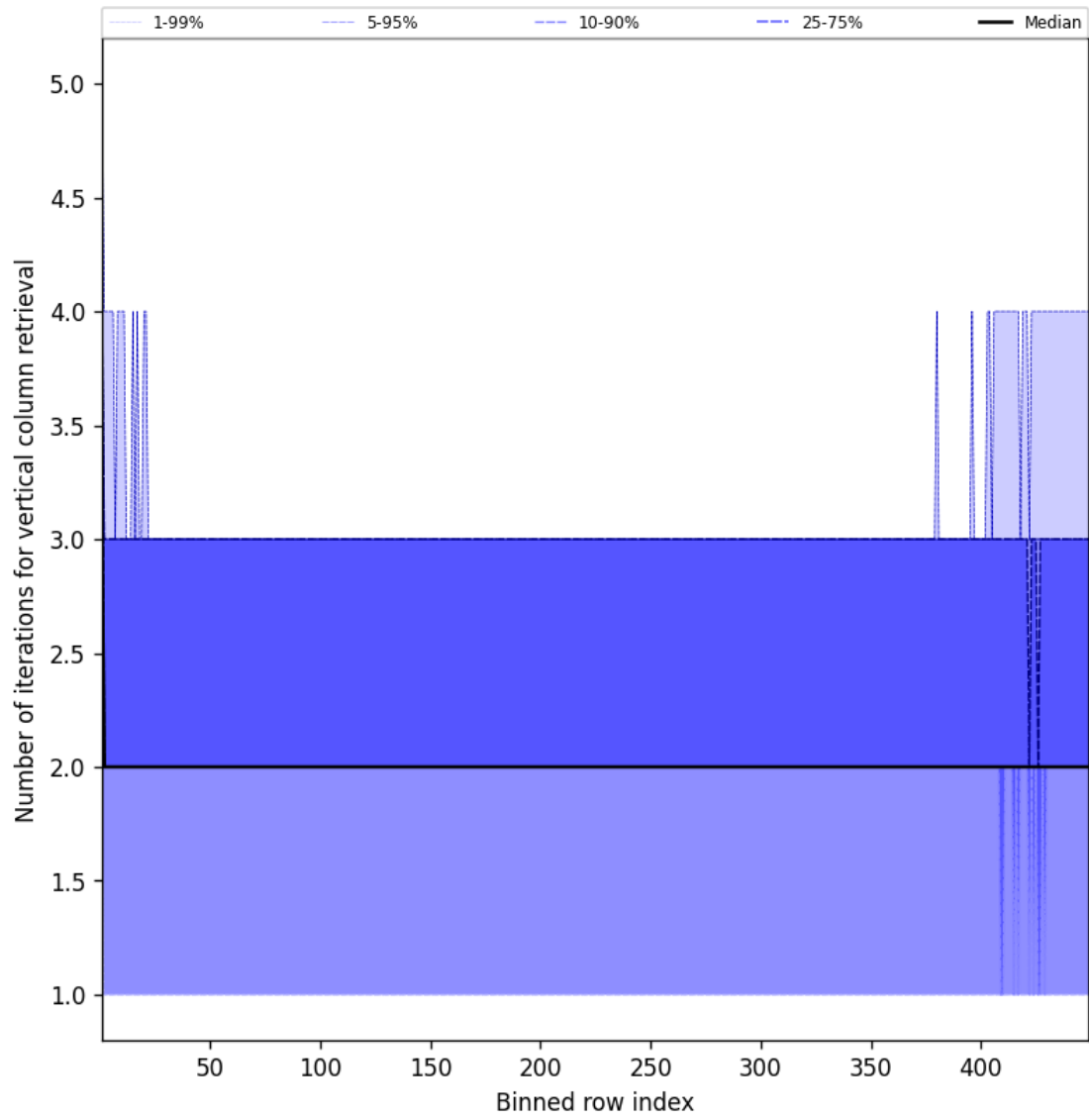
Figure 51: Along track statistics of “Number of iterations for vertical column retrieval” for 2025-09-25 to 2025-09-26
