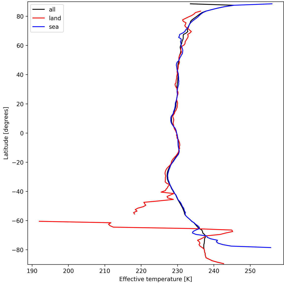
Figure 26: Zonal average of “Effective temperature” for 2025-09-25 to 2025-09-26.
