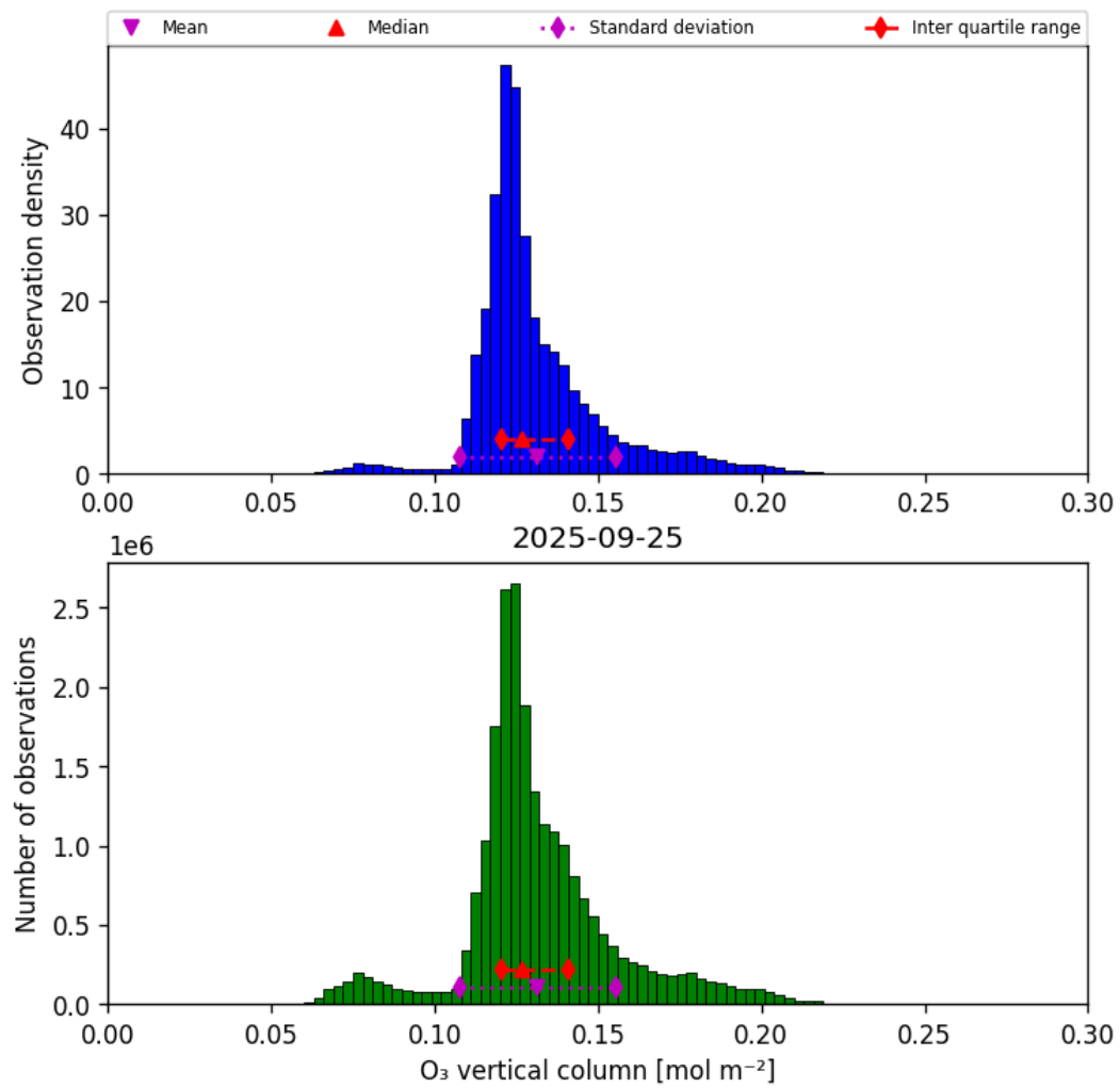
Figure 29: Histogram of “O 3 vertical column” for 2025-09-25 to 2025-09-26
