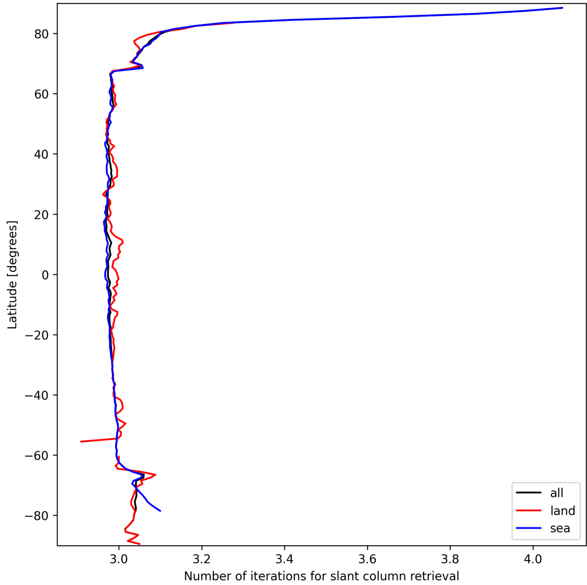
Figure 21: Zonal average of “Number of iterations for slant column retrieval” for 2025-09-25 to 2025-09-26.
