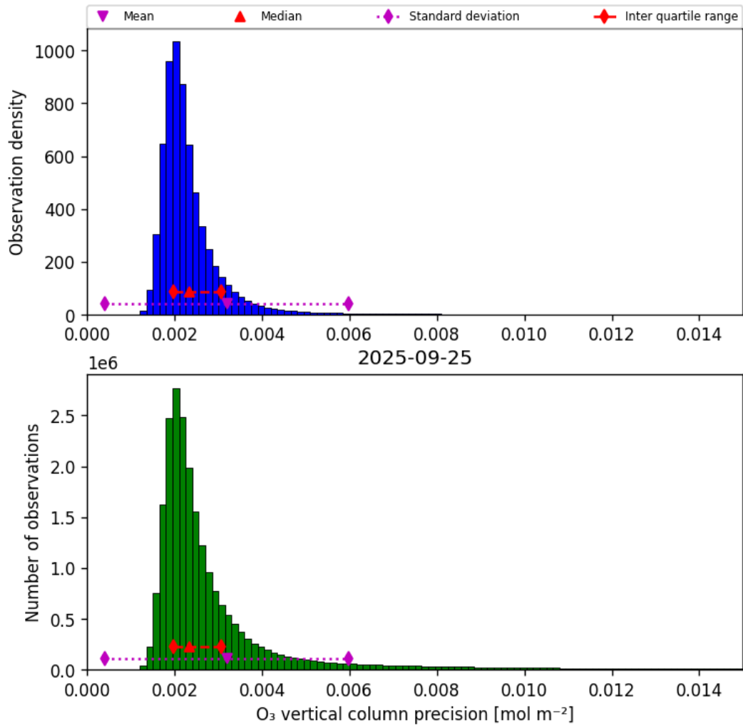
Figure 30: Histogram of “O 3 vertical column precision” for 2025-09-25 to 2025-09-26
