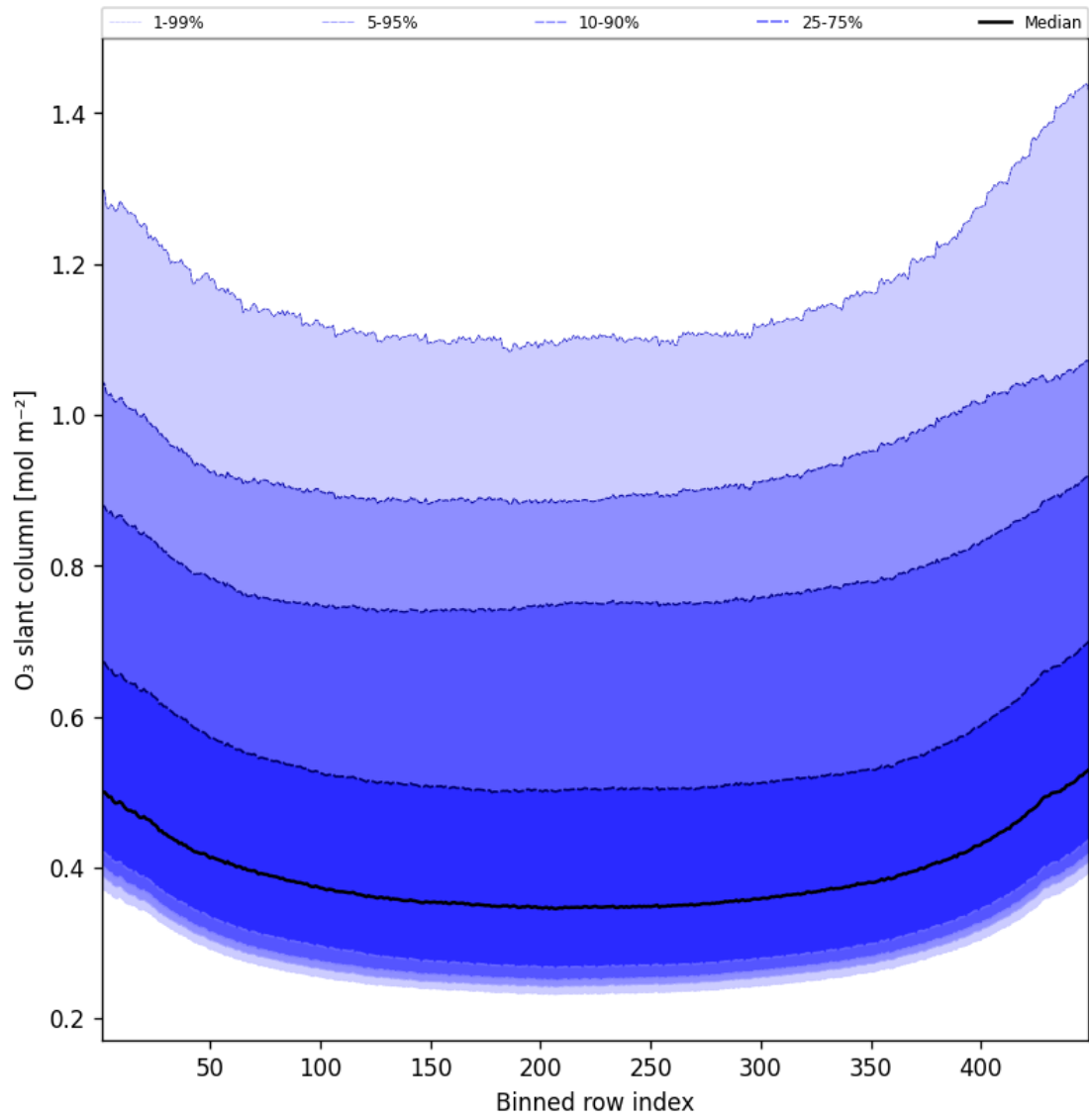
Figure 43: Along track statistics of “O 3 slant column” for 2025-09-25 to 2025-09-26
