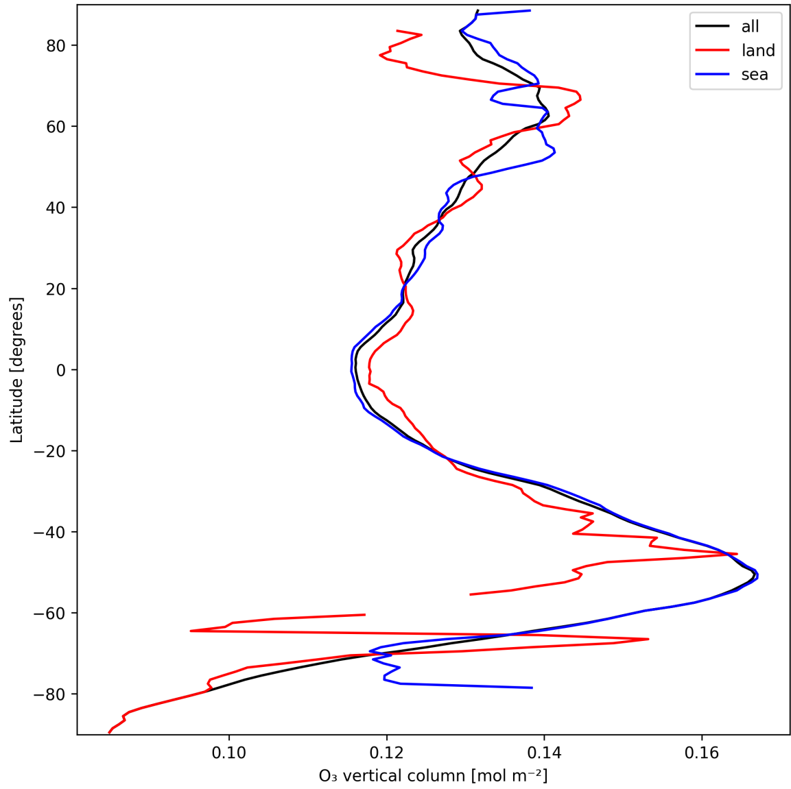
Figure 17: Zonal average of “O 3 vertical column” for 2025-09-25 to 2025-09-26.
