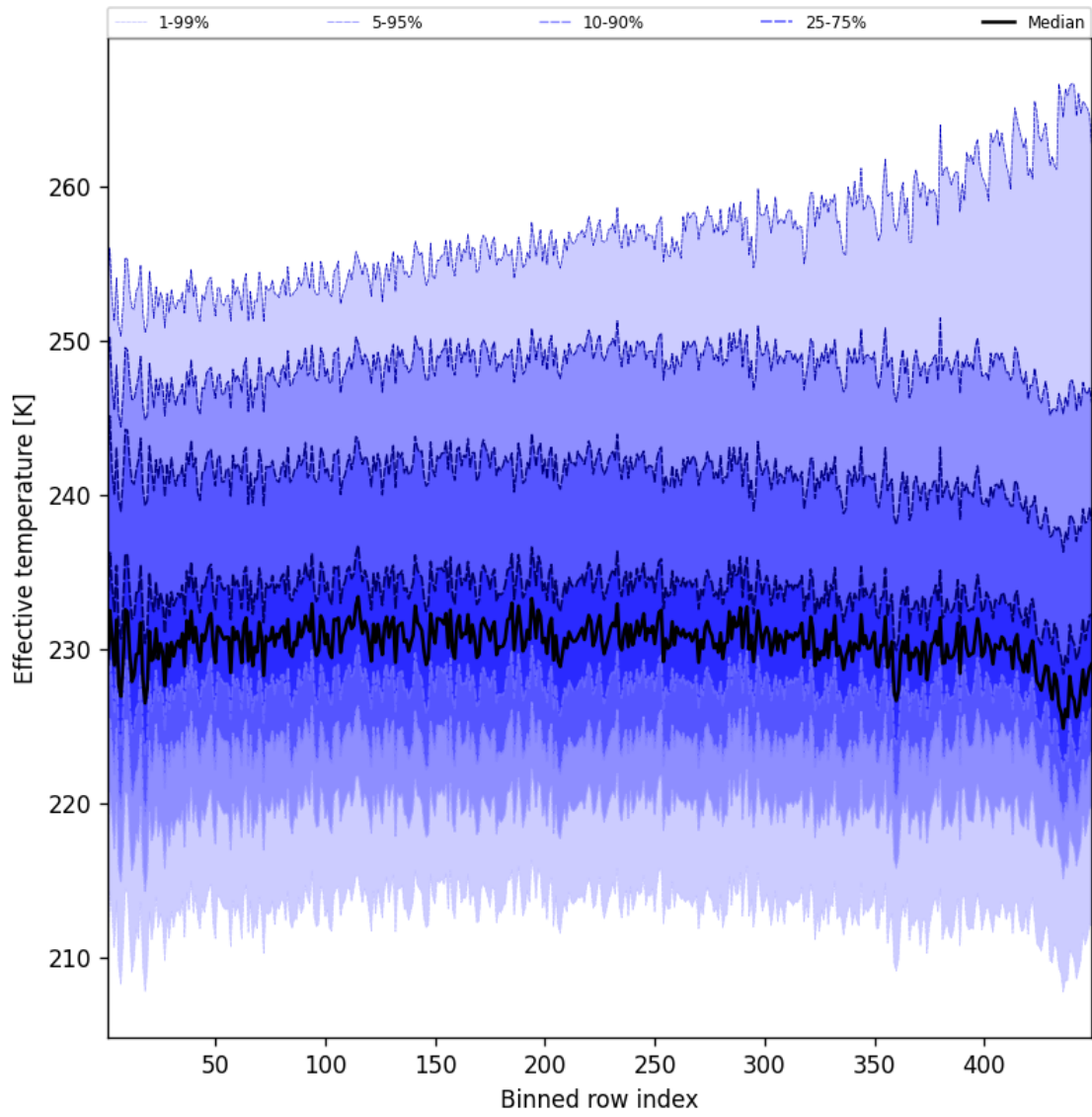
Figure 50: Along track statistics of “Effective temperature” for 2025-09-25 to 2025-09-26
