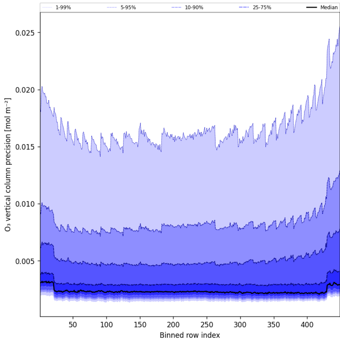
Figure 42: Along track statistics of “O 3 vertical column precision” for 2025-09-25 to 2025-09-26
