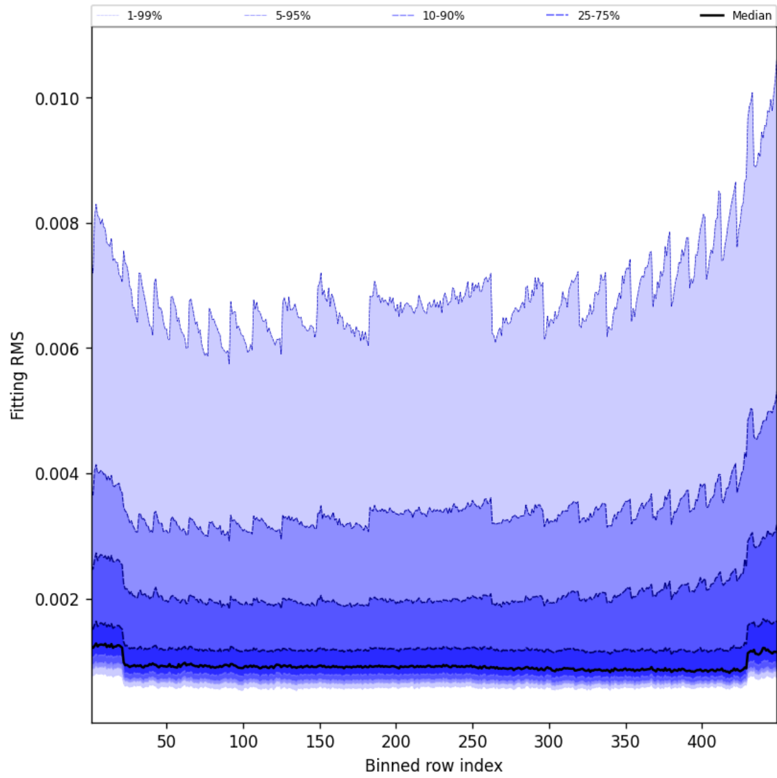
Figure 46: Along track statistics of “Fitting RMS” for 2025-09-25 to 2025-09-26
