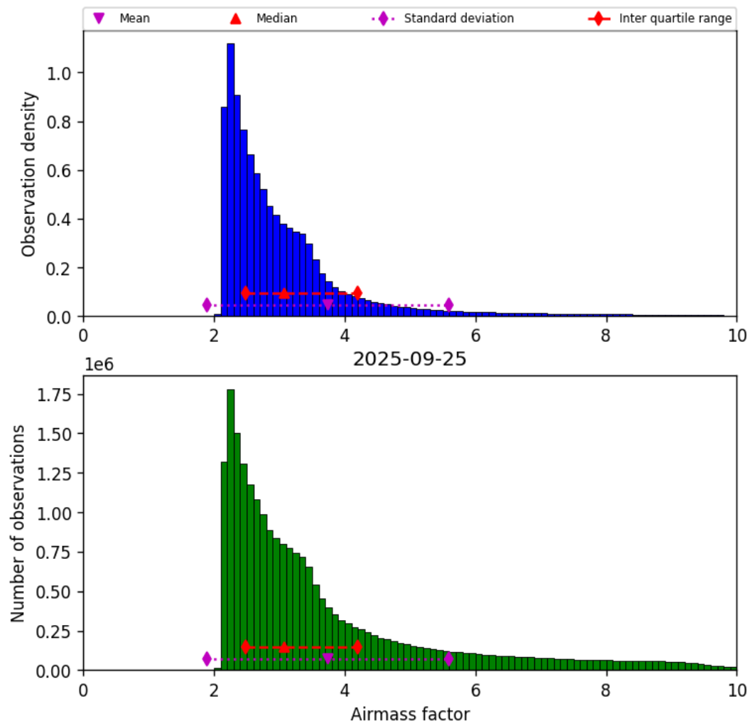
Figure 37: Histogram of “Airmass factor” for 2025-09-25 to 2025-09-26
