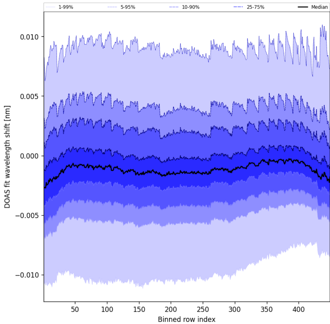
Figure 47: Along track statistics of “DOAS fit wavelength shift” for 2025-09-25 to 2025-09-26
