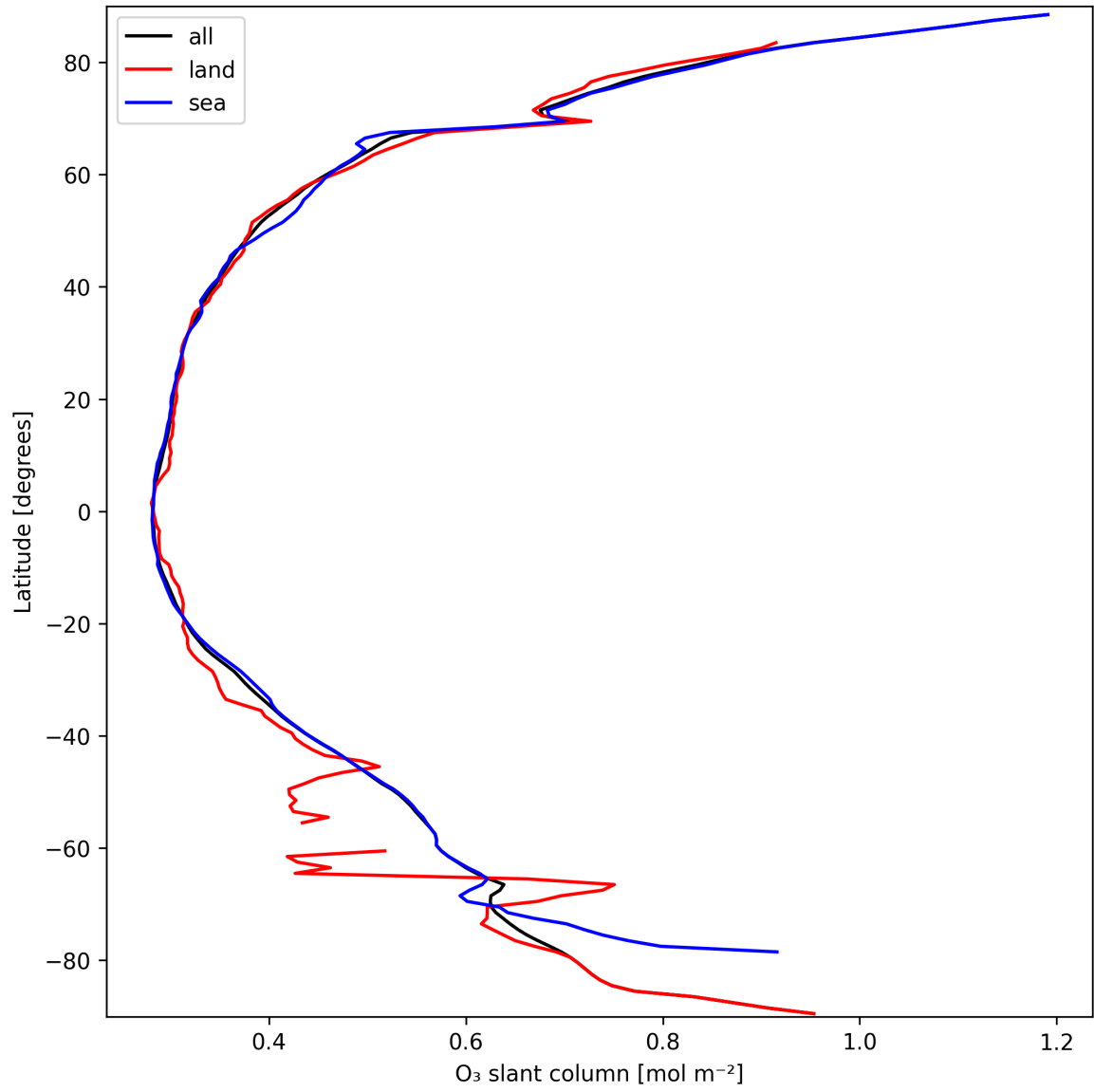
Figure 19: Zonal average of “O 3 slant column” for 2025-09-25 to 2025-09-26.
