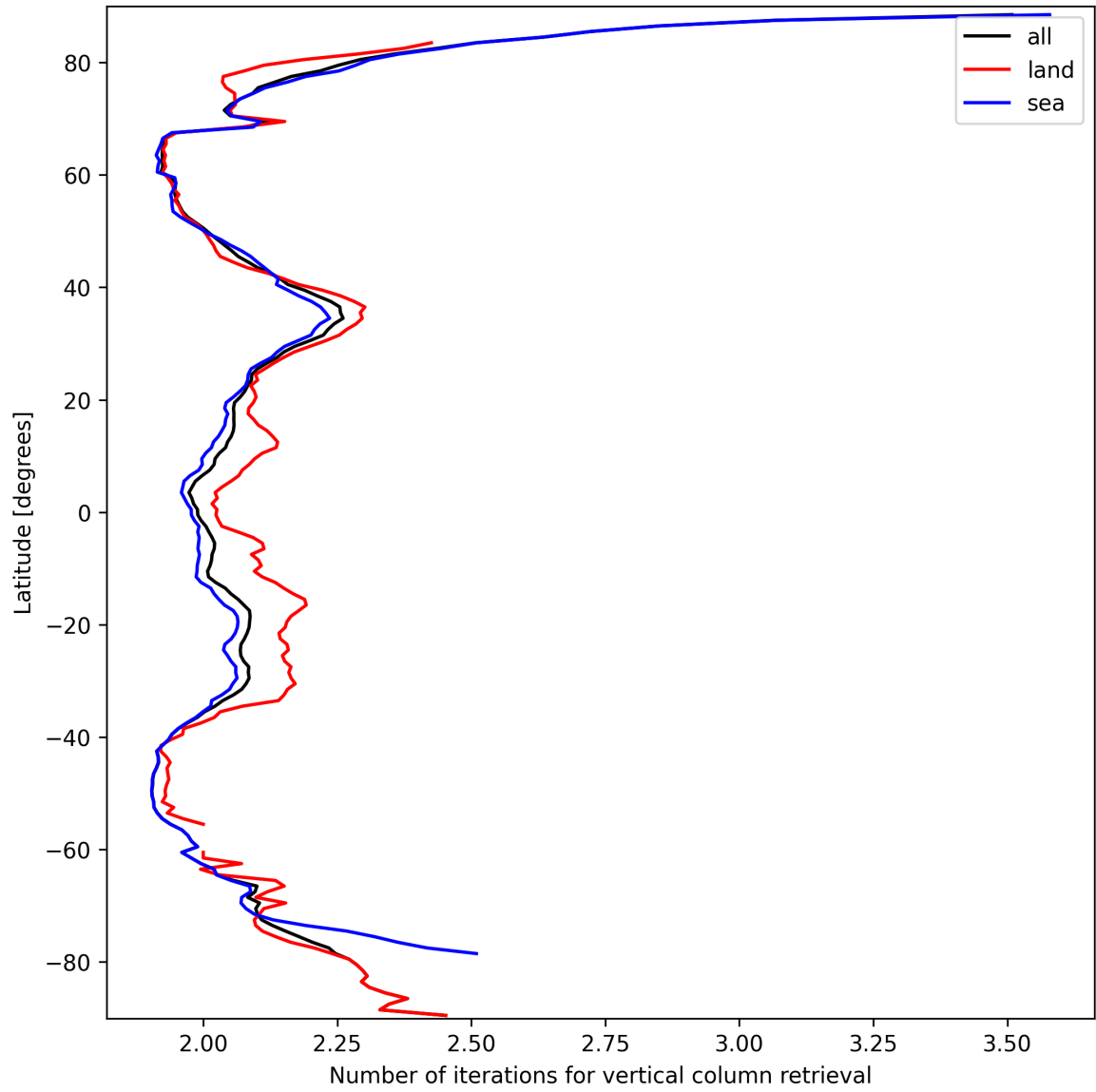
Figure 27: Zonal average of “Number of iterations for vertical column retrieval” for 2025-09-25 to 2025-09-26.
