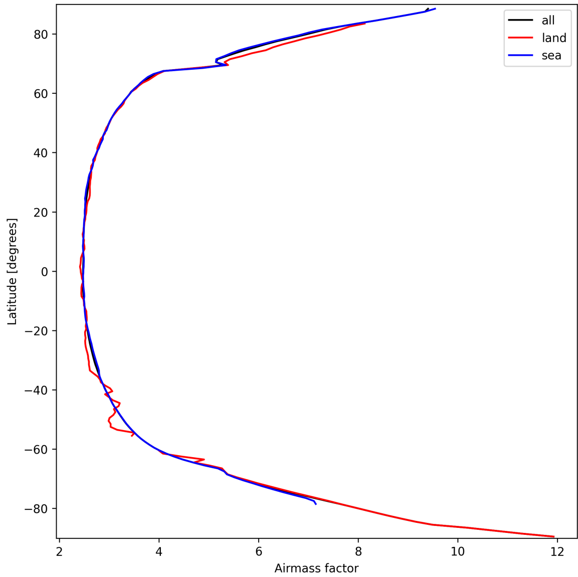
Figure 25: Zonal average of “Airmass factor” for 2025-09-25 to 2025-09-26.
