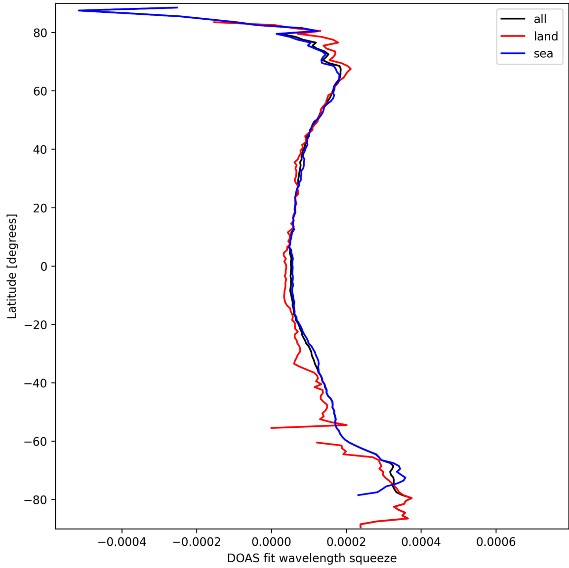
Figure 24: Zonal average of "DOAS fit wavelength squeeze" for 2025-09-25 to 2025-09-26.
