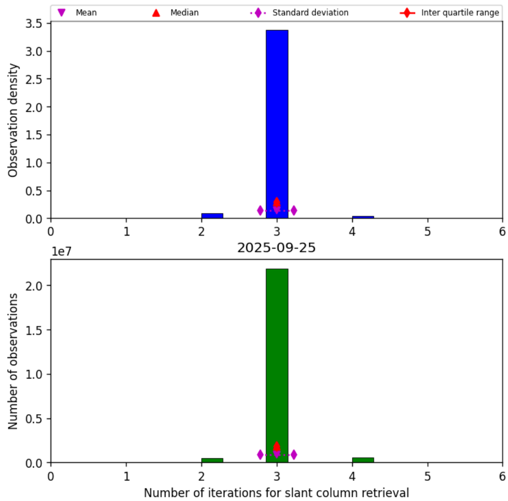
Figure 33: Histogram of “Number of iterations for slant column retrieval” for 2025-09-25 to 2025-09-26
