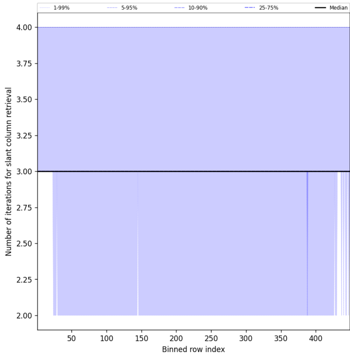
Figure 45: Along track statistics of “Number of iterations for slant column retrieval” for 2025-09-25 to 2025-09-26
