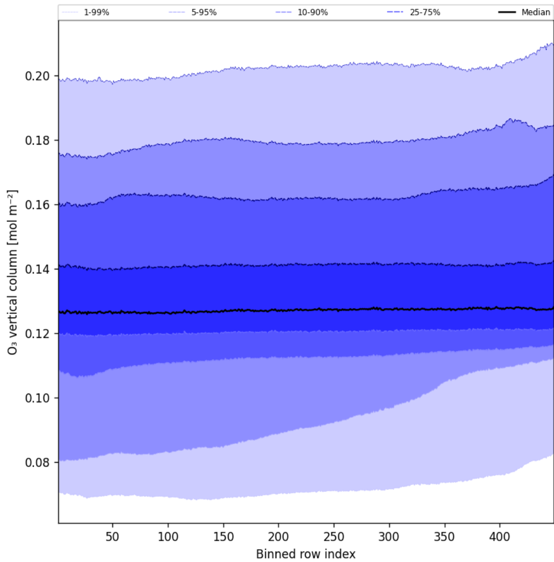
Figure 41: Along track statistics of “O 3 vertical column” for 2025-09-25 to 2025-09-26
