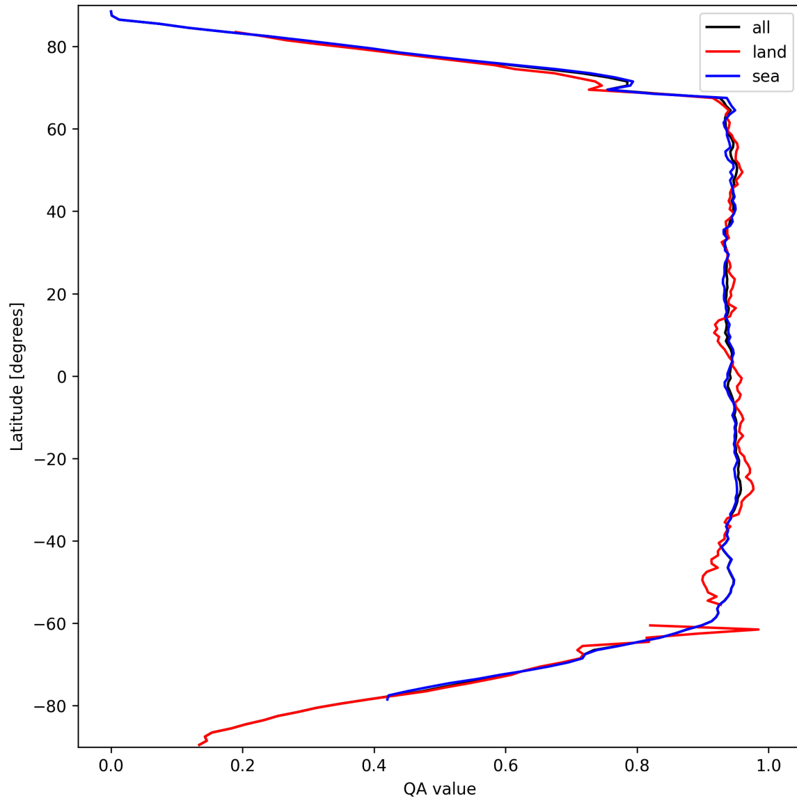
Figure 16: Zonal average of “QA value” for 2025-09-25 to 2025-09-26.
