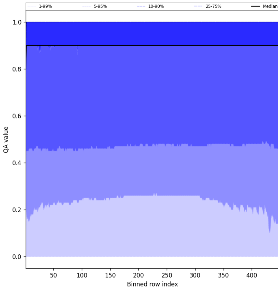
Figure 40: Along track statistics of “QA value” for 2025-09-25 to 2025-09-26
