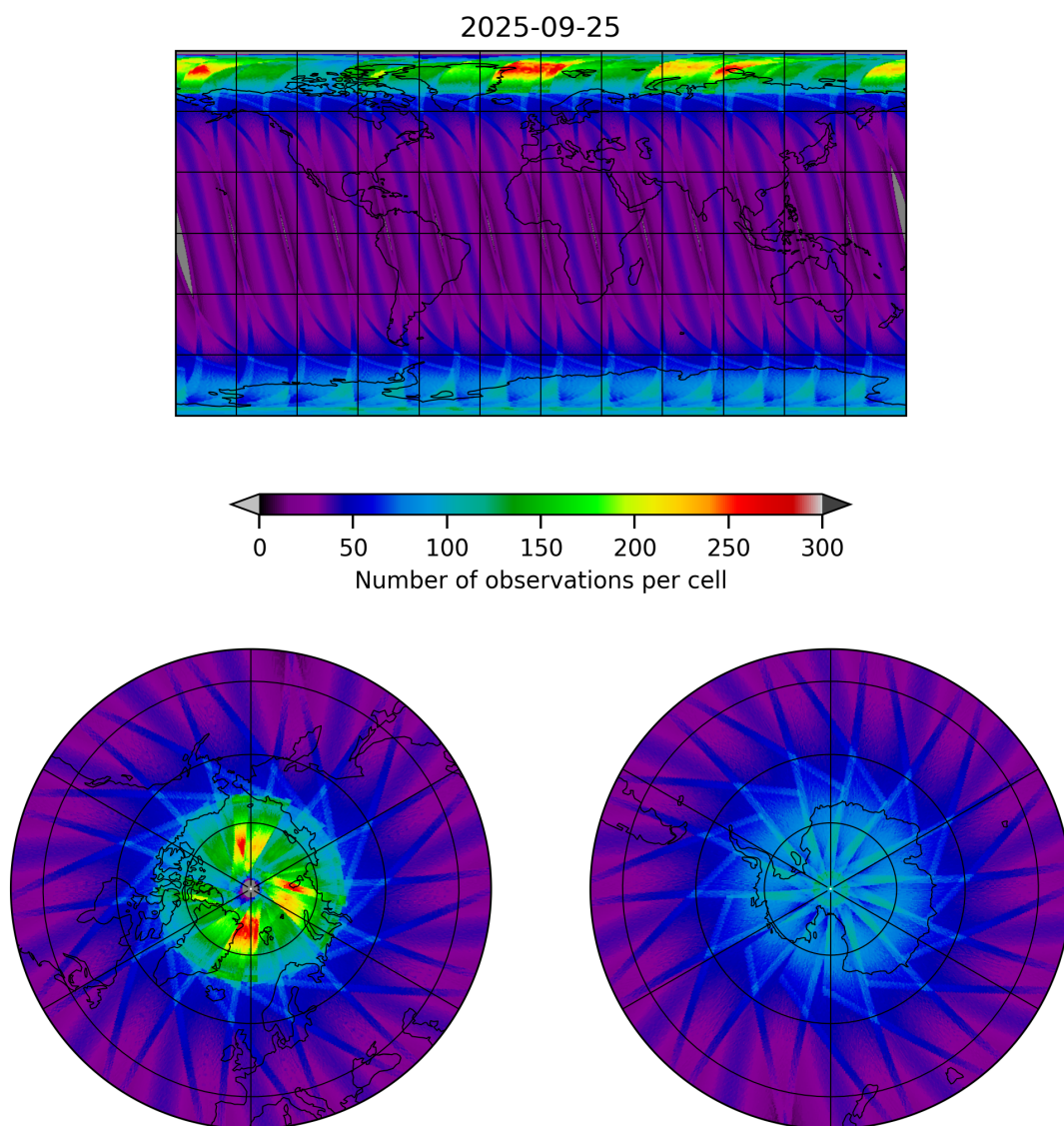
Figure 15: Map of the number of observations for 2025-09-25 to 2025-09-26
