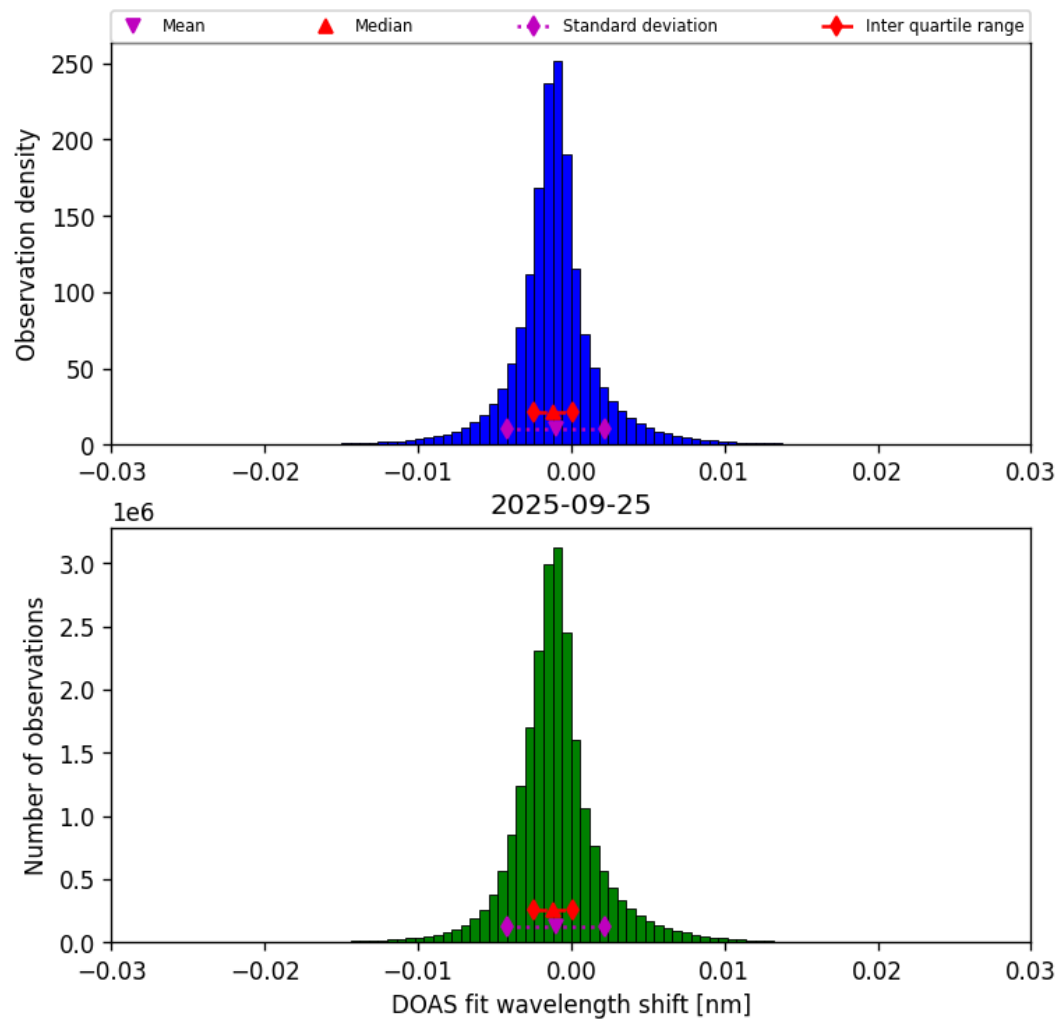
Figure 35: Histogram of “DOAS fit wavelength shift” for 2025-09-25 to 2025-09-26
