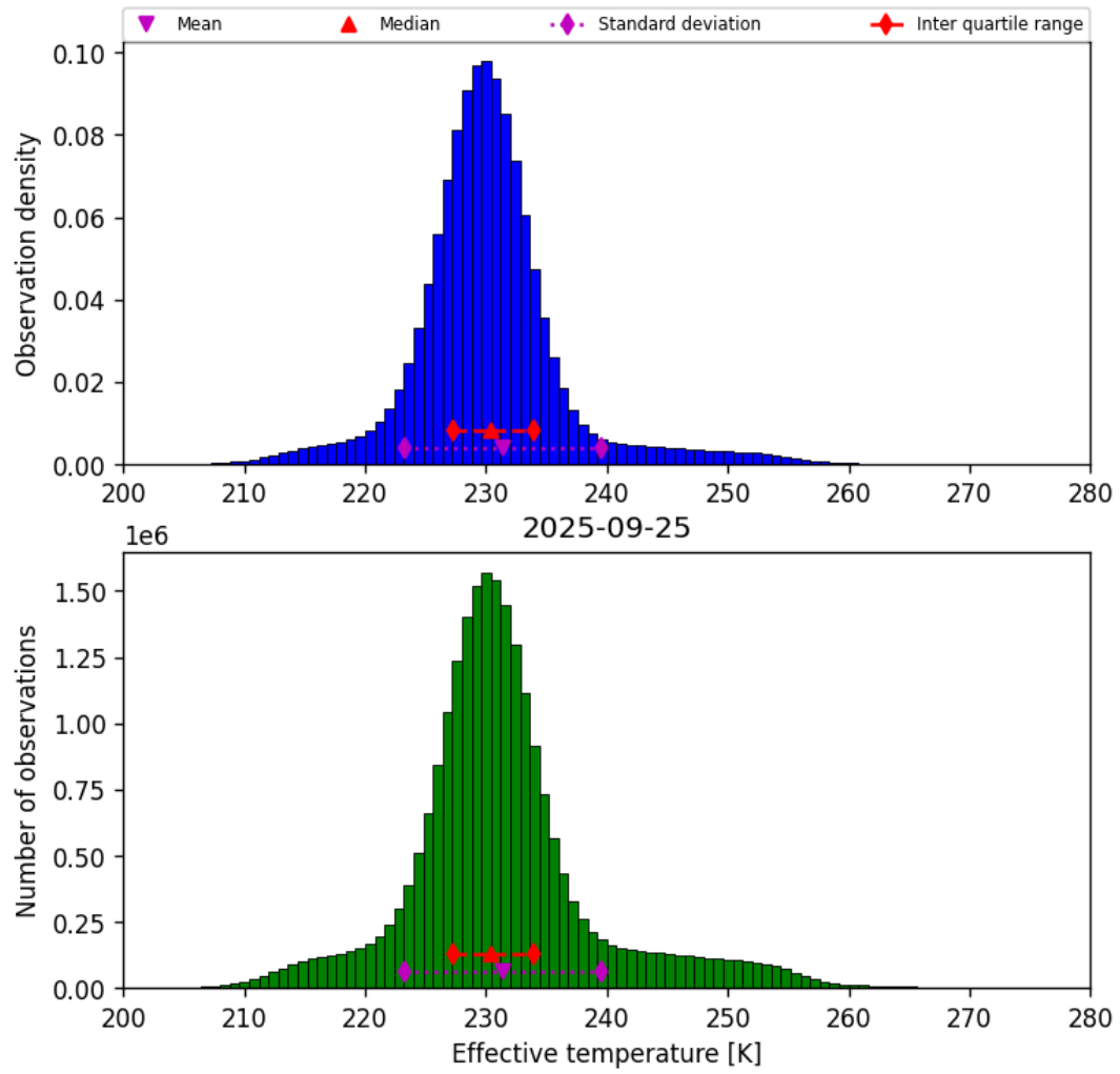
Figure 38: Histogram of “Effective temperature” for 2025-09-25 to 2025-09-26
