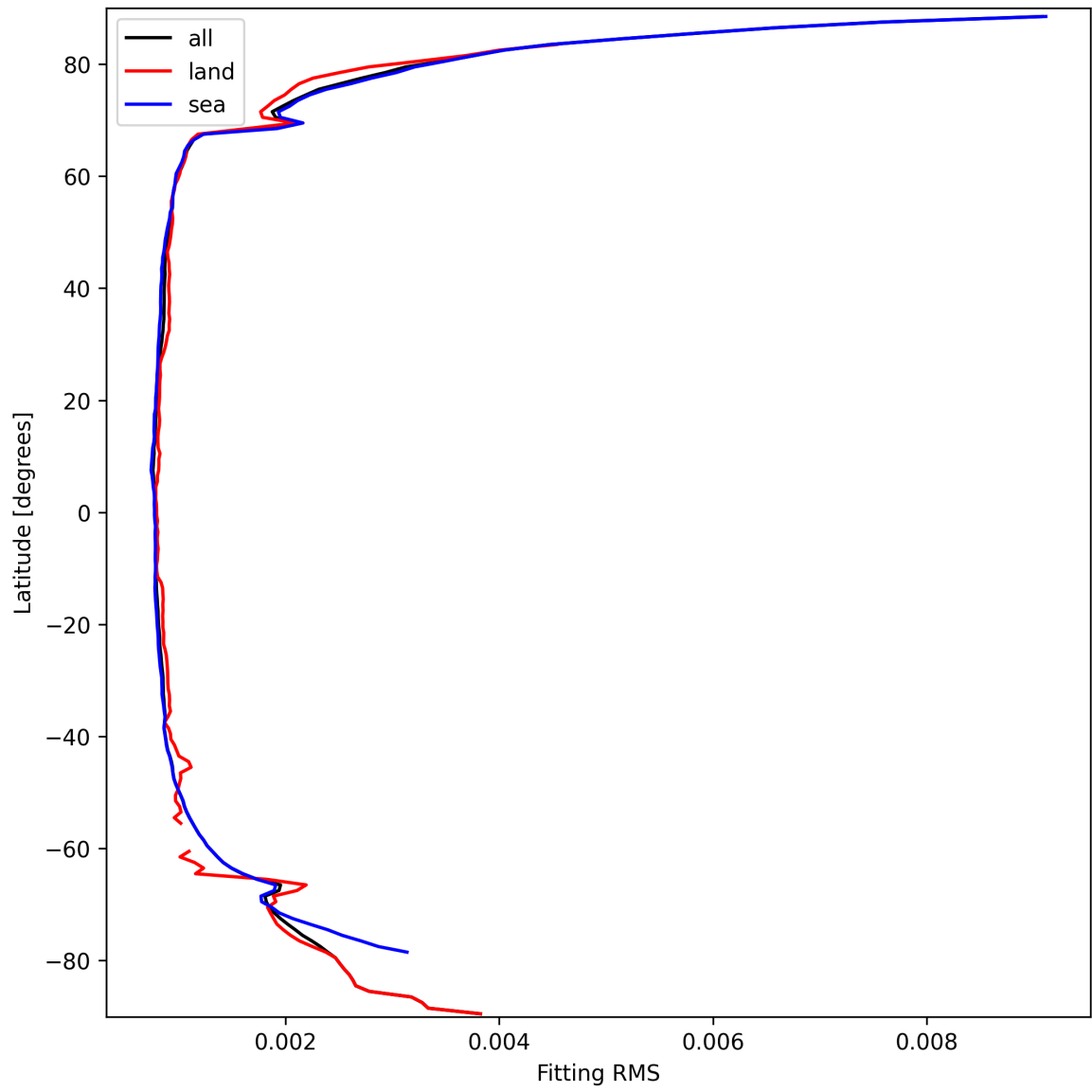
Figure 22: Zonal average of “Fitting RMS” for 2025-09-25 to 2025-09-26.
