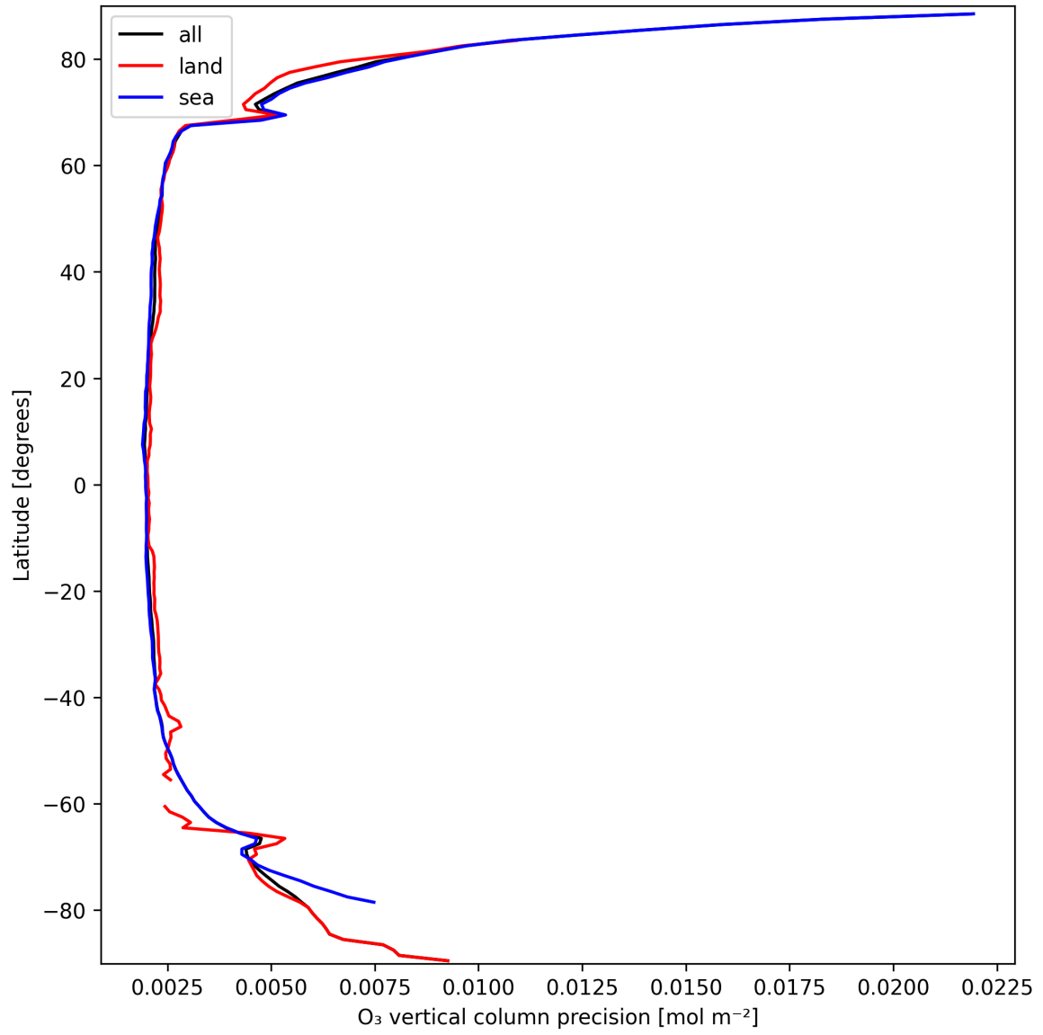
Figure 18: Zonal average of “O 3 vertical column precision” for 2025-09-25 to 2025-09-26.
