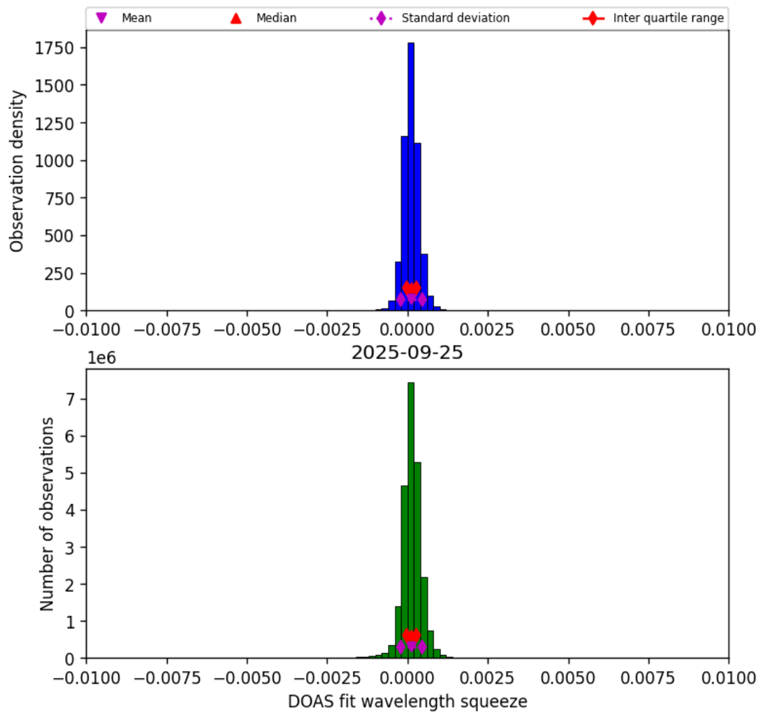
Figure 36: Histogram of “DOAS fit wavelength squeeze” for 2025-09-25 to 2025-09-26
