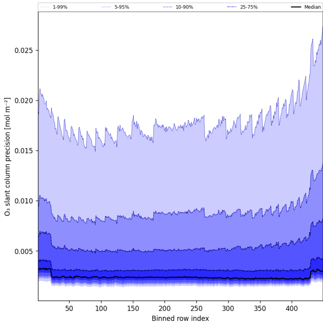
Figure 44: Along track statistics of “O 3 slant column precision” for 2025-09-25 to 2025-09-26
