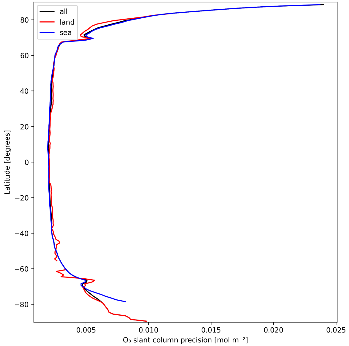
Figure 20: Zonal average of “O 3 slant column precision” for 2025-09-25 to 2025-09-26.
