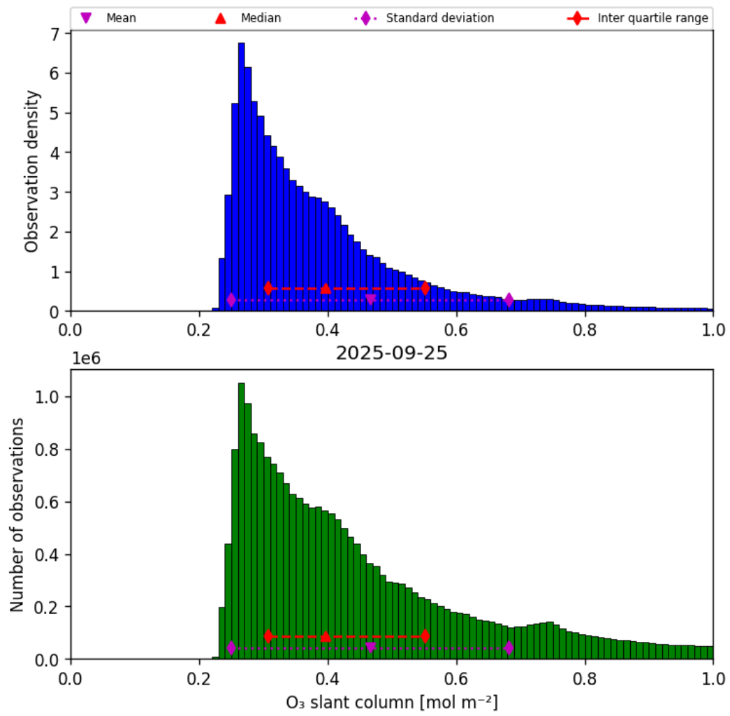
Figure 31: Histogram of “O 3 slant column” for 2025-09-25 to 2025-09-26
