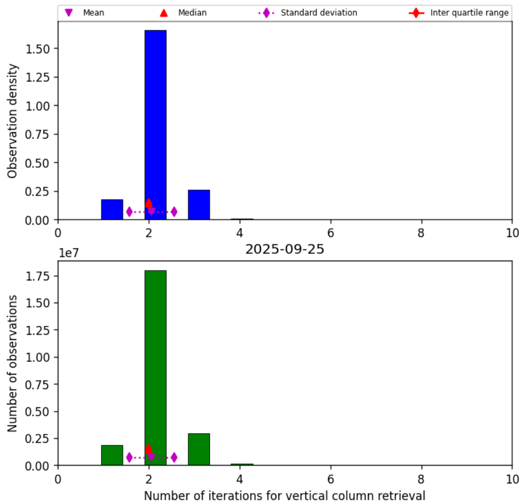
Figure 39: Histogram of “Number of iterations for vertical column retrieval” for 2025-09-25 to 2025-09-26
