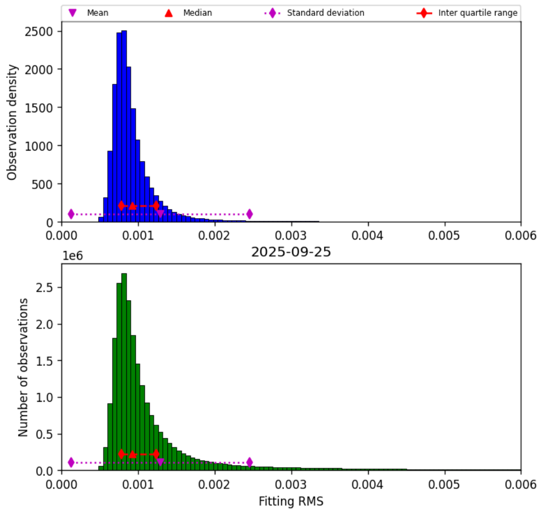
Figure 34: Histogram of “Fitting RMS” for 2025-09-25 to 2025-09-26
