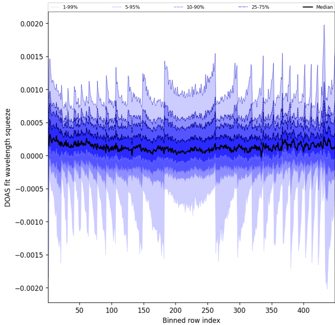
Figure 48: Along track statistics of “DOAS fit wavelength squeeze” for 2025-09-25 to 2025-09-26
