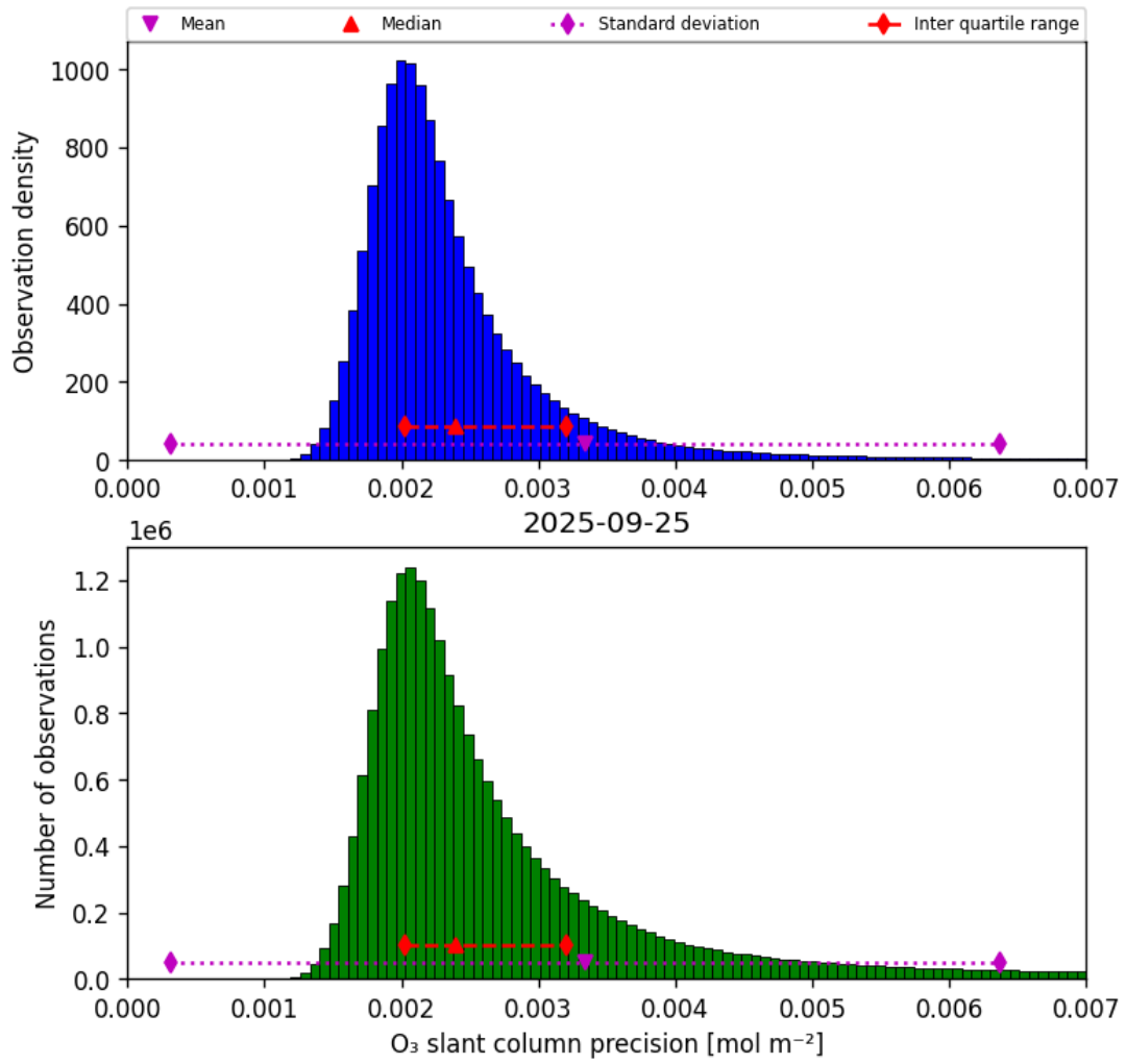
Figure 32: Histogram of “O 3 slant column precision” for 2025-09-25 to 2025-09-26
