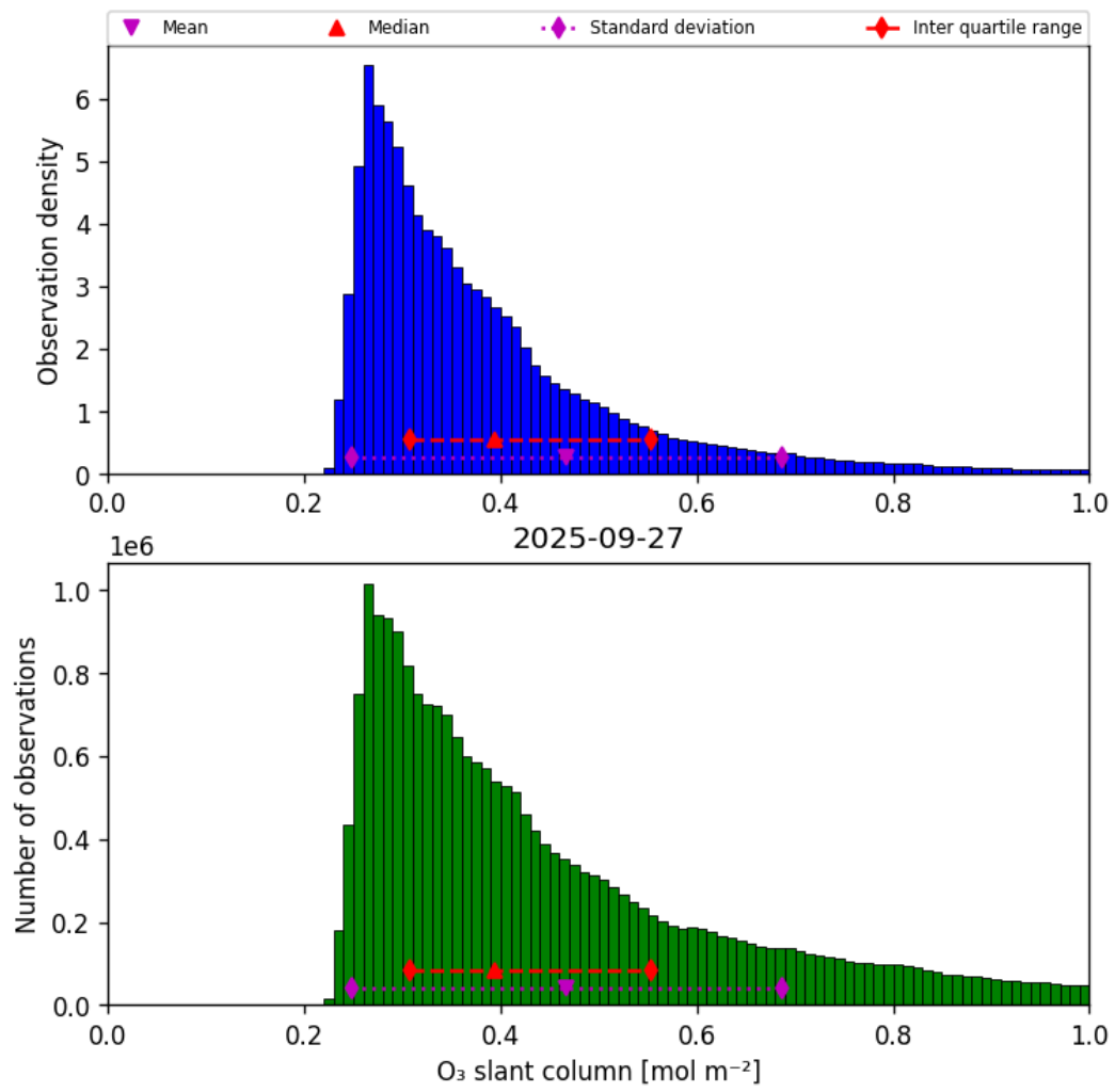
Figure 31: Histogram of “O 3 slant column” for 2025-09-27 to 2025-09-28
