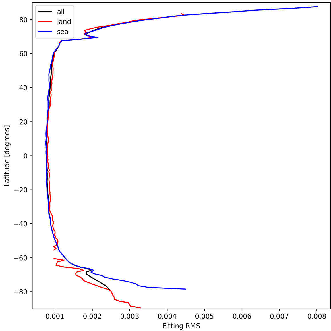
Figure 22: Zonal average of “Fitting RMS” for 2025-09-27 to 2025-09-28.
