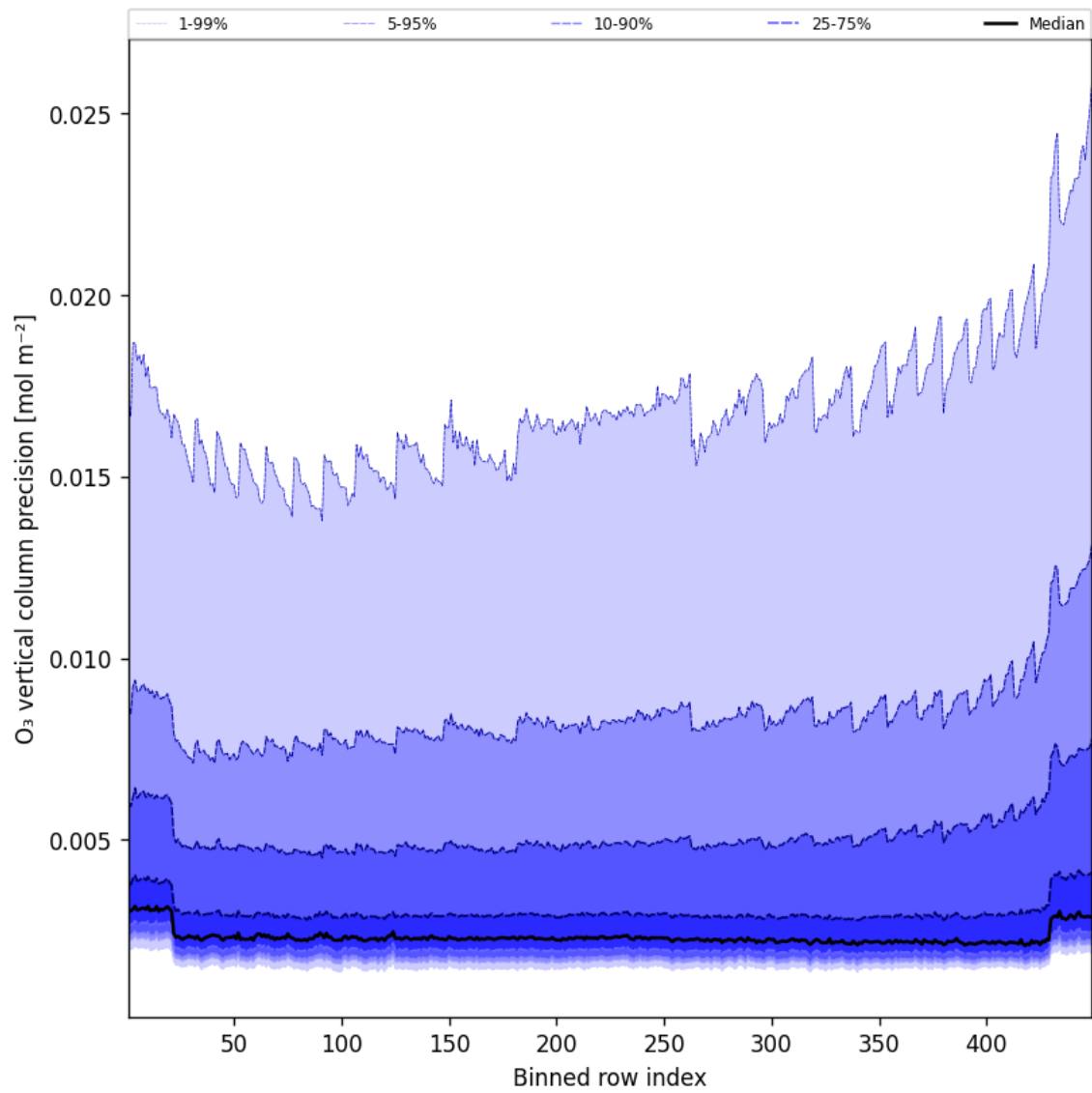
Figure 42: Along track statistics of “O 3 vertical column precision” for 2025-09-27 to 2025-09-28
