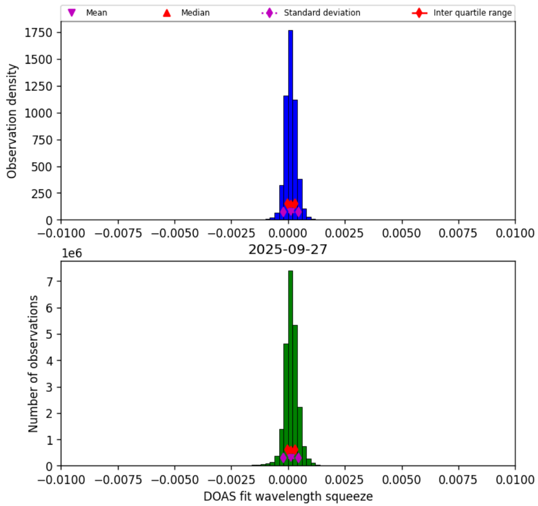
Figure 36: Histogram of “DOAS fit wavelength squeeze” for 2025-09-27 to 2025-09-28
