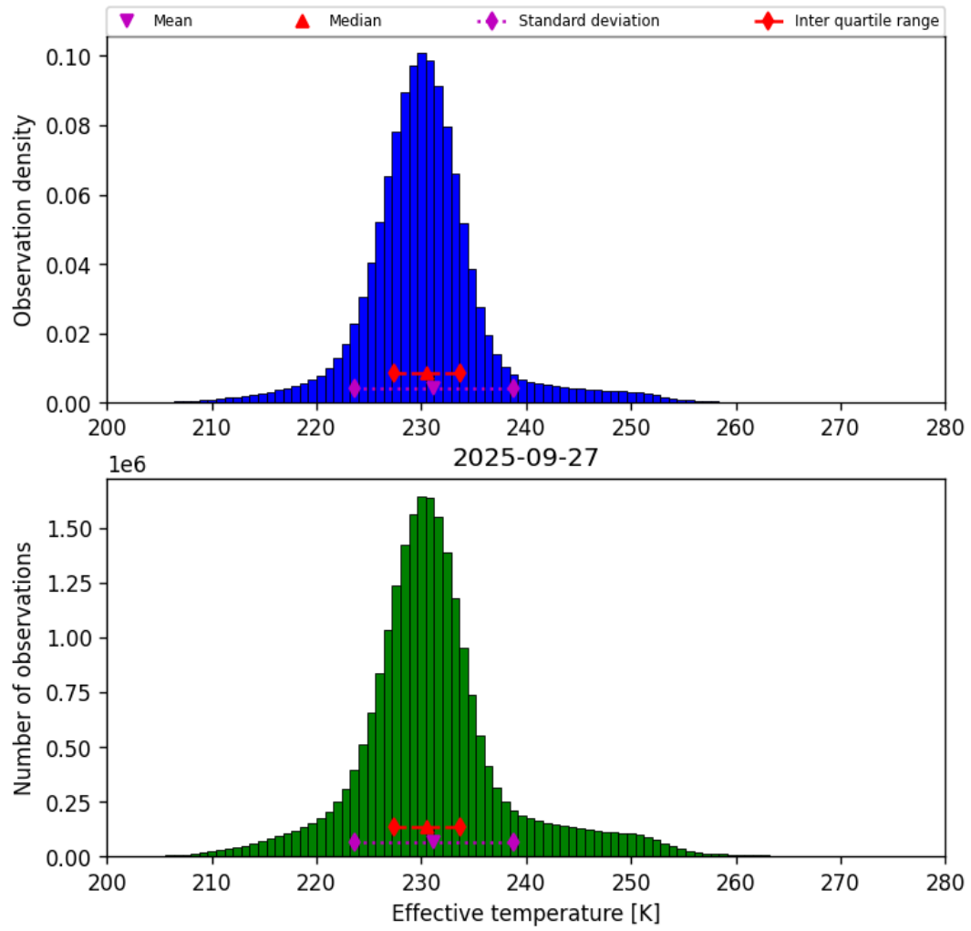
Figure 38: Histogram of “Effective temperature” for 2025-09-27 to 2025-09-28
