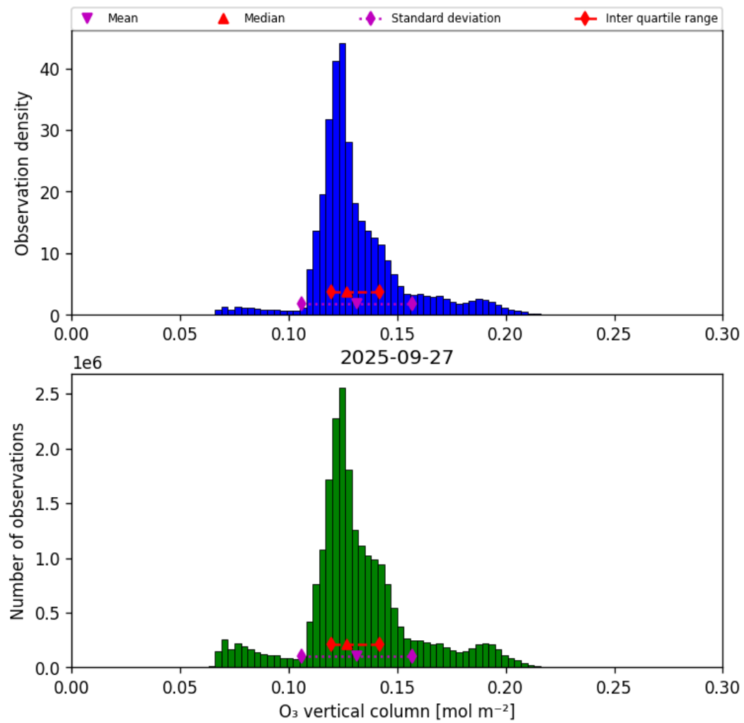
Figure 29: Histogram of “O 3 vertical column” for 2025-09-27 to 2025-09-28
