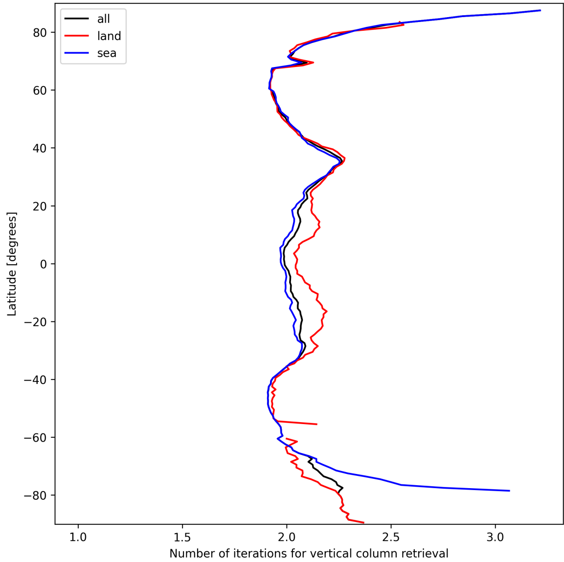
Figure 27: Zonal average of “Number of iterations for vertical column retrieval” for 2025-09-27 to 2025-09-28.
