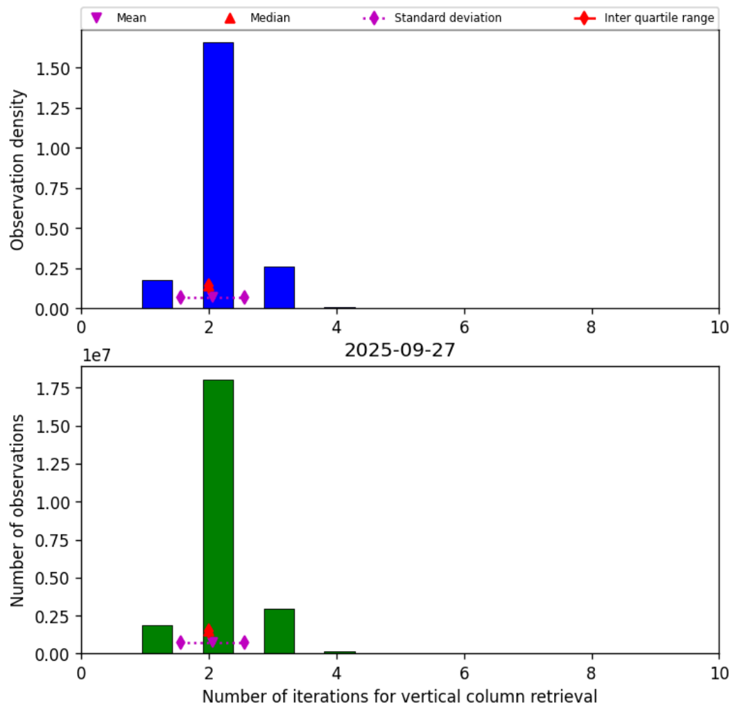
Figure 39: Histogram of “Number of iterations for vertical column retrieval” for 2025-09-27 to 2025-09-28
