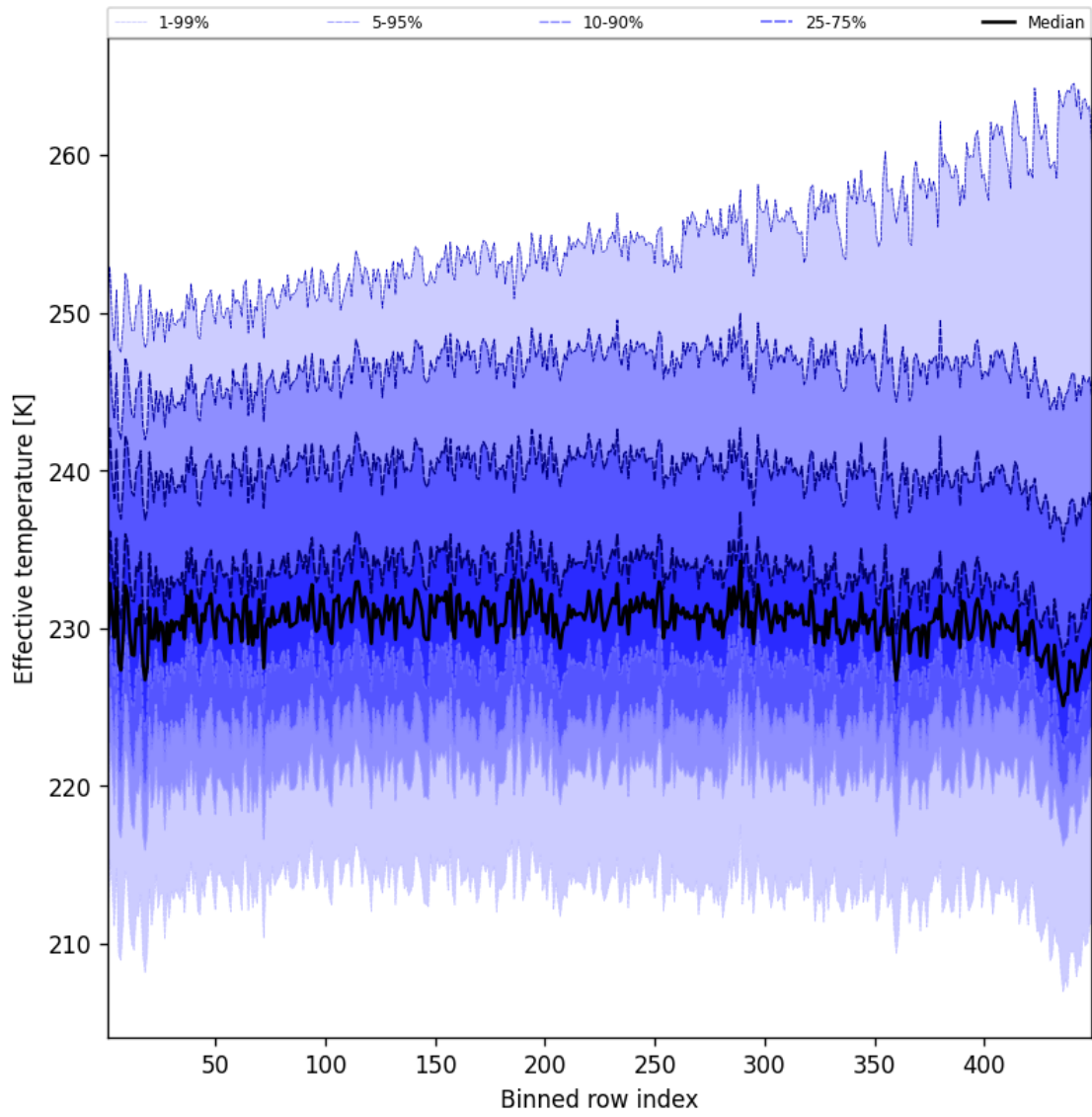
Figure 50: Along track statistics of “Effective temperature” for 2025-09-27 to 2025-09-28
