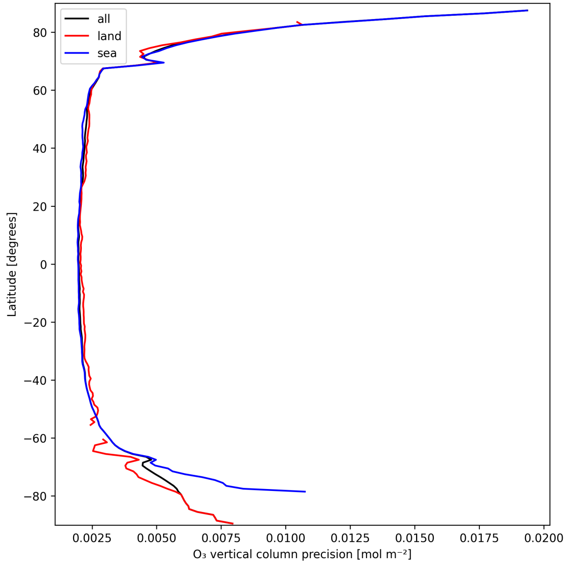
Figure 18: Zonal average of "O 3 vertical column precision" for 2025-09-27 to 2025-09-28.
