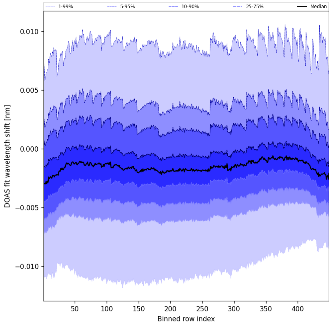
Figure 47: Along track statistics of “DOAS fit wavelength shift” for 2025-09-27 to 2025-09-28
