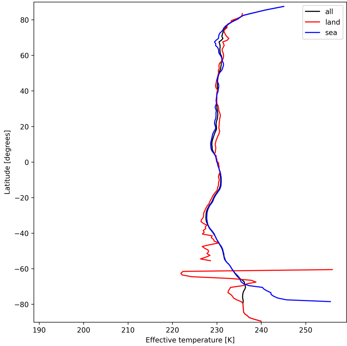
Figure 26: Zonal average of “Effective temperature” for 2025-09-27 to 2025-09-28.
