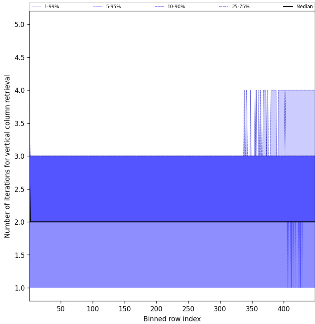
Figure 51: Along track statistics of “Number of iterations for vertical column retrieval” for 2025-09-27 to 2025-09-28
