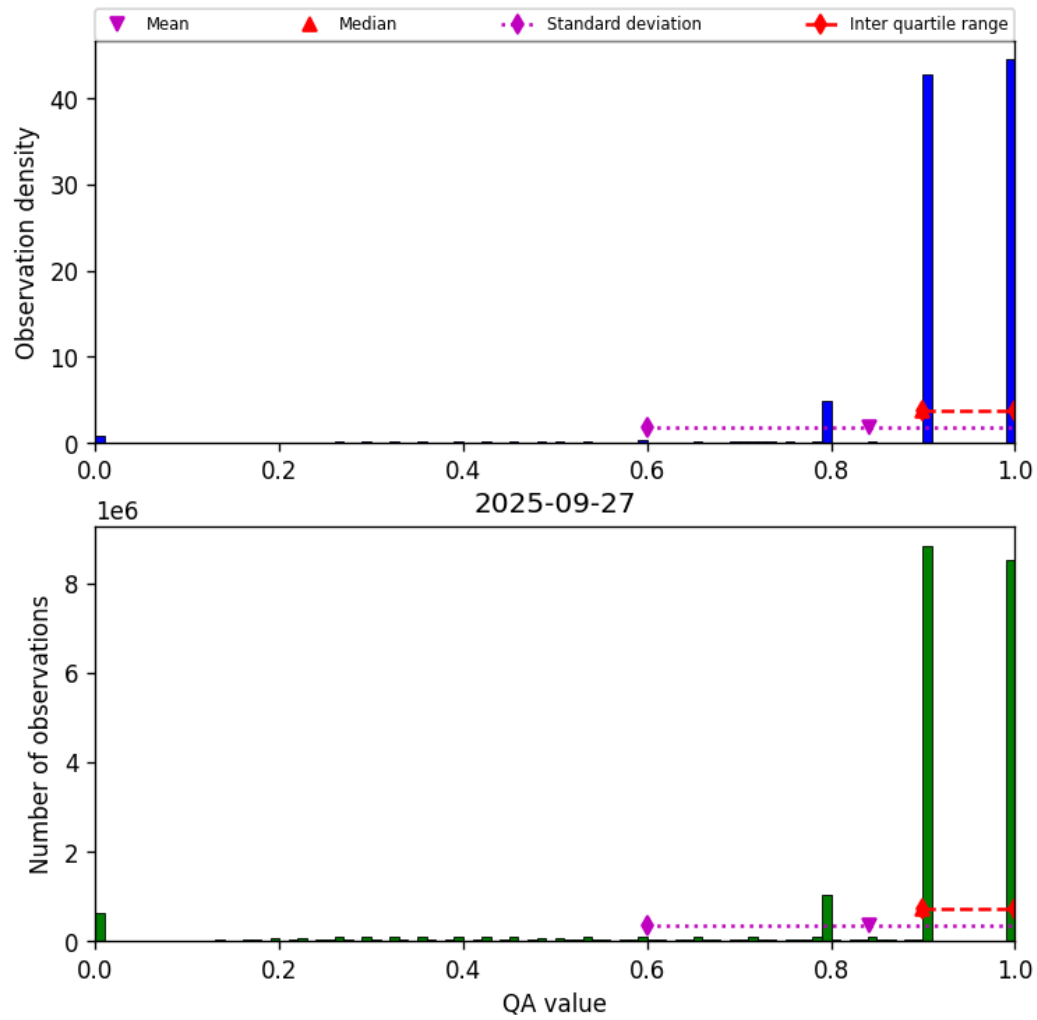
Figure 28: Histogram of “QA value” for 2025-09-27 to 2025-09-28
