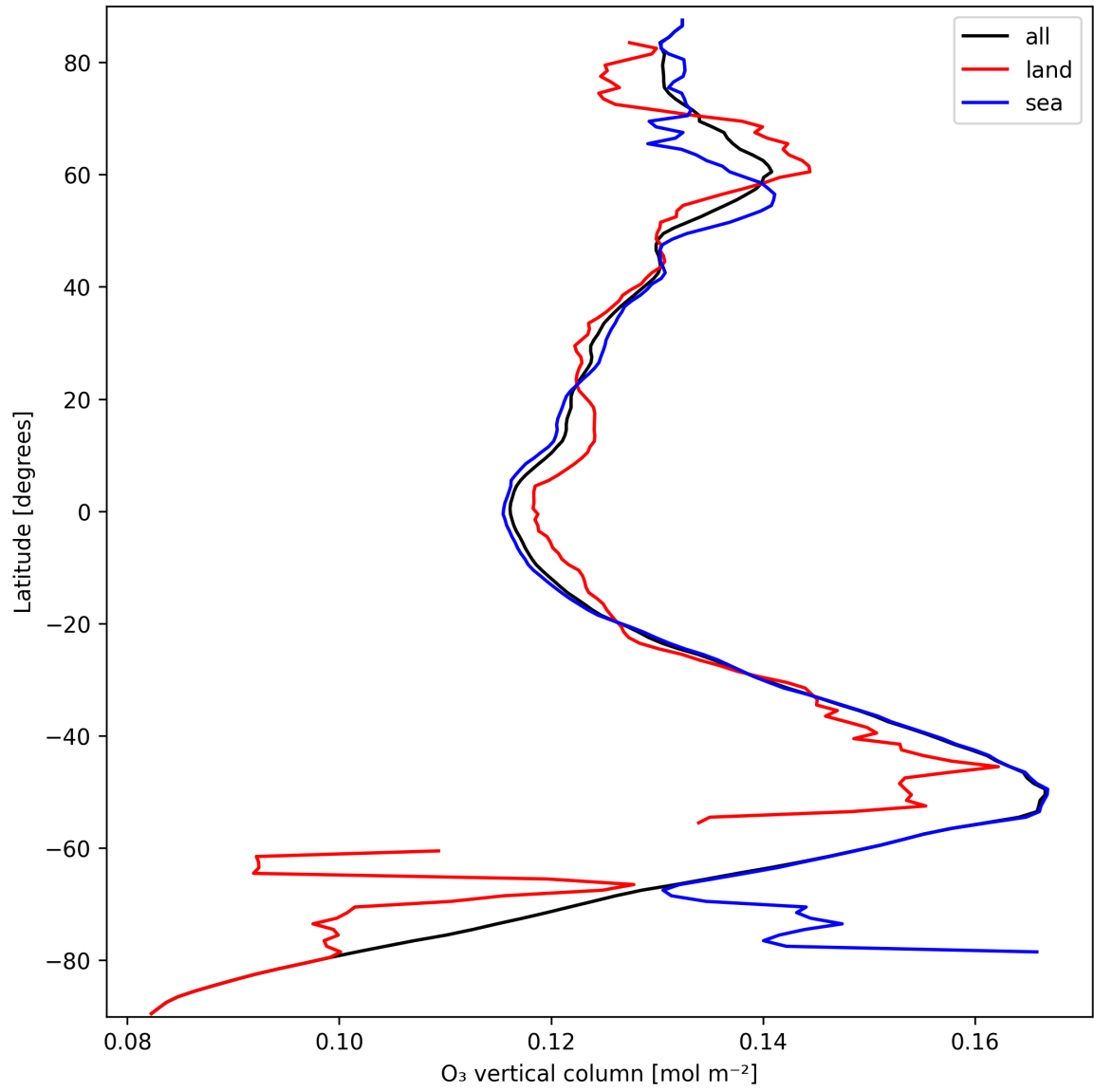
Figure 17: Zonal average of “O 3 vertical column” for 2025-09-27 to 2025-09-28.
