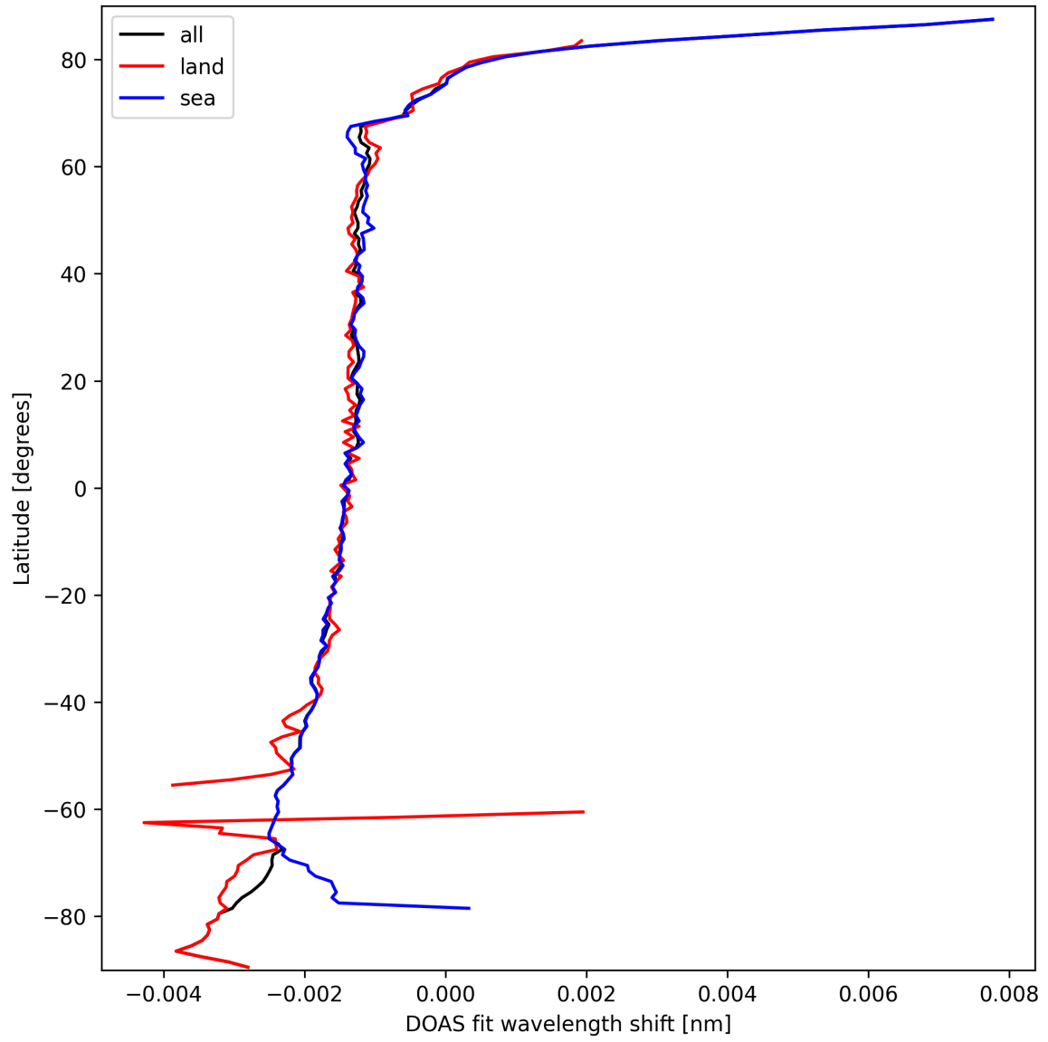
Figure 23: Zonal average of “DOAS fit wavelength shift” for 2025-09-27 to 2025-09-28.
