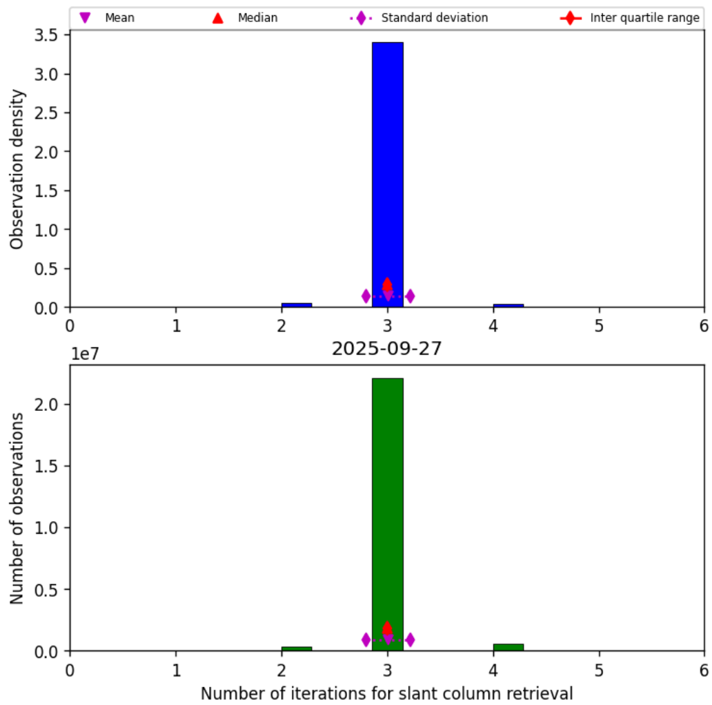
Figure 33: Histogram of “Number of iterations for slant column retrieval” for 2025-09-27 to 2025-09-28
