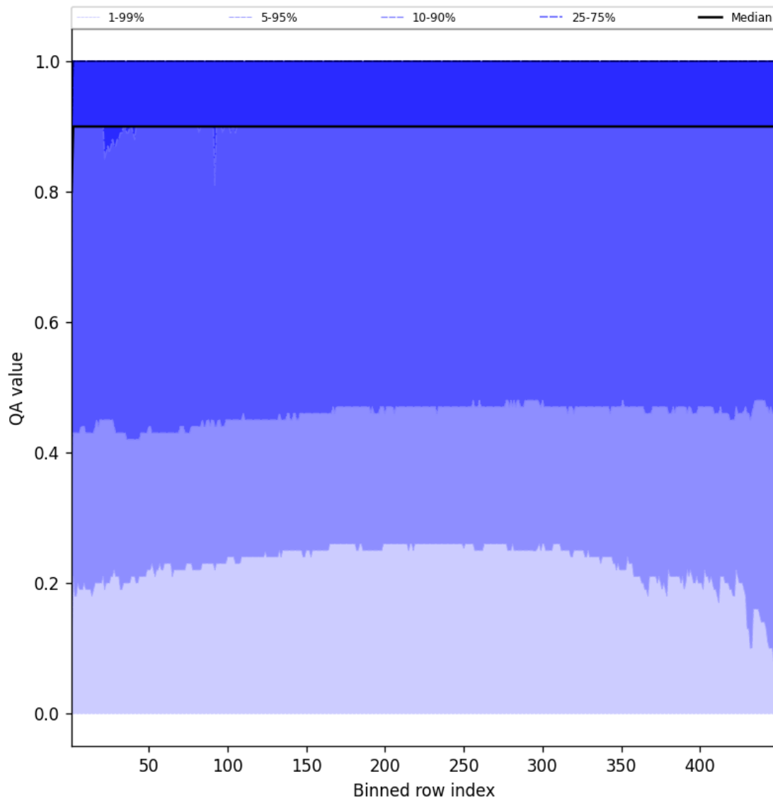
Figure 40: Along track statistics of “QA value” for 2025-09-27 to 2025-09-28
