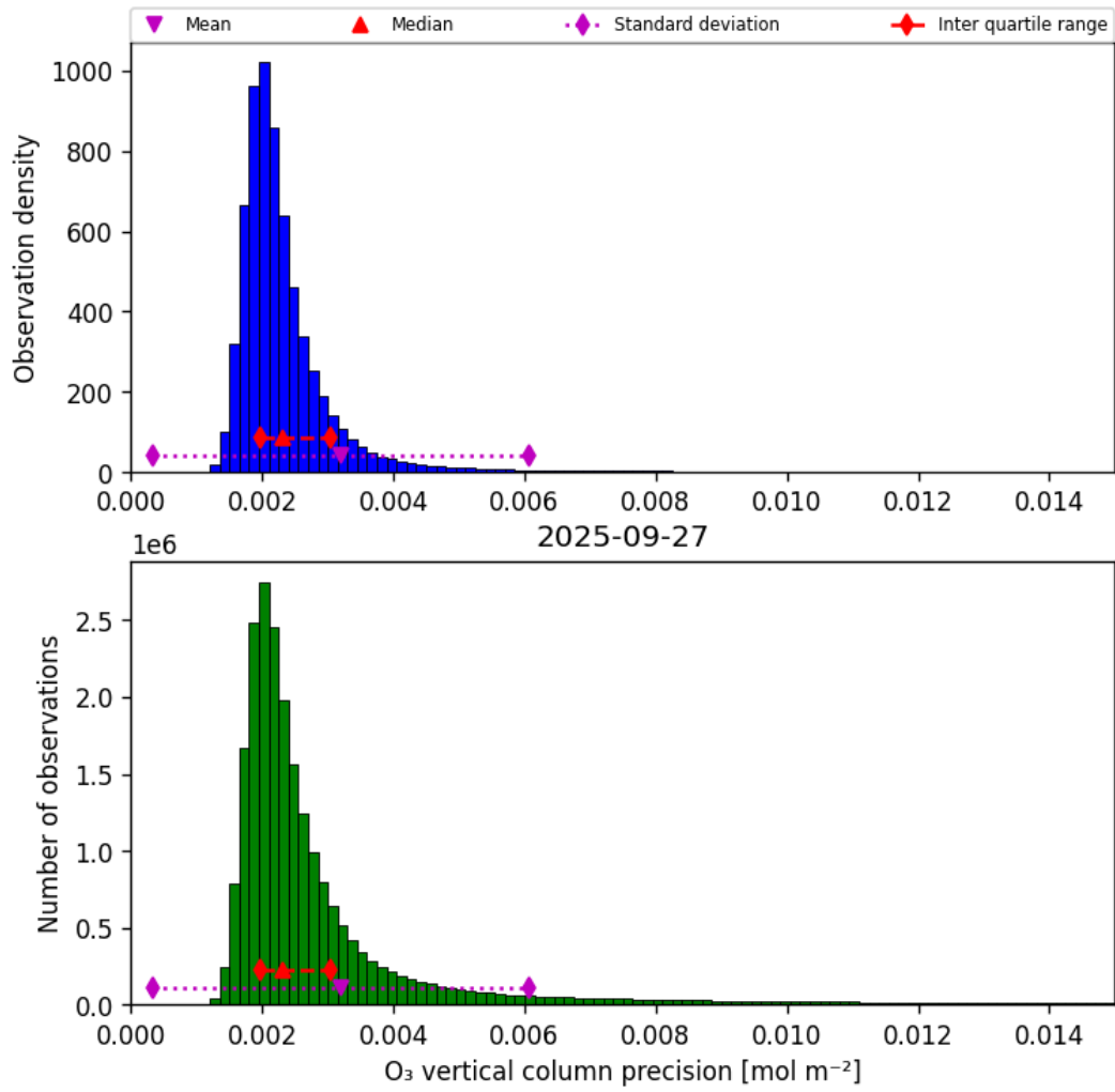
Figure 30: Histogram of “O 3 vertical column precision” for 2025-09-27 to 2025-09-28
