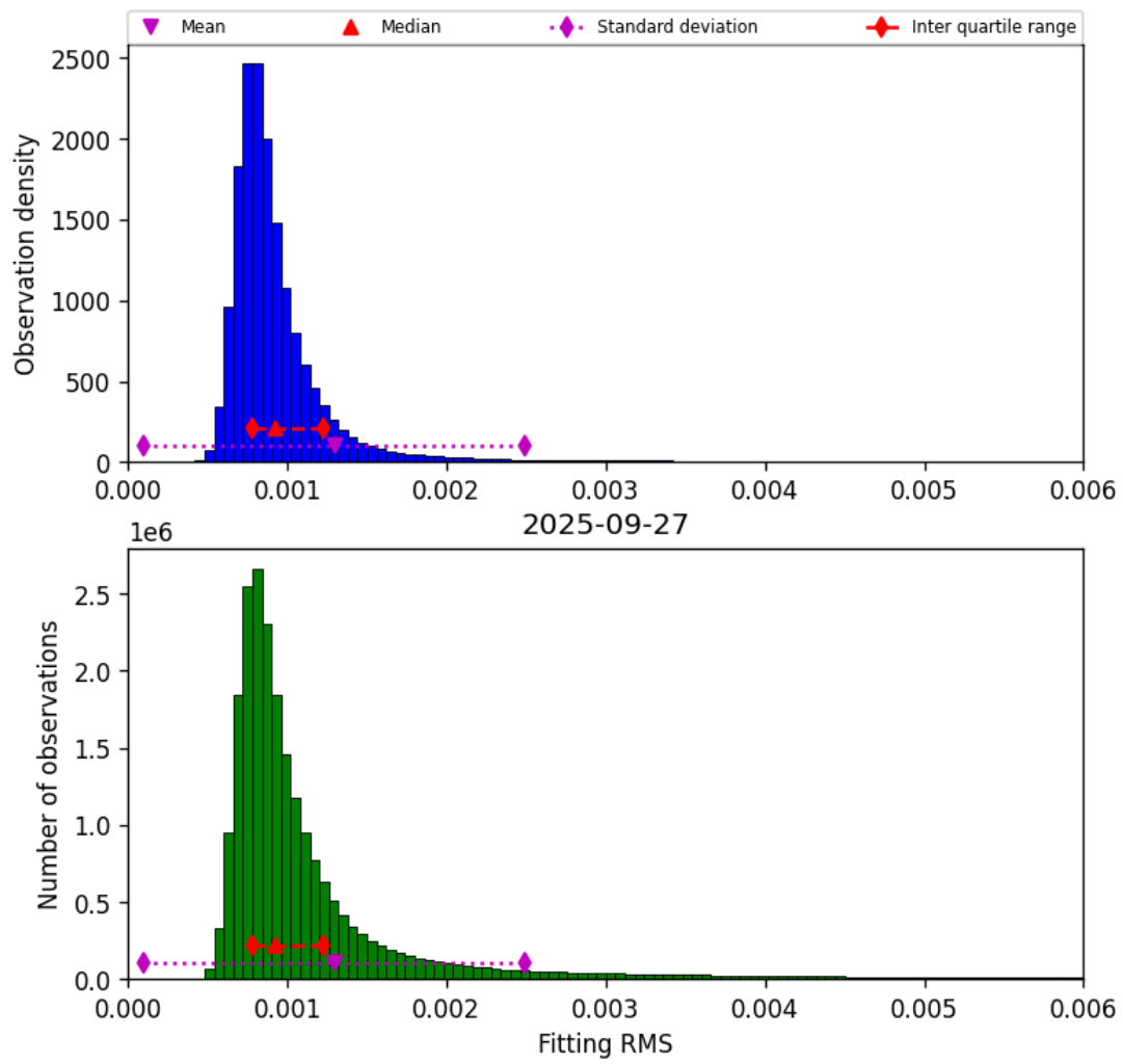
Figure 34: Histogram of “Fitting RMS” for 2025-09-27 to 2025-09-28
