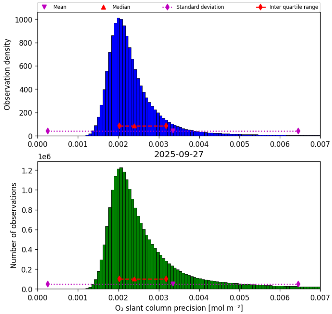
Figure 32: Histogram of “O 3 slant column precision” for 2025-09-27 to 2025-09-28
