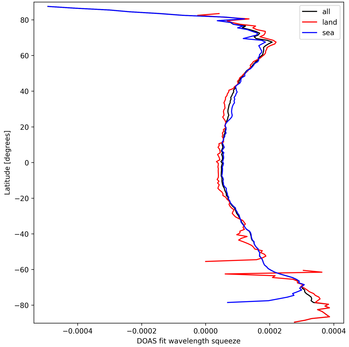
Figure 24: Zonal average of “DOAS fit wavelength squeeze” for 2025-09-27 to 2025-09-28.
