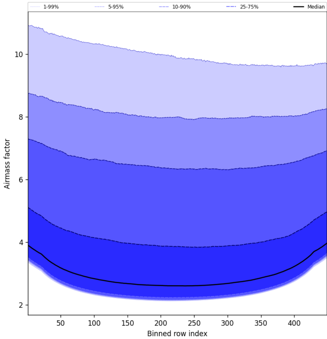
Figure 49: Along track statistics of “Airmass factor” for 2025-09-27 to 2025-09-28
