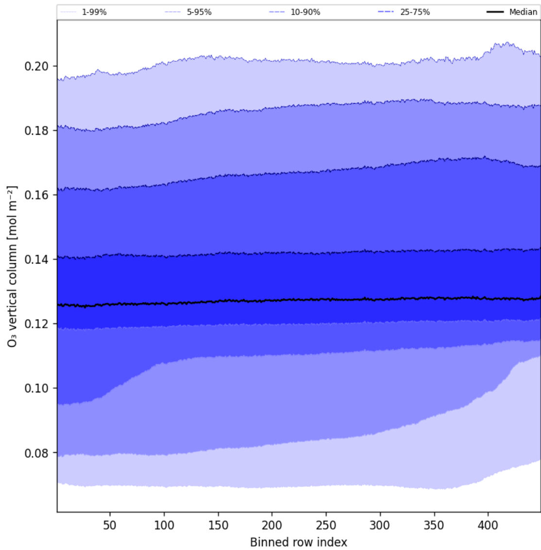
Figure 41: Along track statistics of “O 3 vertical column” for 2025-09-27 to 2025-09-28
