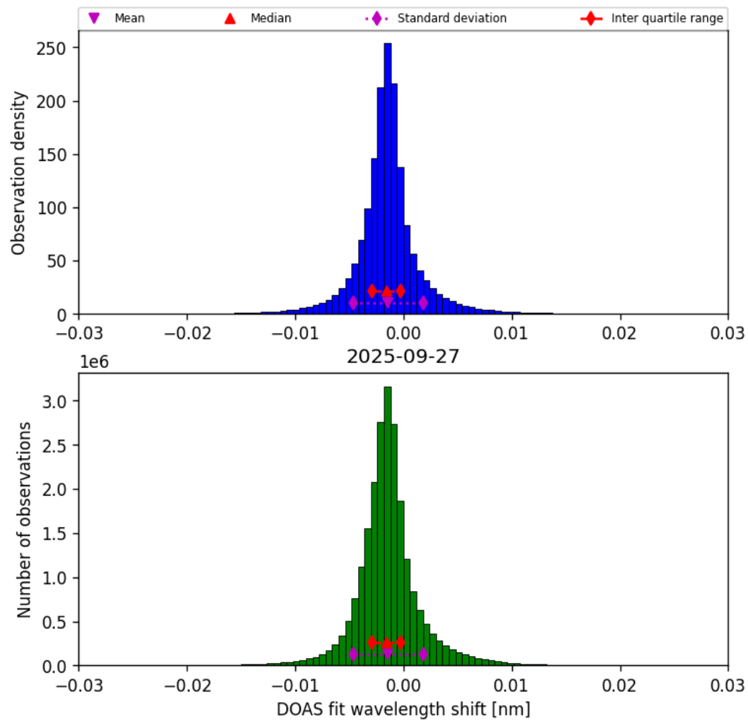
Figure 35: Histogram of “DOAS fit wavelength shift” for 2025-09-27 to 2025-09-28
