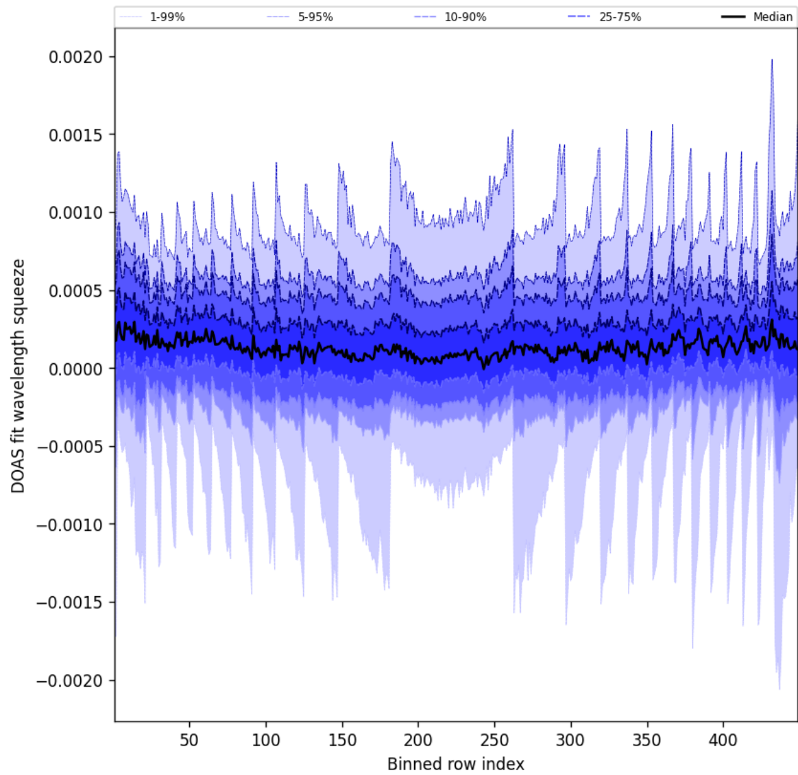
Figure 48: Along track statistics of “DOAS fit wavelength squeeze” for 2025-09-27 to 2025-09-28
