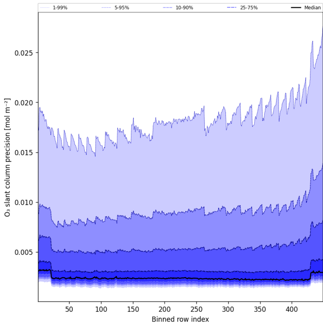
Figure 44: Along track statistics of “O 3 slant column precision” for 2025-09-27 to 2025-09-28
