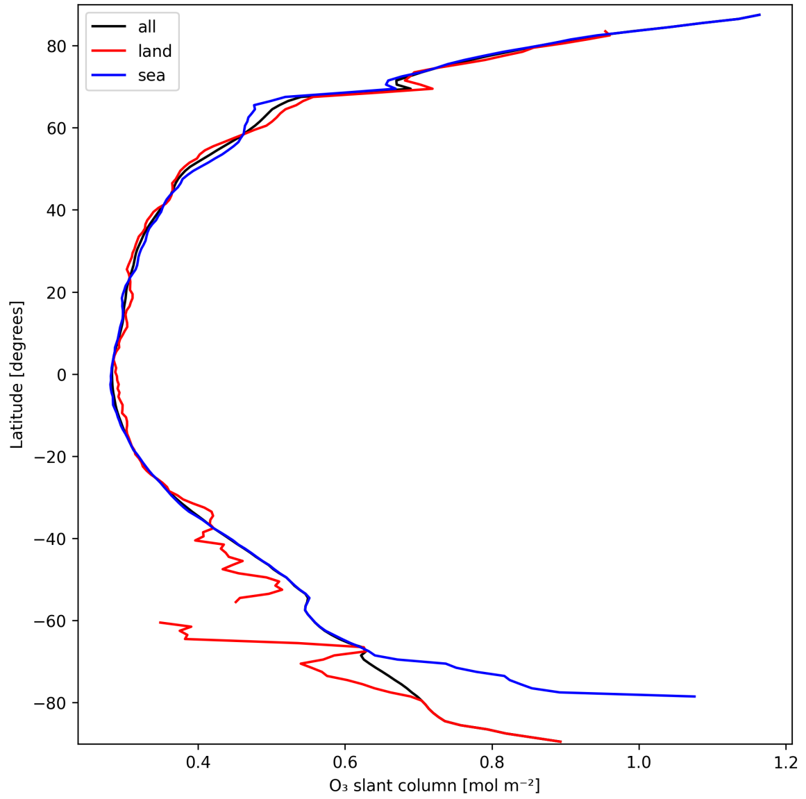
Figure 19: Zonal average of “O 3 slant column” for 2025-09-27 to 2025-09-28.
