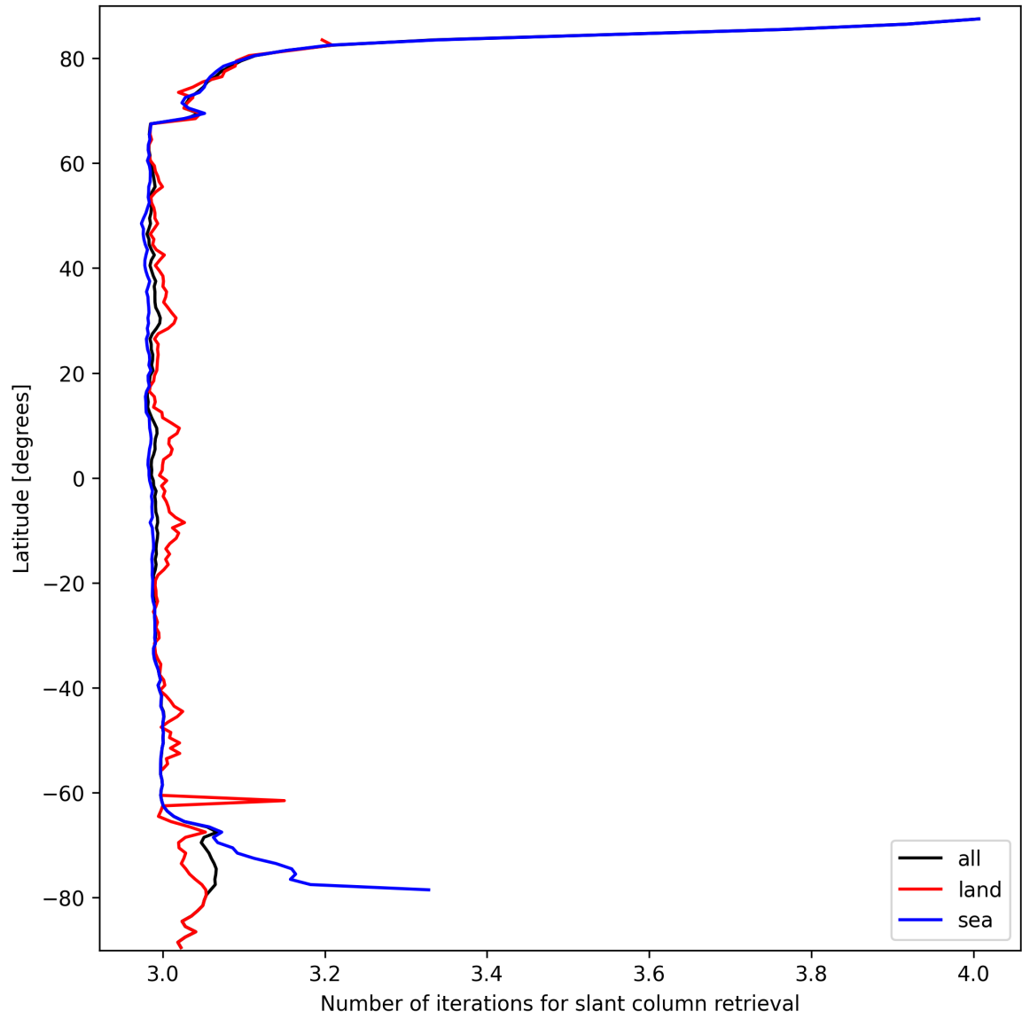
Figure 21: Zonal average of “Number of iterations for slant column retrieval” for 2025-09-27 to 2025-09-28.
