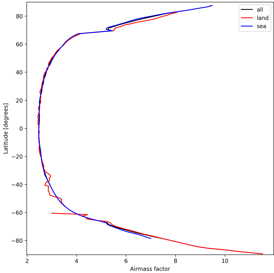
Figure 25: Zonal average of “Airmass factor” for 2025-09-27 to 2025-09-28.
