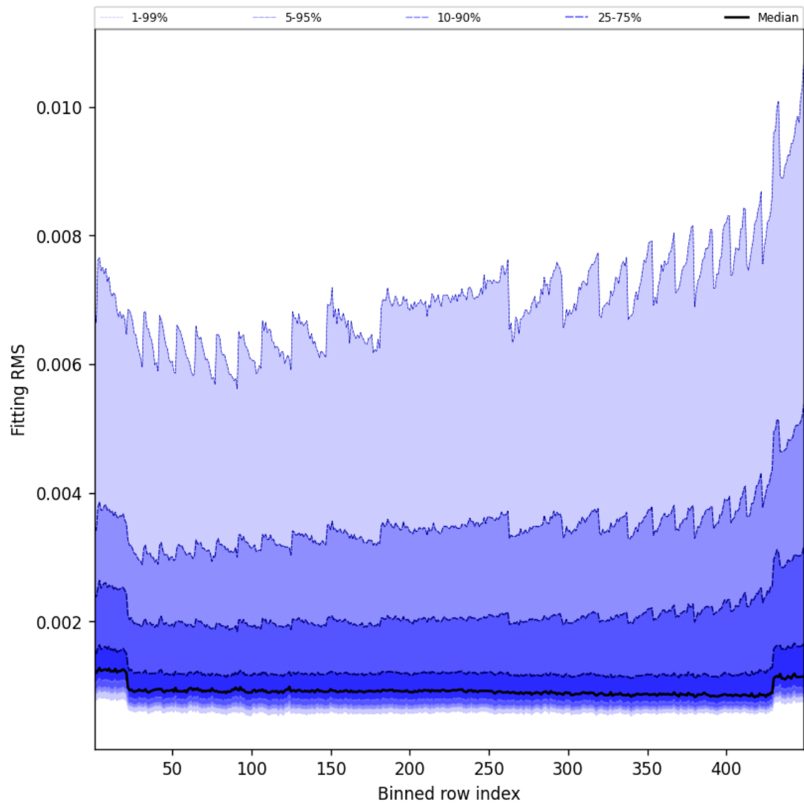
Figure 46: Along track statistics of “Fitting RMS” for 2025-09-27 to 2025-09-28
