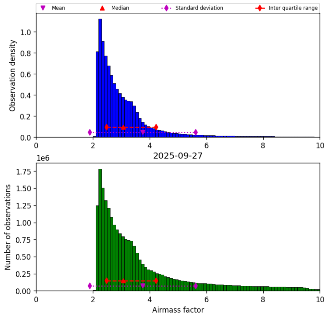
Figure 37: Histogram of “Airmass factor” for 2025-09-27 to 2025-09-28
