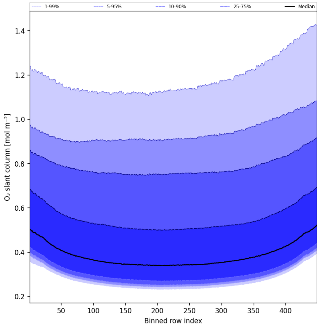
Figure 43: Along track statistics of “O 3 slant column” for 2025-09-27 to 2025-09-28
