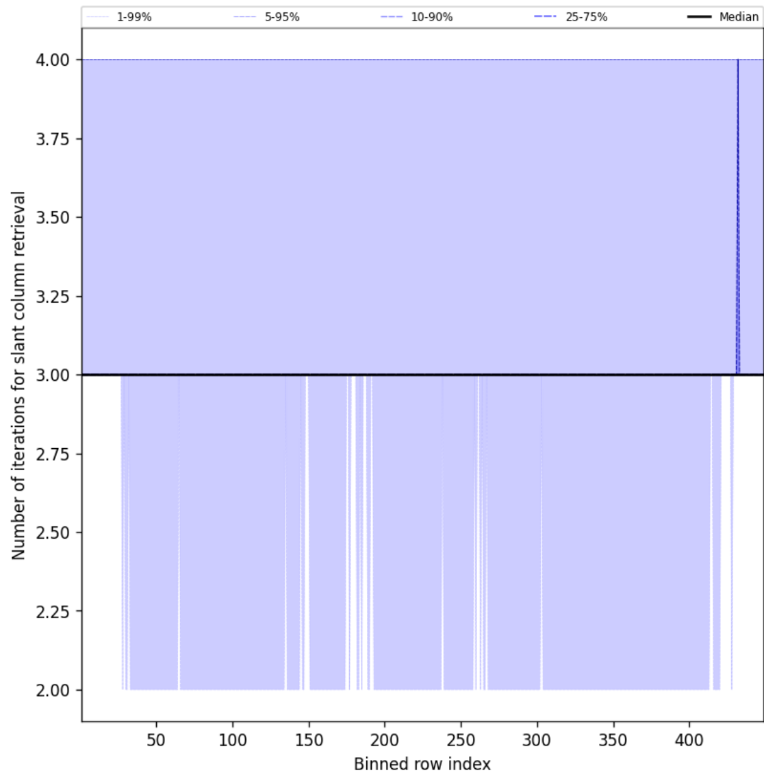
Figure 45: Along track statistics of “Number of iterations for slant column retrieval” for 2025-09-27 to 2025-09-28
