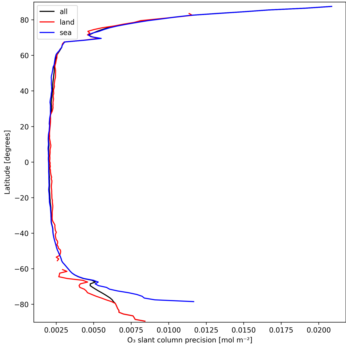
Figure 20: Zonal average of "O 3 slant column precision" for 2025-09-27 to 2025-09-28.
