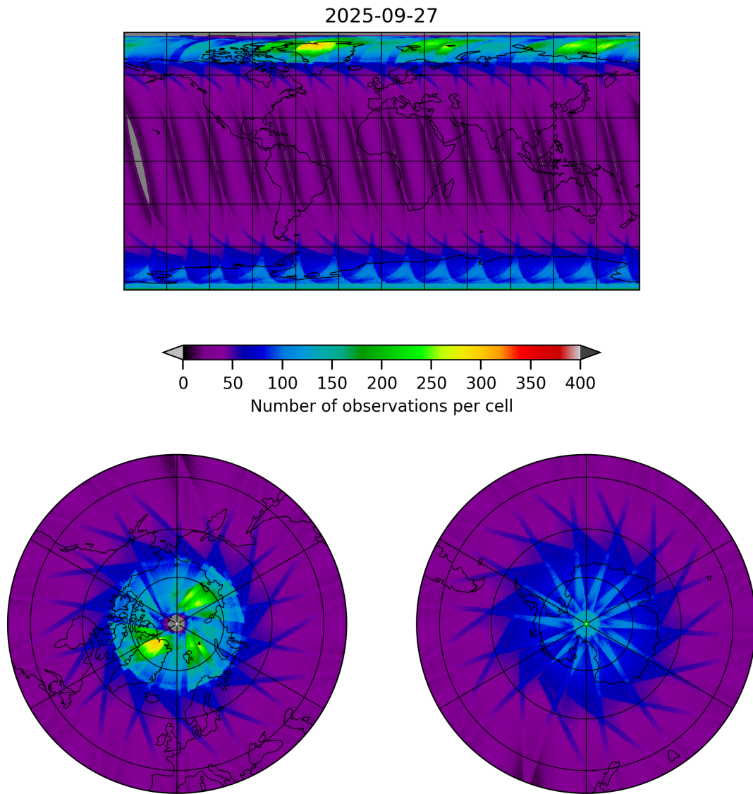
Figure 15: Map of the number of observations for 2025-09-27 to 2025-09-28
