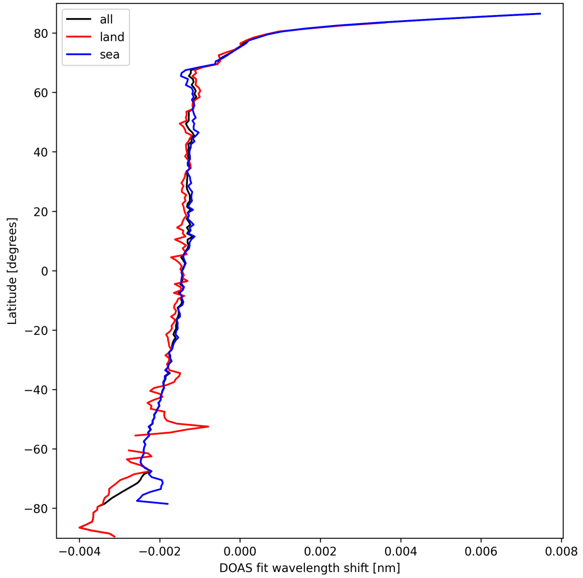
Figure 23: Zonal average of “DOAS fit wavelength shift” for 2025-09-28 to 2025-09-29.
