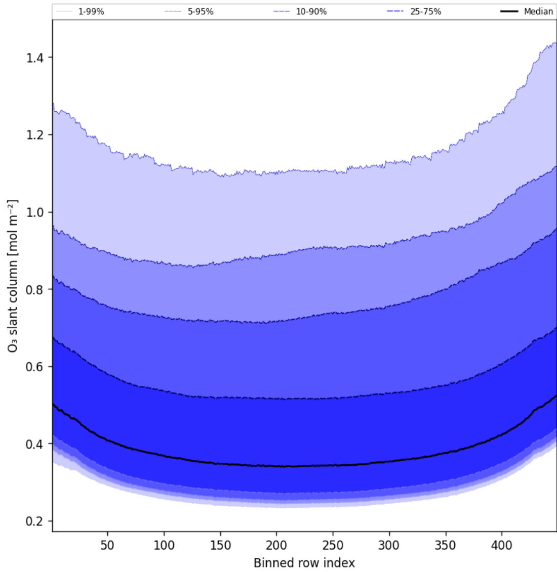
Figure 43: Along track statistics of “O 3 slant column” for 2025-09-28 to 2025-09-29
