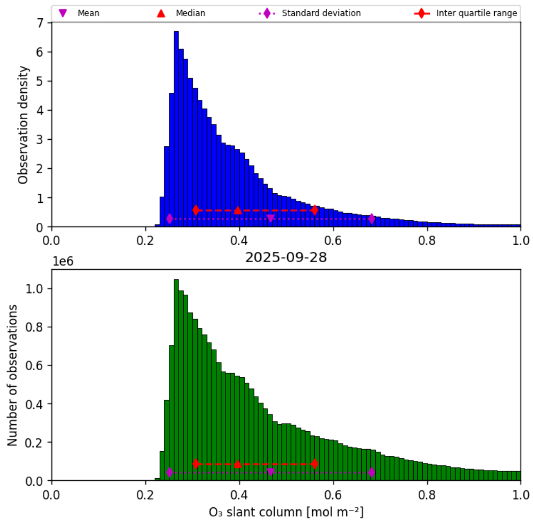
Figure 31: Histogram of “O 3 slant column” for 2025-09-28 to 2025-09-29
