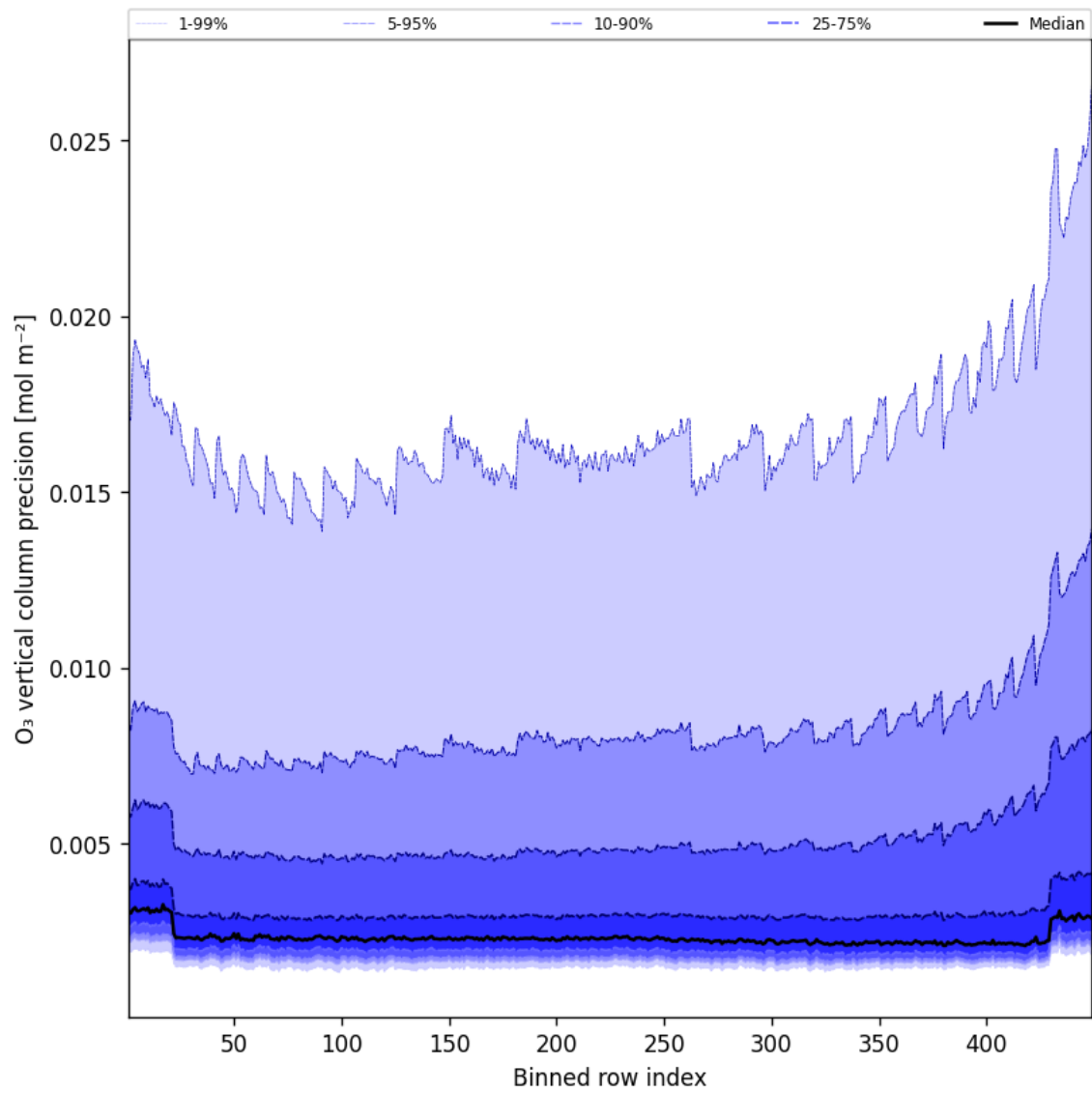
Figure 42: Along track statistics of “O 3 vertical column precision” for 2025-09-28 to 2025-09-29
