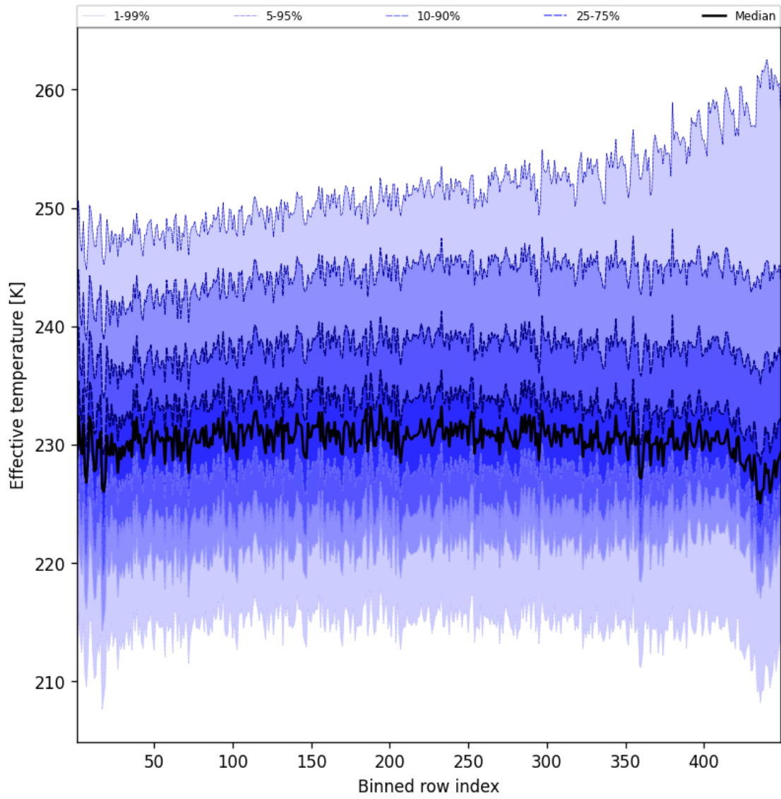
Figure 50: Along track statistics of “Effective temperature” for 2025-09-28 to 2025-09-29
