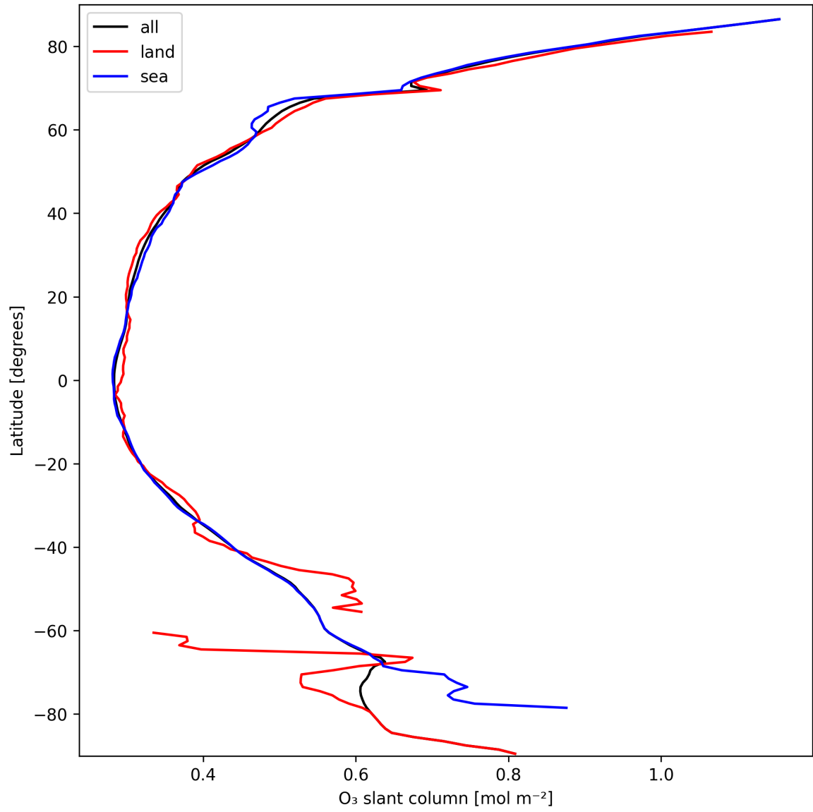
Figure 19: Zonal average of “O 3 slant column” for 2025-09-28 to 2025-09-29.
