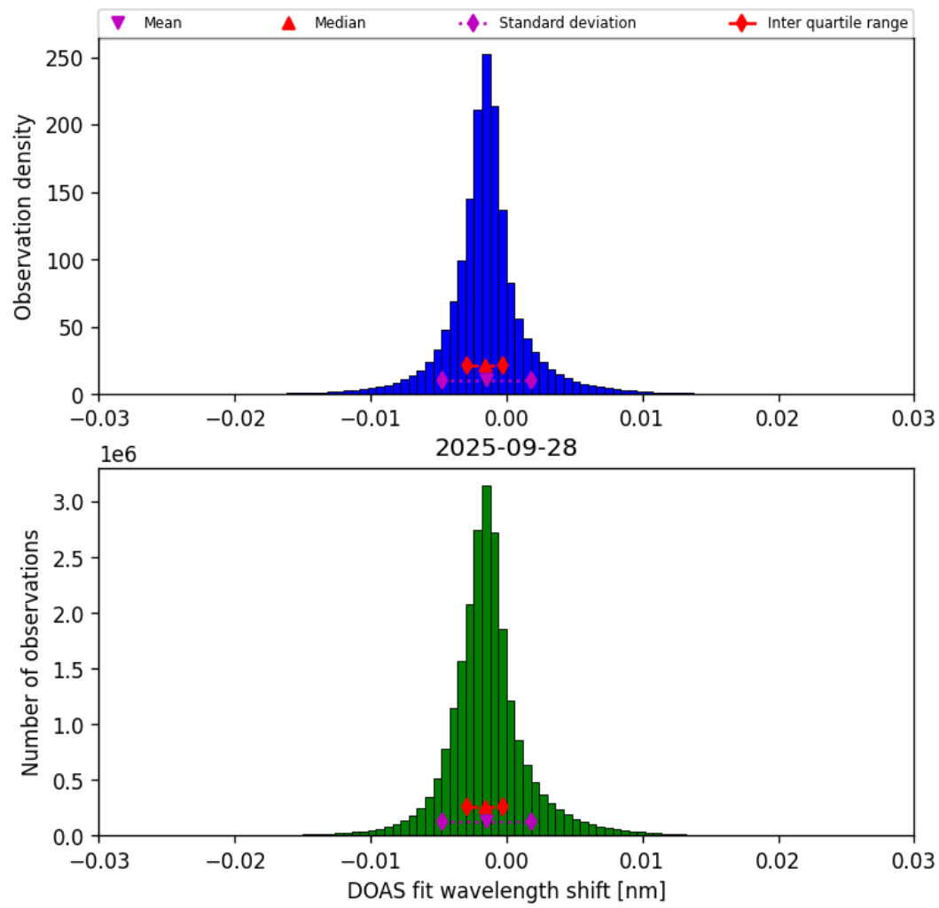
Figure 35: Histogram of “DOAS fit wavelength shift” for 2025-09-28 to 2025-09-29
