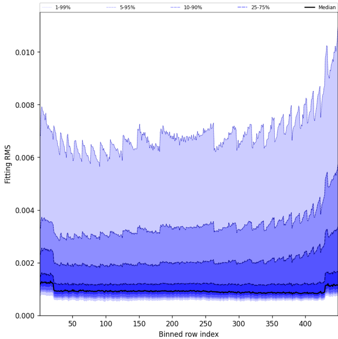
Figure 46: Along track statistics of “Fitting RMS” for 2025-09-28 to 2025-09-29
