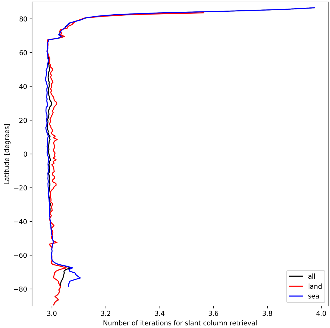
Figure 21: Zonal average of “Number of iterations for slant column retrieval” for 2025-09-28 to 2025-09-29.
