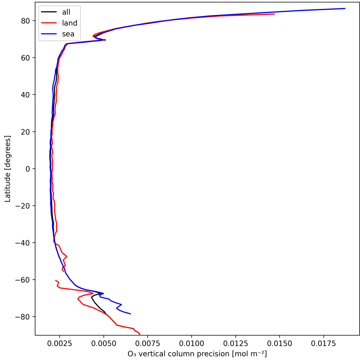
Figure 18: Zonal average of “O 3 vertical column precision” for 2025-09-28 to 2025-09-29.
