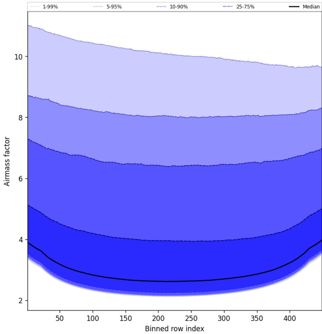
Figure 49: Along track statistics of “Airmass factor” for 2025-09-28 to 2025-09-29
