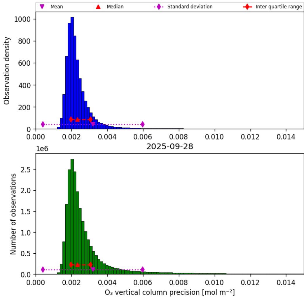
Figure 30: Histogram of “O 3 vertical column precision” for 2025-09-28 to 2025-09-29
