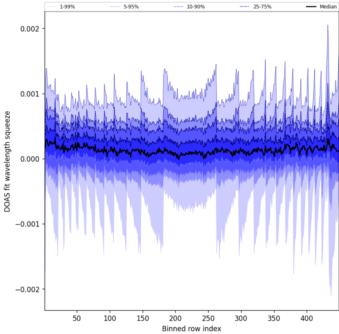
Figure 48: Along track statistics of “DOAS fit wavelength squeeze” for 2025-09-28 to 2025-09-29
