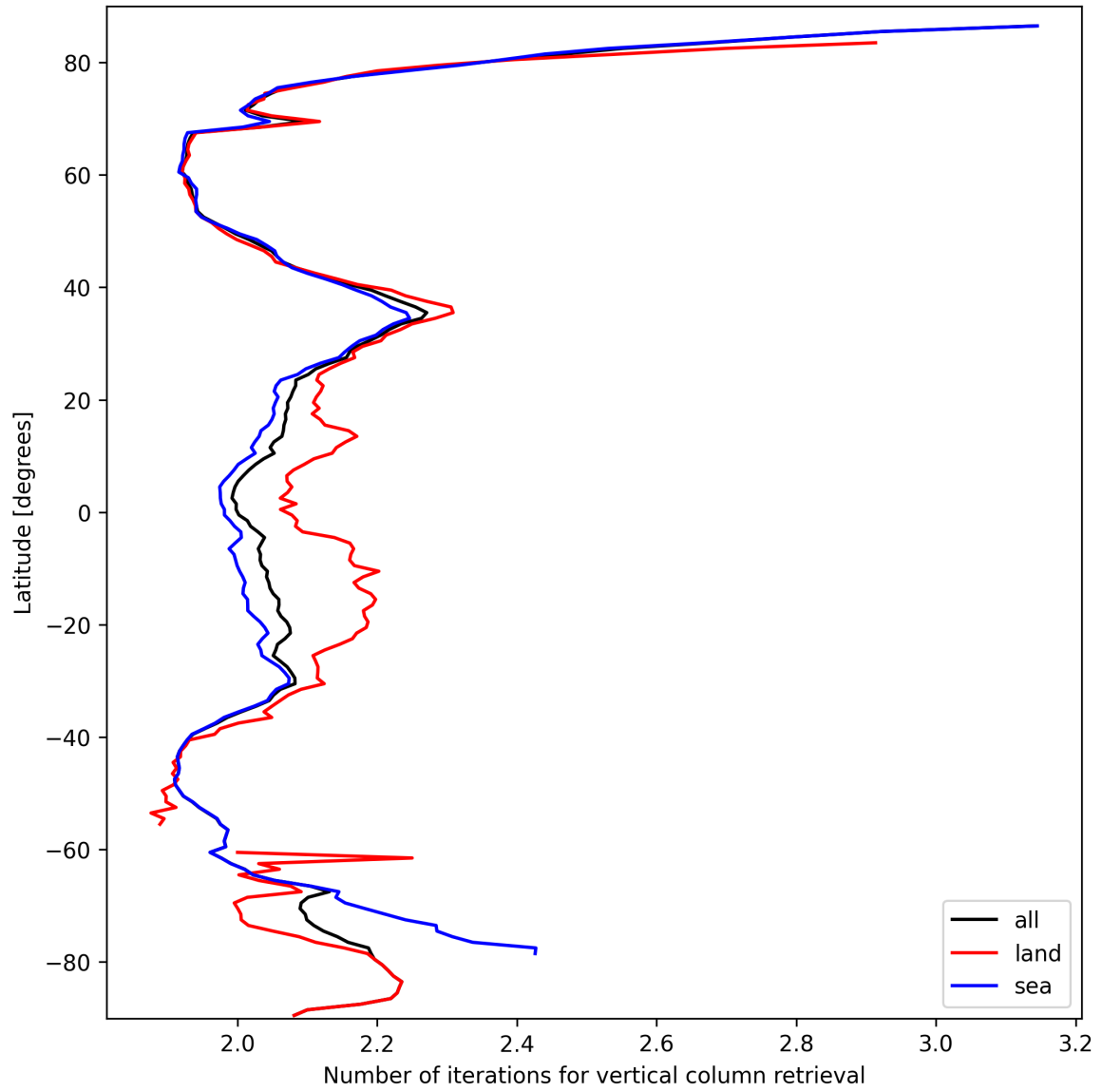
Figure 27: Zonal average of “Number of iterations for vertical column retrieval” for 2025-09-28 to 2025-09-29.
