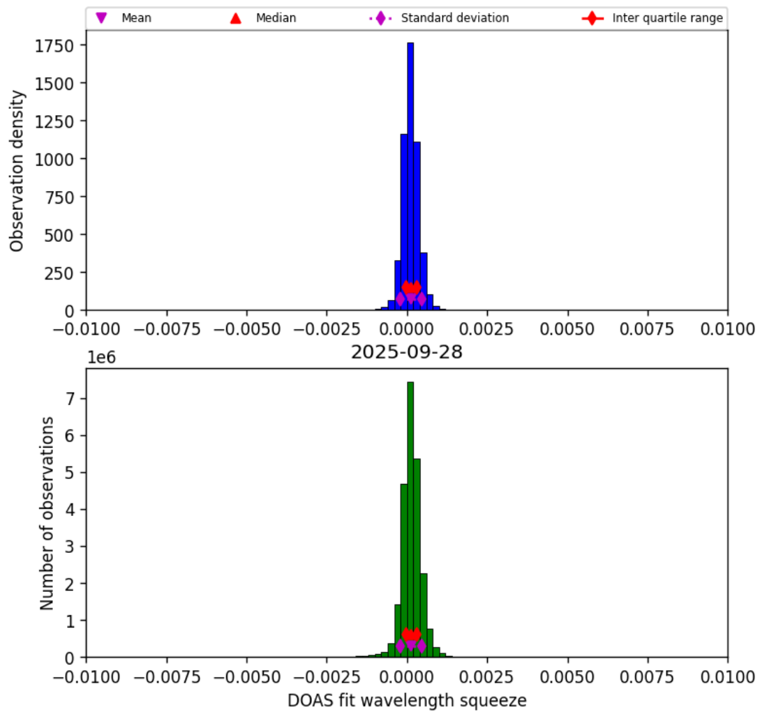
Figure 36: Histogram of “DOAS fit wavelength squeeze” for 2025-09-28 to 2025-09-29
