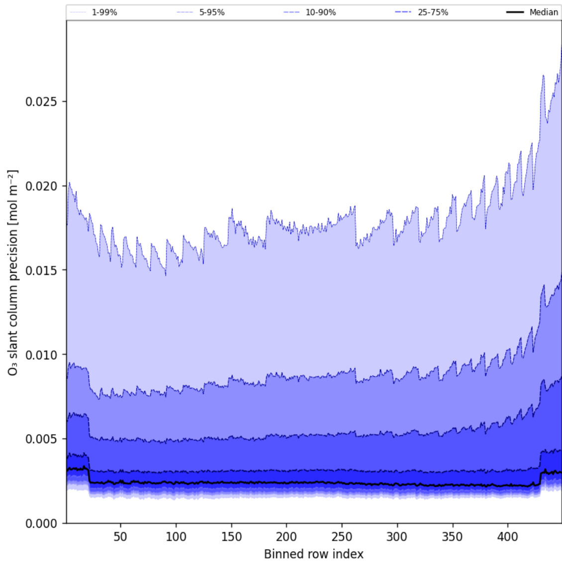
Figure 44: Along track statistics of “O 3 slant column precision” for 2025-09-28 to 2025-09-29
