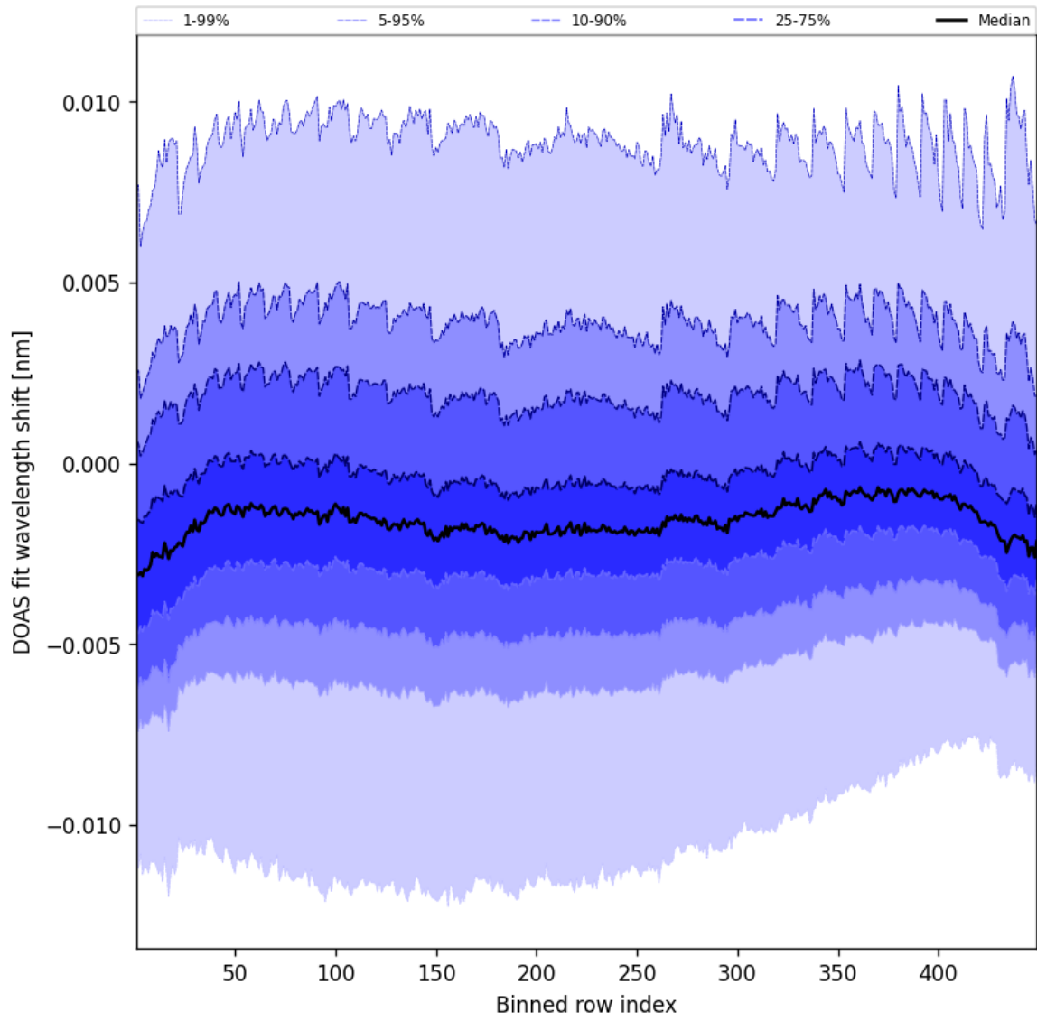
Figure 47: Along track statistics of “DOAS fit wavelength shift” for 2025-09-28 to 2025-09-29
