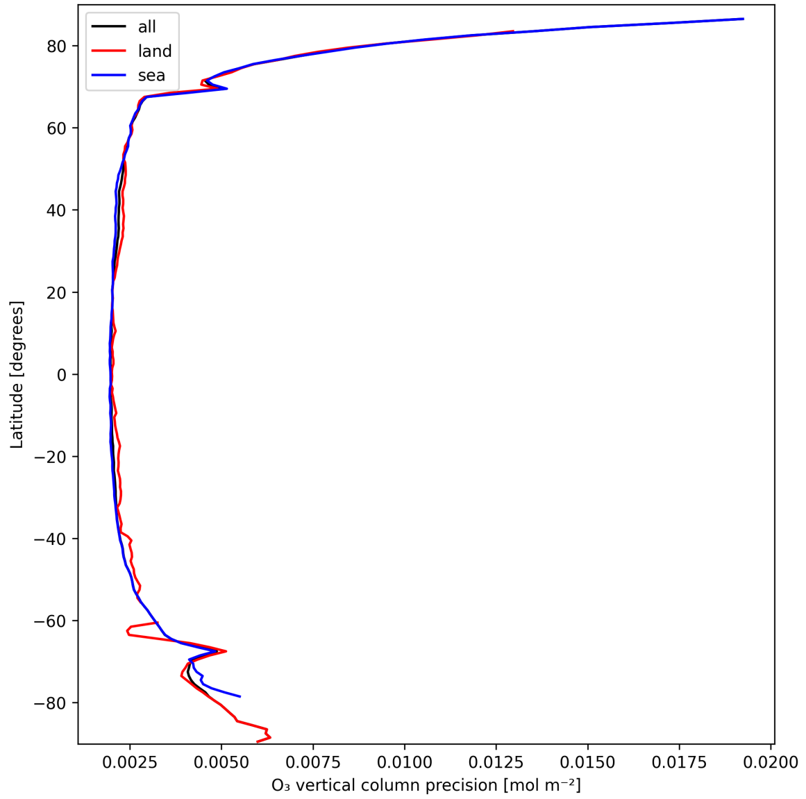
Figure 18: Zonal average of “O 3 vertical column precision” for 2025-09-29 to 2025-09-29.
