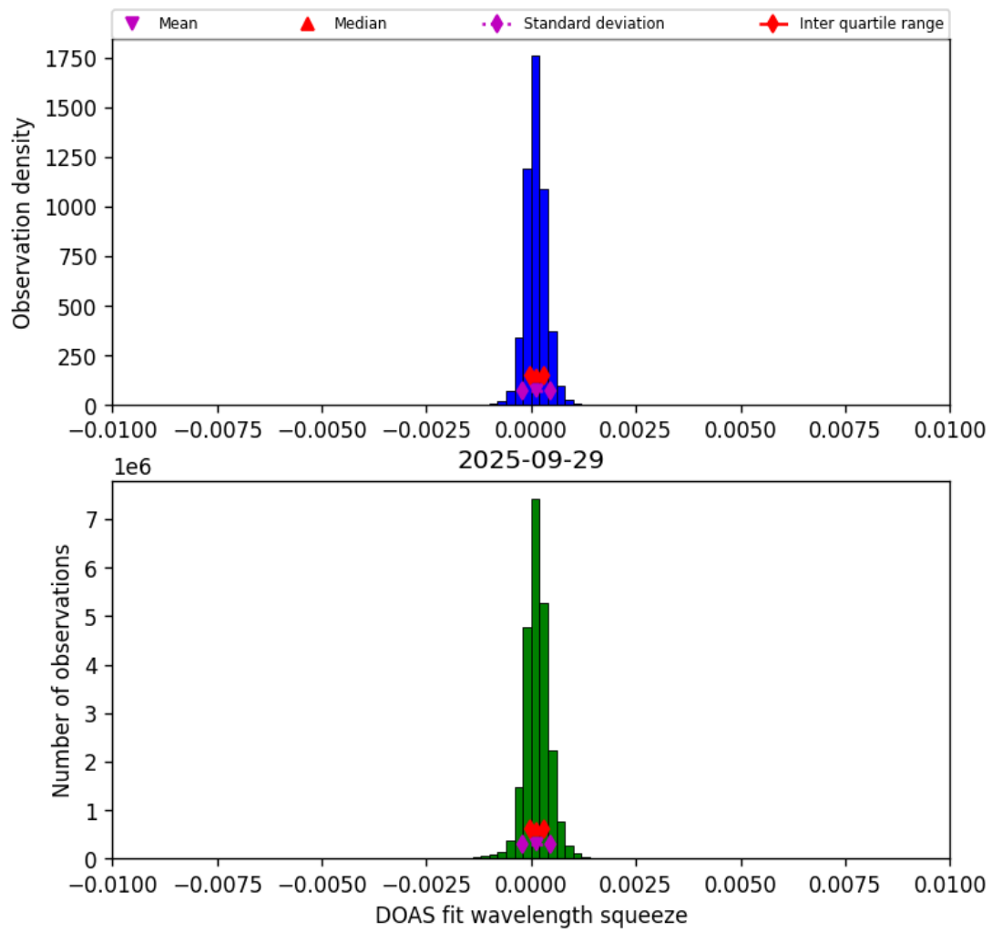
Figure 36: Histogram of “DOAS fit wavelength squeeze” for 2025-09-29 to 2025-09-29
