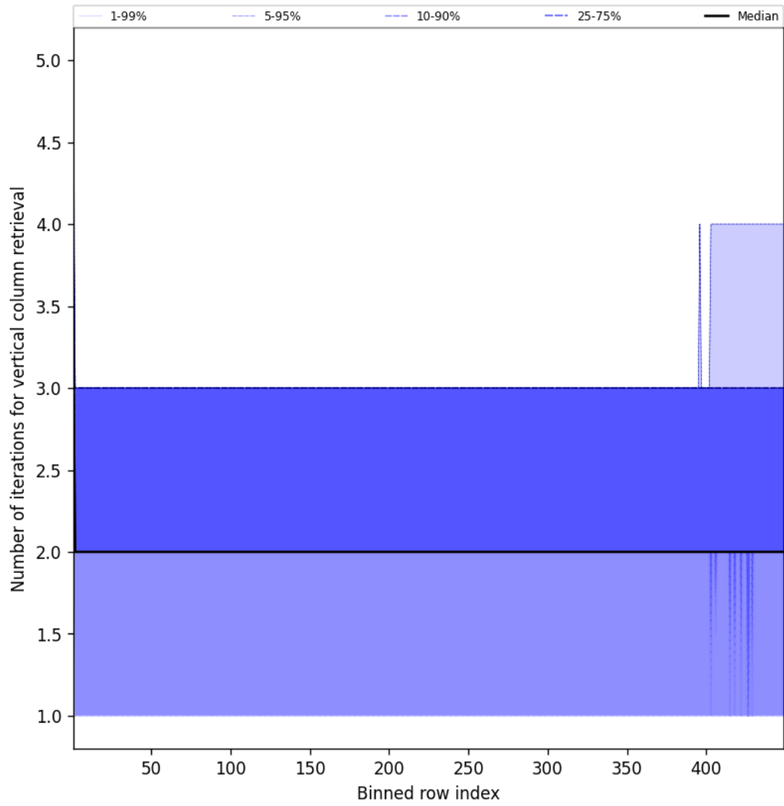
Figure 51: Along track statistics of “Number of iterations for vertical column retrieval” for 2025-09-29 to 2025-09-29
