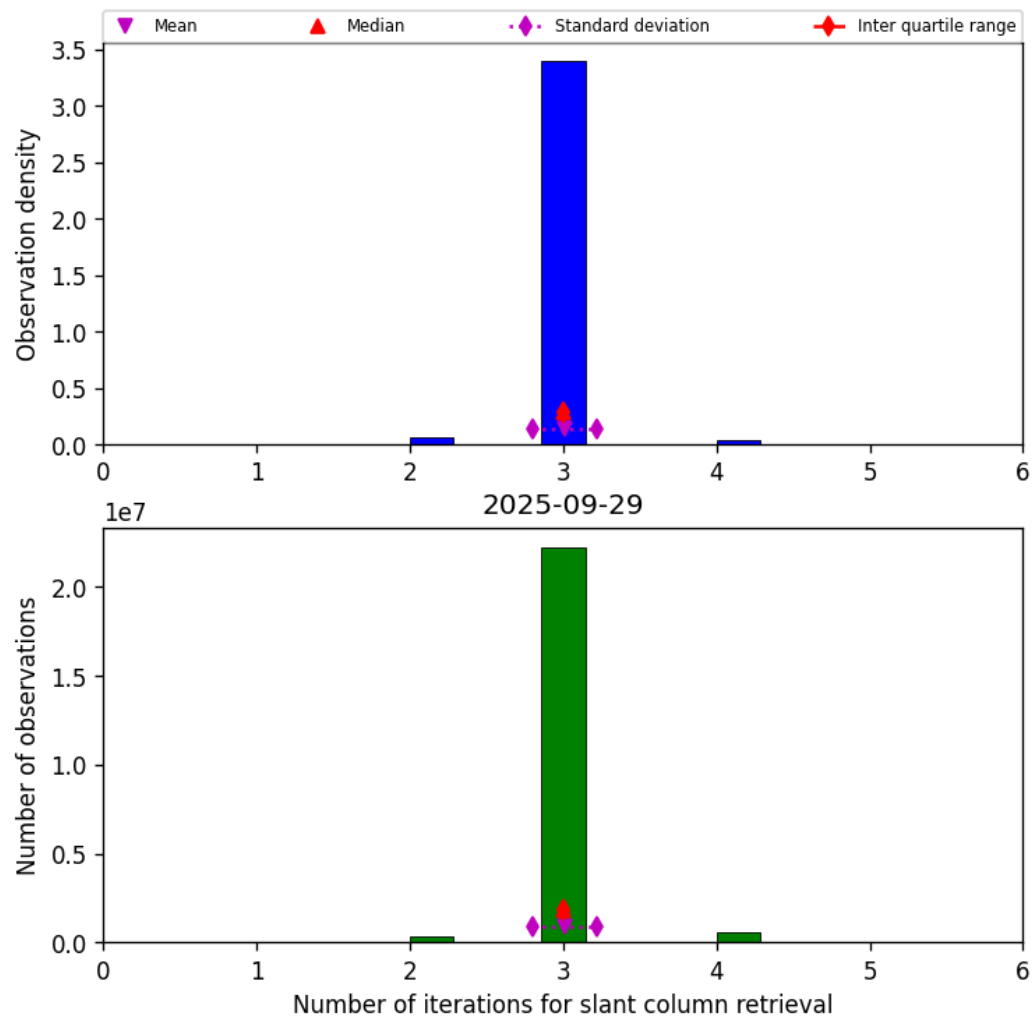
Figure 33: Histogram of “Number of iterations for slant column retrieval” for 2025-09-29 to 2025-09-29
