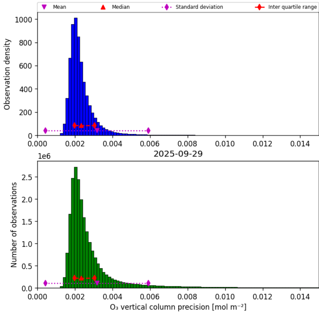
Figure 30: Histogram of "O 3 vertical column precision" for 2025-09-29 to 2025-09-29
