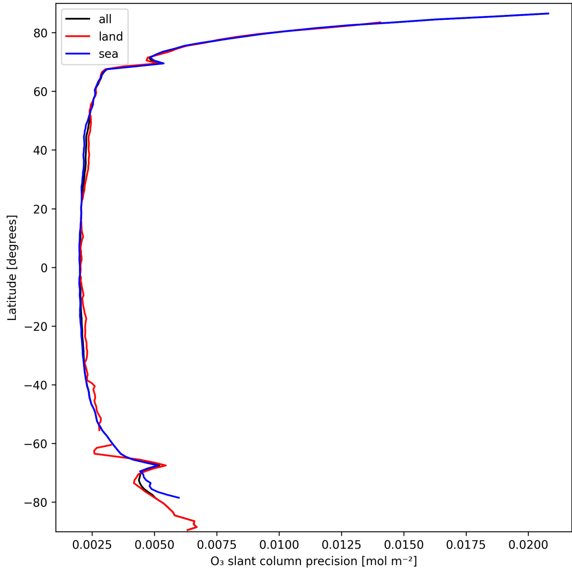
Figure 20: Zonal average of “O 3 slant column precision” for 2025-09-29 to 2025-09-29.
