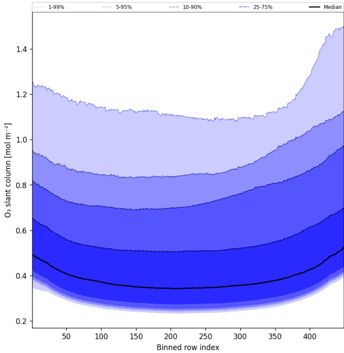
Figure 43: Along track statistics of “O 3 slant column” for 2025-09-29 to 2025-09-29
