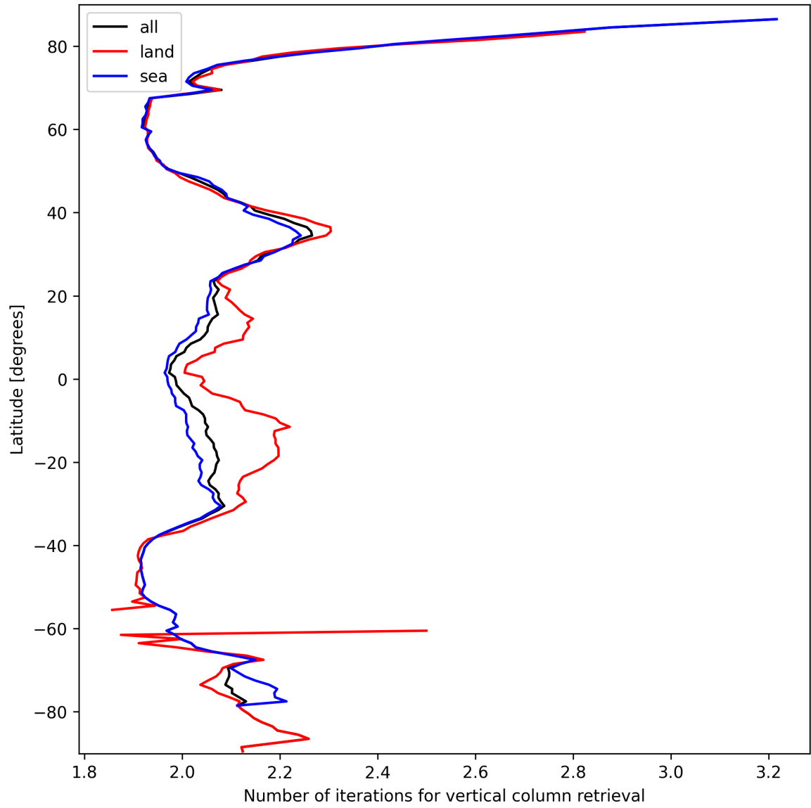
Figure 27: Zonal average of “Number of iterations for vertical column retrieval” for 2025-09-29 to 2025-09-29.
