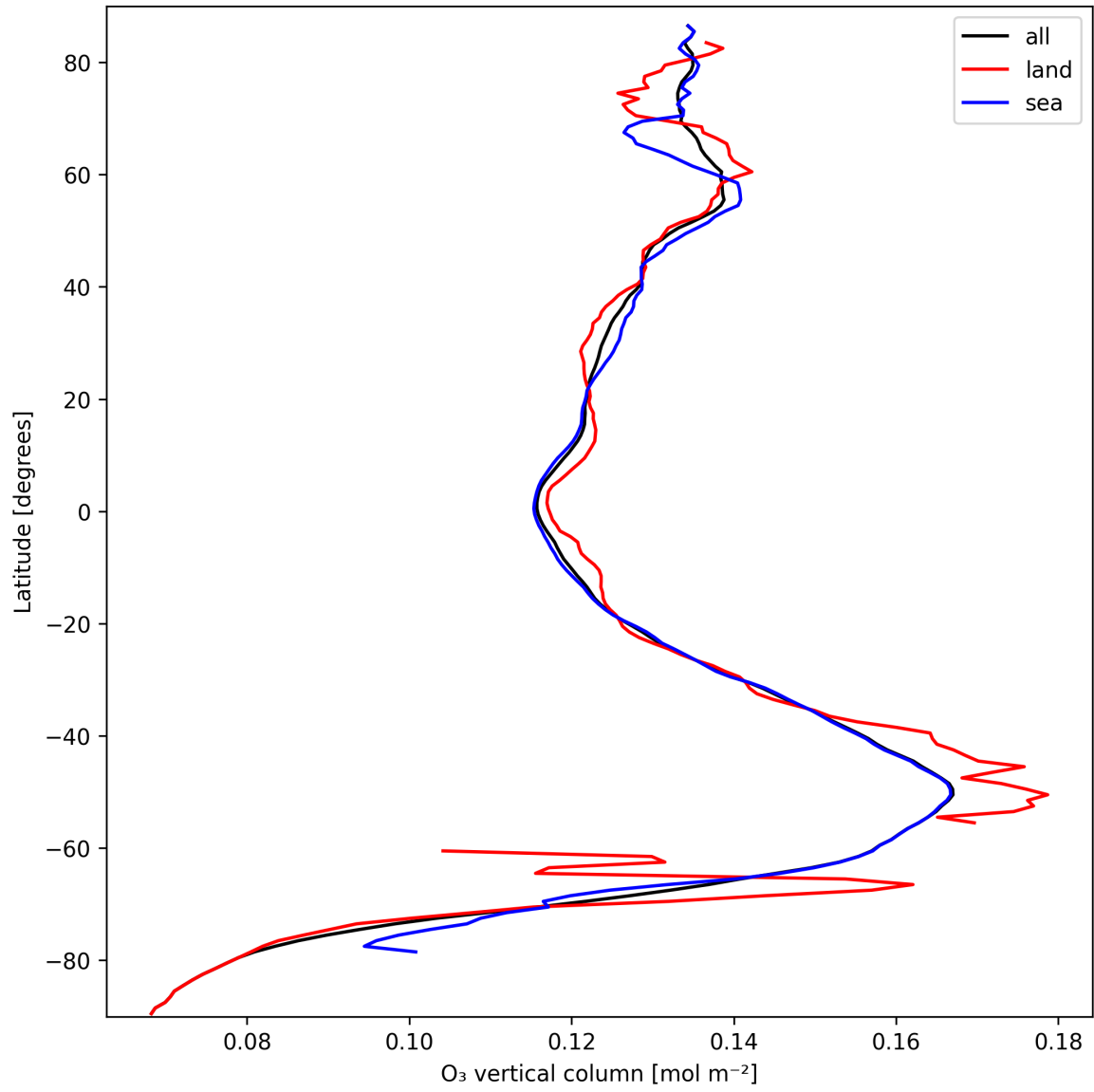
Figure 17: Zonal average of “O 3 vertical column” for 2025-09-29 to 2025-09-29.
