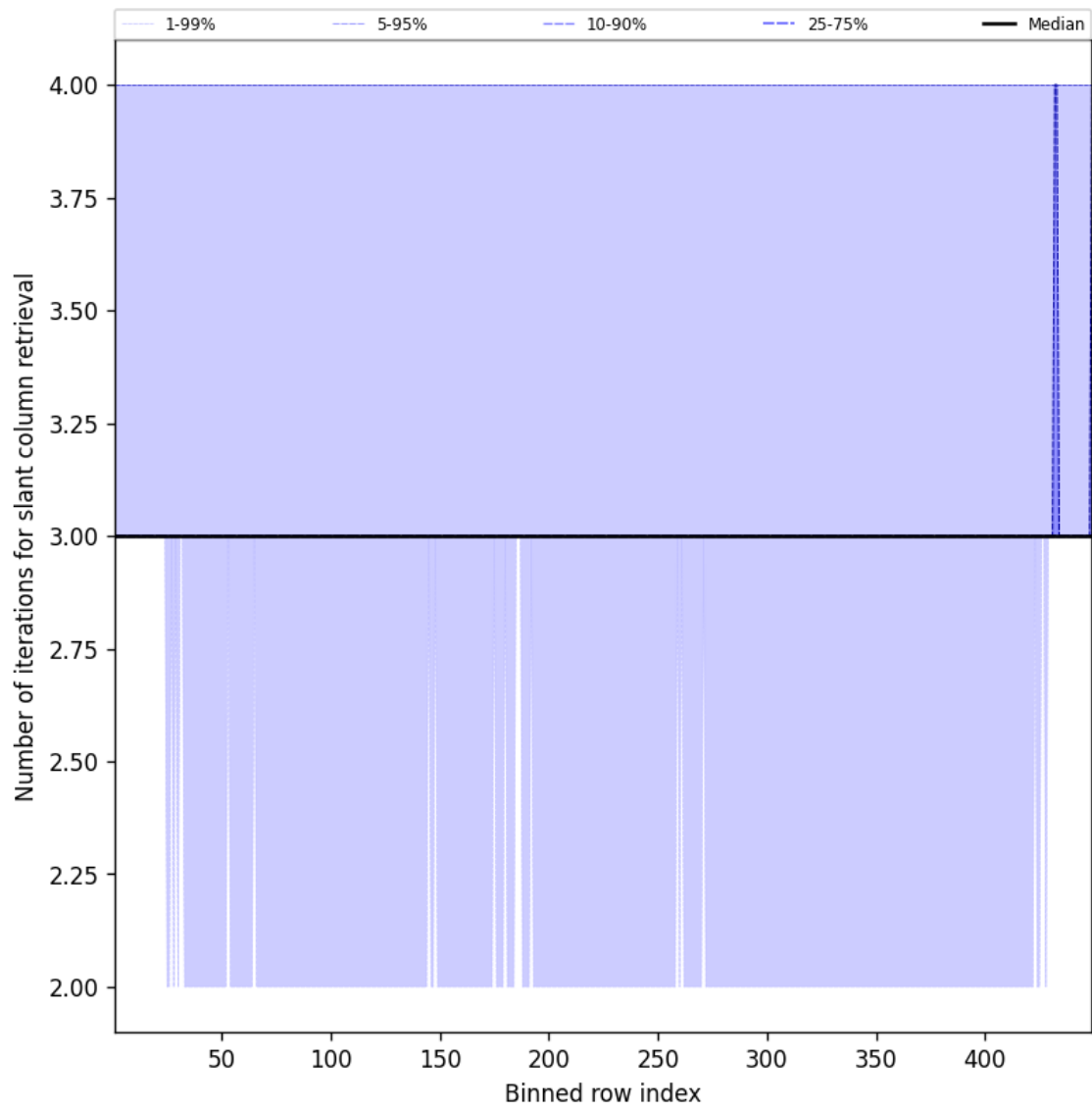
Figure 45: Along track statistics of “Number of iterations for slant column retrieval” for 2025-09-29 to 2025-09-29
