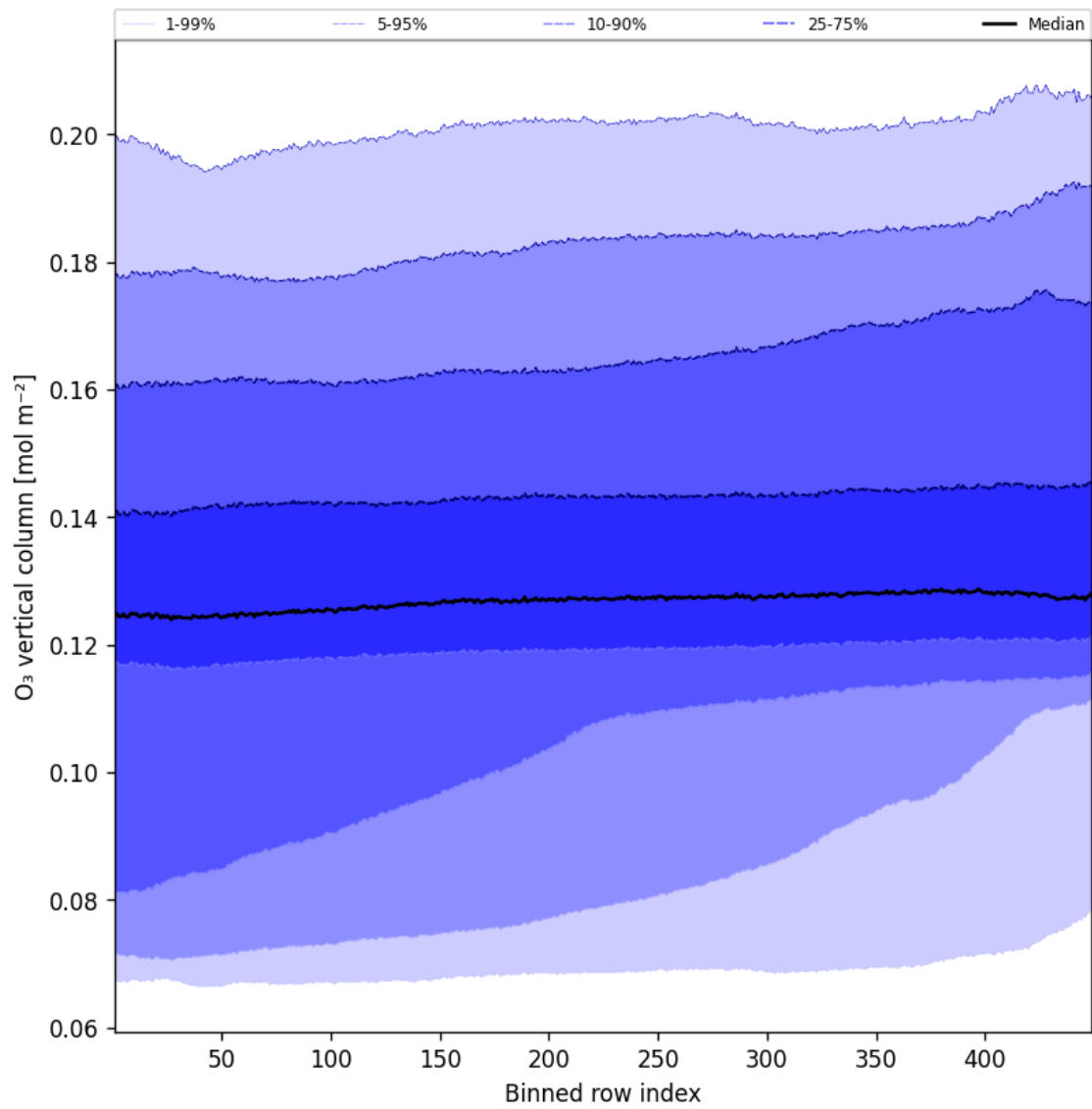
Figure 41: Along track statistics of “O 3 vertical column” for 2025-09-29 to 2025-09-29
