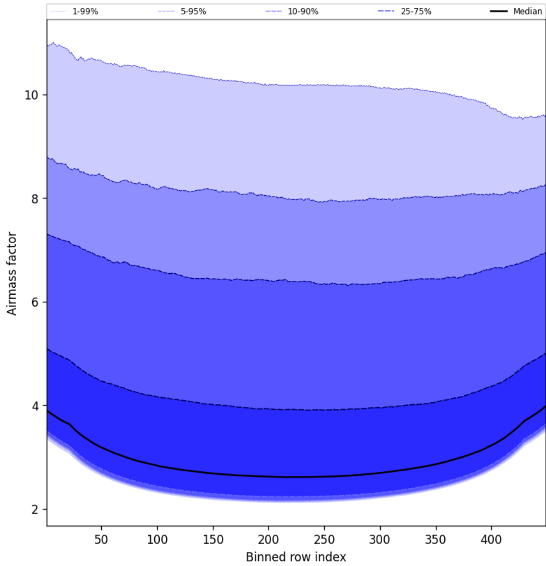
Figure 49: Along track statistics of “Airmass factor” for 2025-09-29 to 2025-09-29
