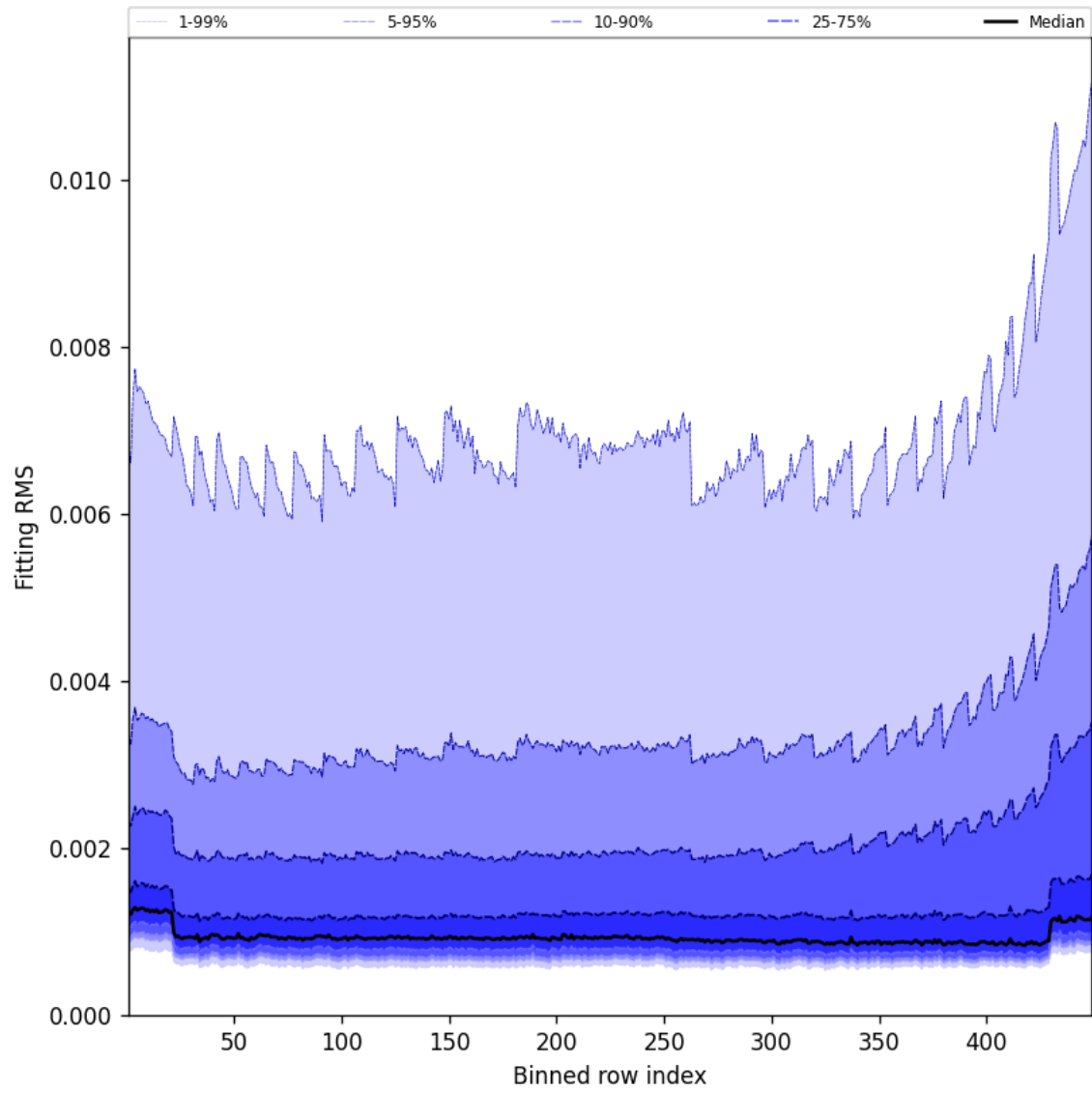
Figure 46: Along track statistics of “Fitting RMS” for 2025-09-29 to 2025-09-29
