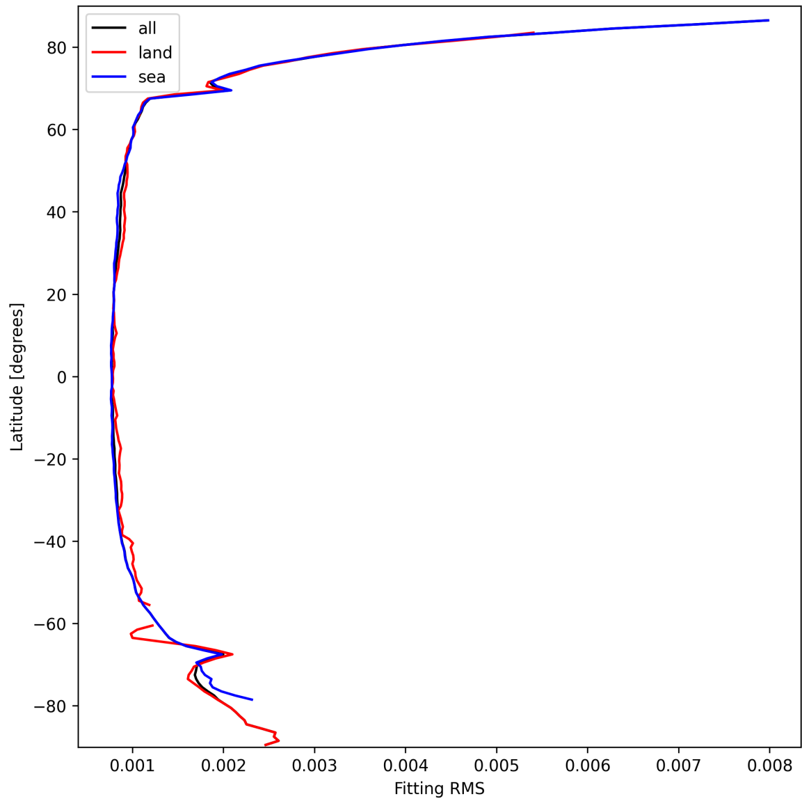
Figure 22: Zonal average of “Fitting RMS” for 2025-09-29 to 2025-09-29.
