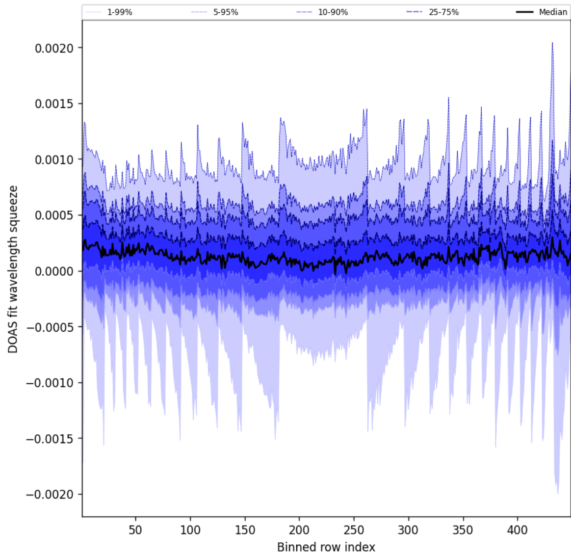
Figure 48: Along track statistics of “DOAS fit wavelength squeeze” for 2025-09-29 to 2025-09-29
