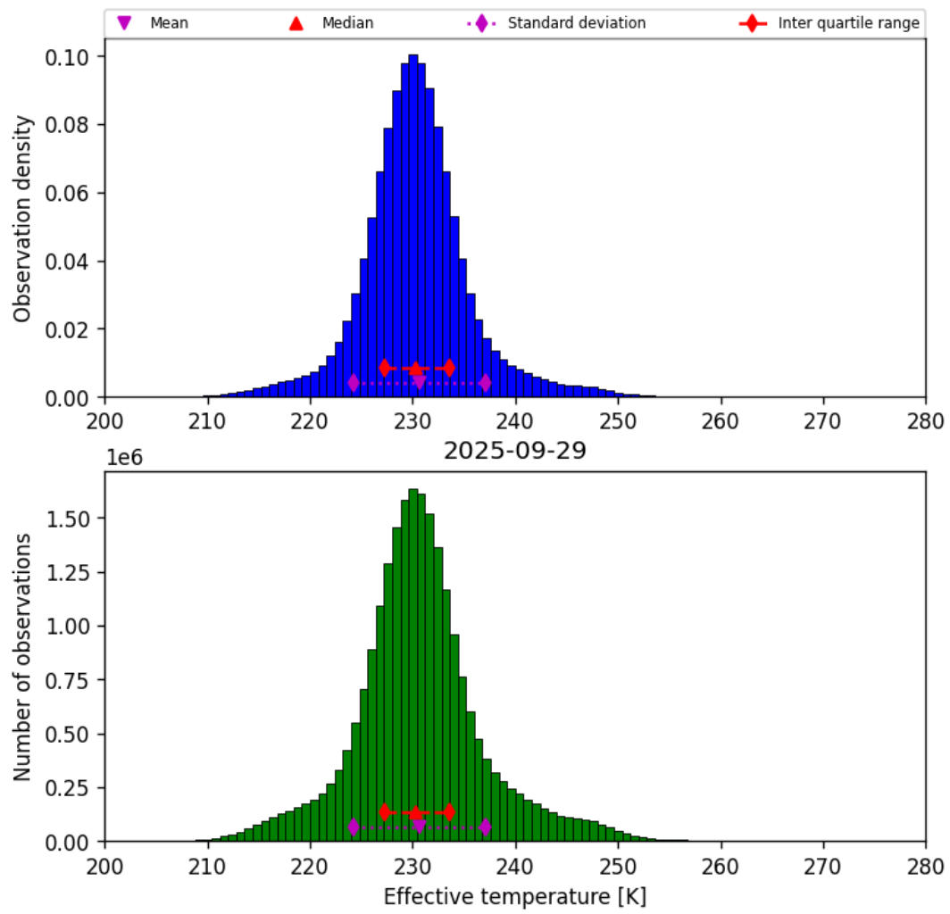
Figure 38: Histogram of “Effective temperature” for 2025-09-29 to 2025-09-29
