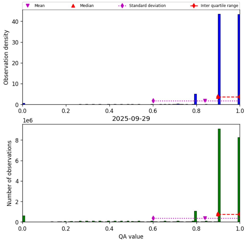
Figure 28: Histogram of “QA value” for 2025-09-29 to 2025-09-29
