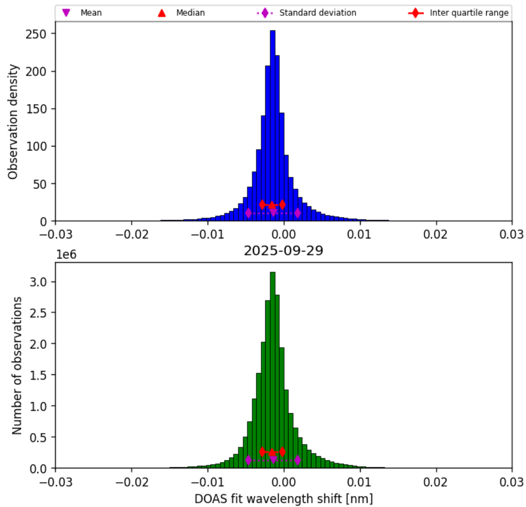
Figure 35: Histogram of “DOAS fit wavelength shift” for 2025-09-29 to 2025-09-29
