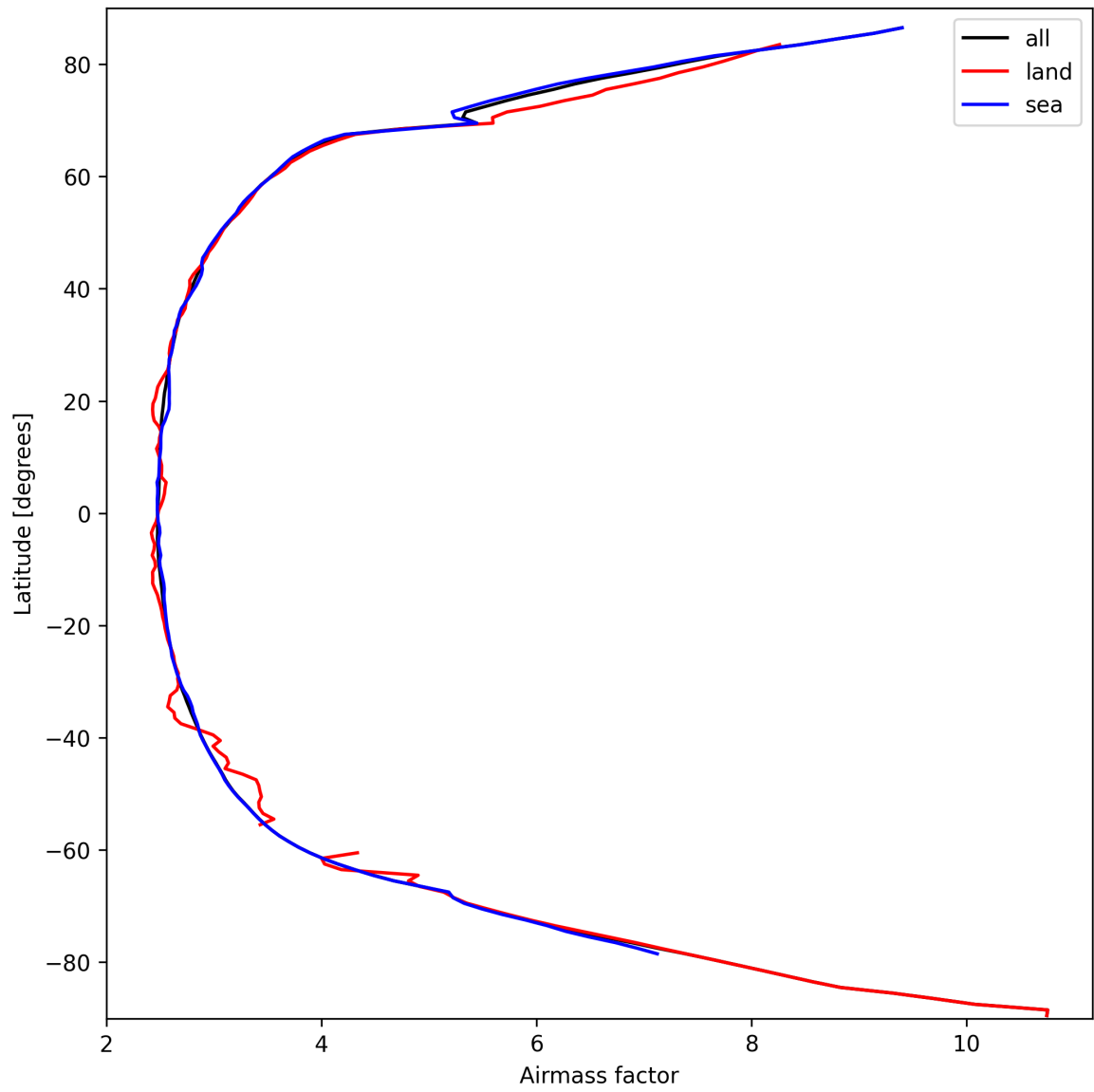
Figure 25: Zonal average of “Airmass factor” for 2025-09-29 to 2025-09-29.
