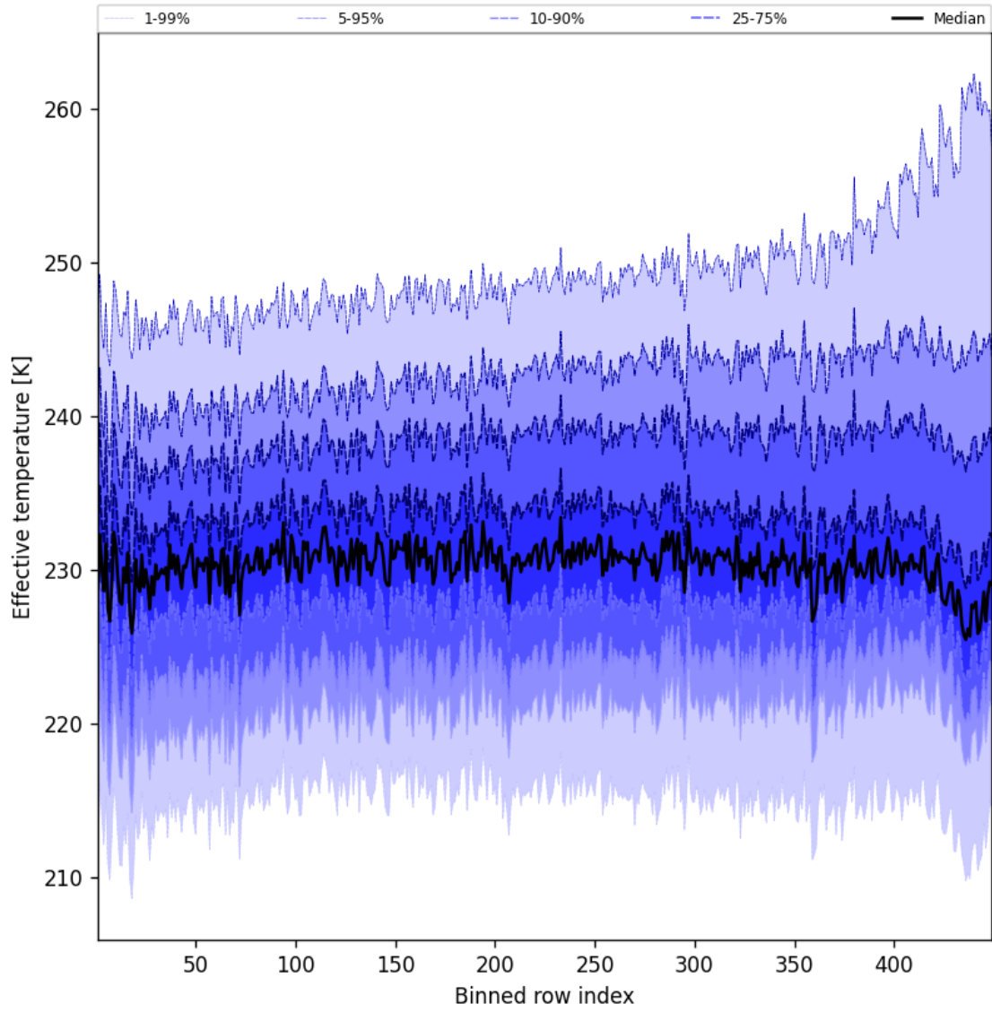
Figure 50: Along track statistics of “Effective temperature” for 2025-09-29 to 2025-09-29
