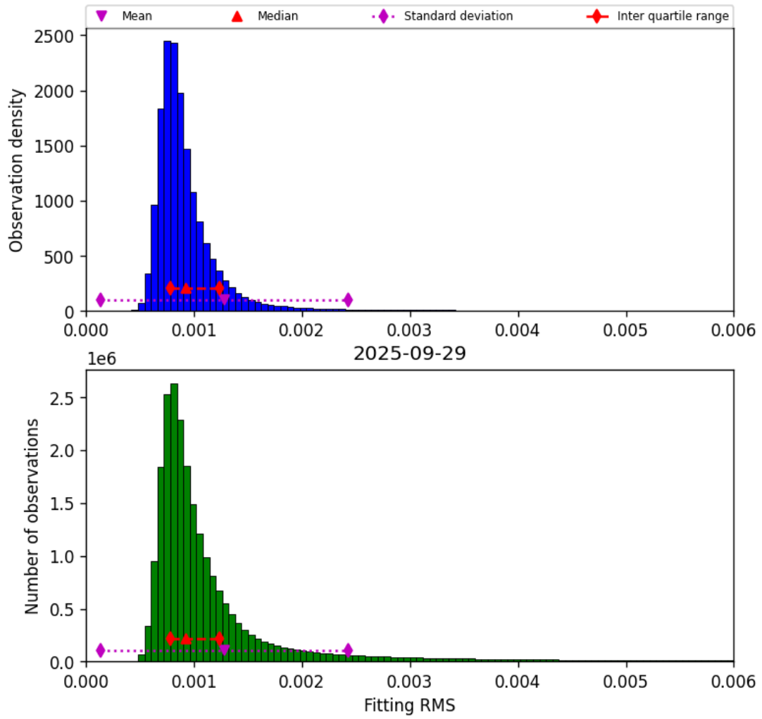
Figure 34: Histogram of “Fitting RMS” for 2025-09-29 to 2025-09-29
