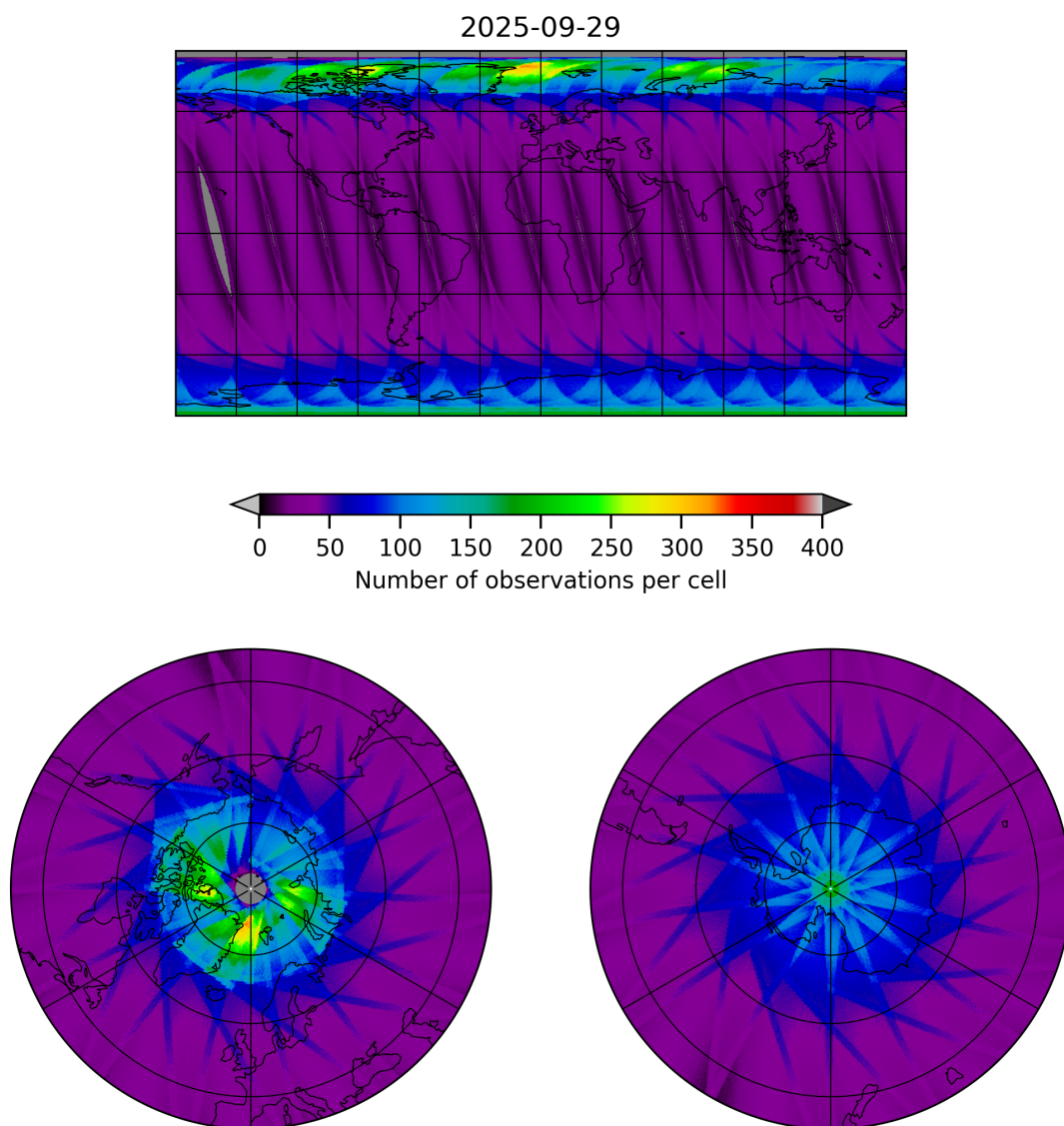
Figure 15: Map of the number of observations for 2025-09-29 to 2025-09-29
