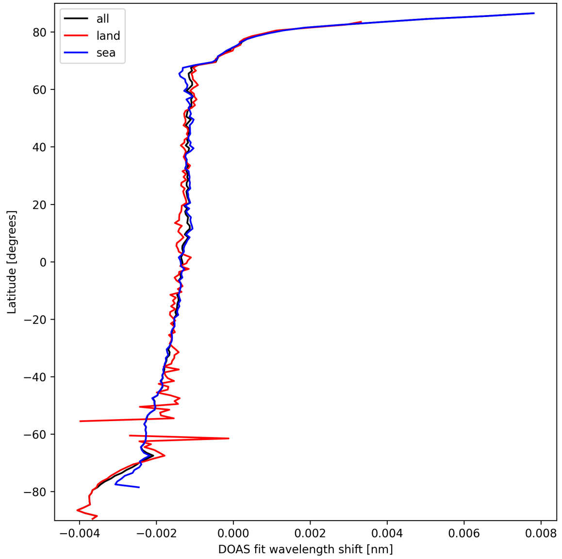
Figure 23: Zonal average of "DOAS fit wavelength shift" for 2025-09-29 to 2025-09-29.
