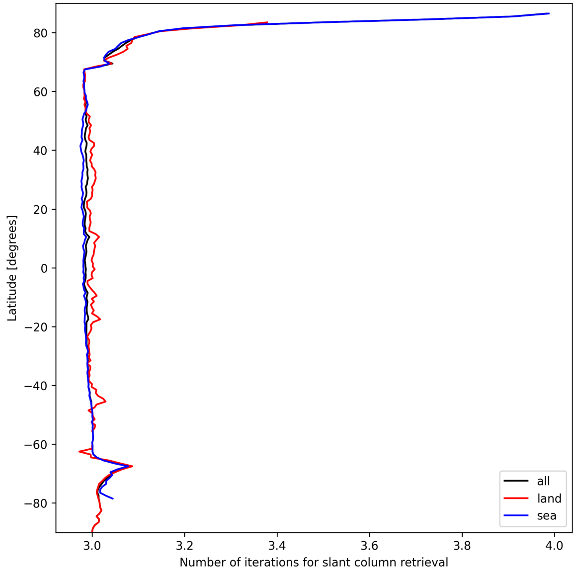
Figure 21: Zonal average of “Number of iterations for slant column retrieval” for 2025-09-29 to 2025-09-29.
