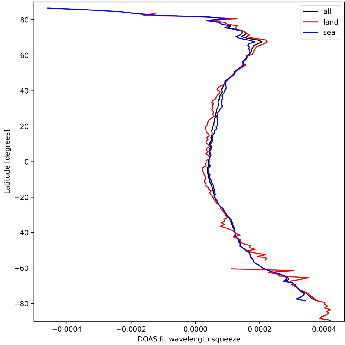
Figure 24: Zonal average of “DOAS fit wavelength squeeze” for 2025-09-29 to 2025-09-29.
