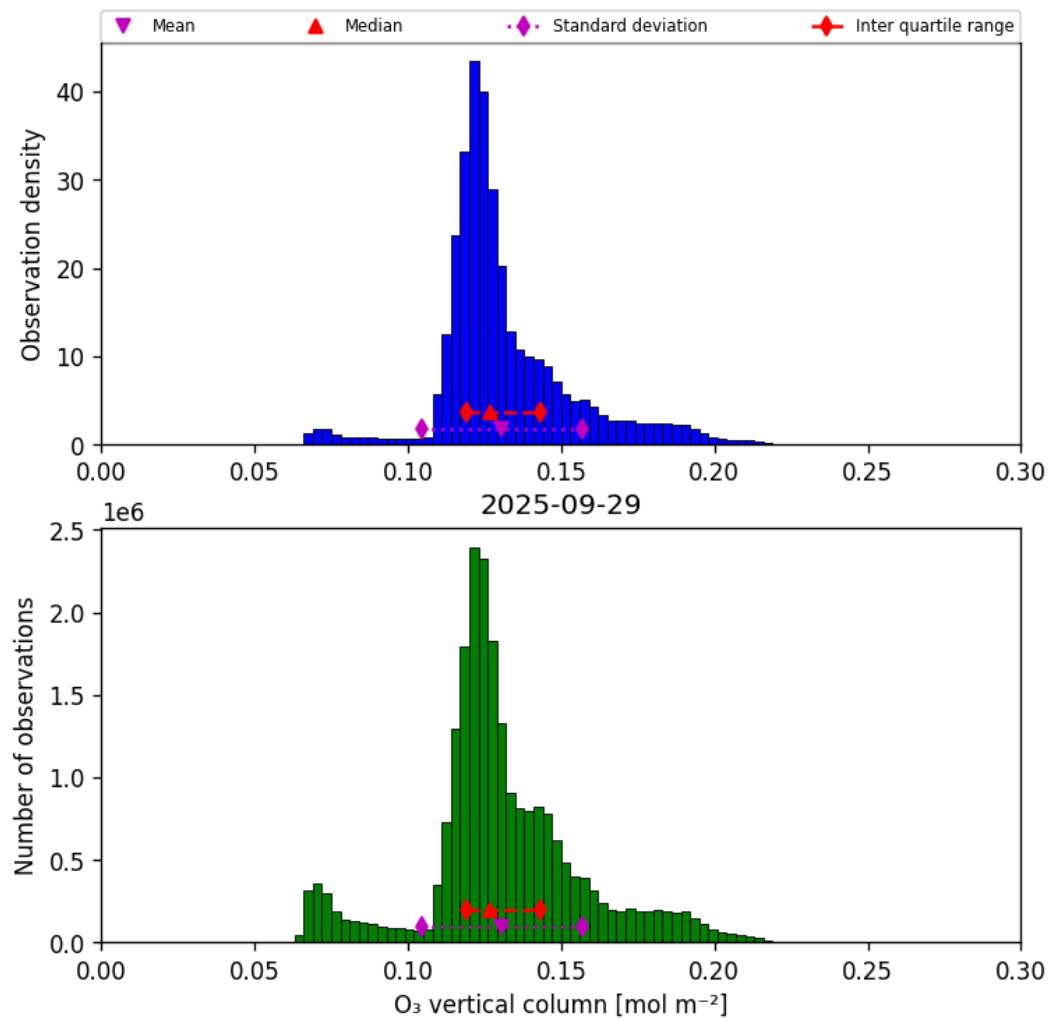
Figure 29: Histogram of “O 3 vertical column” for 2025-09-29 to 2025-09-29
