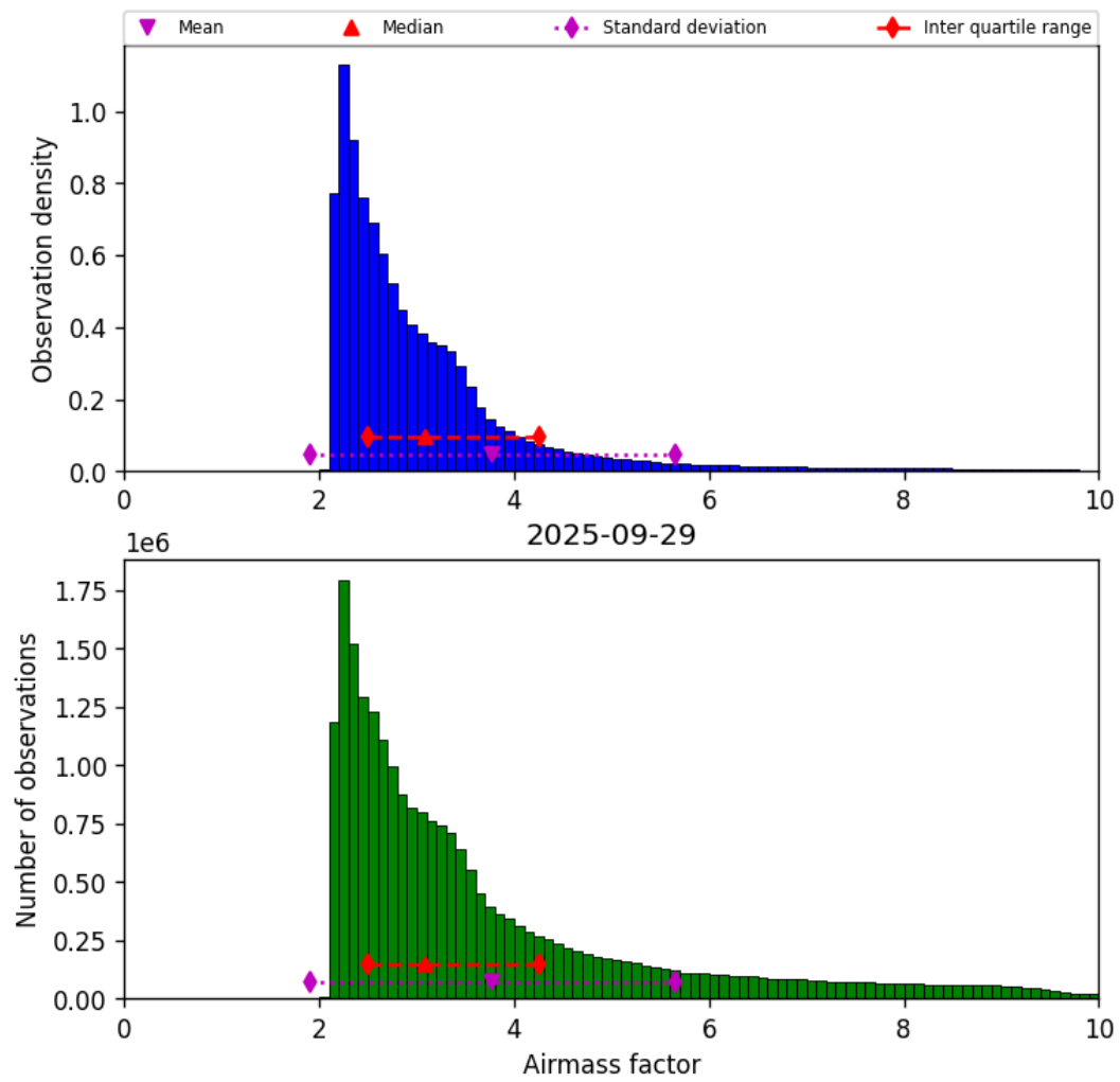
Figure 37: Histogram of “Airmass factor” for 2025-09-29 to 2025-09-29
