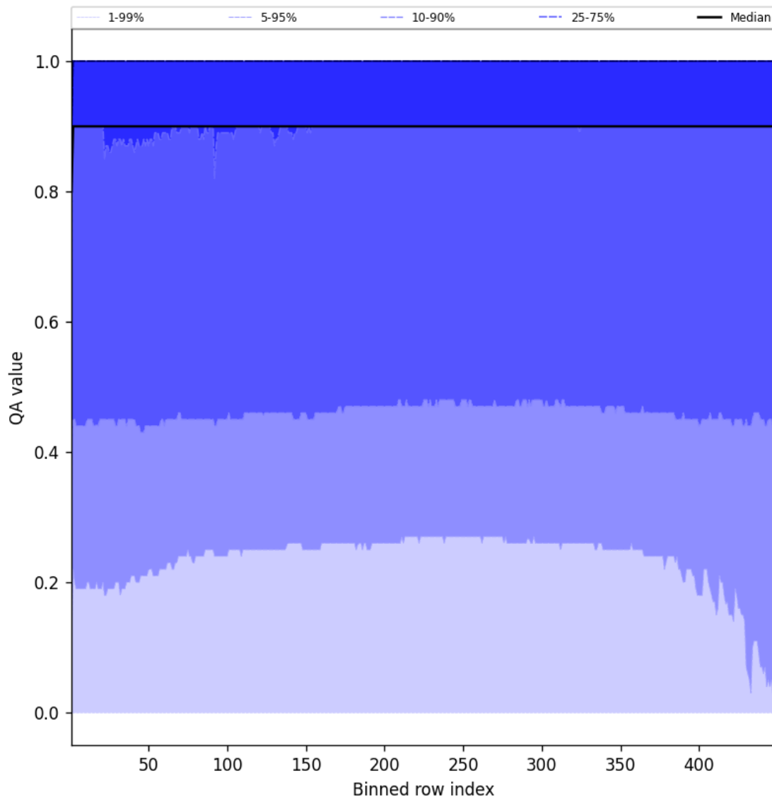
Figure 40: Along track statistics of “QA value” for 2025-09-29 to 2025-09-29
