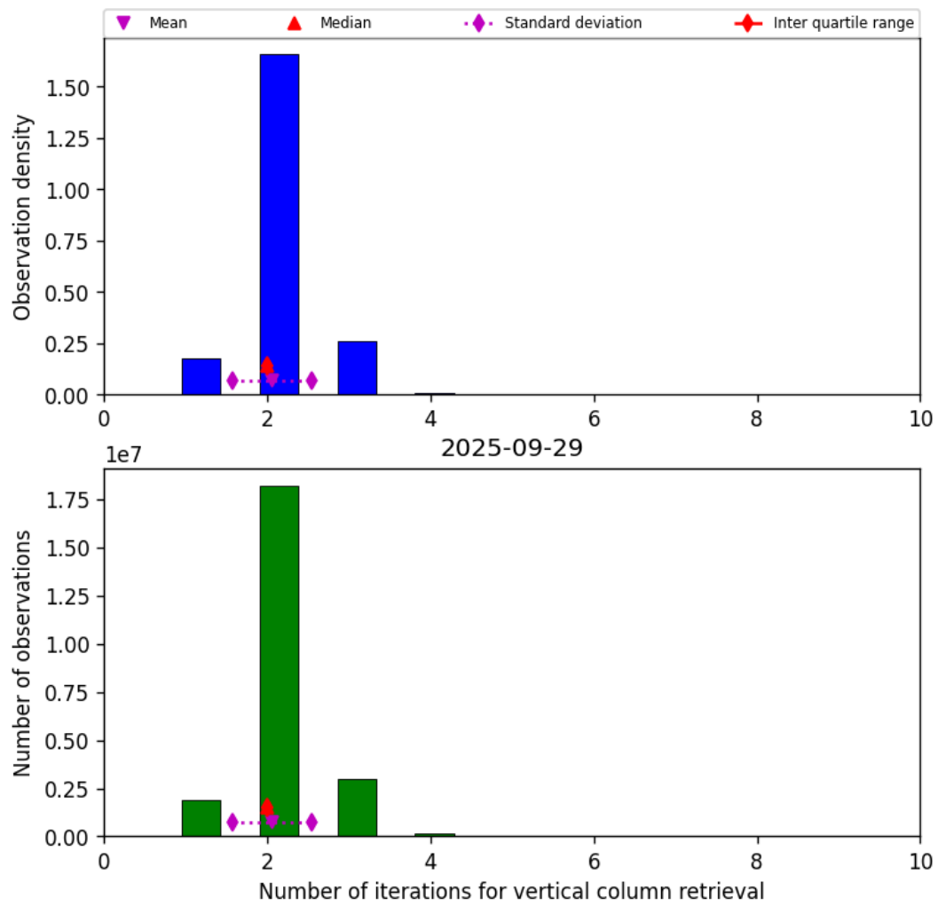
Figure 39: Histogram of “Number of iterations for vertical column retrieval” for 2025-09-29 to 2025-09-29
