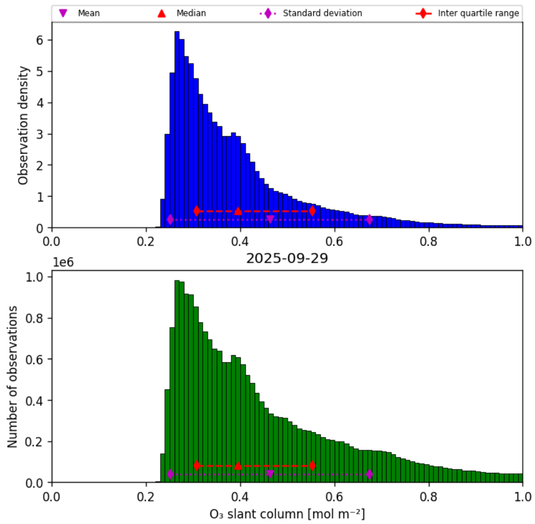
Figure 31: Histogram of “O 3 slant column” for 2025-09-29 to 2025-09-29
