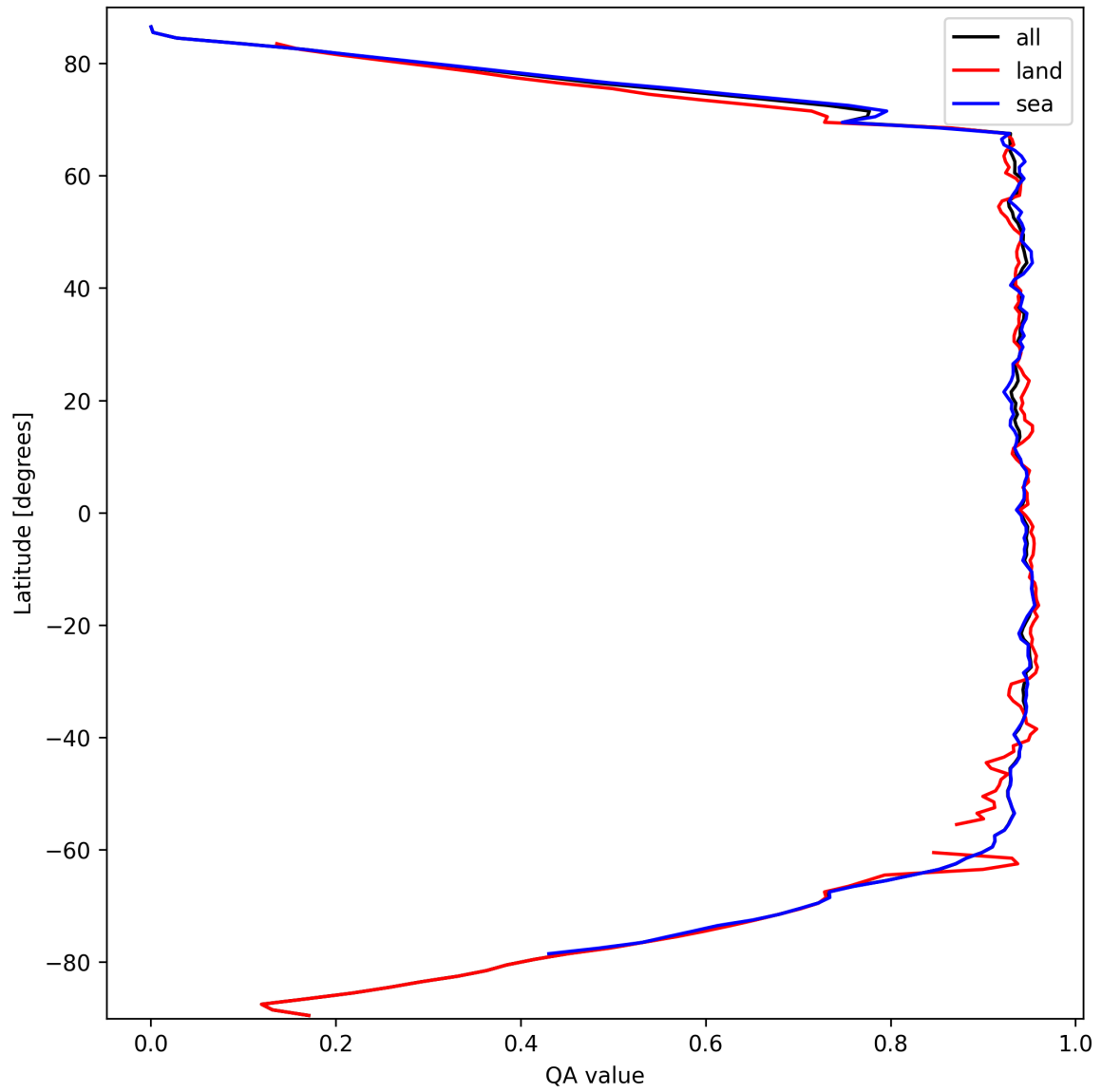
Figure 16: Zonal average of “QA value” for 2025-09-29 to 2025-09-29.
