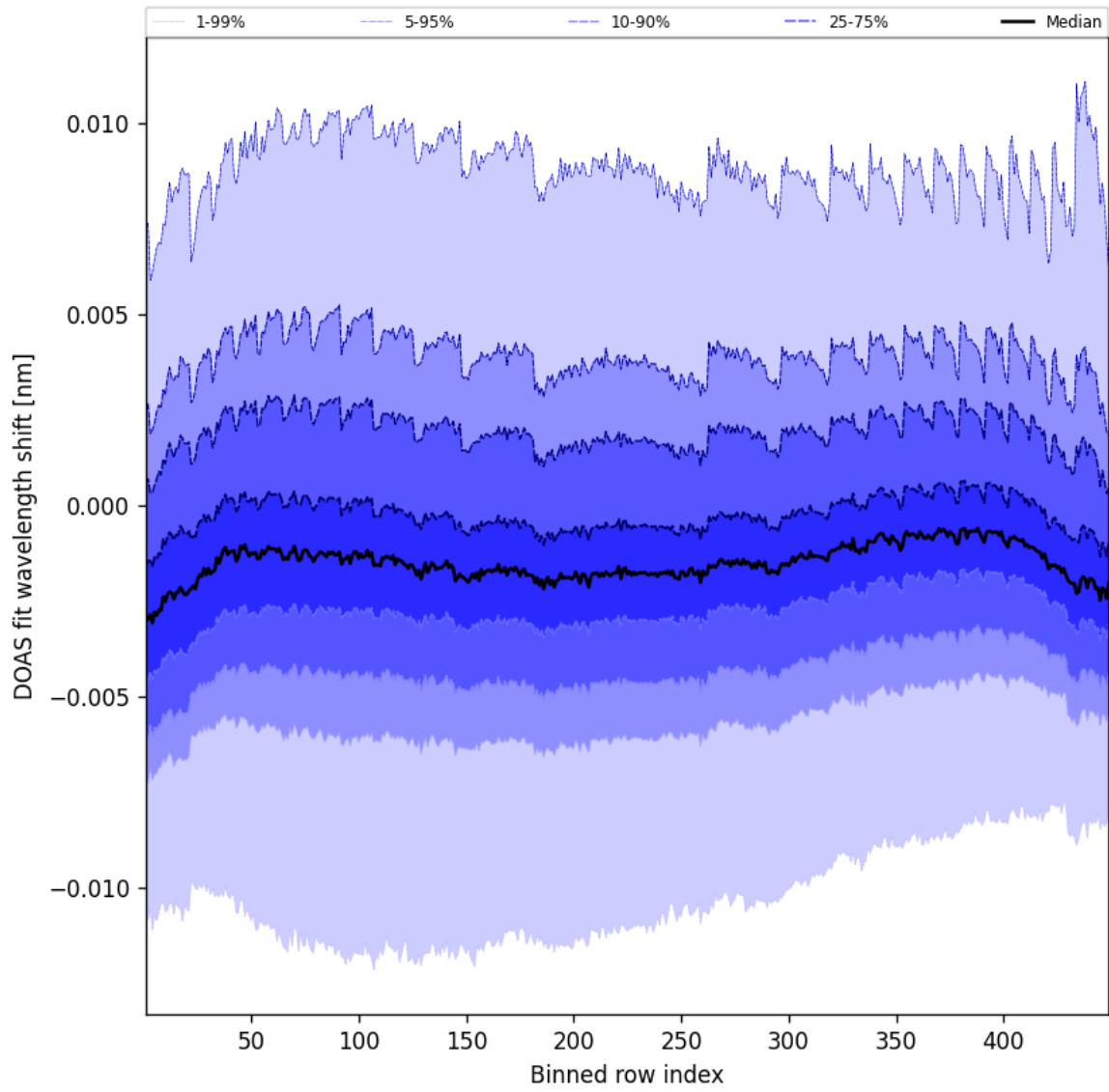
Figure 47: Along track statistics of “DOAS fit wavelength shift” for 2025-09-29 to 2025-09-29
