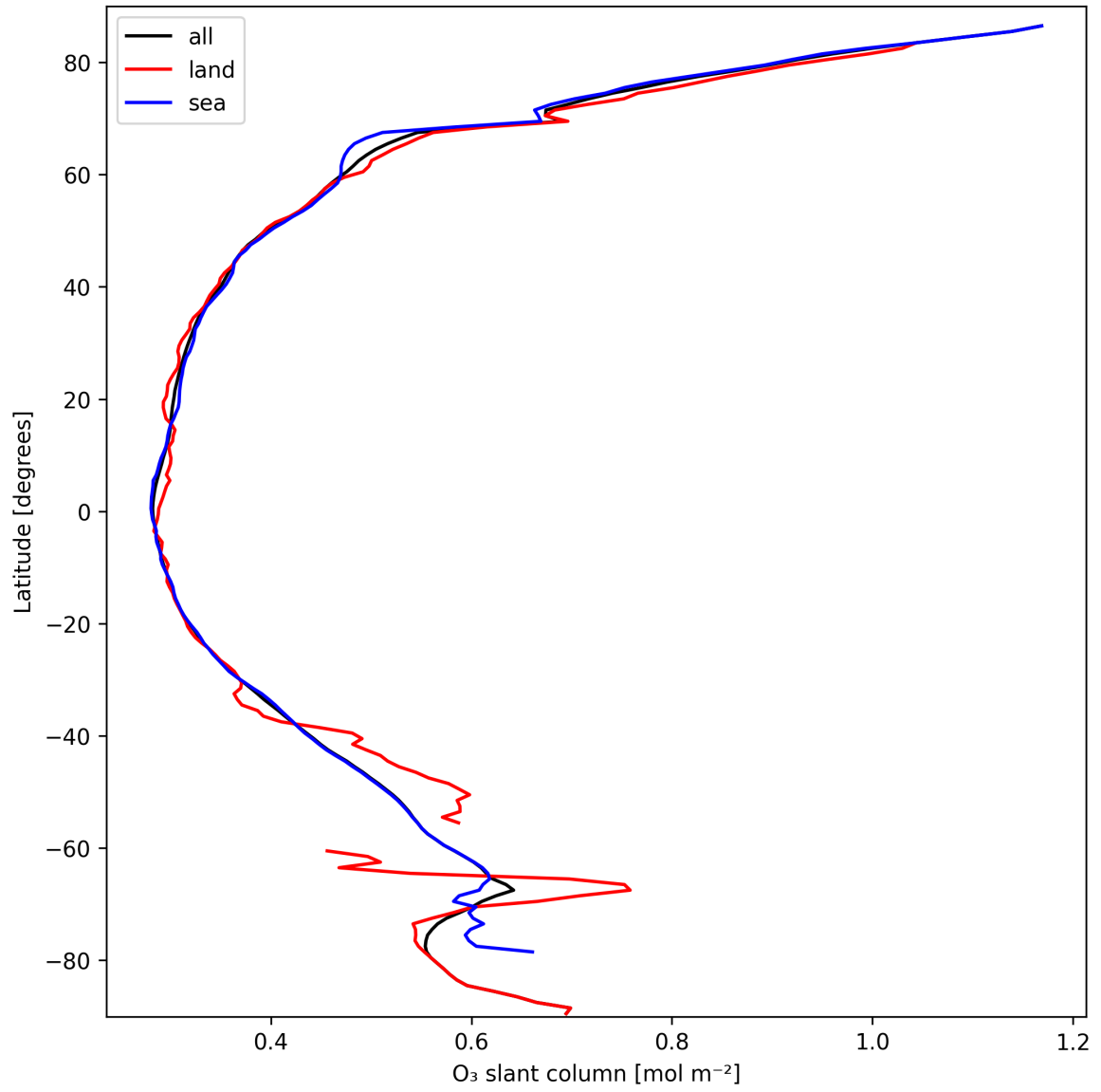
Figure 19: Zonal average of “O 3 slant column” for 2025-09-29 to 2025-09-29.
