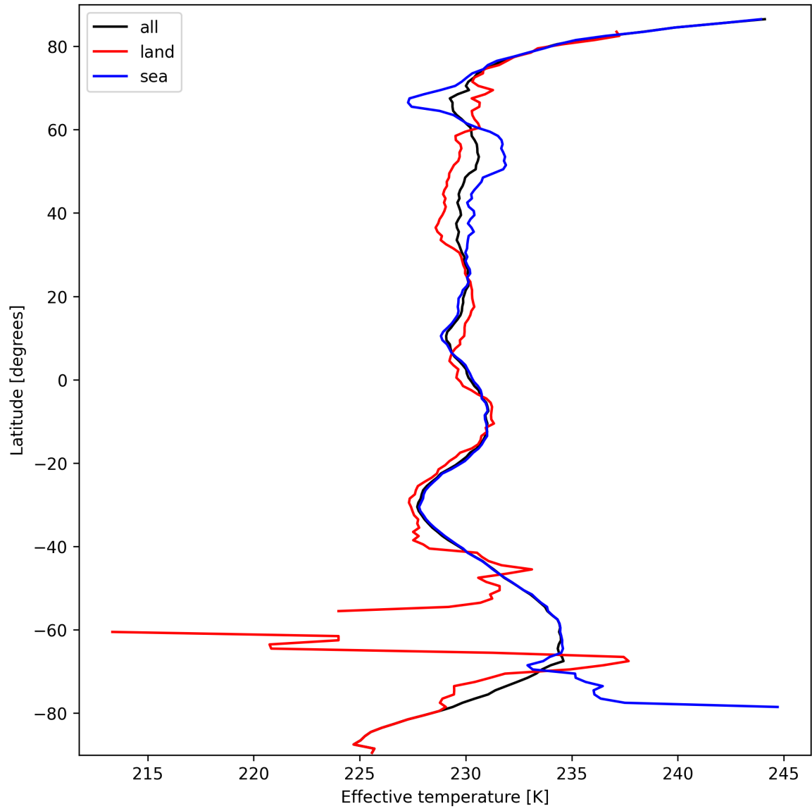
Figure 26: Zonal average of “Effective temperature” for 2025-09-29 to 2025-09-29.
