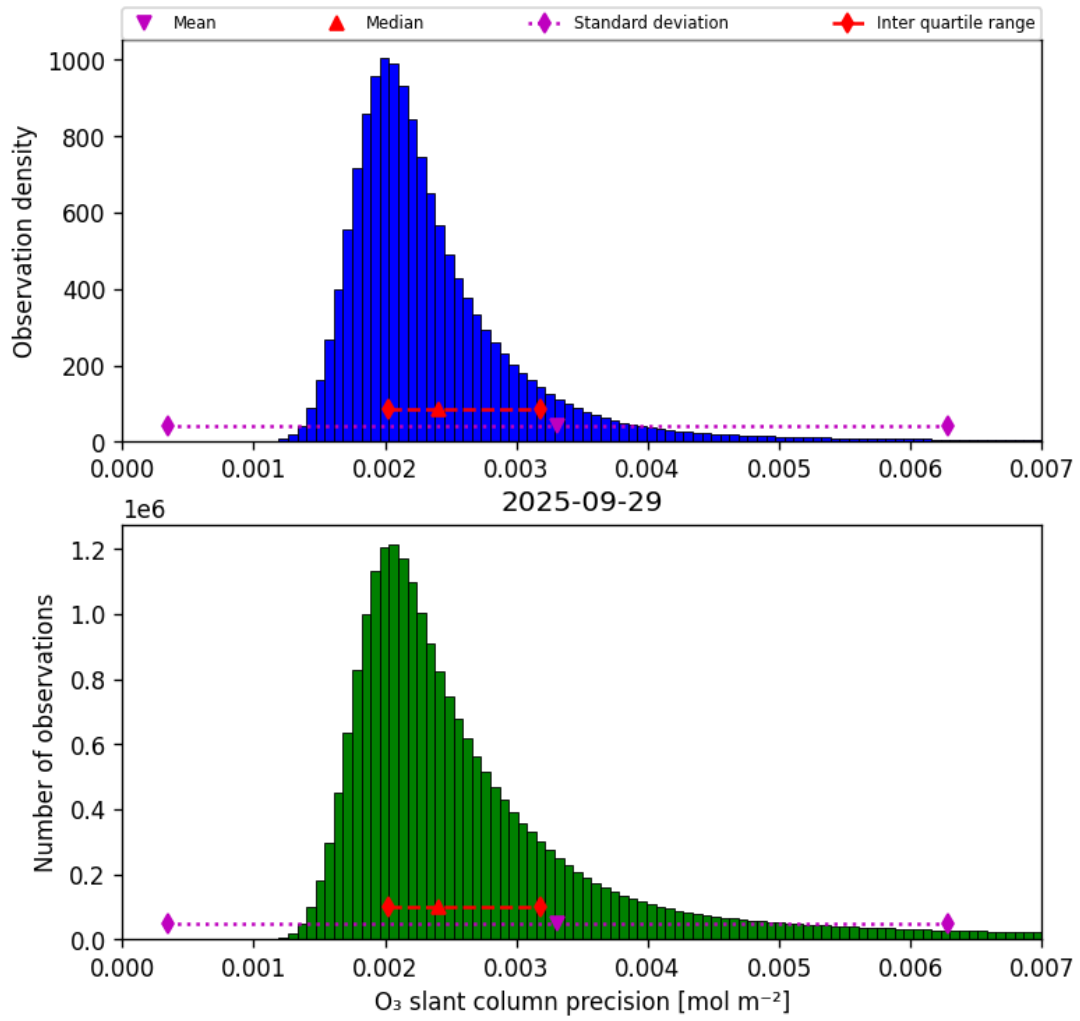
Figure 32: Histogram of “O 3 slant column precision” for 2025-09-29 to 2025-09-29
