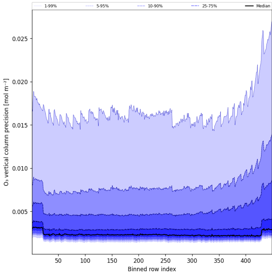
Figure 42: Along track statistics of “O 3 vertical column precision” for 2025-09-29 to 2025-09-29
