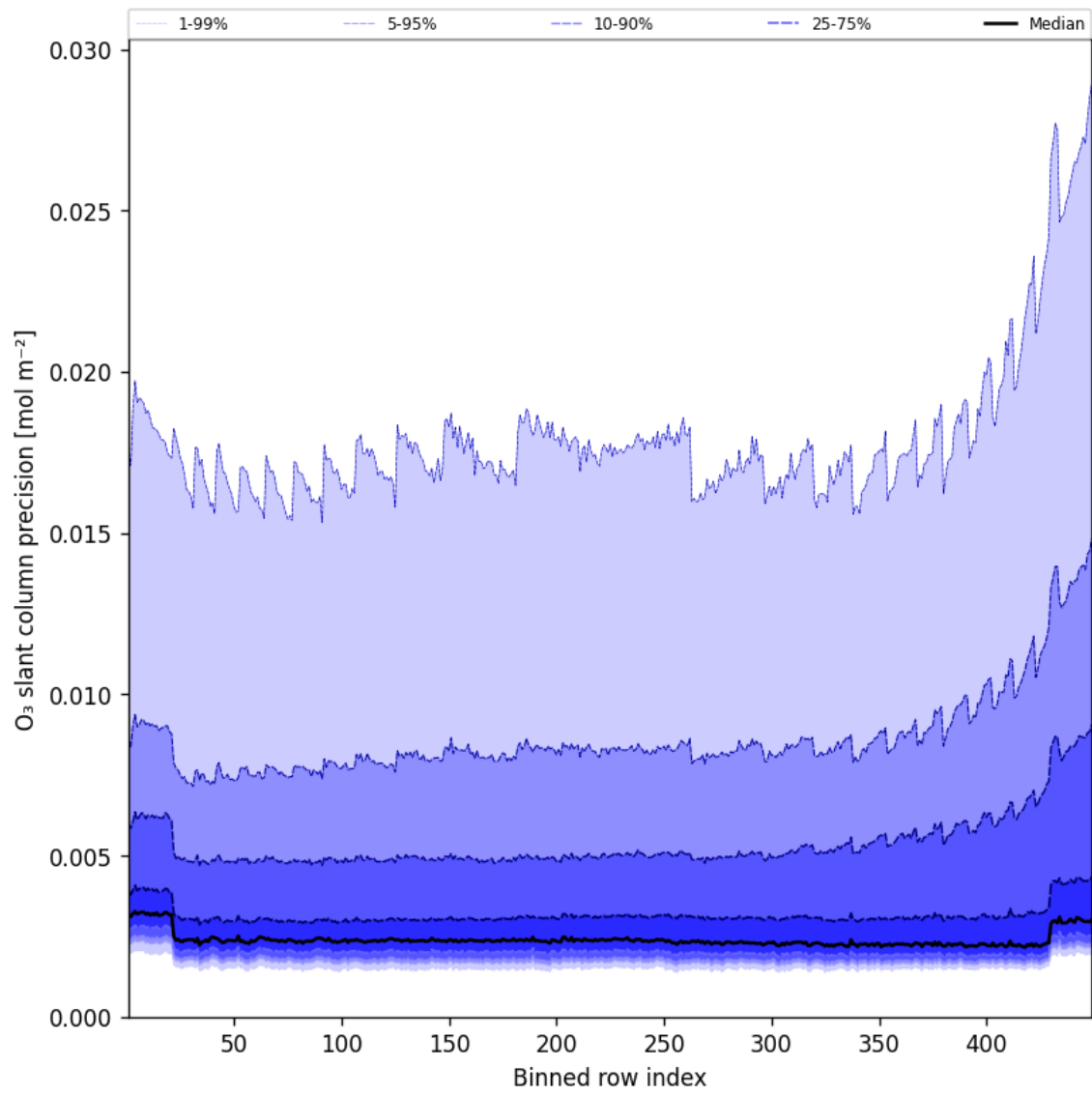
Figure 44: Along track statistics of “O 3 slant column precision” for 2025-09-29 to 2025-09-29
