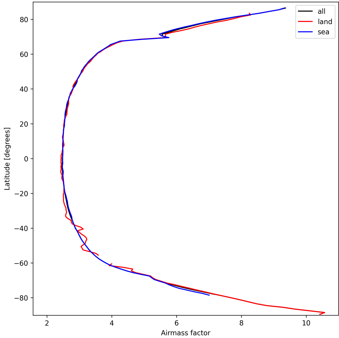
Figure 25: Zonal average of “Airmass factor” for 2025-09-30 to 2025-10-01.
