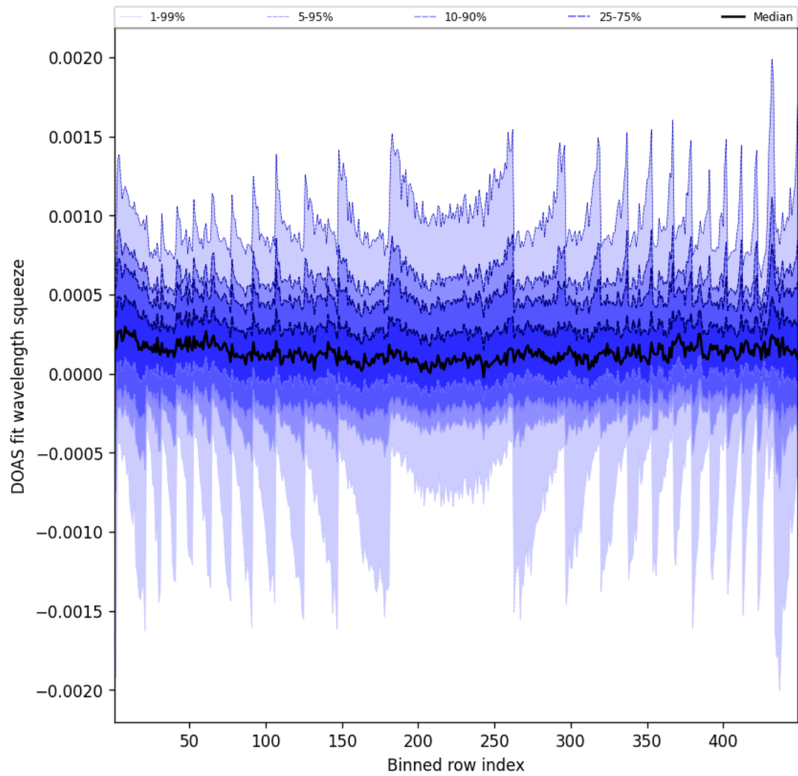
Figure 48: Along track statistics of “DOAS fit wavelength squeeze” for 2025-09-30 to 2025-10-01
