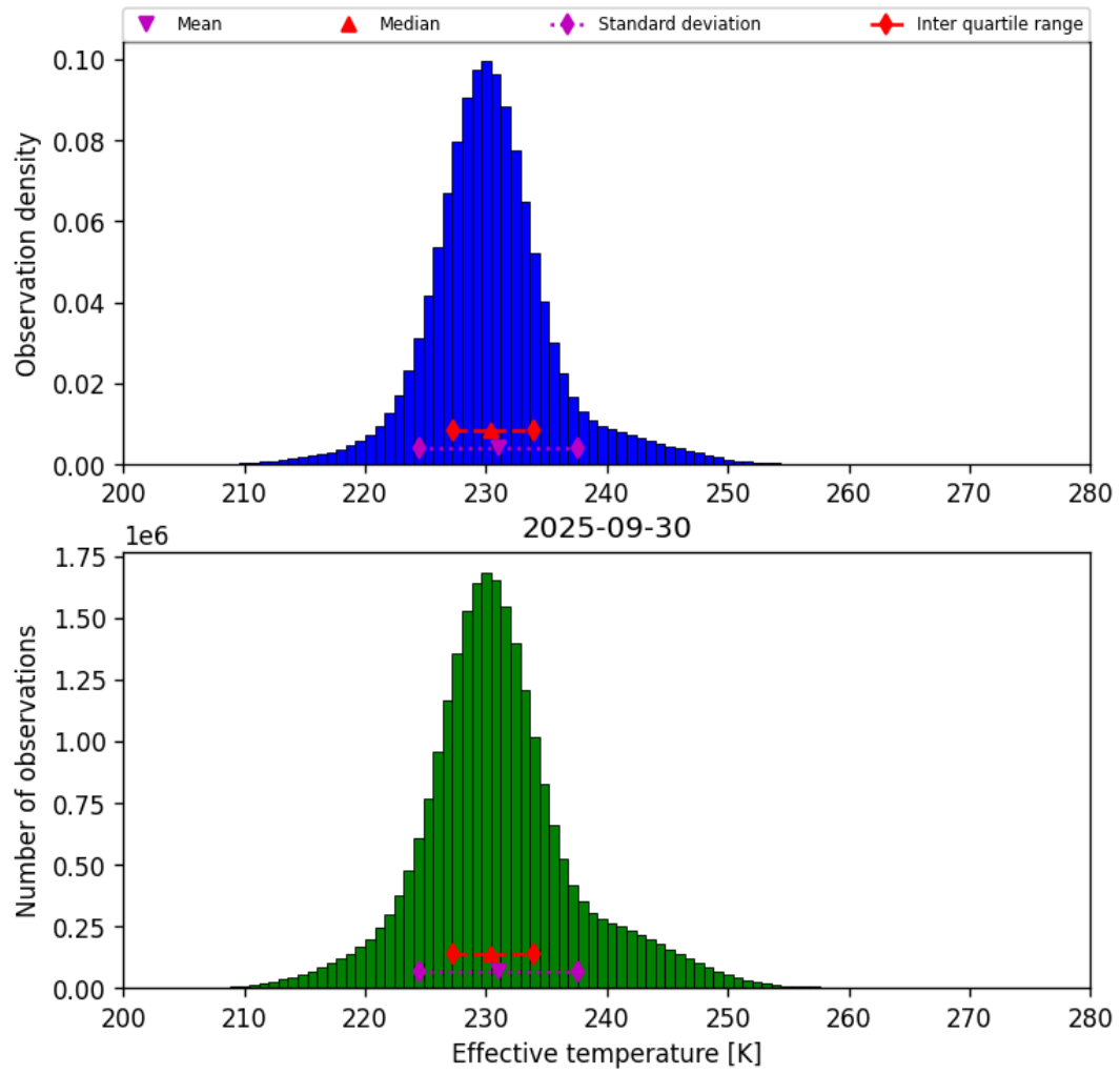
Figure 38: Histogram of “Effective temperature” for 2025-09-30 to 2025-10-01
