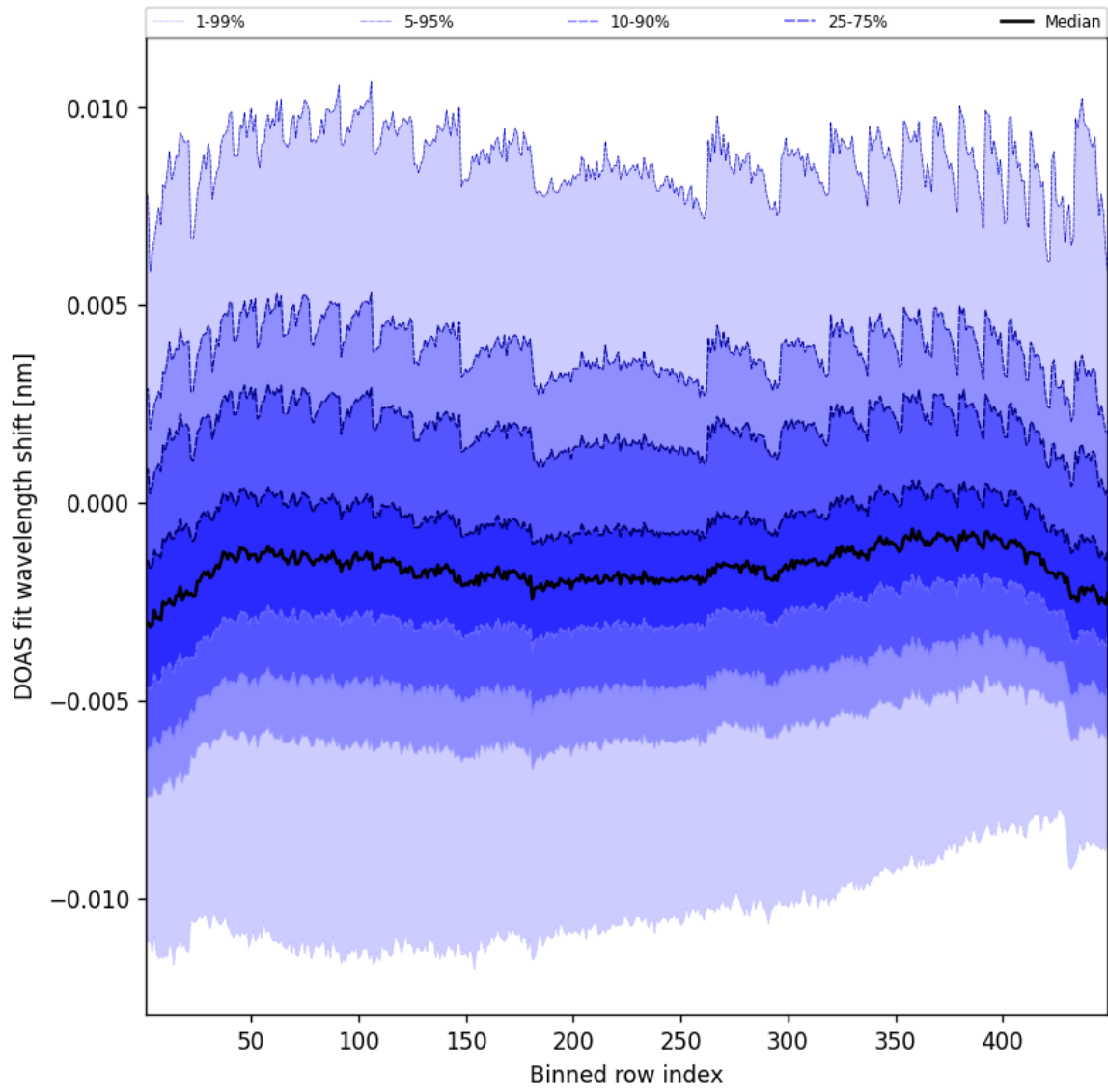
Figure 47: Along track statistics of “DOAS fit wavelength shift” for 2025-09-30 to 2025-10-01
