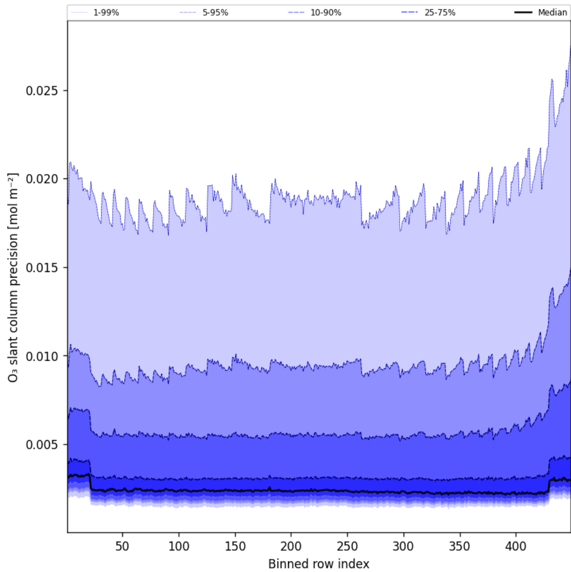
Figure 44: Along track statistics of “O 3 slant column precision” for 2025-09-30 to 2025-10-01
