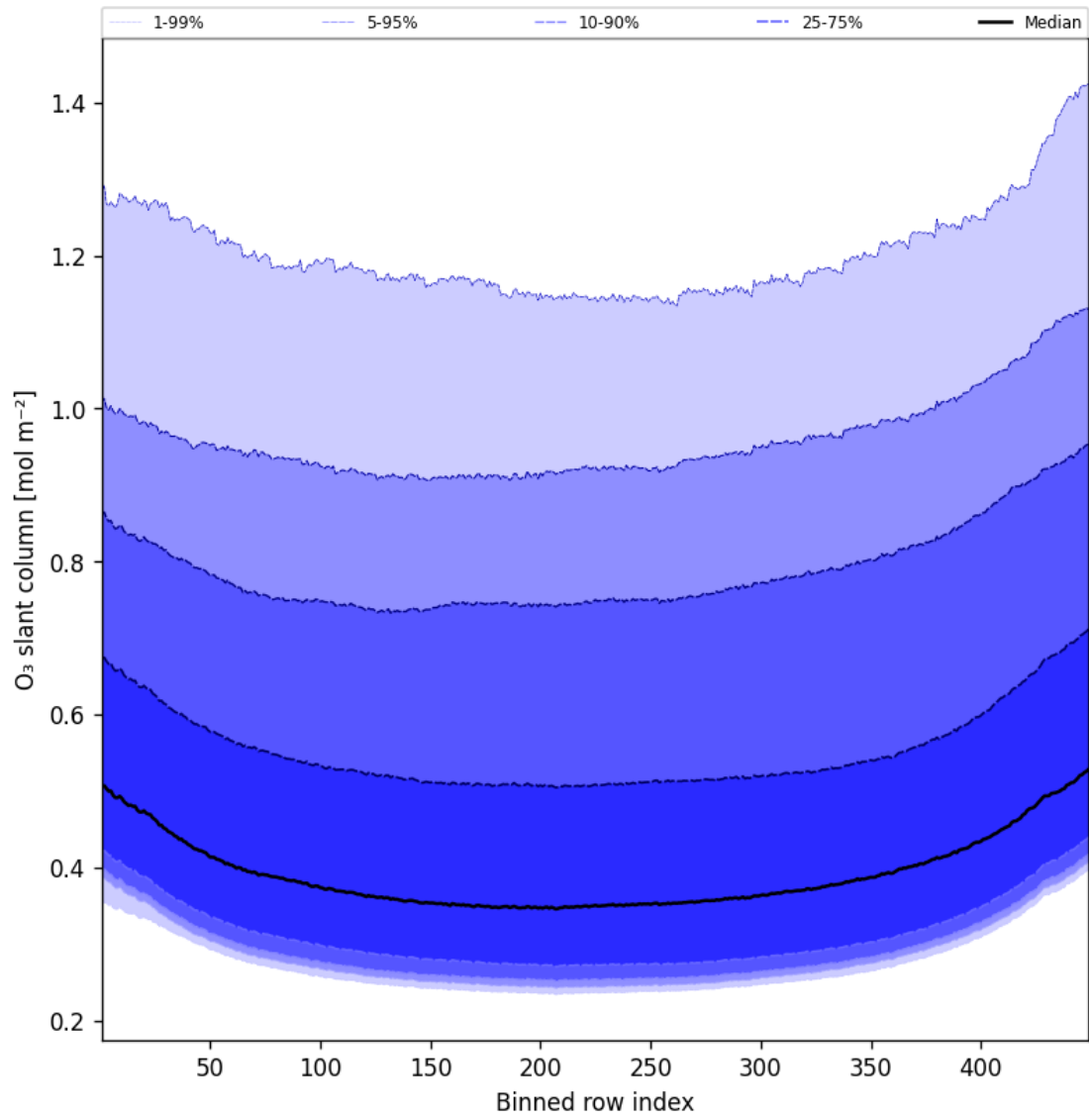
Figure 43: Along track statistics of “O 3 slant column” for 2025-09-30 to 2025-10-01
