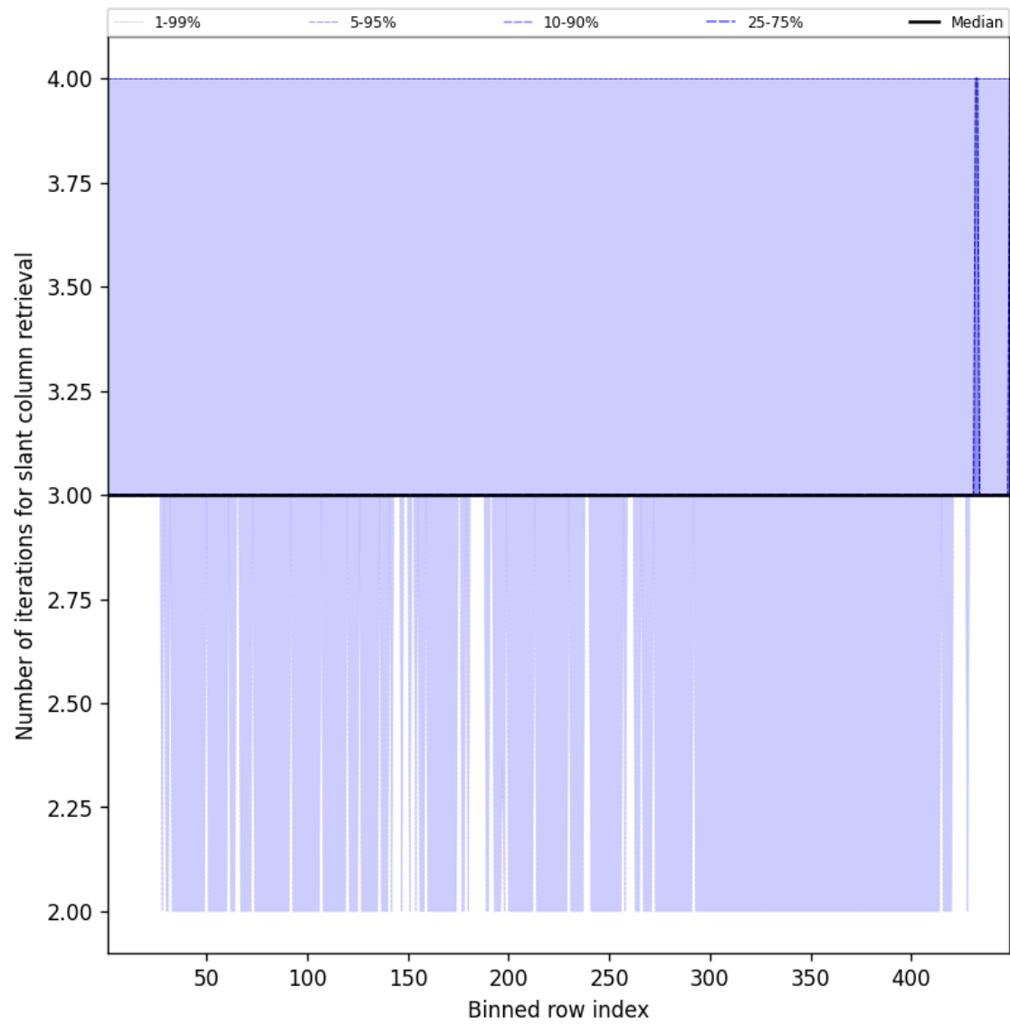
Figure 45: Along track statistics of “Number of iterations for slant column retrieval” for 2025-09-30 to 2025-10-01
