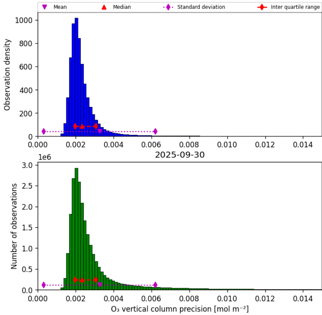
Figure 30: Histogram of “O 3 vertical column precision” for 2025-09-30 to 2025-10-01
