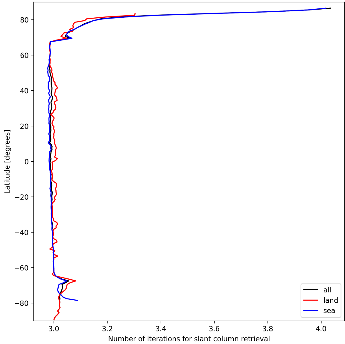
Figure 21: Zonal average of “Number of iterations for slant column retrieval” for 2025-09-30 to 2025-10-01.
