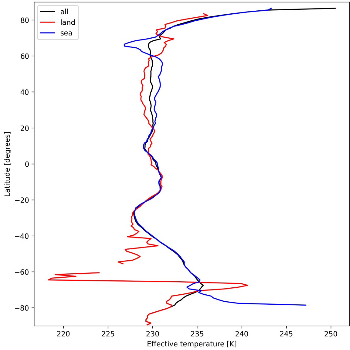
Figure 26: Zonal average of "Effective temperature" for 2025-09-30 to 2025-10-01.
