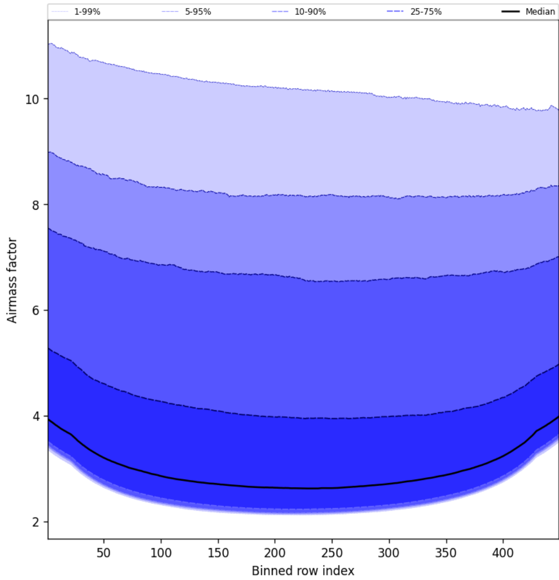
Figure 49: Along track statistics of “Airmass factor” for 2025-09-30 to 2025-10-01
