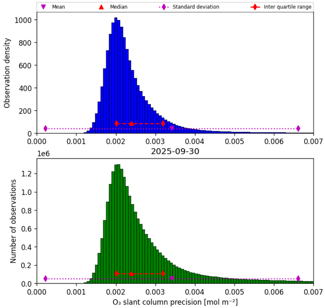
Figure 32: Histogram of “O 3 slant column precision” for 2025-09-30 to 2025-10-01
