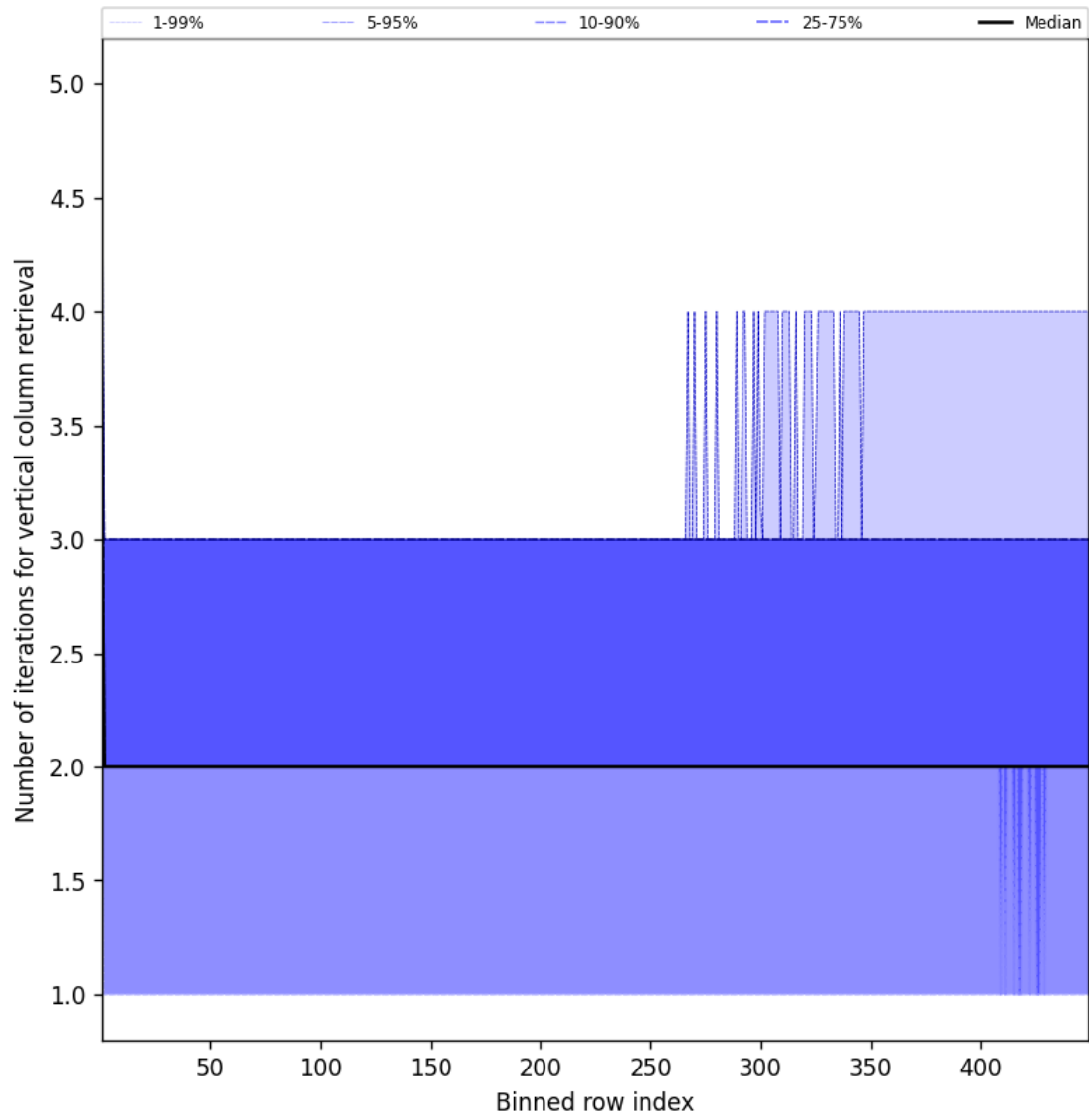
Figure 51: Along track statistics of “Number of iterations for vertical column retrieval” for 2025-09-30 to 2025-10-01
