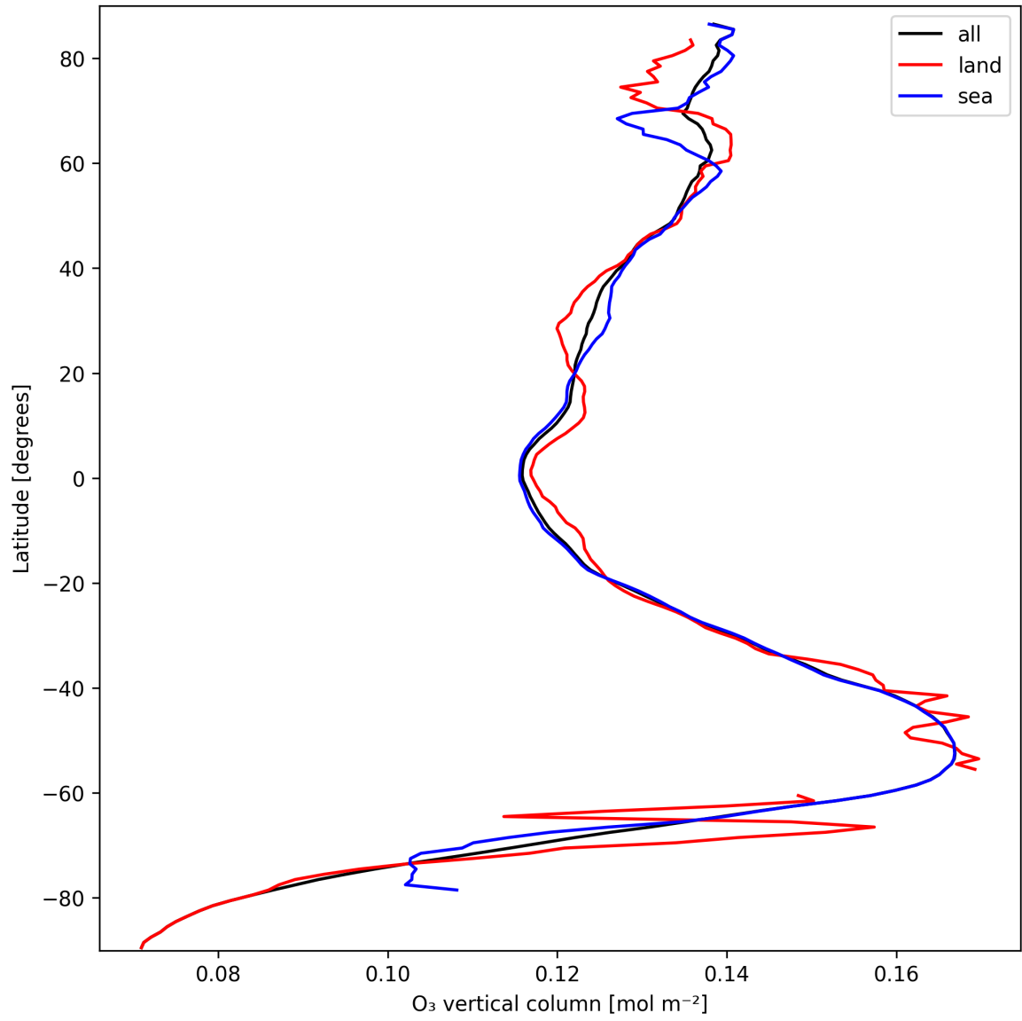
Figure 17: Zonal average of “O 3 vertical column” for 2025-09-30 to 2025-10-01.
