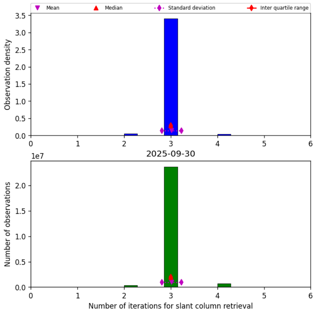
Figure 33: Histogram of “Number of iterations for slant column retrieval” for 2025-09-30 to 2025-10-01
