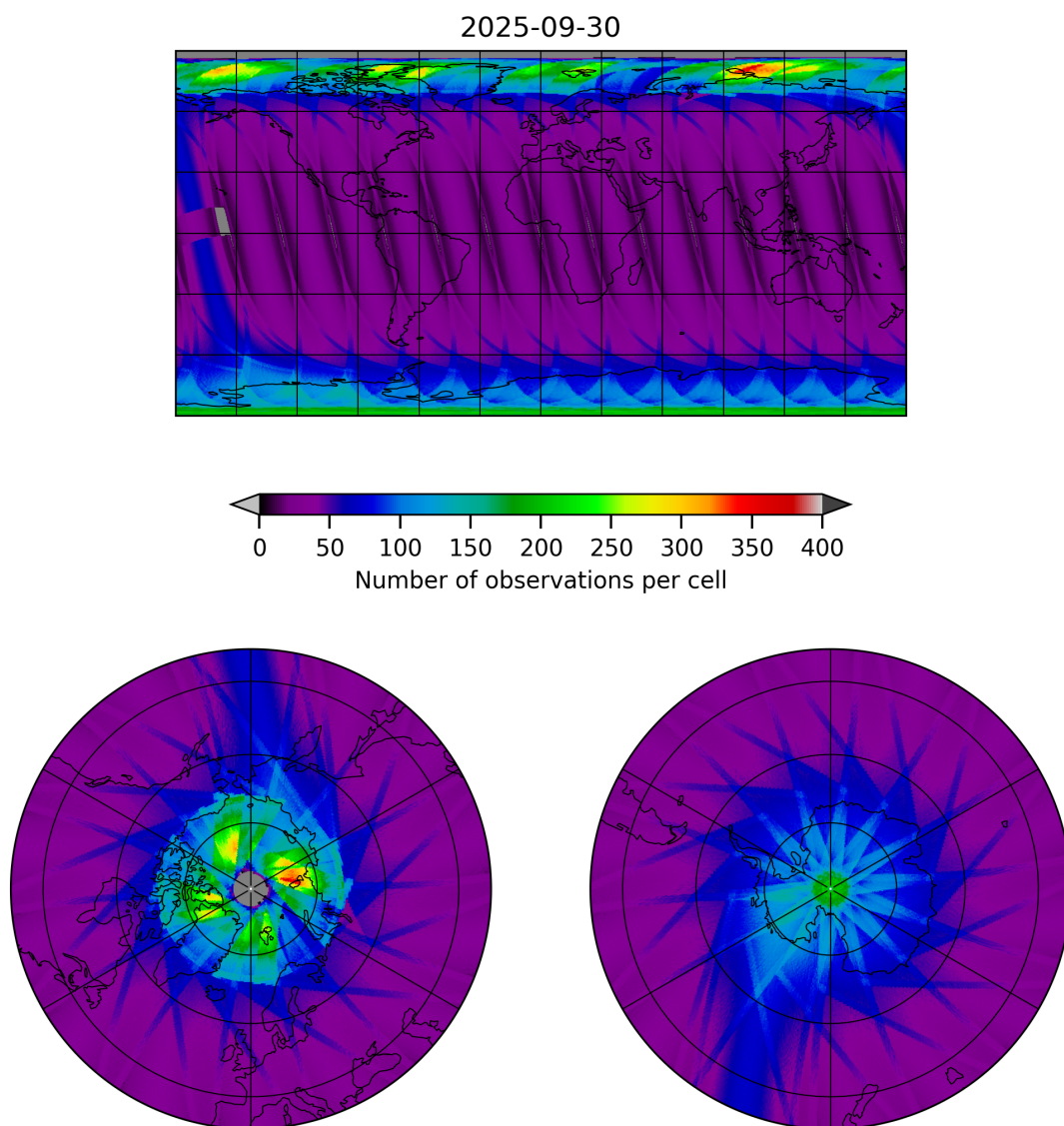
Figure 15: Map of the number of observations for 2025-09-30 to 2025-10-01
