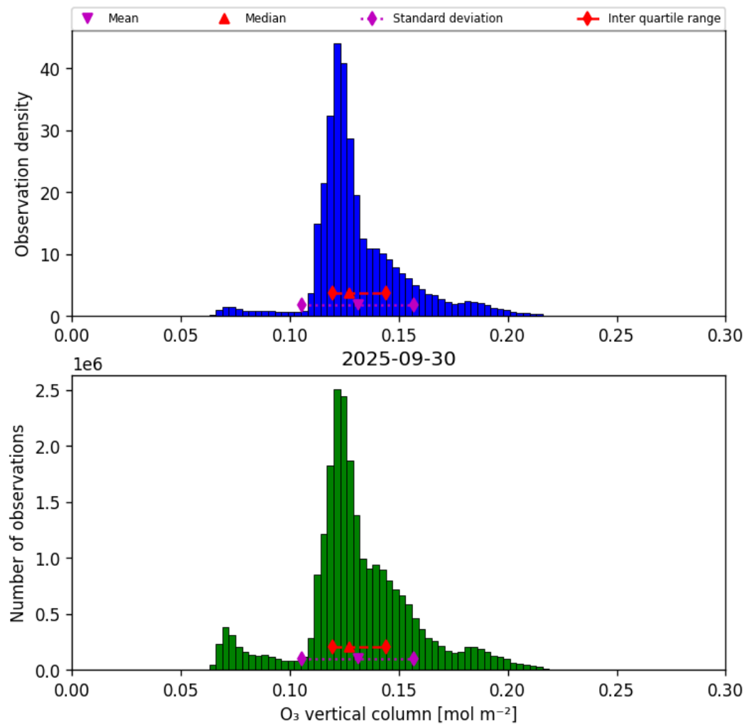
Figure 29: Histogram of “O 3 vertical column” for 2025-09-30 to 2025-10-01
