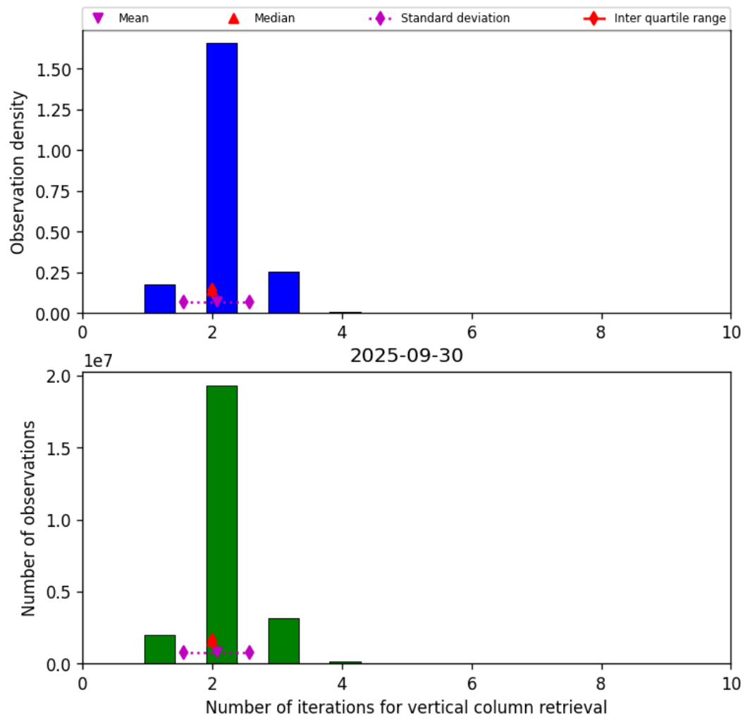
Figure 39: Histogram of “Number of iterations for vertical column retrieval” for 2025-09-30 to 2025-10-01
