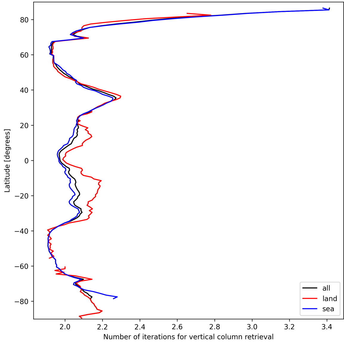
Figure 27: Zonal average of “Number of iterations for vertical column retrieval” for 2025-09-30 to 2025-10-01.
