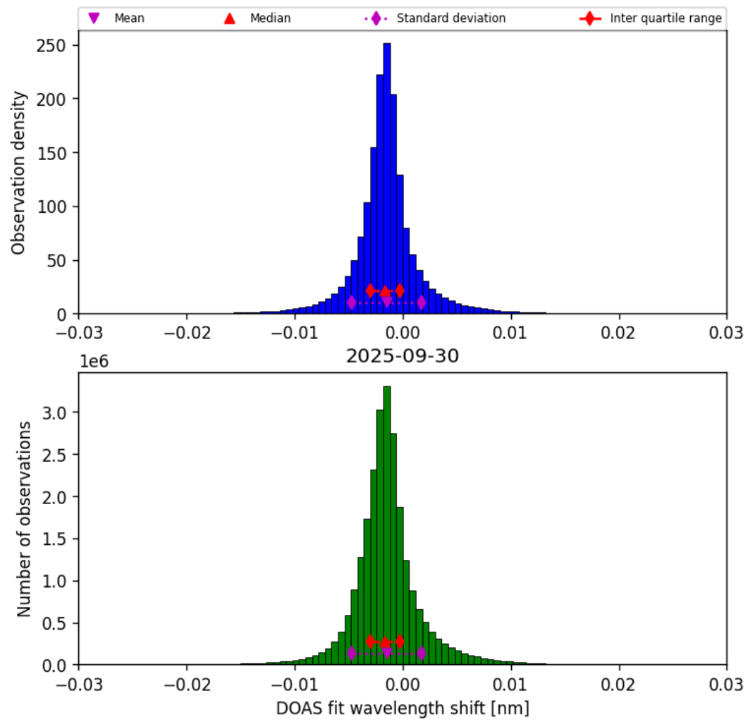
Figure 35: Histogram of “DOAS fit wavelength shift” for 2025-09-30 to 2025-10-01
