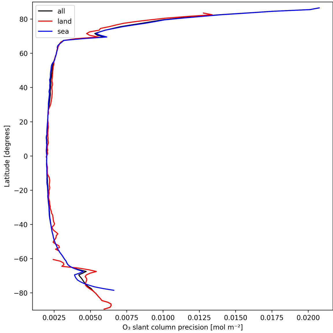
Figure 20: Zonal average of “O 3 slant column precision” for 2025-09-30 to 2025-10-01.
