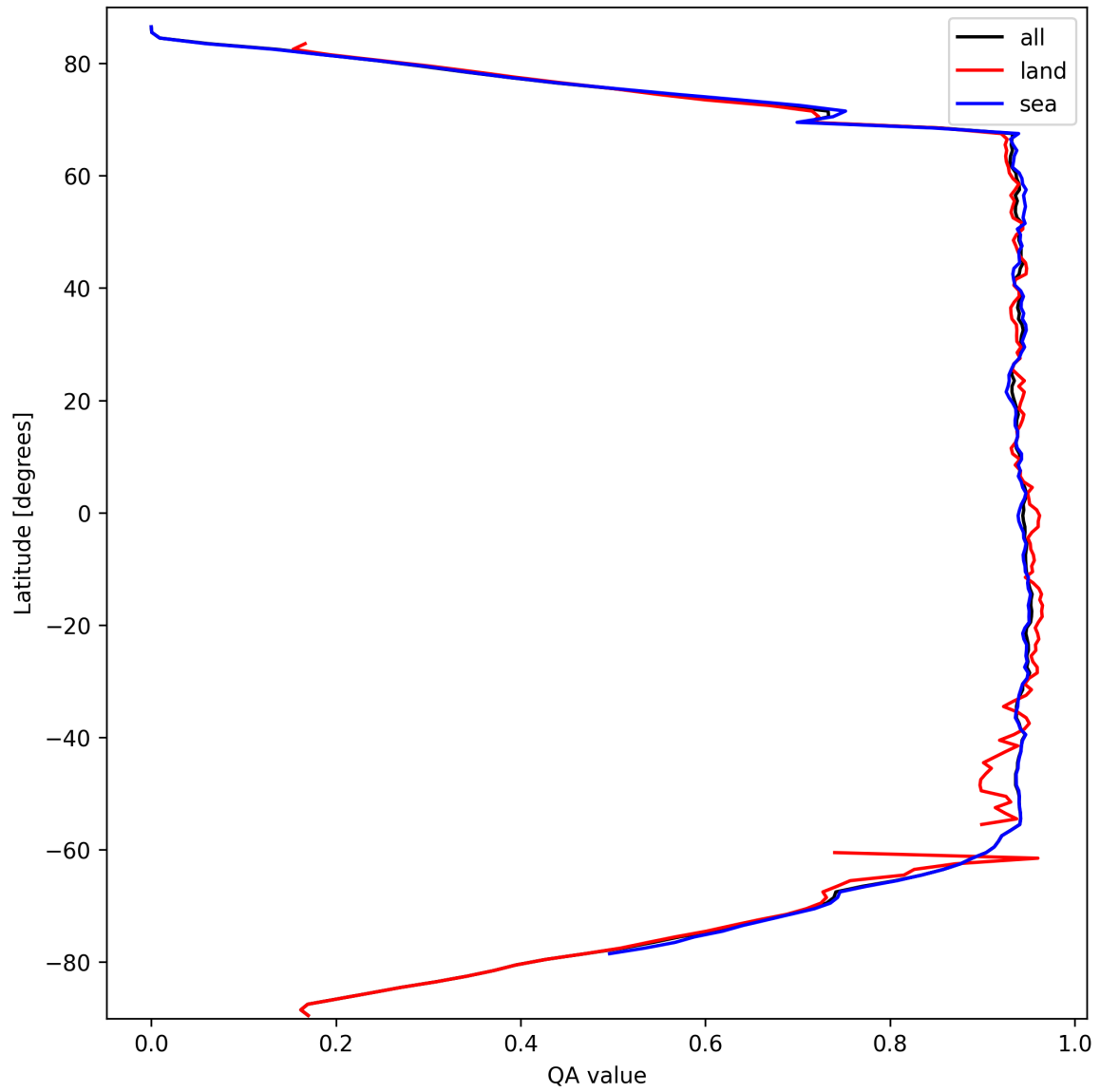
Figure 16: Zonal average of “QA value” for 2025-09-30 to 2025-10-01.
