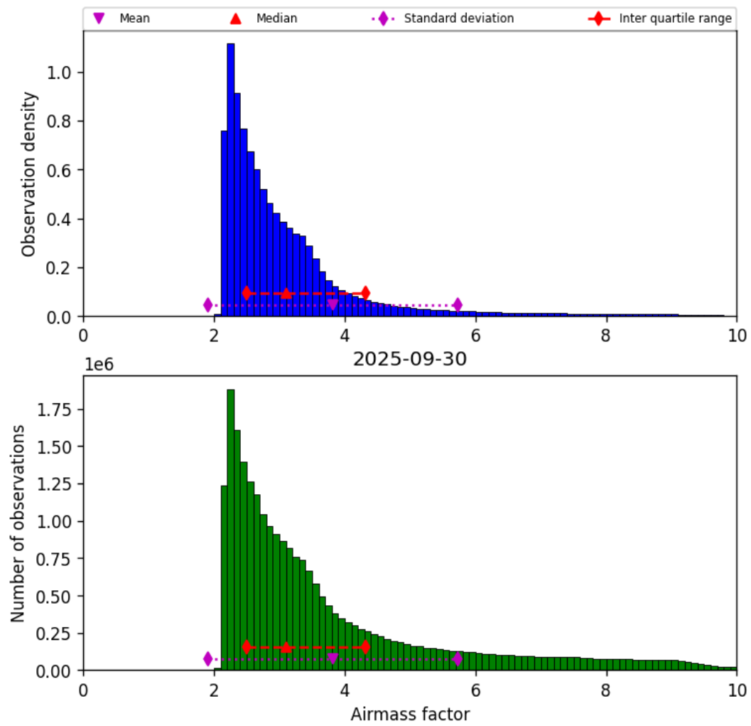
Figure 37: Histogram of “Airmass factor” for 2025-09-30 to 2025-10-01
