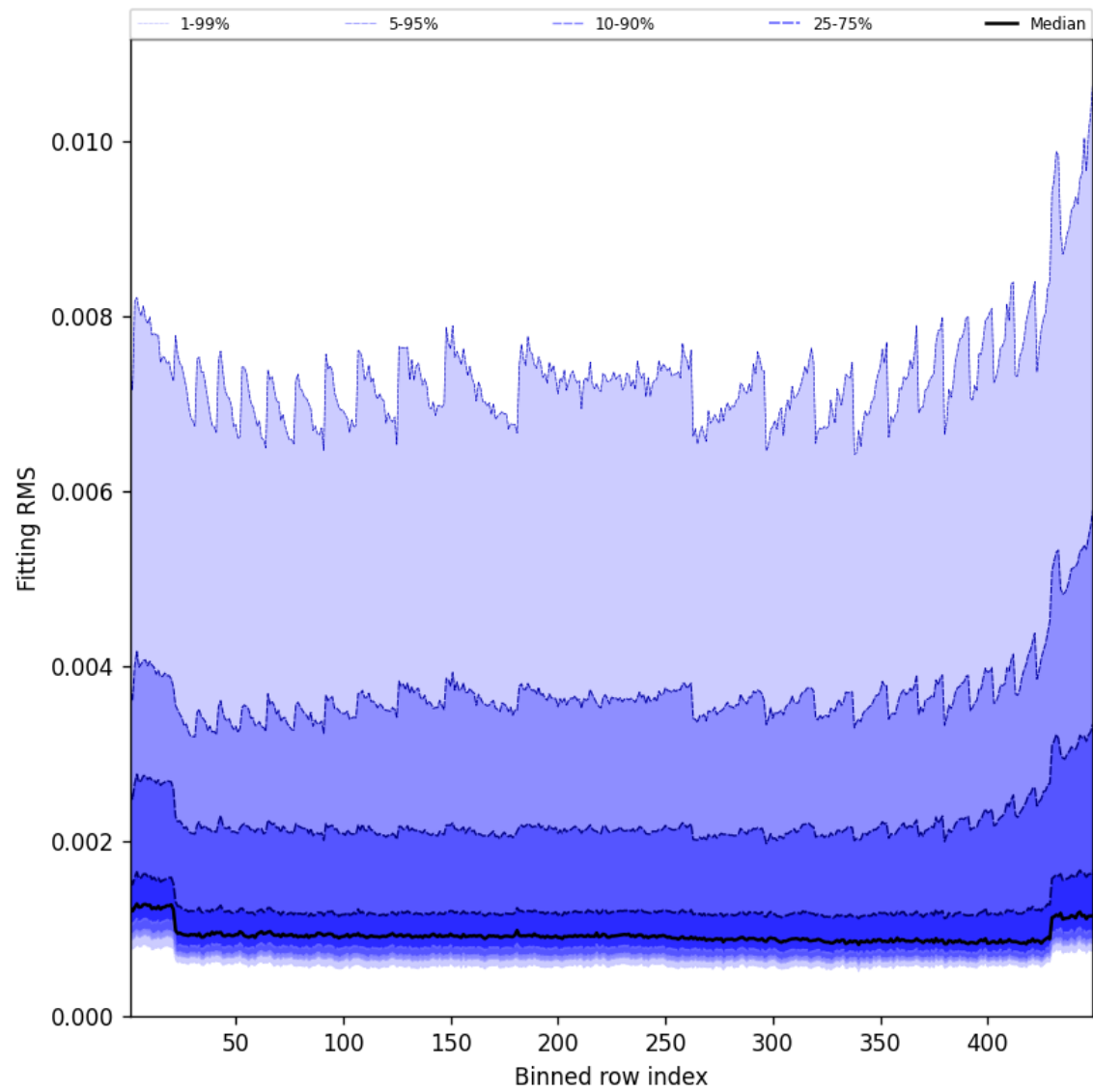
Figure 46: Along track statistics of “Fitting RMS” for 2025-09-30 to 2025-10-01
