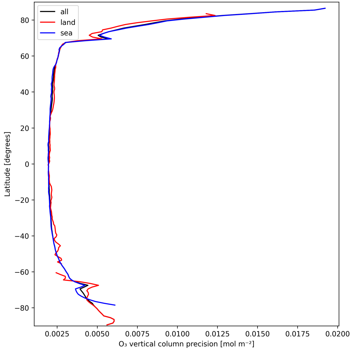
Figure 18: Zonal average of “O 3 vertical column precision” for 2025-09-30 to 2025-10-01.
