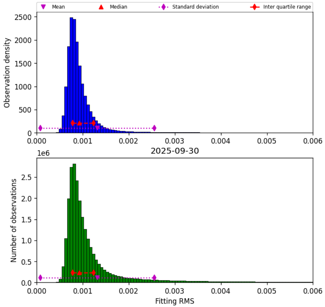
Figure 34: Histogram of “Fitting RMS” for 2025-09-30 to 2025-10-01
