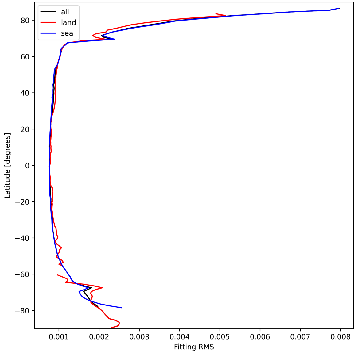
Figure 22: Zonal average of “Fitting RMS” for 2025-09-30 to 2025-10-01.
