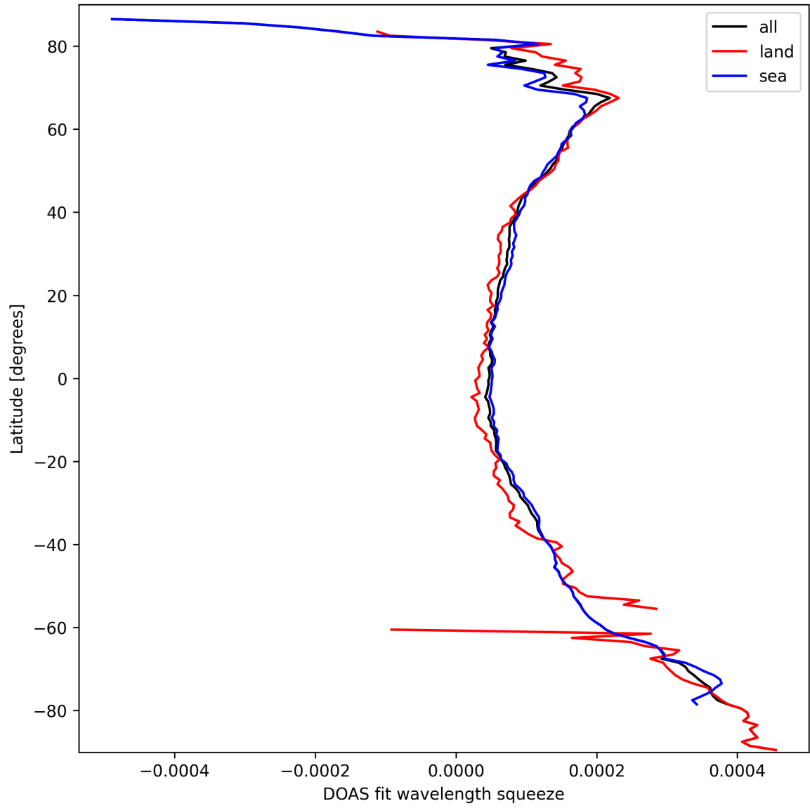
Figure 24: Zonal average of “DOAS fit wavelength squeeze” for 2025-09-30 to 2025-10-01.
