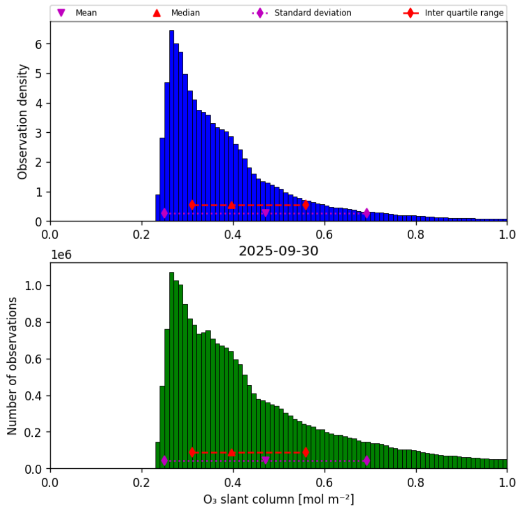
Figure 31: Histogram of “O 3 slant column” for 2025-09-30 to 2025-10-01
