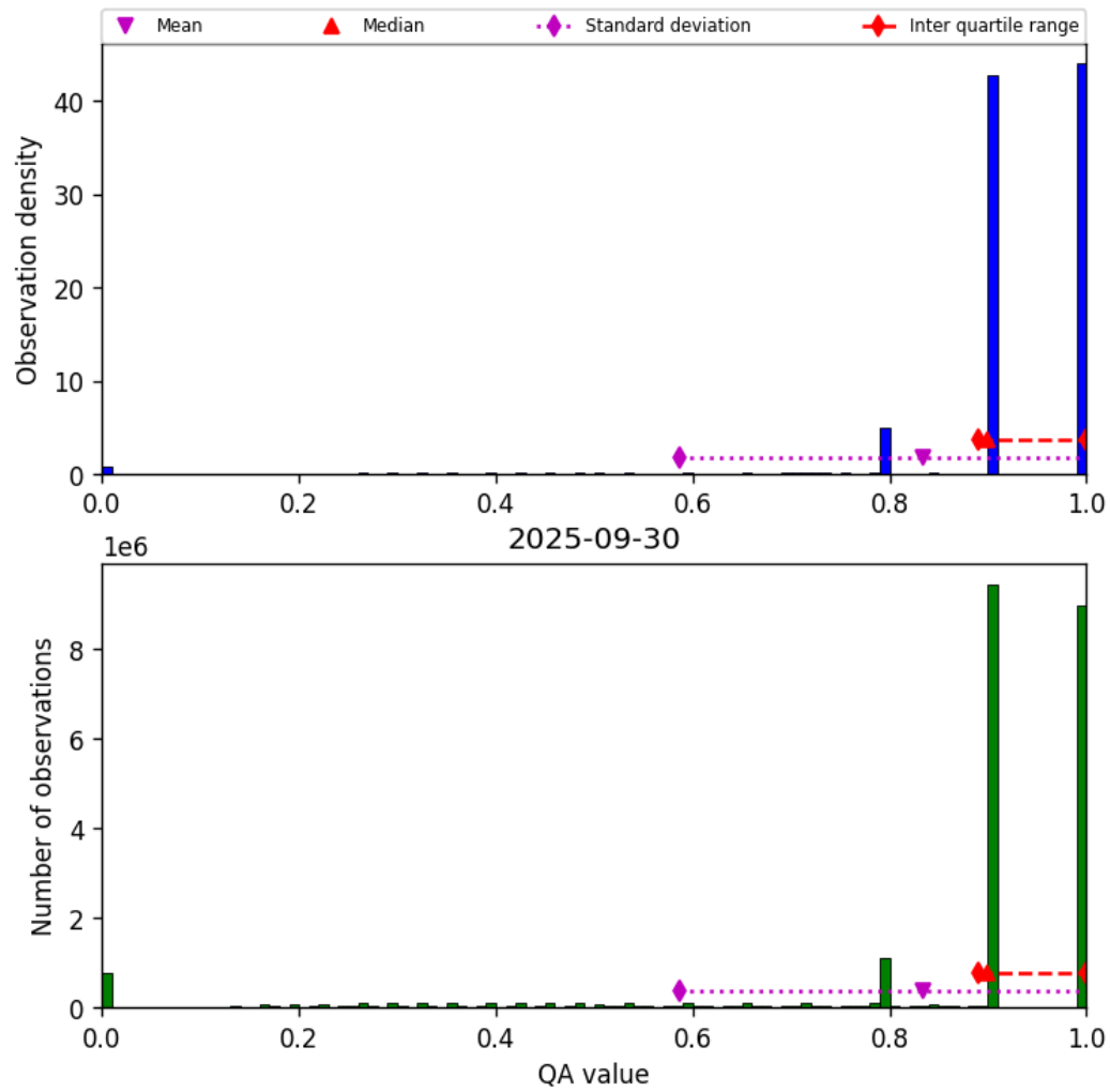
Figure 28: Histogram of “QA value” for 2025-09-30 to 2025-10-01
