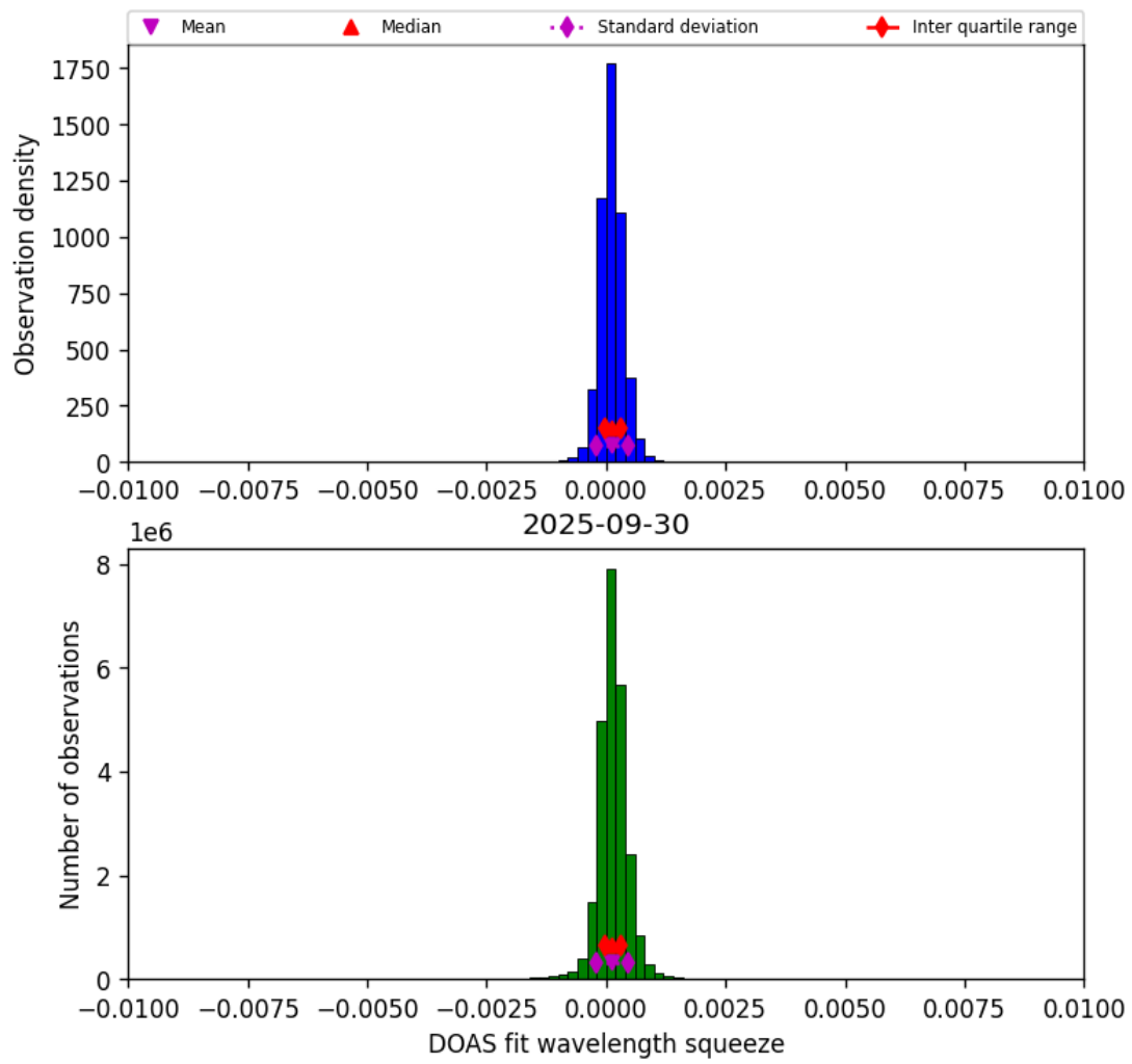
Figure 36: Histogram of “DOAS fit wavelength squeeze” for 2025-09-30 to 2025-10-01
