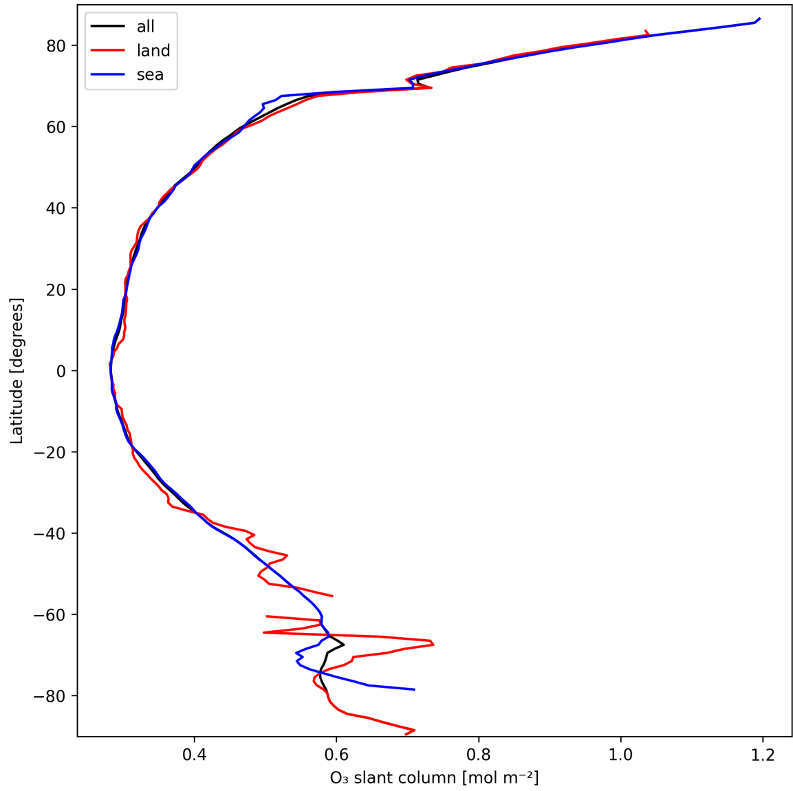
Figure 19: Zonal average of “O 3 slant column” for 2025-09-30 to 2025-10-01.
