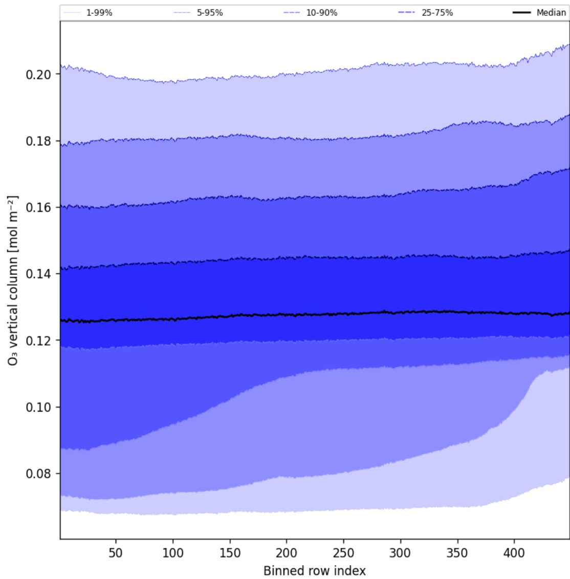
Figure 41: Along track statistics of “O 3 vertical column” for 2025-09-30 to 2025-10-01
