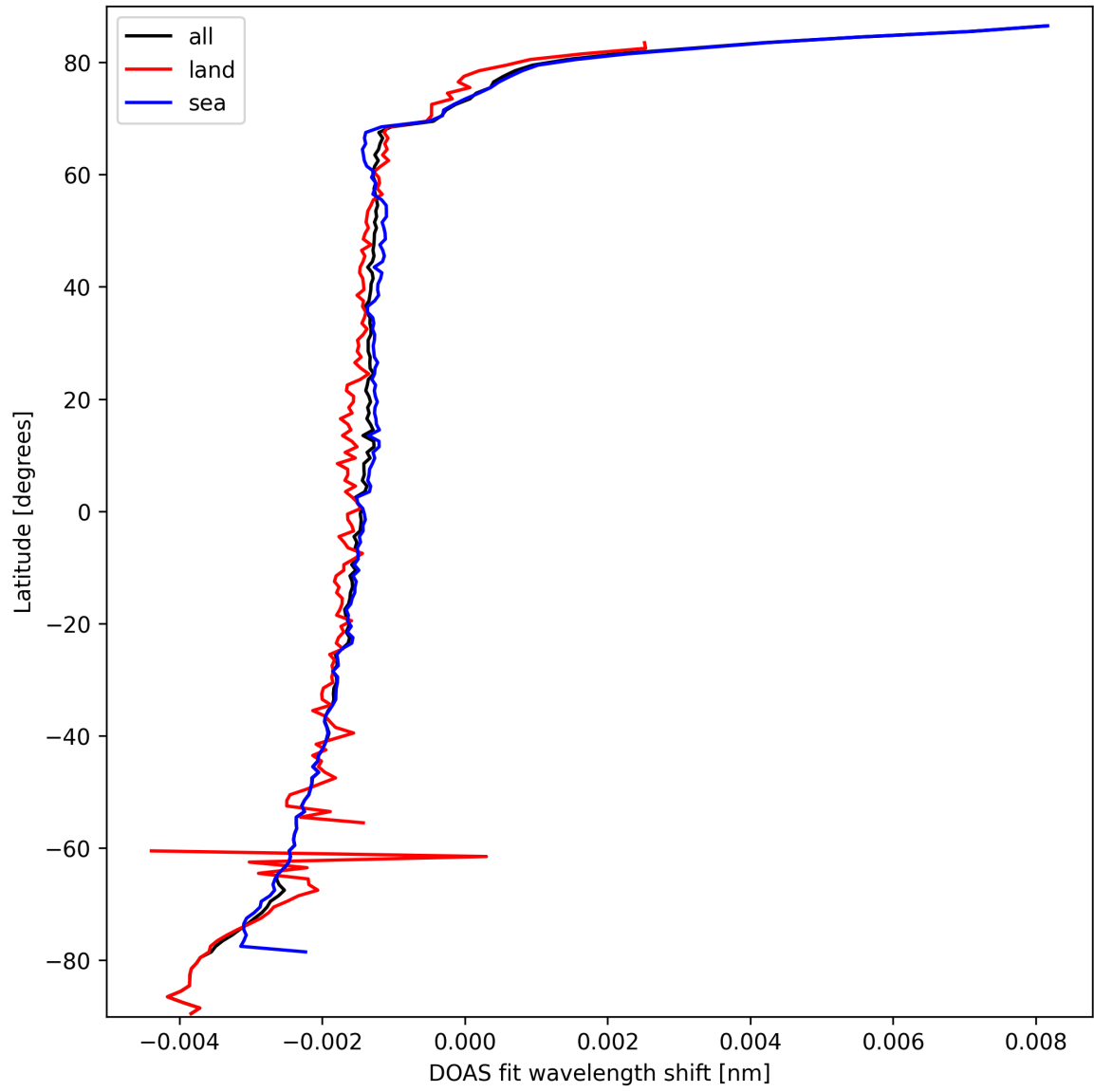
Figure 23: Zonal average of “DOAS fit wavelength shift” for 2025-09-30 to 2025-10-01.
