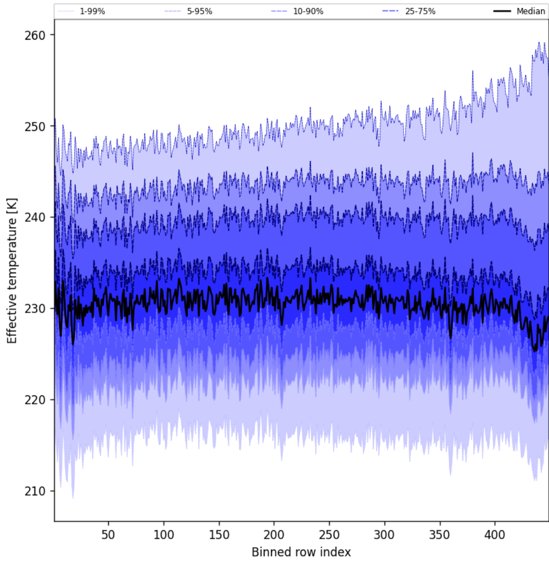
Figure 50: Along track statistics of “Effective temperature” for 2025-09-30 to 2025-10-01
