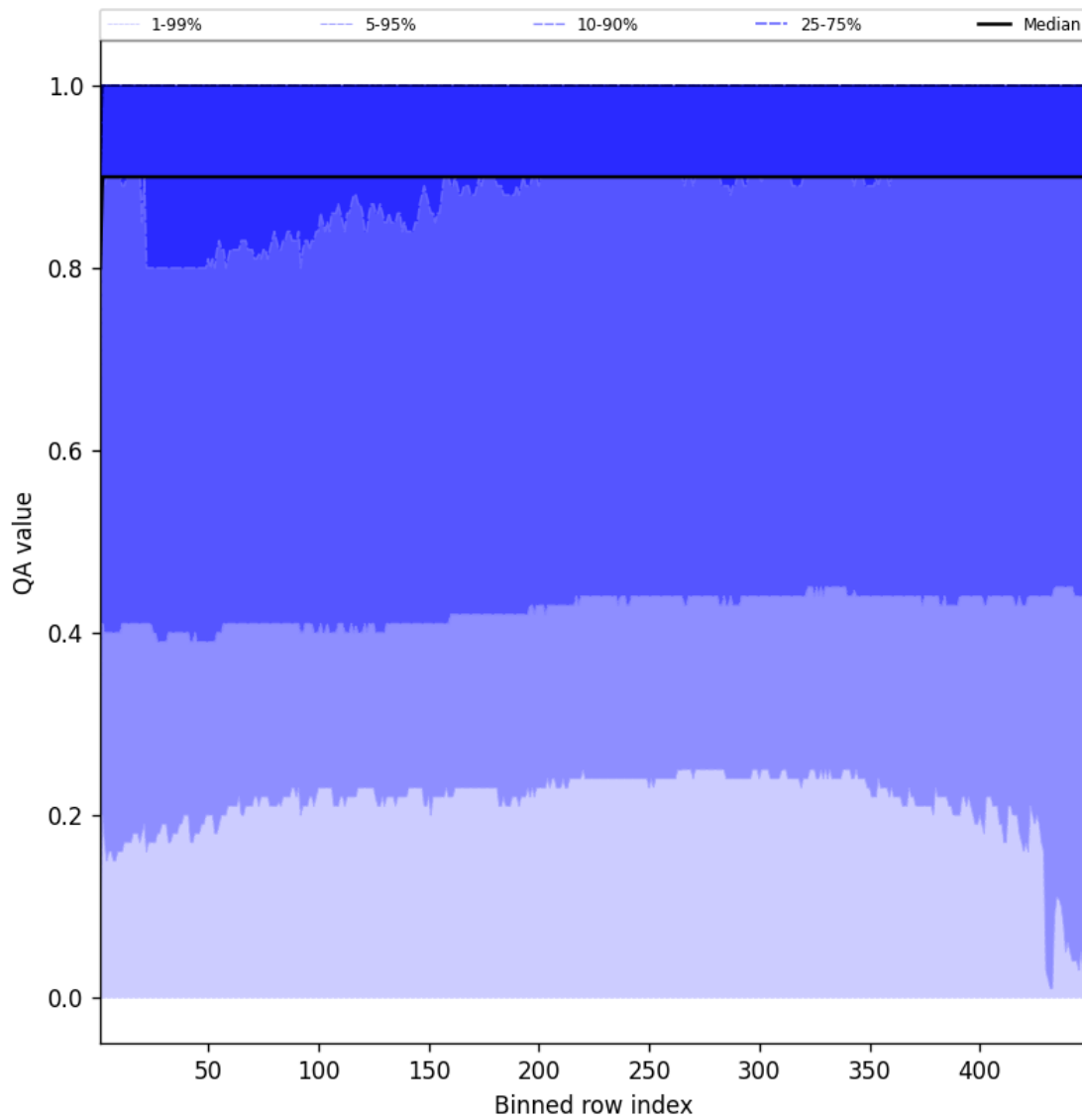
Figure 40: Along track statistics of “QA value” for 2025-09-30 to 2025-10-01
