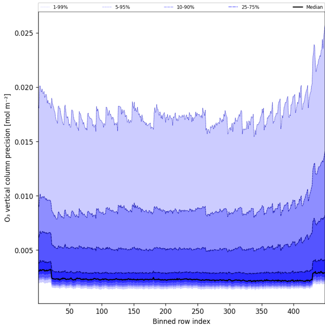
Figure 42: Along track statistics of “O 3 vertical column precision” for 2025-09-30 to 2025-10-01
