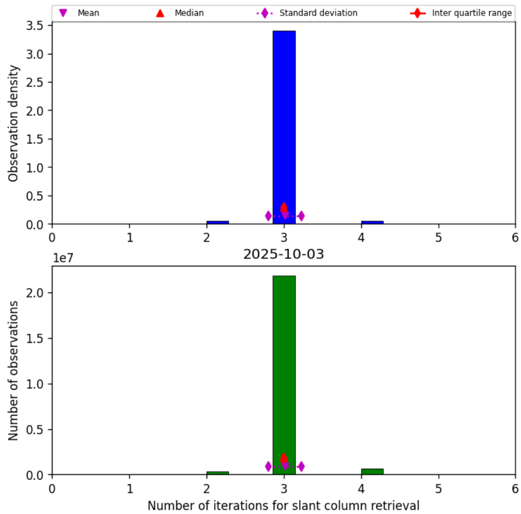
Figure 33: Histogram of “Number of iterations for slant column retrieval” for 2025-10-03 to 2025-10-04
