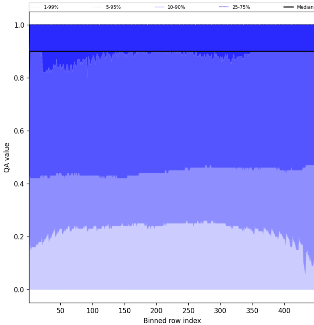
Figure 40: Along track statistics of “QA value” for 2025-10-03 to 2025-10-04
