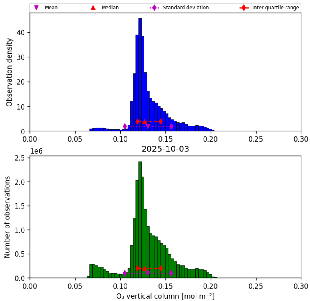
Figure 29: Histogram of “O 3 vertical column” for 2025-10-03 to 2025-10-04
