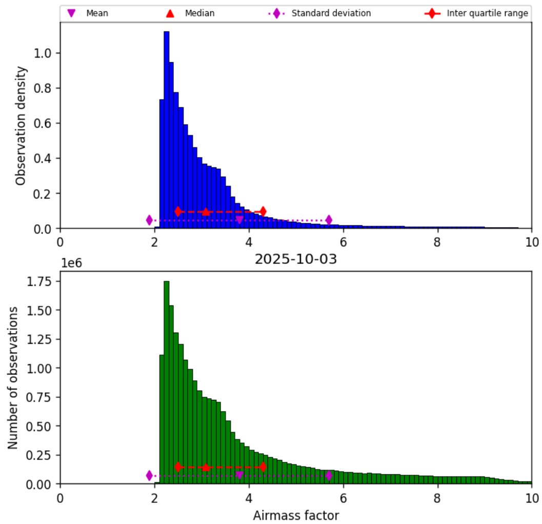
Figure 37: Histogram of “Airmass factor” for 2025-10-03 to 2025-10-04
