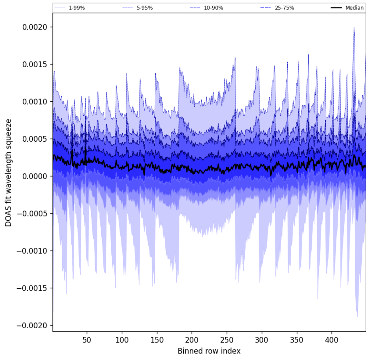
Figure 48: Along track statistics of “DOAS fit wavelength squeeze” for 2025-10-03 to 2025-10-04
