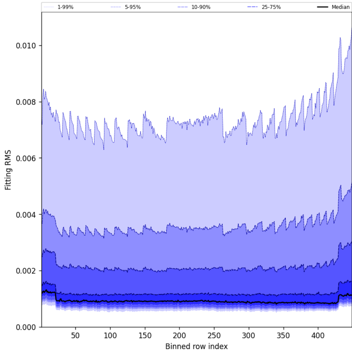
Figure 46: Along track statistics of “Fitting RMS” for 2025-10-03 to 2025-10-04
