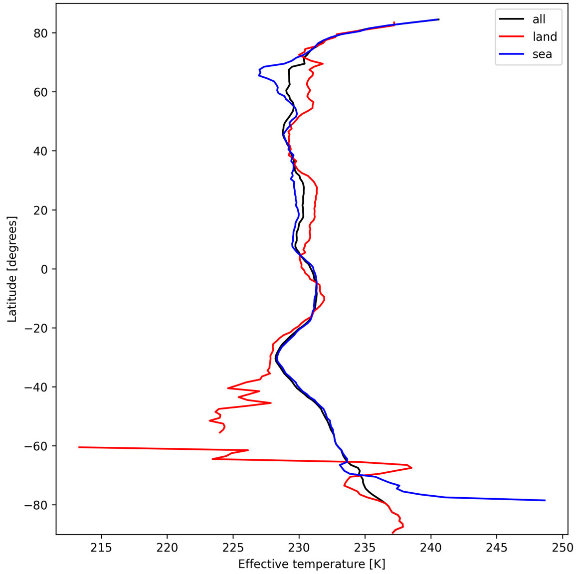
Figure 26: Zonal average of "Effective temperature" for 2025-10-03 to 2025-10-04.
