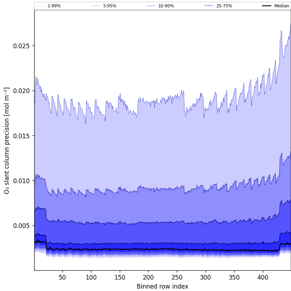
Figure 44: Along track statistics of “O 3 slant column precision” for 2025-10-03 to 2025-10-04
