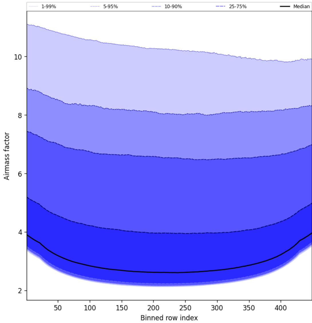
Figure 49: Along track statistics of “Airmass factor” for 2025-10-03 to 2025-10-04
