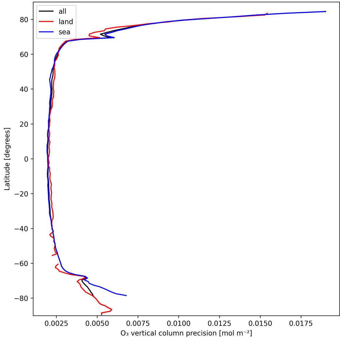
Figure 18: Zonal average of “O 3 vertical column precision” for 2025-10-03 to 2025-10-04.
