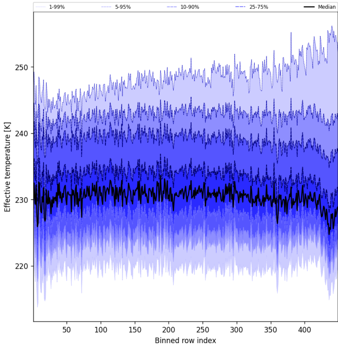
Figure 50: Along track statistics of “Effective temperature” for 2025-10-03 to 2025-10-04
