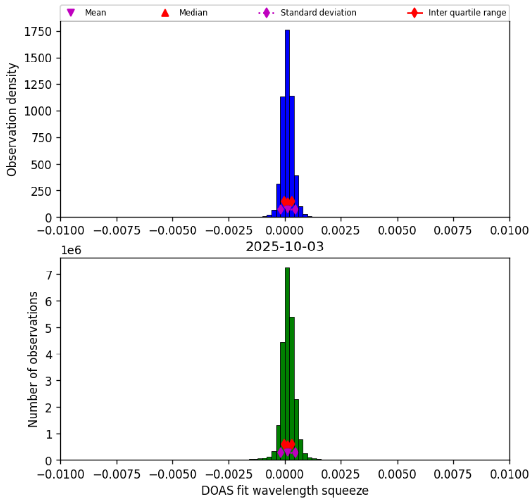
Figure 36: Histogram of “DOAS fit wavelength squeeze” for 2025-10-03 to 2025-10-04
