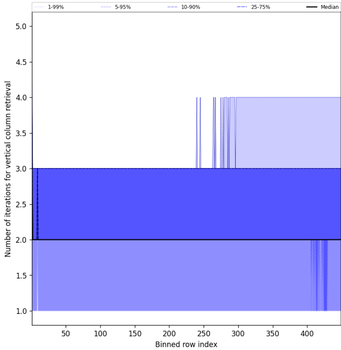
Figure 51: Along track statistics of “Number of iterations for vertical column retrieval” for 2025-10-03 to 2025-10-04
