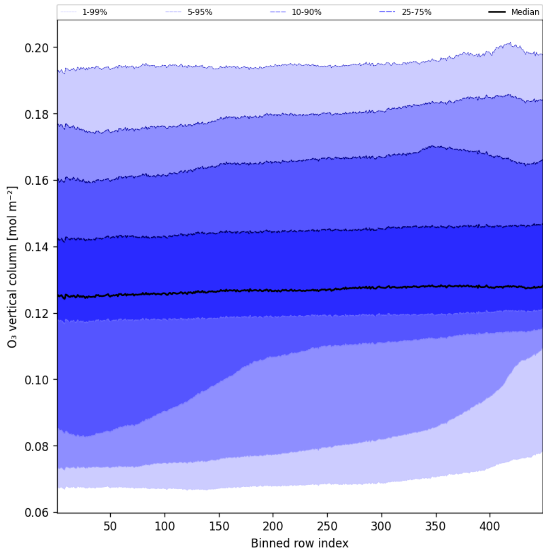
Figure 41: Along track statistics of “O 3 vertical column” for 2025-10-03 to 2025-10-04
