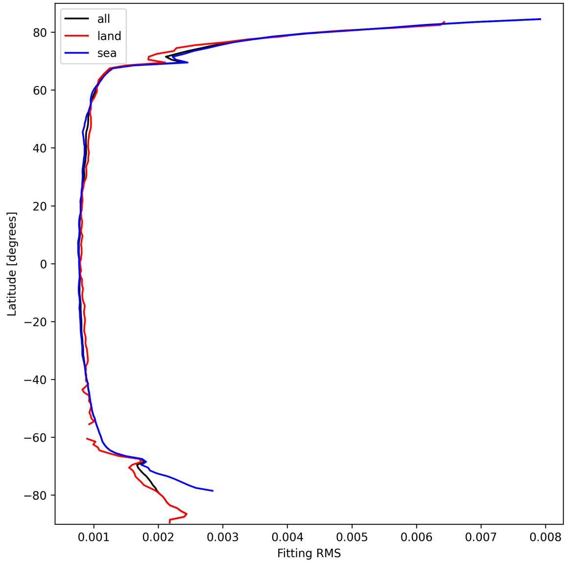
Figure 22: Zonal average of “Fitting RMS” for 2025-10-03 to 2025-10-04.
