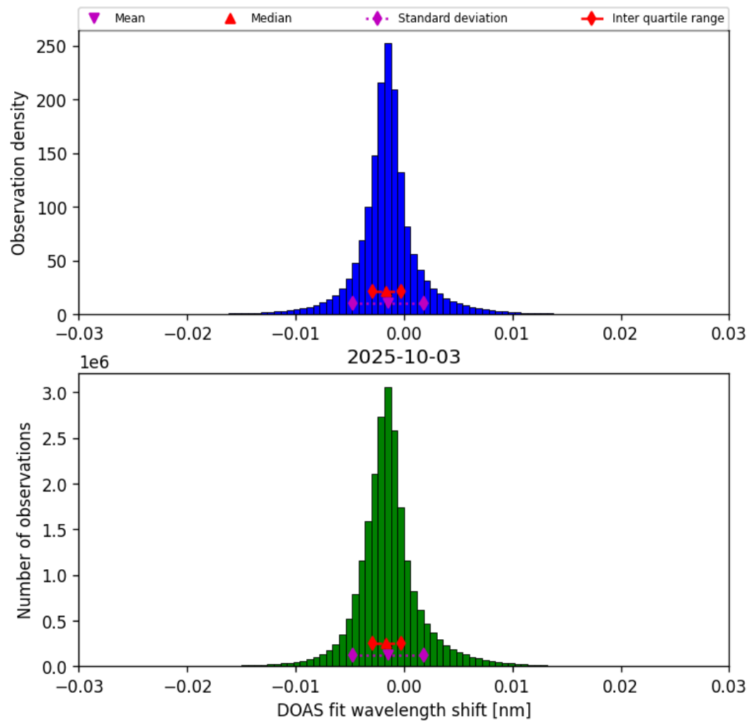
Figure 35: Histogram of “DOAS fit wavelength shift” for 2025-10-03 to 2025-10-04
