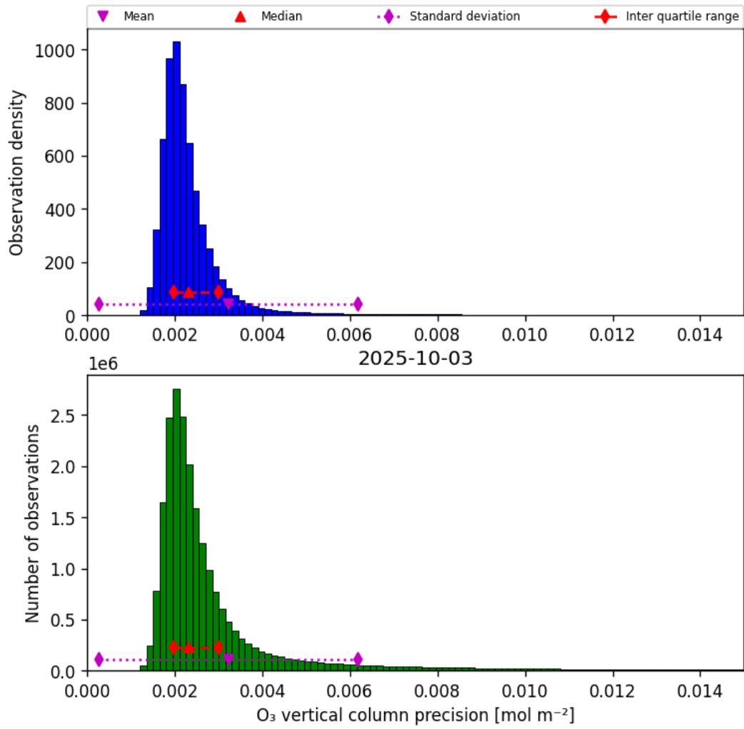
Figure 30: Histogram of “O 3 vertical column precision” for 2025-10-03 to 2025-10-04
