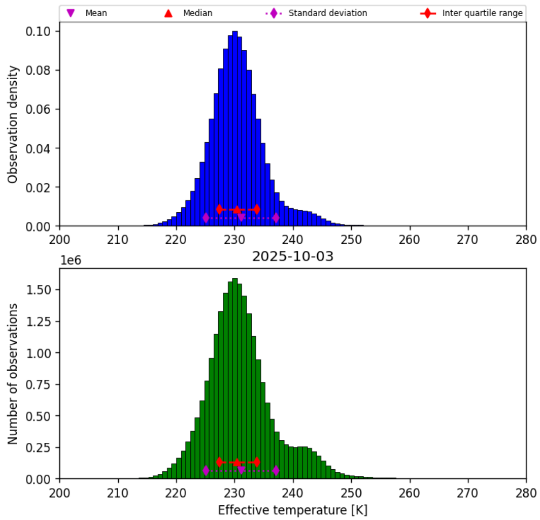
Figure 38: Histogram of “Effective temperature” for 2025-10-03 to 2025-10-04
