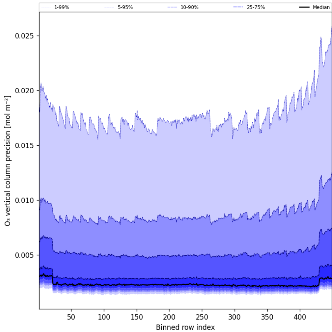
Figure 42: Along track statistics of “O 3 vertical column precision” for 2025-10-03 to 2025-10-04
