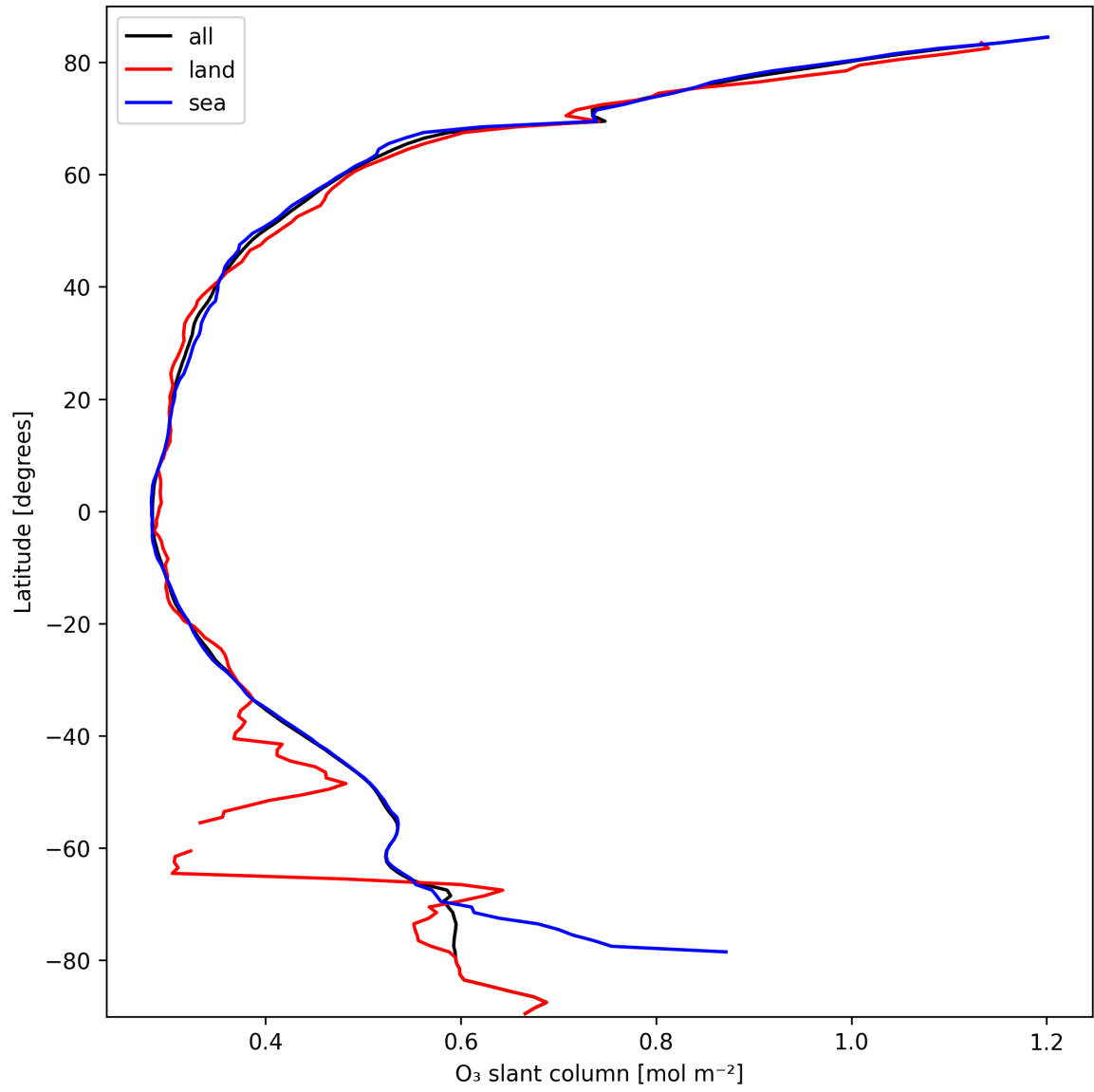
Figure 19: Zonal average of “O 3 slant column” for 2025-10-03 to 2025-10-04.
