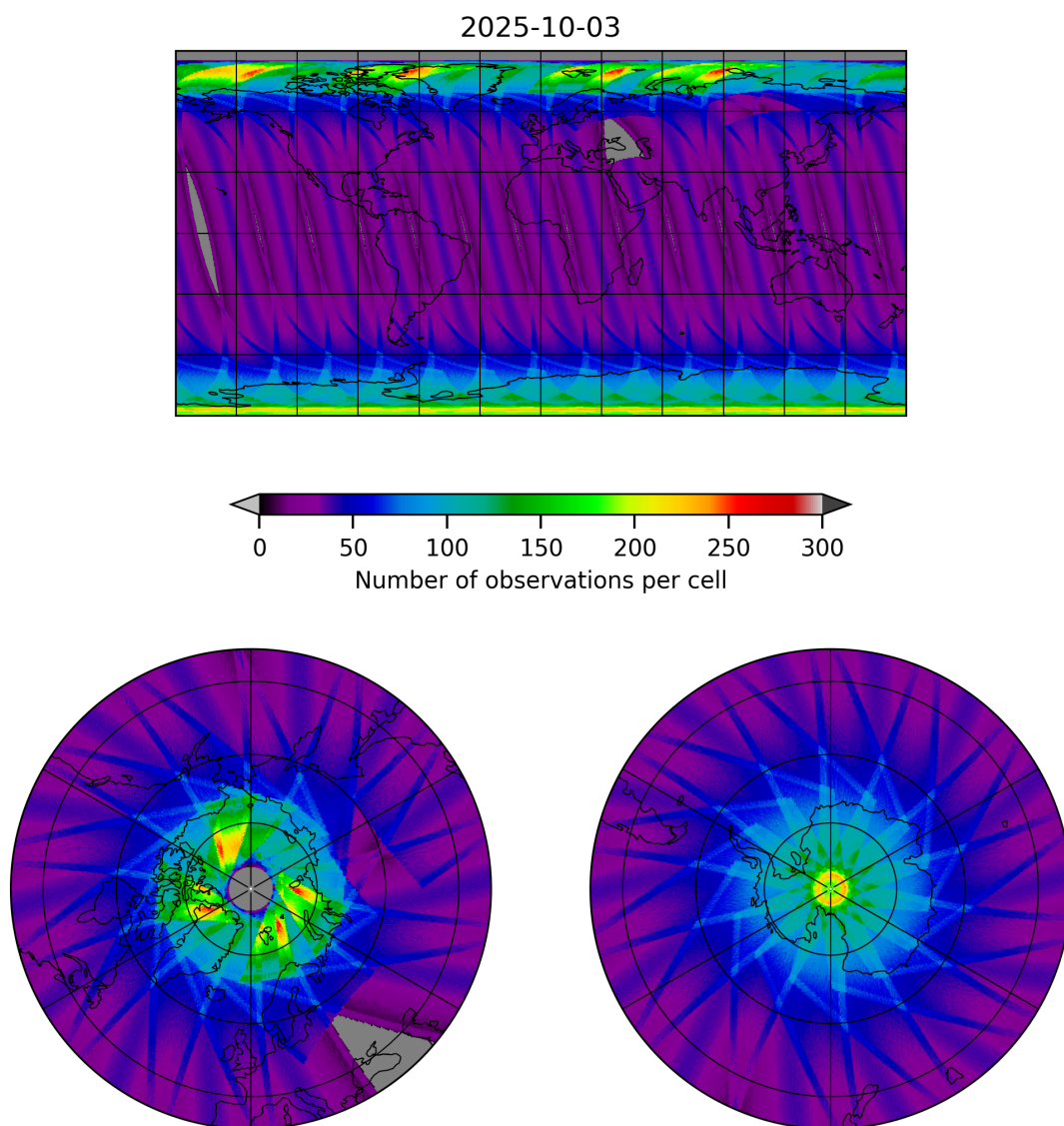
Figure 15: Map of the number of observations for 2025-10-03 to 2025-10-04
