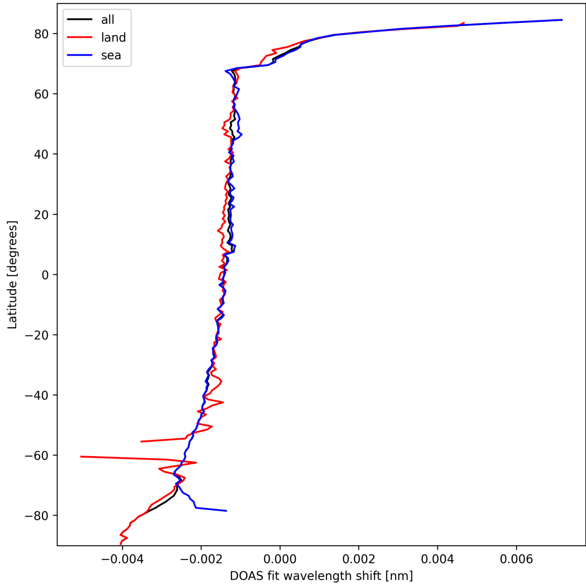
Figure 23: Zonal average of “DOAS fit wavelength shift” for 2025-10-03 to 2025-10-04.
