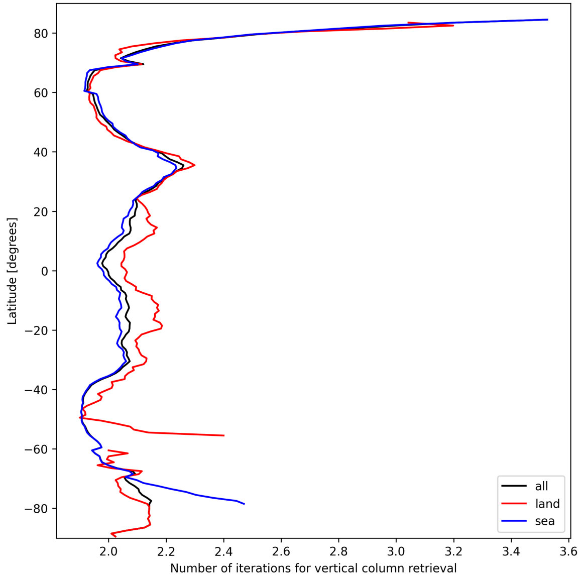
Figure 27: Zonal average of “Number of iterations for vertical column retrieval” for 2025-10-03 to 2025-10-04.
