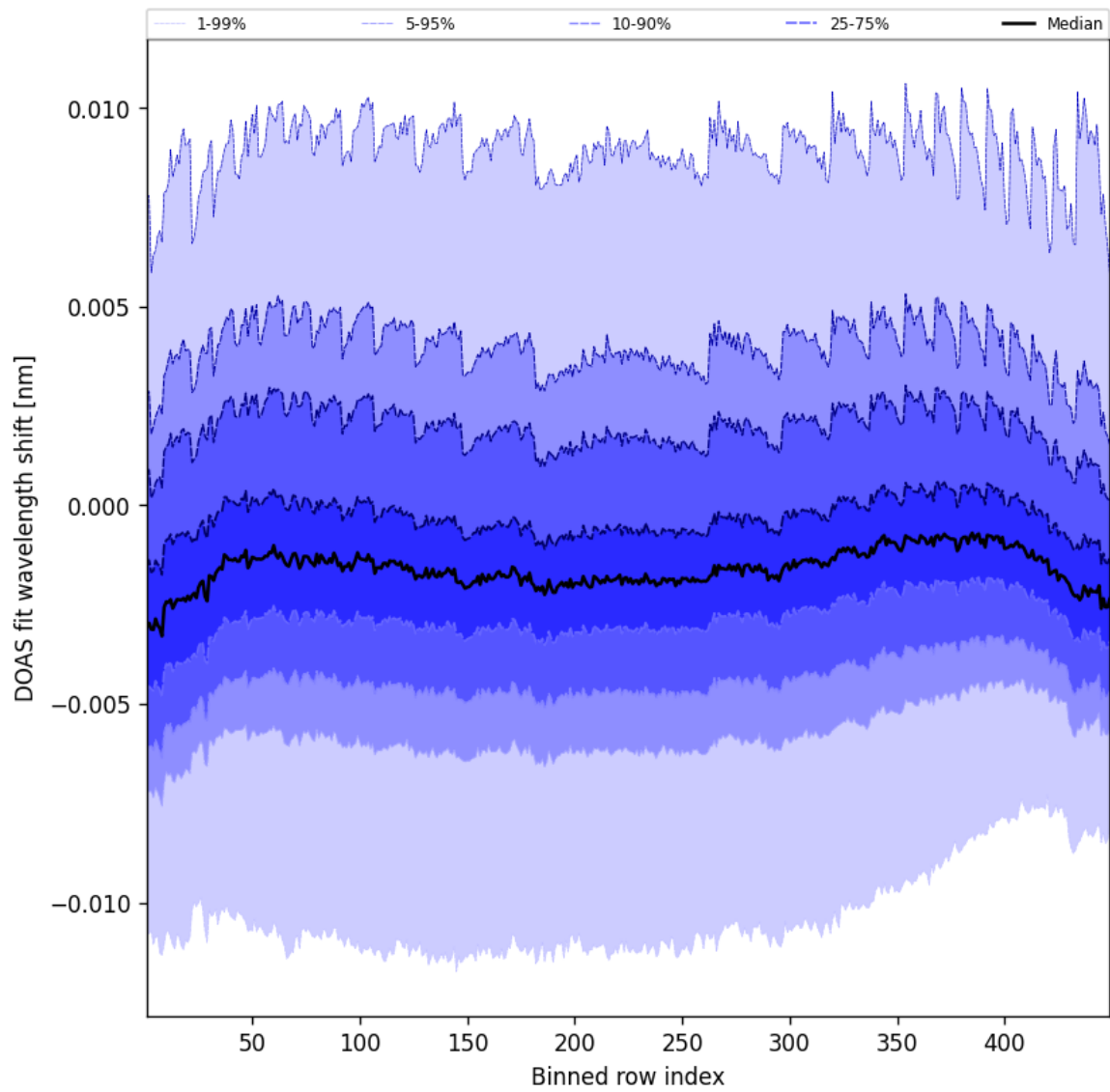
Figure 47: Along track statistics of “DOAS fit wavelength shift” for 2025-10-03 to 2025-10-04
