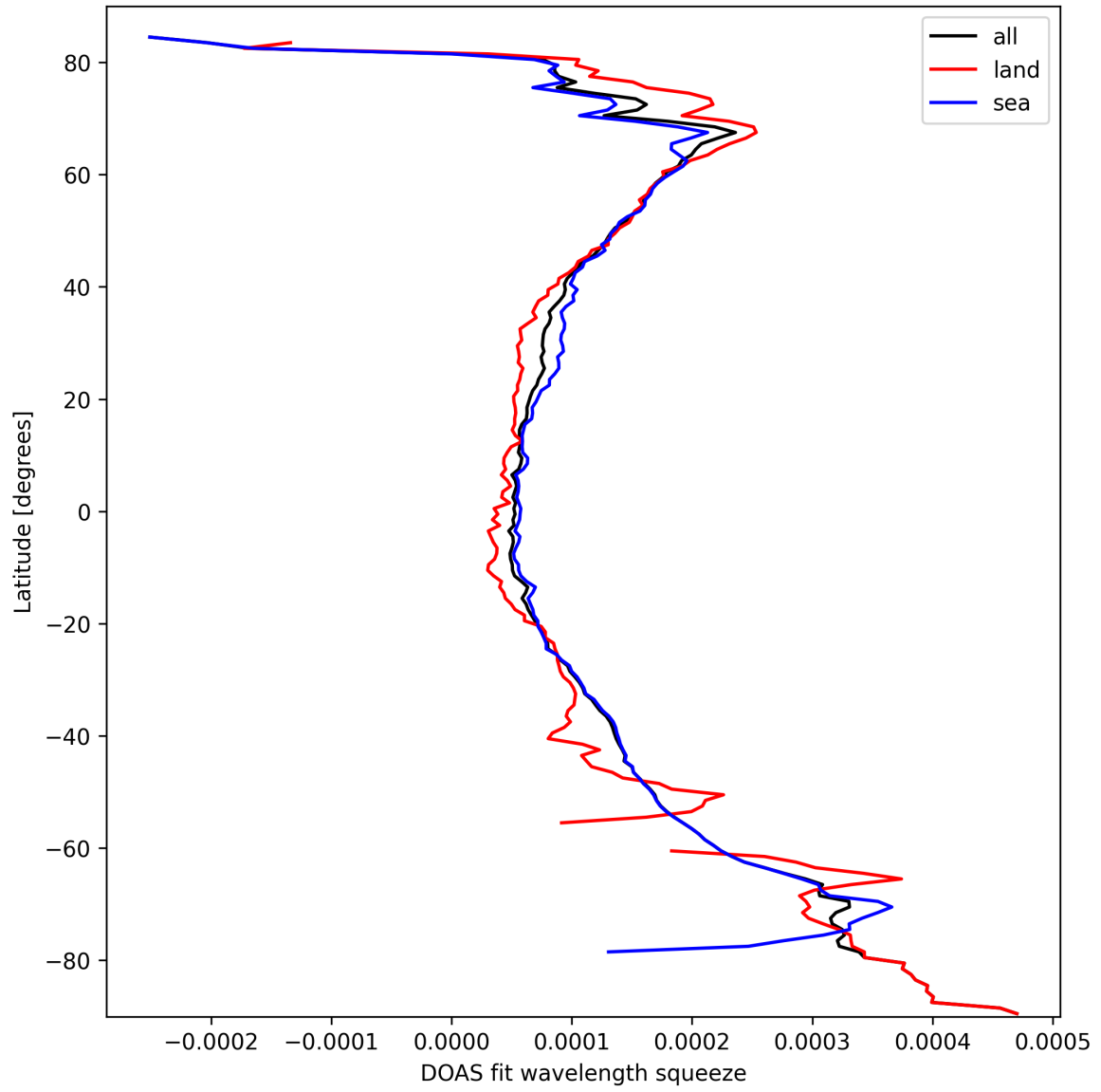
Figure 24: Zonal average of “DOAS fit wavelength squeeze” for 2025-10-03 to 2025-10-04.
