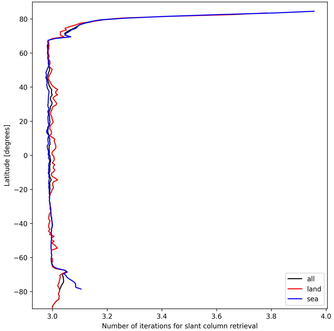
Figure 21: Zonal average of “Number of iterations for slant column retrieval” for 2025-10-03 to 2025-10-04.
