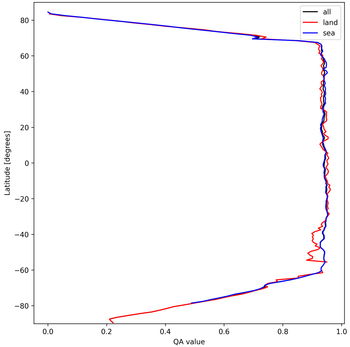
Figure 16: Zonal average of “QA value” for 2025-10-03 to 2025-10-04.
