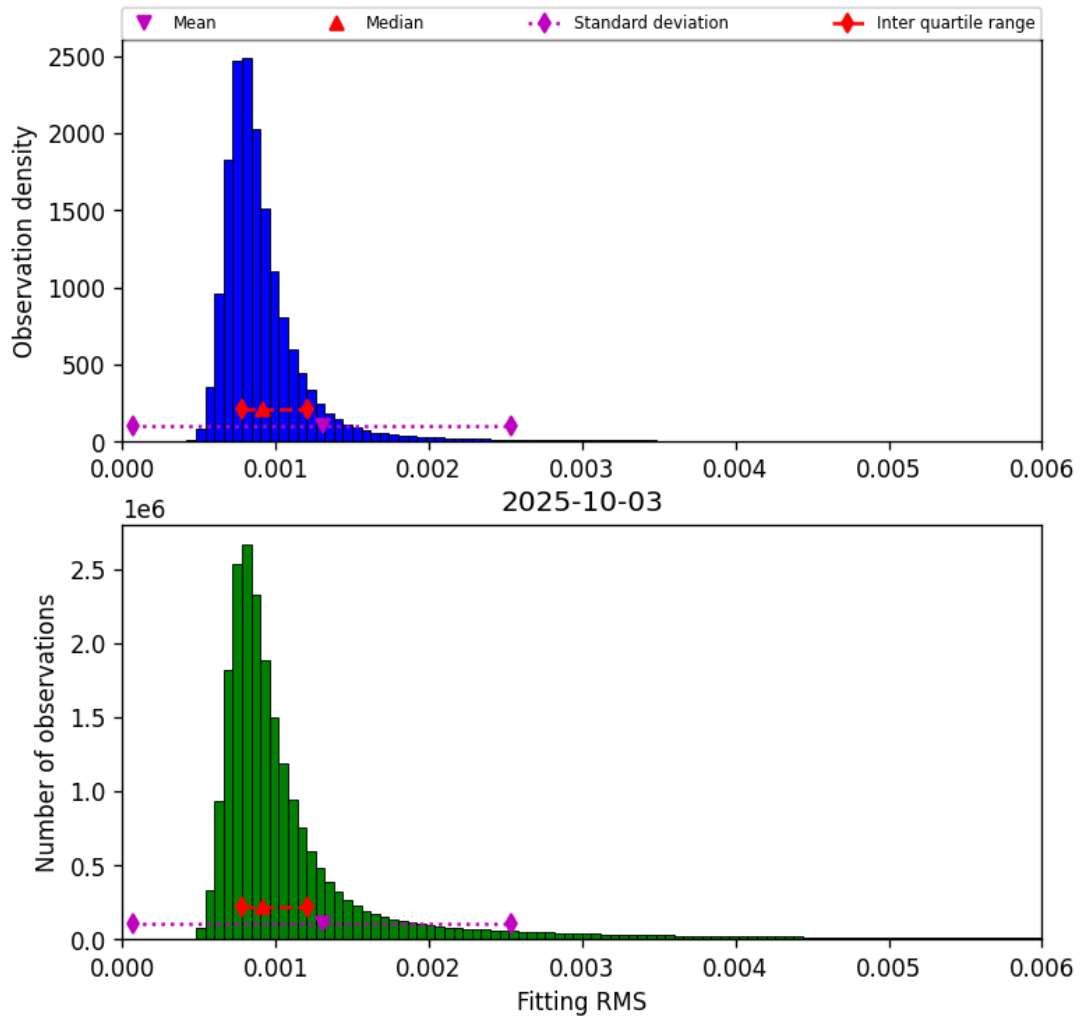
Figure 34: Histogram of “Fitting RMS” for 2025-10-03 to 2025-10-04
