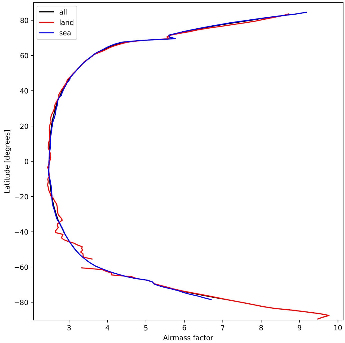
Figure 25: Zonal average of “Airmass factor” for 2025-10-03 to 2025-10-04.
