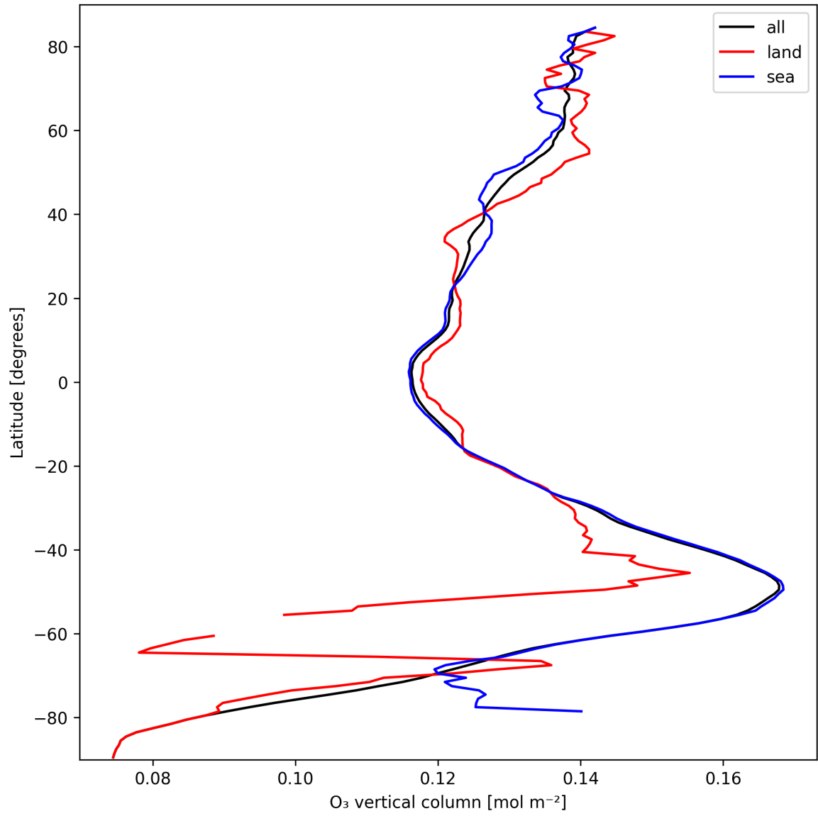
Figure 17: Zonal average of “O 3 vertical column” for 2025-10-03 to 2025-10-04.
