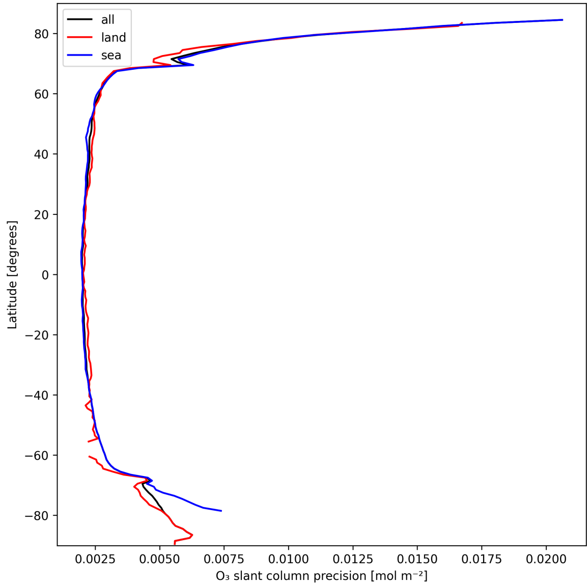
Figure 20: Zonal average of “O 3 slant column precision” for 2025-10-03 to 2025-10-04.
