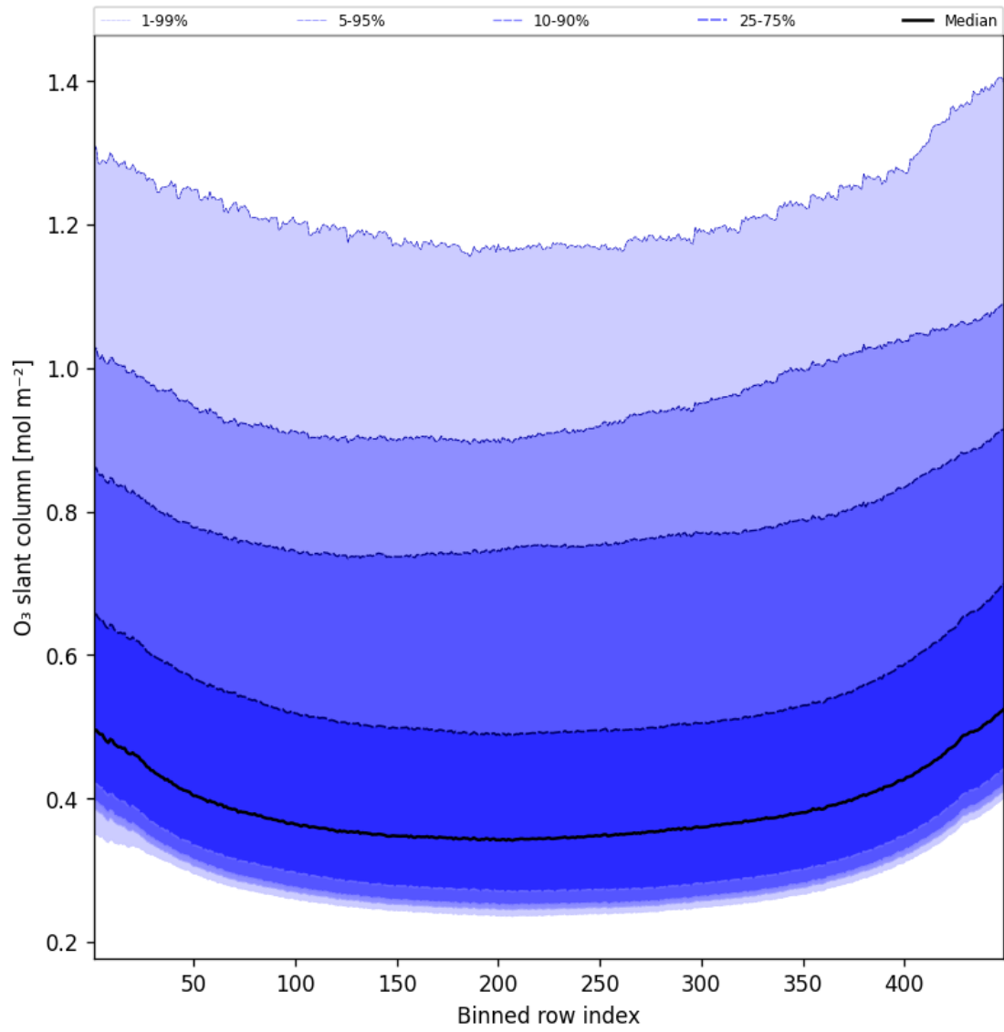
Figure 43: Along track statistics of “O 3 slant column” for 2025-10-03 to 2025-10-04
