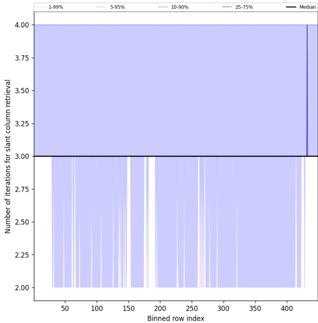
Figure 45: Along track statistics of “Number of iterations for slant column retrieval” for 2025-10-03 to 2025-10-04
