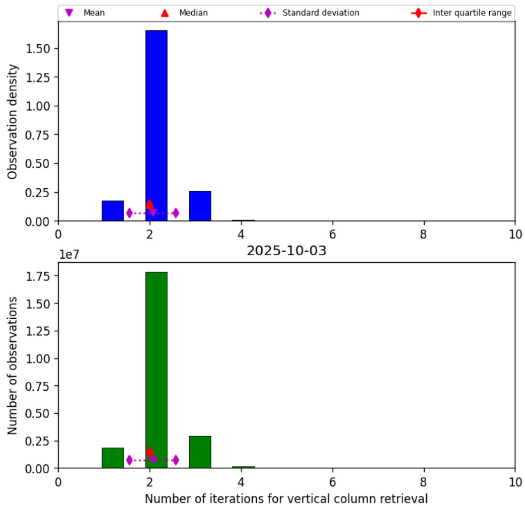
Figure 39: Histogram of “Number of iterations for vertical column retrieval” for 2025-10-03 to 2025-10-04
