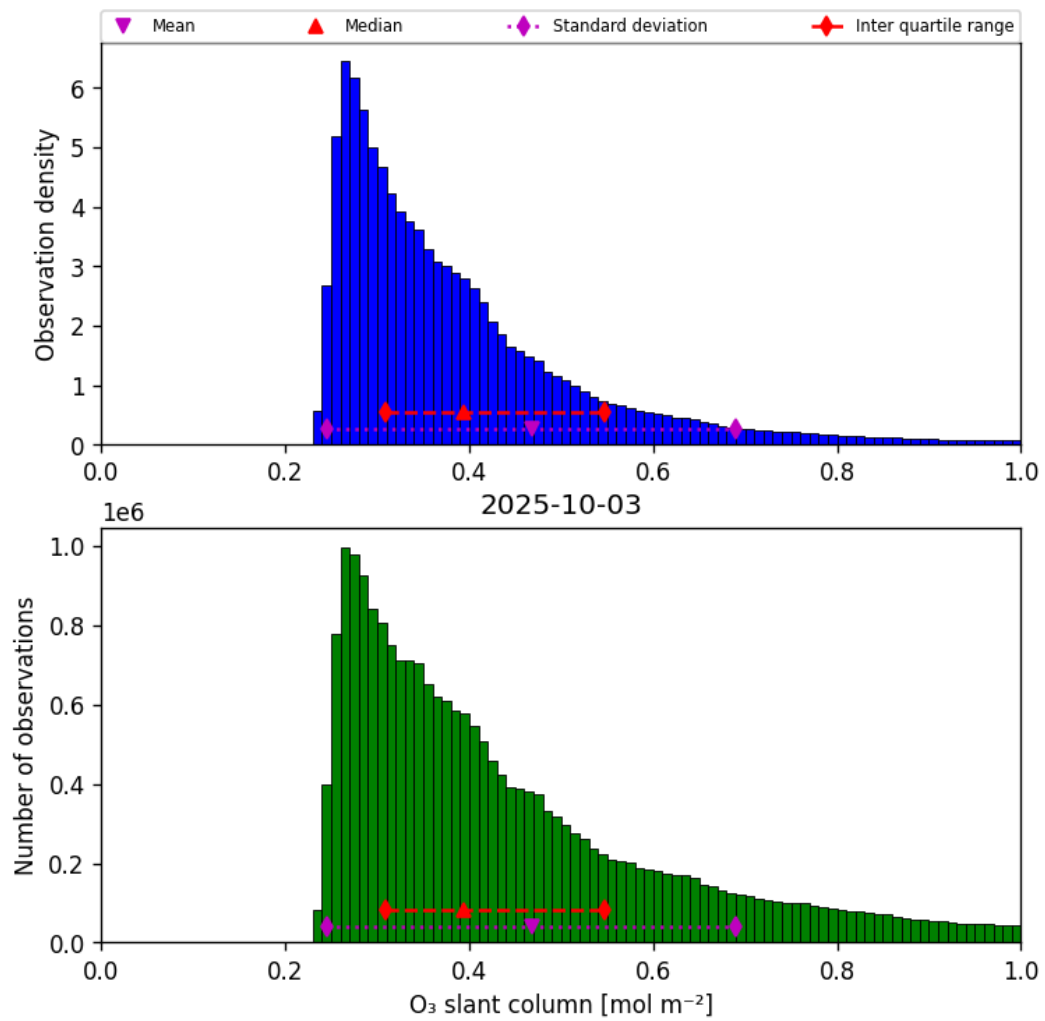
Figure 31: Histogram of “O 3 slant column” for 2025-10-03 to 2025-10-04
