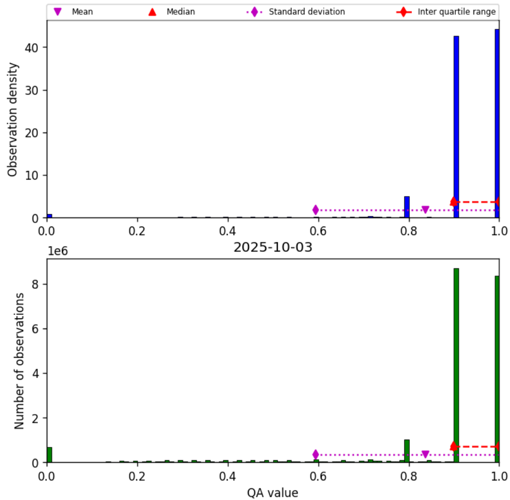
Figure 28: Histogram of “QA value” for 2025-10-03 to 2025-10-04
