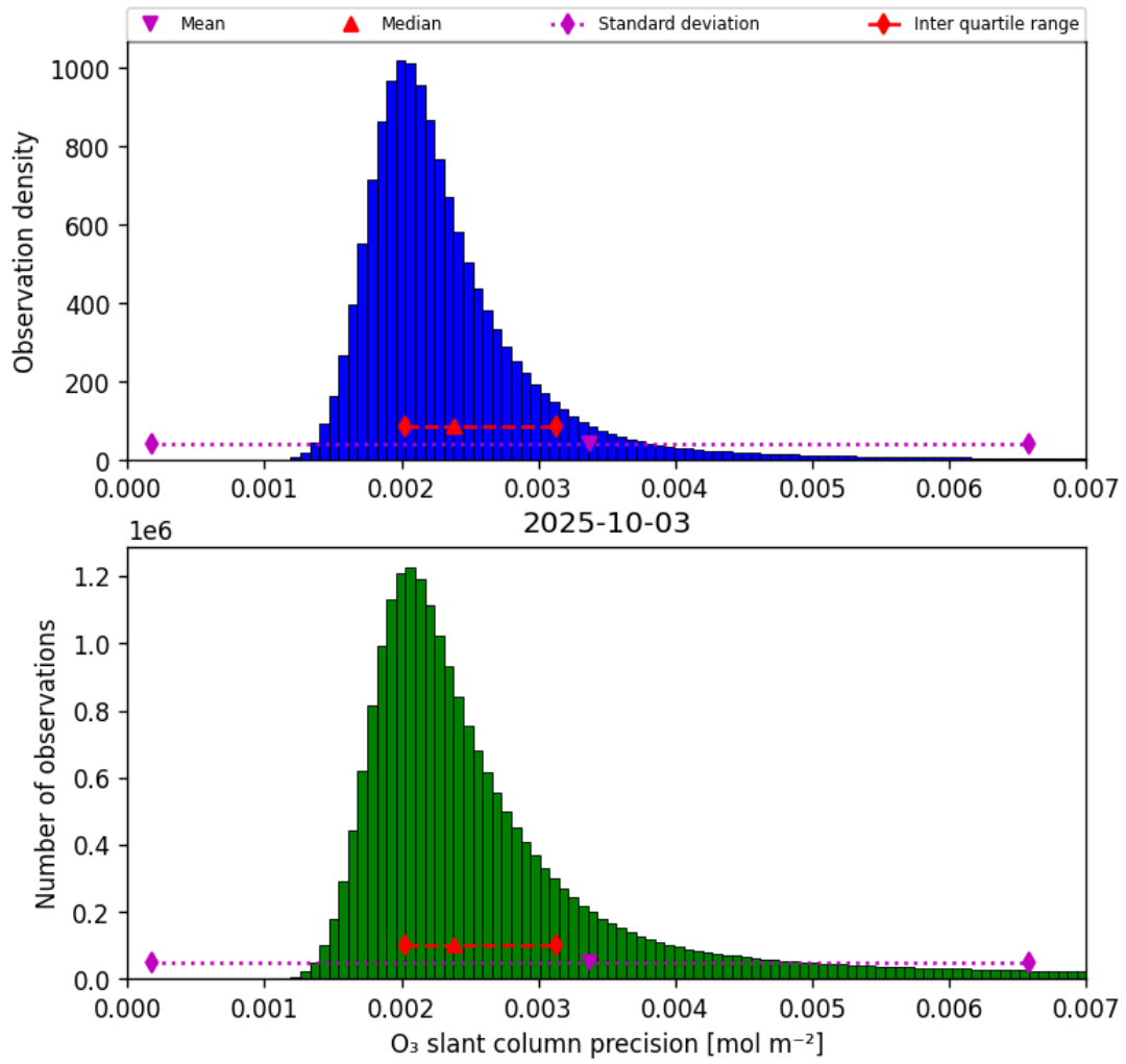
Figure 32: Histogram of “O 3 slant column precision” for 2025-10-03 to 2025-10-04
