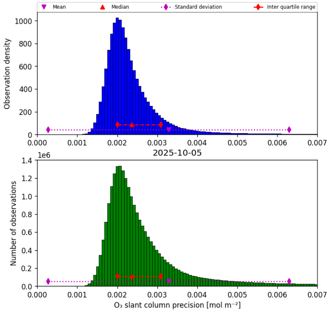
Figure 32: Histogram of “O 3 slant column precision” for 2025-10-05 to 2025-10-06
