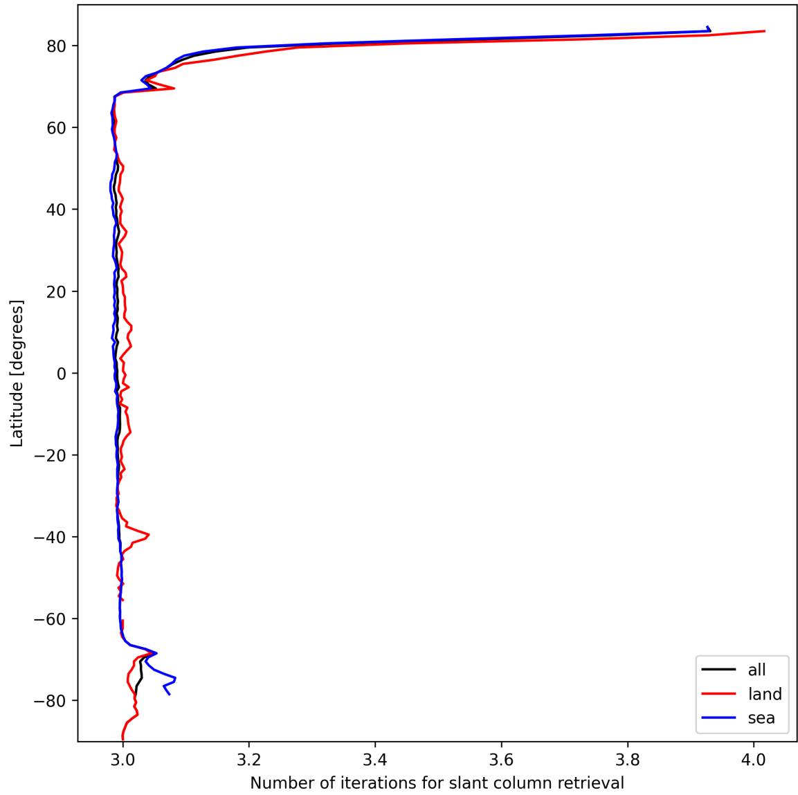
Figure 21: Zonal average of “Number of iterations for slant column retrieval” for 2025-10-05 to 2025-10-06.
