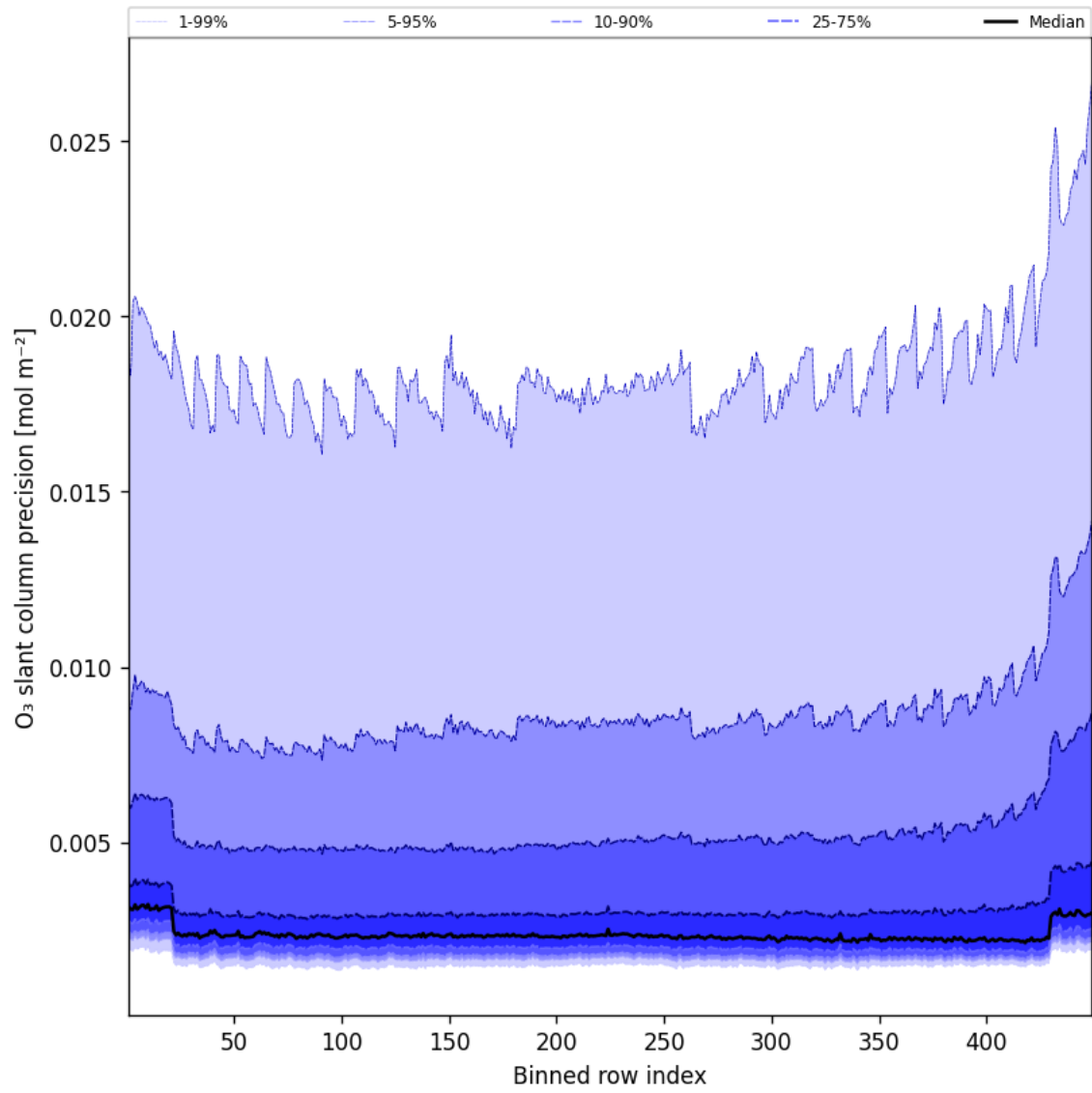
Figure 44: Along track statistics of “O 3 slant column precision” for 2025-10-05 to 2025-10-06
