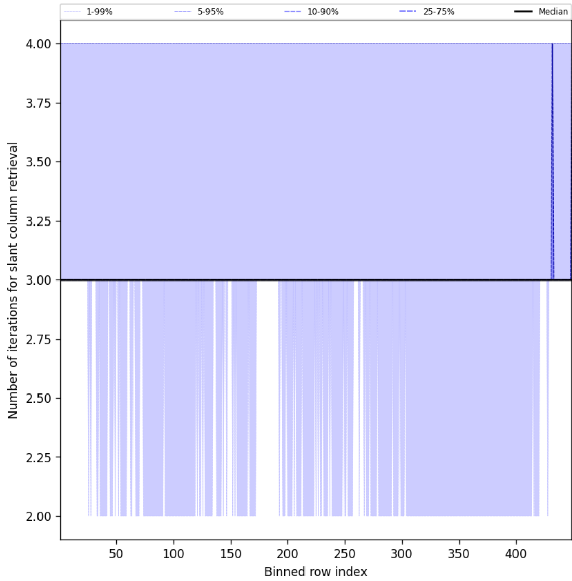
Figure 45: Along track statistics of “Number of iterations for slant column retrieval” for 2025-10-05 to 2025-10-06
