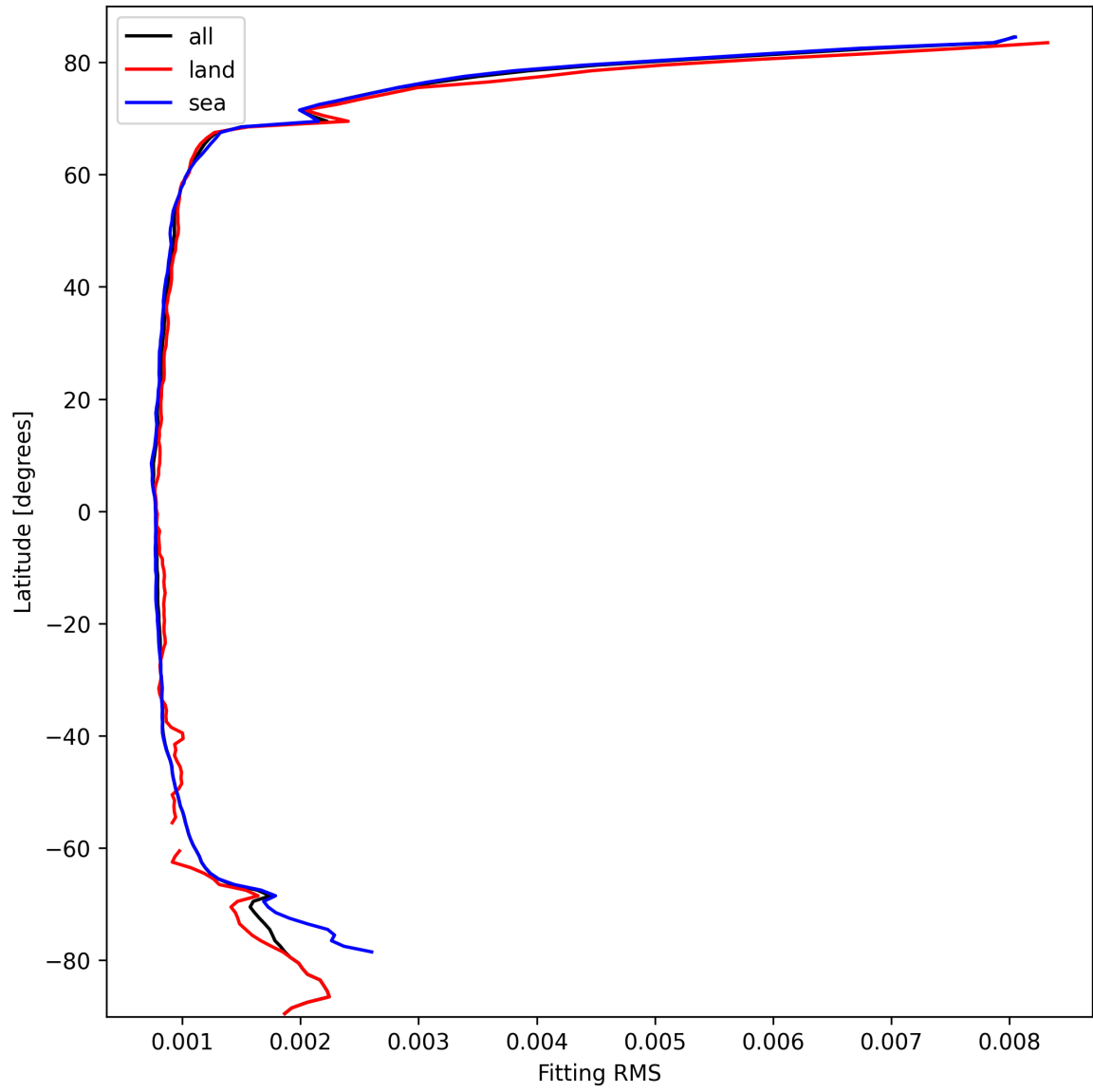
Figure 22: Zonal average of “Fitting RMS” for 2025-10-05 to 2025-10-06.
