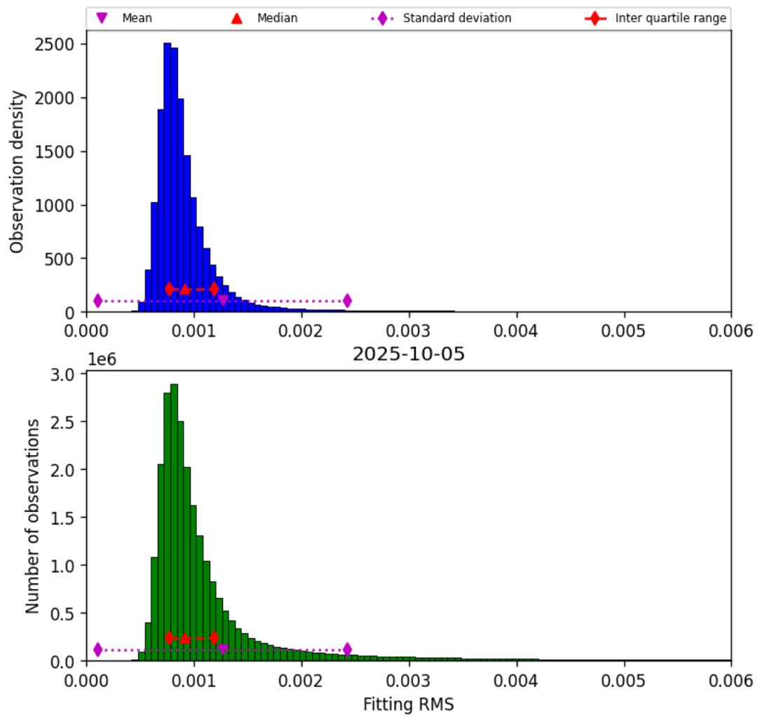
Figure 34: Histogram of “Fitting RMS” for 2025-10-05 to 2025-10-06
