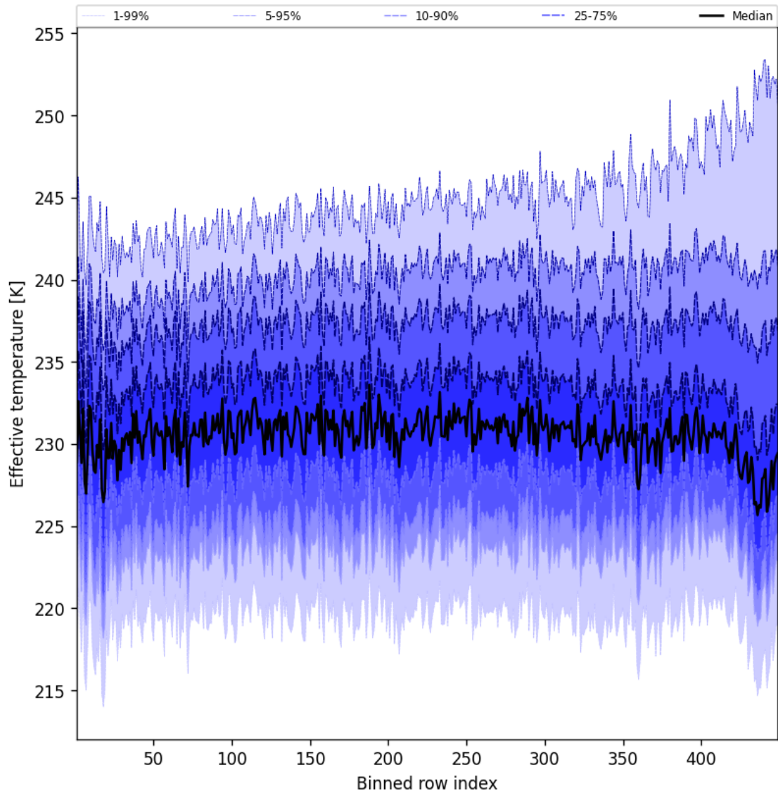
Figure 50: Along track statistics of “Effective temperature” for 2025-10-05 to 2025-10-06
