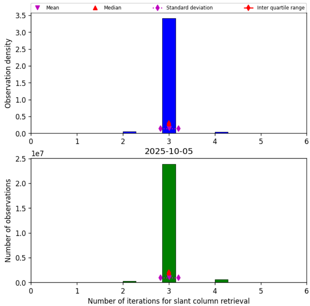
Figure 33: Histogram of “Number of iterations for slant column retrieval” for 2025-10-05 to 2025-10-06
