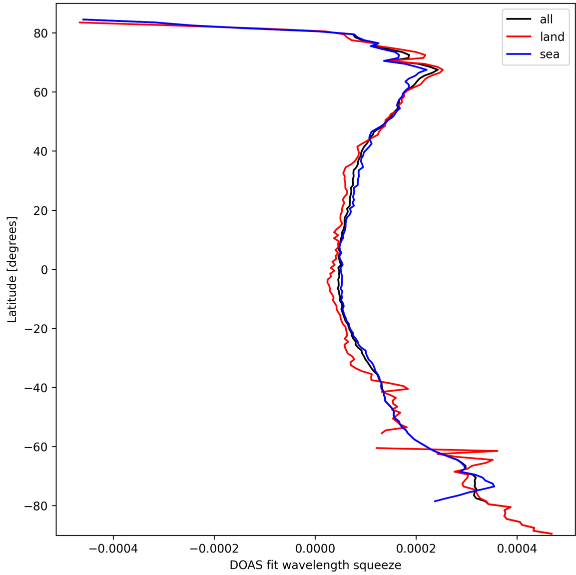
Figure 24: Zonal average of “DOAS fit wavelength squeeze” for 2025-10-05 to 2025-10-06.
