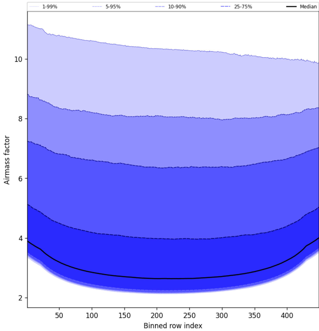
Figure 49: Along track statistics of “Airmass factor” for 2025-10-05 to 2025-10-06
