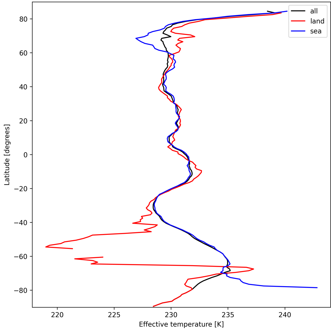
Figure 26: Zonal average of "Effective temperature" for 2025-10-05 to 2025-10-06.
