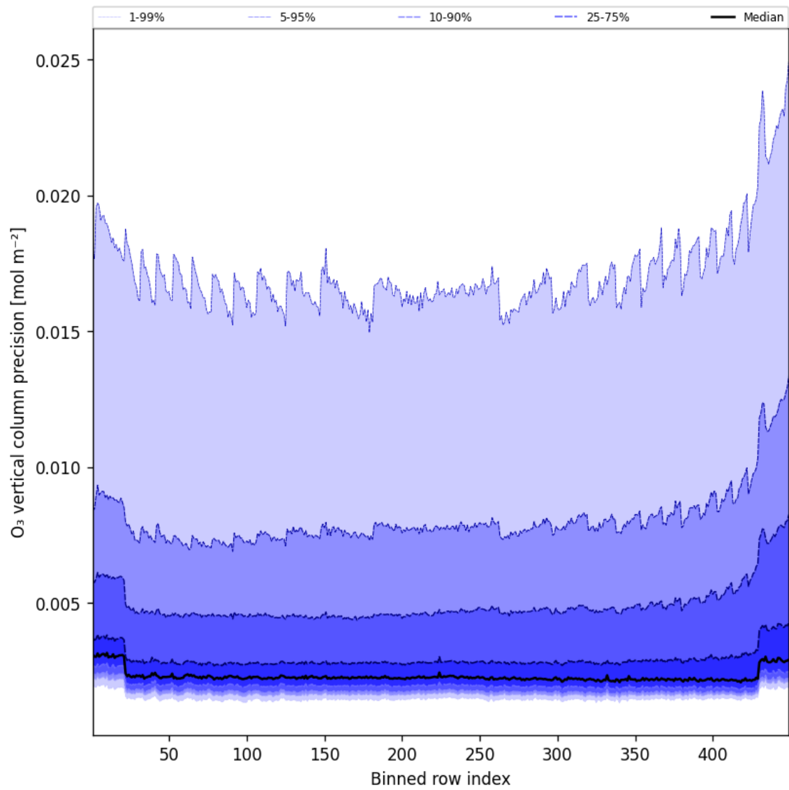
Figure 42: Along track statistics of “O 3 vertical column precision” for 2025-10-05 to 2025-10-06
