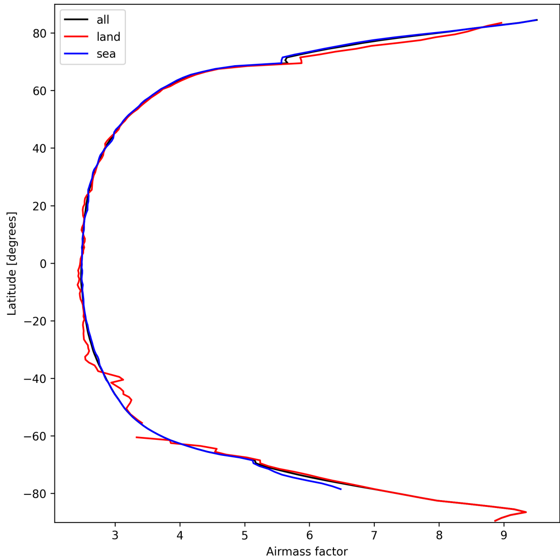
Figure 25: Zonal average of “Airmass factor” for 2025-10-05 to 2025-10-06.
