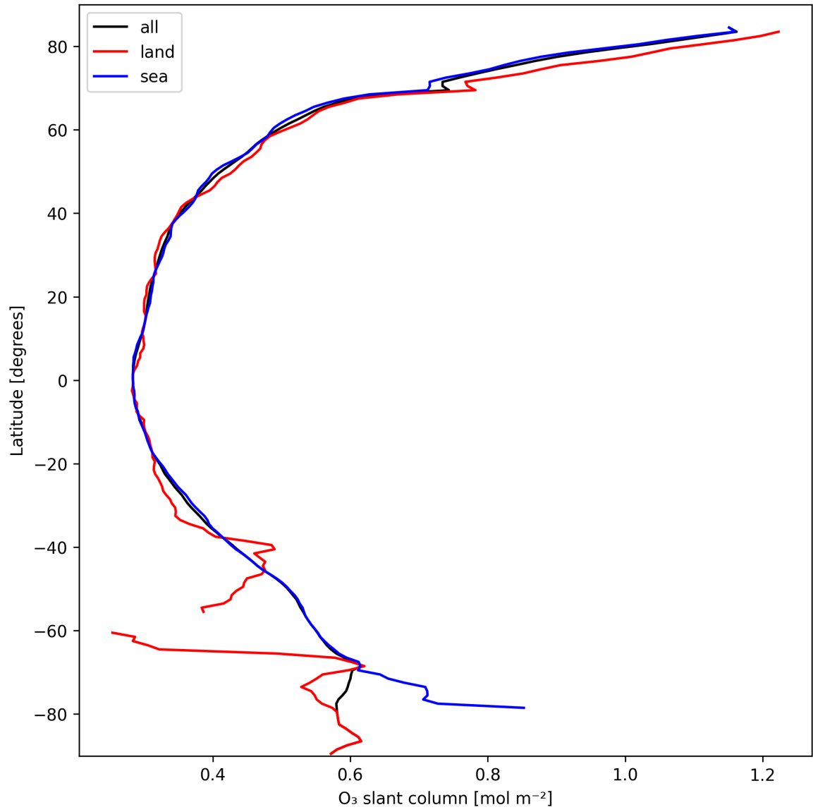
Figure 19: Zonal average of “O 3 slant column” for 2025-10-05 to 2025-10-06.
