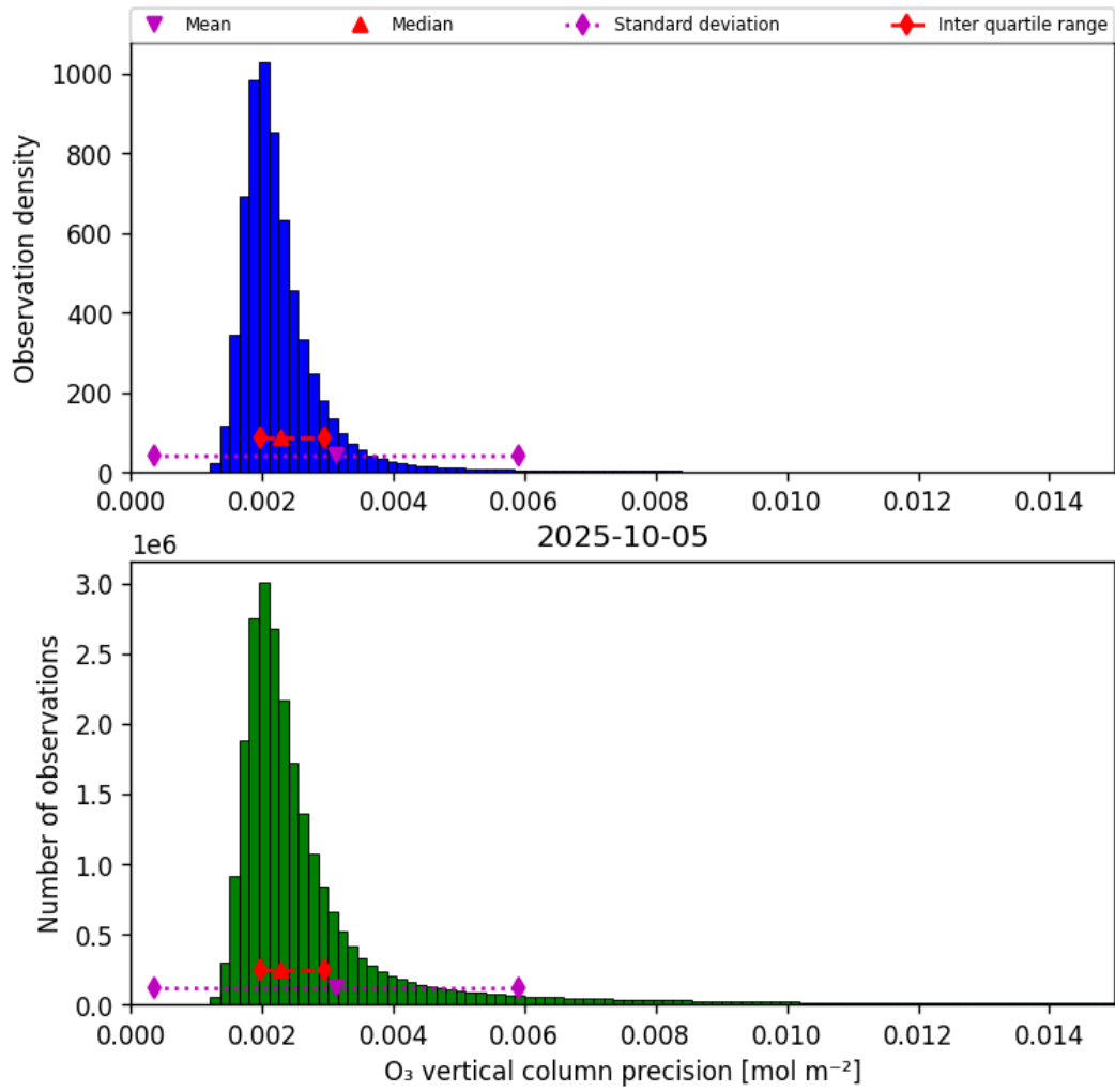
Figure 30: Histogram of "O 3 vertical column precision" for 2025-10-05 to 2025-10-06
