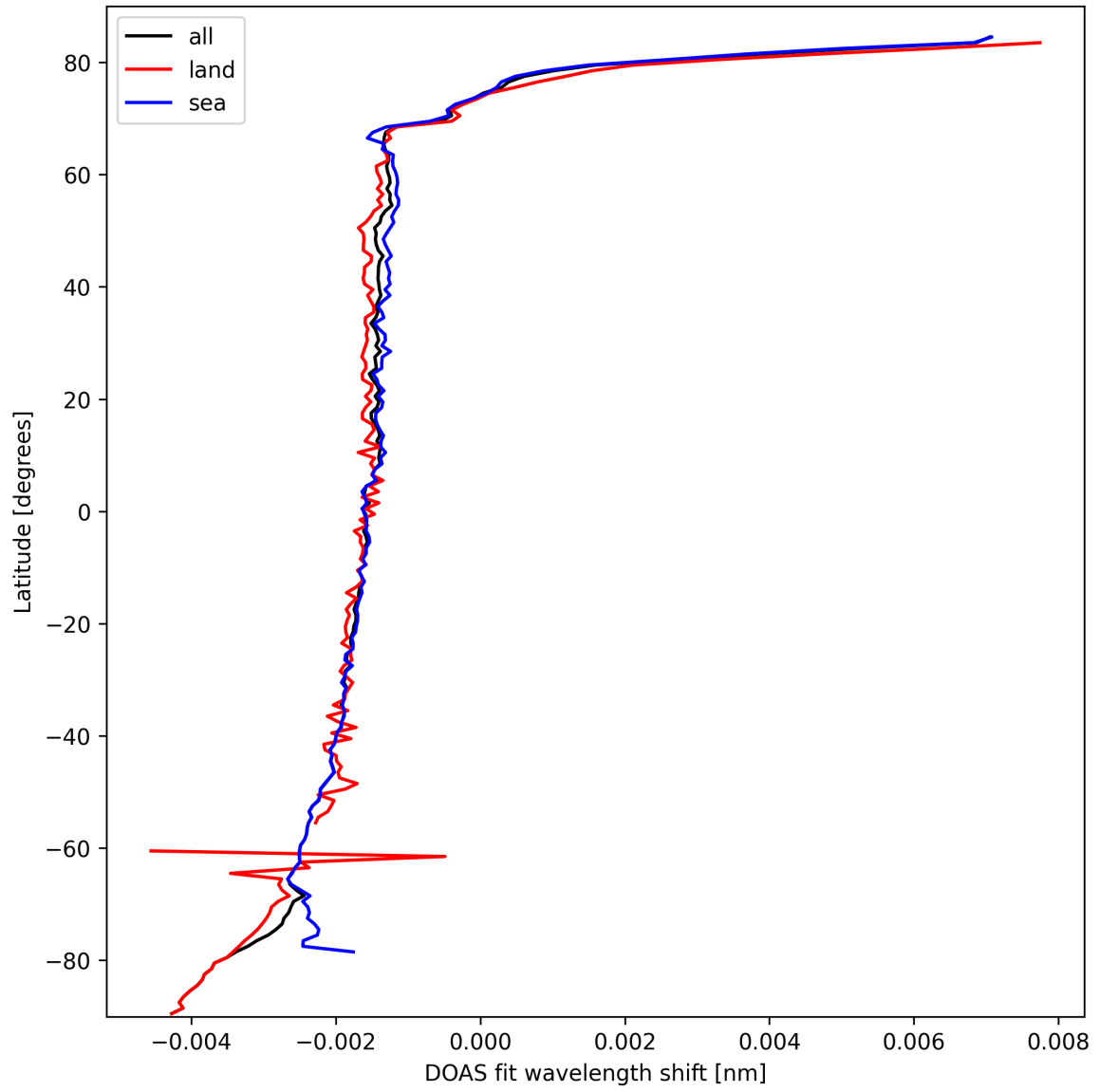
Figure 23: Zonal average of “DOAS fit wavelength shift” for 2025-10-05 to 2025-10-06.
