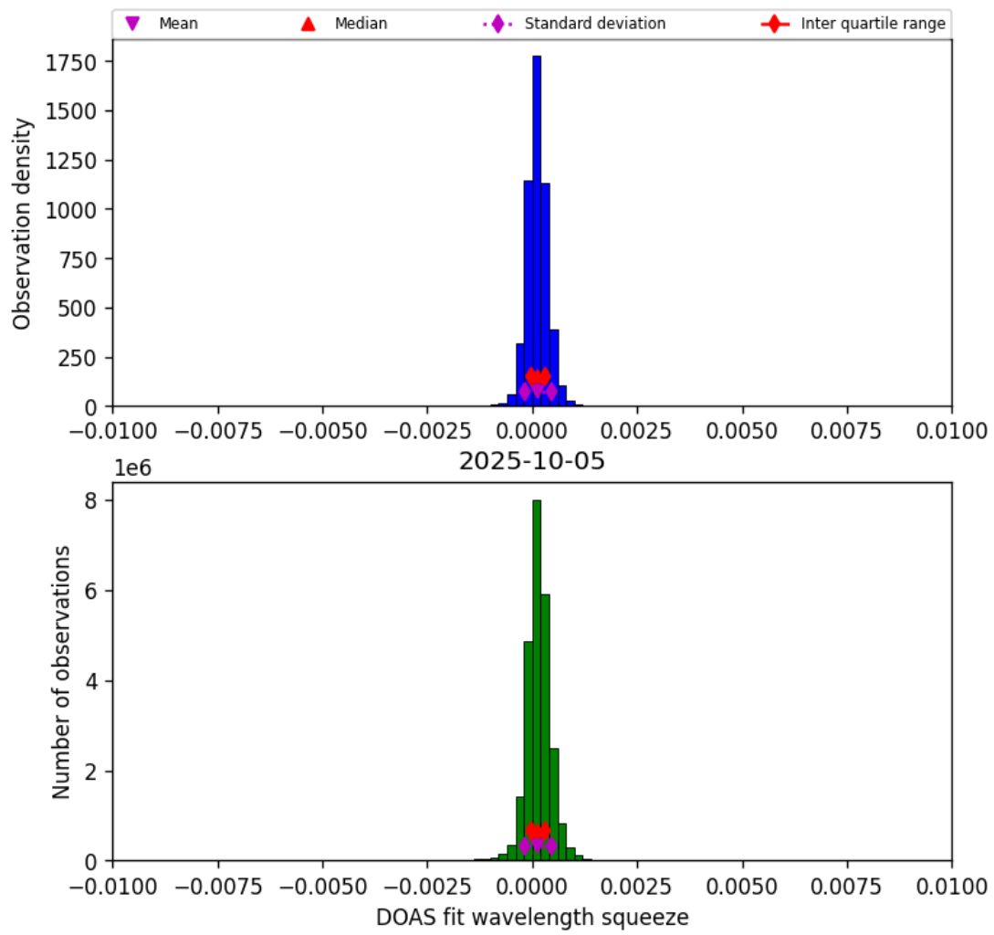
Figure 36: Histogram of “DOAS fit wavelength squeeze” for 2025-10-05 to 2025-10-06
