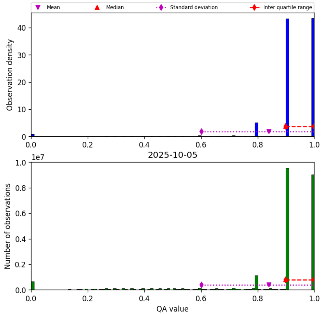
Figure 28: Histogram of “QA value” for 2025-10-05 to 2025-10-06
