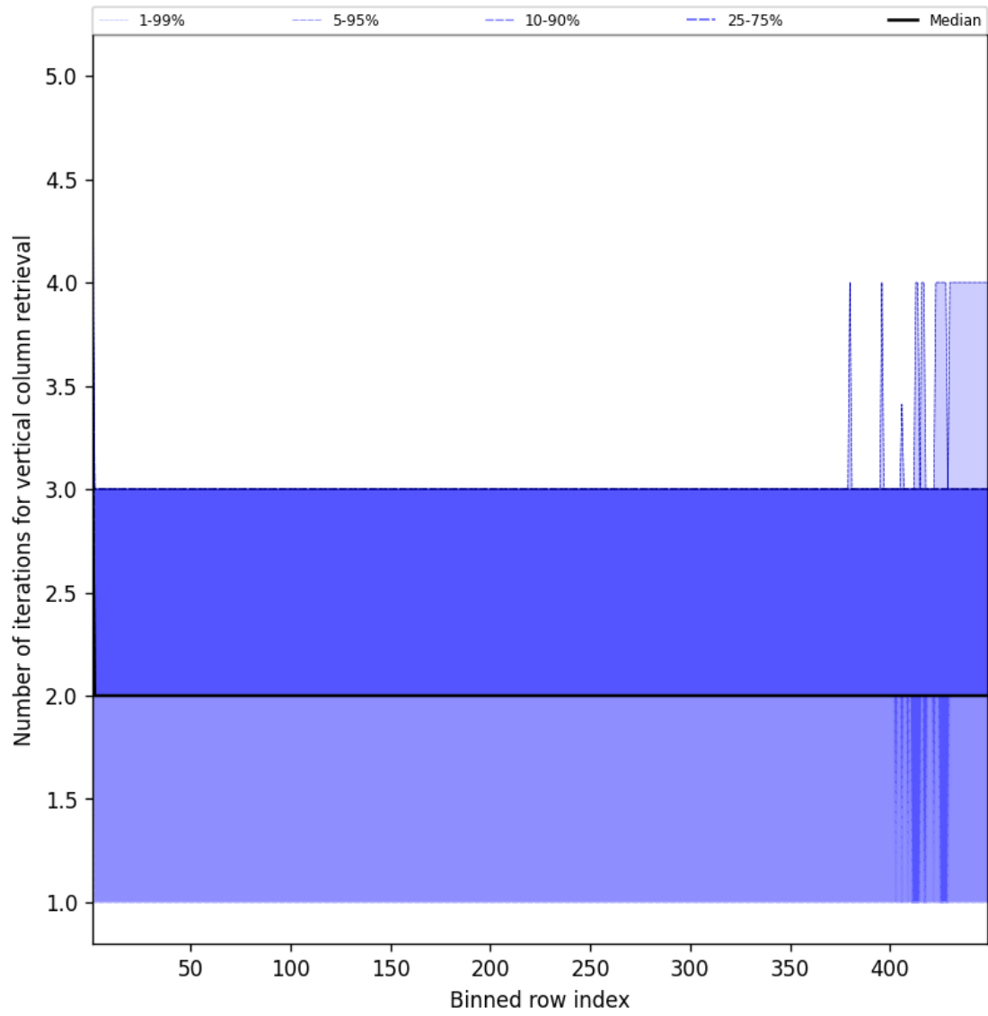
Figure 51: Along track statistics of “Number of iterations for vertical column retrieval” for 2025-10-05 to 2025-10-06
