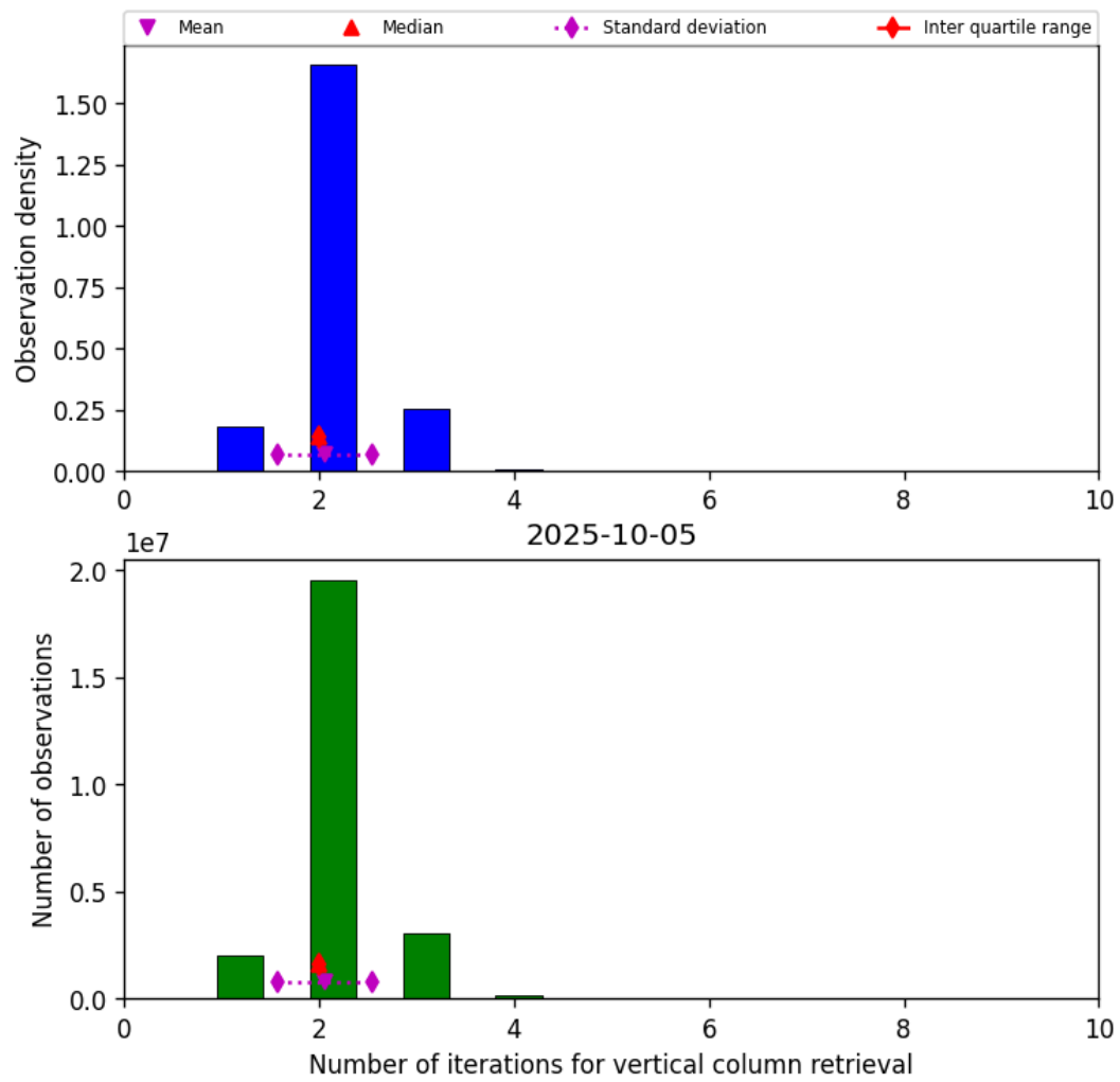
Figure 39: Histogram of “Number of iterations for vertical column retrieval” for 2025-10-05 to 2025-10-06
