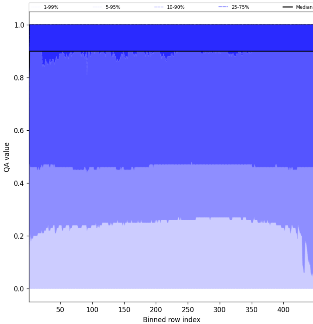
Figure 40: Along track statistics of “QA value” for 2025-10-05 to 2025-10-06
