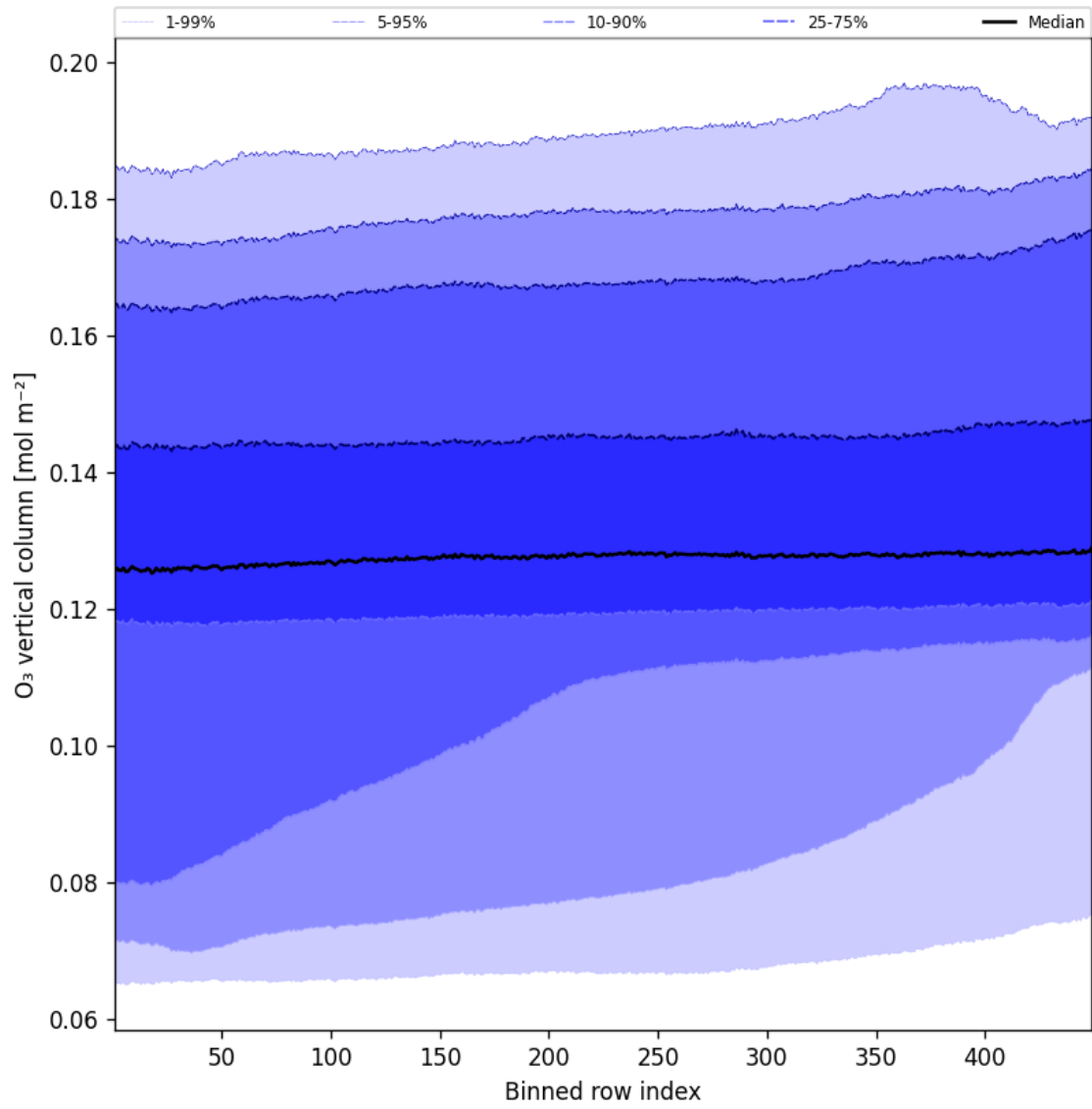
Figure 41: Along track statistics of "O 3 vertical column" for 2025-10-05 to 2025-10-06
