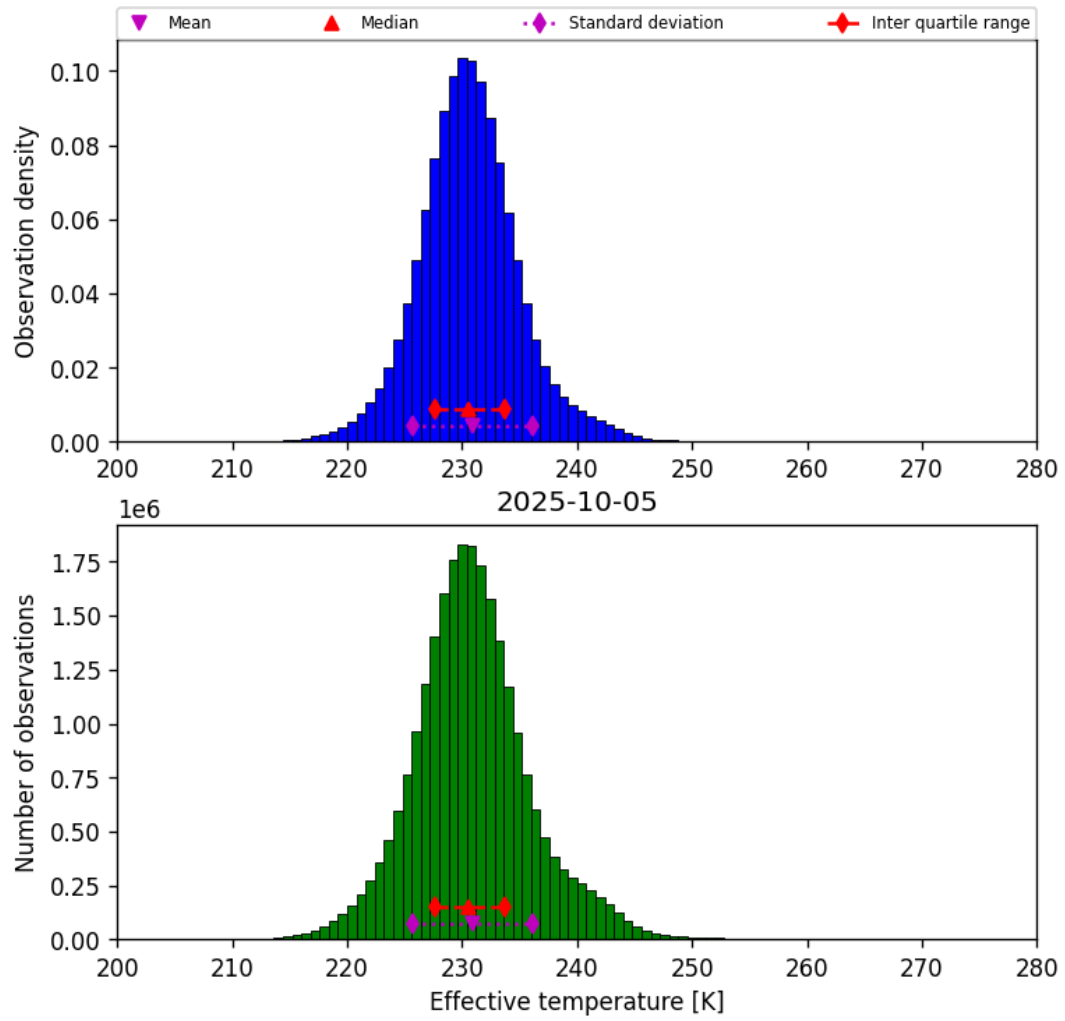
Figure 38: Histogram of “Effective temperature” for 2025-10-05 to 2025-10-06
