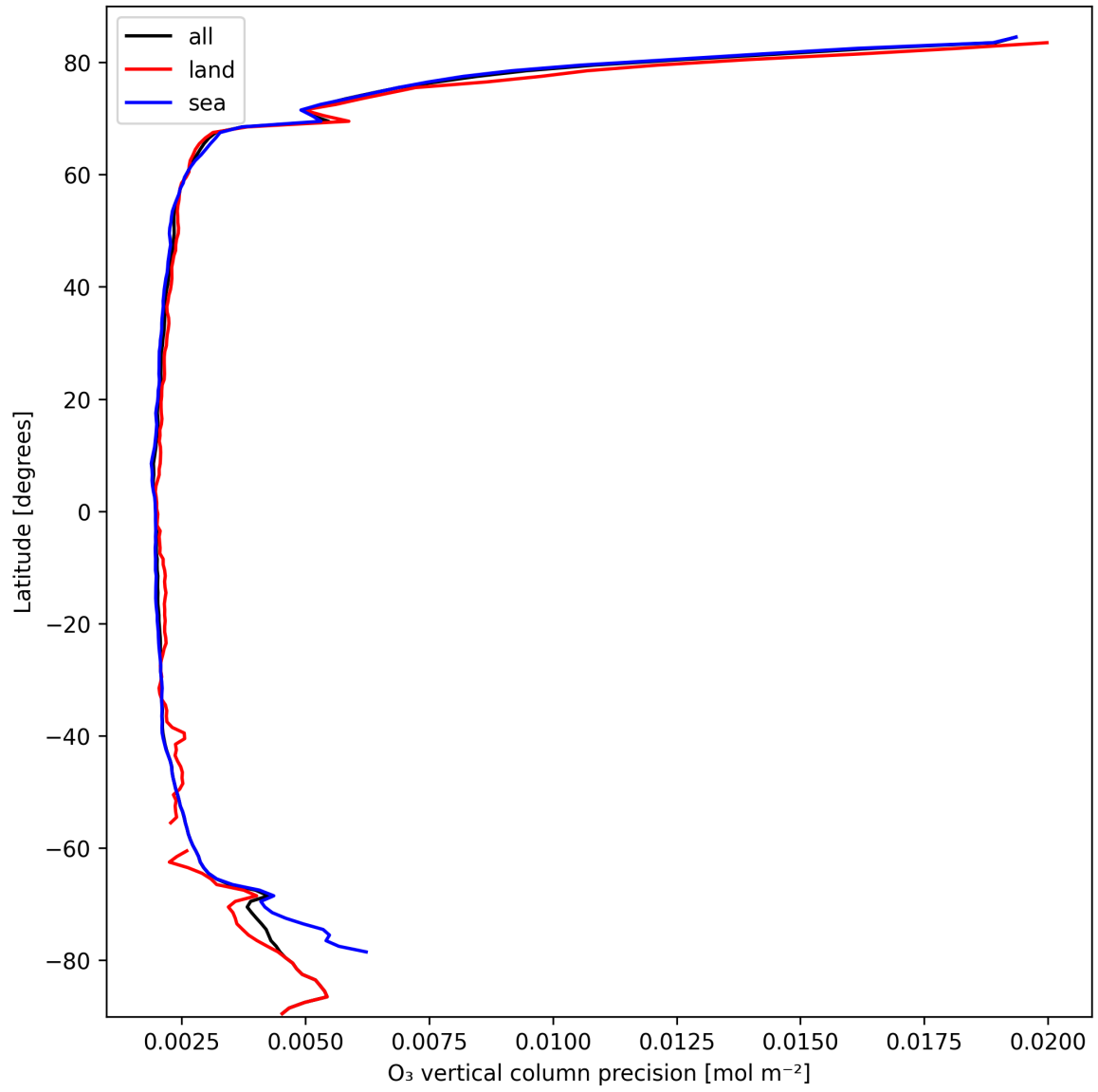
Figure 18: Zonal average of “O 3 vertical column precision” for 2025-10-05 to 2025-10-06.
