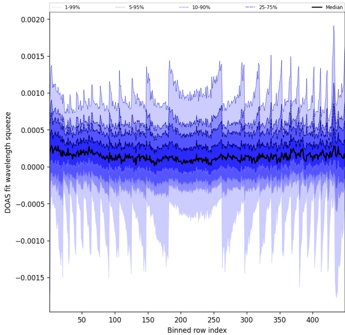
Figure 48: Along track statistics of “DOAS fit wavelength squeeze” for 2025-10-05 to 2025-10-06
