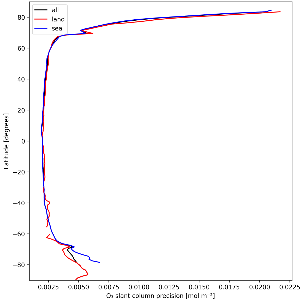
Figure 20: Zonal average of “O 3 slant column precision” for 2025-10-05 to 2025-10-06.
