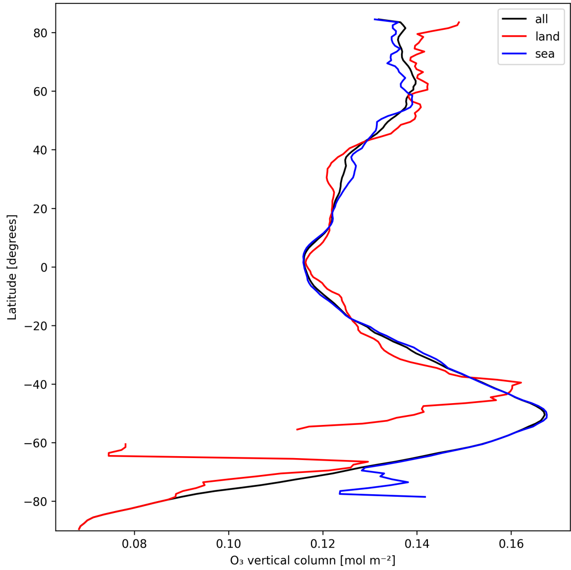
Figure 17: Zonal average of “O 3 vertical column” for 2025-10-05 to 2025-10-06.
