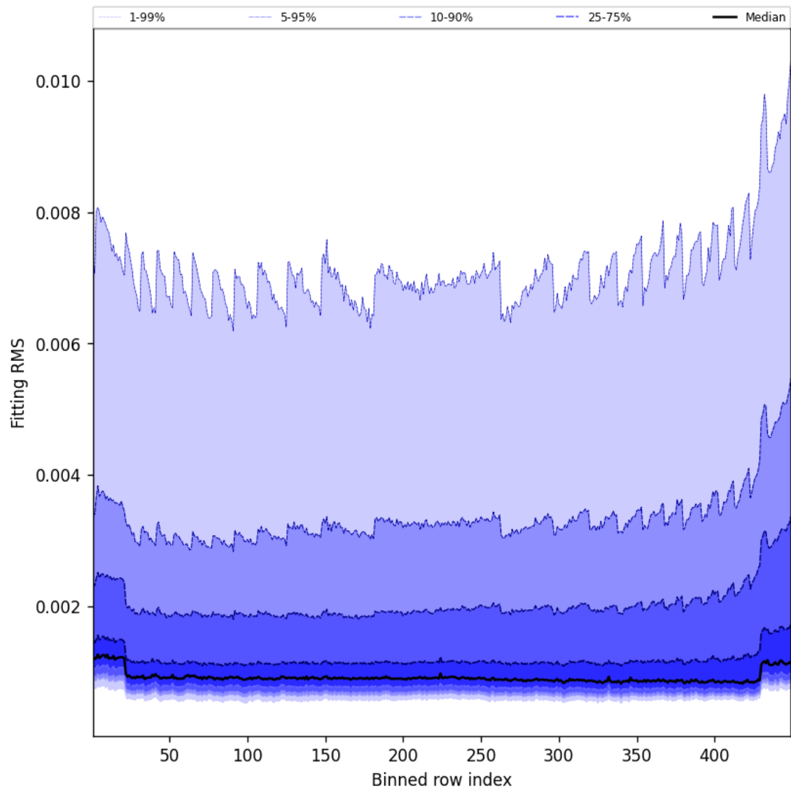
Figure 46: Along track statistics of “Fitting RMS” for 2025-10-05 to 2025-10-06
