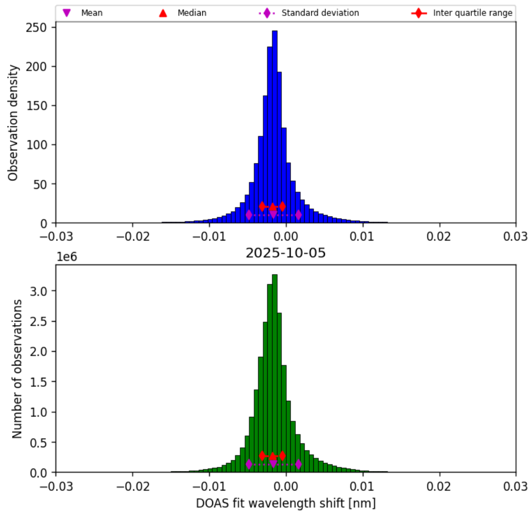
Figure 35: Histogram of “DOAS fit wavelength shift” for 2025-10-05 to 2025-10-06
