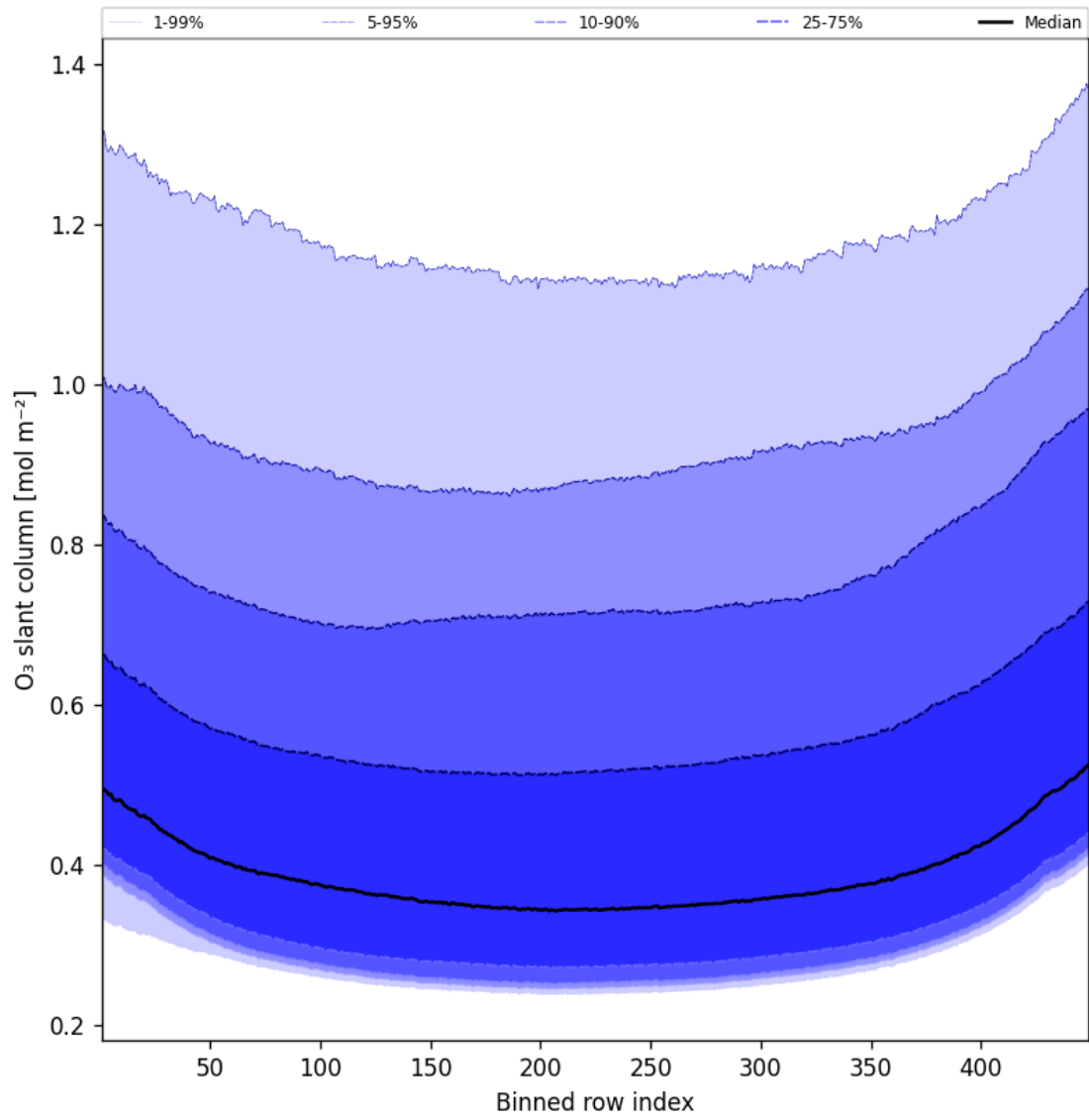
Figure 43: Along track statistics of “O 3 slant column” for 2025-10-05 to 2025-10-06
