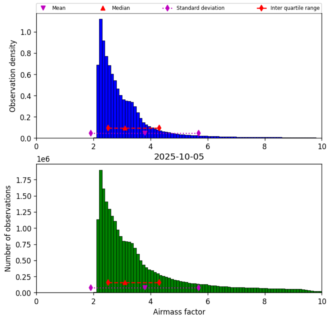
Figure 37: Histogram of “Airmass factor” for 2025-10-05 to 2025-10-06
