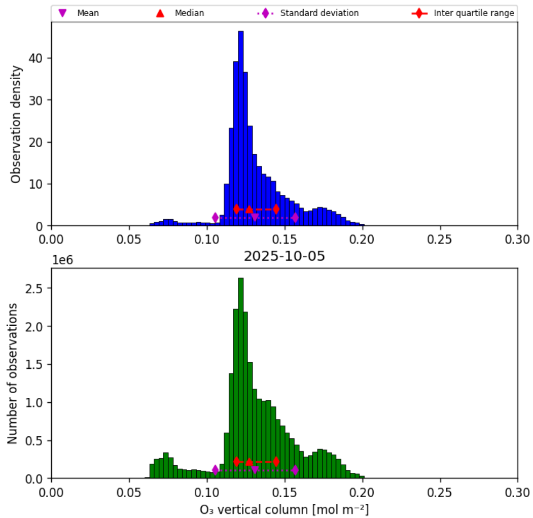
Figure 29: Histogram of “O 3 vertical column” for 2025-10-05 to 2025-10-06
