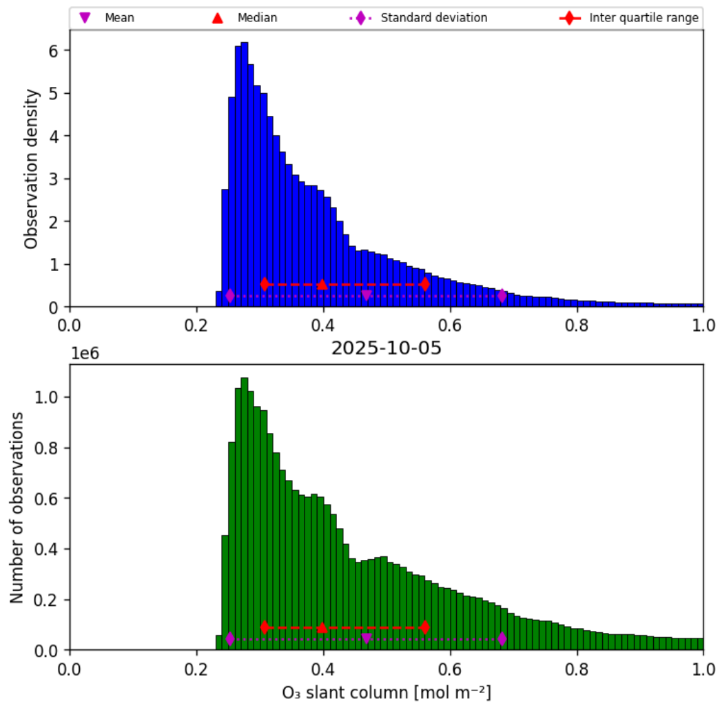
Figure 31: Histogram of “O 3 slant column” for 2025-10-05 to 2025-10-06
