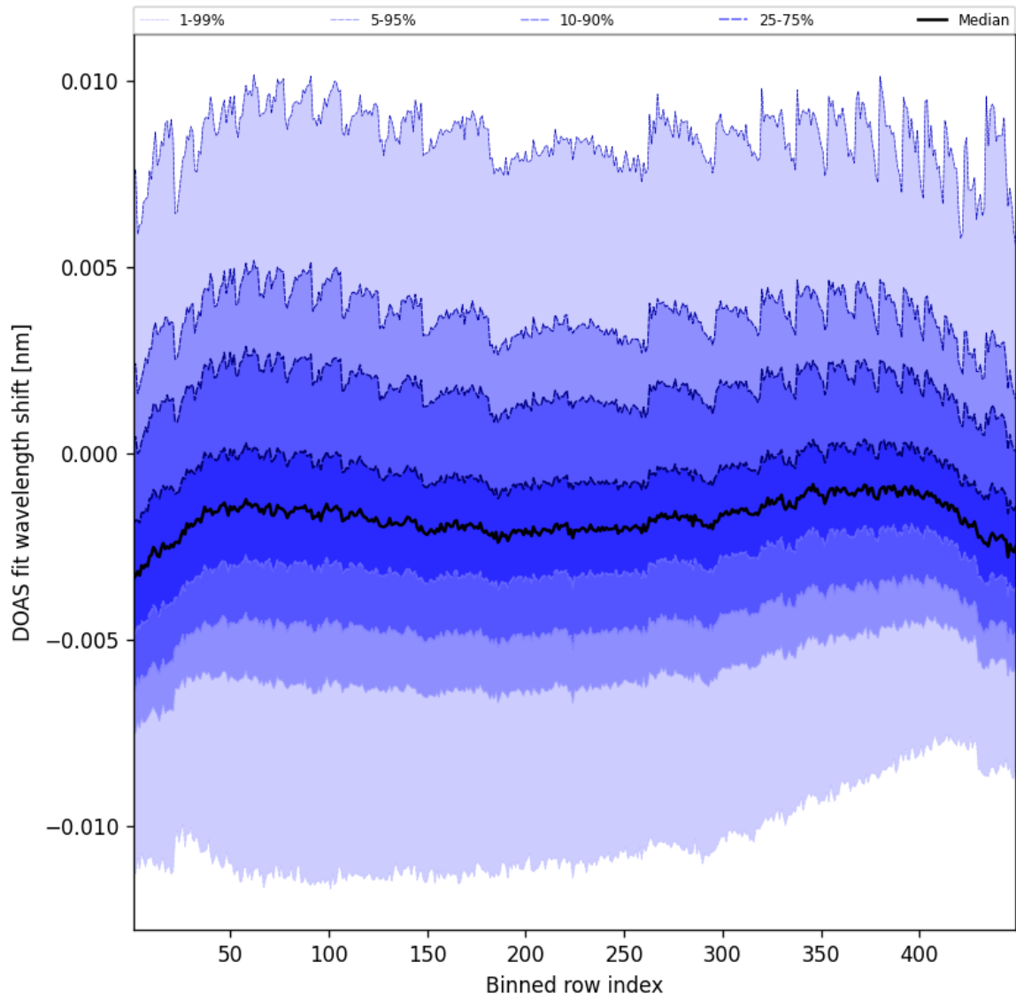
Figure 47: Along track statistics of “DOAS fit wavelength shift” for 2025-10-05 to 2025-10-06
