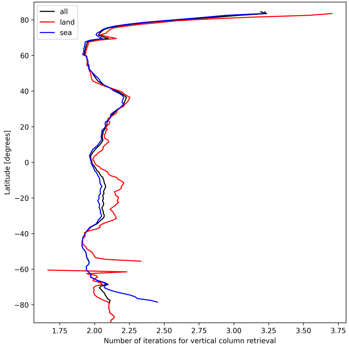
Figure 27: Zonal average of “Number of iterations for vertical column retrieval” for 2025-10-05 to 2025-10-06.
