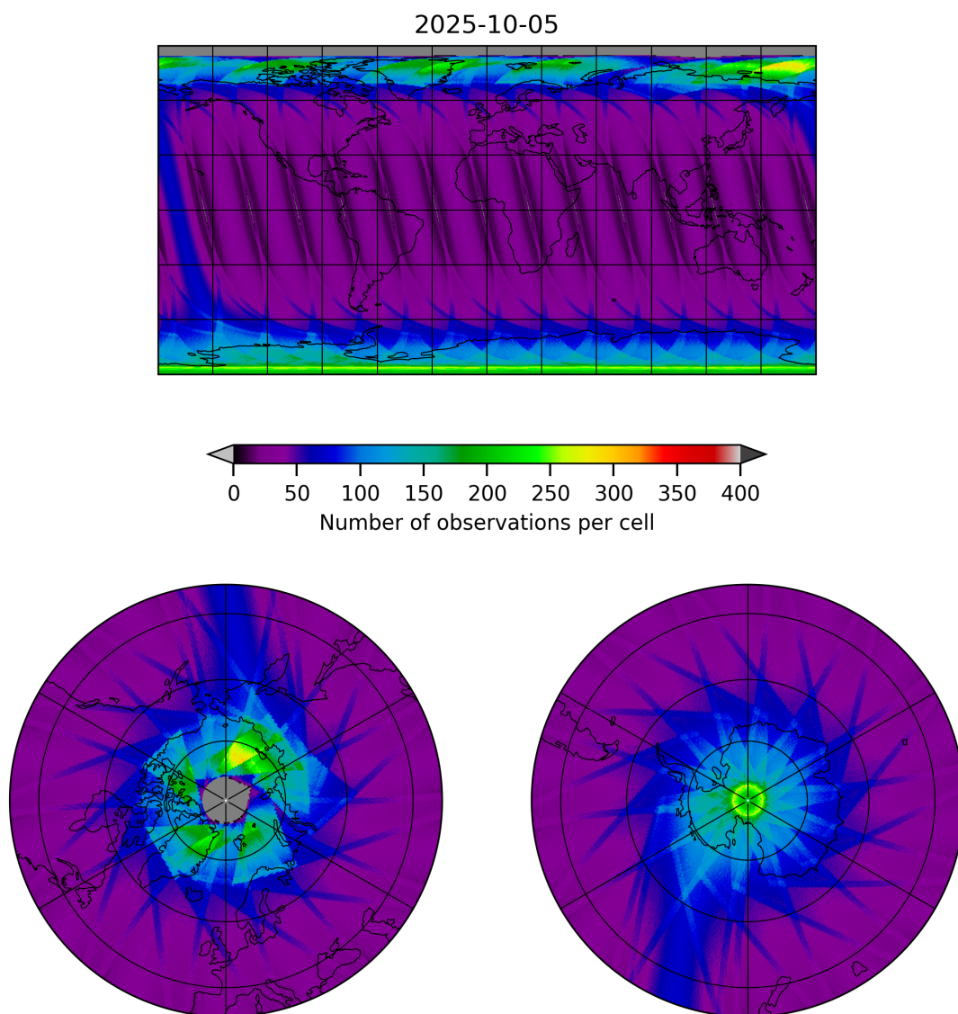
Figure 15: Map of the number of observations for 2025-10-05 to 2025-10-06
