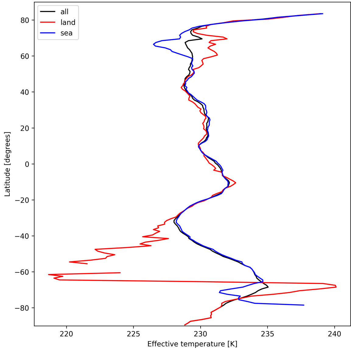
Figure 26: Zonal average of “Effective temperature” for 2025-10-06 to 2025-10-07.
