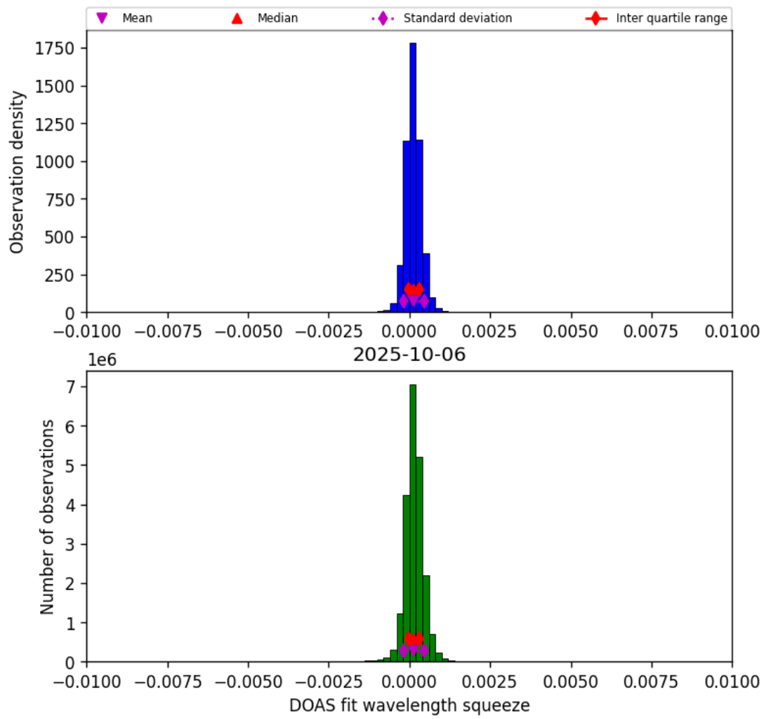
Figure 36: Histogram of “DOAS fit wavelength squeeze” for 2025-10-06 to 2025-10-07
