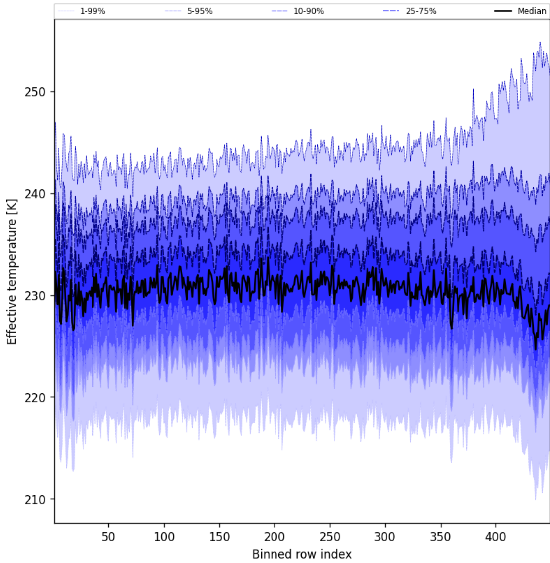
Figure 50: Along track statistics of “Effective temperature” for 2025-10-06 to 2025-10-07
