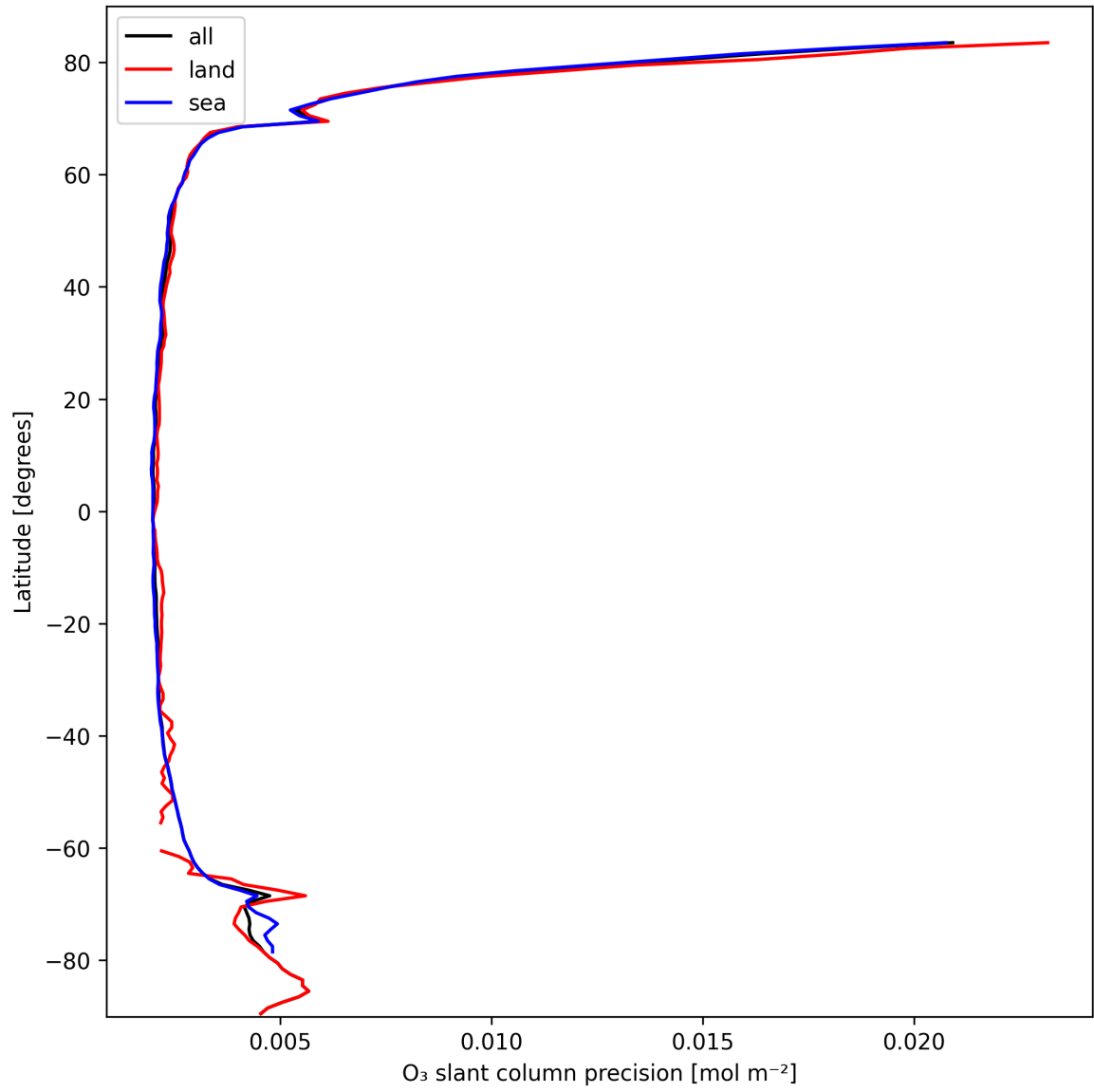
Figure 20: Zonal average of “O 3 slant column precision” for 2025-10-06 to 2025-10-07.
