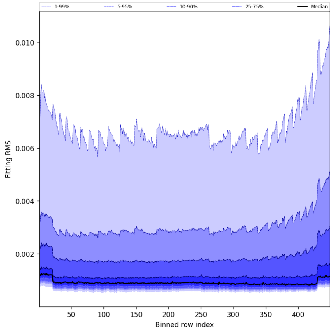
Figure 46: Along track statistics of “Fitting RMS” for 2025-10-06 to 2025-10-07
