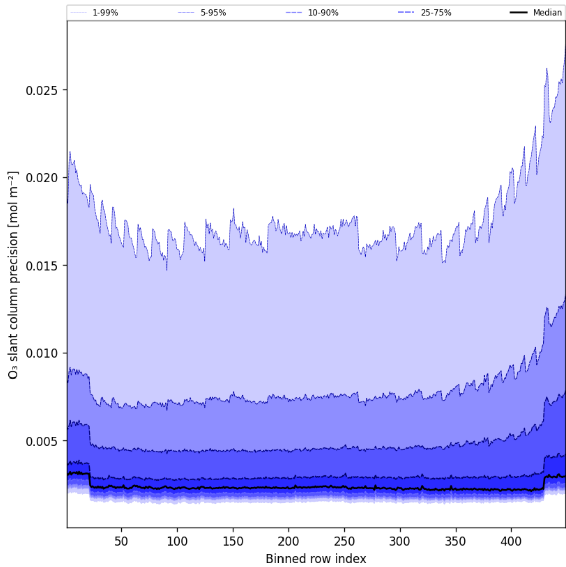
Figure 44: Along track statistics of “O 3 slant column precision” for 2025-10-06 to 2025-10-07
