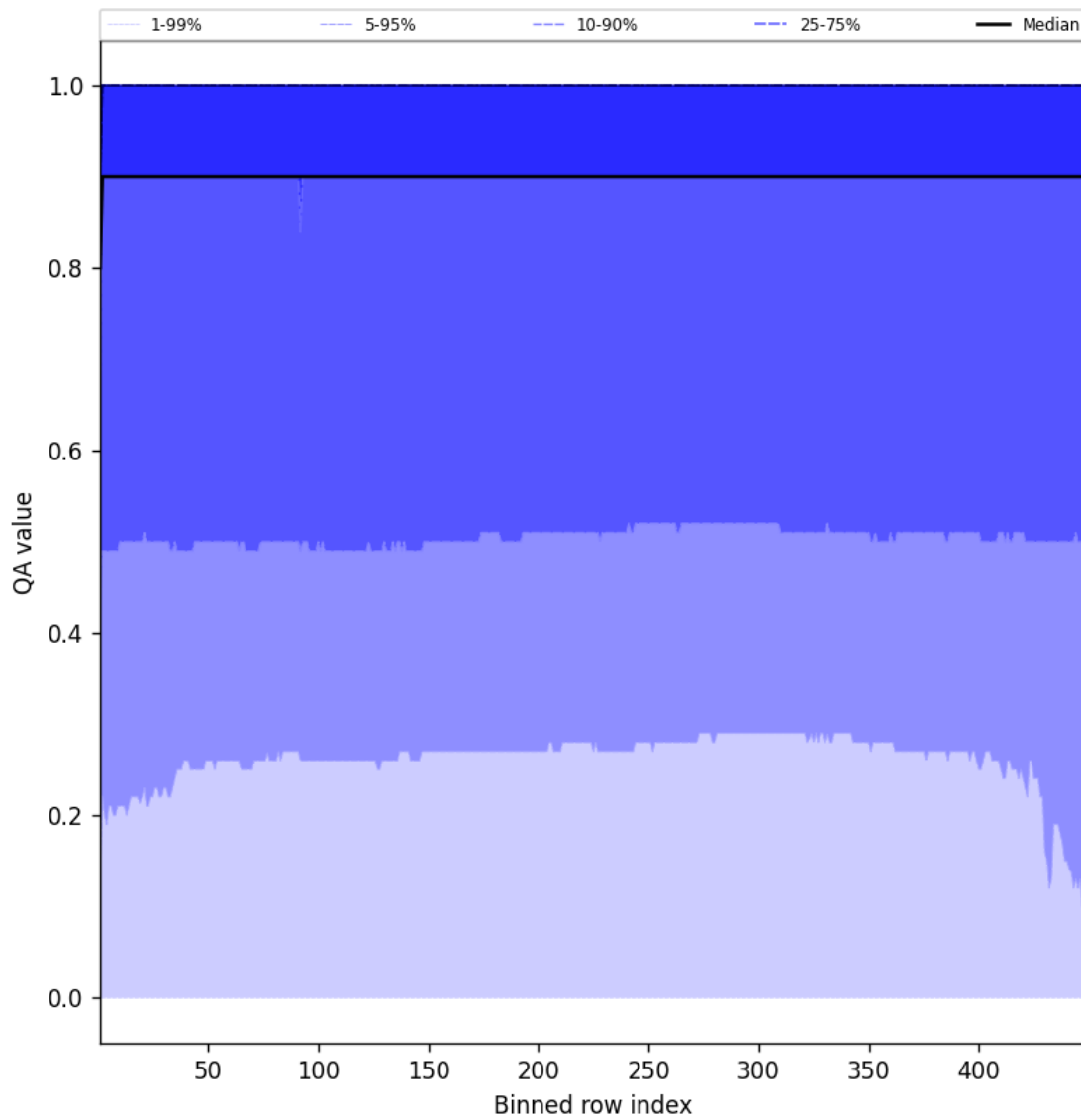
Figure 40: Along track statistics of “QA value” for 2025-10-06 to 2025-10-07
