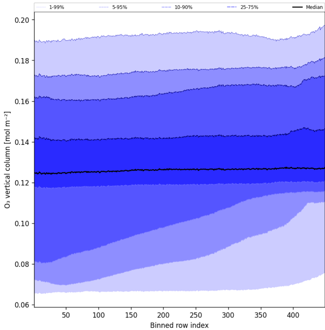
Figure 41: Along track statistics of “O 3 vertical column” for 2025-10-06 to 2025-10-07
