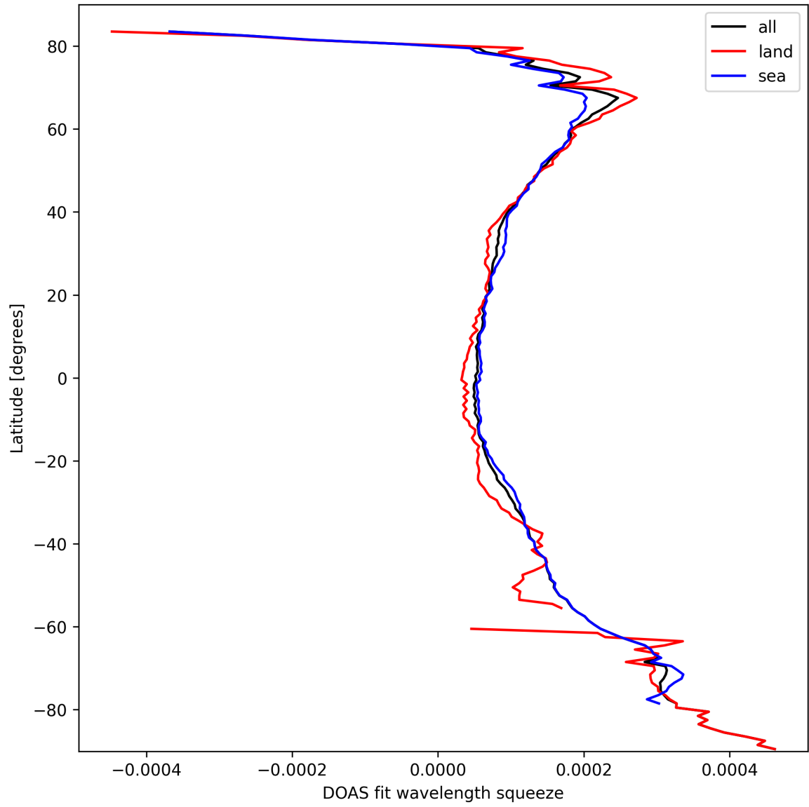
Figure 24: Zonal average of “DOAS fit wavelength squeeze” for 2025-10-06 to 2025-10-07.
