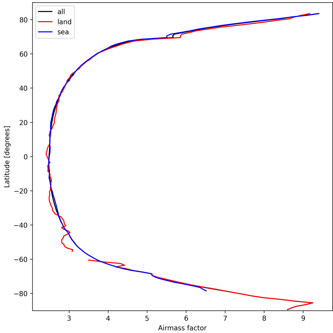
Figure 25: Zonal average of “Airmass factor” for 2025-10-06 to 2025-10-07.
