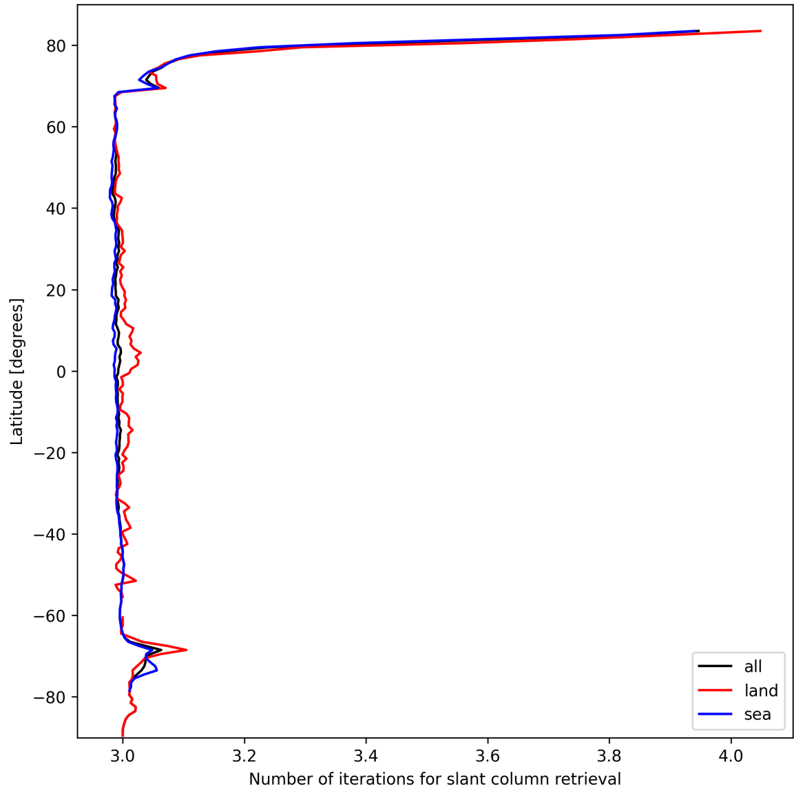
Figure 21: Zonal average of “Number of iterations for slant column retrieval” for 2025-10-06 to 2025-10-07.
