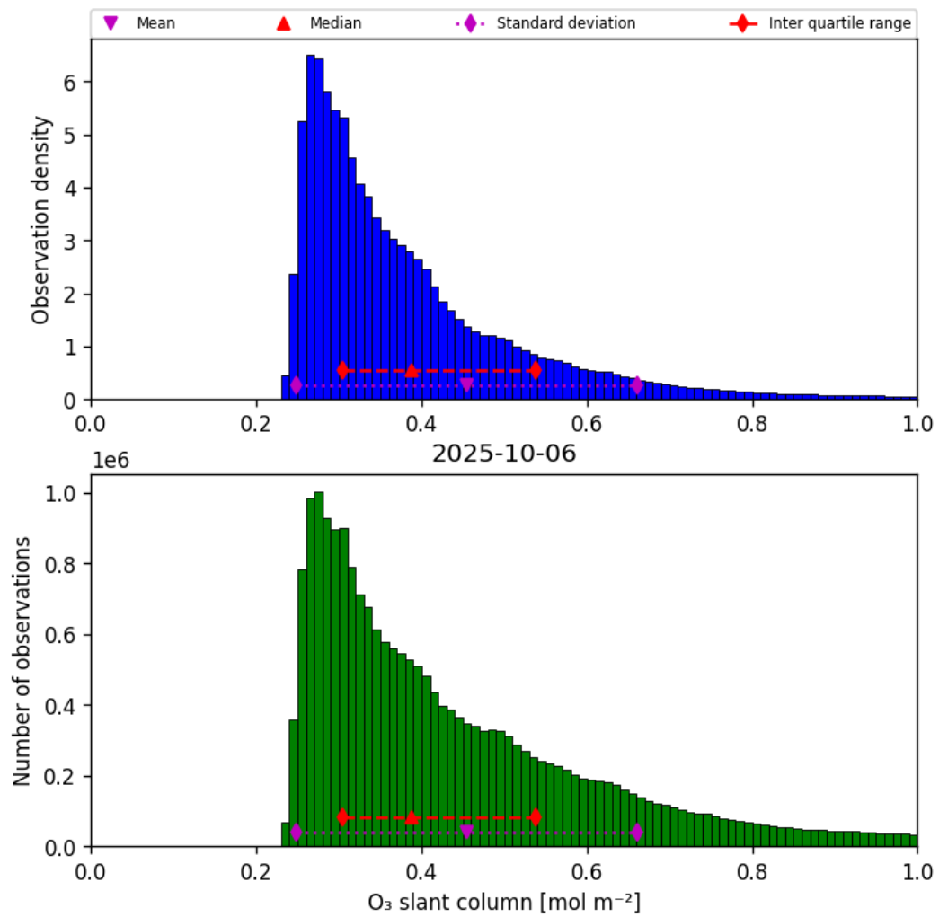
Figure 31: Histogram of “O 3 slant column” for 2025-10-06 to 2025-10-07
