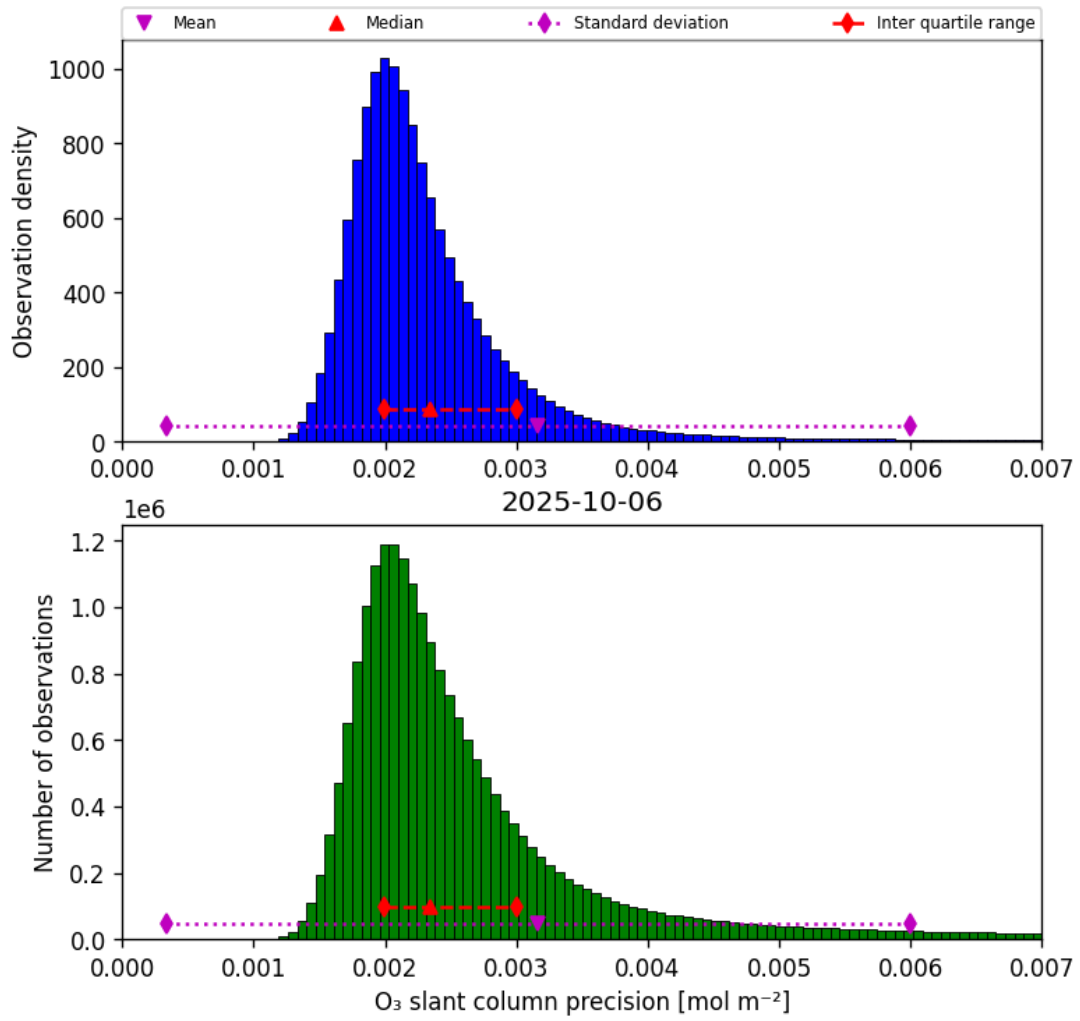
Figure 32: Histogram of “O 3 slant column precision” for 2025-10-06 to 2025-10-07
