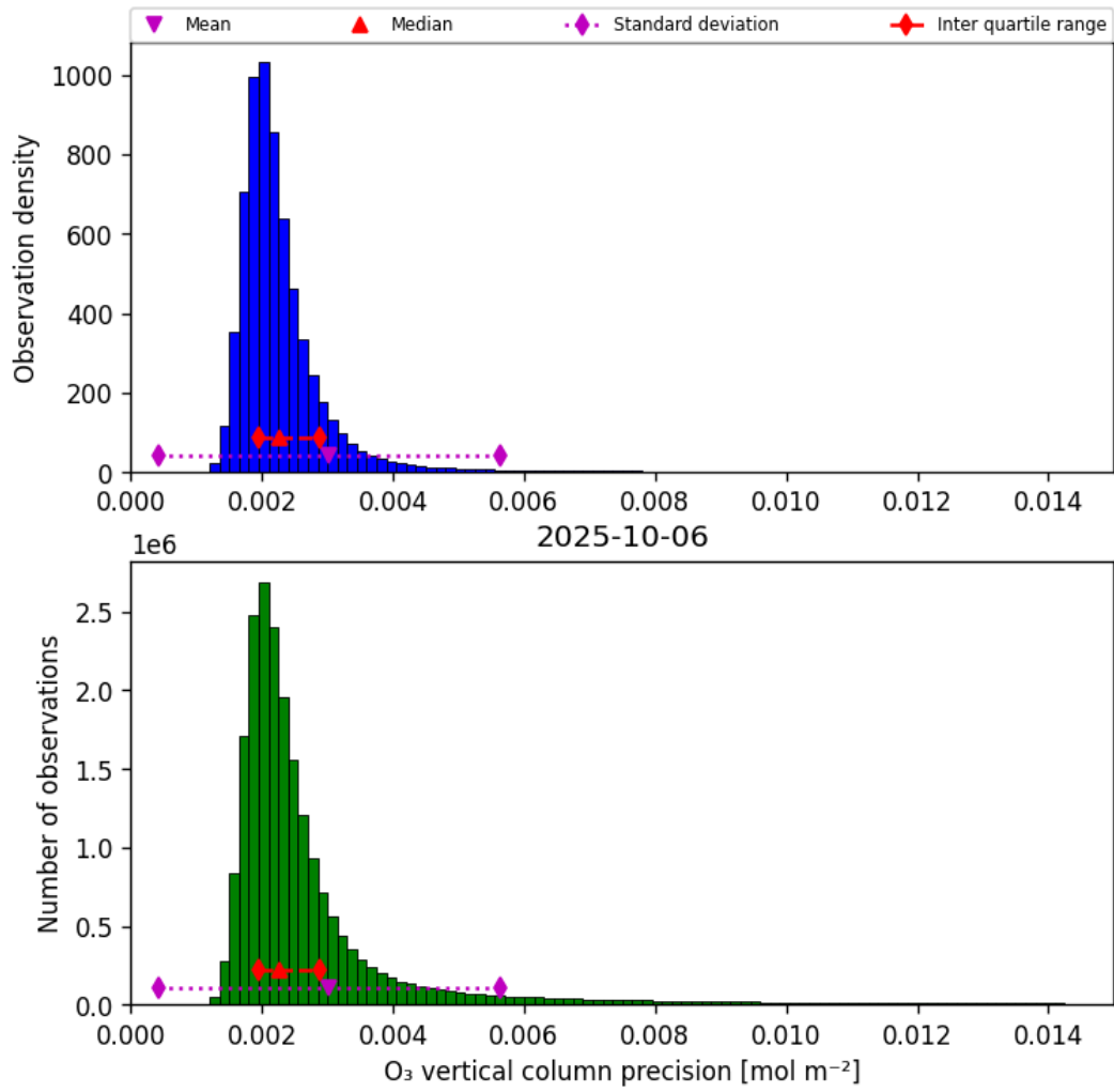
Figure 30: Histogram of “O 3 vertical column precision” for 2025-10-06 to 2025-10-07
