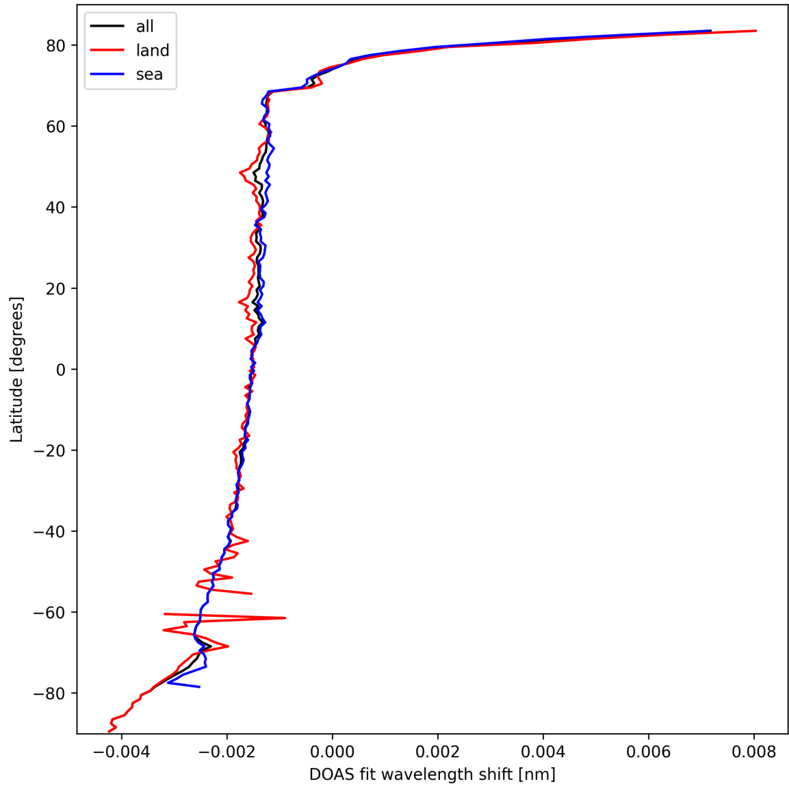
Figure 23: Zonal average of “DOAS fit wavelength shift” for 2025-10-06 to 2025-10-07.
