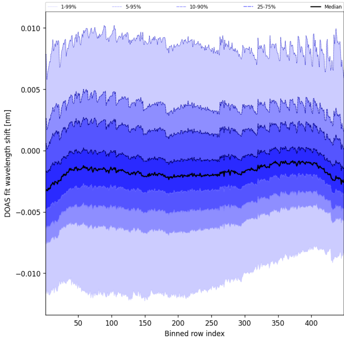
Figure 47: Along track statistics of “DOAS fit wavelength shift” for 2025-10-06 to 2025-10-07
