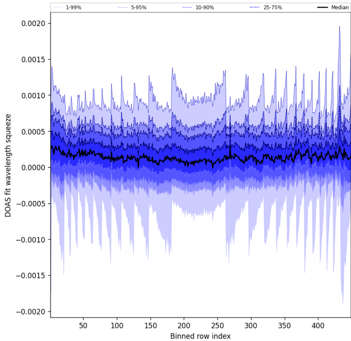
Figure 48: Along track statistics of “DOAS fit wavelength squeeze” for 2025-10-06 to 2025-10-07
