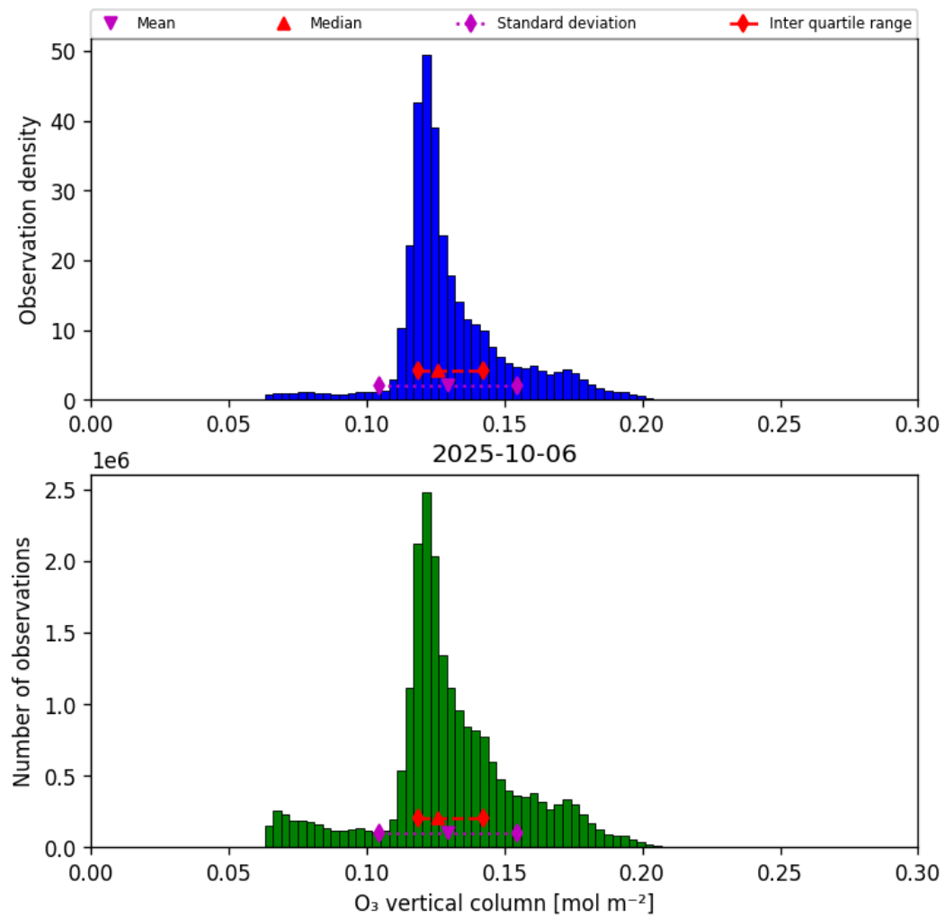
Figure 29: Histogram of “O 3 vertical column” for 2025-10-06 to 2025-10-07
