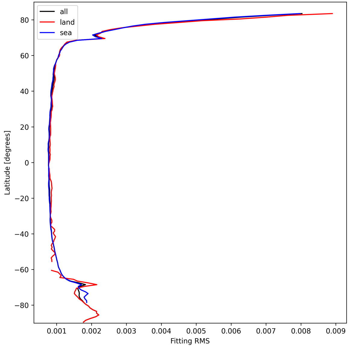
Figure 22: Zonal average of “Fitting RMS” for 2025-10-06 to 2025-10-07.
