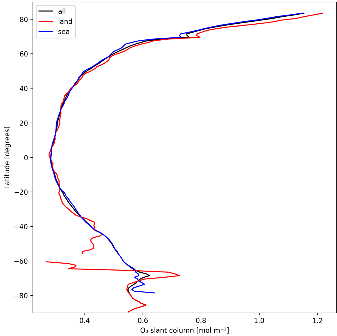
Figure 19: Zonal average of “O 3 slant column” for 2025-10-06 to 2025-10-07.
