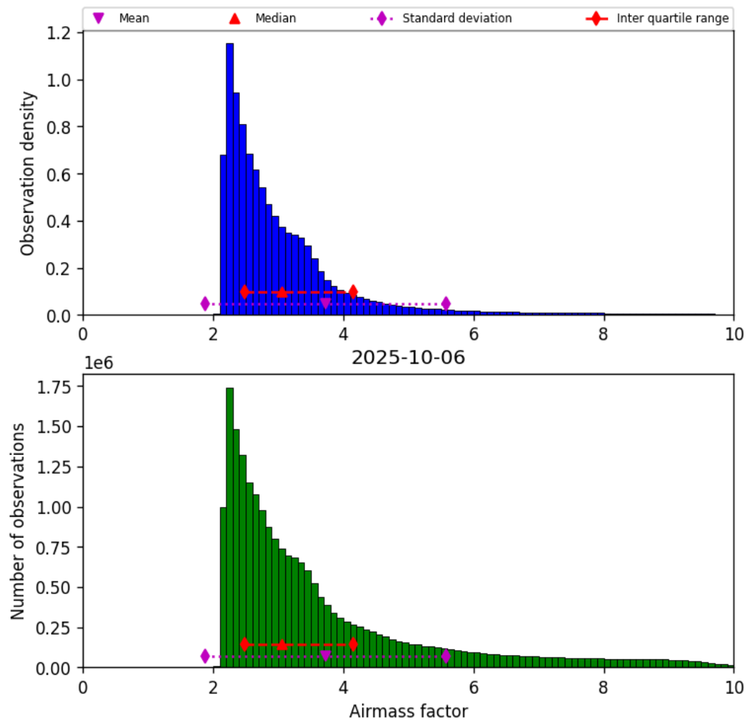
Figure 37: Histogram of “Airmass factor” for 2025-10-06 to 2025-10-07
