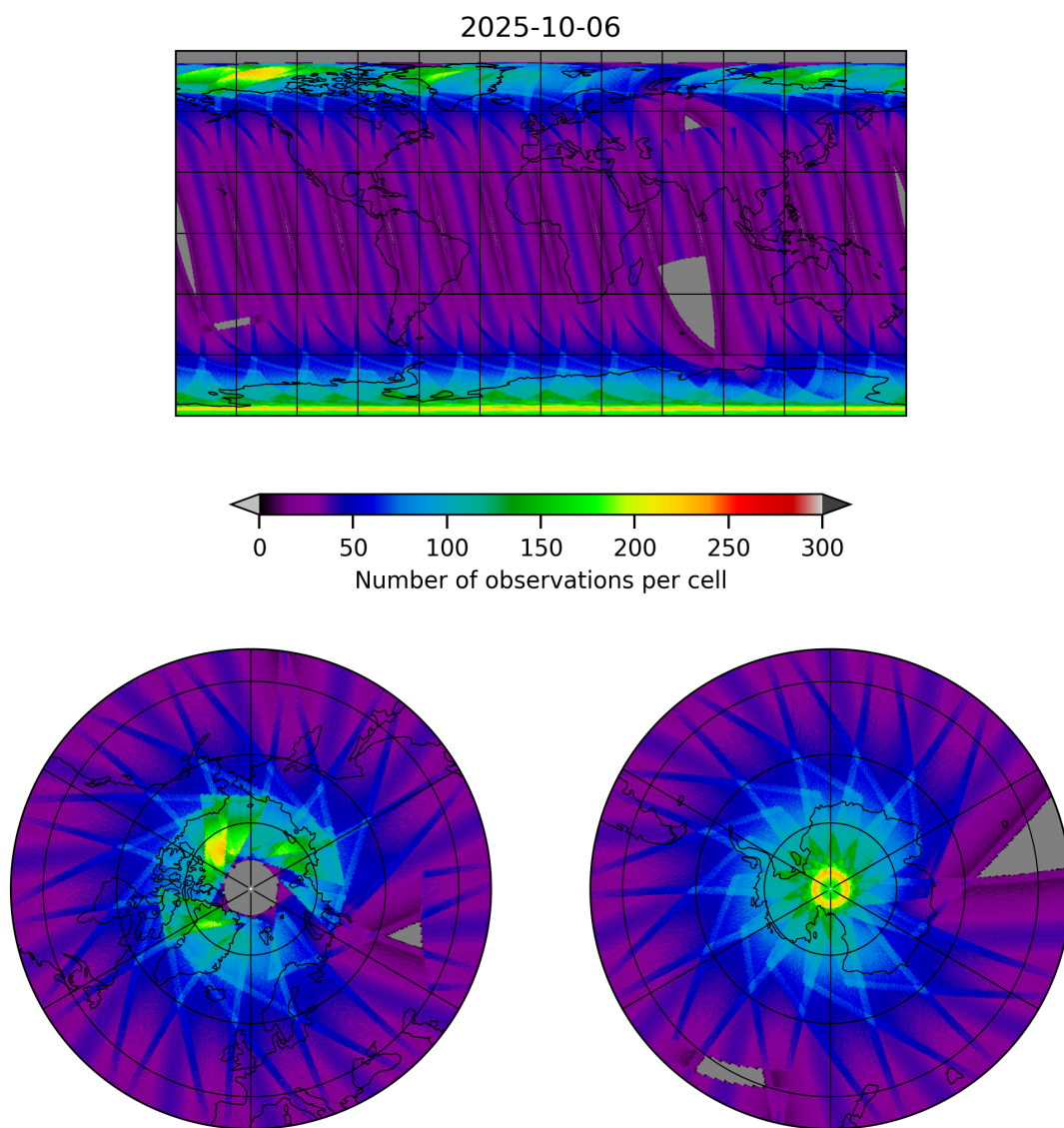
Figure 15: Map of the number of observations for 2025-10-06 to 2025-10-07
