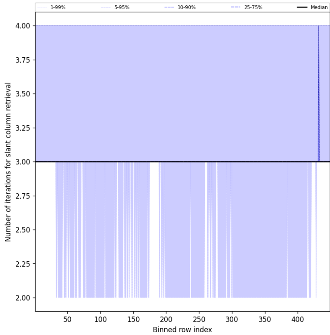
Figure 45: Along track statistics of “Number of iterations for slant column retrieval” for 2025-10-06 to 2025-10-07
