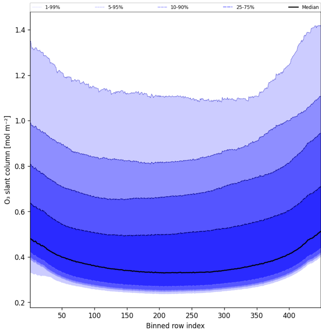
Figure 43: Along track statistics of “O 3 slant column” for 2025-10-06 to 2025-10-07
