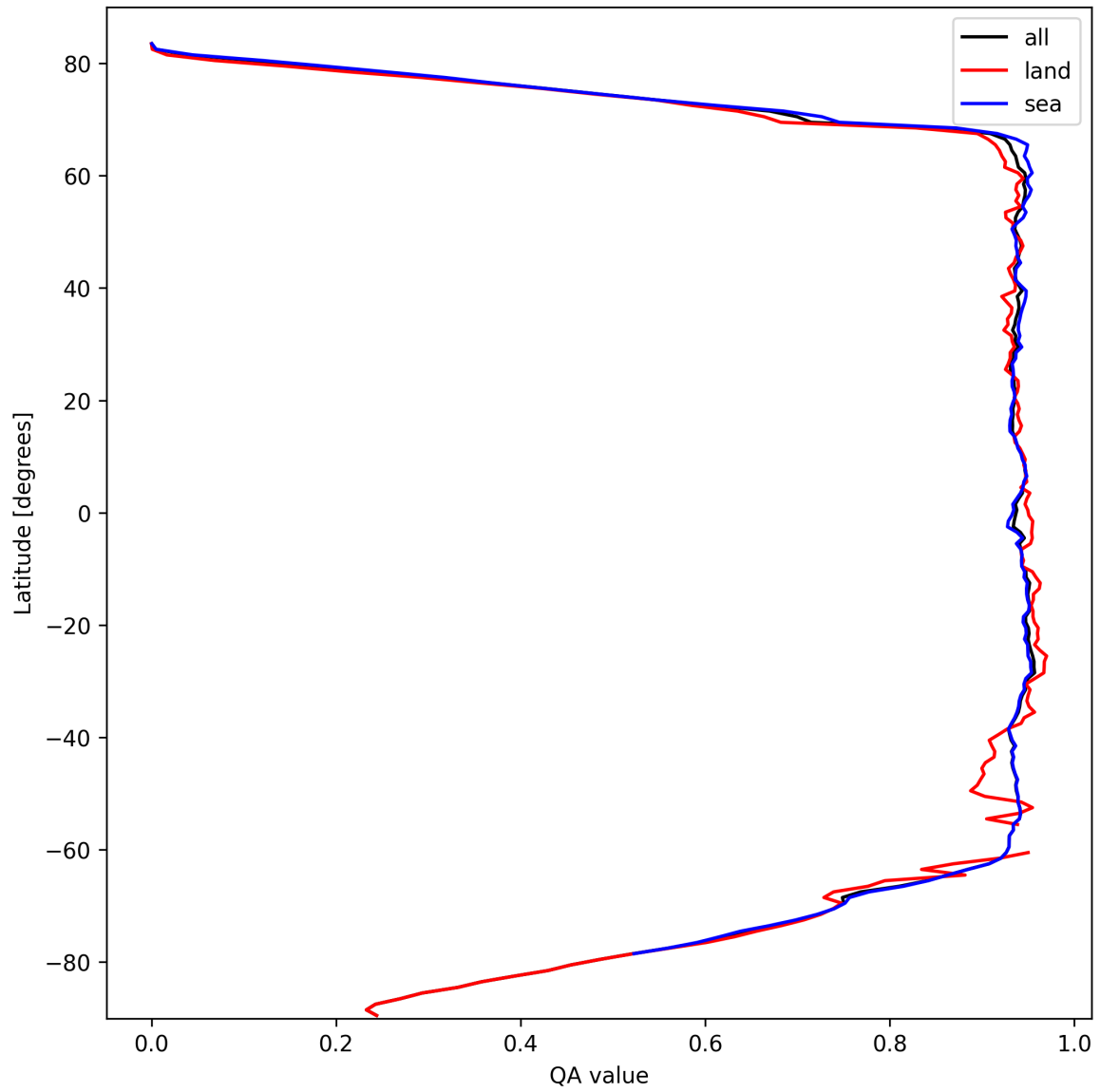
Figure 16: Zonal average of “QA value” for 2025-10-06 to 2025-10-07.
