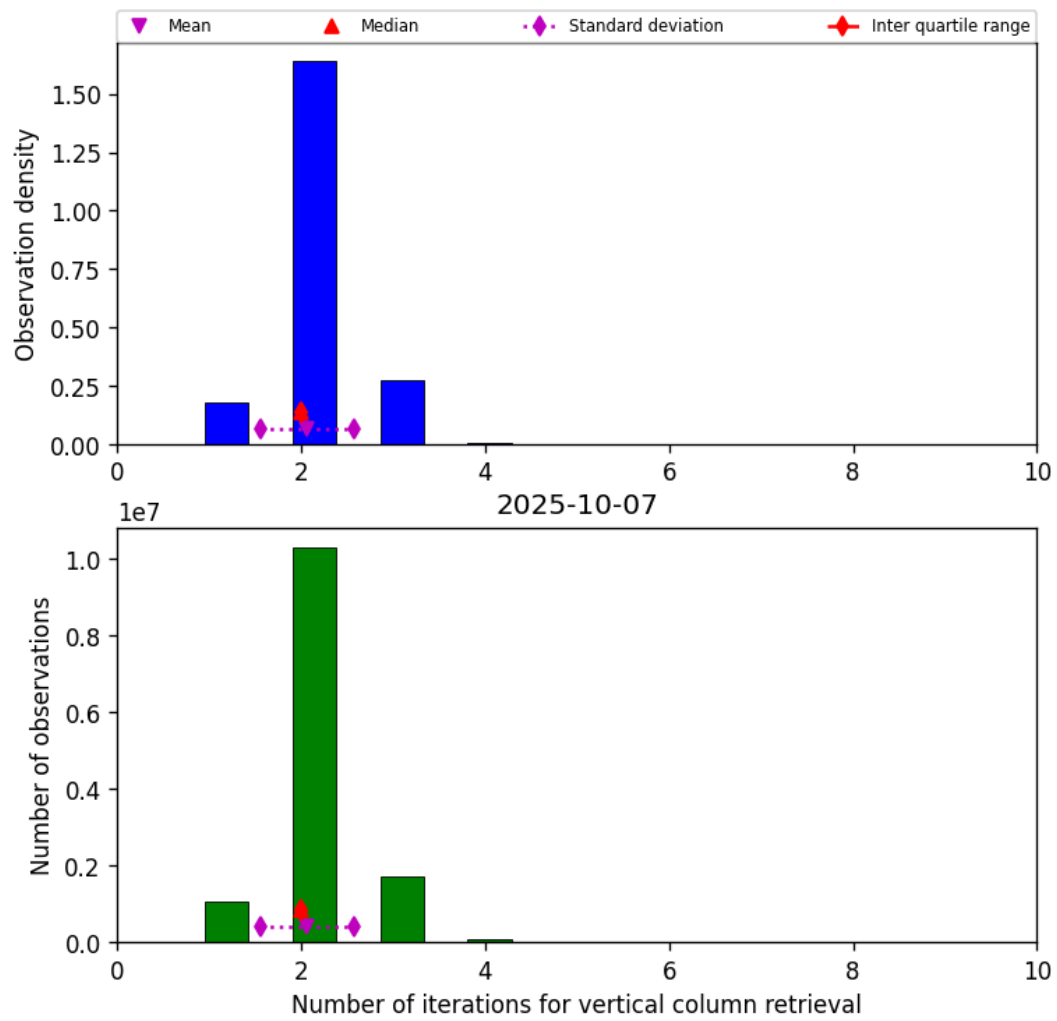
Figure 39: Histogram of “Number of iterations for vertical column retrieval” for 2025-10-07 to 2025-10-07
