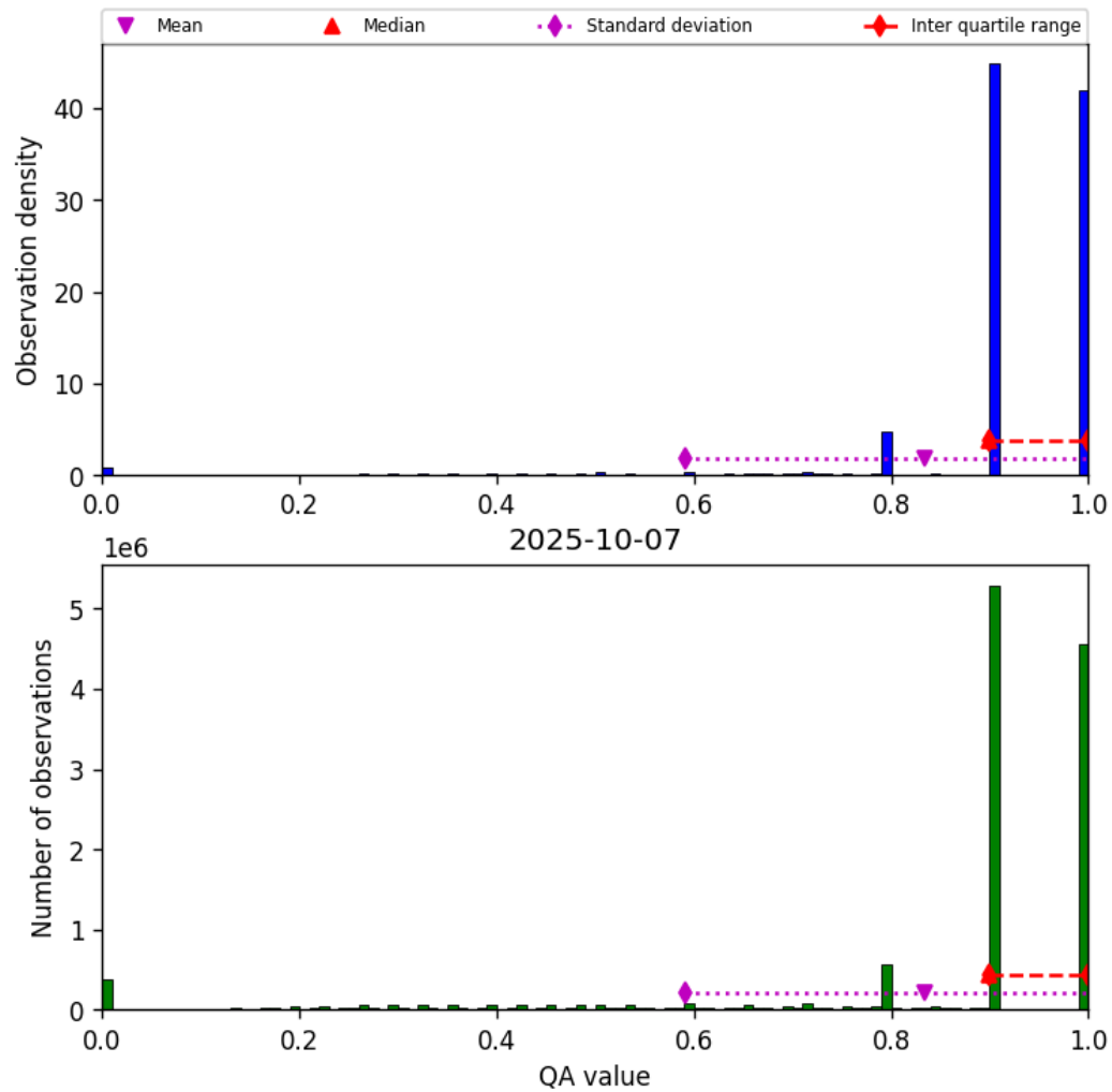
Figure 28: Histogram of “QA value” for 2025-10-07 to 2025-10-07
