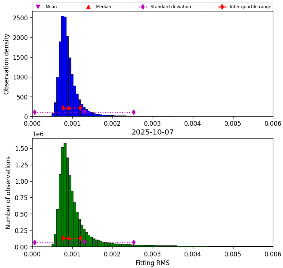
Figure 34: Histogram of “Fitting RMS” for 2025-10-07 to 2025-10-07
