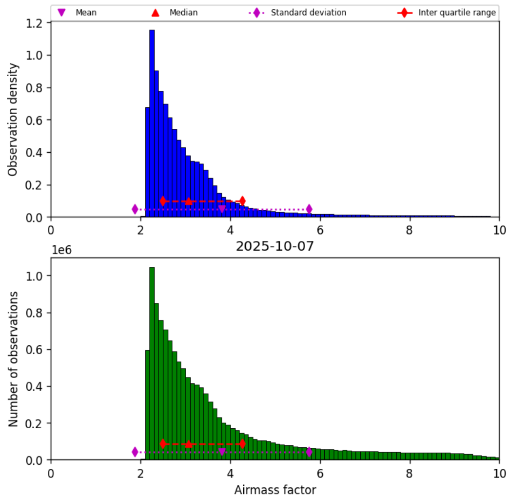
Figure 37: Histogram of “Airmass factor” for 2025-10-07 to 2025-10-07
