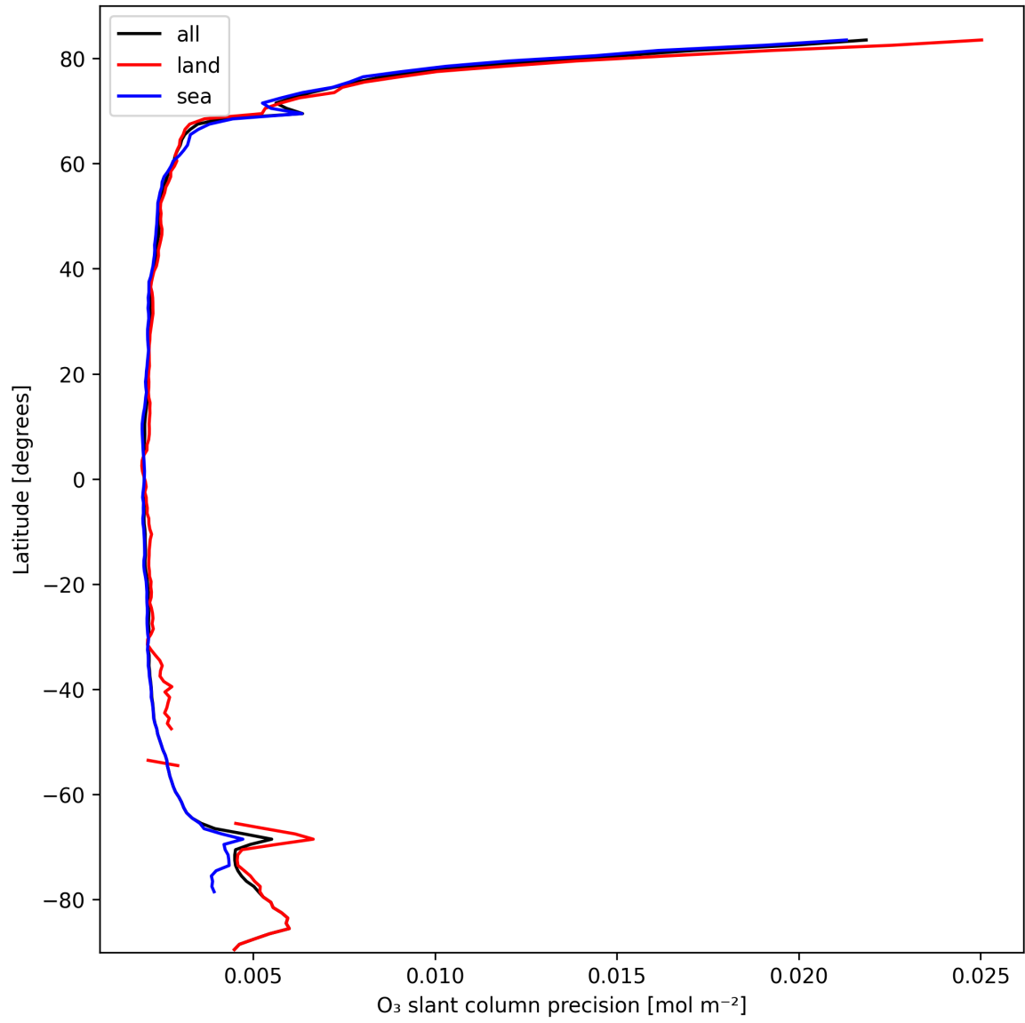
Figure 20: Zonal average of “O 3 slant column precision” for 2025-10-07 to 2025-10-07.
