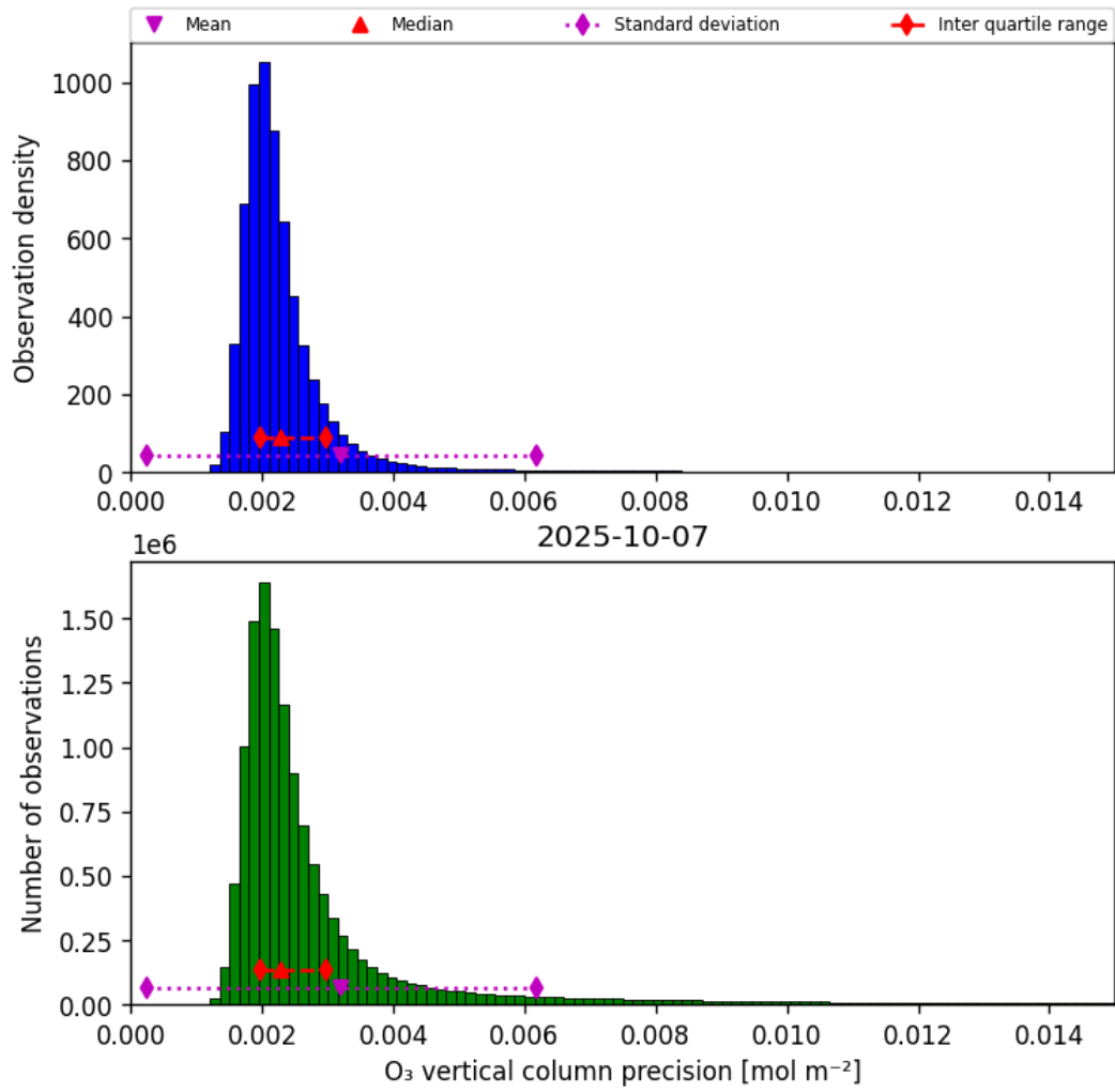
Figure 30: Histogram of “O 3 vertical column precision” for 2025-10-07 to 2025-10-07
