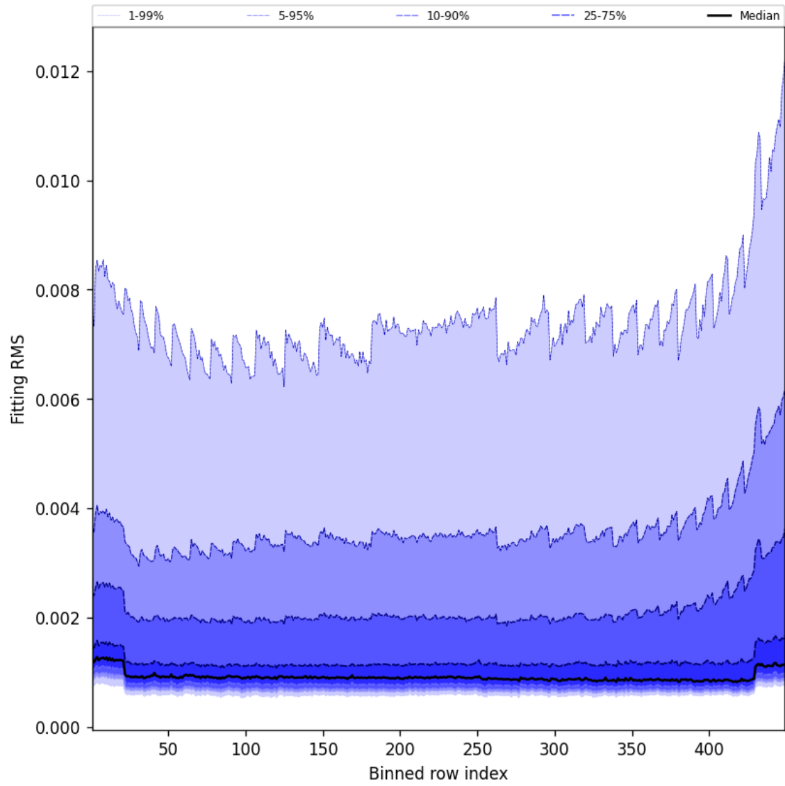
Figure 46: Along track statistics of “Fitting RMS” for 2025-10-07 to 2025-10-07
