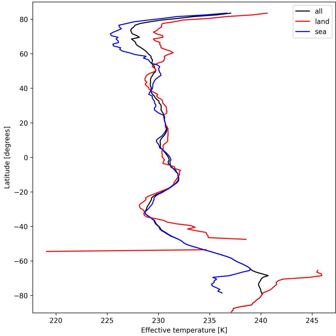
Figure 26: Zonal average of “Effective temperature” for 2025-10-07 to 2025-10-07.
