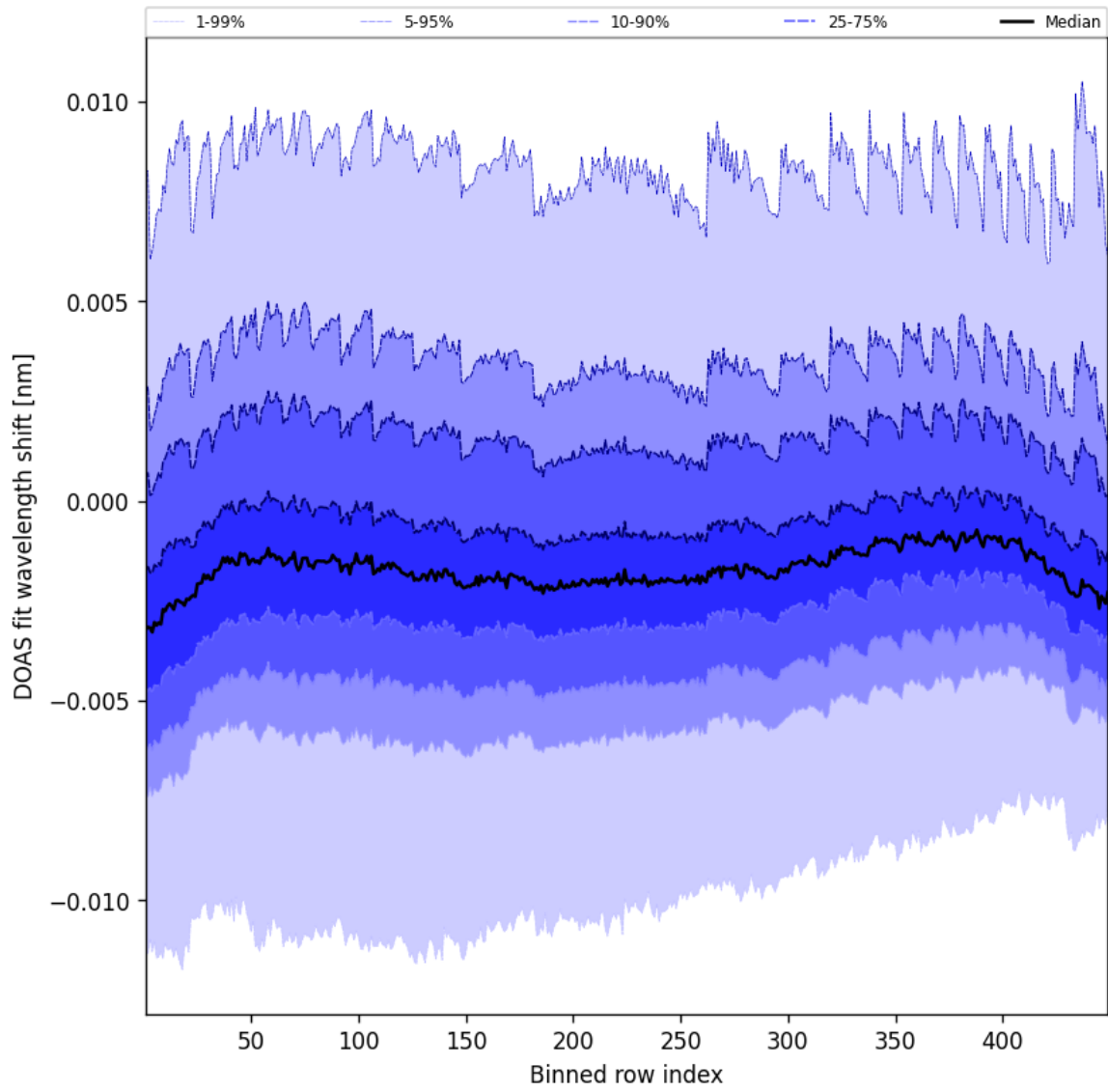
Figure 47: Along track statistics of “DOAS fit wavelength shift” for 2025-10-07 to 2025-10-07
