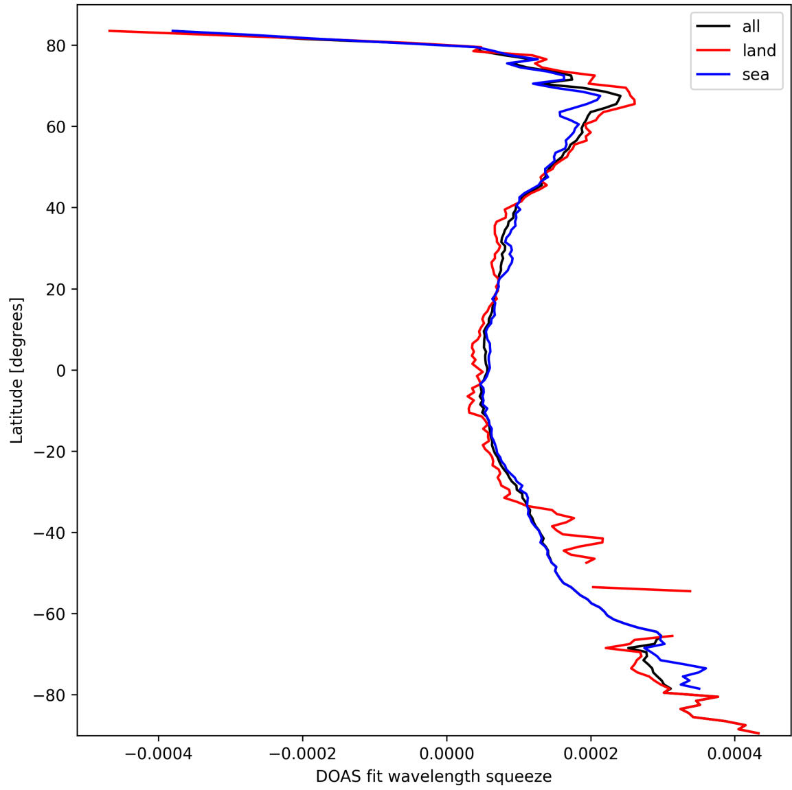
Figure 24: Zonal average of “DOAS fit wavelength squeeze” for 2025-10-07 to 2025-10-07.
