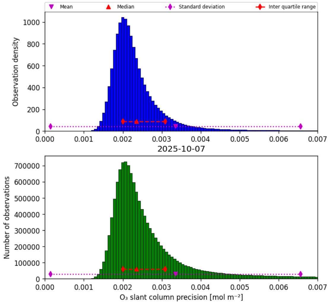
Figure 32: Histogram of "O 3 slant column precision" for 2025-10-07 to 2025-10-07
