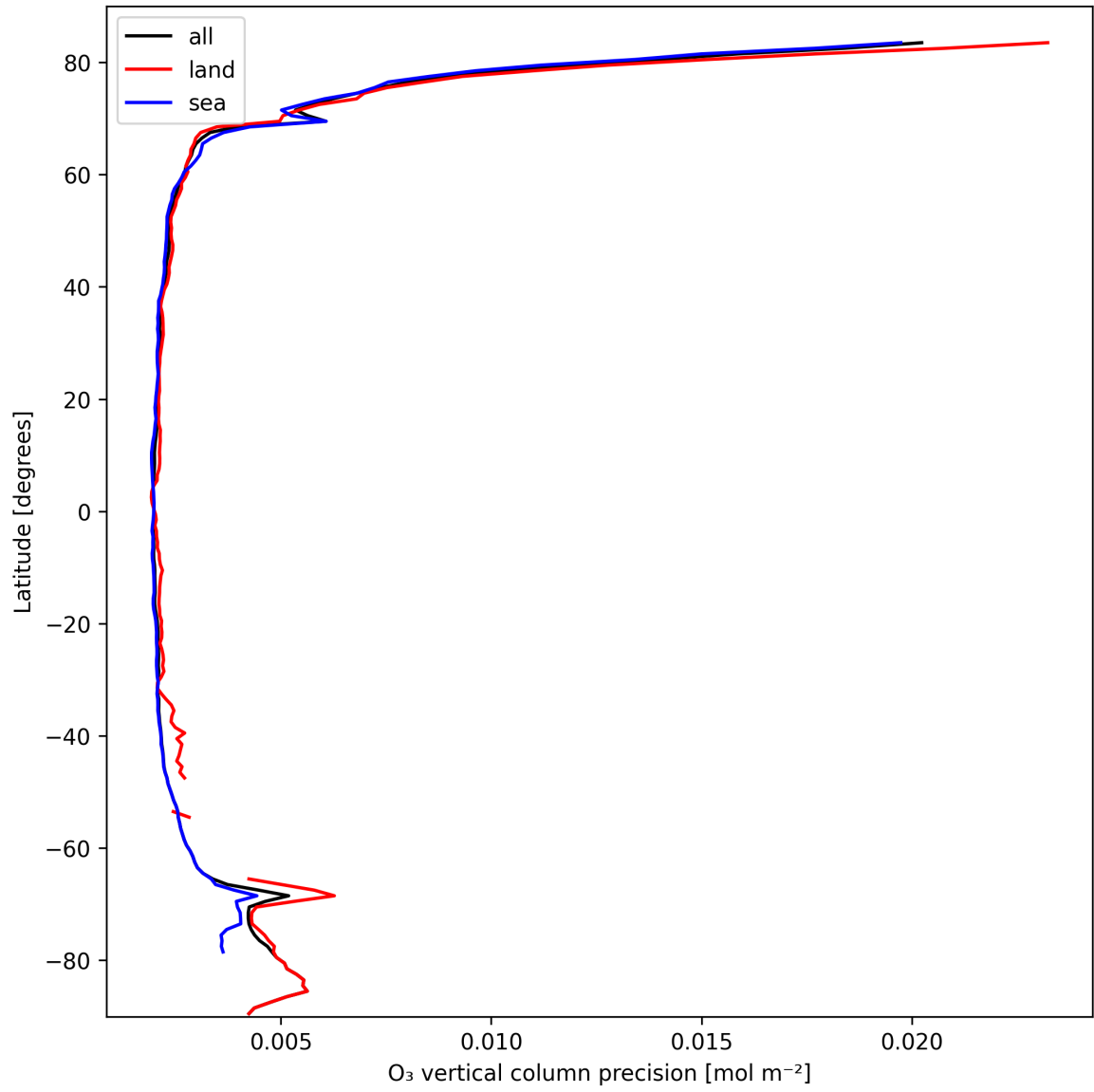
Figure 18: Zonal average of “O 3 vertical column precision” for 2025-10-07 to 2025-10-07.
