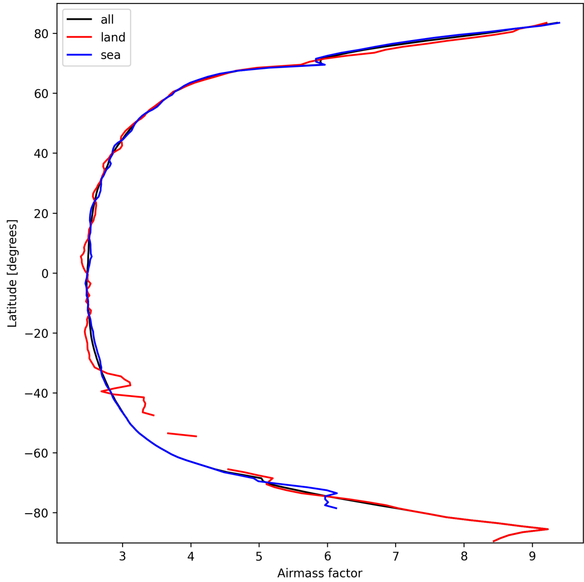
Figure 25: Zonal average of “Airmass factor” for 2025-10-07 to 2025-10-07.
