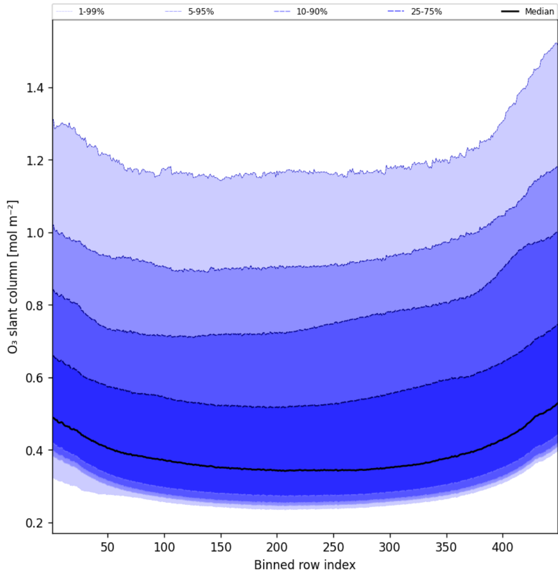
Figure 43: Along track statistics of “O 3 slant column” for 2025-10-07 to 2025-10-07
