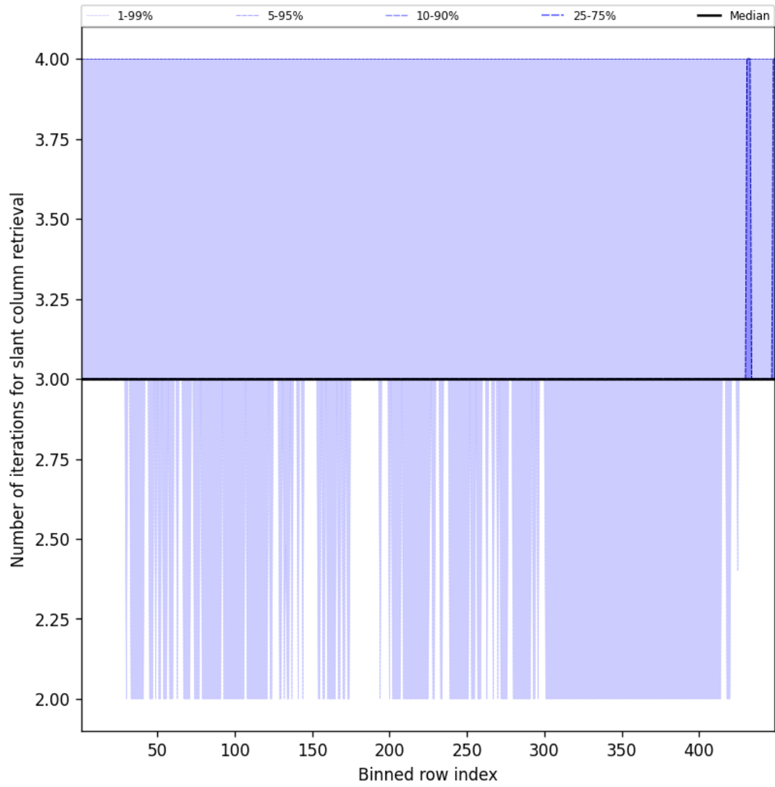
Figure 45: Along track statistics of “Number of iterations for slant column retrieval” for 2025-10-07 to 2025-10-07
