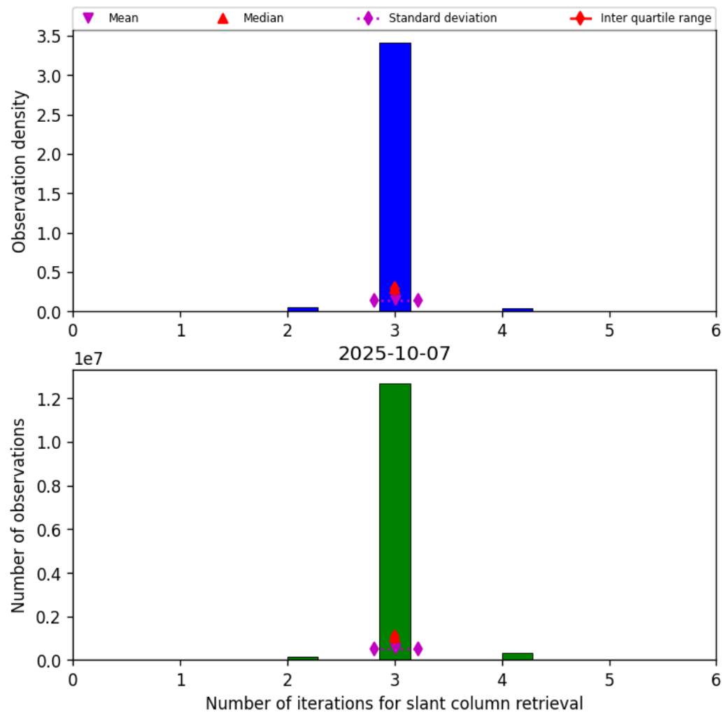
Figure 33: Histogram of “Number of iterations for slant column retrieval” for 2025-10-07 to 2025-10-07
