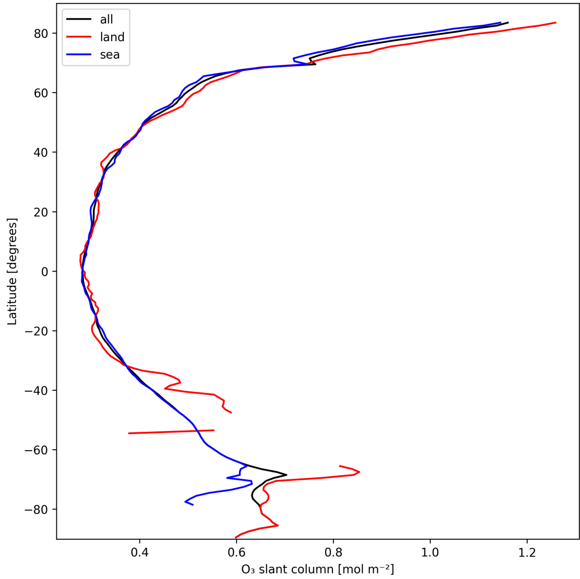
Figure 19: Zonal average of “O 3 slant column” for 2025-10-07 to 2025-10-07.
