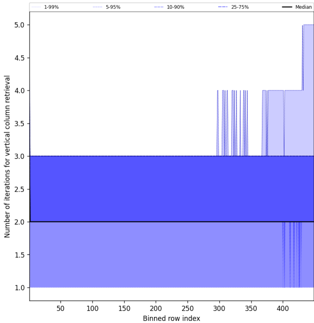
Figure 51: Along track statistics of “Number of iterations for vertical column retrieval” for 2025-10-07 to 2025-10-07
