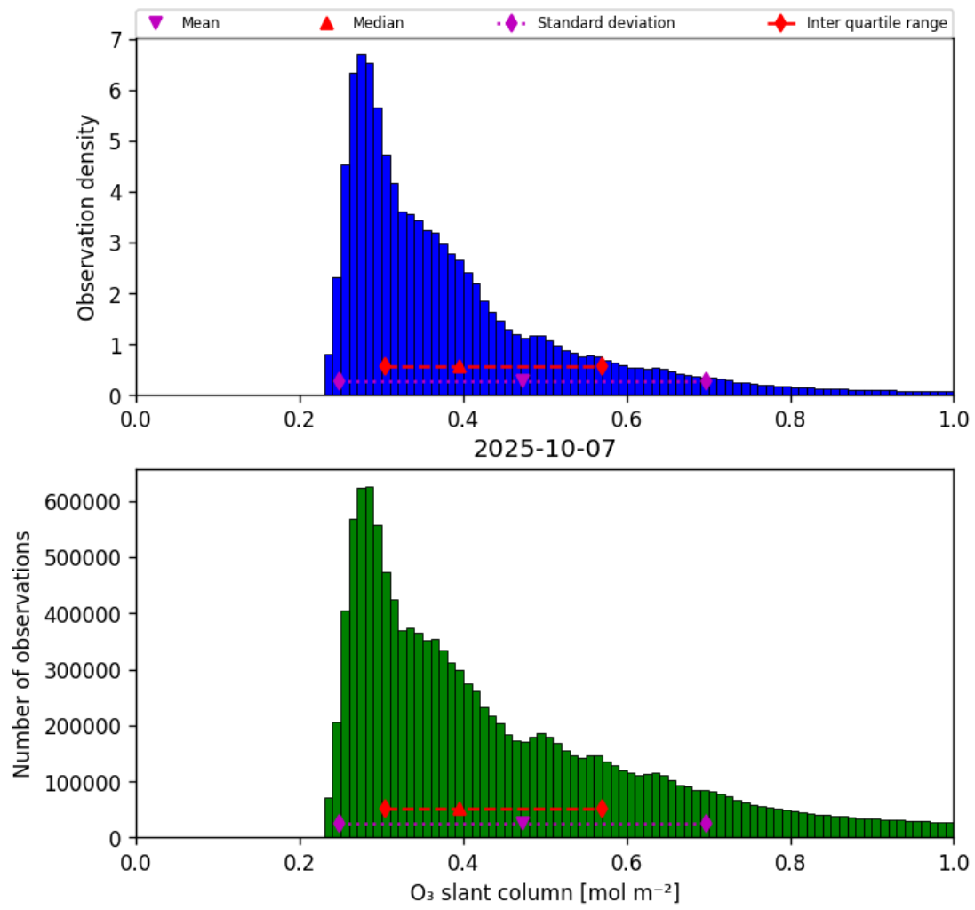
Figure 31: Histogram of “O 3 slant column” for 2025-10-07 to 2025-10-07
