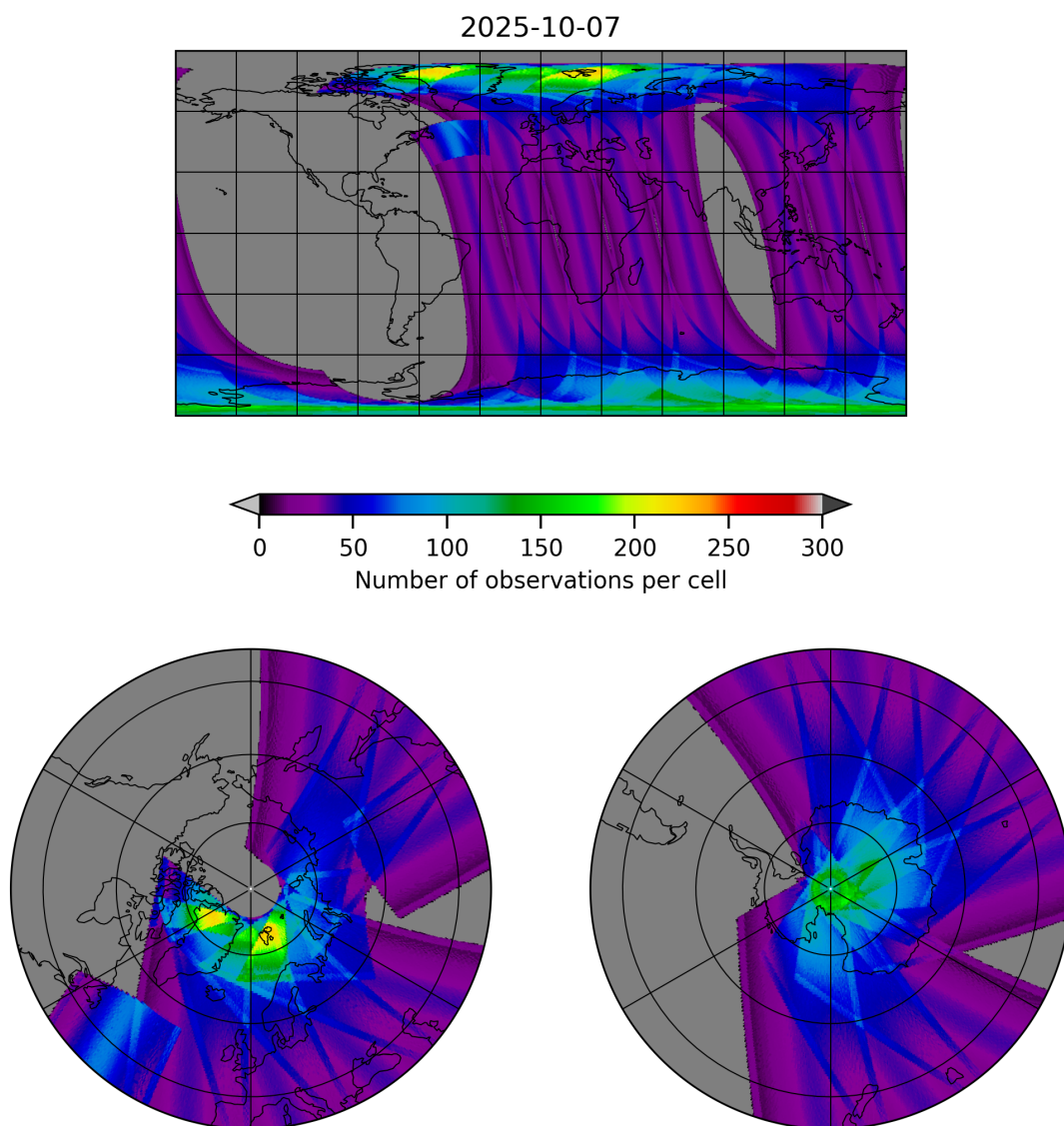
Figure 15: Map of the number of observations for 2025-10-07 to 2025-10-07
