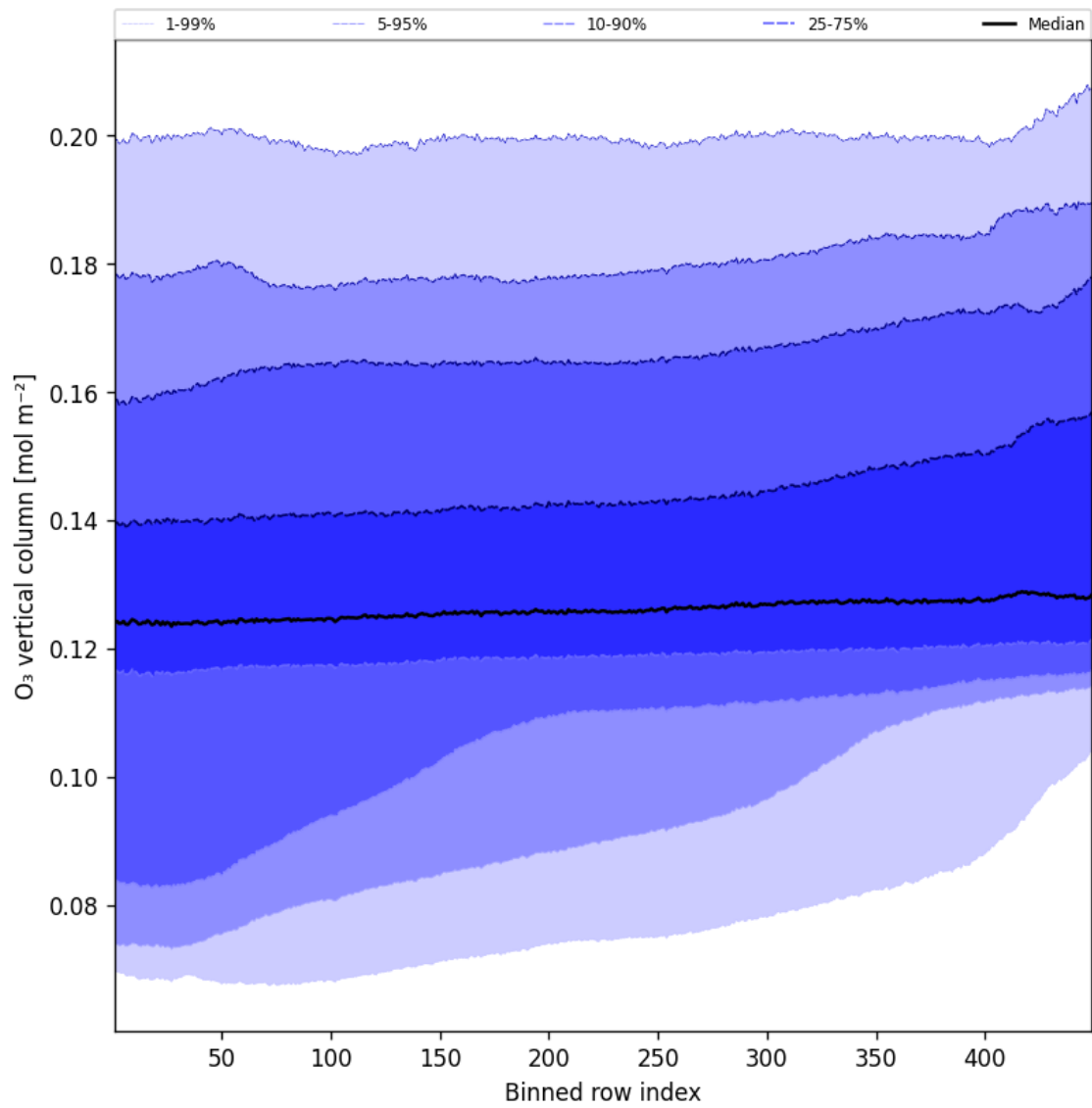
Figure 41: Along track statistics of “O 3 vertical column” for 2025-10-07 to 2025-10-07
