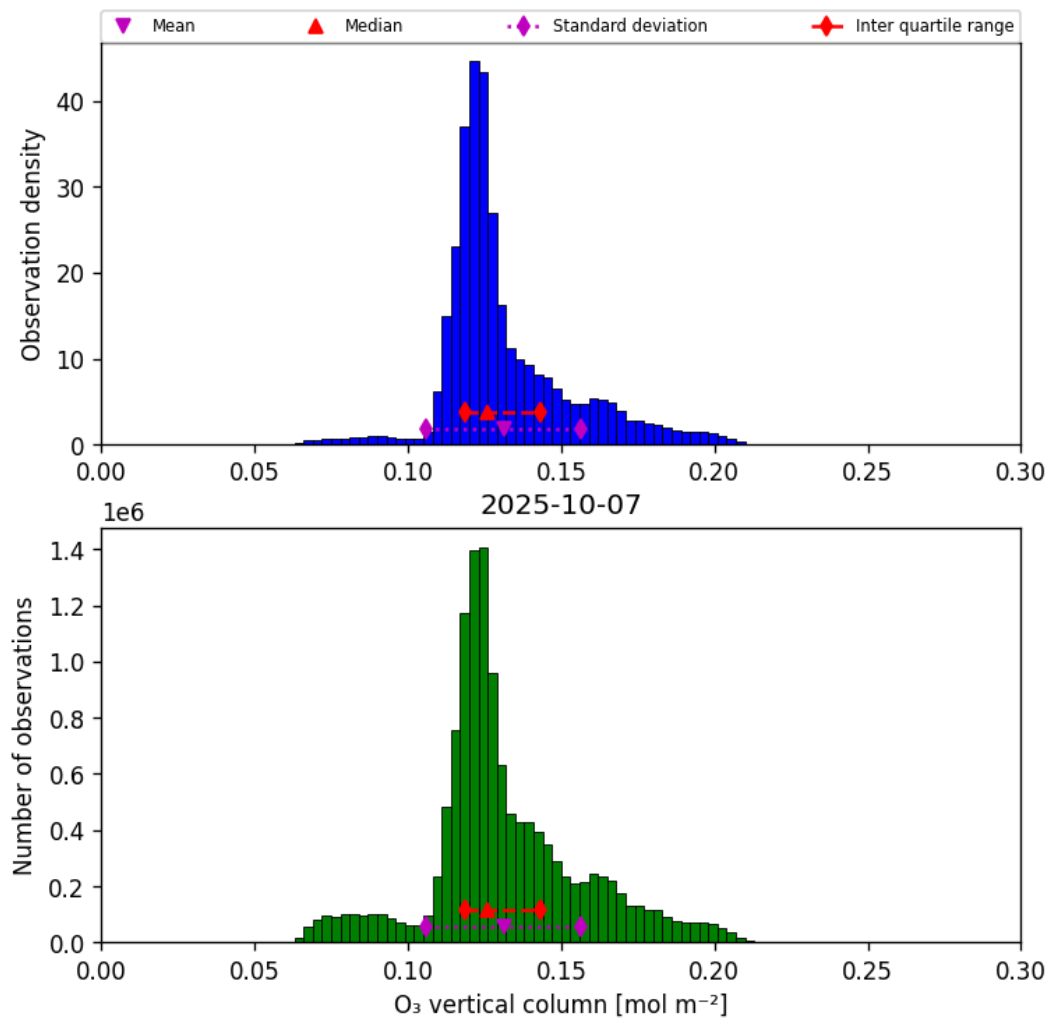
Figure 29: Histogram of “O 3 vertical column” for 2025-10-07 to 2025-10-07
