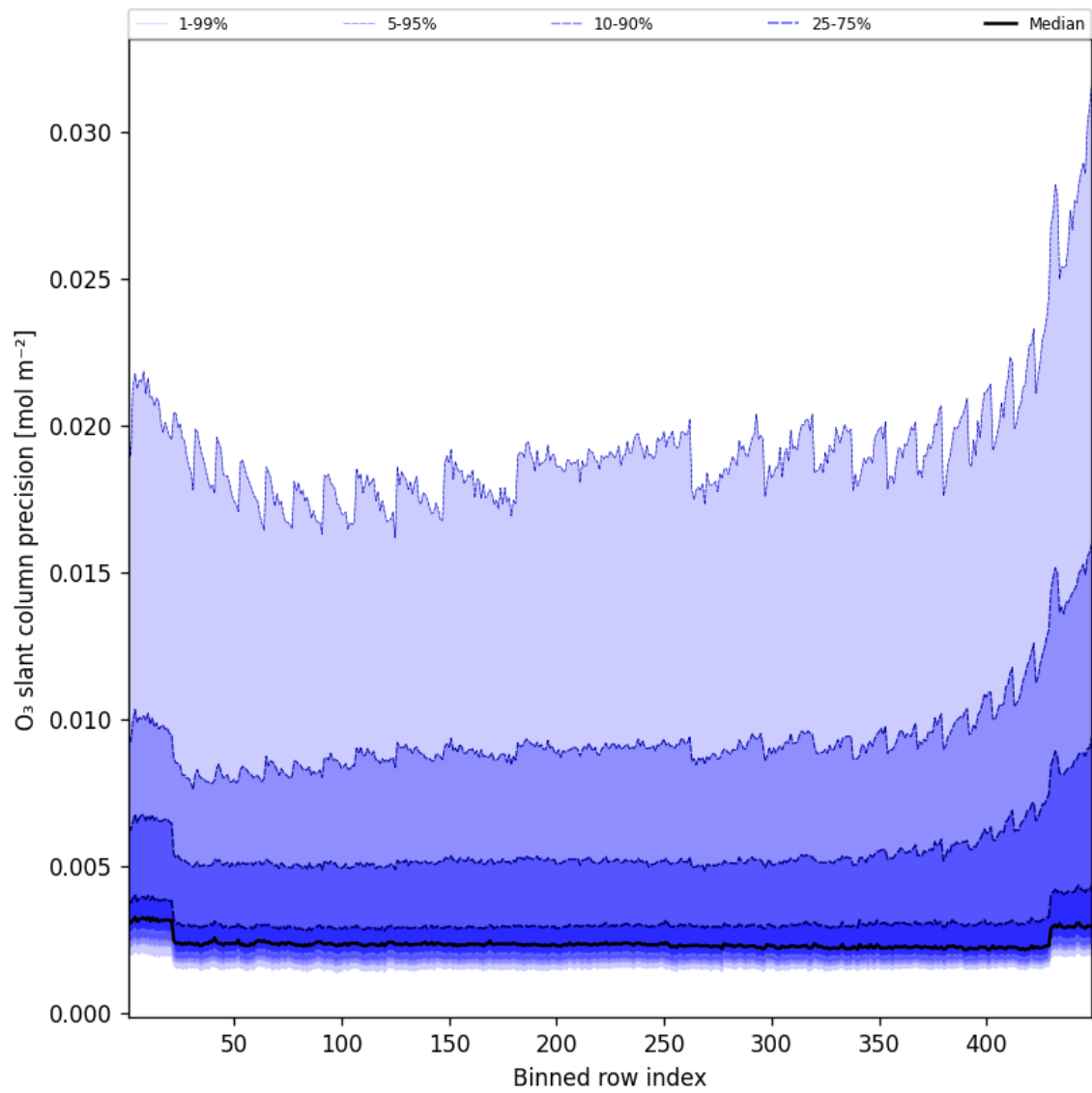
Figure 44: Along track statistics of “O 3 slant column precision” for 2025-10-07 to 2025-10-07
