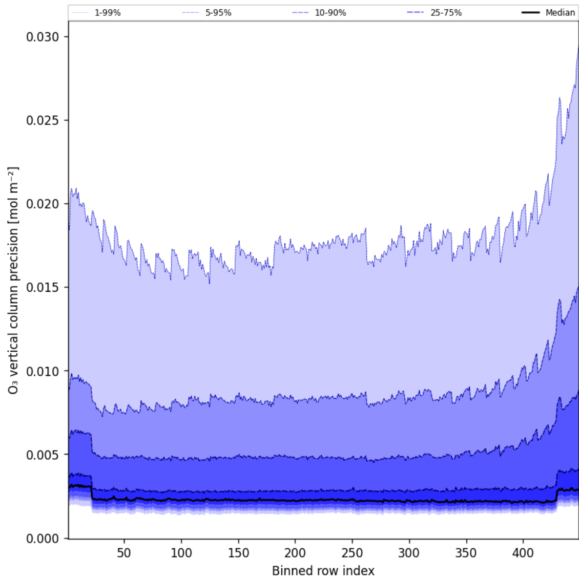
Figure 42: Along track statistics of “O 3 vertical column precision” for 2025-10-07 to 2025-10-07
