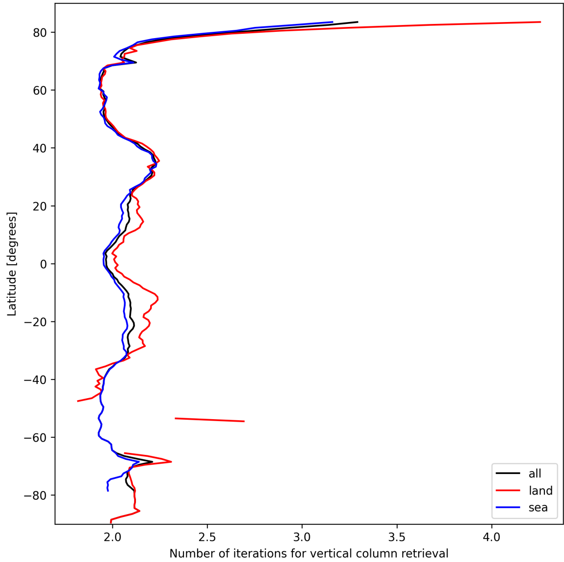
Figure 27: Zonal average of “Number of iterations for vertical column retrieval” for 2025-10-07 to 2025-10-07.
