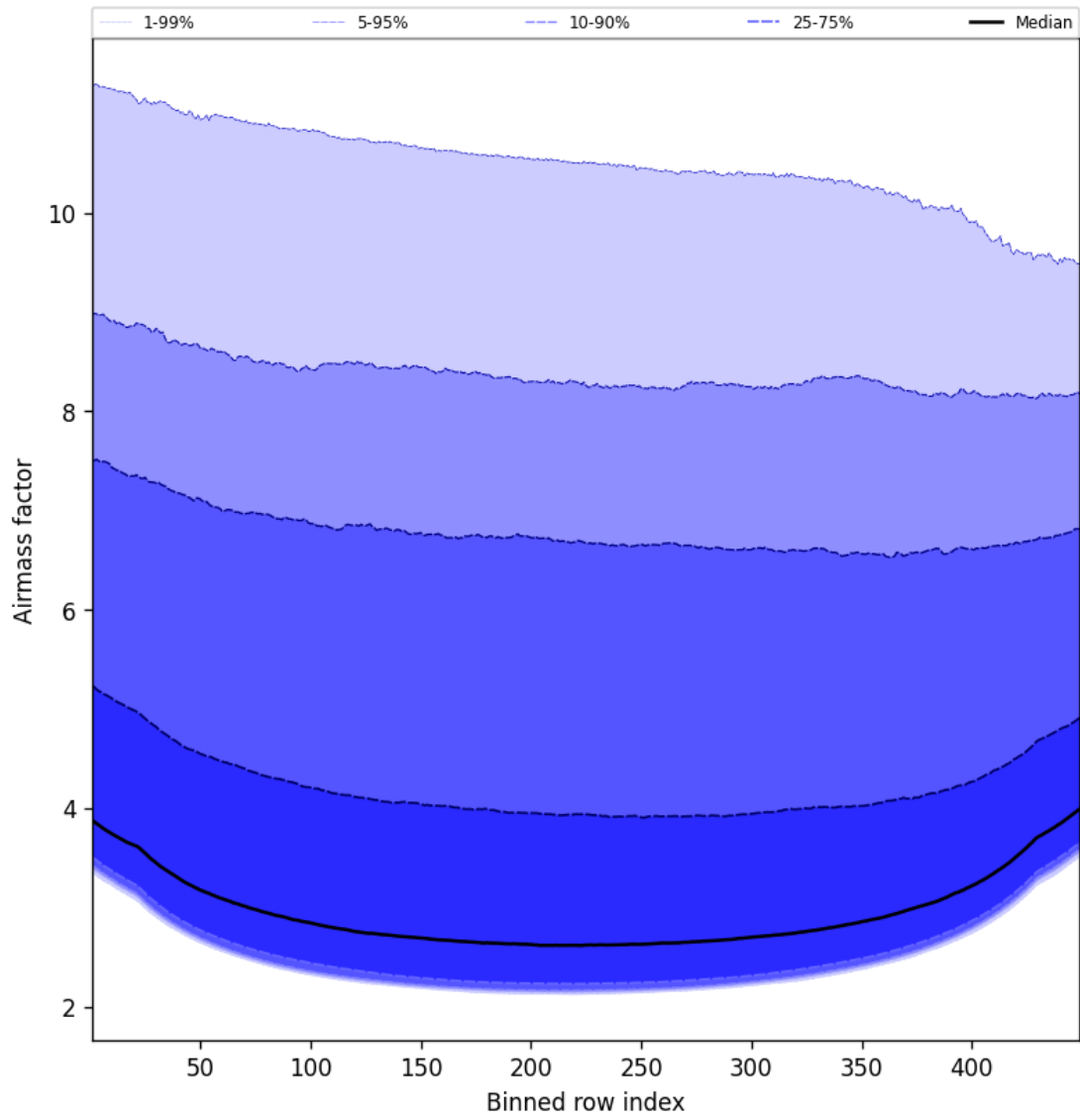
Figure 49: Along track statistics of “Airmass factor” for 2025-10-07 to 2025-10-07
