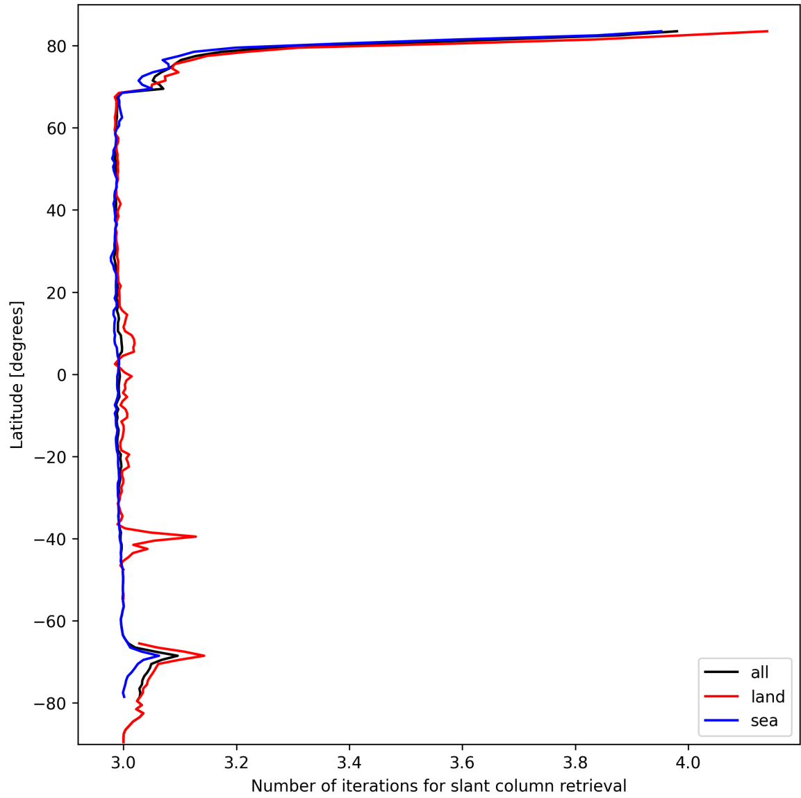
Figure 21: Zonal average of “Number of iterations for slant column retrieval” for 2025-10-07 to 2025-10-07.
