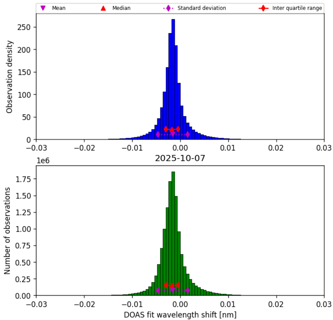
Figure 35: Histogram of “DOAS fit wavelength shift” for 2025-10-07 to 2025-10-07
