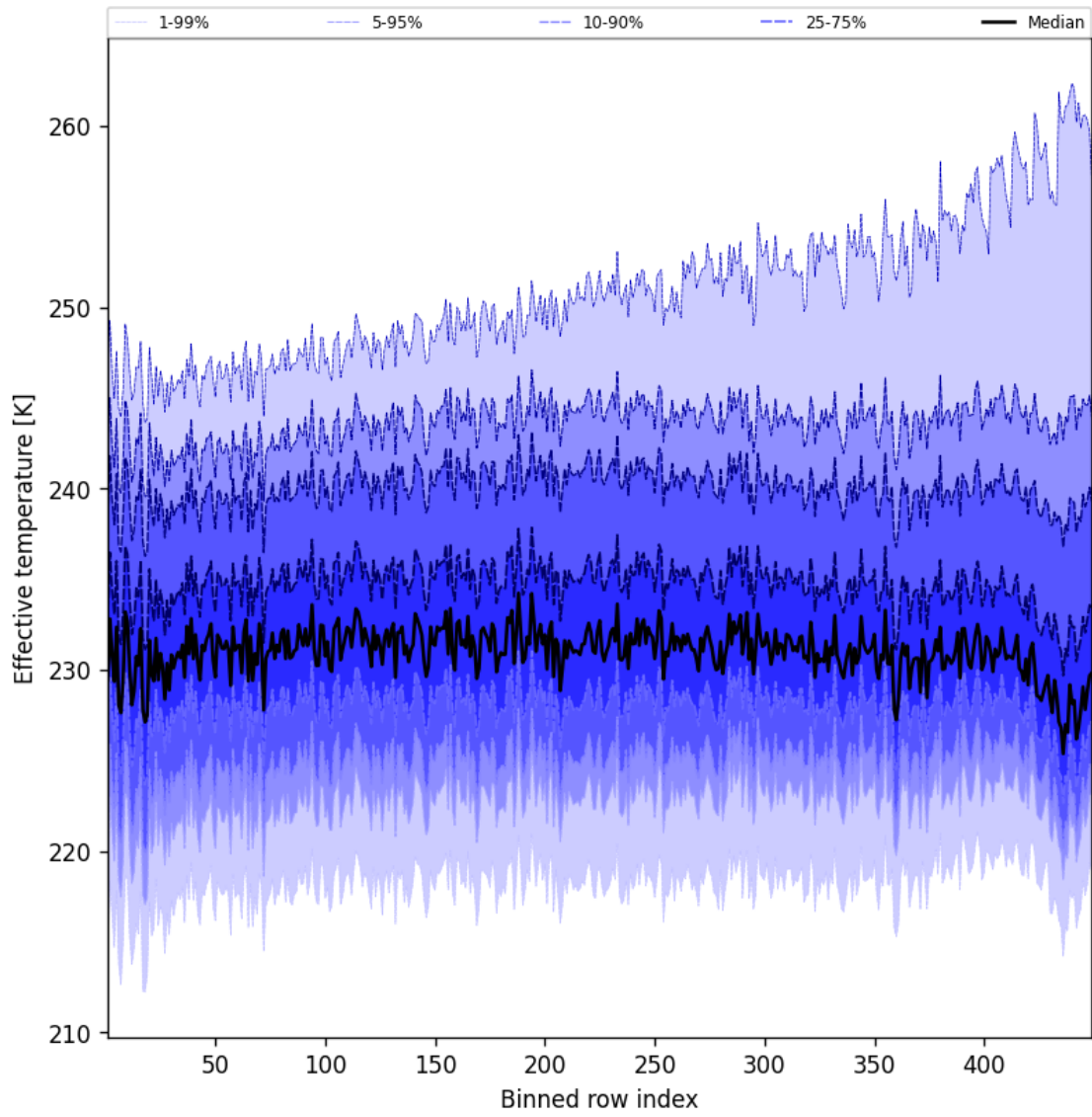
Figure 50: Along track statistics of “Effective temperature” for 2025-10-07 to 2025-10-07
