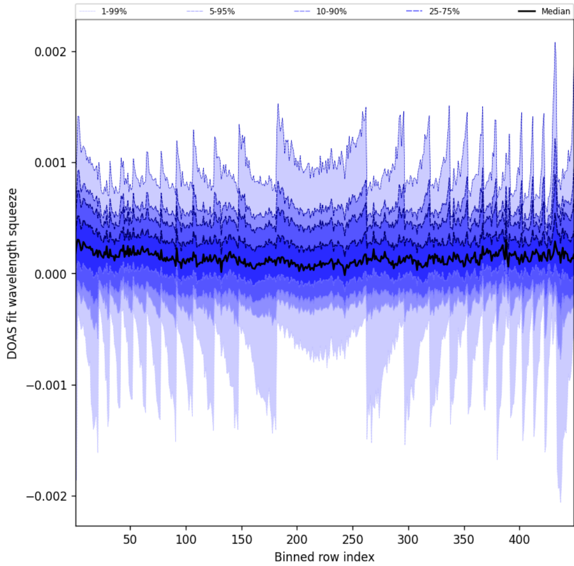
Figure 48: Along track statistics of “DOAS fit wavelength squeeze” for 2025-10-07 to 2025-10-07
