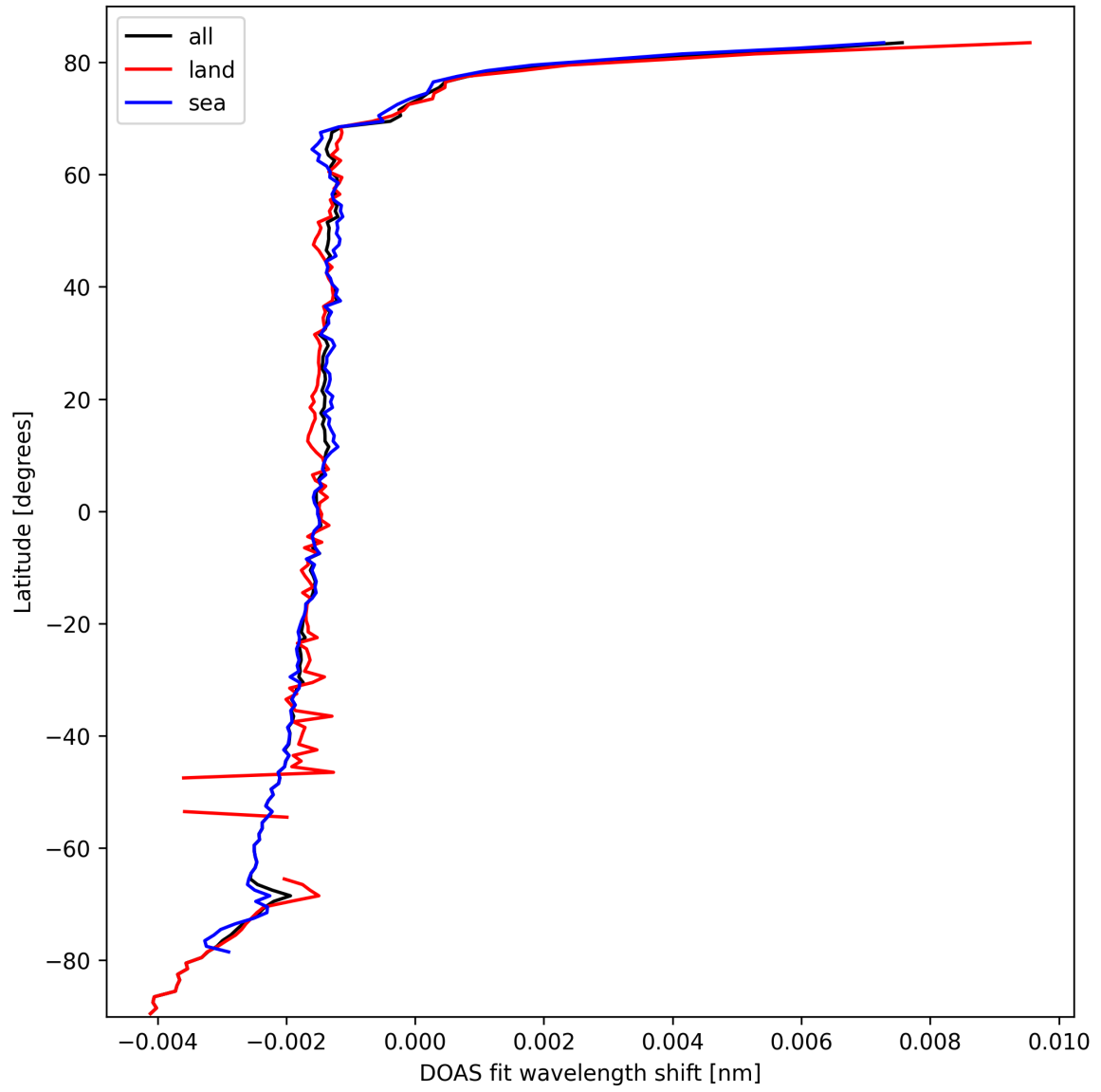
Figure 23: Zonal average of “DOAS fit wavelength shift” for 2025-10-07 to 2025-10-07.
