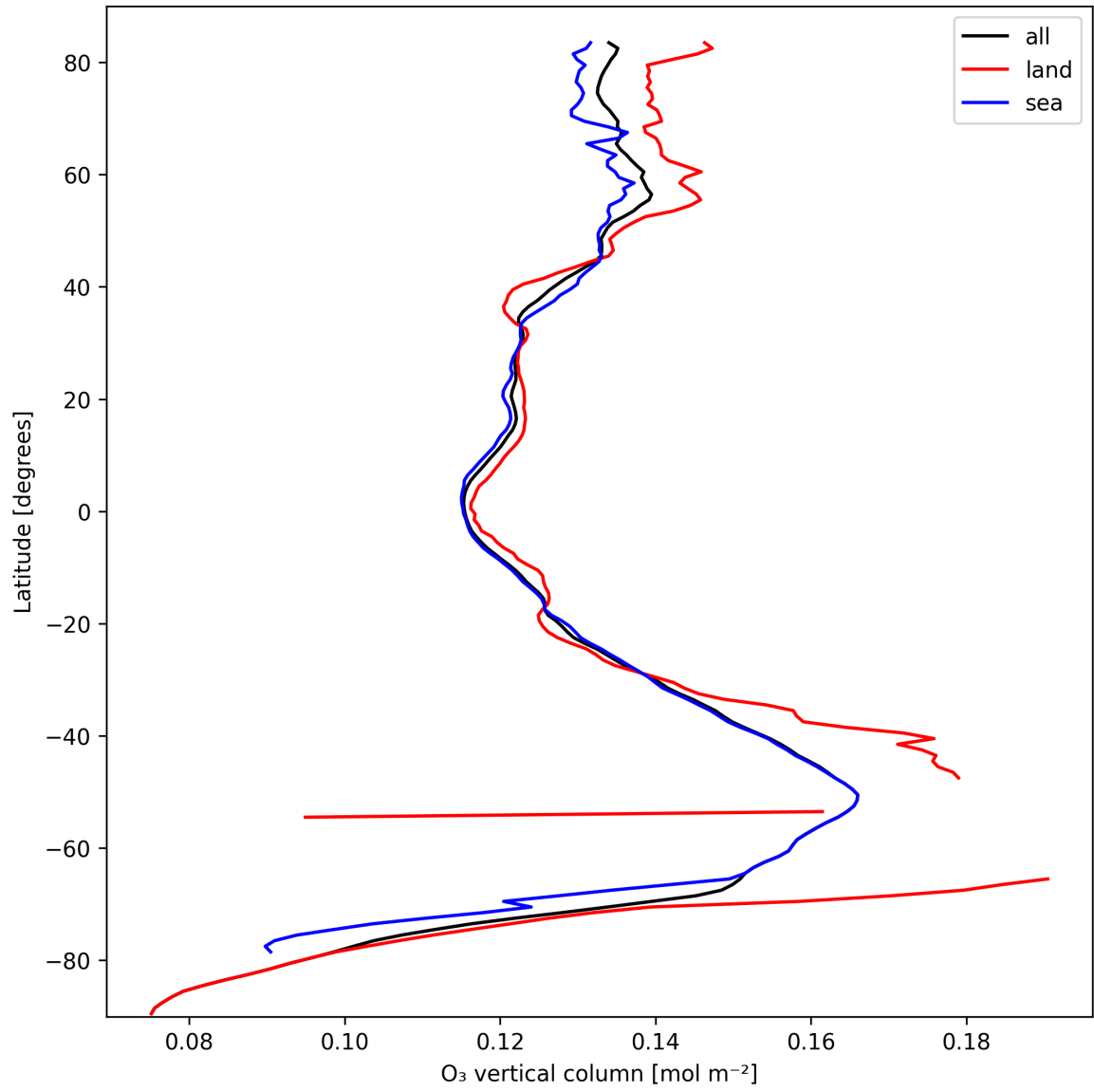
Figure 17: Zonal average of “O 3 vertical column” for 2025-10-07 to 2025-10-07.
