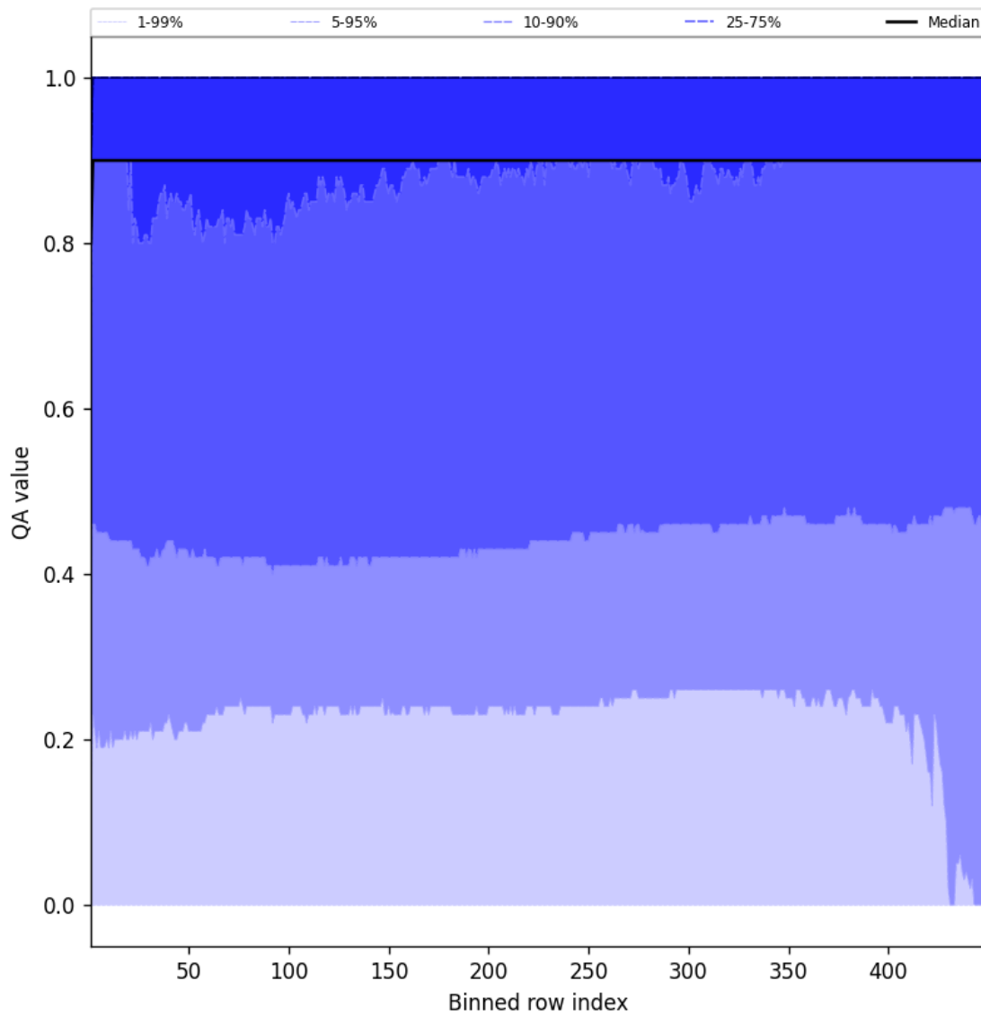
Figure 40: Along track statistics of “QA value” for 2025-10-07 to 2025-10-07
