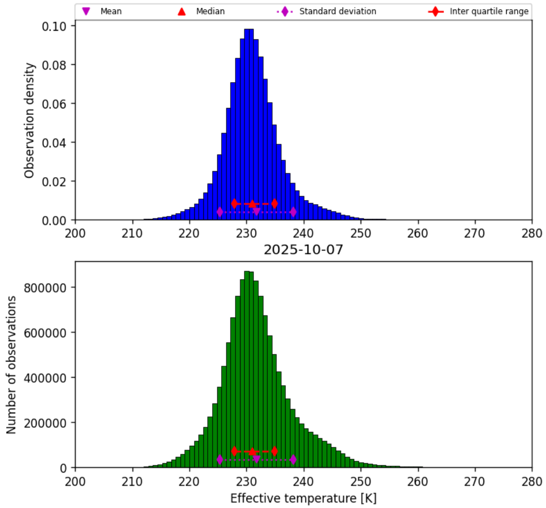
Figure 38: Histogram of “Effective temperature” for 2025-10-07 to 2025-10-07
