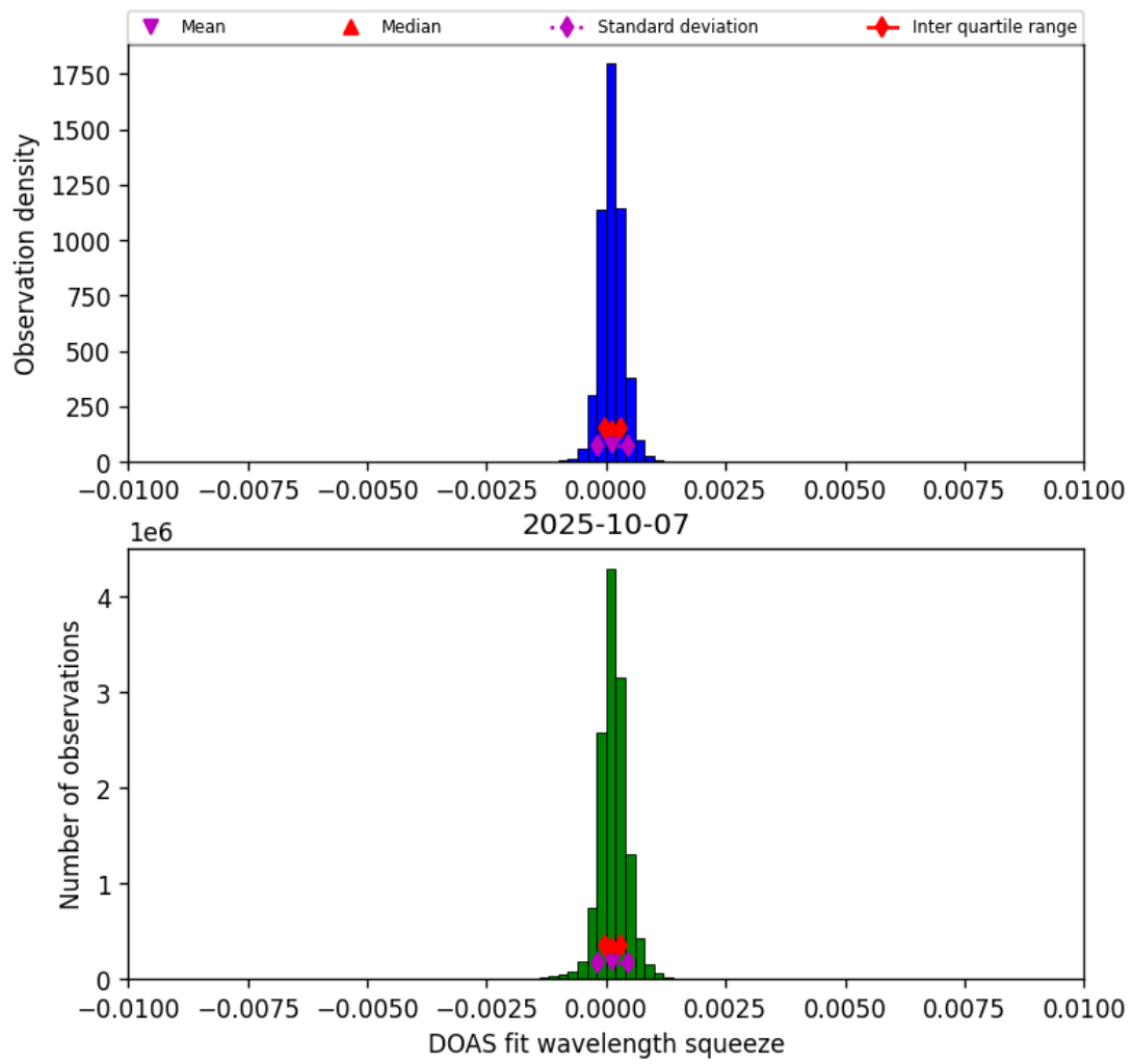
Figure 36: Histogram of “DOAS fit wavelength squeeze” for 2025-10-07 to 2025-10-07
