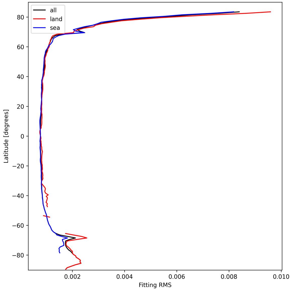
Figure 22: Zonal average of “Fitting RMS” for 2025-10-07 to 2025-10-07.
