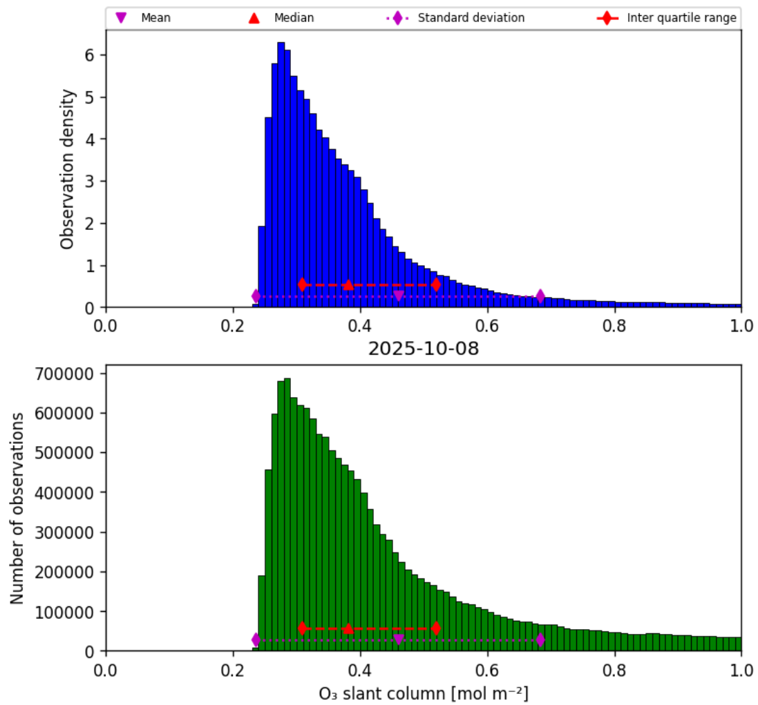
Figure 31: Histogram of “O 3 slant column” for 2025-10-08 to 2025-10-09
