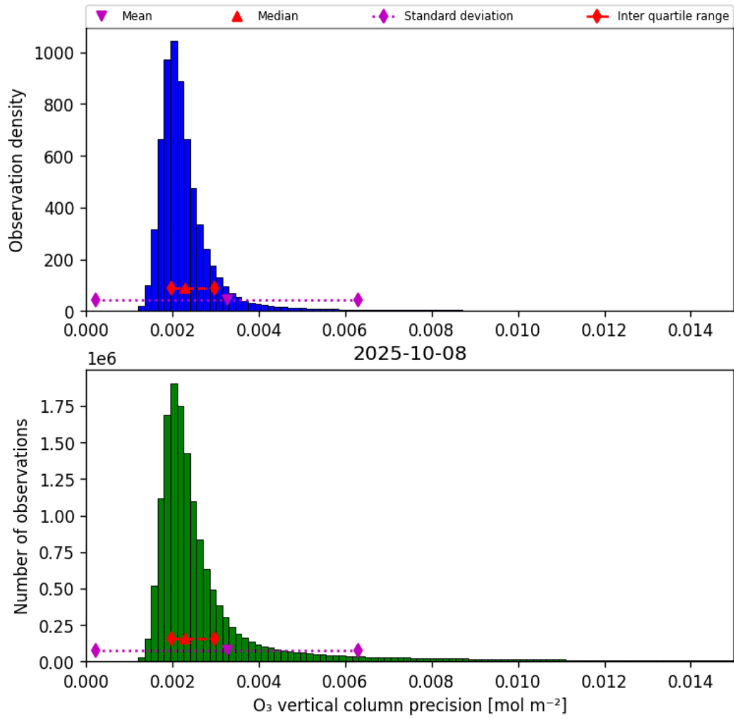
Figure 30: Histogram of “O 3 vertical column precision” for 2025-10-08 to 2025-10-09
