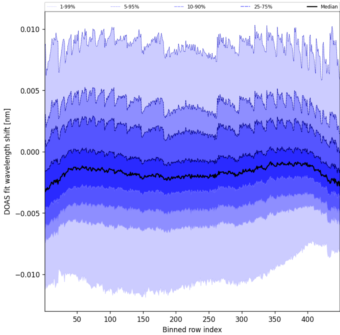
Figure 47: Along track statistics of “DOAS fit wavelength shift” for 2025-10-08 to 2025-10-09
