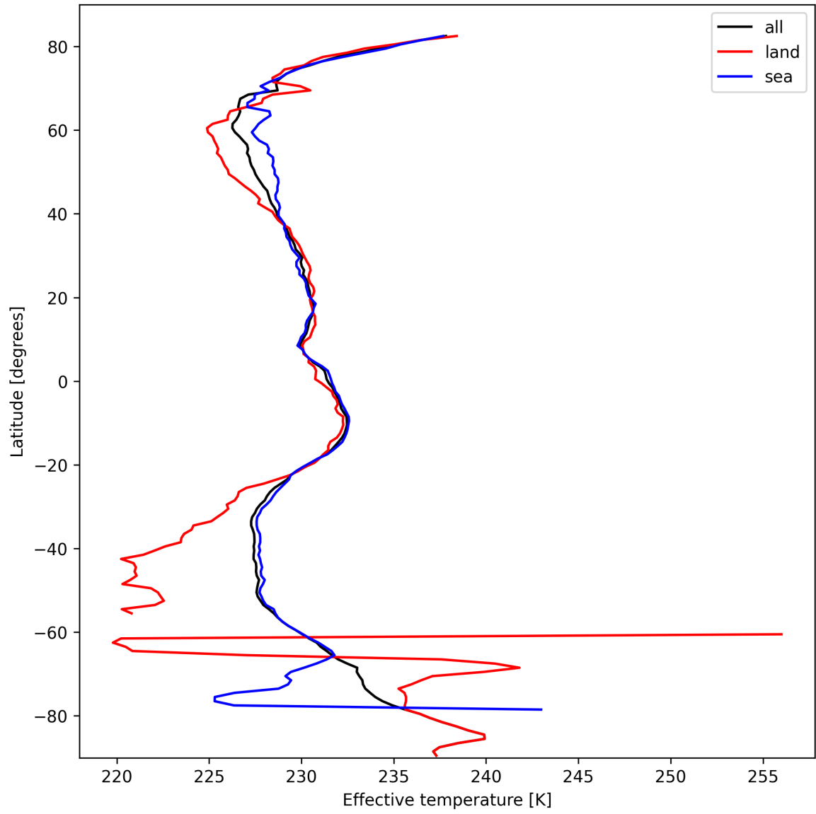
Figure 26: Zonal average of “Effective temperature” for 2025-10-08 to 2025-10-09.
