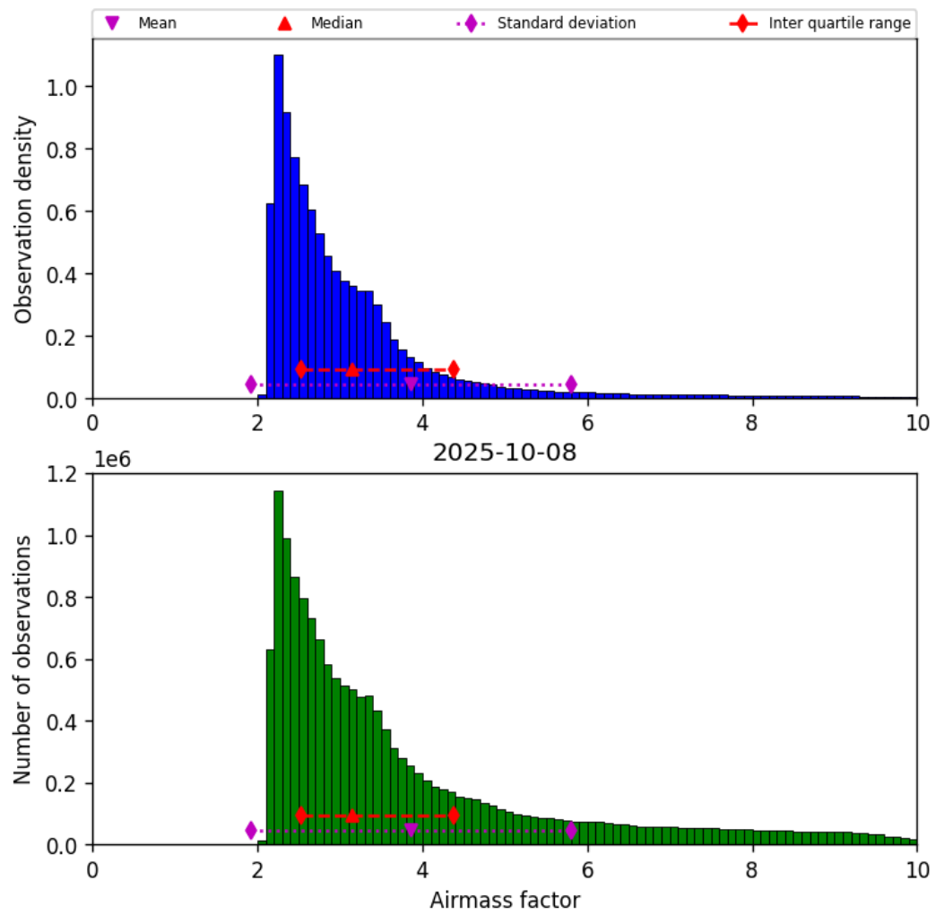
Figure 37: Histogram of “Airmass factor” for 2025-10-08 to 2025-10-09
