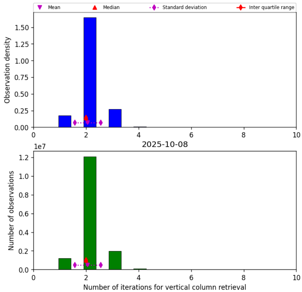
Figure 39: Histogram of “Number of iterations for vertical column retrieval” for 2025-10-08 to 2025-10-09
