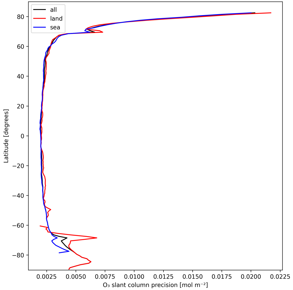
Figure 20: Zonal average of “O 3 slant column precision” for 2025-10-08 to 2025-10-09.
