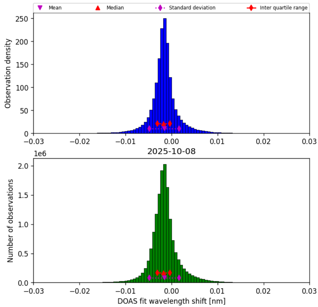
Figure 35: Histogram of “DOAS fit wavelength shift” for 2025-10-08 to 2025-10-09
