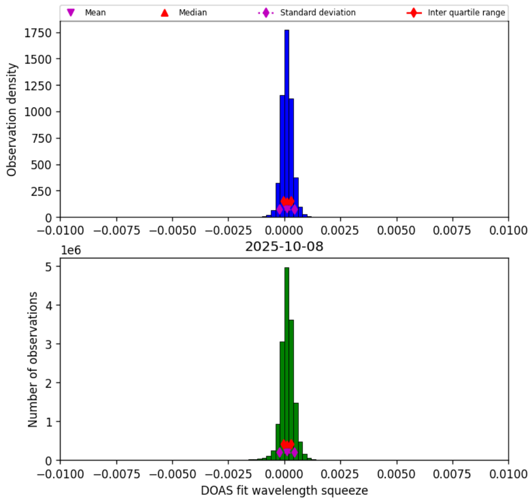
Figure 36: Histogram of “DOAS fit wavelength squeeze” for 2025-10-08 to 2025-10-09
