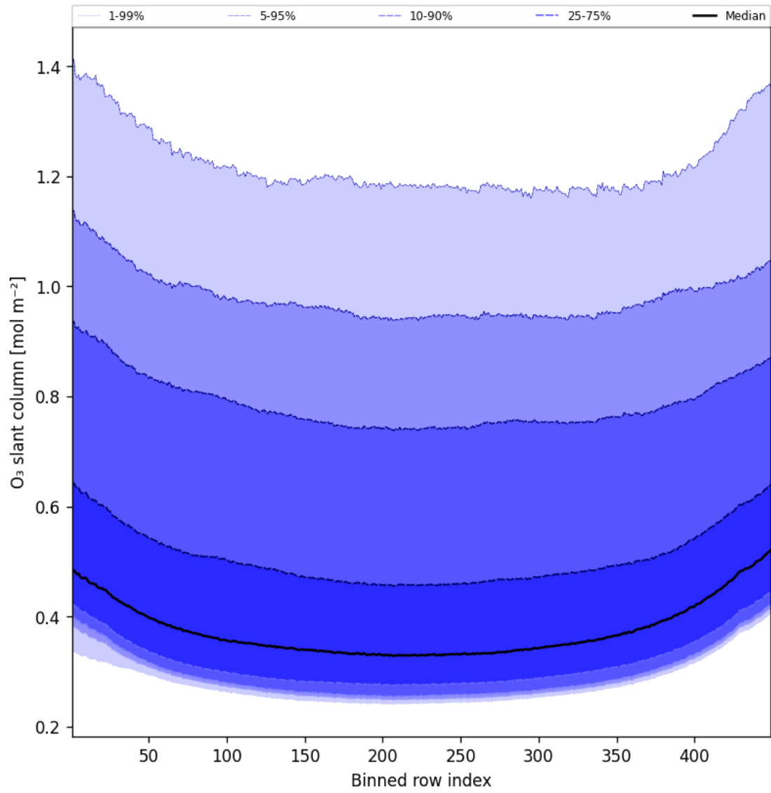
Figure 43: Along track statistics of “O 3 slant column” for 2025-10-08 to 2025-10-09
