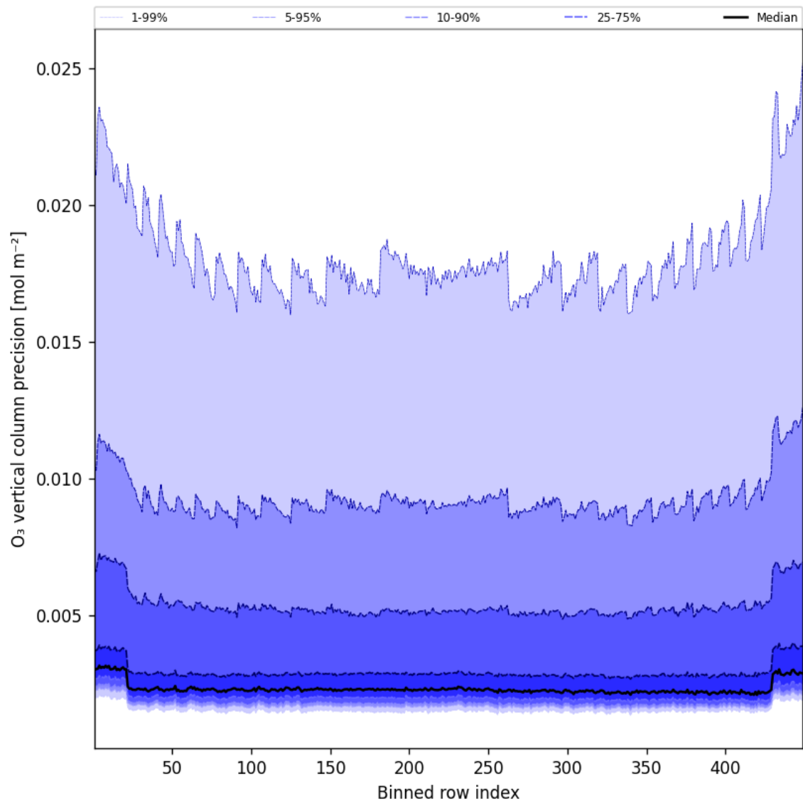
Figure 42: Along track statistics of “O 3 vertical column precision” for 2025-10-08 to 2025-10-09
