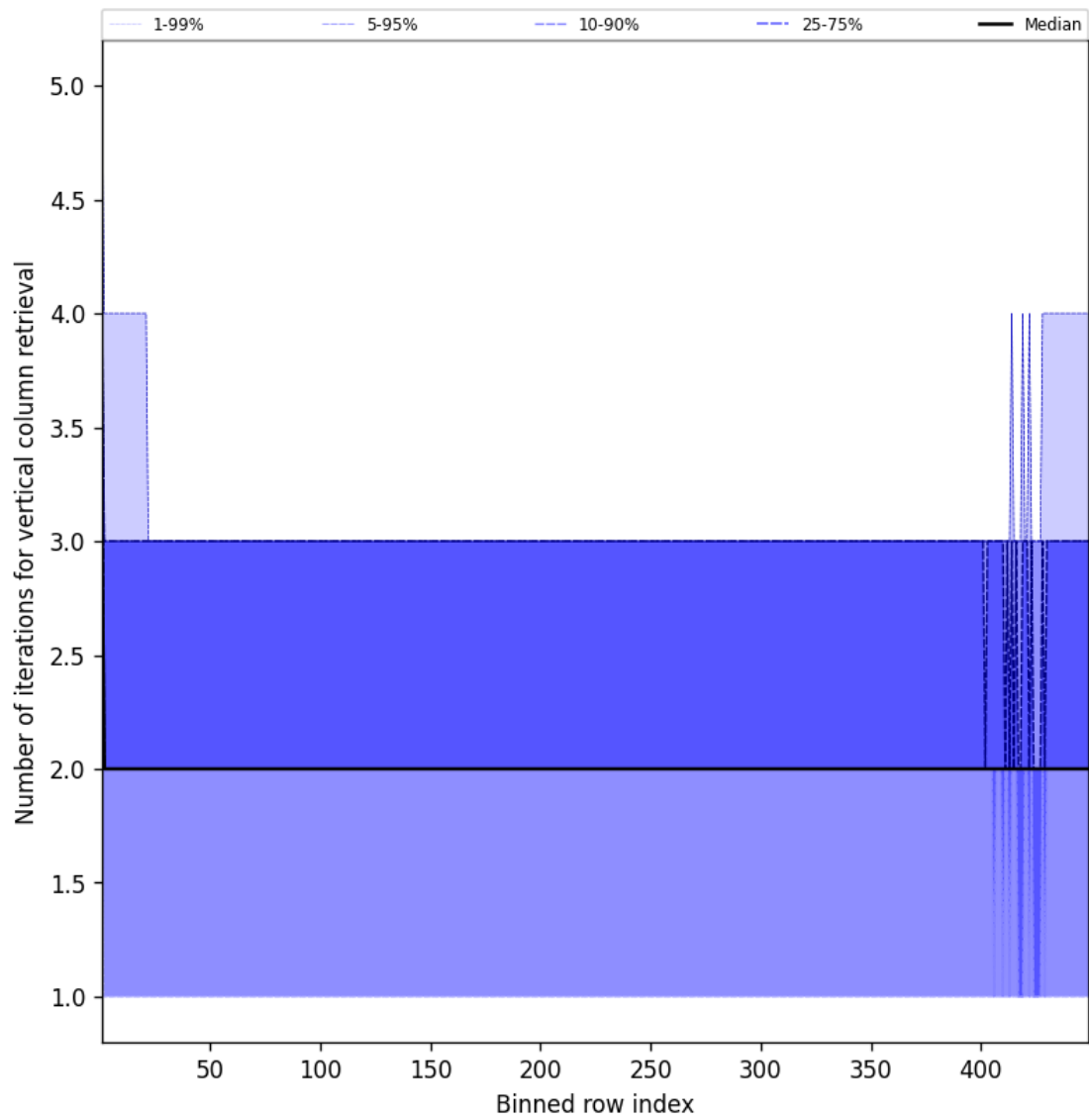
Figure 51: Along track statistics of “Number of iterations for vertical column retrieval” for 2025-10-08 to 2025-10-09
