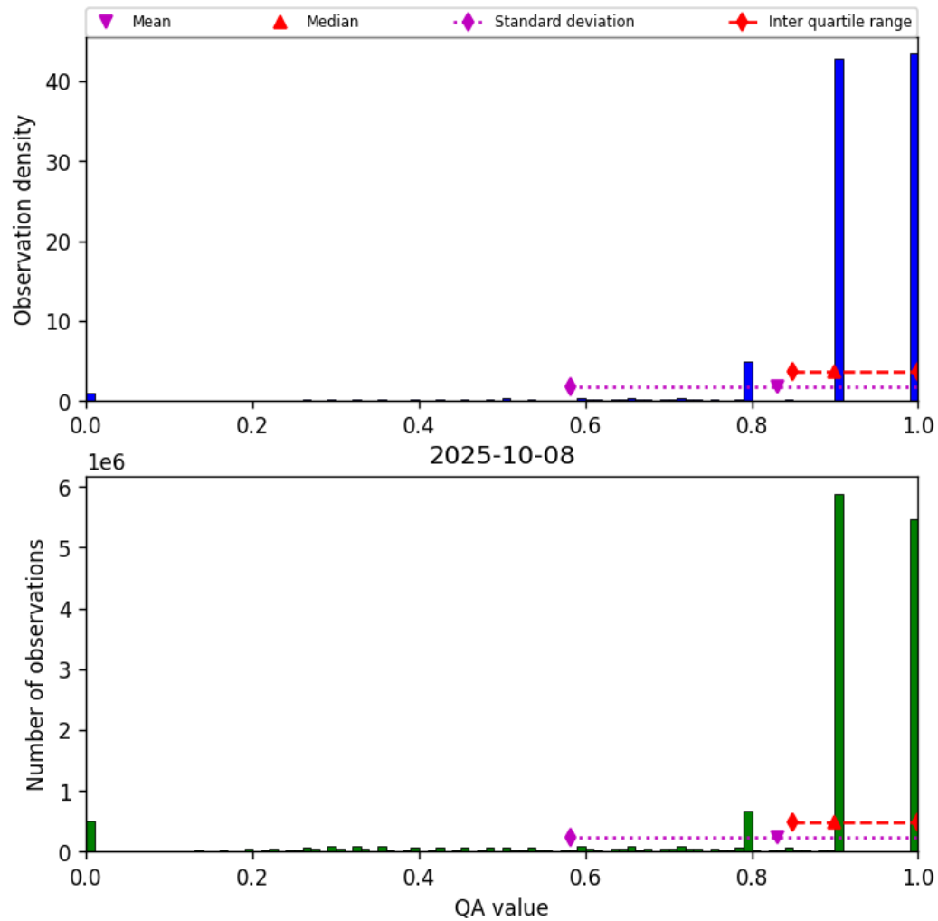
Figure 28: Histogram of “QA value” for 2025-10-08 to 2025-10-09
