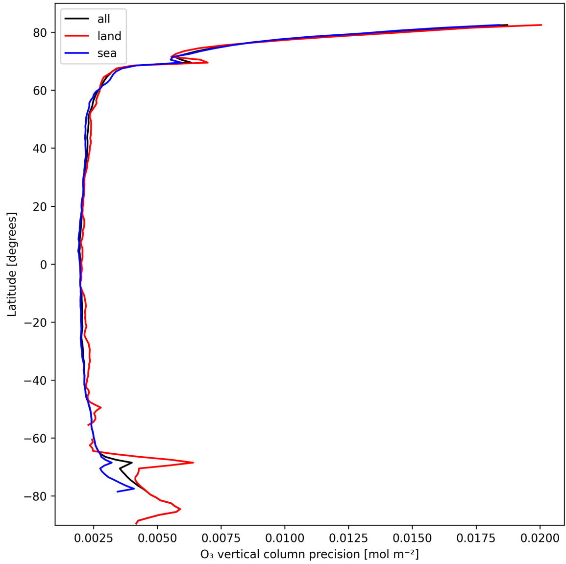
Figure 18: Zonal average of “O 3 vertical column precision” for 2025-10-08 to 2025-10-09.
