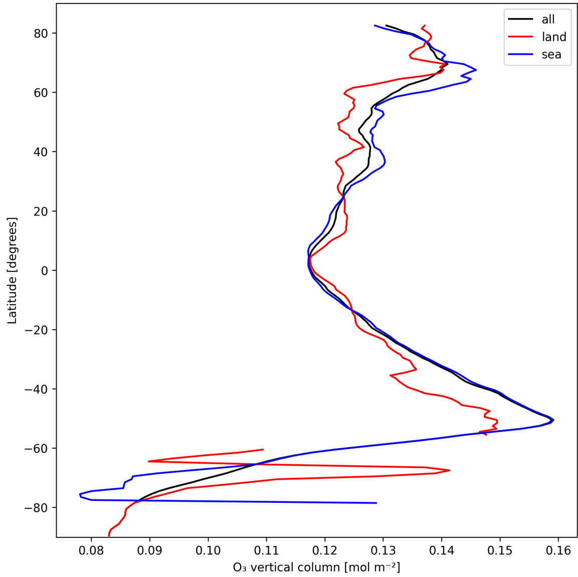
Figure 17: Zonal average of “O 3 vertical column” for 2025-10-08 to 2025-10-09.
