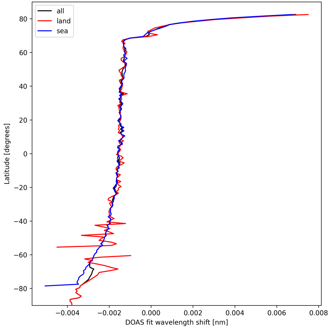
Figure 23: Zonal average of “DOAS fit wavelength shift” for 2025-10-08 to 2025-10-09.
