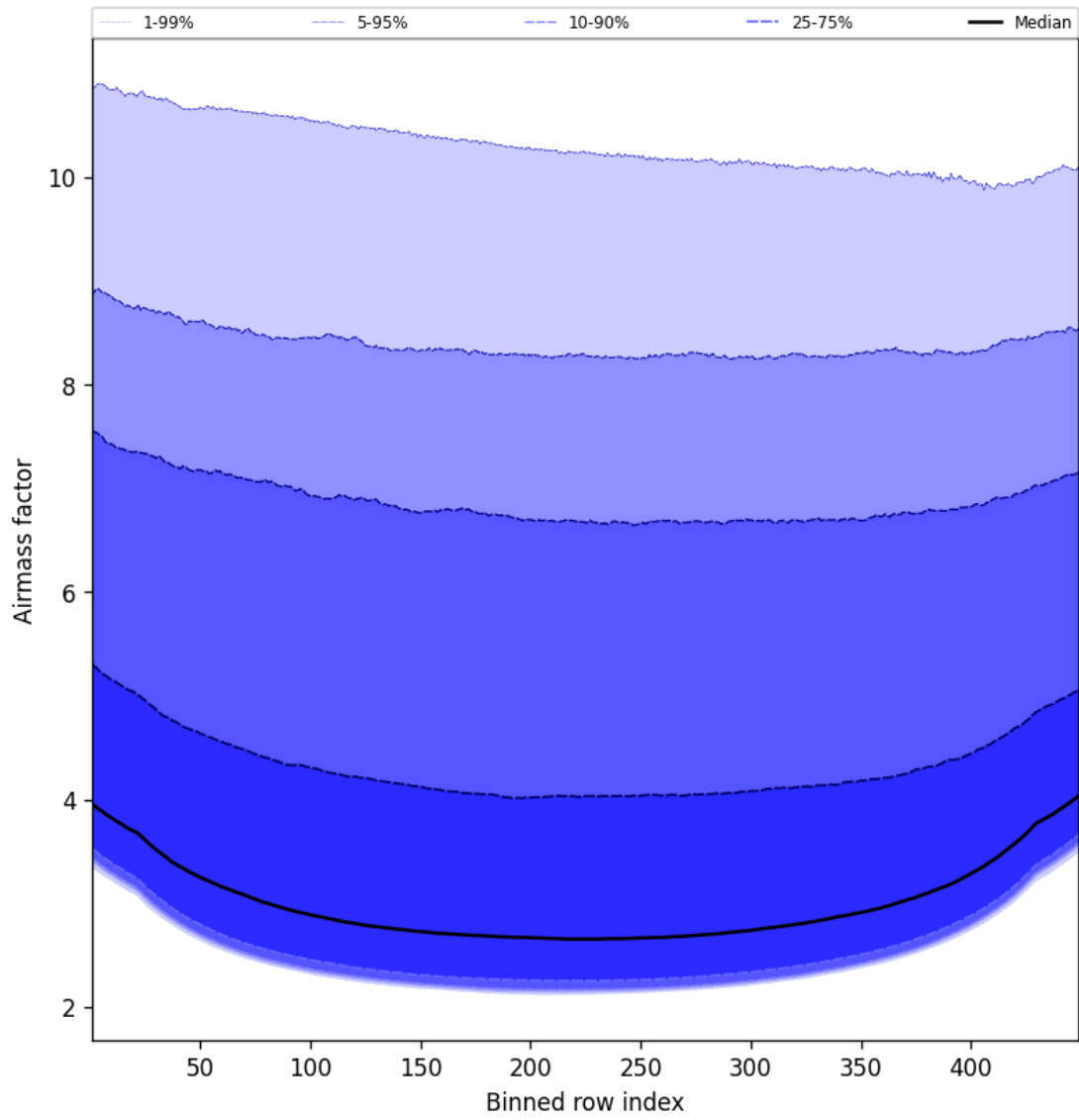
Figure 49: Along track statistics of “Airmass factor” for 2025-10-08 to 2025-10-09
