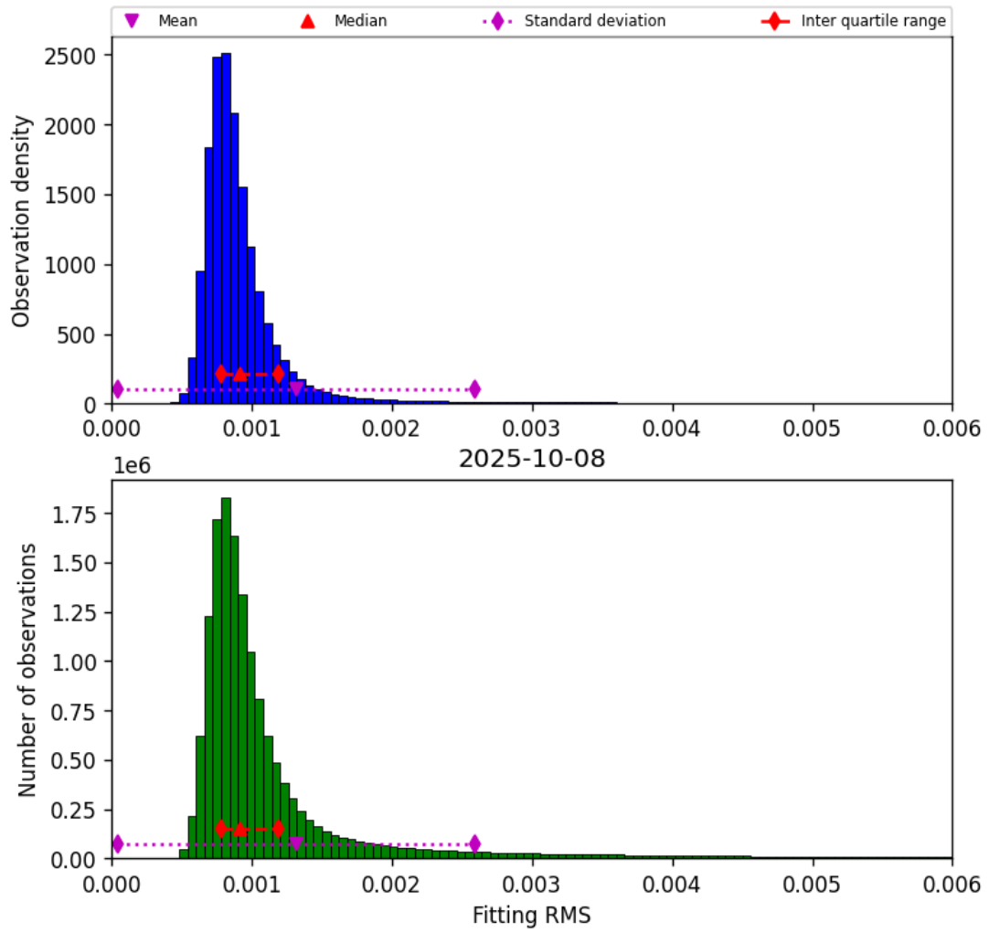
Figure 34: Histogram of “Fitting RMS” for 2025-10-08 to 2025-10-09
