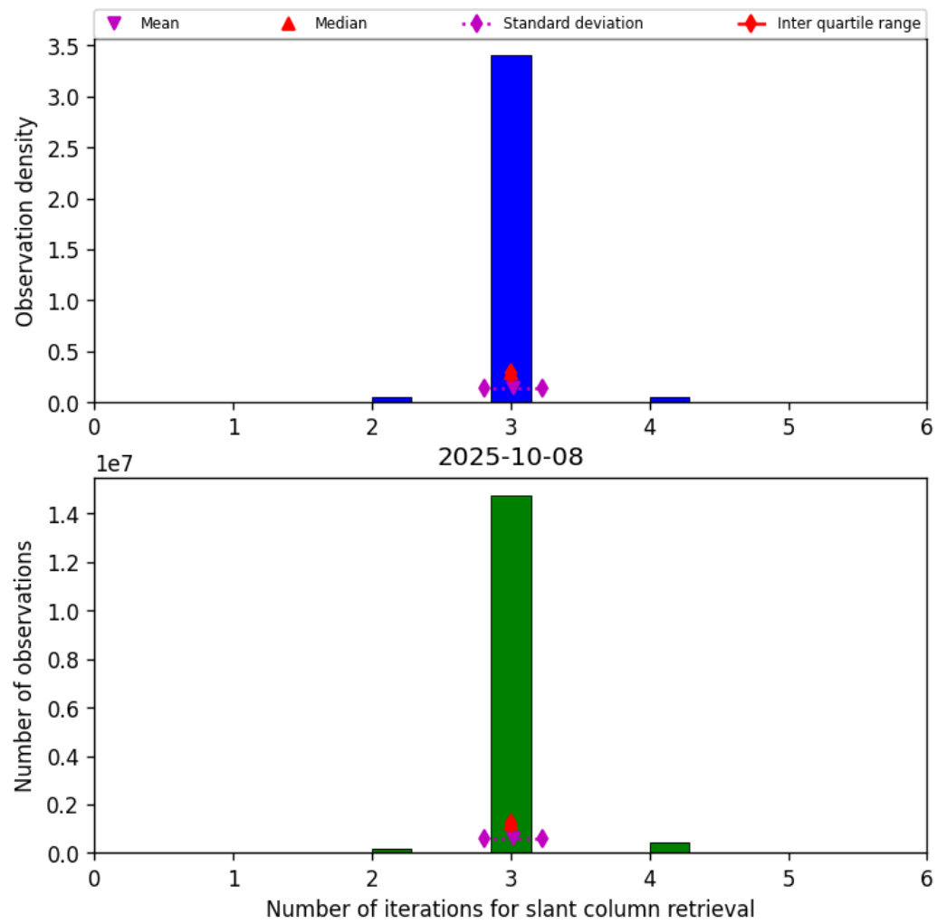
Figure 33: Histogram of “Number of iterations for slant column retrieval” for 2025-10-08 to 2025-10-09
