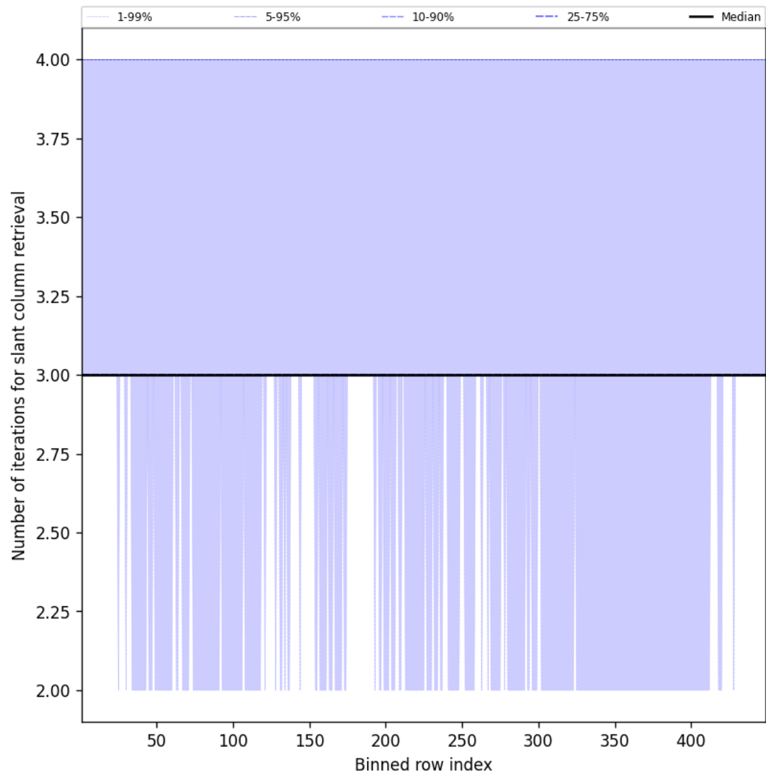
Figure 45: Along track statistics of “Number of iterations for slant column retrieval” for 2025-10-08 to 2025-10-09
