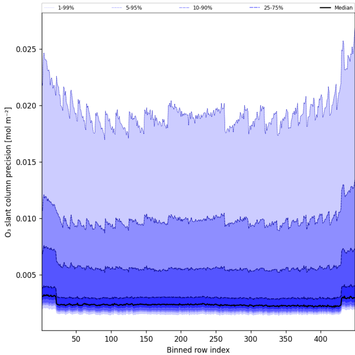
Figure 44: Along track statistics of “O 3 slant column precision” for 2025-10-08 to 2025-10-09
