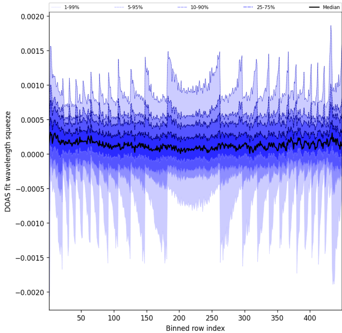
Figure 48: Along track statistics of “DOAS fit wavelength squeeze” for 2025-10-08 to 2025-10-09
