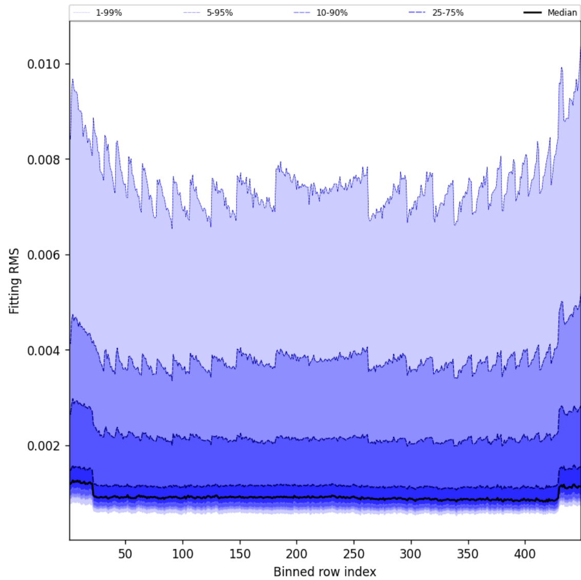
Figure 46: Along track statistics of “Fitting RMS” for 2025-10-08 to 2025-10-09
