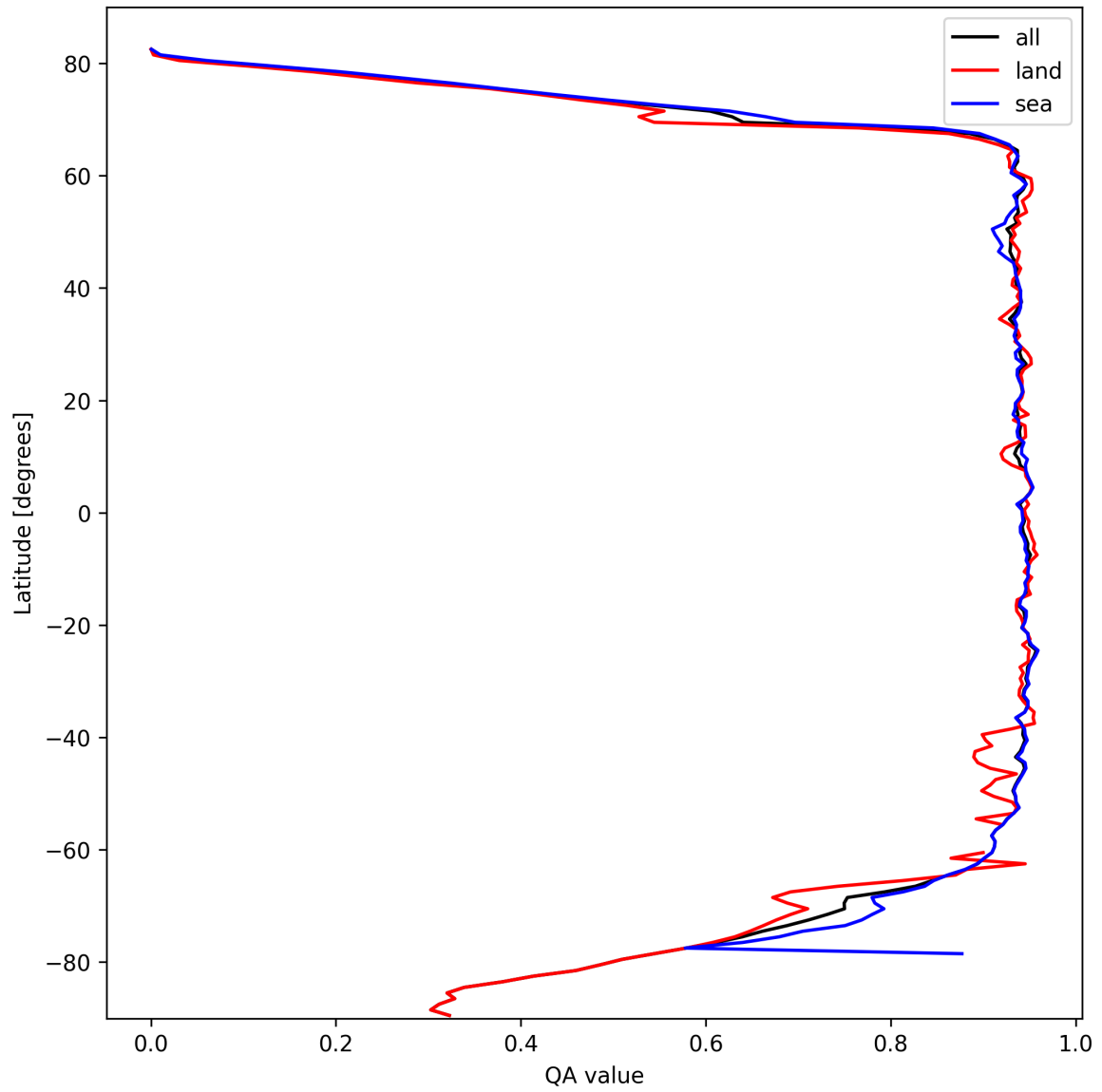
Figure 16: Zonal average of “QA value” for 2025-10-08 to 2025-10-09.
