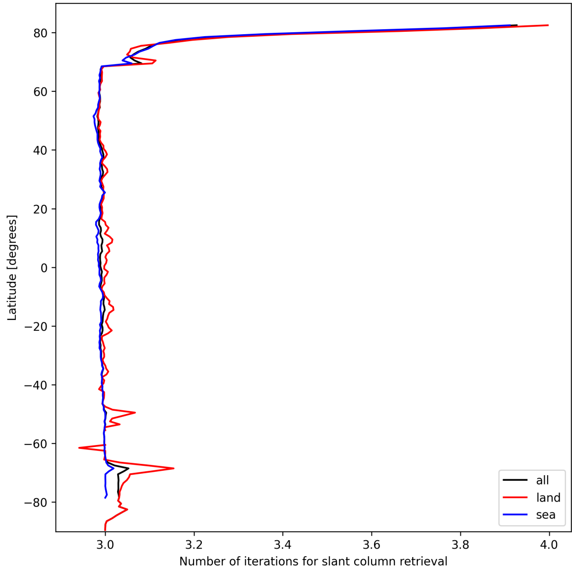
Figure 21: Zonal average of “Number of iterations for slant column retrieval” for 2025-10-08 to 2025-10-09.
