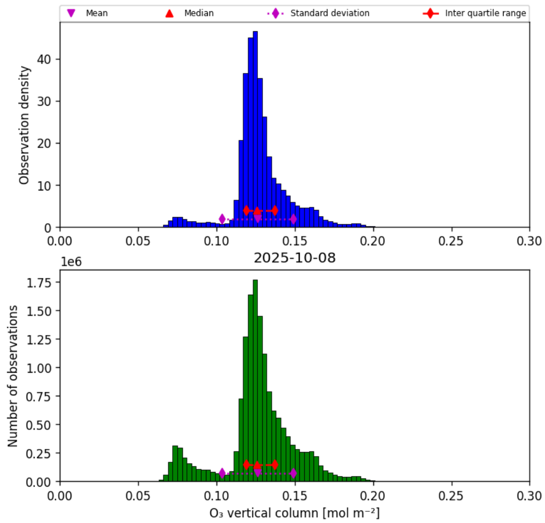
Figure 29: Histogram of “O 3 vertical column” for 2025-10-08 to 2025-10-09
