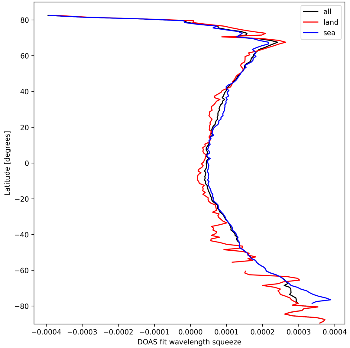
Figure 24: Zonal average of “DOAS fit wavelength squeeze” for 2025-10-08 to 2025-10-09.
