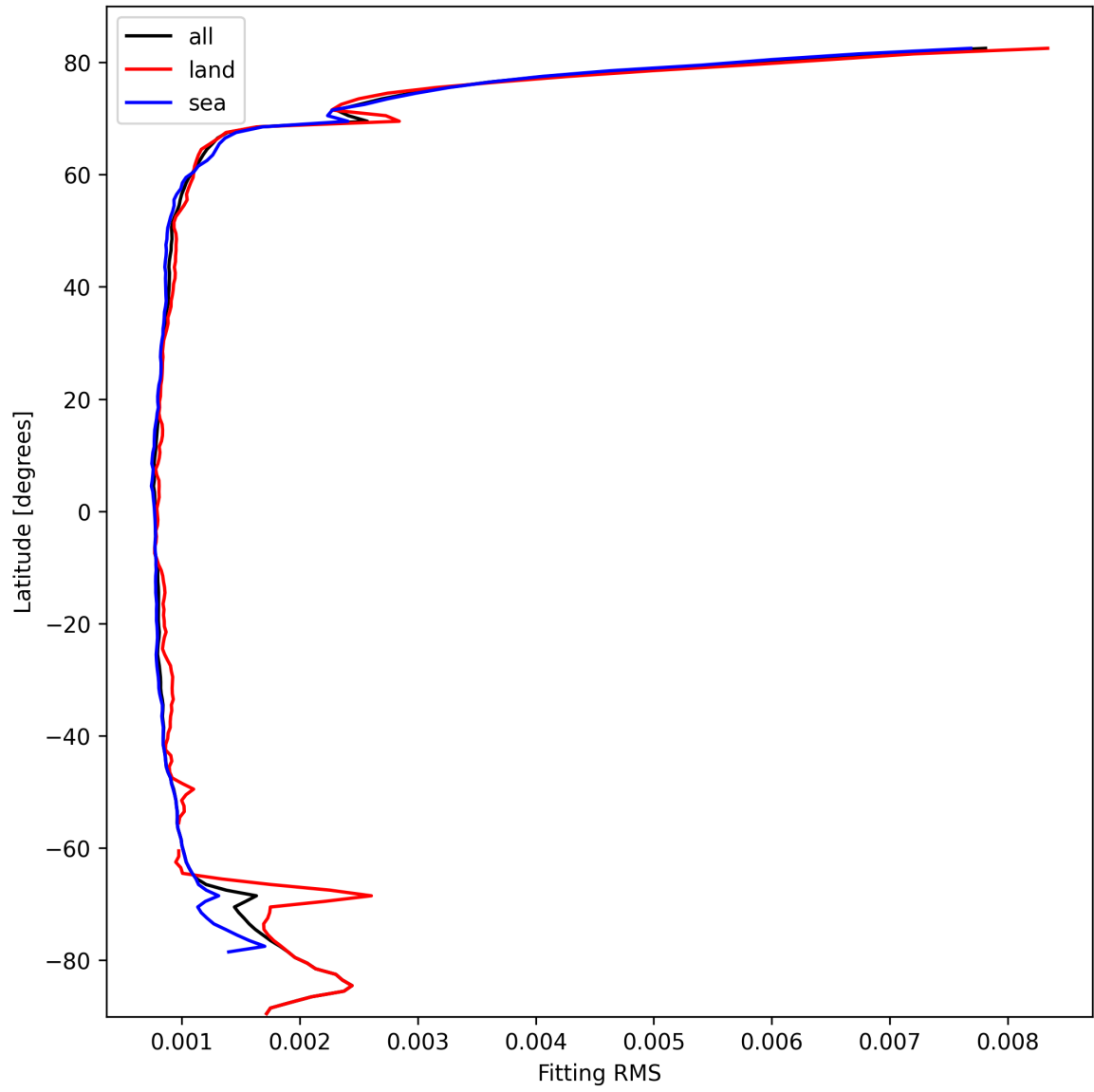
Figure 22: Zonal average of “Fitting RMS” for 2025-10-08 to 2025-10-09.
