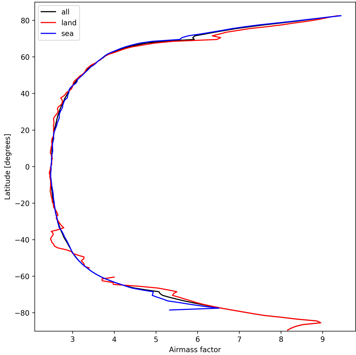
Figure 25: Zonal average of “Airmass factor” for 2025-10-08 to 2025-10-09.
