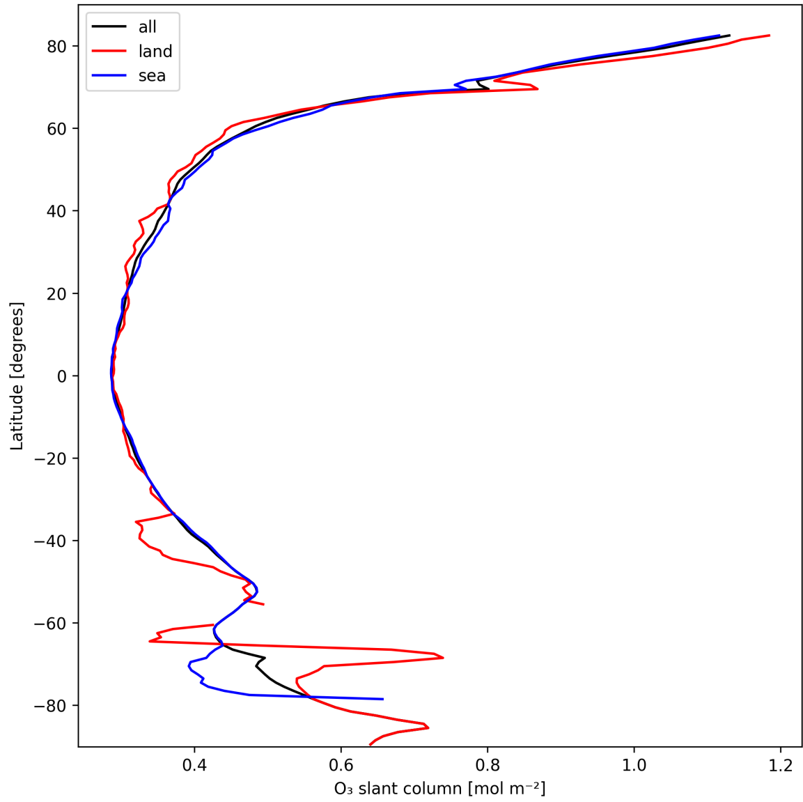
Figure 19: Zonal average of “O 3 slant column” for 2025-10-08 to 2025-10-09.
