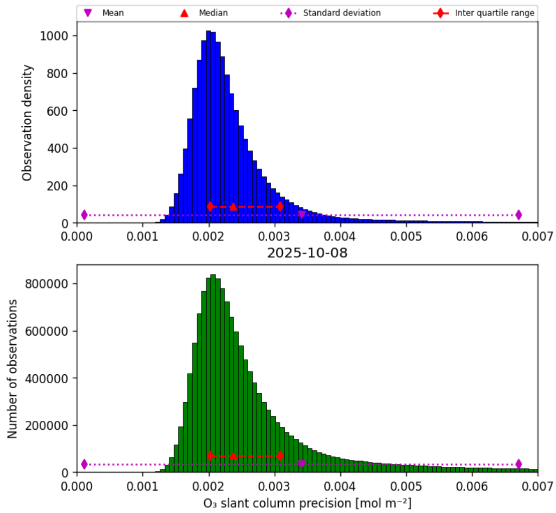
Figure 32: Histogram of “O 3 slant column precision” for 2025-10-08 to 2025-10-09
