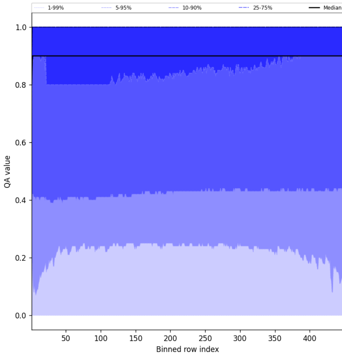
Figure 40: Along track statistics of “QA value” for 2025-10-08 to 2025-10-09
