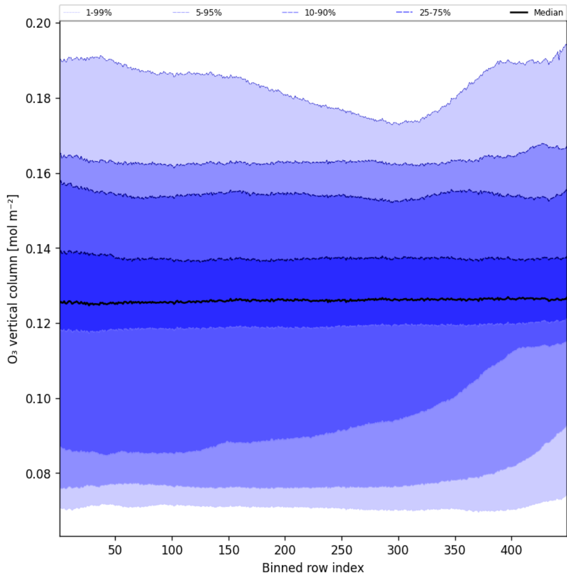
Figure 41: Along track statistics of “O 3 vertical column” for 2025-10-08 to 2025-10-09
