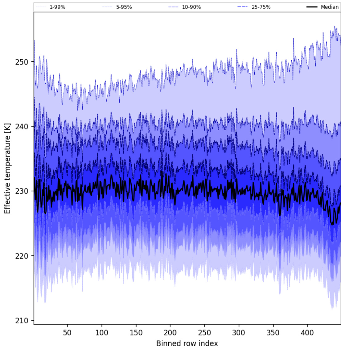
Figure 50: Along track statistics of “Effective temperature” for 2025-10-08 to 2025-10-09
