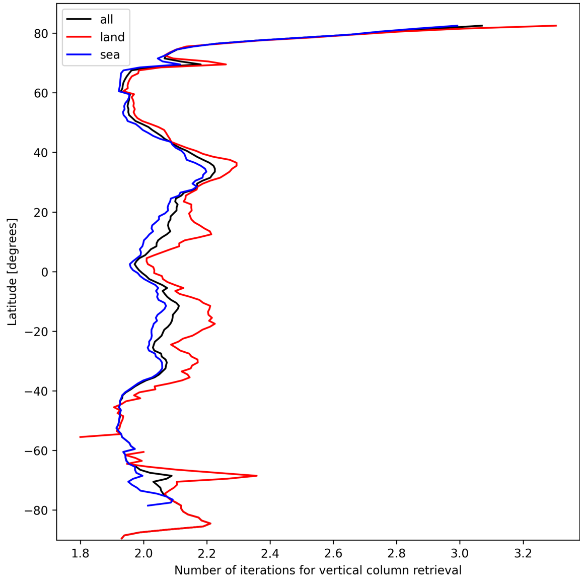
Figure 27: Zonal average of “Number of iterations for vertical column retrieval” for 2025-10-08 to 2025-10-09.
