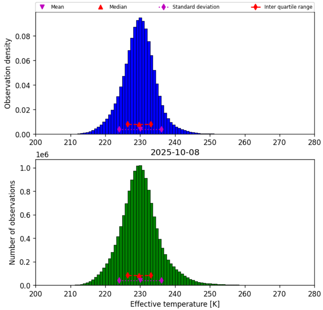
Figure 38: Histogram of “Effective temperature” for 2025-10-08 to 2025-10-09
