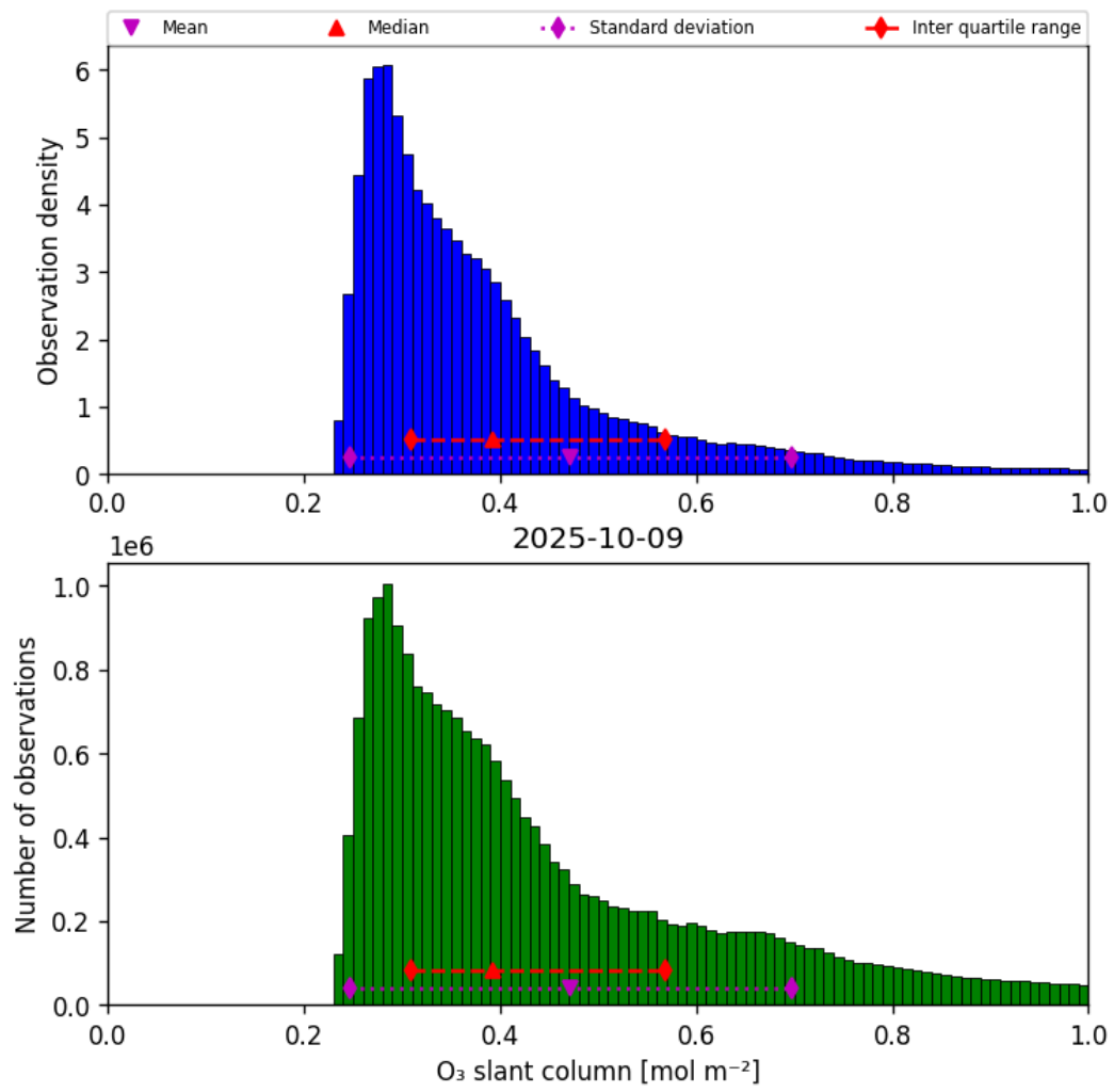
Figure 31: Histogram of “O 3 slant column” for 2025-10-09 to 2025-10-09
