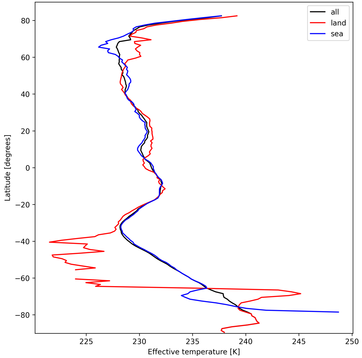
Figure 26: Zonal average of “Effective temperature” for 2025-10-09 to 2025-10-09.
