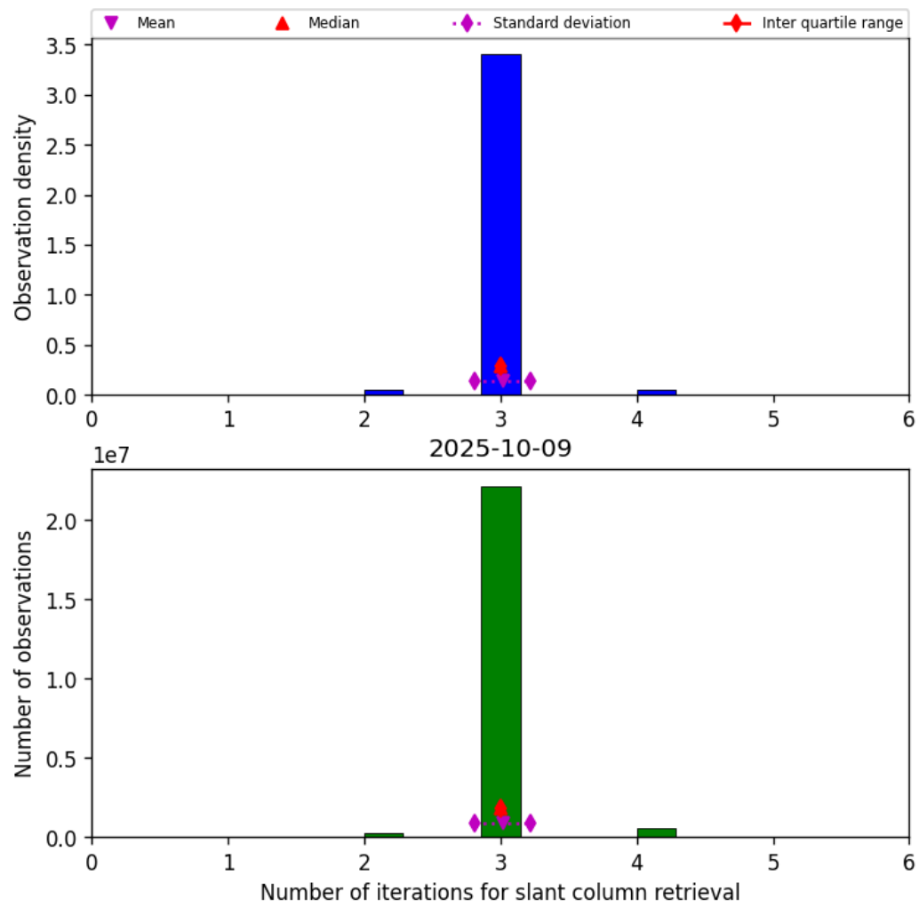
Figure 33: Histogram of “Number of iterations for slant column retrieval” for 2025-10-09 to 2025-10-09
