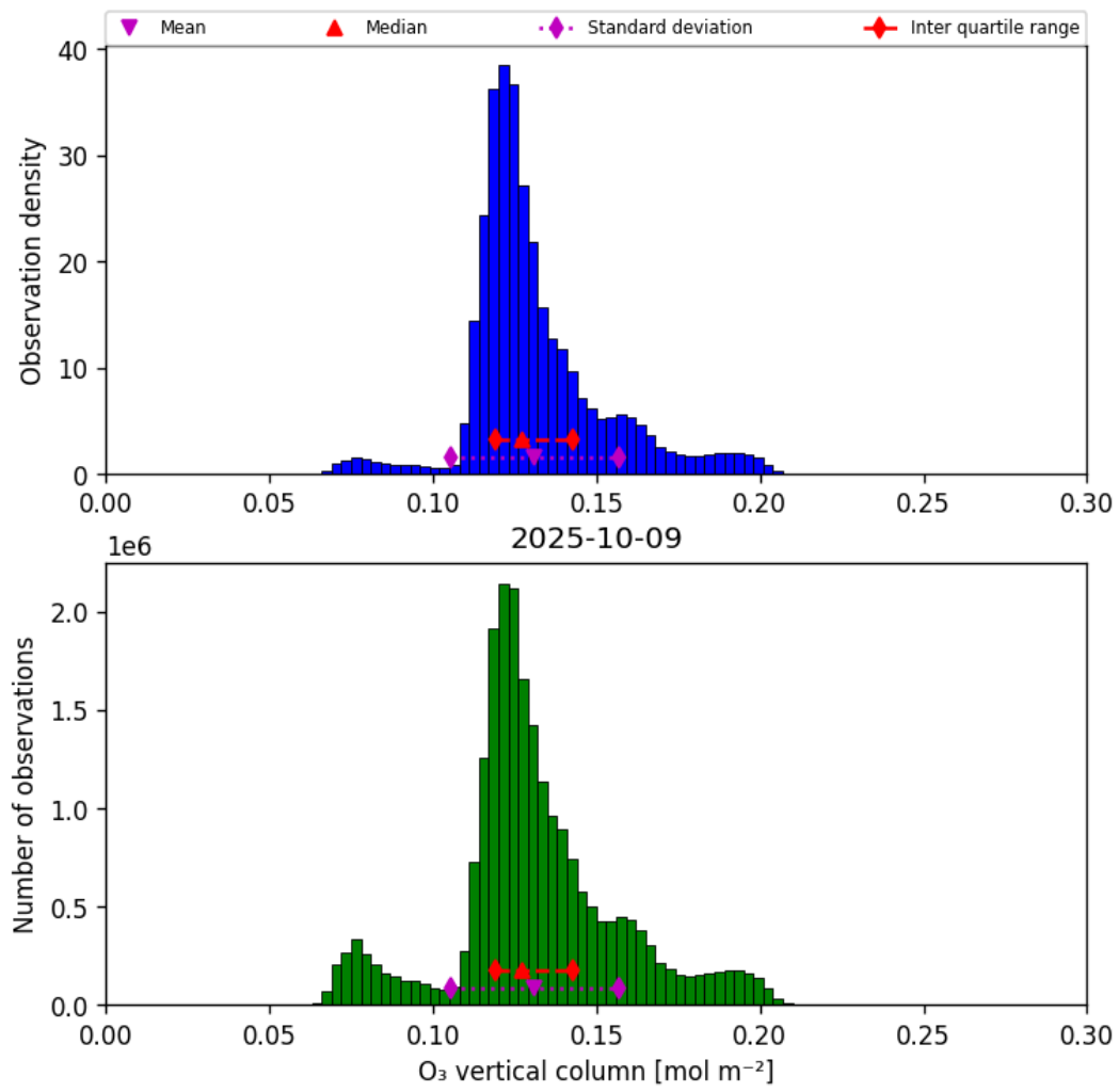
Figure 29: Histogram of “O 3 vertical column” for 2025-10-09 to 2025-10-09
