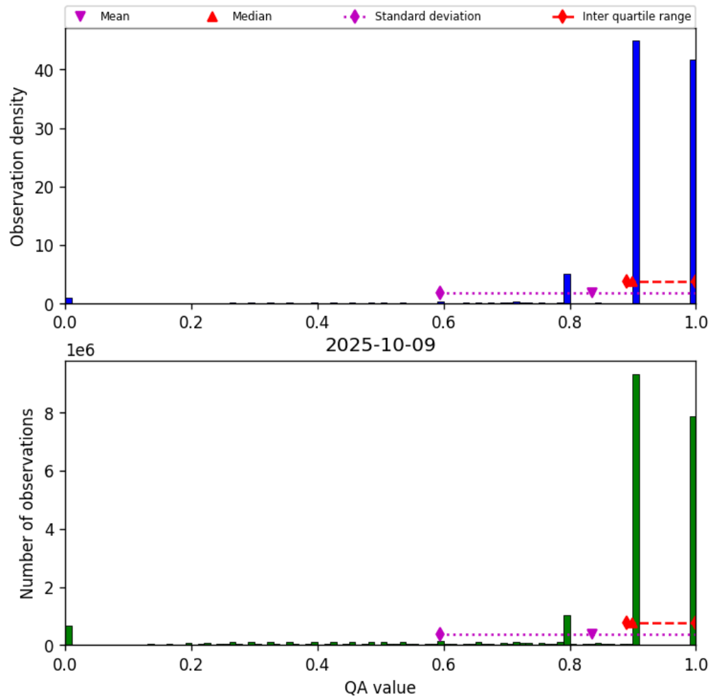
Figure 28: Histogram of “QA value” for 2025-10-09 to 2025-10-09
