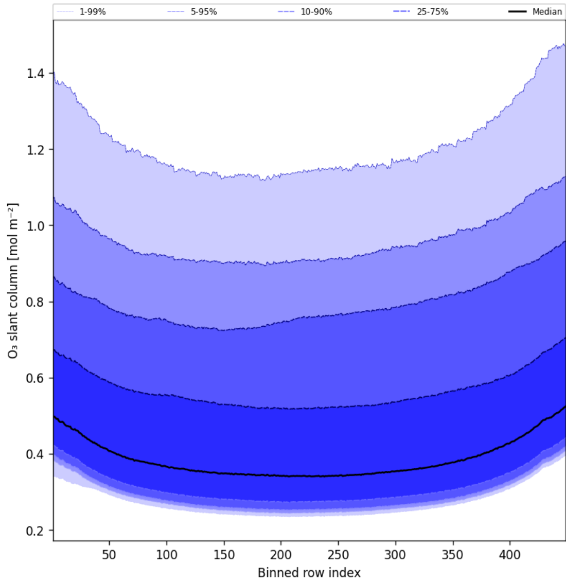
Figure 43: Along track statistics of “O 3 slant column” for 2025-10-09 to 2025-10-09
