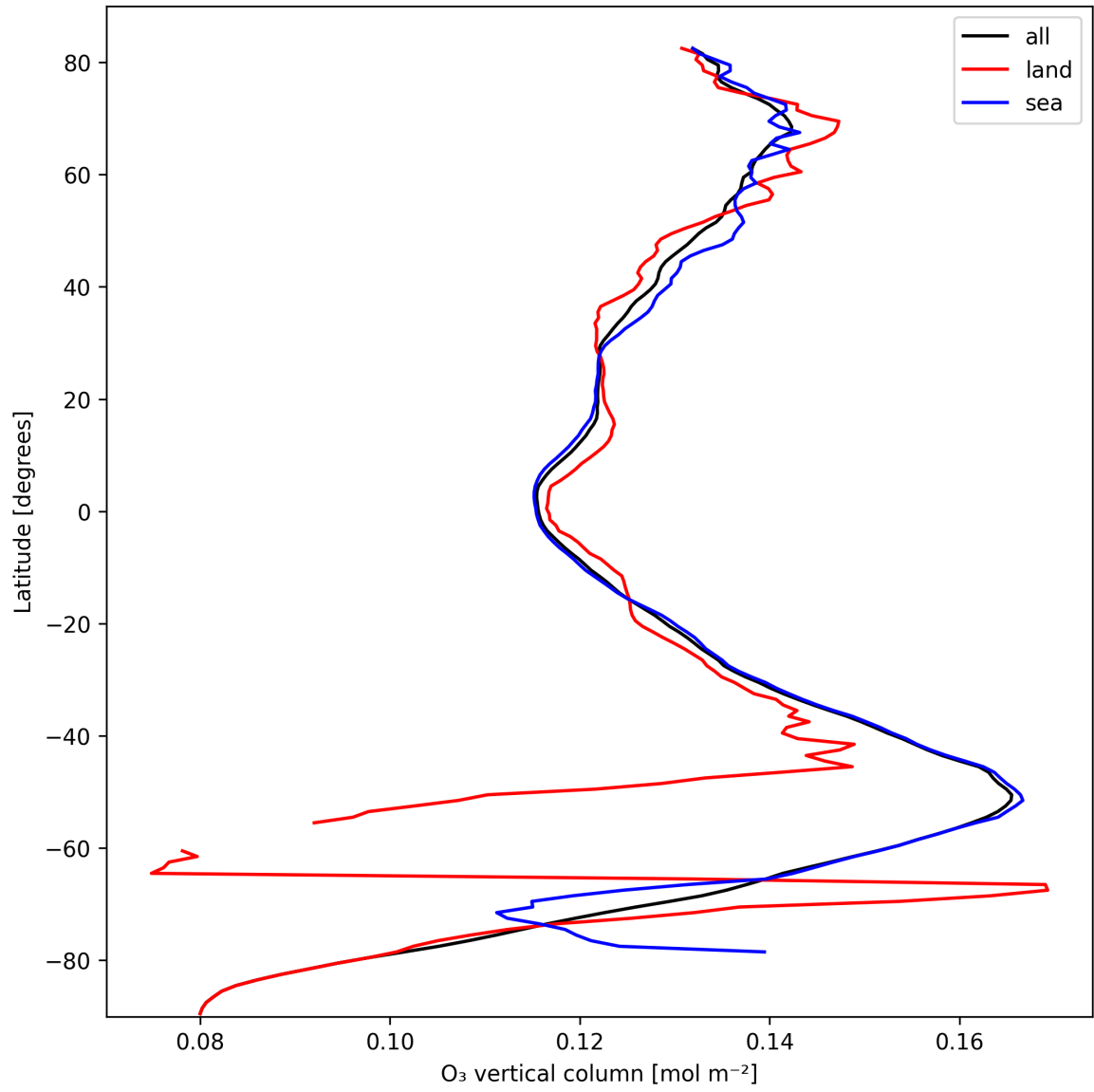
Figure 17: Zonal average of “O 3 vertical column” for 2025-10-09 to 2025-10-09.
