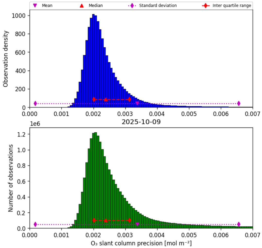
Figure 32: Histogram of “O 3 slant column precision” for 2025-10-09 to 2025-10-09
