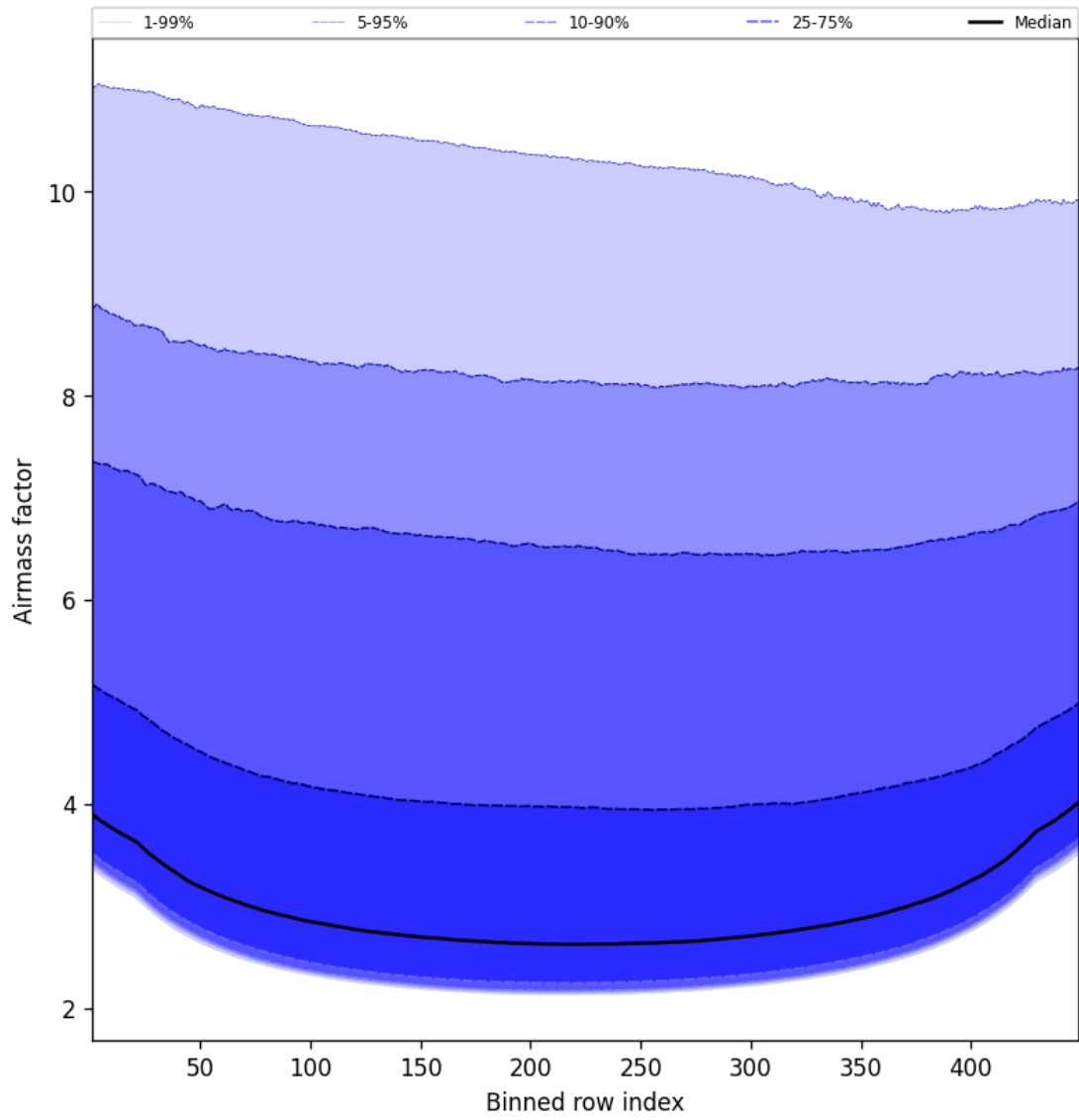
Figure 49: Along track statistics of “Airmass factor” for 2025-10-09 to 2025-10-09
