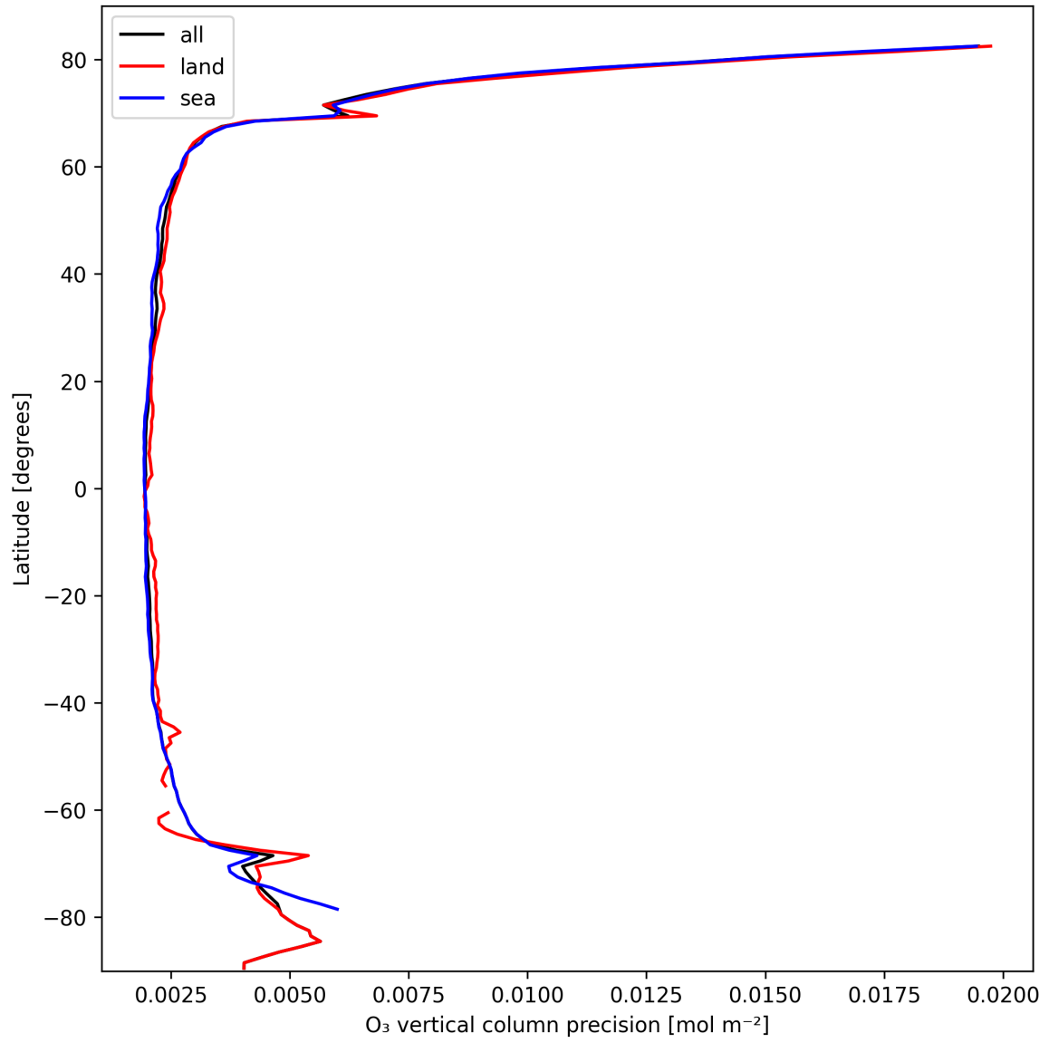
Figure 18: Zonal average of “O 3 vertical column precision” for 2025-10-09 to 2025-10-09.
