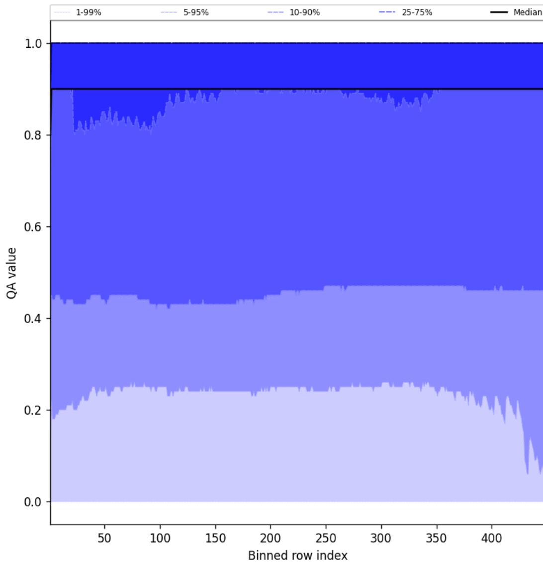
Figure 40: Along track statistics of “QA value” for 2025-10-09 to 2025-10-09
