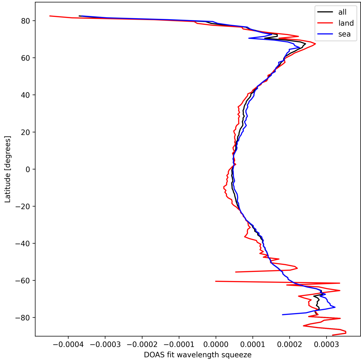
Figure 24: Zonal average of “DOAS fit wavelength squeeze” for 2025-10-09 to 2025-10-09.
