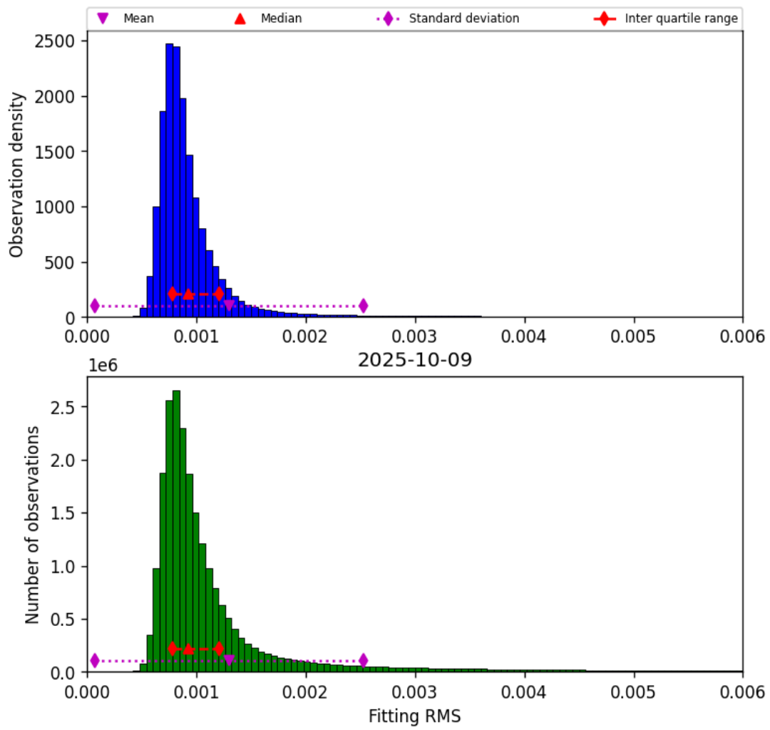
Figure 34: Histogram of “Fitting RMS” for 2025-10-09 to 2025-10-09
