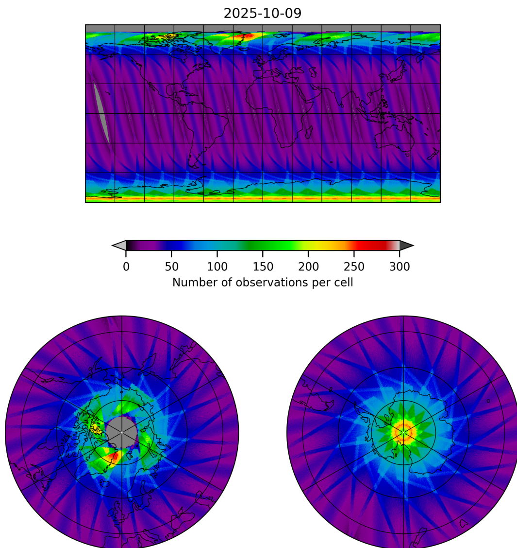
Figure 15: Map of the number of observations for 2025-10-09 to 2025-10-09
