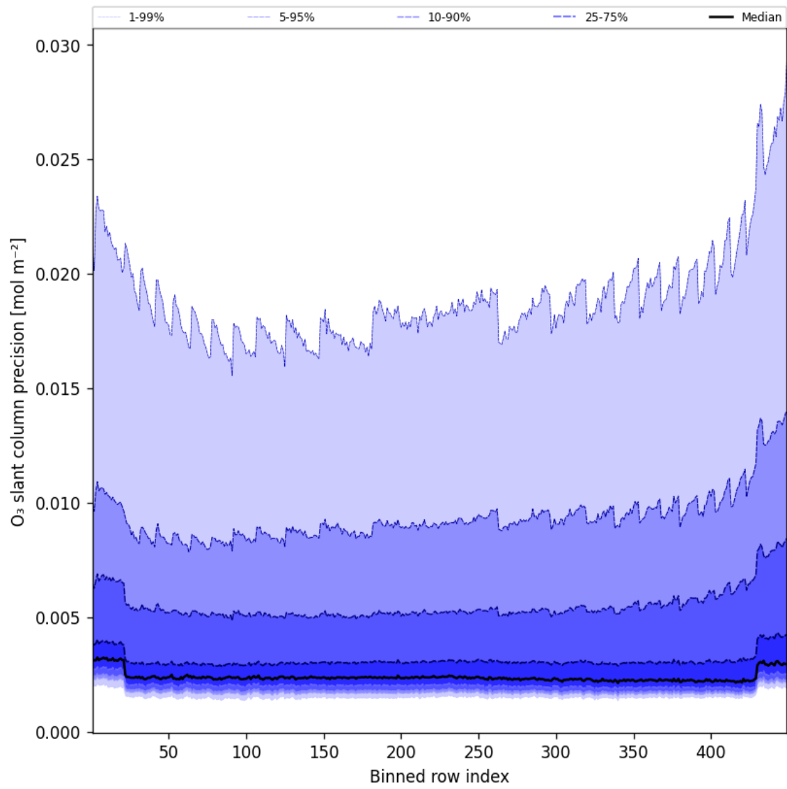
Figure 44: Along track statistics of “O 3 slant column precision” for 2025-10-09 to 2025-10-09
