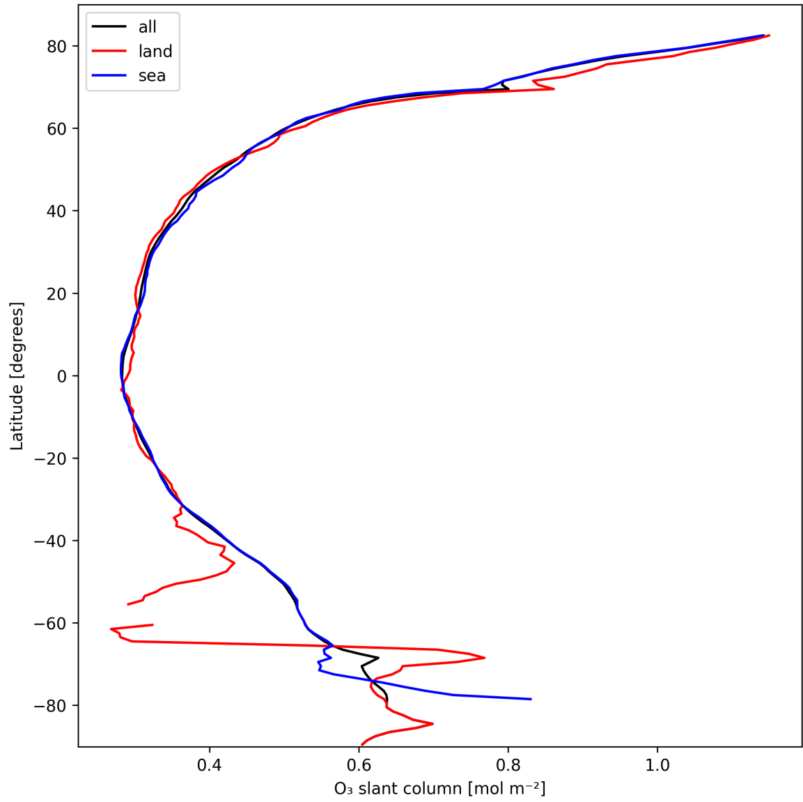
Figure 19: Zonal average of “O 3 slant column” for 2025-10-09 to 2025-10-09.
