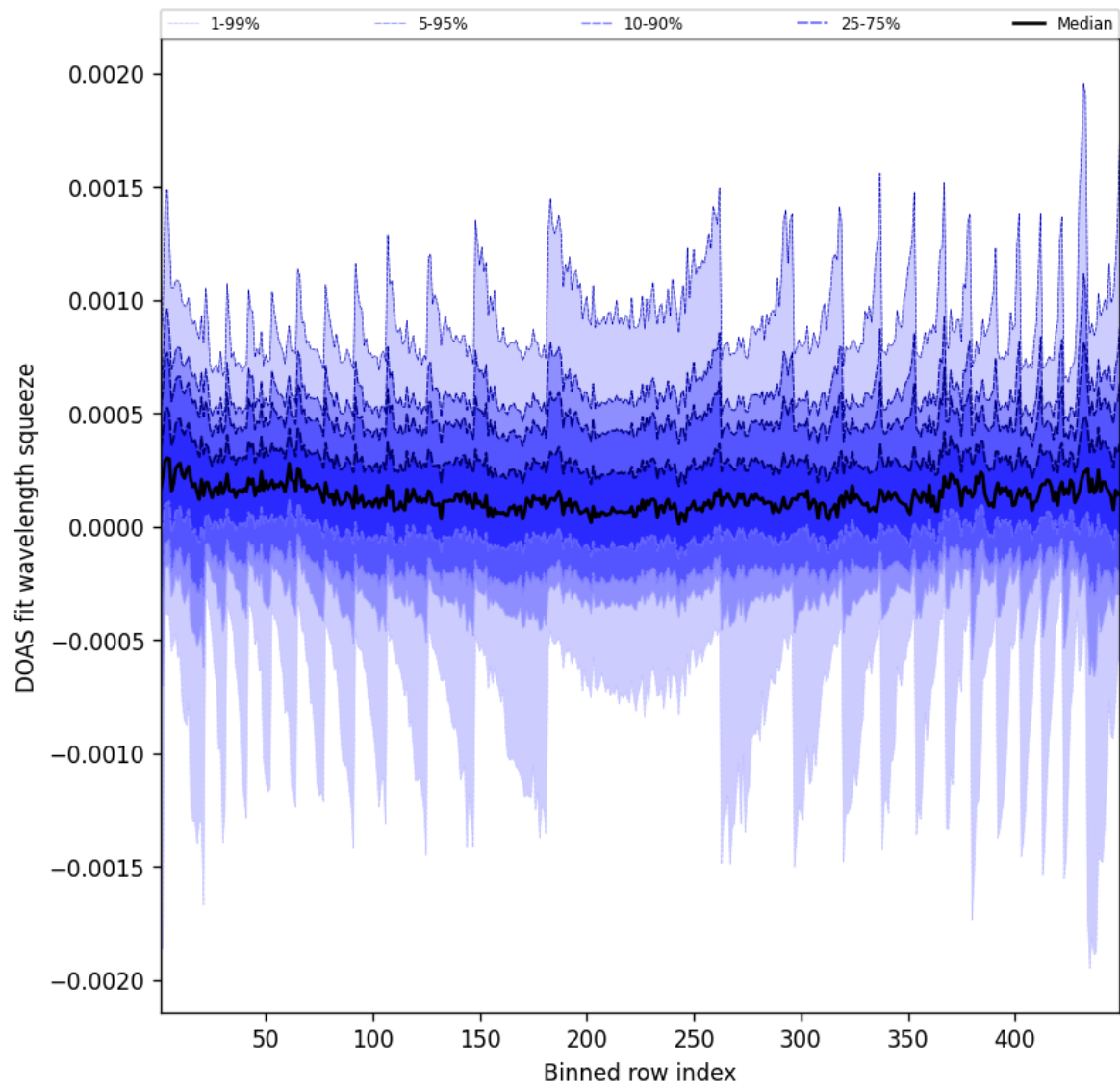
Figure 48: Along track statistics of “DOAS fit wavelength squeeze” for 2025-10-09 to 2025-10-09
