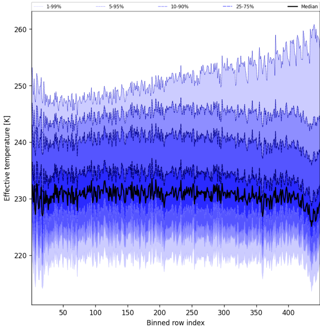
Figure 50: Along track statistics of “Effective temperature” for 2025-10-09 to 2025-10-09
