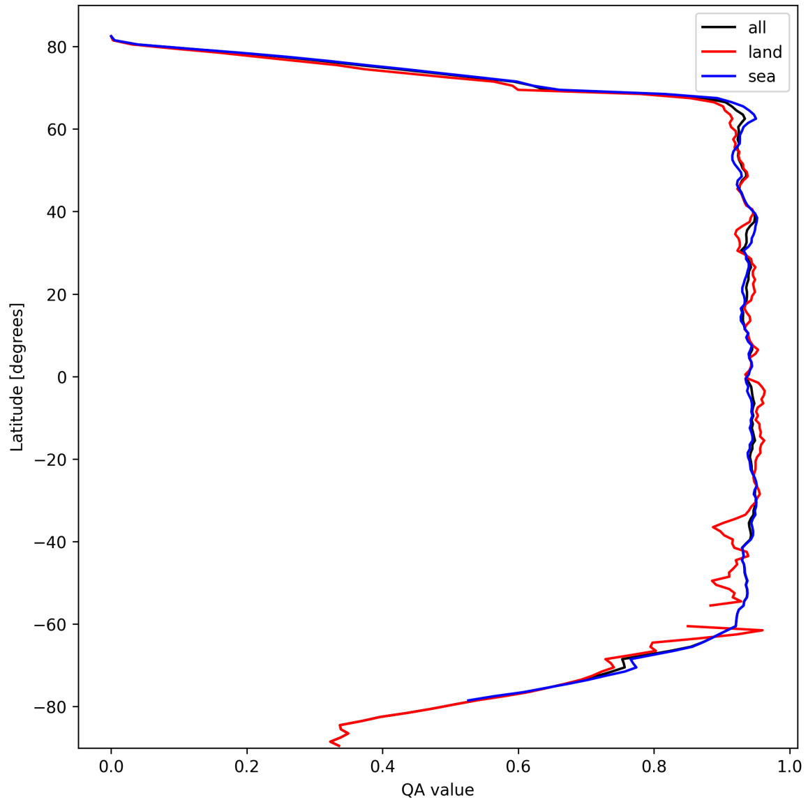
Figure 16: Zonal average of “QA value” for 2025-10-09 to 2025-10-09.
