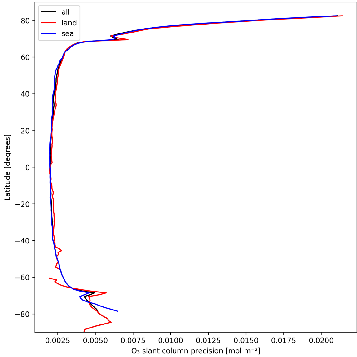
Figure 20: Zonal average of “O 3 slant column precision” for 2025-10-09 to 2025-10-09.
