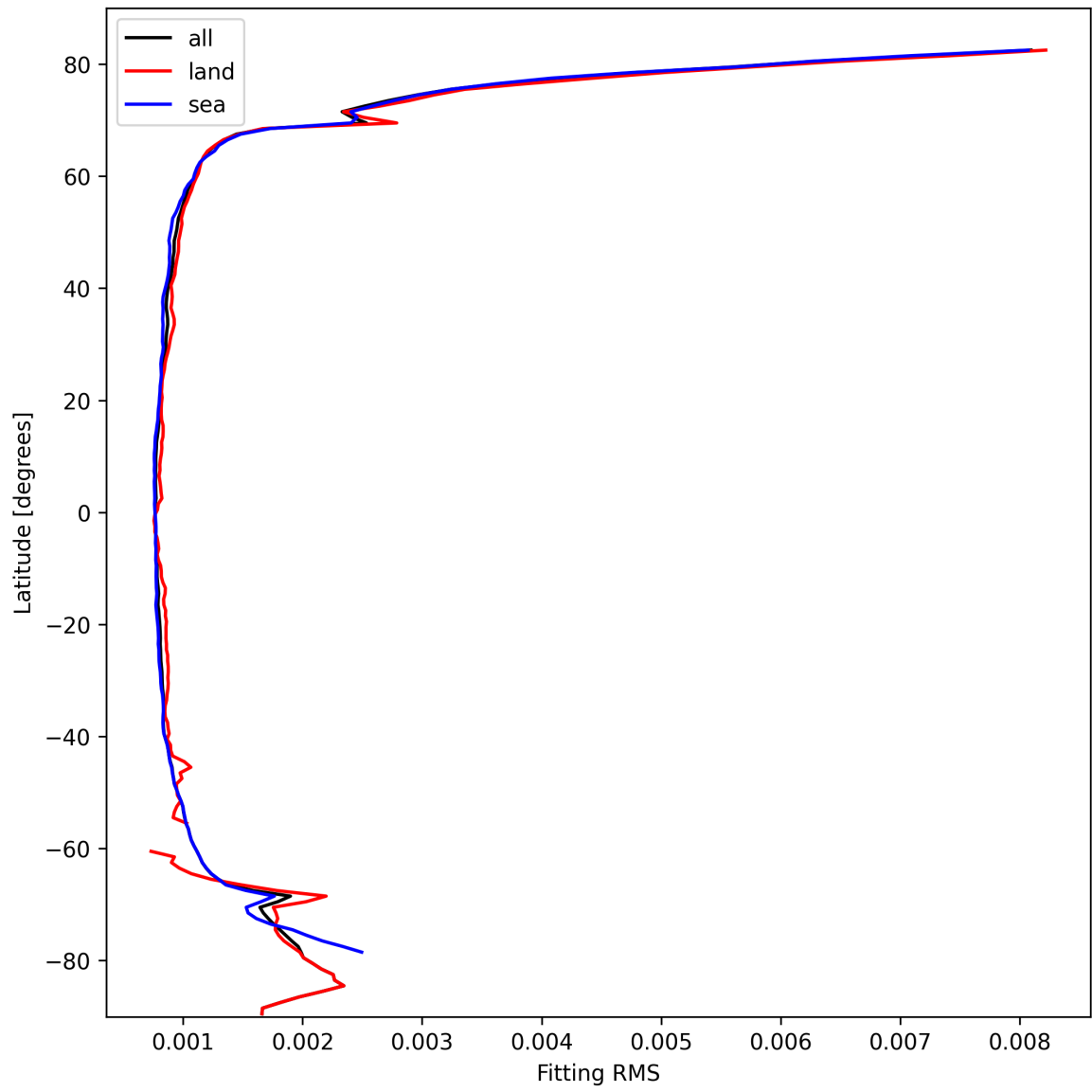
Figure 22: Zonal average of “Fitting RMS” for 2025-10-09 to 2025-10-09.
