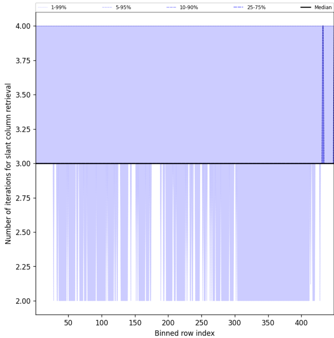
Figure 45: Along track statistics of “Number of iterations for slant column retrieval” for 2025-10-09 to 2025-10-09
