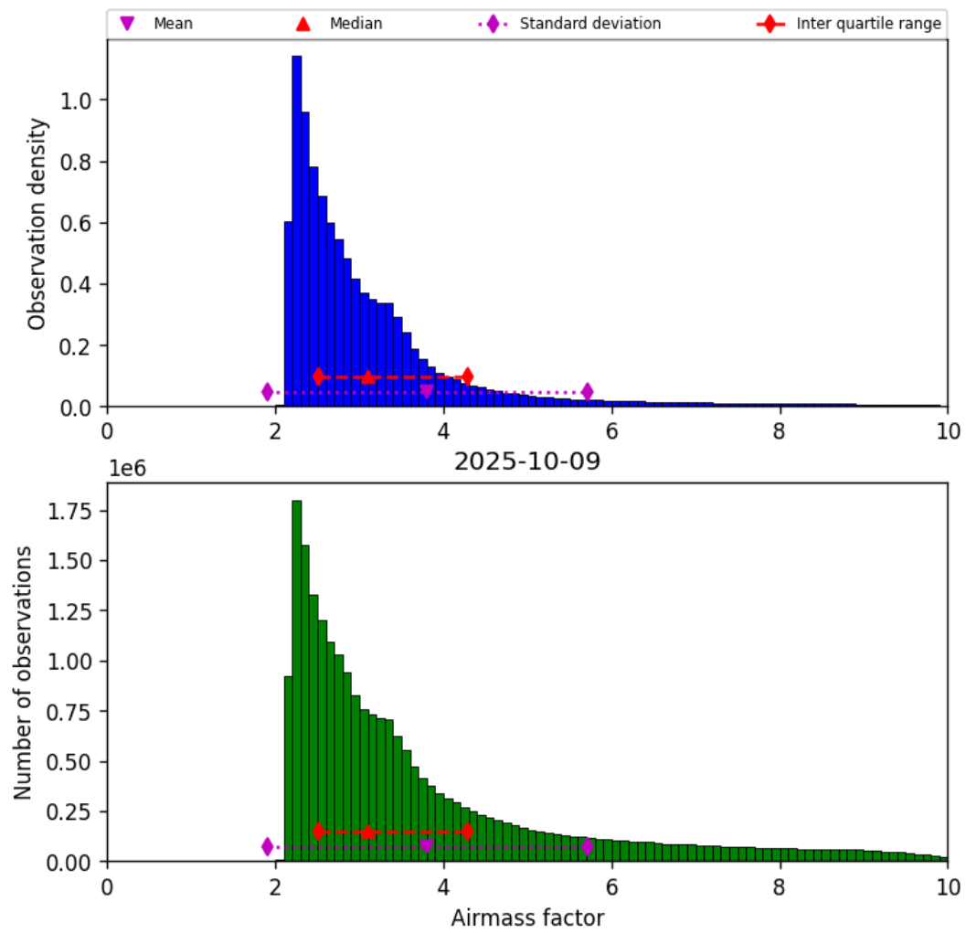
Figure 37: Histogram of “Airmass factor” for 2025-10-09 to 2025-10-09
