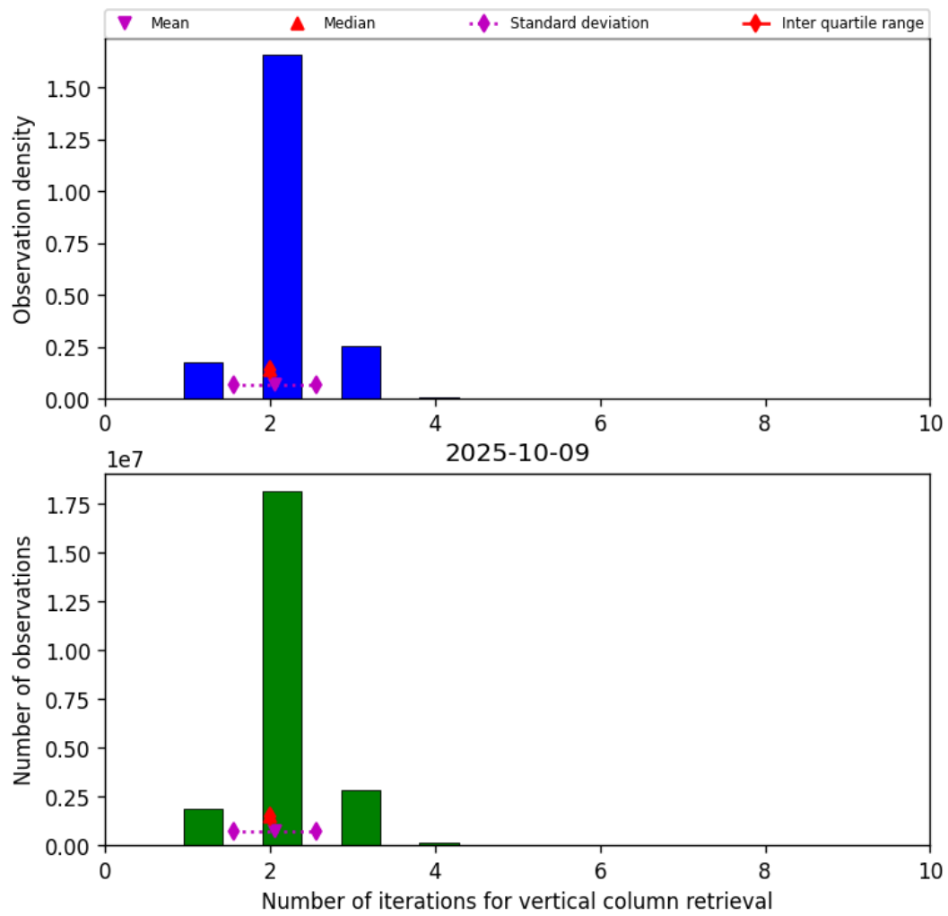
Figure 39: Histogram of “Number of iterations for vertical column retrieval” for 2025-10-09 to 2025-10-09
