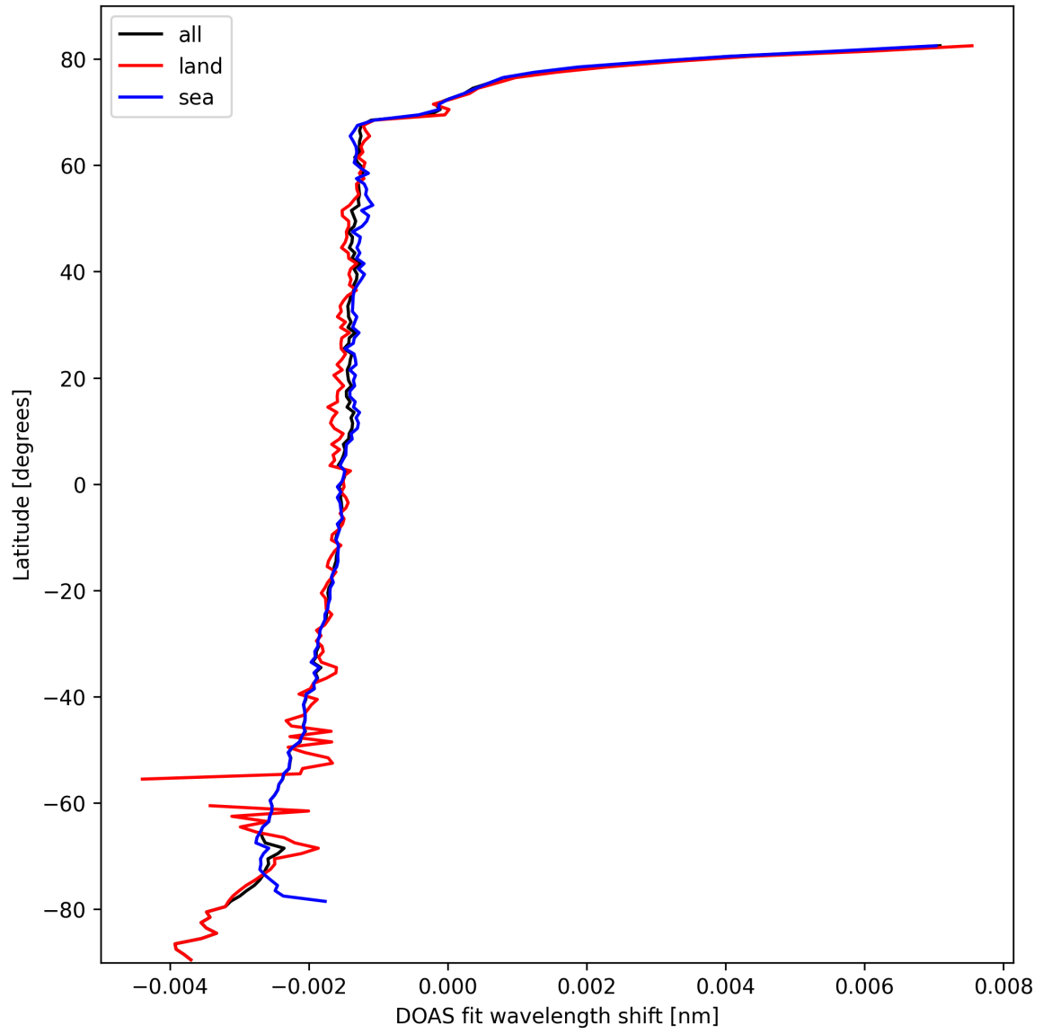
Figure 23: Zonal average of “DOAS fit wavelength shift” for 2025-10-09 to 2025-10-09.
