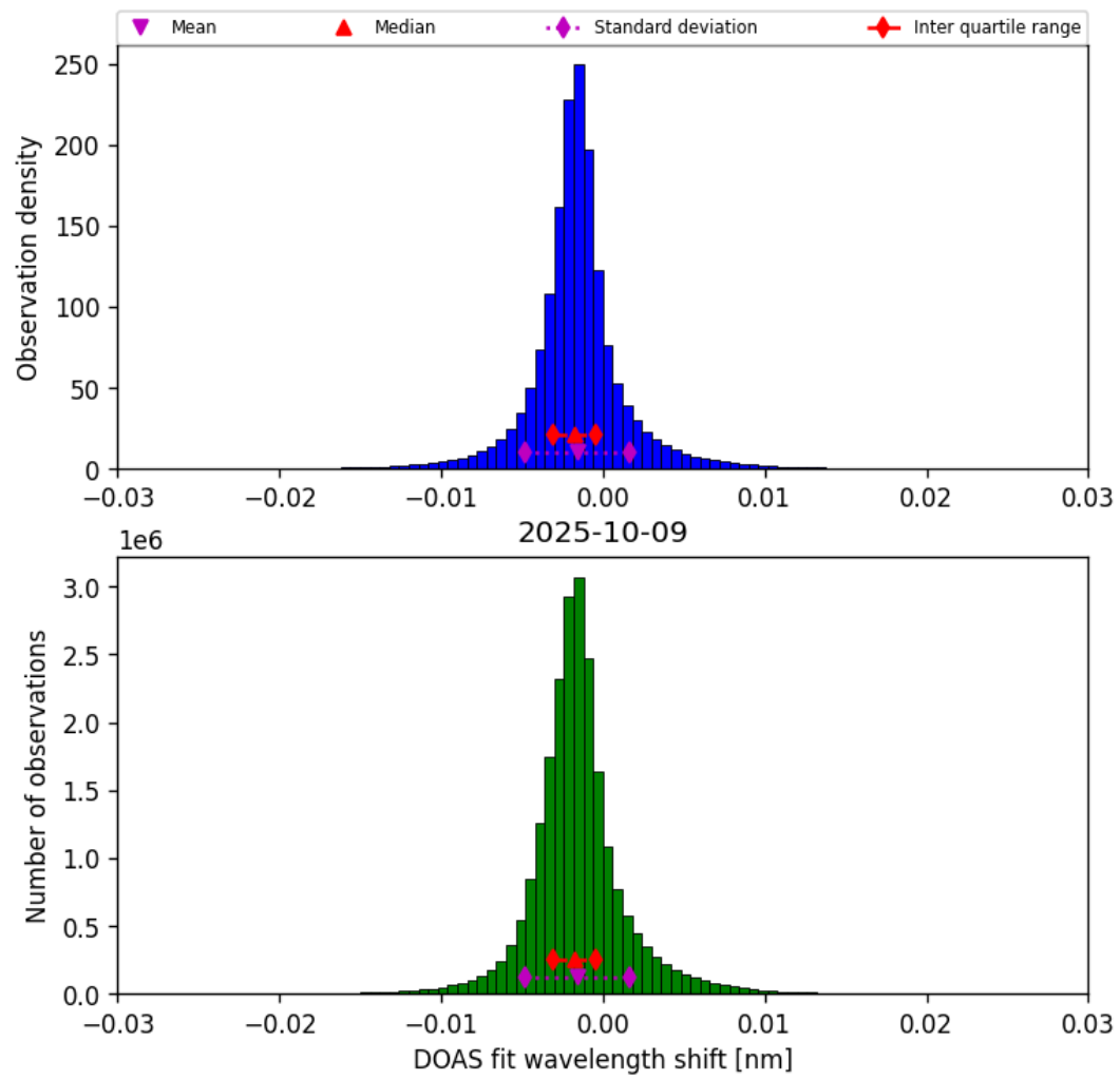
Figure 35: Histogram of “DOAS fit wavelength shift” for 2025-10-09 to 2025-10-09
