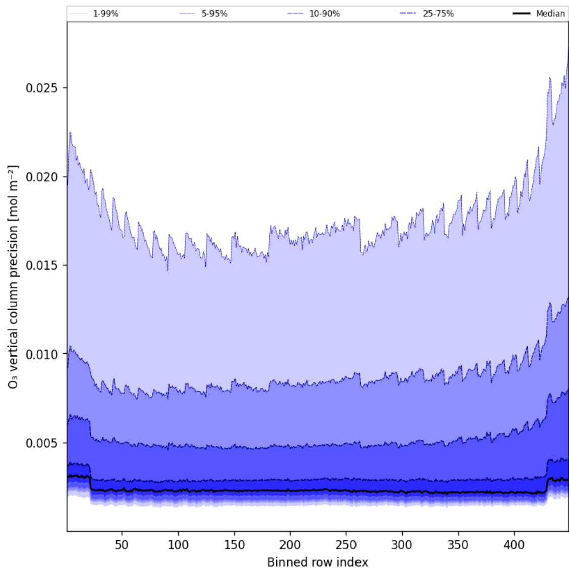
Figure 42: Along track statistics of “O 3 vertical column precision” for 2025-10-09 to 2025-10-09
