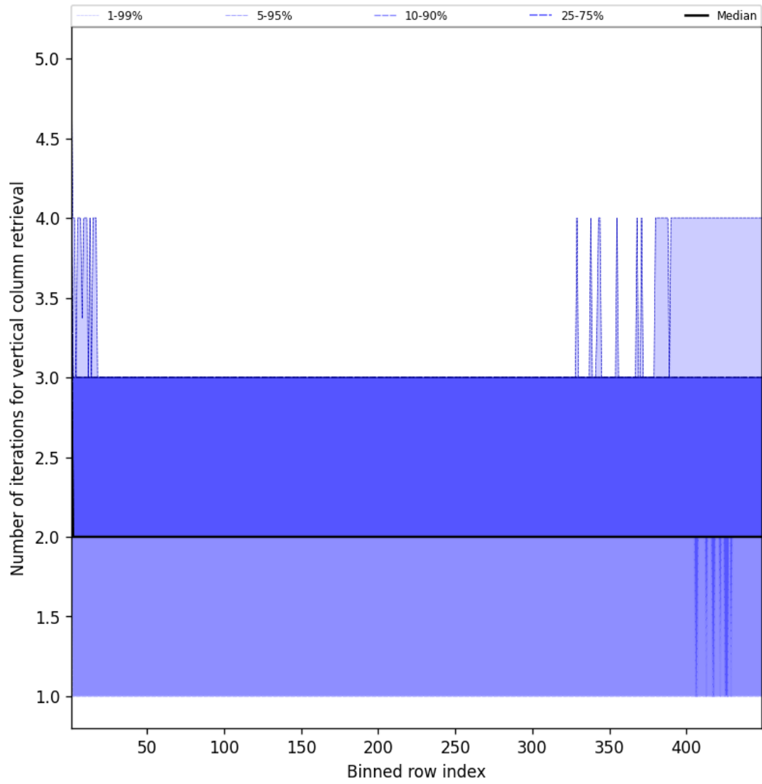
Figure 51: Along track statistics of “Number of iterations for vertical column retrieval” for 2025-10-09 to 2025-10-09
