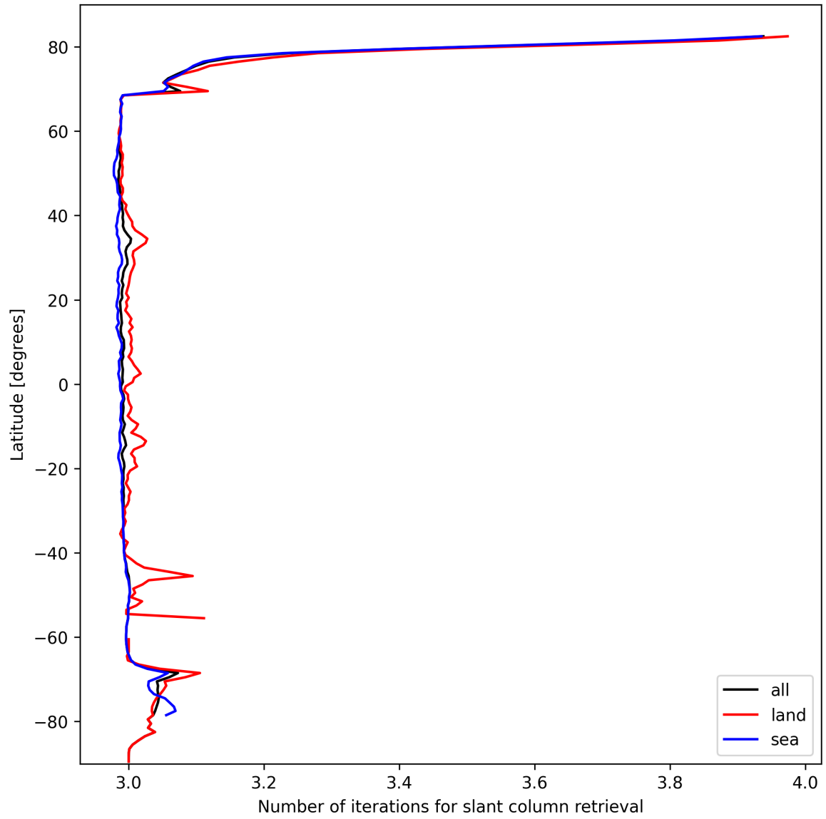
Figure 21: Zonal average of “Number of iterations for slant column retrieval” for 2025-10-09 to 2025-10-09.
