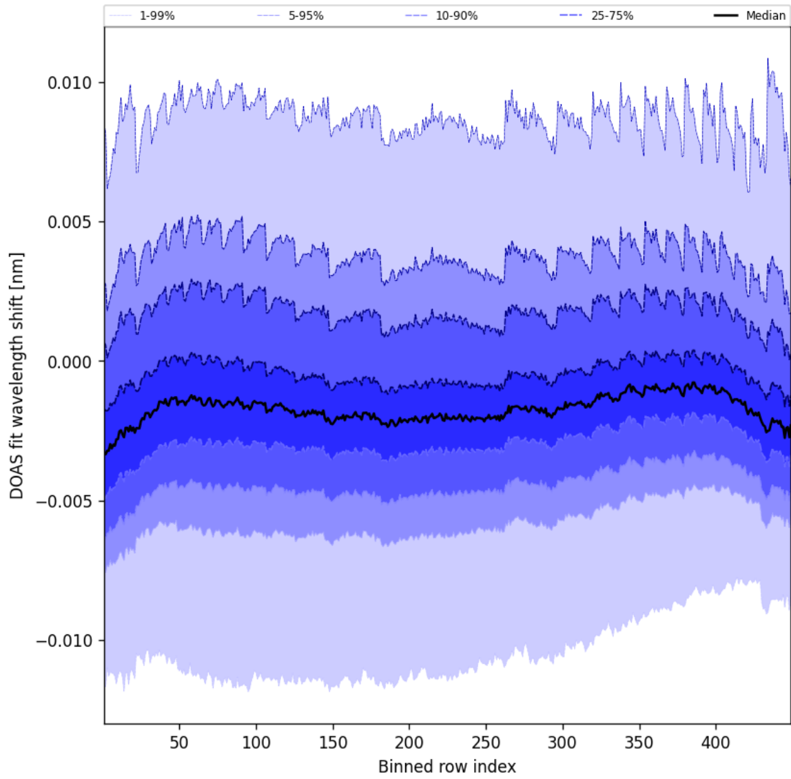
Figure 47: Along track statistics of "DOAS fit wavelength shift" for 2025-10-09 to 2025-10-09
