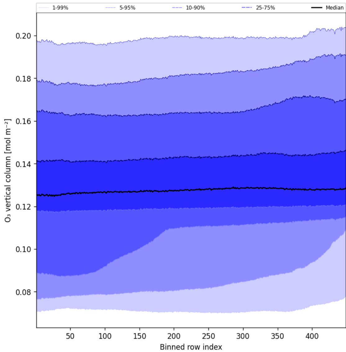
Figure 41: Along track statistics of “O 3 vertical column” for 2025-10-09 to 2025-10-09
