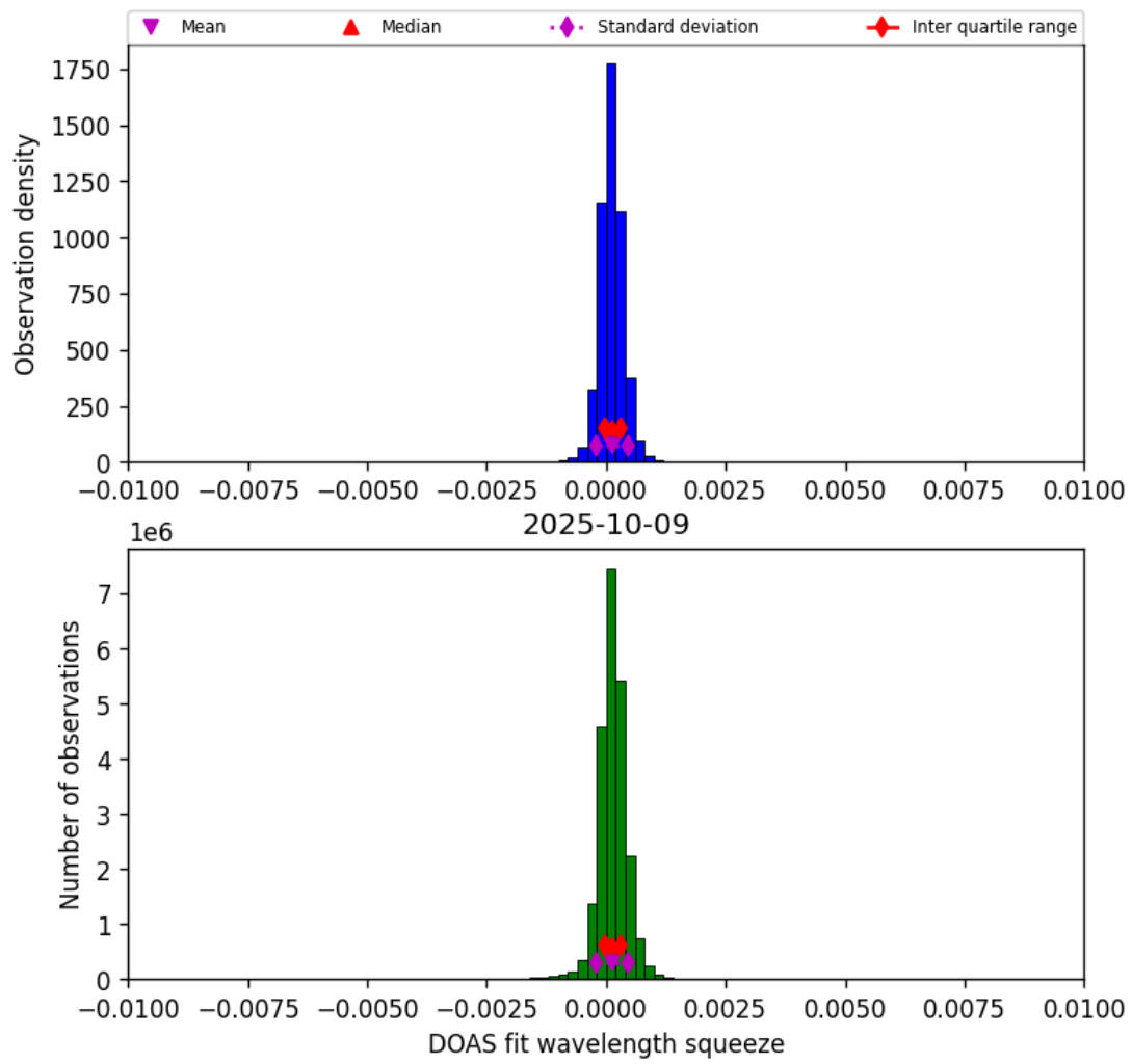
Figure 36: Histogram of “DOAS fit wavelength squeeze” for 2025-10-09 to 2025-10-09
