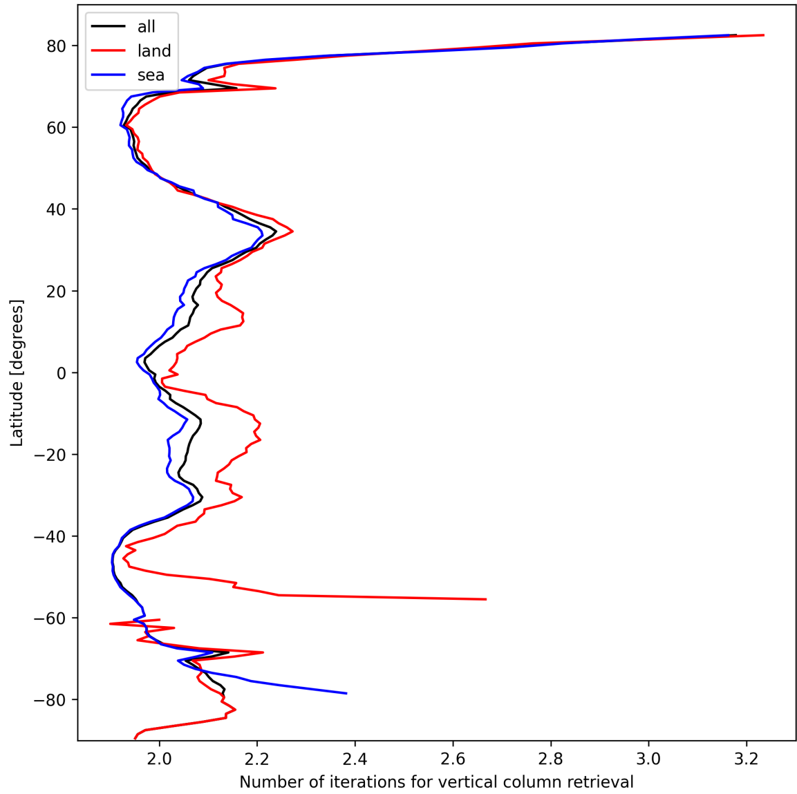
Figure 27: Zonal average of “Number of iterations for vertical column retrieval” for 2025-10-09 to 2025-10-09.
