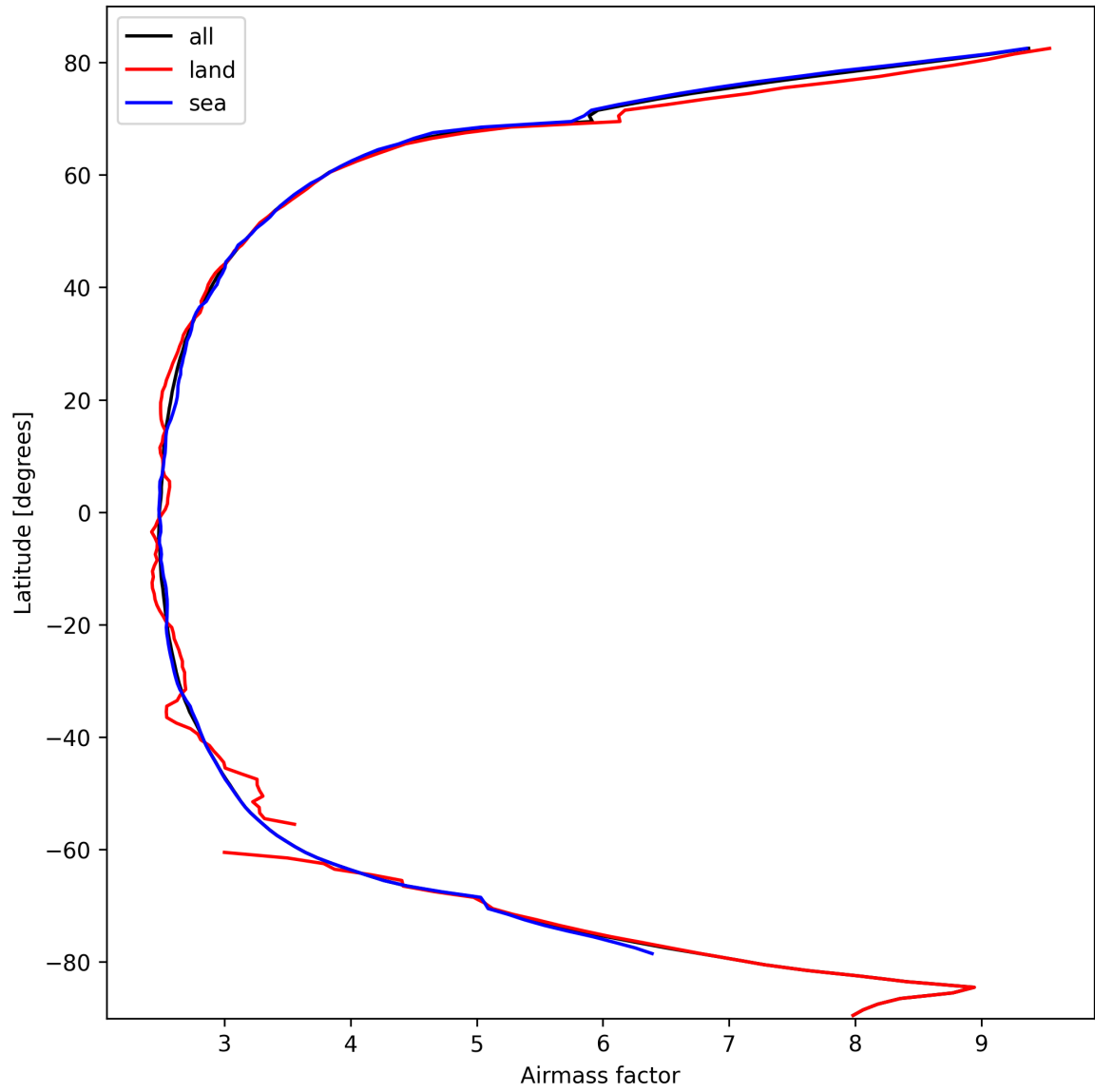
Figure 25: Zonal average of “Airmass factor” for 2025-10-09 to 2025-10-09.
