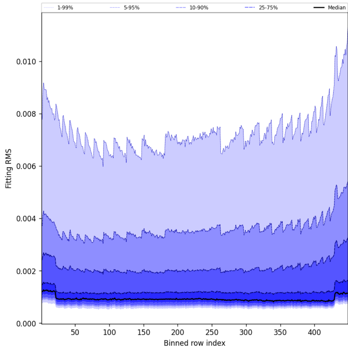
Figure 46: Along track statistics of “Fitting RMS” for 2025-10-09 to 2025-10-09
