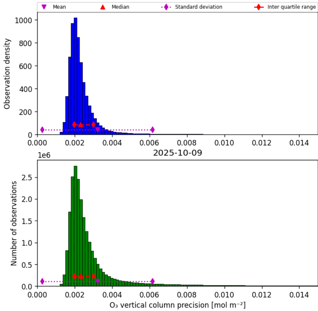
Figure 30: Histogram of "O 3 vertical column precision" for 2025-10-09 to 2025-10-09
