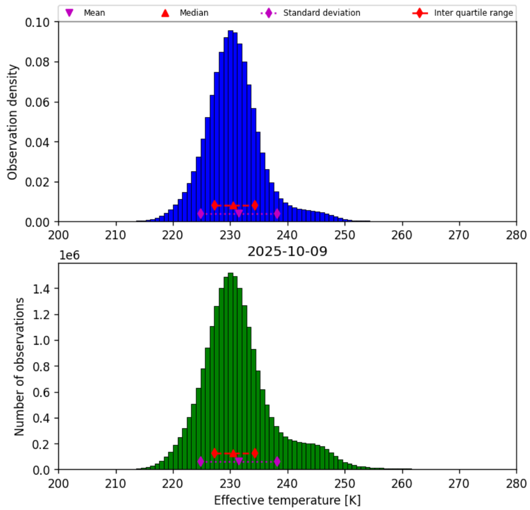
Figure 38: Histogram of “Effective temperature” for 2025-10-09 to 2025-10-09
