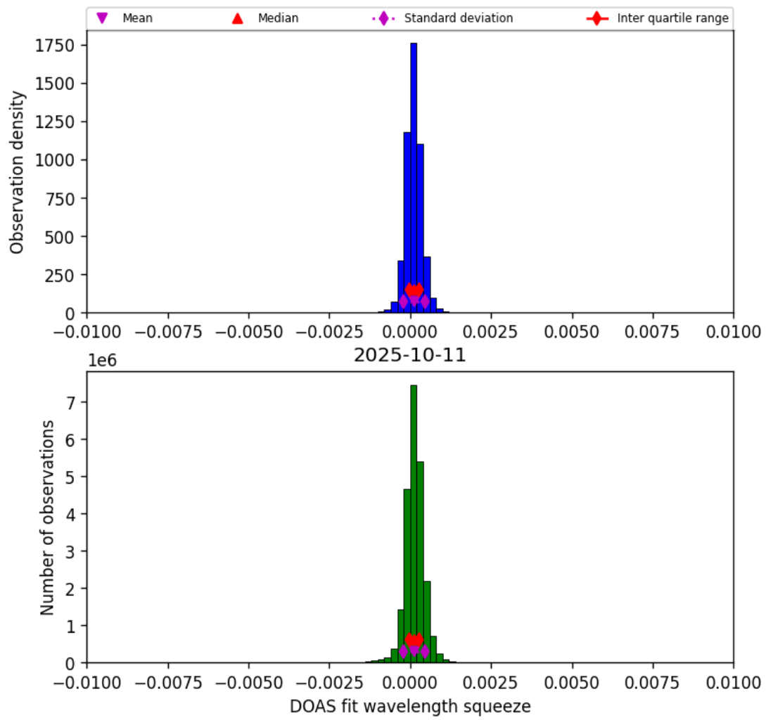
Figure 36: Histogram of “DOAS fit wavelength squeeze” for 2025-10-11 to 2025-10-12
