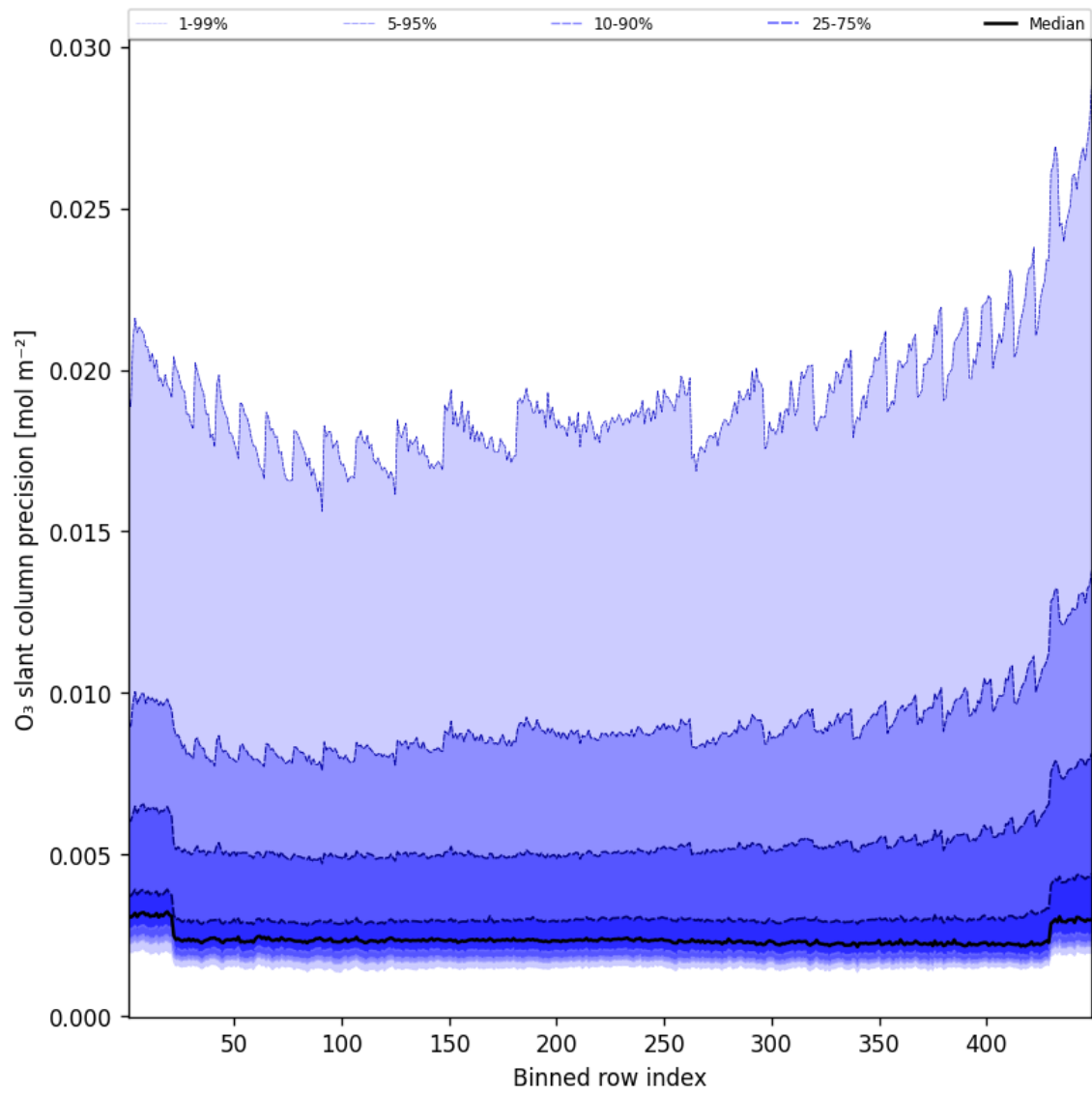
Figure 44: Along track statistics of “O 3 slant column precision” for 2025-10-11 to 2025-10-12
