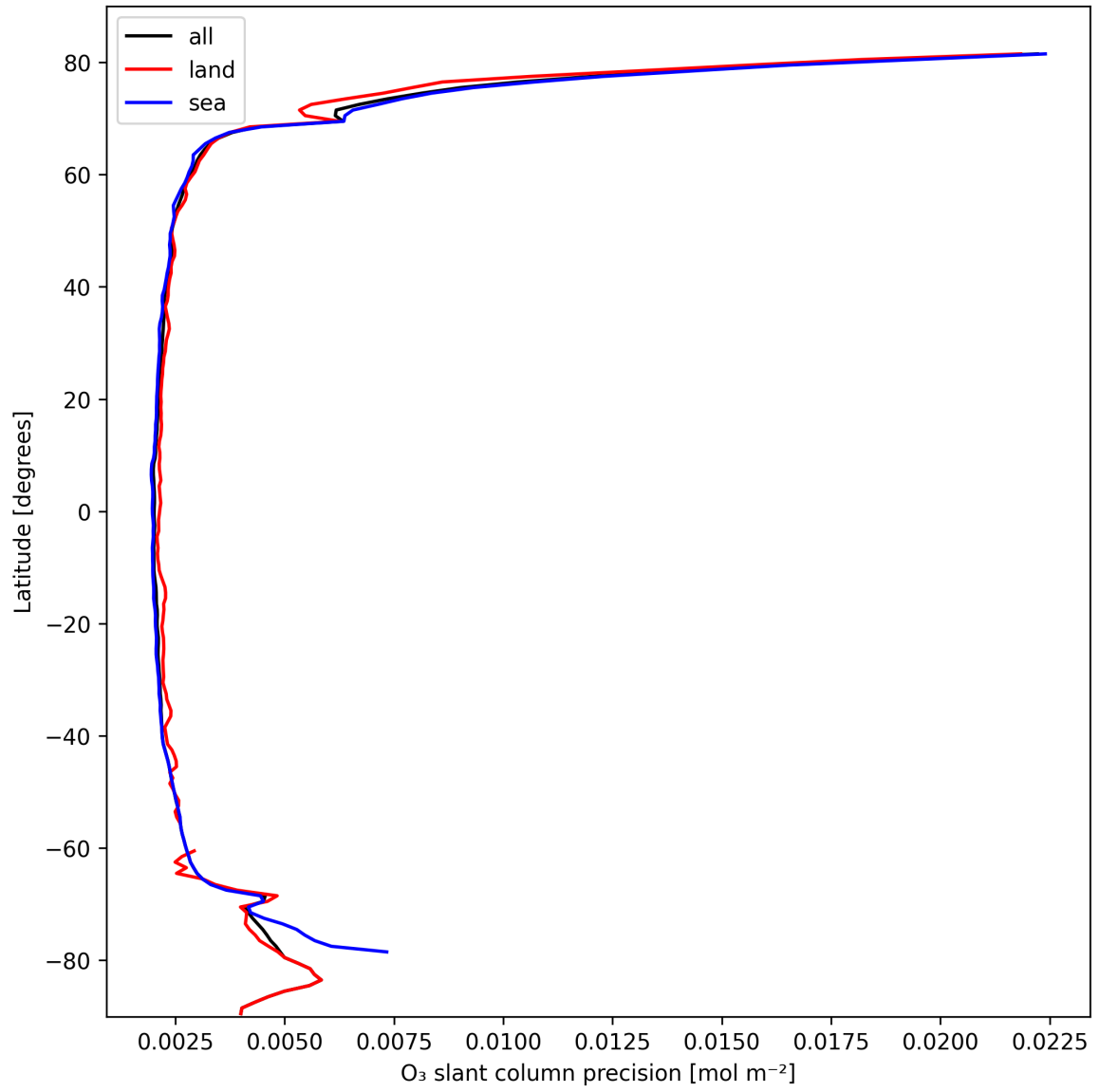
Figure 20: Zonal average of “O 3 slant column precision” for 2025-10-11 to 2025-10-12.
