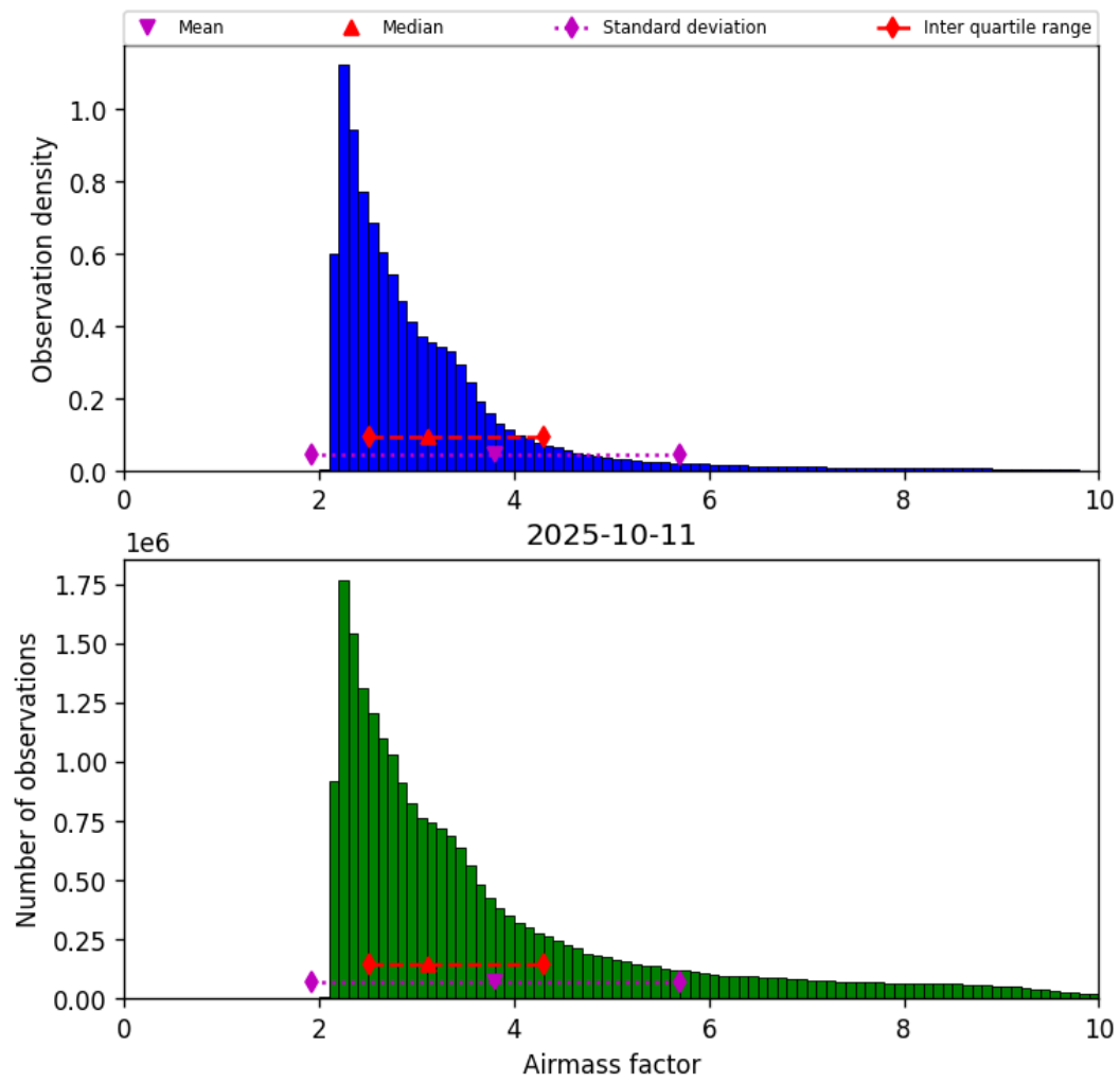
Figure 37: Histogram of “Airmass factor” for 2025-10-11 to 2025-10-12
