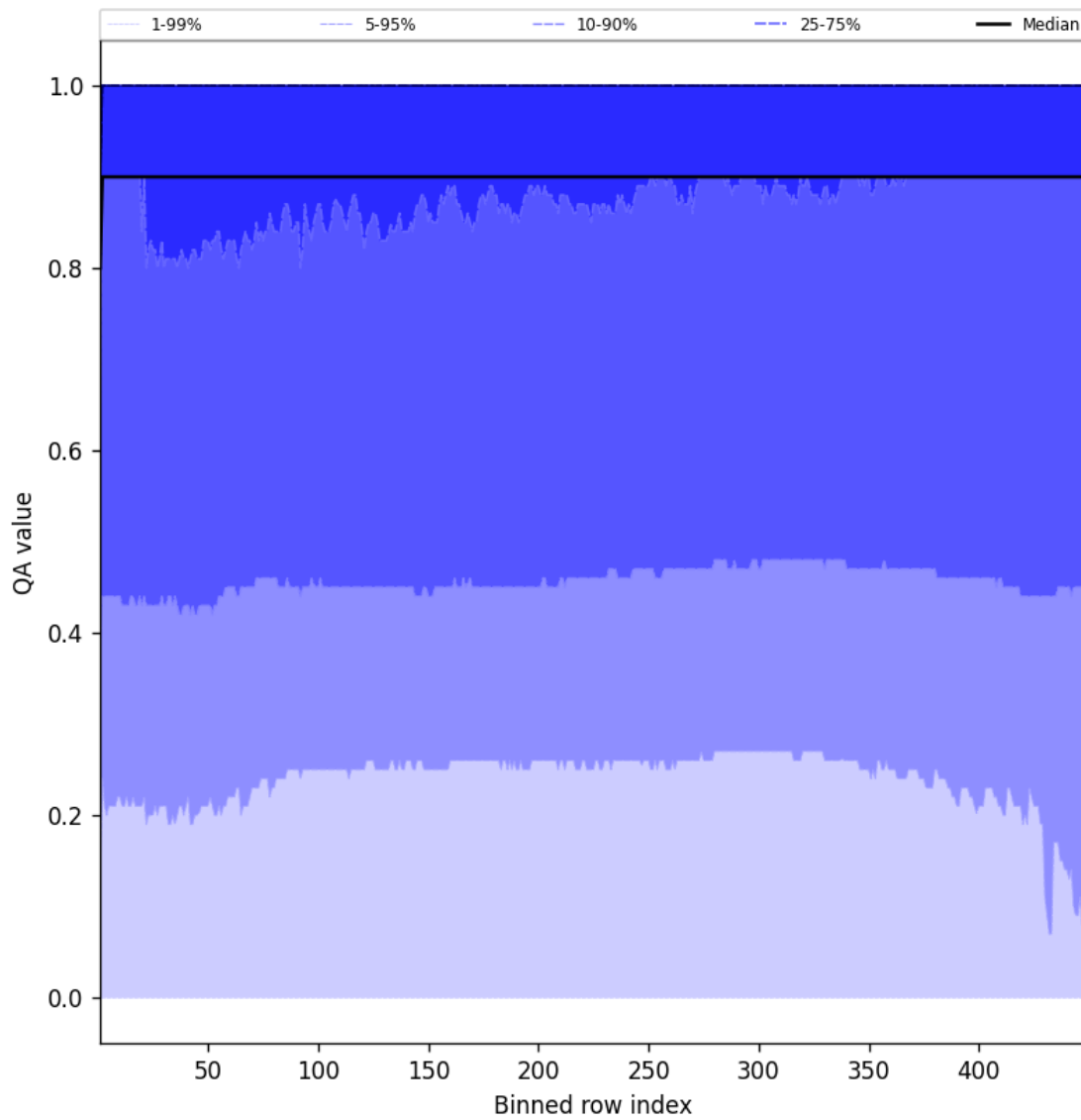
Figure 40: Along track statistics of “QA value” for 2025-10-11 to 2025-10-12
