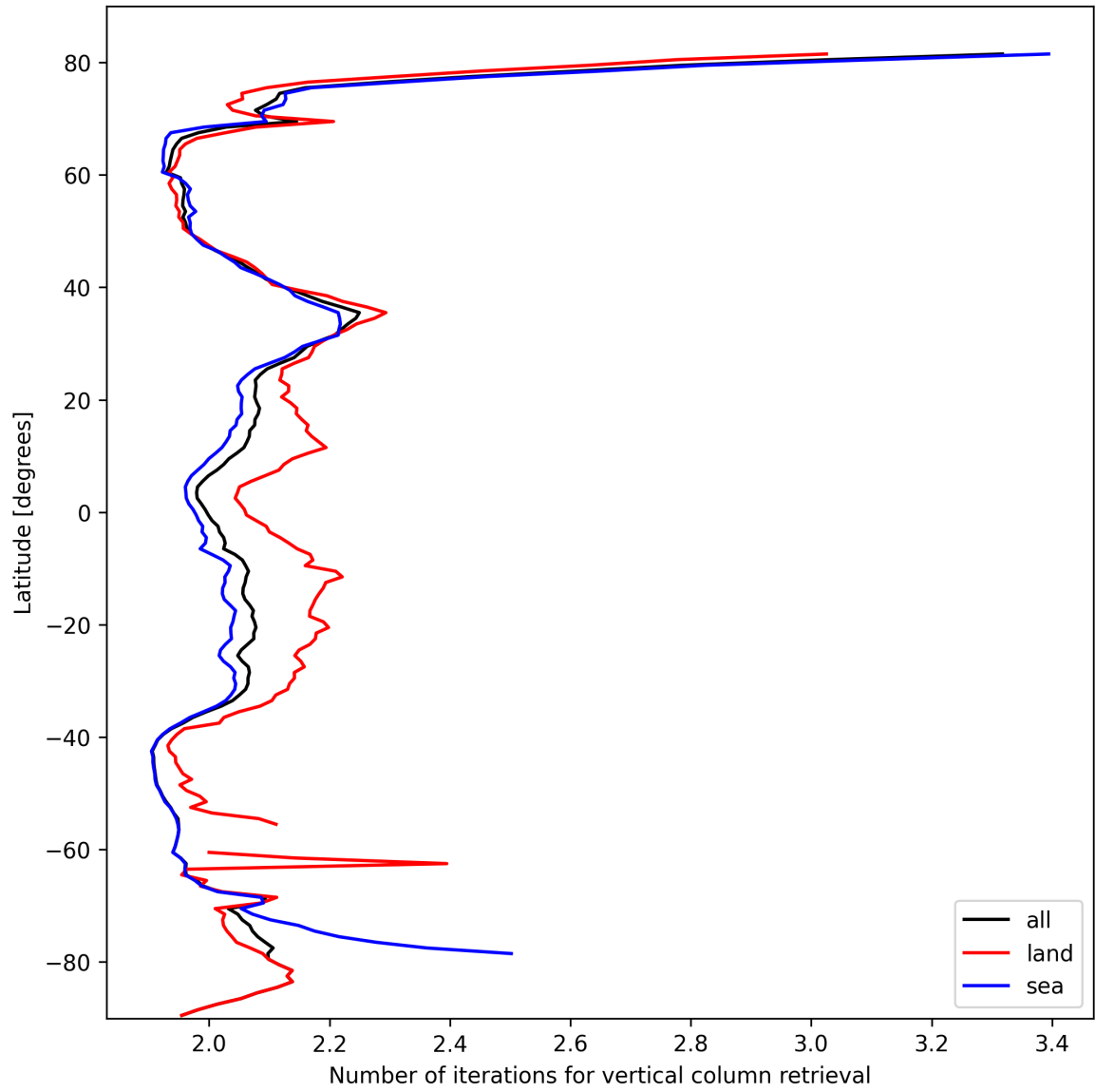
Figure 27: Zonal average of “Number of iterations for vertical column retrieval” for 2025-10-11 to 2025-10-12.
