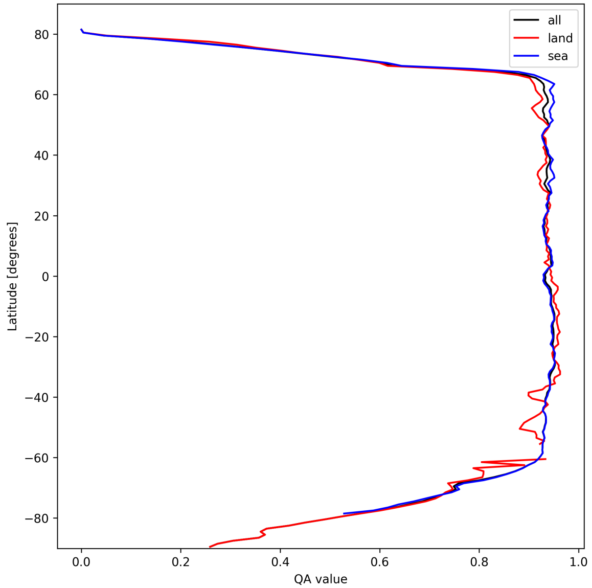
Figure 16: Zonal average of “QA value” for 2025-10-11 to 2025-10-12.
