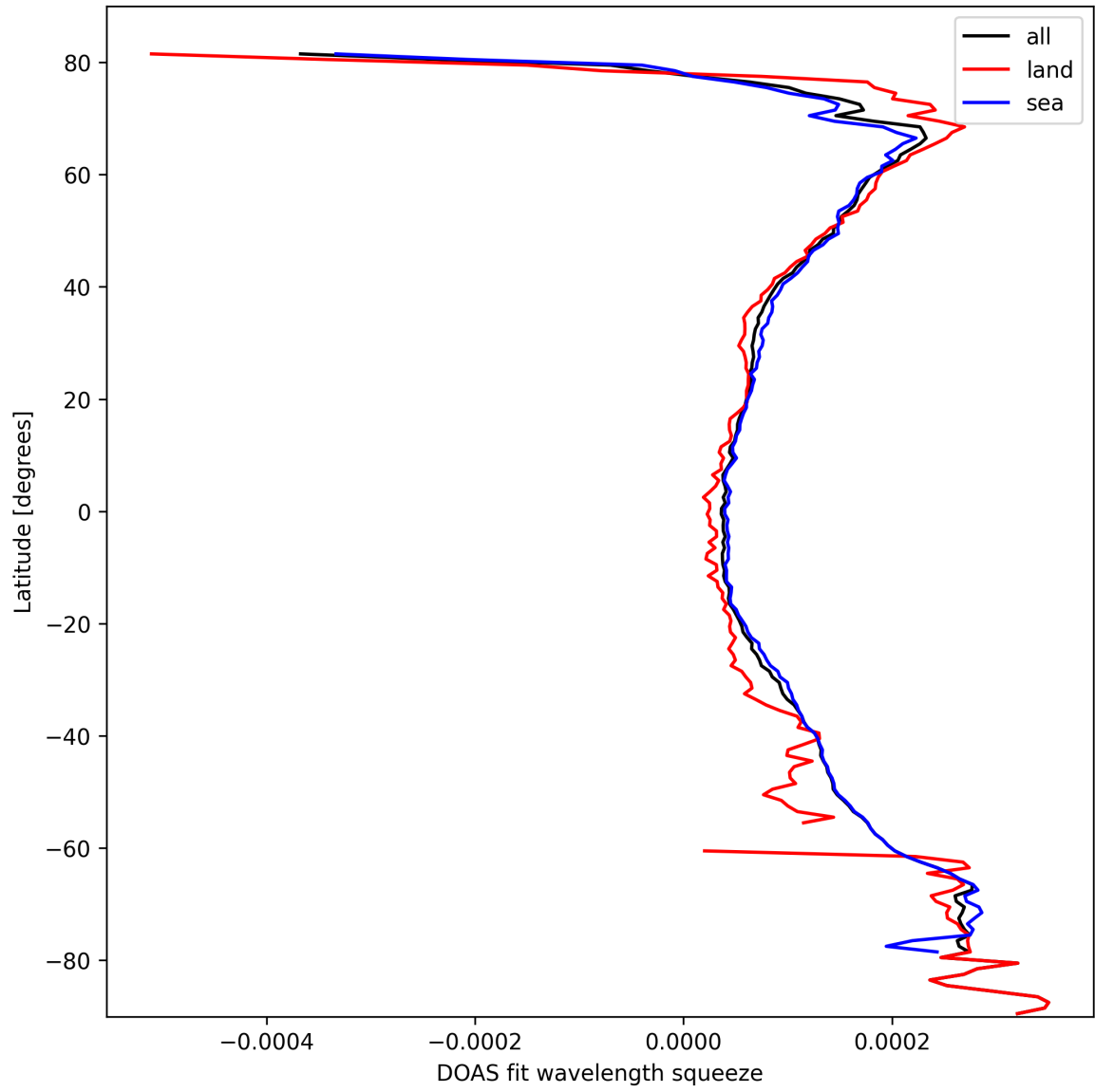
Figure 24: Zonal average of “DOAS fit wavelength squeeze” for 2025-10-11 to 2025-10-12.
