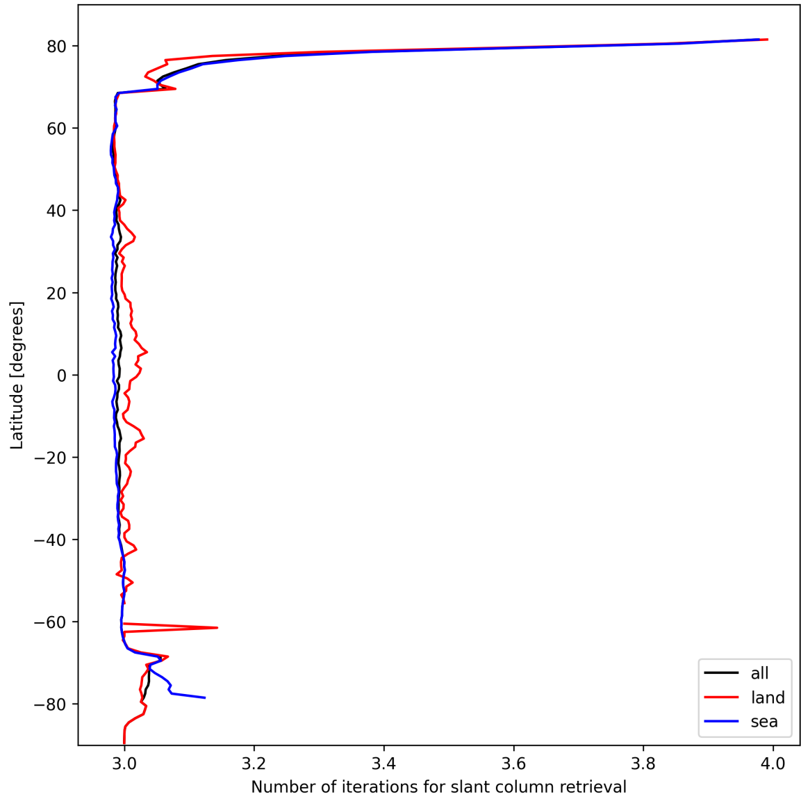
Figure 21: Zonal average of “Number of iterations for slant column retrieval” for 2025-10-11 to 2025-10-12.
