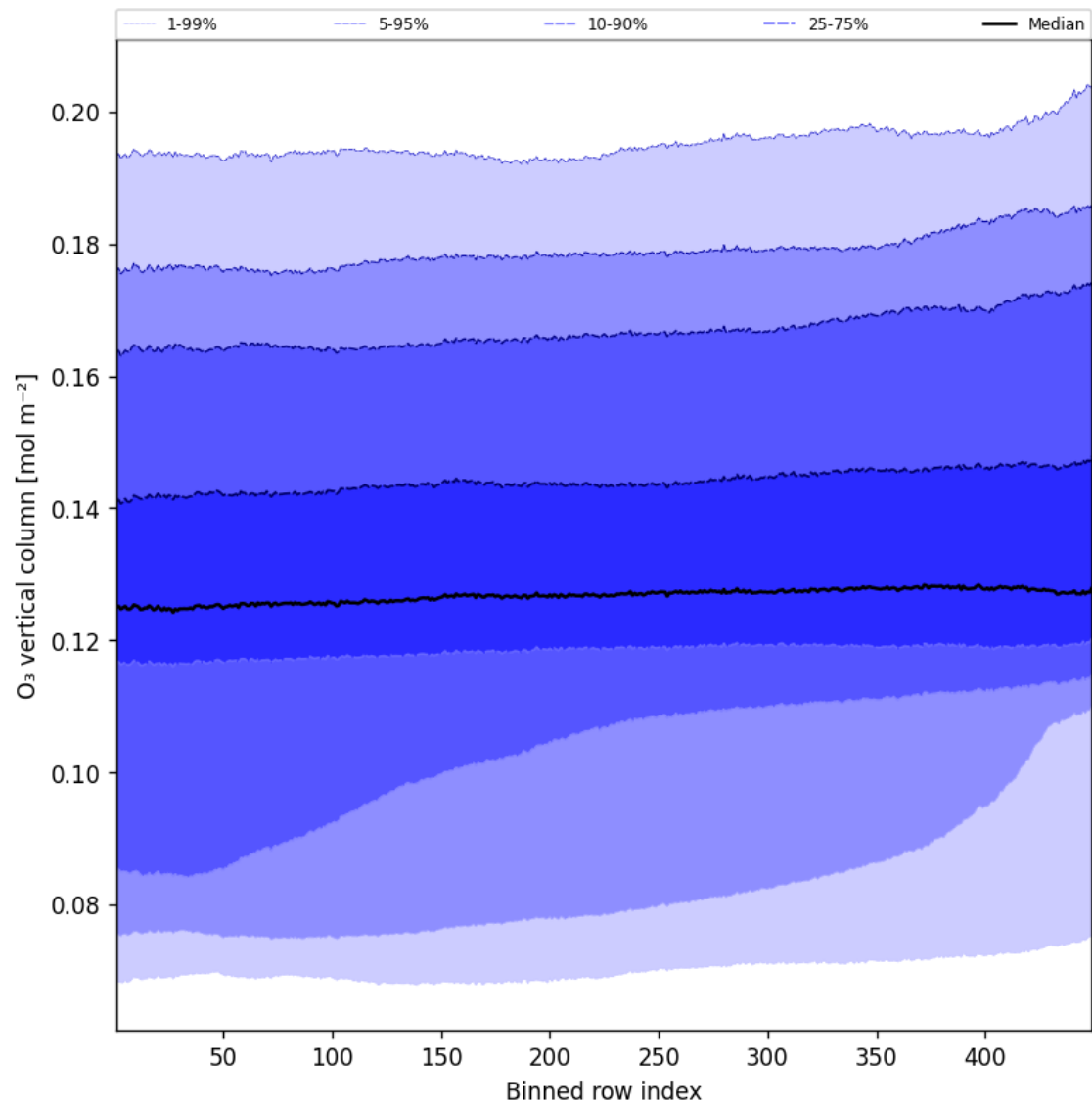
Figure 41: Along track statistics of “O 3 vertical column” for 2025-10-11 to 2025-10-12
