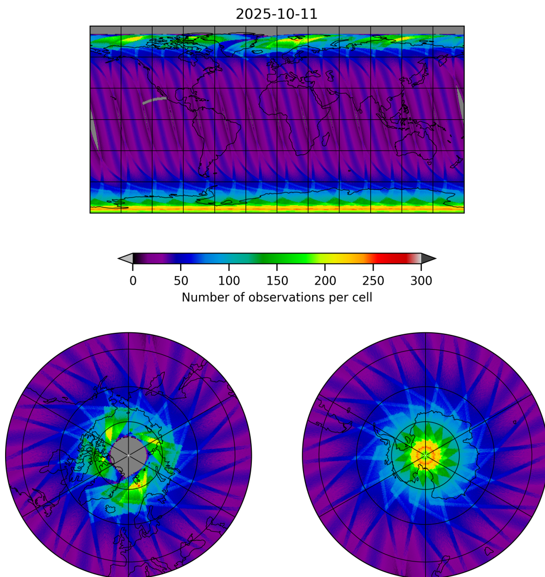
Figure 15: Map of the number of observations for 2025-10-11 to 2025-10-12
