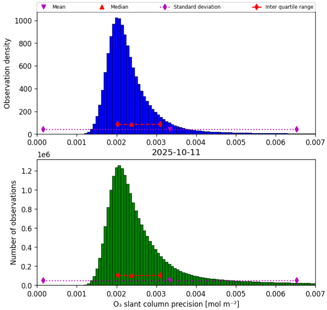
Figure 32: Histogram of “O 3 slant column precision” for 2025-10-11 to 2025-10-12
