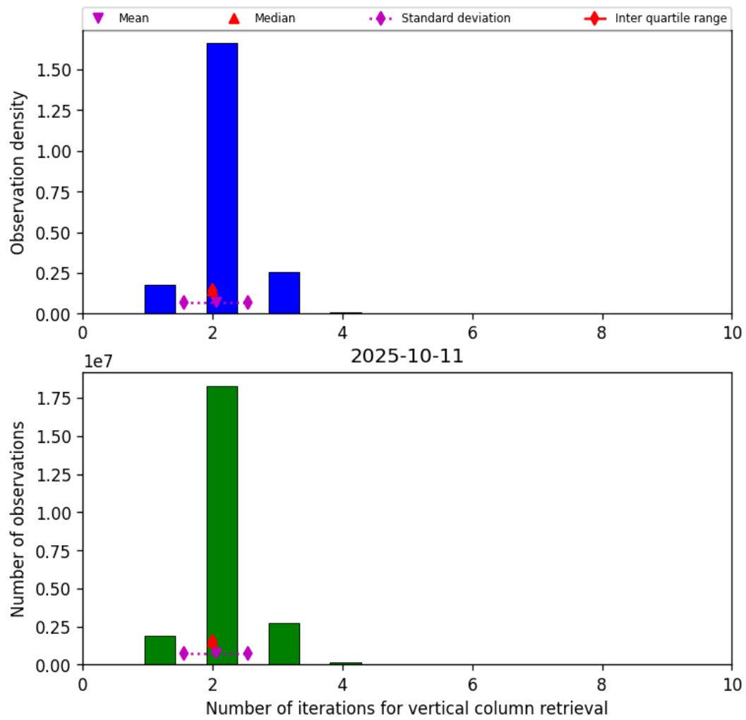
Figure 39: Histogram of “Number of iterations for vertical column retrieval” for 2025-10-11 to 2025-10-12
