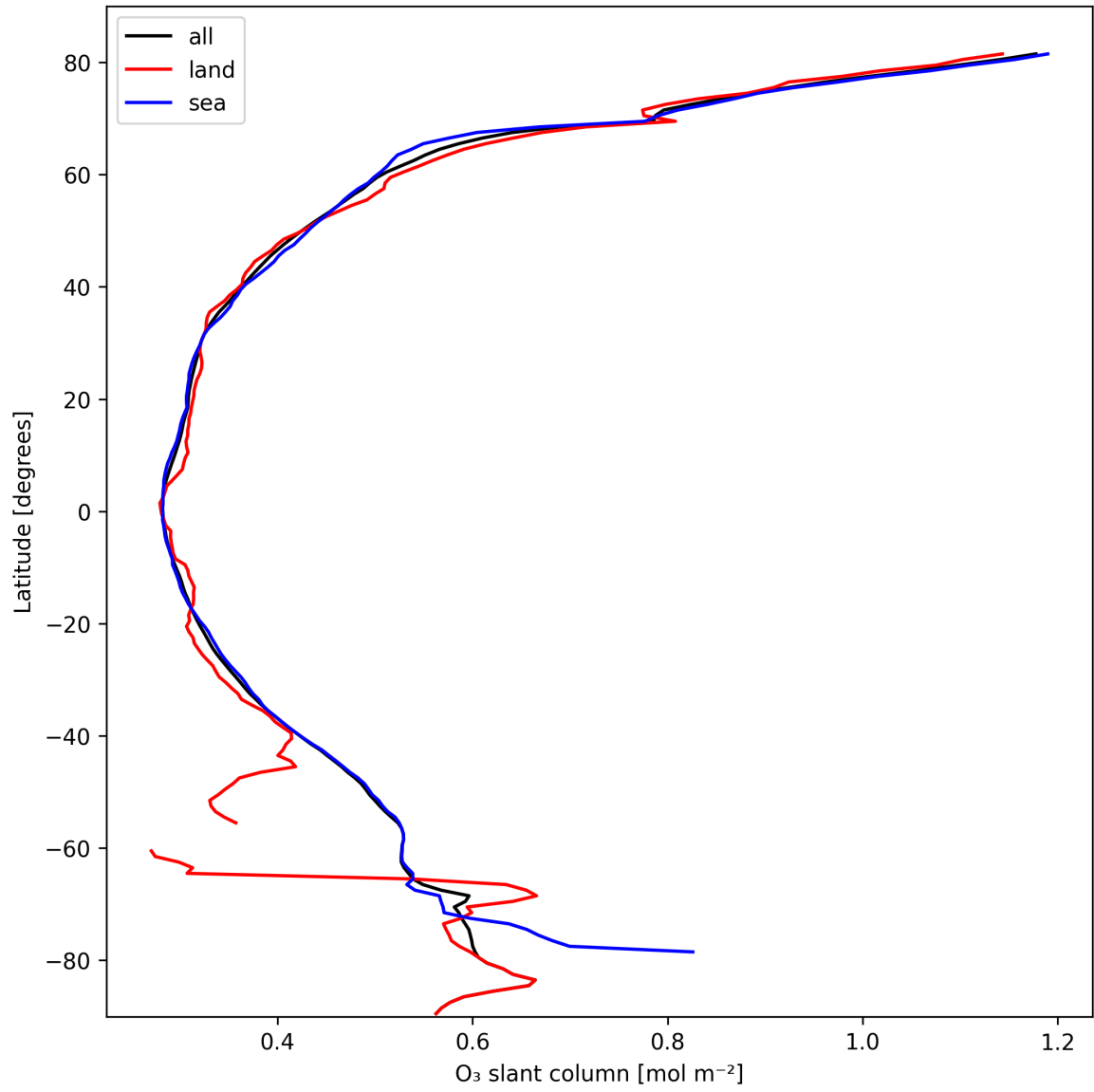
Figure 19: Zonal average of “O 3 slant column” for 2025-10-11 to 2025-10-12.
