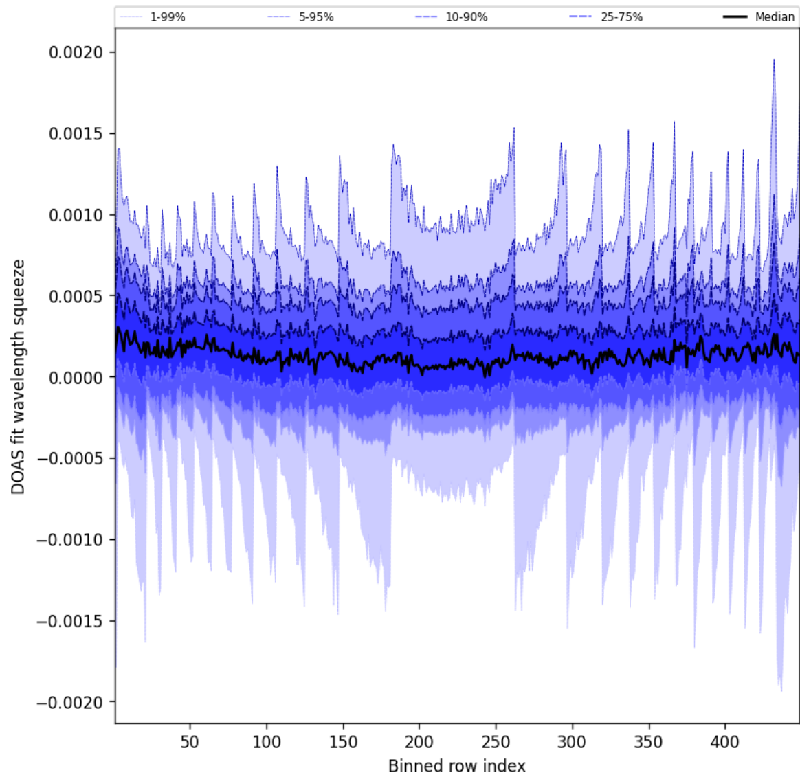
Figure 48: Along track statistics of “DOAS fit wavelength squeeze” for 2025-10-11 to 2025-10-12
