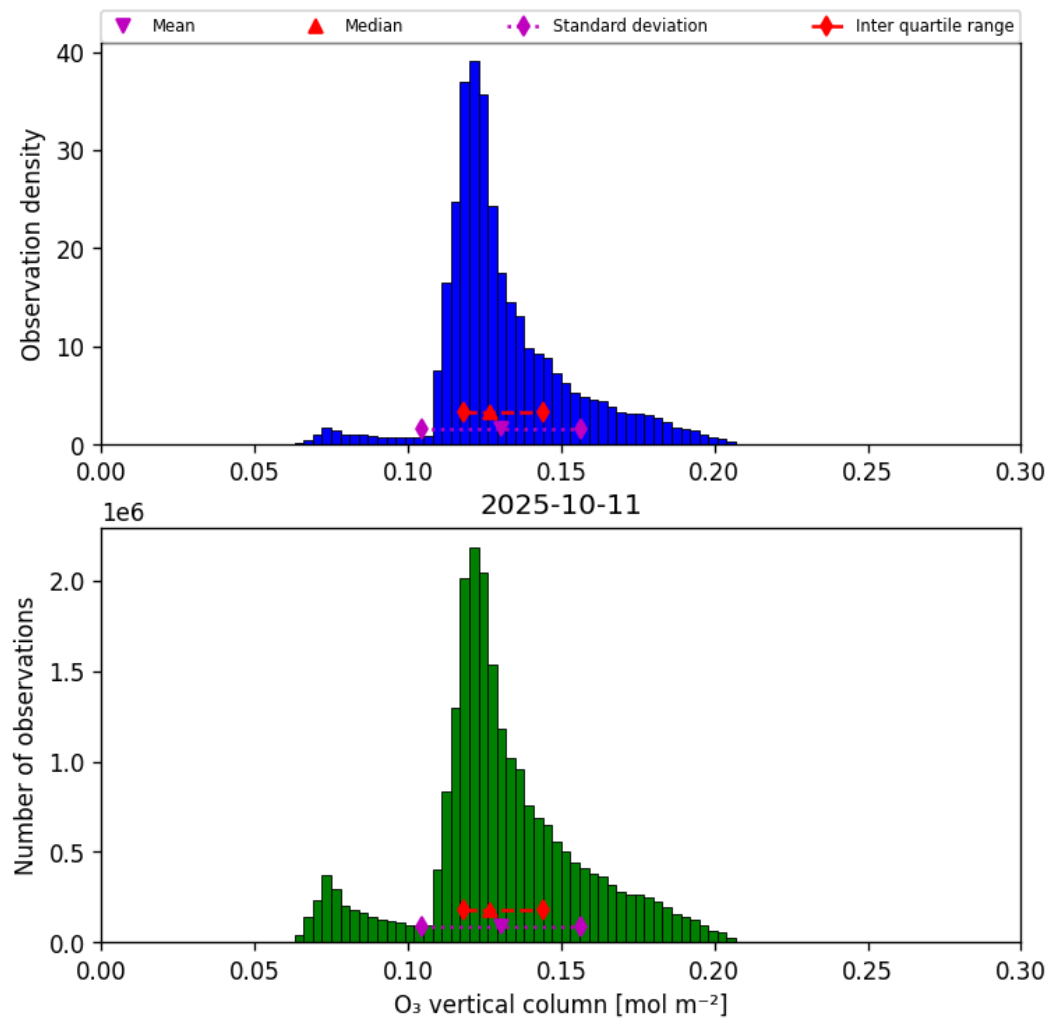
Figure 29: Histogram of “O 3 vertical column” for 2025-10-11 to 2025-10-12
