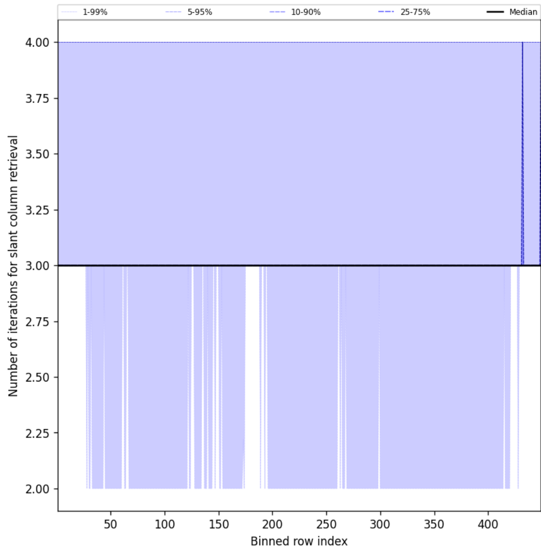
Figure 45: Along track statistics of “Number of iterations for slant column retrieval” for 2025-10-11 to 2025-10-12
