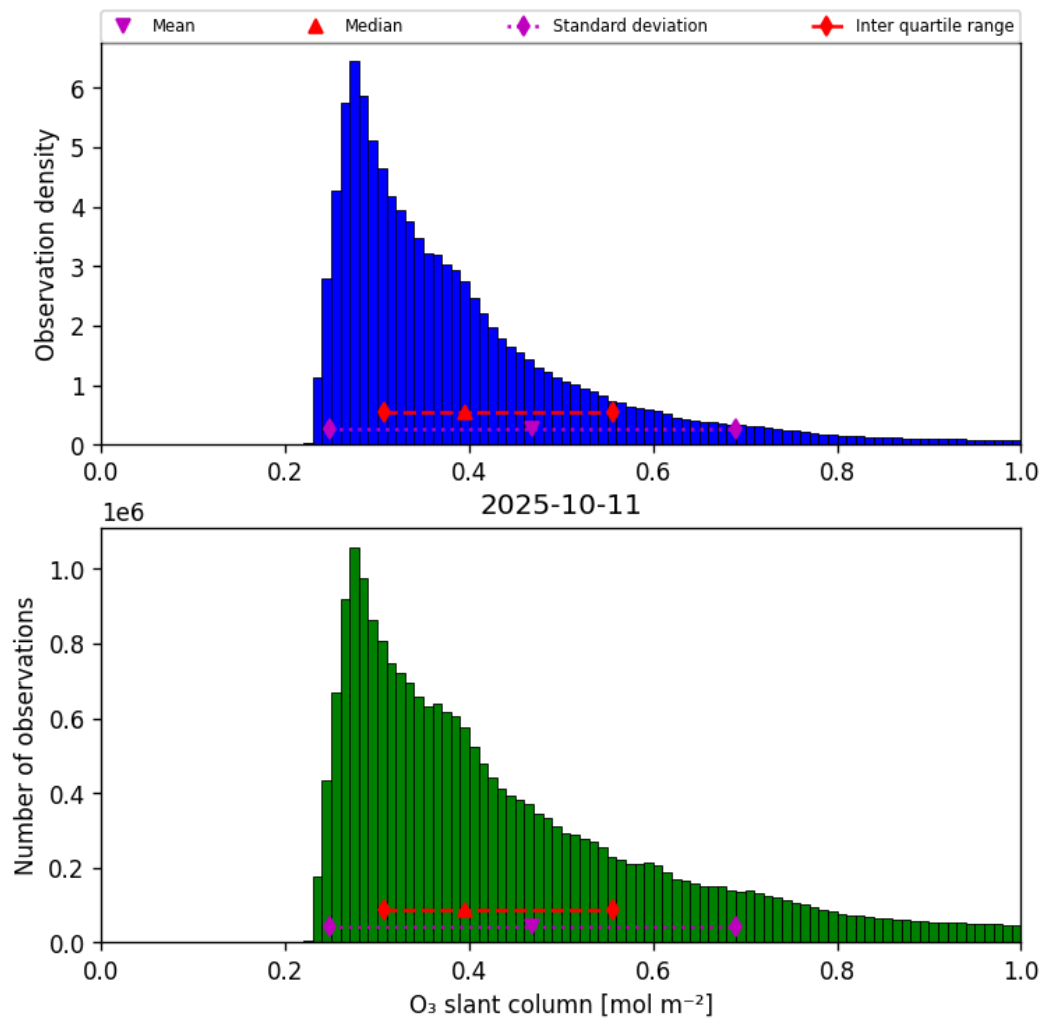
Figure 31: Histogram of “O 3 slant column” for 2025-10-11 to 2025-10-12
