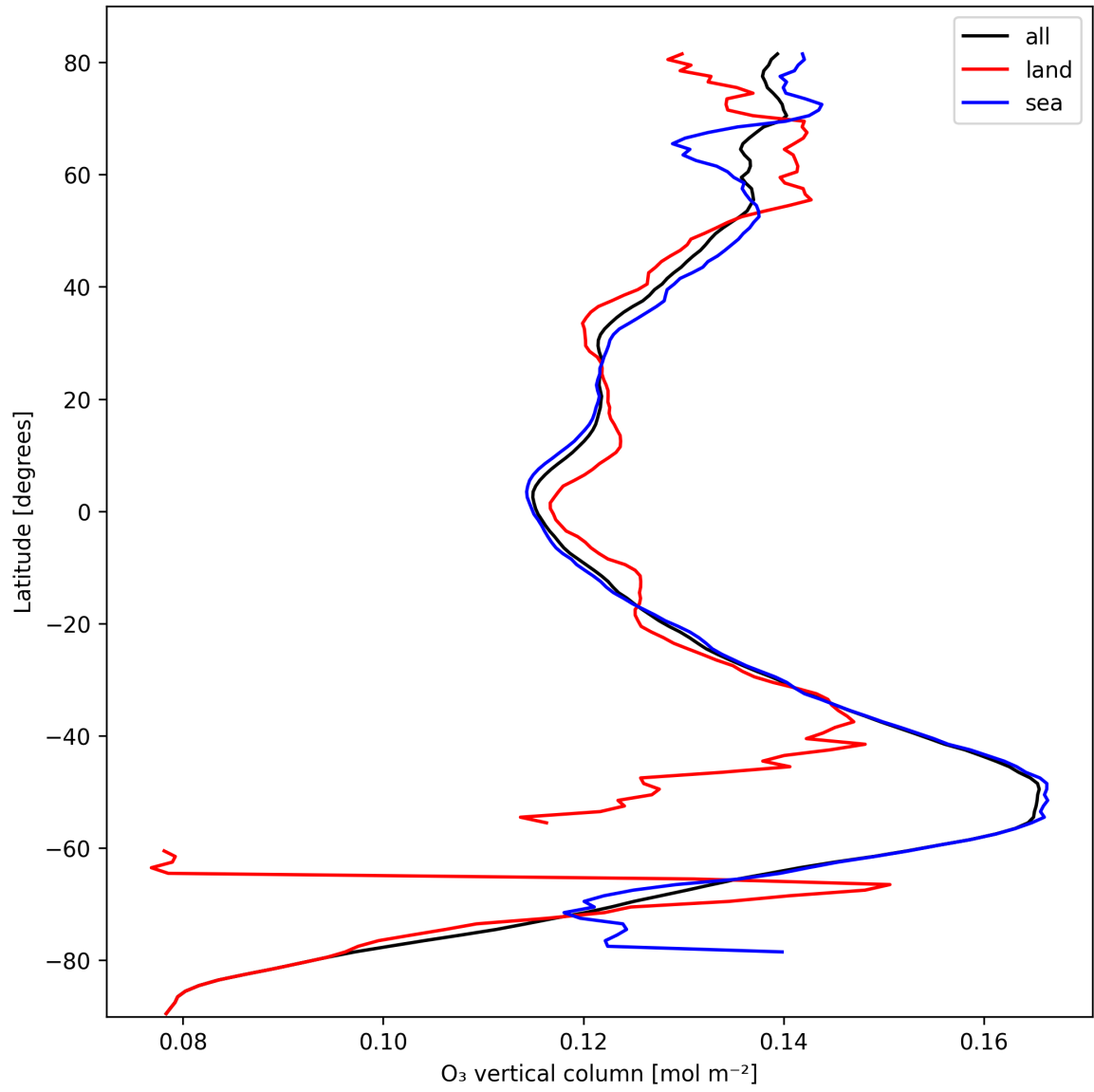
Figure 17: Zonal average of “O 3 vertical column” for 2025-10-11 to 2025-10-12.
