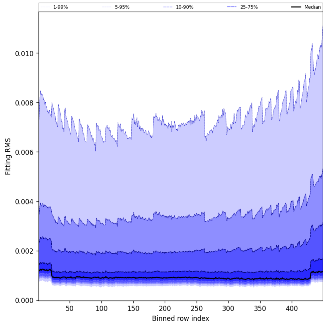
Figure 46: Along track statistics of “Fitting RMS” for 2025-10-11 to 2025-10-12
