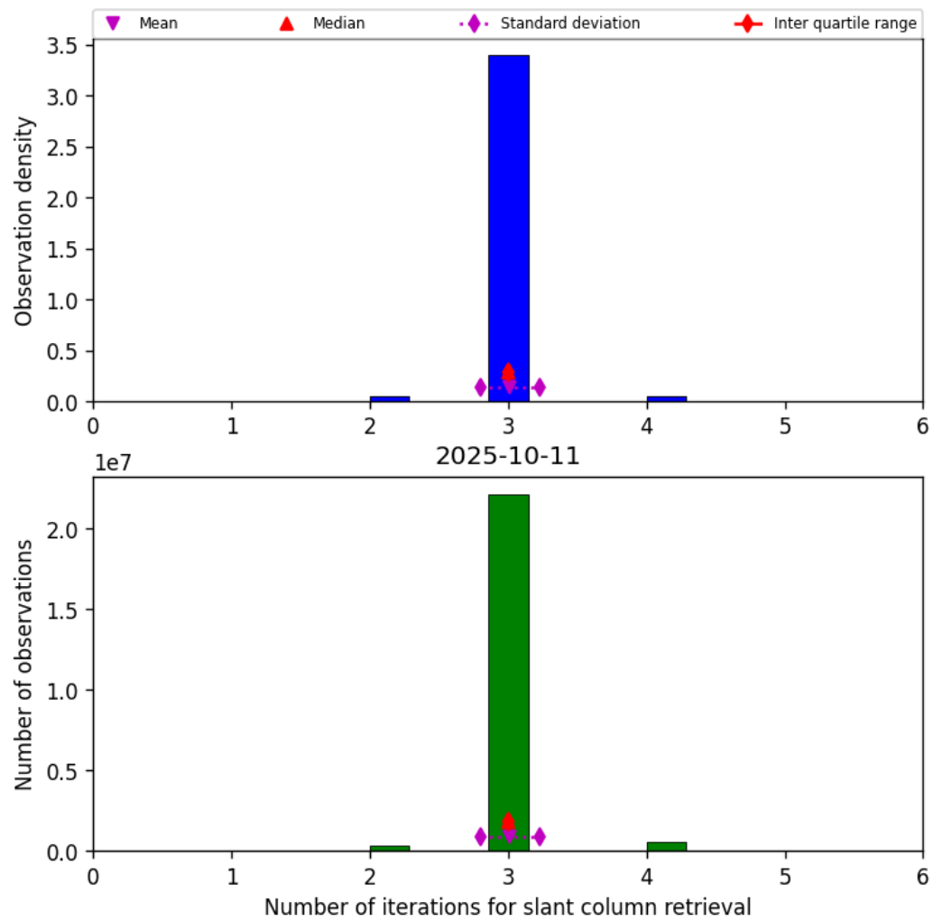
Figure 33: Histogram of “Number of iterations for slant column retrieval” for 2025-10-11 to 2025-10-12
