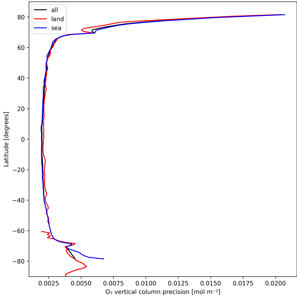
Figure 18: Zonal average of “O 3 vertical column precision” for 2025-10-11 to 2025-10-12.
