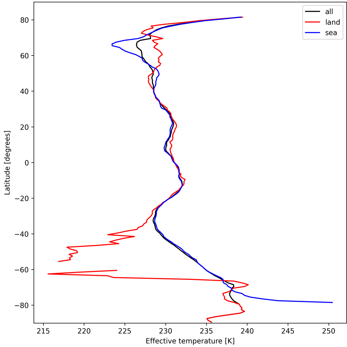
Figure 26: Zonal average of “Effective temperature” for 2025-10-11 to 2025-10-12.
