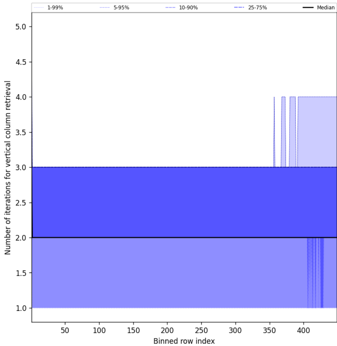
Figure 51: Along track statistics of “Number of iterations for vertical column retrieval” for 2025-10-11 to 2025-10-12
