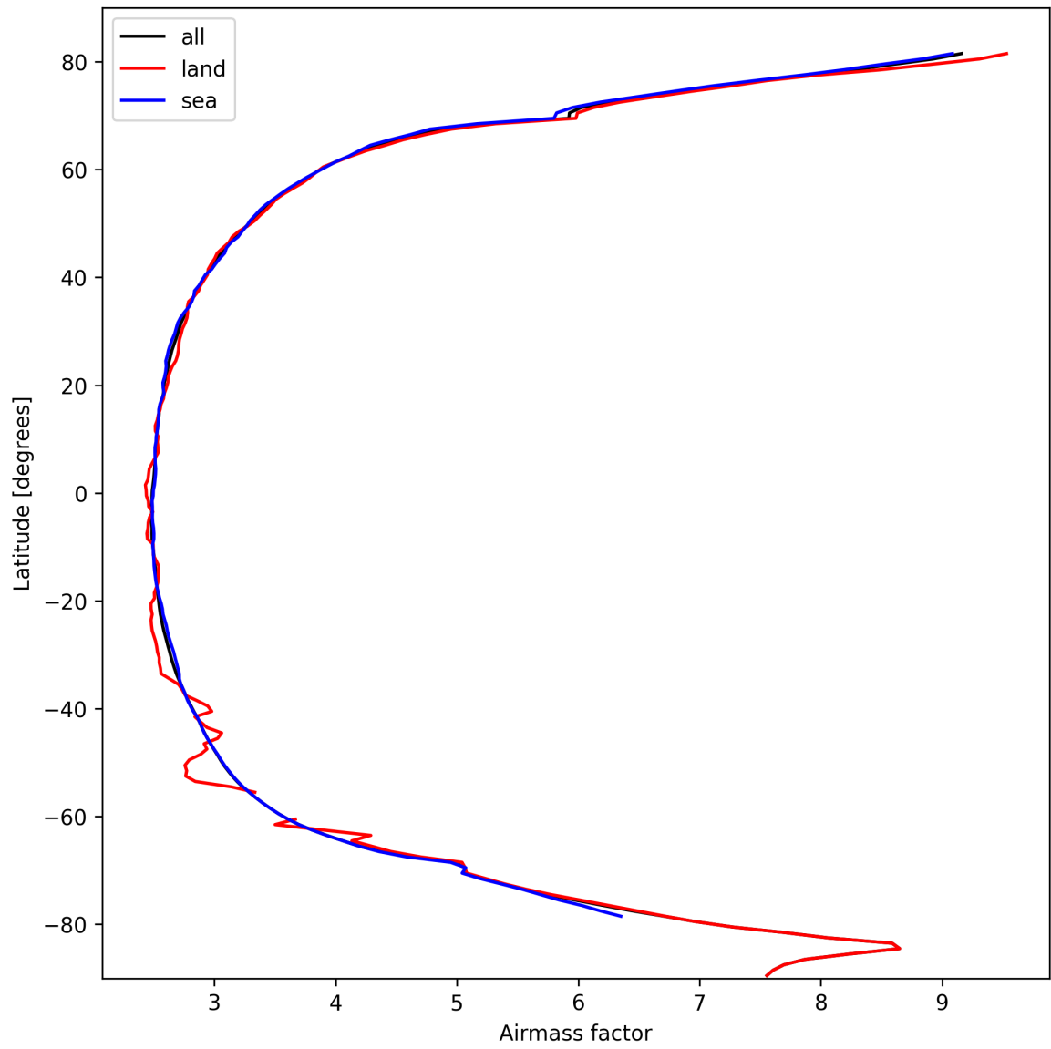
Figure 25: Zonal average of “Airmass factor” for 2025-10-11 to 2025-10-12.
