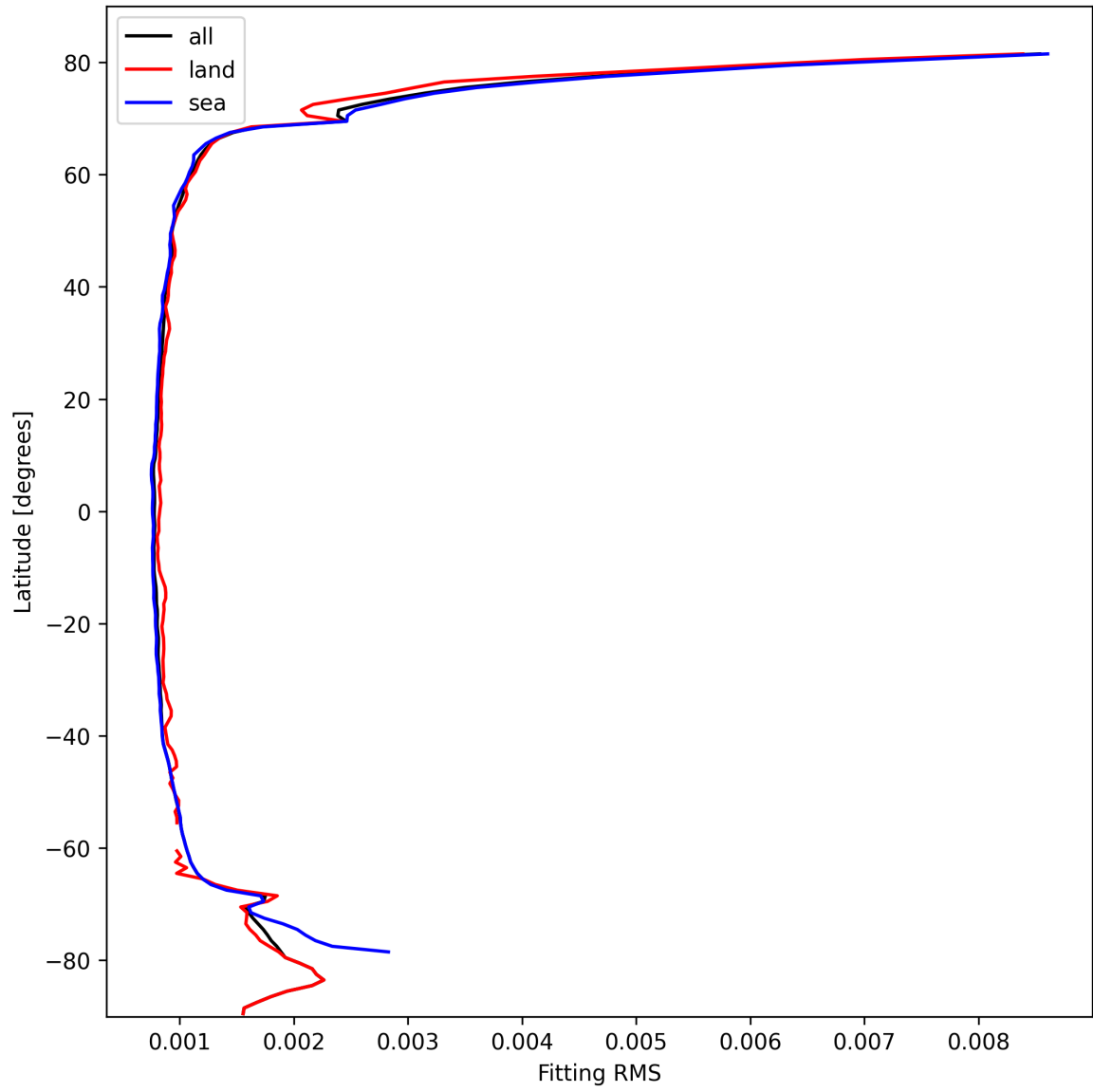
Figure 22: Zonal average of “Fitting RMS” for 2025-10-11 to 2025-10-12.
