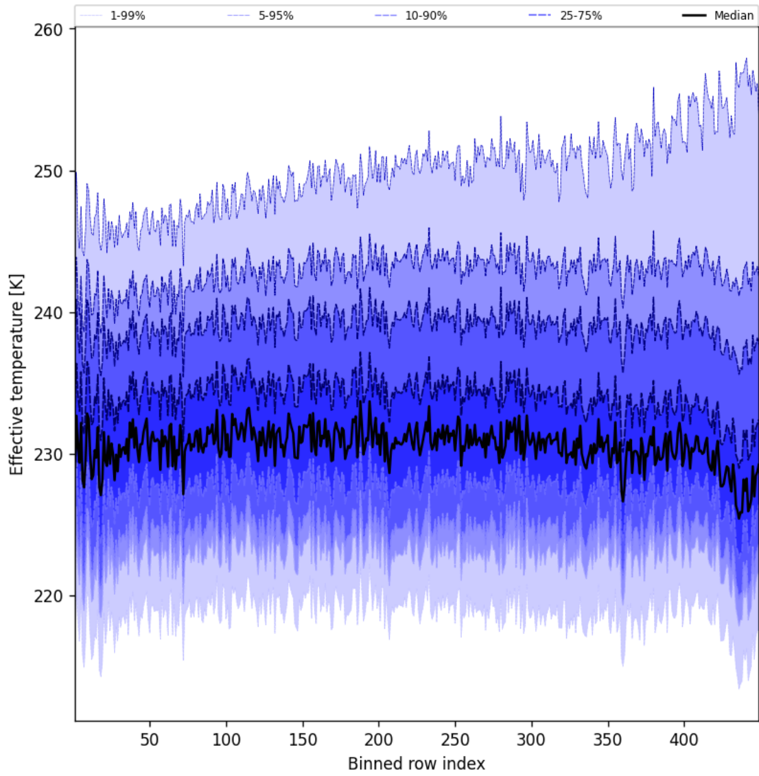
Figure 50: Along track statistics of “Effective temperature” for 2025-10-11 to 2025-10-12
