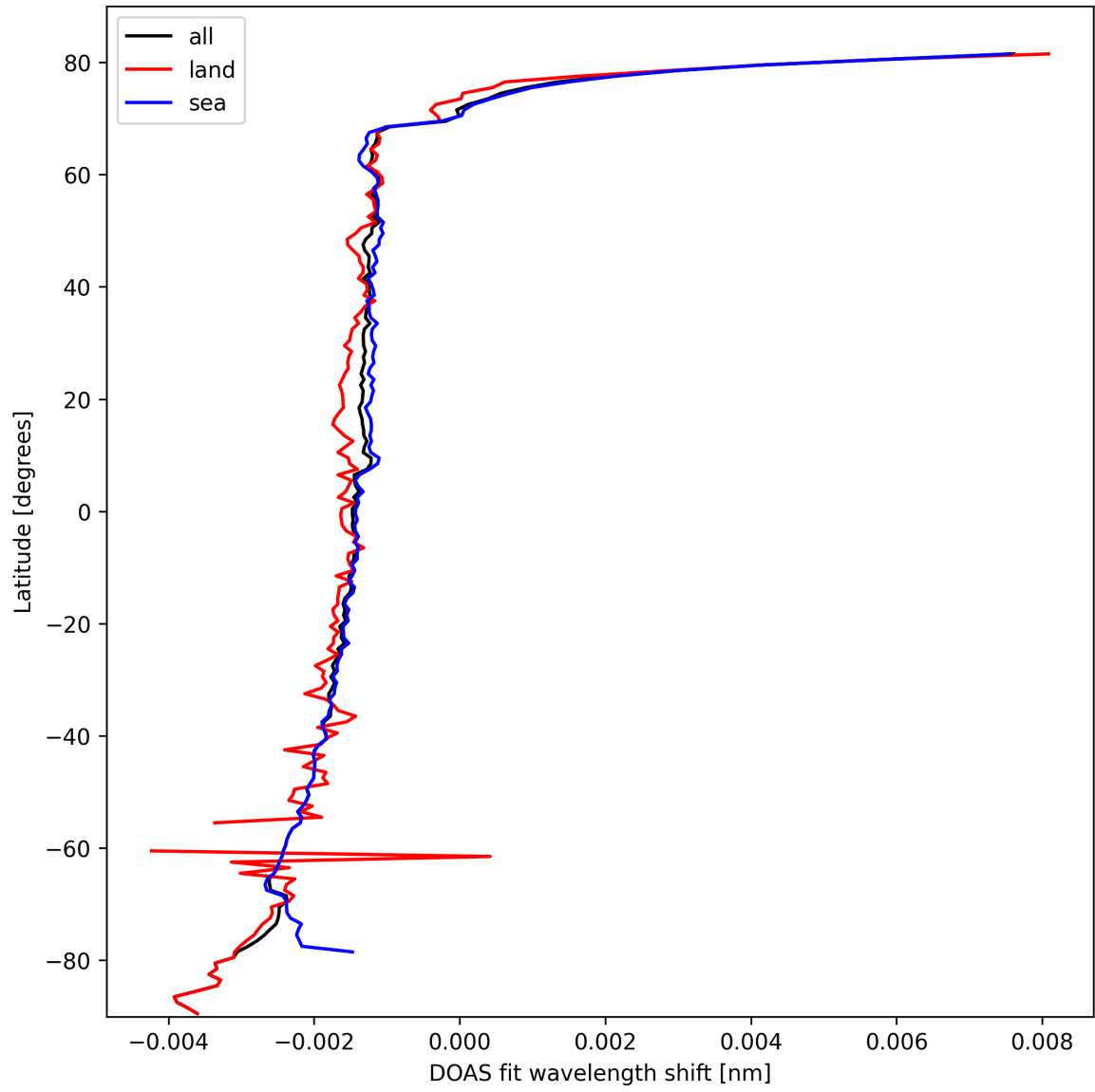
Figure 23: Zonal average of “DOAS fit wavelength shift” for 2025-10-11 to 2025-10-12.
