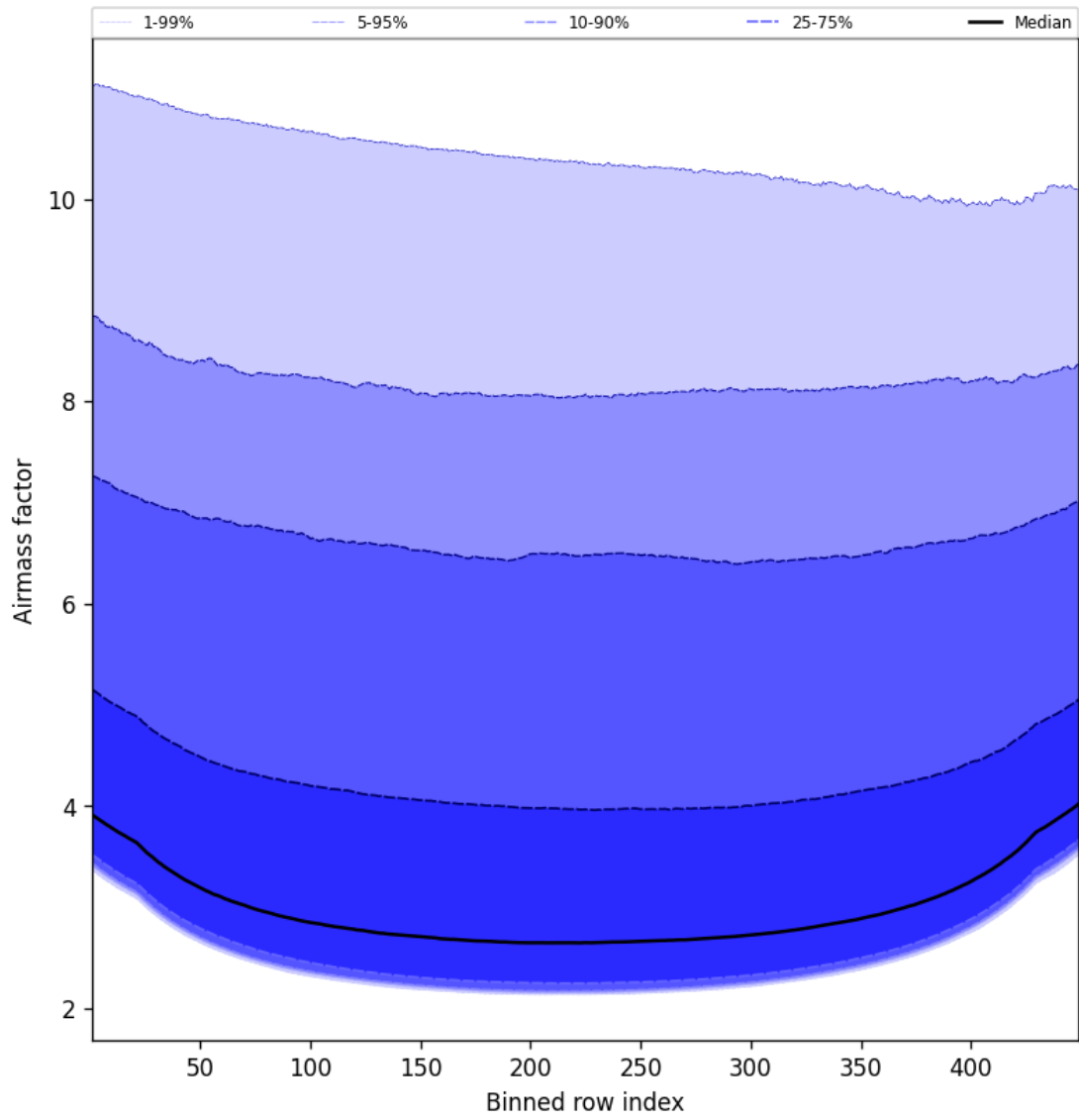
Figure 49: Along track statistics of “Airmass factor” for 2025-10-11 to 2025-10-12
