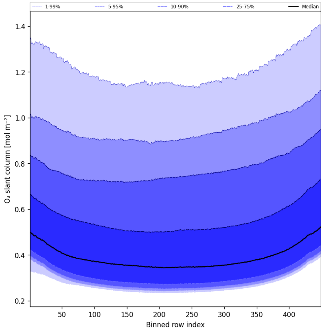
Figure 43: Along track statistics of “O 3 slant column” for 2025-10-11 to 2025-10-12
