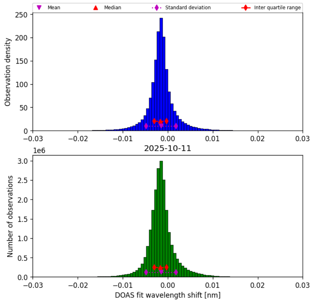
Figure 35: Histogram of “DOAS fit wavelength shift” for 2025-10-11 to 2025-10-12
