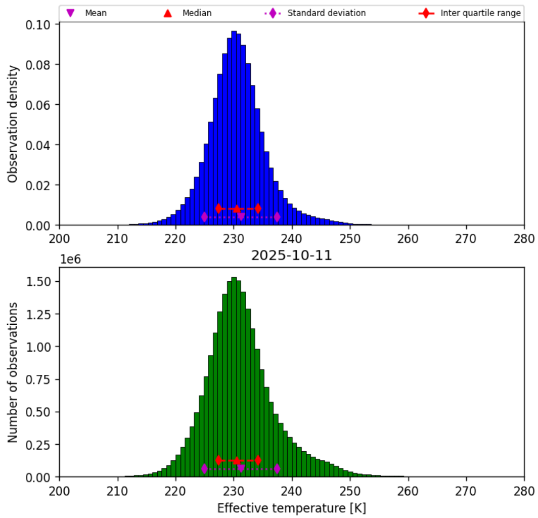
Figure 38: Histogram of “Effective temperature” for 2025-10-11 to 2025-10-12
