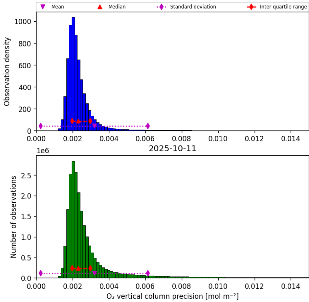
Figure 30: Histogram of “O 3 vertical column precision” for 2025-10-11 to 2025-10-12
