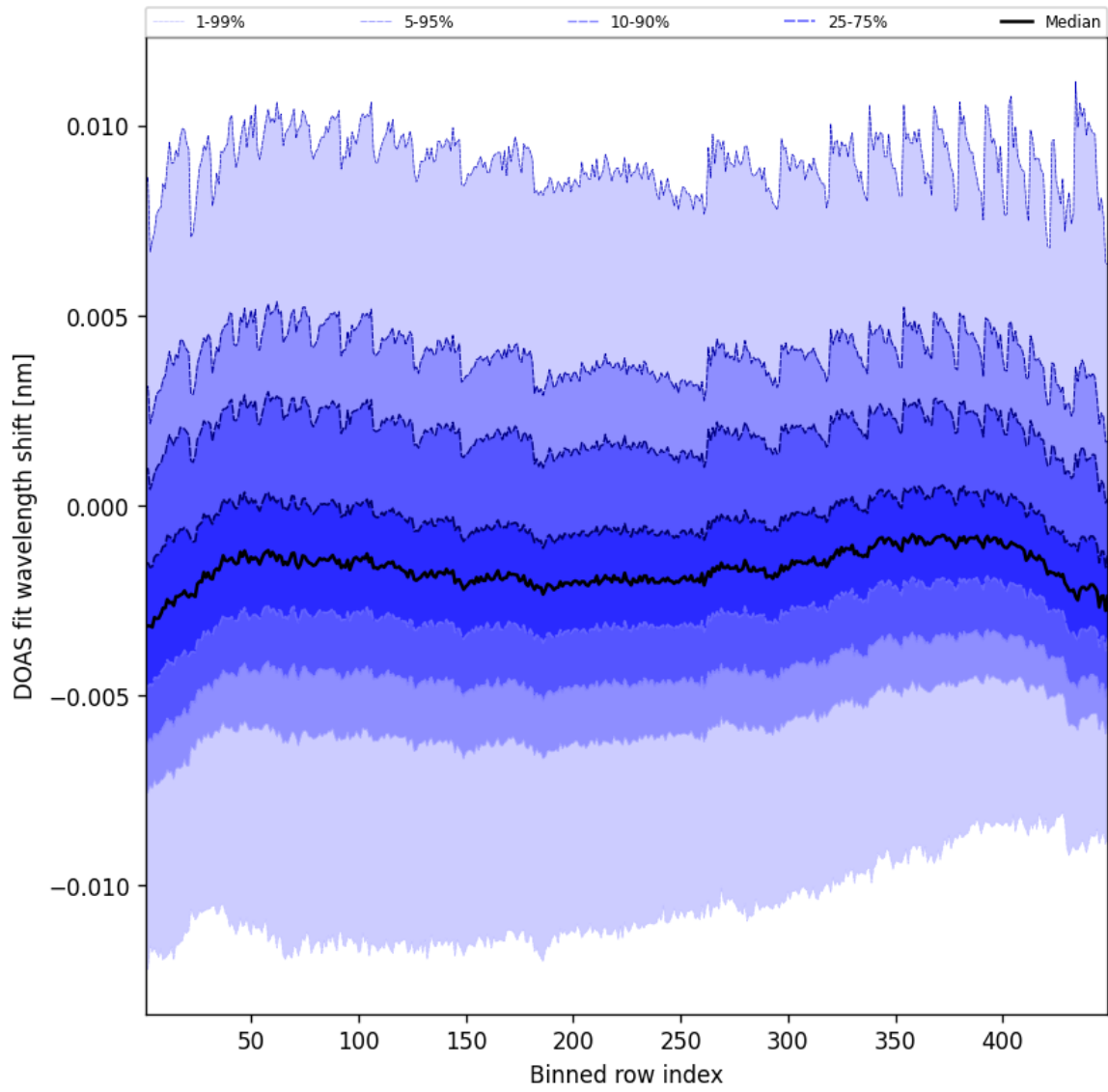
Figure 47: Along track statistics of "DOAS fit wavelength shift" for 2025-10-11 to 2025-10-12
