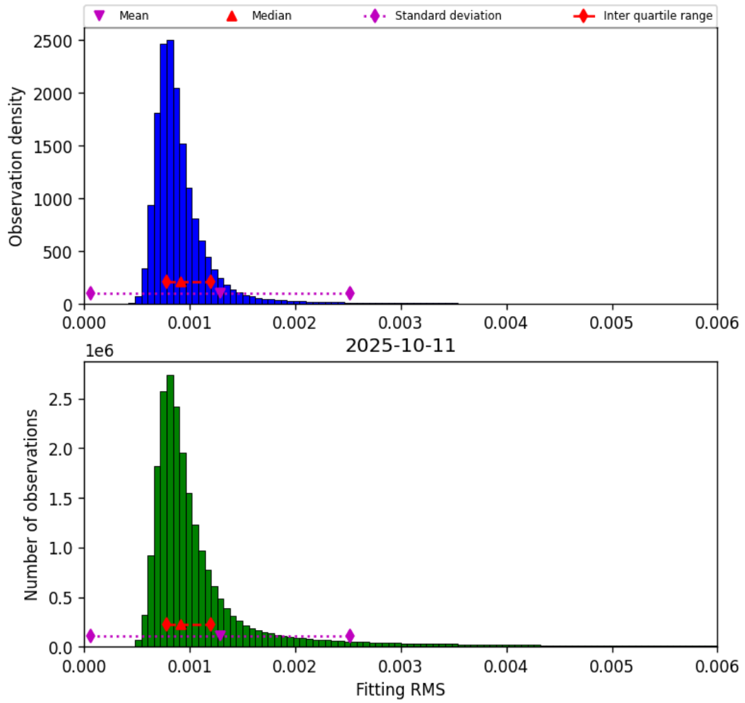
Figure 34: Histogram of “Fitting RMS” for 2025-10-11 to 2025-10-12
