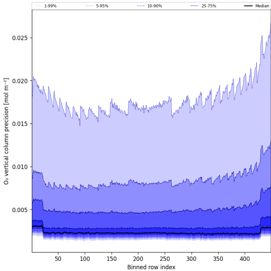
Figure 42: Along track statistics of “O 3 vertical column precision” for 2025-10-11 to 2025-10-12
