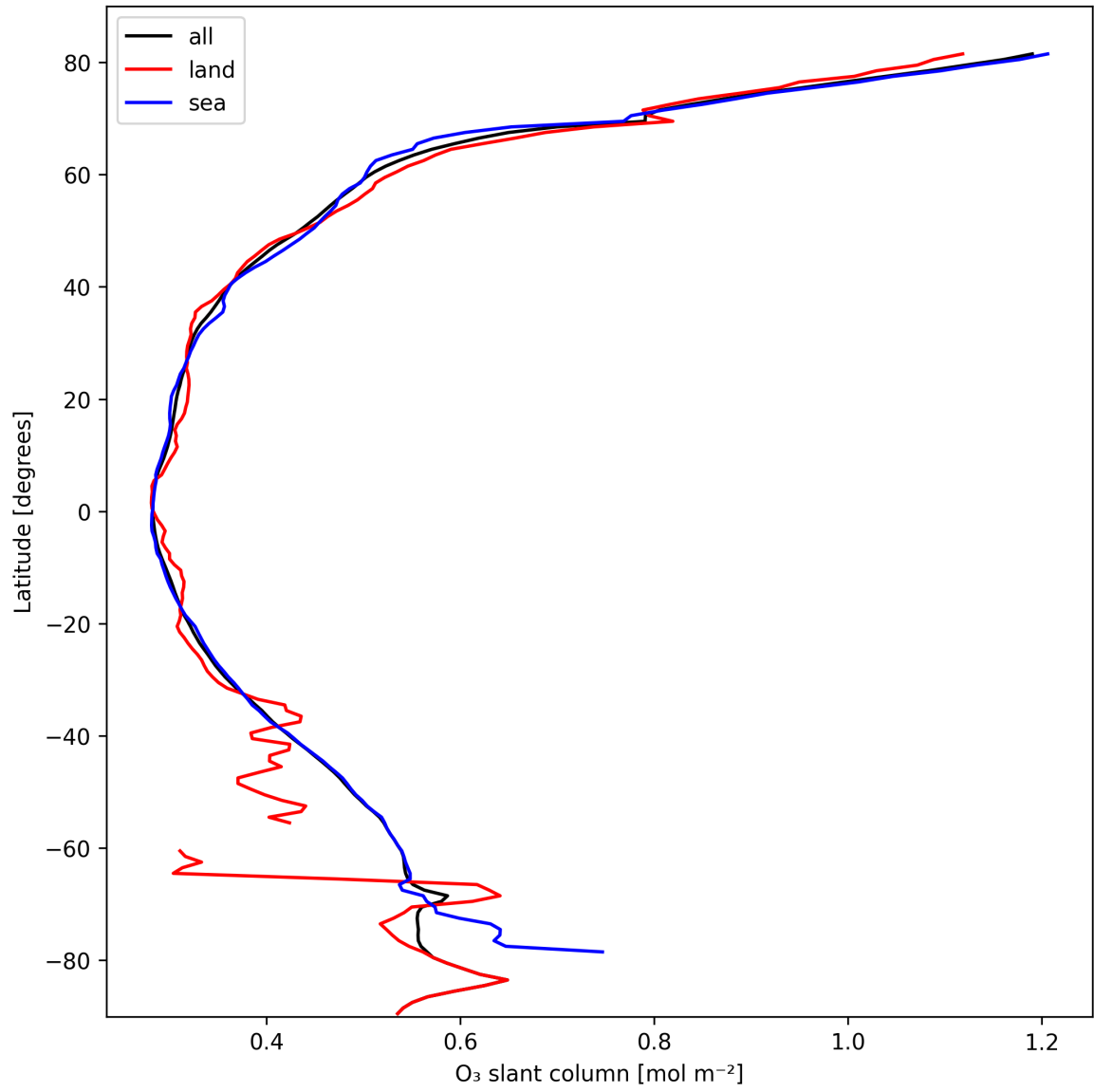
Figure 19: Zonal average of “O 3 slant column” for 2025-10-12 to 2025-10-13.
