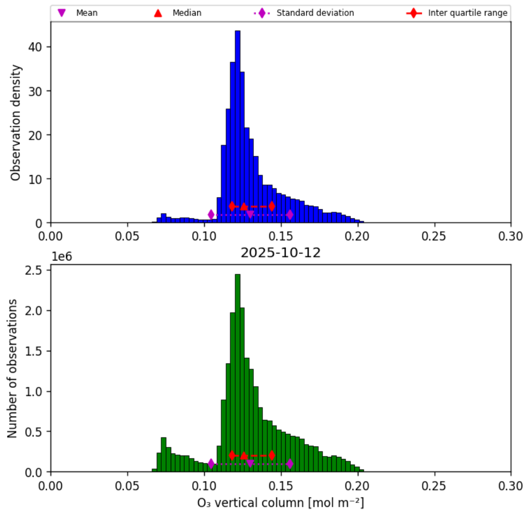
Figure 29: Histogram of “O 3 vertical column” for 2025-10-12 to 2025-10-13
