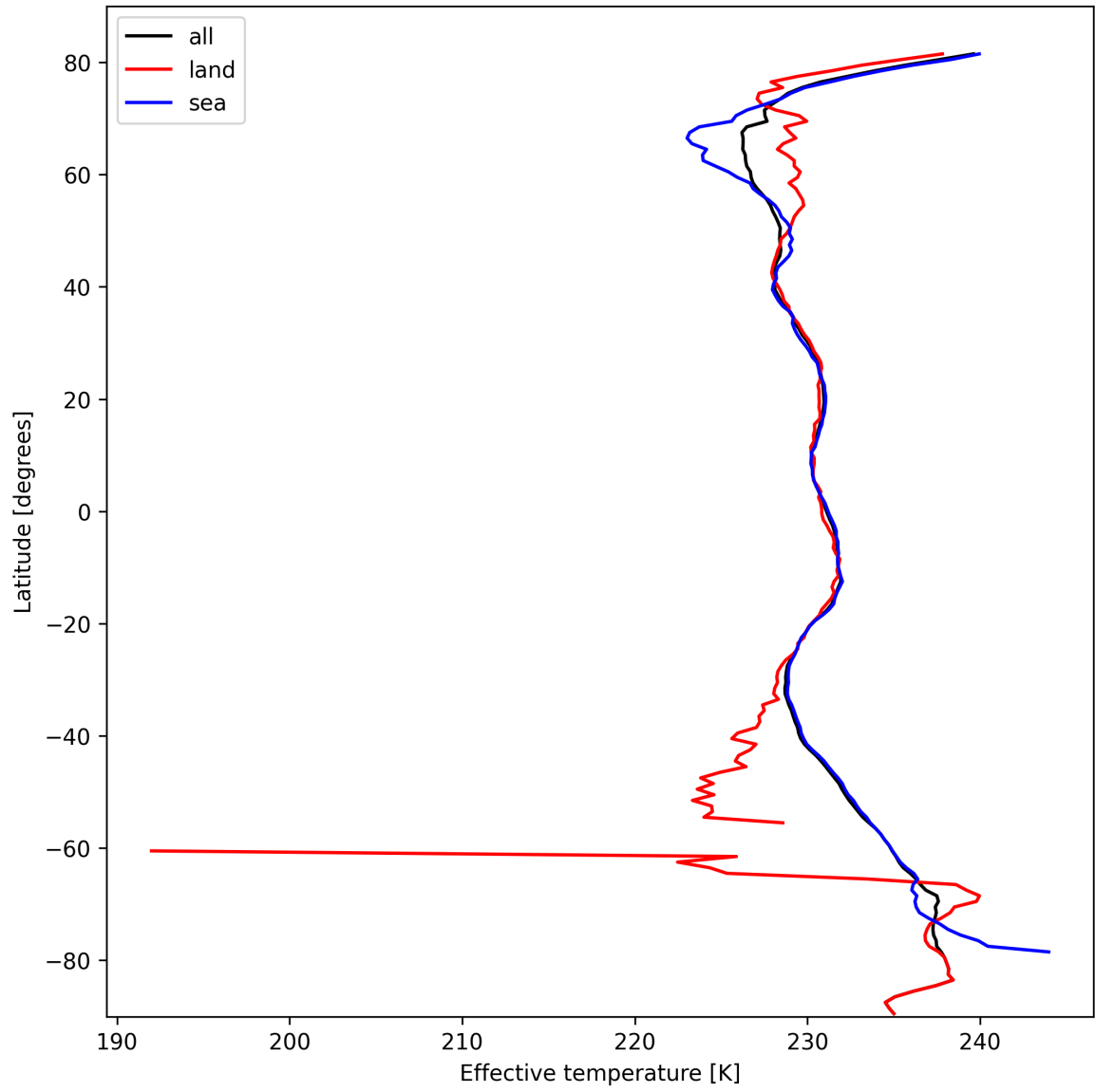
Figure 26: Zonal average of "Effective temperature" for 2025-10-12 to 2025-10-13.
