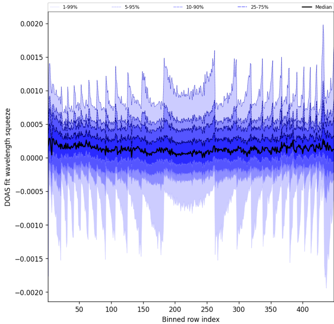
Figure 48: Along track statistics of “DOAS fit wavelength squeeze” for 2025-10-12 to 2025-10-13
