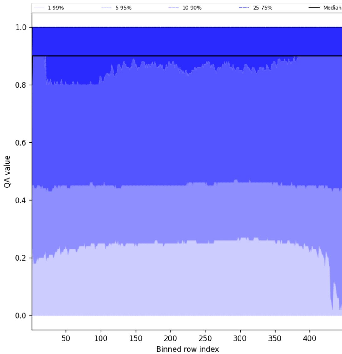
Figure 40: Along track statistics of “QA value” for 2025-10-12 to 2025-10-13
