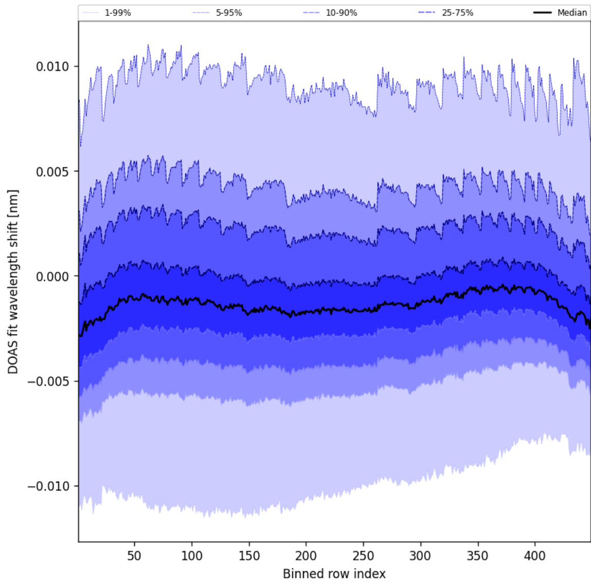
Figure 47: Along track statistics of “DOAS fit wavelength shift” for 2025-10-12 to 2025-10-13
