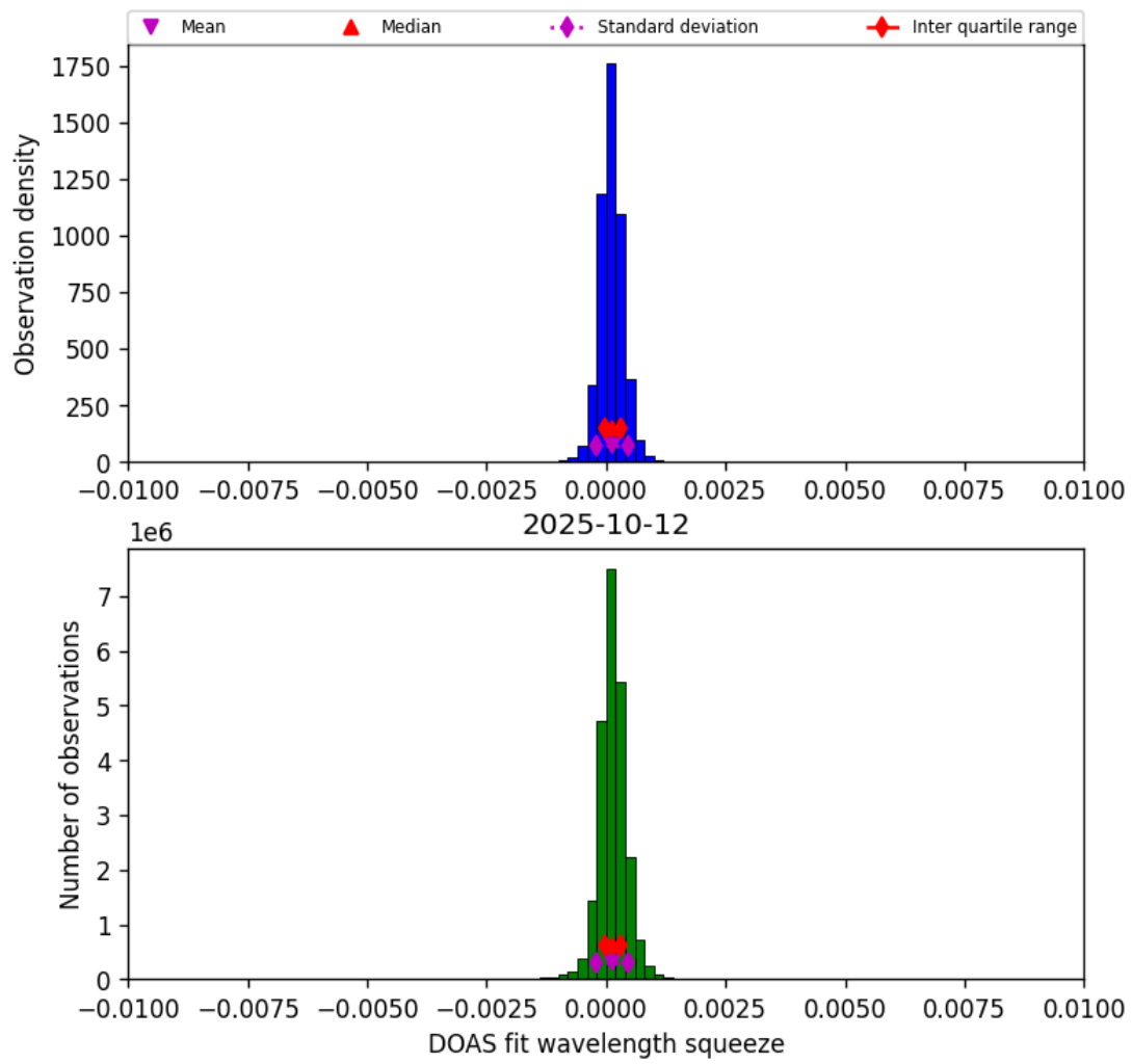
Figure 36: Histogram of “DOAS fit wavelength squeeze” for 2025-10-12 to 2025-10-13
