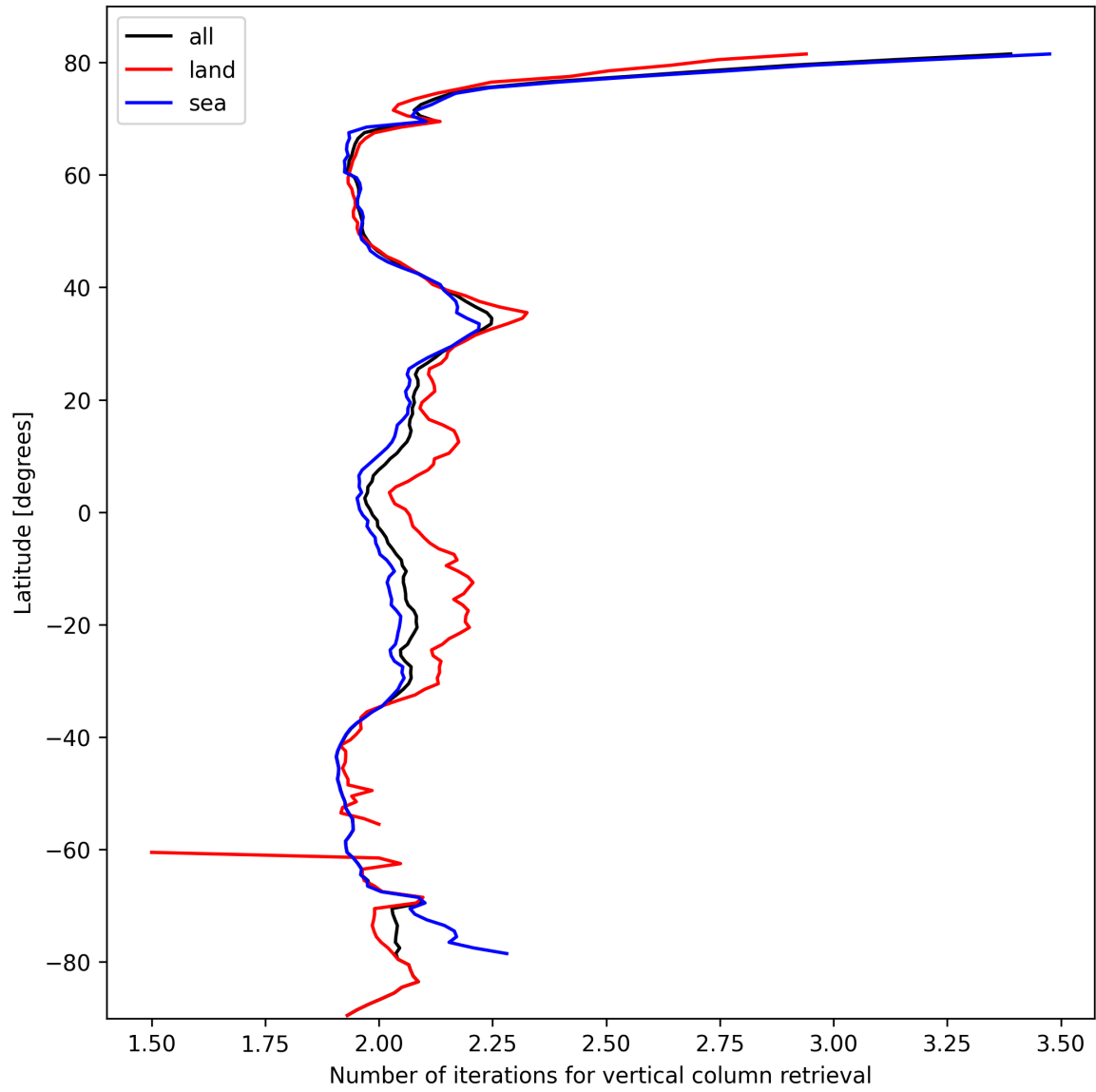
Figure 27: Zonal average of “Number of iterations for vertical column retrieval” for 2025-10-12 to 2025-10-13.
