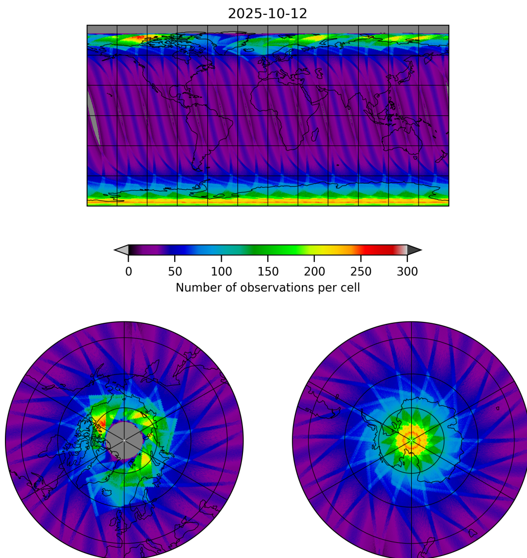
Figure 15: Map of the number of observations for 2025-10-12 to 2025-10-13
