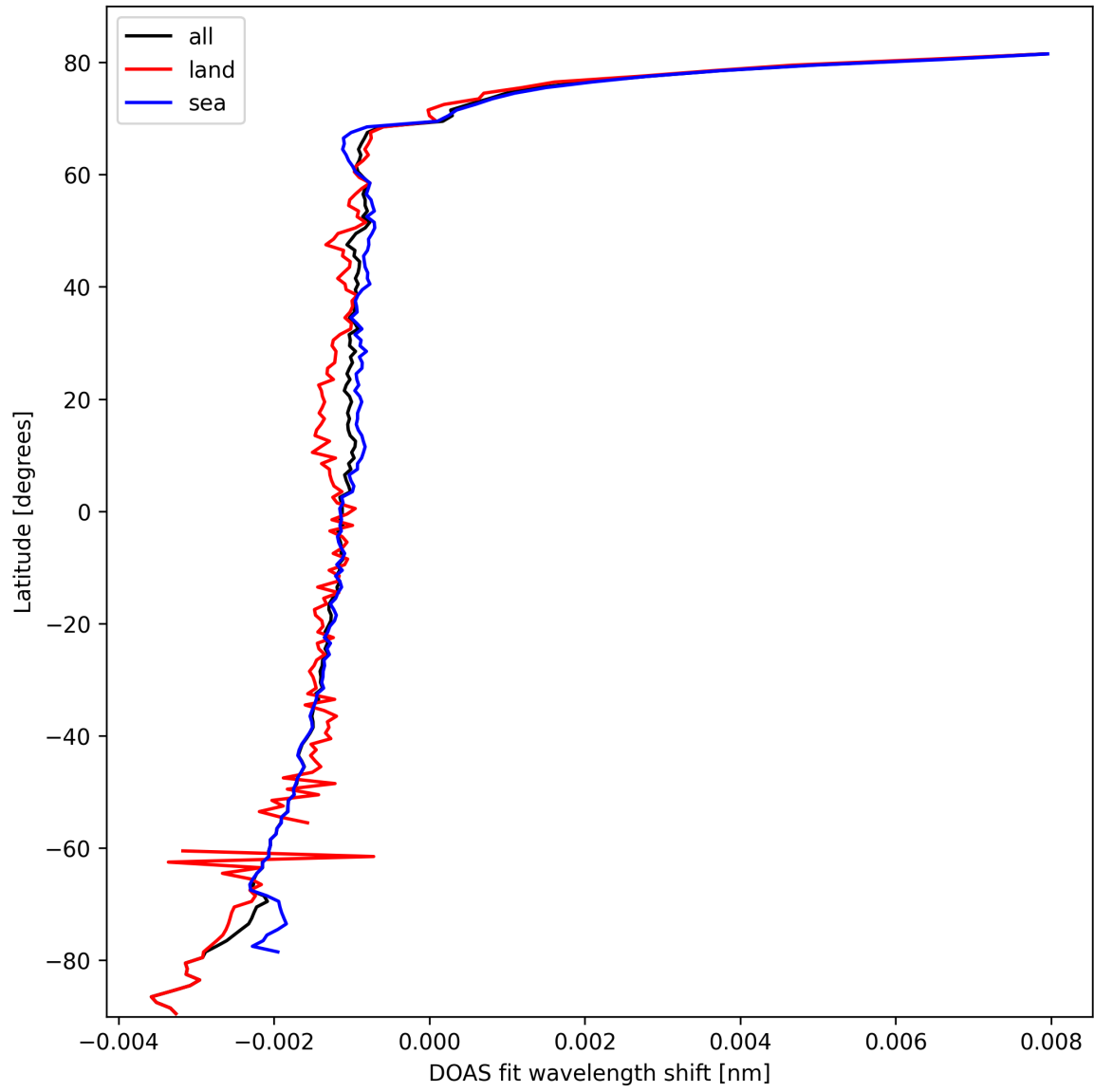
Figure 23: Zonal average of “DOAS fit wavelength shift” for 2025-10-12 to 2025-10-13.
