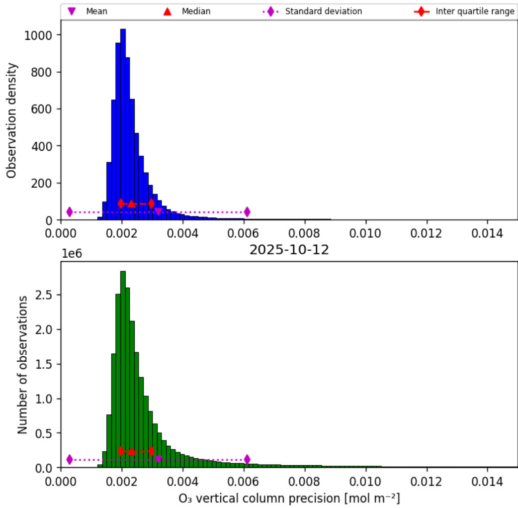
Figure 30: Histogram of “O 3 vertical column precision” for 2025-10-12 to 2025-10-13
