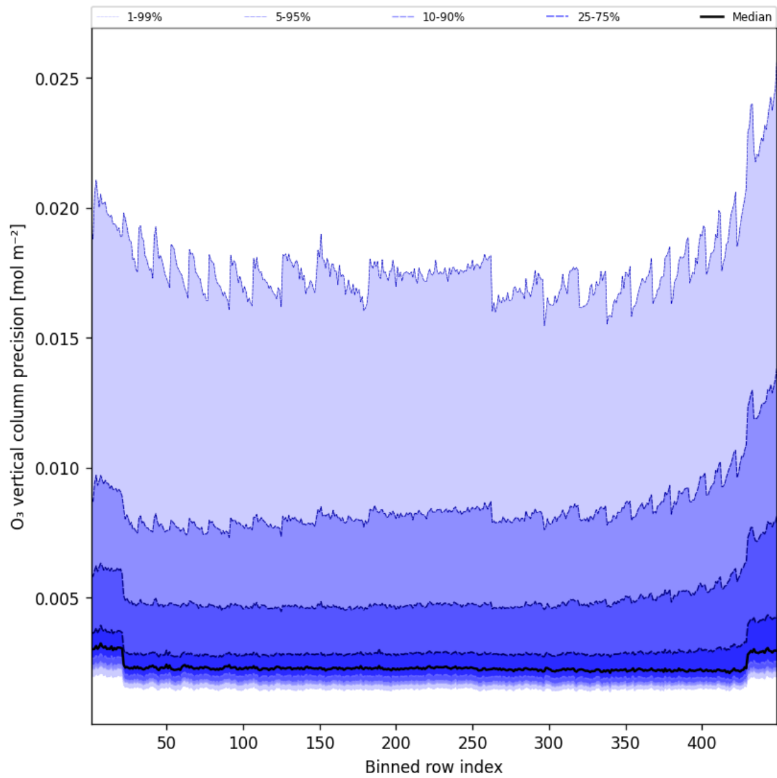
Figure 42: Along track statistics of “O 3 vertical column precision” for 2025-10-12 to 2025-10-13
