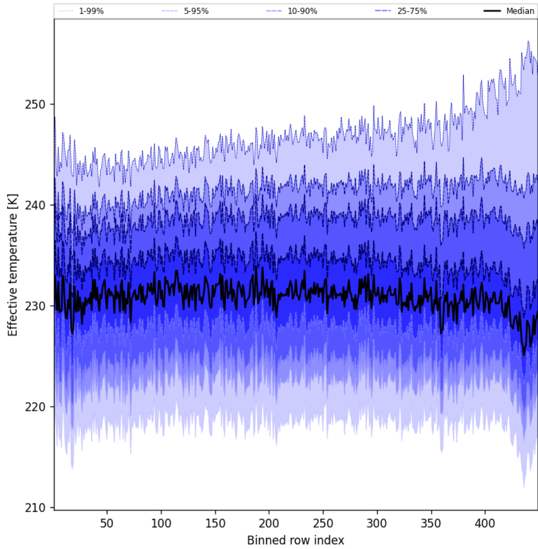
Figure 50: Along track statistics of “Effective temperature” for 2025-10-12 to 2025-10-13
