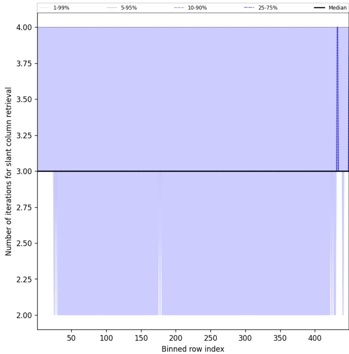
Figure 45: Along track statistics of “Number of iterations for slant column retrieval” for 2025-10-12 to 2025-10-13
