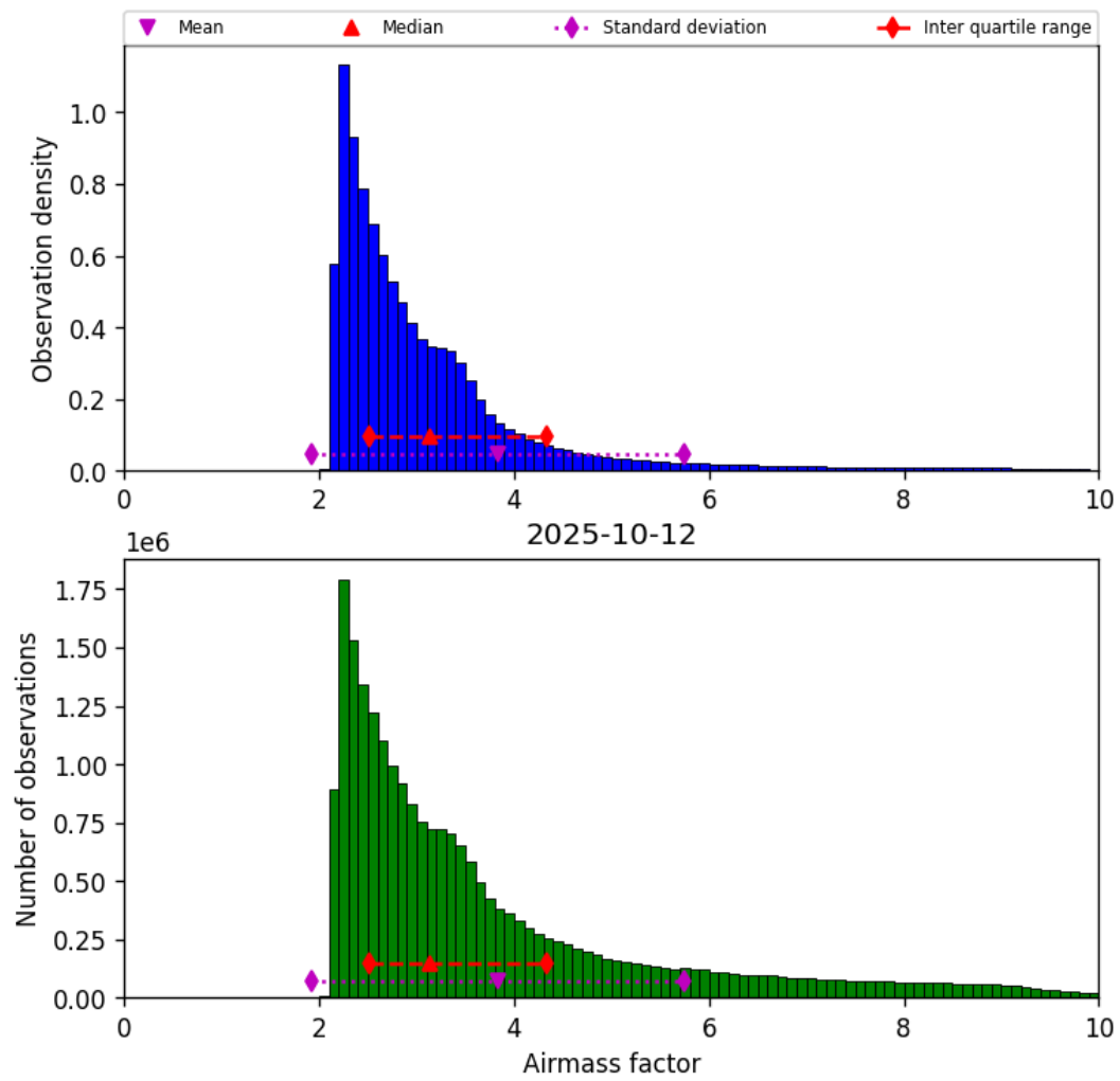
Figure 37: Histogram of “Airmass factor” for 2025-10-12 to 2025-10-13
