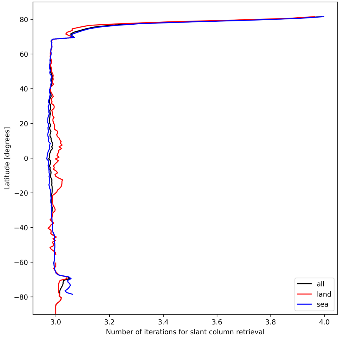
Figure 21: Zonal average of “Number of iterations for slant column retrieval” for 2025-10-12 to 2025-10-13.
