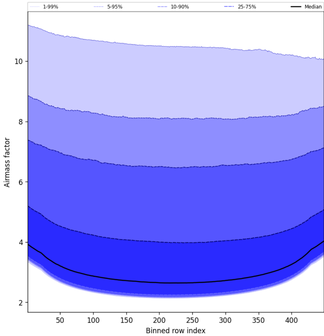
Figure 49: Along track statistics of “Airmass factor” for 2025-10-12 to 2025-10-13
