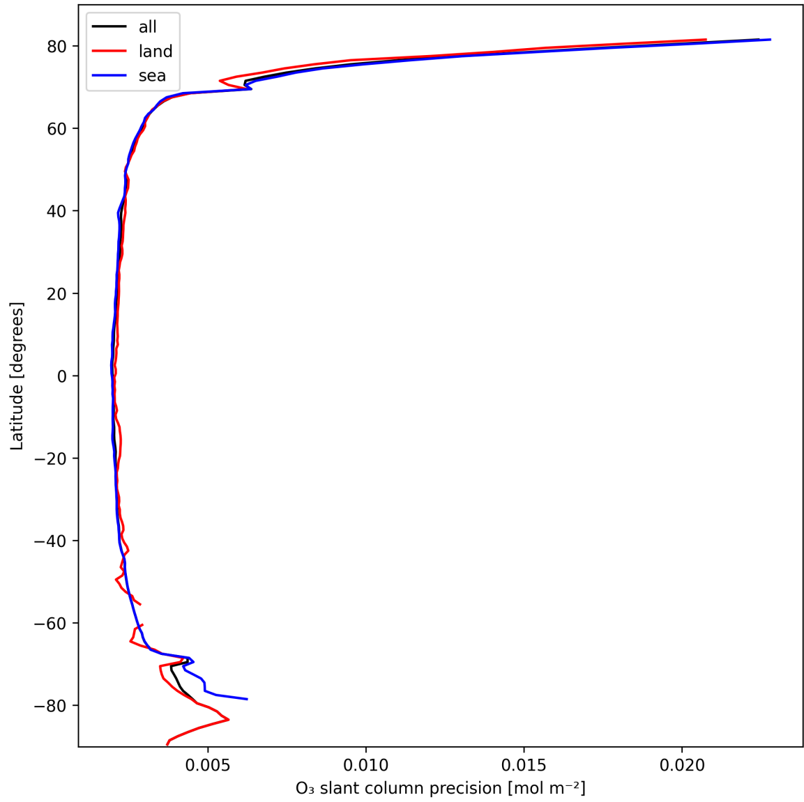
Figure 20: Zonal average of “O 3 slant column precision” for 2025-10-12 to 2025-10-13.
