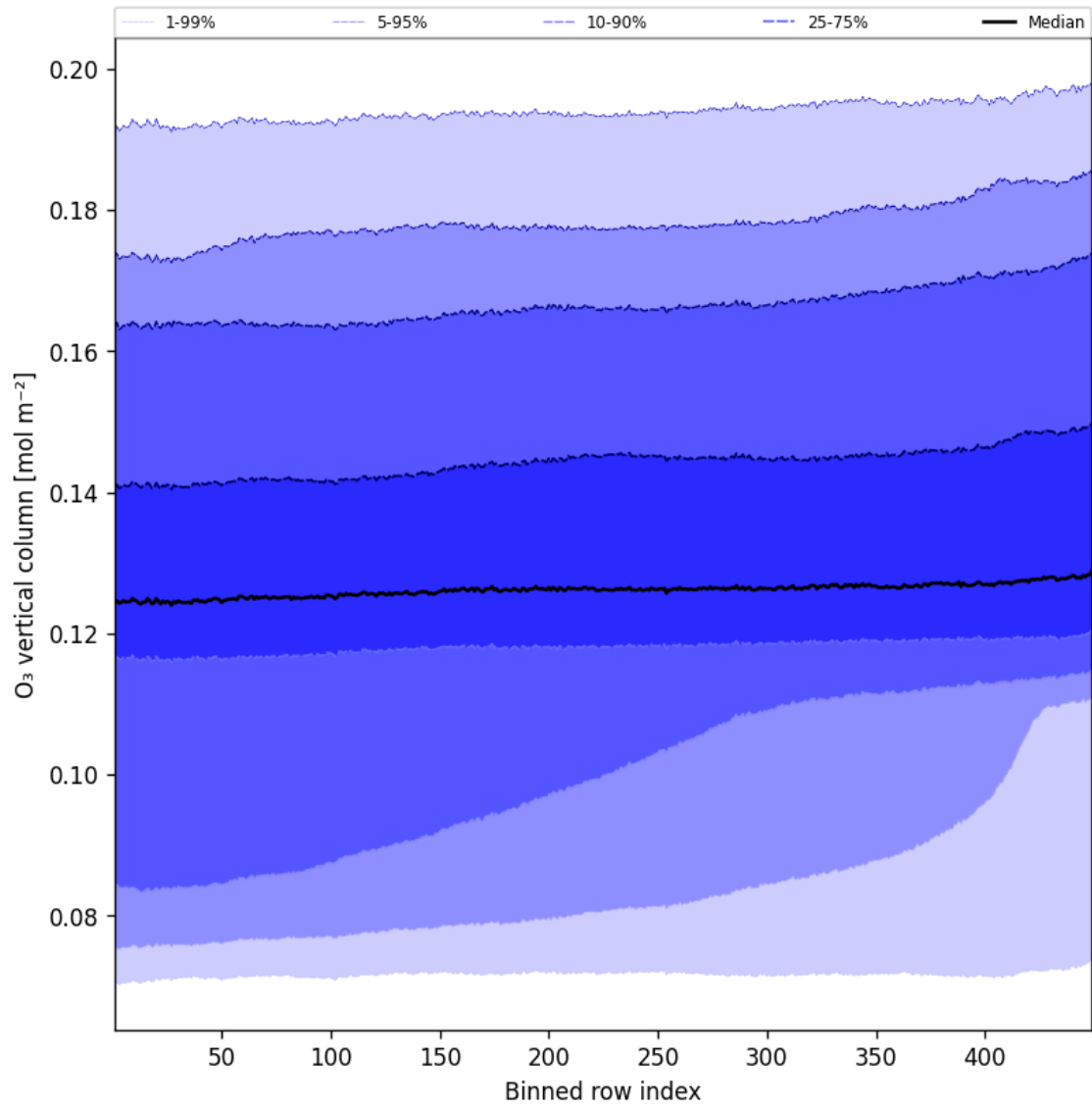
Figure 41: Along track statistics of “O 3 vertical column” for 2025-10-12 to 2025-10-13
