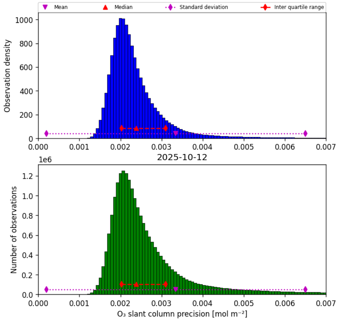
Figure 32: Histogram of “O 3 slant column precision” for 2025-10-12 to 2025-10-13
