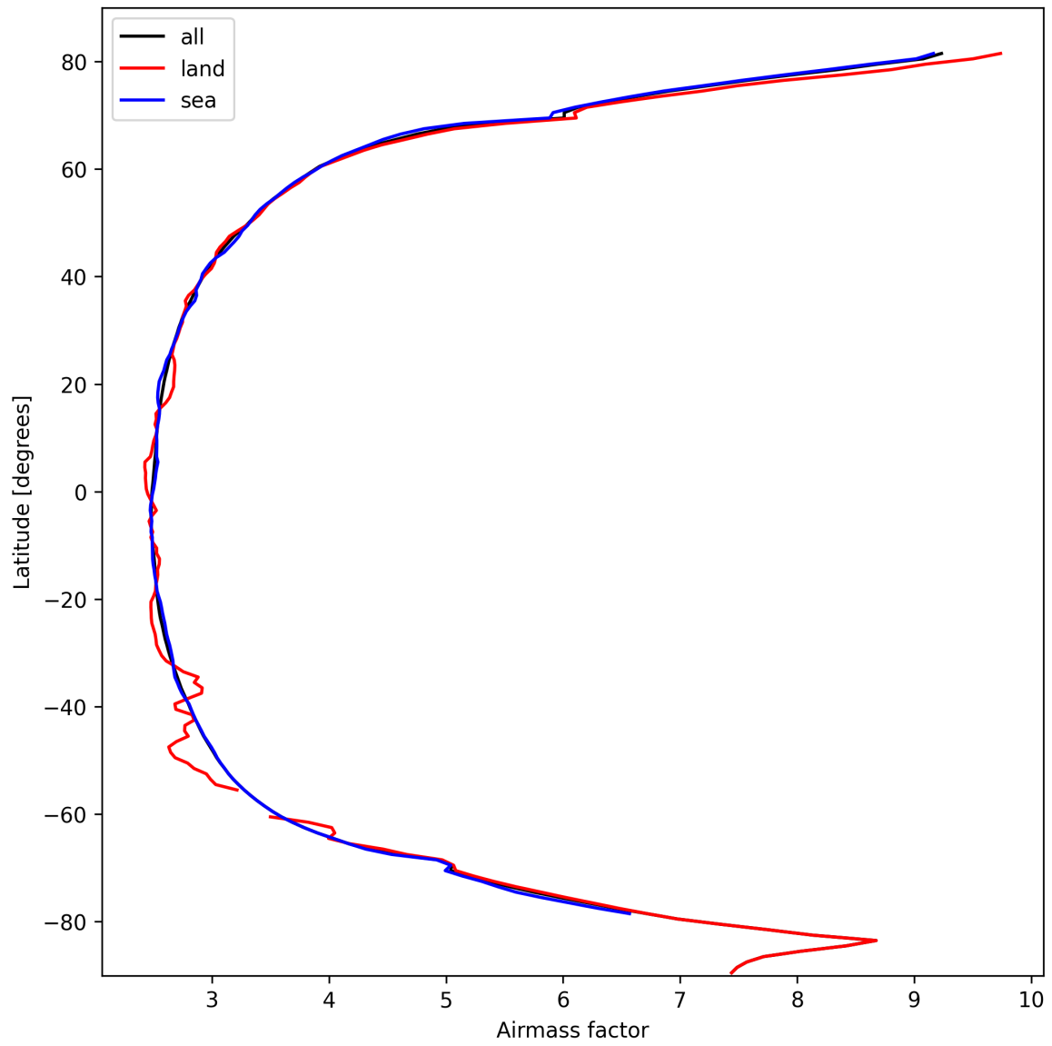
Figure 25: Zonal average of “Airmass factor” for 2025-10-12 to 2025-10-13.
