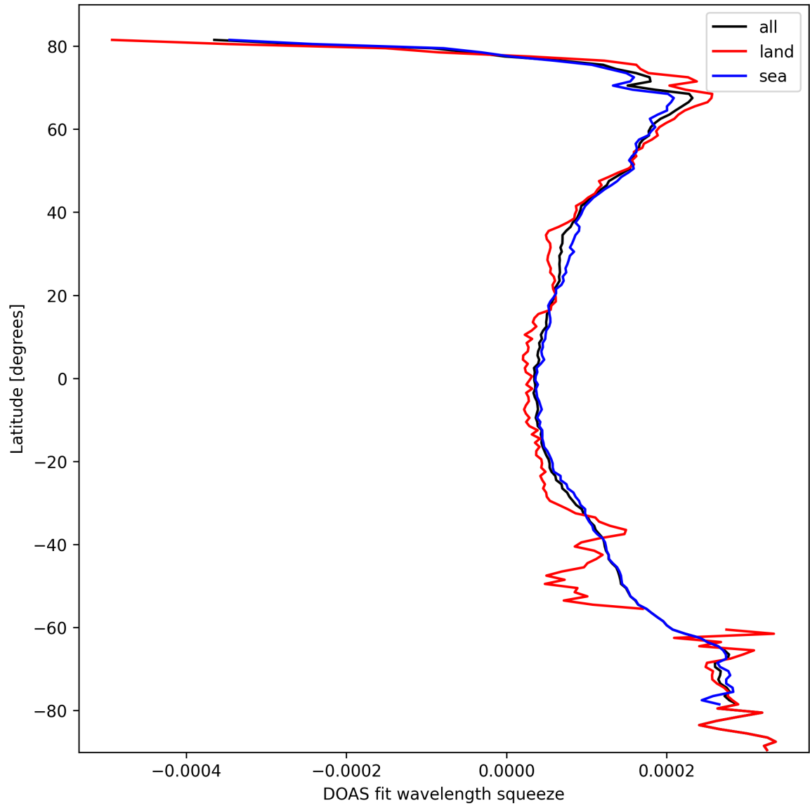
Figure 24: Zonal average of “DOAS fit wavelength squeeze” for 2025-10-12 to 2025-10-13.
