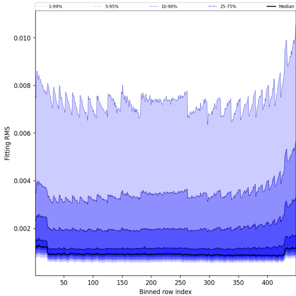
Figure 46: Along track statistics of “Fitting RMS” for 2025-10-12 to 2025-10-13
