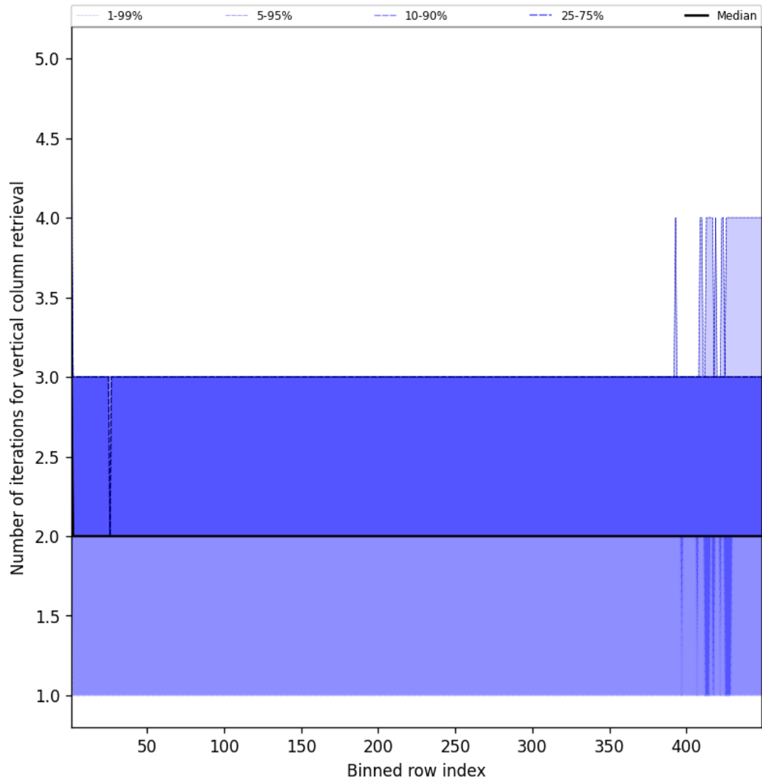
Figure 51: Along track statistics of “Number of iterations for vertical column retrieval” for 2025-10-12 to 2025-10-13
