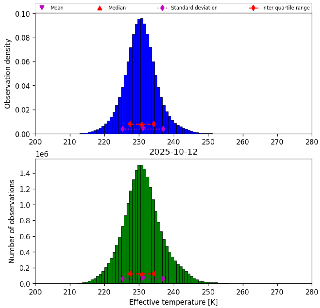
Figure 38: Histogram of “Effective temperature” for 2025-10-12 to 2025-10-13
