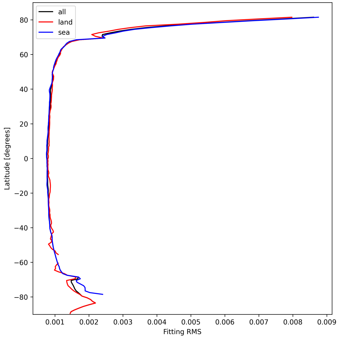
Figure 22: Zonal average of “Fitting RMS” for 2025-10-12 to 2025-10-13.
