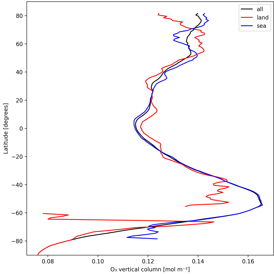
Figure 17: Zonal average of “O 3 vertical column” for 2025-10-12 to 2025-10-13.
