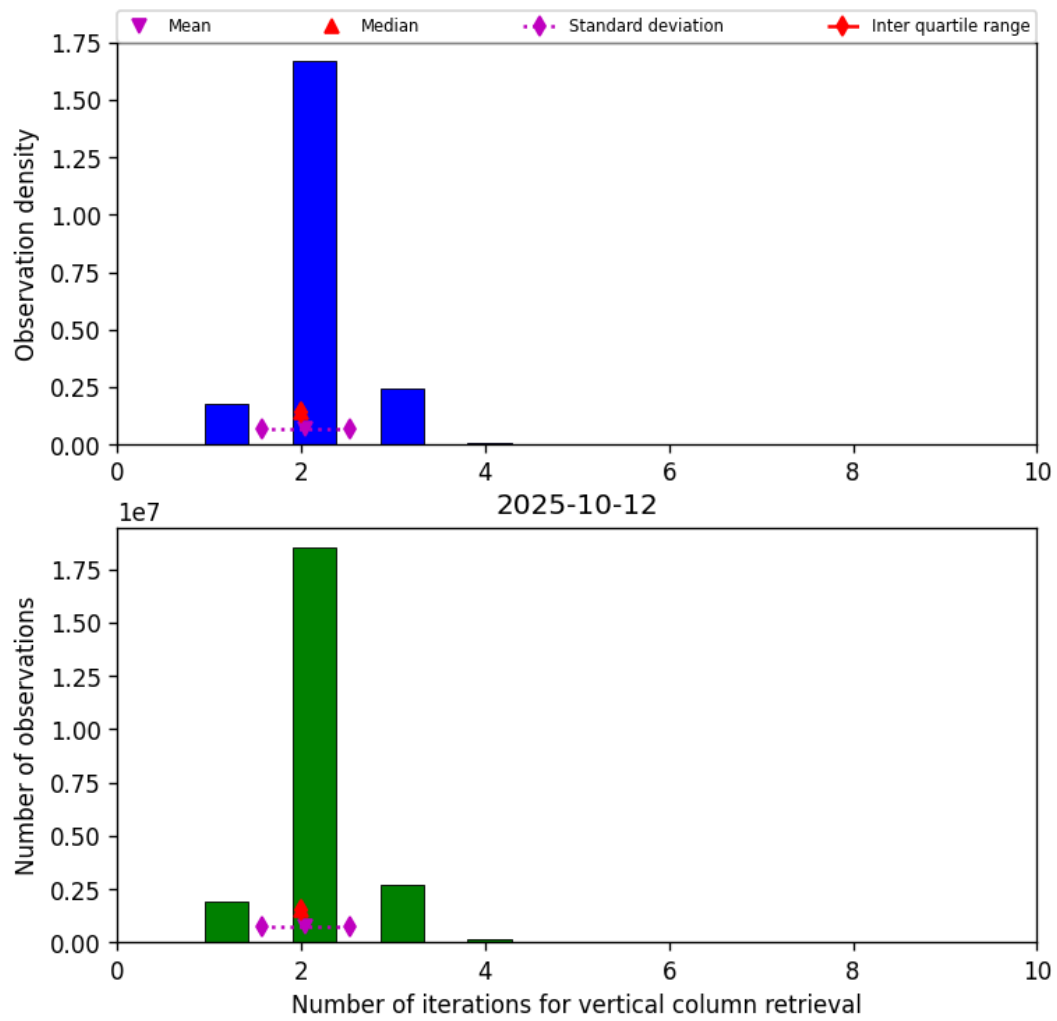
Figure 39: Histogram of “Number of iterations for vertical column retrieval” for 2025-10-12 to 2025-10-13
