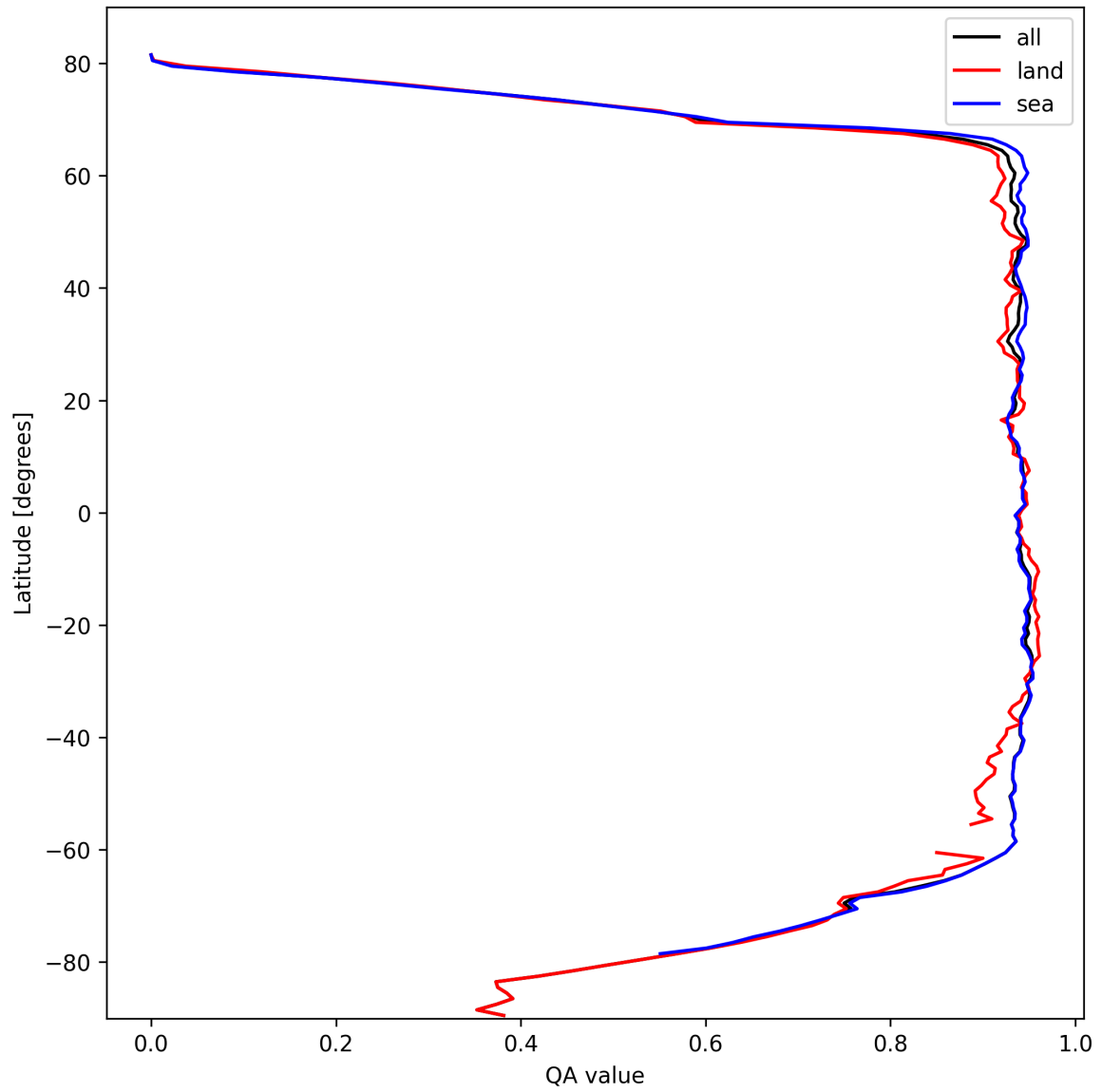
Figure 16: Zonal average of “QA value” for 2025-10-12 to 2025-10-13.
