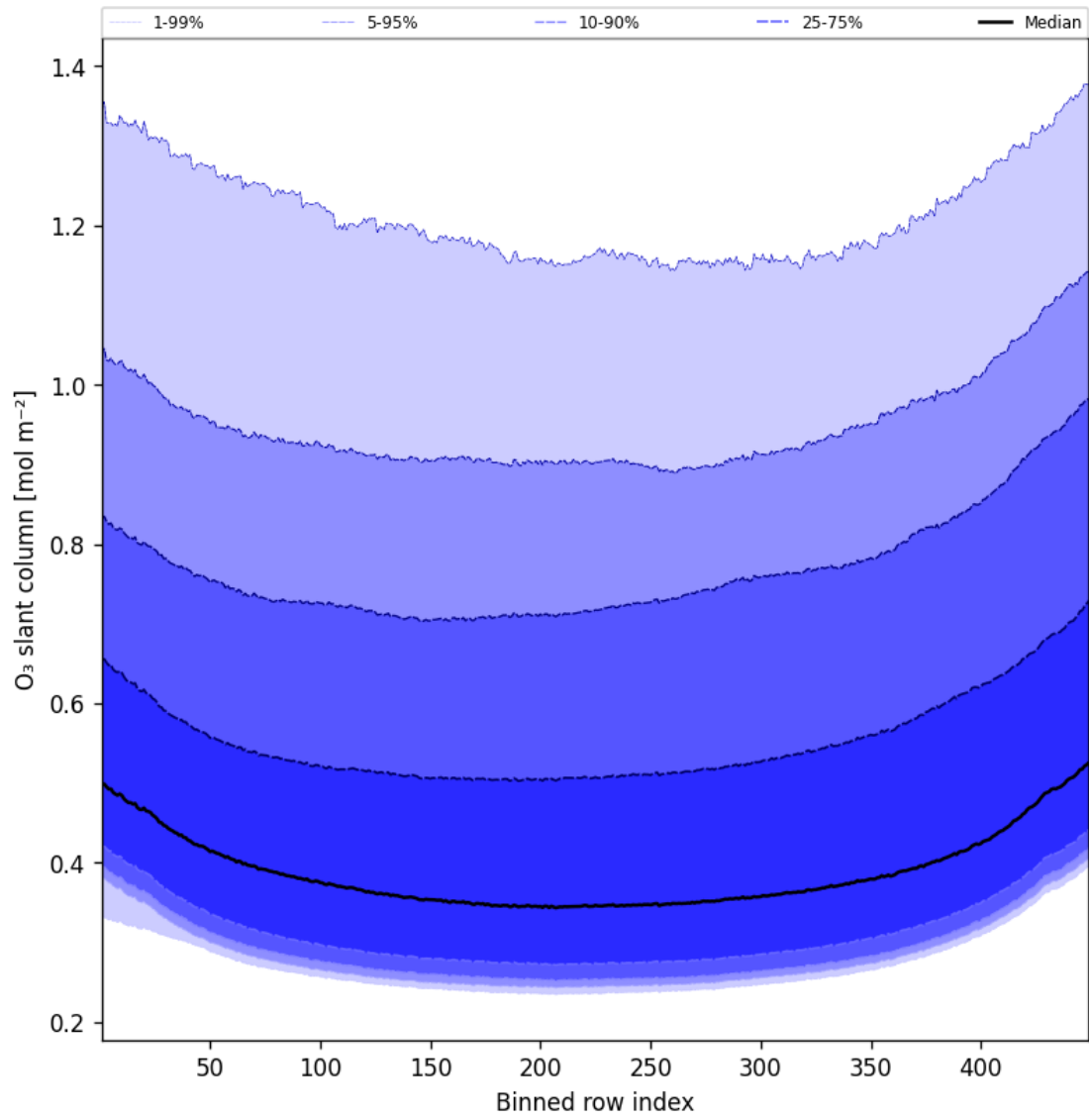
Figure 43: Along track statistics of “O 3 slant column” for 2025-10-12 to 2025-10-13
