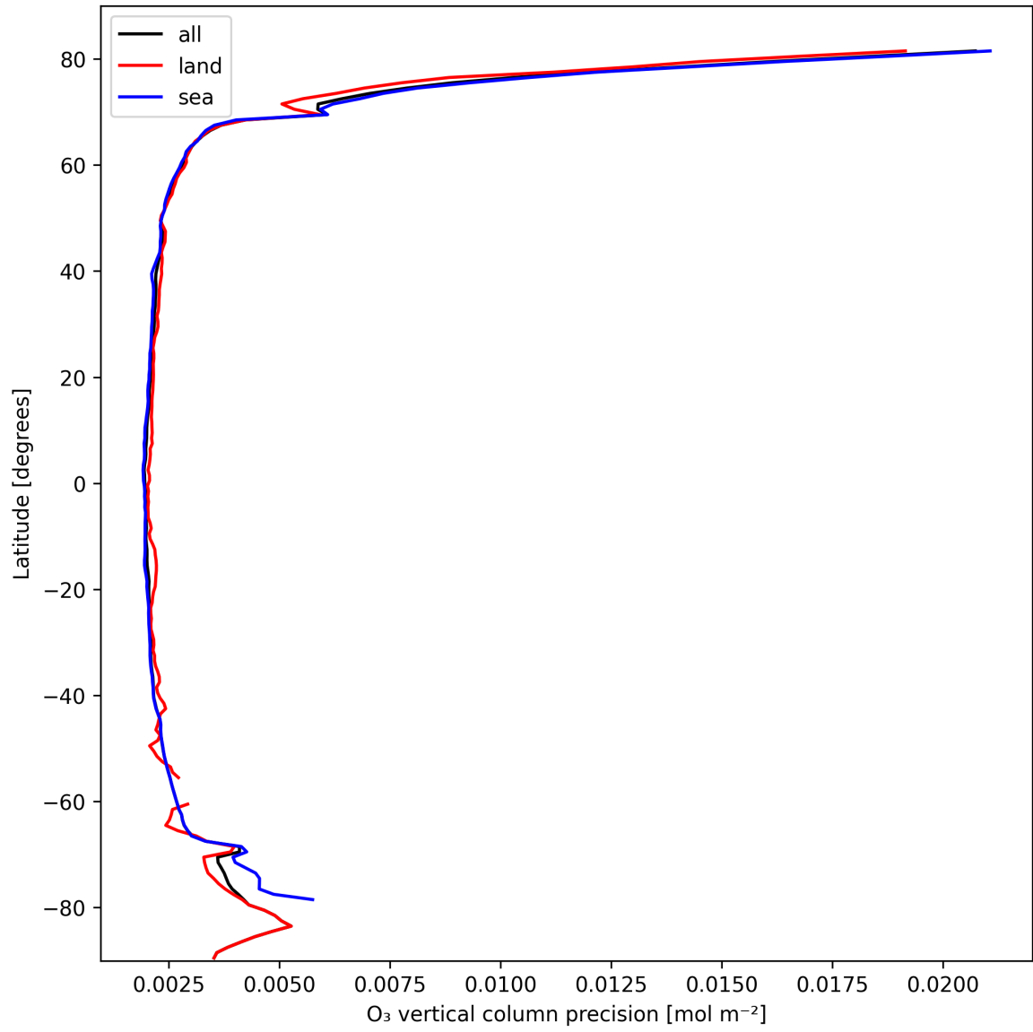
Figure 18: Zonal average of “O 3 vertical column precision” for 2025-10-12 to 2025-10-13.
