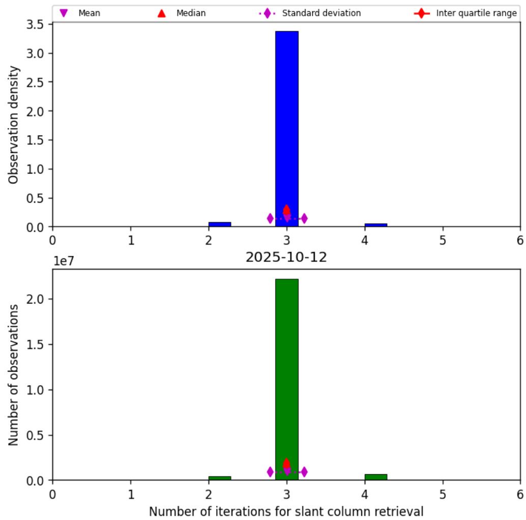
Figure 33: Histogram of “Number of iterations for slant column retrieval” for 2025-10-12 to 2025-10-13
