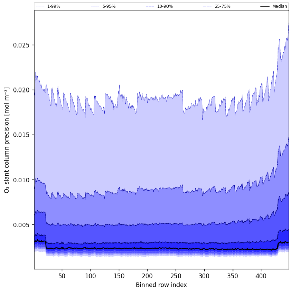
Figure 44: Along track statistics of “O 3 slant column precision” for 2025-10-12 to 2025-10-13
