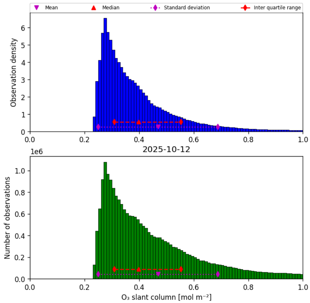
Figure 31: Histogram of “O 3 slant column” for 2025-10-12 to 2025-10-13
