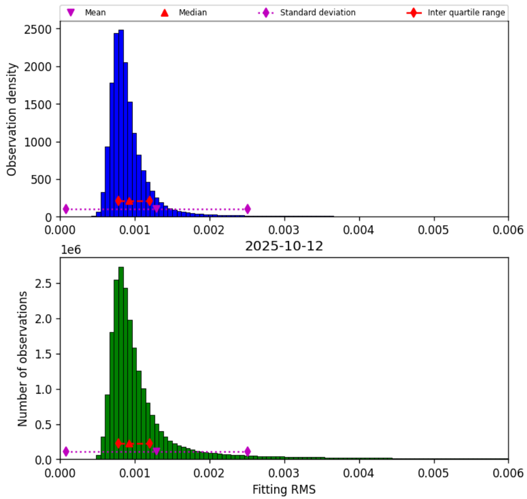
Figure 34: Histogram of “Fitting RMS” for 2025-10-12 to 2025-10-13
