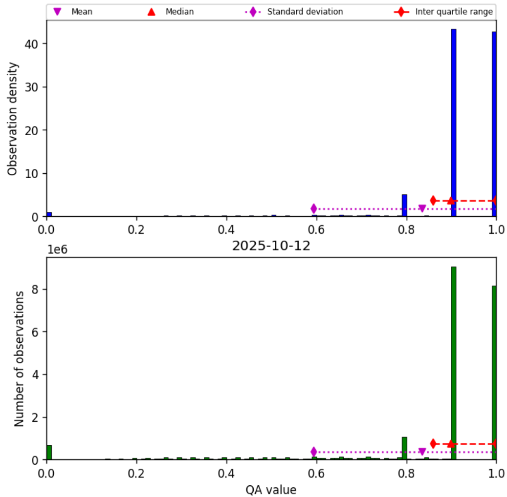
Figure 28: Histogram of “QA value” for 2025-10-12 to 2025-10-13
