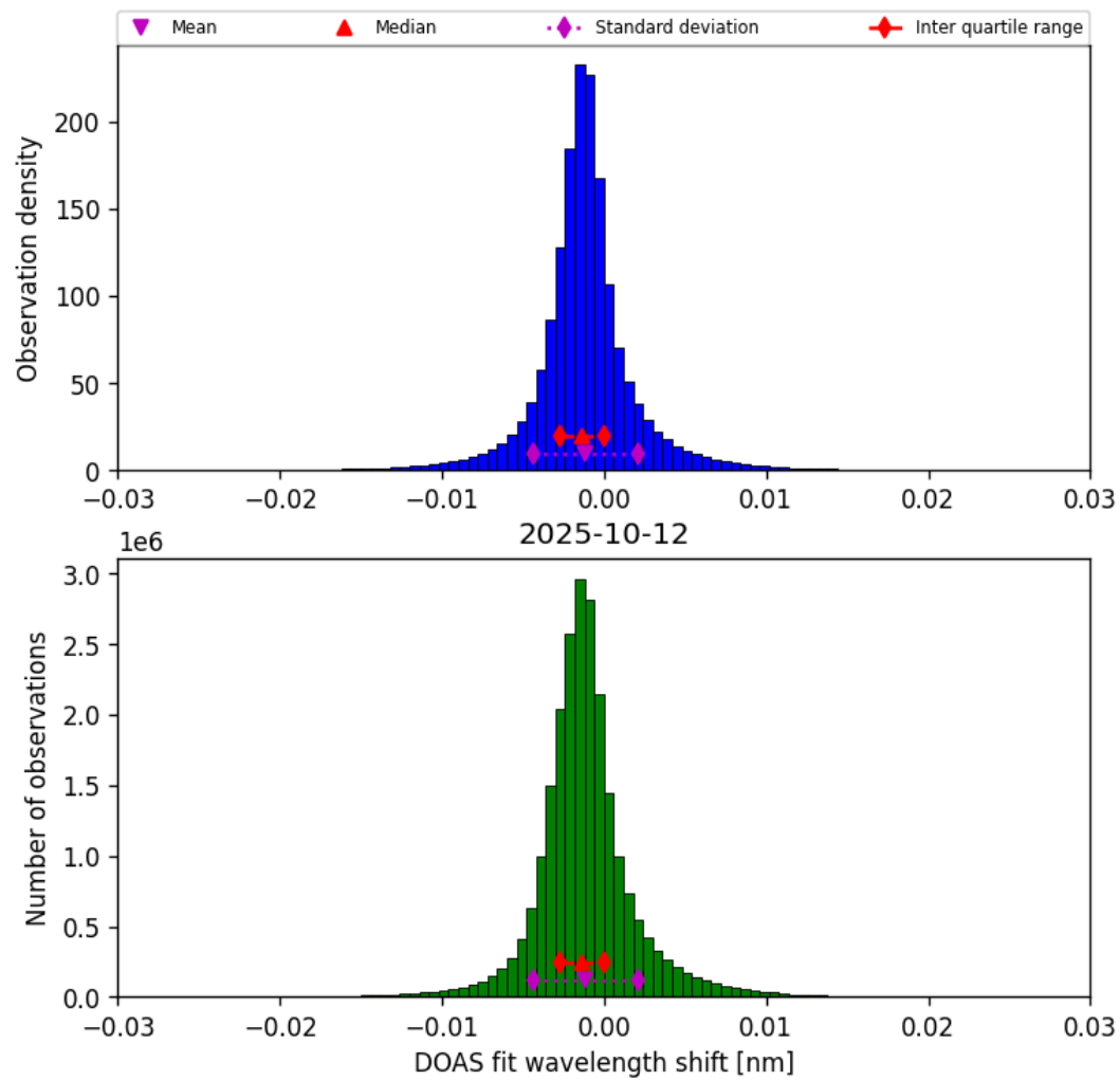
Figure 35: Histogram of “DOAS fit wavelength shift” for 2025-10-12 to 2025-10-13
