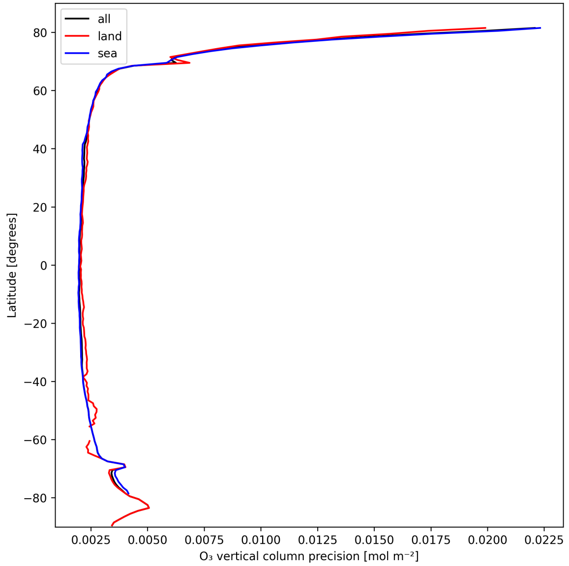
Figure 18: Zonal average of “O 3 vertical column precision” for 2025-10-13 to 2025-10-14.
