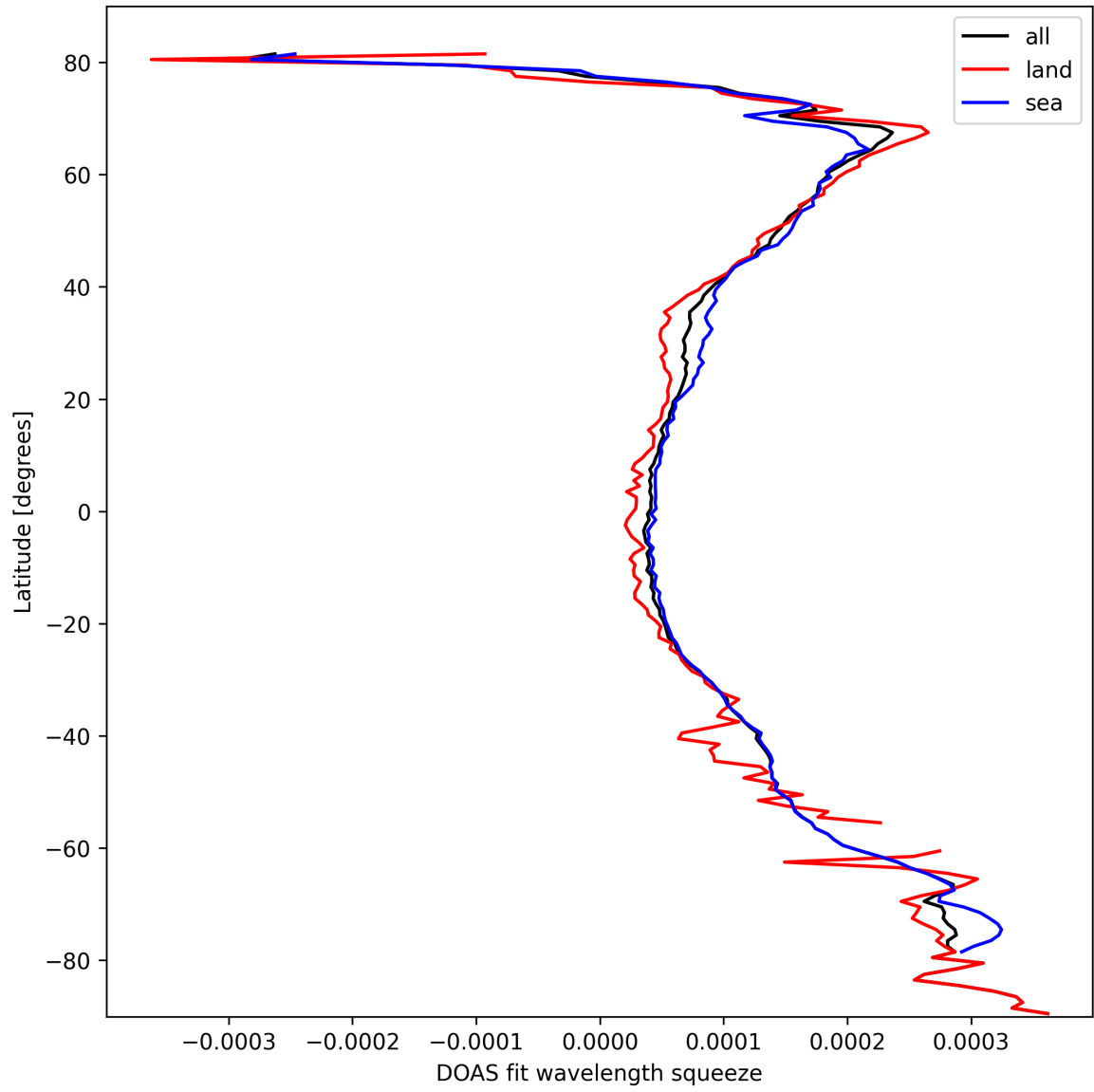
Figure 24: Zonal average of “DOAS fit wavelength squeeze” for 2025-10-13 to 2025-10-14.
