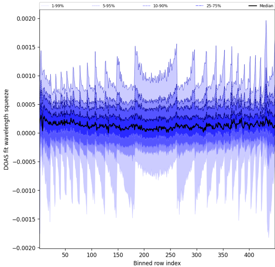
Figure 48: Along track statistics of “DOAS fit wavelength squeeze” for 2025-10-13 to 2025-10-14
