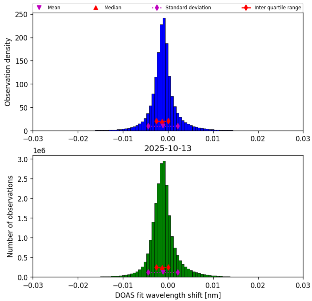
Figure 35: Histogram of “DOAS fit wavelength shift” for 2025-10-13 to 2025-10-14
