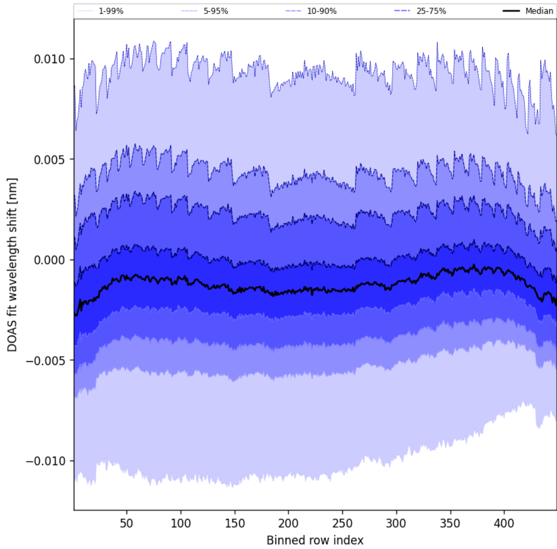
Figure 47: Along track statistics of “DOAS fit wavelength shift” for 2025-10-13 to 2025-10-14
