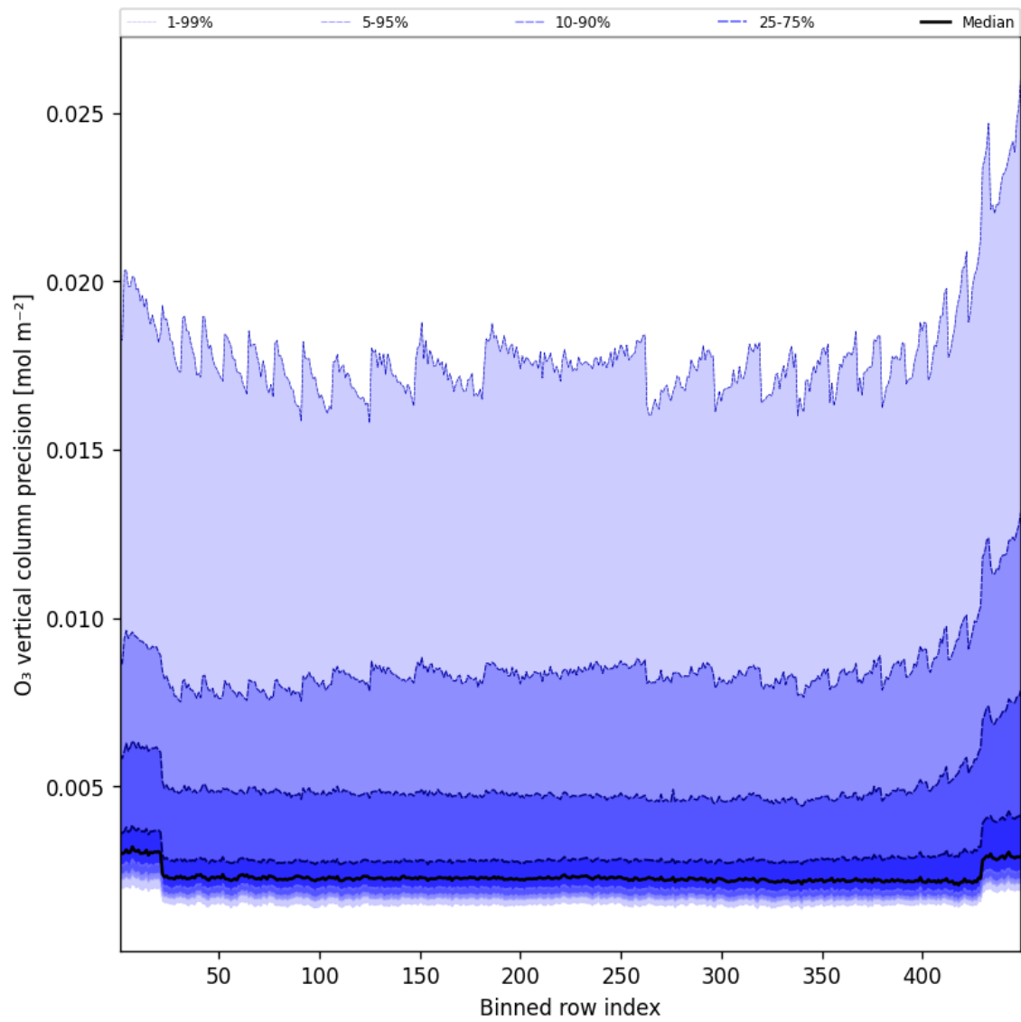
Figure 42: Along track statistics of “O 3 vertical column precision” for 2025-10-13 to 2025-10-14
