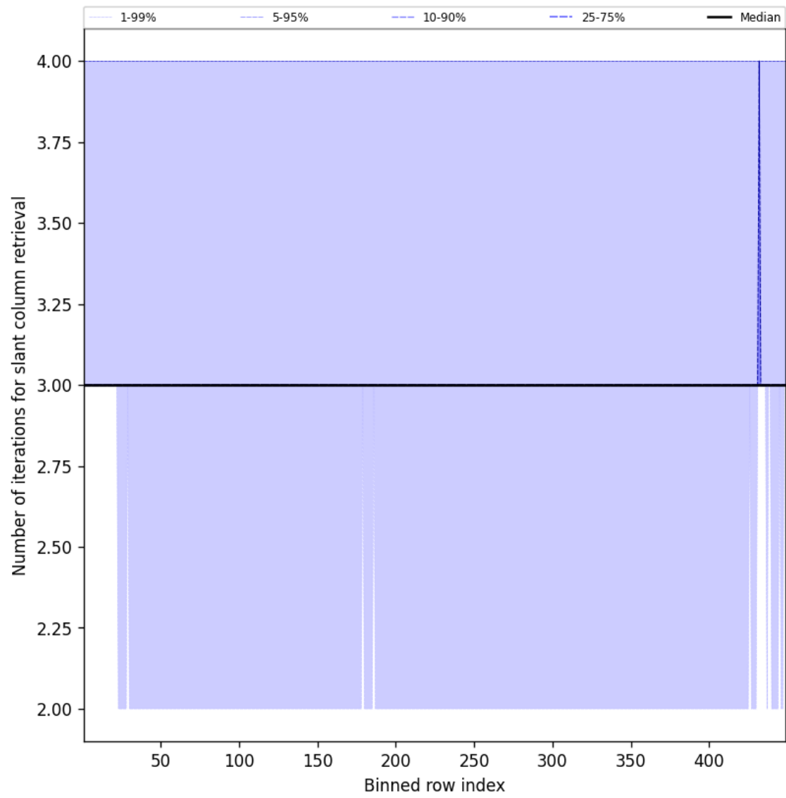
Figure 45: Along track statistics of “Number of iterations for slant column retrieval” for 2025-10-13 to 2025-10-14
