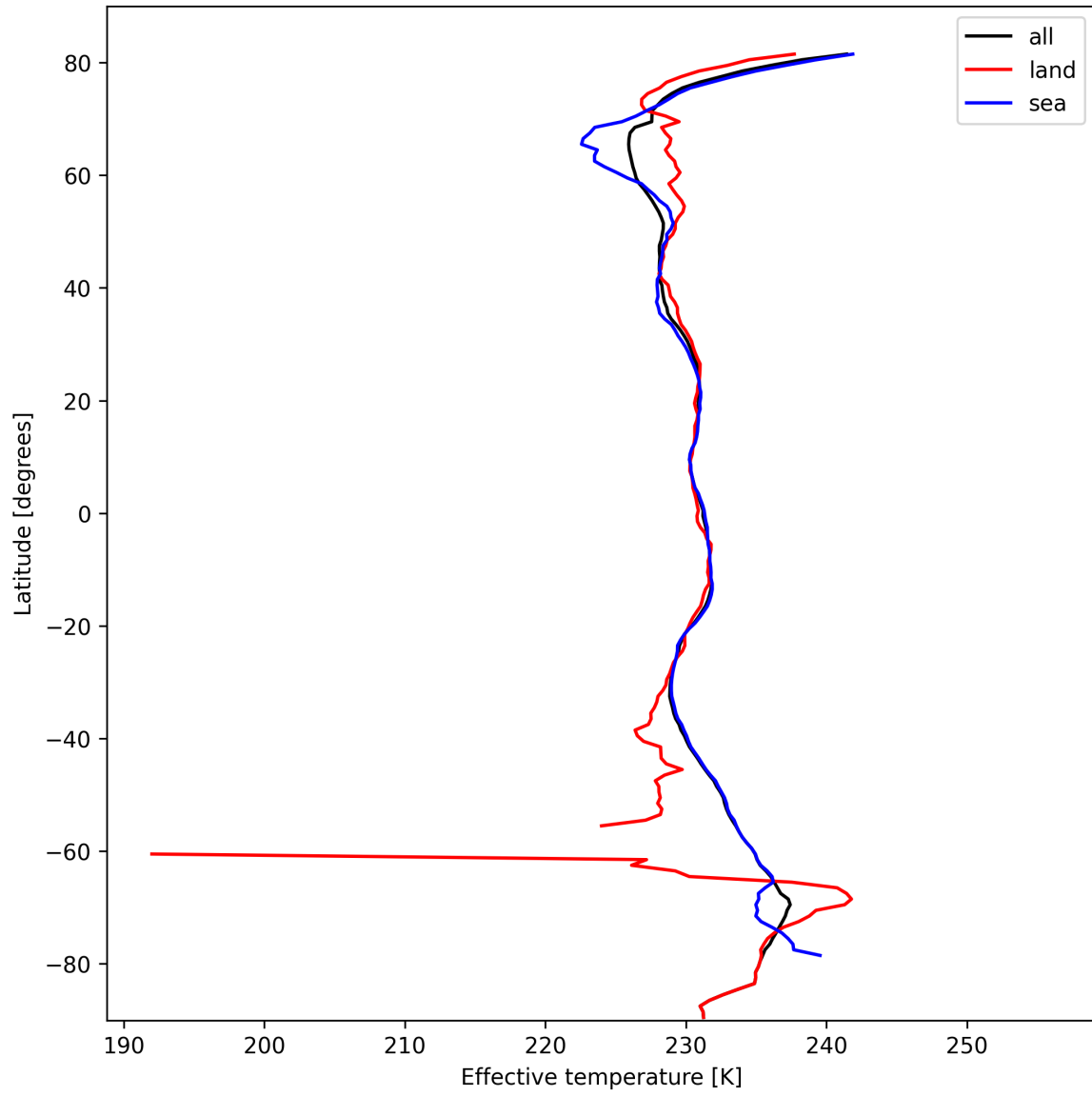
Figure 26: Zonal average of "Effective temperature" for 2025-10-13 to 2025-10-14.
