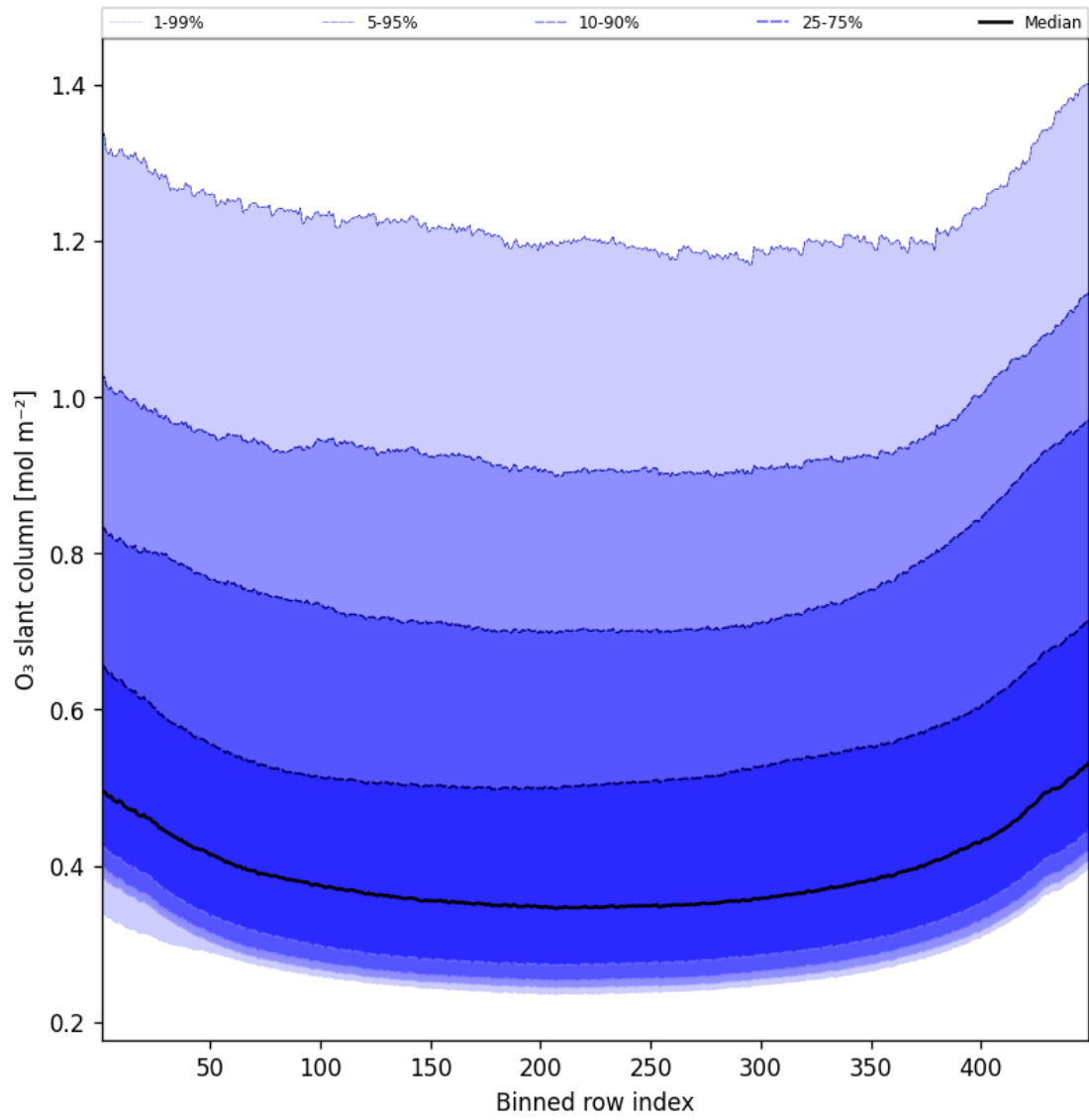
Figure 43: Along track statistics of “O 3 slant column” for 2025-10-13 to 2025-10-14
