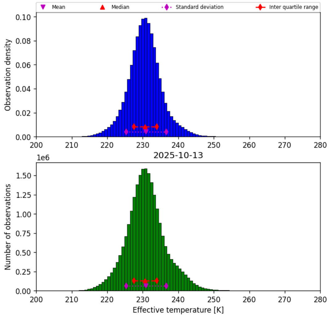
Figure 38: Histogram of “Effective temperature” for 2025-10-13 to 2025-10-14
