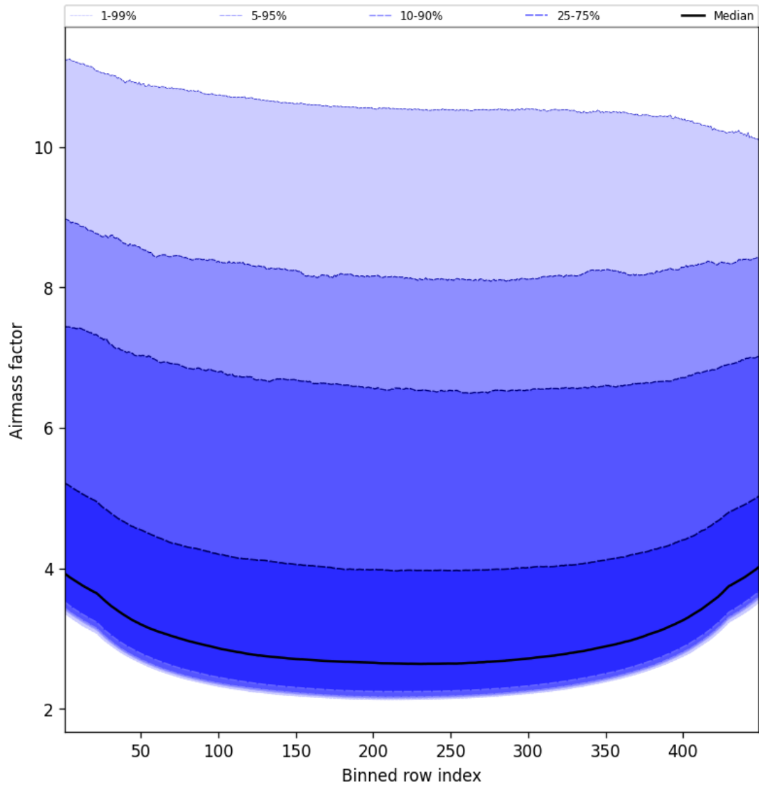
Figure 49: Along track statistics of “Airmass factor” for 2025-10-13 to 2025-10-14
