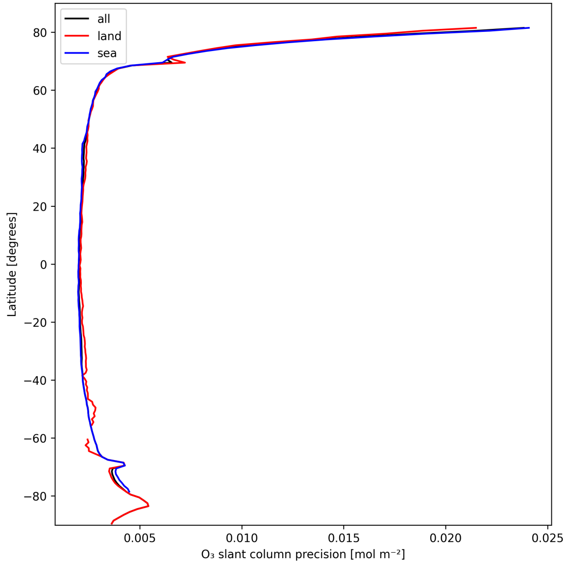
Figure 20: Zonal average of “O 3 slant column precision” for 2025-10-13 to 2025-10-14.
