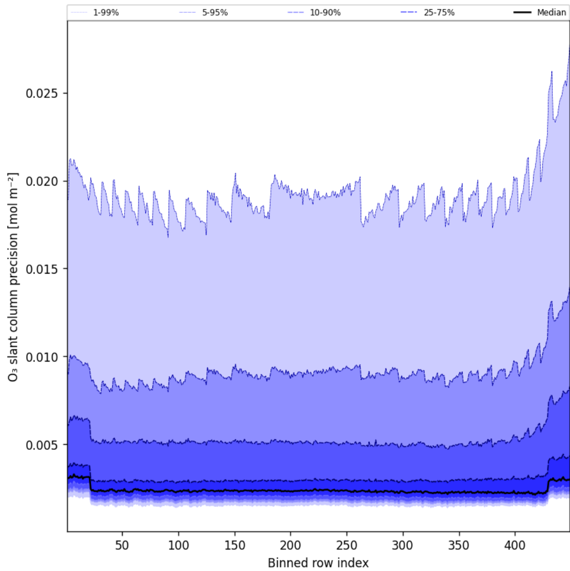
Figure 44: Along track statistics of “O 3 slant column precision” for 2025-10-13 to 2025-10-14
