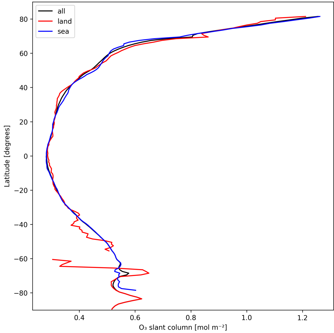
Figure 19: Zonal average of “O 3 slant column” for 2025-10-13 to 2025-10-14.
