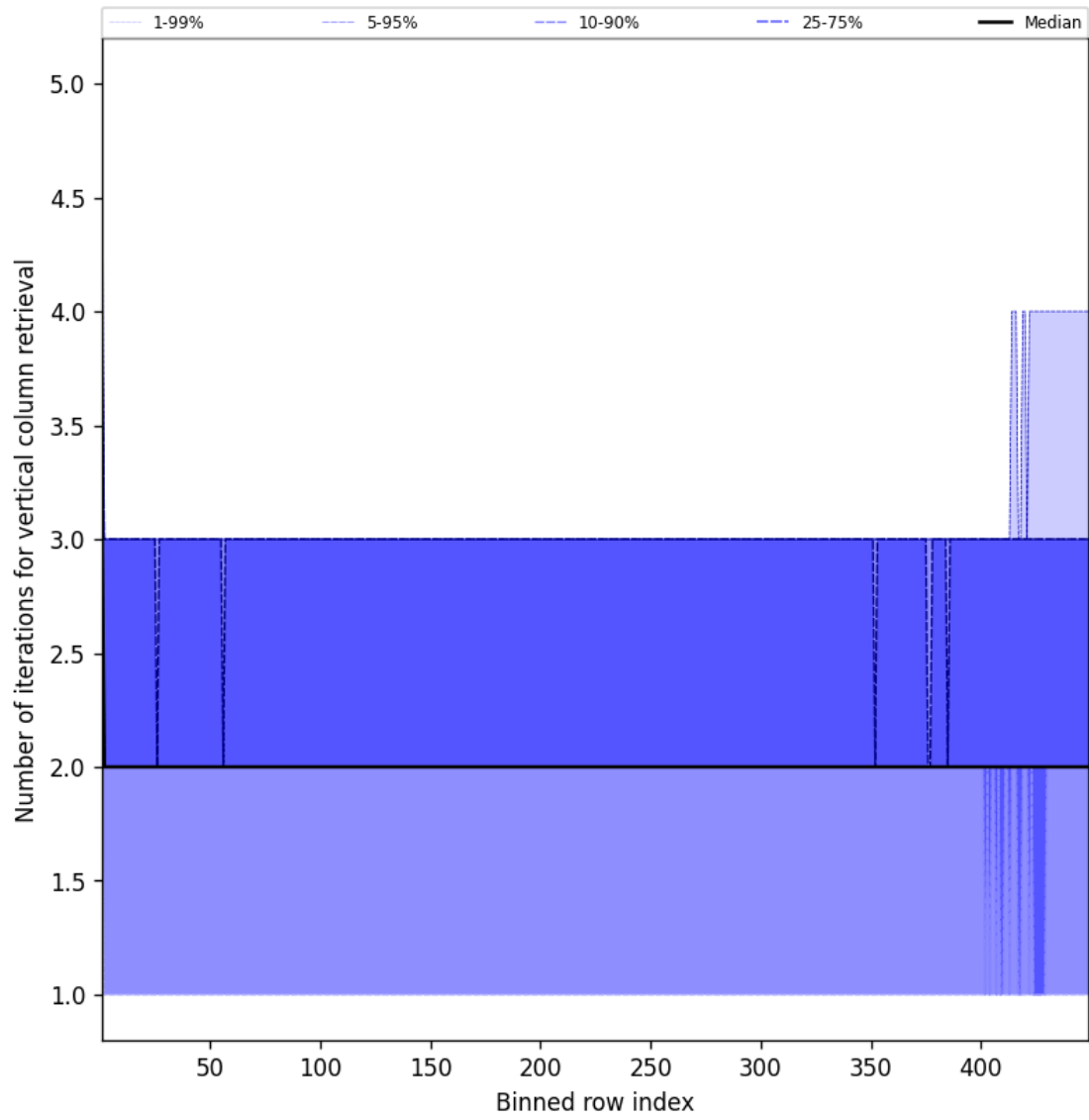
Figure 51: Along track statistics of “Number of iterations for vertical column retrieval” for 2025-10-13 to 2025-10-14
