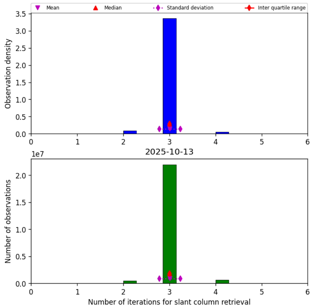
Figure 33: Histogram of “Number of iterations for slant column retrieval” for 2025-10-13 to 2025-10-14
