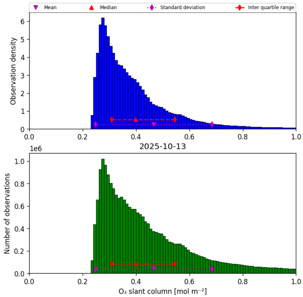
Figure 31: Histogram of “O 3 slant column” for 2025-10-13 to 2025-10-14
