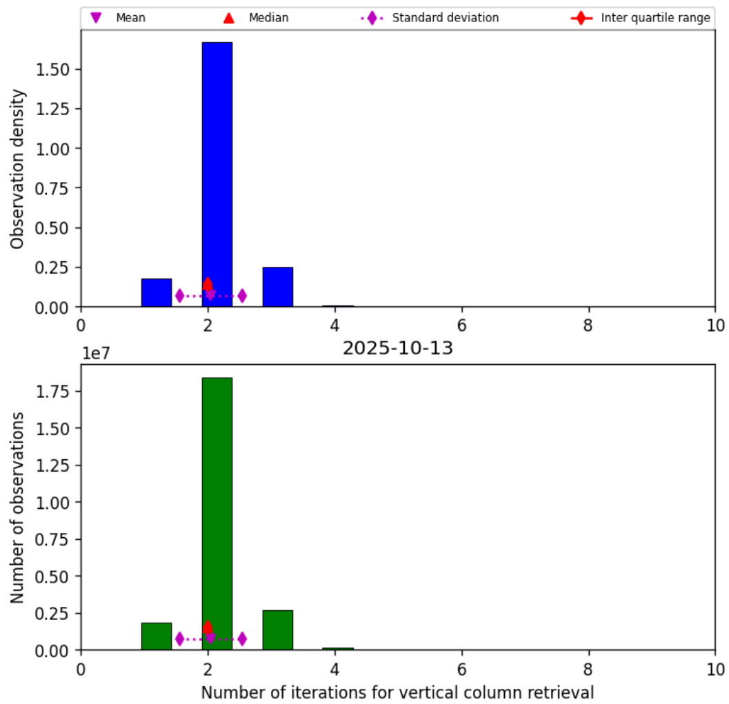
Figure 39: Histogram of “Number of iterations for vertical column retrieval” for 2025-10-13 to 2025-10-14
