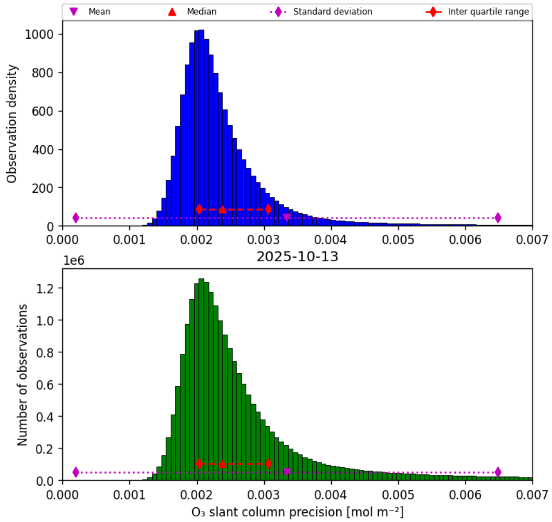
Figure 32: Histogram of “O 3 slant column precision” for 2025-10-13 to 2025-10-14
