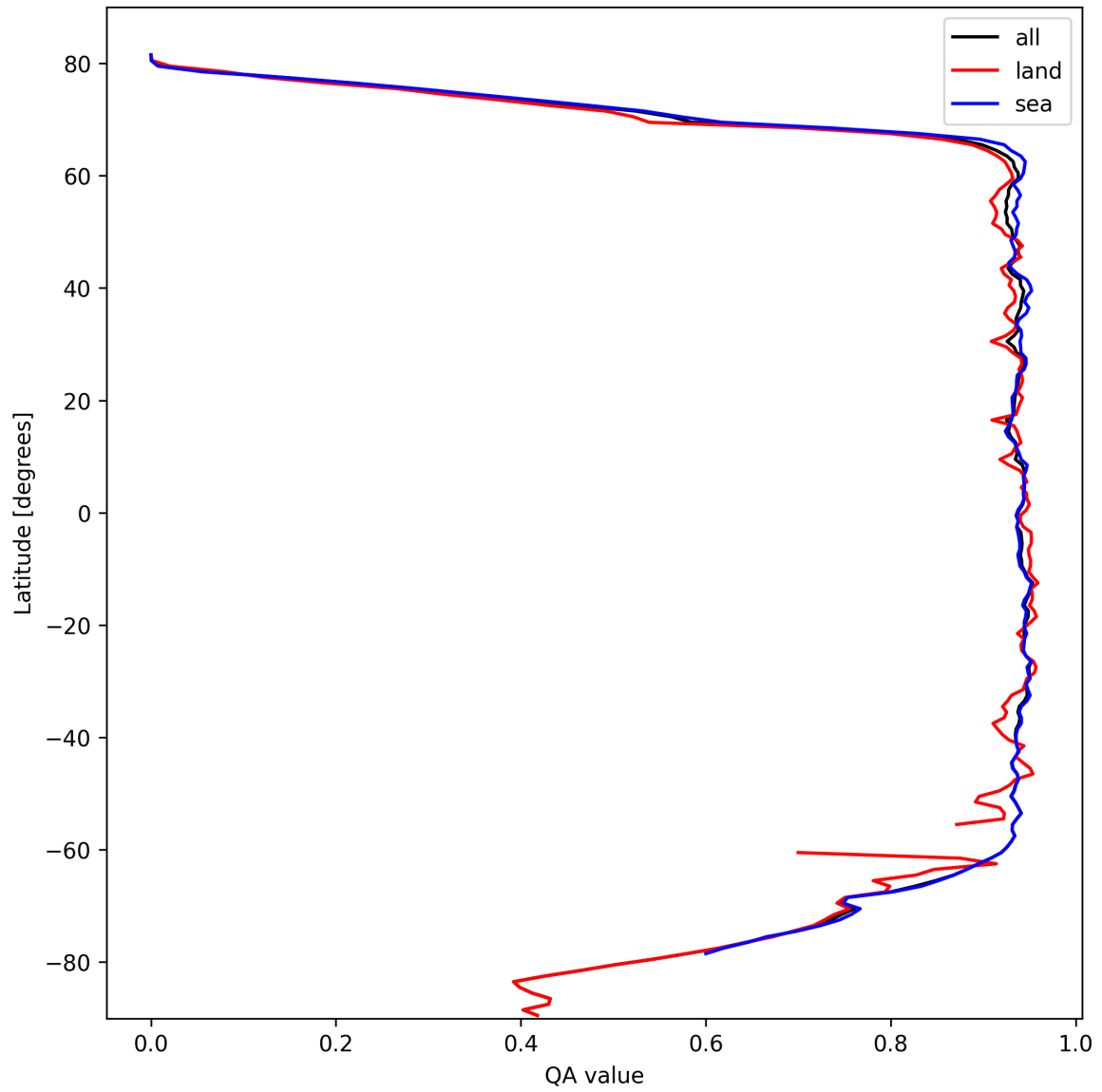
Figure 16: Zonal average of “QA value” for 2025-10-13 to 2025-10-14.
