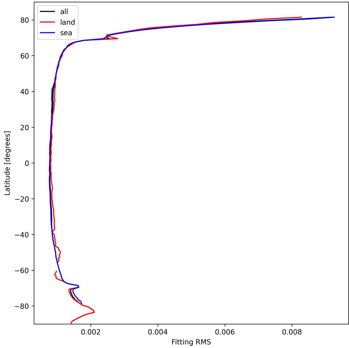
Figure 22: Zonal average of “Fitting RMS” for 2025-10-13 to 2025-10-14.
