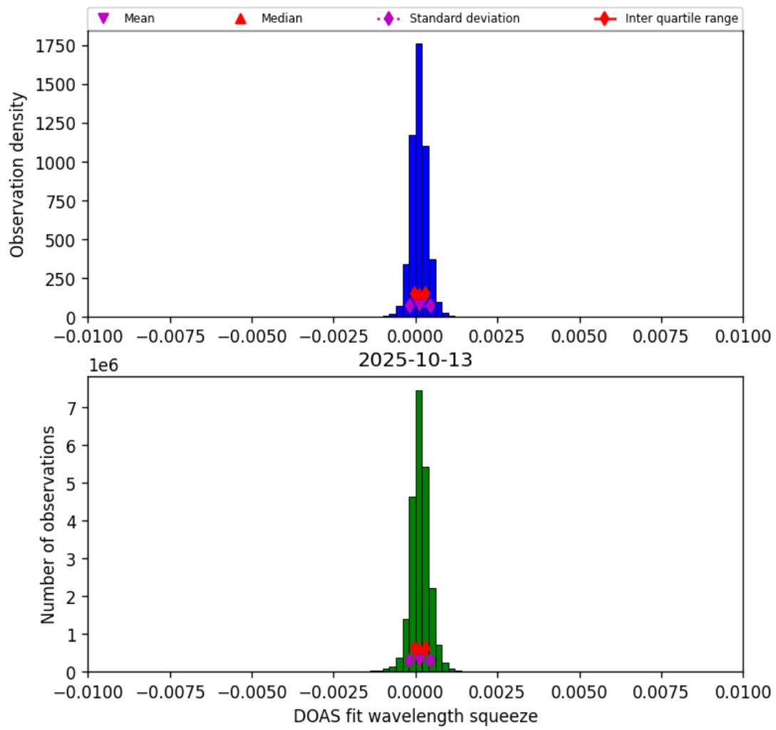
Figure 36: Histogram of “DOAS fit wavelength squeeze” for 2025-10-13 to 2025-10-14
