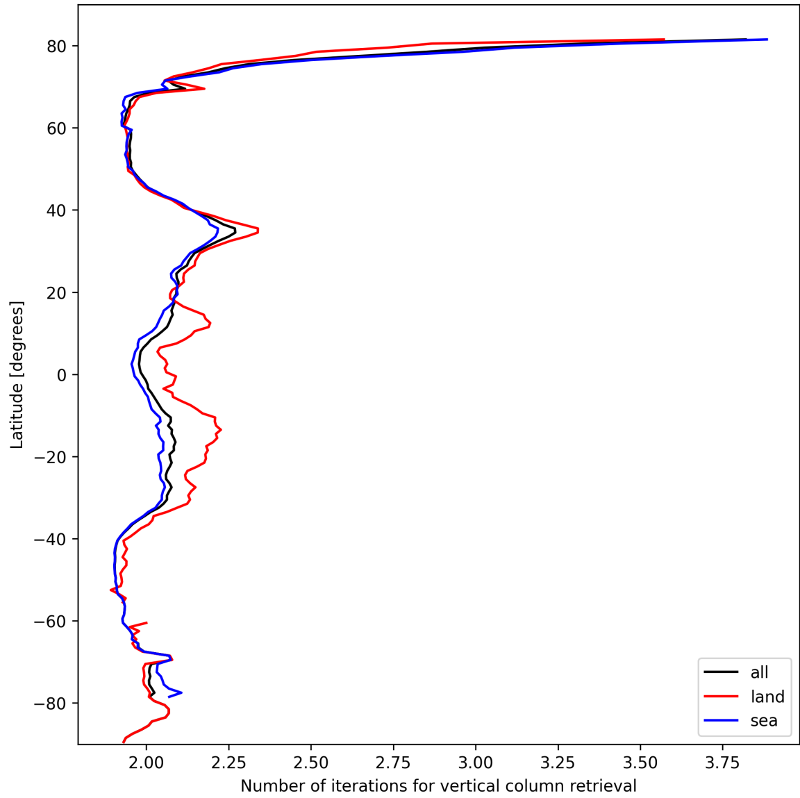
Figure 27: Zonal average of “Number of iterations for vertical column retrieval” for 2025-10-13 to 2025-10-14.
