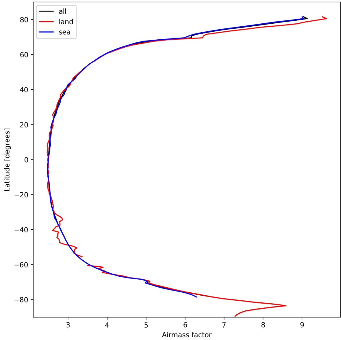
Figure 25: Zonal average of “Airmass factor” for 2025-10-13 to 2025-10-14.
