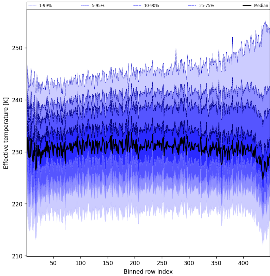
Figure 50: Along track statistics of “Effective temperature” for 2025-10-13 to 2025-10-14
