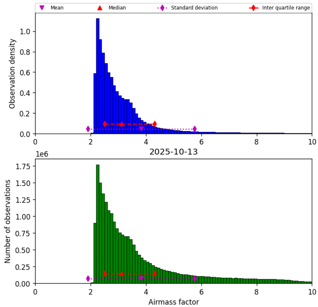
Figure 37: Histogram of “Airmass factor” for 2025-10-13 to 2025-10-14
