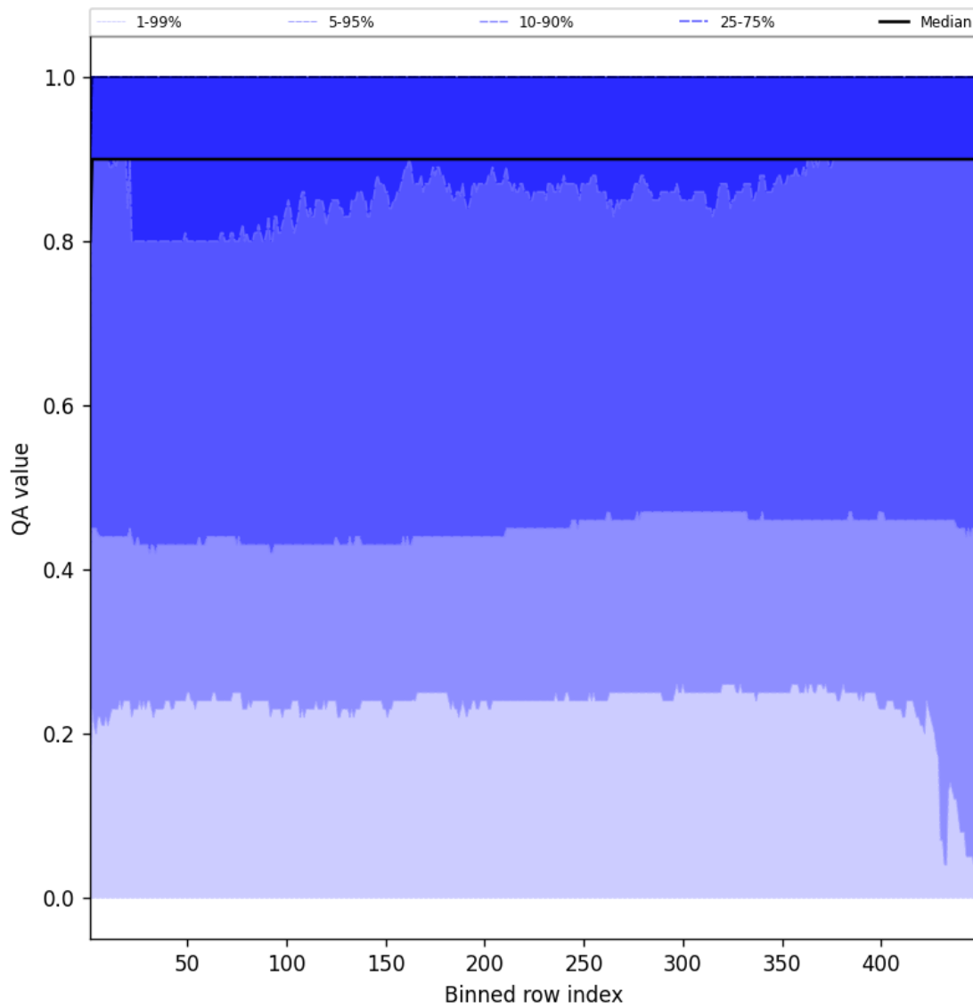
Figure 40: Along track statistics of “QA value” for 2025-10-13 to 2025-10-14
