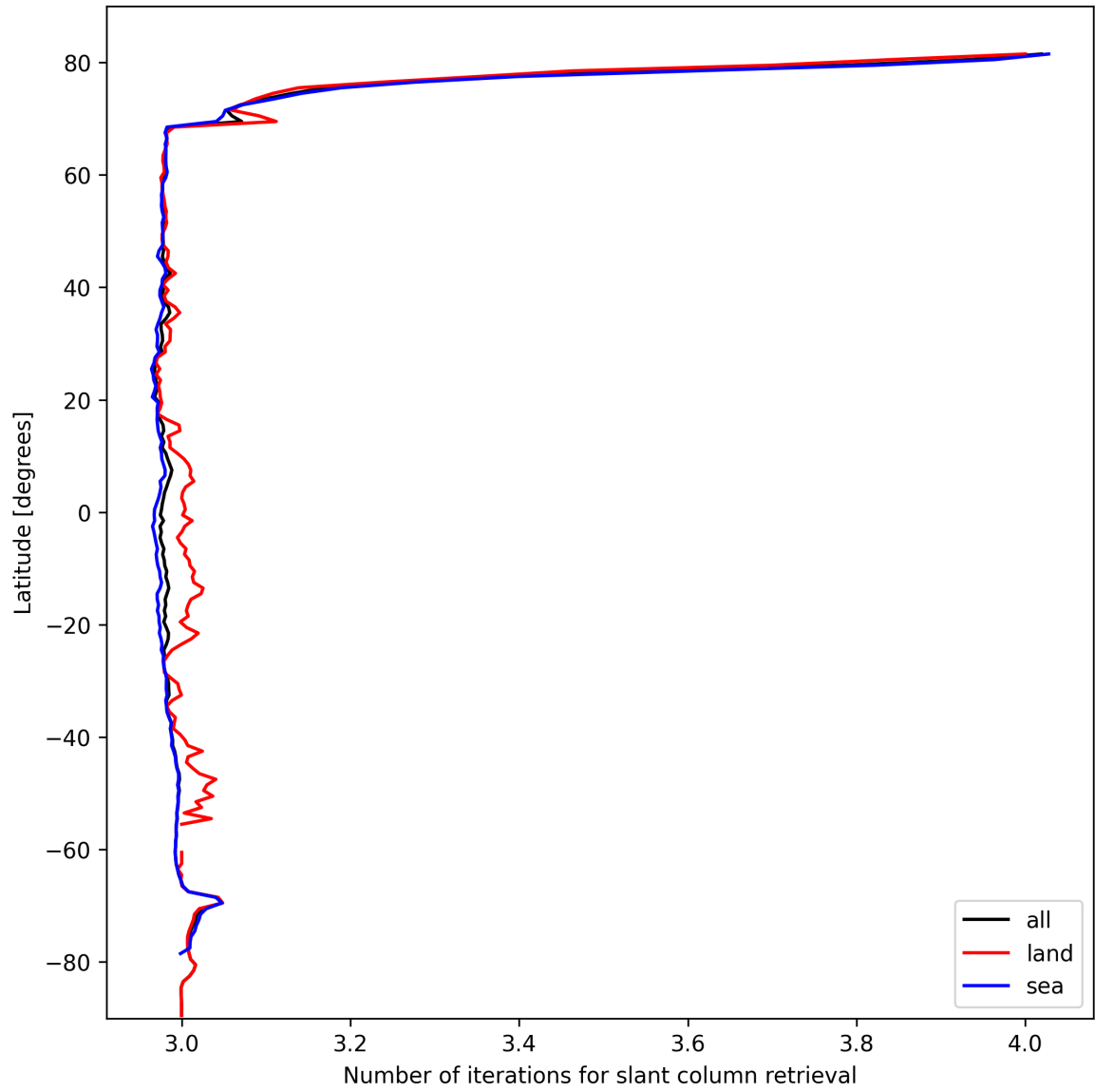
Figure 21: Zonal average of “Number of iterations for slant column retrieval” for 2025-10-13 to 2025-10-14.
