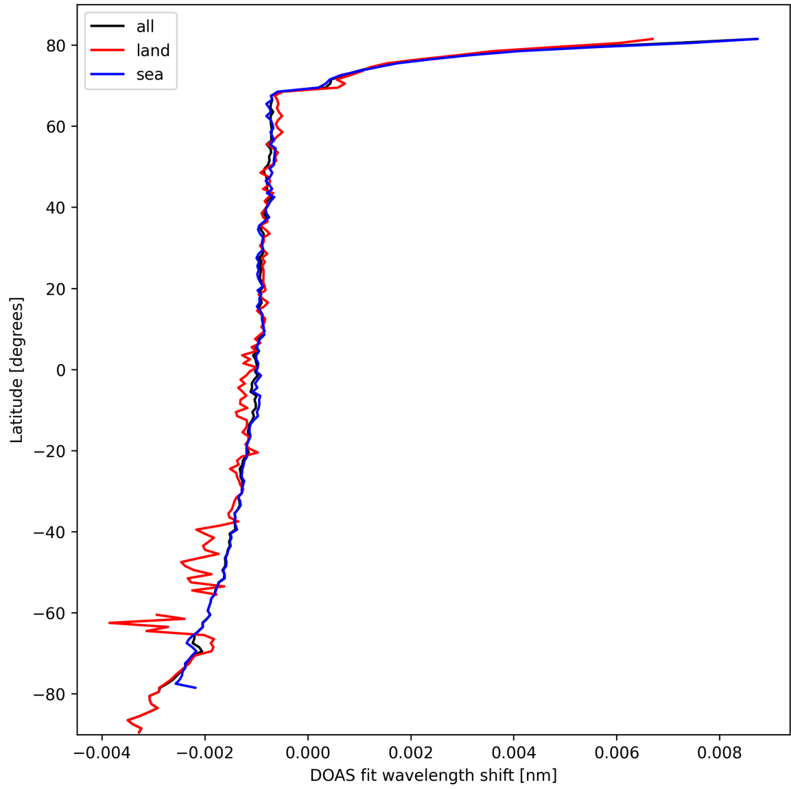
Figure 23: Zonal average of “DOAS fit wavelength shift” for 2025-10-13 to 2025-10-14.
