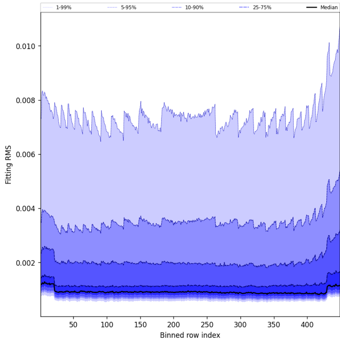
Figure 46: Along track statistics of “Fitting RMS” for 2025-10-13 to 2025-10-14
