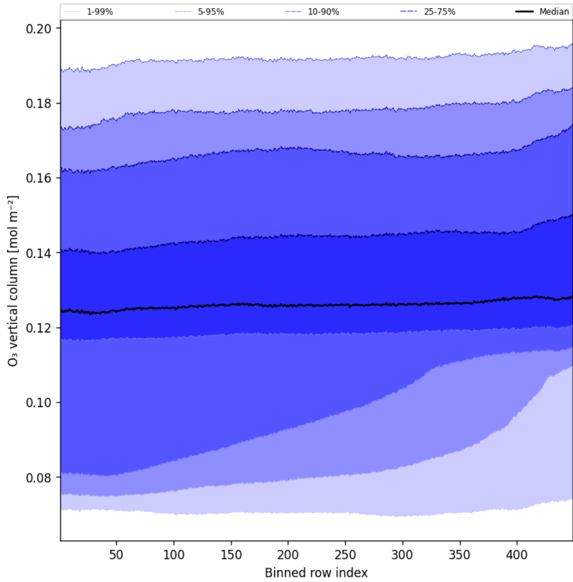
Figure 41: Along track statistics of “O 3 vertical column” for 2025-10-13 to 2025-10-14
