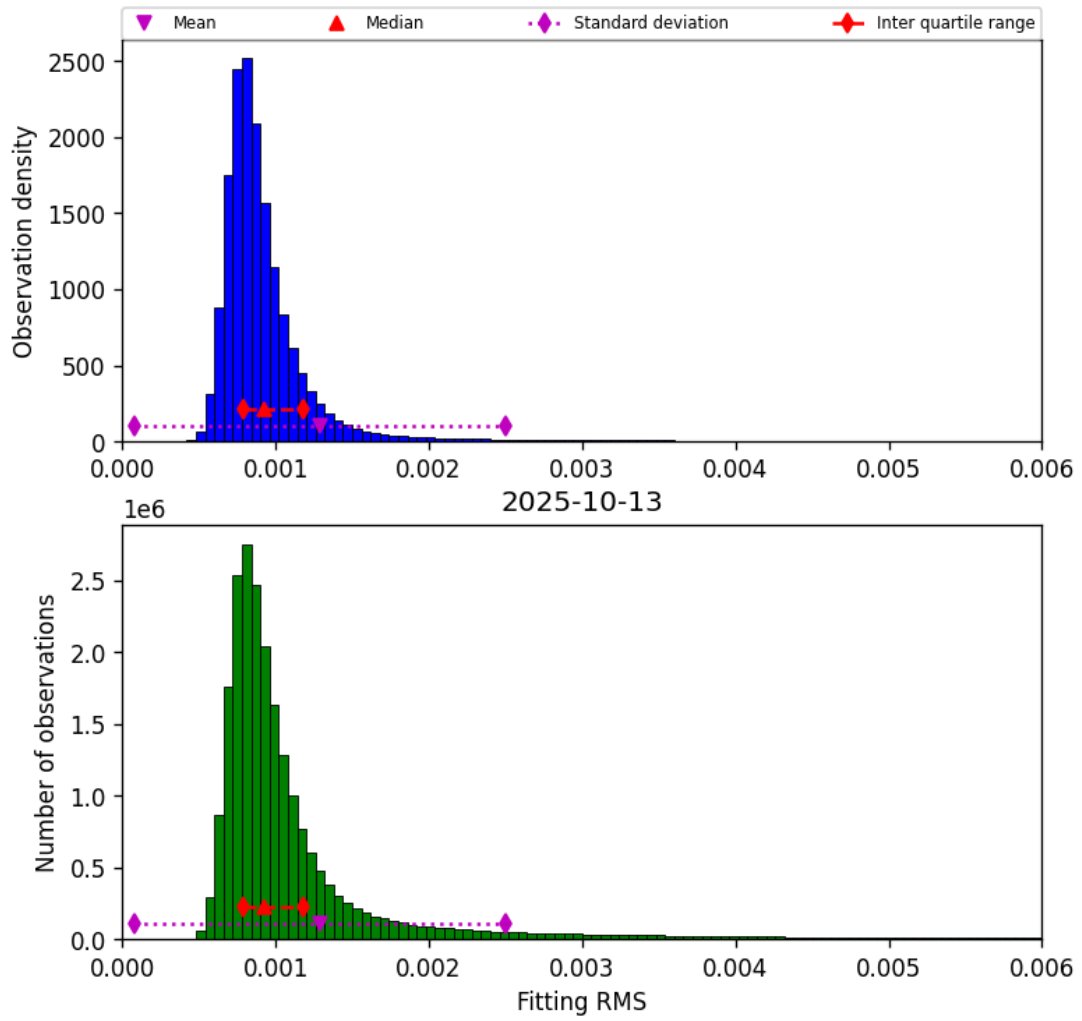
Figure 34: Histogram of “Fitting RMS” for 2025-10-13 to 2025-10-14
