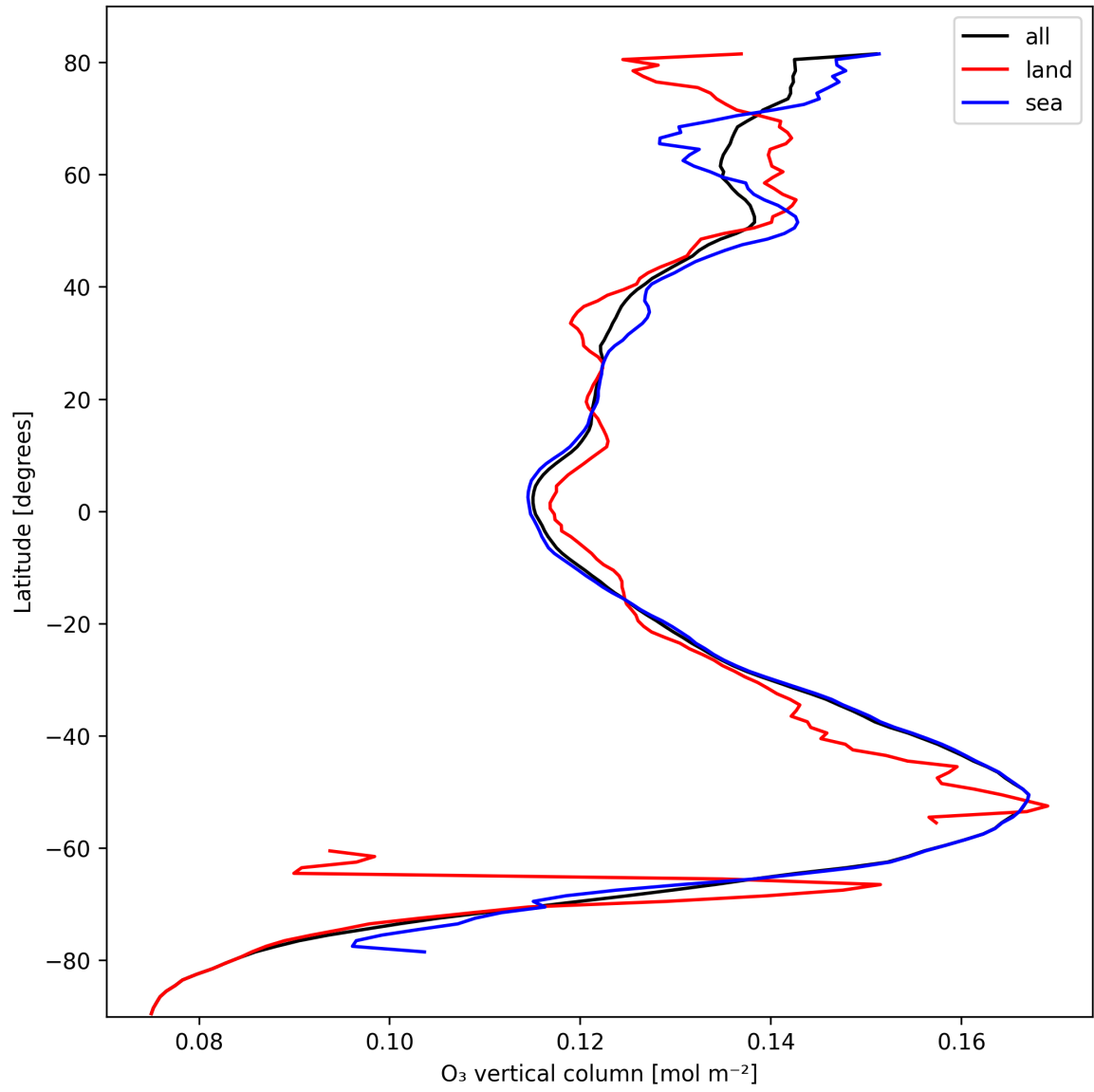
Figure 17: Zonal average of “O 3 vertical column” for 2025-10-13 to 2025-10-14.
