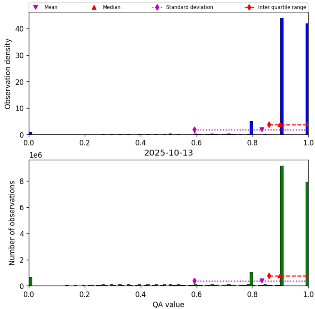
Figure 28: Histogram of “QA value” for 2025-10-13 to 2025-10-14
