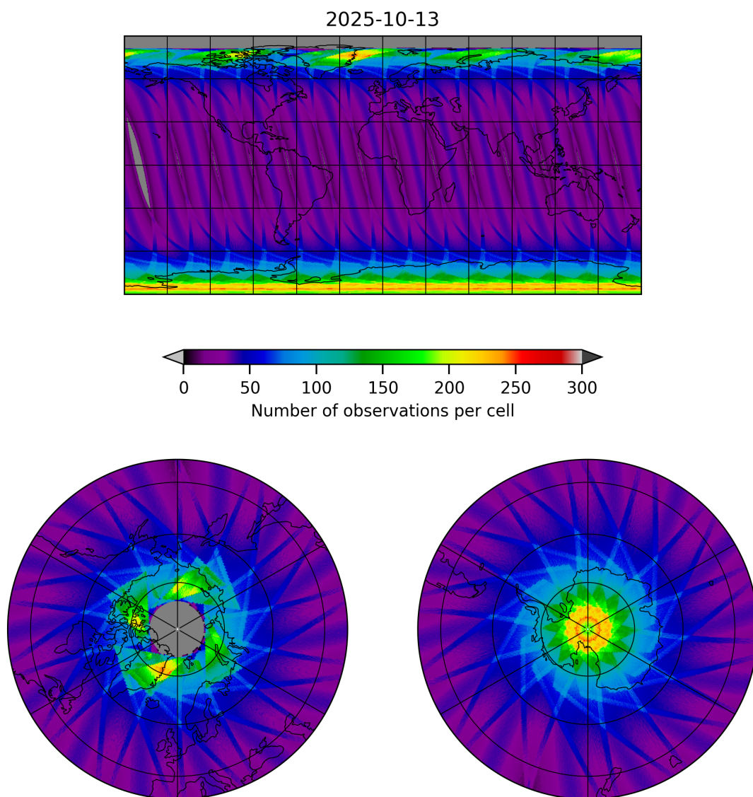
Figure 15: Map of the number of observations for 2025-10-13 to 2025-10-14
