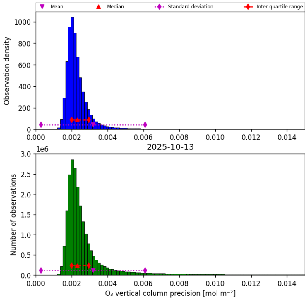
Figure 30: Histogram of “O 3 vertical column precision” for 2025-10-13 to 2025-10-14
