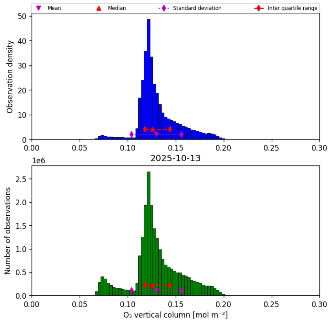
Figure 29: Histogram of “O 3 vertical column” for 2025-10-13 to 2025-10-14
