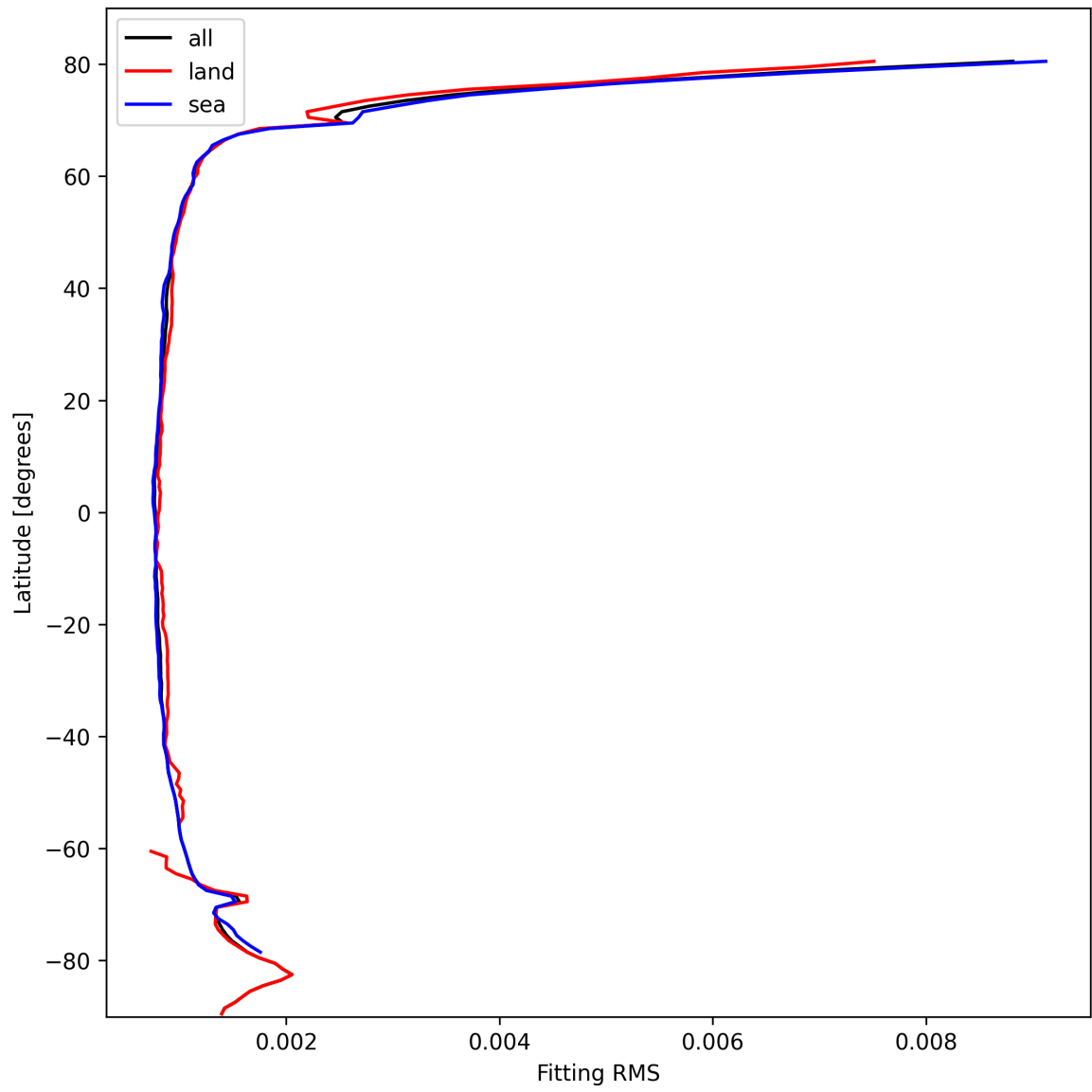
Figure 22: Zonal average of “Fitting RMS” for 2025-10-14 to 2025-10-15.
