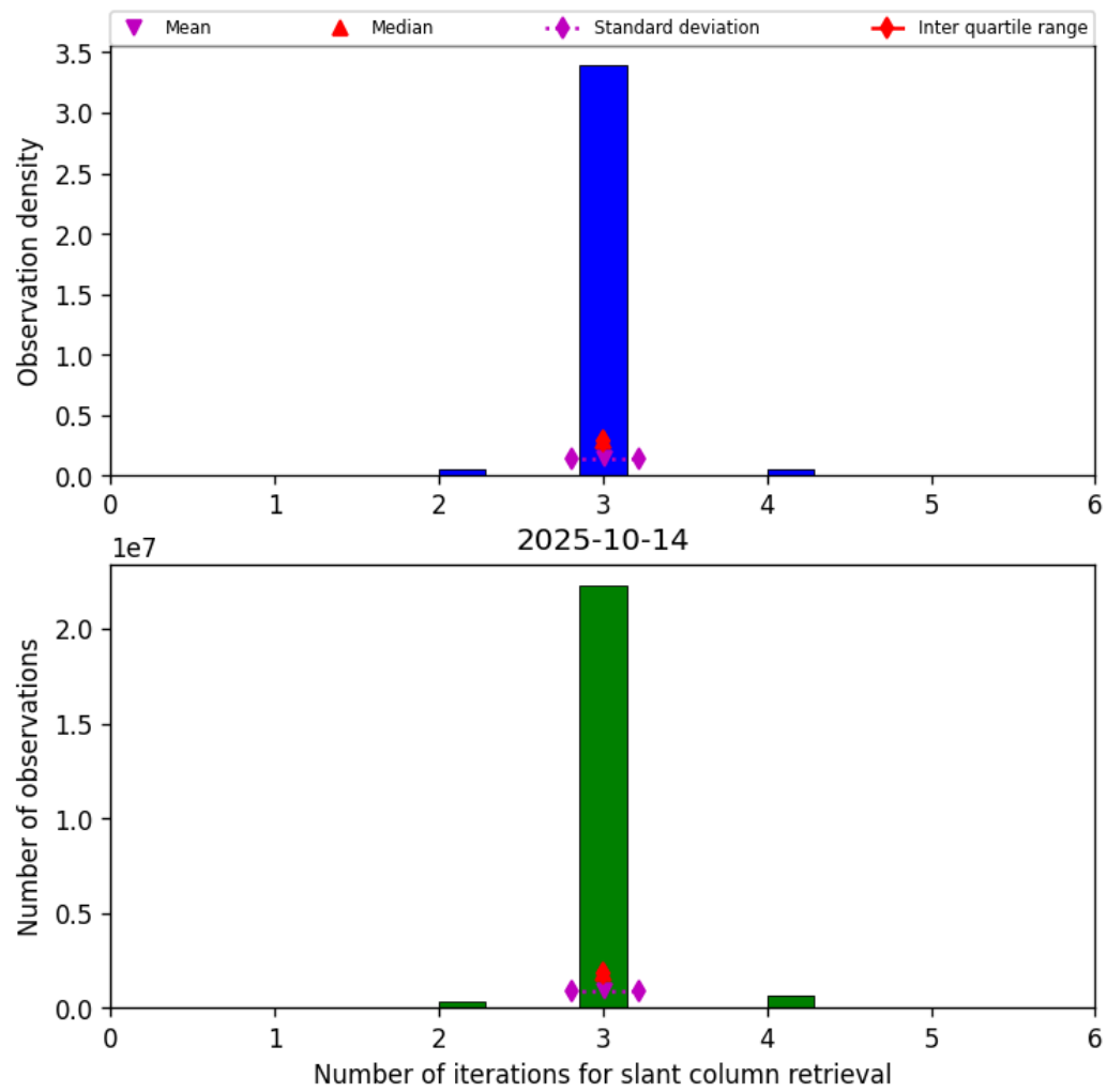
Figure 33: Histogram of “Number of iterations for slant column retrieval” for 2025-10-14 to 2025-10-15
