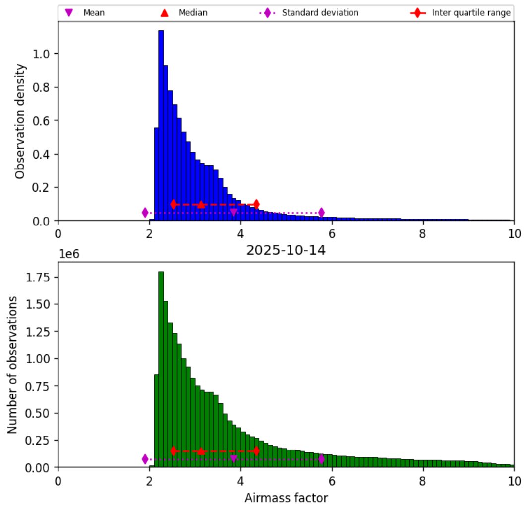
Figure 37: Histogram of “Airmass factor” for 2025-10-14 to 2025-10-15
