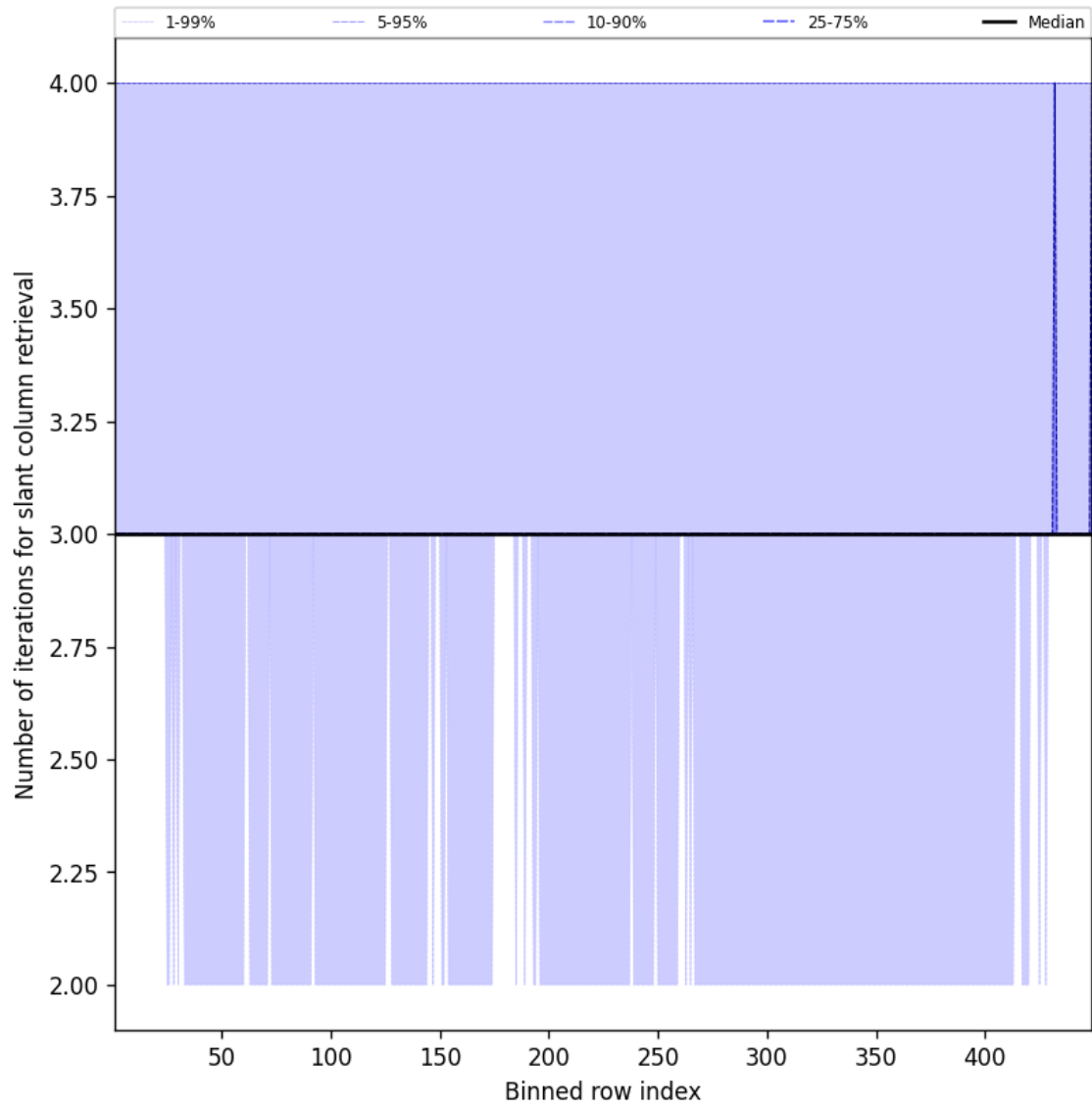
Figure 45: Along track statistics of “Number of iterations for slant column retrieval” for 2025-10-14 to 2025-10-15
