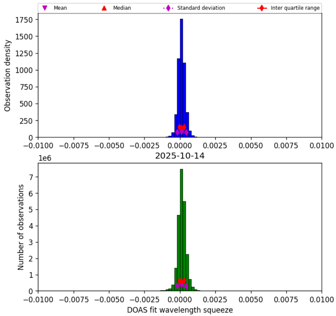
Figure 36: Histogram of “DOAS fit wavelength squeeze” for 2025-10-14 to 2025-10-15
