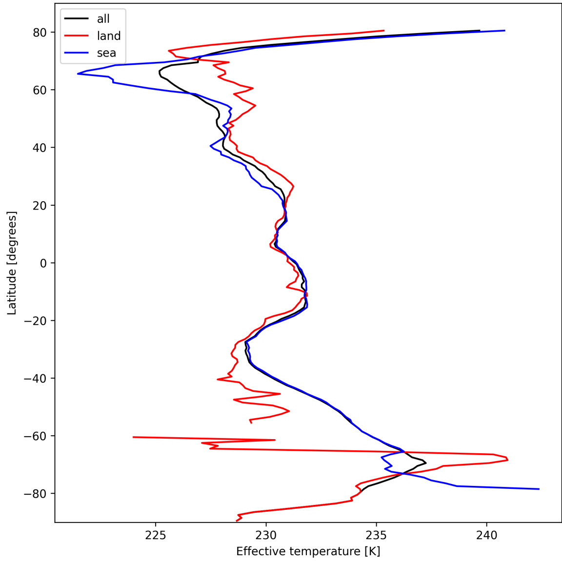
Figure 26: Zonal average of "Effective temperature" for 2025-10-14 to 2025-10-15.
