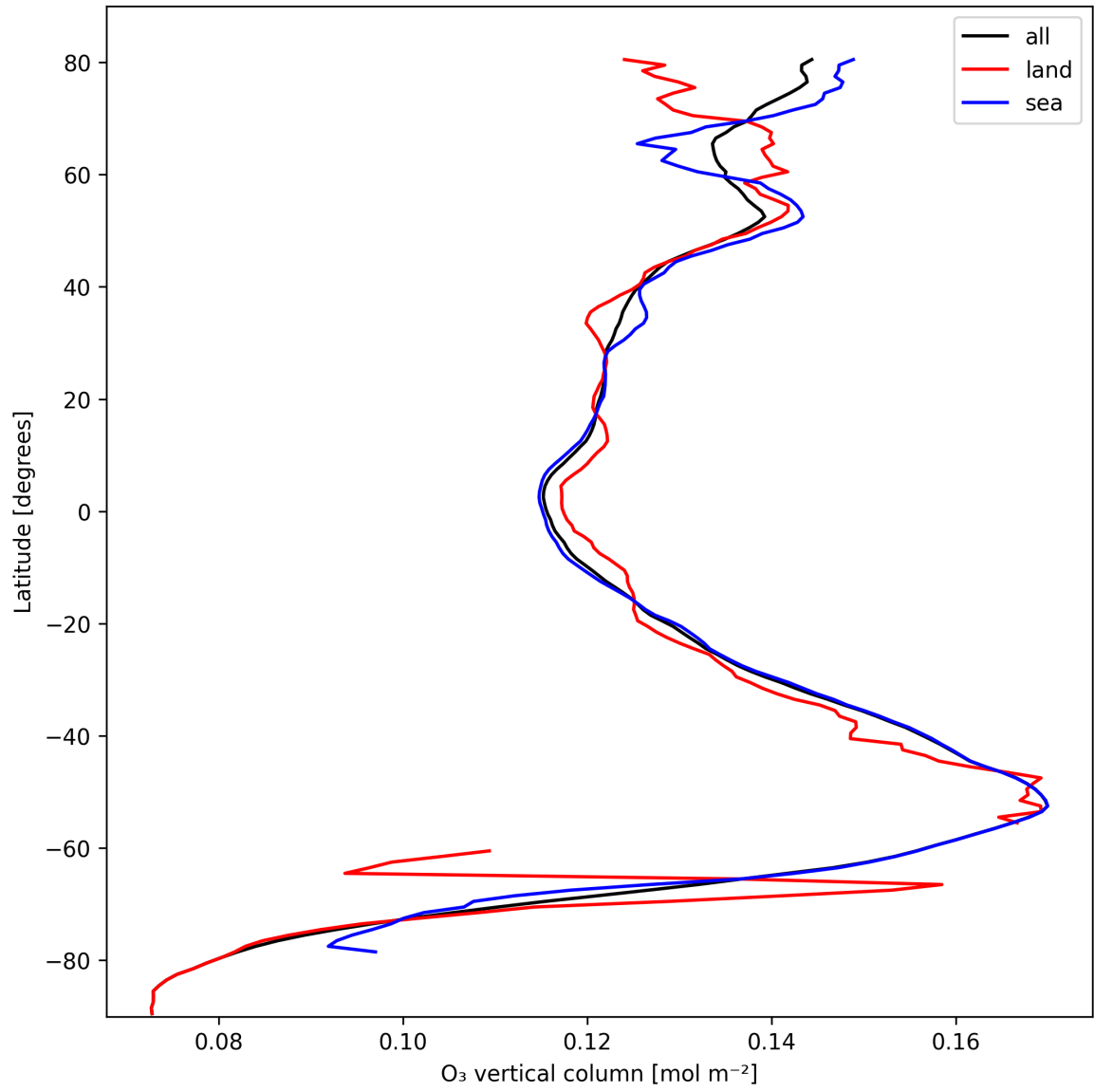
Figure 17: Zonal average of “O 3 vertical column” for 2025-10-14 to 2025-10-15.
