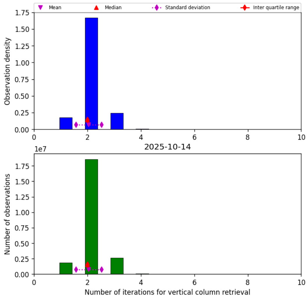
Figure 39: Histogram of “Number of iterations for vertical column retrieval” for 2025-10-14 to 2025-10-15
