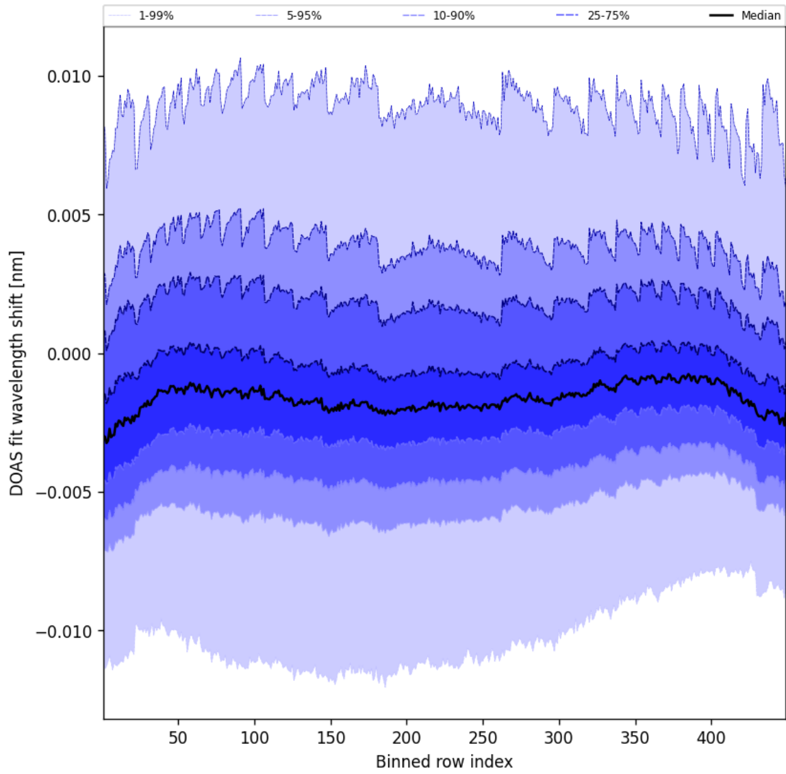
Figure 47: Along track statistics of “DOAS fit wavelength shift” for 2025-10-14 to 2025-10-15
