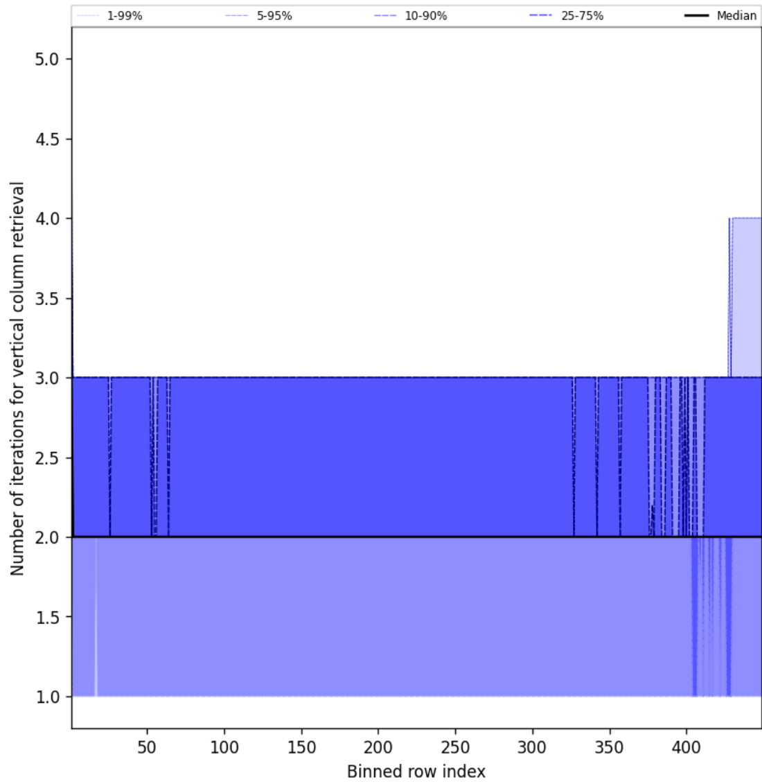
Figure 51: Along track statistics of “Number of iterations for vertical column retrieval” for 2025-10-14 to 2025-10-15
