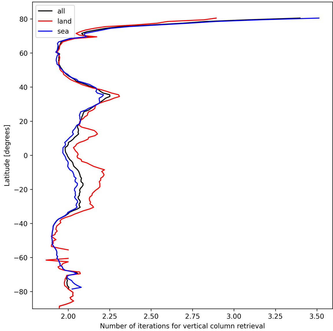
Figure 27: Zonal average of “Number of iterations for vertical column retrieval” for 2025-10-14 to 2025-10-15.
