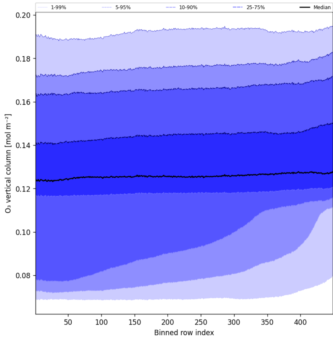
Figure 41: Along track statistics of “O 3 vertical column” for 2025-10-14 to 2025-10-15
