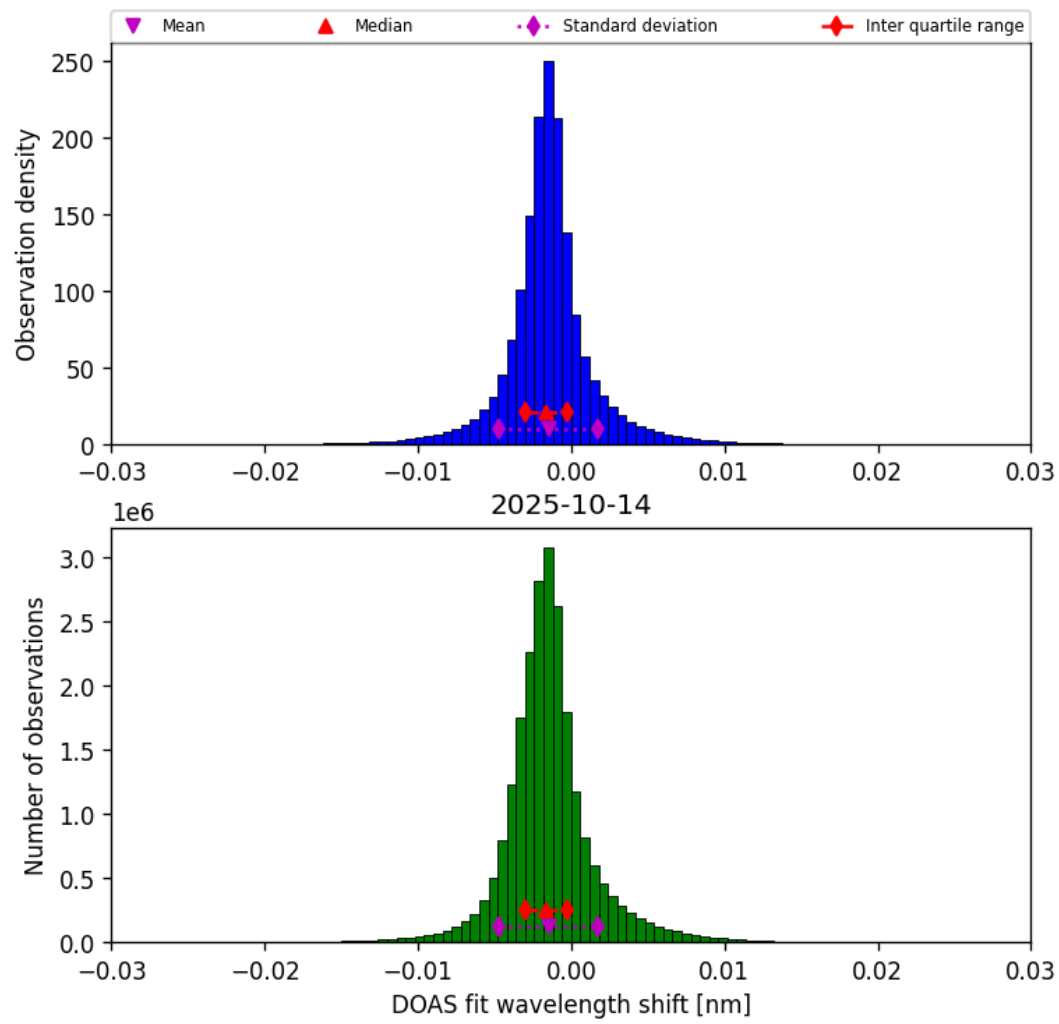
Figure 35: Histogram of “DOAS fit wavelength shift” for 2025-10-14 to 2025-10-15
