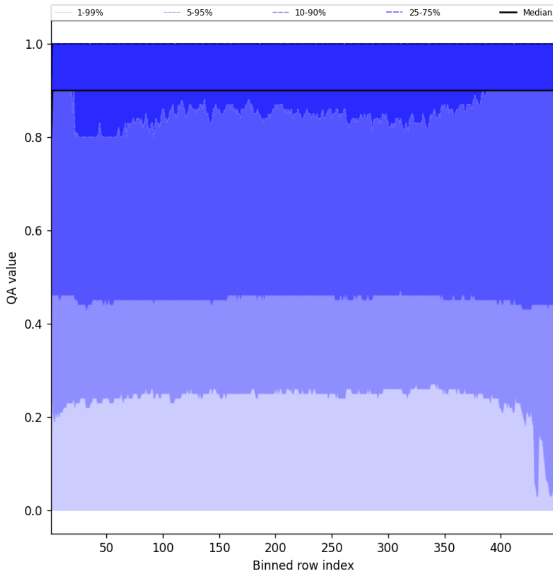
Figure 40: Along track statistics of “QA value” for 2025-10-14 to 2025-10-15
