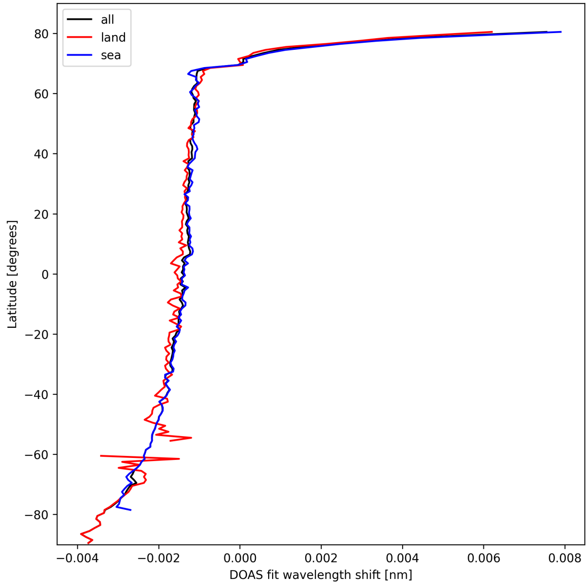
Figure 23: Zonal average of “DOAS fit wavelength shift” for 2025-10-14 to 2025-10-15.
