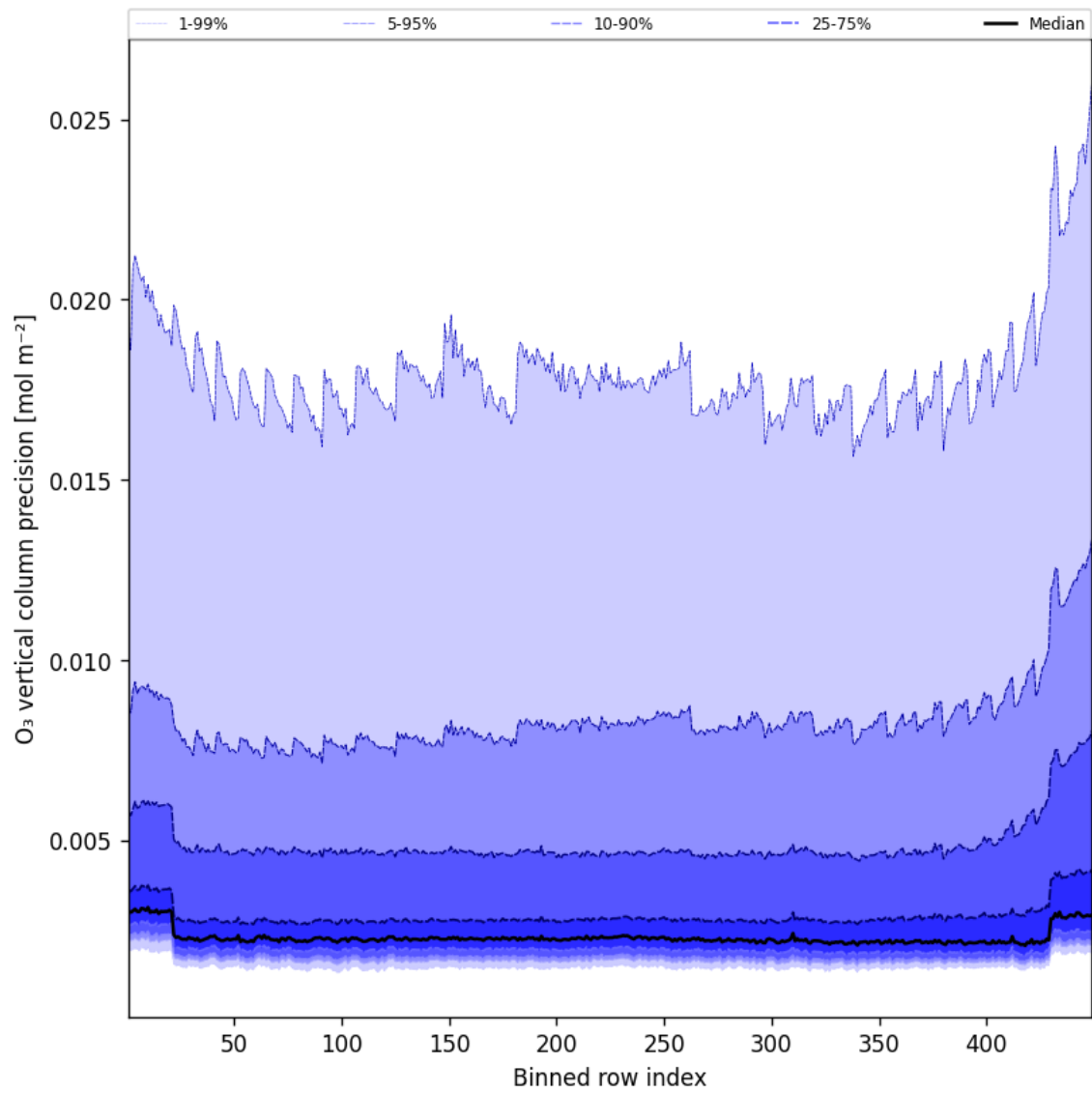
Figure 42: Along track statistics of “O 3 vertical column precision” for 2025-10-14 to 2025-10-15
