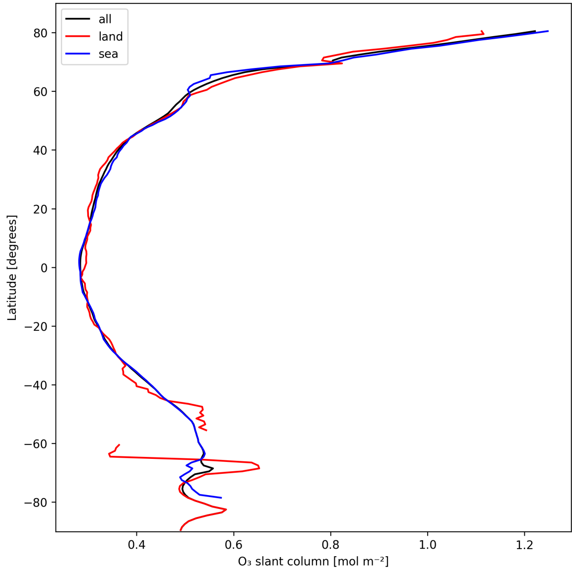
Figure 19: Zonal average of “O 3 slant column” for 2025-10-14 to 2025-10-15.
