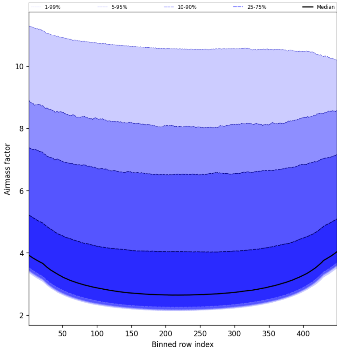
Figure 49: Along track statistics of “Airmass factor” for 2025-10-14 to 2025-10-15
