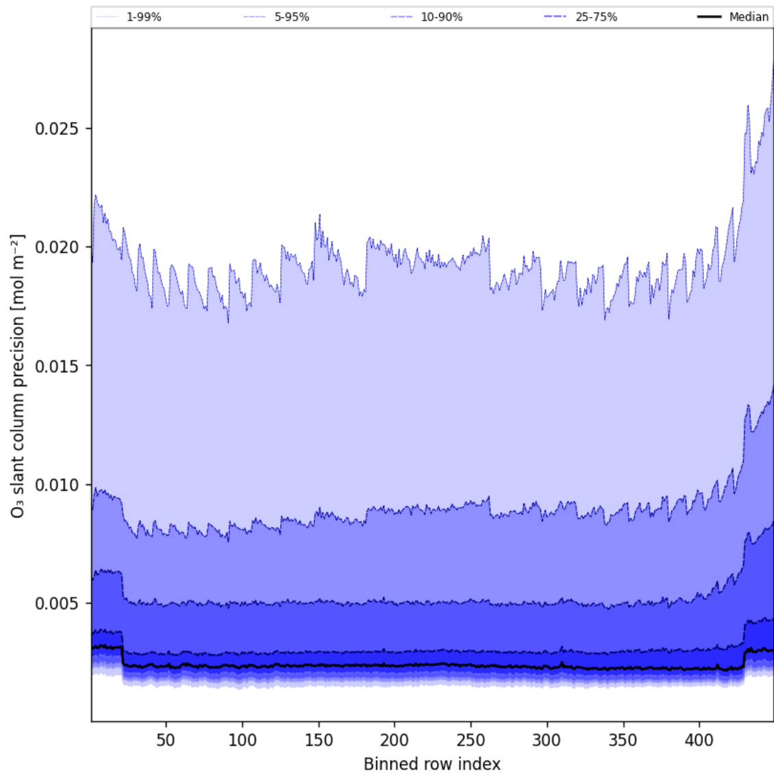
Figure 44: Along track statistics of “O 3 slant column precision” for 2025-10-14 to 2025-10-15
