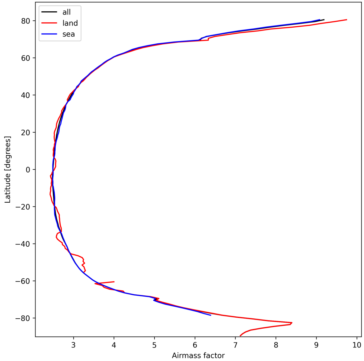
Figure 25: Zonal average of “Airmass factor” for 2025-10-14 to 2025-10-15.
