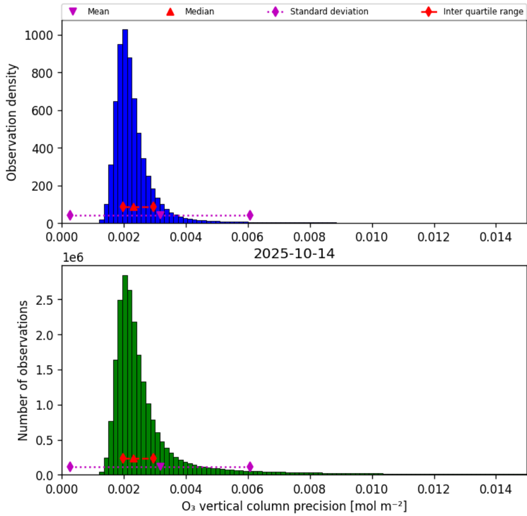
Figure 30: Histogram of “O 3 vertical column precision” for 2025-10-14 to 2025-10-15
