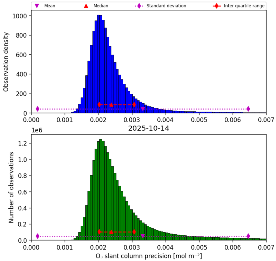
Figure 32: Histogram of “O 3 slant column precision” for 2025-10-14 to 2025-10-15
