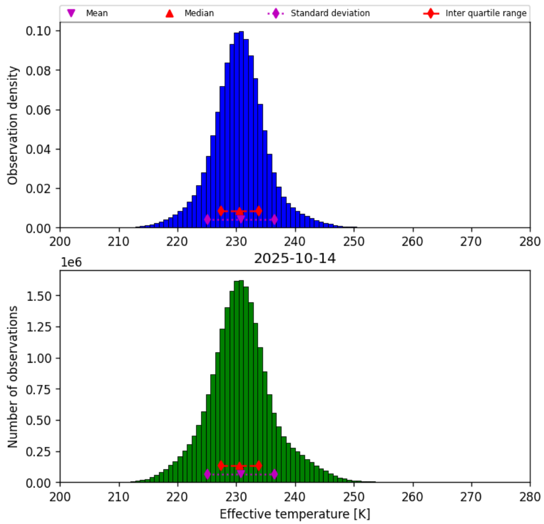
Figure 38: Histogram of “Effective temperature” for 2025-10-14 to 2025-10-15
