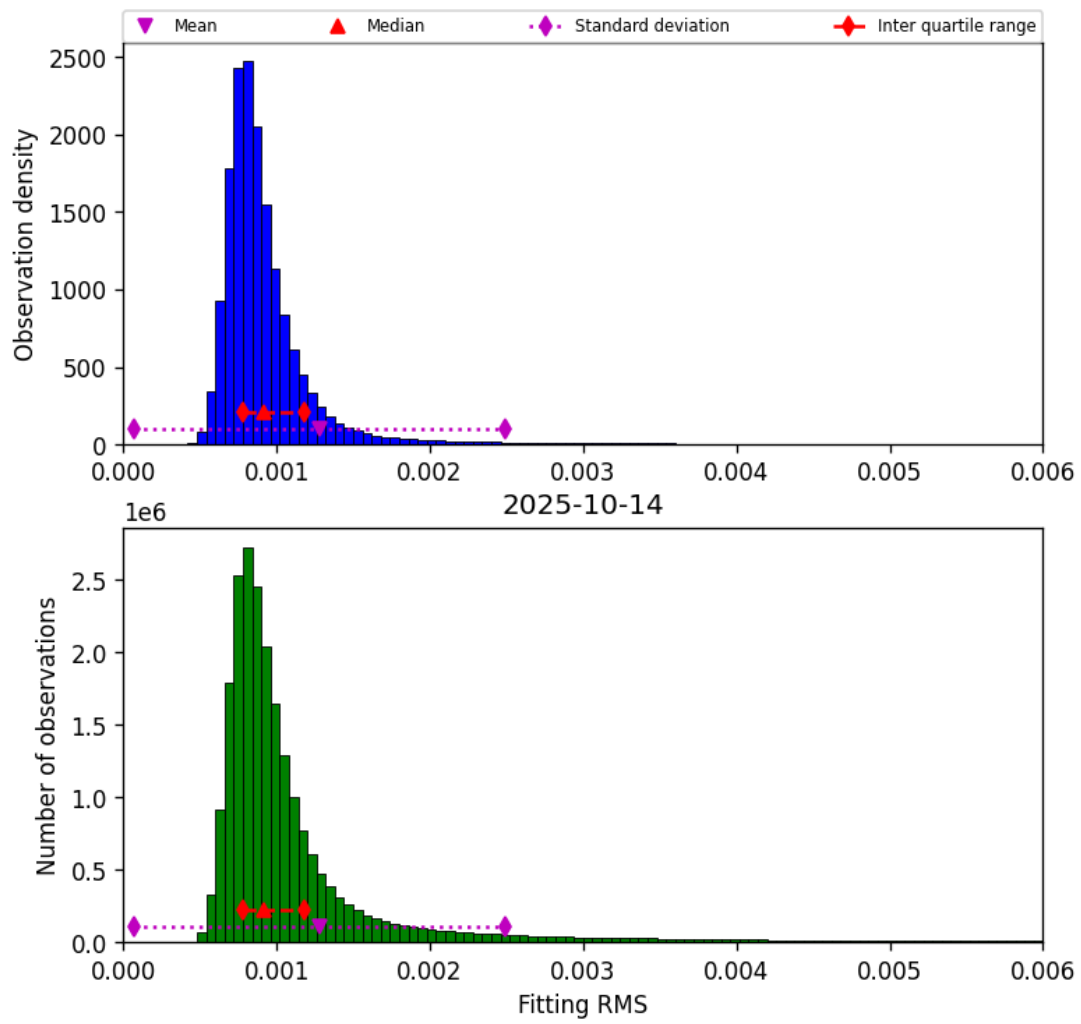
Figure 34: Histogram of “Fitting RMS” for 2025-10-14 to 2025-10-15
