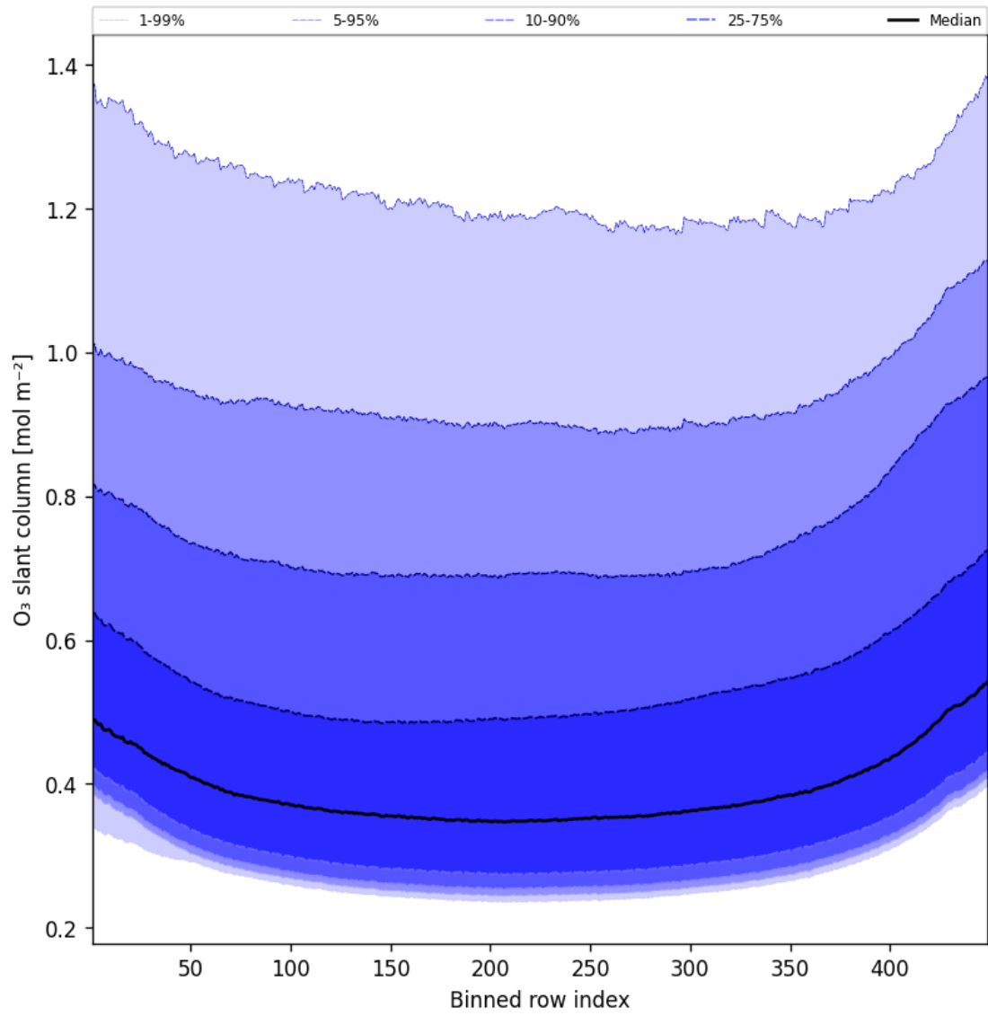
Figure 43: Along track statistics of “O 3 slant column” for 2025-10-14 to 2025-10-15
