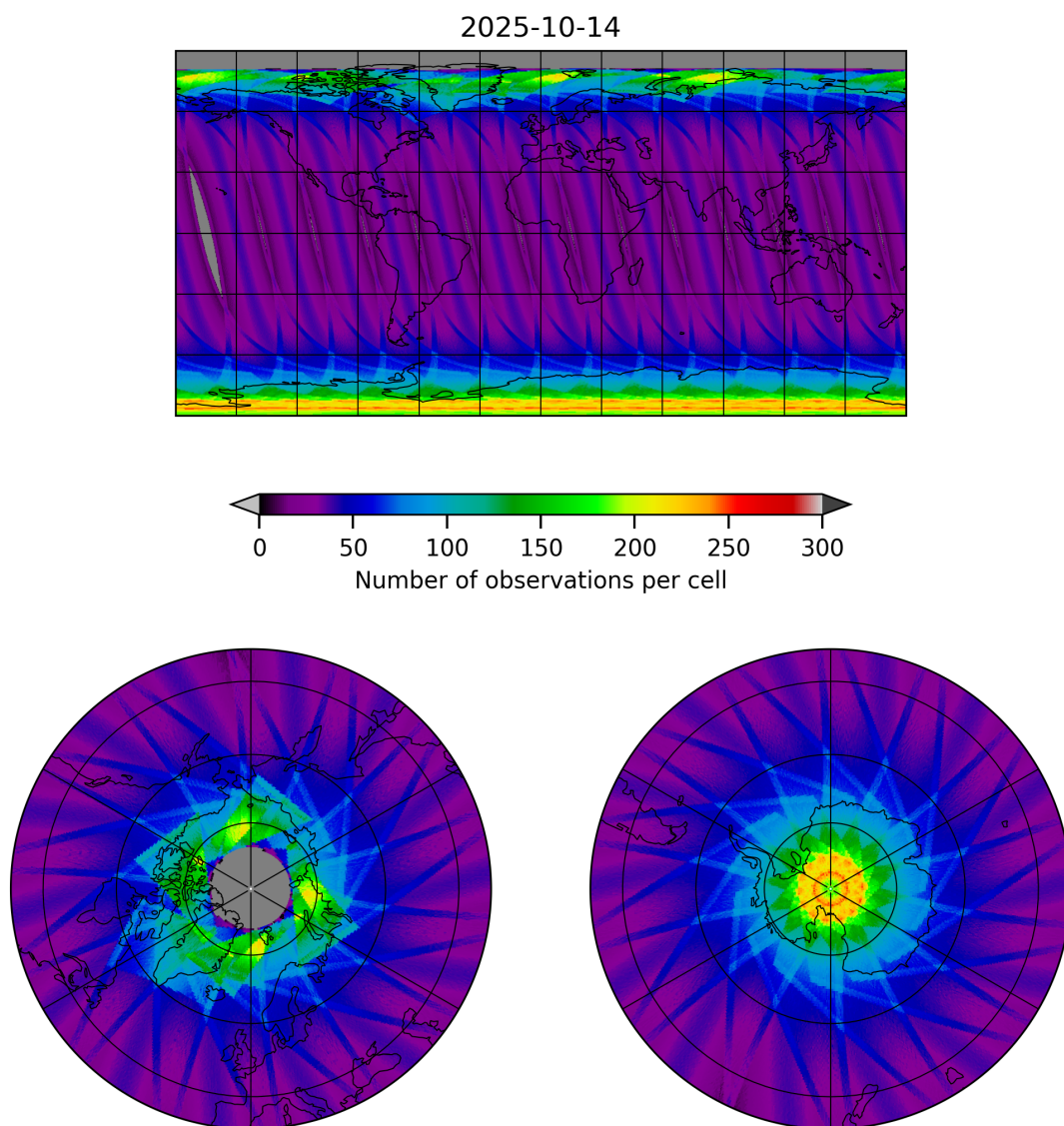
Figure 15: Map of the number of observations for 2025-10-14 to 2025-10-15
