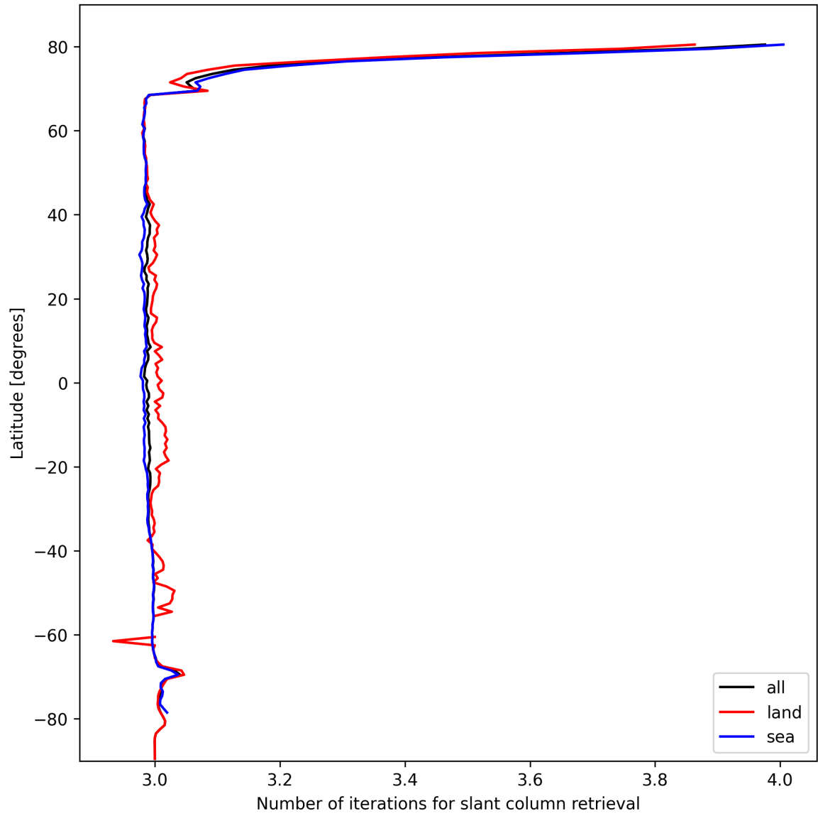
Figure 21: Zonal average of “Number of iterations for slant column retrieval” for 2025-10-14 to 2025-10-15.
