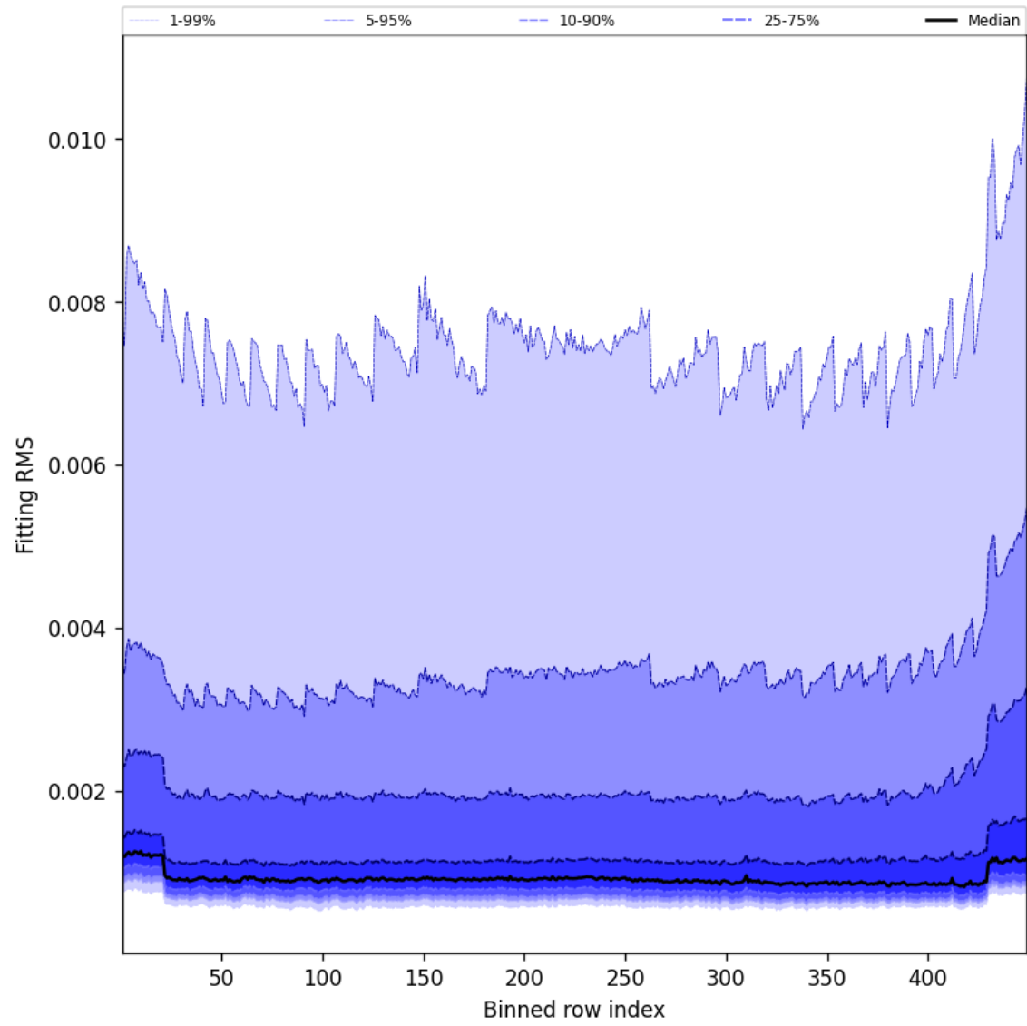
Figure 46: Along track statistics of “Fitting RMS” for 2025-10-14 to 2025-10-15
