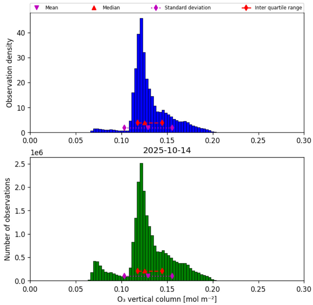
Figure 29: Histogram of “O 3 vertical column” for 2025-10-14 to 2025-10-15
