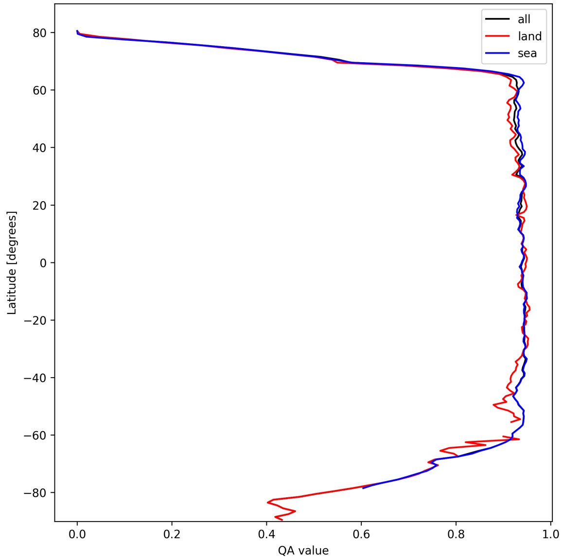
Figure 16: Zonal average of “QA value” for 2025-10-14 to 2025-10-15.
