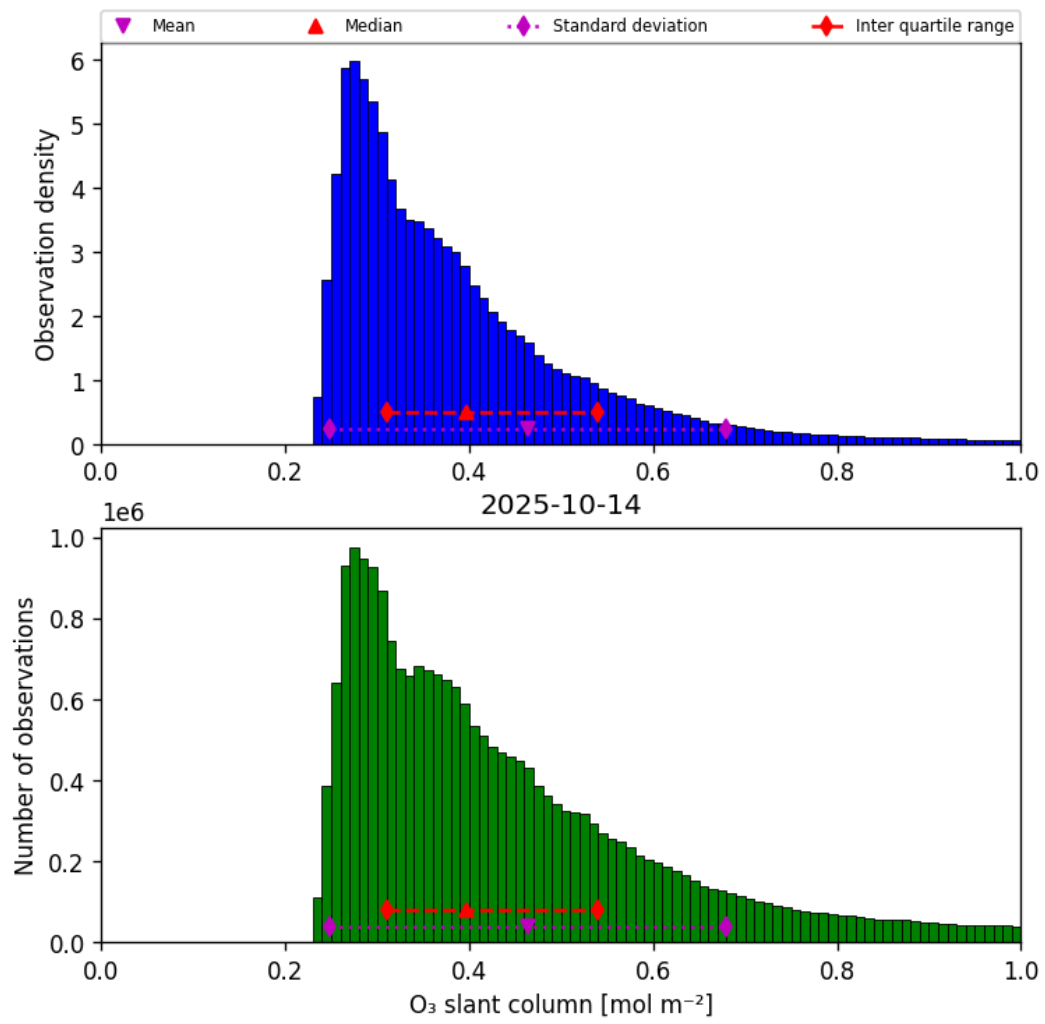
Figure 31: Histogram of “O 3 slant column” for 2025-10-14 to 2025-10-15
