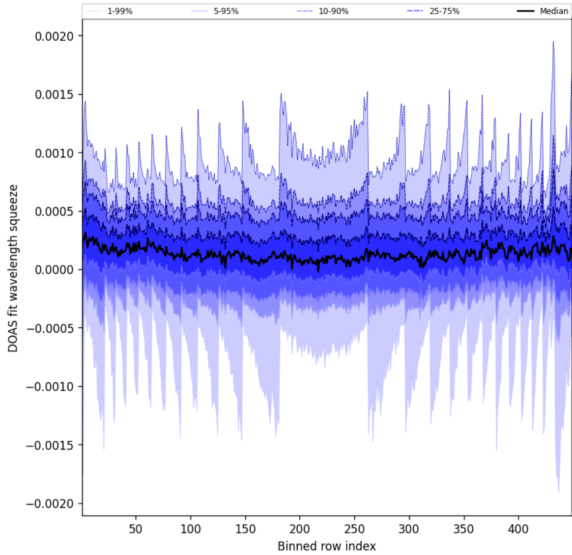
Figure 48: Along track statistics of “DOAS fit wavelength squeeze” for 2025-10-14 to 2025-10-15
