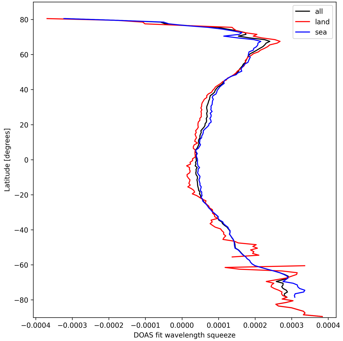
Figure 24: Zonal average of “DOAS fit wavelength squeeze” for 2025-10-14 to 2025-10-15.
