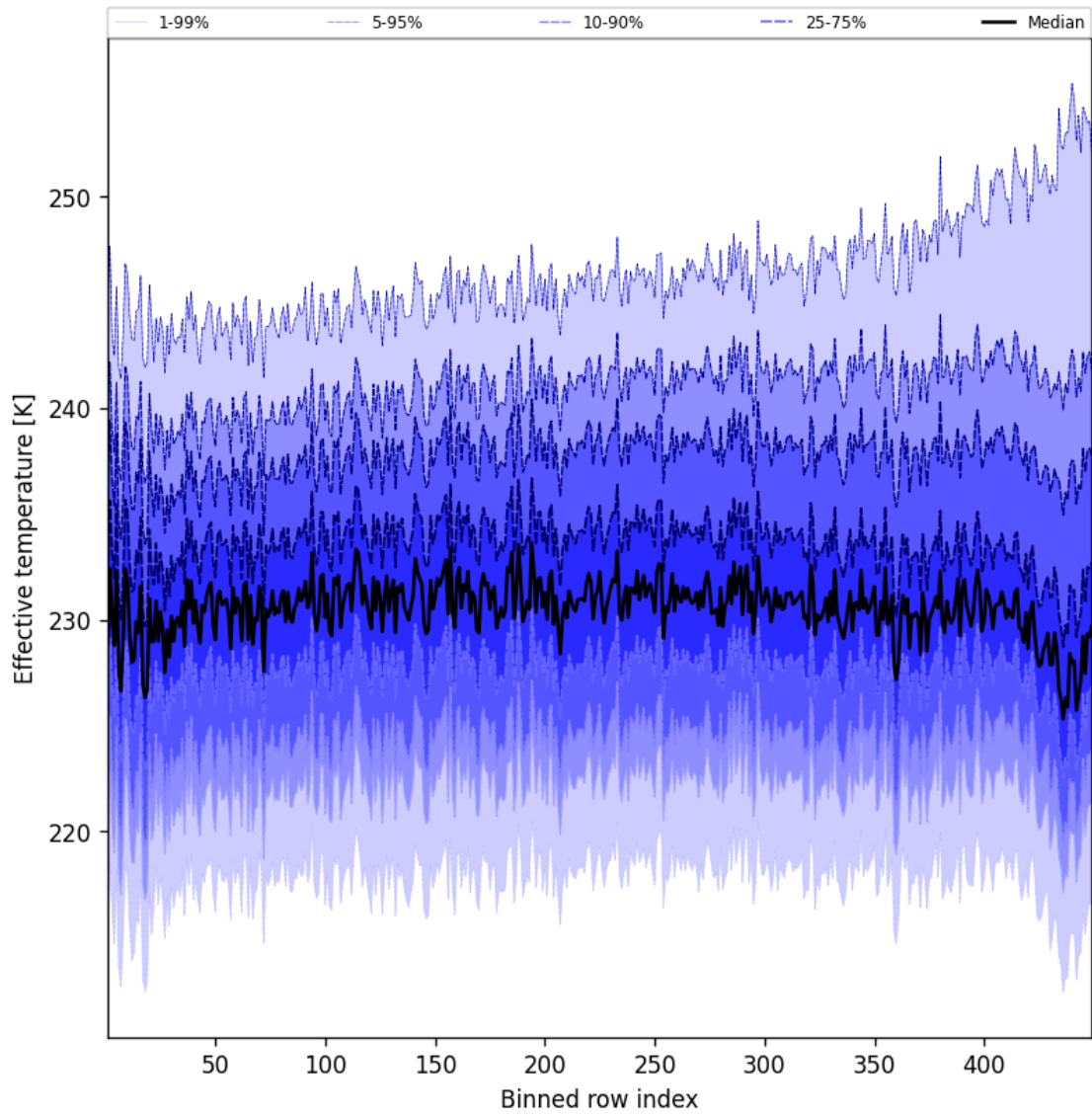
Figure 50: Along track statistics of “Effective temperature” for 2025-10-14 to 2025-10-15
