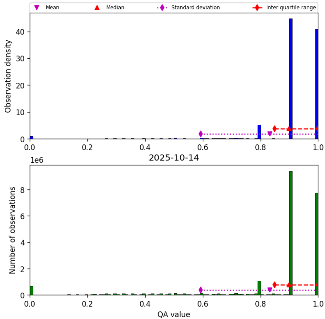
Figure 28: Histogram of “QA value” for 2025-10-14 to 2025-10-15
