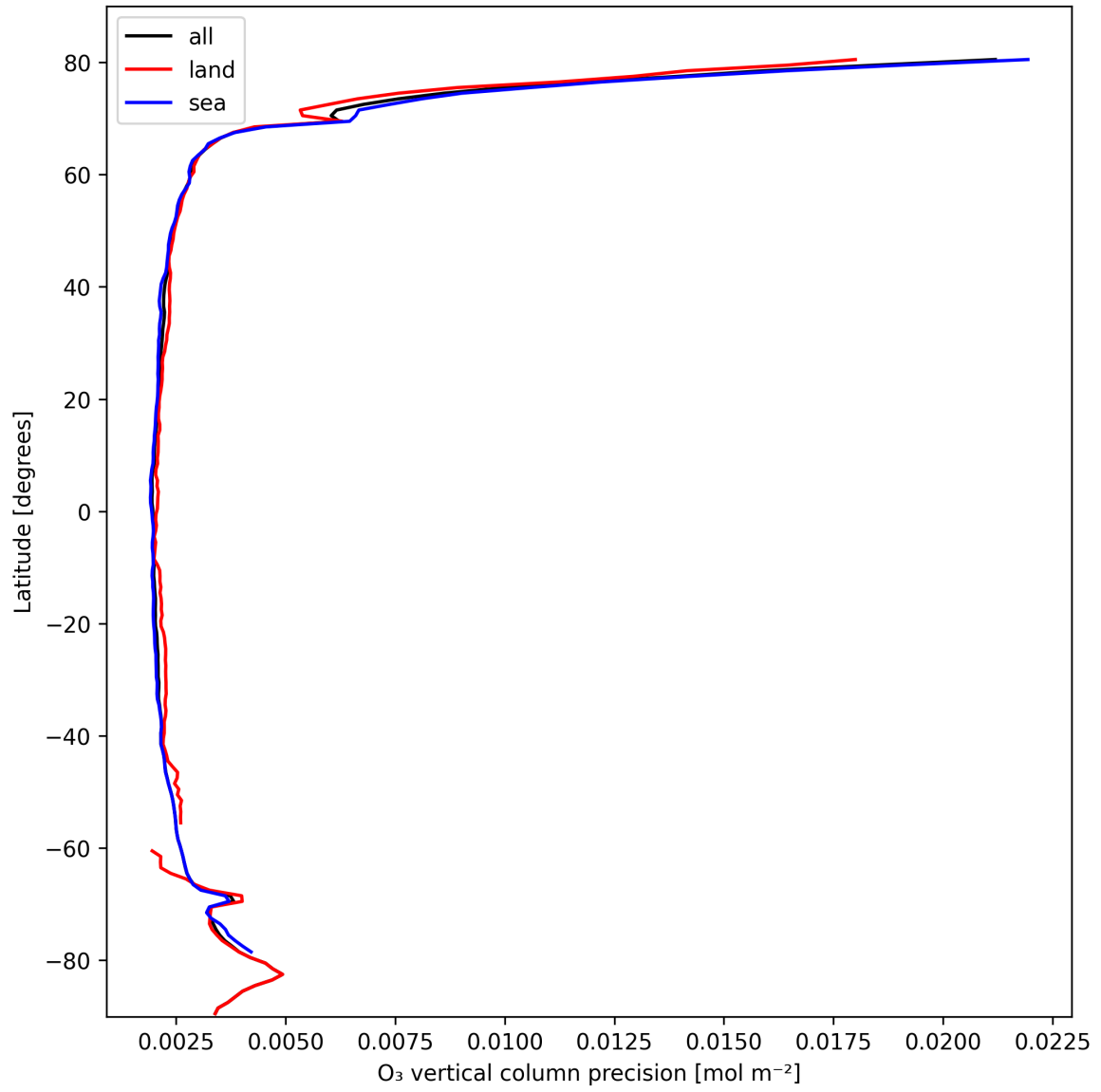
Figure 18: Zonal average of “O 3 vertical column precision” for 2025-10-14 to 2025-10-15.
