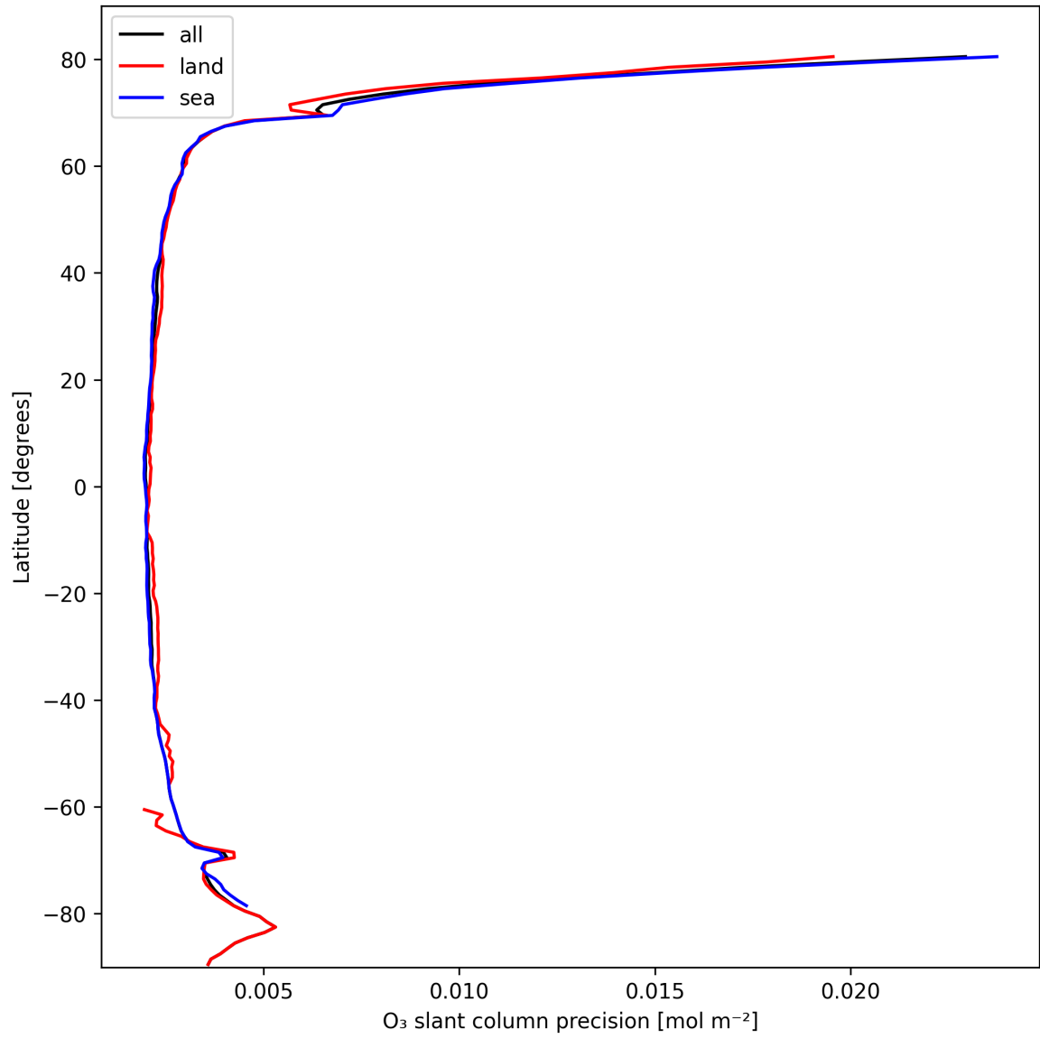
Figure 20: Zonal average of “O 3 slant column precision” for 2025-10-14 to 2025-10-15.
