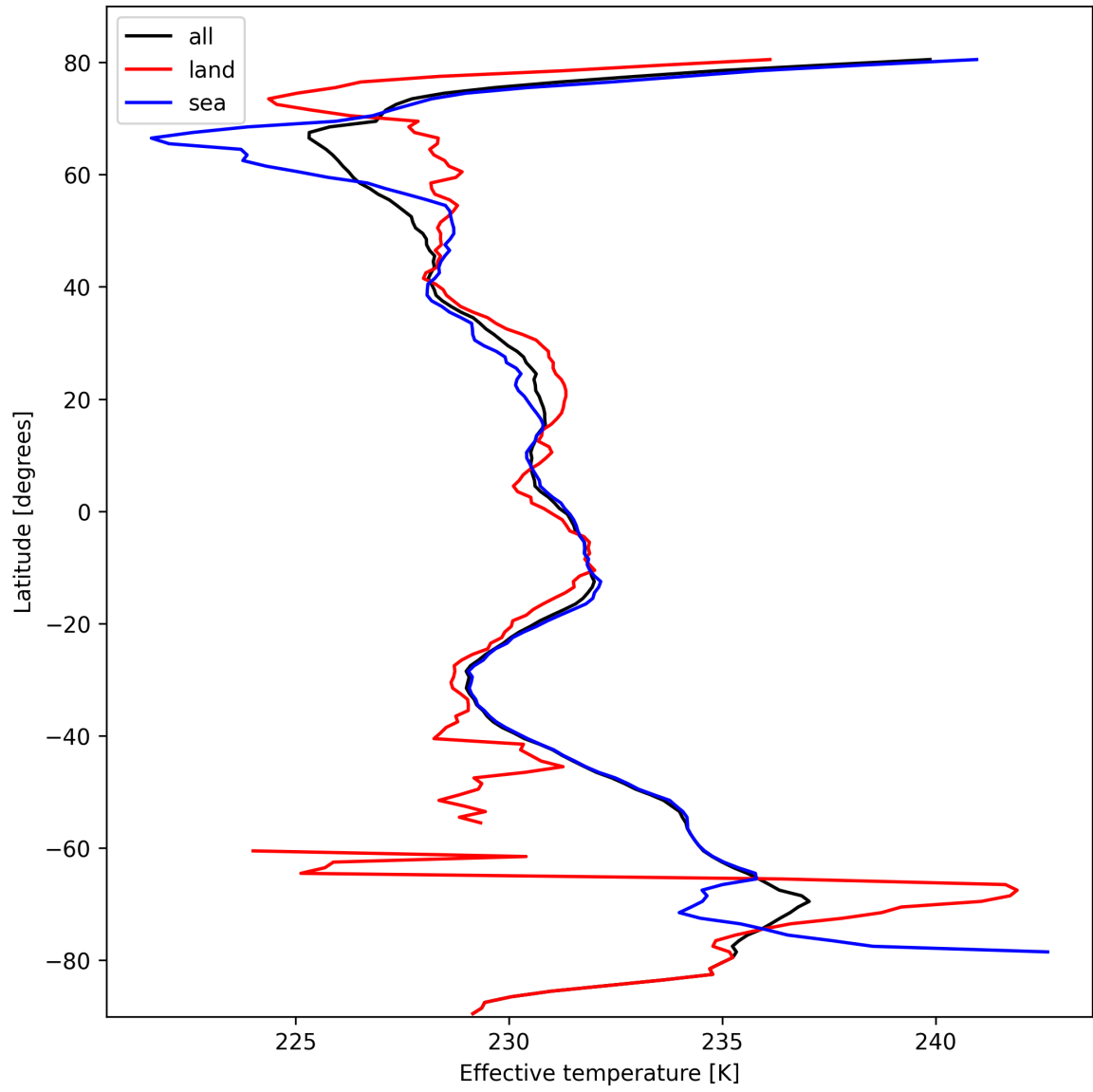
Figure 26: Zonal average of “Effective temperature” for 2025-10-15 to 2025-10-15.
