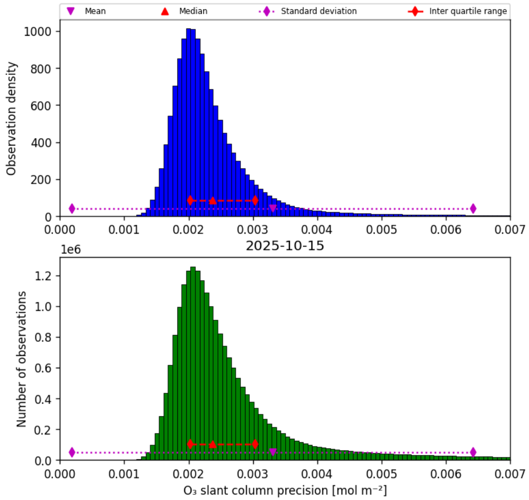
Figure 32: Histogram of “O 3 slant column precision” for 2025-10-15 to 2025-10-15
