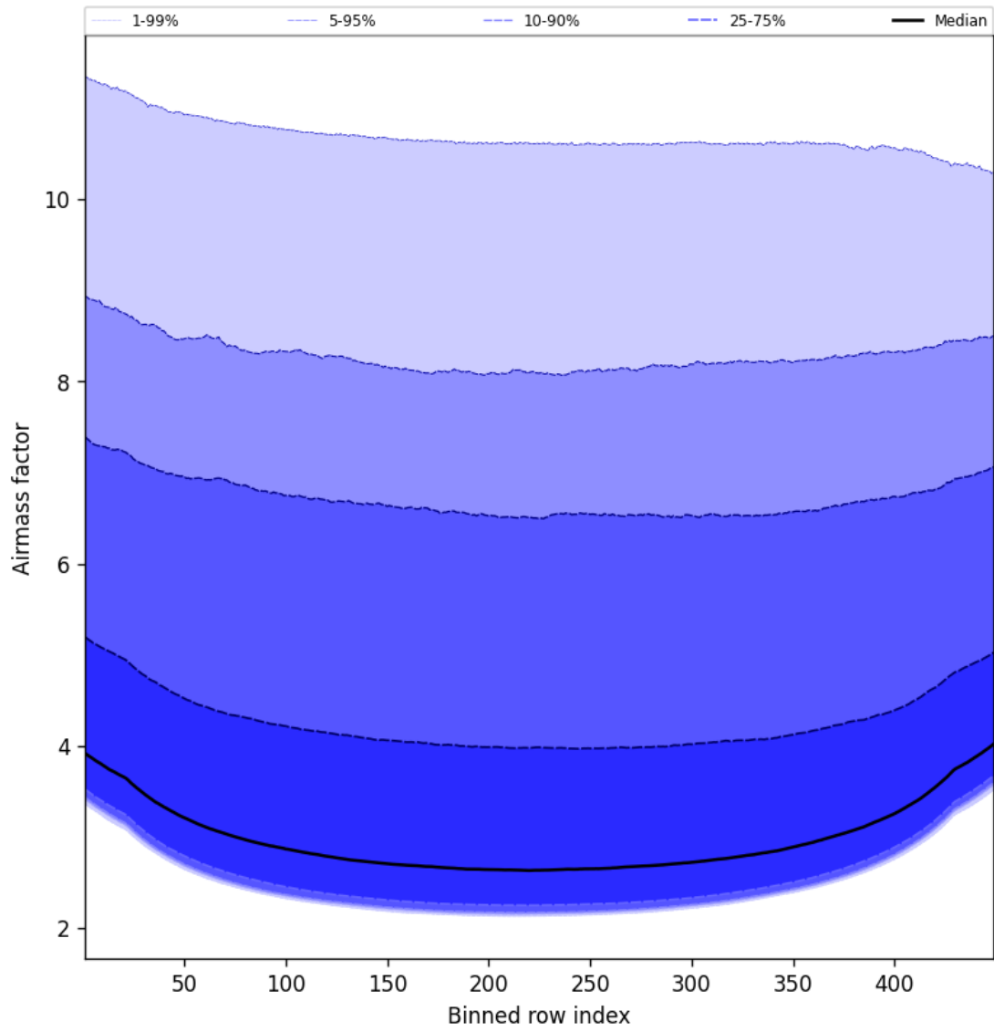
Figure 49: Along track statistics of “Airmass factor” for 2025-10-15 to 2025-10-15
