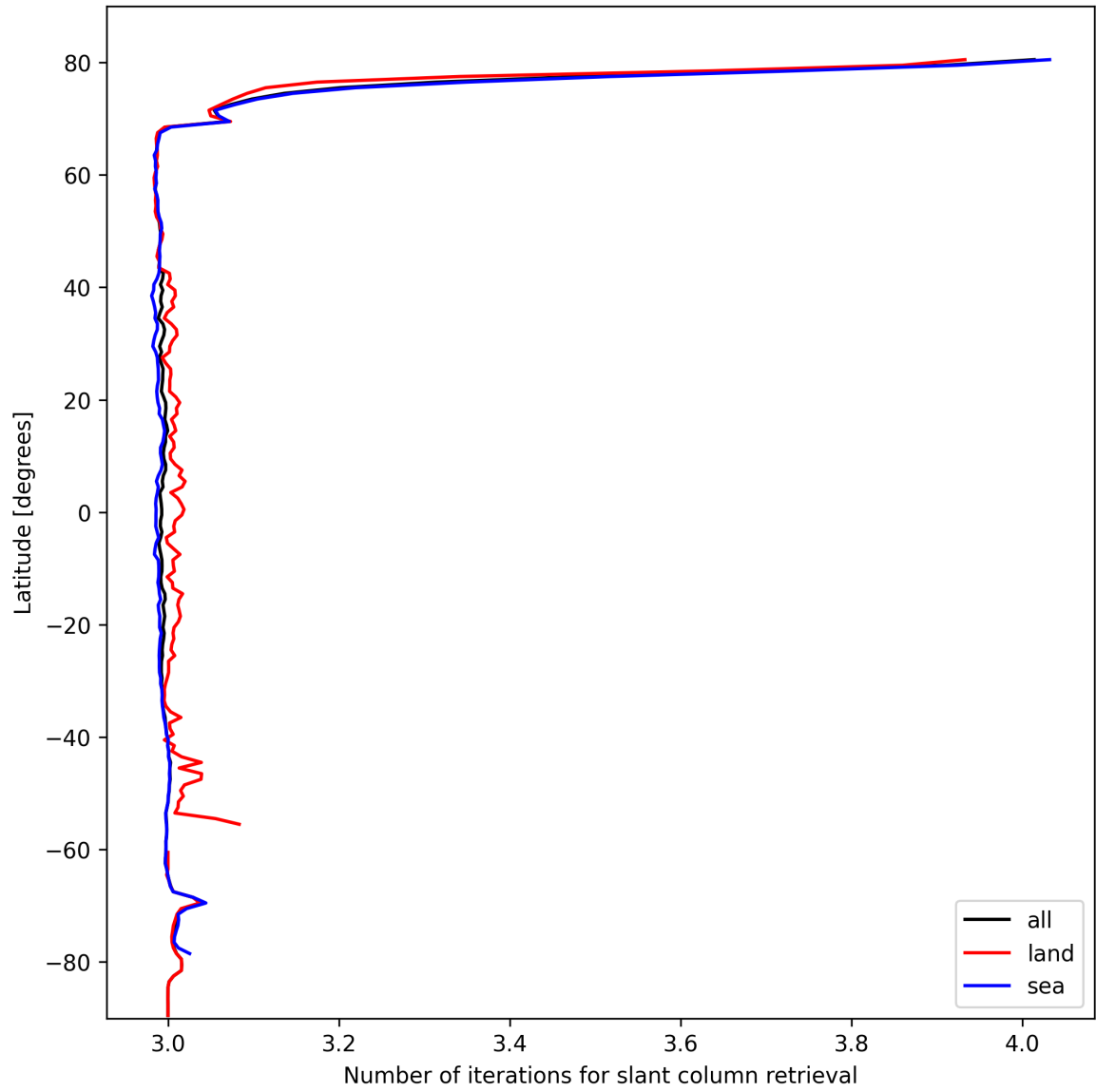
Figure 21: Zonal average of “Number of iterations for slant column retrieval” for 2025-10-15 to 2025-10-15.
