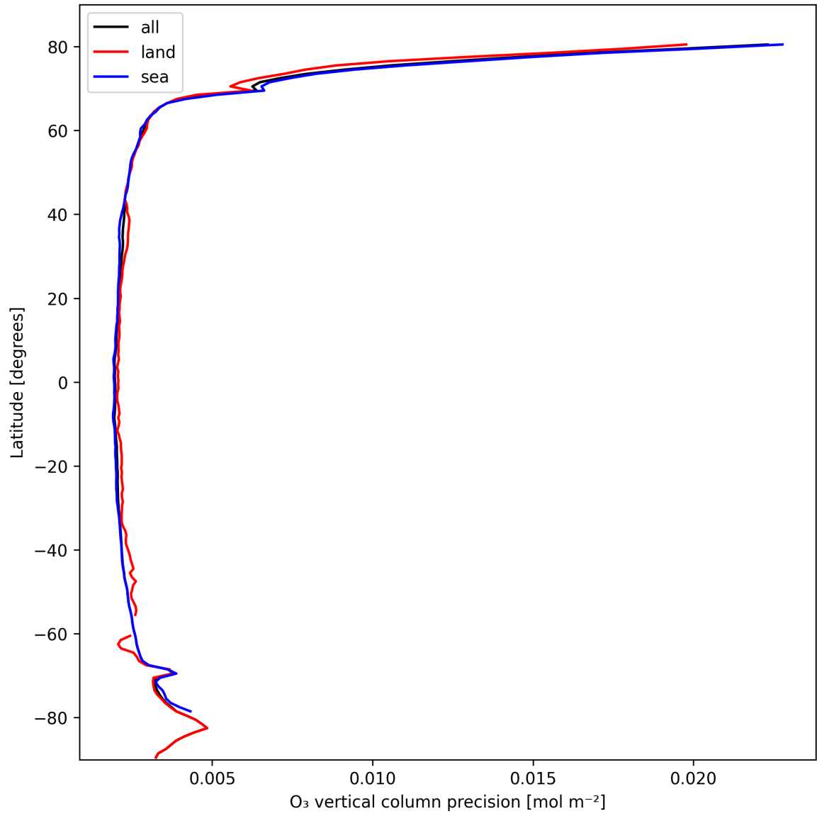
Figure 18: Zonal average of “O 3 vertical column precision” for 2025-10-15 to 2025-10-15.
