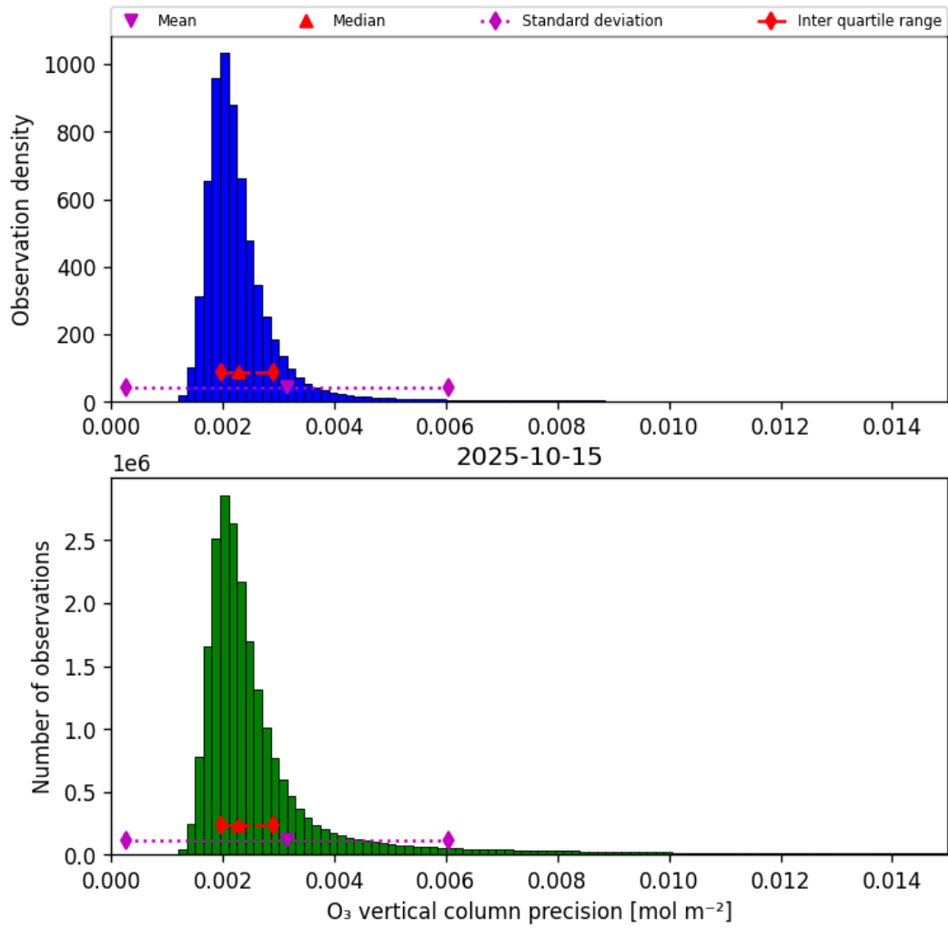
Figure 30: Histogram of “O 3 vertical column precision” for 2025-10-15 to 2025-10-15
