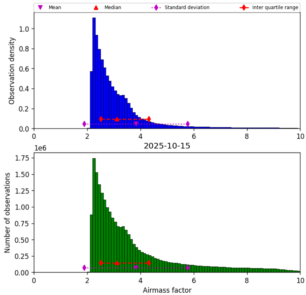
Figure 37: Histogram of “Airmass factor” for 2025-10-15 to 2025-10-15
