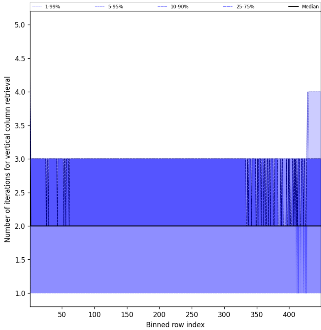
Figure 51: Along track statistics of “Number of iterations for vertical column retrieval” for 2025-10-15 to 2025-10-15
