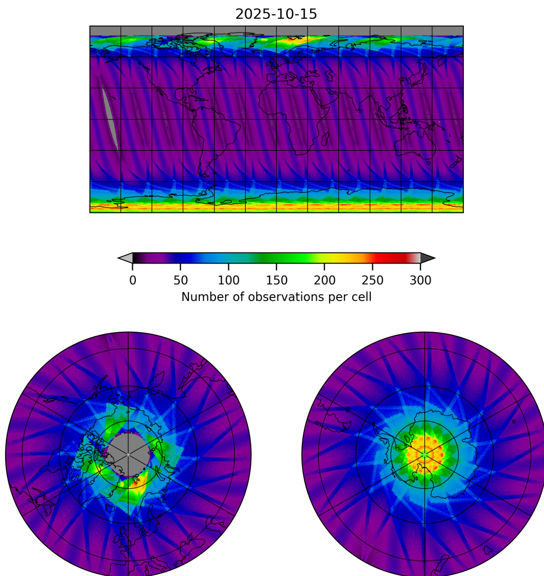
Figure 15: Map of the number of observations for 2025-10-15 to 2025-10-15
