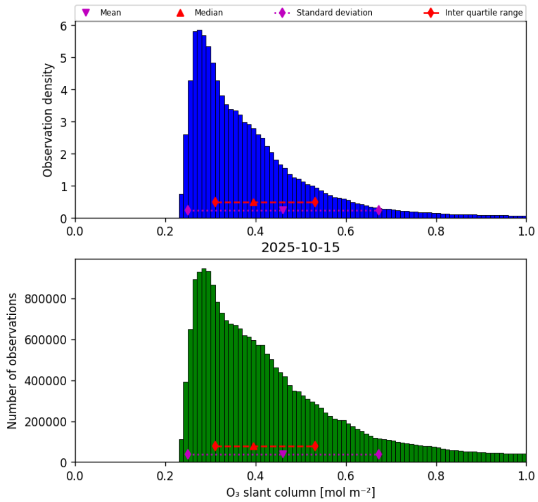
Figure 31: Histogram of “O 3 slant column” for 2025-10-15 to 2025-10-15
