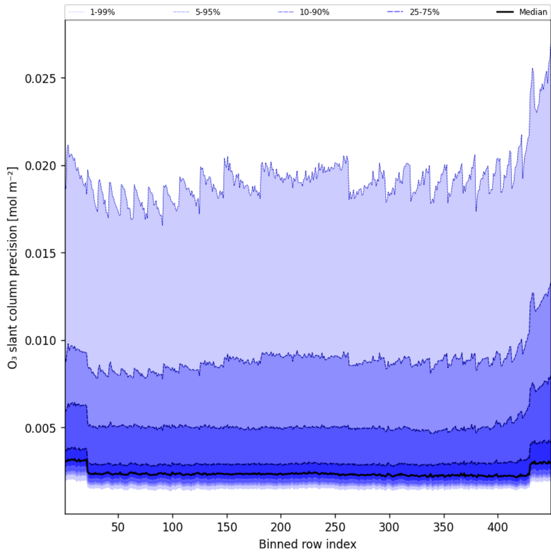
Figure 44: Along track statistics of “O 3 slant column precision” for 2025-10-15 to 2025-10-15
