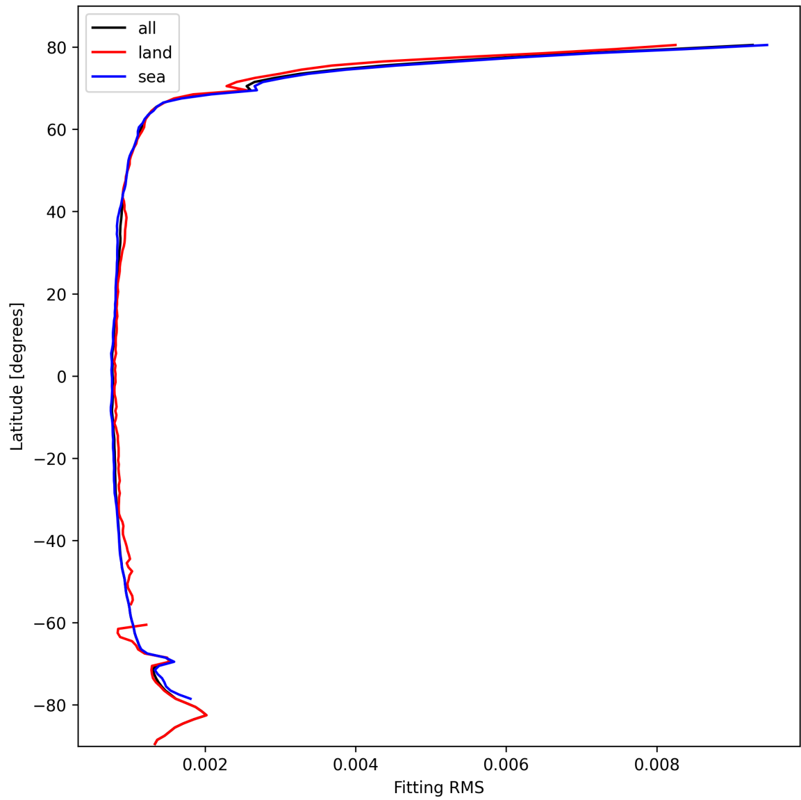
Figure 22: Zonal average of “Fitting RMS” for 2025-10-15 to 2025-10-15.
