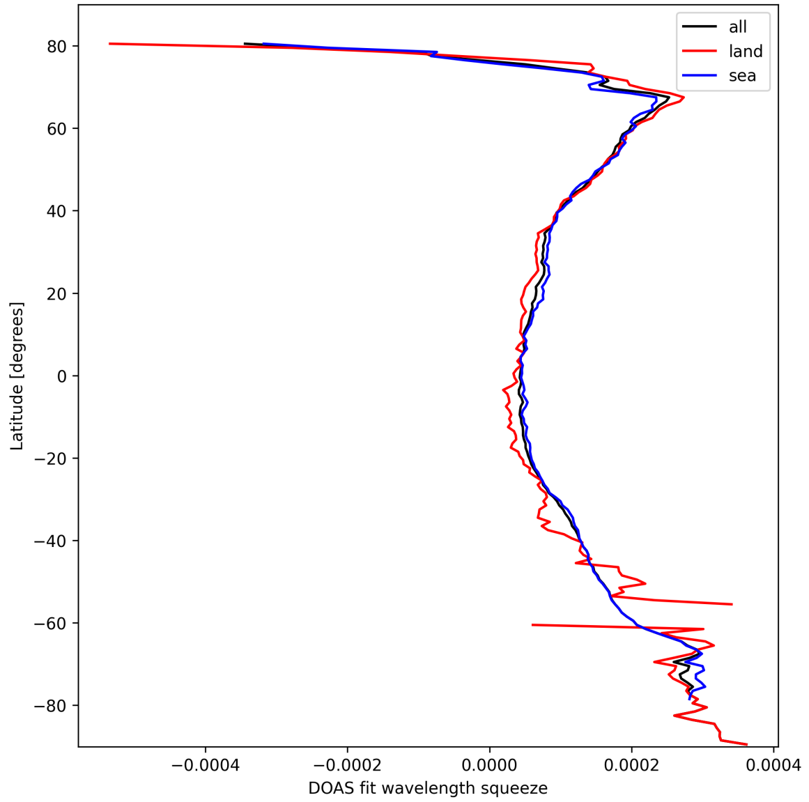
Figure 24: Zonal average of “DOAS fit wavelength squeeze” for 2025-10-15 to 2025-10-15.
