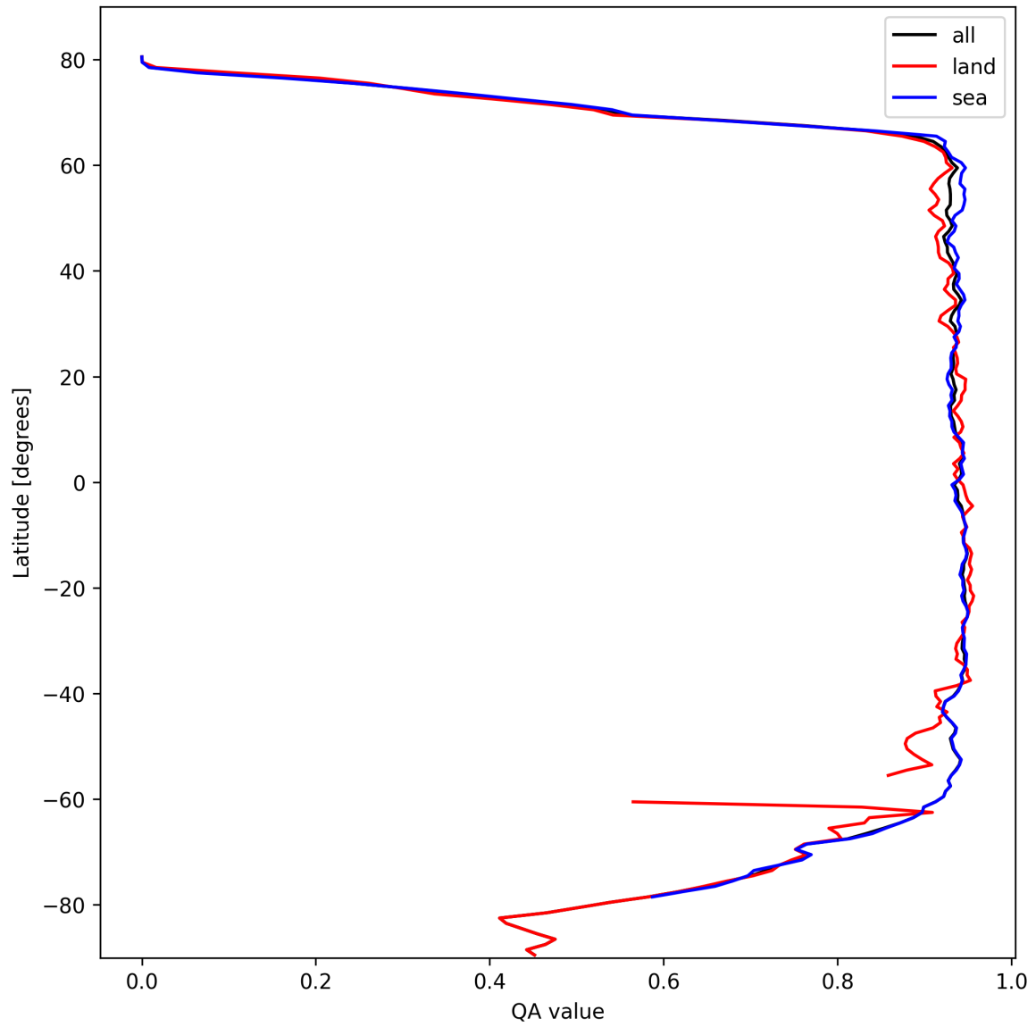
Figure 16: Zonal average of “QA value” for 2025-10-15 to 2025-10-15.
