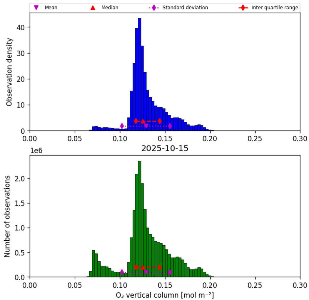
Figure 29: Histogram of “O 3 vertical column” for 2025-10-15 to 2025-10-15
