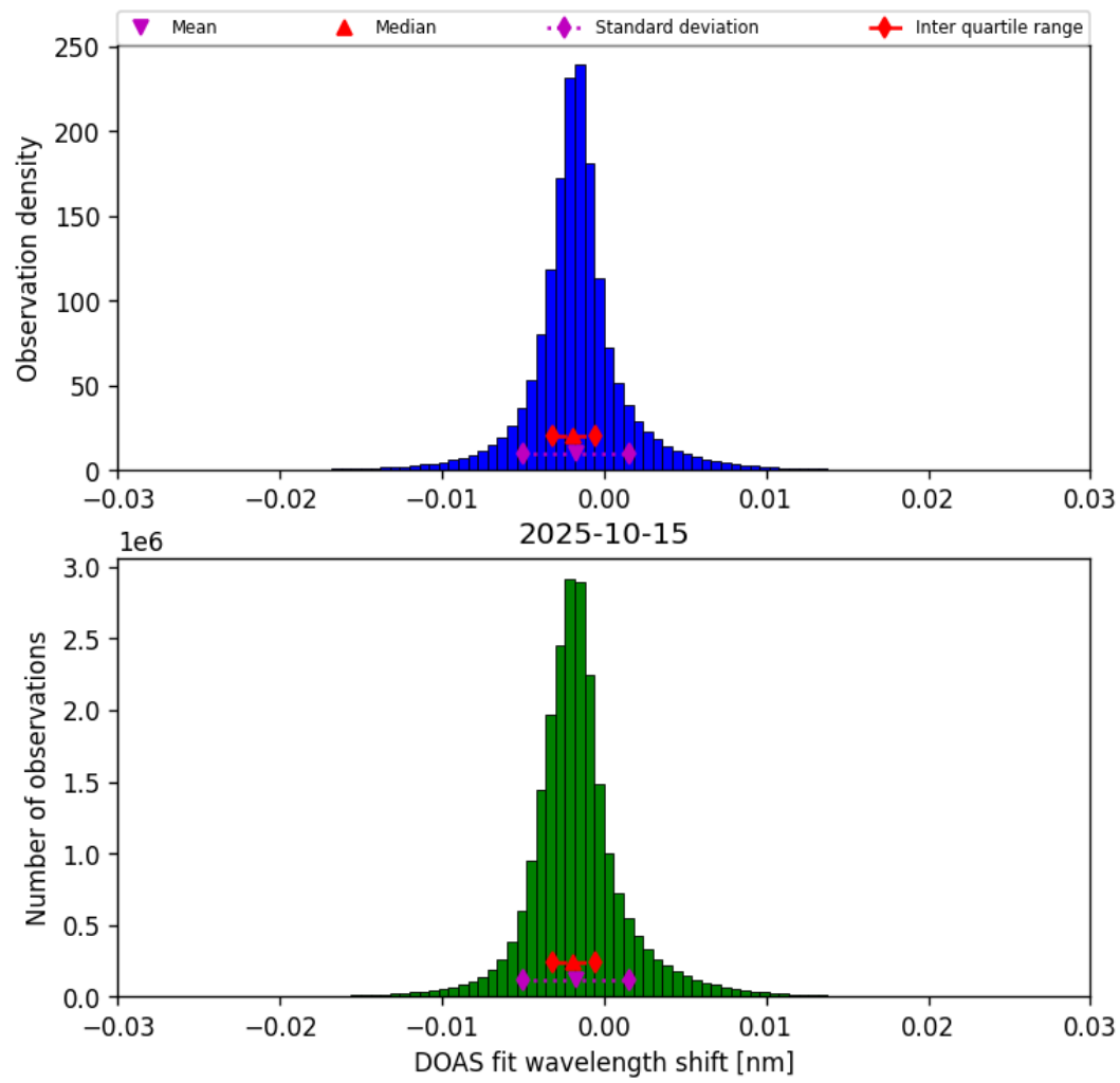
Figure 35: Histogram of “DOAS fit wavelength shift” for 2025-10-15 to 2025-10-15
