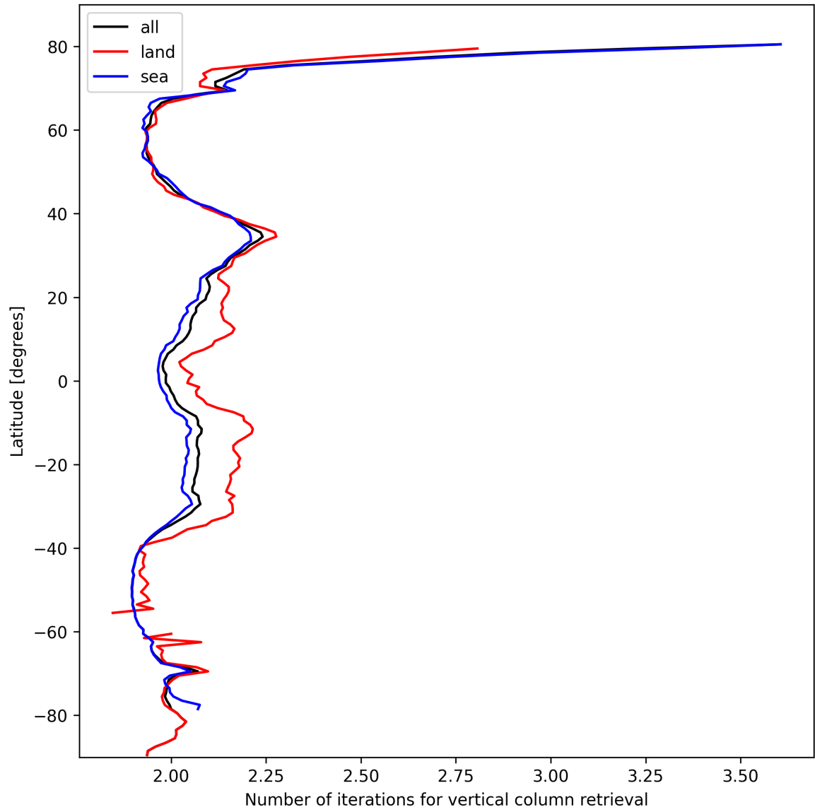
Figure 27: Zonal average of “Number of iterations for vertical column retrieval” for 2025-10-16 to 2025-10-17.
