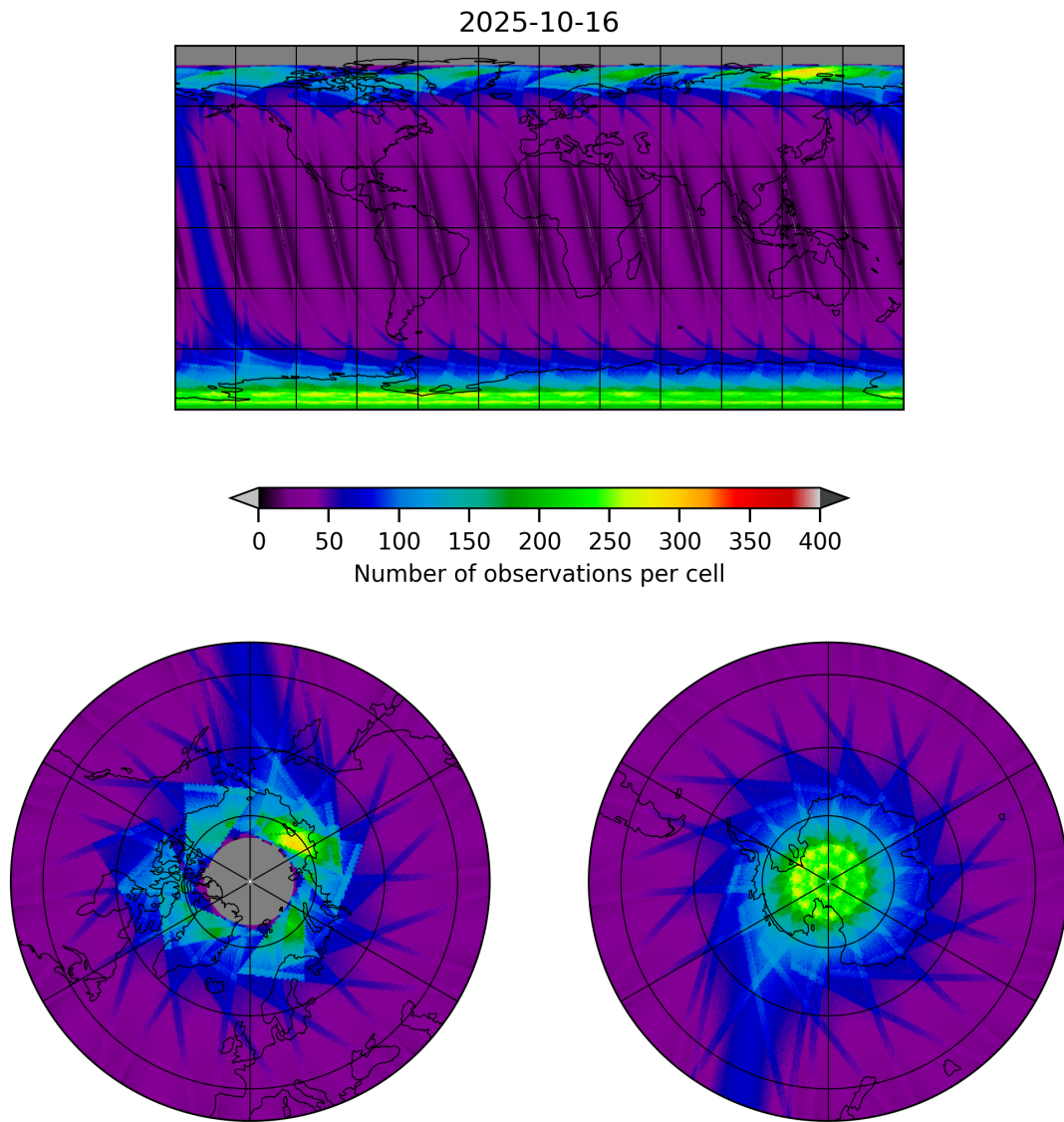
Figure 15: Map of the number of observations for 2025-10-16 to 2025-10-17
