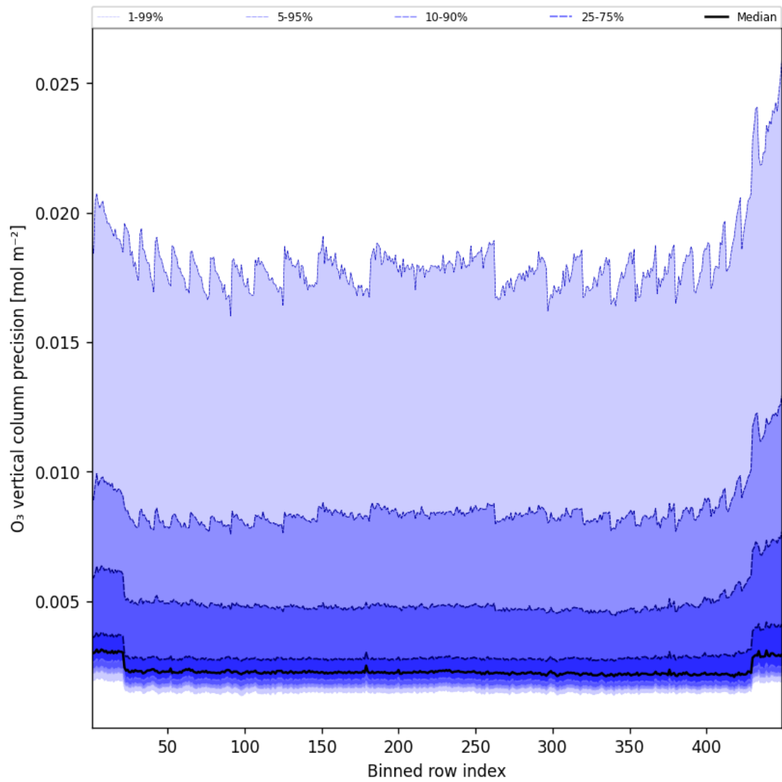
Figure 42: Along track statistics of “O 3 vertical column precision” for 2025-10-16 to 2025-10-17
