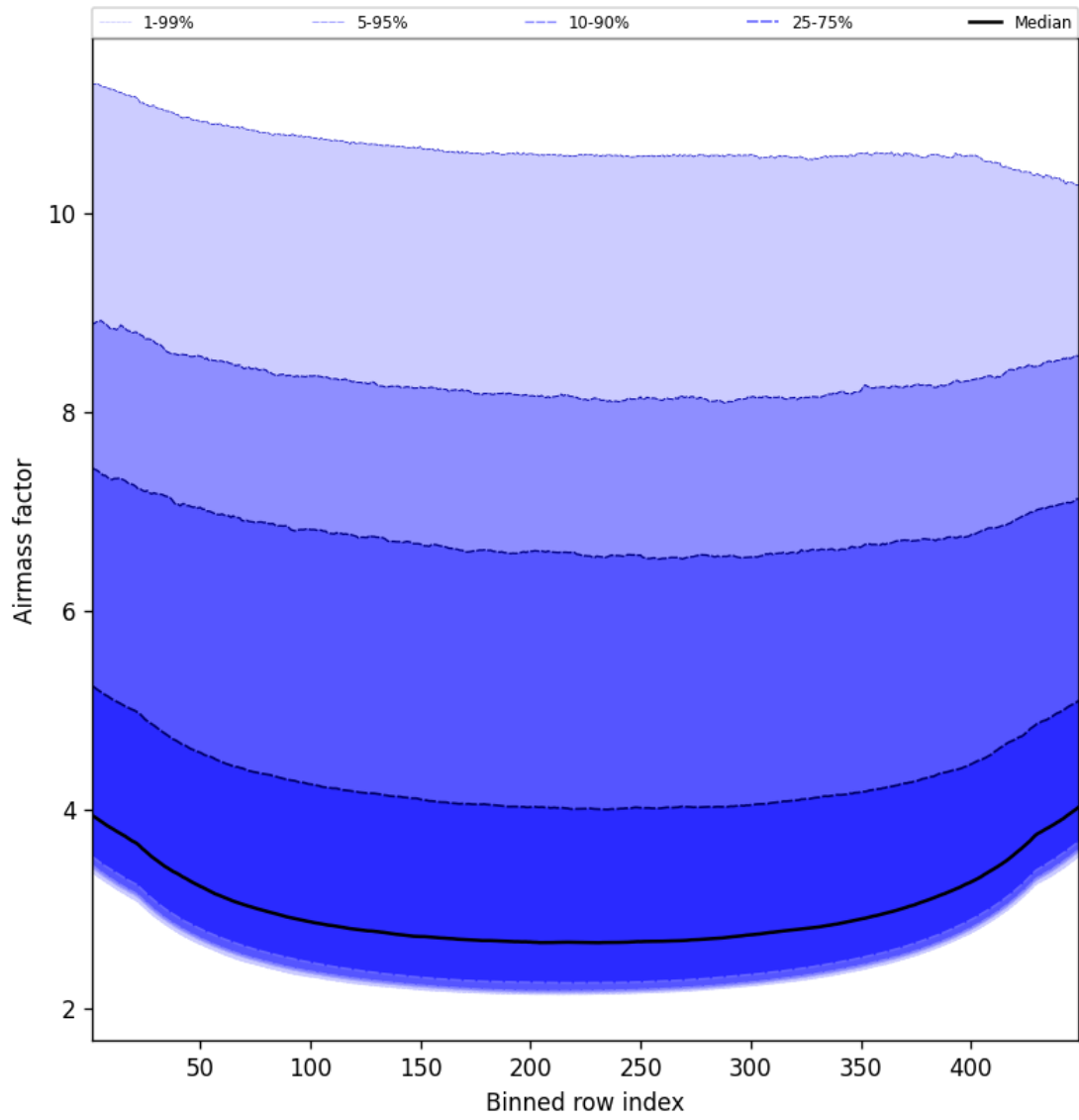
Figure 49: Along track statistics of “Airmass factor” for 2025-10-16 to 2025-10-17
