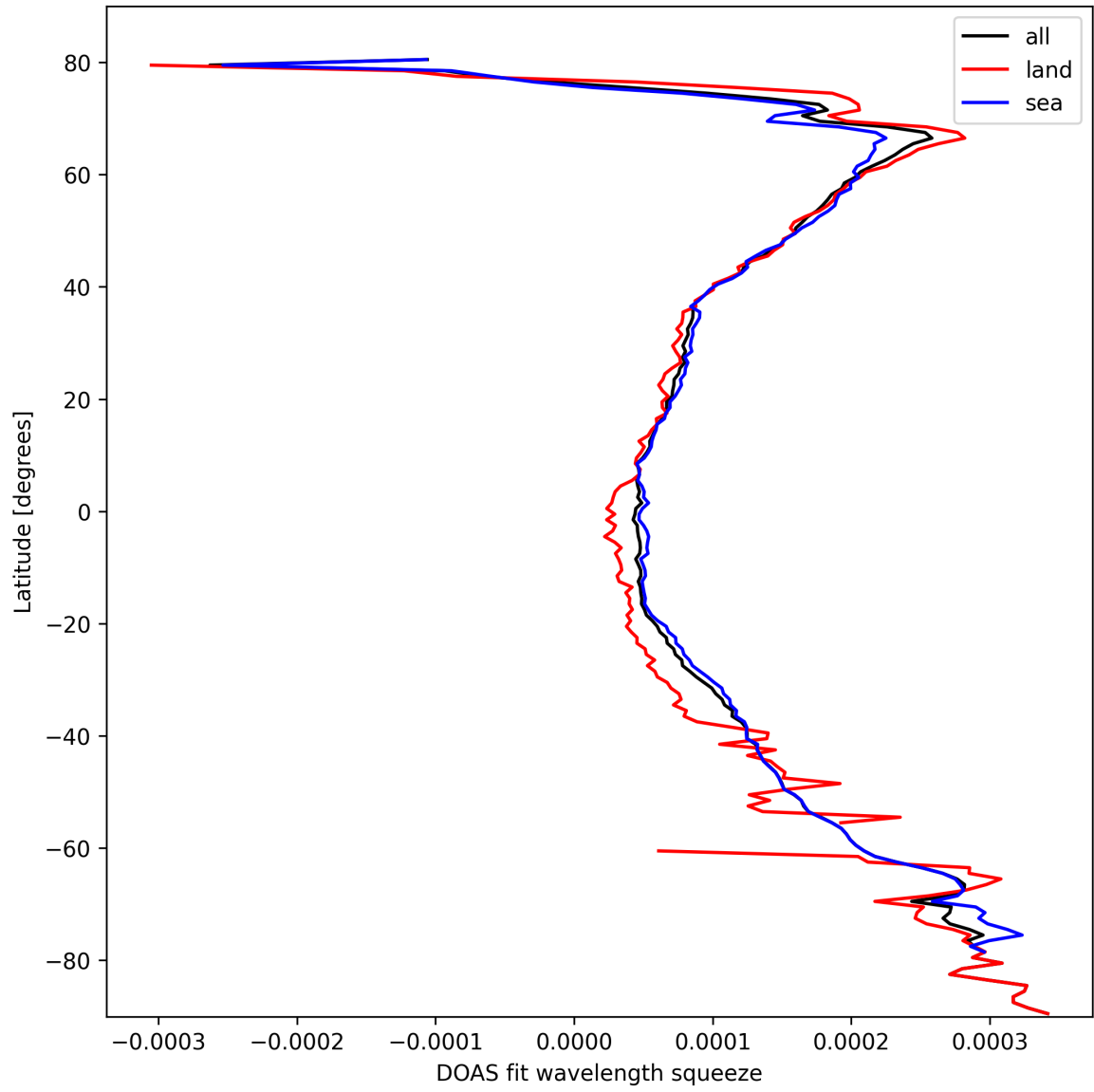
Figure 24: Zonal average of “DOAS fit wavelength squeeze” for 2025-10-16 to 2025-10-17.
