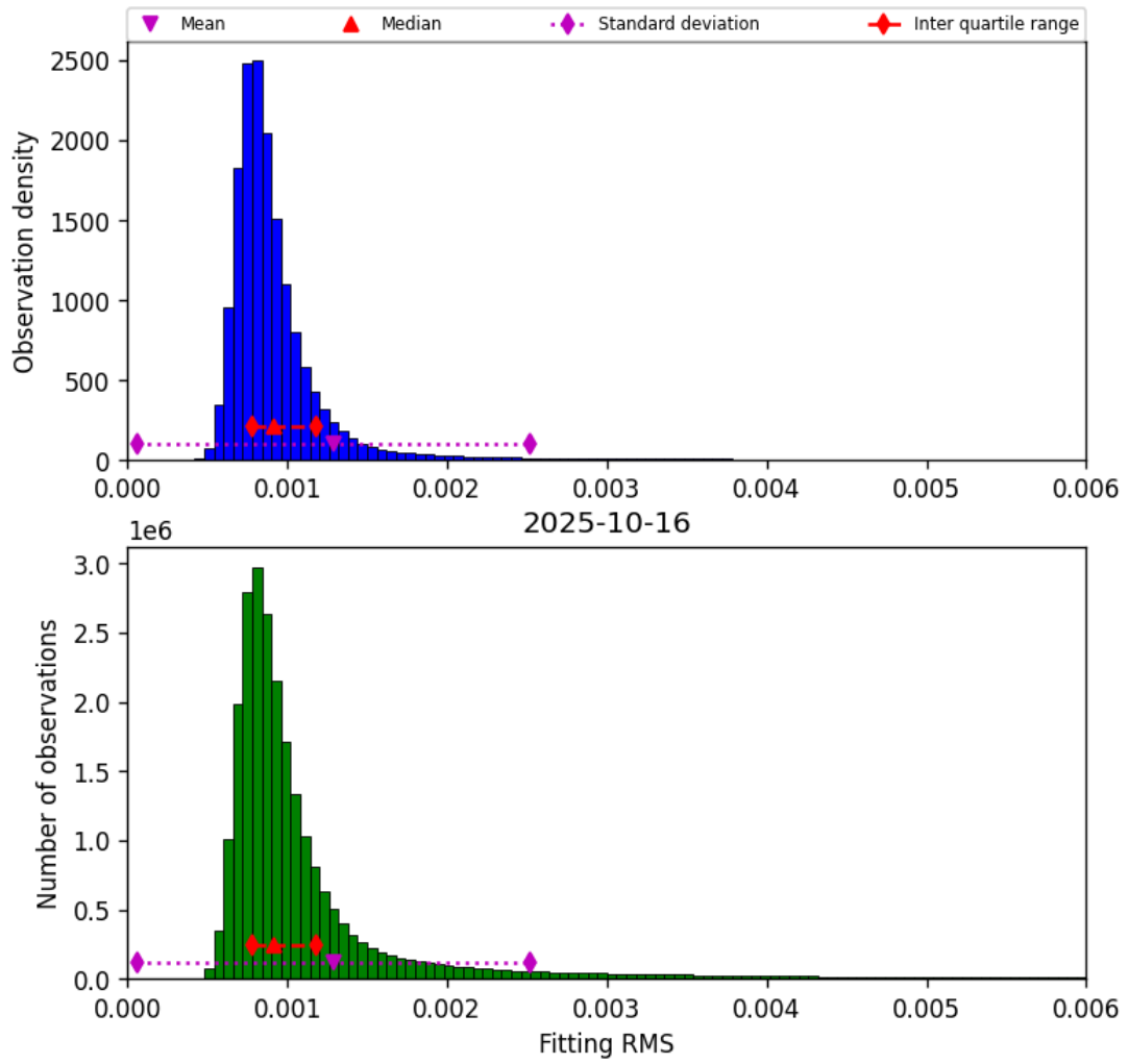
Figure 34: Histogram of “Fitting RMS” for 2025-10-16 to 2025-10-17
