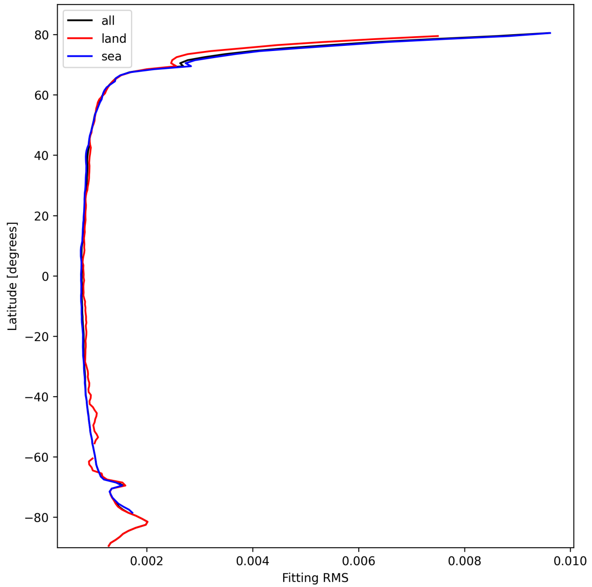
Figure 22: Zonal average of “Fitting RMS” for 2025-10-16 to 2025-10-17.
