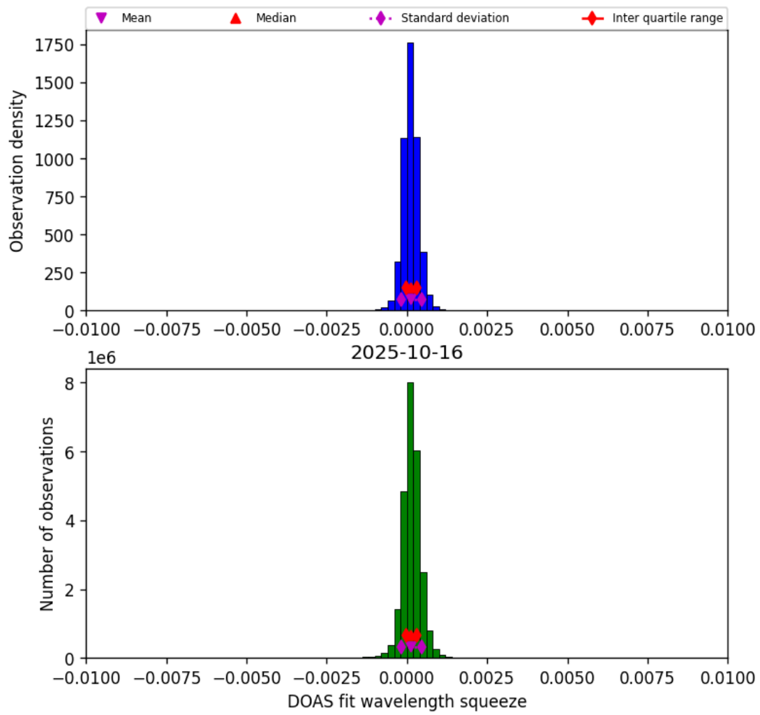
Figure 36: Histogram of “DOAS fit wavelength squeeze” for 2025-10-16 to 2025-10-17
