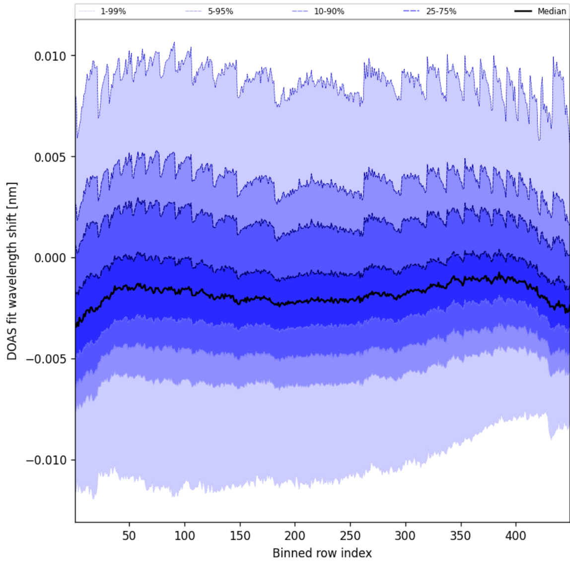
Figure 47: Along track statistics of “DOAS fit wavelength shift” for 2025-10-16 to 2025-10-17
