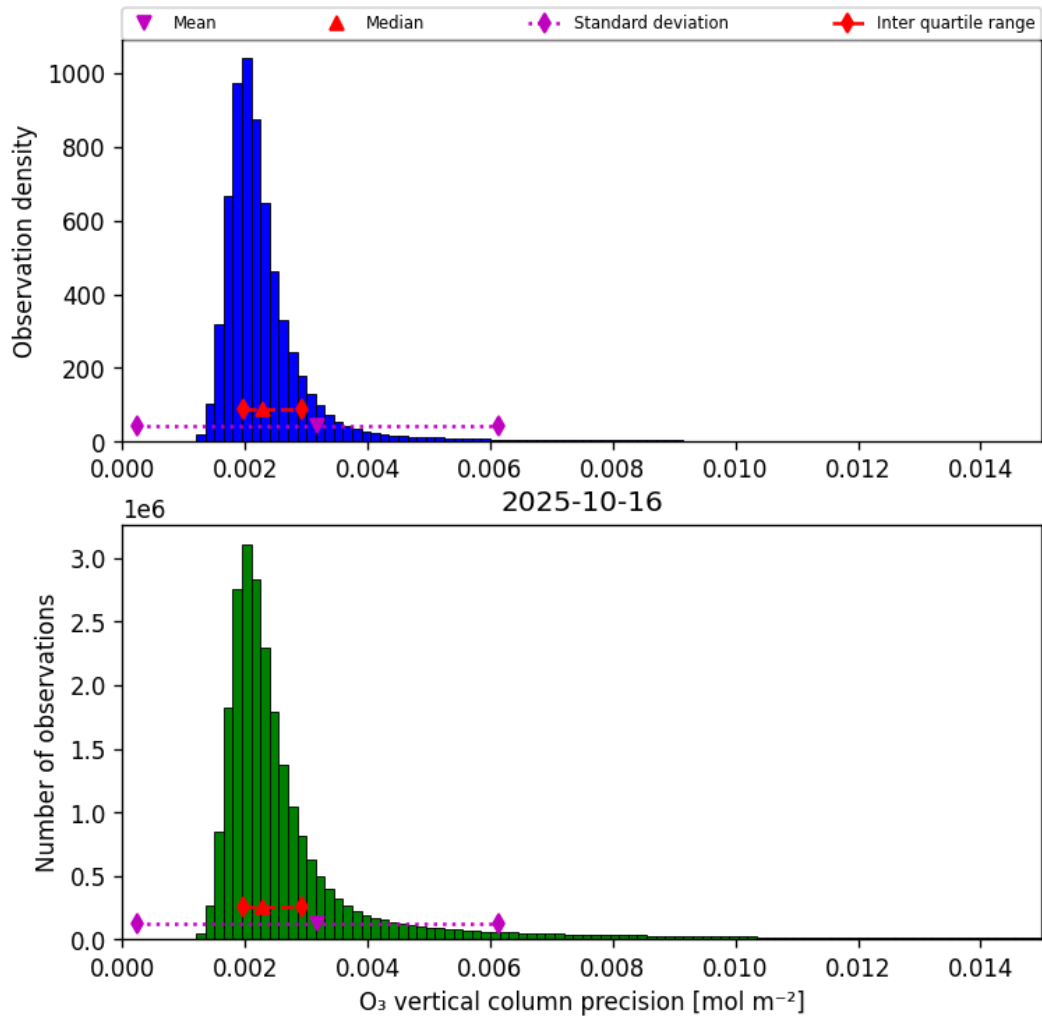
Figure 30: Histogram of “O 3 vertical column precision” for 2025-10-16 to 2025-10-17
