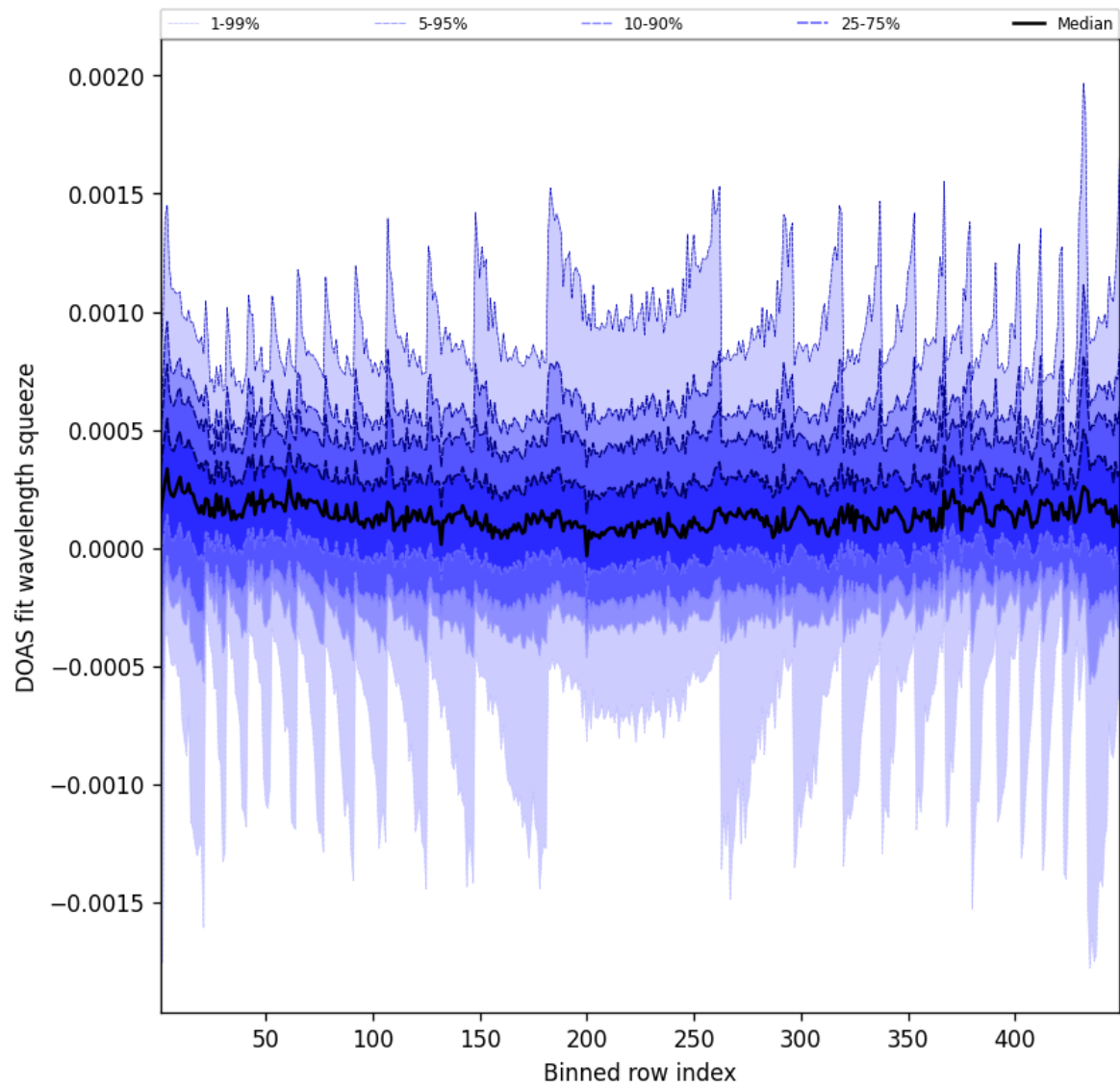
Figure 48: Along track statistics of “DOAS fit wavelength squeeze” for 2025-10-16 to 2025-10-17
