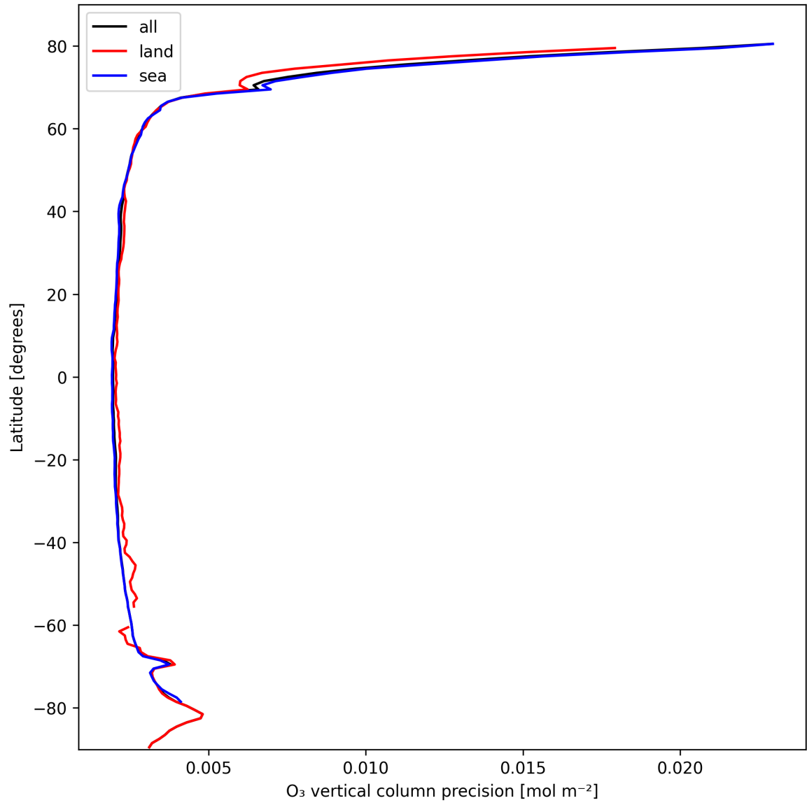
Figure 18: Zonal average of “O 3 vertical column precision” for 2025-10-16 to 2025-10-17.
