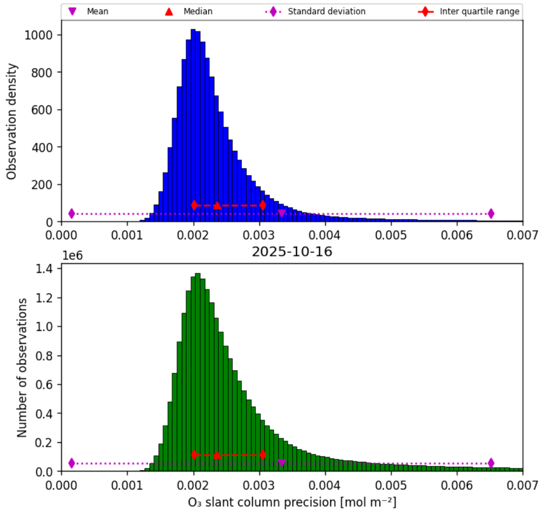
Figure 32: Histogram of “O 3 slant column precision” for 2025-10-16 to 2025-10-17
