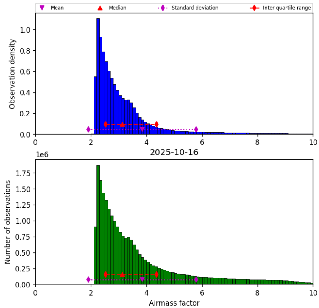
Figure 37: Histogram of “Airmass factor” for 2025-10-16 to 2025-10-17
