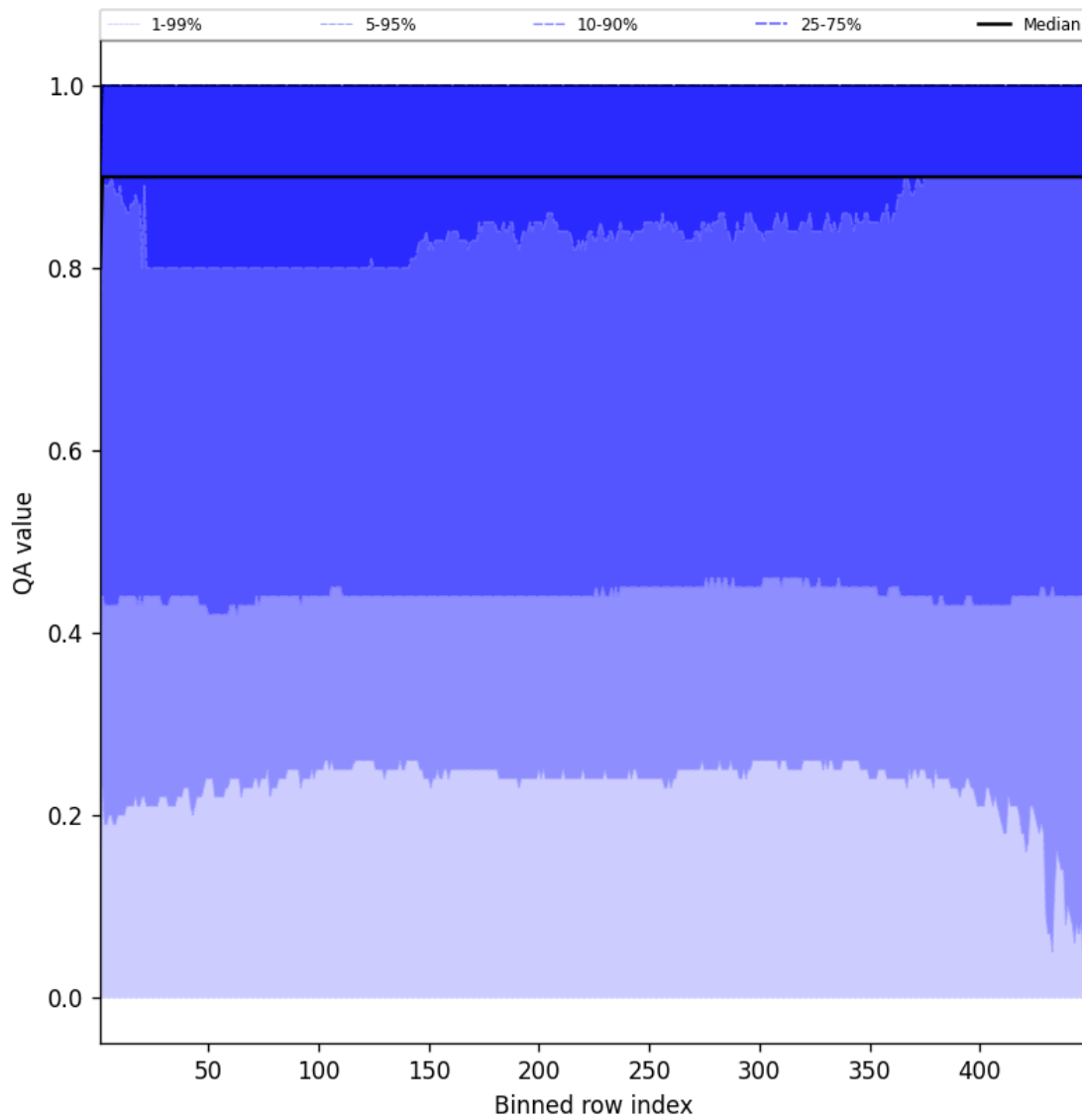
Figure 40: Along track statistics of “QA value” for 2025-10-16 to 2025-10-17
