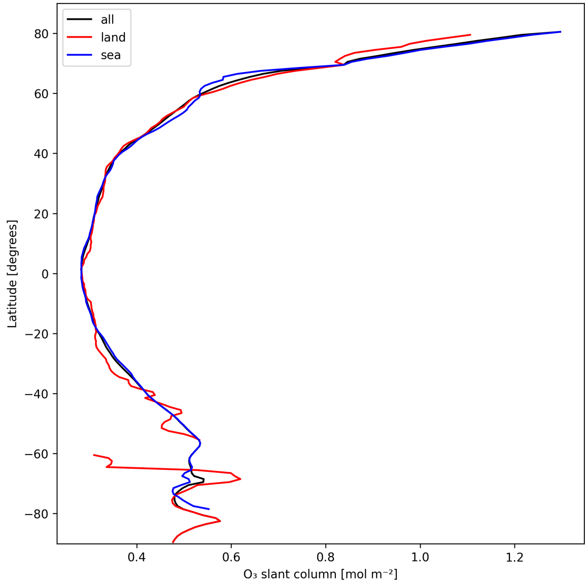
Figure 19: Zonal average of “O 3 slant column” for 2025-10-16 to 2025-10-17.
