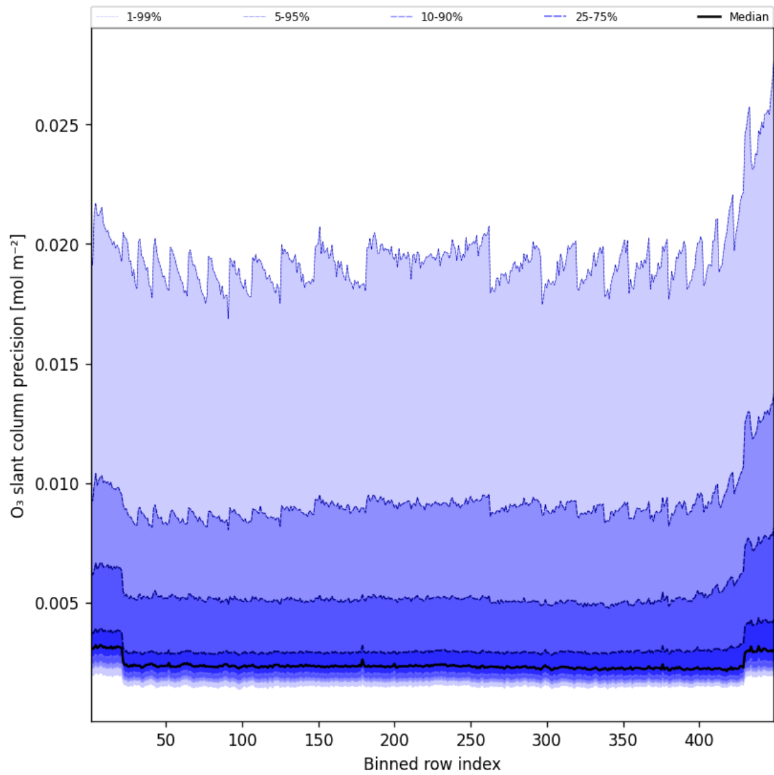
Figure 44: Along track statistics of “O 3 slant column precision” for 2025-10-16 to 2025-10-17
