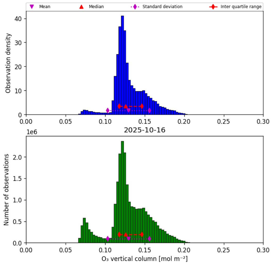
Figure 29: Histogram of “O 3 vertical column” for 2025-10-16 to 2025-10-17
