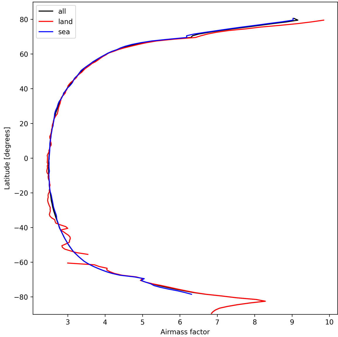
Figure 25: Zonal average of “Airmass factor” for 2025-10-16 to 2025-10-17.
