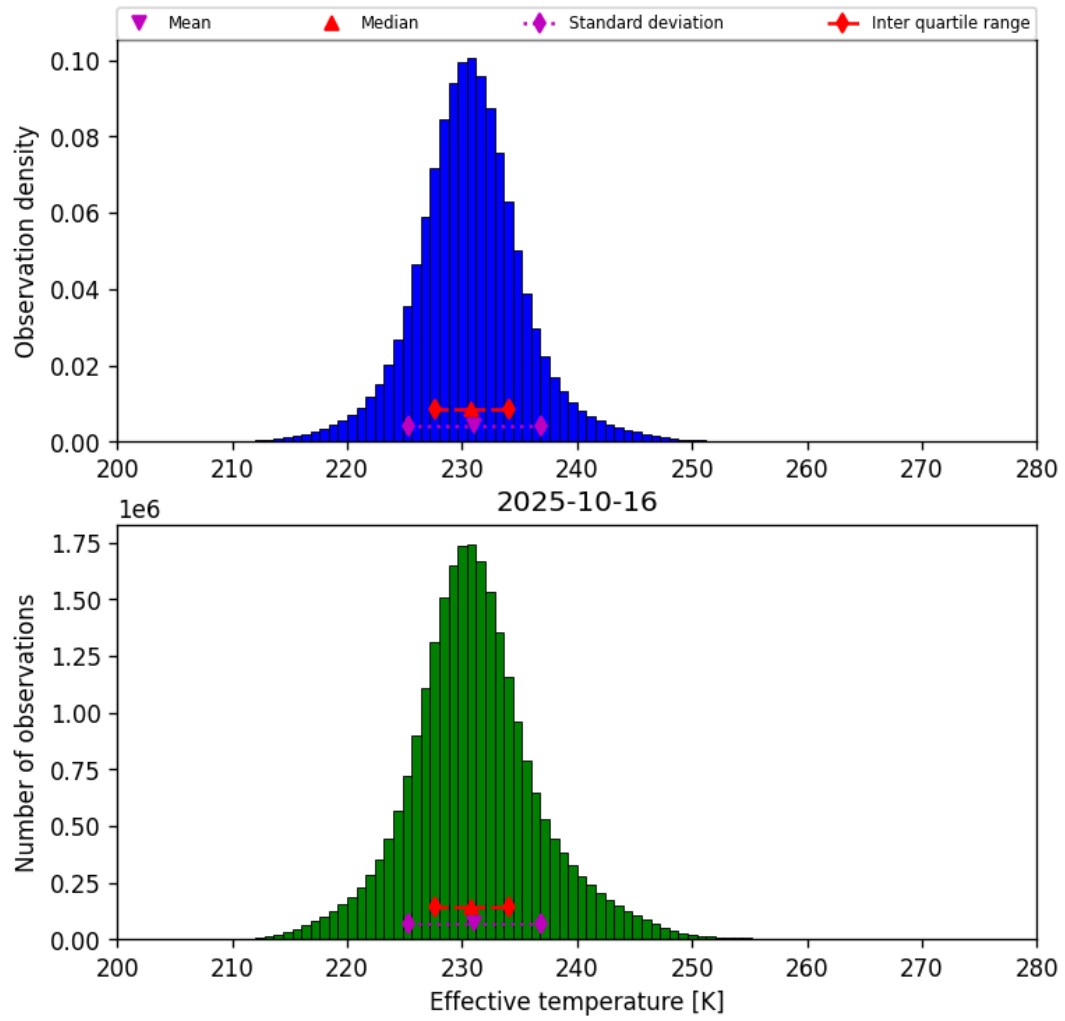
Figure 38: Histogram of “Effective temperature” for 2025-10-16 to 2025-10-17
