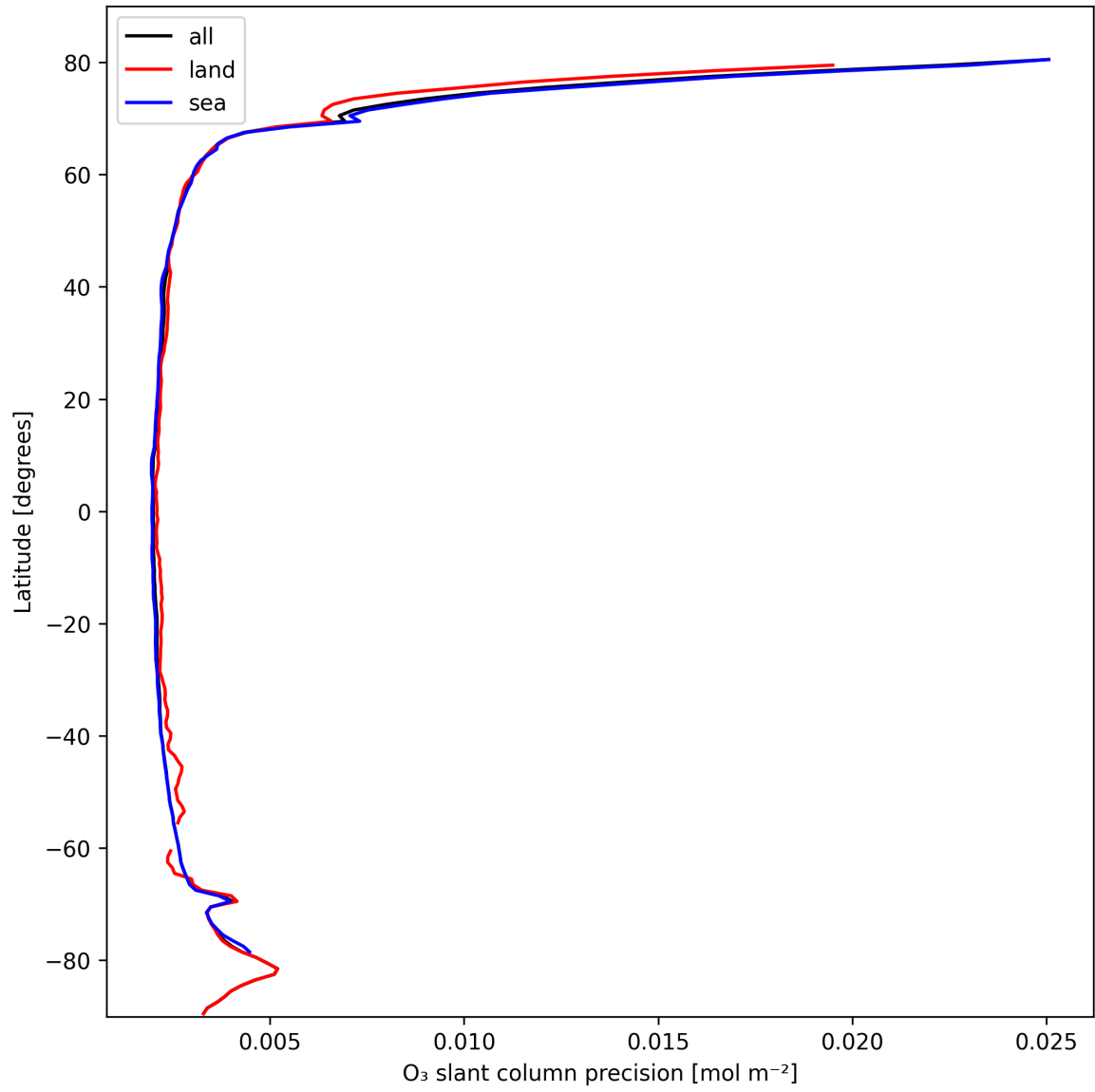
Figure 20: Zonal average of “O 3 slant column precision” for 2025-10-16 to 2025-10-17.
