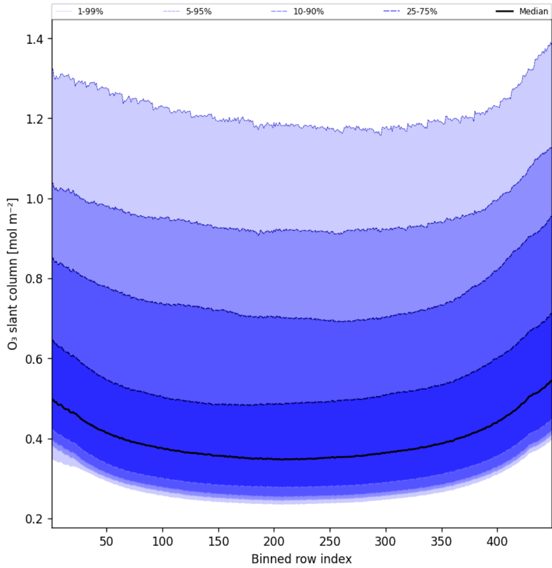
Figure 43: Along track statistics of “O 3 slant column” for 2025-10-16 to 2025-10-17
