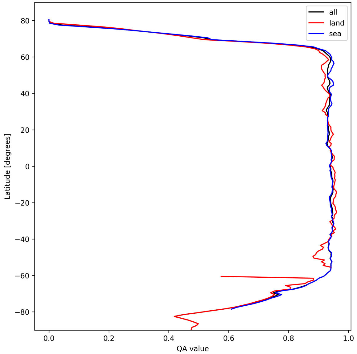
Figure 16: Zonal average of “QA value” for 2025-10-16 to 2025-10-17.
