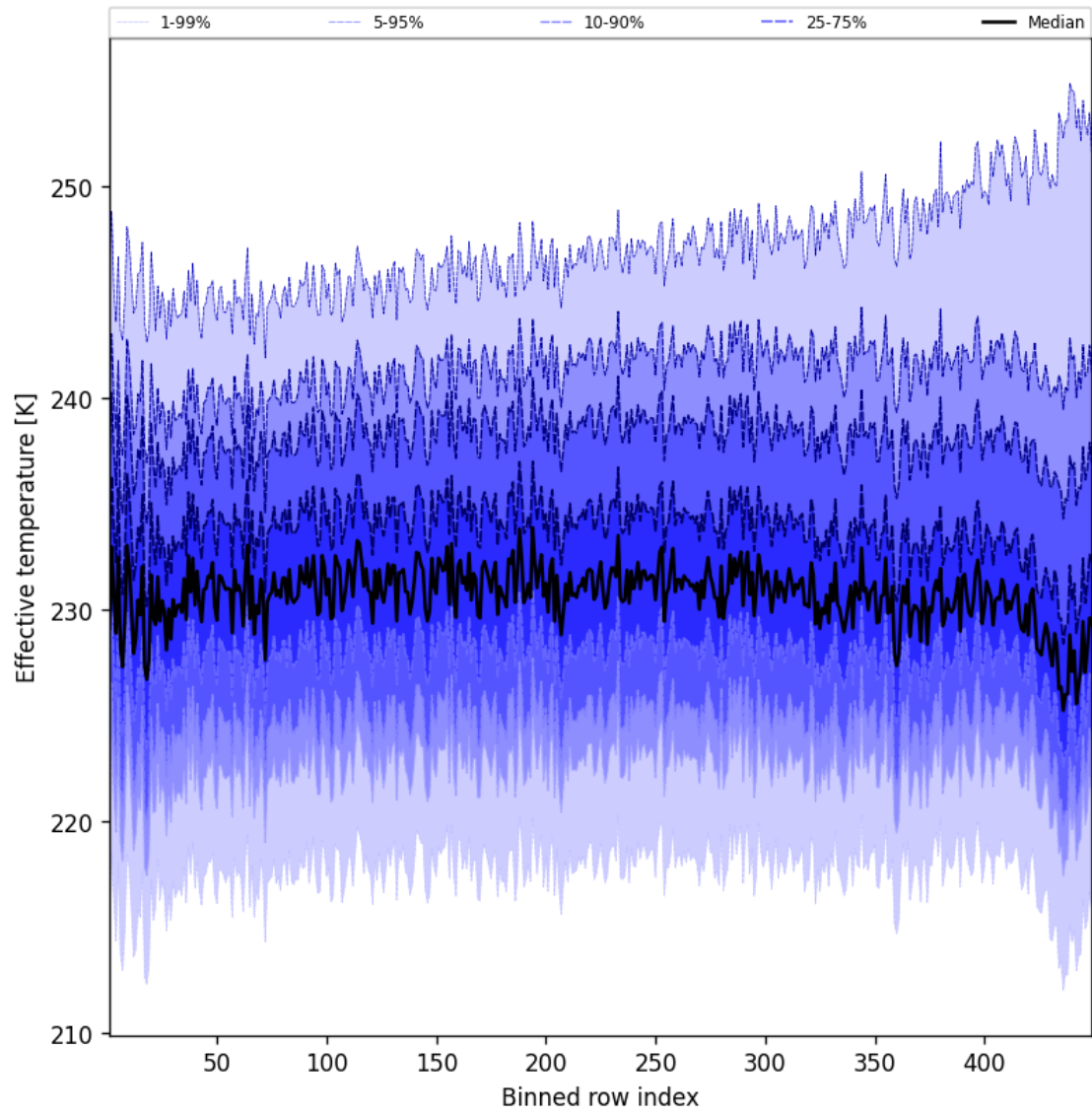
Figure 50: Along track statistics of “Effective temperature” for 2025-10-16 to 2025-10-17
