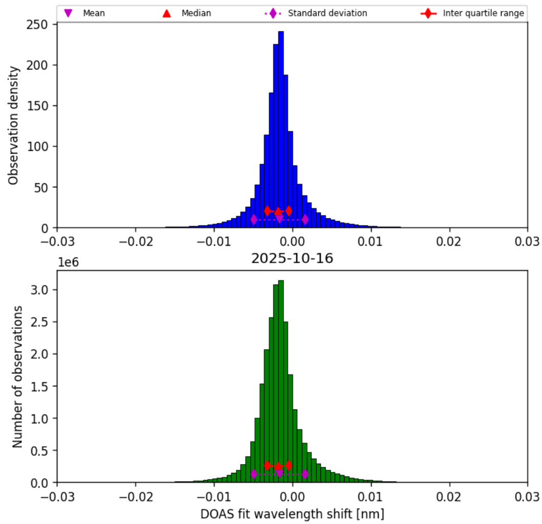
Figure 35: Histogram of “DOAS fit wavelength shift” for 2025-10-16 to 2025-10-17
