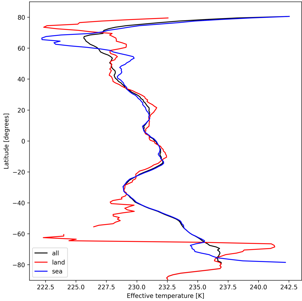
Figure 26: Zonal average of “Effective temperature” for 2025-10-16 to 2025-10-17.
