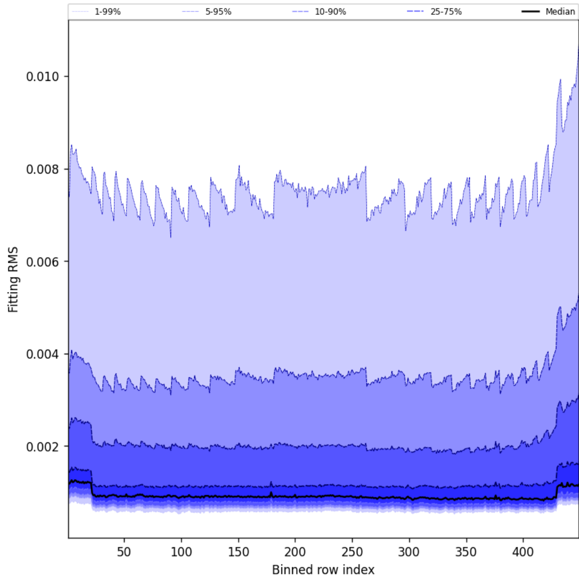
Figure 46: Along track statistics of “Fitting RMS” for 2025-10-16 to 2025-10-17
