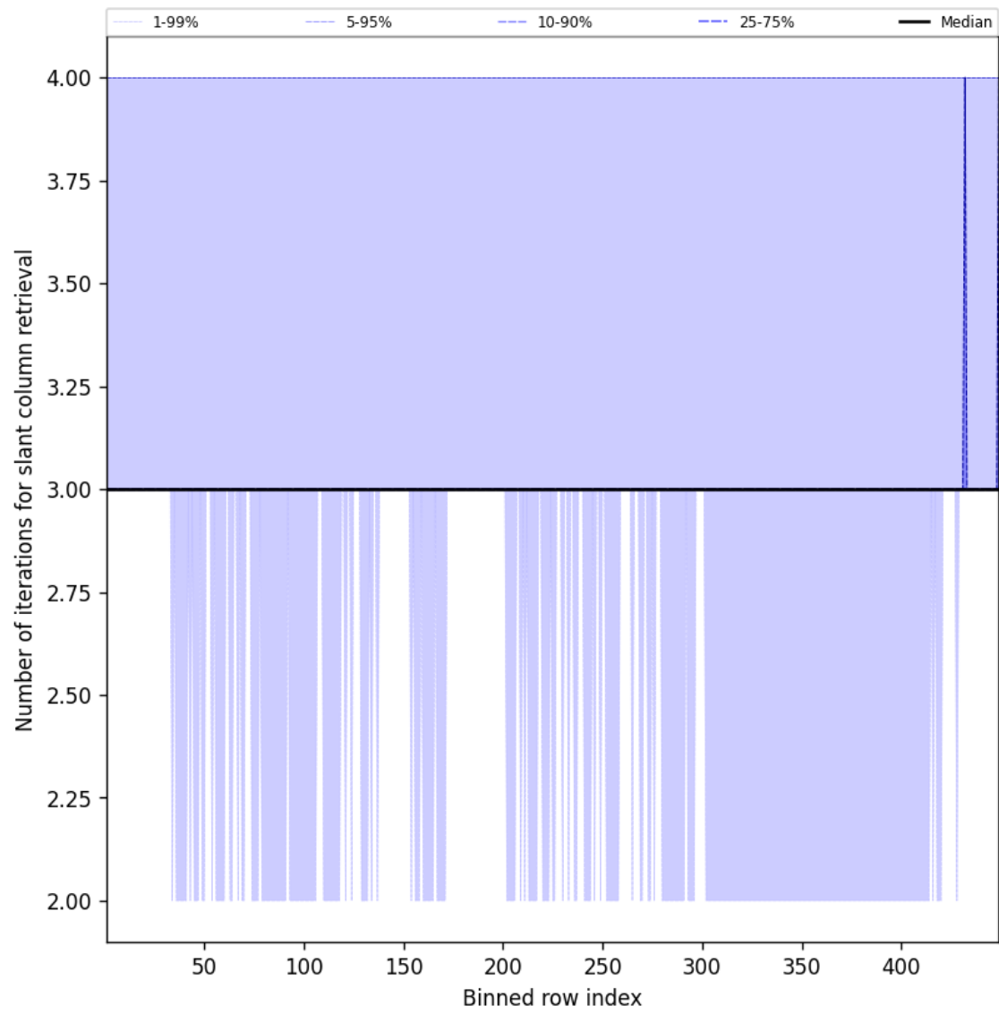
Figure 45: Along track statistics of “Number of iterations for slant column retrieval” for 2025-10-16 to 2025-10-17
