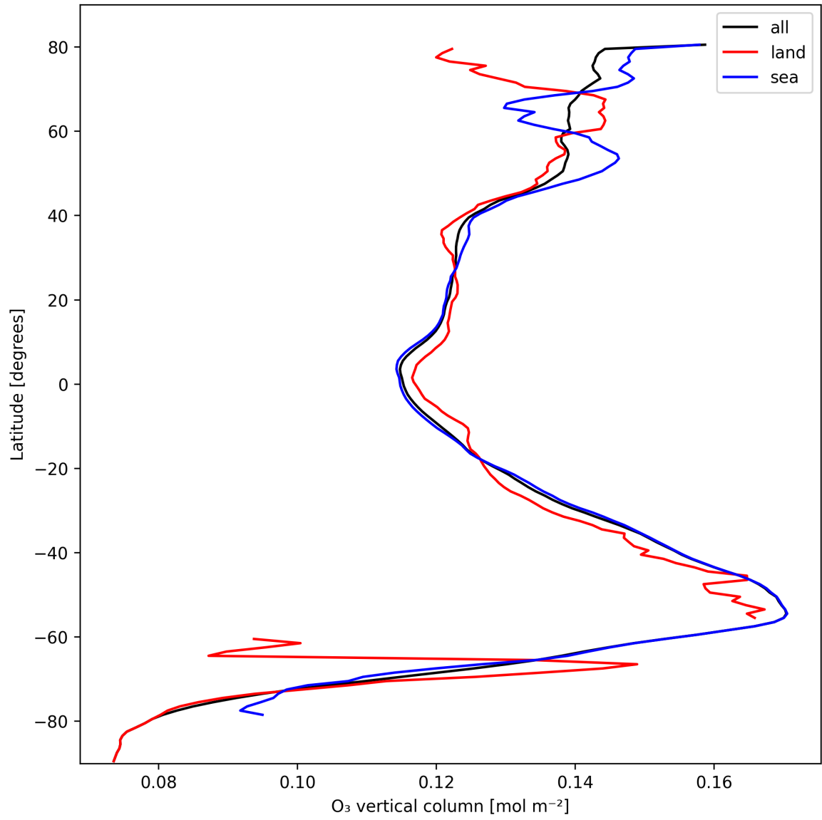
Figure 17: Zonal average of “O 3 vertical column” for 2025-10-16 to 2025-10-17.
