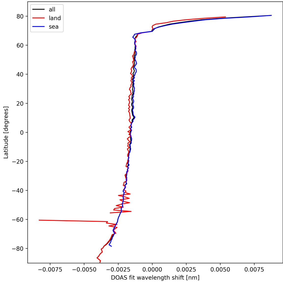
Figure 23: Zonal average of “DOAS fit wavelength shift” for 2025-10-16 to 2025-10-17.
