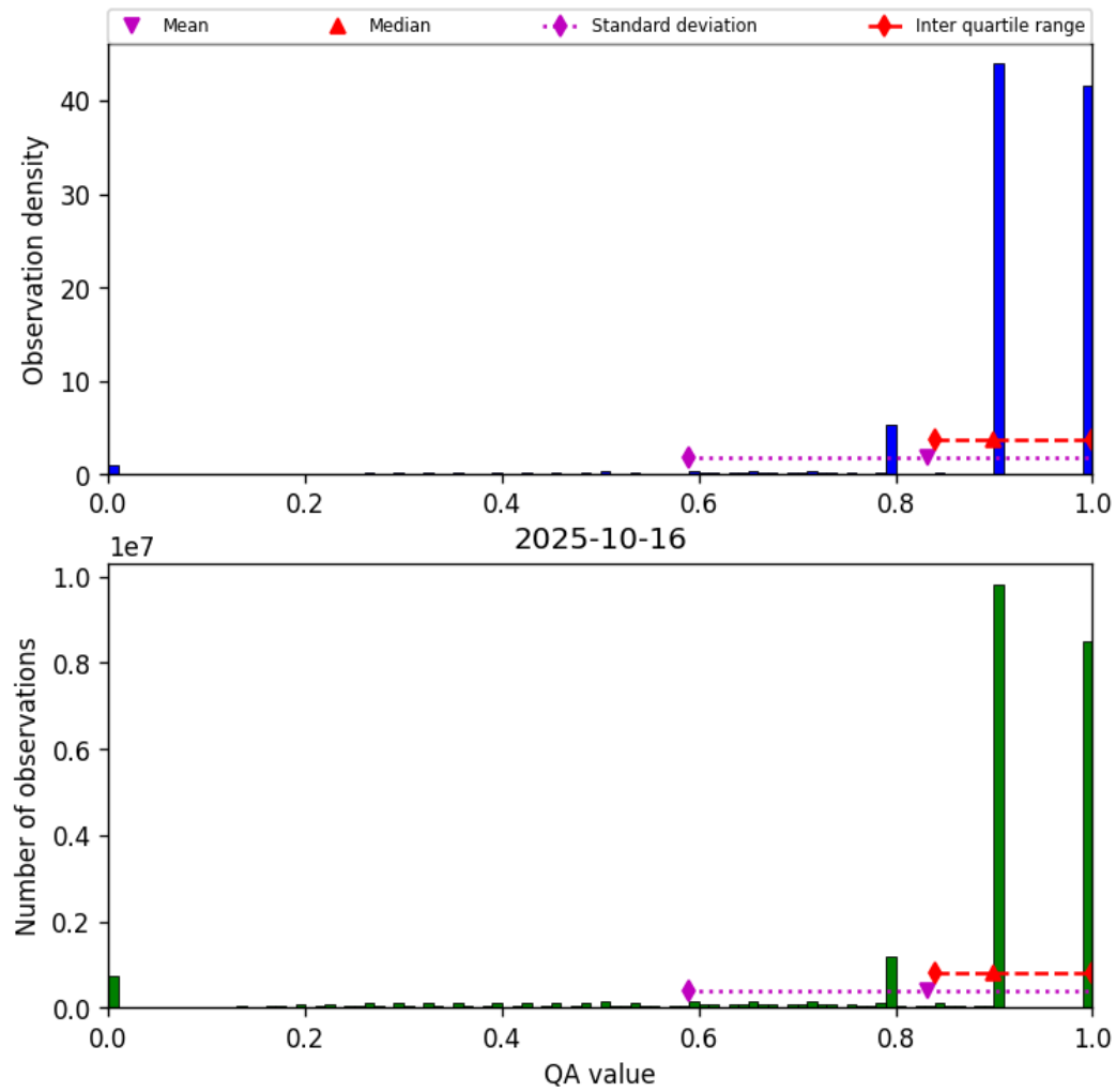
Figure 28: Histogram of “QA value” for 2025-10-16 to 2025-10-17
