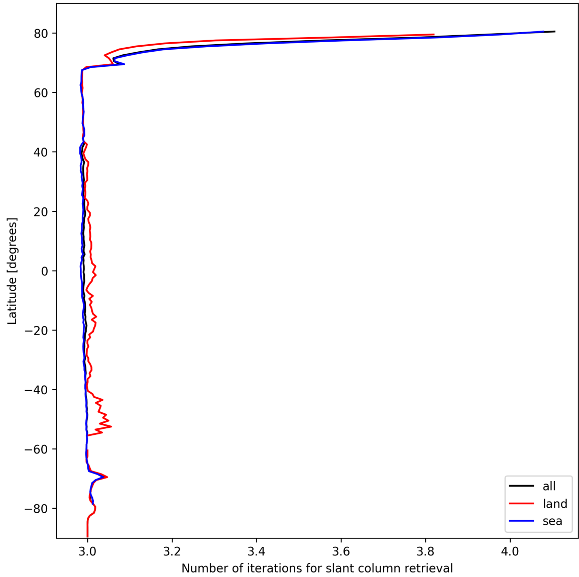
Figure 21: Zonal average of “Number of iterations for slant column retrieval” for 2025-10-16 to 2025-10-17.
