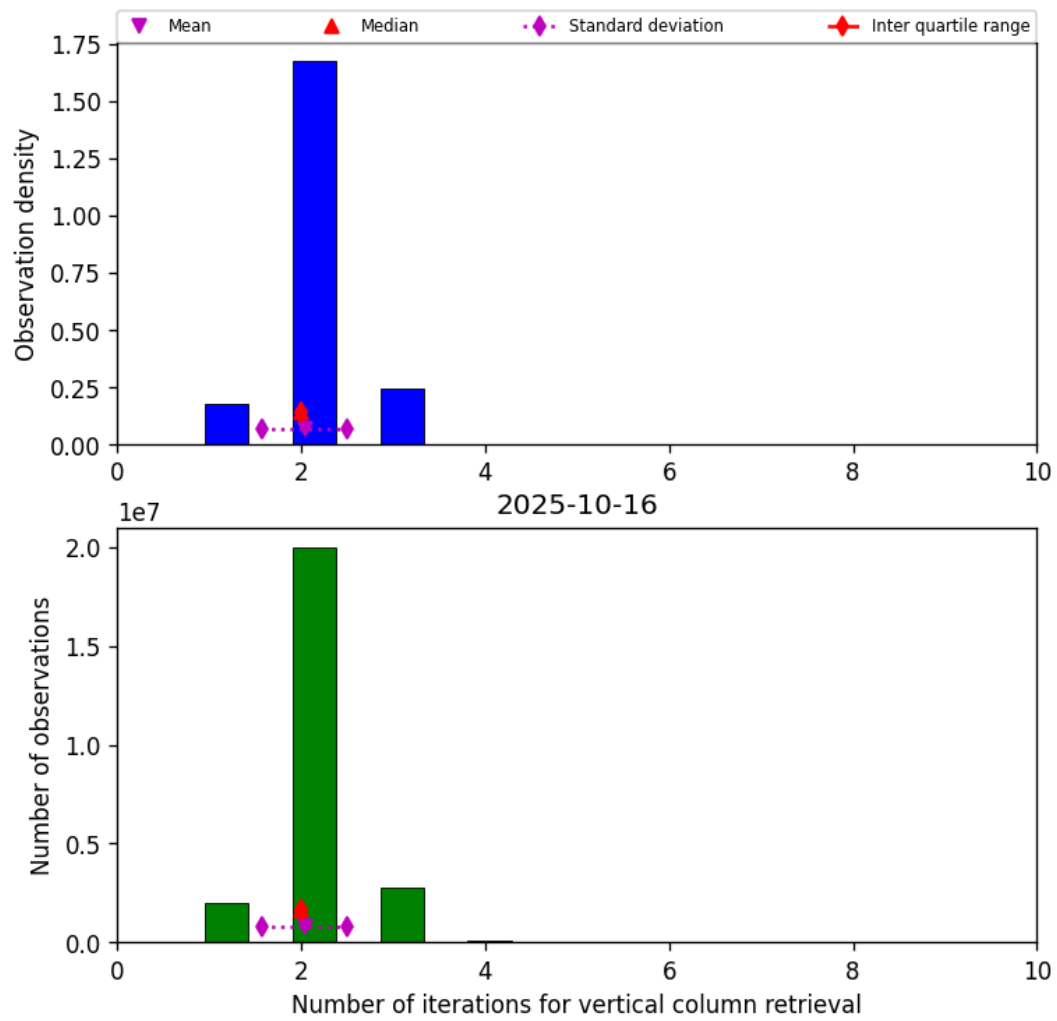
Figure 39: Histogram of “Number of iterations for vertical column retrieval” for 2025-10-16 to 2025-10-17
