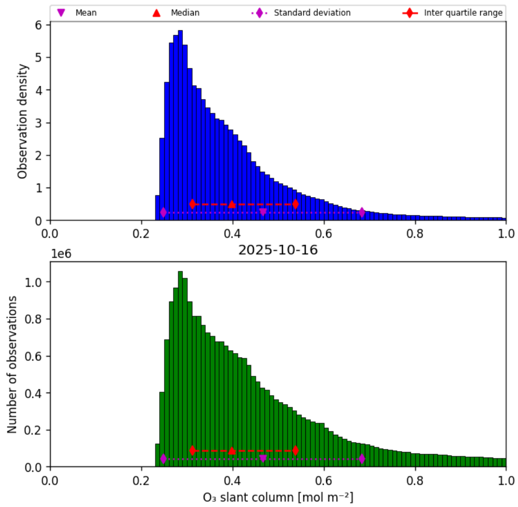
Figure 31: Histogram of “O 3 slant column” for 2025-10-16 to 2025-10-17
