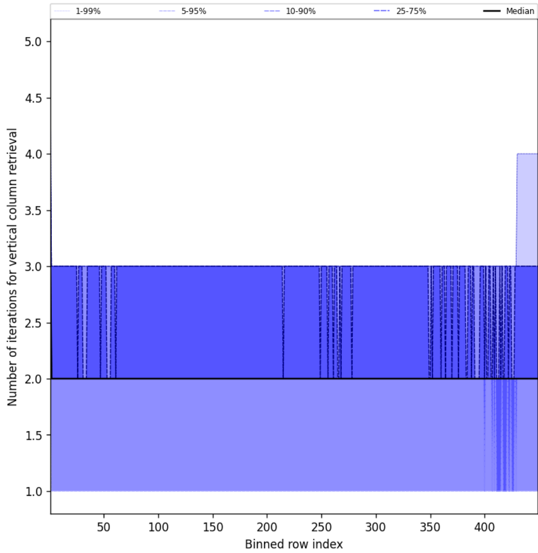
Figure 51: Along track statistics of “Number of iterations for vertical column retrieval” for 2025-10-16 to 2025-10-17
