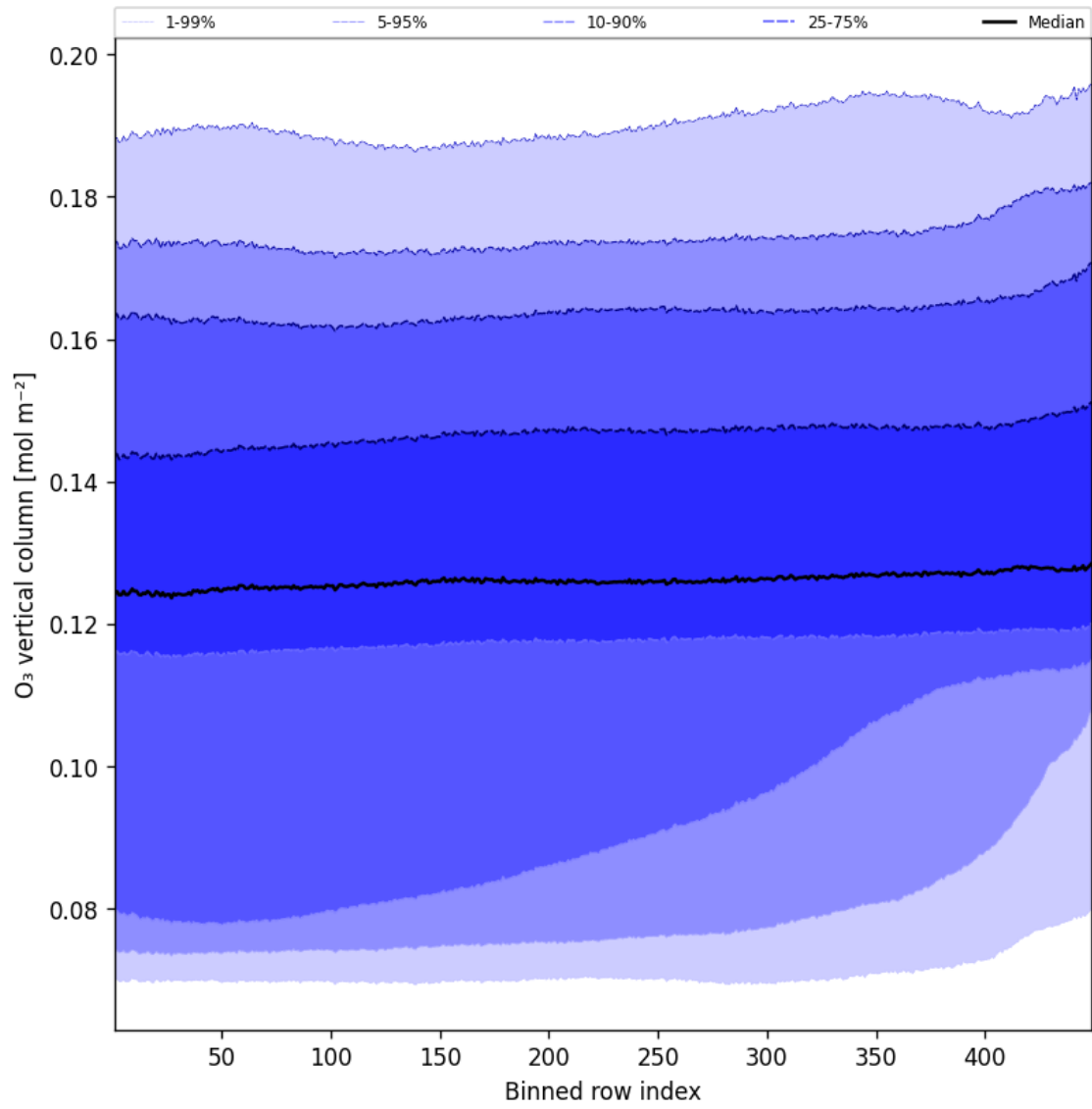
Figure 41: Along track statistics of “O 3 vertical column” for 2025-10-16 to 2025-10-17
