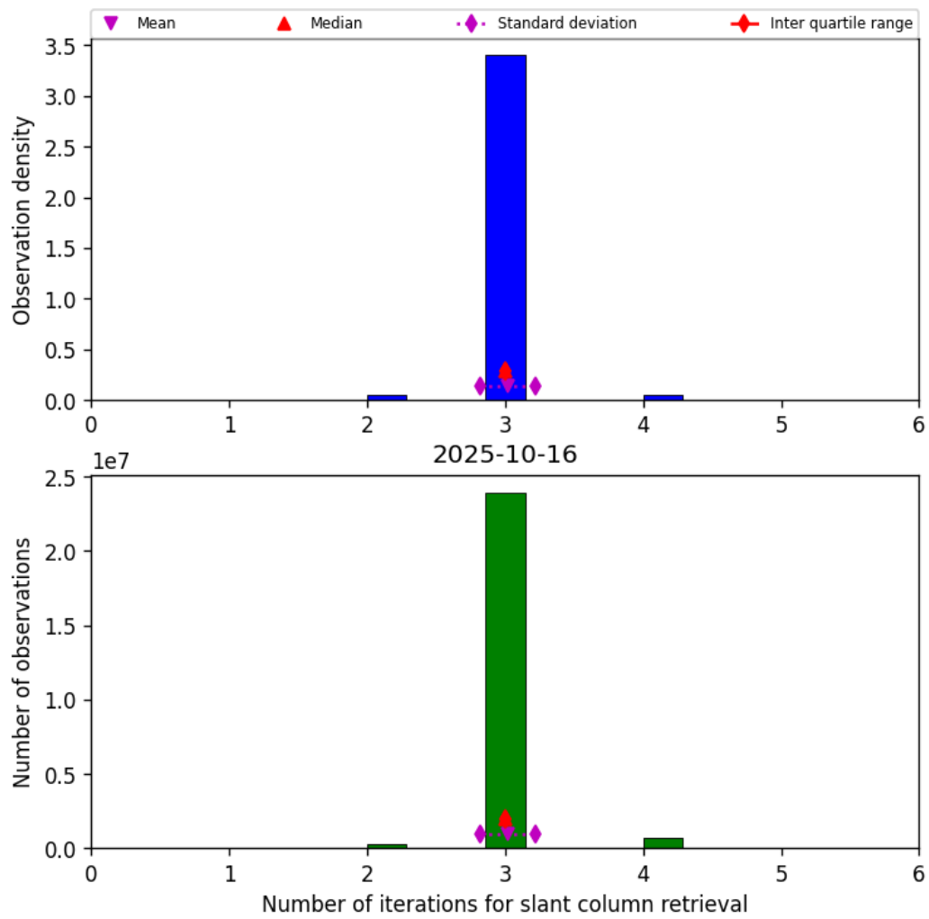
Figure 33: Histogram of “Number of iterations for slant column retrieval” for 2025-10-16 to 2025-10-17
