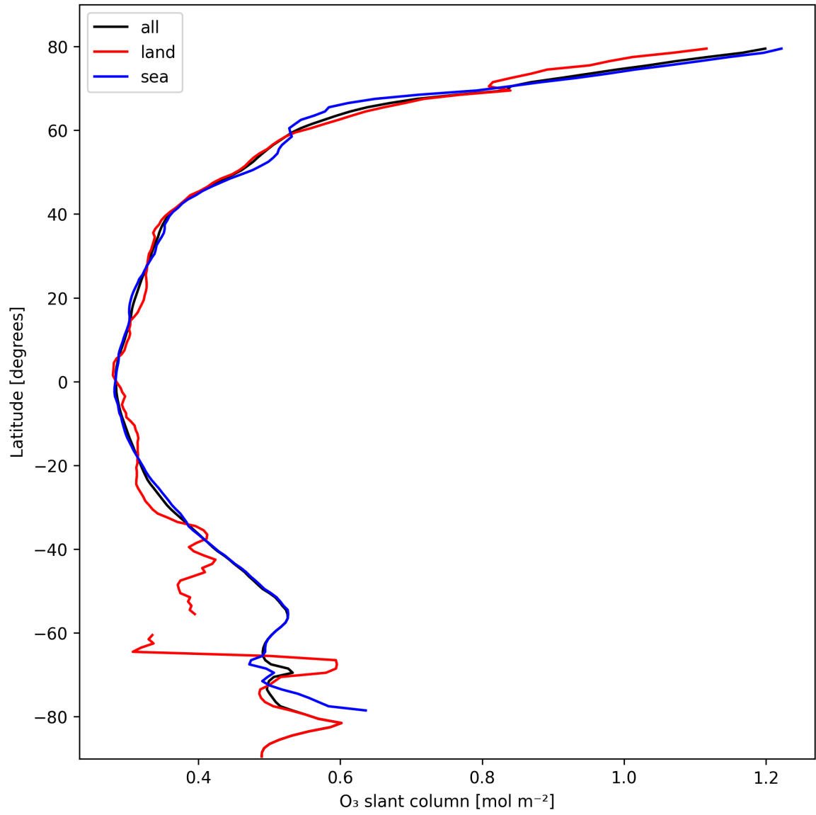
Figure 19: Zonal average of “O 3 slant column” for 2025-10-17 to 2025-10-18.
