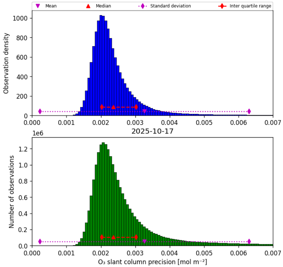
Figure 32: Histogram of “O 3 slant column precision” for 2025-10-17 to 2025-10-18
