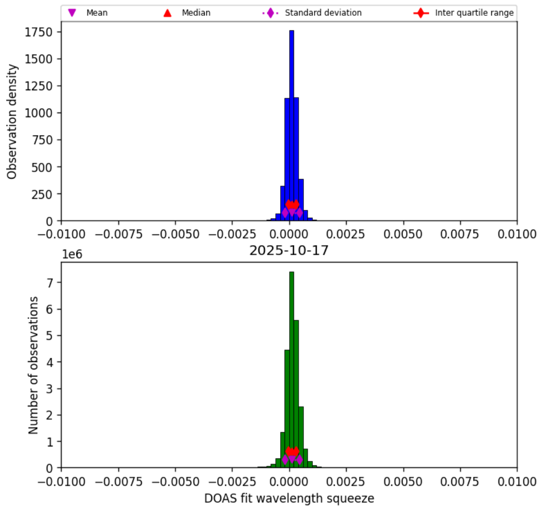
Figure 36: Histogram of “DOAS fit wavelength squeeze” for 2025-10-17 to 2025-10-18
