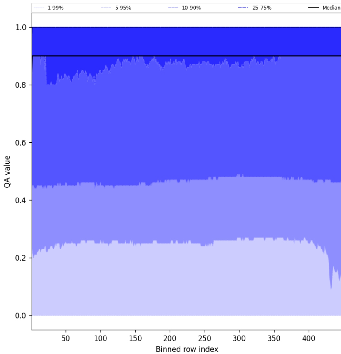
Figure 40: Along track statistics of “QA value” for 2025-10-17 to 2025-10-18
