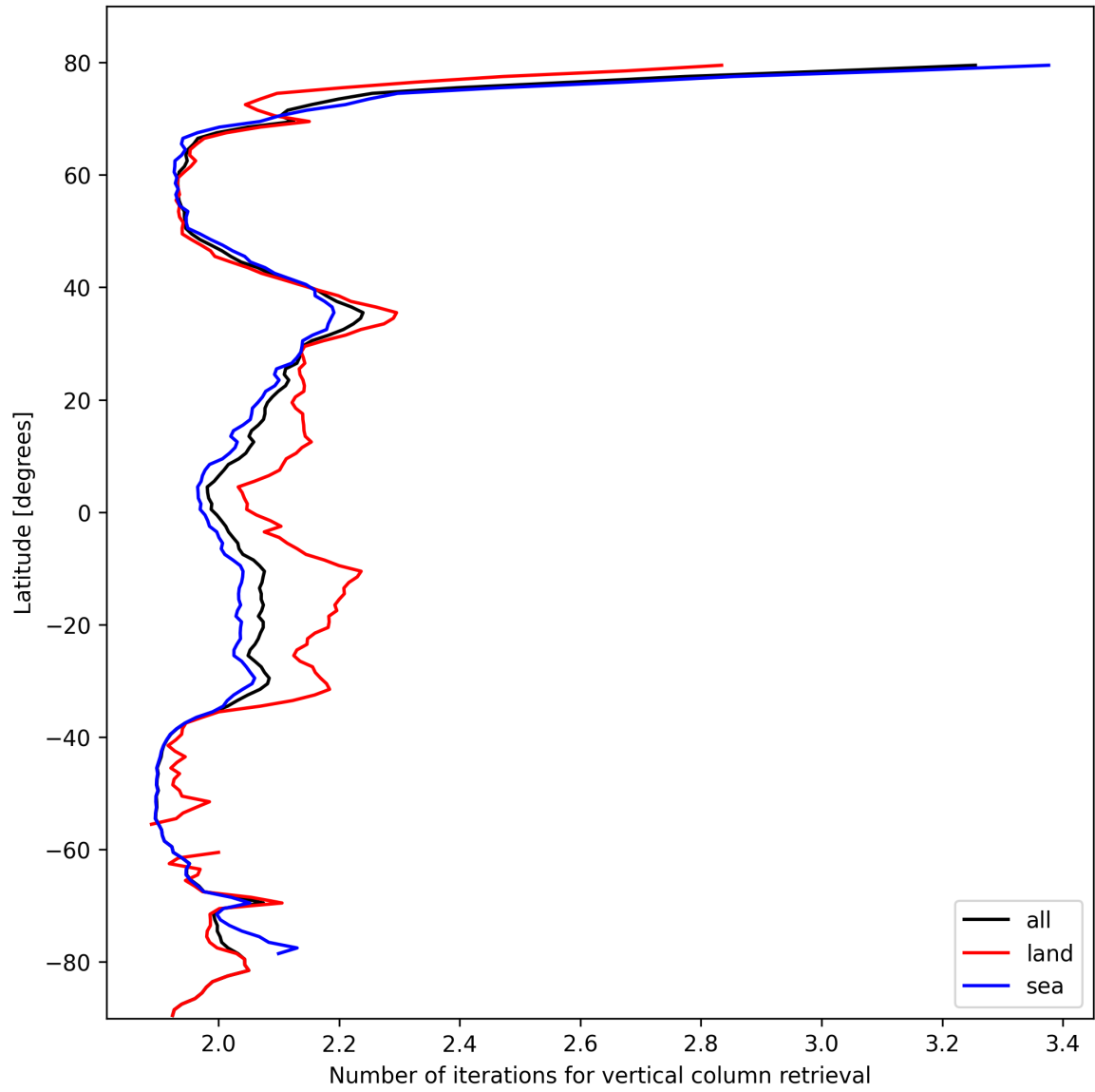
Figure 27: Zonal average of “Number of iterations for vertical column retrieval” for 2025-10-17 to 2025-10-18.
