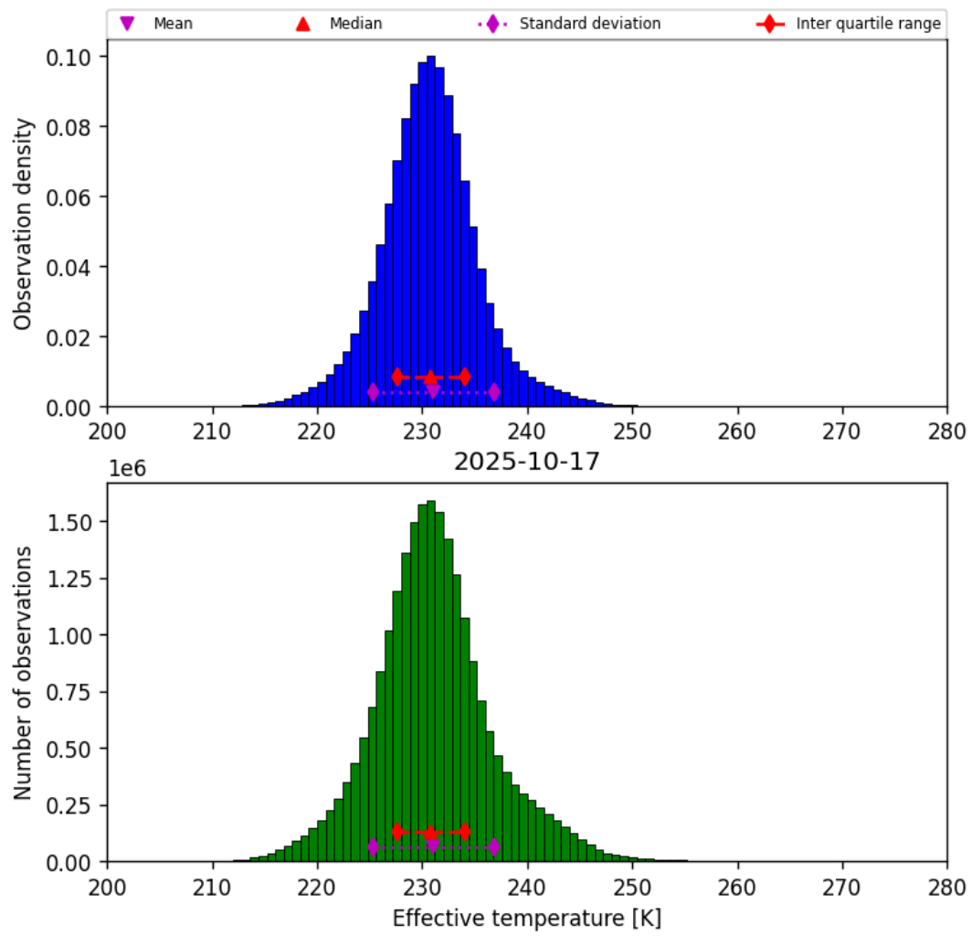
Figure 38: Histogram of “Effective temperature” for 2025-10-17 to 2025-10-18
