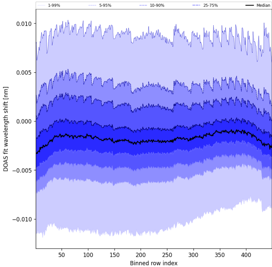
Figure 47: Along track statistics of “DOAS fit wavelength shift” for 2025-10-17 to 2025-10-18
