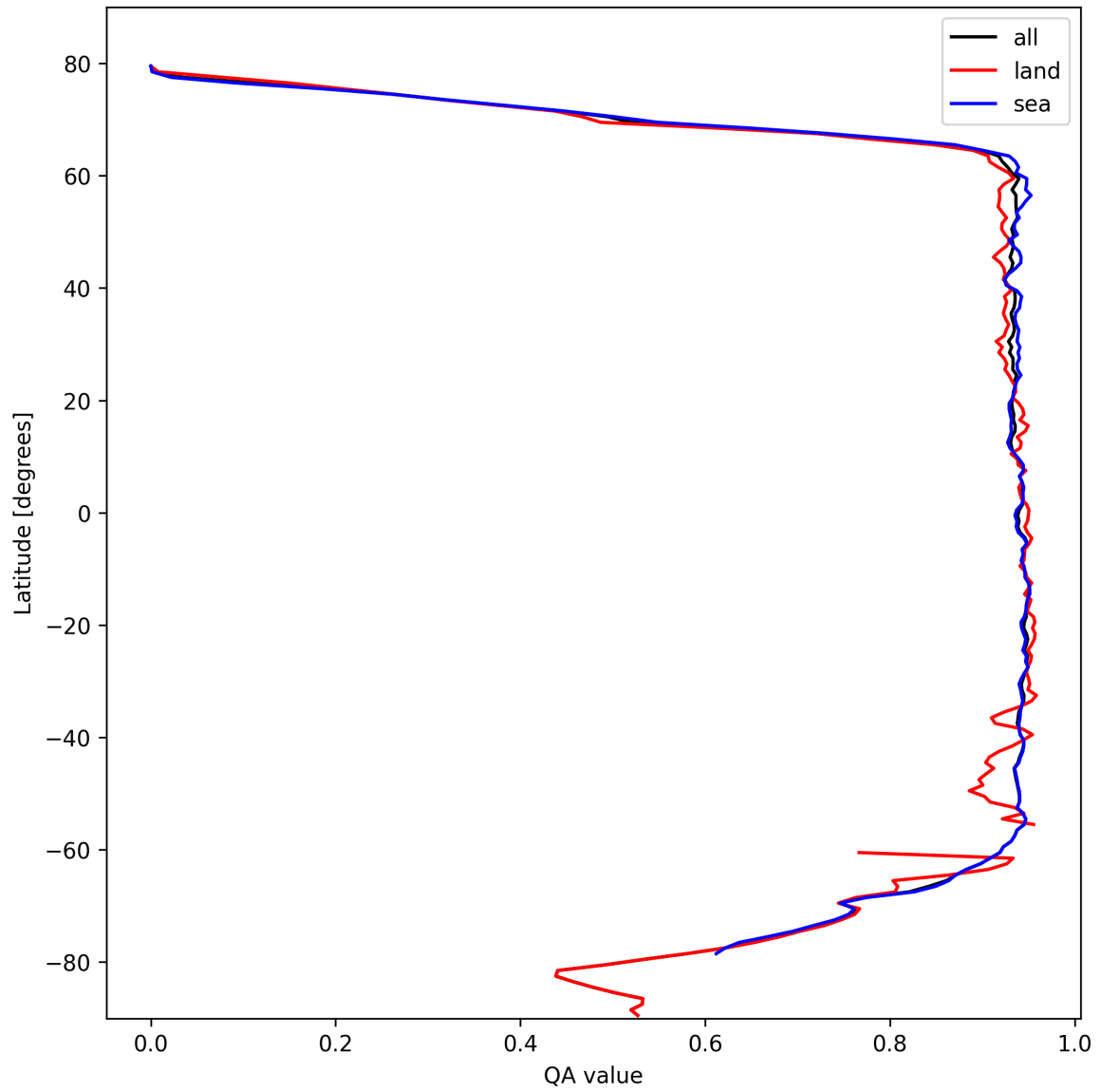
Figure 16: Zonal average of “QA value” for 2025-10-17 to 2025-10-18.
