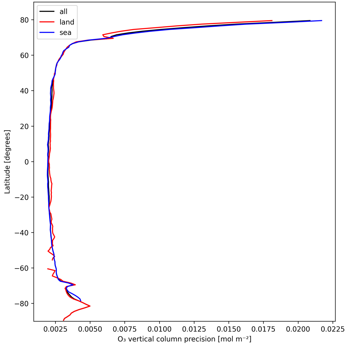
Figure 18: Zonal average of “O 3 vertical column precision” for 2025-10-17 to 2025-10-18.
