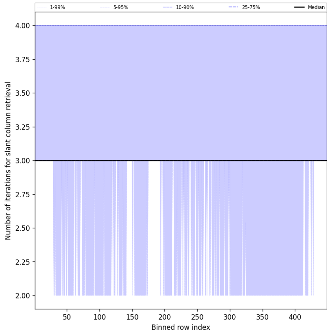
Figure 45: Along track statistics of “Number of iterations for slant column retrieval” for 2025-10-17 to 2025-10-18
