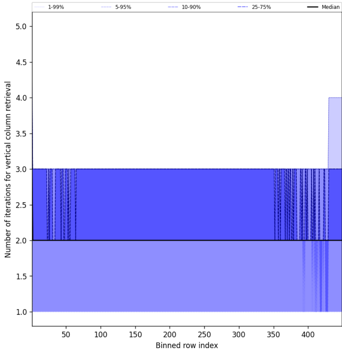
Figure 51: Along track statistics of “Number of iterations for vertical column retrieval” for 2025-10-17 to 2025-10-18
