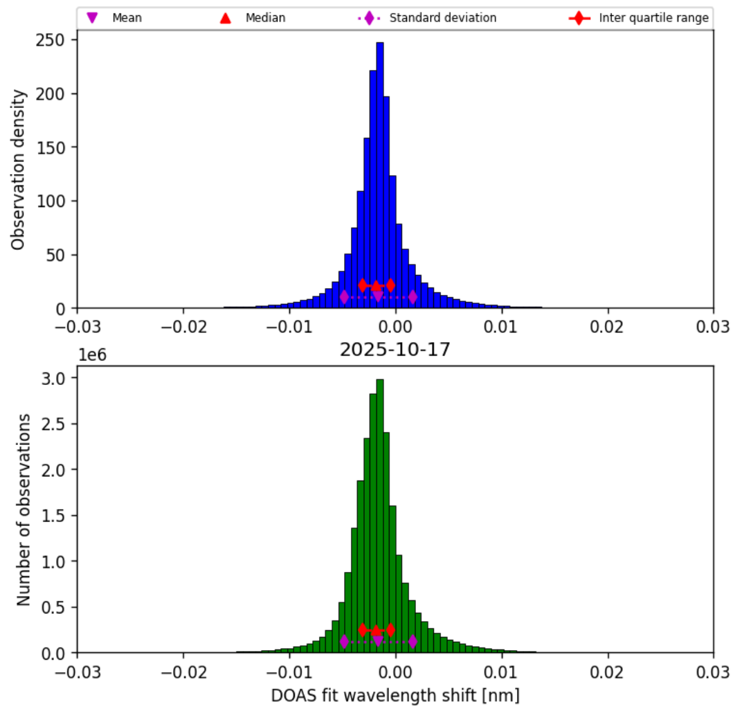
Figure 35: Histogram of “DOAS fit wavelength shift” for 2025-10-17 to 2025-10-18
