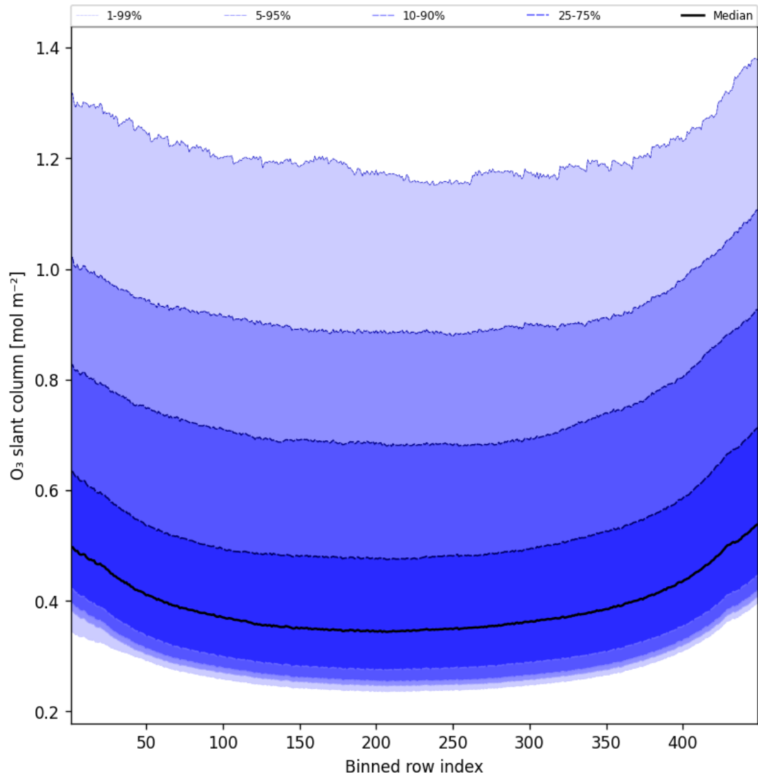
Figure 43: Along track statistics of “O 3 slant column” for 2025-10-17 to 2025-10-18
