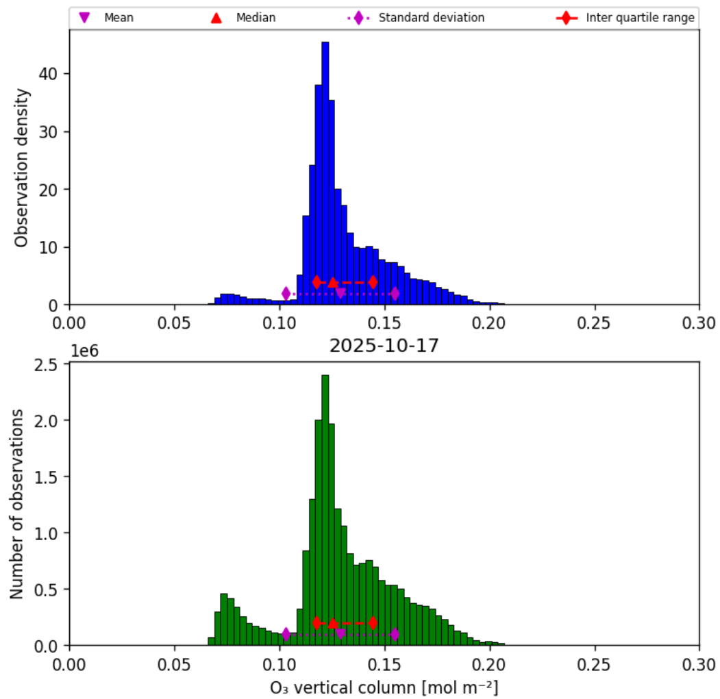
Figure 29: Histogram of “O 3 vertical column” for 2025-10-17 to 2025-10-18
