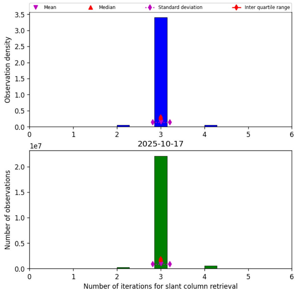
Figure 33: Histogram of “Number of iterations for slant column retrieval” for 2025-10-17 to 2025-10-18
