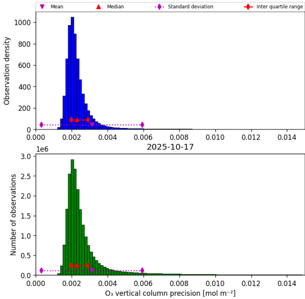
Figure 30: Histogram of “O 3 vertical column precision” for 2025-10-17 to 2025-10-18
