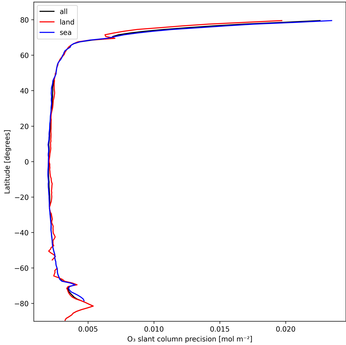
Figure 20: Zonal average of "O 3 slant column precision" for 2025-10-17 to 2025-10-18.
