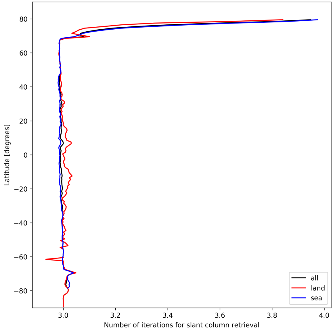
Figure 21: Zonal average of “Number of iterations for slant column retrieval” for 2025-10-17 to 2025-10-18.
