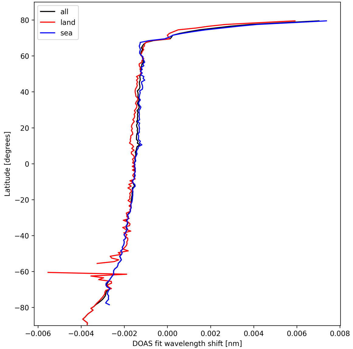
Figure 23: Zonal average of “DOAS fit wavelength shift” for 2025-10-17 to 2025-10-18.
