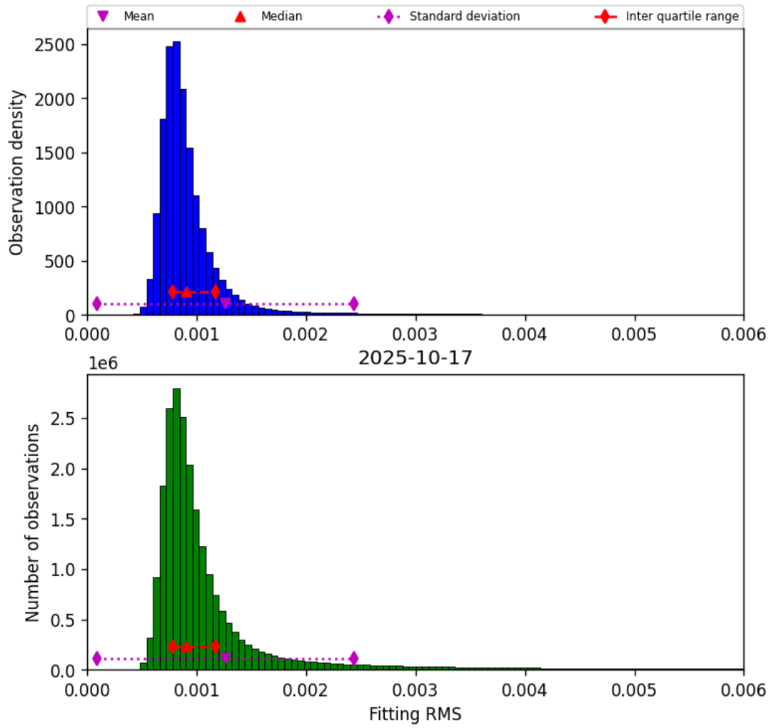
Figure 34: Histogram of “Fitting RMS” for 2025-10-17 to 2025-10-18
