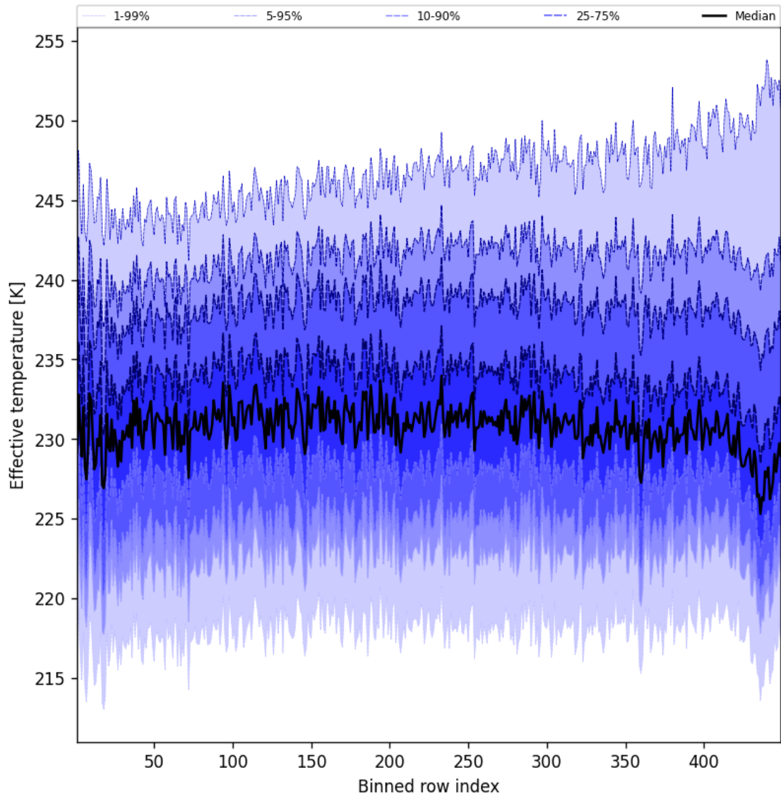
Figure 50: Along track statistics of “Effective temperature” for 2025-10-17 to 2025-10-18
