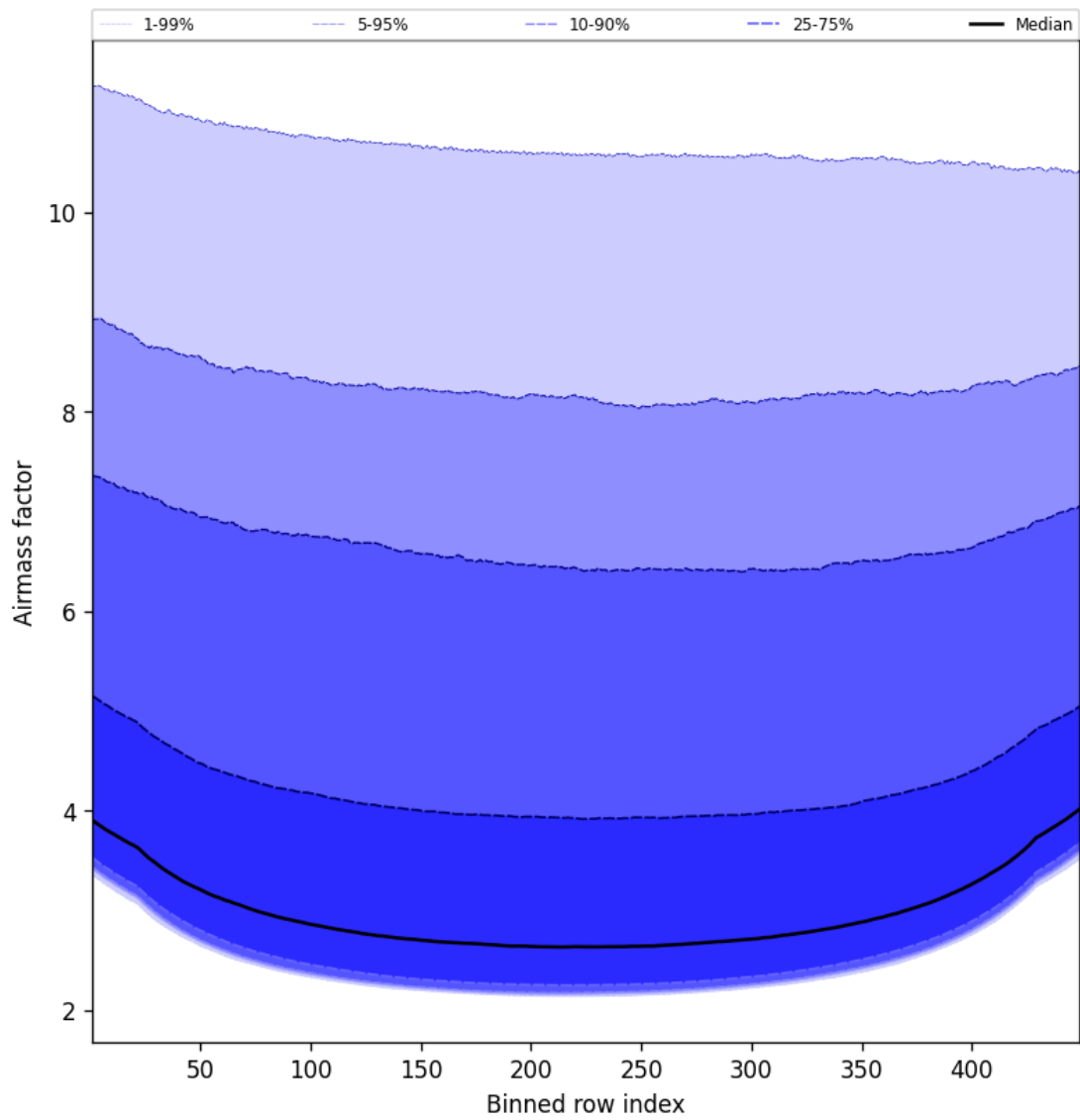
Figure 49: Along track statistics of “Airmass factor” for 2025-10-17 to 2025-10-18
