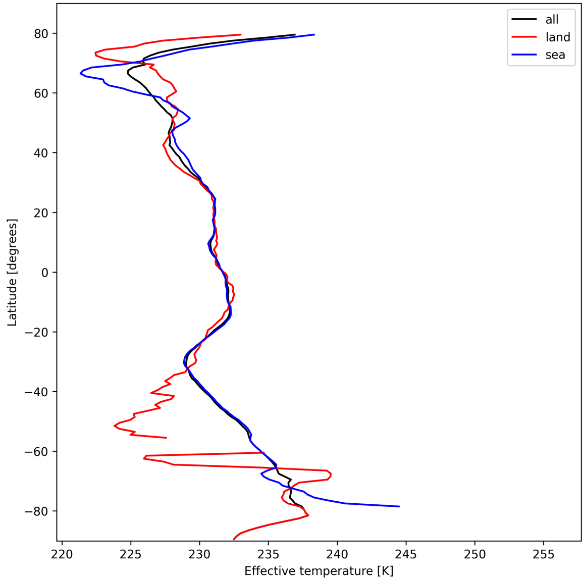
Figure 26: Zonal average of "Effective temperature" for 2025-10-17 to 2025-10-18.
