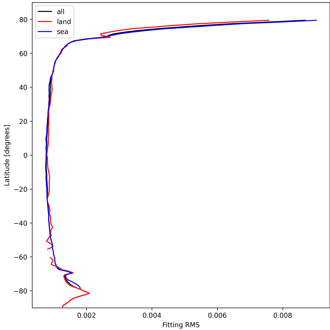
Figure 22: Zonal average of “Fitting RMS” for 2025-10-17 to 2025-10-18.
