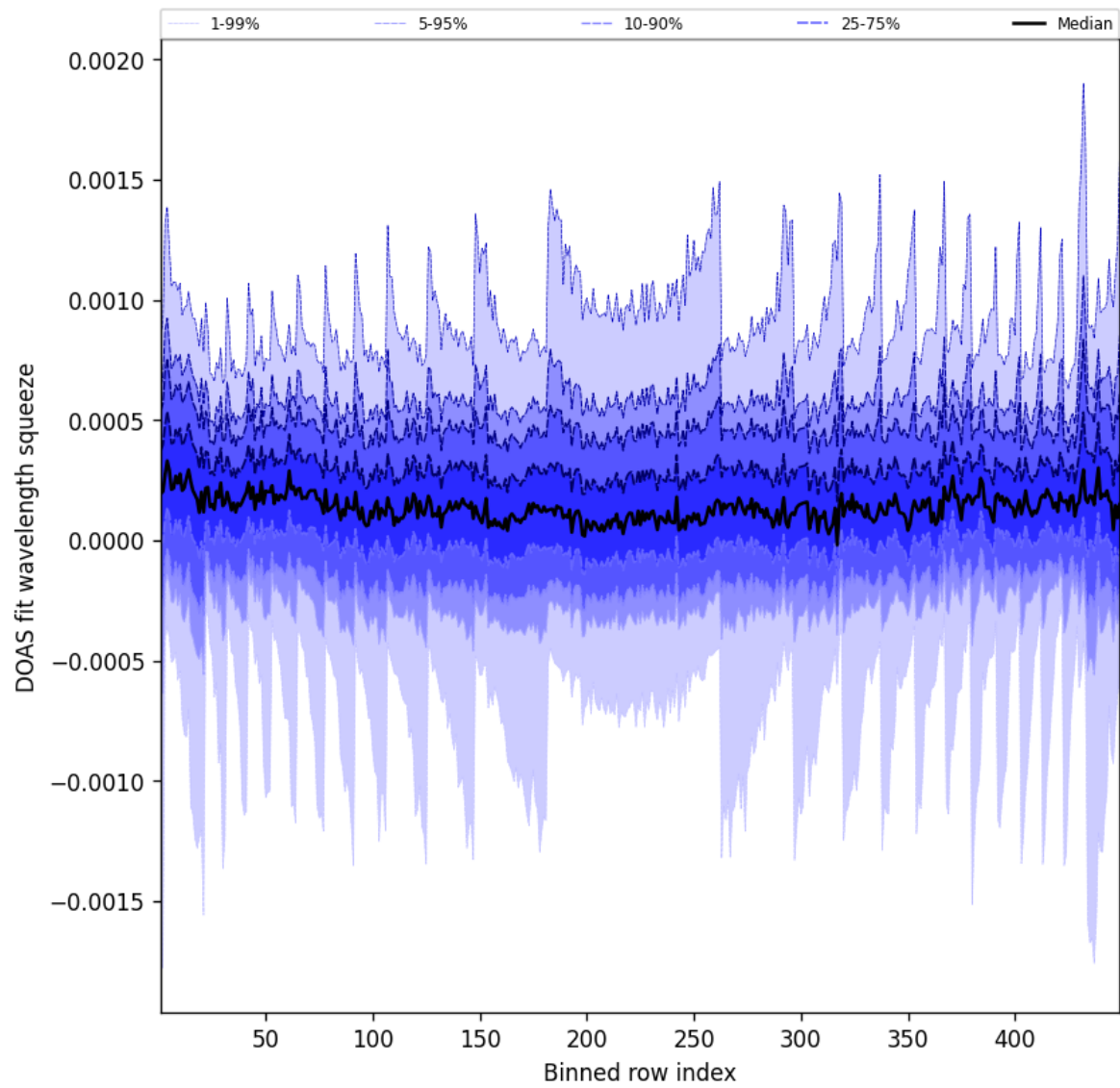
Figure 48: Along track statistics of “DOAS fit wavelength squeeze” for 2025-10-17 to 2025-10-18
