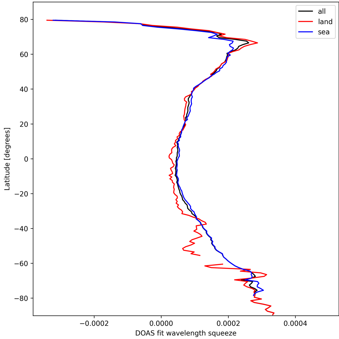
Figure 24: Zonal average of “DOAS fit wavelength squeeze” for 2025-10-17 to 2025-10-18.
