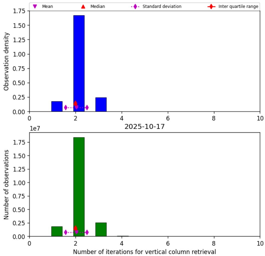
Figure 39: Histogram of “Number of iterations for vertical column retrieval” for 2025-10-17 to 2025-10-18
