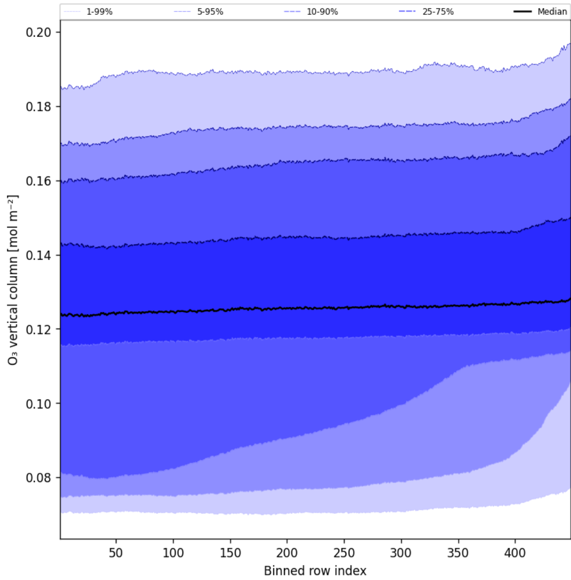
Figure 41: Along track statistics of "O 3 vertical column" for 2025-10-17 to 2025-10-18
