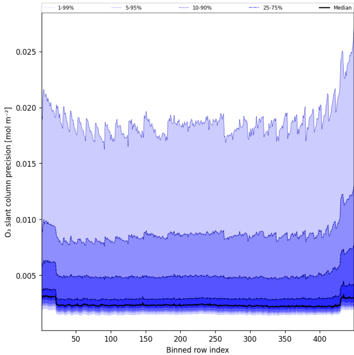
Figure 44: Along track statistics of “O 3 slant column precision” for 2025-10-17 to 2025-10-18
