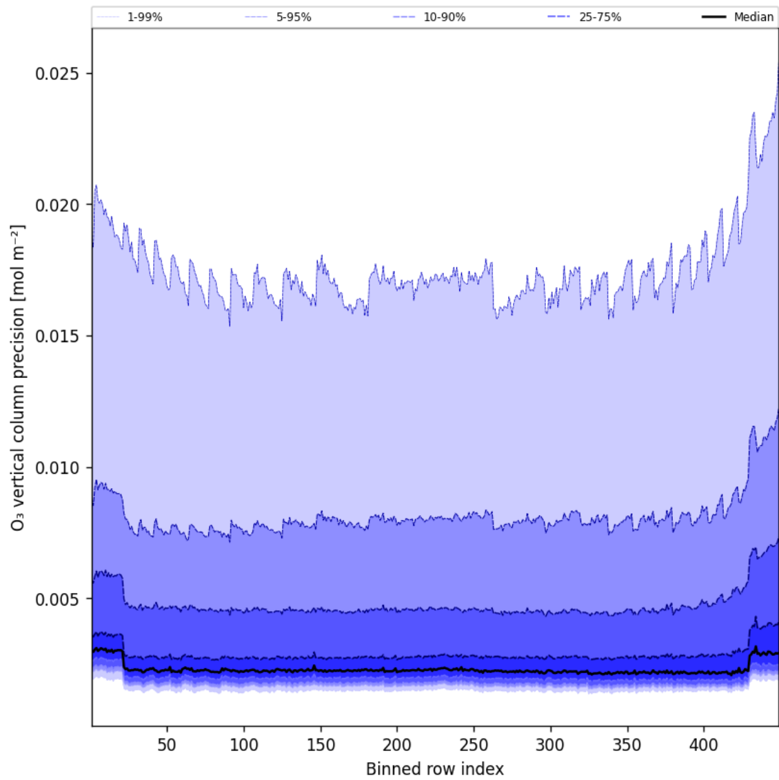
Figure 42: Along track statistics of “O 3 vertical column precision” for 2025-10-17 to 2025-10-18
