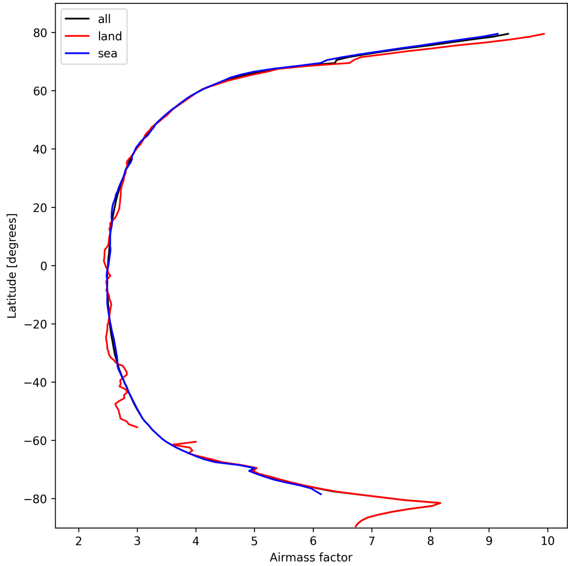
Figure 25: Zonal average of “Airmass factor” for 2025-10-17 to 2025-10-18.
