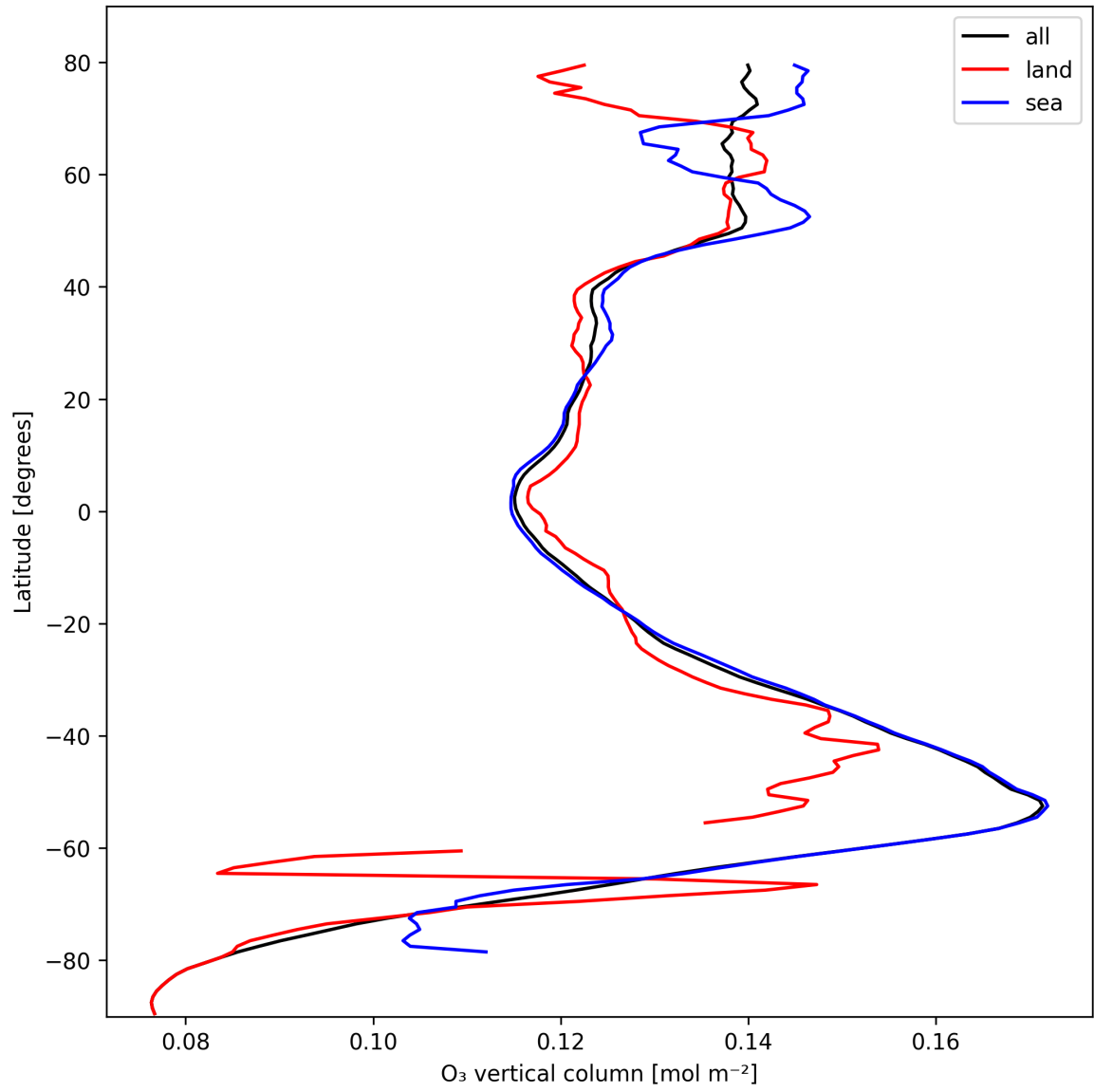
Figure 17: Zonal average of “O 3 vertical column” for 2025-10-17 to 2025-10-18.
