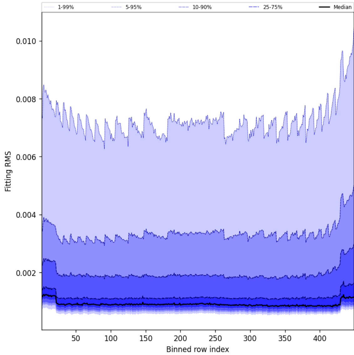
Figure 46: Along track statistics of “Fitting RMS” for 2025-10-17 to 2025-10-18
