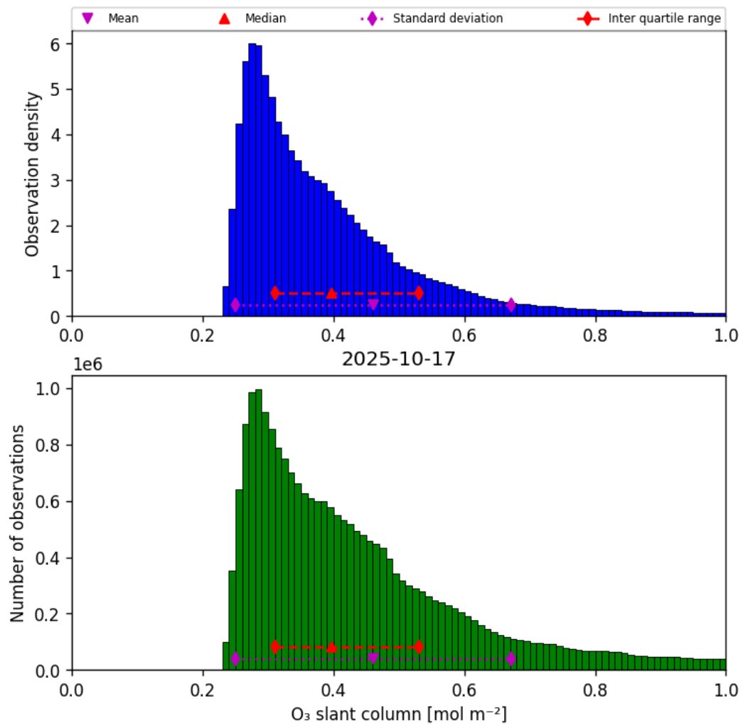
Figure 31: Histogram of “O 3 slant column” for 2025-10-17 to 2025-10-18
