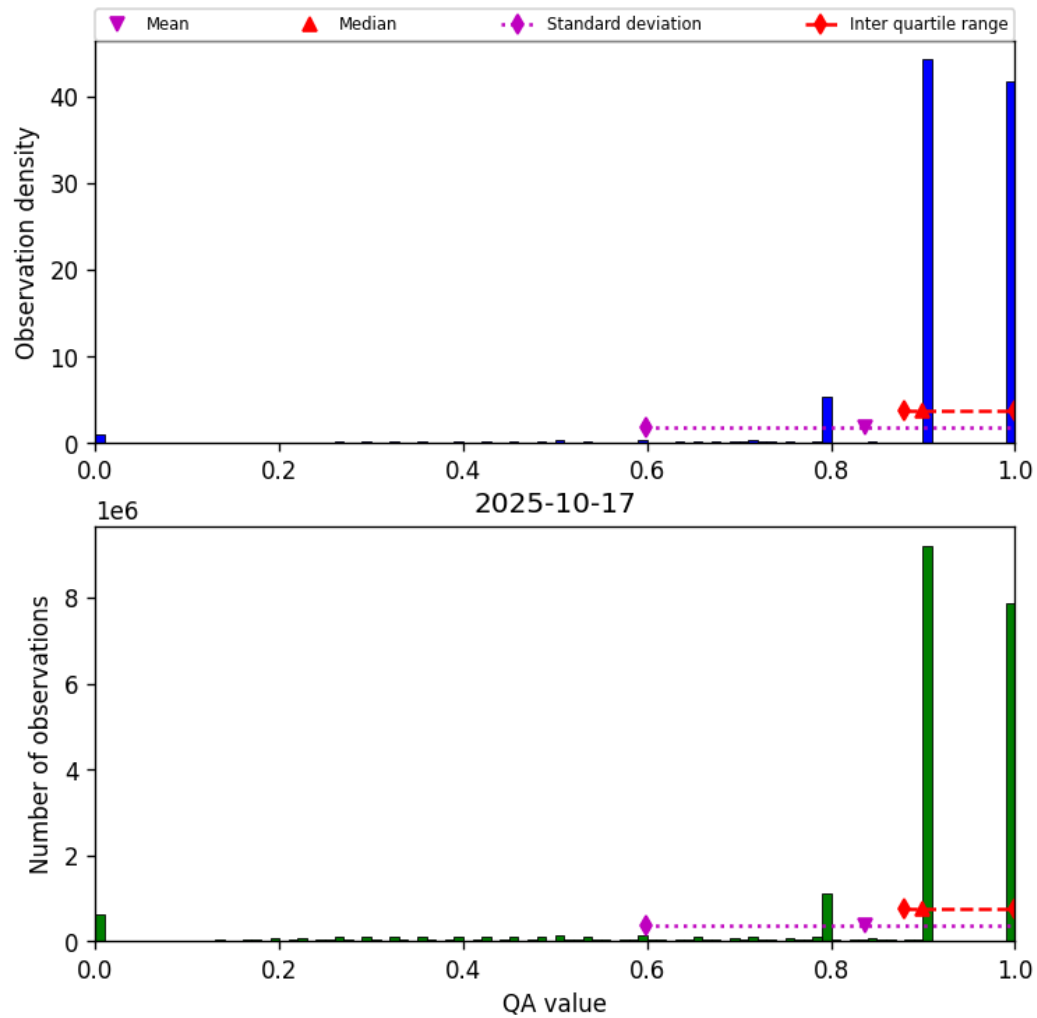
Figure 28: Histogram of “QA value” for 2025-10-17 to 2025-10-18
