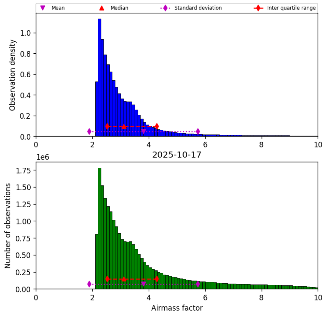
Figure 37: Histogram of “Airmass factor” for 2025-10-17 to 2025-10-18
