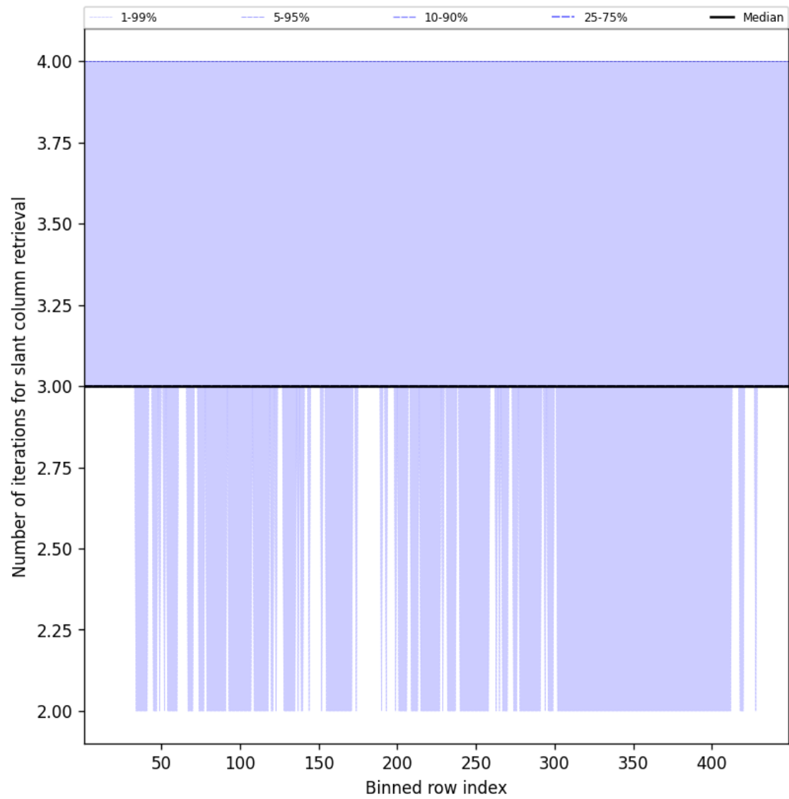
Figure 45: Along track statistics of “Number of iterations for slant column retrieval” for 2025-10-18 to 2025-10-19
