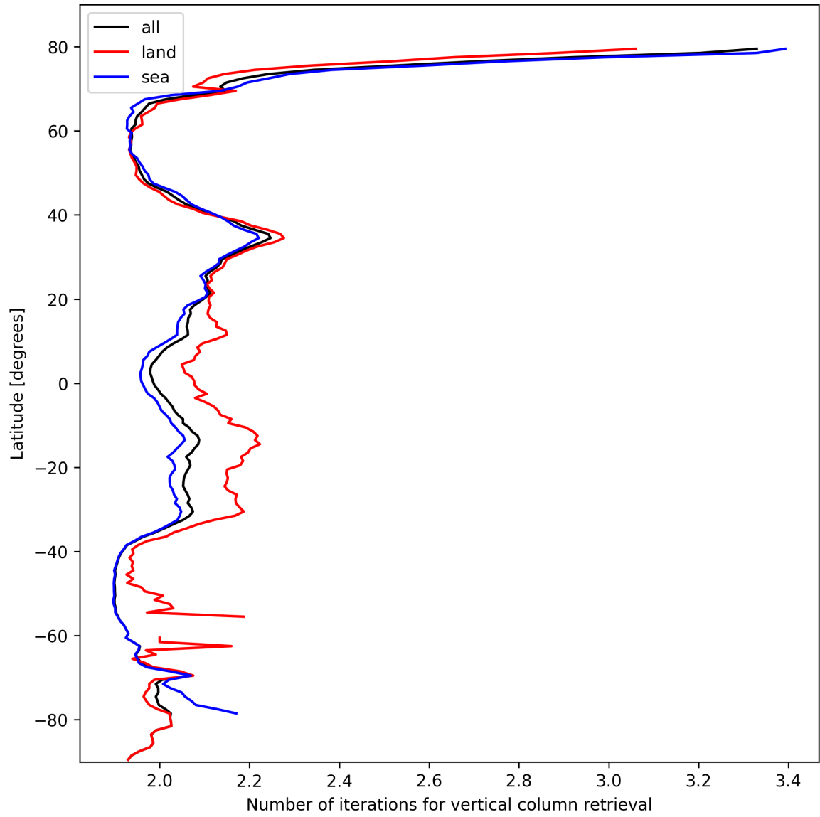
Figure 27: Zonal average of “Number of iterations for vertical column retrieval” for 2025-10-18 to 2025-10-19.
