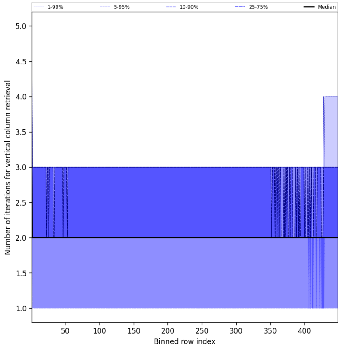
Figure 51: Along track statistics of “Number of iterations for vertical column retrieval” for 2025-10-18 to 2025-10-19
