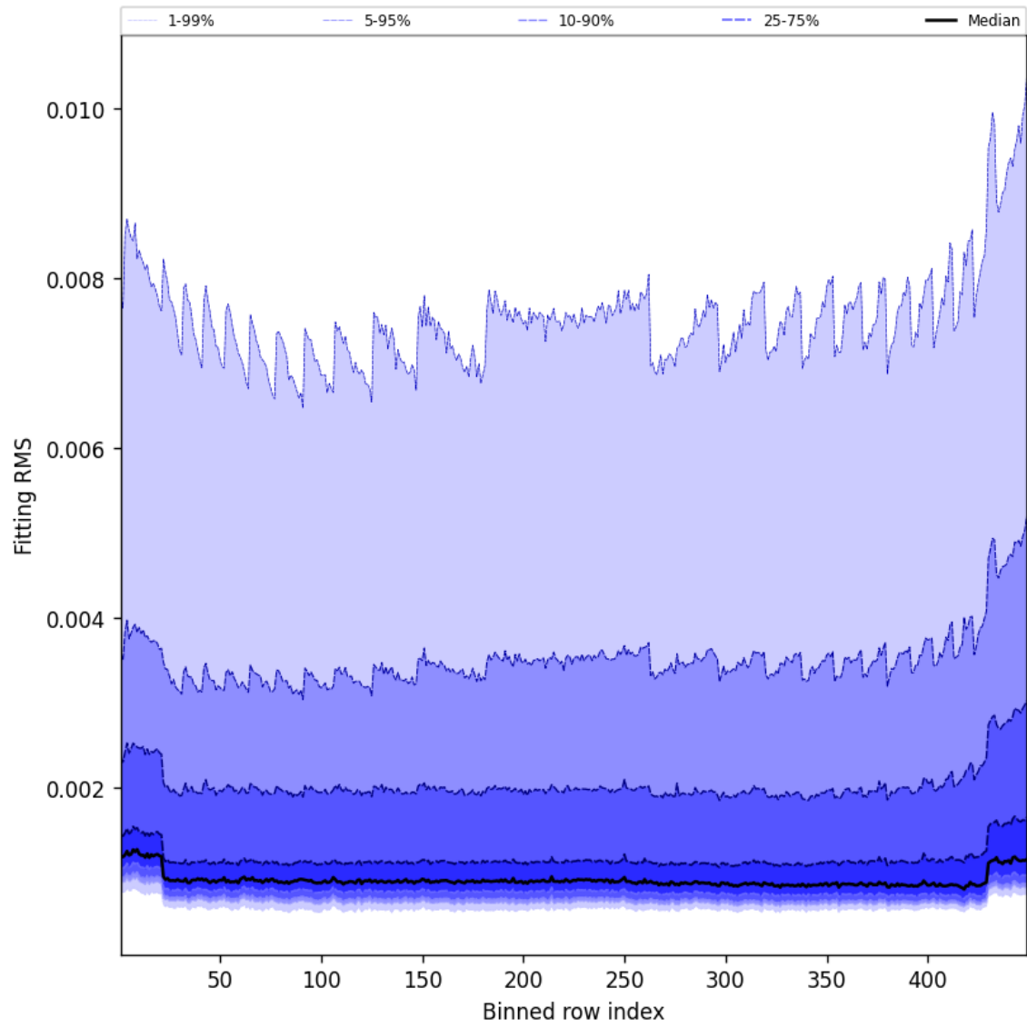
Figure 46: Along track statistics of “Fitting RMS” for 2025-10-18 to 2025-10-19
