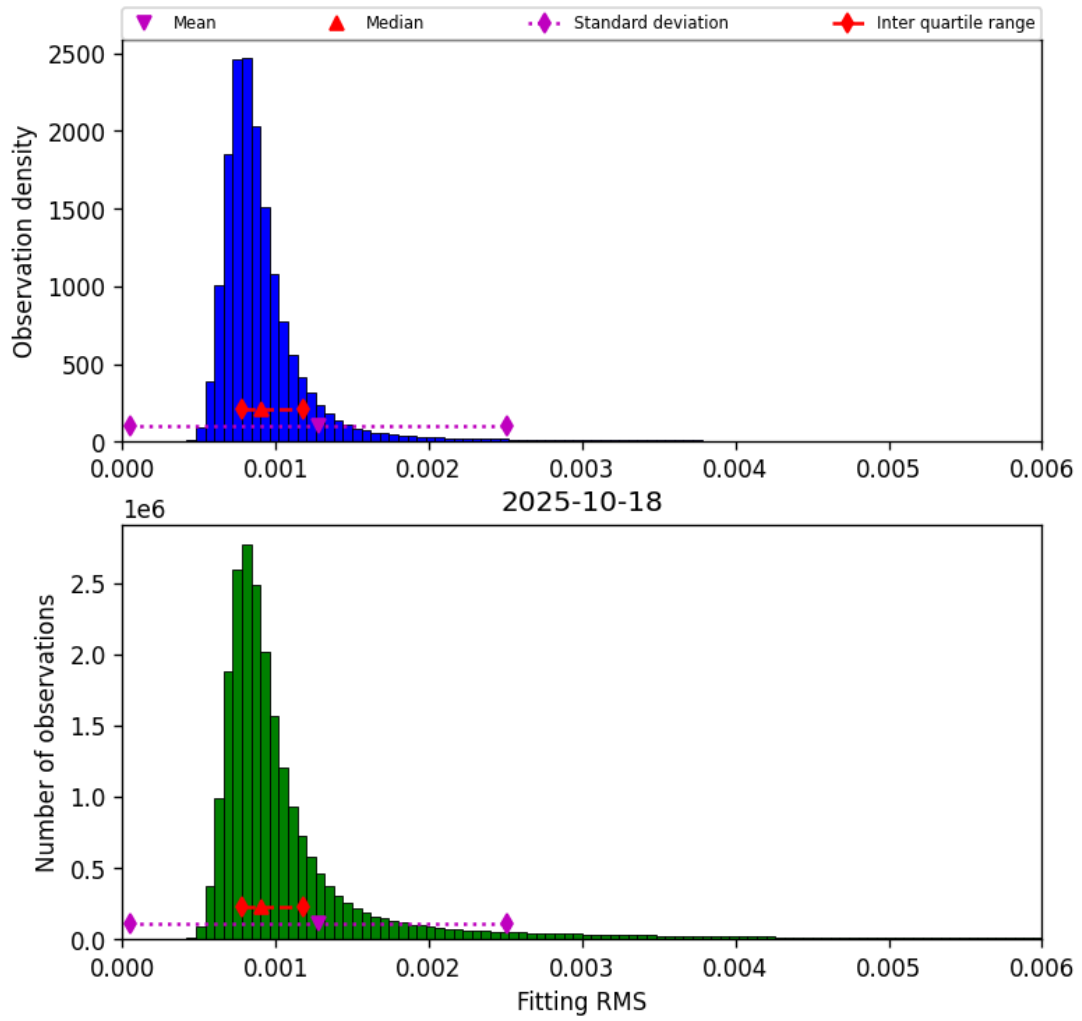
Figure 34: Histogram of “Fitting RMS” for 2025-10-18 to 2025-10-19
