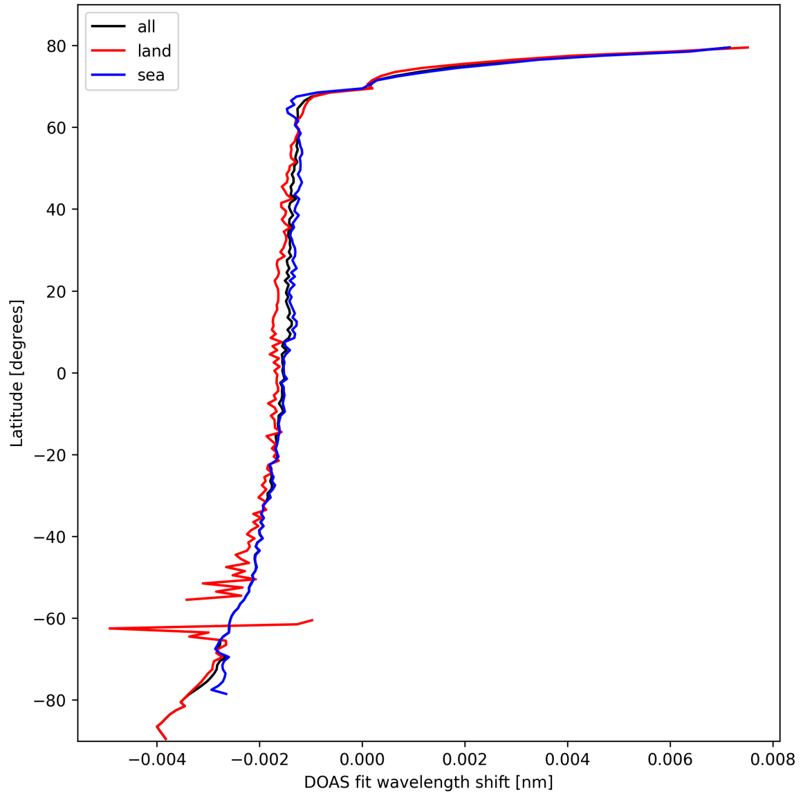
Figure 23: Zonal average of “DOAS fit wavelength shift” for 2025-10-18 to 2025-10-19.
