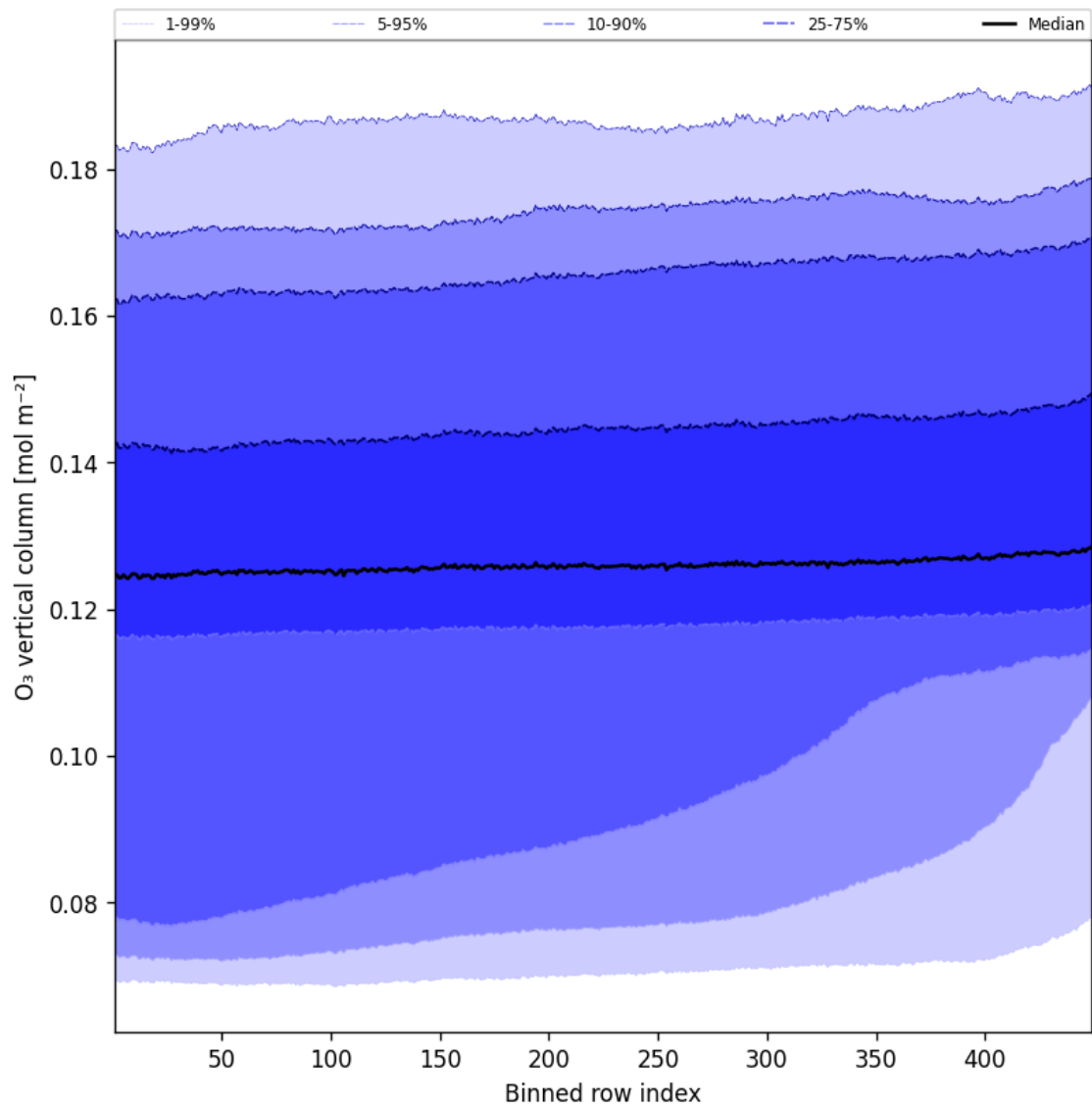
Figure 41: Along track statistics of “O 3 vertical column” for 2025-10-18 to 2025-10-19
