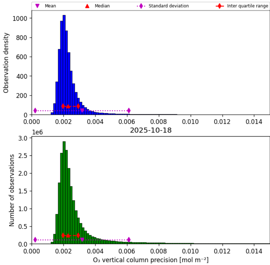
Figure 30: Histogram of “O 3 vertical column precision” for 2025-10-18 to 2025-10-19
