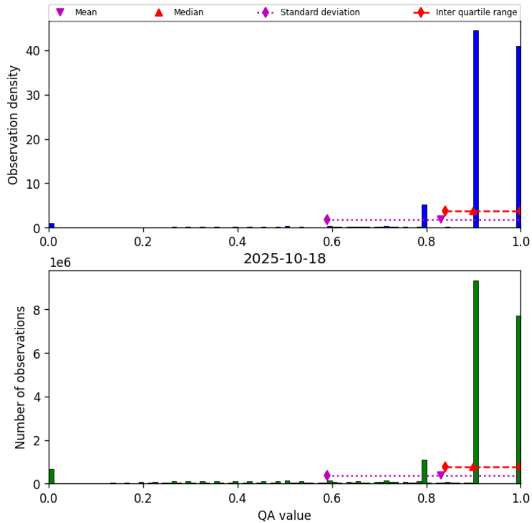
Figure 28: Histogram of “QA value” for 2025-10-18 to 2025-10-19
