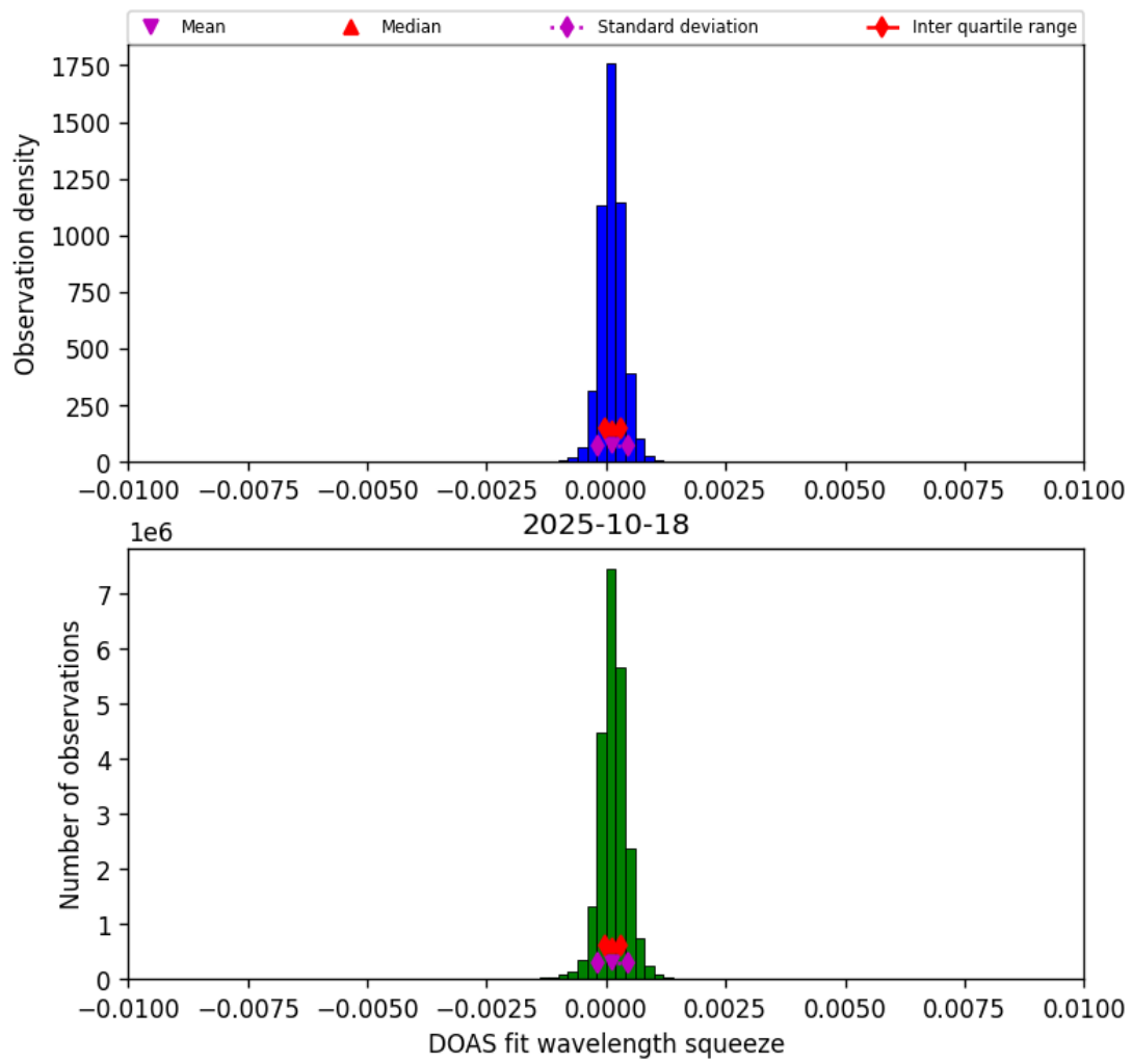
Figure 36: Histogram of “DOAS fit wavelength squeeze” for 2025-10-18 to 2025-10-19
