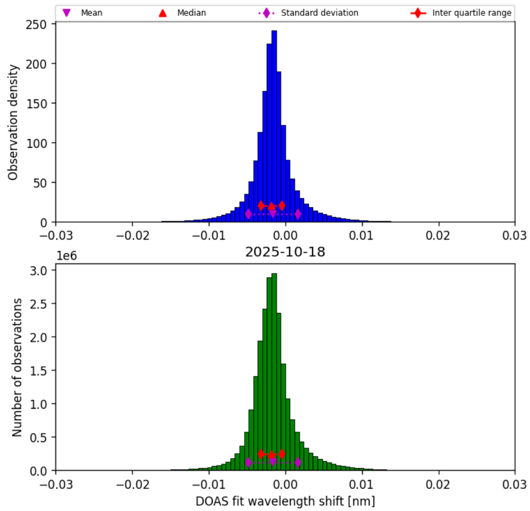
Figure 35: Histogram of “DOAS fit wavelength shift” for 2025-10-18 to 2025-10-19
