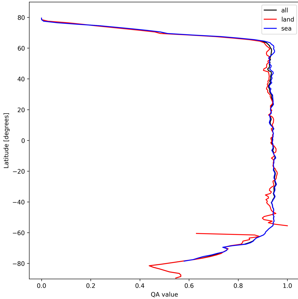
Figure 16: Zonal average of “QA value” for 2025-10-18 to 2025-10-19.
