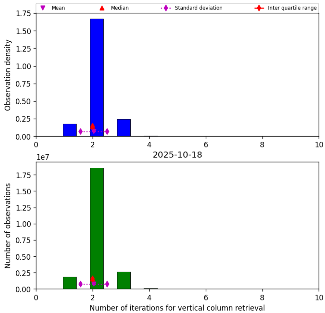
Figure 39: Histogram of “Number of iterations for vertical column retrieval” for 2025-10-18 to 2025-10-19
