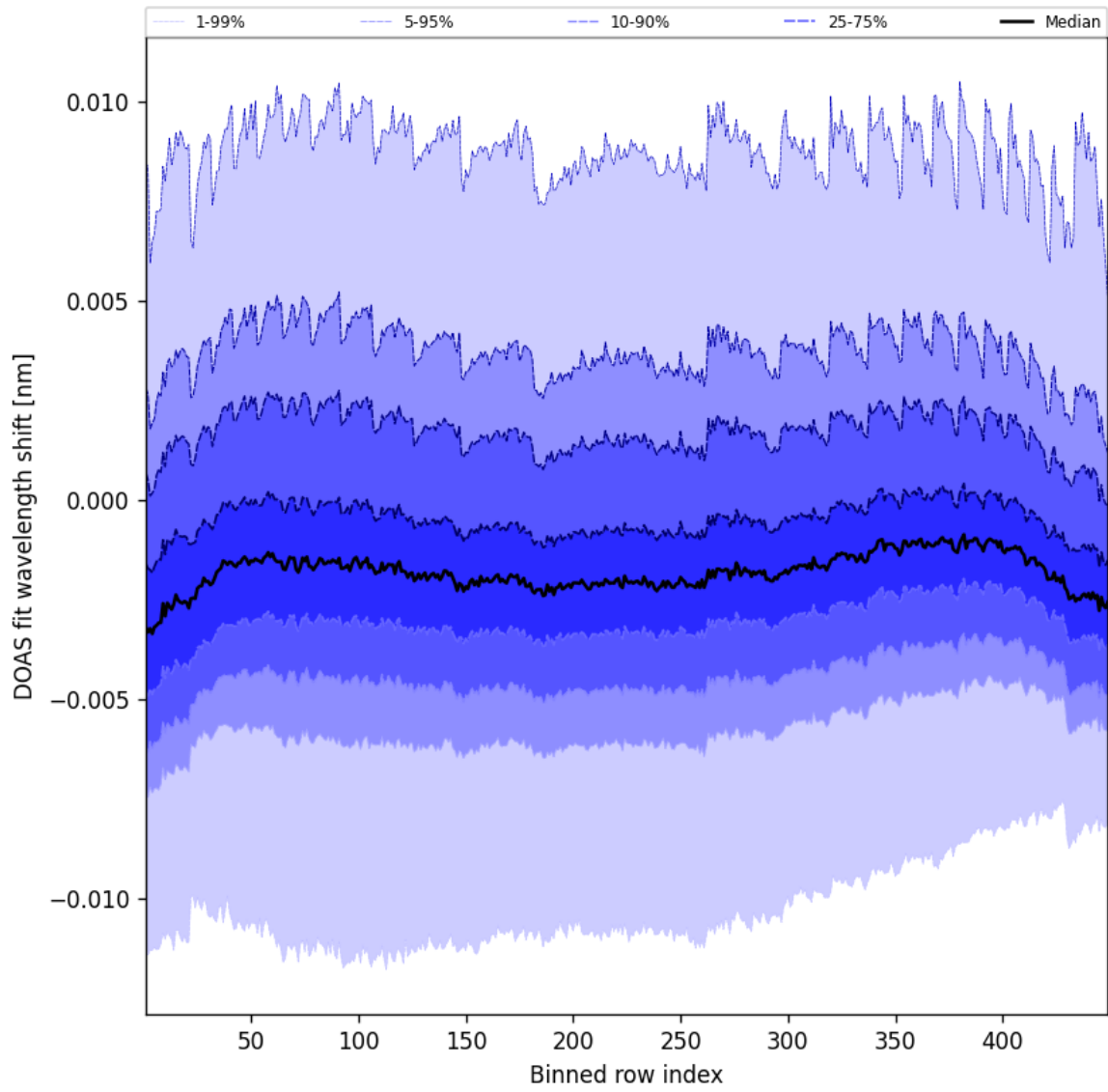
Figure 47: Along track statistics of “DOAS fit wavelength shift” for 2025-10-18 to 2025-10-19
