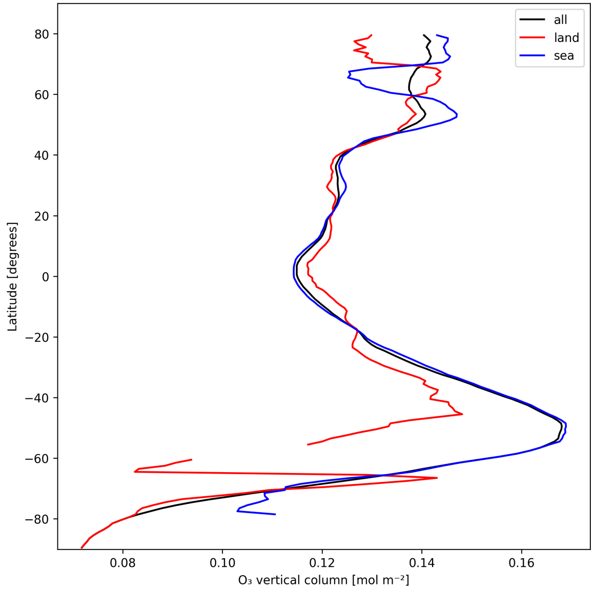
Figure 17: Zonal average of “O 3 vertical column” for 2025-10-18 to 2025-10-19.
