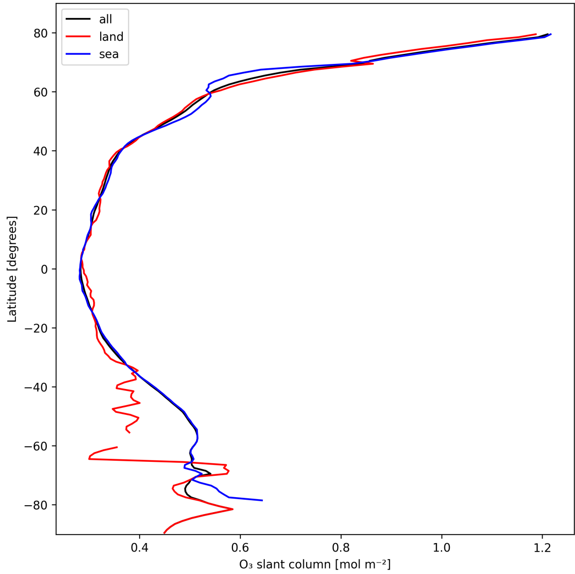
Figure 19: Zonal average of “O 3 slant column” for 2025-10-18 to 2025-10-19.
