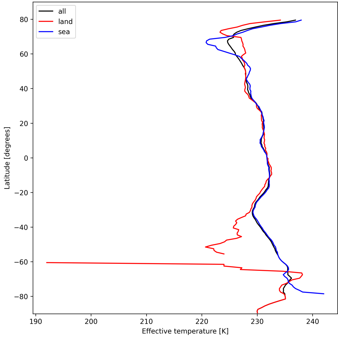
Figure 26: Zonal average of "Effective temperature" for 2025-10-18 to 2025-10-19.
