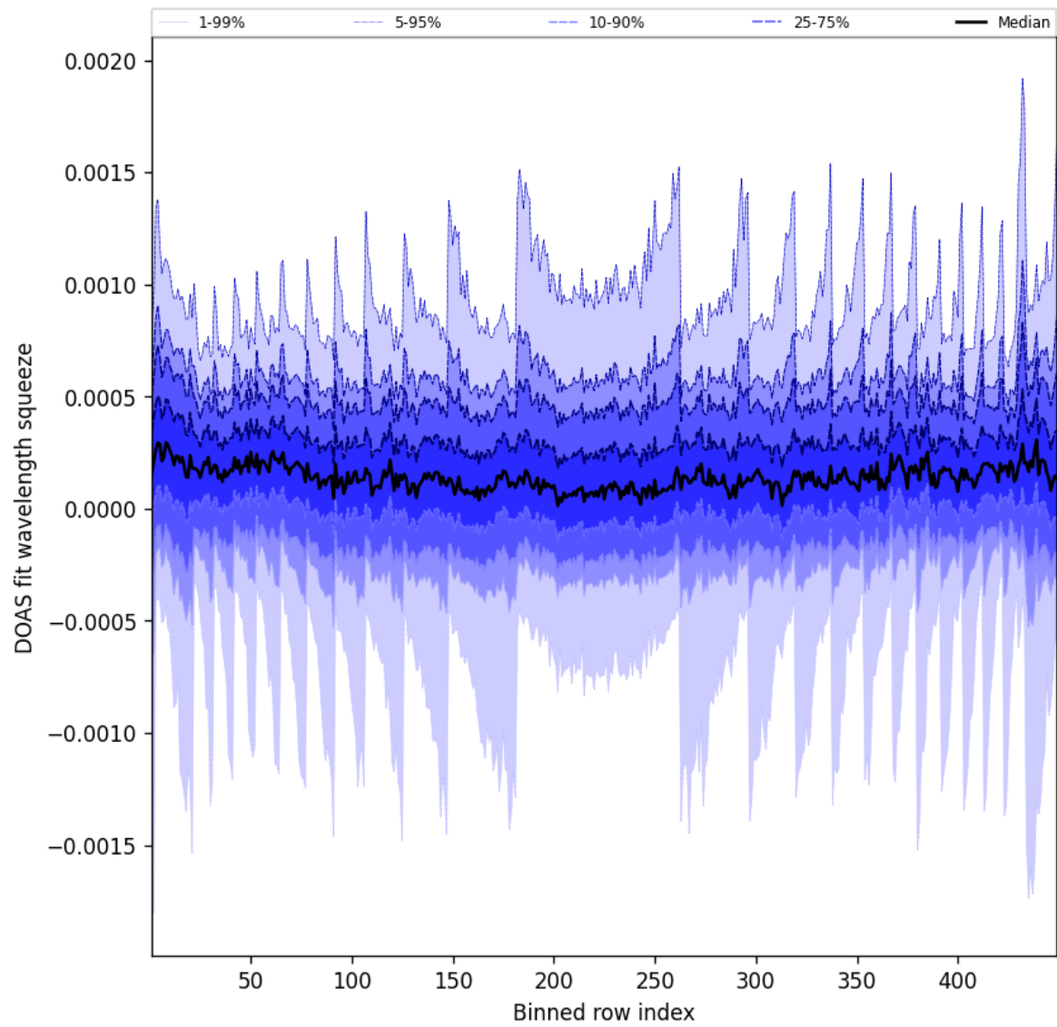
Figure 48: Along track statistics of “DOAS fit wavelength squeeze” for 2025-10-18 to 2025-10-19
