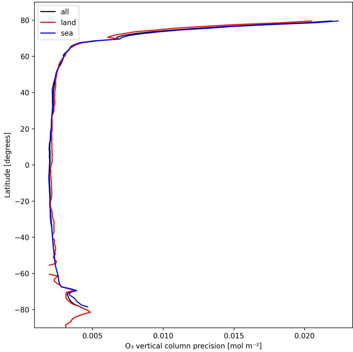
Figure 18: Zonal average of “O 3 vertical column precision” for 2025-10-18 to 2025-10-19.
