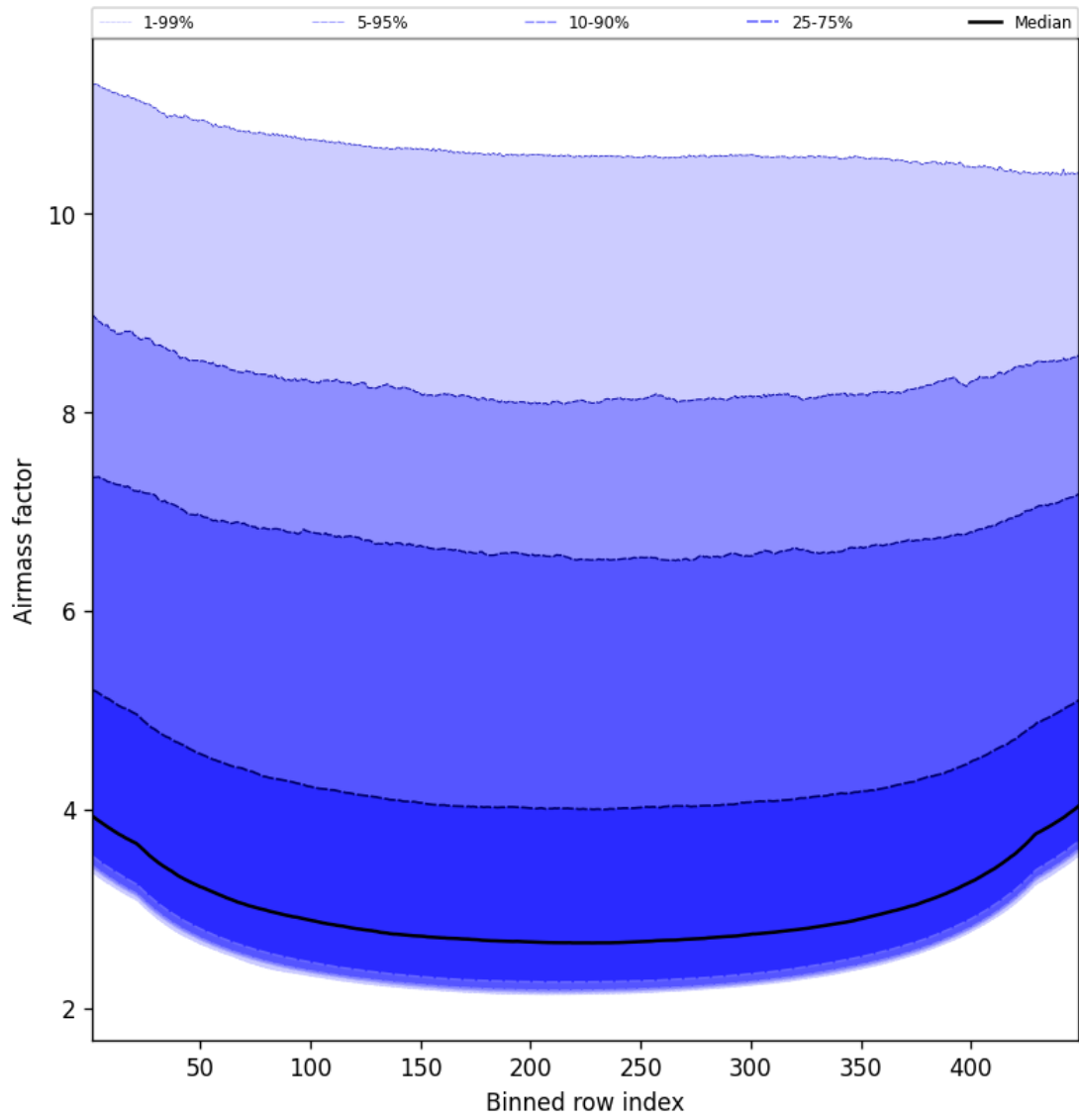
Figure 49: Along track statistics of “Airmass factor” for 2025-10-18 to 2025-10-19
