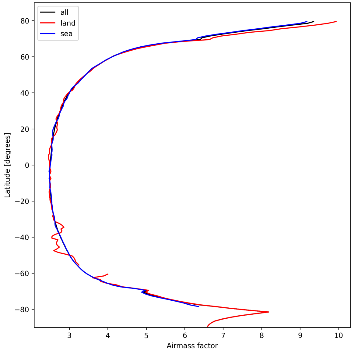
Figure 25: Zonal average of “Airmass factor” for 2025-10-18 to 2025-10-19.
