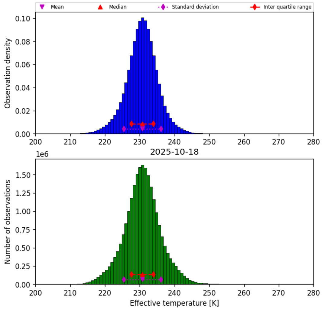
Figure 38: Histogram of “Effective temperature” for 2025-10-18 to 2025-10-19
