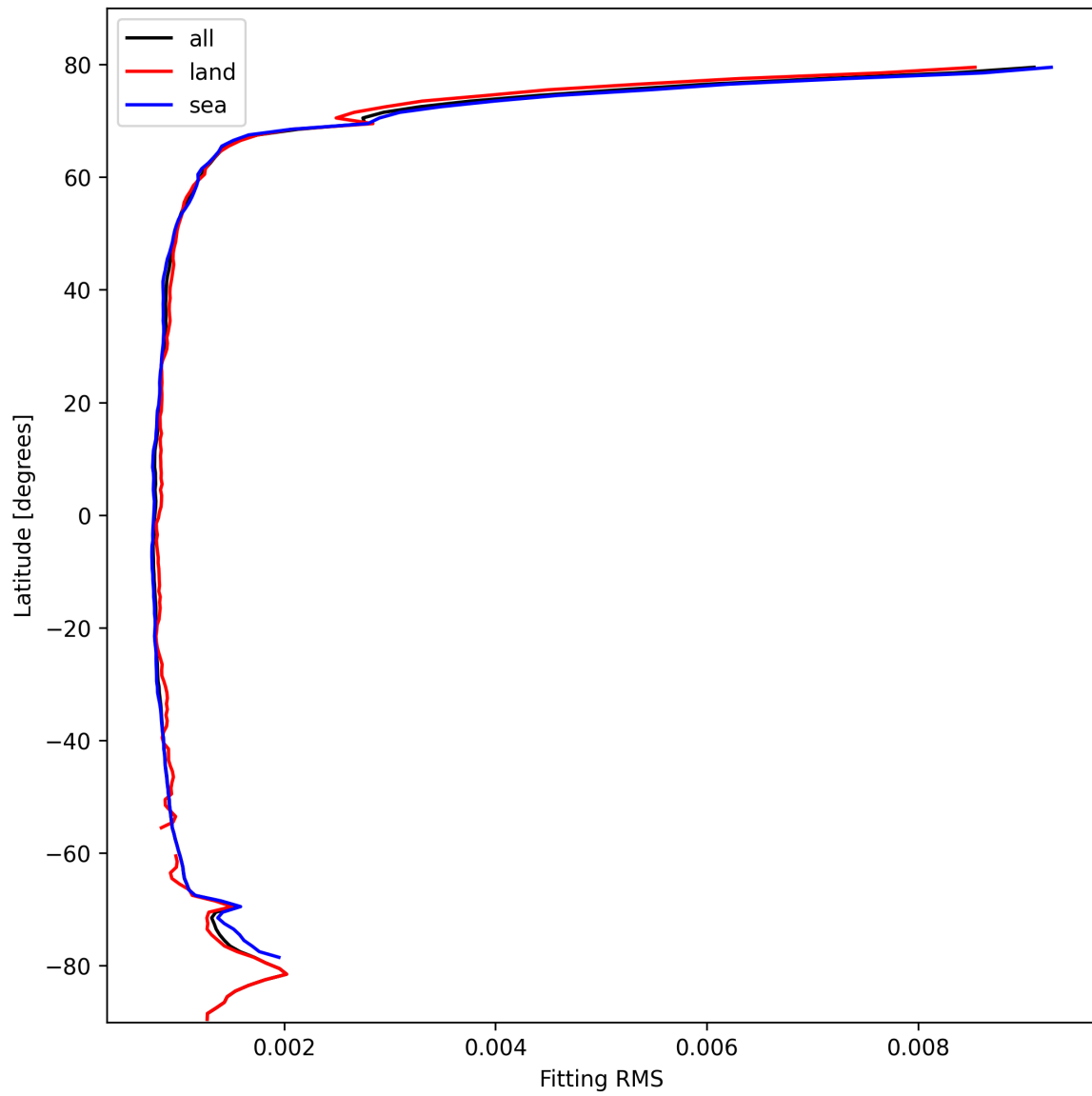
Figure 22: Zonal average of “Fitting RMS” for 2025-10-18 to 2025-10-19.
