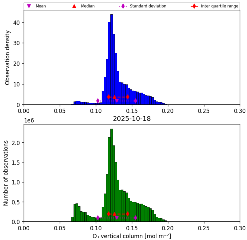
Figure 29: Histogram of “O 3 vertical column” for 2025-10-18 to 2025-10-19
