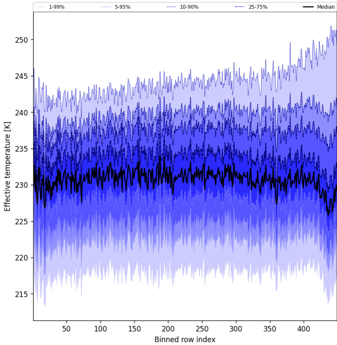
Figure 50: Along track statistics of “Effective temperature” for 2025-10-18 to 2025-10-19
