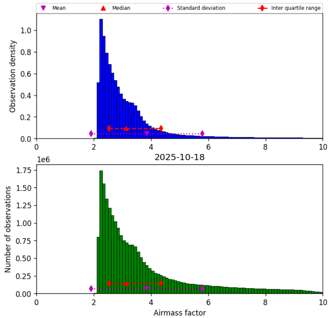
Figure 37: Histogram of “Airmass factor” for 2025-10-18 to 2025-10-19
