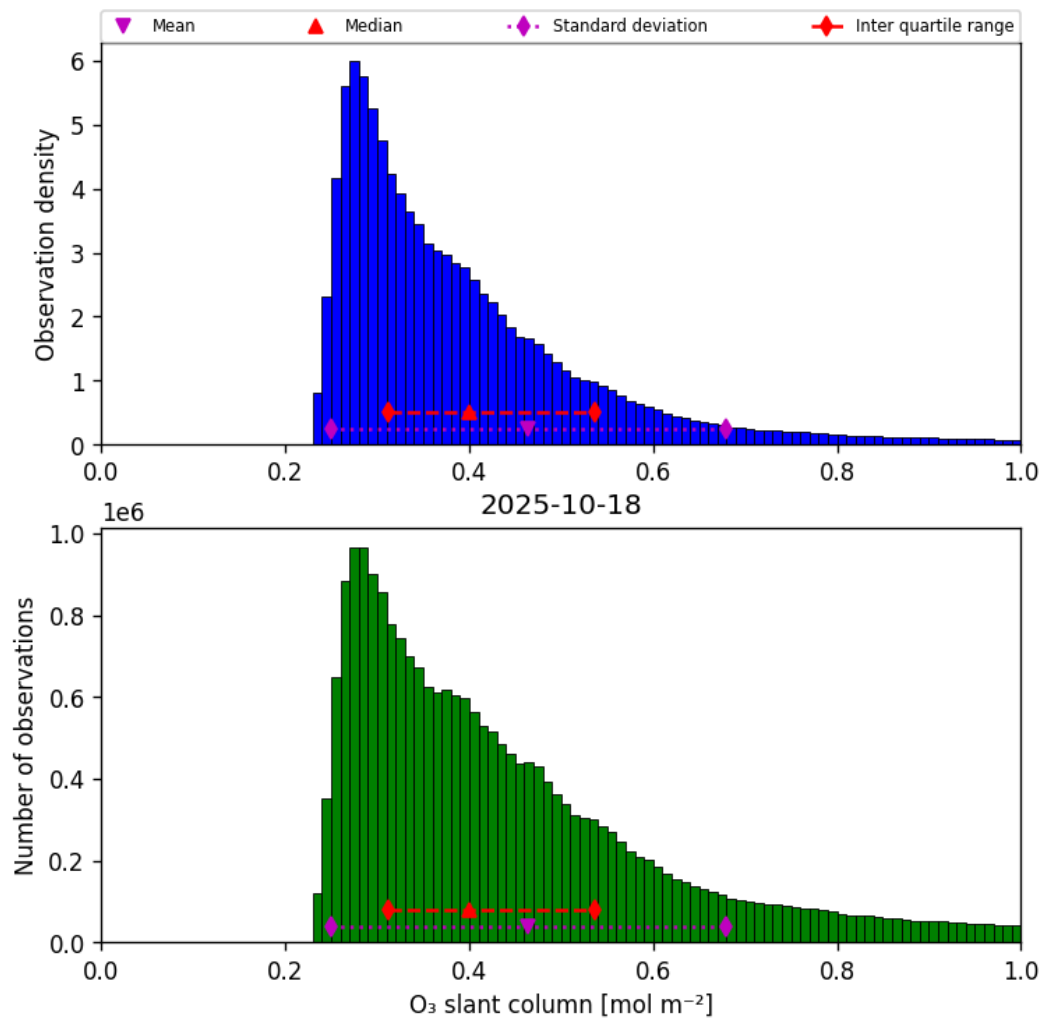
Figure 31: Histogram of “O 3 slant column” for 2025-10-18 to 2025-10-19
