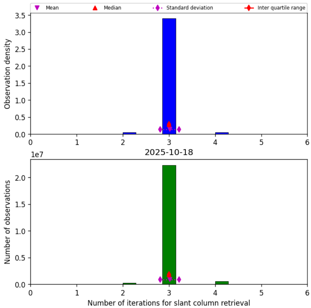
Figure 33: Histogram of "Number of iterations for slant column retrieval" for 2025-10-18 to 2025-10-19
