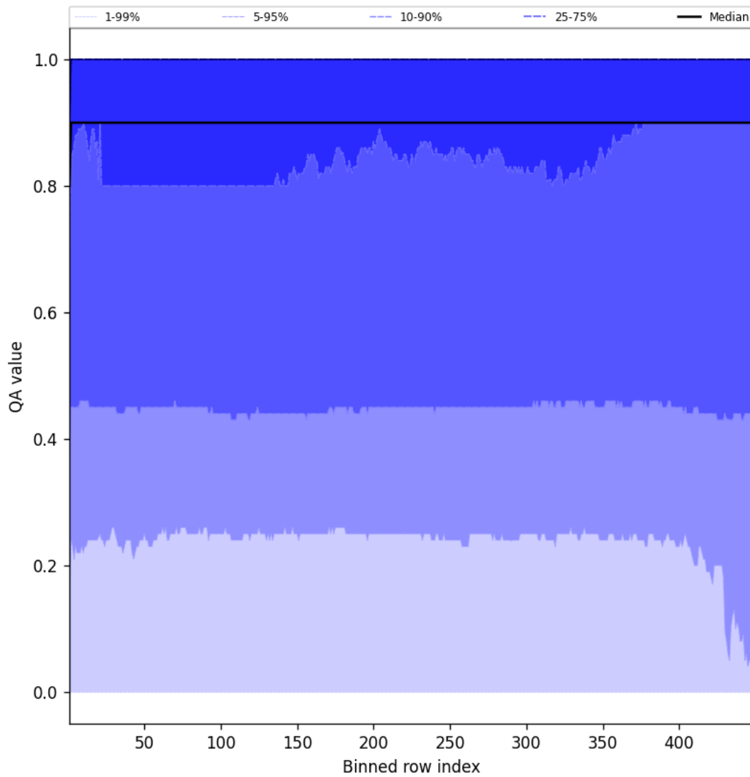
Figure 40: Along track statistics of “QA value” for 2025-10-18 to 2025-10-19
