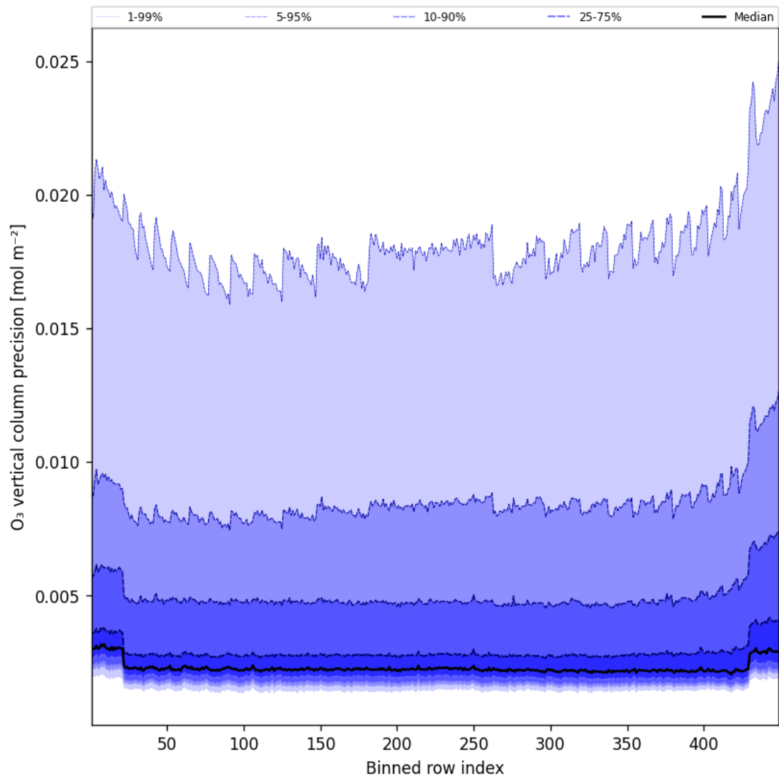
Figure 42: Along track statistics of “O 3 vertical column precision” for 2025-10-18 to 2025-10-19
