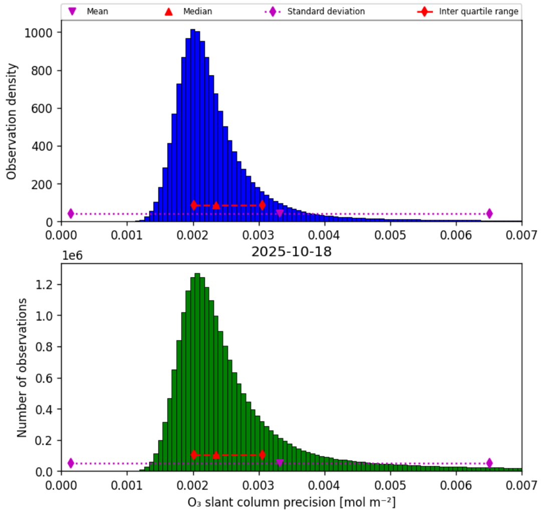
Figure 32: Histogram of “O 3 slant column precision” for 2025-10-18 to 2025-10-19
