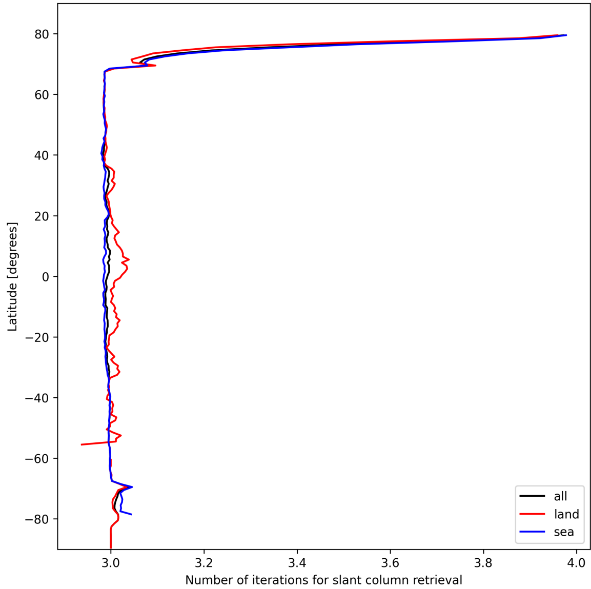
Figure 21: Zonal average of “Number of iterations for slant column retrieval” for 2025-10-18 to 2025-10-19.
