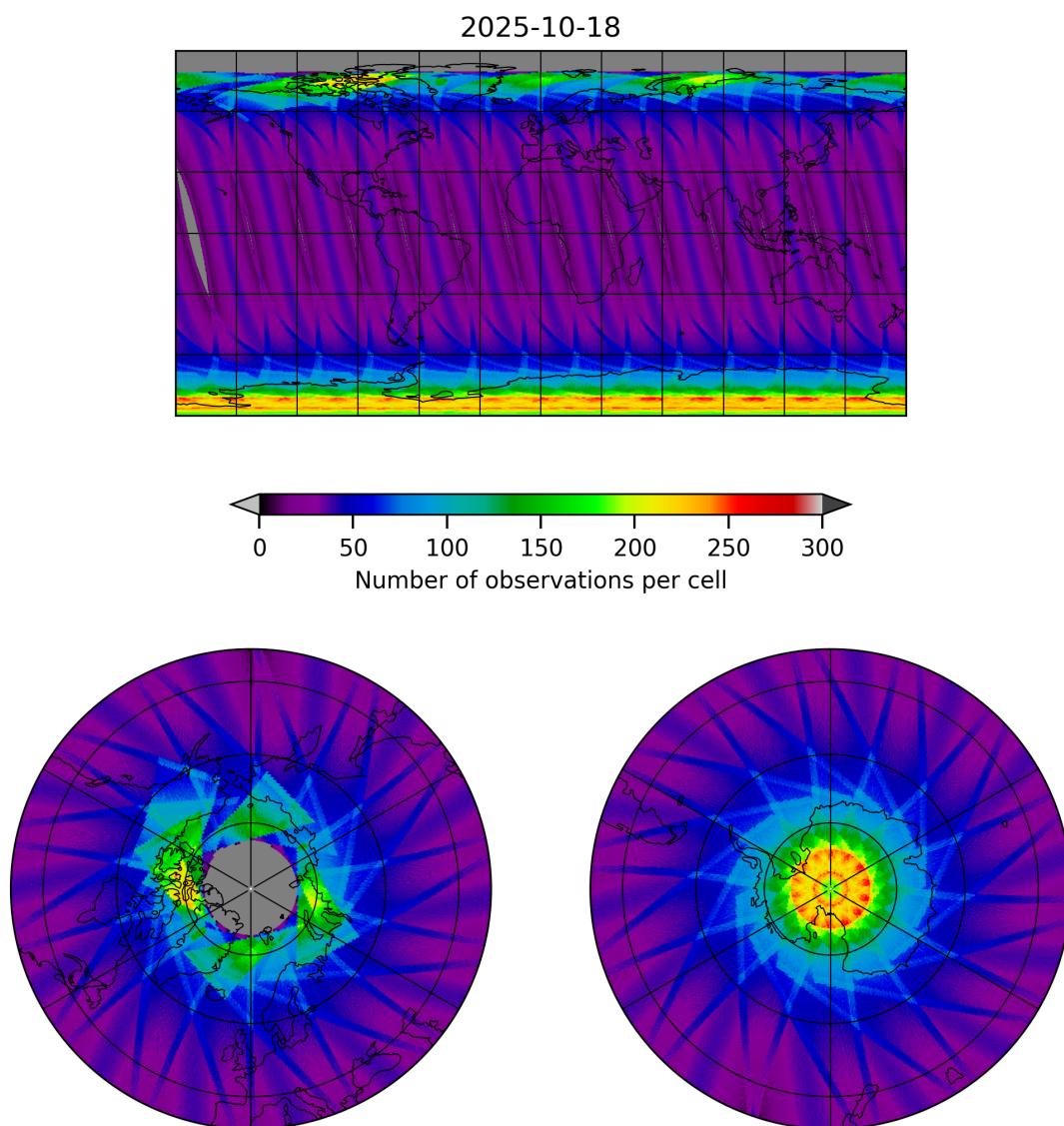
Figure 15: Map of the number of observations for 2025-10-18 to 2025-10-19
