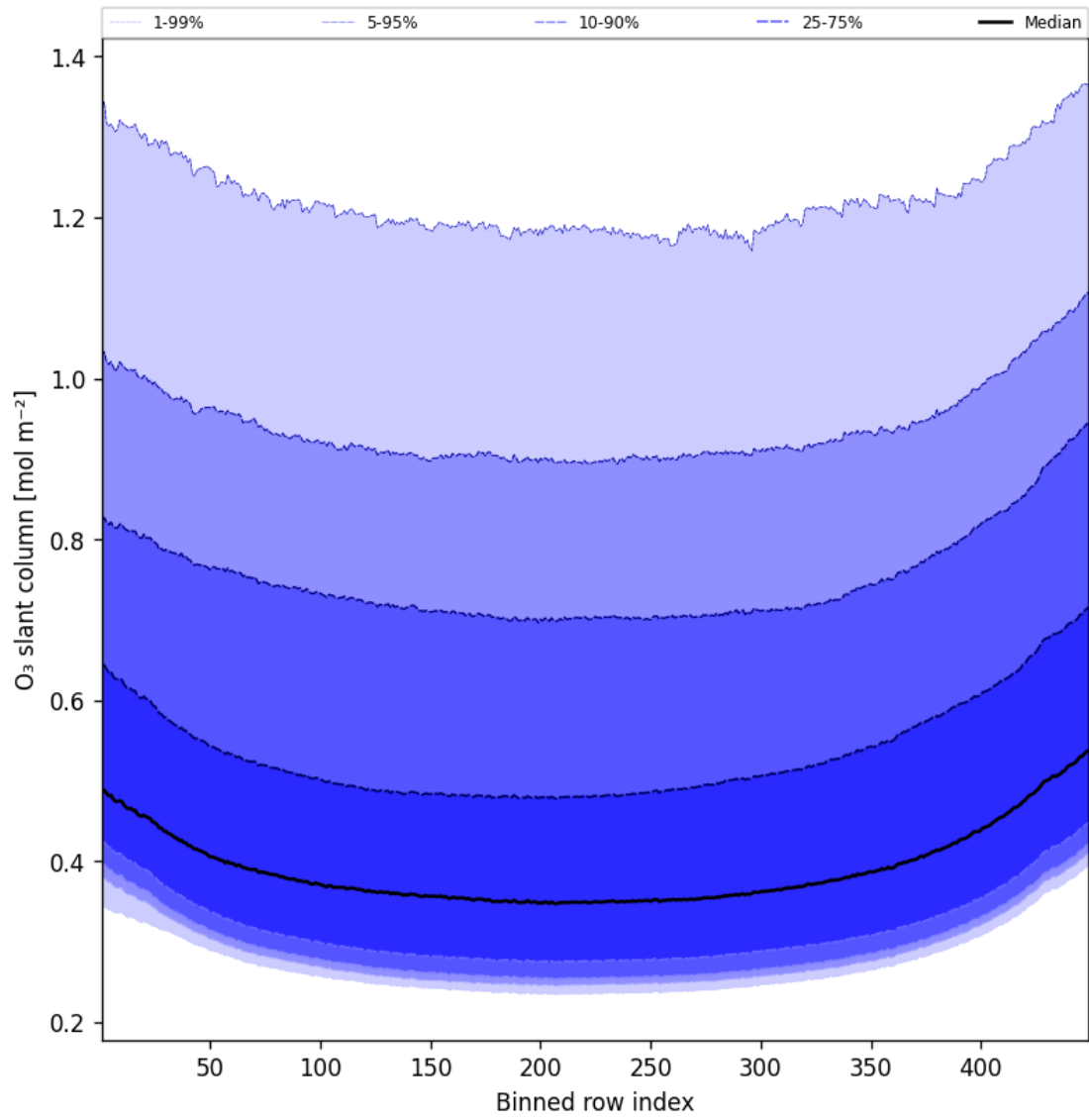
Figure 43: Along track statistics of “O 3 slant column” for 2025-10-18 to 2025-10-19
