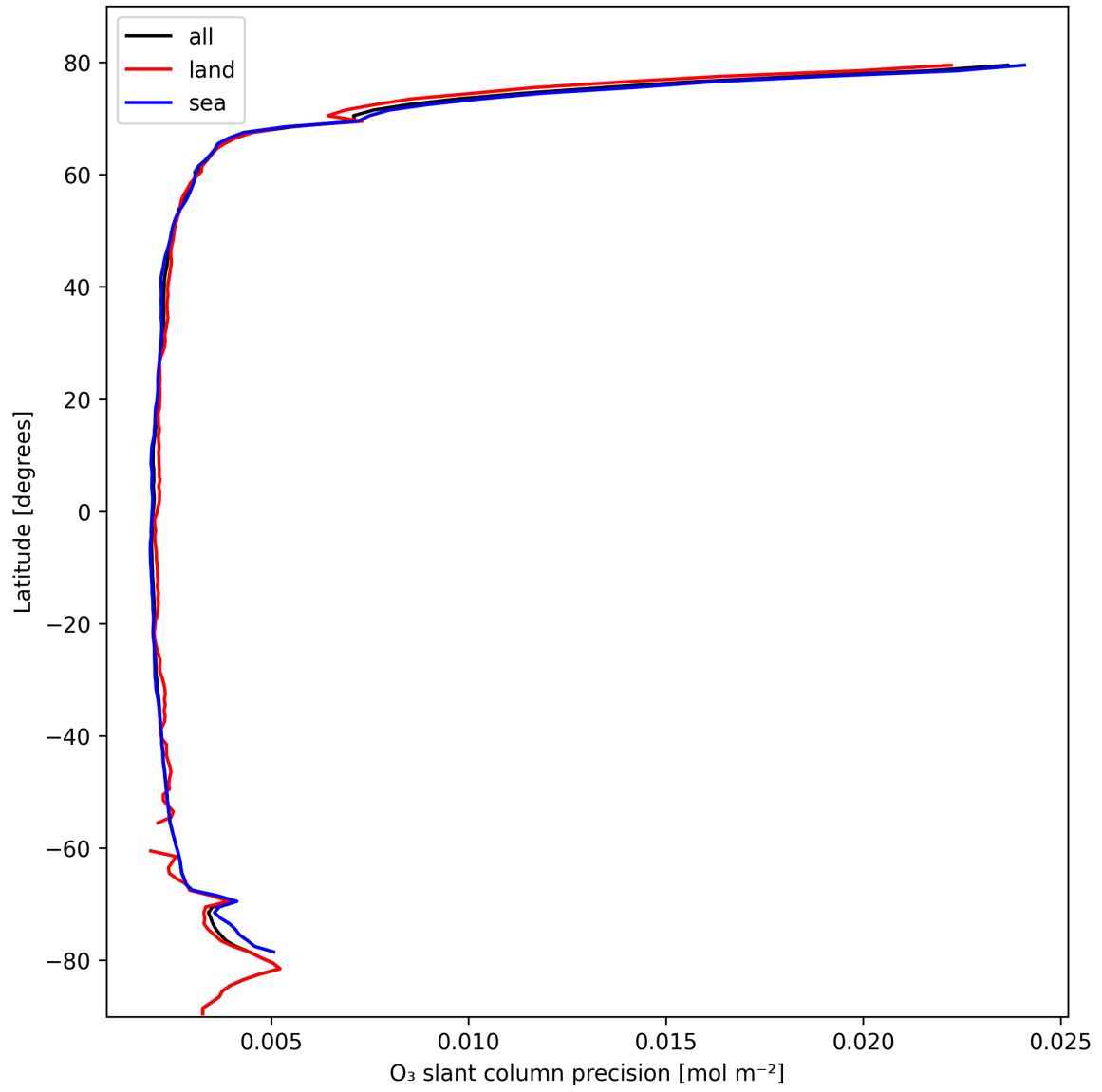
Figure 20: Zonal average of “O 3 slant column precision” for 2025-10-18 to 2025-10-19.
