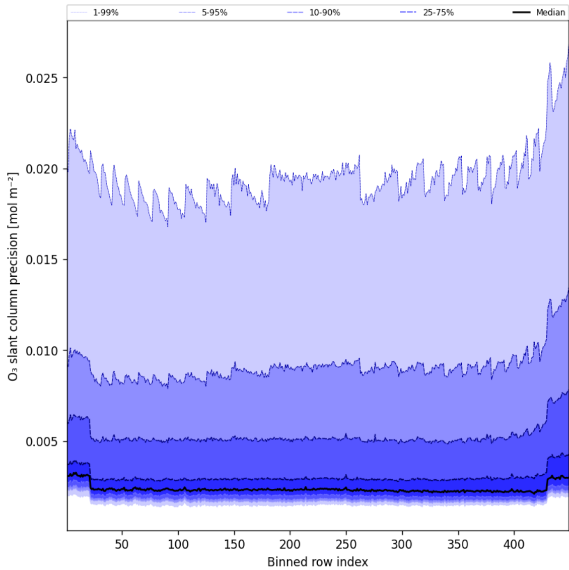
Figure 44: Along track statistics of “O 3 slant column precision” for 2025-10-18 to 2025-10-19
