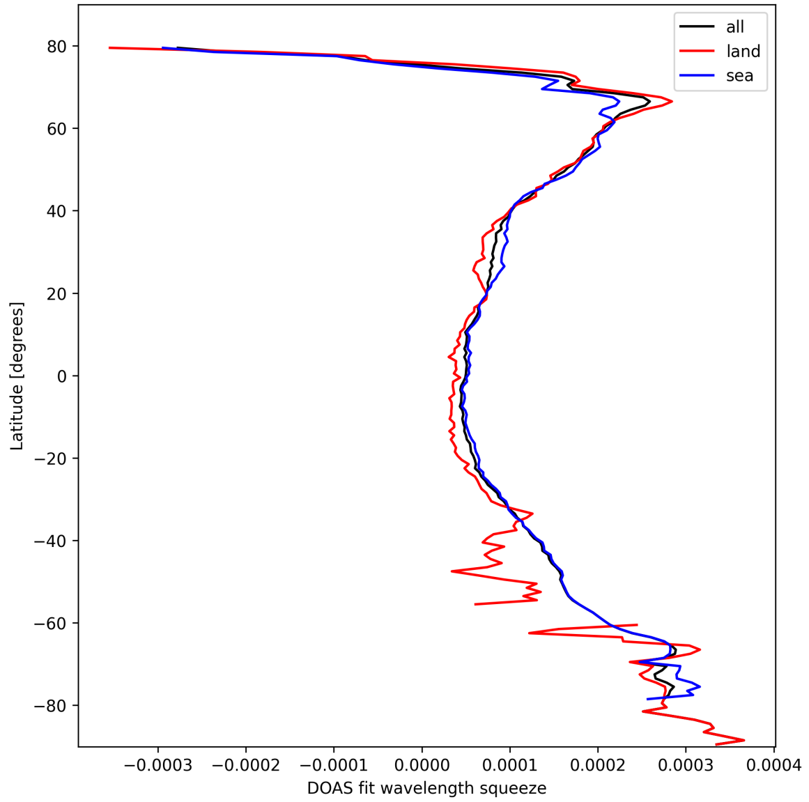
Figure 24: Zonal average of “DOAS fit wavelength squeeze” for 2025-10-18 to 2025-10-19.
