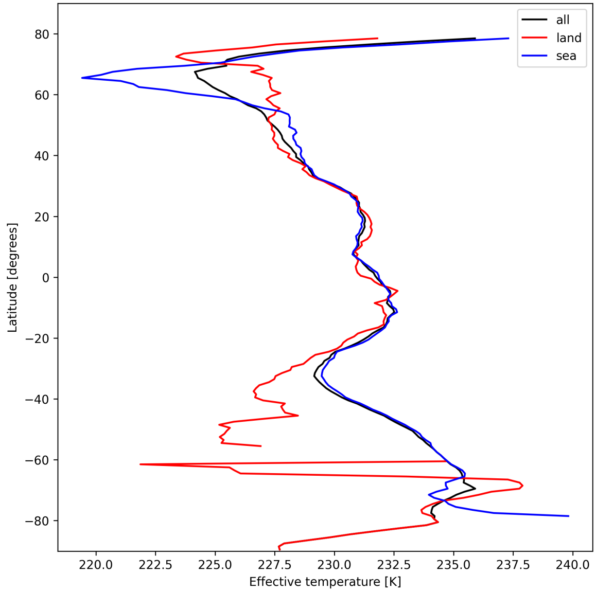
Figure 26: Zonal average of “Effective temperature” for 2025-10-19 to 2025-10-20.
