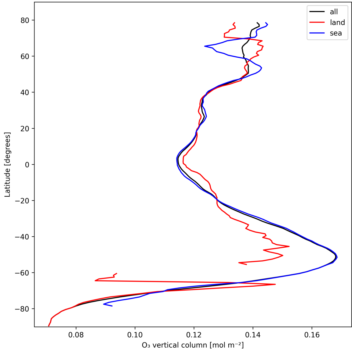
Figure 17: Zonal average of “O 3 vertical column” for 2025-10-19 to 2025-10-20.
