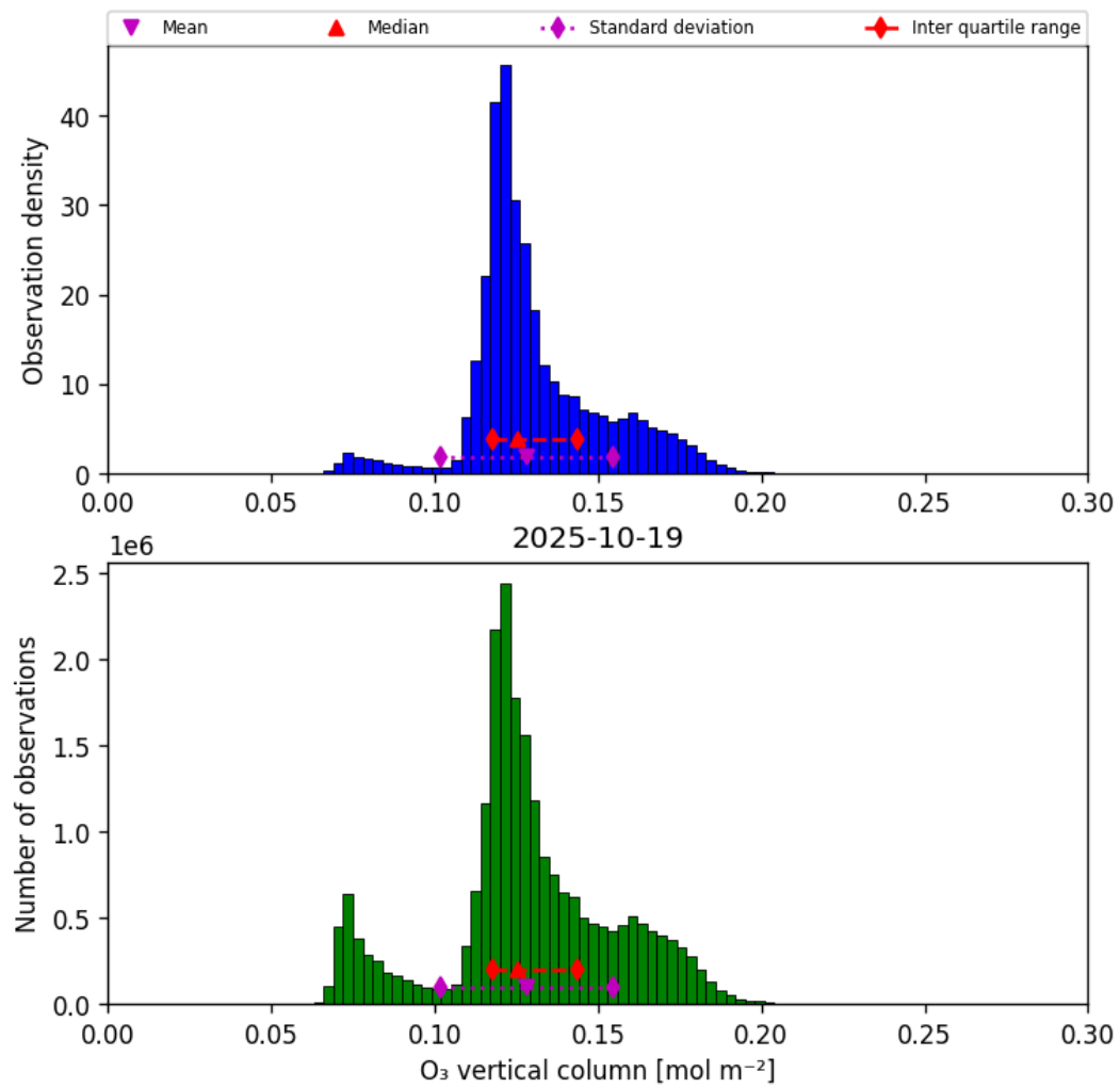
Figure 29: Histogram of “O 3 vertical column” for 2025-10-19 to 2025-10-20
