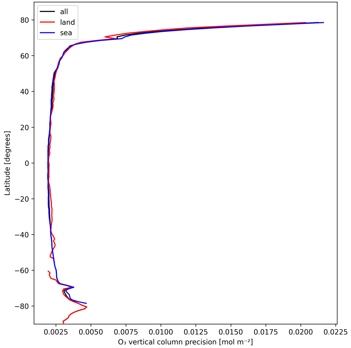
Figure 18: Zonal average of “O 3 vertical column precision” for 2025-10-19 to 2025-10-20.
