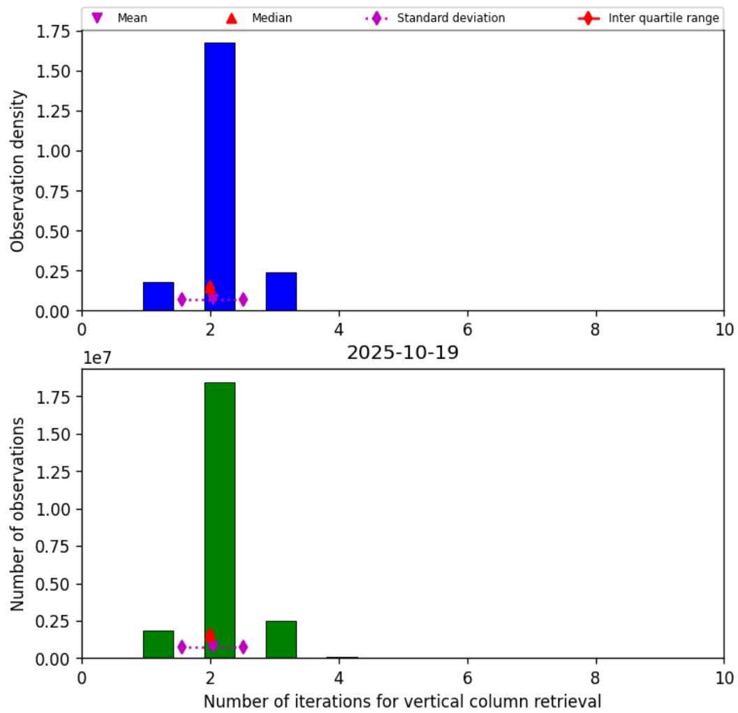
Figure 39: Histogram of “Number of iterations for vertical column retrieval” for 2025-10-19 to 2025-10-20
