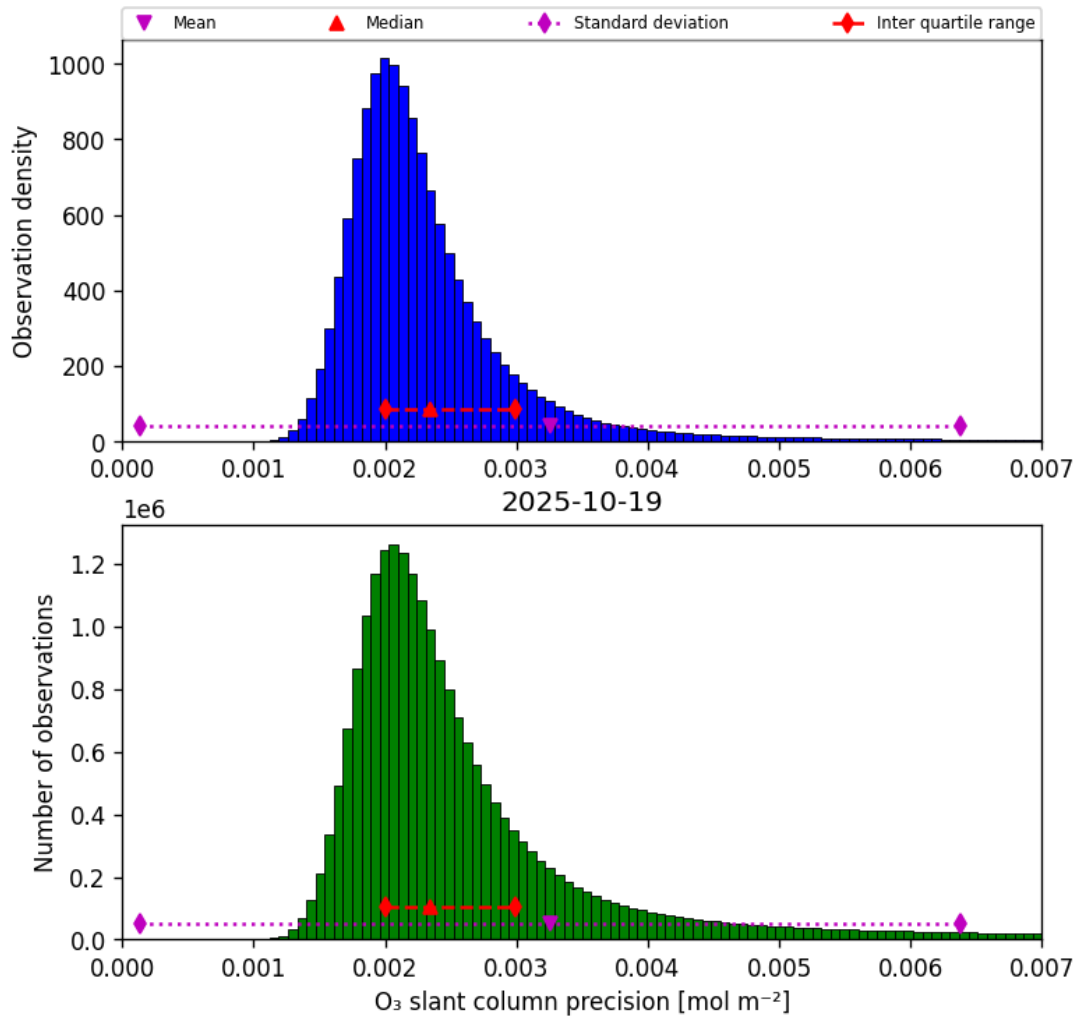
Figure 32: Histogram of “O 3 slant column precision” for 2025-10-19 to 2025-10-20
