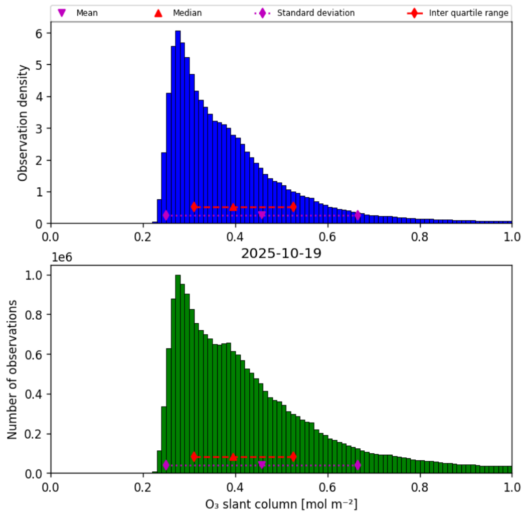
Figure 31: Histogram of “O 3 slant column” for 2025-10-19 to 2025-10-20
