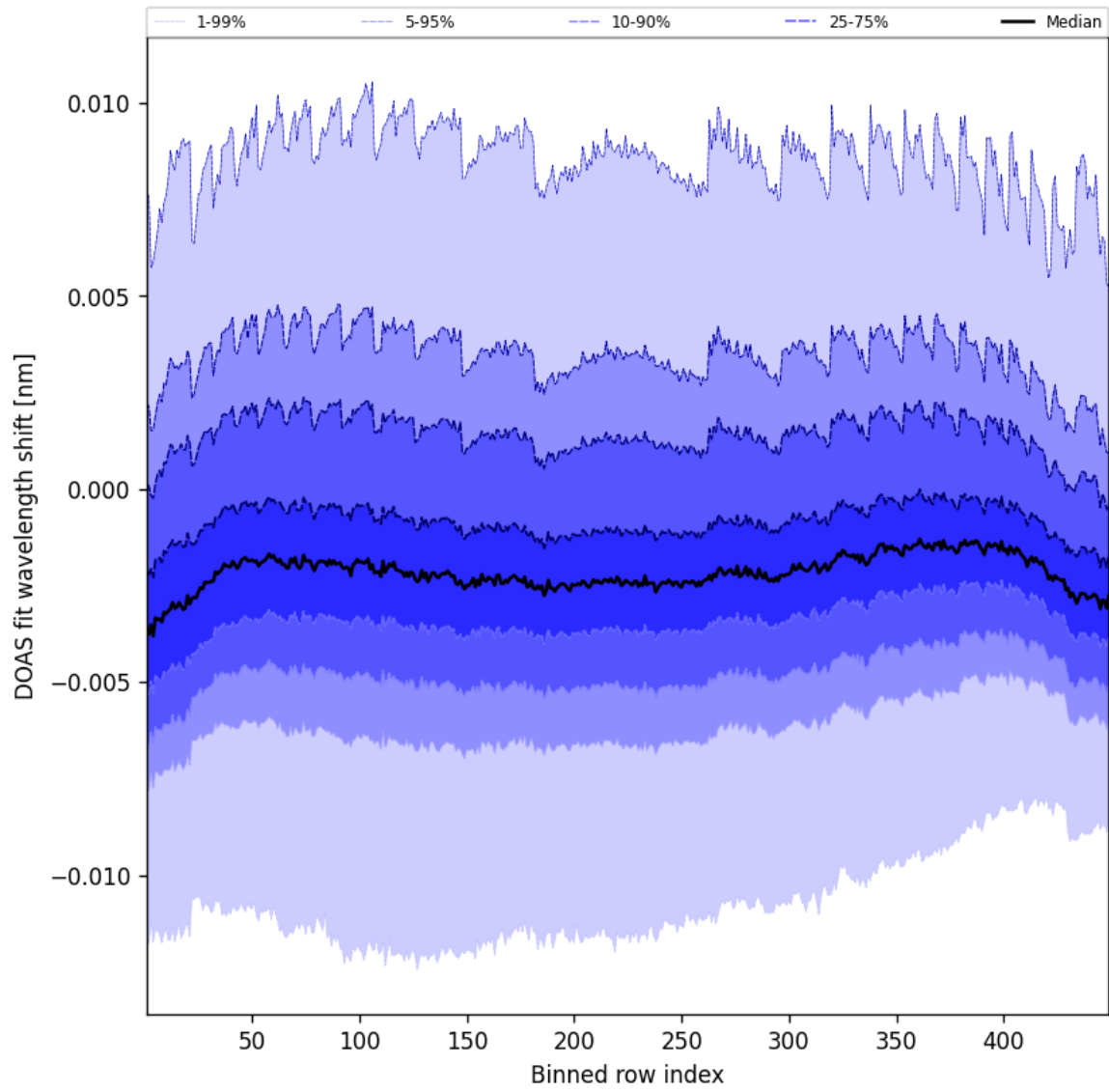
Figure 47: Along track statistics of “DOAS fit wavelength shift” for 2025-10-19 to 2025-10-20
