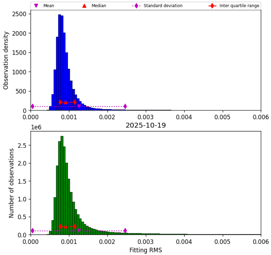
Figure 34: Histogram of “Fitting RMS” for 2025-10-19 to 2025-10-20
