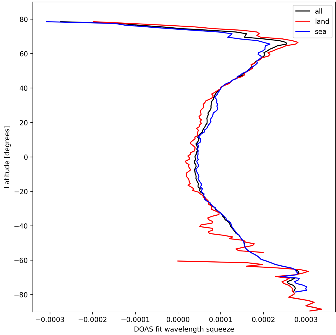
Figure 24: Zonal average of “DOAS fit wavelength squeeze” for 2025-10-19 to 2025-10-20.
