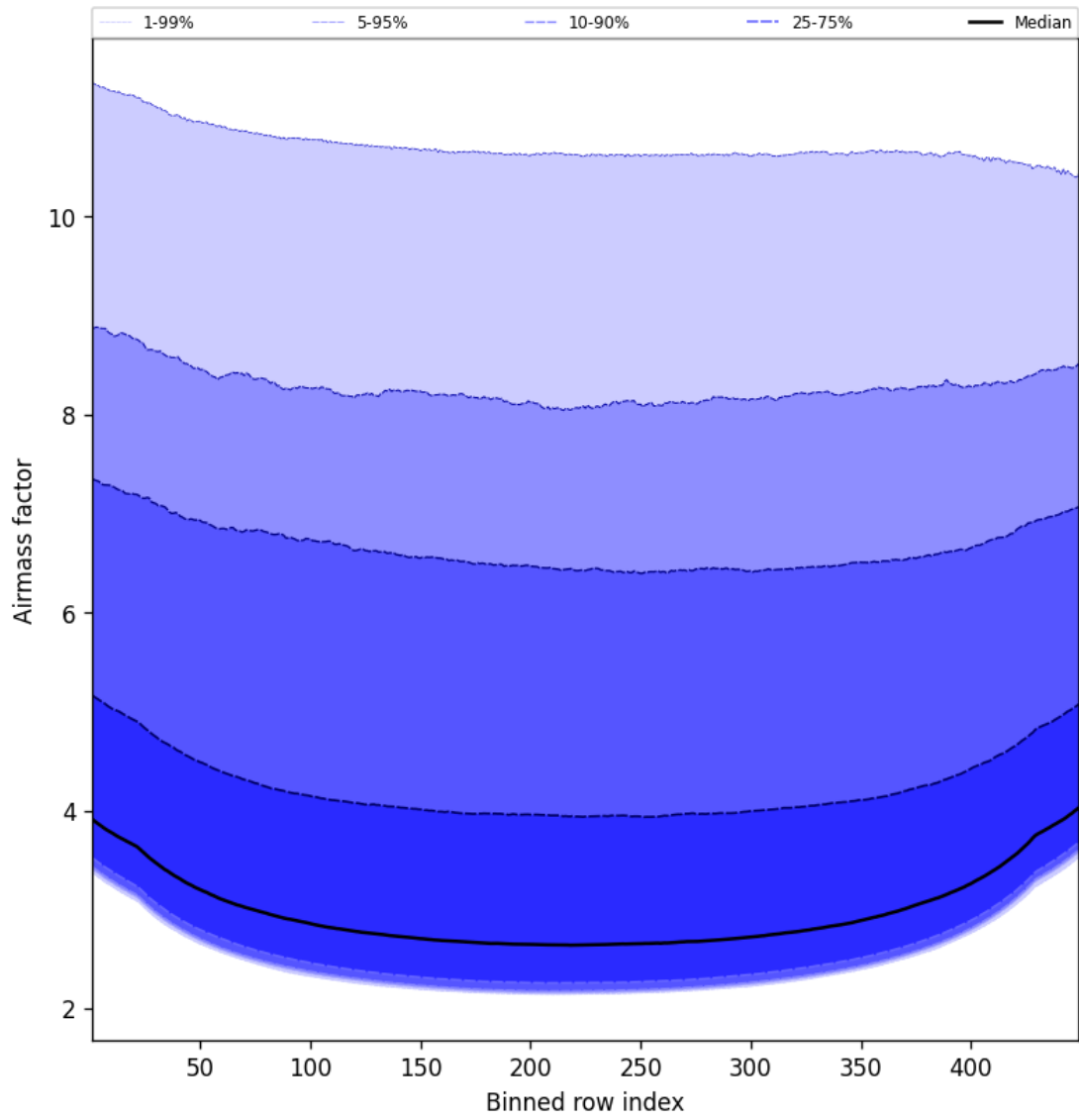
Figure 49: Along track statistics of “Airmass factor” for 2025-10-19 to 2025-10-20
