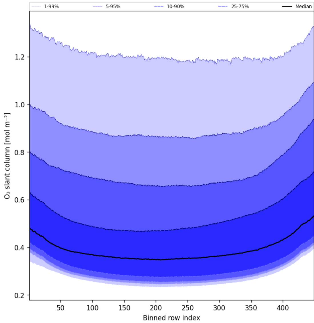
Figure 43: Along track statistics of “O 3 slant column” for 2025-10-19 to 2025-10-20
