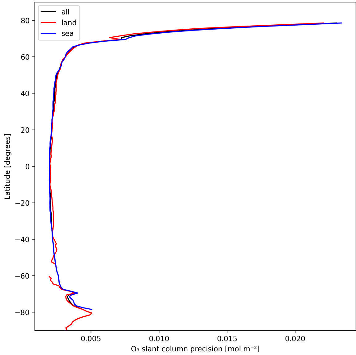
Figure 20: Zonal average of "O 3 slant column precision" for 2025-10-19 to 2025-10-20.
