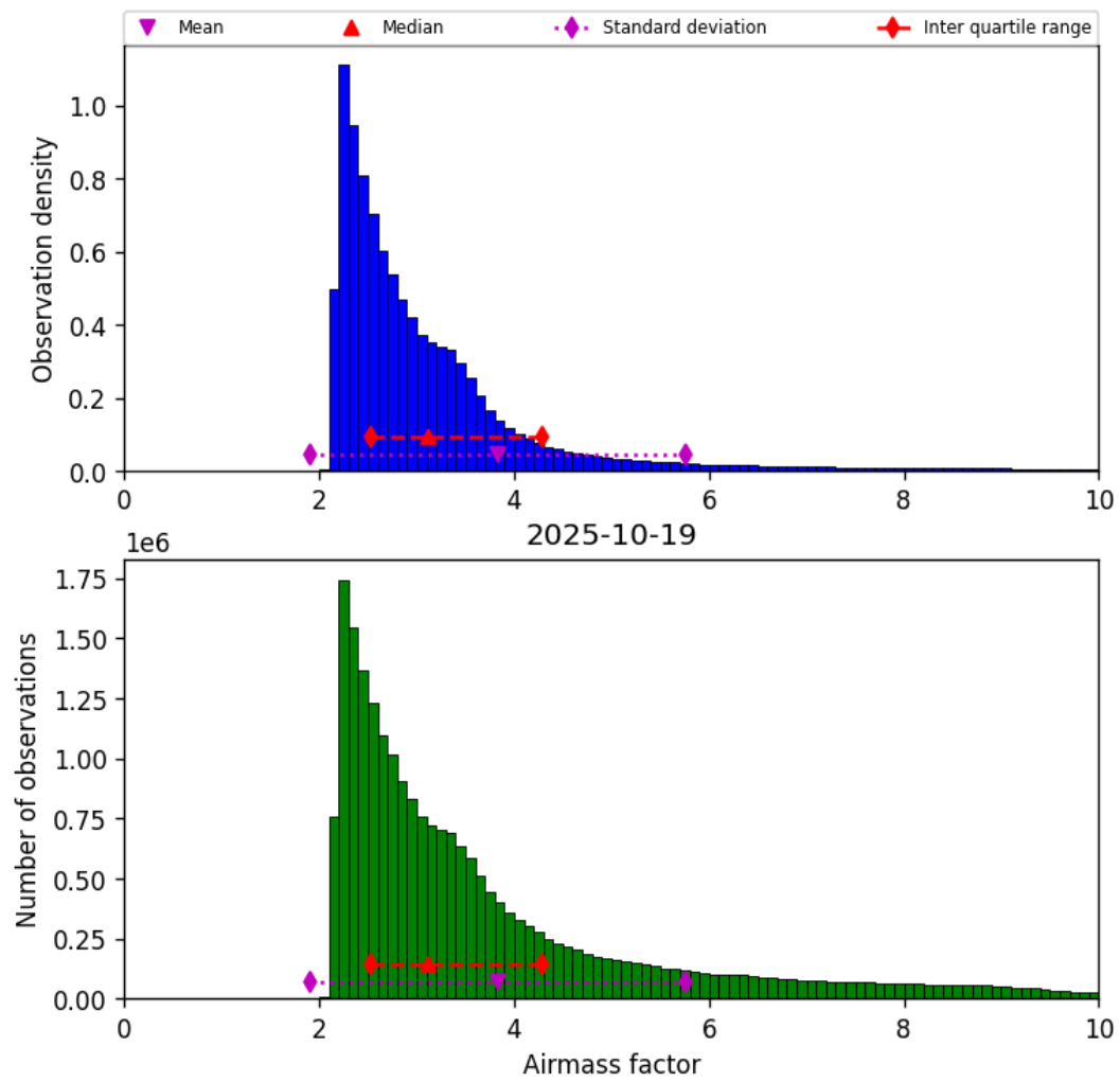
Figure 37: Histogram of “Airmass factor” for 2025-10-19 to 2025-10-20
