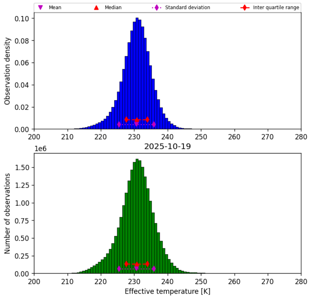
Figure 38: Histogram of “Effective temperature” for 2025-10-19 to 2025-10-20
