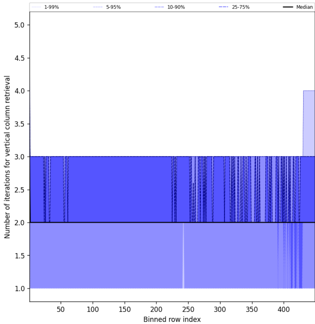
Figure 51: Along track statistics of “Number of iterations for vertical column retrieval” for 2025-10-19 to 2025-10-20
