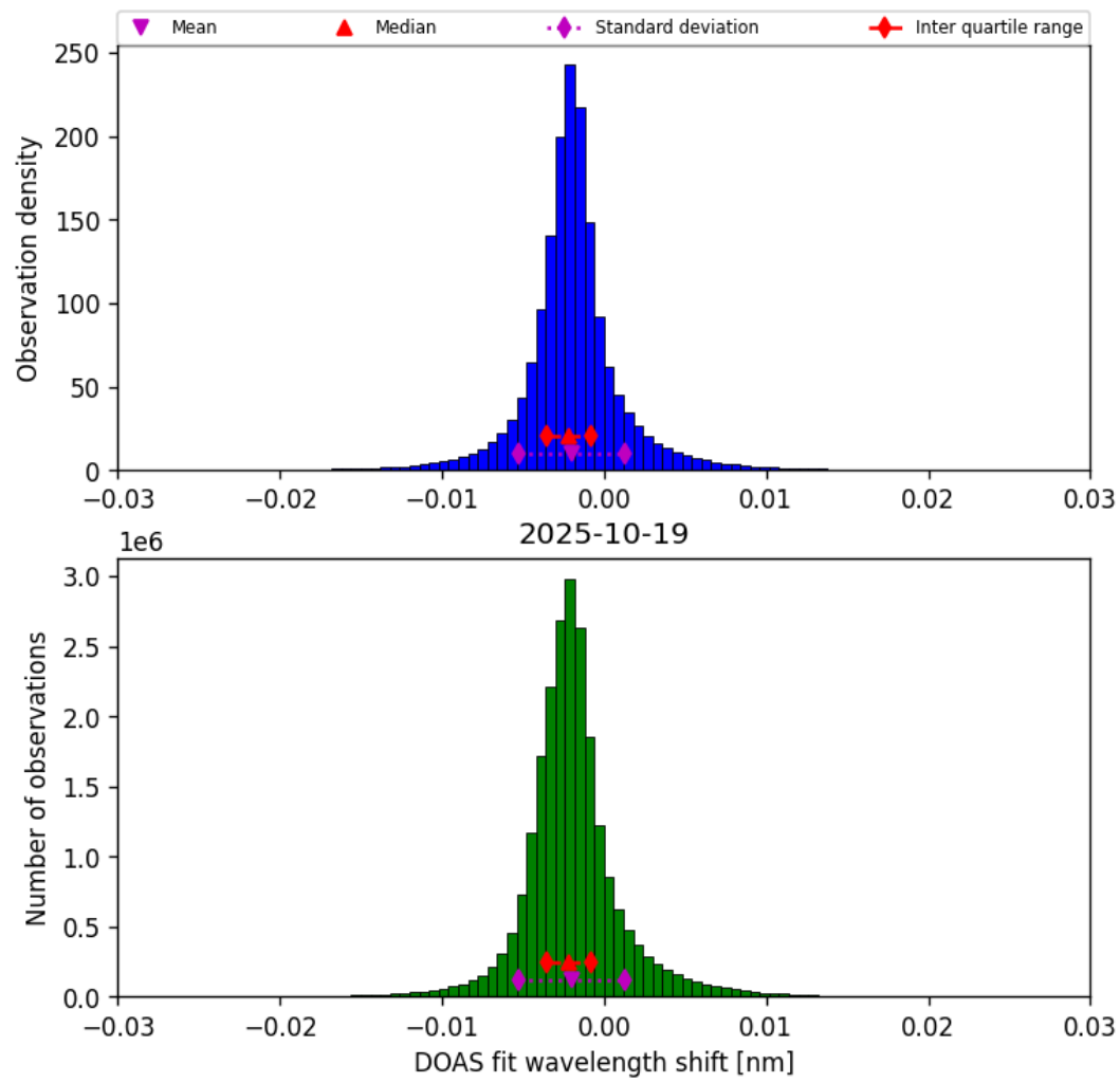
Figure 35: Histogram of “DOAS fit wavelength shift” for 2025-10-19 to 2025-10-20
