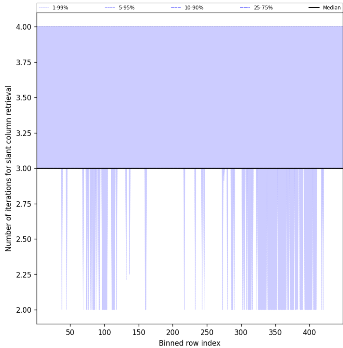
Figure 45: Along track statistics of “Number of iterations for slant column retrieval” for 2025-10-19 to 2025-10-20
