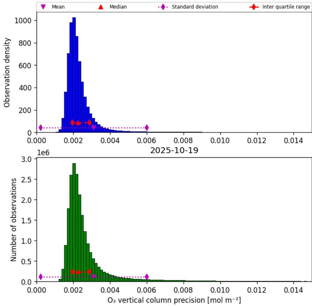
Figure 30: Histogram of “O 3 vertical column precision” for 2025-10-19 to 2025-10-20
