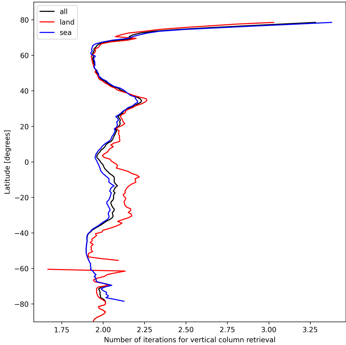
Figure 27: Zonal average of “Number of iterations for vertical column retrieval” for 2025-10-19 to 2025-10-20.
