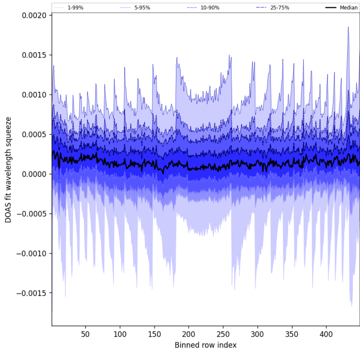
Figure 48: Along track statistics of “DOAS fit wavelength squeeze” for 2025-10-19 to 2025-10-20
