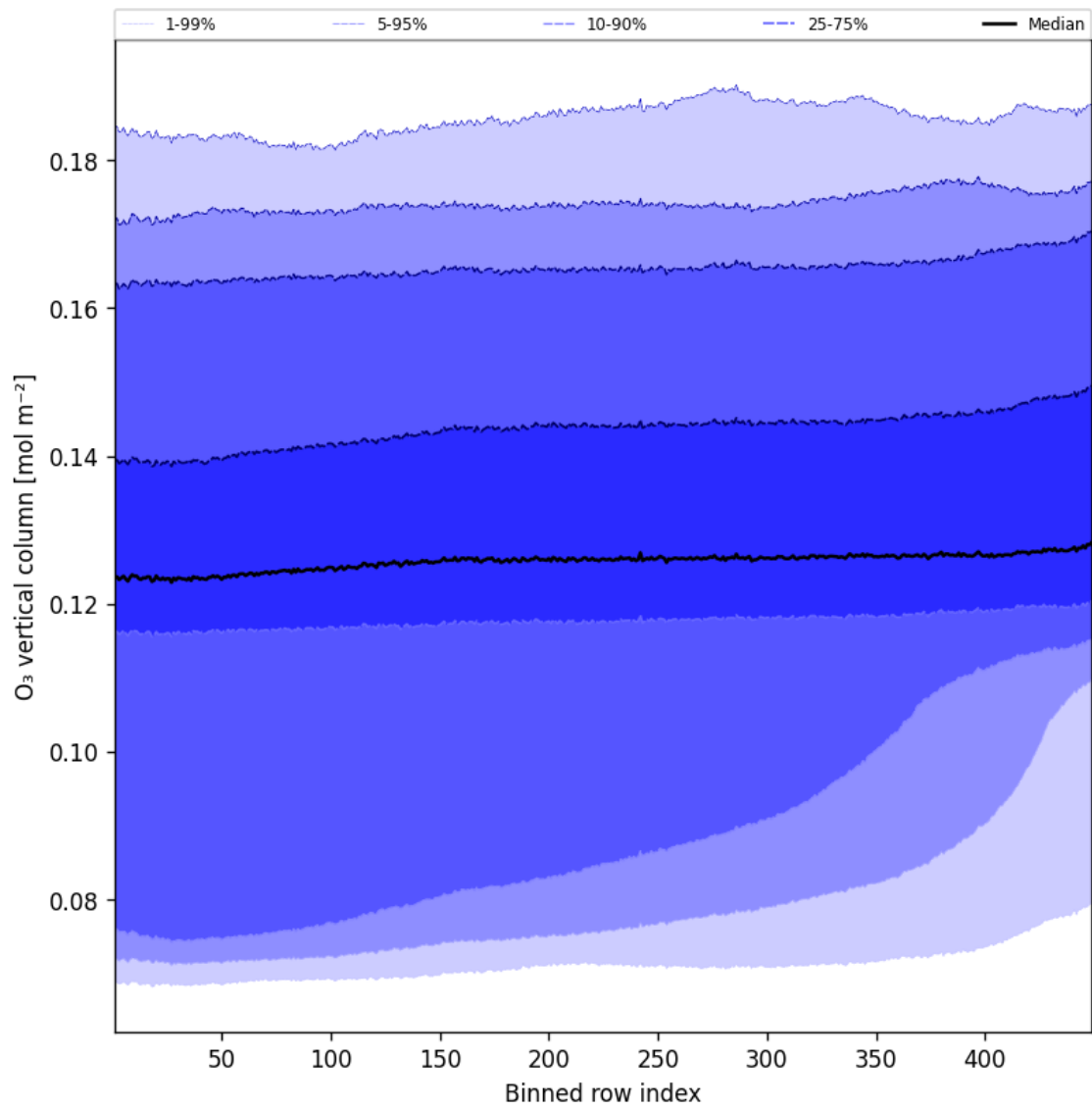
Figure 41: Along track statistics of “O 3 vertical column” for 2025-10-19 to 2025-10-20
