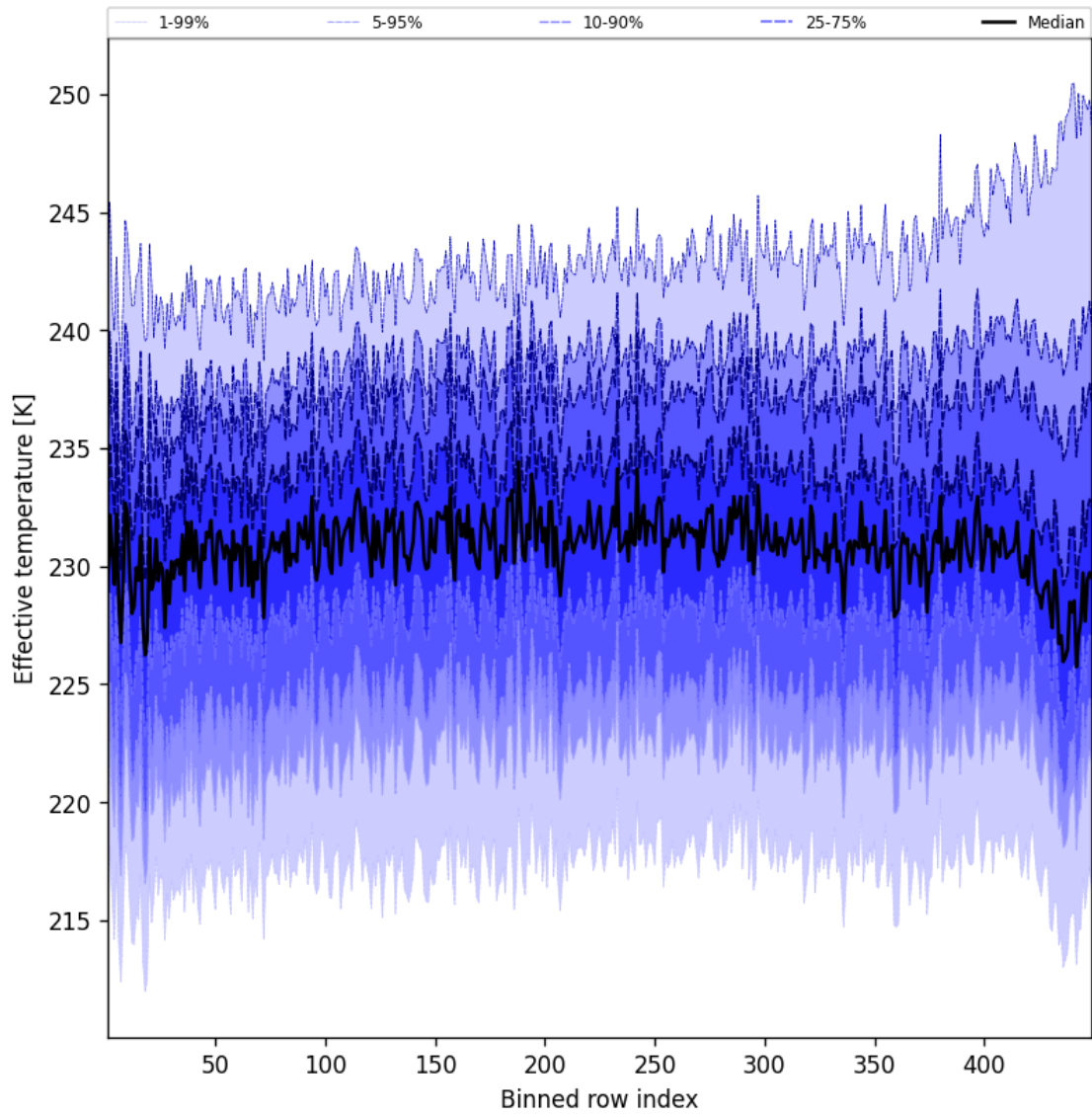
Figure 50: Along track statistics of “Effective temperature” for 2025-10-19 to 2025-10-20
