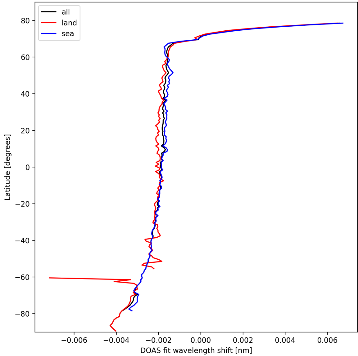
Figure 23: Zonal average of “DOAS fit wavelength shift” for 2025-10-19 to 2025-10-20.
