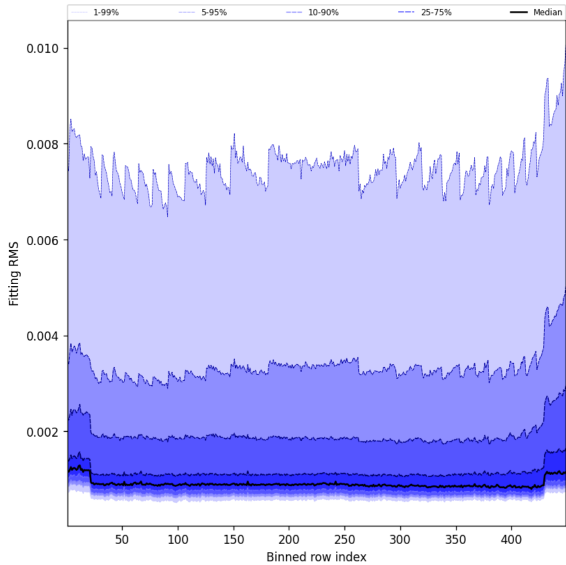
Figure 46: Along track statistics of “Fitting RMS” for 2025-10-19 to 2025-10-20
