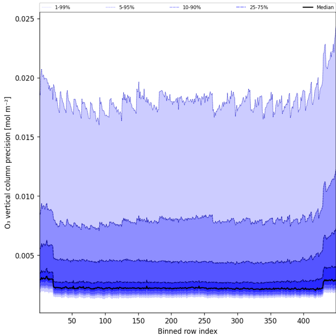
Figure 42: Along track statistics of “O 3 vertical column precision” for 2025-10-19 to 2025-10-20
