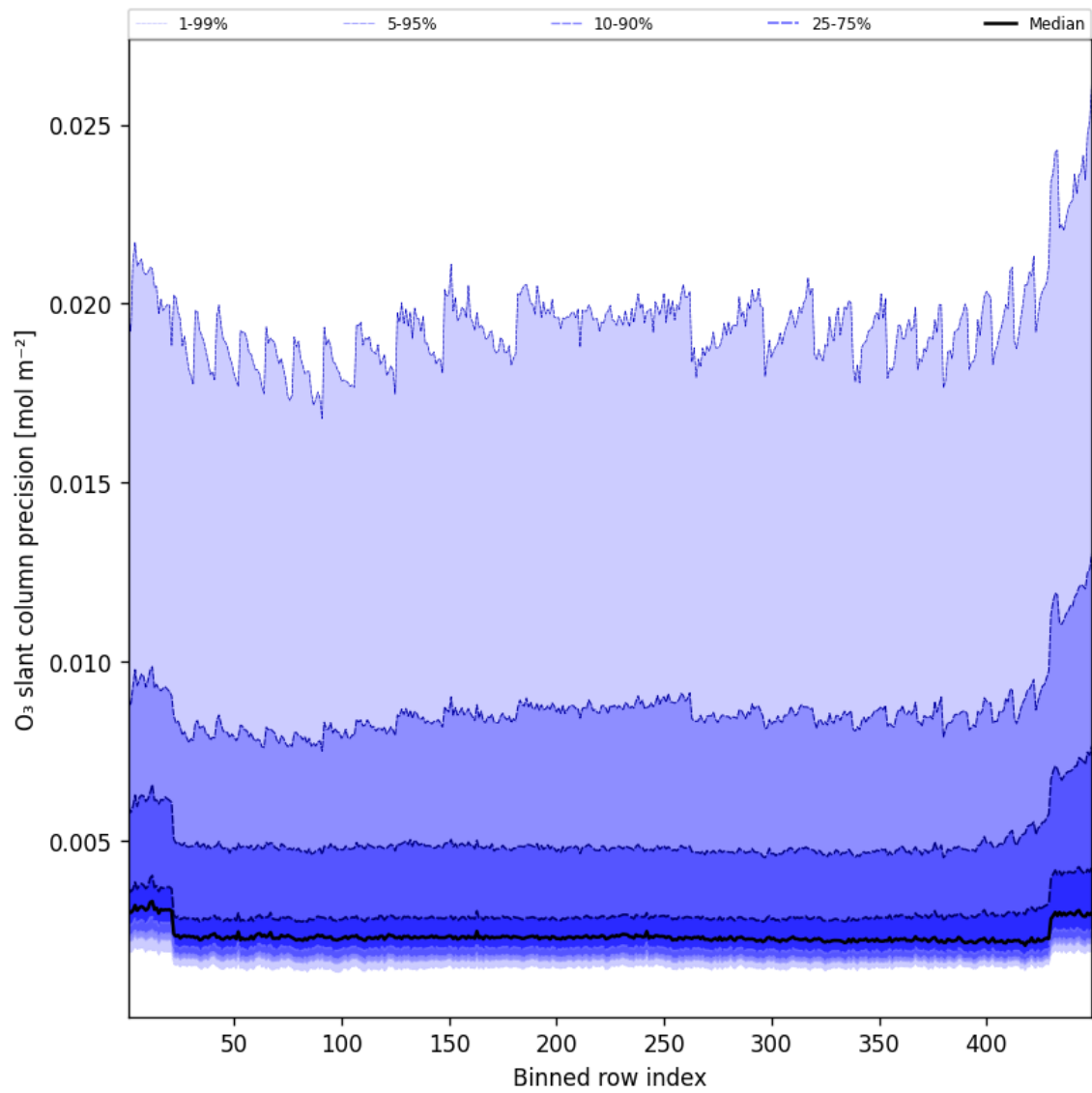
Figure 44: Along track statistics of “O 3 slant column precision” for 2025-10-19 to 2025-10-20
