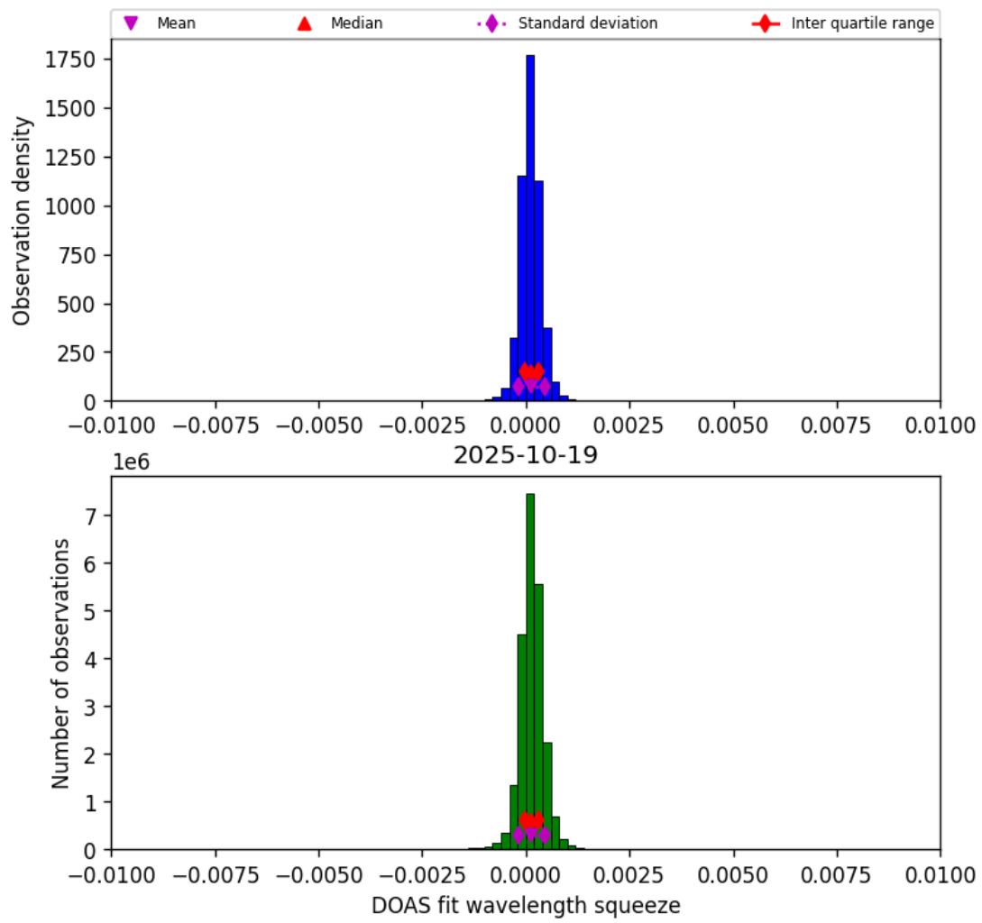
Figure 36: Histogram of “DOAS fit wavelength squeeze” for 2025-10-19 to 2025-10-20
