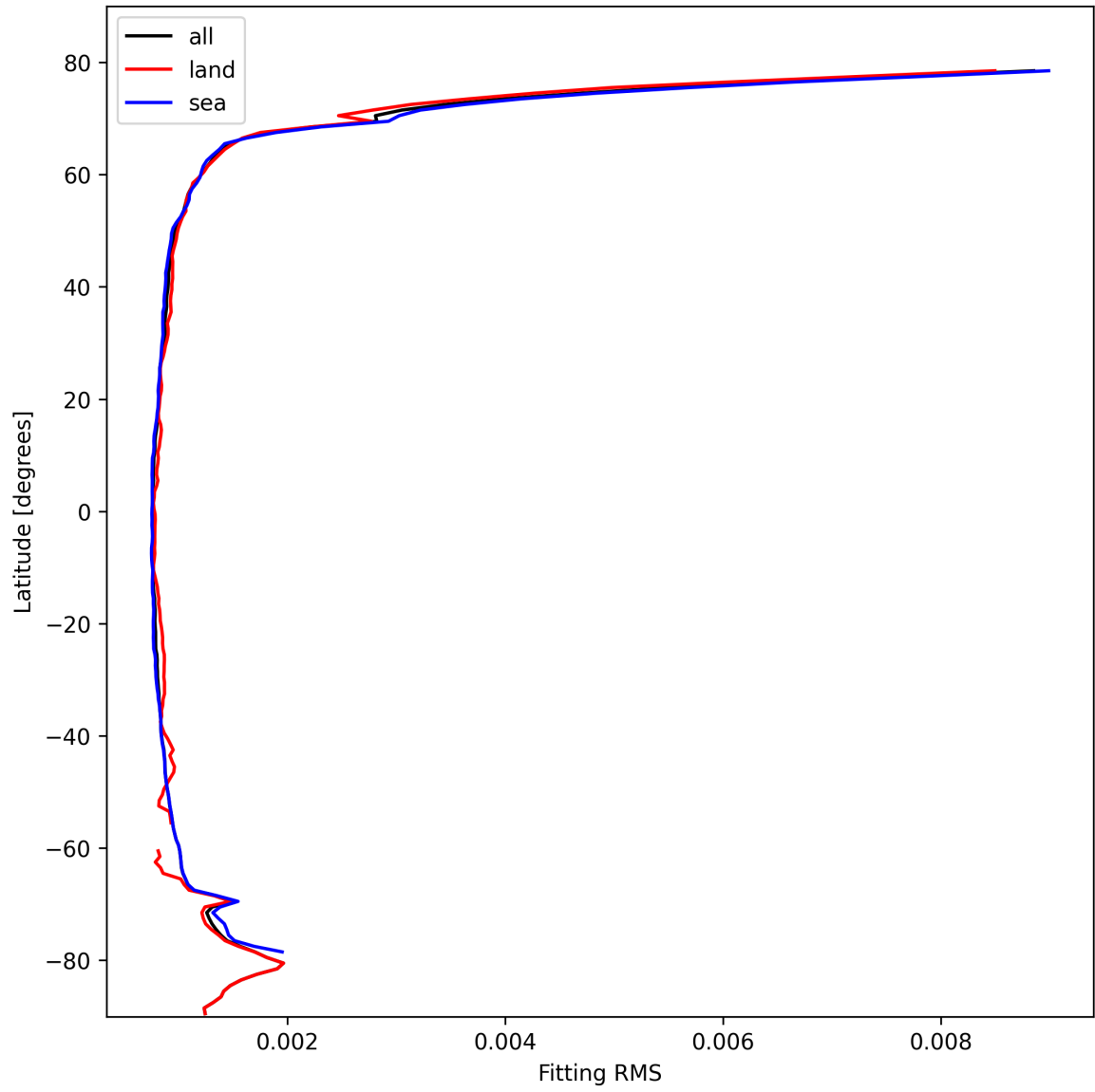
Figure 22: Zonal average of “Fitting RMS” for 2025-10-19 to 2025-10-20.
