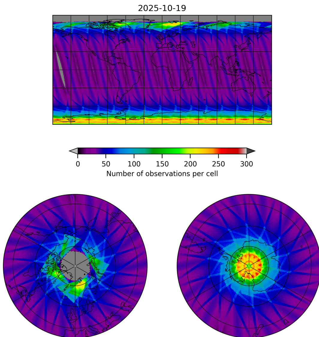
Figure 15: Map of the number of observations for 2025-10-19 to 2025-10-20
