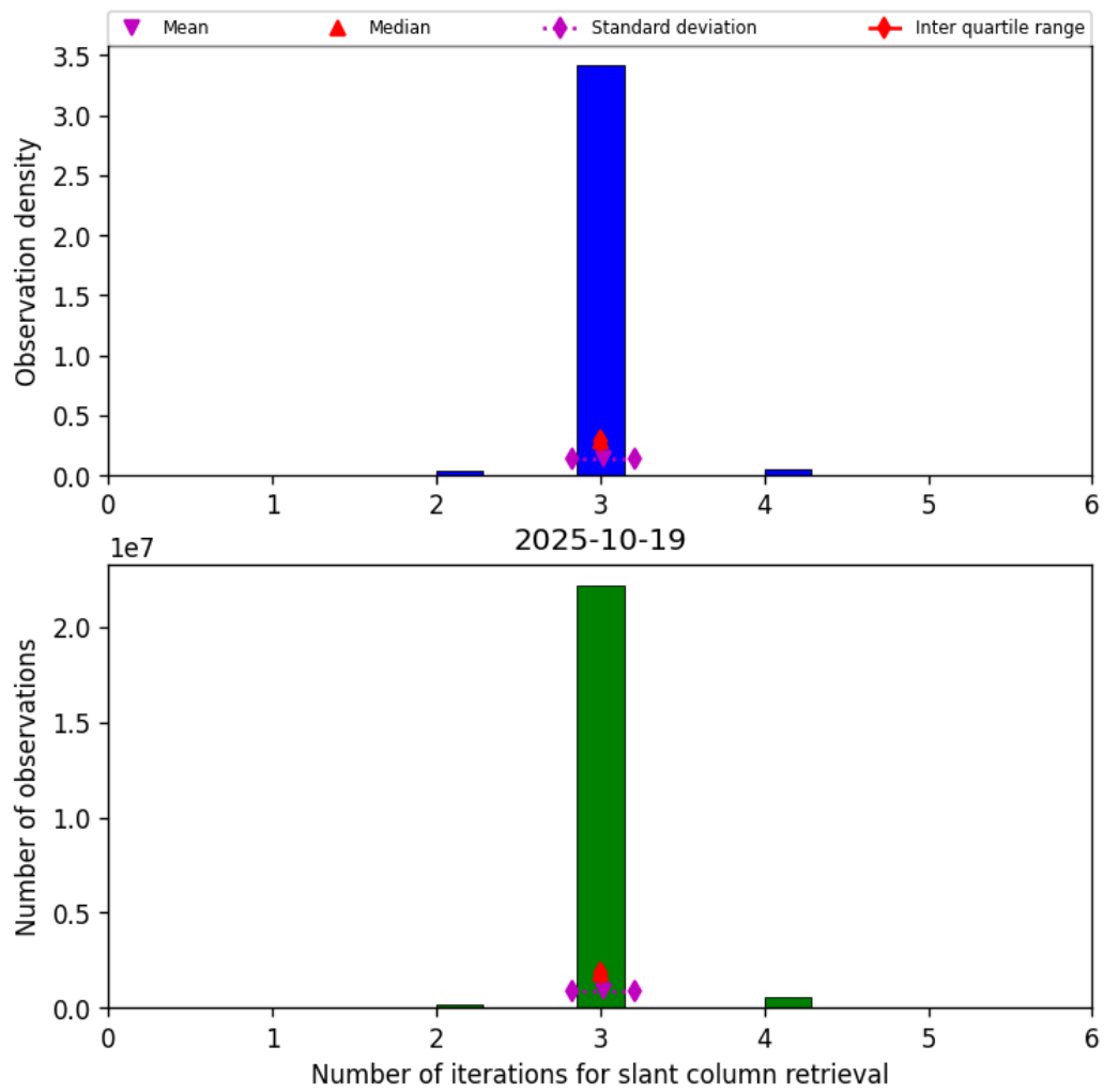
Figure 33: Histogram of “Number of iterations for slant column retrieval” for 2025-10-19 to 2025-10-20
