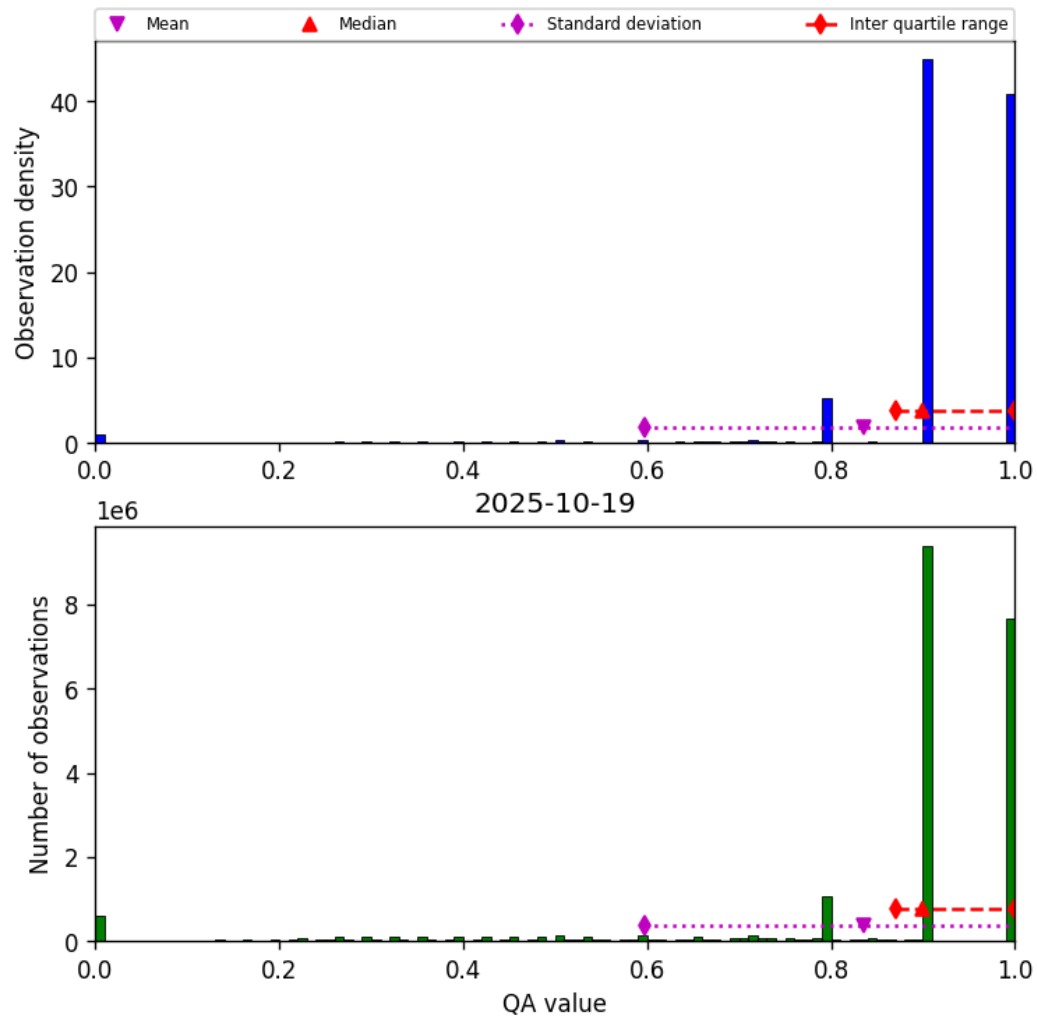
Figure 28: Histogram of “QA value” for 2025-10-19 to 2025-10-20
