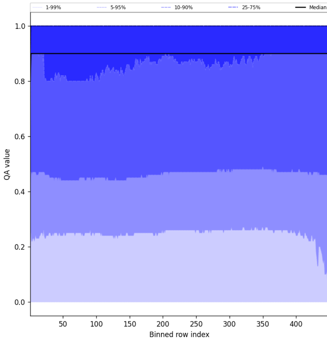
Figure 40: Along track statistics of “QA value” for 2025-10-19 to 2025-10-20
