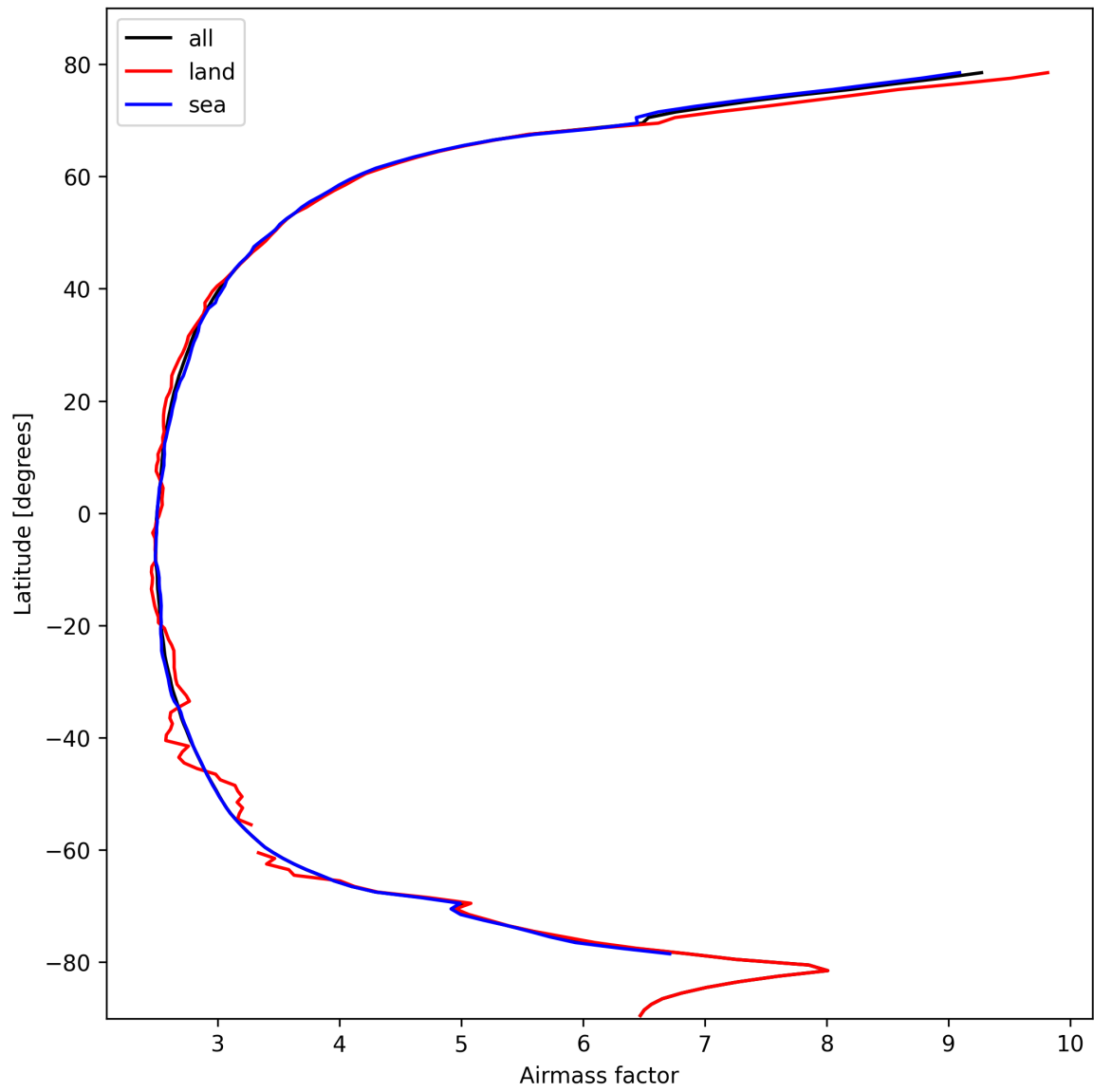
Figure 25: Zonal average of “Airmass factor” for 2025-10-19 to 2025-10-20.
