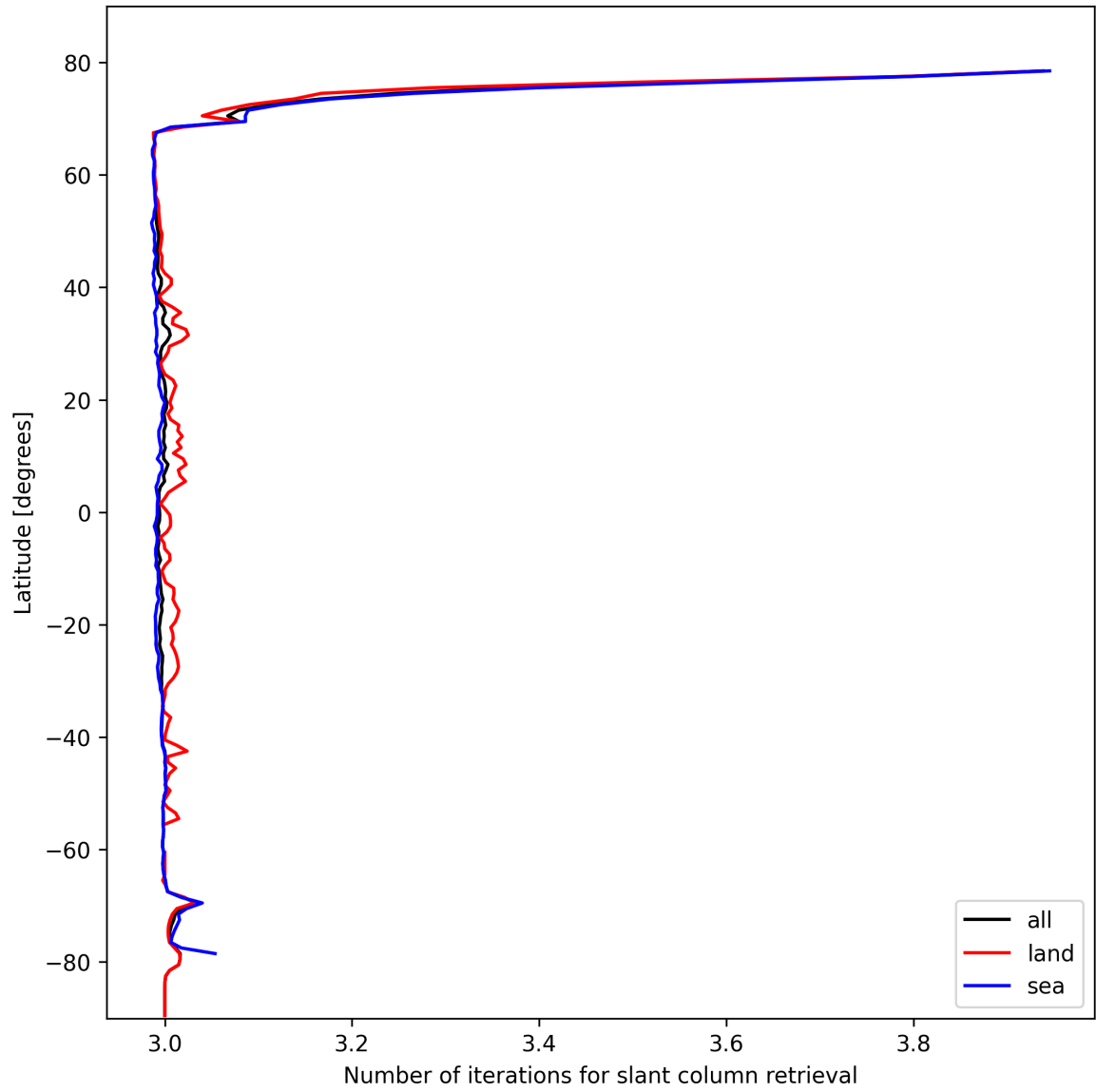
Figure 21: Zonal average of “Number of iterations for slant column retrieval” for 2025-10-19 to 2025-10-20.
