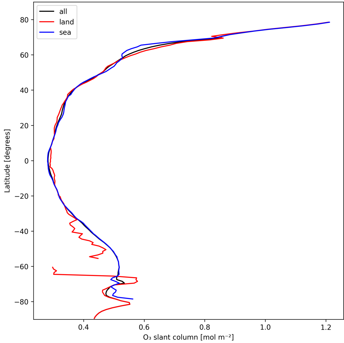
Figure 19: Zonal average of “O 3 slant column” for 2025-10-19 to 2025-10-20.
