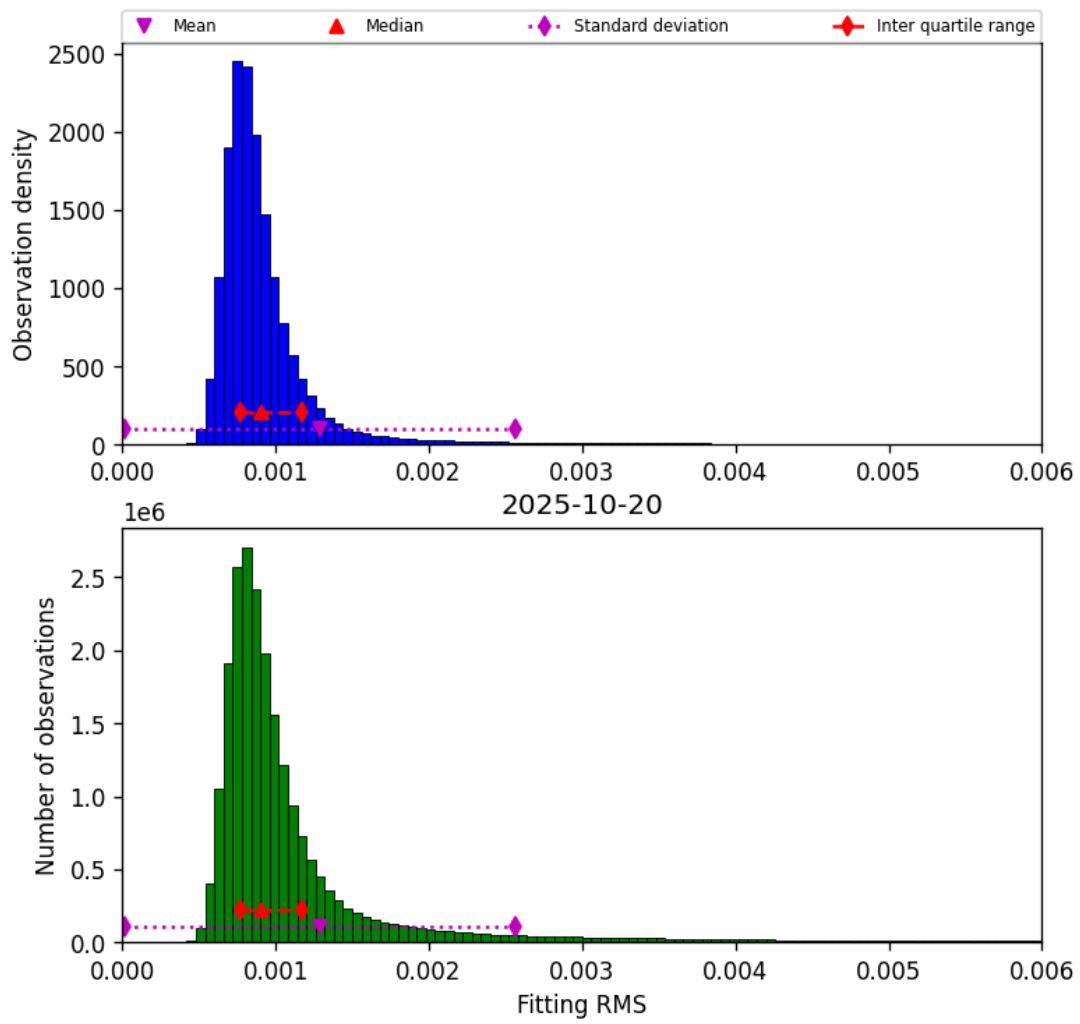
Figure 34: Histogram of “Fitting RMS” for 2025-10-20 to 2025-10-20
