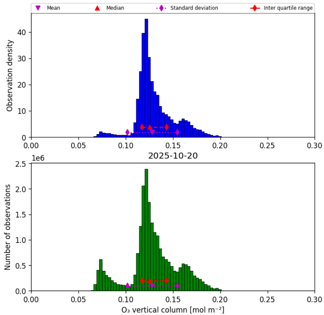
Figure 29: Histogram of “O 3 vertical column” for 2025-10-20 to 2025-10-20
