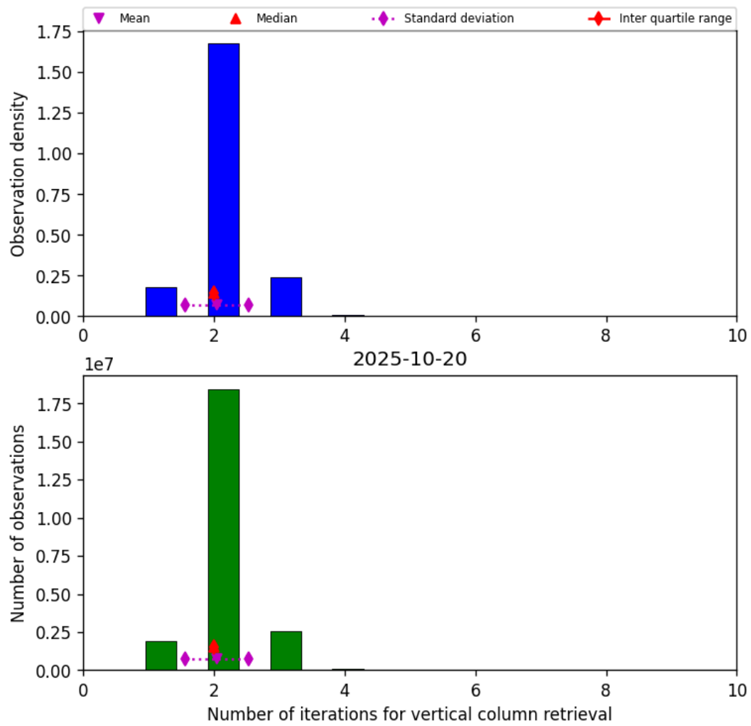
Figure 39: Histogram of “Number of iterations for vertical column retrieval” for 2025-10-20 to 2025-10-20
