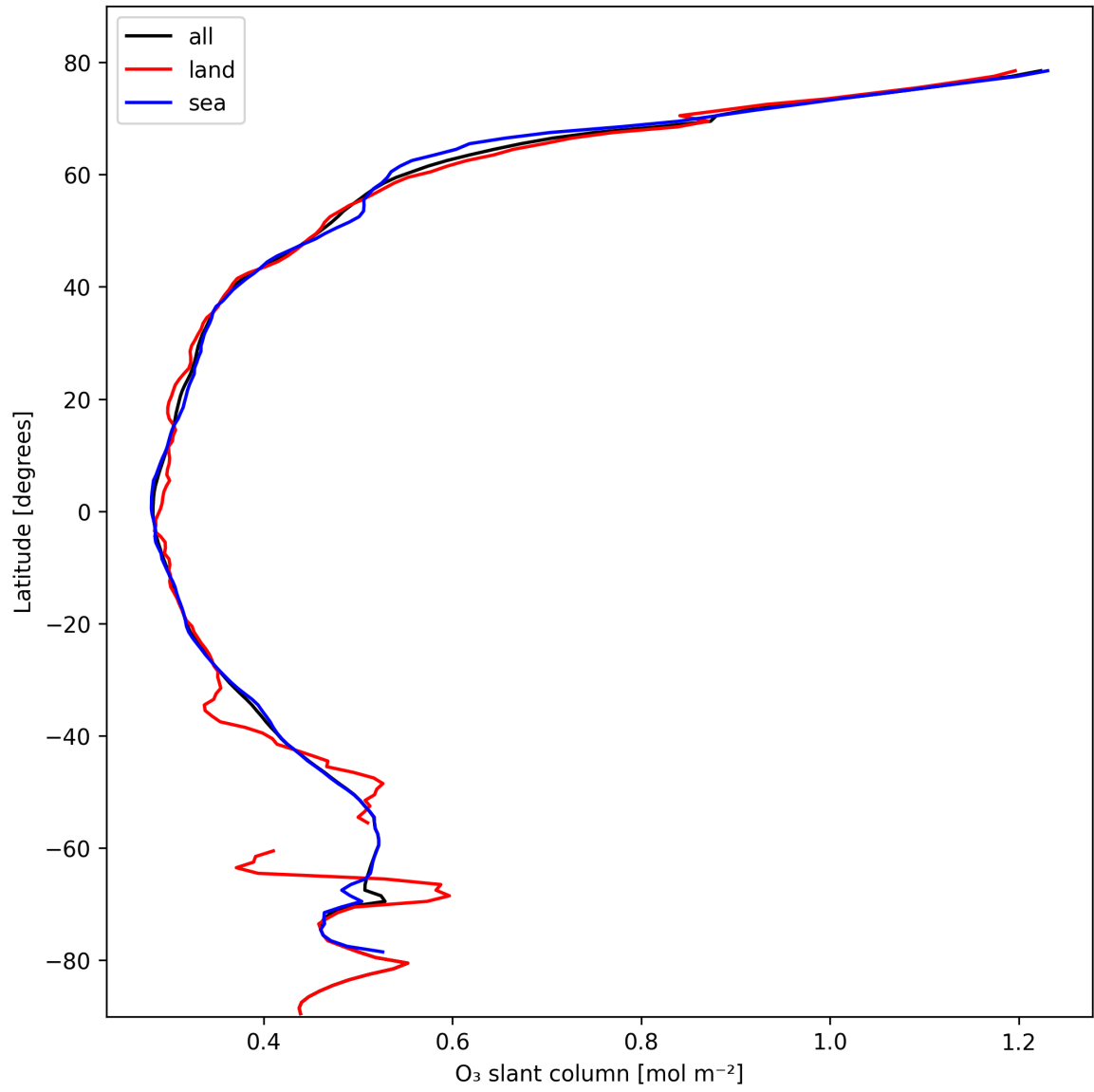
Figure 19: Zonal average of “O 3 slant column” for 2025-10-20 to 2025-10-20.
