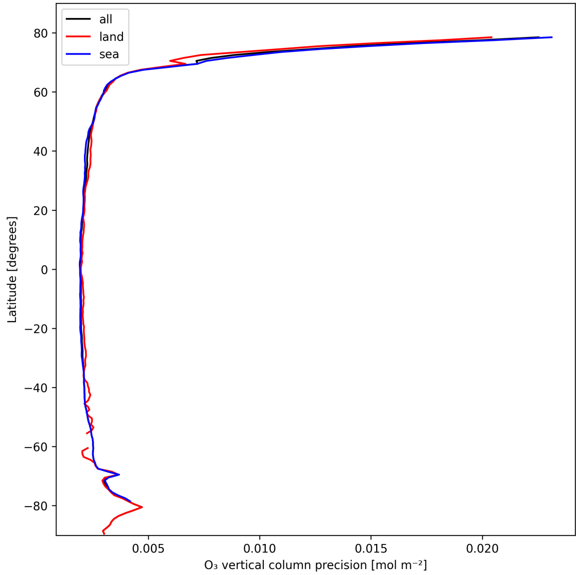
Figure 18: Zonal average of “O 3 vertical column precision” for 2025-10-20 to 2025-10-20.
