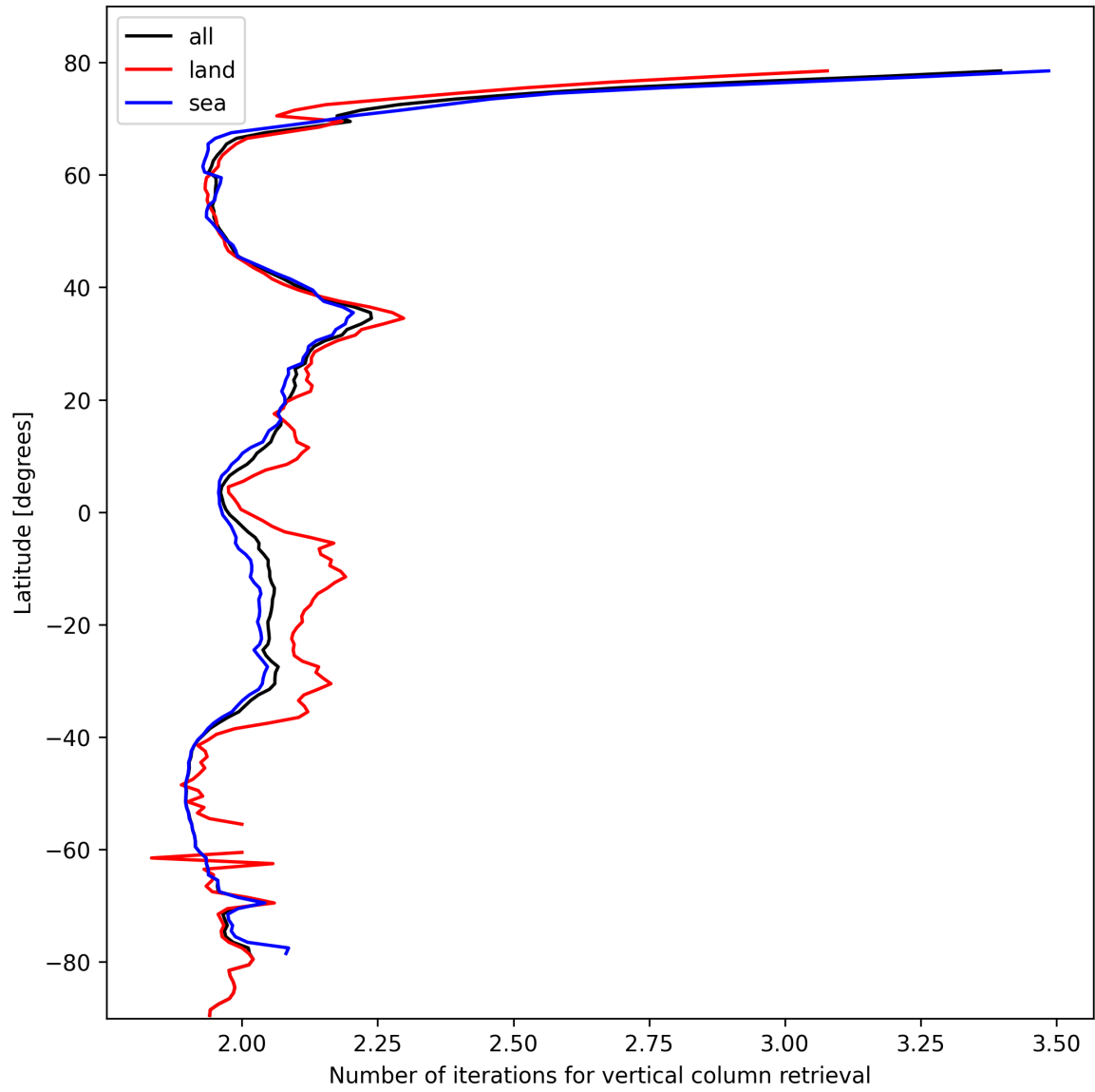
Figure 27: Zonal average of “Number of iterations for vertical column retrieval” for 2025-10-20 to 2025-10-20.
