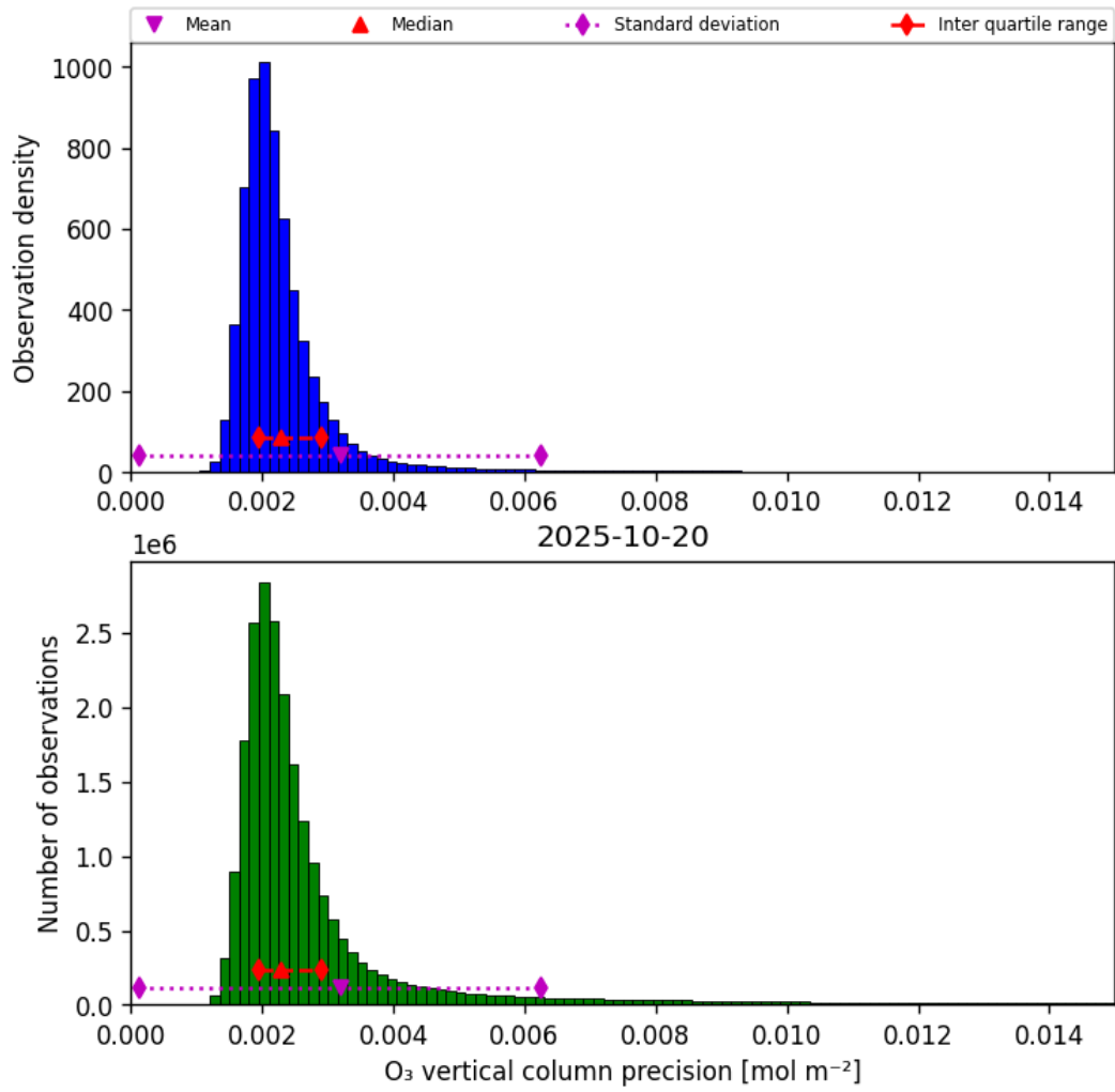
Figure 30: Histogram of “O 3 vertical column precision” for 2025-10-20 to 2025-10-20
