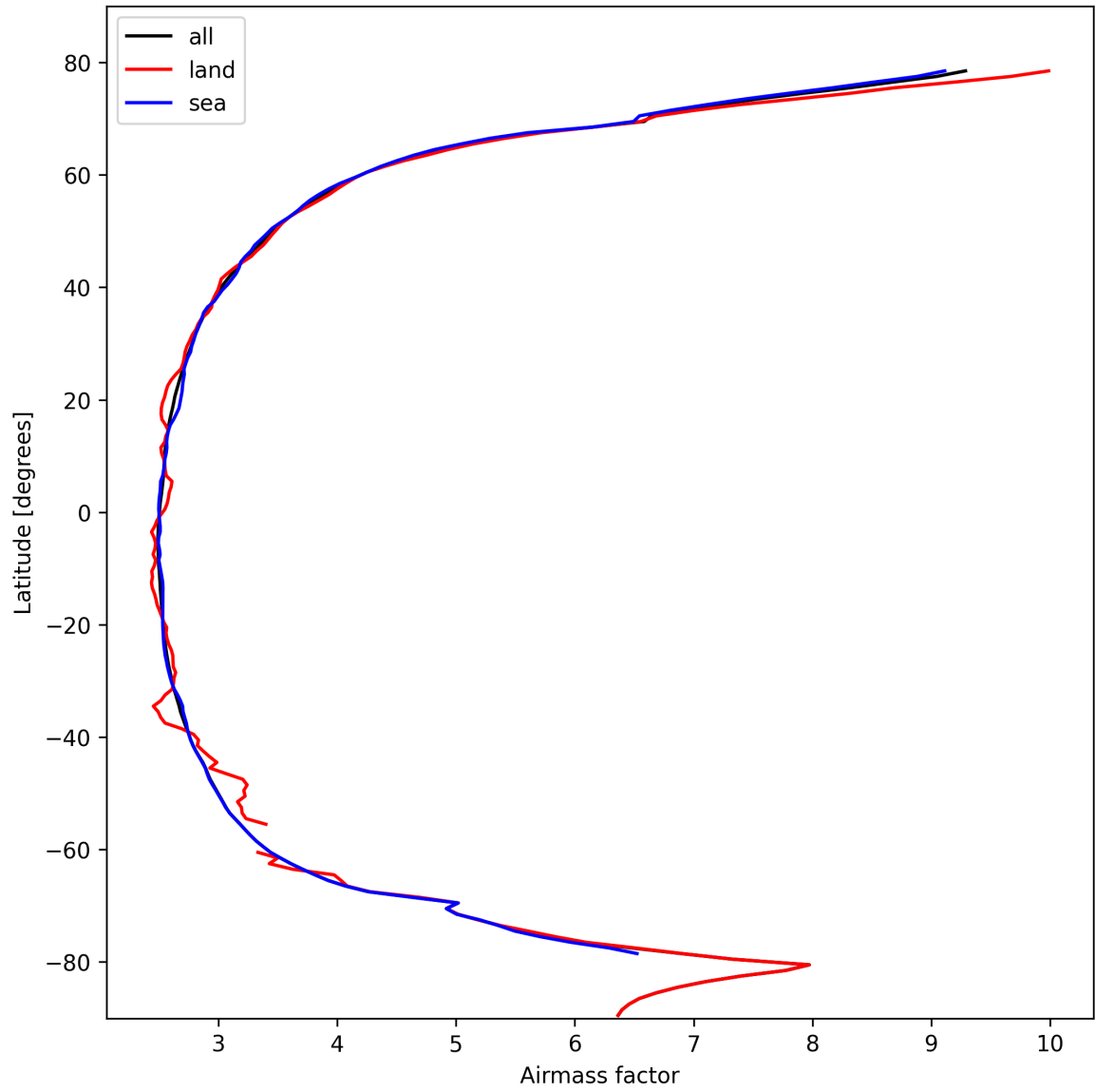
Figure 25: Zonal average of “Airmass factor” for 2025-10-20 to 2025-10-20.
