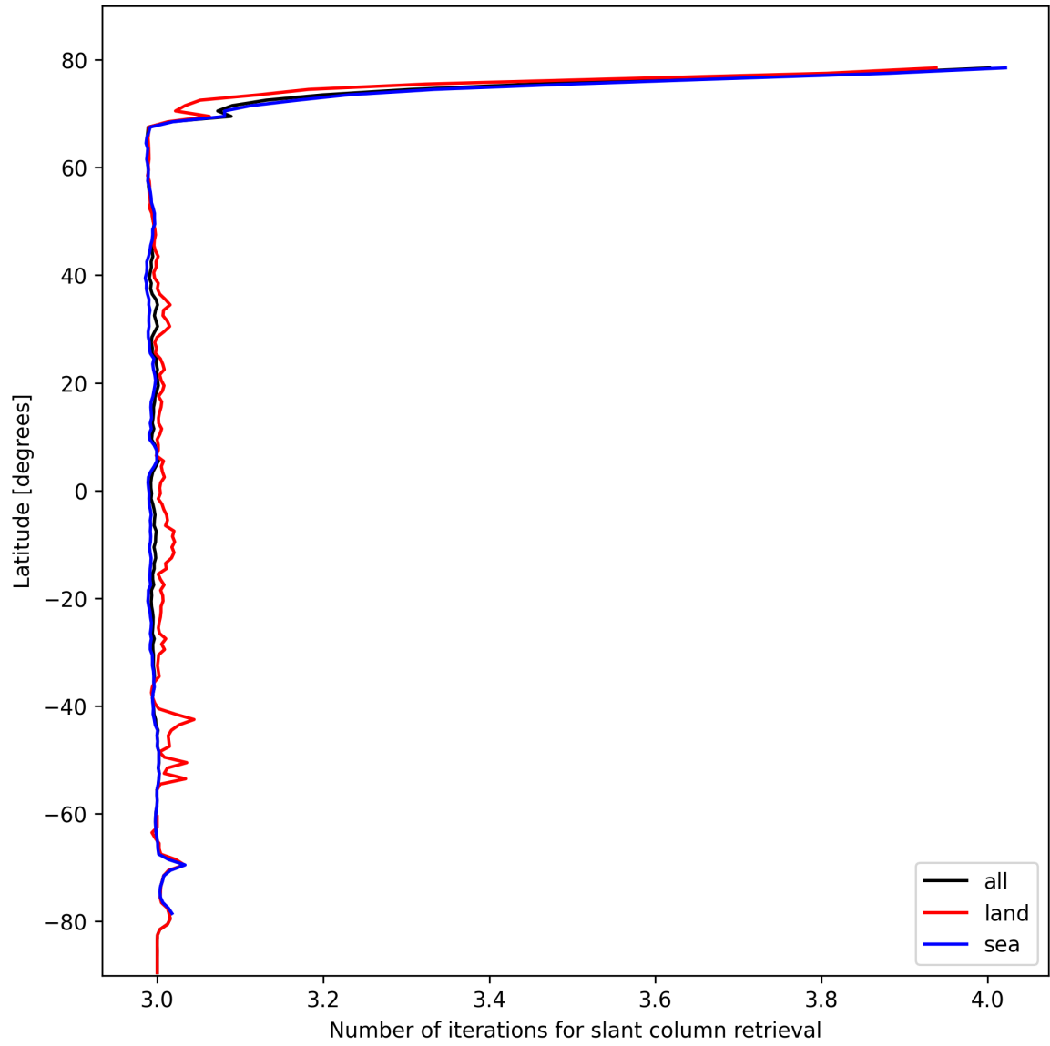
Figure 21: Zonal average of “Number of iterations for slant column retrieval” for 2025-10-20 to 2025-10-20.
