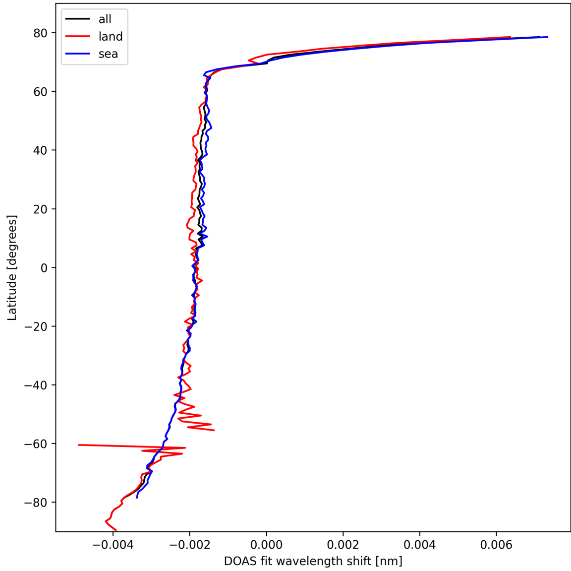
Figure 23: Zonal average of “DOAS fit wavelength shift” for 2025-10-20 to 2025-10-20.
