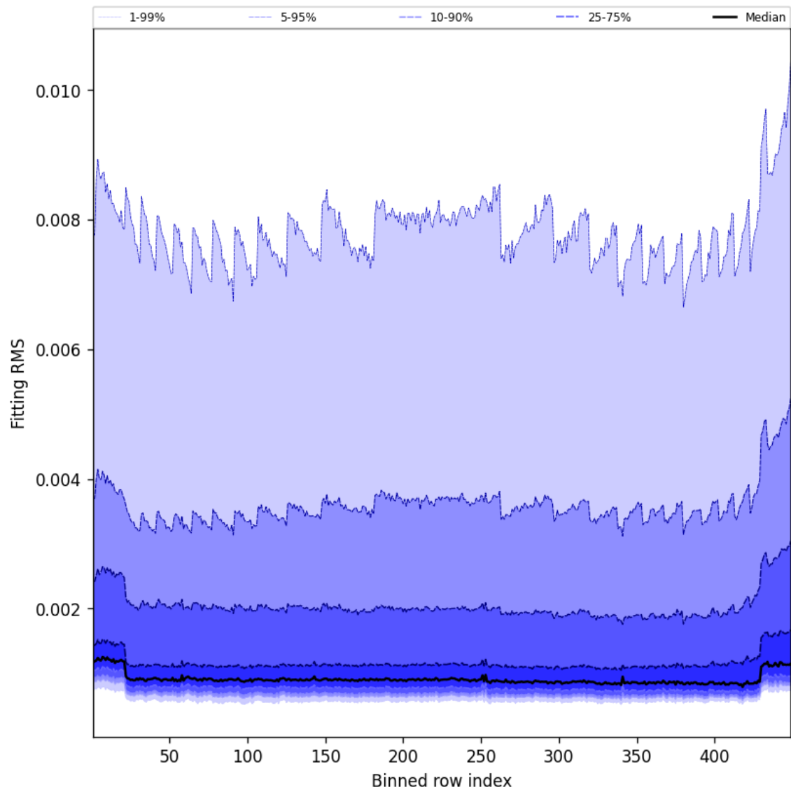
Figure 46: Along track statistics of “Fitting RMS” for 2025-10-20 to 2025-10-20
