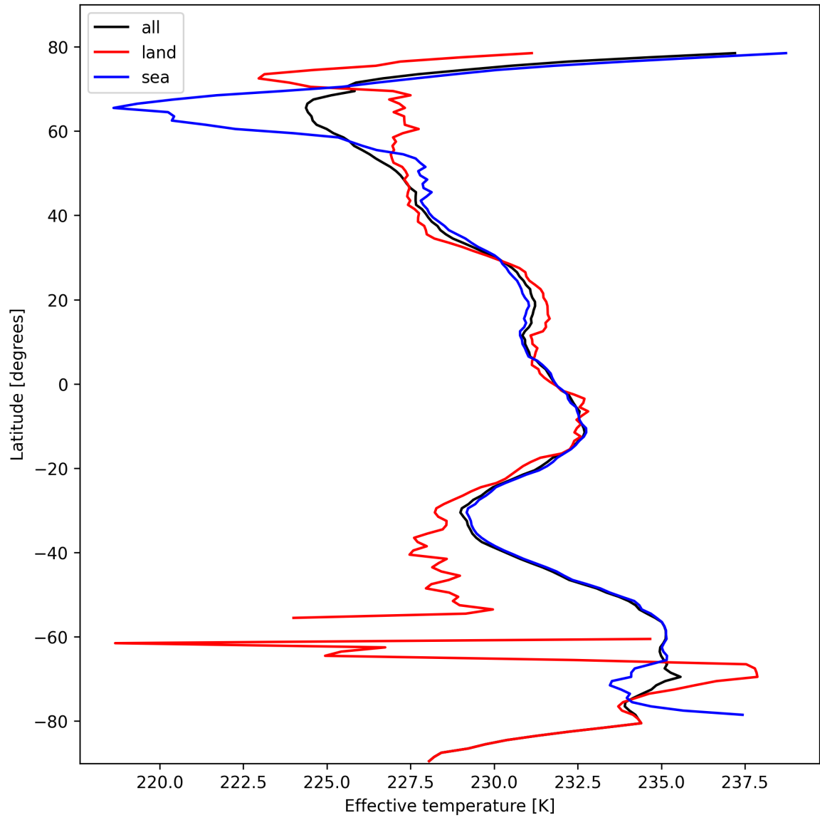
Figure 26: Zonal average of “Effective temperature” for 2025-10-20 to 2025-10-20.
