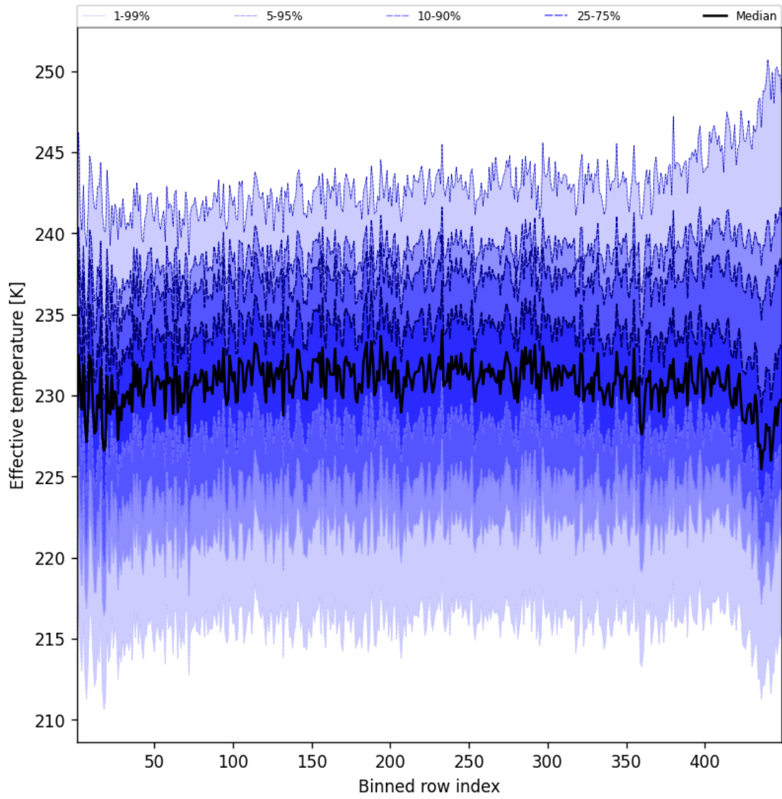
Figure 50: Along track statistics of “Effective temperature” for 2025-10-20 to 2025-10-20
