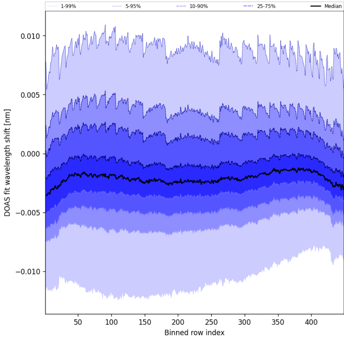
Figure 47: Along track statistics of “DOAS fit wavelength shift” for 2025-10-20 to 2025-10-20
