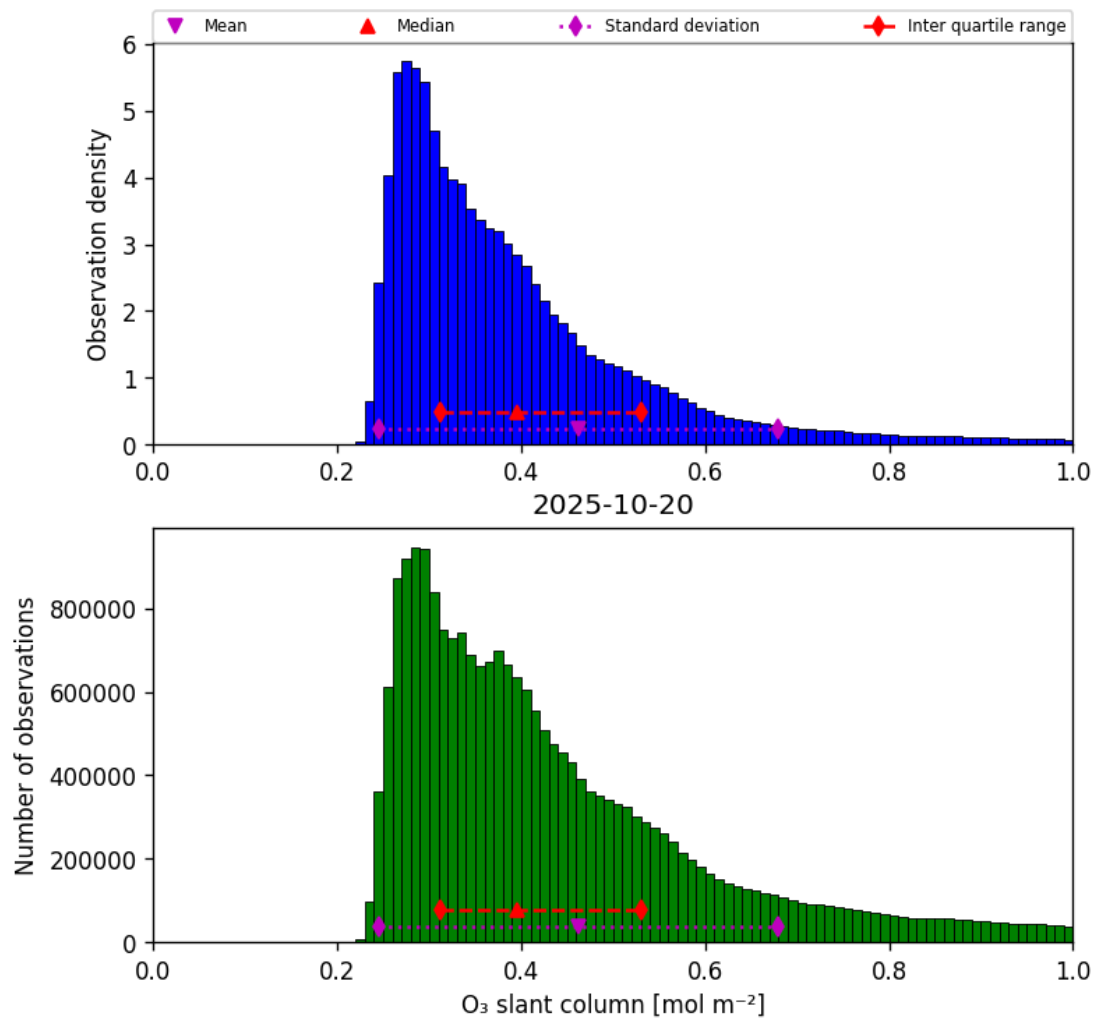
Figure 31: Histogram of “O 3 slant column” for 2025-10-20 to 2025-10-20
