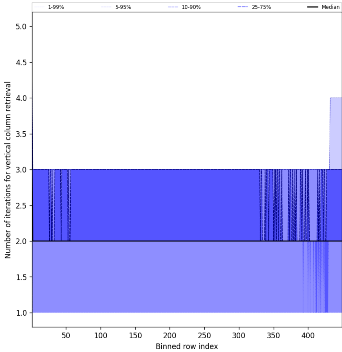
Figure 51: Along track statistics of “Number of iterations for vertical column retrieval” for 2025-10-20 to 2025-10-20
