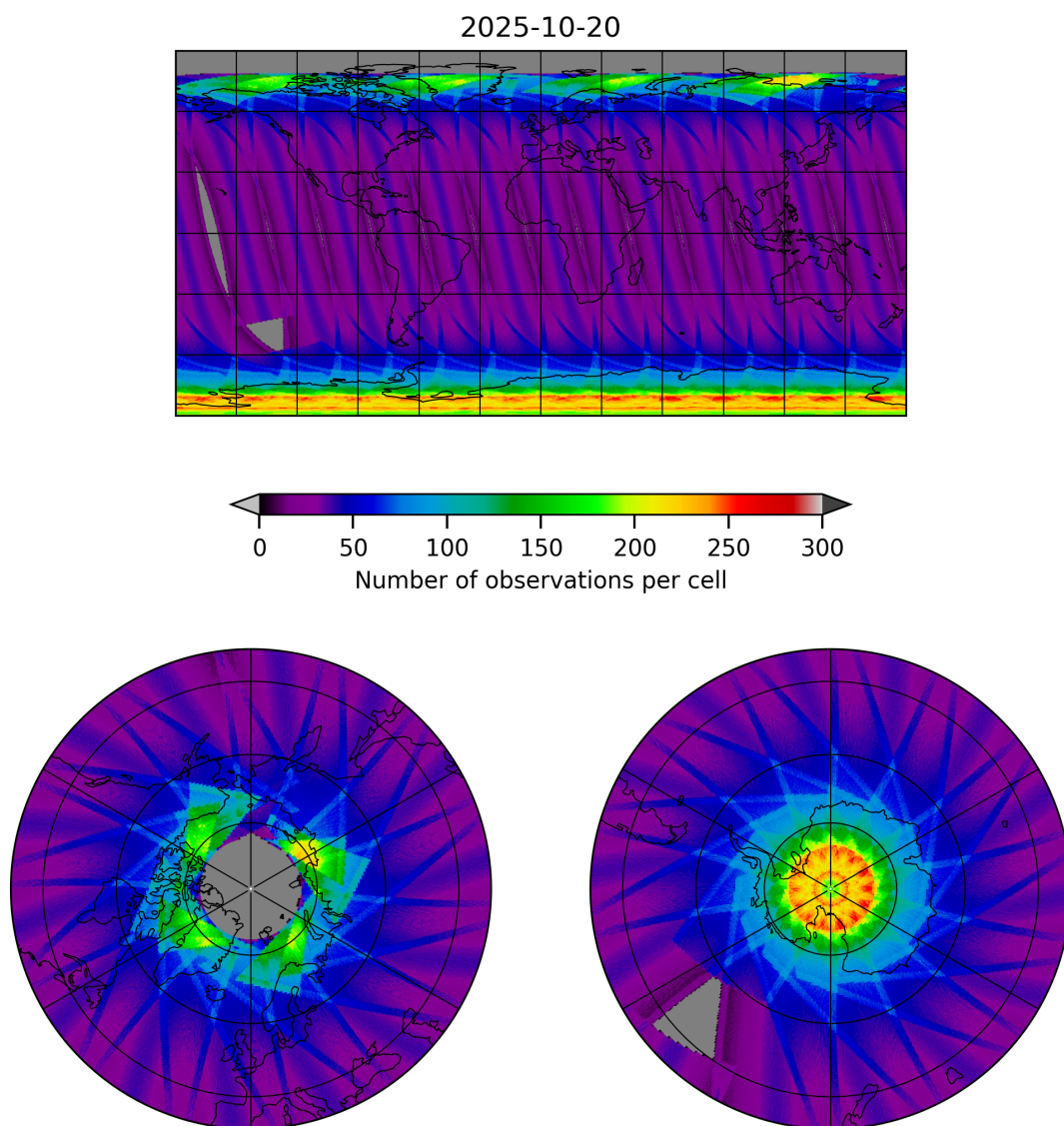
Figure 15: Map of the number of observations for 2025-10-20 to 2025-10-20
