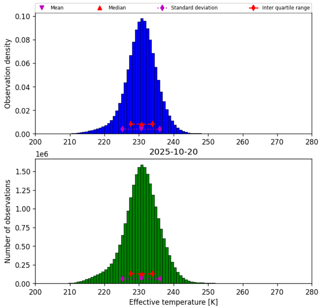
Figure 38: Histogram of “Effective temperature” for 2025-10-20 to 2025-10-20
