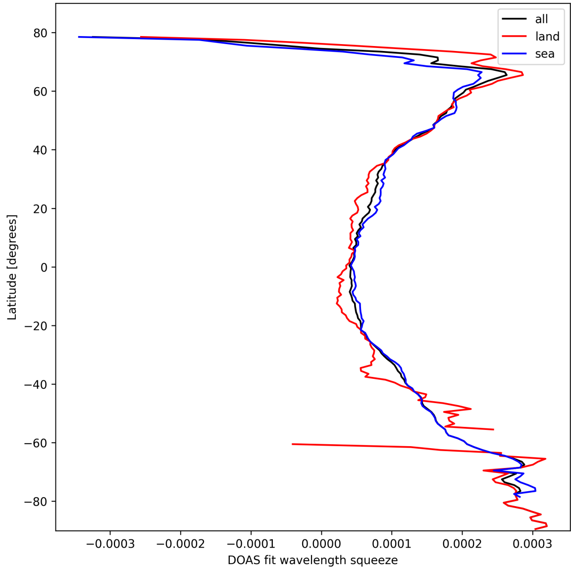
Figure 24: Zonal average of “DOAS fit wavelength squeeze” for 2025-10-20 to 2025-10-20.
