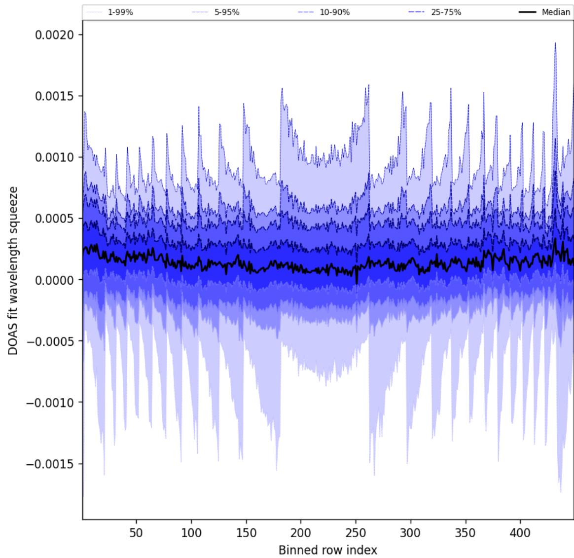
Figure 48: Along track statistics of “DOAS fit wavelength squeeze” for 2025-10-20 to 2025-10-20
