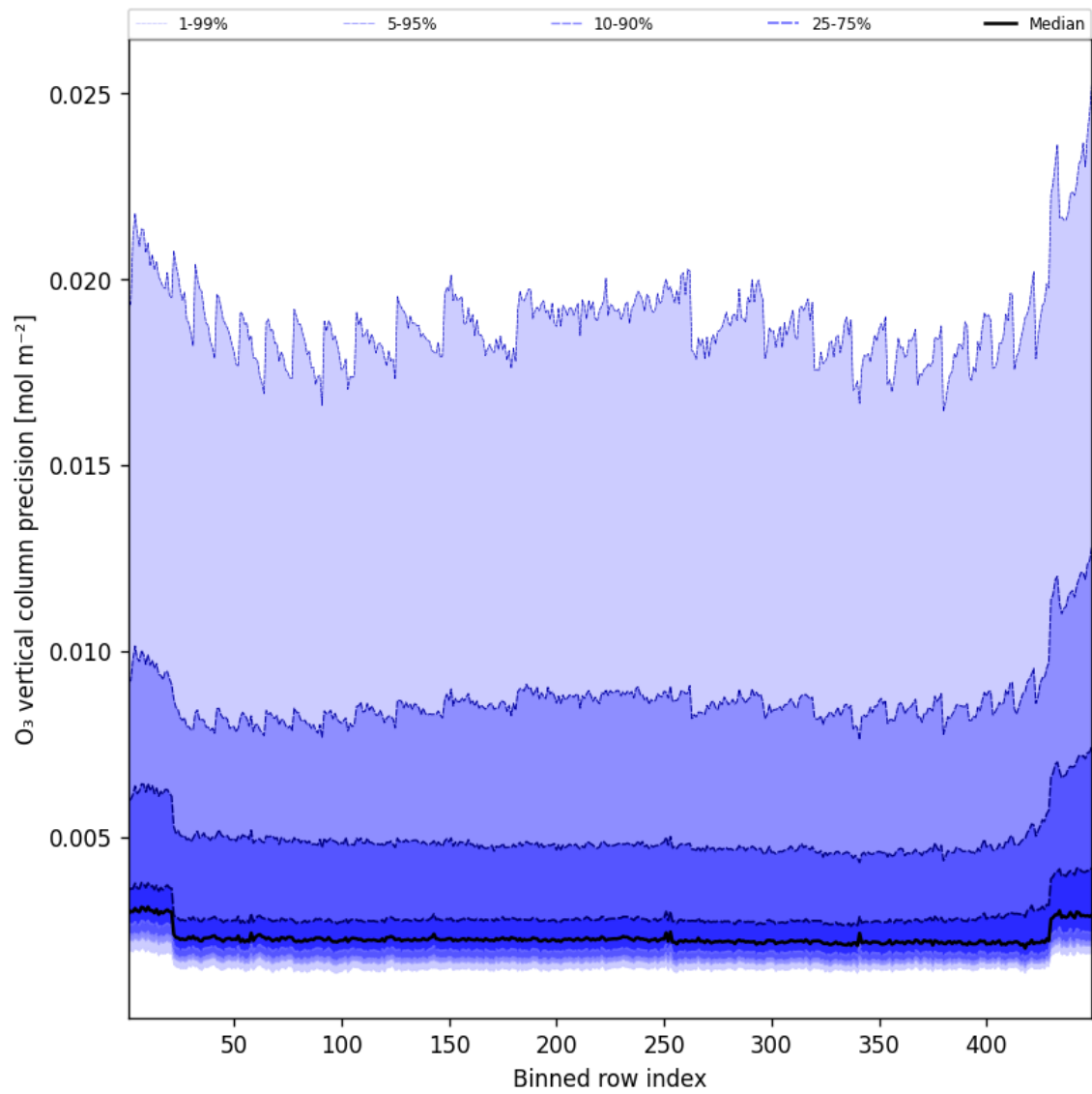
Figure 42: Along track statistics of “O 3 vertical column precision” for 2025-10-20 to 2025-10-20
