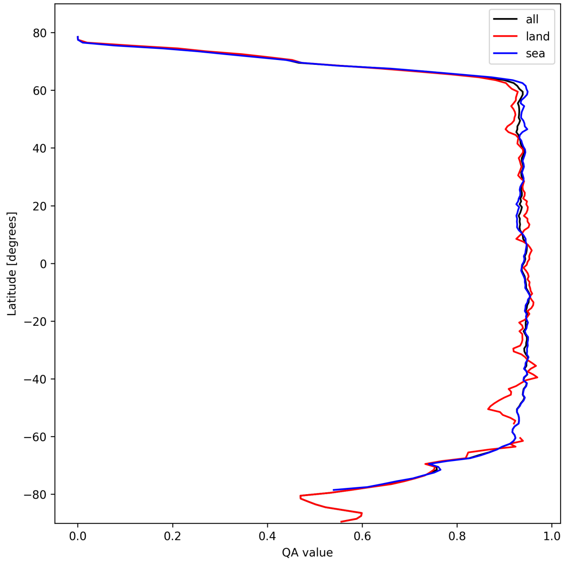
Figure 16: Zonal average of “QA value” for 2025-10-20 to 2025-10-20.
