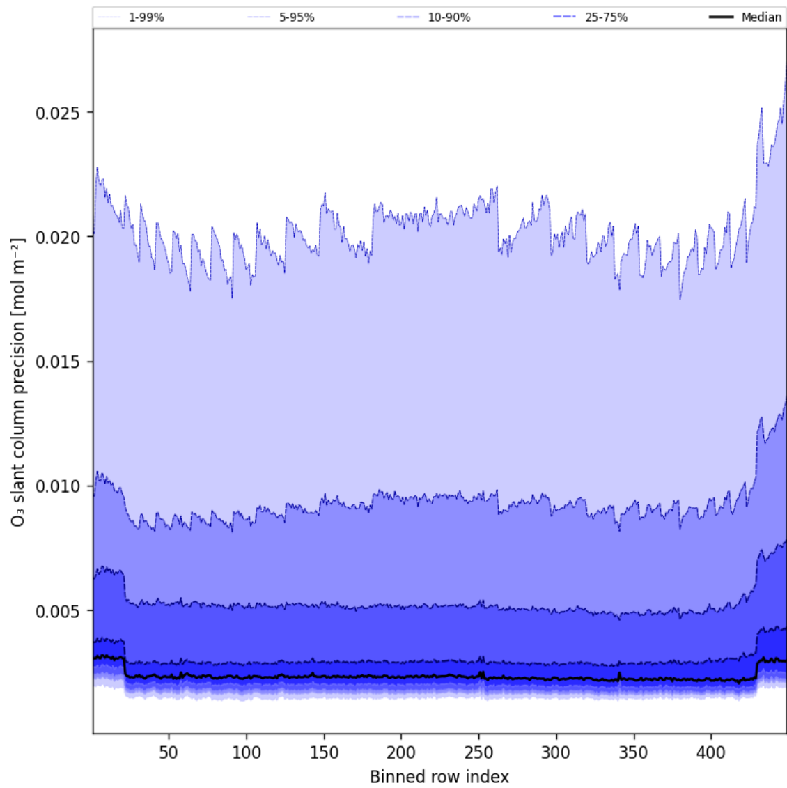
Figure 44: Along track statistics of “O 3 slant column precision” for 2025-10-20 to 2025-10-20
