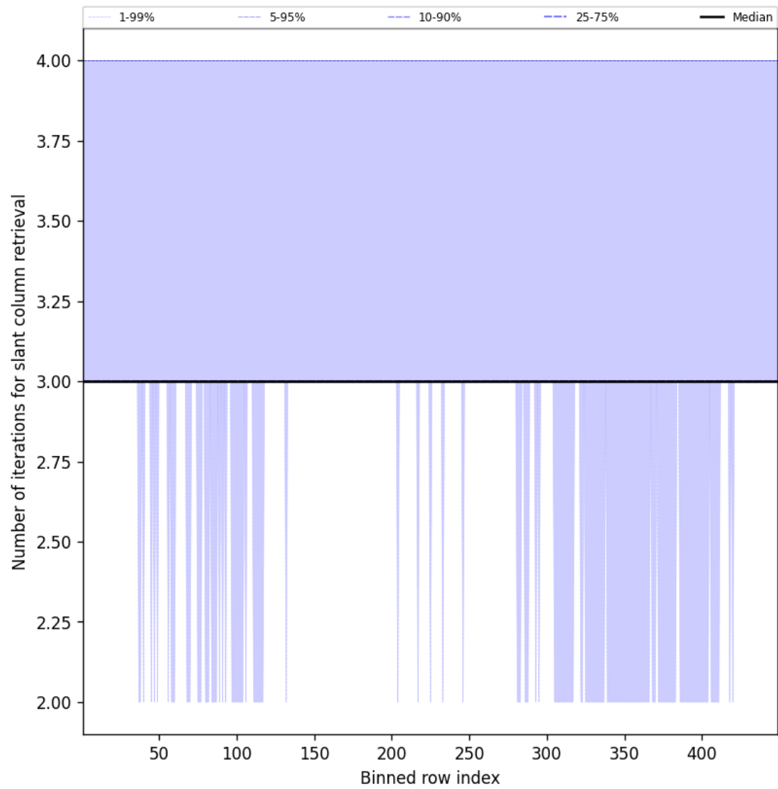
Figure 45: Along track statistics of “Number of iterations for slant column retrieval” for 2025-10-20 to 2025-10-20
