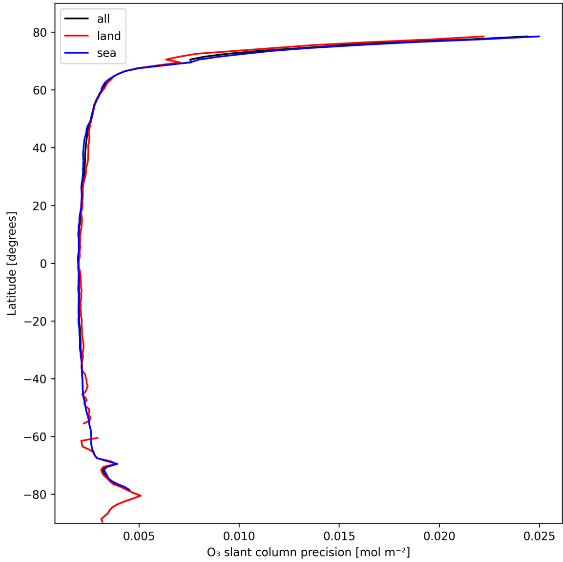
Figure 20: Zonal average of “O 3 slant column precision” for 2025-10-20 to 2025-10-20.
