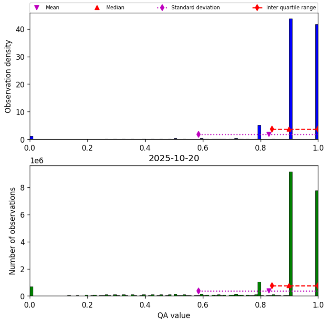
Figure 28: Histogram of “QA value” for 2025-10-20 to 2025-10-20
