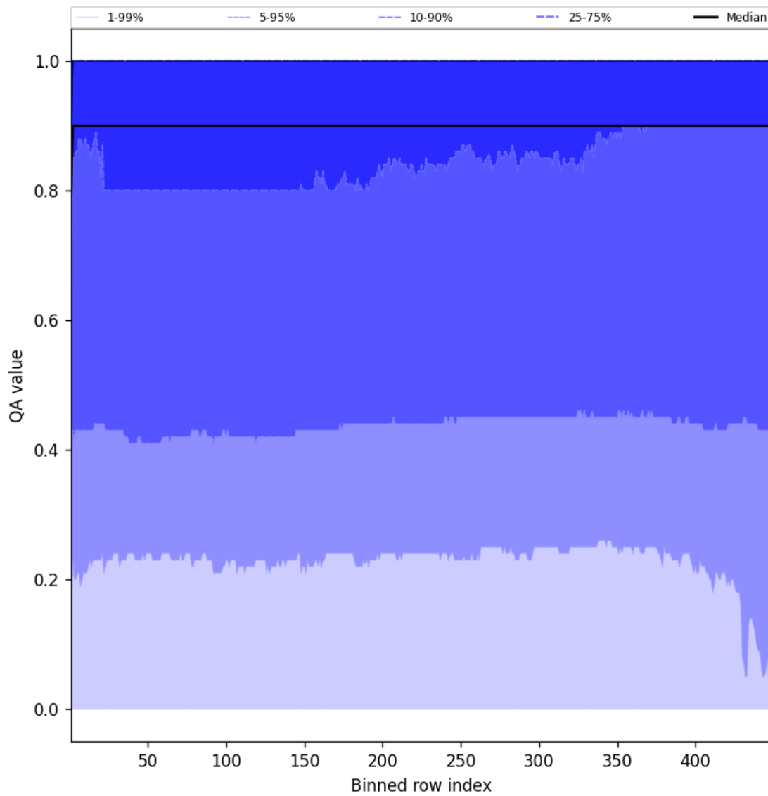
Figure 40: Along track statistics of “QA value” for 2025-10-20 to 2025-10-20
