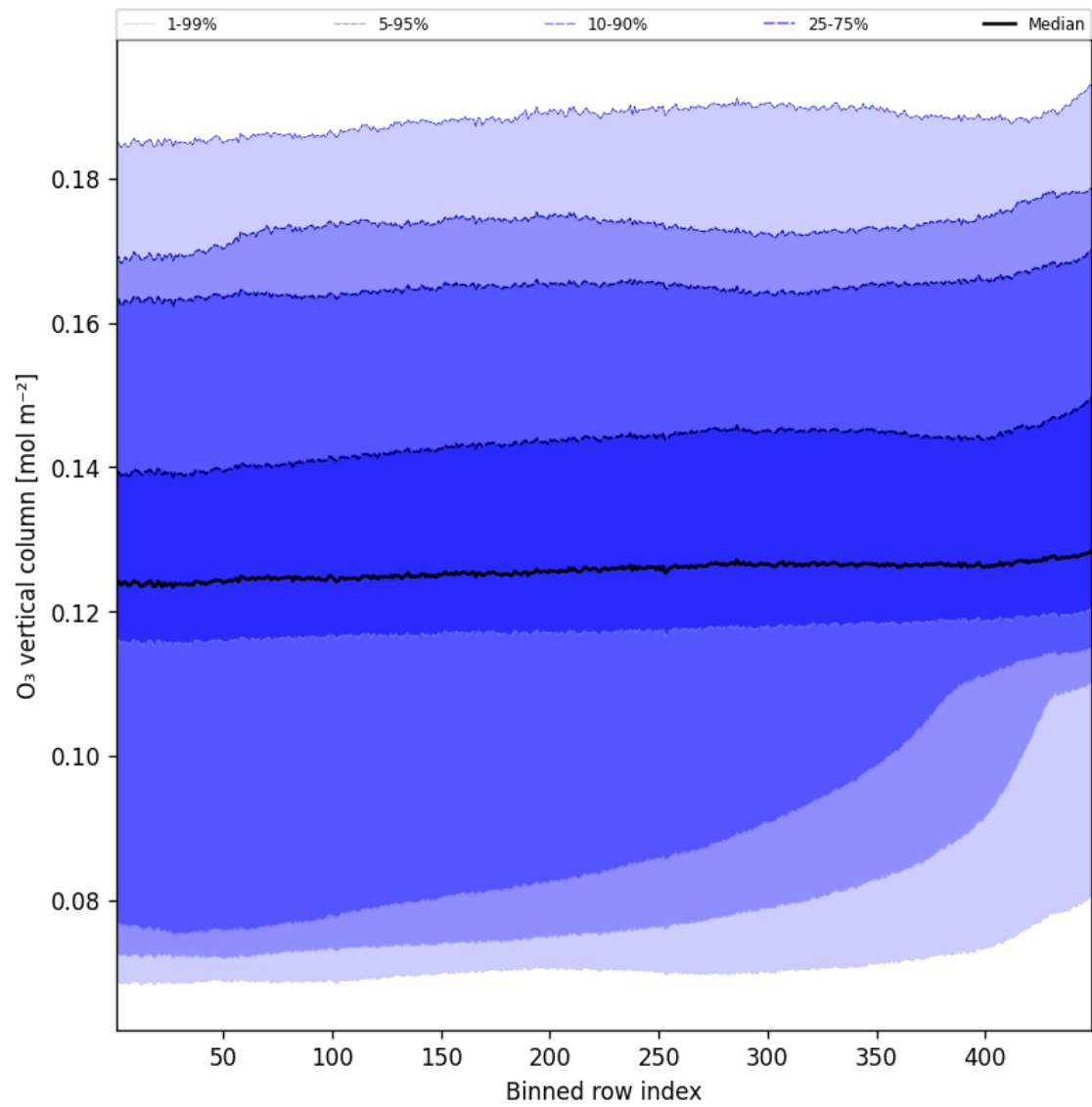
Figure 41: Along track statistics of “O 3 vertical column” for 2025-10-20 to 2025-10-20
