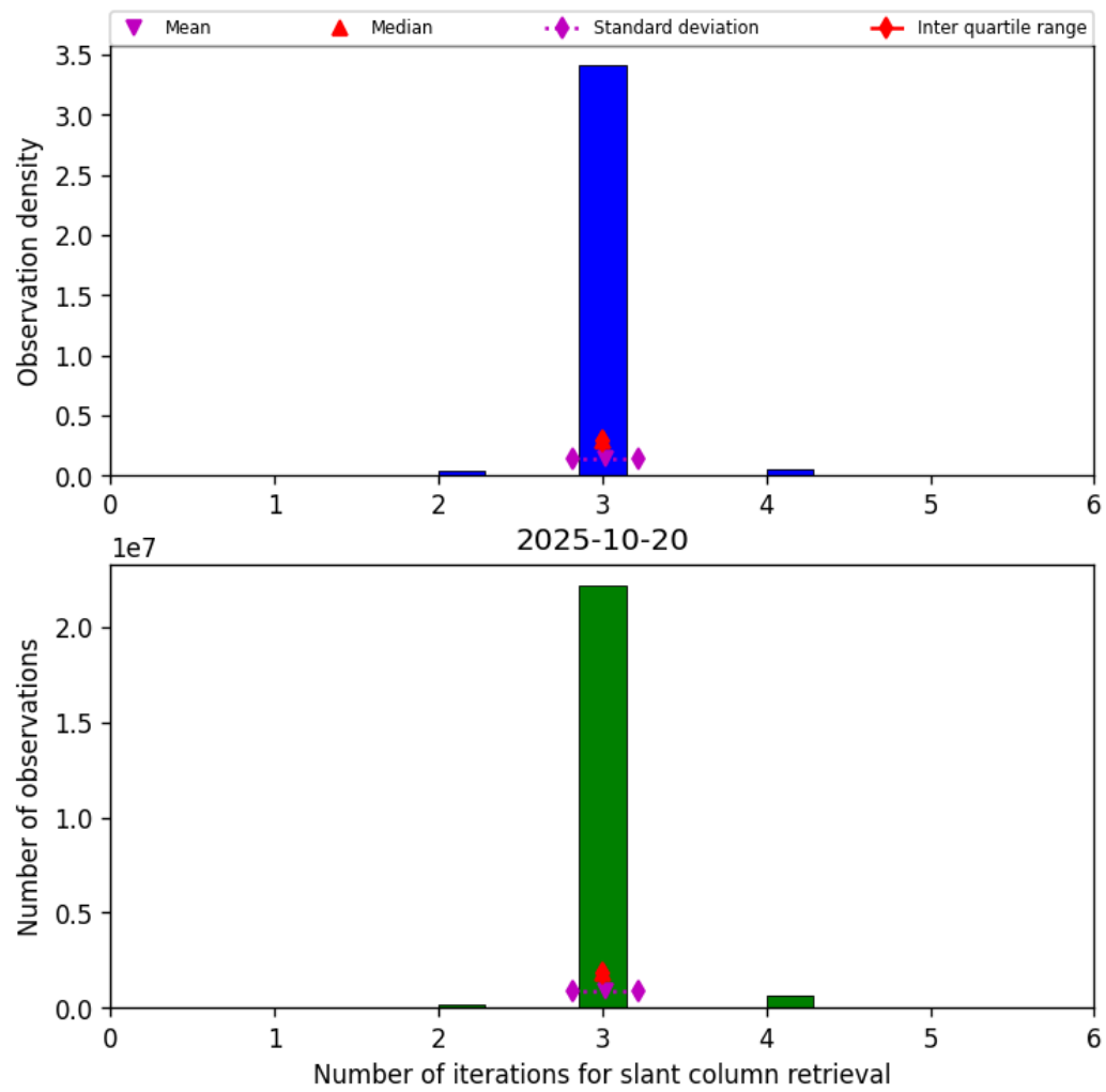
Figure 33: Histogram of “Number of iterations for slant column retrieval” for 2025-10-20 to 2025-10-20
