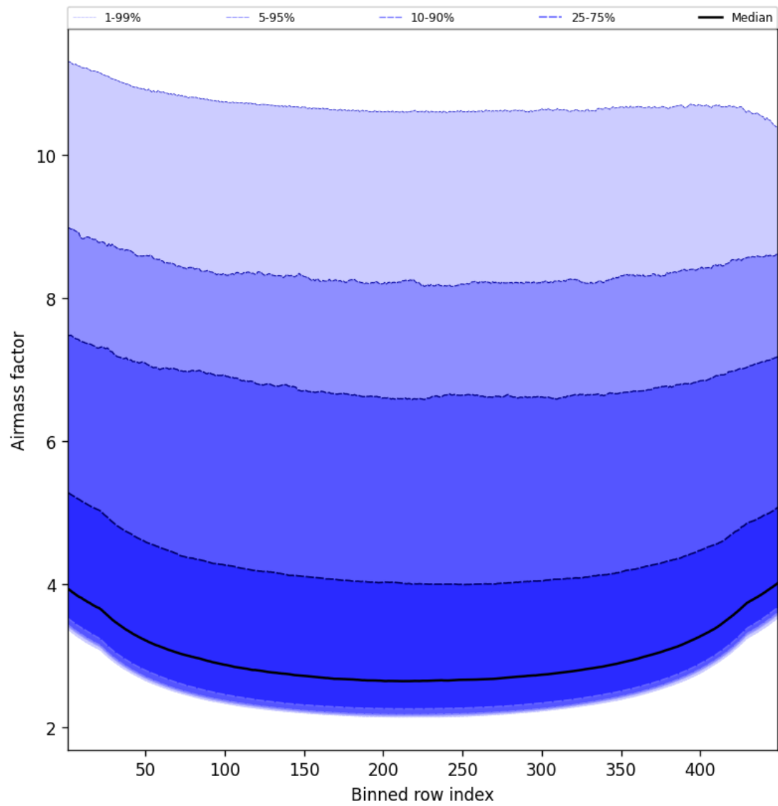
Figure 49: Along track statistics of “Airmass factor” for 2025-10-20 to 2025-10-20
