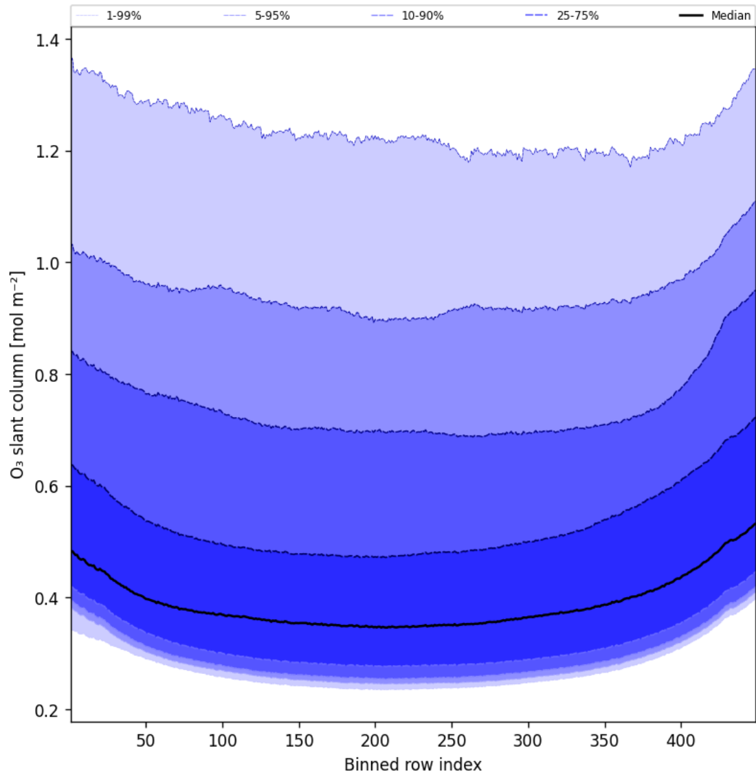
Figure 43: Along track statistics of “O 3 slant column” for 2025-10-20 to 2025-10-20
