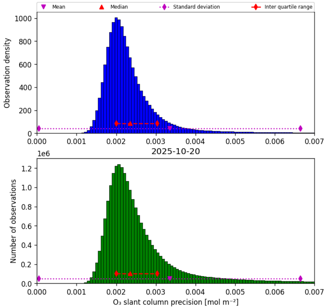
Figure 32: Histogram of “O 3 slant column precision” for 2025-10-20 to 2025-10-20
