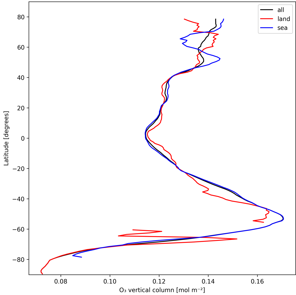
Figure 17: Zonal average of “O 3 vertical column” for 2025-10-20 to 2025-10-20.
