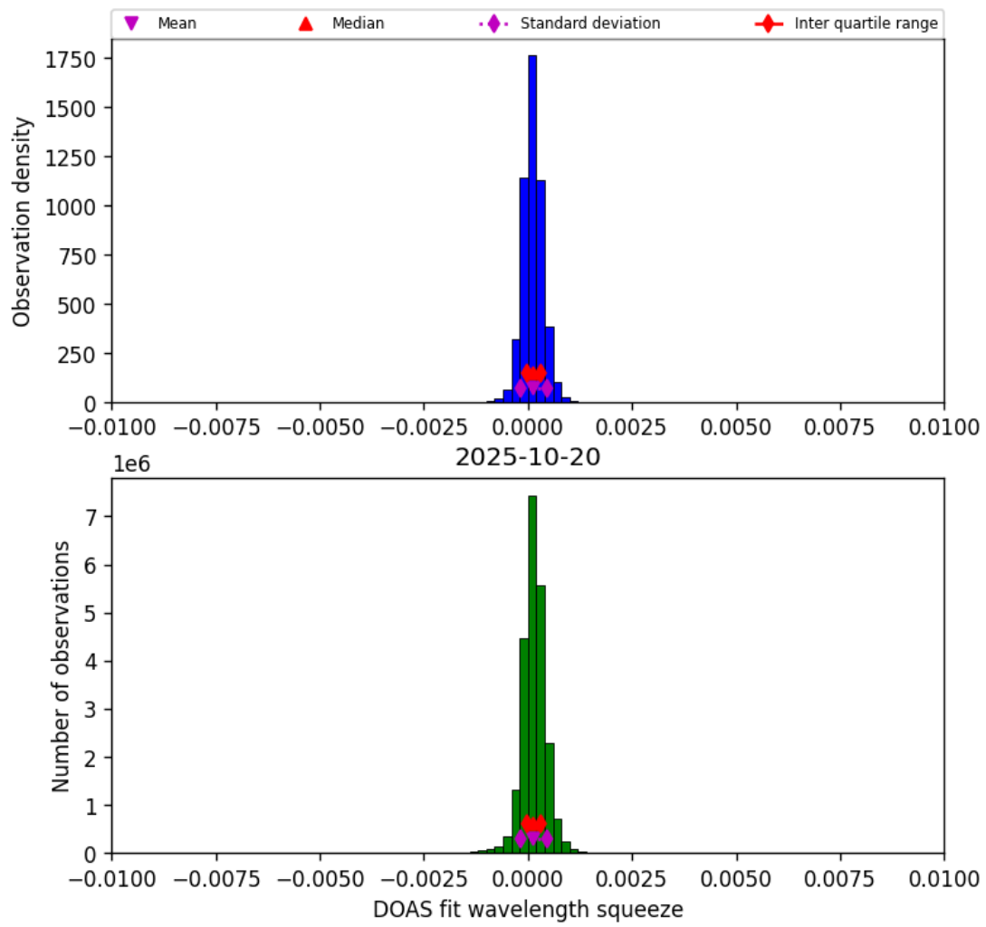
Figure 36: Histogram of “DOAS fit wavelength squeeze” for 2025-10-20 to 2025-10-20
