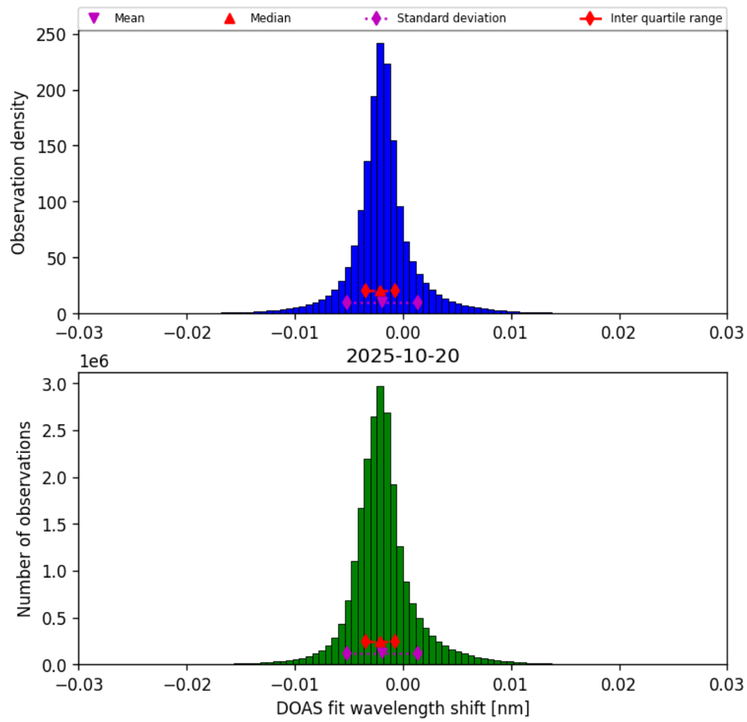
Figure 35: Histogram of “DOAS fit wavelength shift” for 2025-10-20 to 2025-10-20
