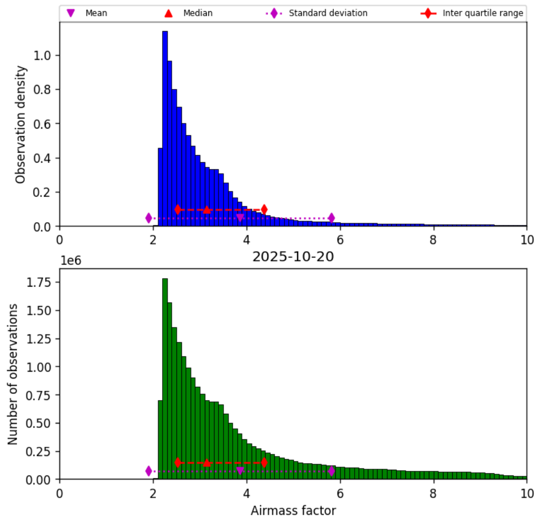
Figure 37: Histogram of “Airmass factor” for 2025-10-20 to 2025-10-20
