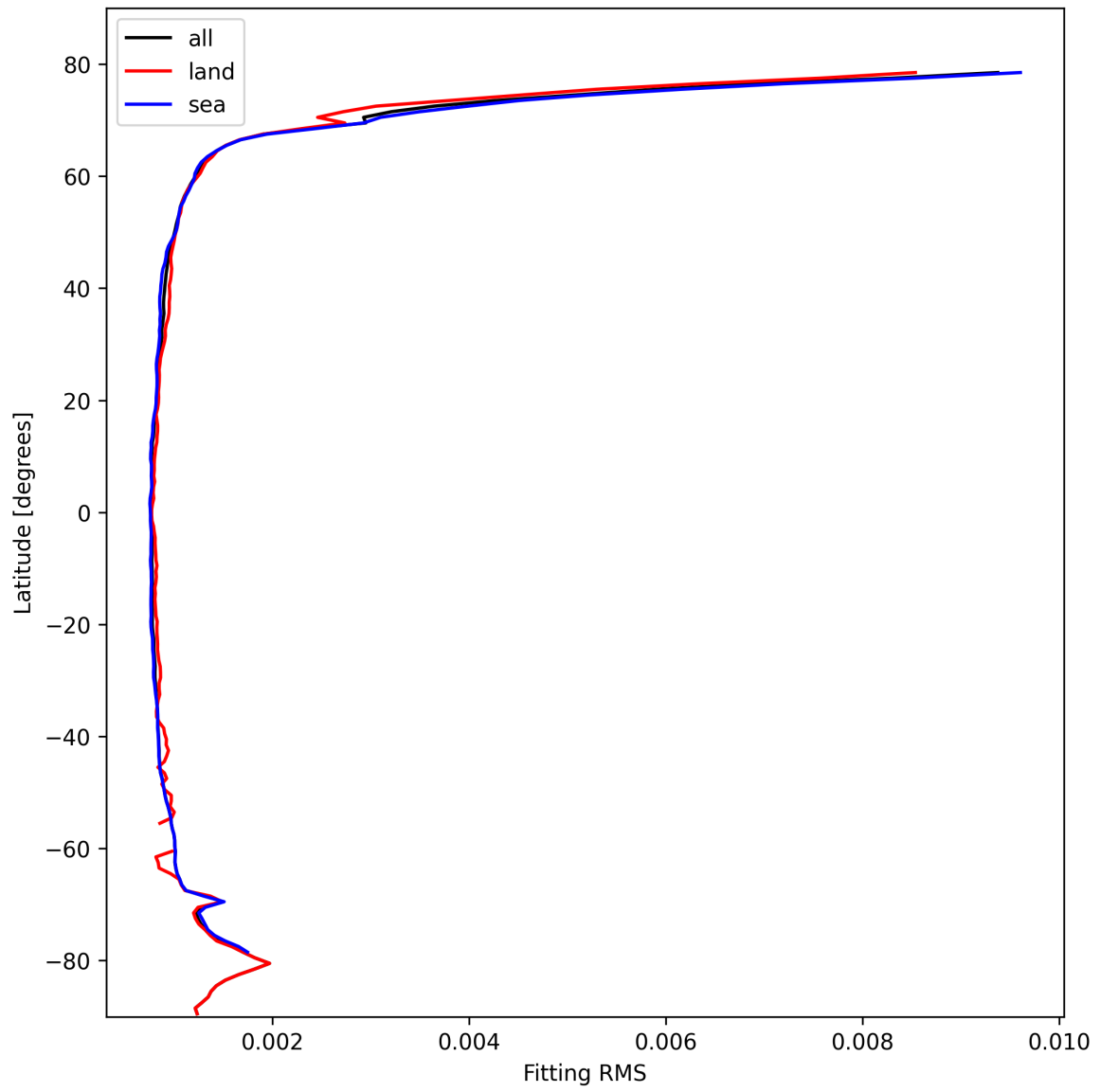
Figure 22: Zonal average of “Fitting RMS” for 2025-10-20 to 2025-10-20.
