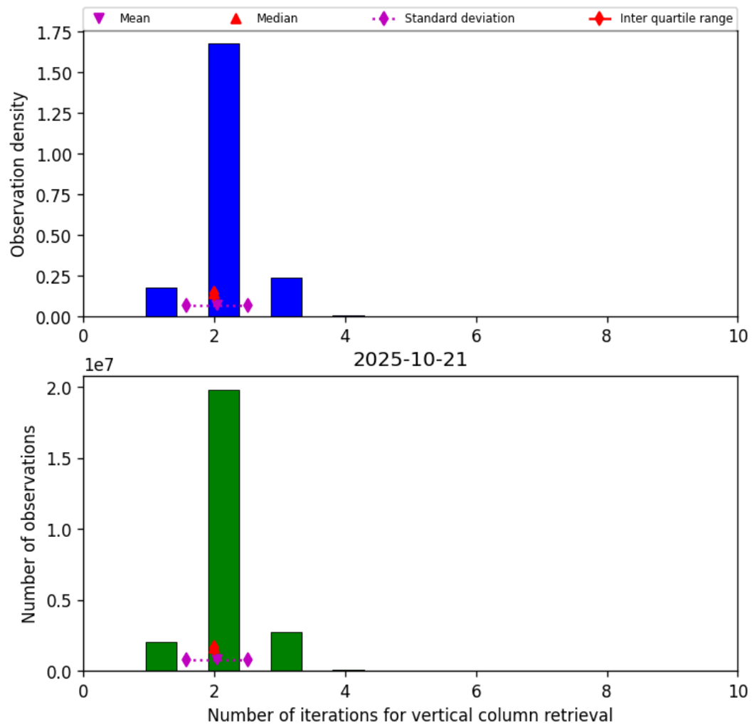
Figure 39: Histogram of “Number of iterations for vertical column retrieval” for 2025-10-21 to 2025-10-22
