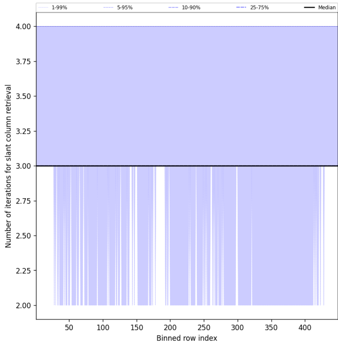
Figure 45: Along track statistics of “Number of iterations for slant column retrieval” for 2025-10-21 to 2025-10-22
