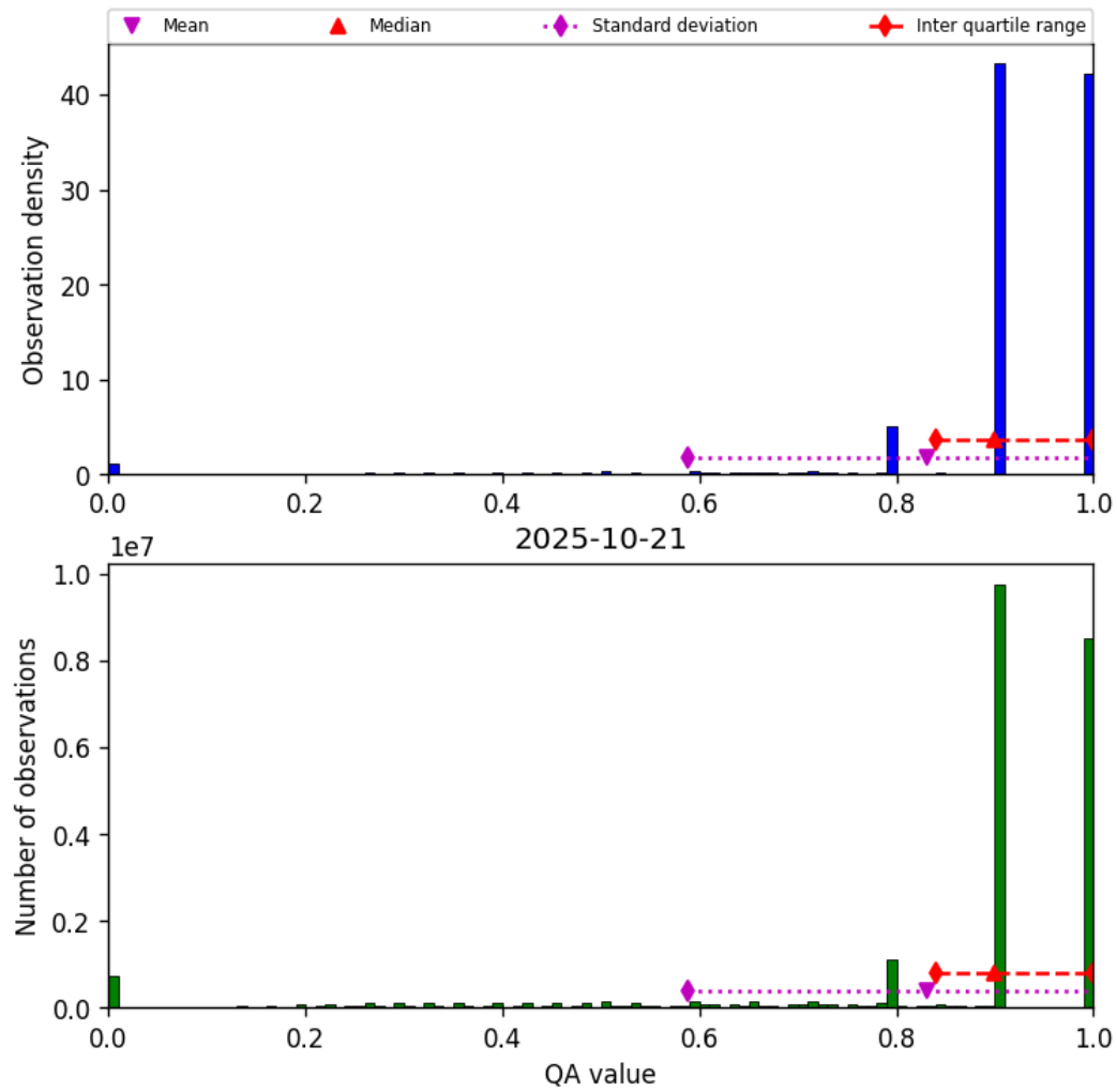
Figure 28: Histogram of “QA value” for 2025-10-21 to 2025-10-22
