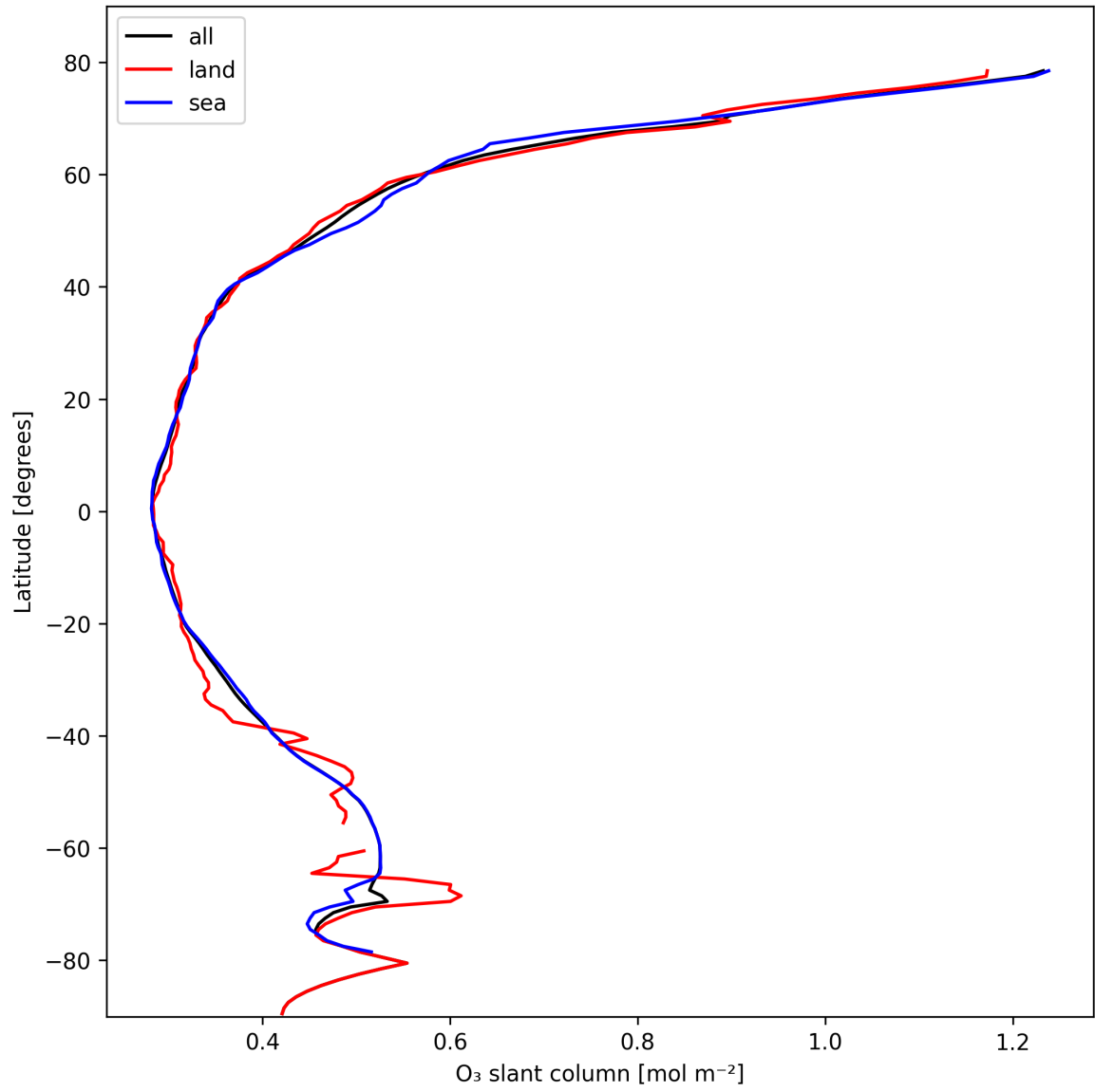
Figure 19: Zonal average of “O 3 slant column” for 2025-10-21 to 2025-10-22.
