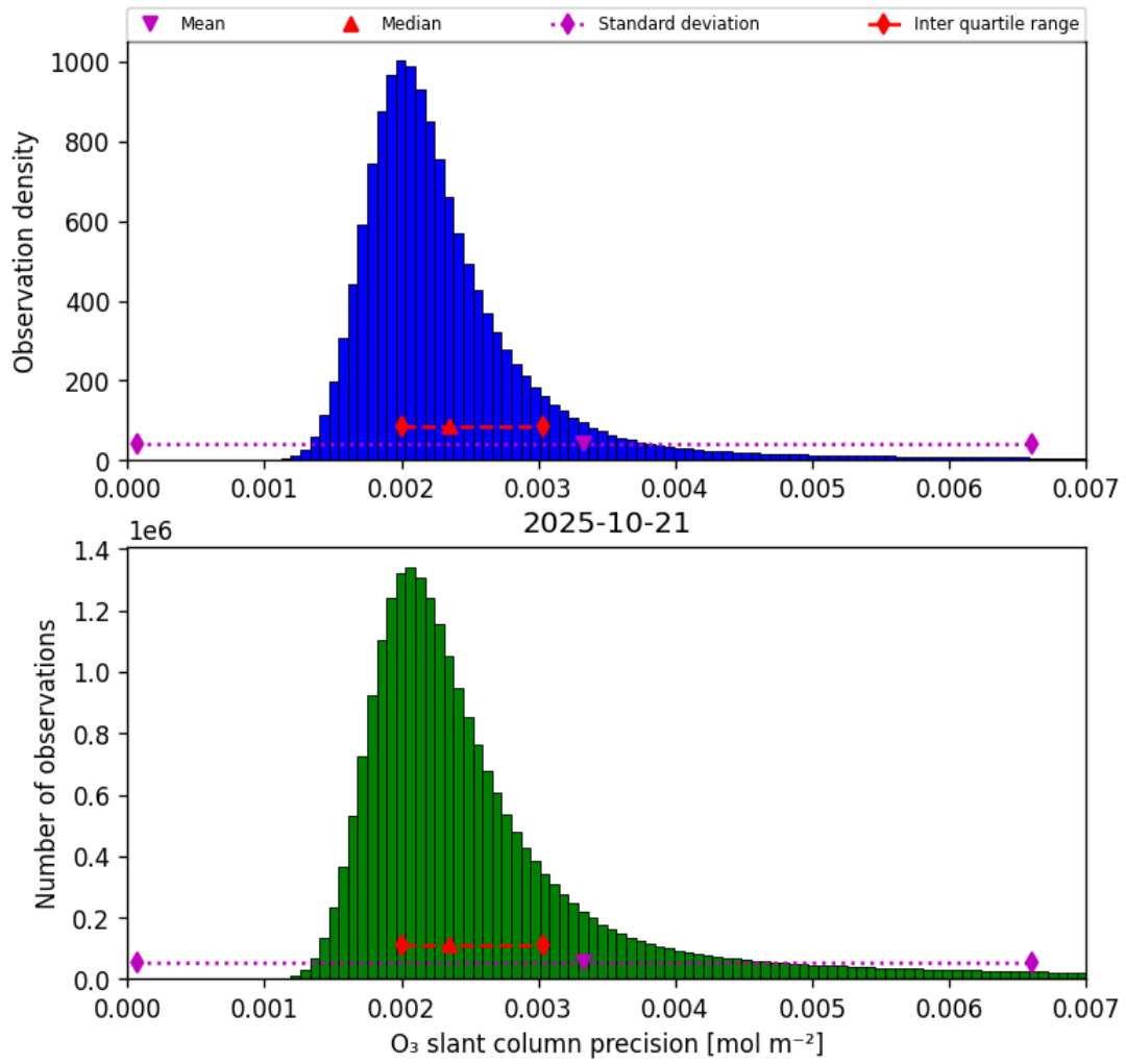
Figure 32: Histogram of “O 3 slant column precision” for 2025-10-21 to 2025-10-22
