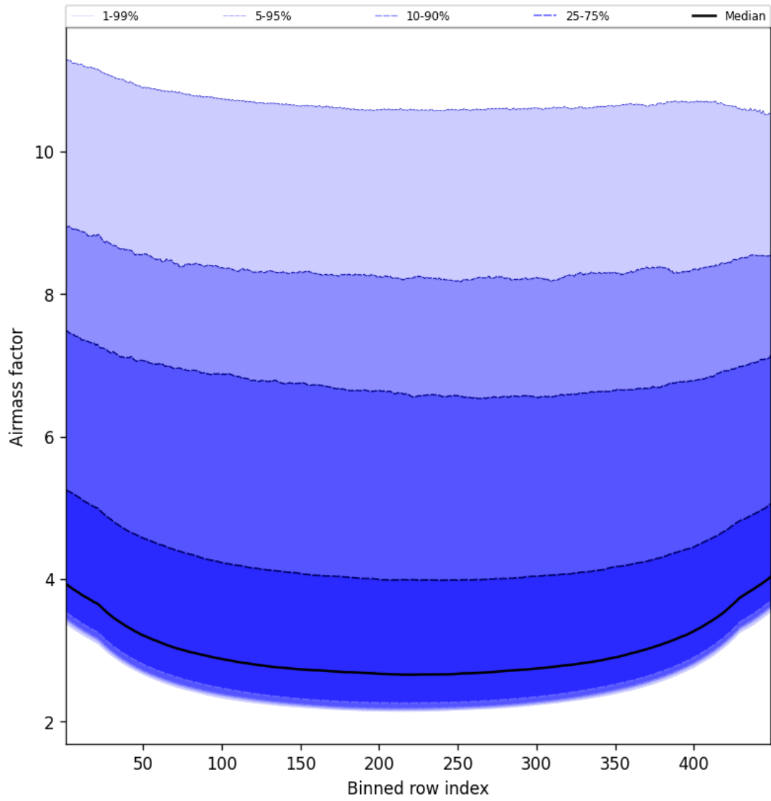
Figure 49: Along track statistics of “Airmass factor” for 2025-10-21 to 2025-10-22
