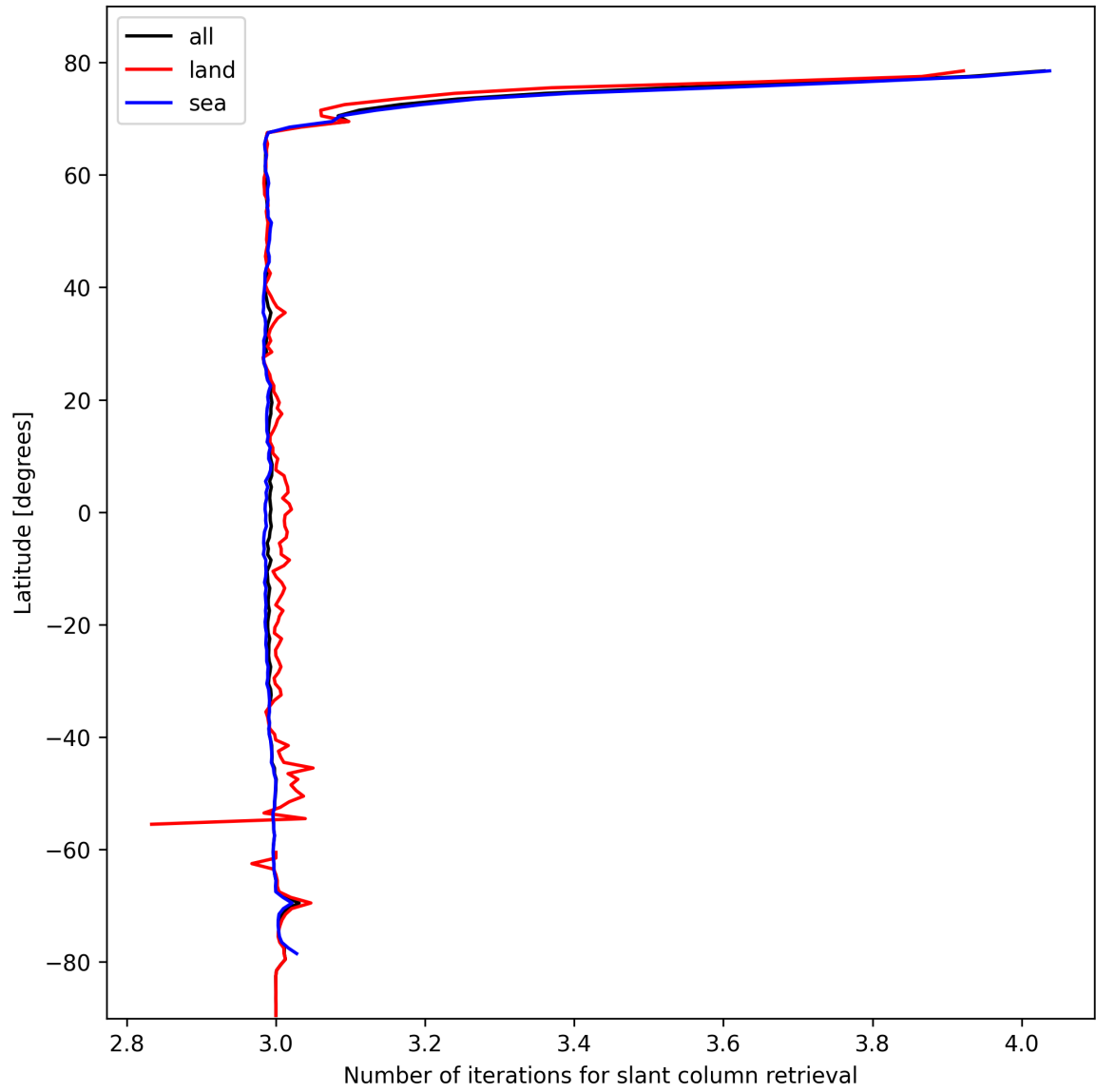
Figure 21: Zonal average of “Number of iterations for slant column retrieval” for 2025-10-21 to 2025-10-22.
