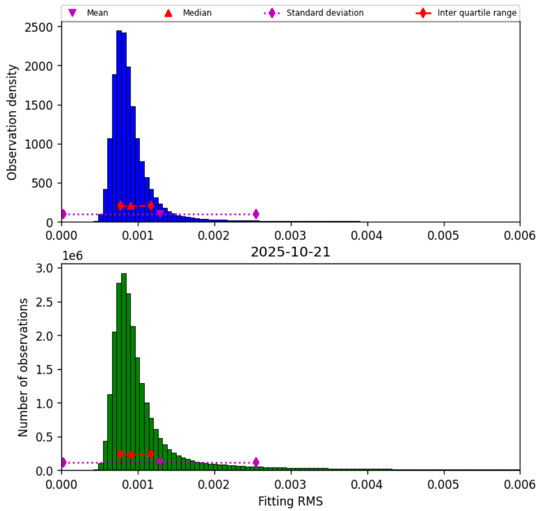
Figure 34: Histogram of “Fitting RMS” for 2025-10-21 to 2025-10-22
