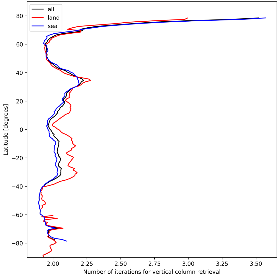
Figure 27: Zonal average of “Number of iterations for vertical column retrieval” for 2025-10-21 to 2025-10-22.
