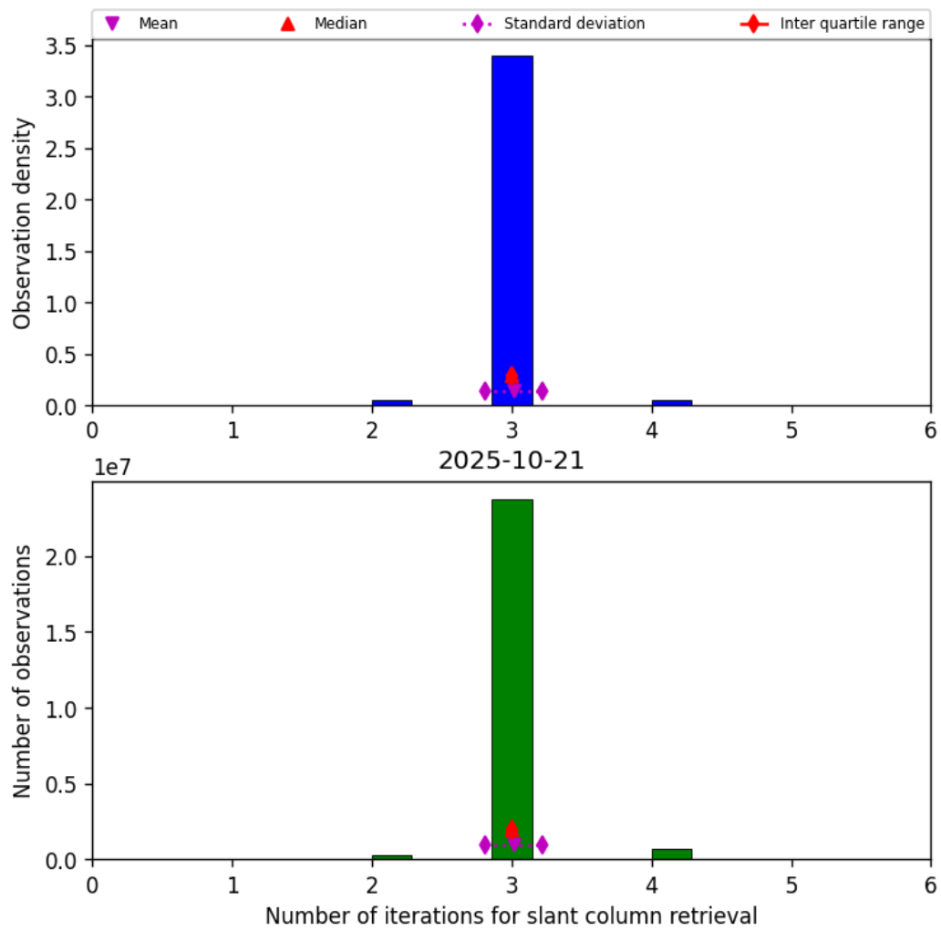
Figure 33: Histogram of “Number of iterations for slant column retrieval” for 2025-10-21 to 2025-10-22
