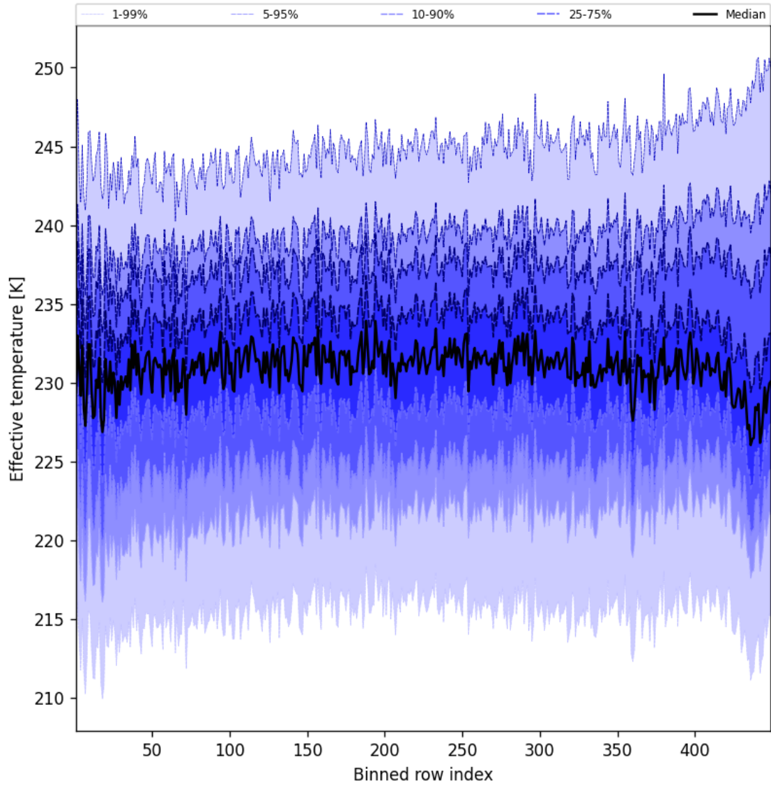
Figure 50: Along track statistics of “Effective temperature” for 2025-10-21 to 2025-10-22
