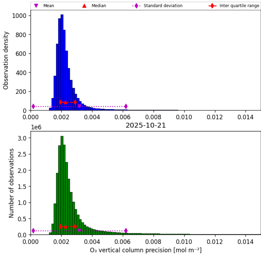
Figure 30: Histogram of “O 3 vertical column precision” for 2025-10-21 to 2025-10-22
