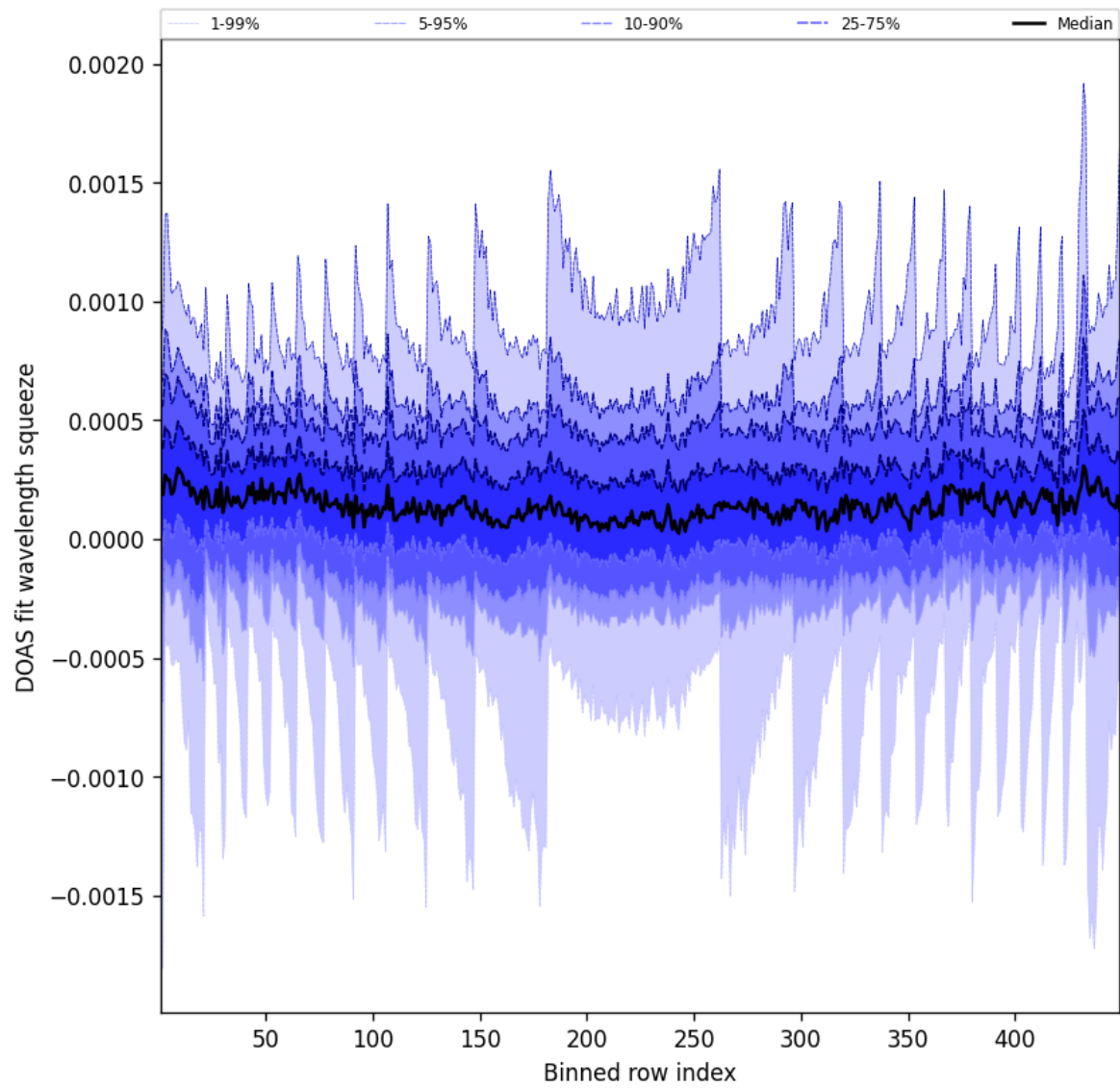
Figure 48: Along track statistics of “DOAS fit wavelength squeeze” for 2025-10-21 to 2025-10-22
