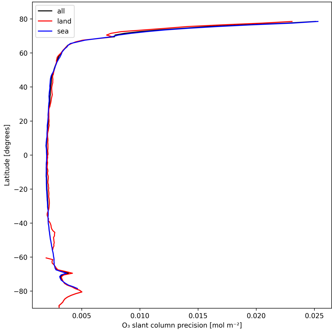
Figure 20: Zonal average of “O 3 slant column precision” for 2025-10-21 to 2025-10-22.
