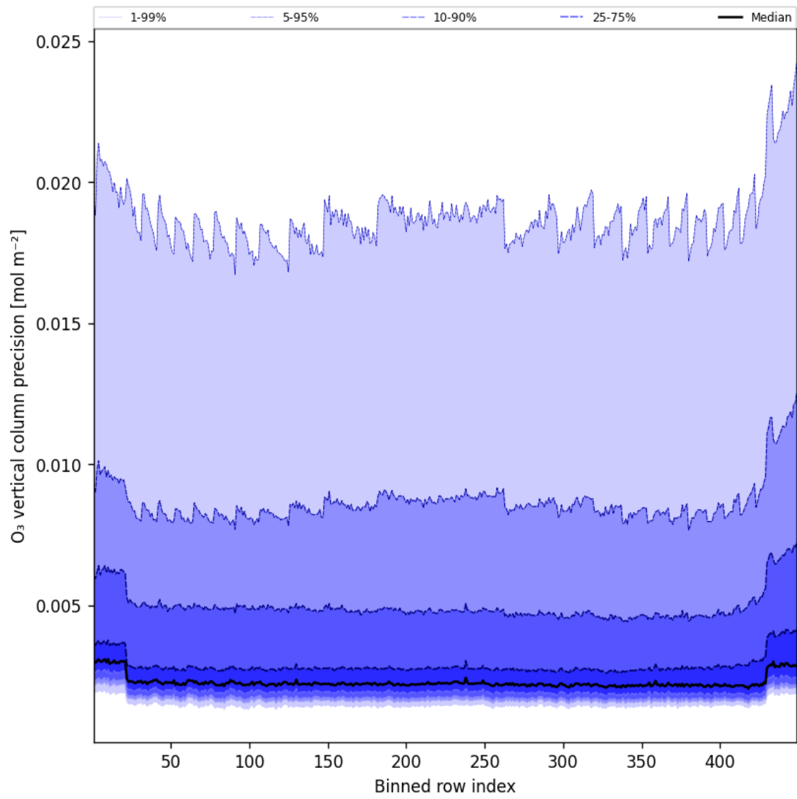
Figure 42: Along track statistics of “O 3 vertical column precision” for 2025-10-21 to 2025-10-22
