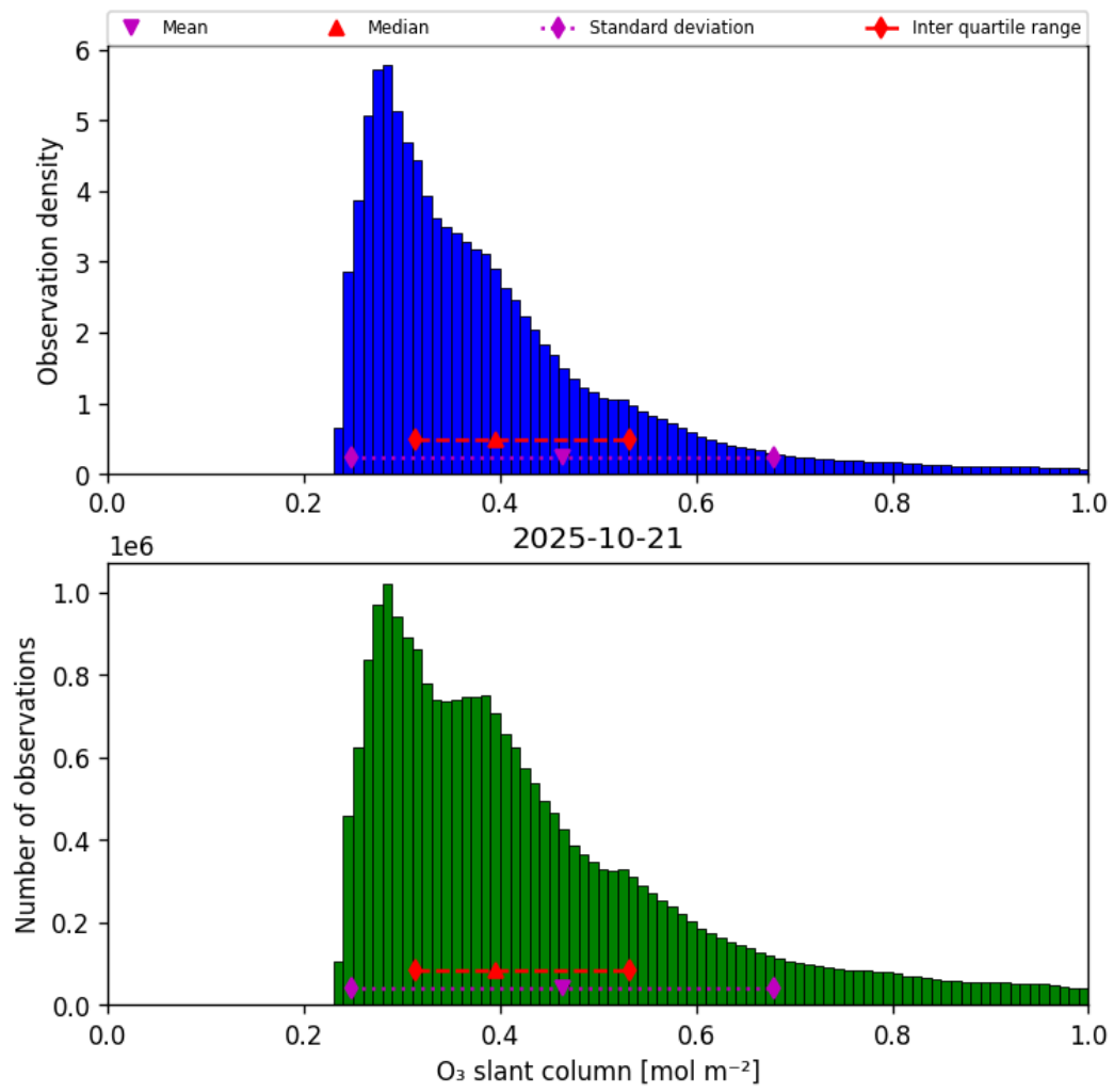
Figure 31: Histogram of “O 3 slant column” for 2025-10-21 to 2025-10-22
