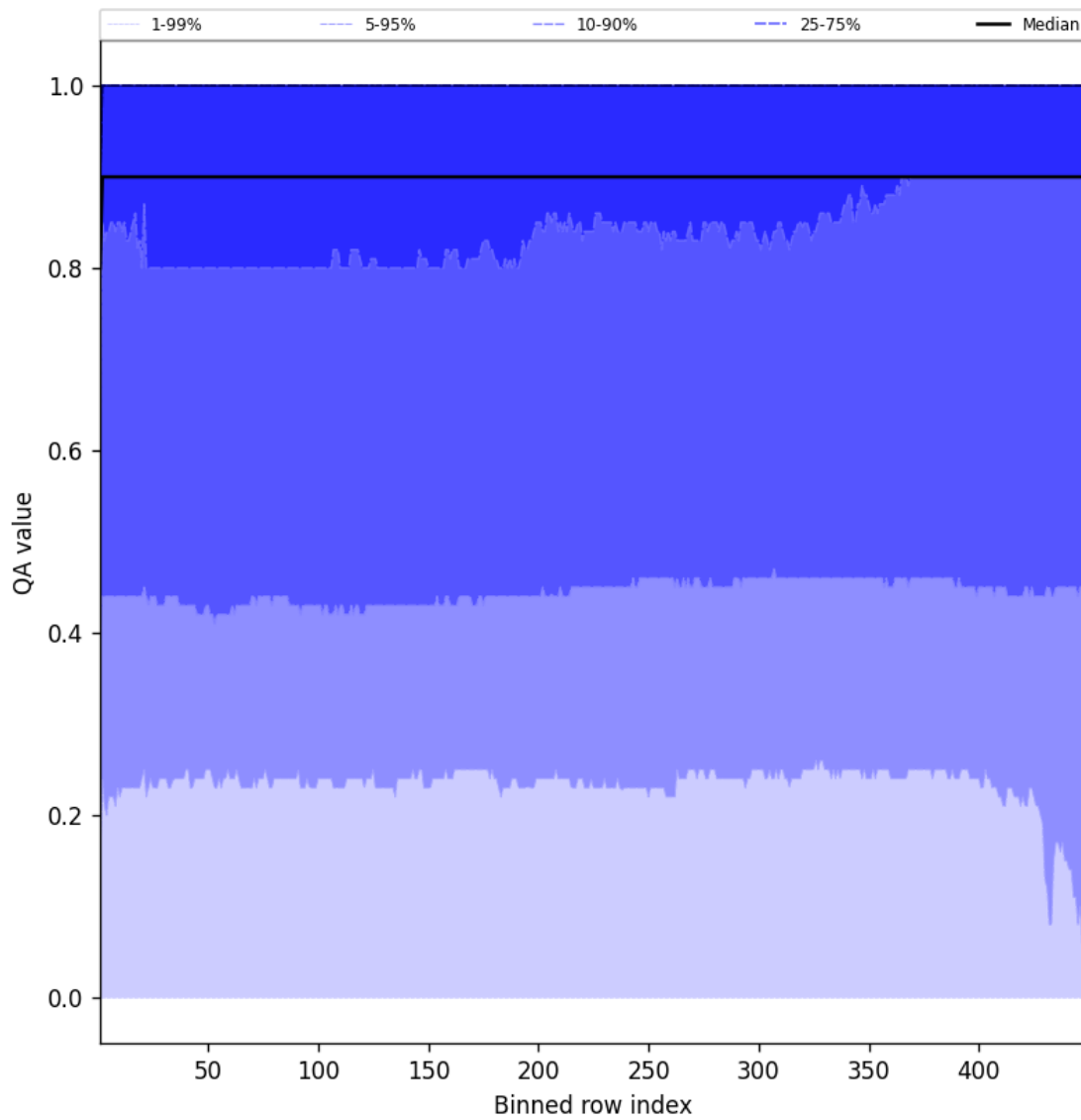
Figure 40: Along track statistics of “QA value” for 2025-10-21 to 2025-10-22
