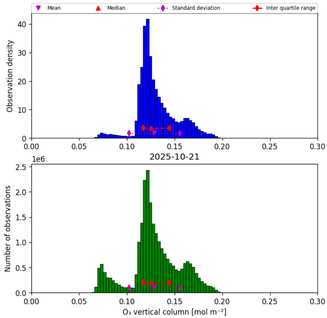
Figure 29: Histogram of “O 3 vertical column” for 2025-10-21 to 2025-10-22
