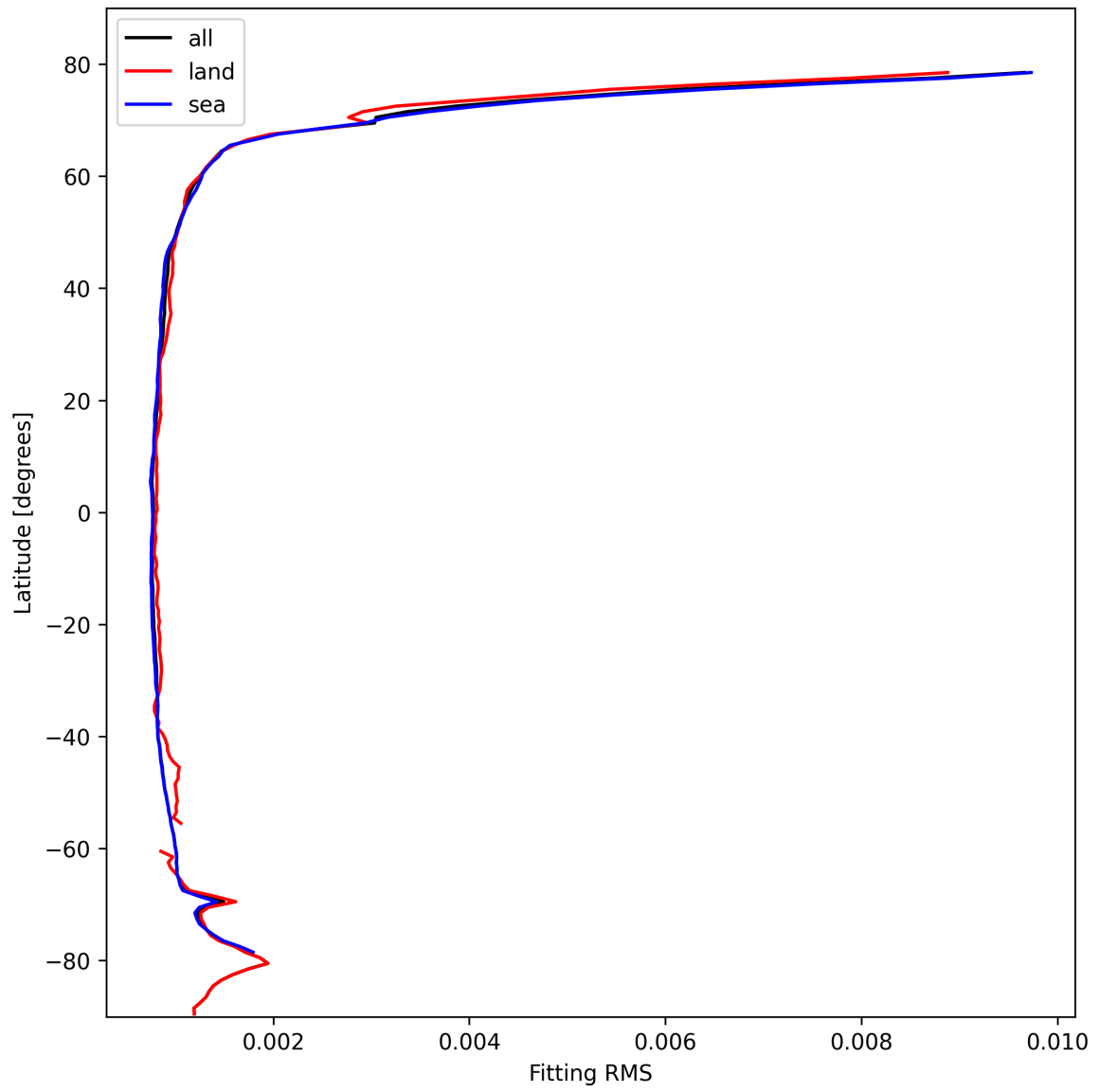
Figure 22: Zonal average of “Fitting RMS” for 2025-10-21 to 2025-10-22.
