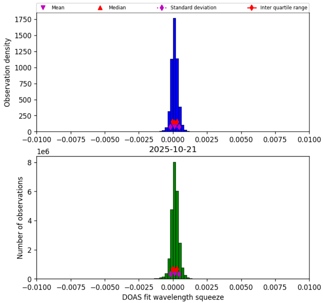
Figure 36: Histogram of “DOAS fit wavelength squeeze” for 2025-10-21 to 2025-10-22
