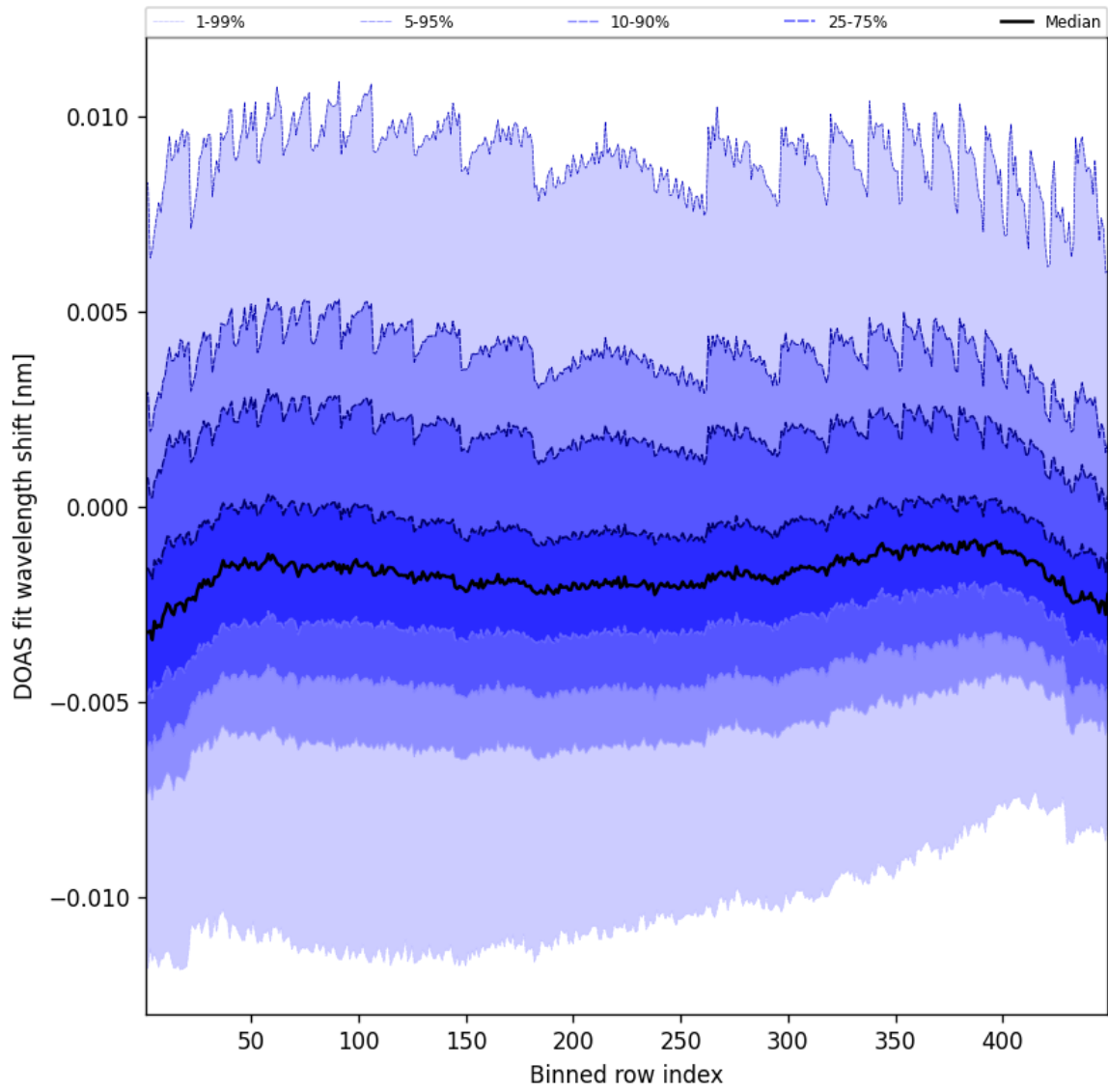
Figure 47: Along track statistics of “DOAS fit wavelength shift” for 2025-10-21 to 2025-10-22
