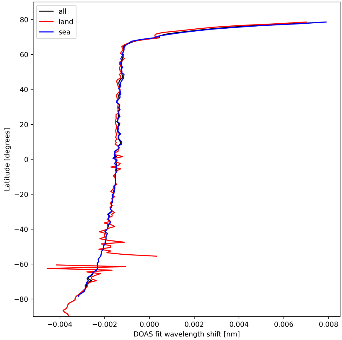
Figure 23: Zonal average of “DOAS fit wavelength shift” for 2025-10-21 to 2025-10-22.
