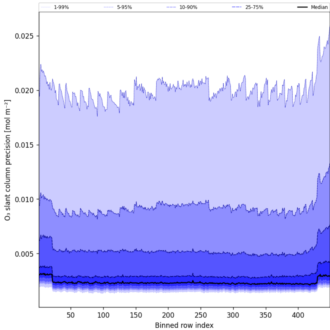
Figure 44: Along track statistics of “O 3 slant column precision” for 2025-10-21 to 2025-10-22
