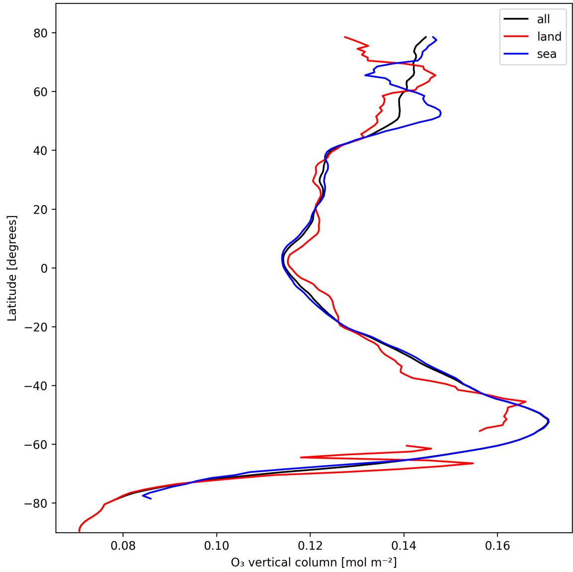
Figure 17: Zonal average of “O 3 vertical column” for 2025-10-21 to 2025-10-22.
