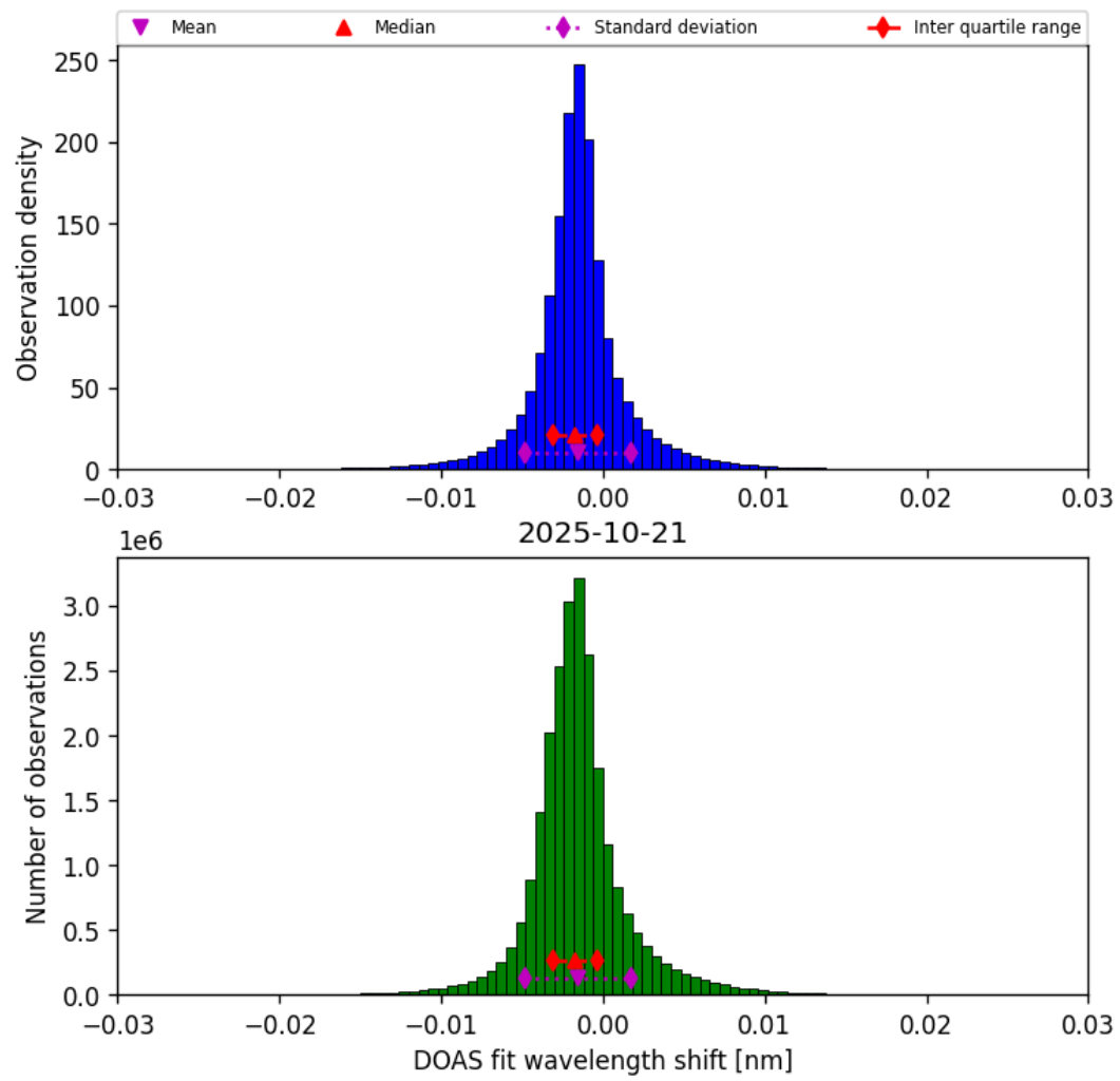
Figure 35: Histogram of “DOAS fit wavelength shift” for 2025-10-21 to 2025-10-22
