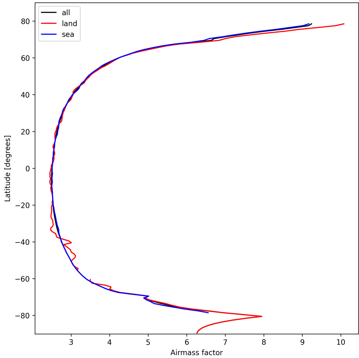
Figure 25: Zonal average of “Airmass factor” for 2025-10-21 to 2025-10-22.
