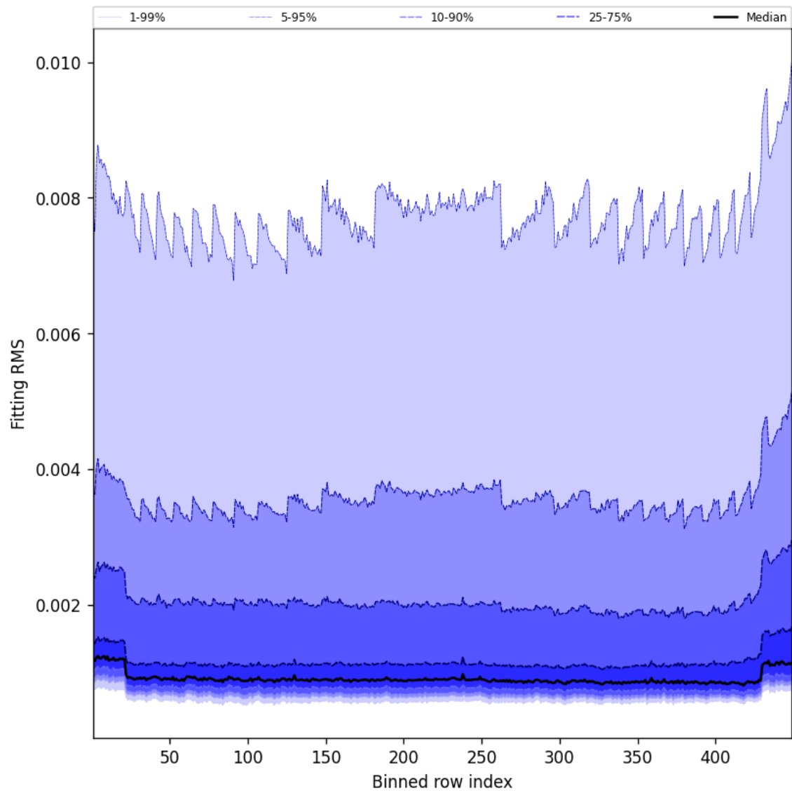
Figure 46: Along track statistics of “Fitting RMS” for 2025-10-21 to 2025-10-22
