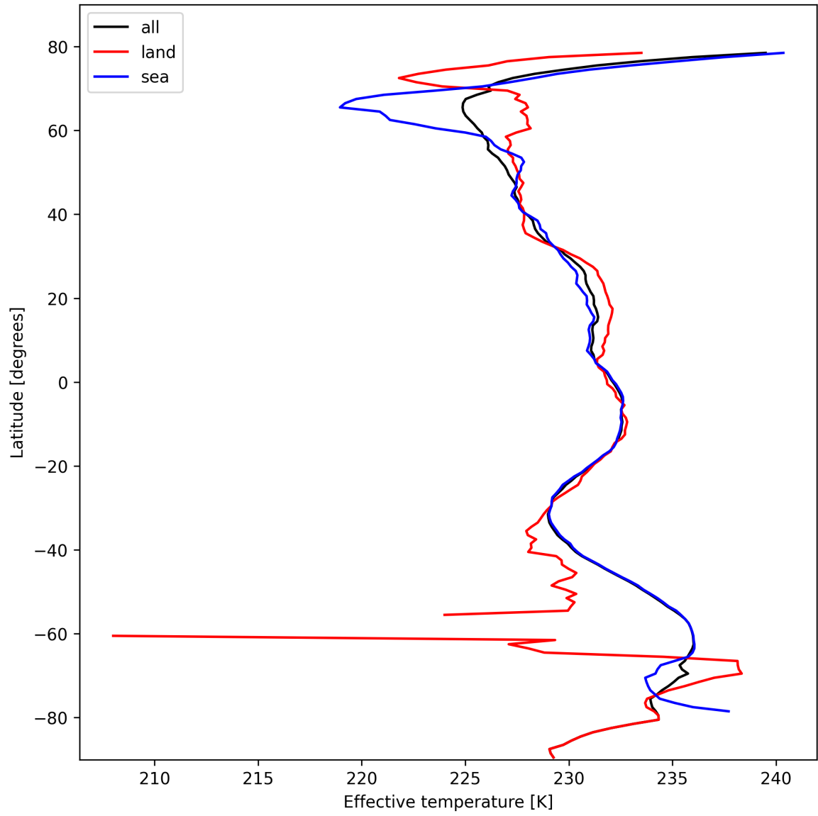
Figure 26: Zonal average of “Effective temperature” for 2025-10-21 to 2025-10-22.
