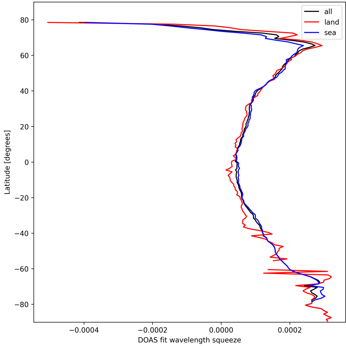
Figure 24: Zonal average of “DOAS fit wavelength squeeze” for 2025-10-21 to 2025-10-22.
