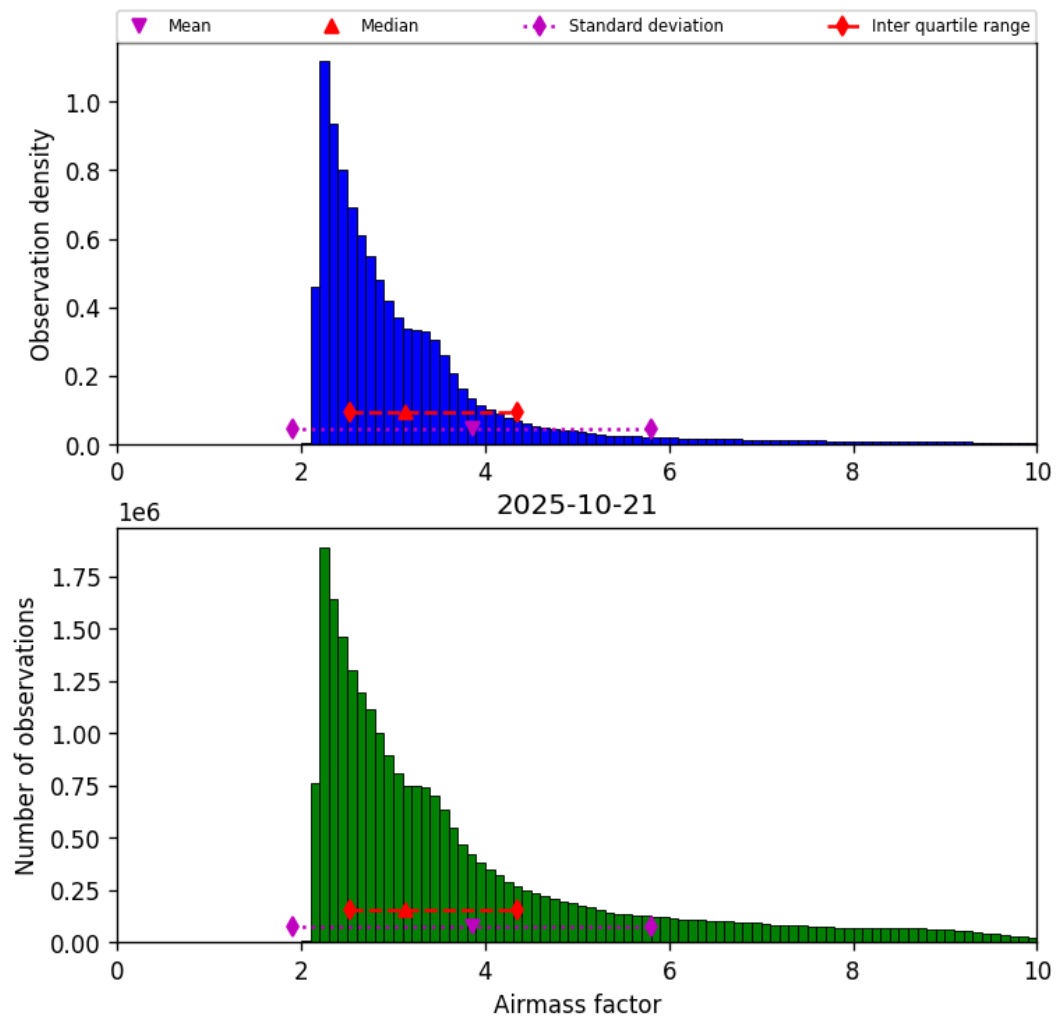
Figure 37: Histogram of “Airmass factor” for 2025-10-21 to 2025-10-22
