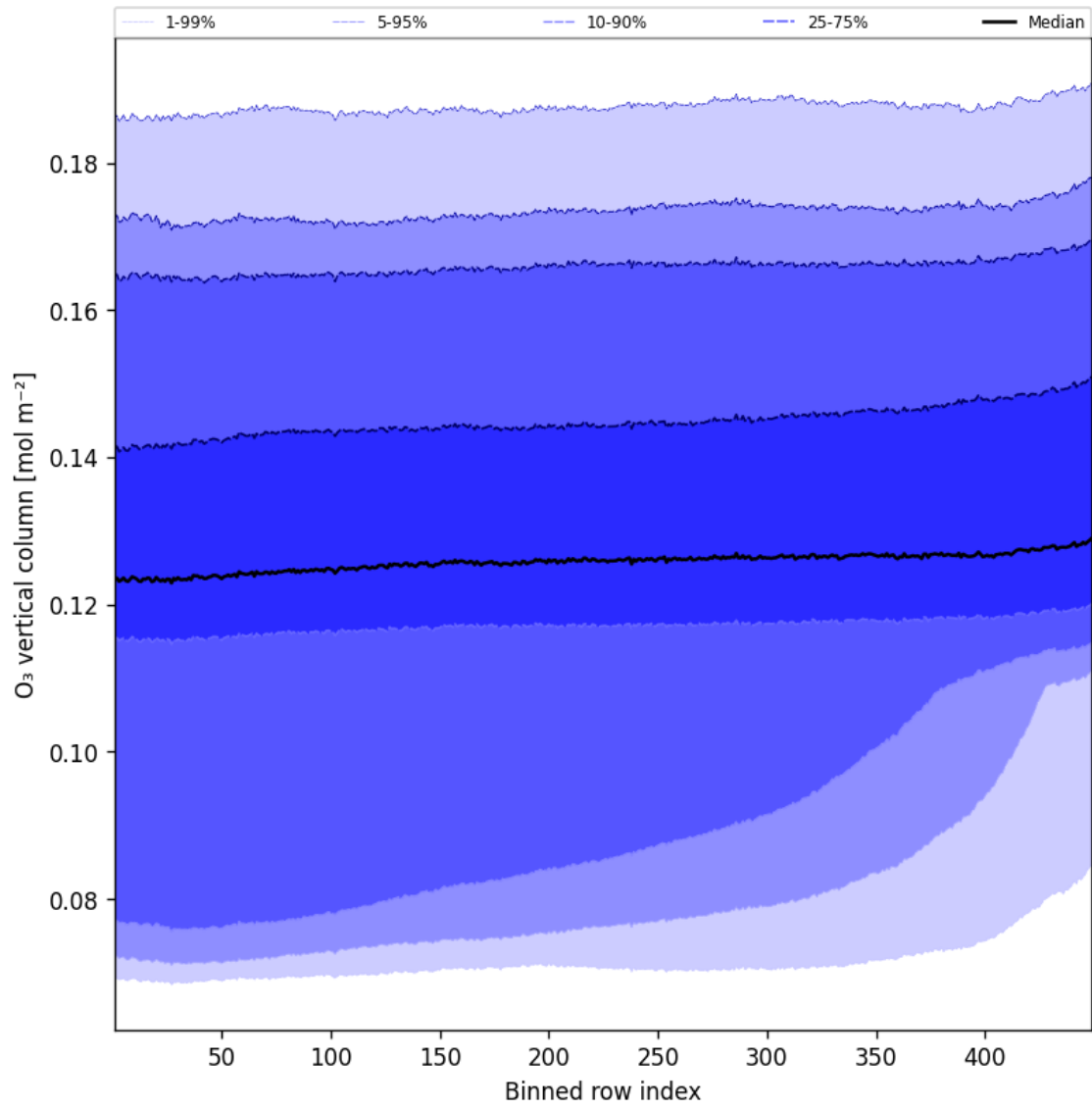
Figure 41: Along track statistics of “O 3 vertical column” for 2025-10-21 to 2025-10-22
