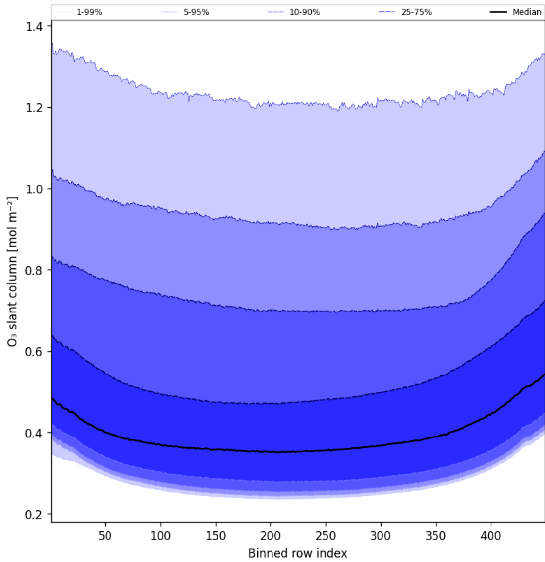
Figure 43: Along track statistics of “O 3 slant column” for 2025-10-21 to 2025-10-22
