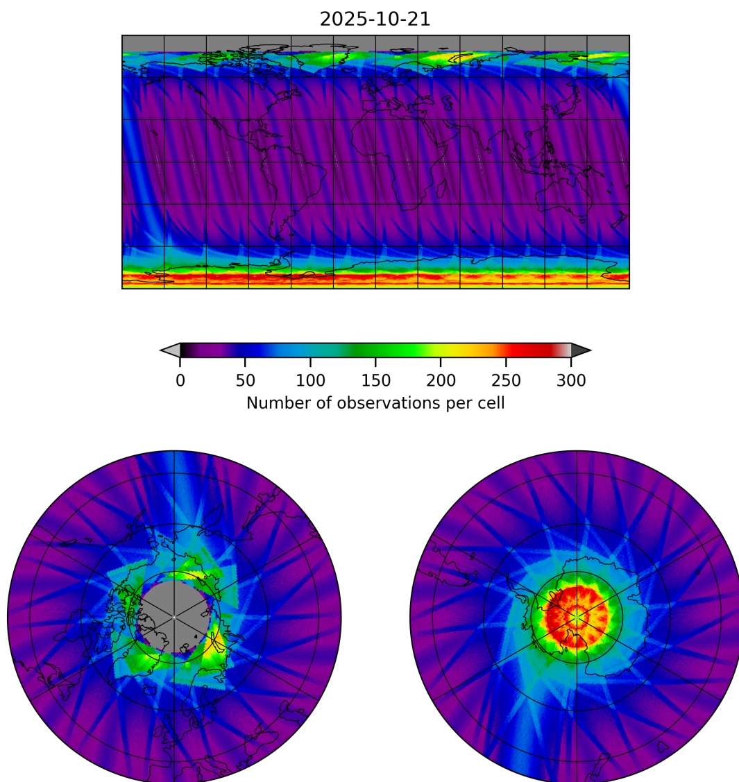
Figure 15: Map of the number of observations for 2025-10-21 to 2025-10-22
