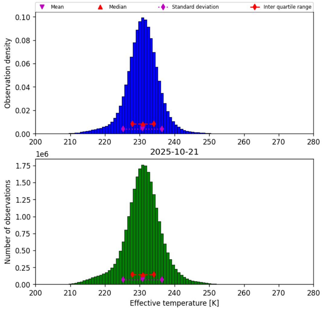
Figure 38: Histogram of “Effective temperature” for 2025-10-21 to 2025-10-22
