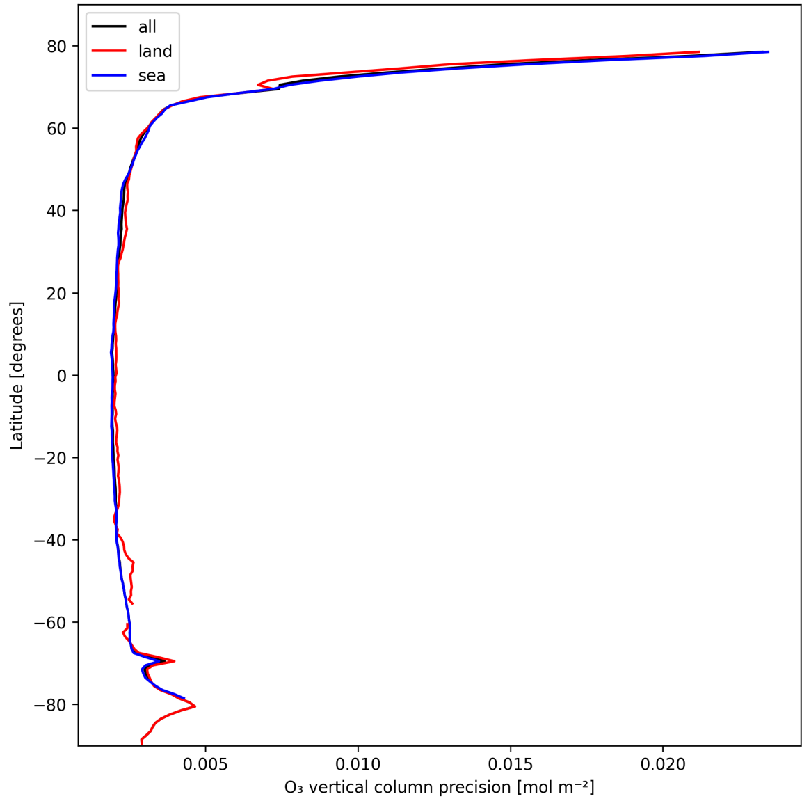
Figure 18: Zonal average of “O 3 vertical column precision” for 2025-10-21 to 2025-10-22.
