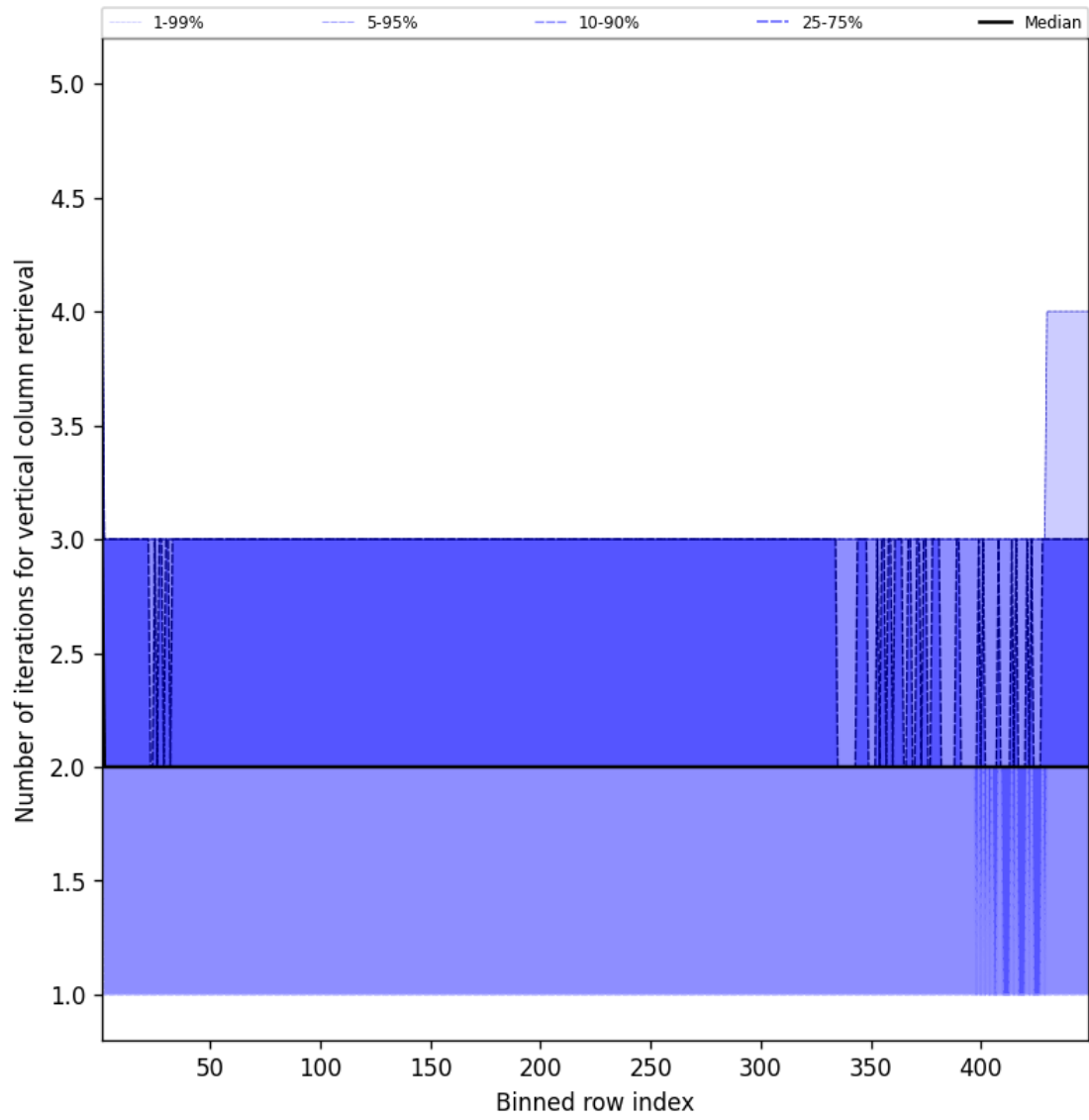
Figure 51: Along track statistics of “Number of iterations for vertical column retrieval” for 2025-10-21 to 2025-10-22
