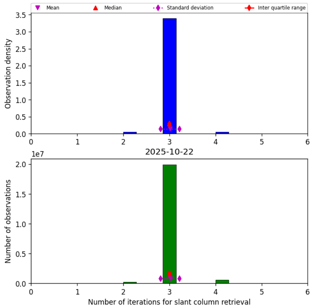
Figure 33: Histogram of “Number of iterations for slant column retrieval” for 2025-10-22 to 2025-10-23
