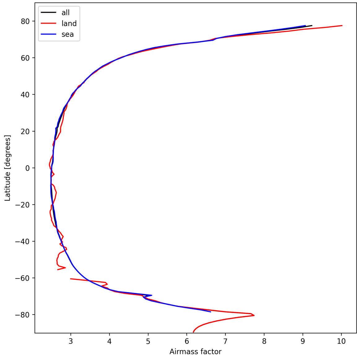
Figure 25: Zonal average of “Airmass factor” for 2025-10-22 to 2025-10-23.
