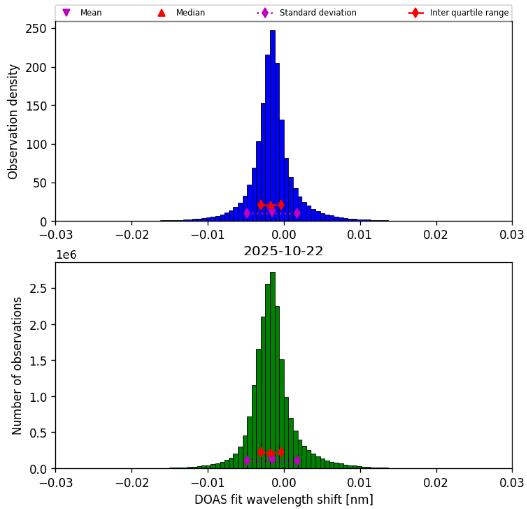
Figure 35: Histogram of “DOAS fit wavelength shift” for 2025-10-22 to 2025-10-23
