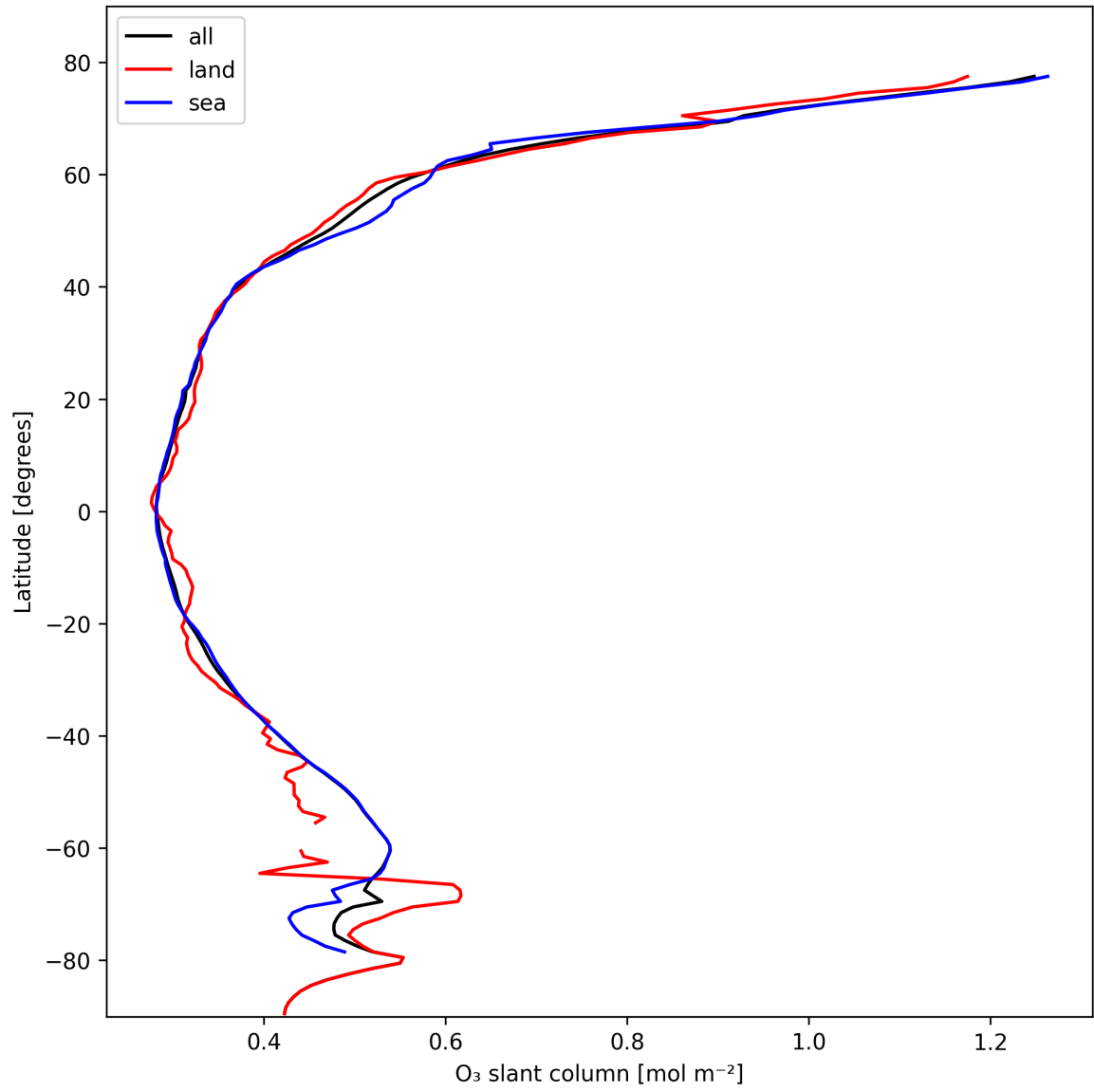
Figure 19: Zonal average of “O 3 slant column” for 2025-10-22 to 2025-10-23.
