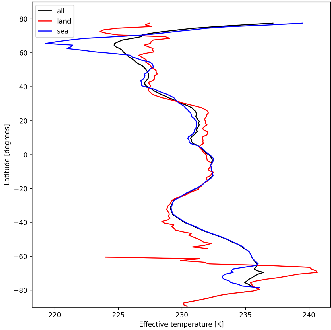
Figure 26: Zonal average of “Effective temperature” for 2025-10-22 to 2025-10-23.
