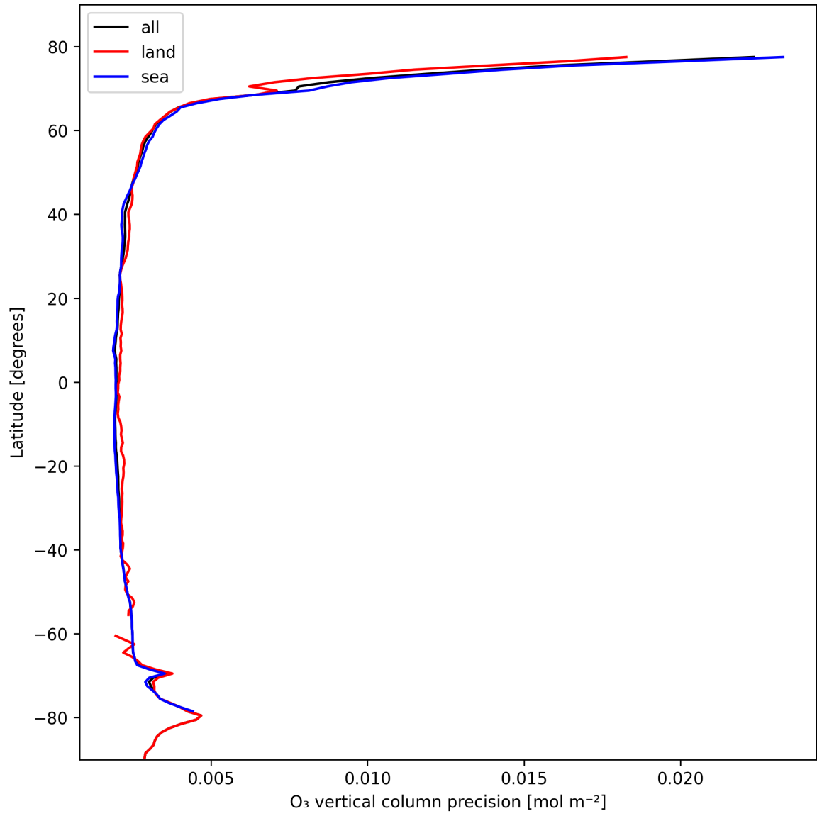
Figure 18: Zonal average of “O 3 vertical column precision” for 2025-10-22 to 2025-10-23.
