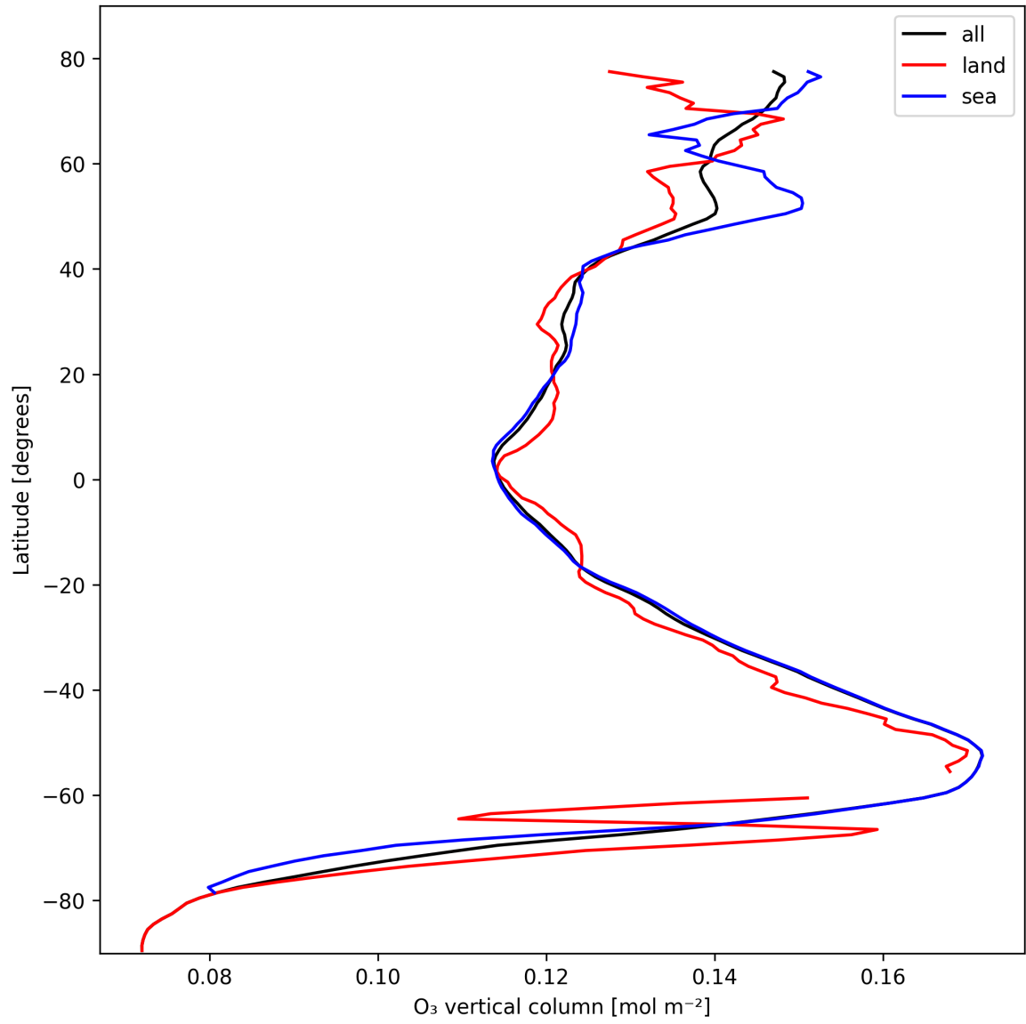
Figure 17: Zonal average of “O 3 vertical column” for 2025-10-22 to 2025-10-23.
