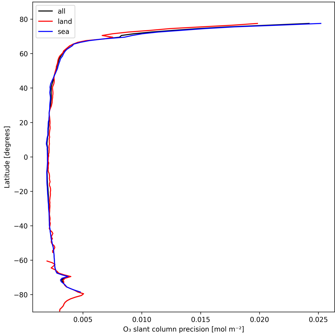
Figure 20: Zonal average of “O 3 slant column precision” for 2025-10-22 to 2025-10-23.
