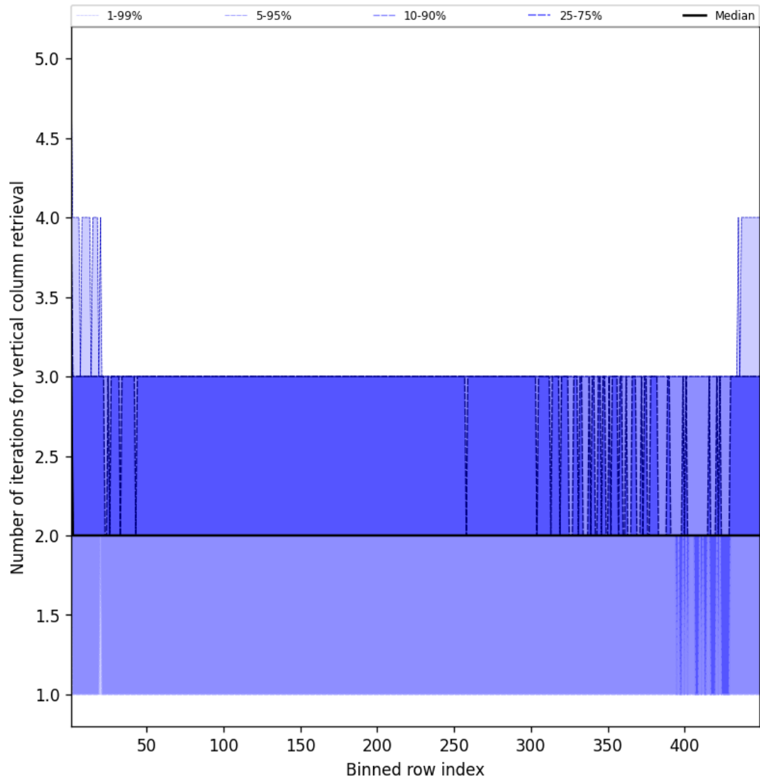
Figure 51: Along track statistics of “Number of iterations for vertical column retrieval” for 2025-10-22 to 2025-10-23
