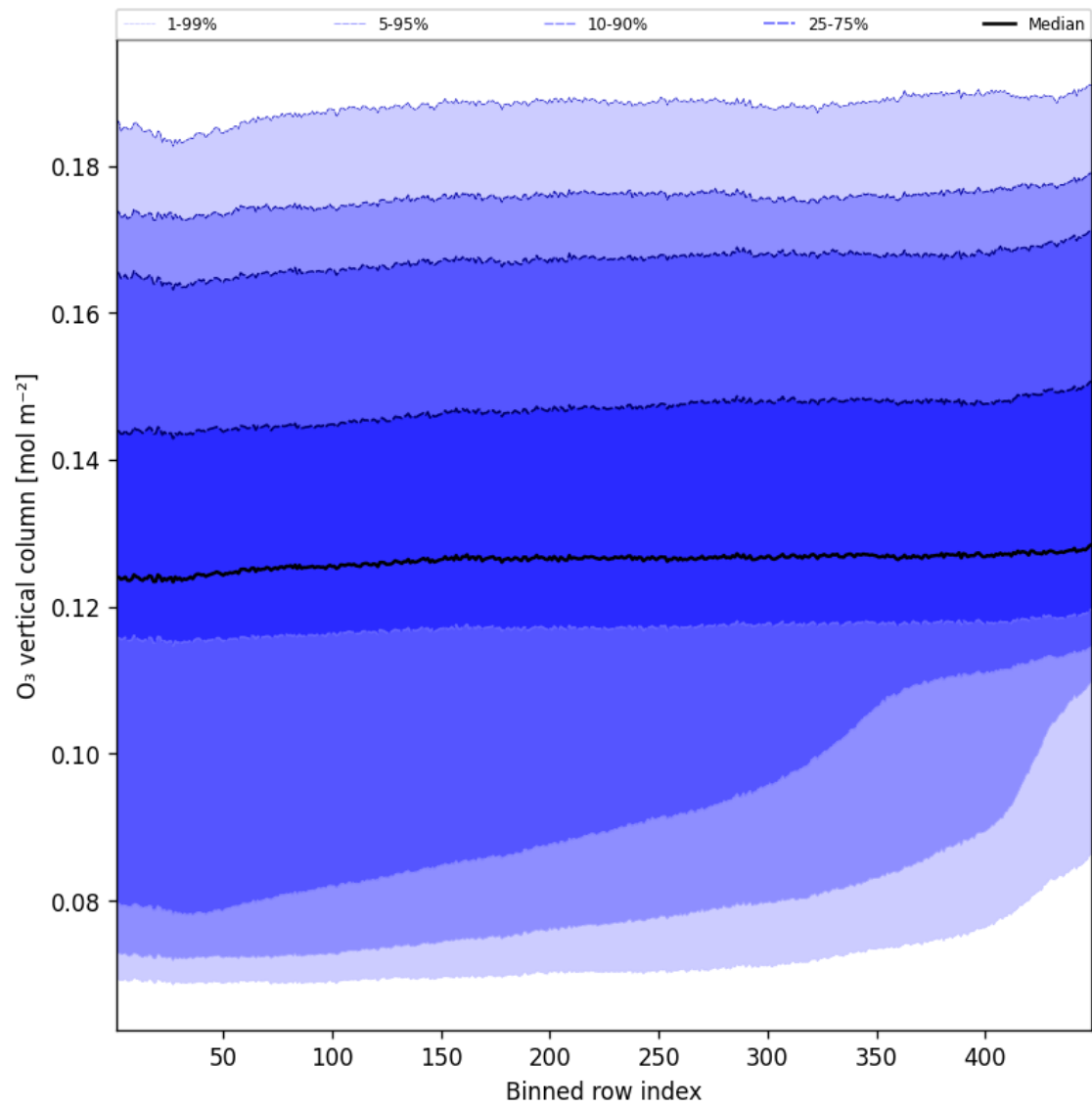
Figure 41: Along track statistics of “O 3 vertical column” for 2025-10-22 to 2025-10-23
