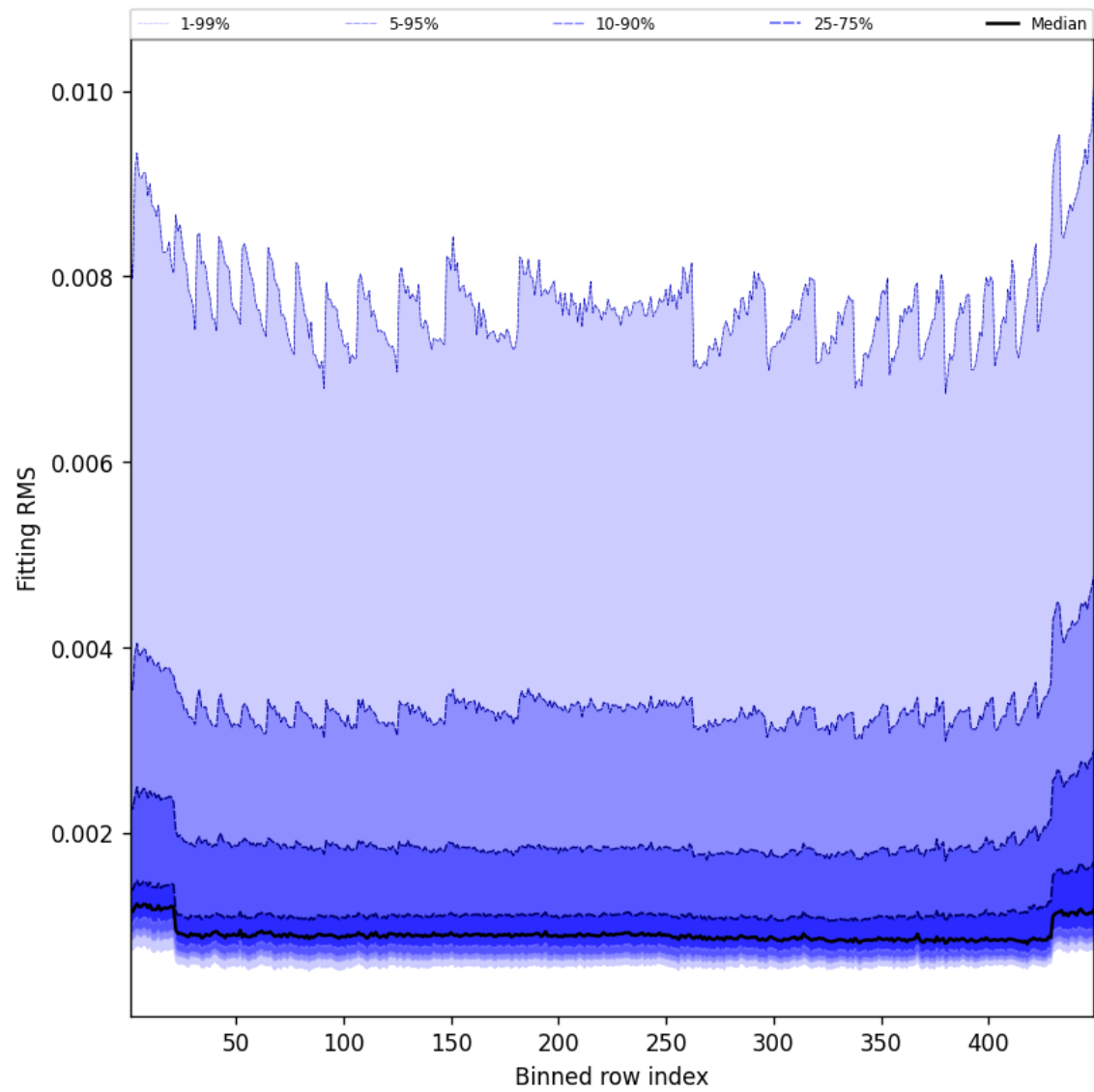
Figure 46: Along track statistics of “Fitting RMS” for 2025-10-22 to 2025-10-23
