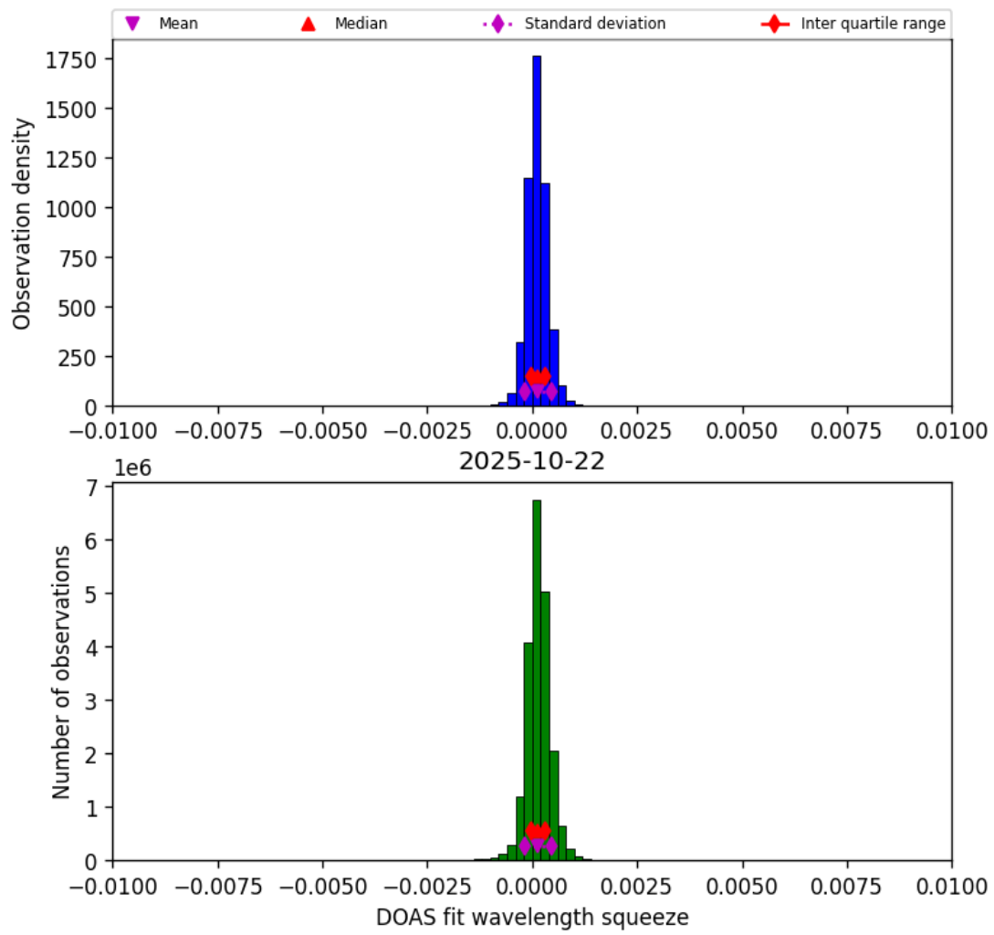
Figure 36: Histogram of “DOAS fit wavelength squeeze” for 2025-10-22 to 2025-10-23
