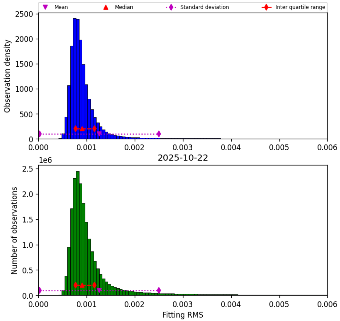
Figure 34: Histogram of “Fitting RMS” for 2025-10-22 to 2025-10-23
