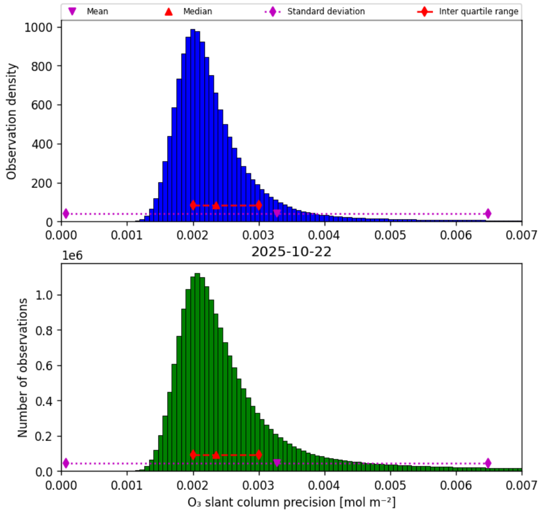
Figure 32: Histogram of “O 3 slant column precision” for 2025-10-22 to 2025-10-23
