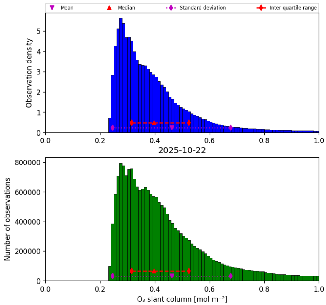
Figure 31: Histogram of “O 3 slant column” for 2025-10-22 to 2025-10-23
