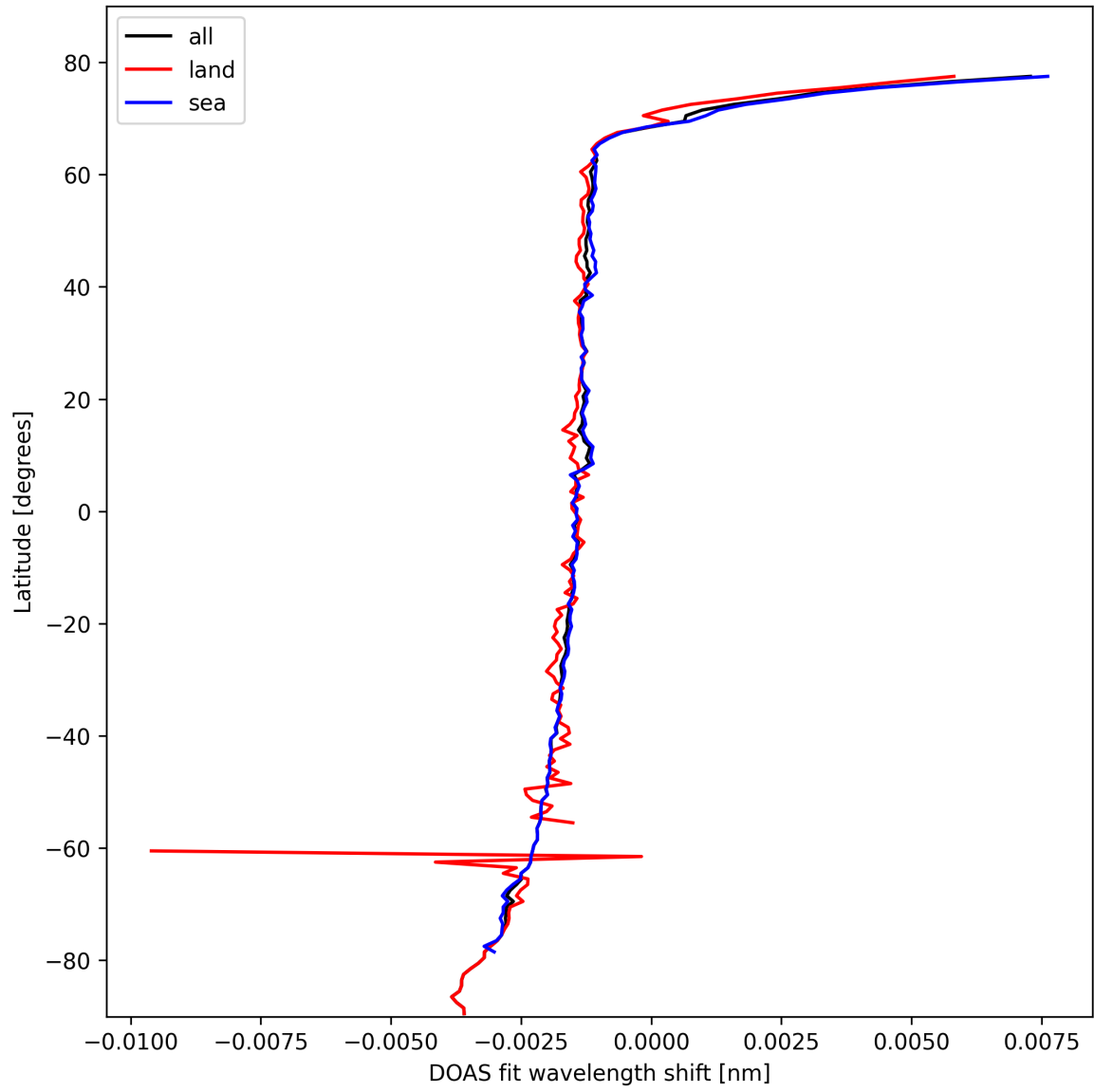
Figure 23: Zonal average of “DOAS fit wavelength shift” for 2025-10-22 to 2025-10-23.
