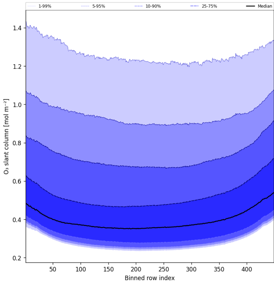
Figure 43: Along track statistics of “O 3 slant column” for 2025-10-22 to 2025-10-23
