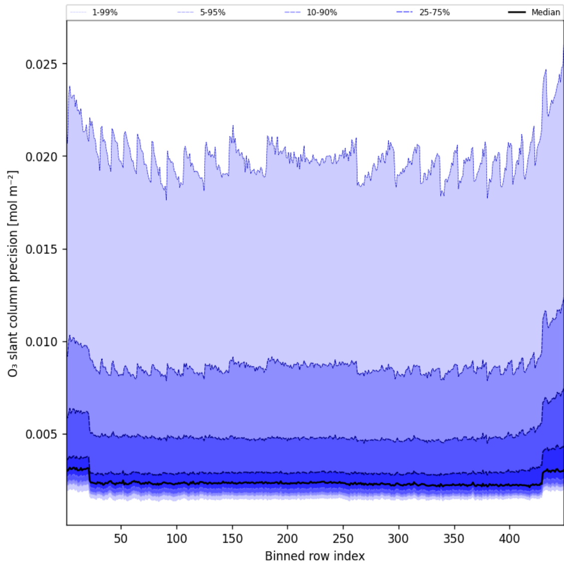
Figure 44: Along track statistics of “O 3 slant column precision” for 2025-10-22 to 2025-10-23
