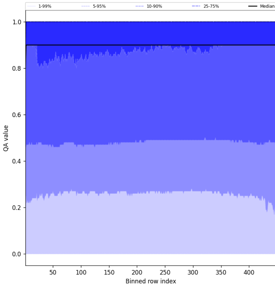
Figure 40: Along track statistics of “QA value” for 2025-10-22 to 2025-10-23
