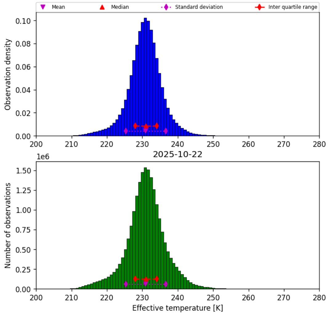
Figure 38: Histogram of “Effective temperature” for 2025-10-22 to 2025-10-23
