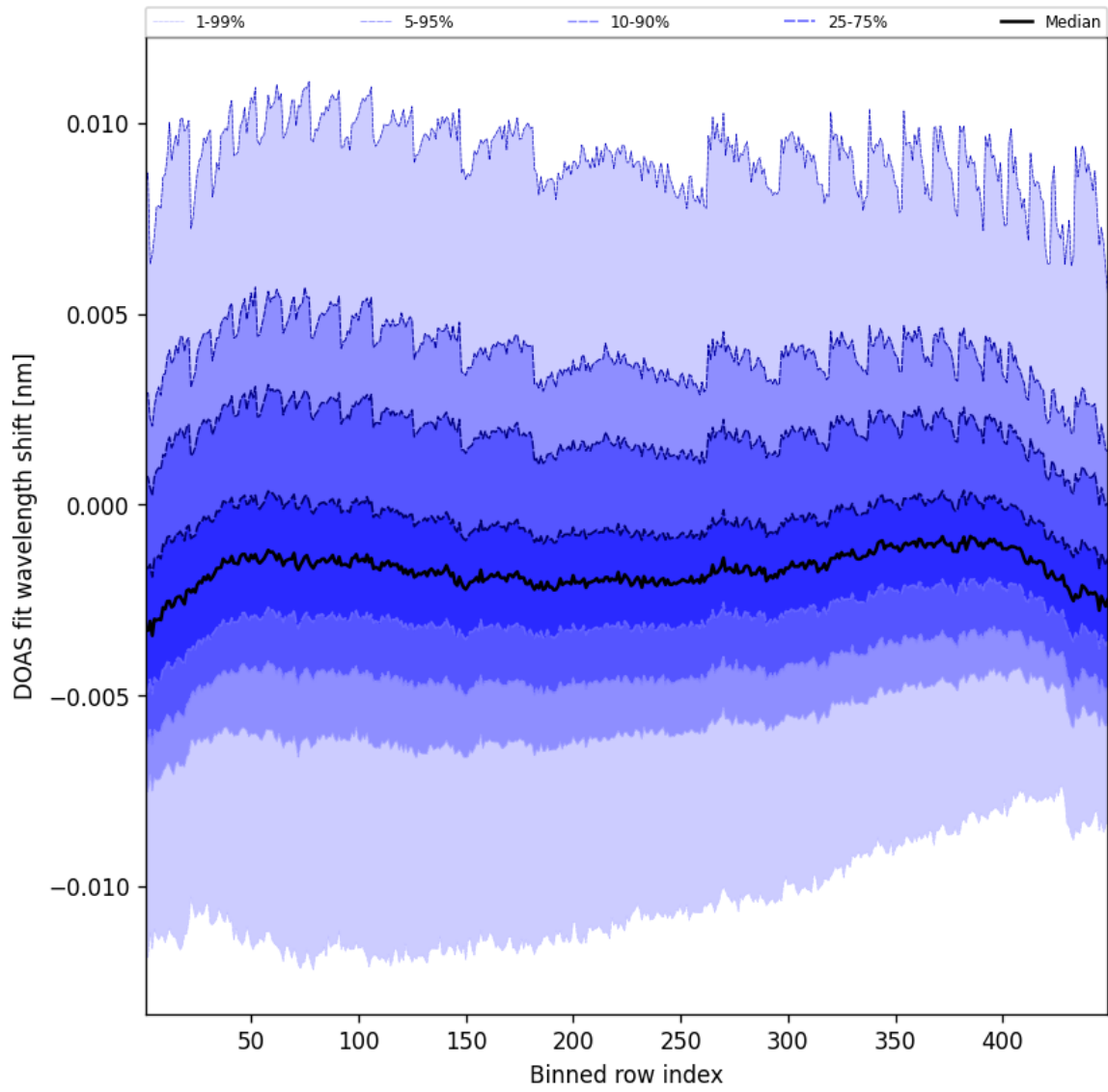
Figure 47: Along track statistics of “DOAS fit wavelength shift” for 2025-10-22 to 2025-10-23
