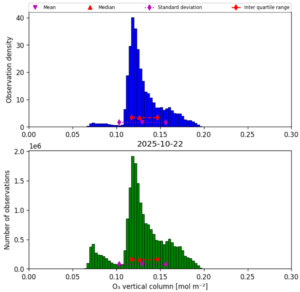
Figure 29: Histogram of “O 3 vertical column” for 2025-10-22 to 2025-10-23
