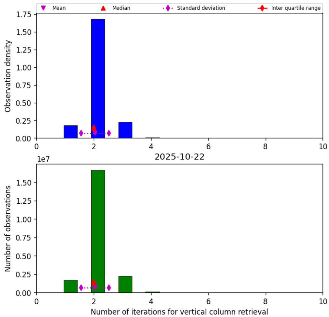
Figure 39: Histogram of “Number of iterations for vertical column retrieval” for 2025-10-22 to 2025-10-23
