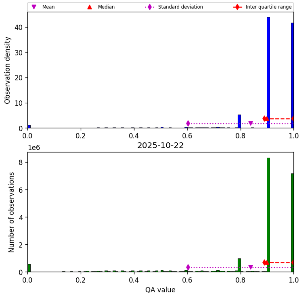
Figure 28: Histogram of “QA value” for 2025-10-22 to 2025-10-23
