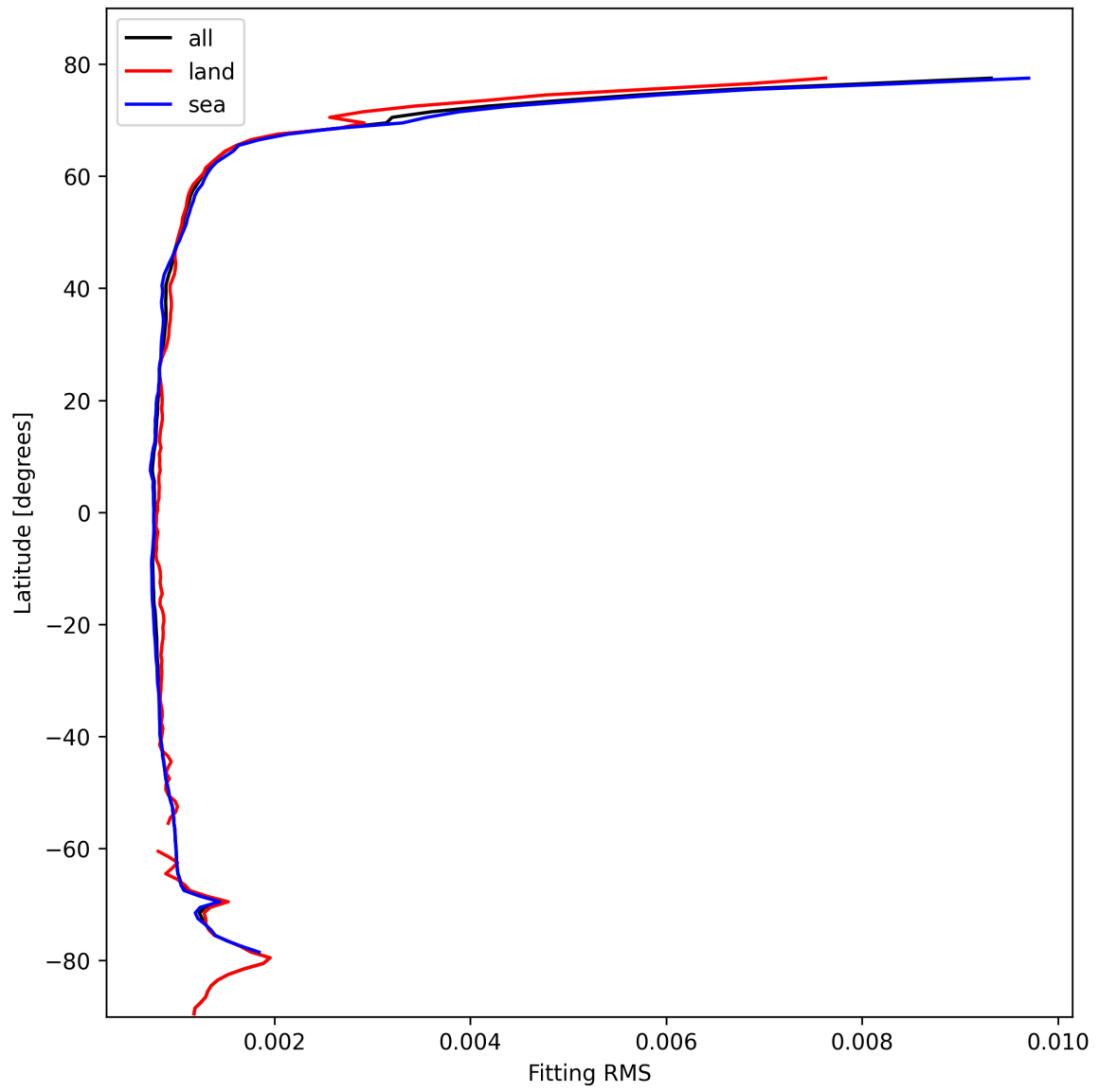
Figure 22: Zonal average of “Fitting RMS” for 2025-10-22 to 2025-10-23.
