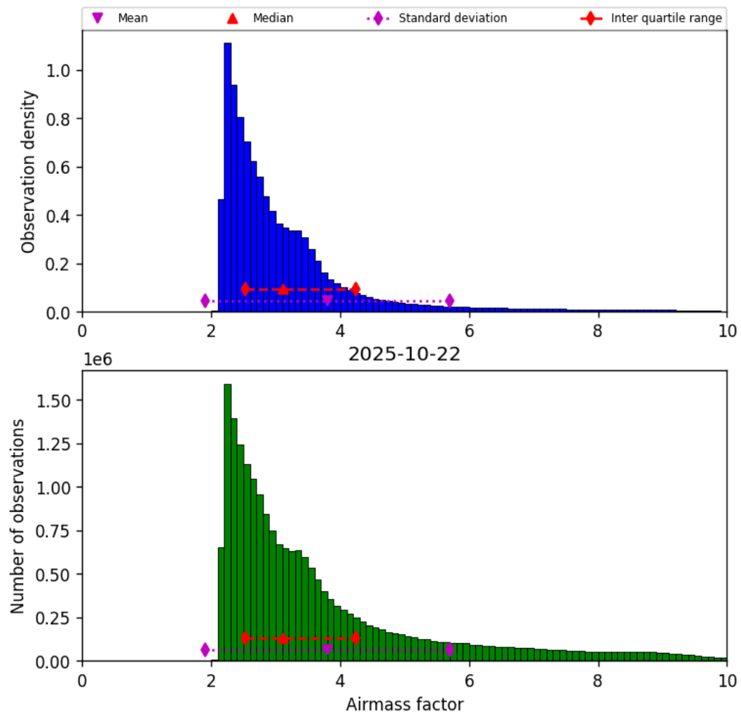
Figure 37: Histogram of “Airmass factor” for 2025-10-22 to 2025-10-23
