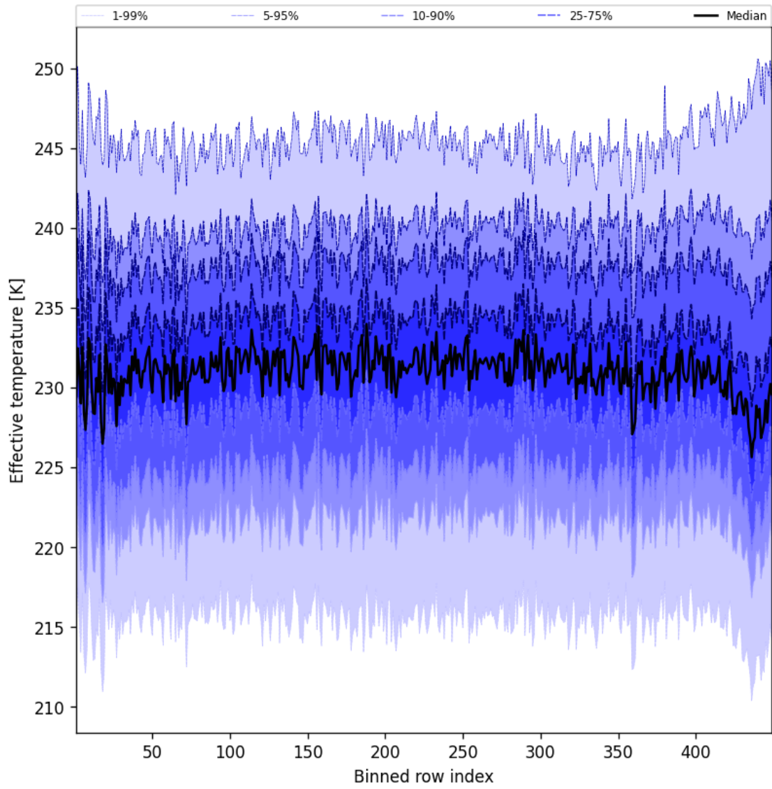
Figure 50: Along track statistics of “Effective temperature” for 2025-10-22 to 2025-10-23
