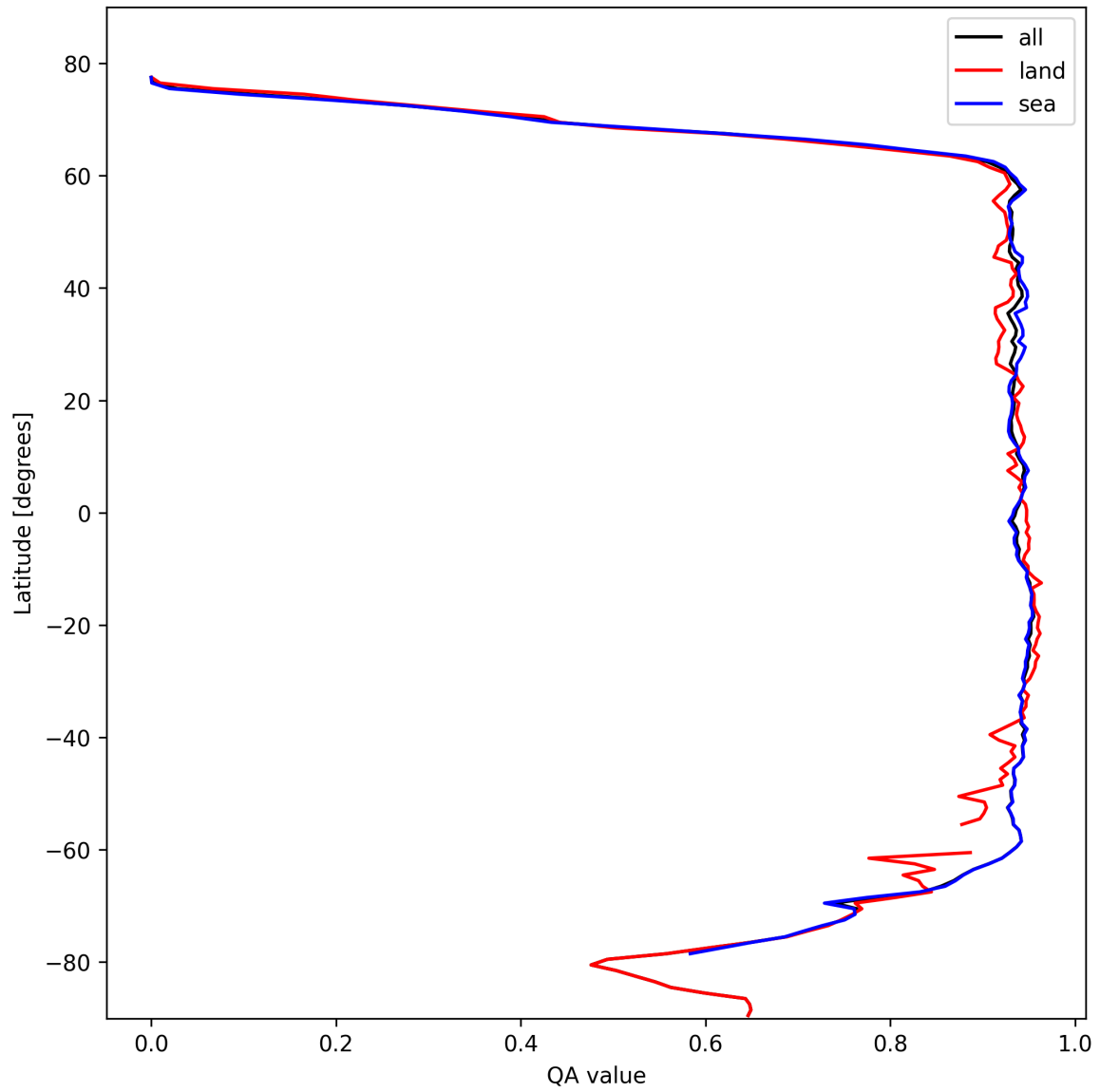
Figure 16: Zonal average of “QA value” for 2025-10-22 to 2025-10-23.
