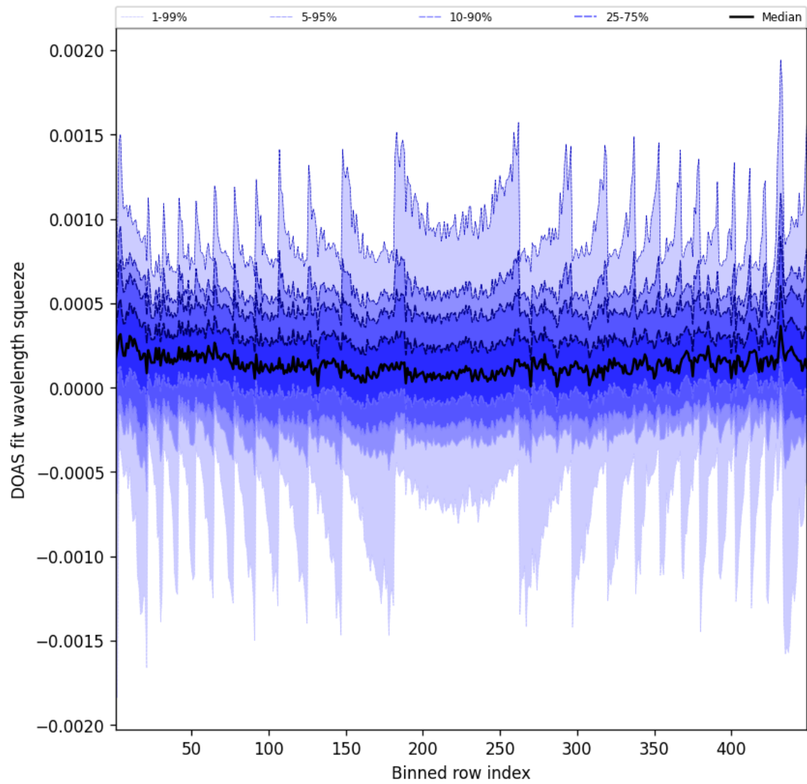
Figure 48: Along track statistics of “DOAS fit wavelength squeeze” for 2025-10-22 to 2025-10-23
