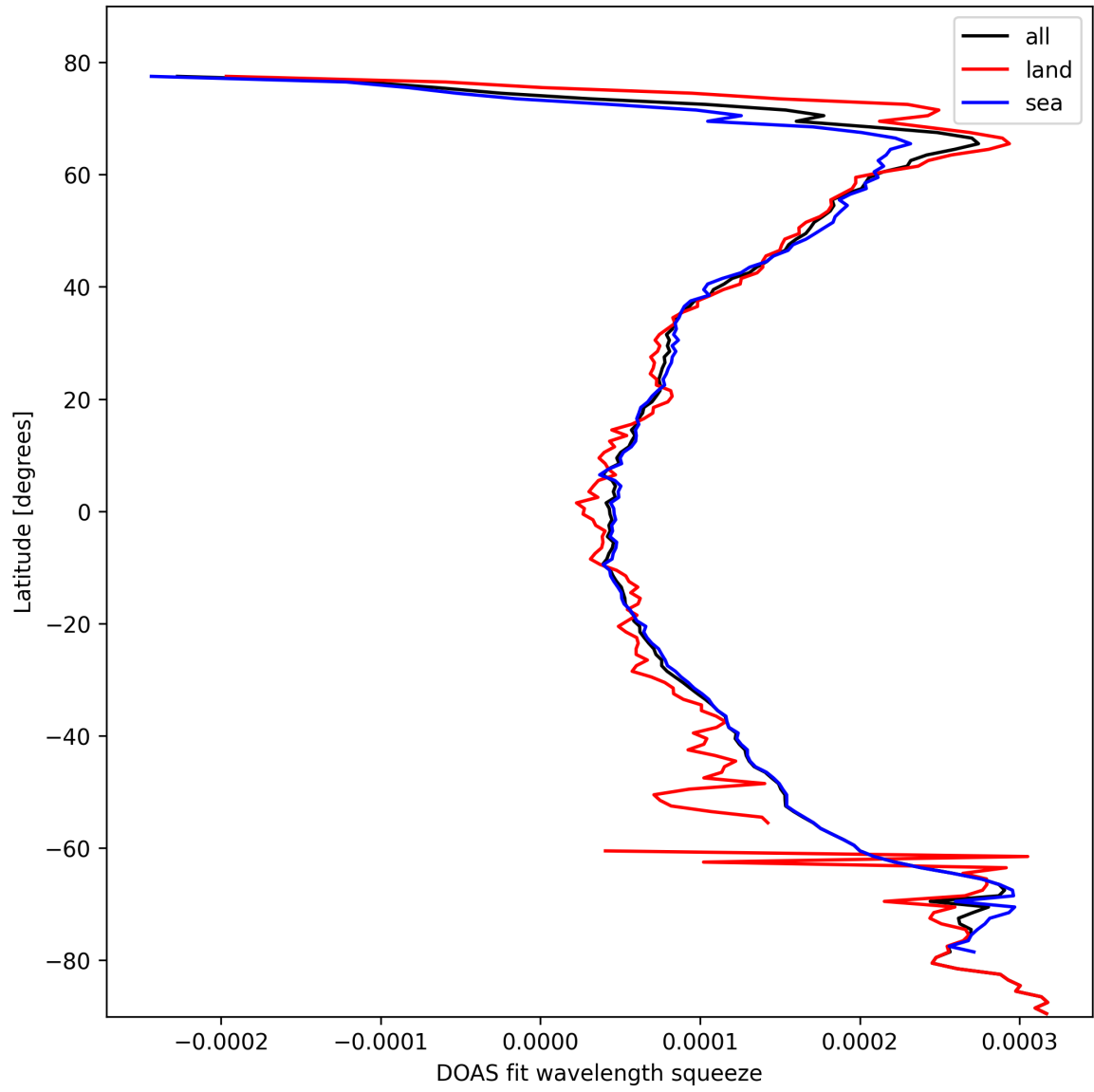
Figure 24: Zonal average of “DOAS fit wavelength squeeze” for 2025-10-22 to 2025-10-23.
