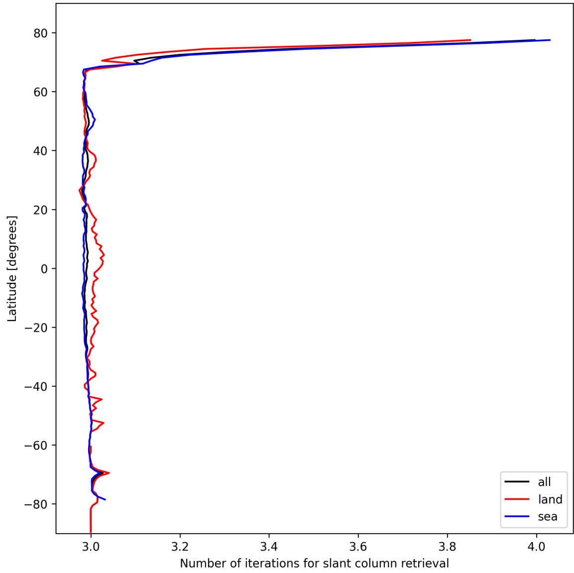
Figure 21: Zonal average of “Number of iterations for slant column retrieval” for 2025-10-22 to 2025-10-23.
