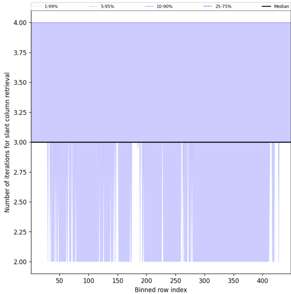
Figure 45: Along track statistics of “Number of iterations for slant column retrieval” for 2025-10-22 to 2025-10-23
