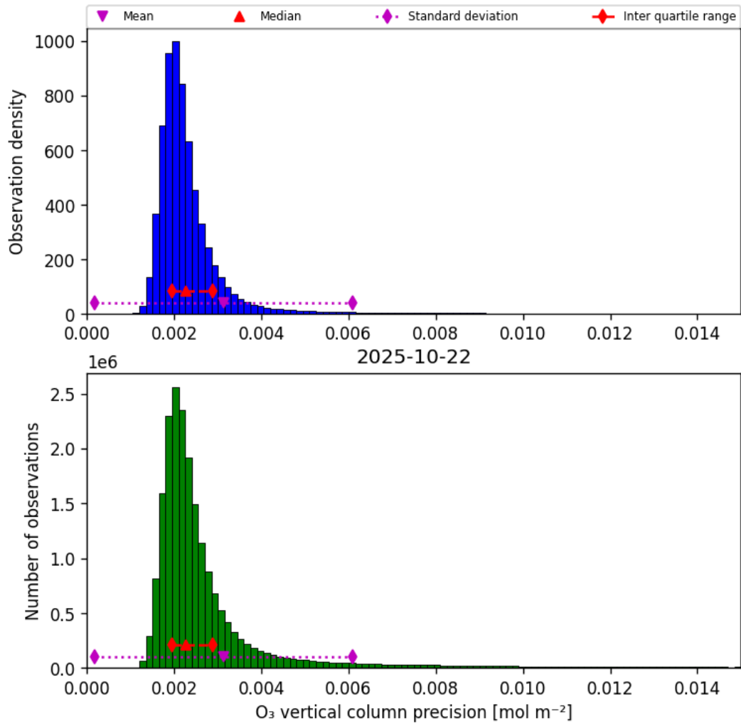
Figure 30: Histogram of “O 3 vertical column precision” for 2025-10-22 to 2025-10-23
