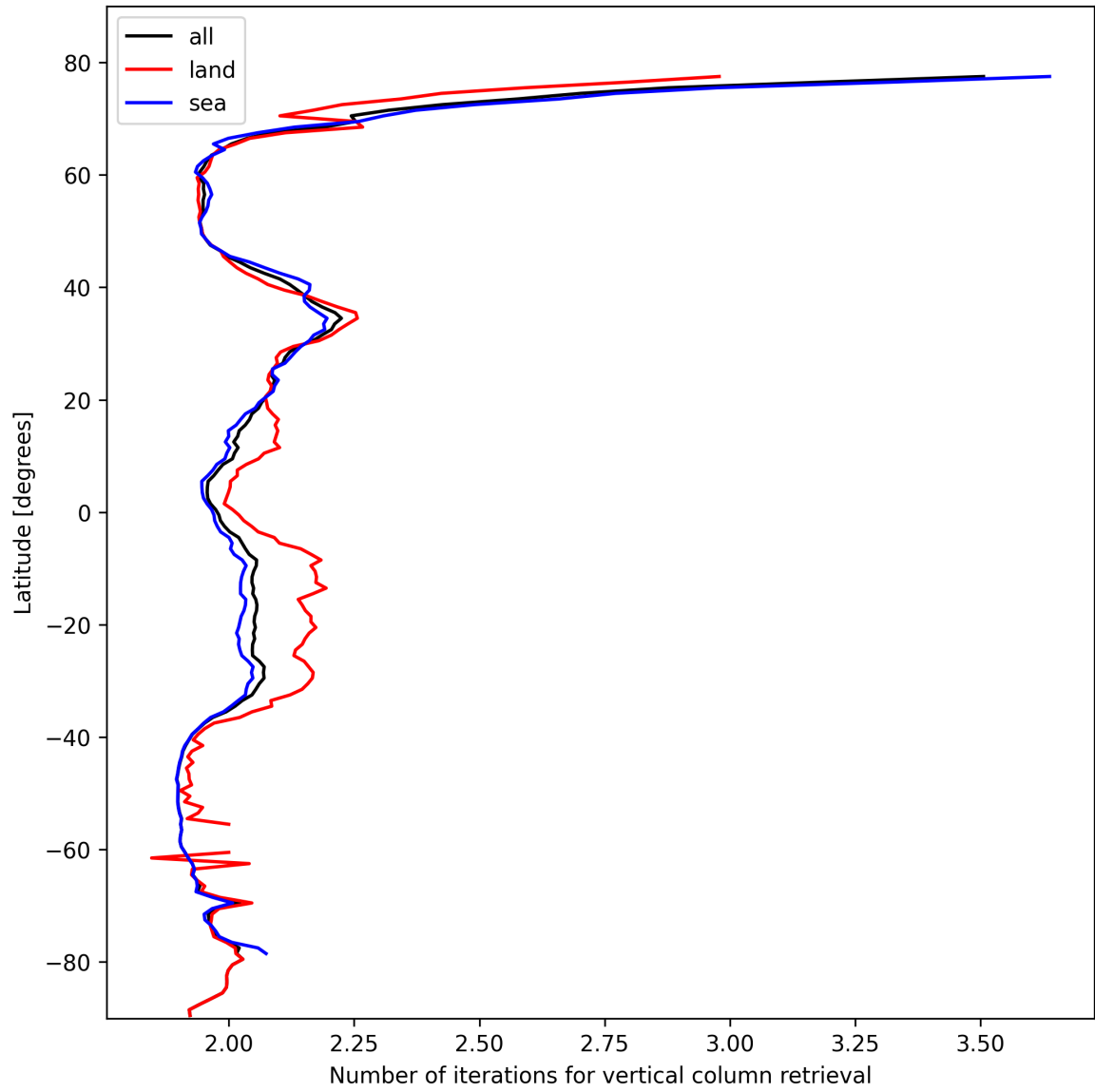
Figure 27: Zonal average of “Number of iterations for vertical column retrieval” for 2025-10-22 to 2025-10-23.
