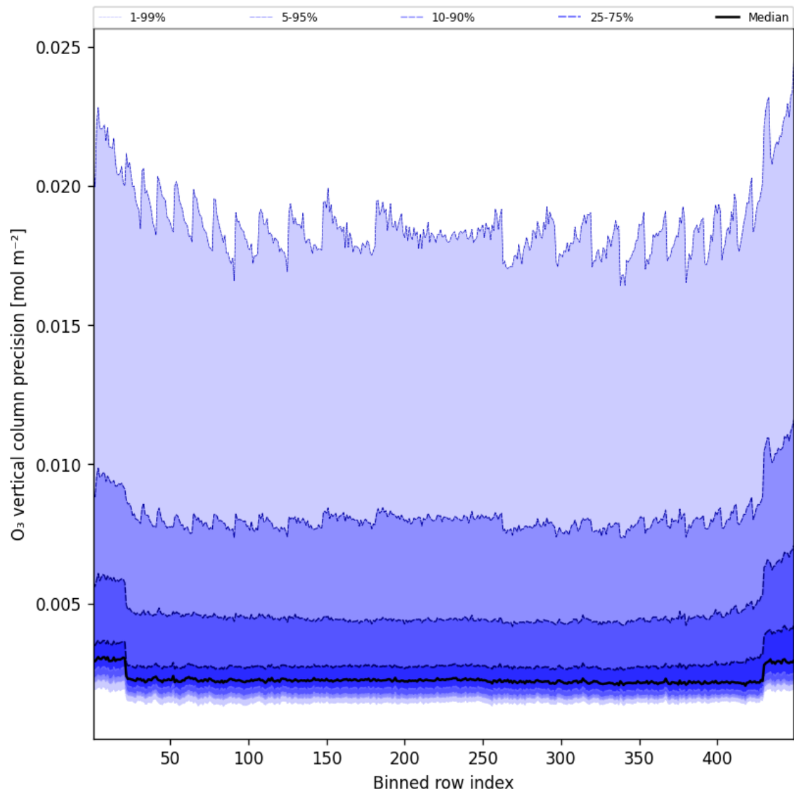
Figure 42: Along track statistics of “O 3 vertical column precision” for 2025-10-22 to 2025-10-23
