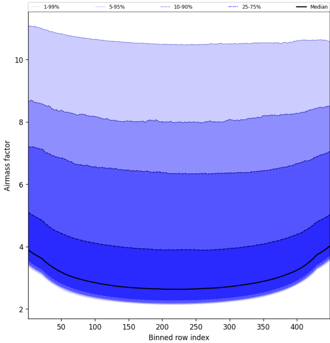
Figure 49: Along track statistics of “Airmass factor” for 2025-10-22 to 2025-10-23
