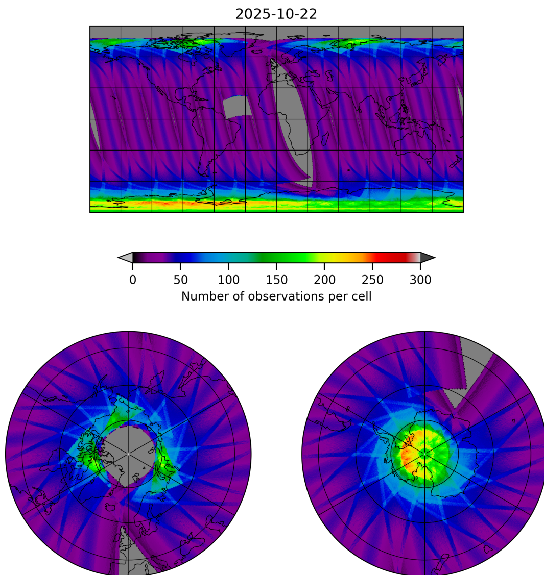
Figure 15: Map of the number of observations for 2025-10-22 to 2025-10-23
