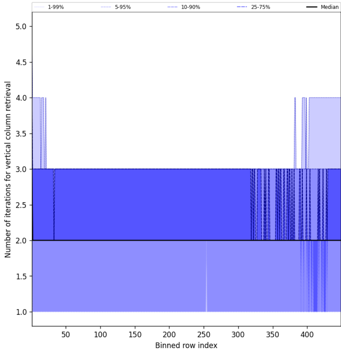
Figure 51: Along track statistics of “Number of iterations for vertical column retrieval” for 2025-10-24 to 2025-10-25
