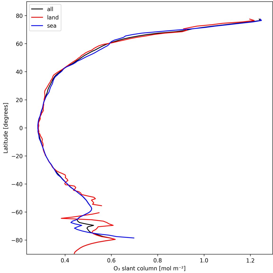
Figure 19: Zonal average of “O 3 slant column” for 2025-10-24 to 2025-10-25.
