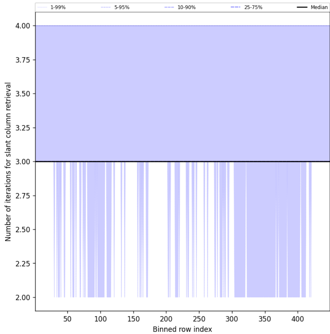
Figure 45: Along track statistics of “Number of iterations for slant column retrieval” for 2025-10-24 to 2025-10-25
