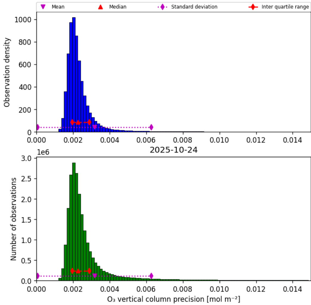
Figure 30: Histogram of “O 3 vertical column precision” for 2025-10-24 to 2025-10-25
