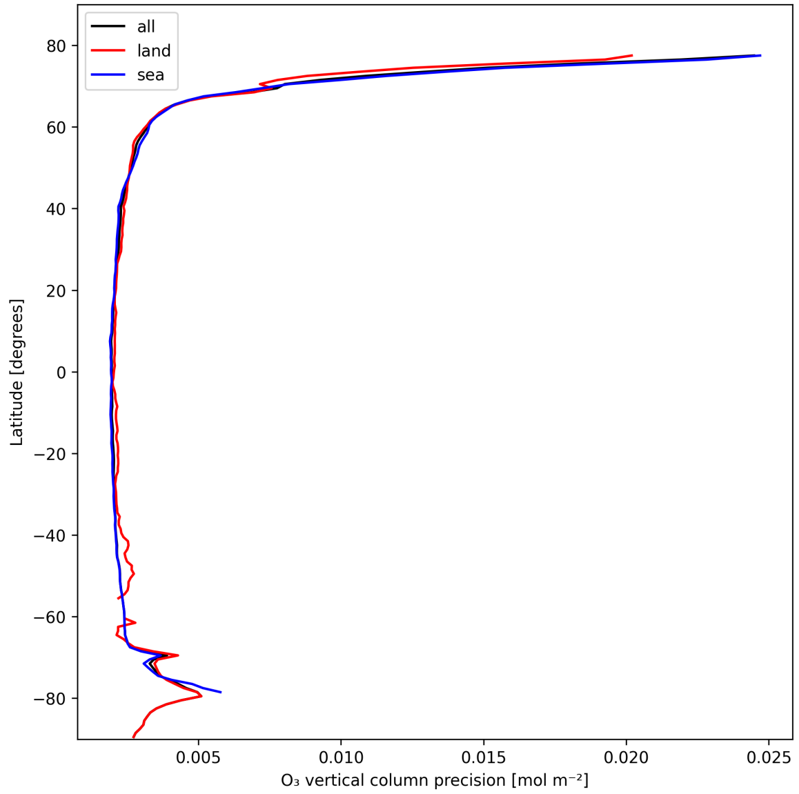
Figure 18: Zonal average of “O 3 vertical column precision” for 2025-10-24 to 2025-10-25.
