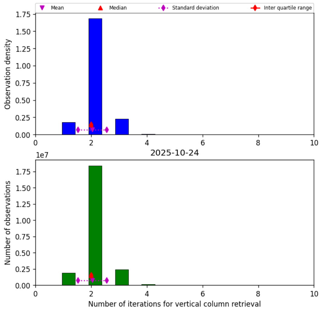
Figure 39: Histogram of “Number of iterations for vertical column retrieval” for 2025-10-24 to 2025-10-25
