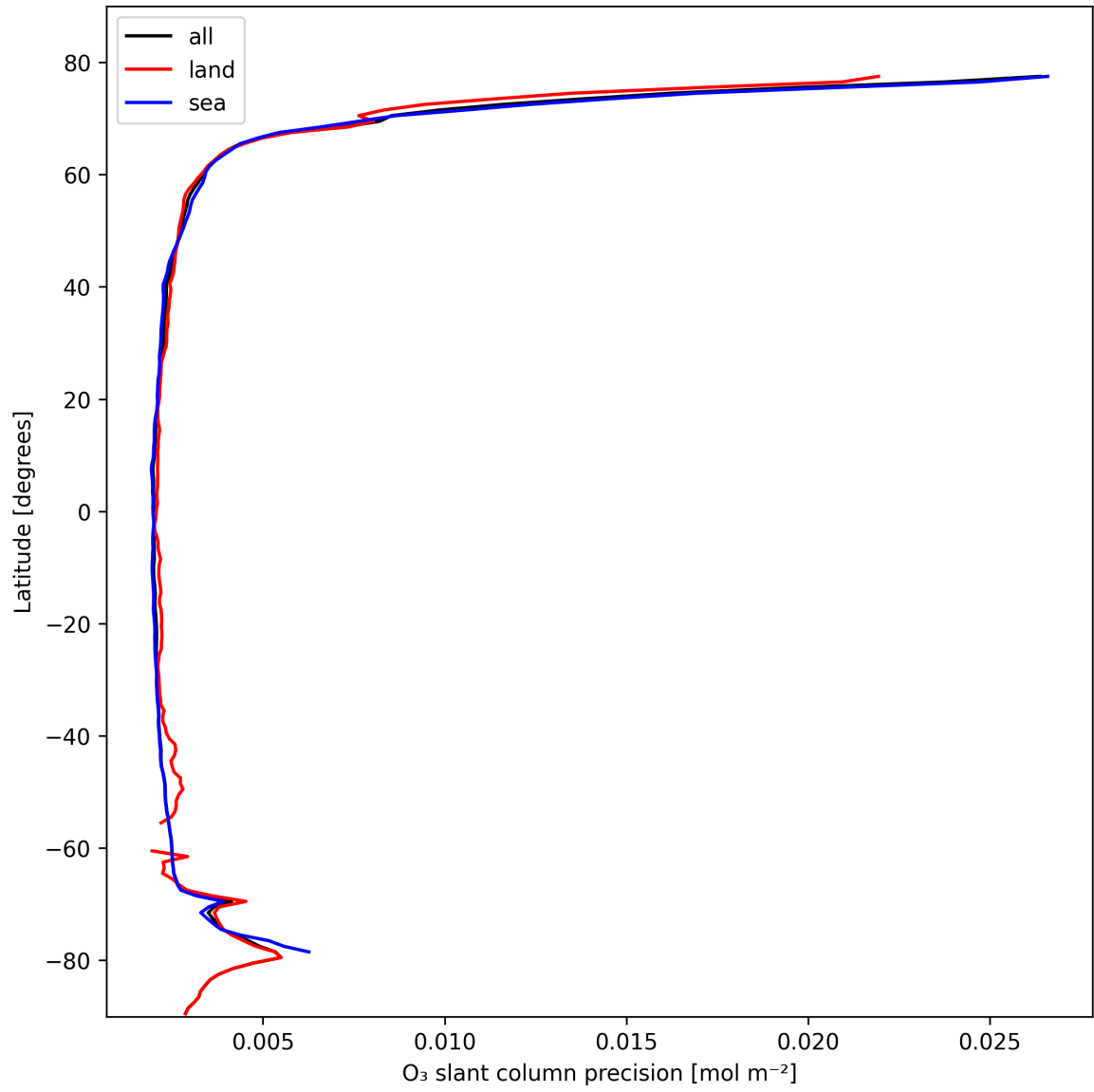
Figure 20: Zonal average of “O 3 slant column precision” for 2025-10-24 to 2025-10-25.
