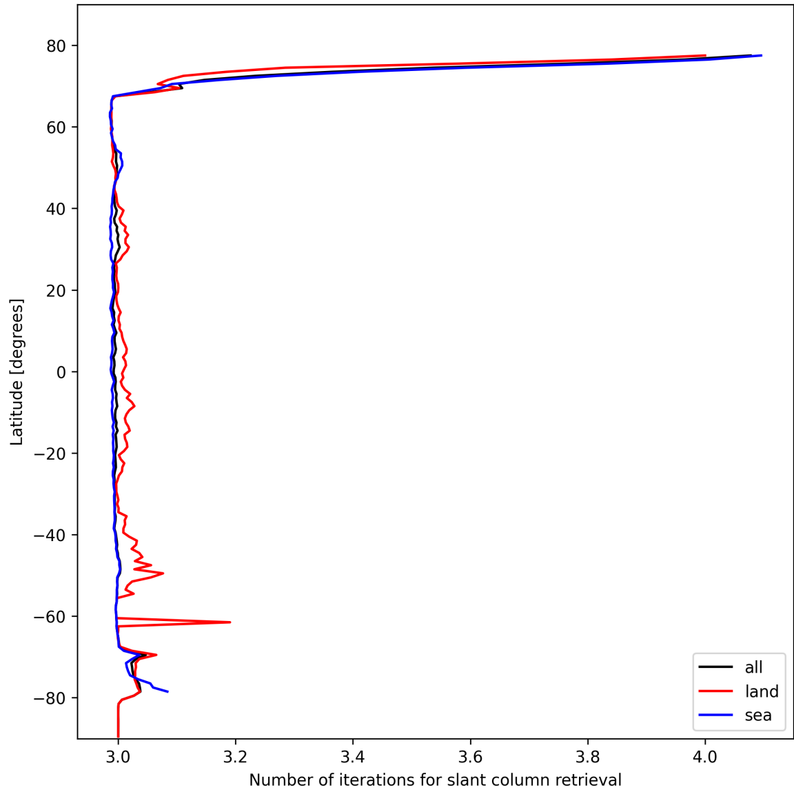
Figure 21: Zonal average of “Number of iterations for slant column retrieval” for 2025-10-24 to 2025-10-25.
