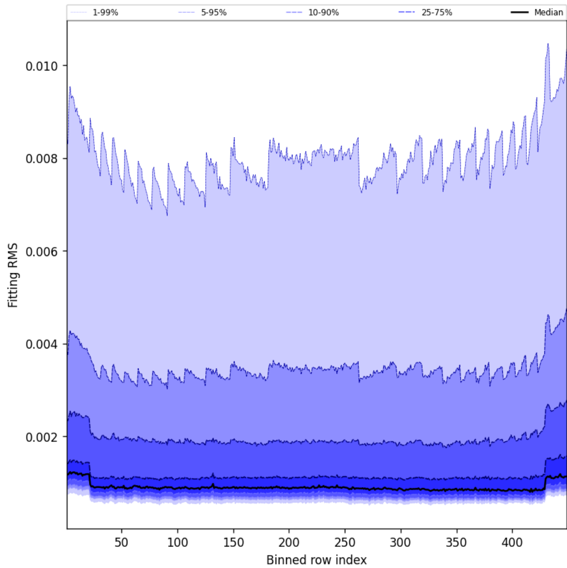
Figure 46: Along track statistics of “Fitting RMS” for 2025-10-24 to 2025-10-25
