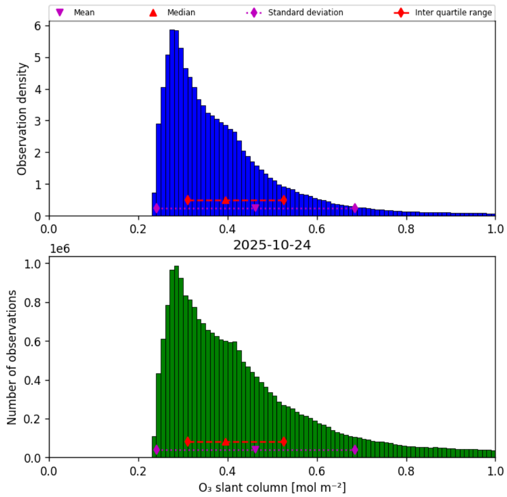
Figure 31: Histogram of “O 3 slant column” for 2025-10-24 to 2025-10-25
