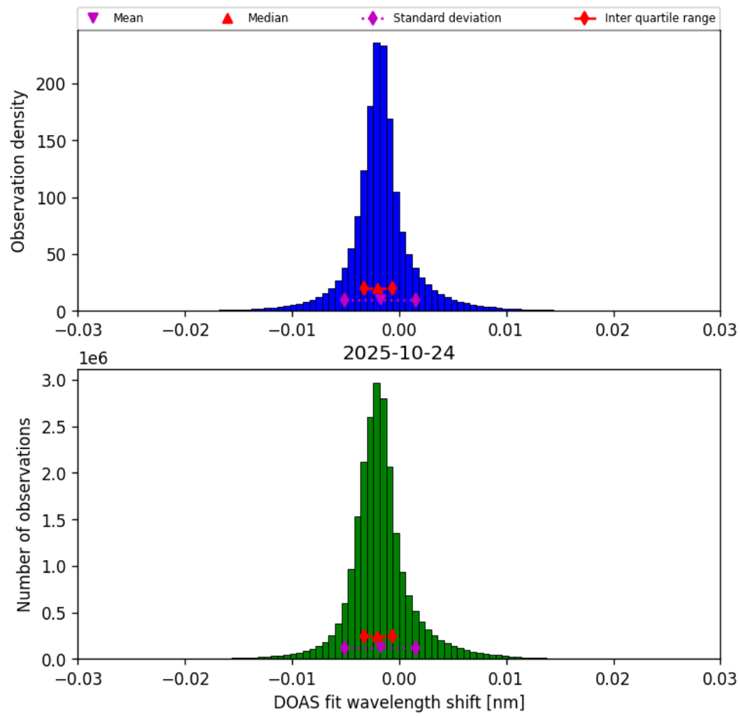
Figure 35: Histogram of “DOAS fit wavelength shift” for 2025-10-24 to 2025-10-25
