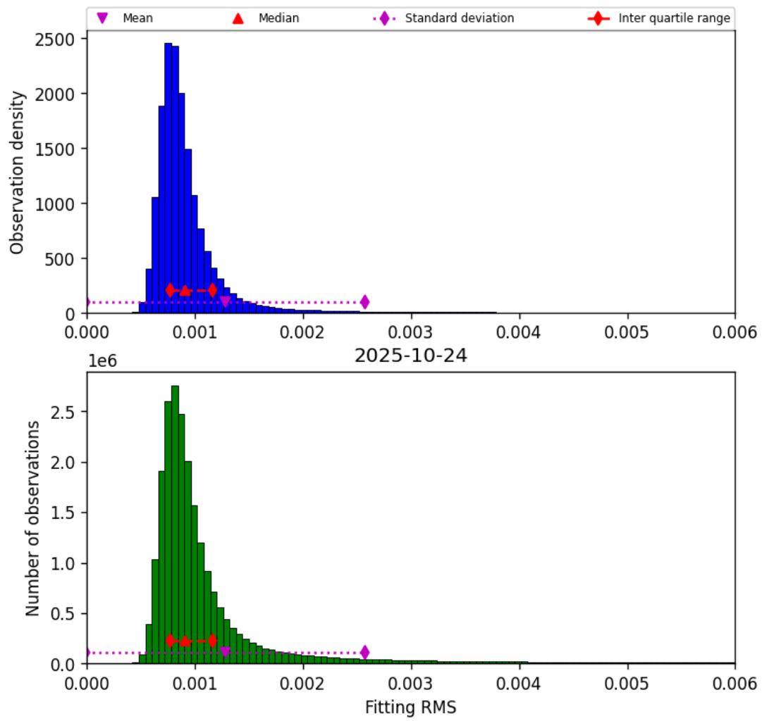
Figure 34: Histogram of “Fitting RMS” for 2025-10-24 to 2025-10-25
