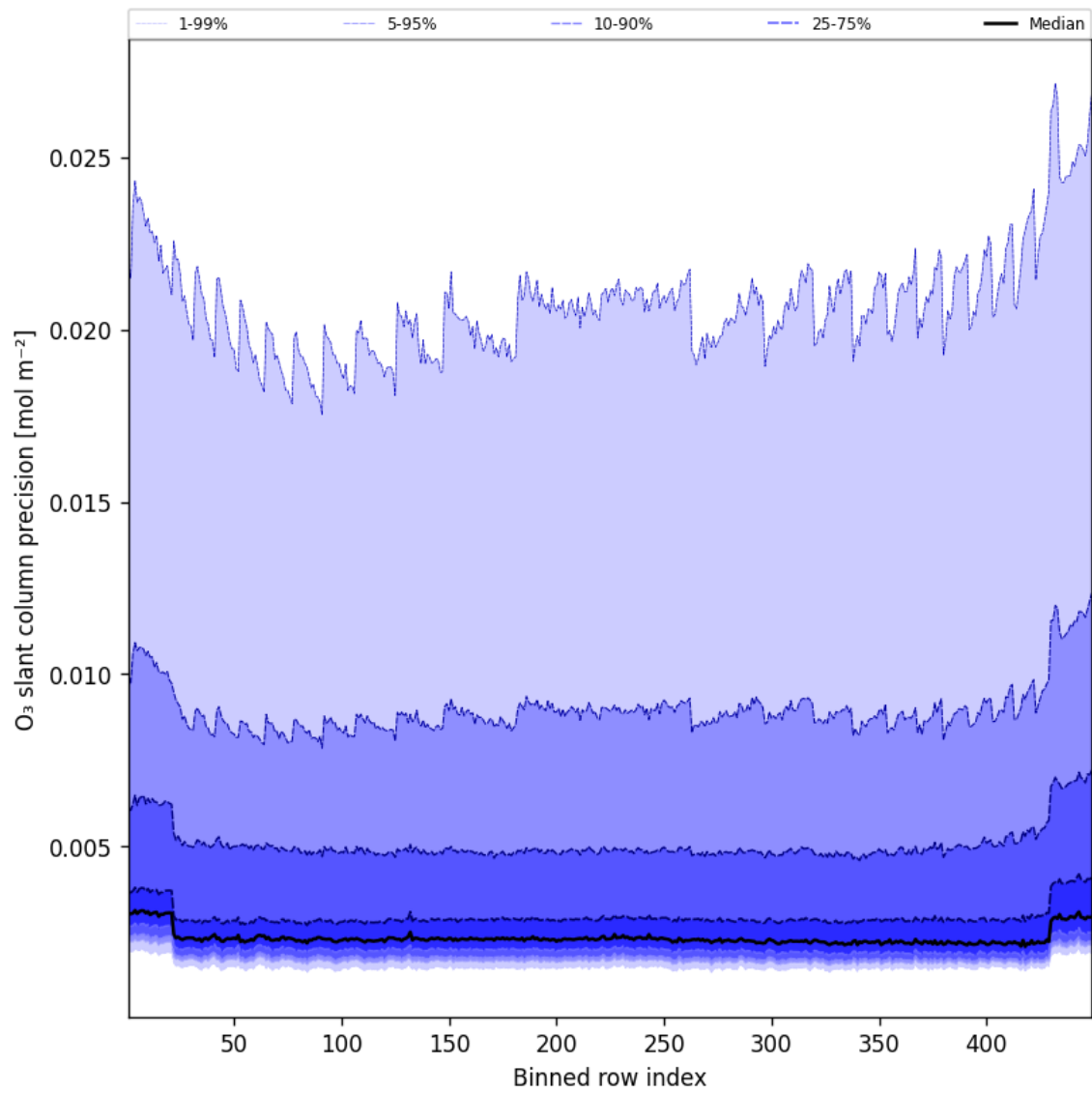
Figure 44: Along track statistics of “O 3 slant column precision” for 2025-10-24 to 2025-10-25
