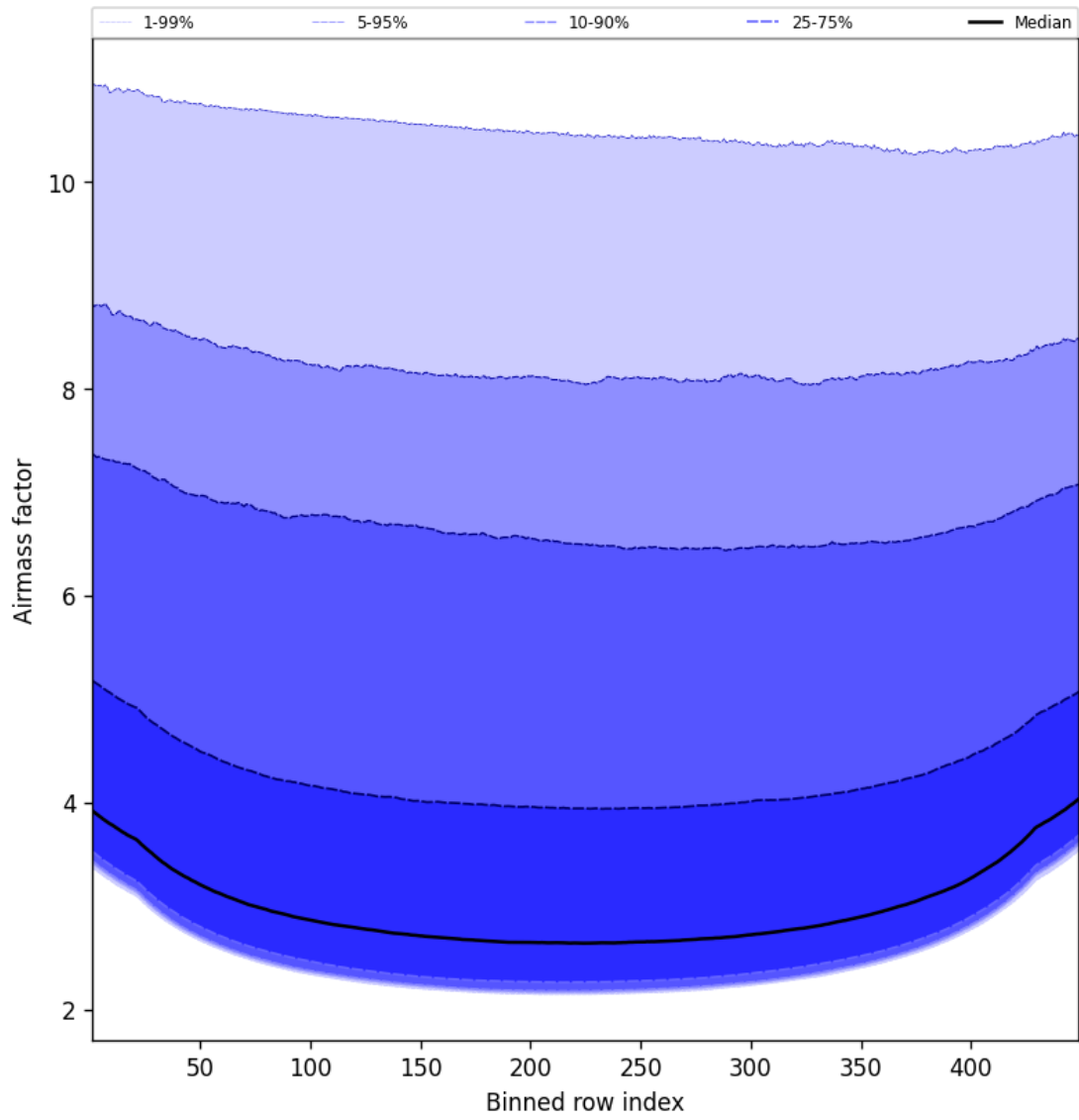
Figure 49: Along track statistics of “Airmass factor” for 2025-10-24 to 2025-10-25
