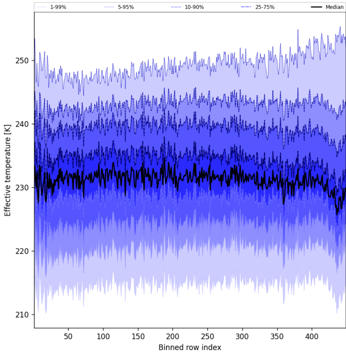
Figure 50: Along track statistics of “Effective temperature” for 2025-10-24 to 2025-10-25
