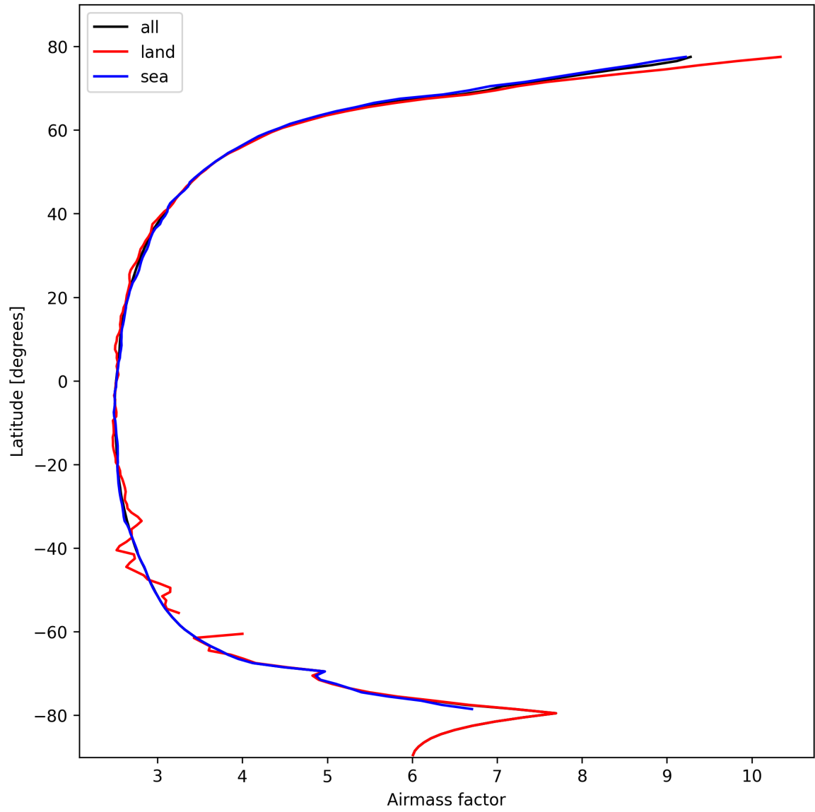
Figure 25: Zonal average of “Airmass factor” for 2025-10-24 to 2025-10-25.
