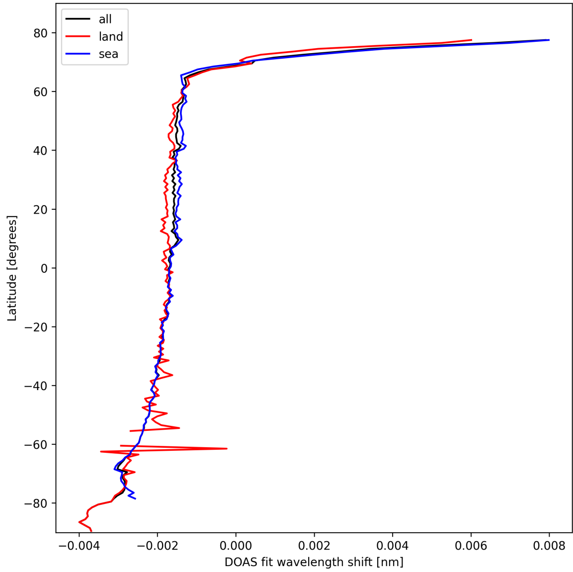
Figure 23: Zonal average of “DOAS fit wavelength shift” for 2025-10-24 to 2025-10-25.
