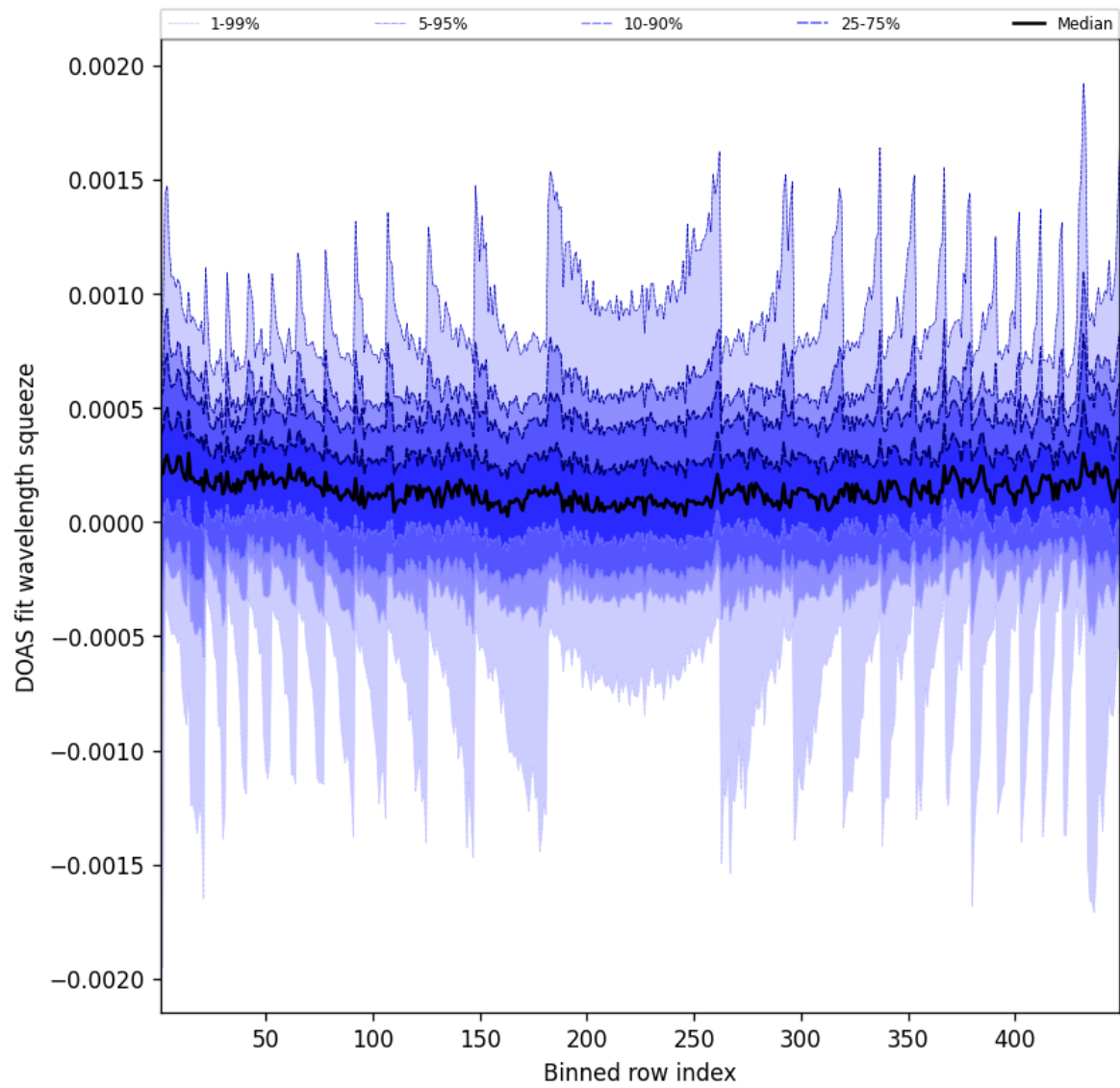
Figure 48: Along track statistics of “DOAS fit wavelength squeeze” for 2025-10-24 to 2025-10-25
