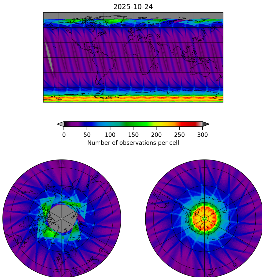
Figure 15: Map of the number of observations for 2025-10-24 to 2025-10-25
