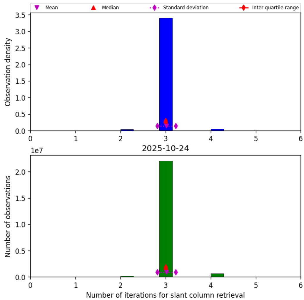
Figure 33: Histogram of “Number of iterations for slant column retrieval” for 2025-10-24 to 2025-10-25
