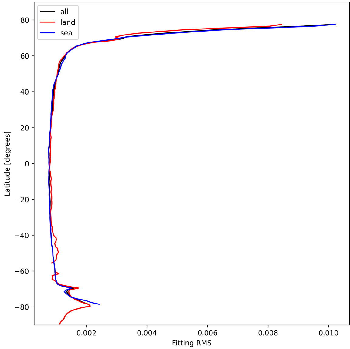
Figure 22: Zonal average of “Fitting RMS” for 2025-10-24 to 2025-10-25.
