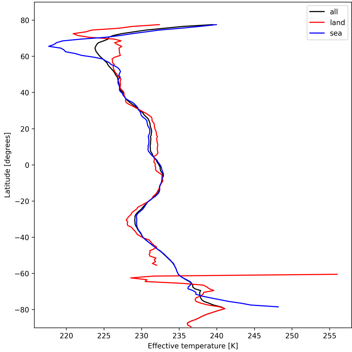
Figure 26: Zonal average of "Effective temperature" for 2025-10-24 to 2025-10-25.
