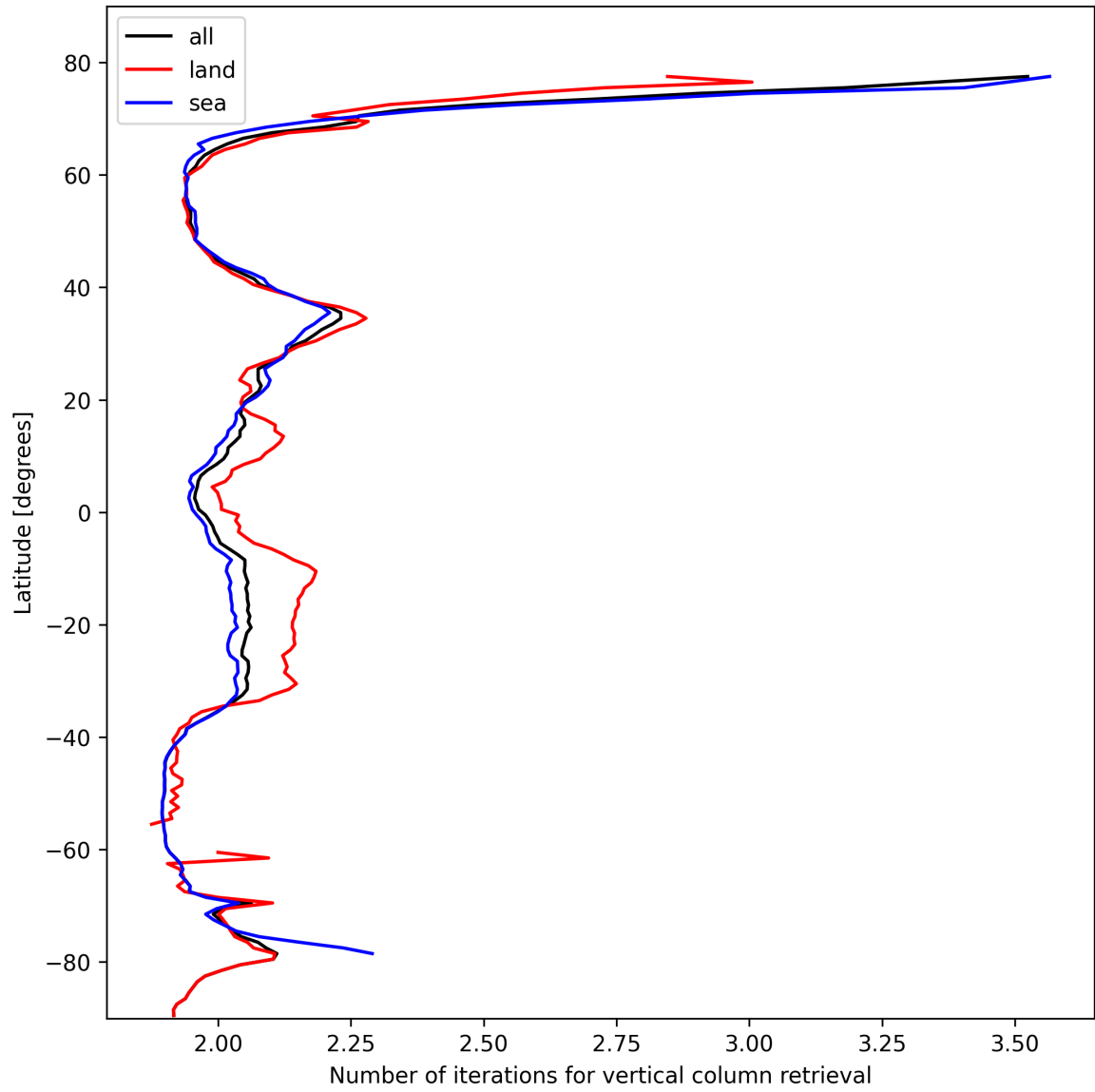
Figure 27: Zonal average of “Number of iterations for vertical column retrieval” for 2025-10-24 to 2025-10-25.
