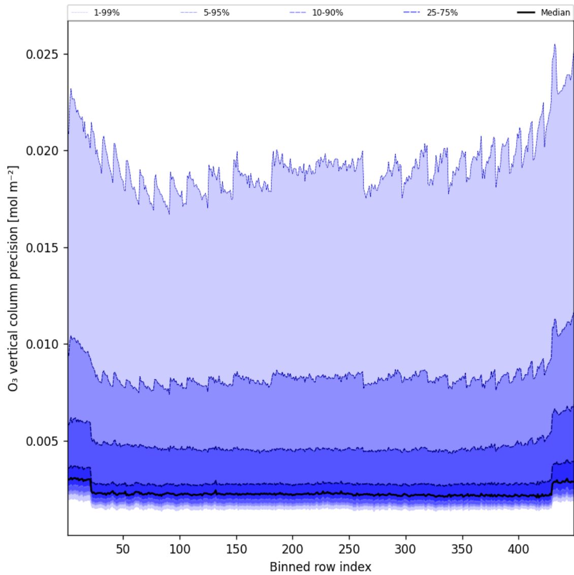
Figure 42: Along track statistics of “O 3 vertical column precision” for 2025-10-24 to 2025-10-25
