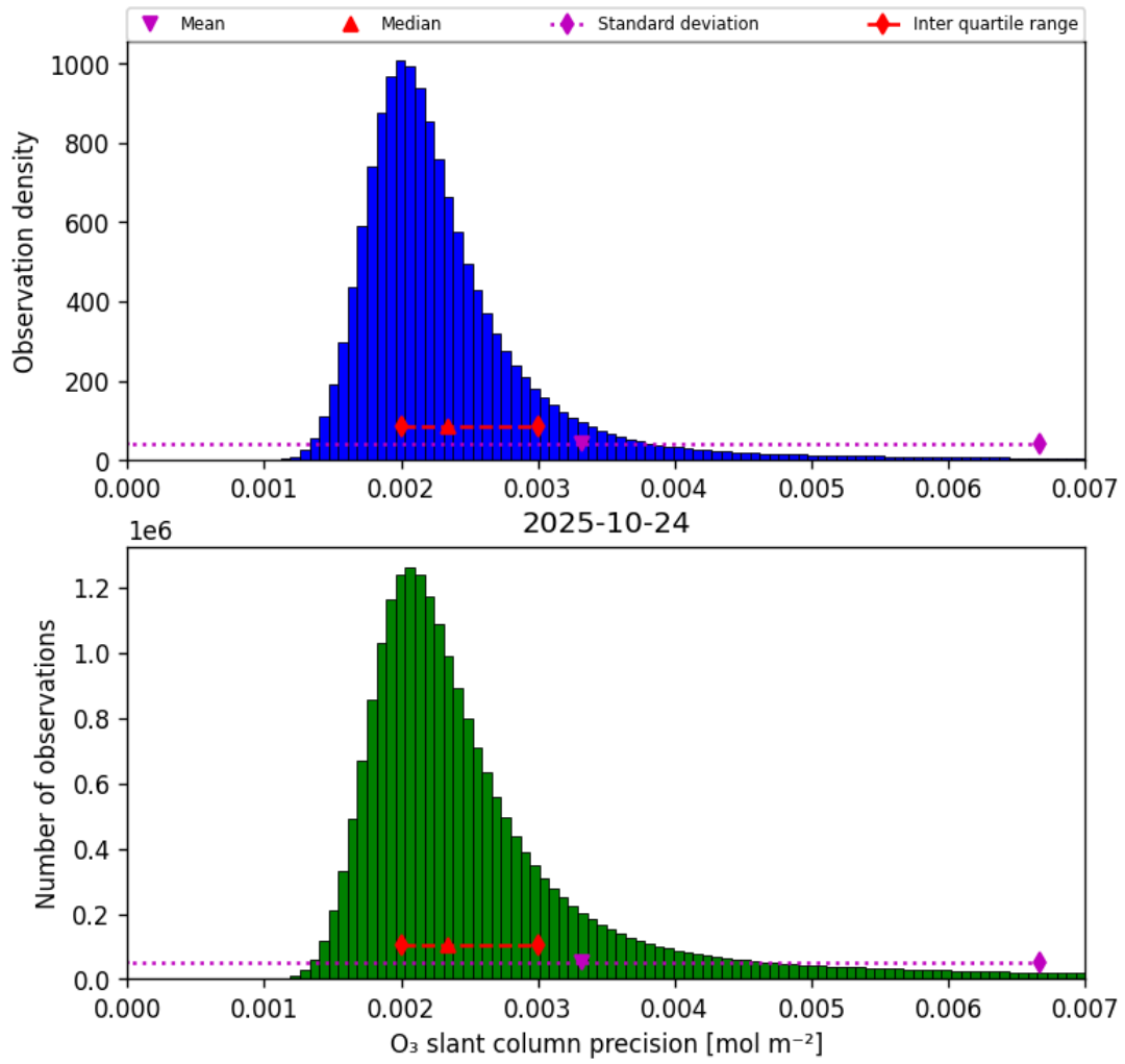
Figure 32: Histogram of “O 3 slant column precision” for 2025-10-24 to 2025-10-25
