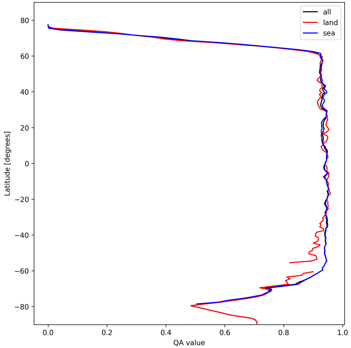
Figure 16: Zonal average of “QA value” for 2025-10-24 to 2025-10-25.
