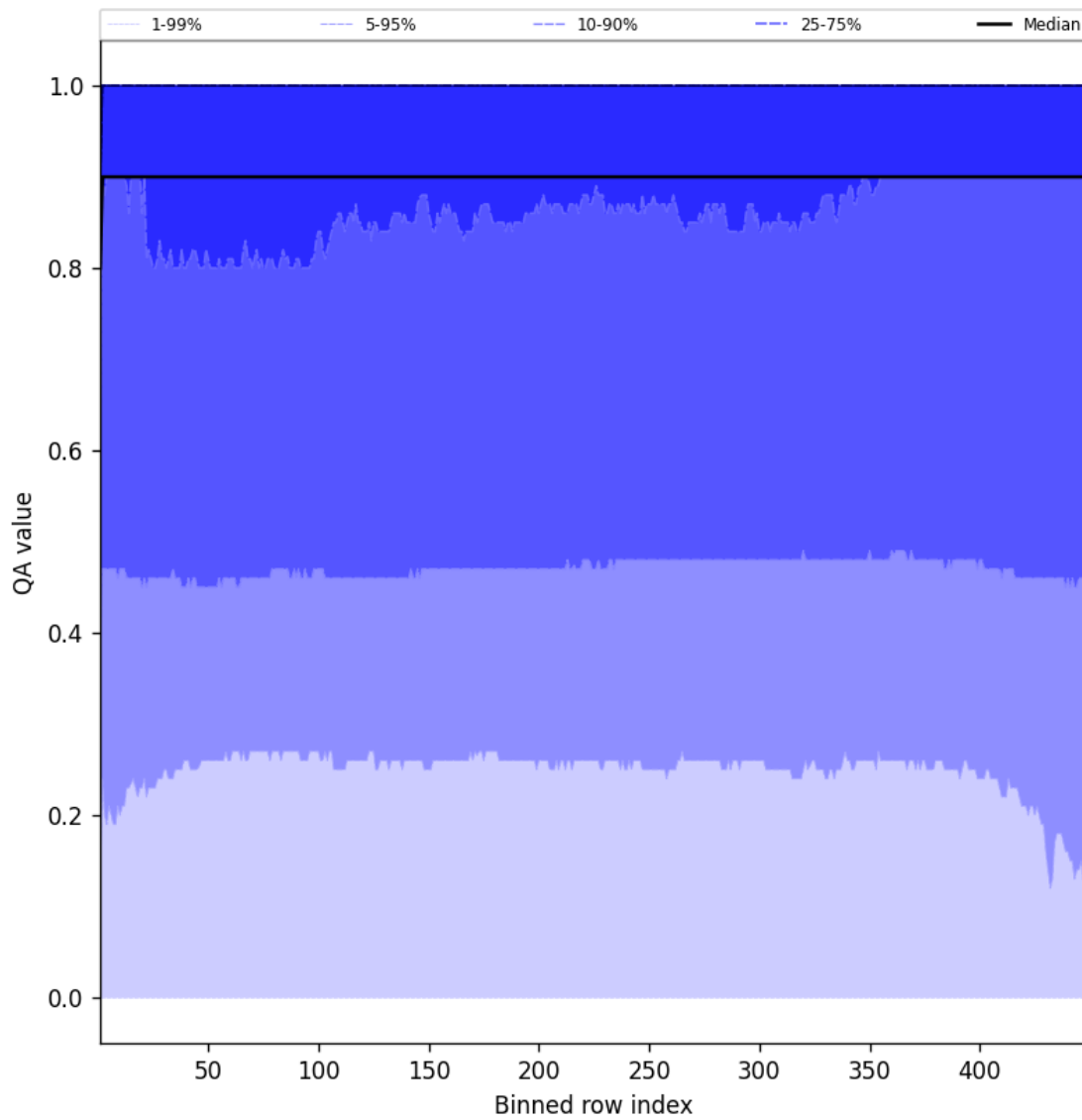
Figure 40: Along track statistics of “QA value” for 2025-10-24 to 2025-10-25
