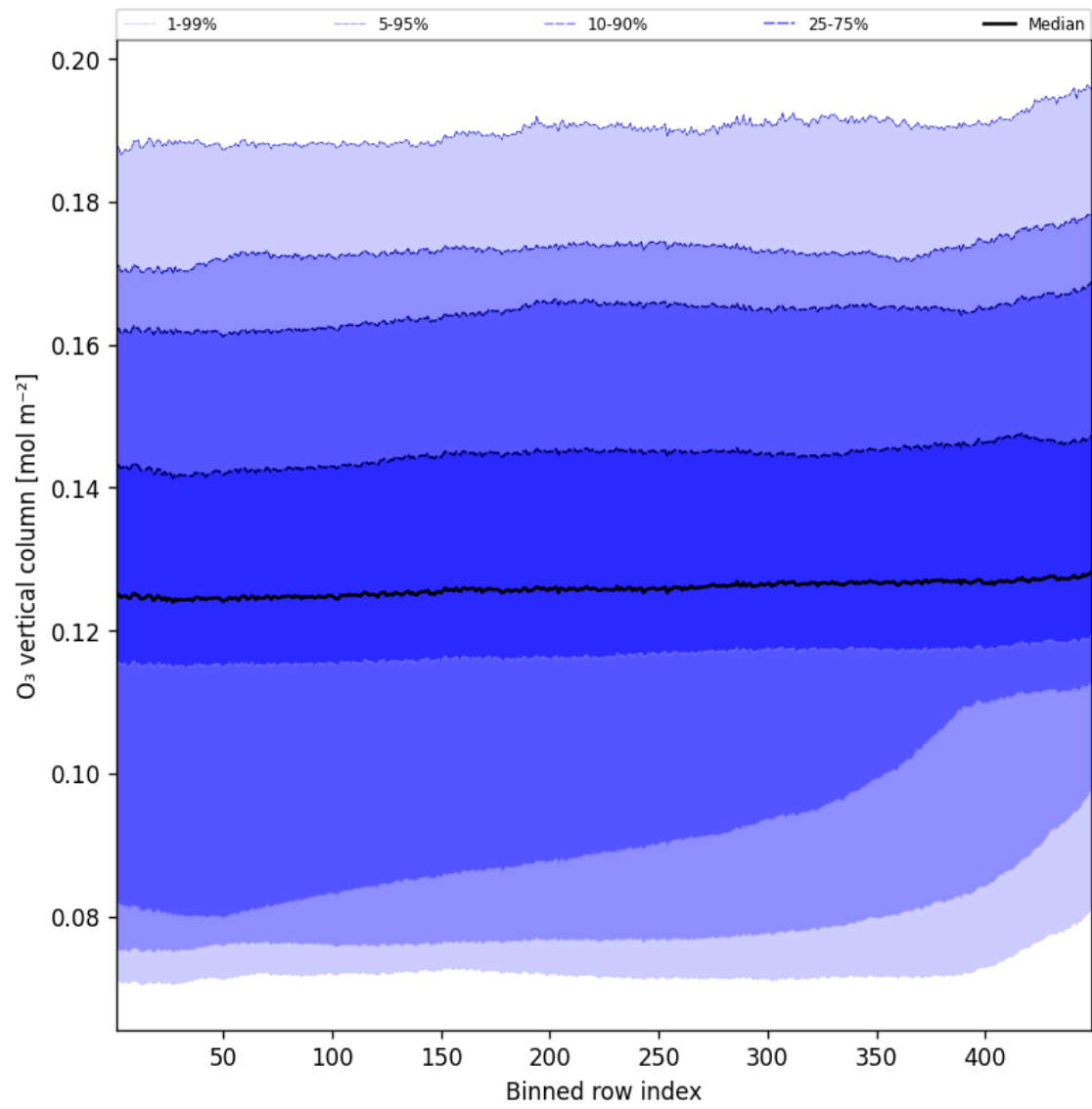
Figure 41: Along track statistics of “O 3 vertical column” for 2025-10-24 to 2025-10-25
