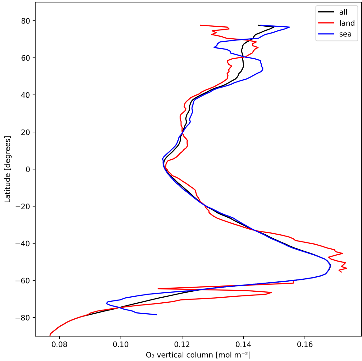
Figure 17: Zonal average of “O 3 vertical column” for 2025-10-24 to 2025-10-25.
