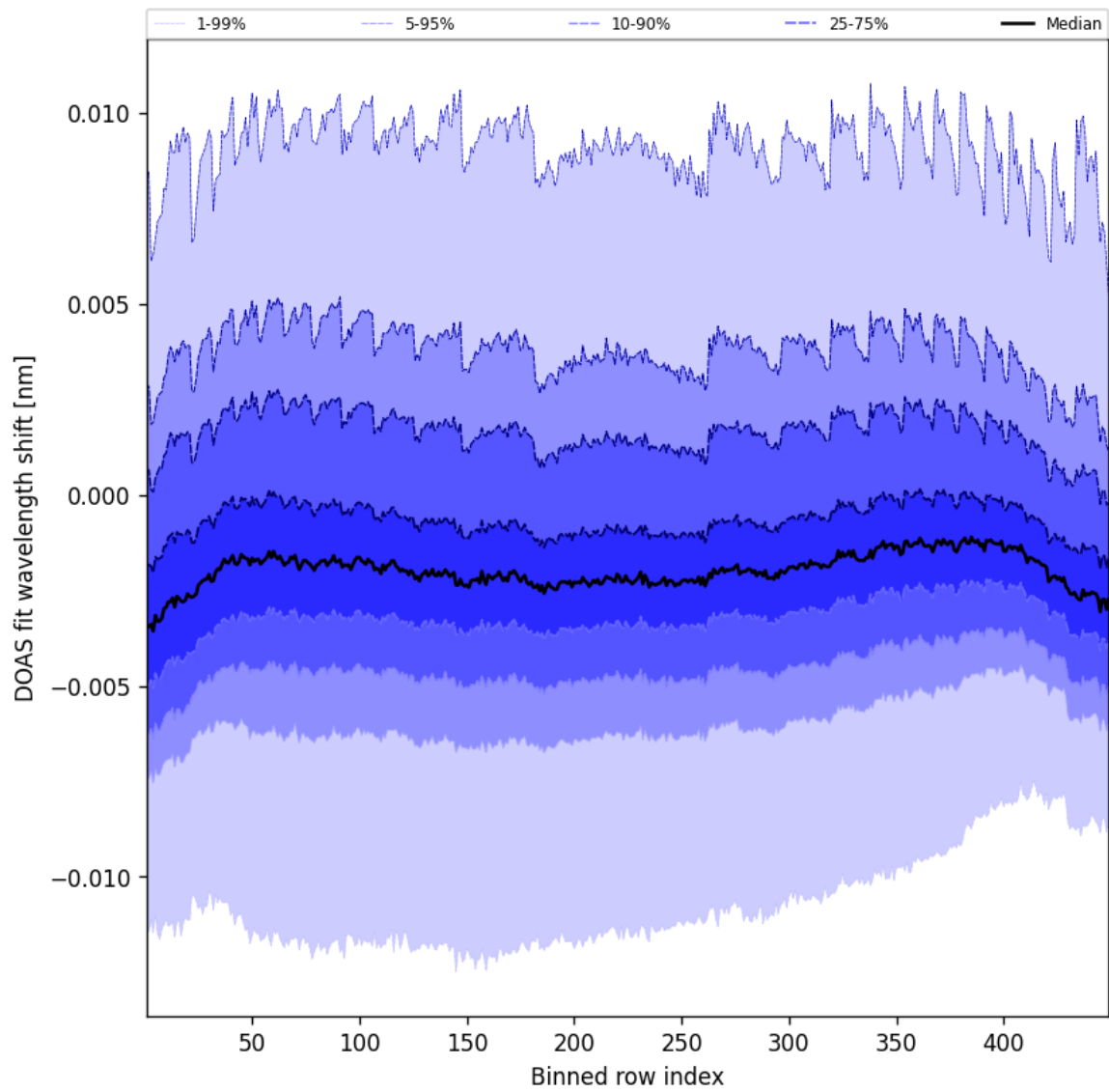
Figure 47: Along track statistics of “DOAS fit wavelength shift” for 2025-10-24 to 2025-10-25
