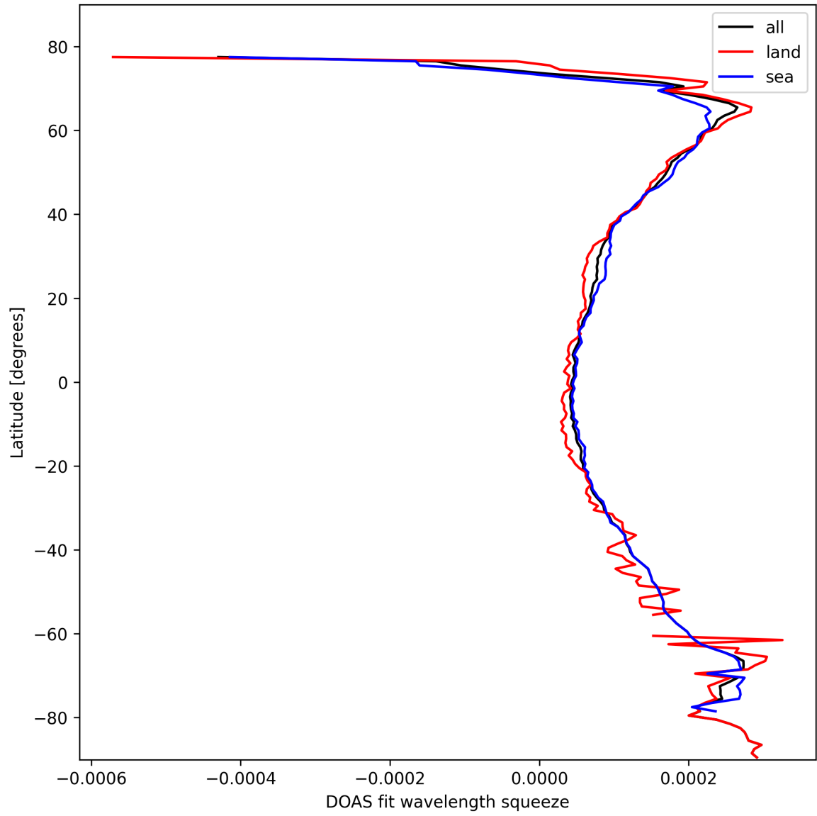
Figure 24: Zonal average of “DOAS fit wavelength squeeze” for 2025-10-24 to 2025-10-25.
