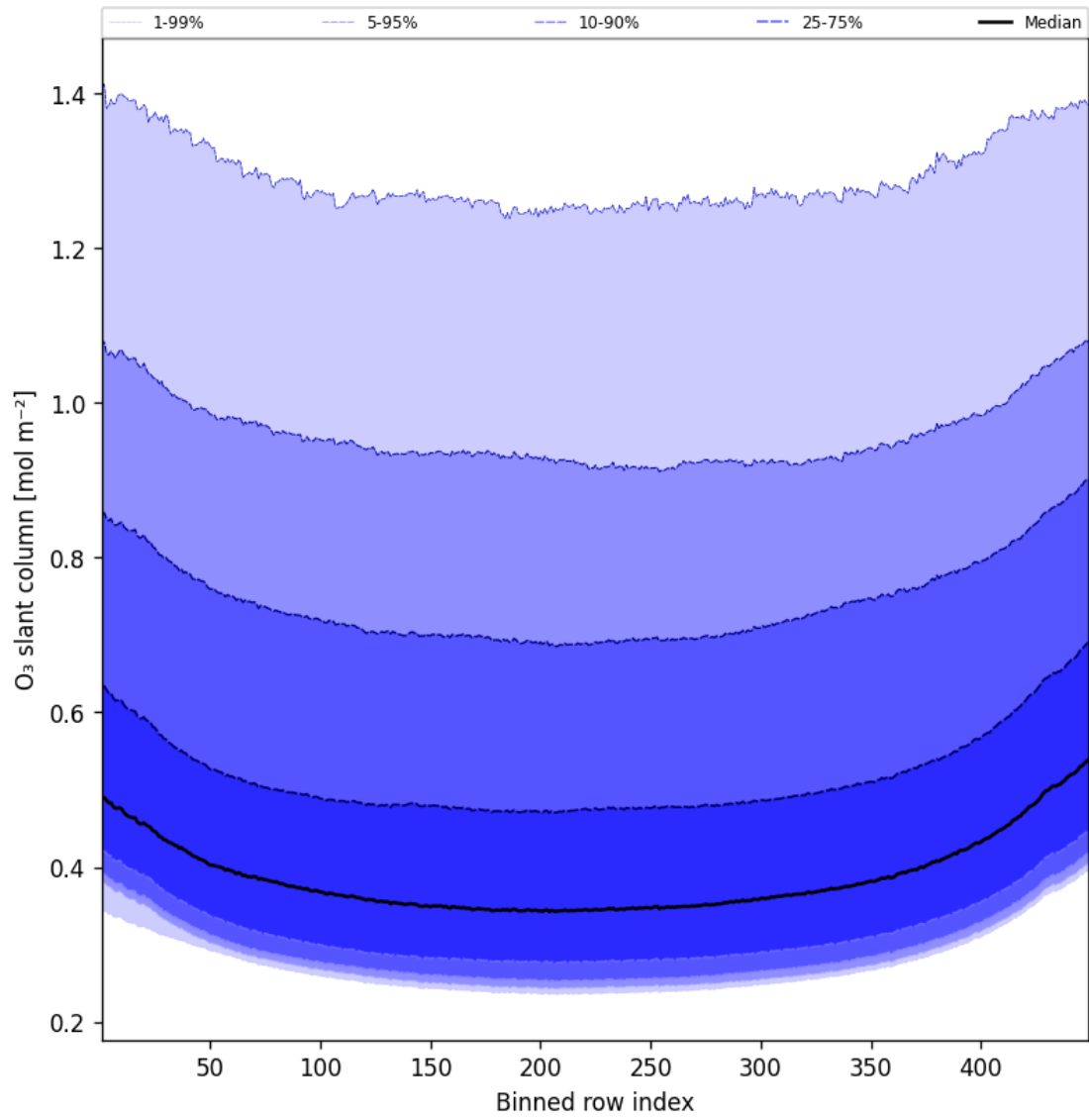
Figure 43: Along track statistics of “O 3 slant column” for 2025-10-24 to 2025-10-25
