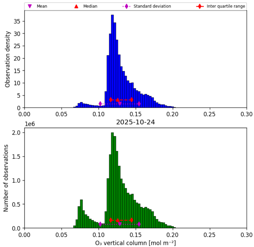
Figure 29: Histogram of “O 3 vertical column” for 2025-10-24 to 2025-10-25
