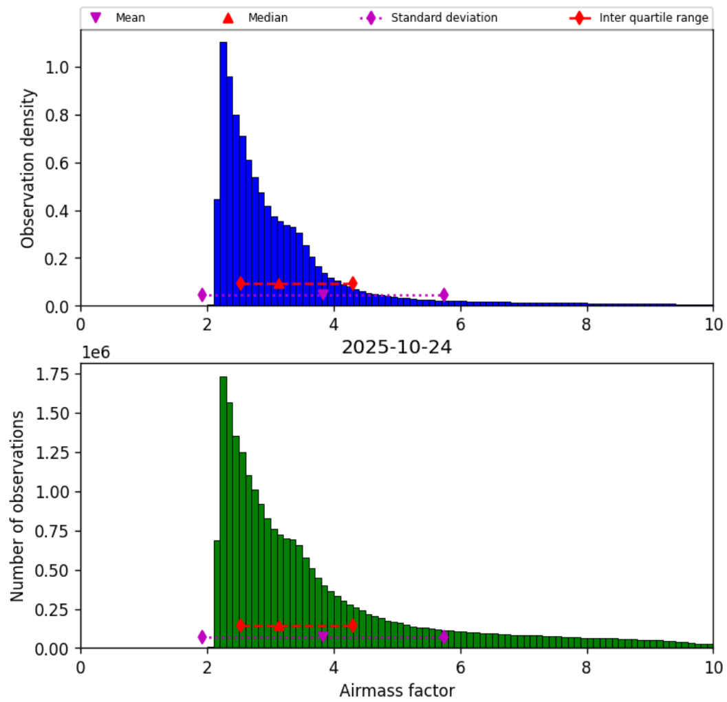
Figure 37: Histogram of “Airmass factor” for 2025-10-24 to 2025-10-25
