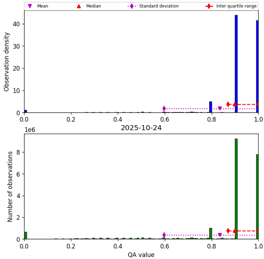
Figure 28: Histogram of “QA value” for 2025-10-24 to 2025-10-25
