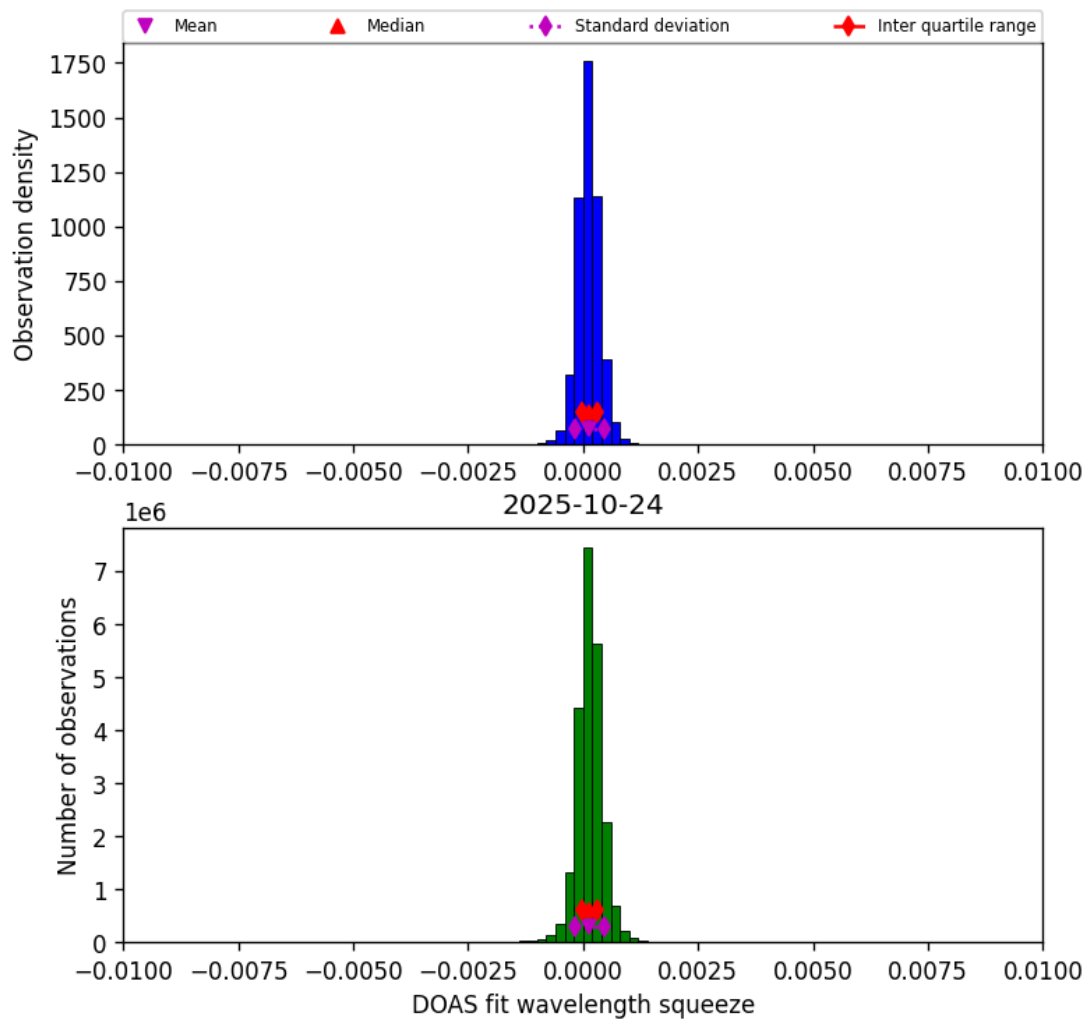
Figure 36: Histogram of “DOAS fit wavelength squeeze” for 2025-10-24 to 2025-10-25
