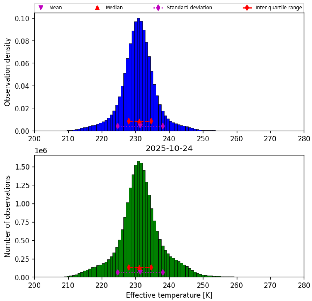
Figure 38: Histogram of “Effective temperature” for 2025-10-24 to 2025-10-25
