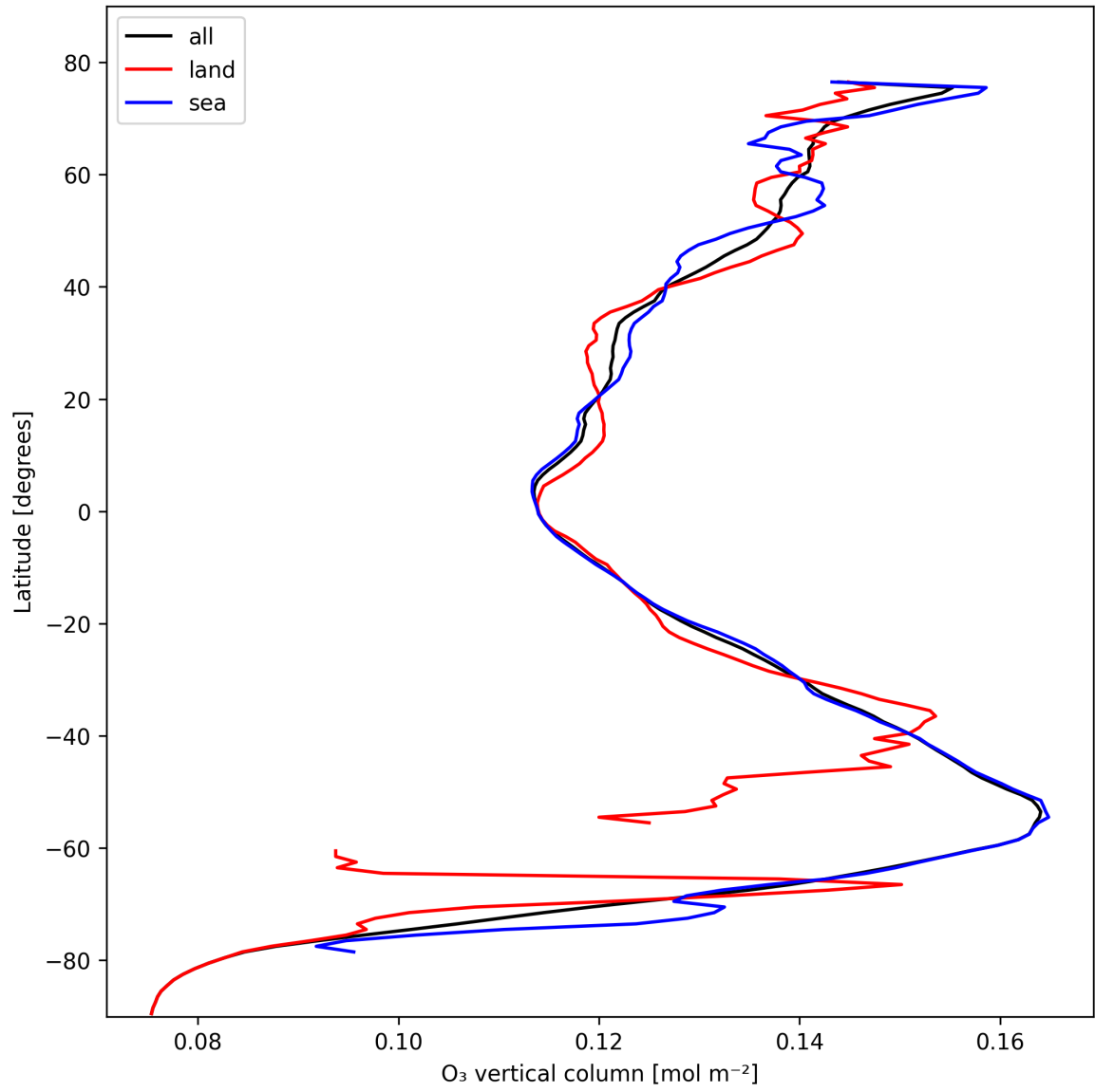
Figure 17: Zonal average of “O 3 vertical column” for 2025-10-27 to 2025-10-28.
