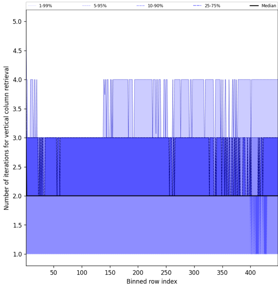
Figure 51: Along track statistics of “Number of iterations for vertical column retrieval” for 2025-10-27 to 2025-10-28
