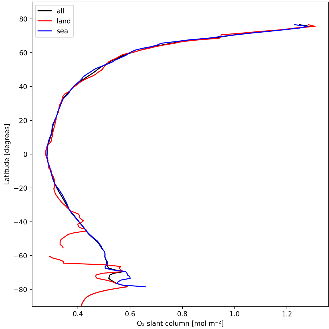
Figure 19: Zonal average of “O 3 slant column” for 2025-10-27 to 2025-10-28.
