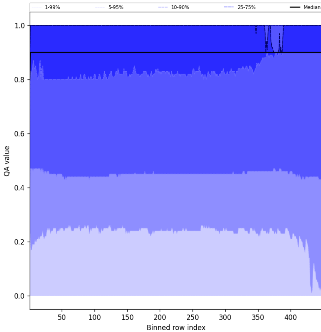
Figure 40: Along track statistics of “QA value” for 2025-10-27 to 2025-10-28
