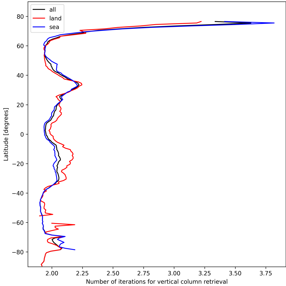
Figure 27: Zonal average of “Number of iterations for vertical column retrieval” for 2025-10-27 to 2025-10-28.
