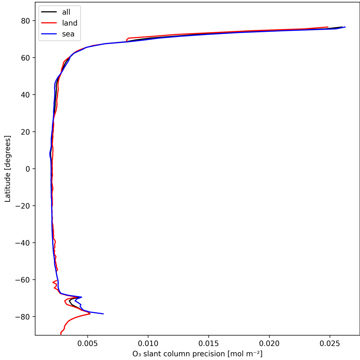
Figure 20: Zonal average of “O 3 slant column precision” for 2025-10-27 to 2025-10-28.
