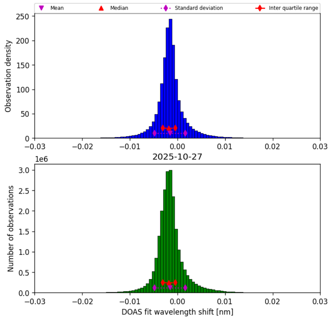
Figure 35: Histogram of “DOAS fit wavelength shift” for 2025-10-27 to 2025-10-28
