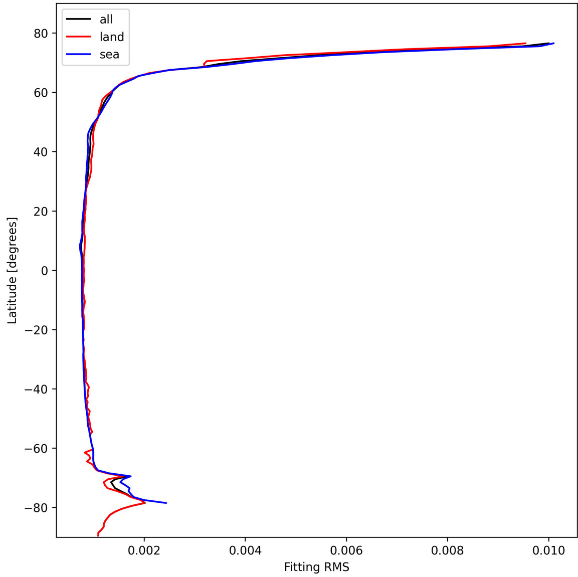
Figure 22: Zonal average of “Fitting RMS” for 2025-10-27 to 2025-10-28.
