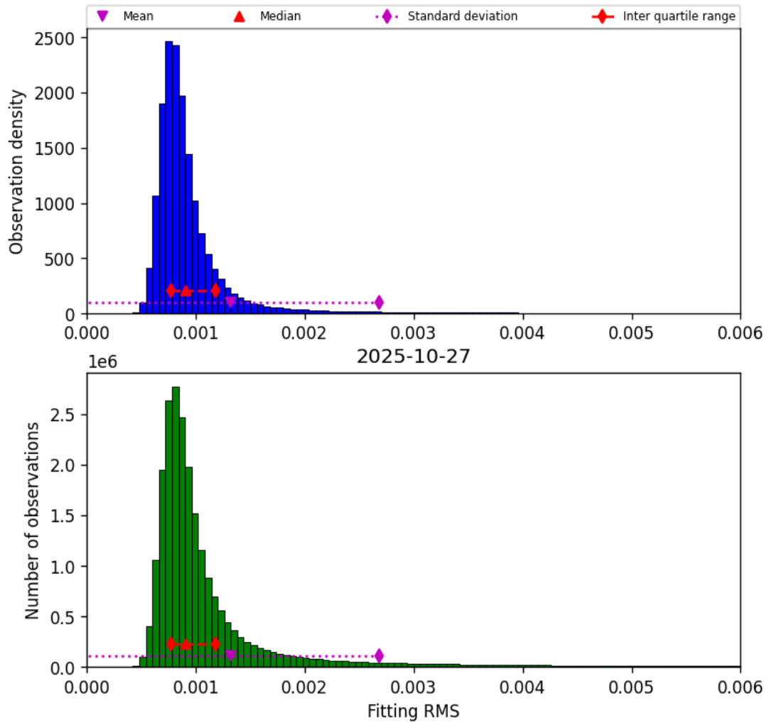
Figure 34: Histogram of “Fitting RMS” for 2025-10-27 to 2025-10-28
