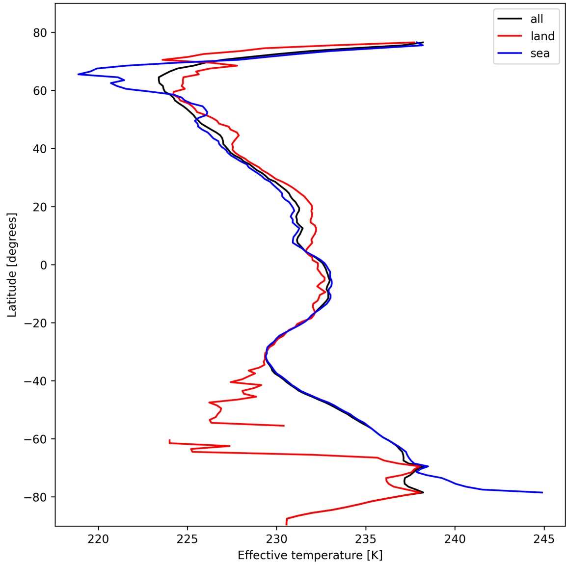
Figure 26: Zonal average of “Effective temperature” for 2025-10-27 to 2025-10-28.
