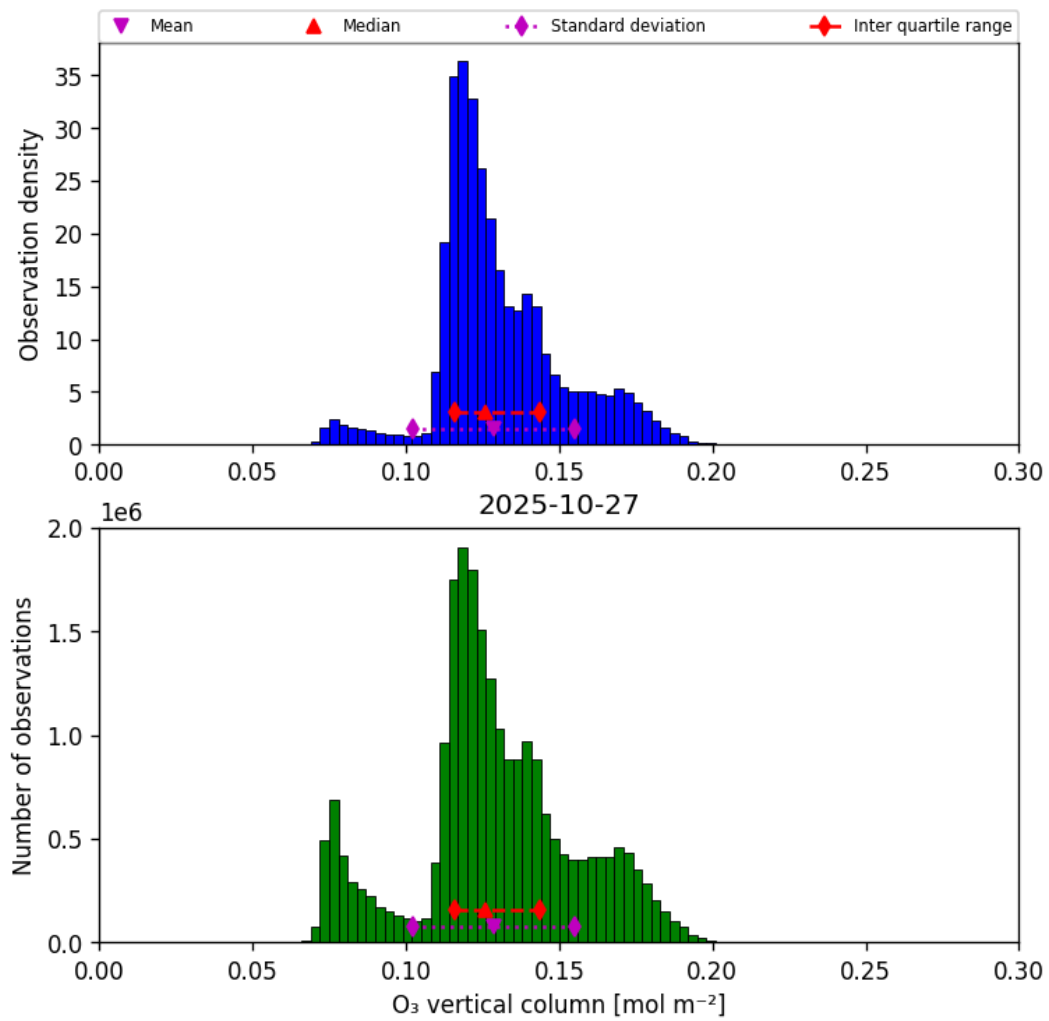
Figure 29: Histogram of “O 3 vertical column” for 2025-10-27 to 2025-10-28
