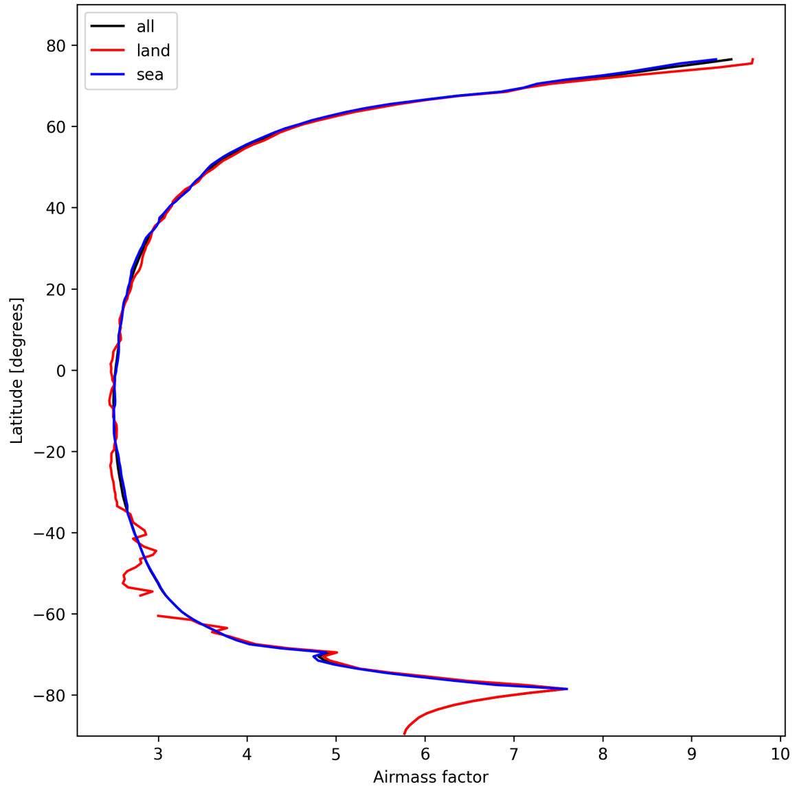
Figure 25: Zonal average of “Airmass factor” for 2025-10-27 to 2025-10-28.
