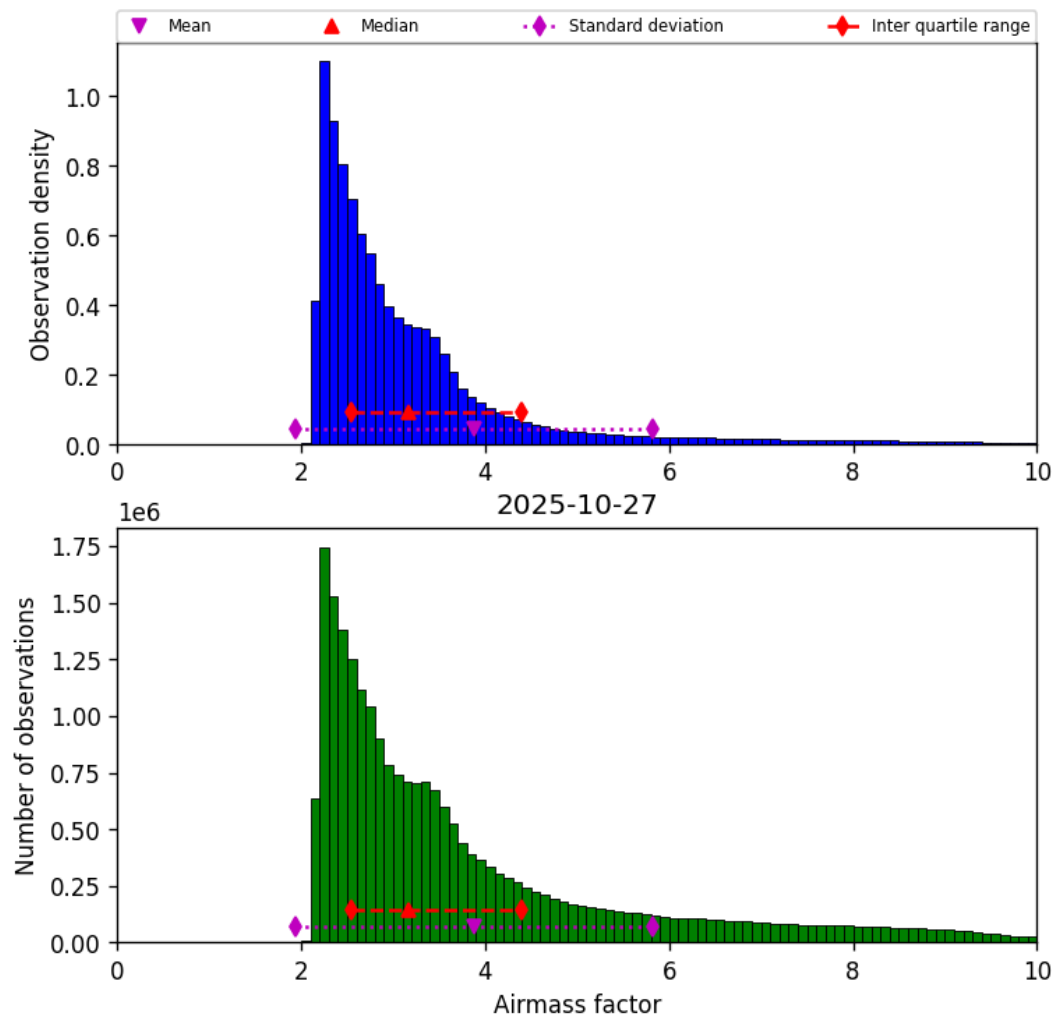
Figure 37: Histogram of “Airmass factor” for 2025-10-27 to 2025-10-28
