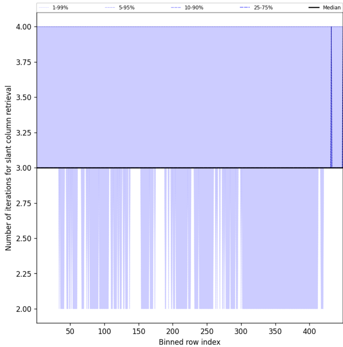
Figure 45: Along track statistics of “Number of iterations for slant column retrieval” for 2025-10-27 to 2025-10-28
