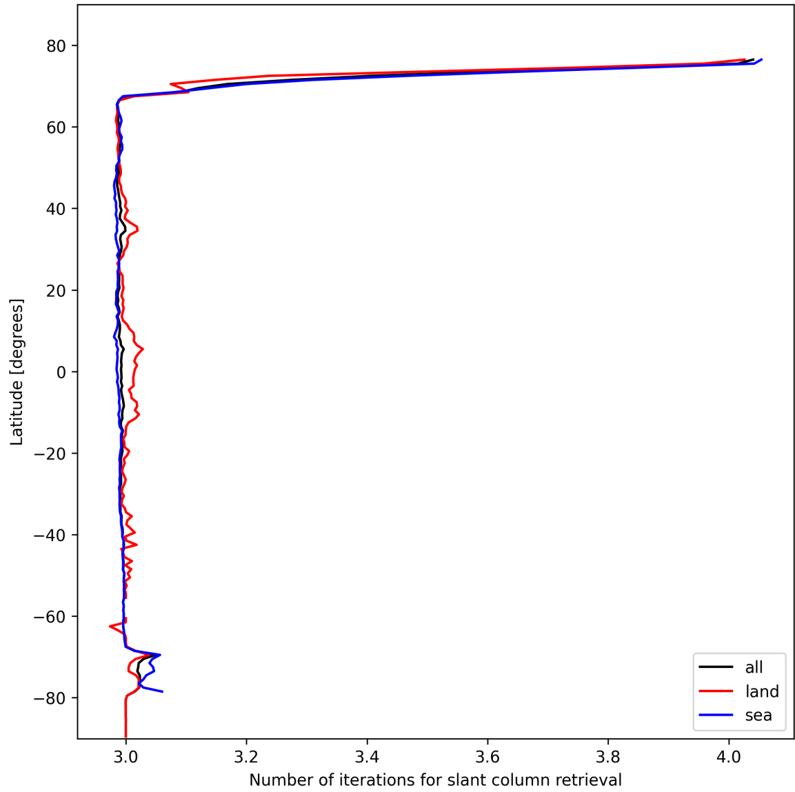
Figure 21: Zonal average of “Number of iterations for slant column retrieval” for 2025-10-27 to 2025-10-28.
