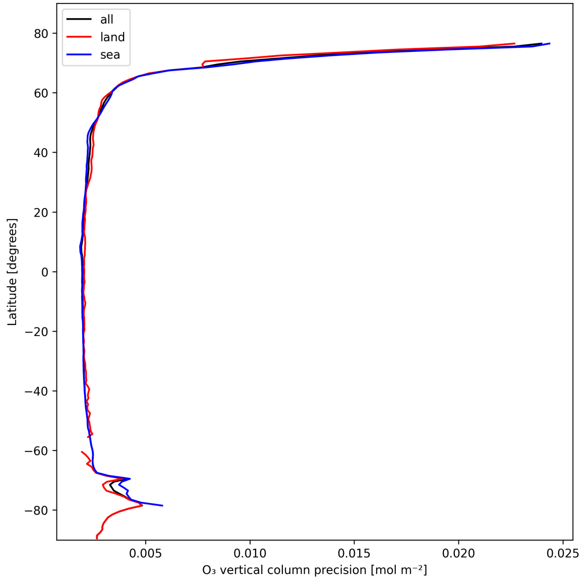
Figure 18: Zonal average of “O 3 vertical column precision” for 2025-10-27 to 2025-10-28.
