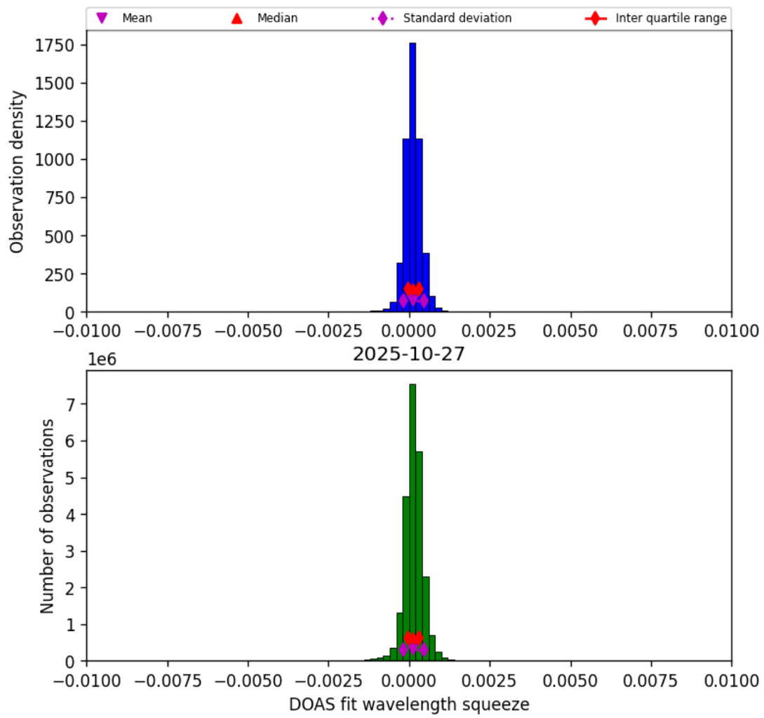
Figure 36: Histogram of “DOAS fit wavelength squeeze” for 2025-10-27 to 2025-10-28
