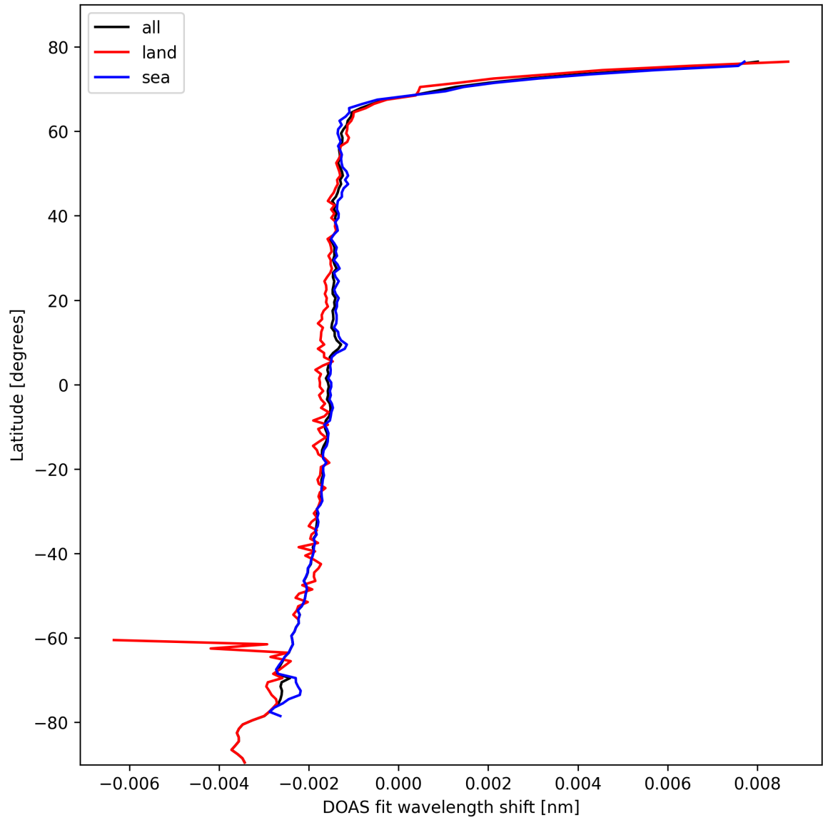
Figure 23: Zonal average of “DOAS fit wavelength shift” for 2025-10-27 to 2025-10-28.
