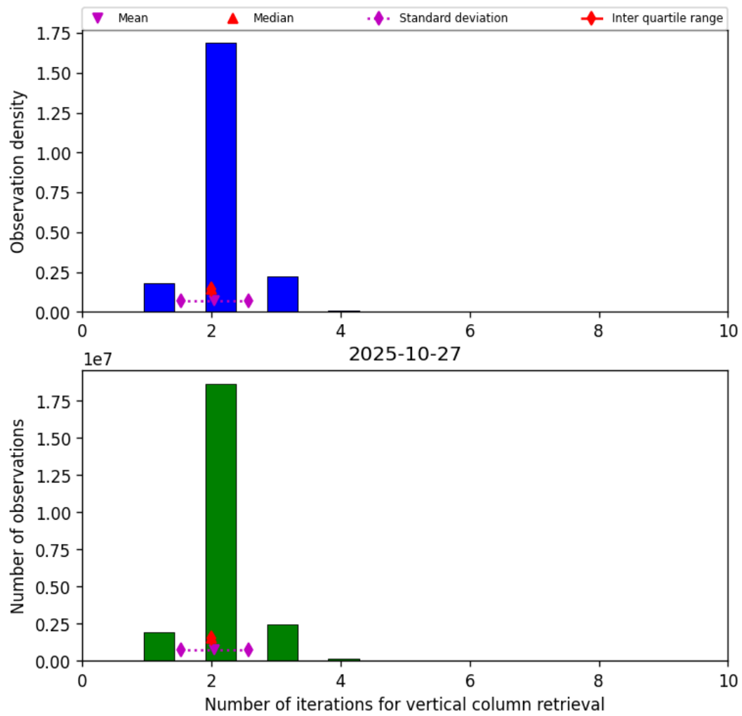
Figure 39: Histogram of “Number of iterations for vertical column retrieval” for 2025-10-27 to 2025-10-28
