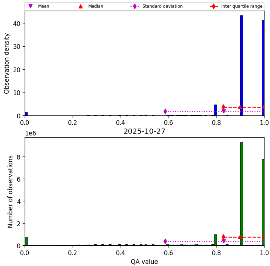
Figure 28: Histogram of “QA value” for 2025-10-27 to 2025-10-28
