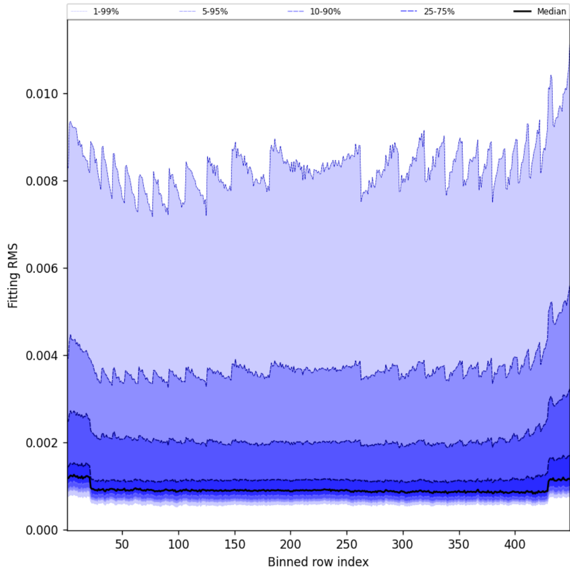
Figure 46: Along track statistics of “Fitting RMS” for 2025-10-27 to 2025-10-28
