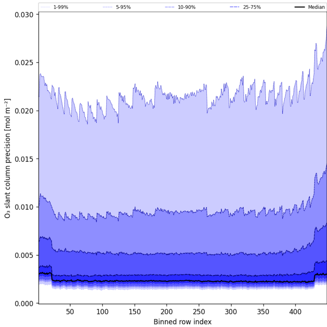
Figure 44: Along track statistics of “O 3 slant column precision” for 2025-10-27 to 2025-10-28
