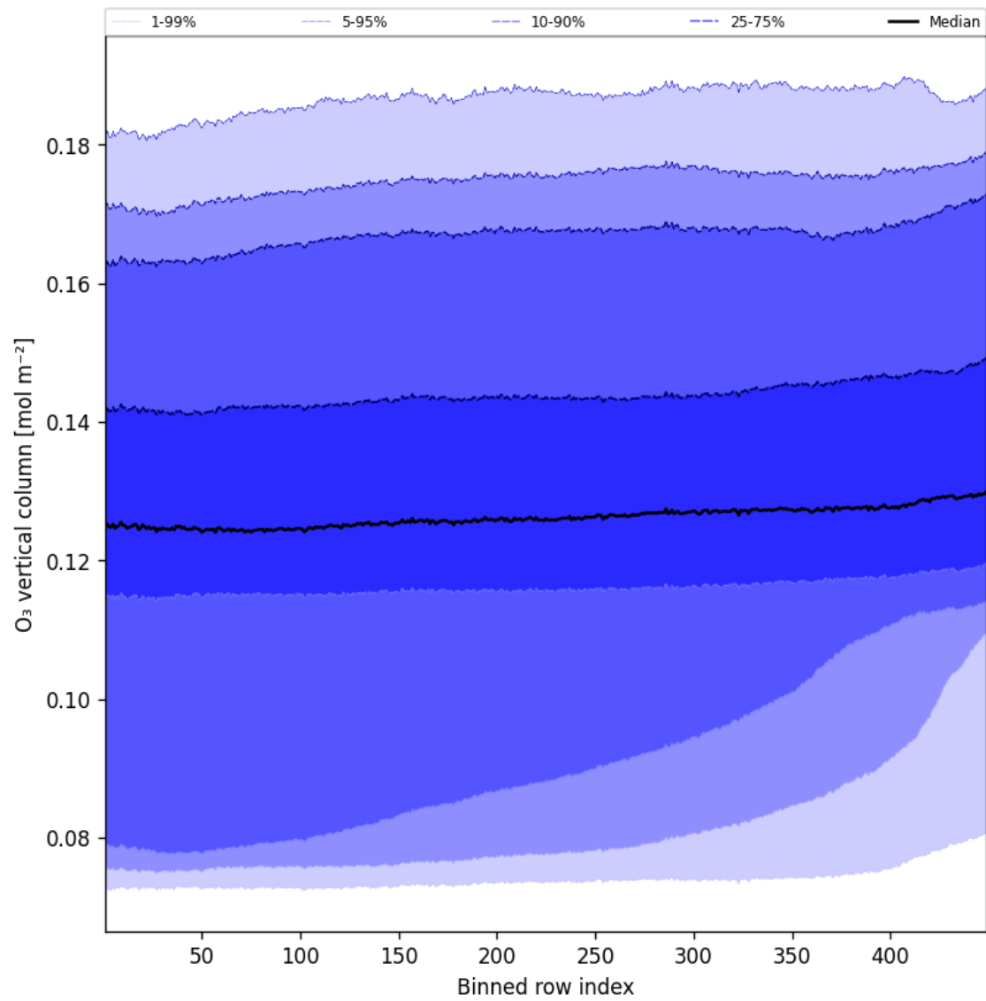
Figure 41: Along track statistics of “O 3 vertical column” for 2025-10-27 to 2025-10-28
