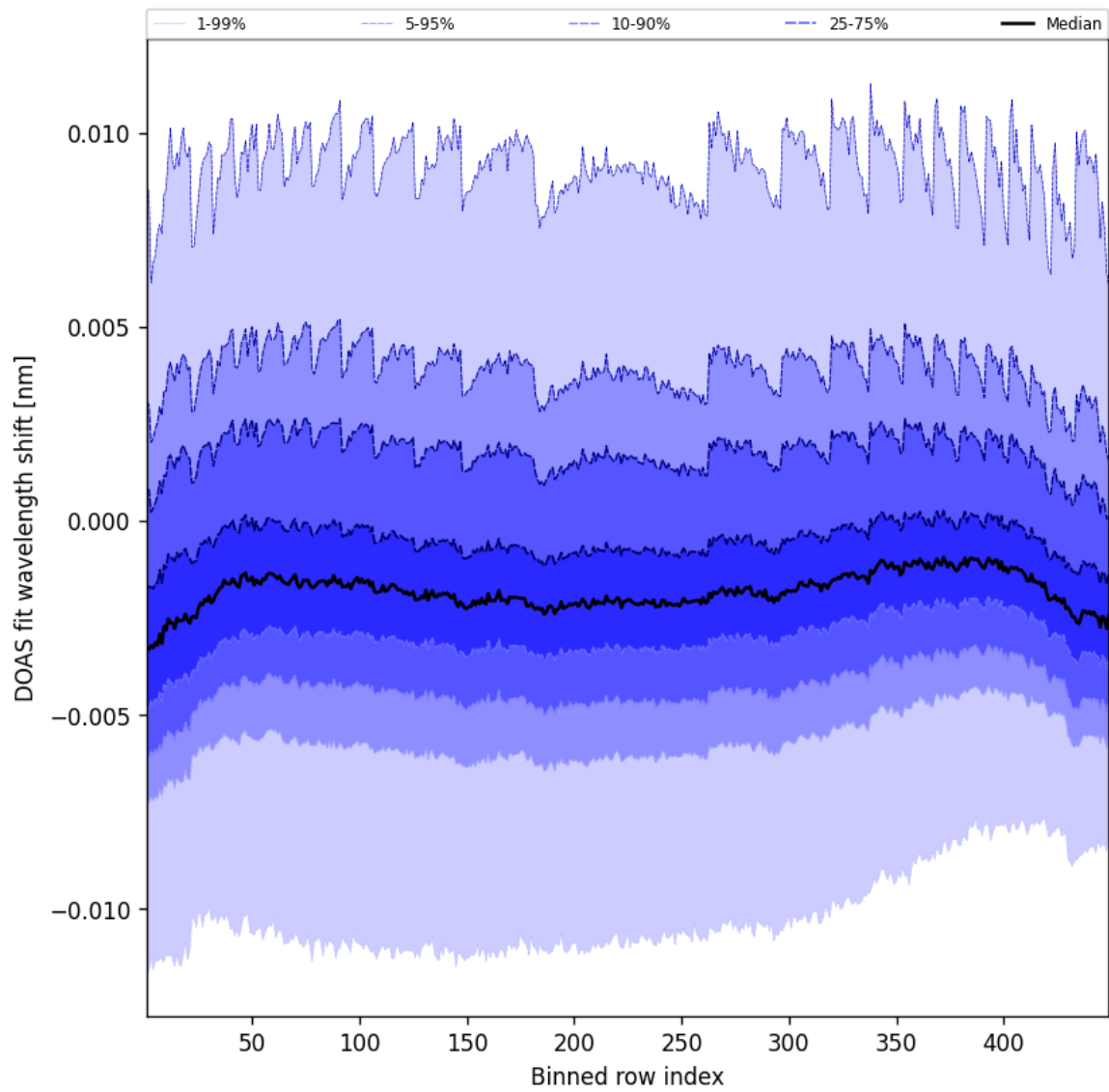
Figure 47: Along track statistics of “DOAS fit wavelength shift” for 2025-10-27 to 2025-10-28
