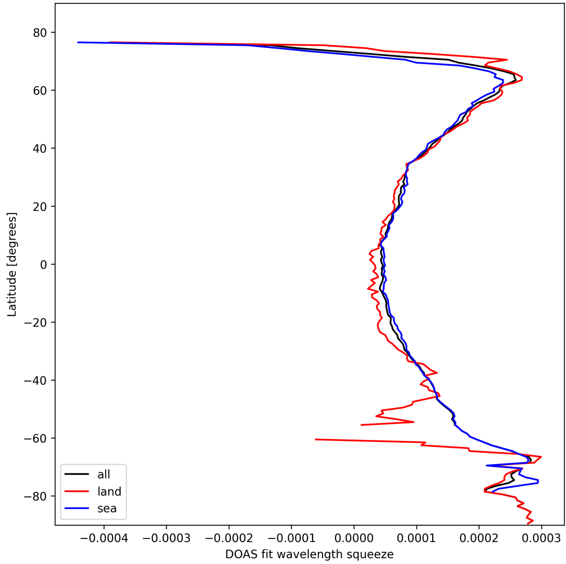
Figure 24: Zonal average of “DOAS fit wavelength squeeze” for 2025-10-27 to 2025-10-28.
