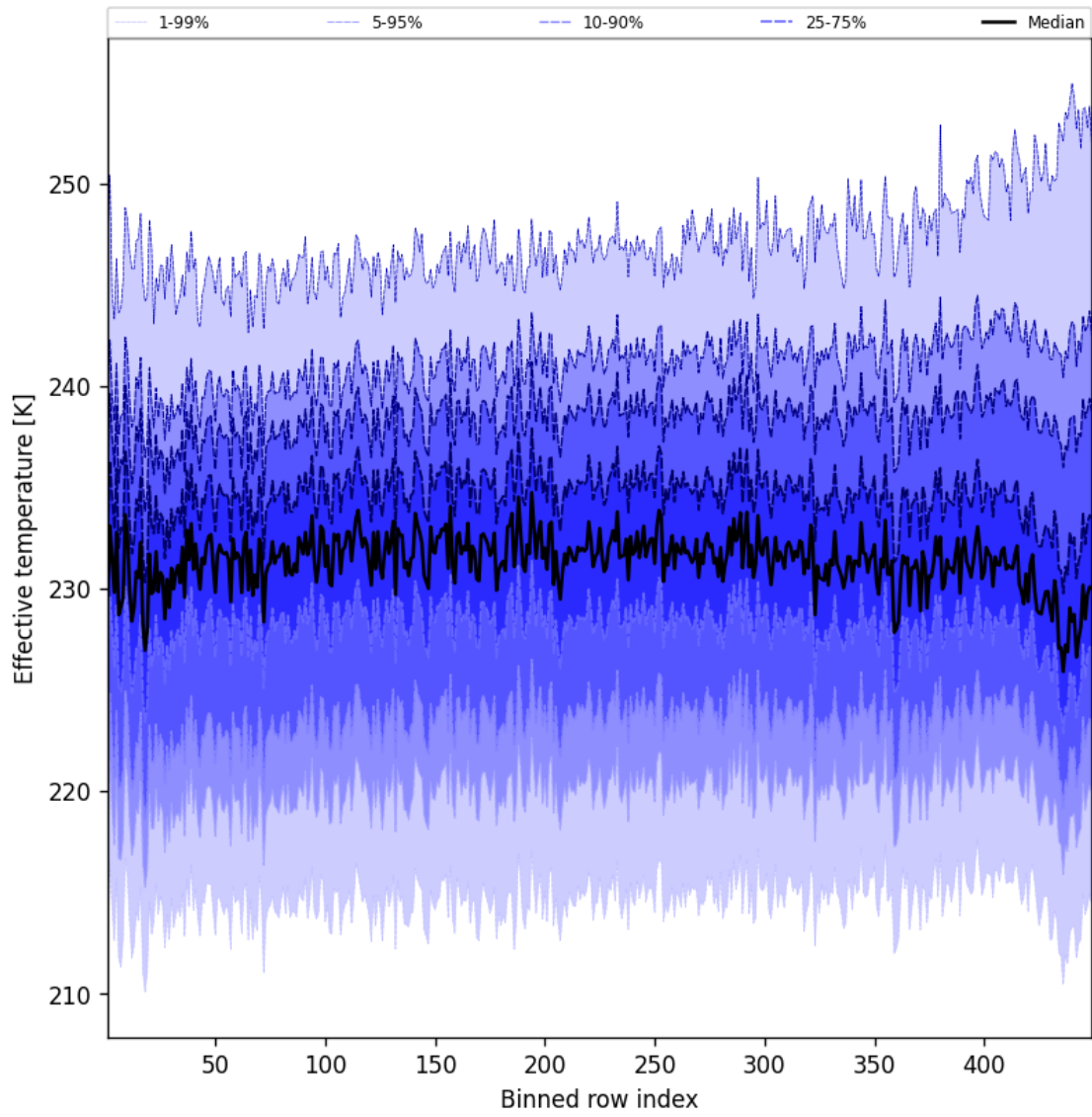
Figure 50: Along track statistics of “Effective temperature” for 2025-10-27 to 2025-10-28
