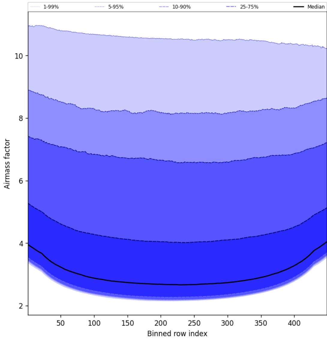
Figure 49: Along track statistics of “Airmass factor” for 2025-10-27 to 2025-10-28
