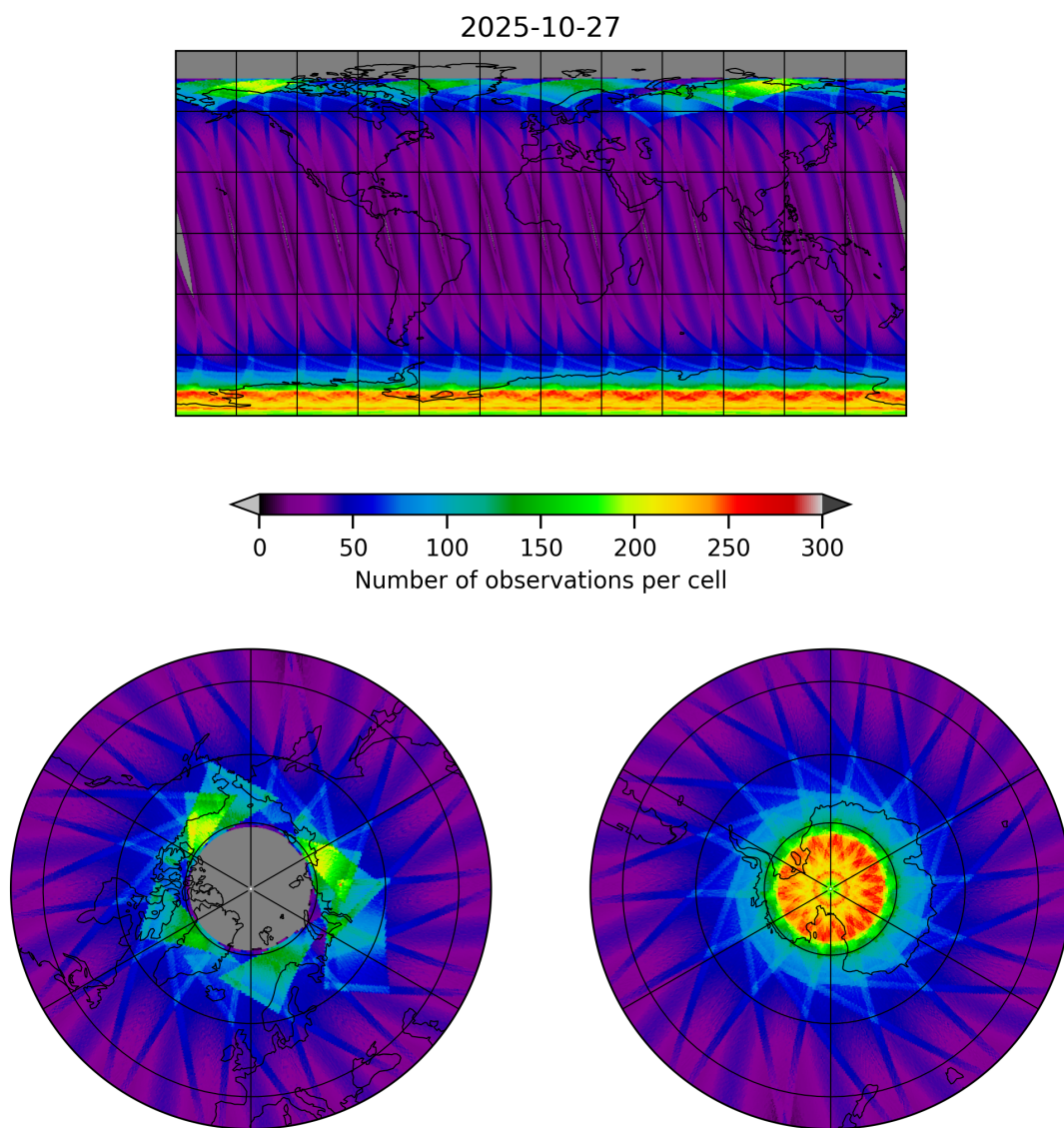
Figure 15: Map of the number of observations for 2025-10-27 to 2025-10-28
