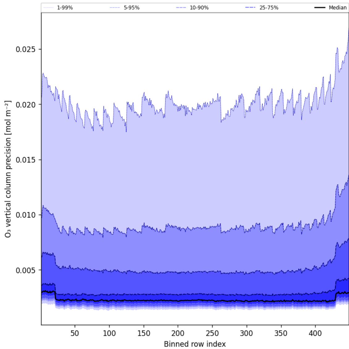
Figure 42: Along track statistics of “O 3 vertical column precision” for 2025-10-27 to 2025-10-28
