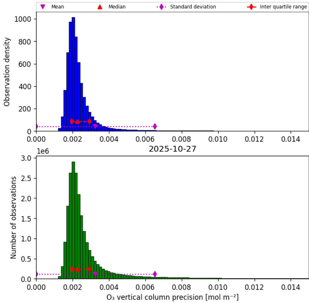
Figure 30: Histogram of “O 3 vertical column precision” for 2025-10-27 to 2025-10-28
