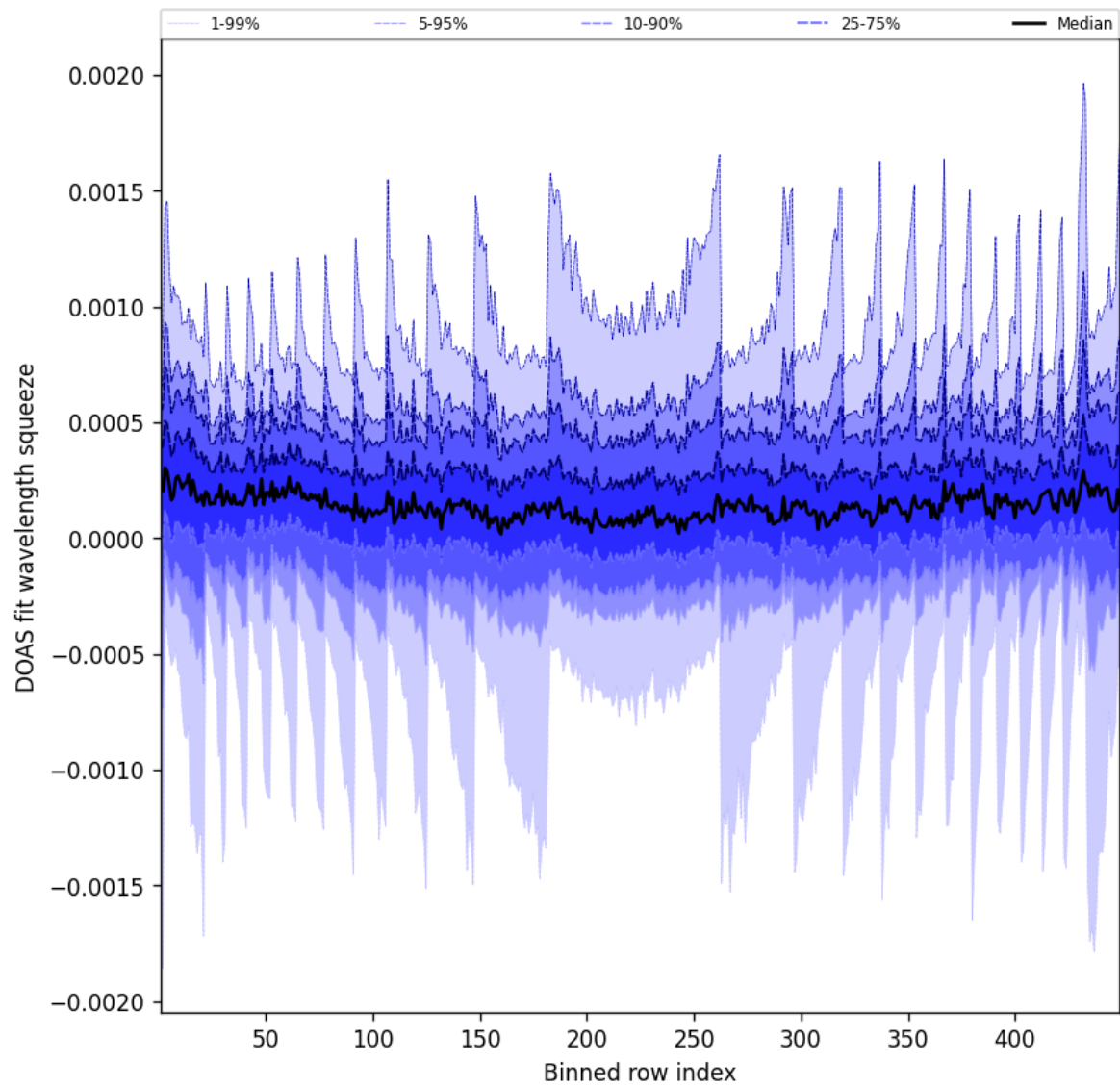
Figure 48: Along track statistics of “DOAS fit wavelength squeeze” for 2025-10-27 to 2025-10-28
