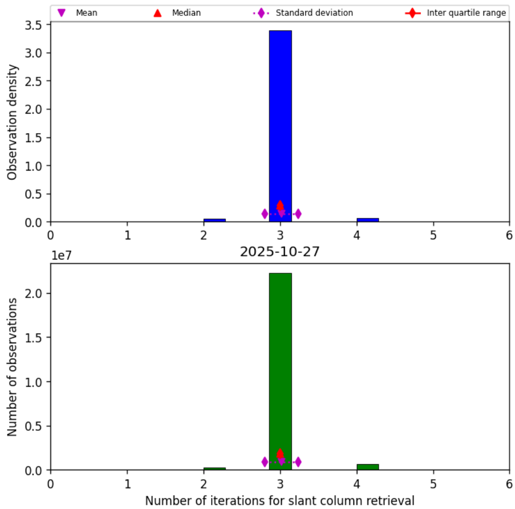
Figure 33: Histogram of “Number of iterations for slant column retrieval” for 2025-10-27 to 2025-10-28
