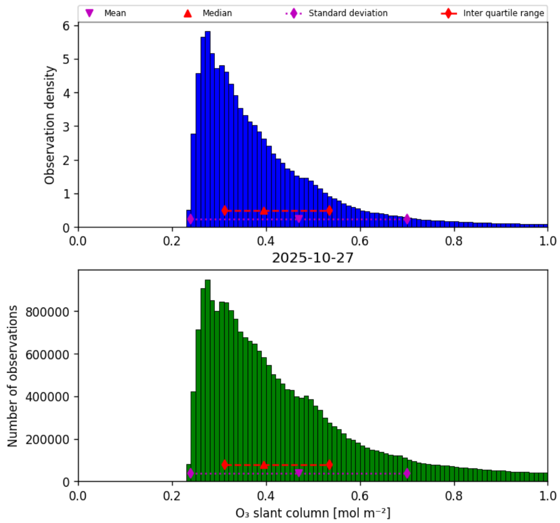
Figure 31: Histogram of “O 3 slant column” for 2025-10-27 to 2025-10-28
