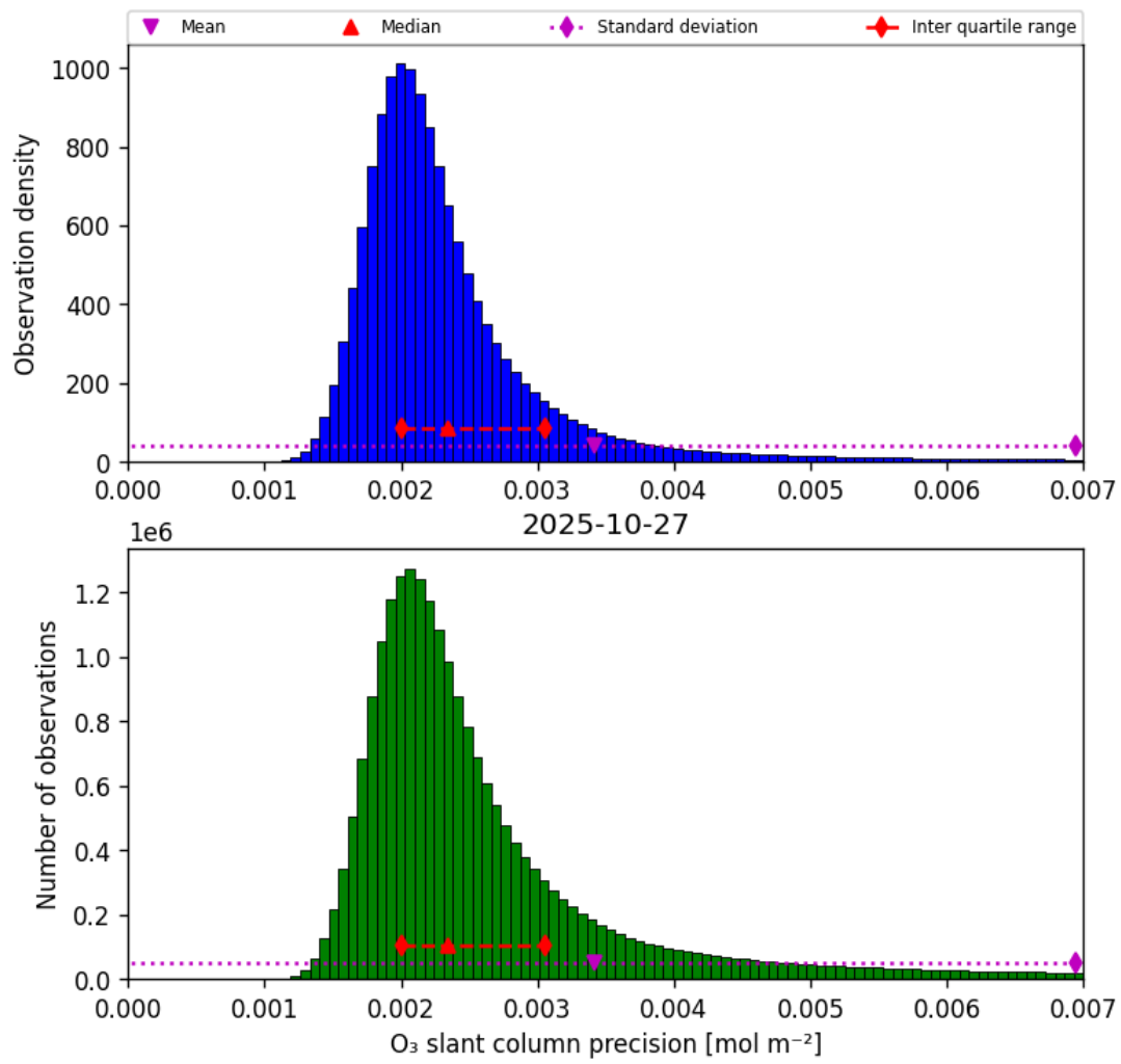
Figure 32: Histogram of “O 3 slant column precision” for 2025-10-27 to 2025-10-28
