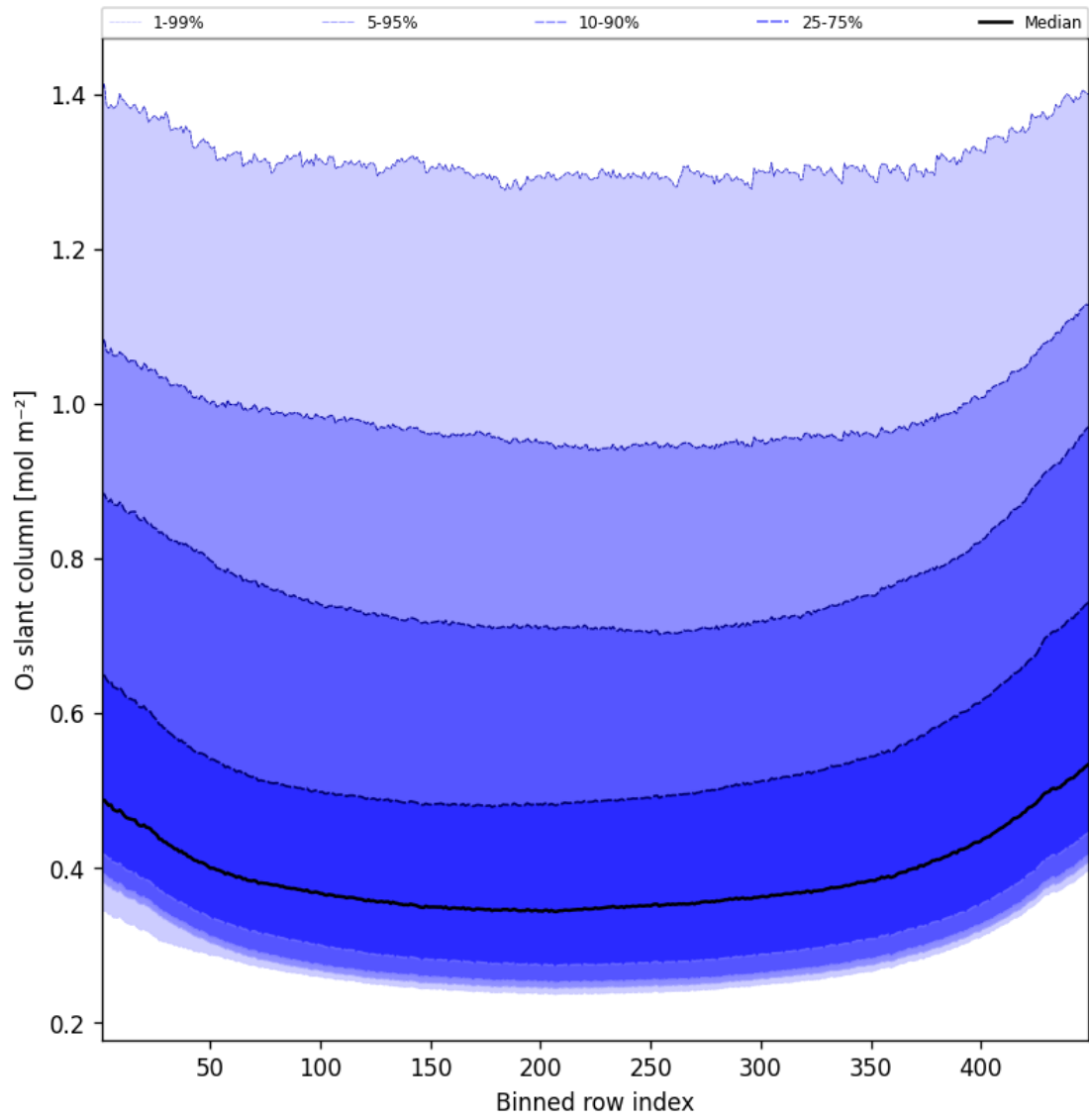
Figure 43: Along track statistics of “O 3 slant column” for 2025-10-27 to 2025-10-28
