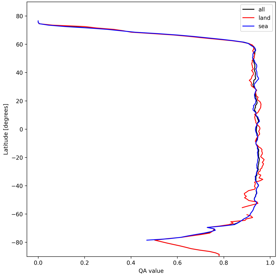
Figure 16: Zonal average of “QA value” for 2025-10-27 to 2025-10-28.
