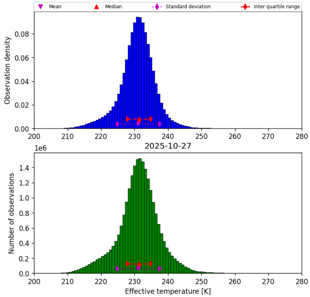
Figure 38: Histogram of “Effective temperature” for 2025-10-27 to 2025-10-28
