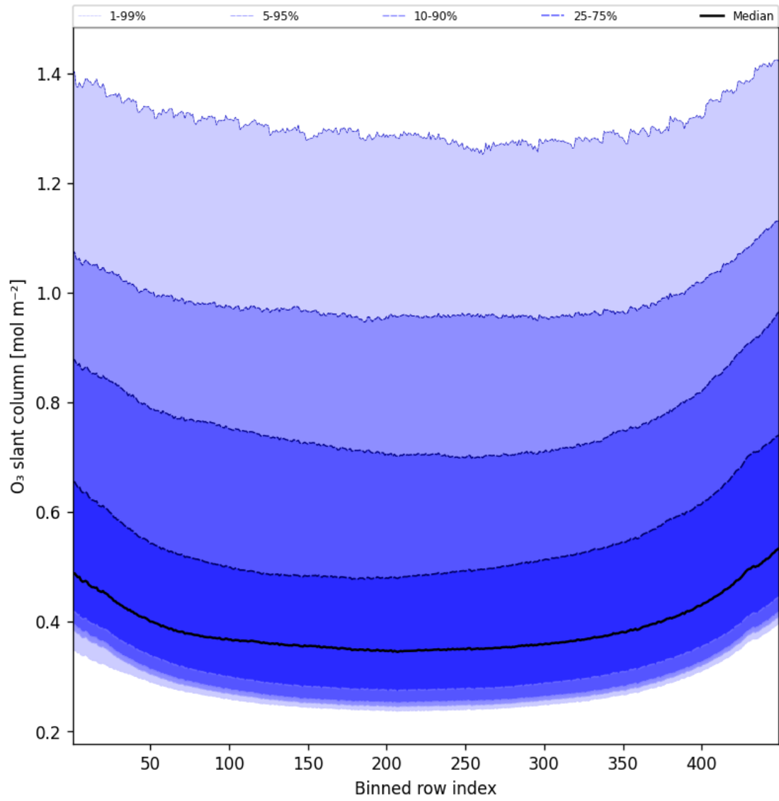
Figure 43: Along track statistics of “O 3 slant column” for 2025-10-28 to 2025-10-29
