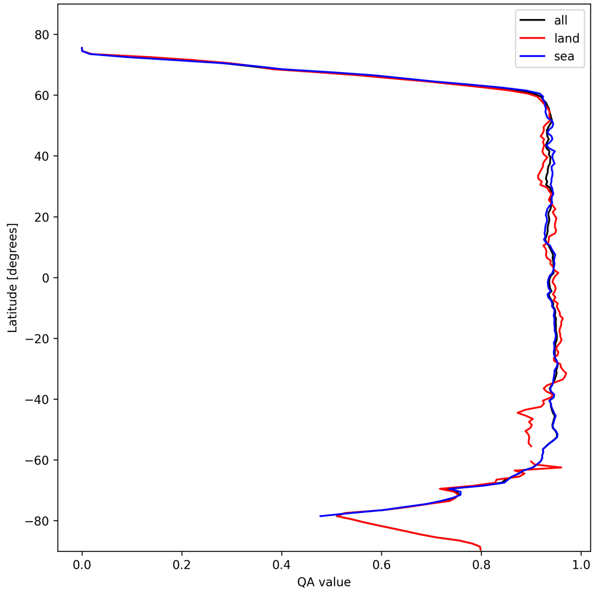
Figure 16: Zonal average of “QA value” for 2025-10-28 to 2025-10-29.
