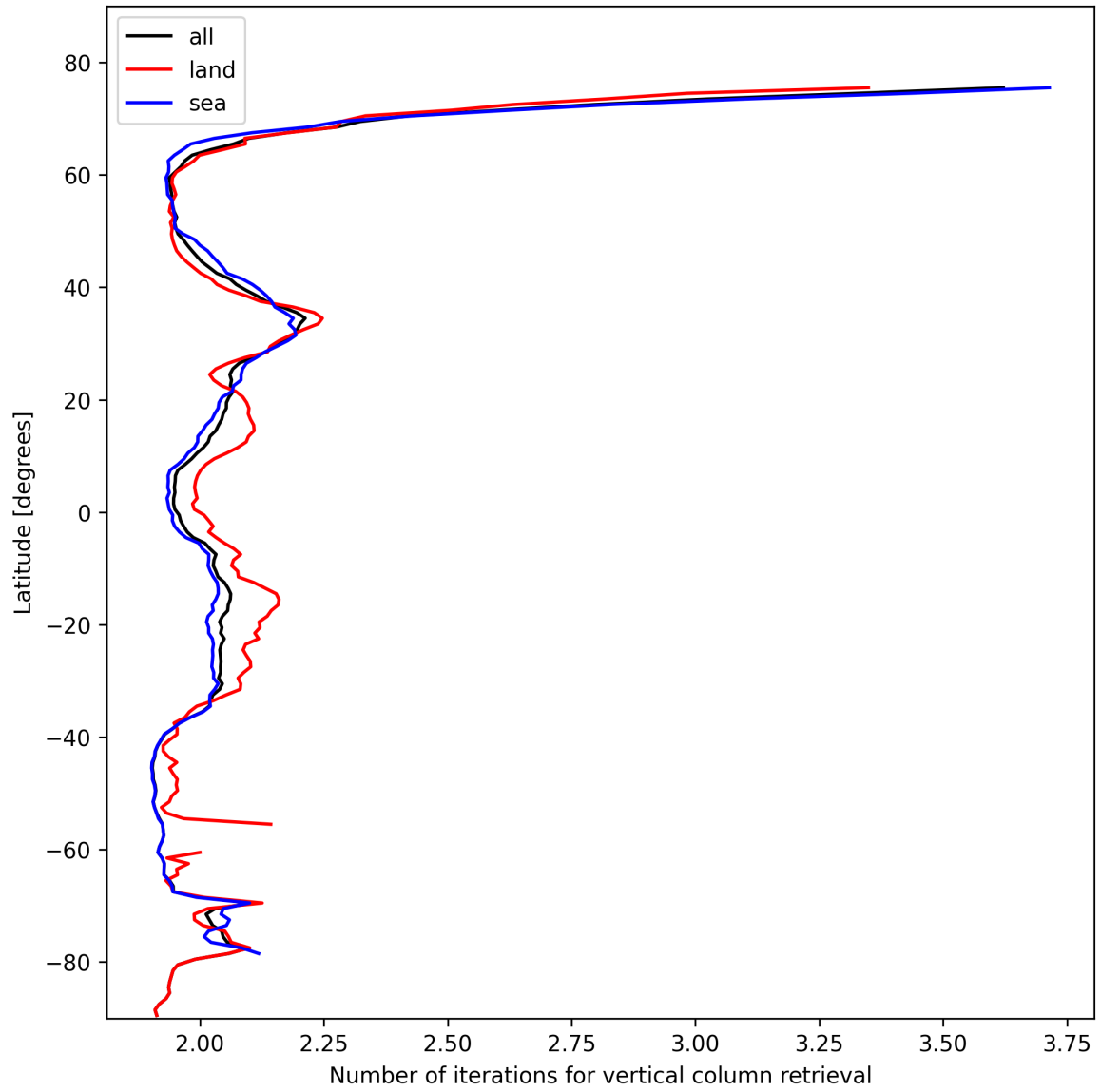
Figure 27: Zonal average of “Number of iterations for vertical column retrieval” for 2025-10-28 to 2025-10-29.
