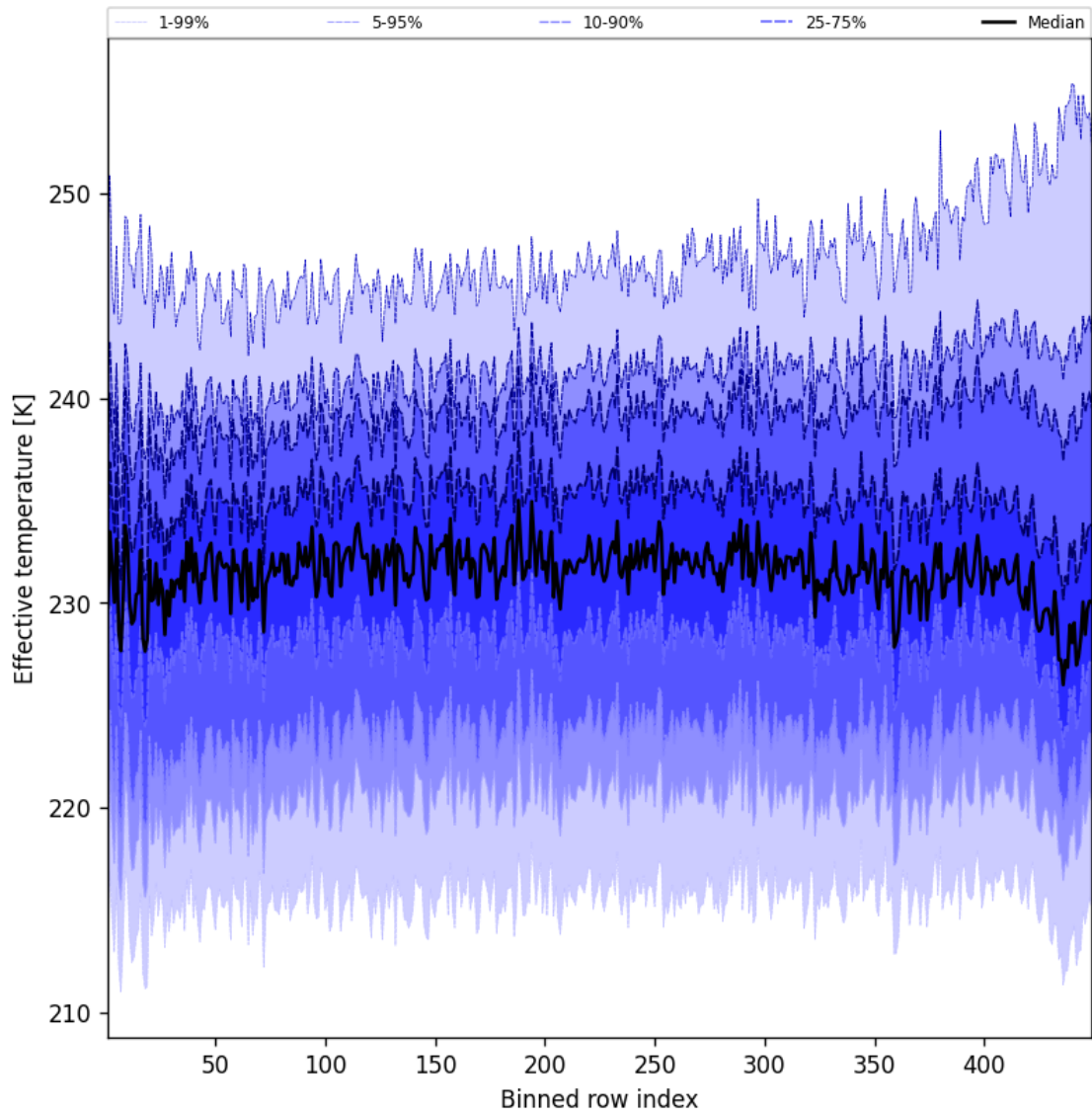
Figure 50: Along track statistics of “Effective temperature” for 2025-10-28 to 2025-10-29
