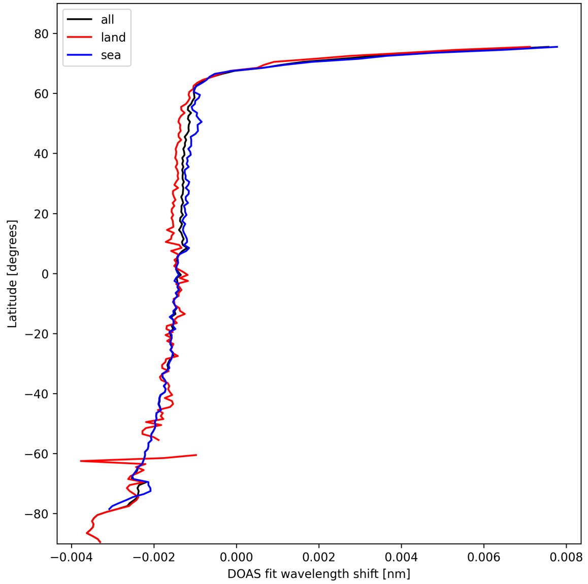
Figure 23: Zonal average of “DOAS fit wavelength shift” for 2025-10-28 to 2025-10-29.
