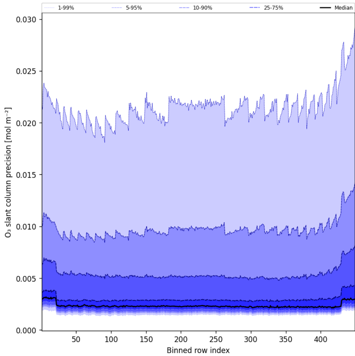
Figure 44: Along track statistics of “O 3 slant column precision” for 2025-10-28 to 2025-10-29
