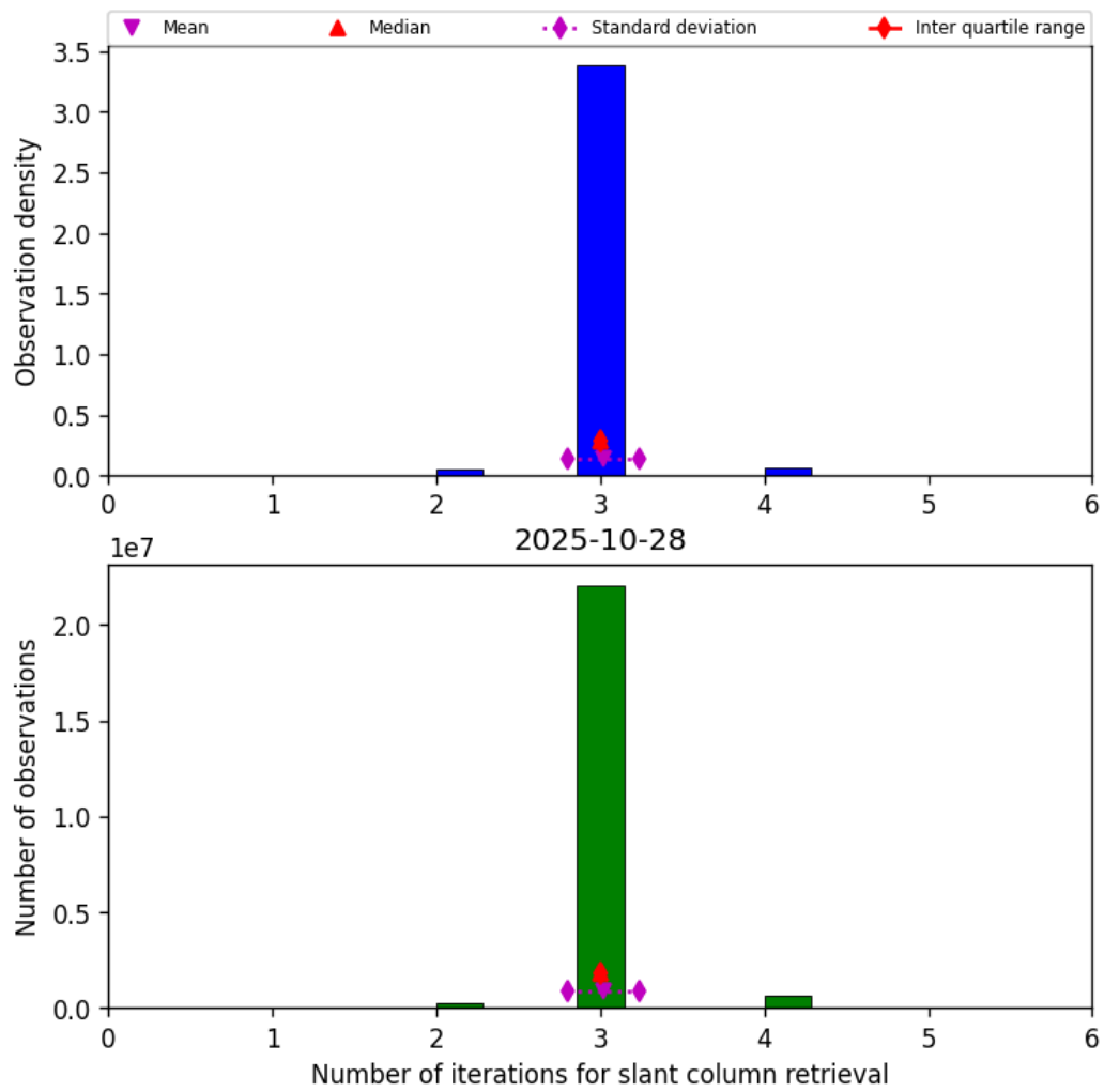
Figure 33: Histogram of “Number of iterations for slant column retrieval” for 2025-10-28 to 2025-10-29
