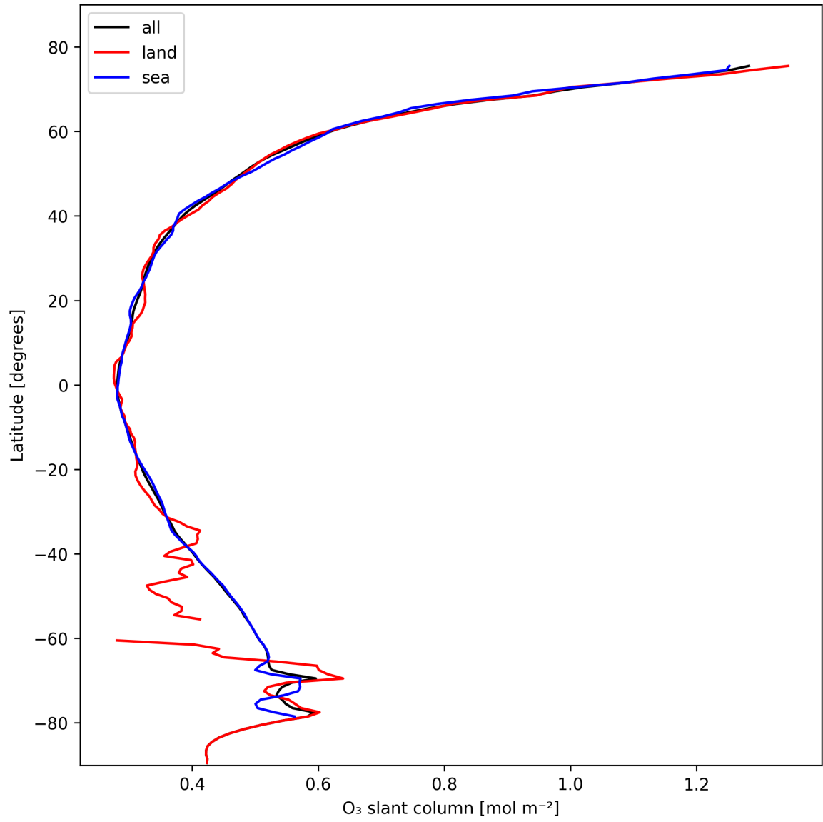
Figure 19: Zonal average of “O 3 slant column” for 2025-10-28 to 2025-10-29.
