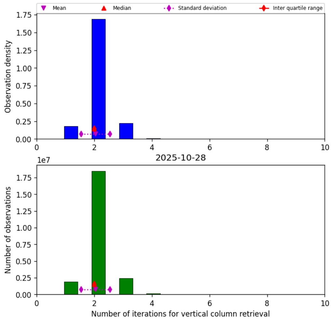
Figure 39: Histogram of “Number of iterations for vertical column retrieval” for 2025-10-28 to 2025-10-29
