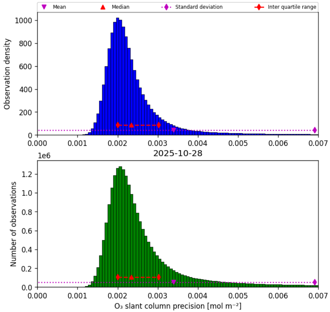
Figure 32: Histogram of “O 3 slant column precision” for 2025-10-28 to 2025-10-29
