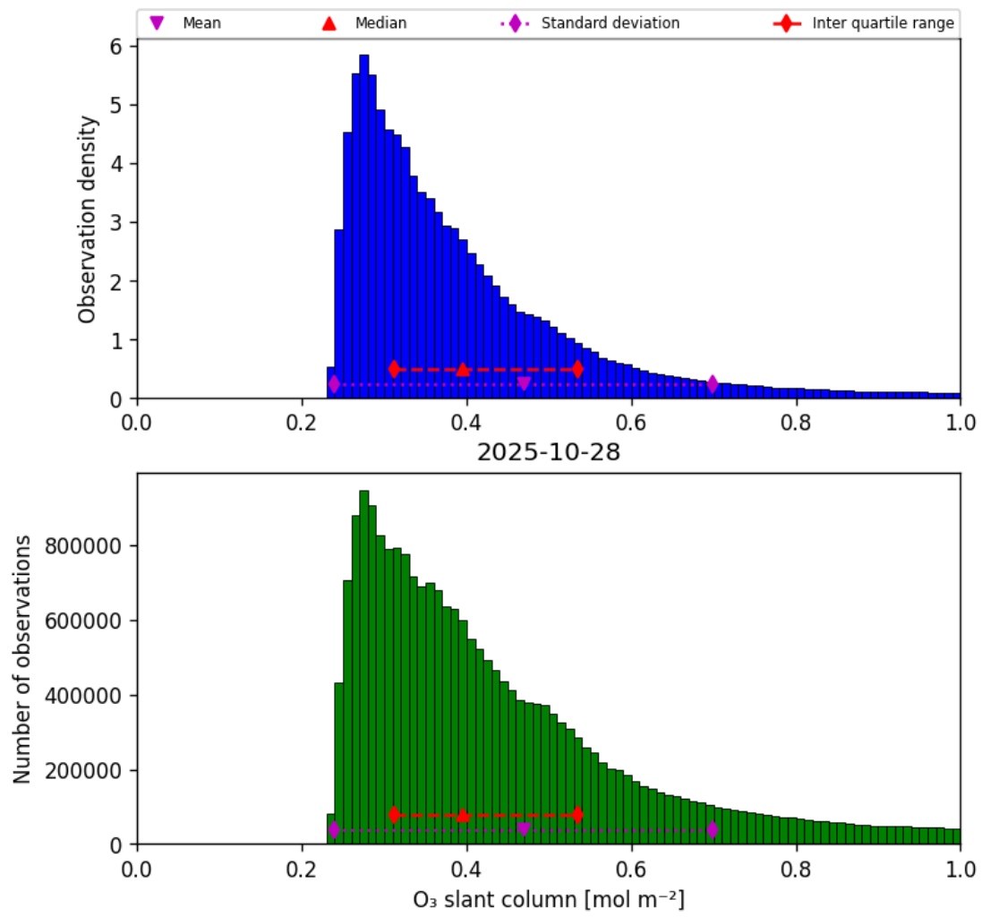
Figure 31: Histogram of “O 3 slant column” for 2025-10-28 to 2025-10-29
