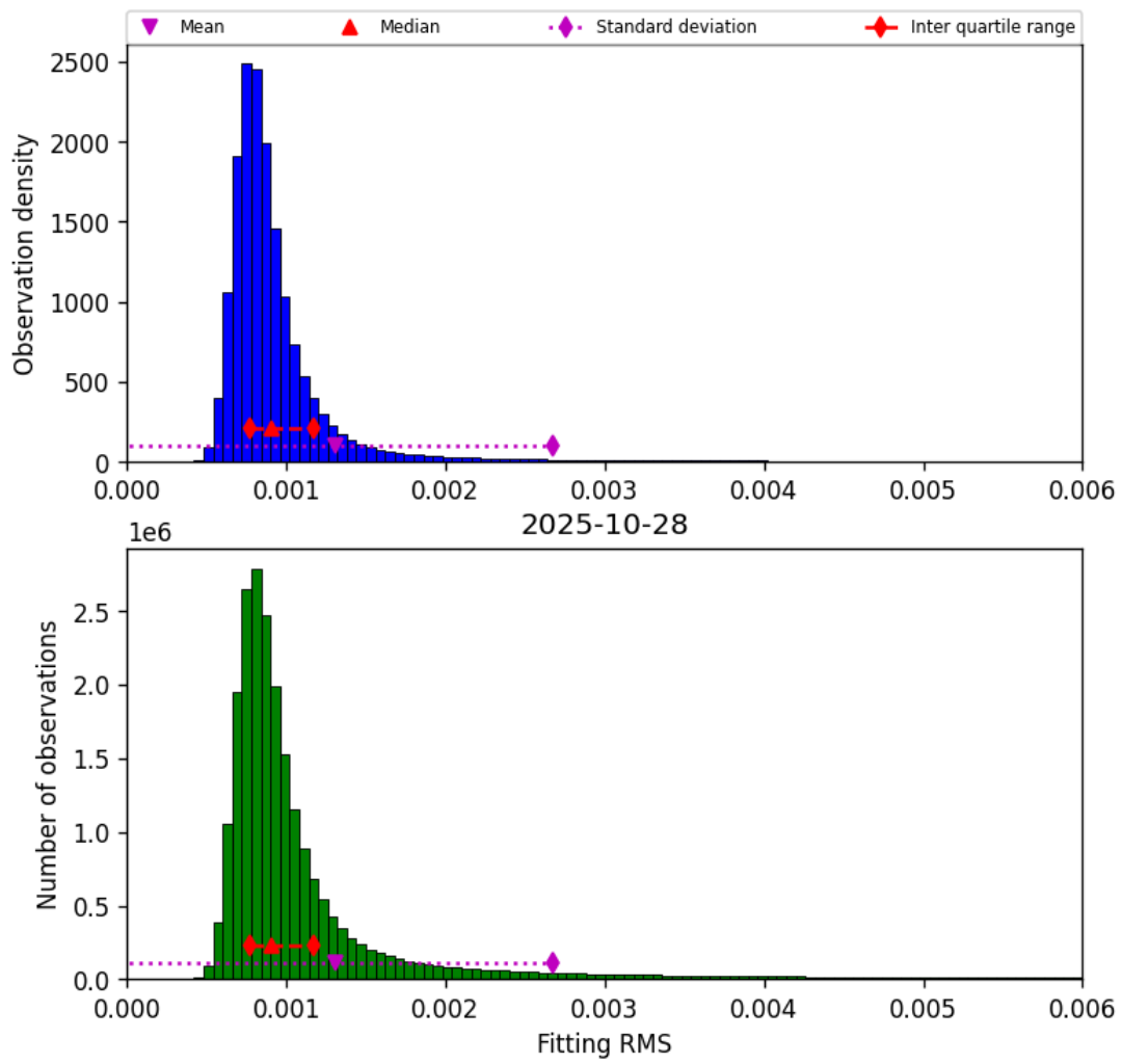
Figure 34: Histogram of “Fitting RMS” for 2025-10-28 to 2025-10-29
