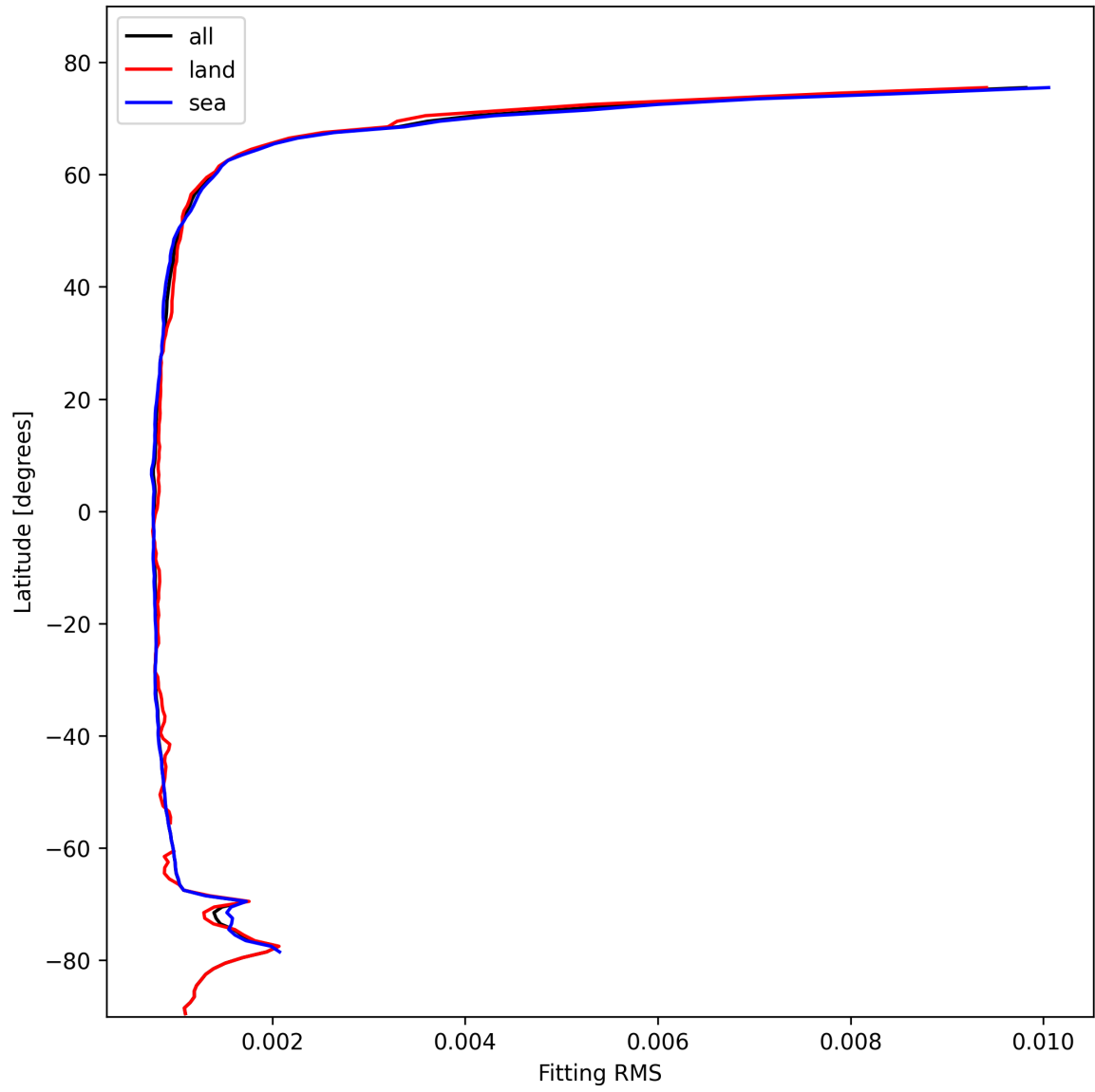
Figure 22: Zonal average of “Fitting RMS” for 2025-10-28 to 2025-10-29.
