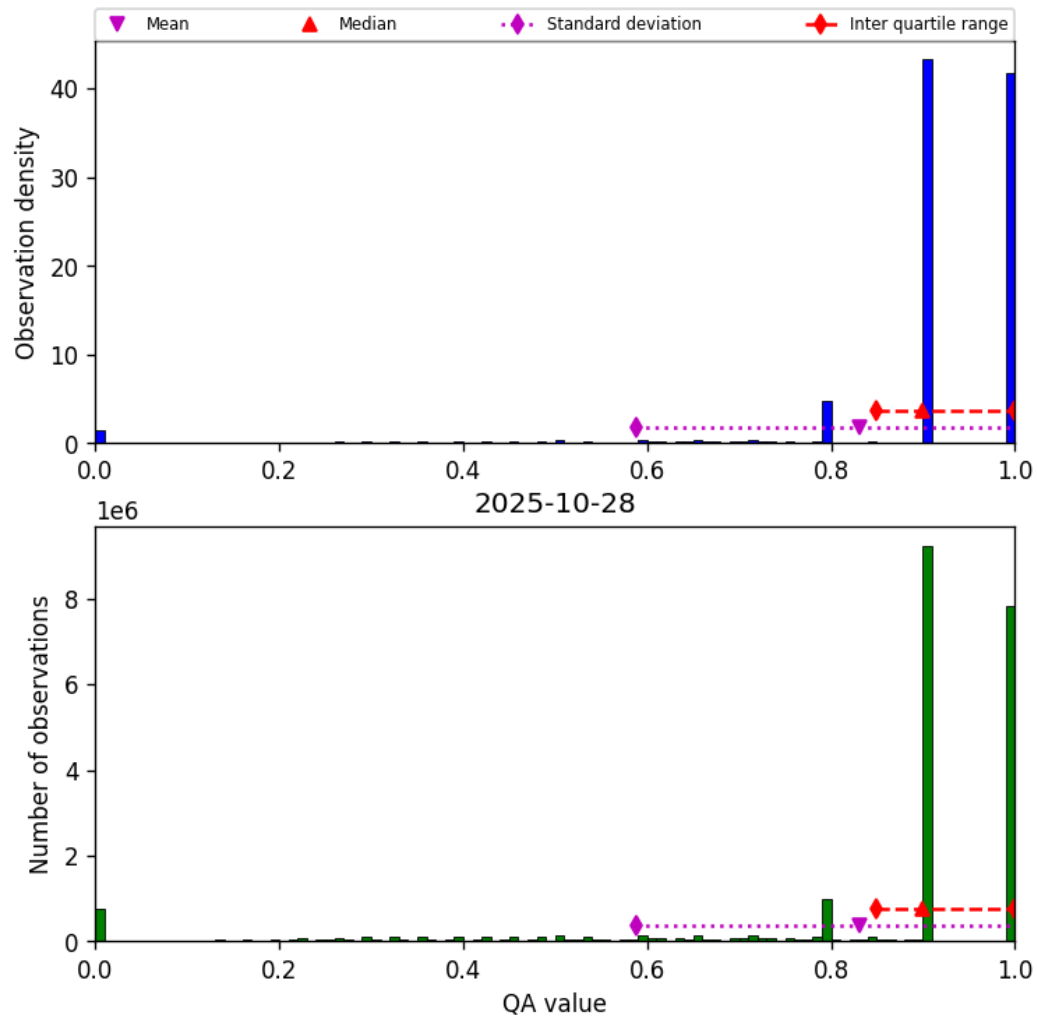
Figure 28: Histogram of “QA value” for 2025-10-28 to 2025-10-29
