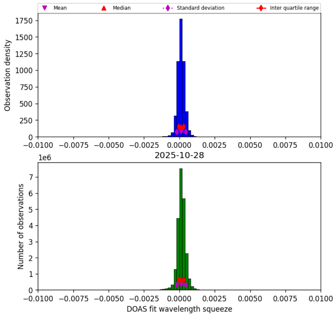
Figure 36: Histogram of “DOAS fit wavelength squeeze” for 2025-10-28 to 2025-10-29
