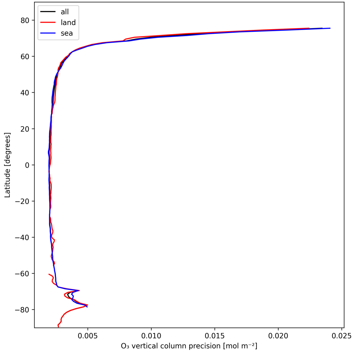
Figure 18: Zonal average of “O 3 vertical column precision” for 2025-10-28 to 2025-10-29.
