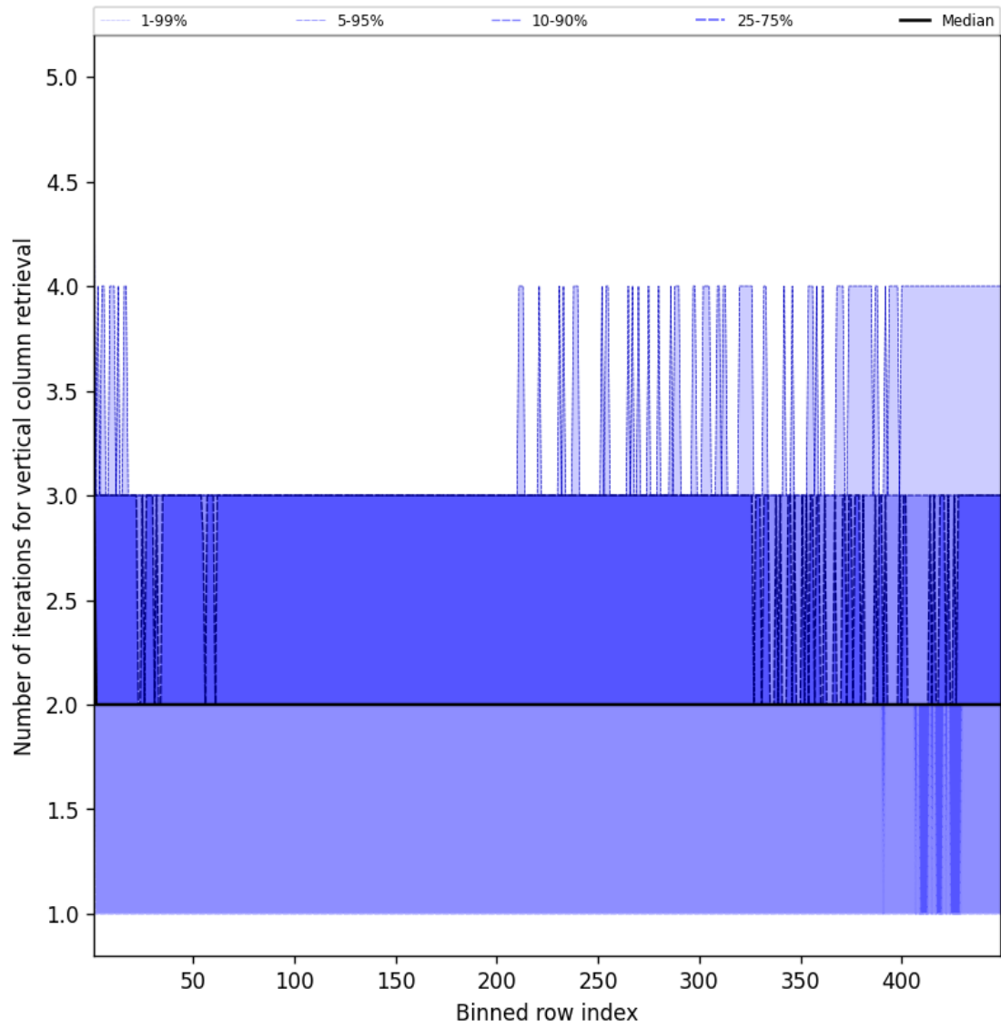
Figure 51: Along track statistics of “Number of iterations for vertical column retrieval” for 2025-10-28 to 2025-10-29
