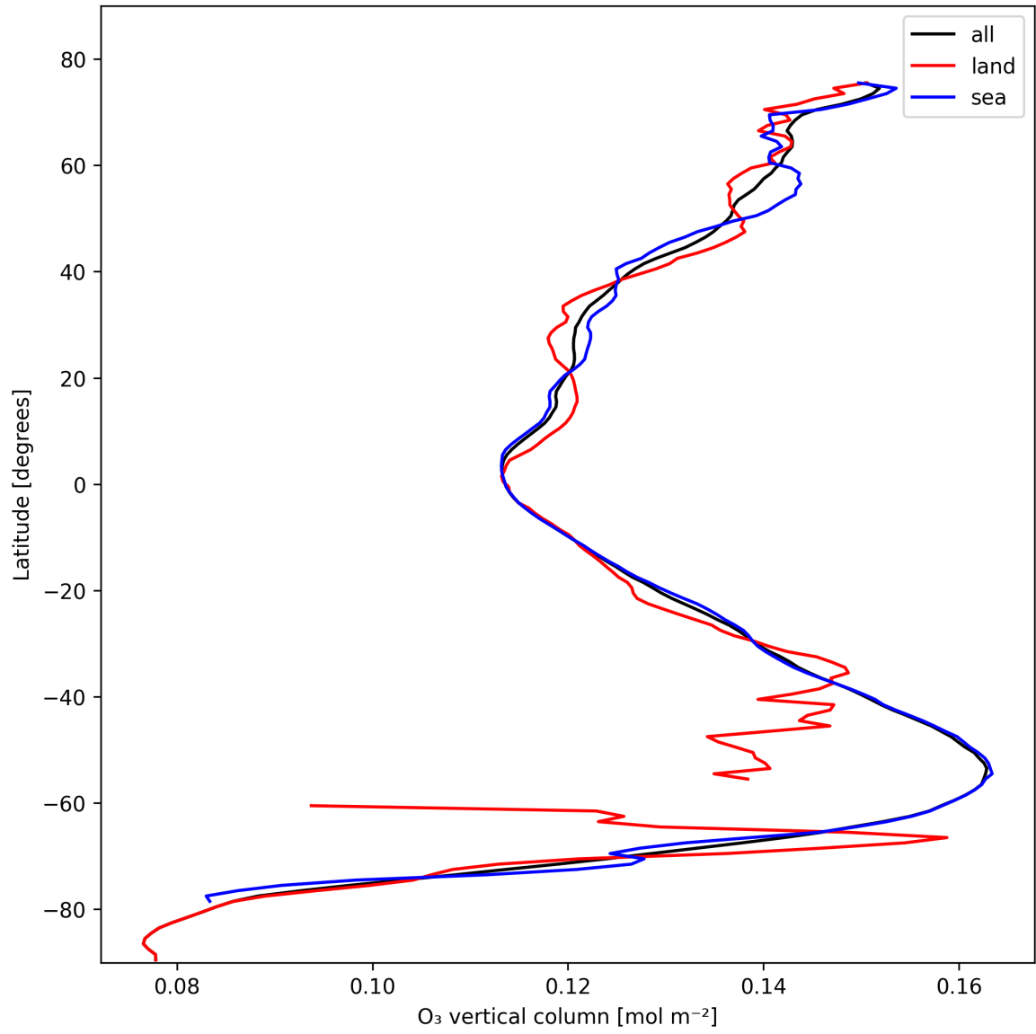
Figure 17: Zonal average of “O 3 vertical column” for 2025-10-28 to 2025-10-29.
