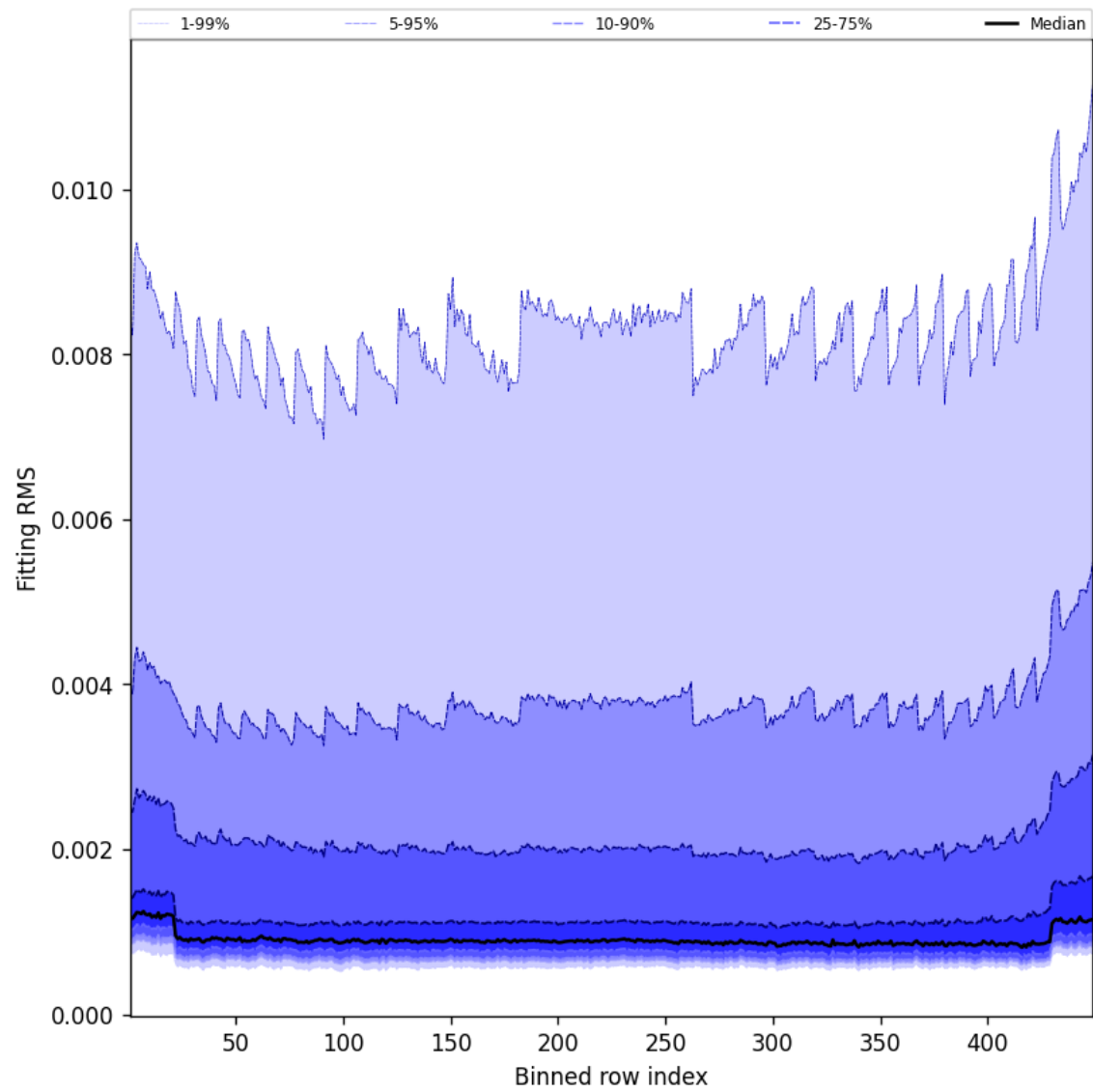
Figure 46: Along track statistics of “Fitting RMS” for 2025-10-28 to 2025-10-29
