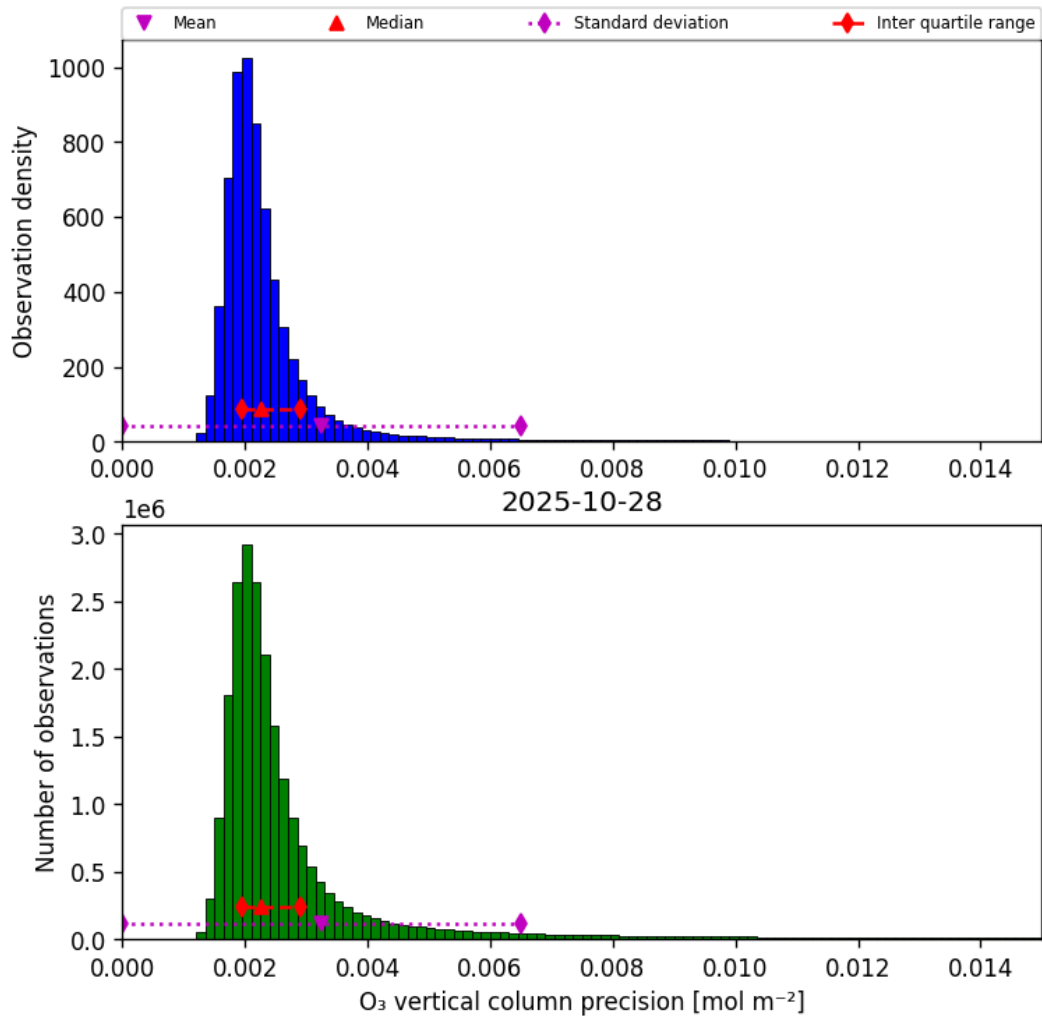
Figure 30: Histogram of “O 3 vertical column precision” for 2025-10-28 to 2025-10-29
