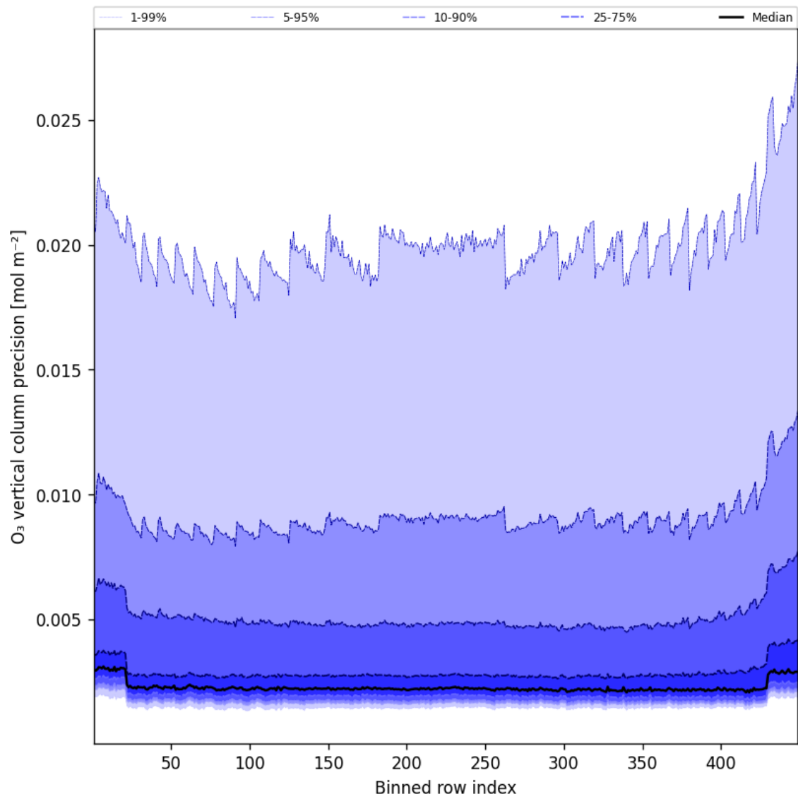
Figure 42: Along track statistics of “O 3 vertical column precision” for 2025-10-28 to 2025-10-29
