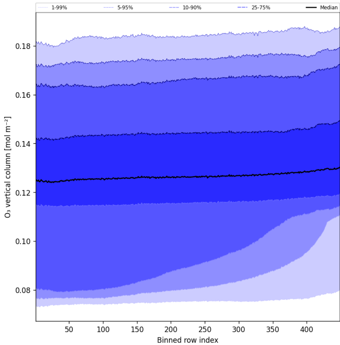
Figure 41: Along track statistics of “O 3 vertical column” for 2025-10-28 to 2025-10-29
