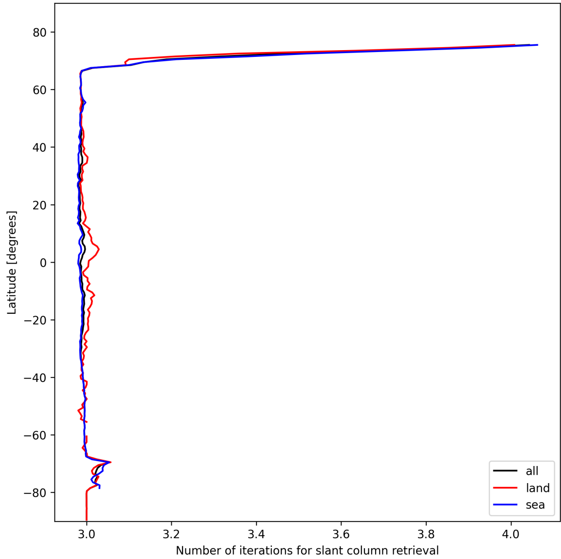
Figure 21: Zonal average of “Number of iterations for slant column retrieval” for 2025-10-28 to 2025-10-29.
