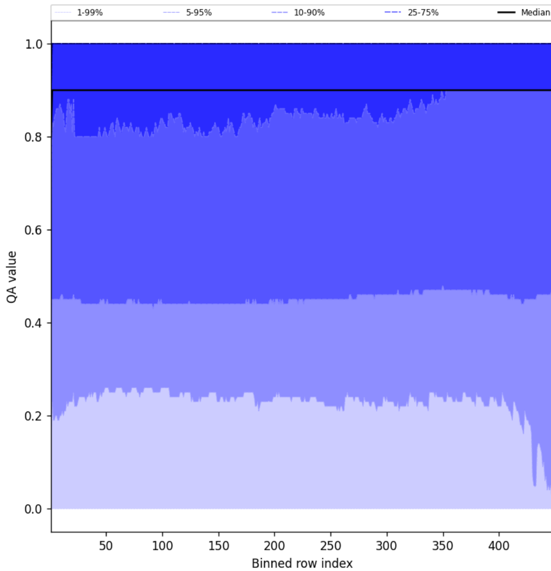
Figure 40: Along track statistics of “QA value” for 2025-10-28 to 2025-10-29
