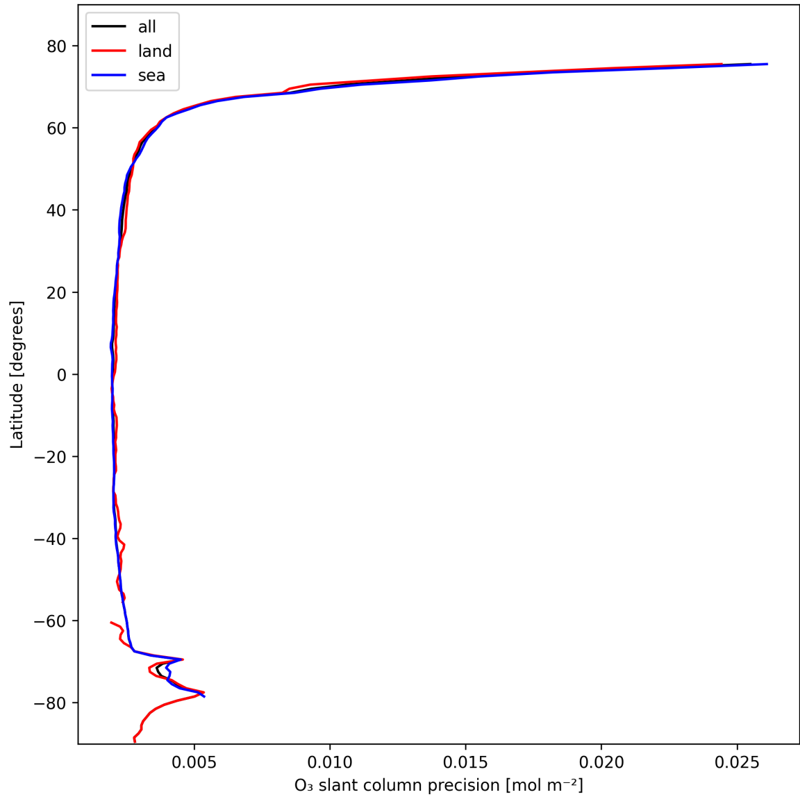
Figure 20: Zonal average of “O 3 slant column precision” for 2025-10-28 to 2025-10-29.
