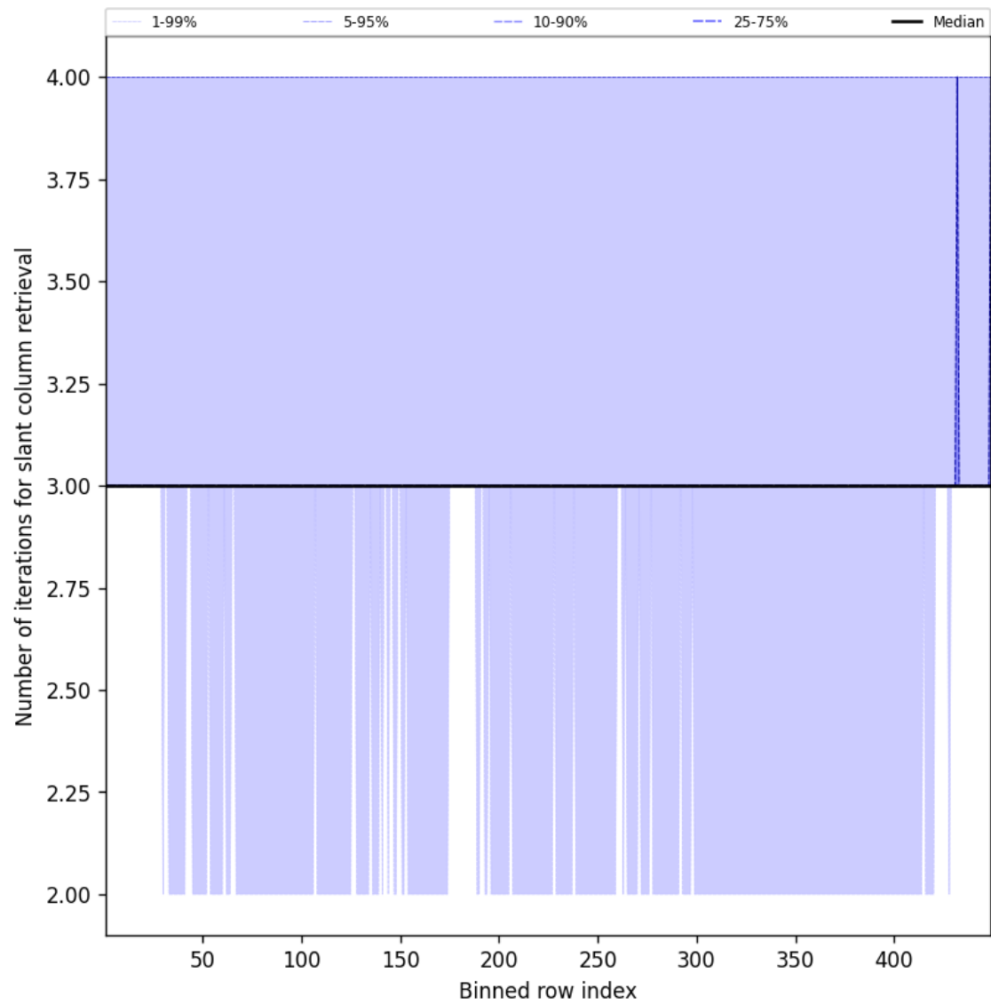
Figure 45: Along track statistics of “Number of iterations for slant column retrieval” for 2025-10-28 to 2025-10-29
