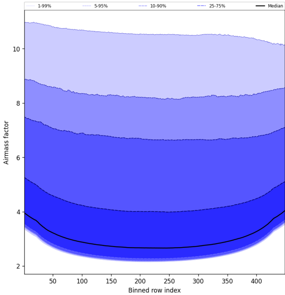
Figure 49: Along track statistics of “Airmass factor” for 2025-10-28 to 2025-10-29
