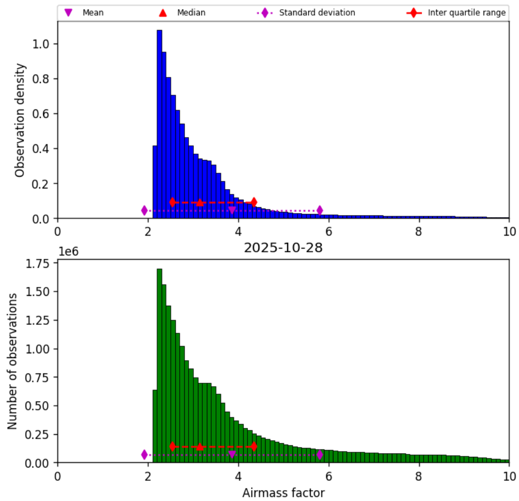
Figure 37: Histogram of “Airmass factor” for 2025-10-28 to 2025-10-29
