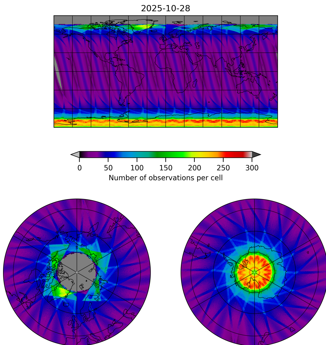
Figure 15: Map of the number of observations for 2025-10-28 to 2025-10-29
