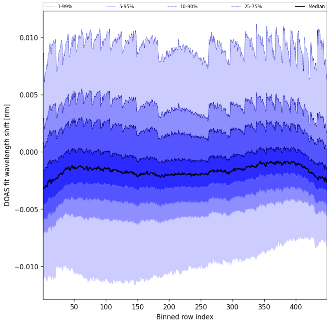
Figure 47: Along track statistics of “DOAS fit wavelength shift” for 2025-10-28 to 2025-10-29
