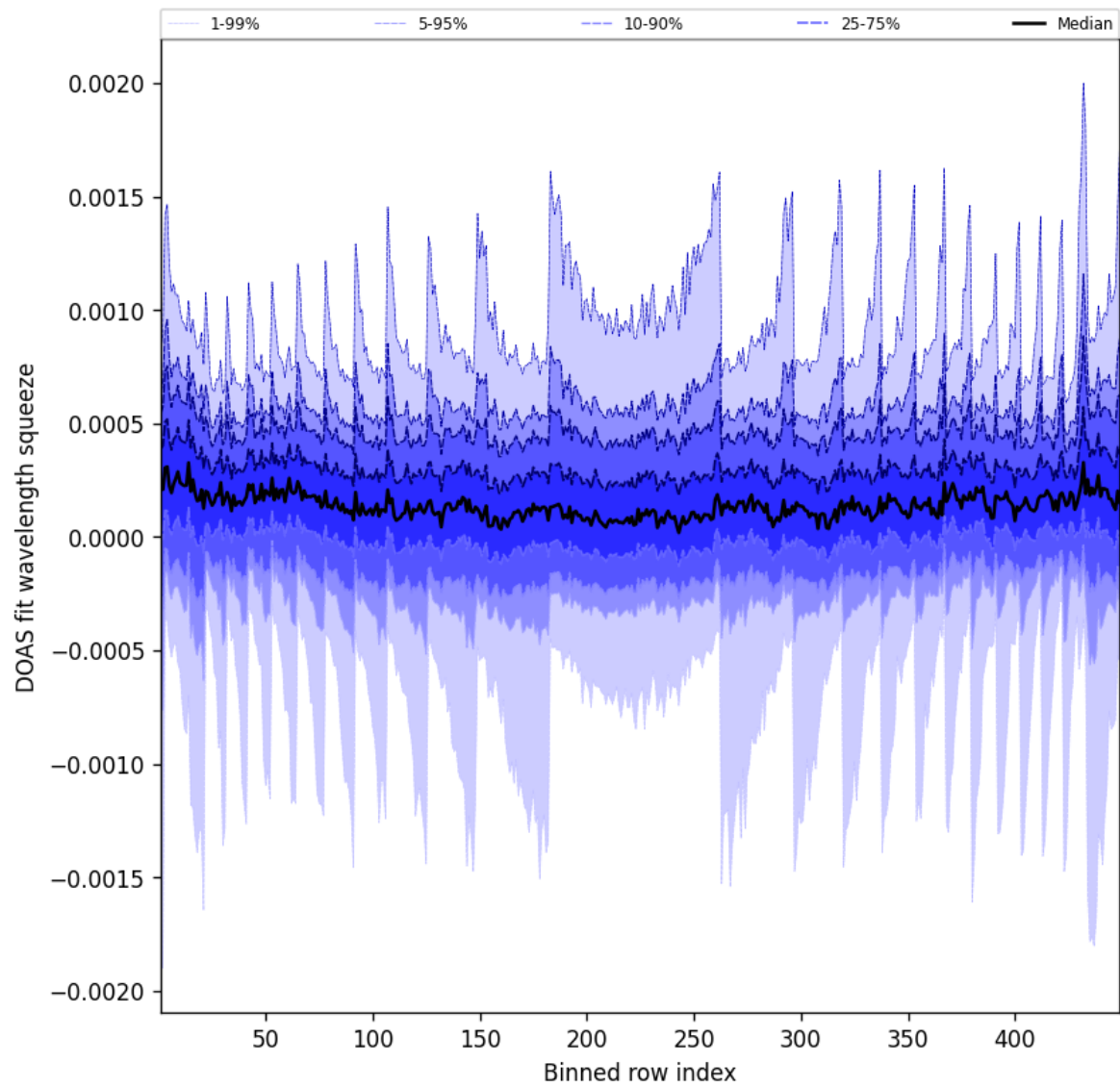
Figure 48: Along track statistics of “DOAS fit wavelength squeeze” for 2025-10-28 to 2025-10-29
