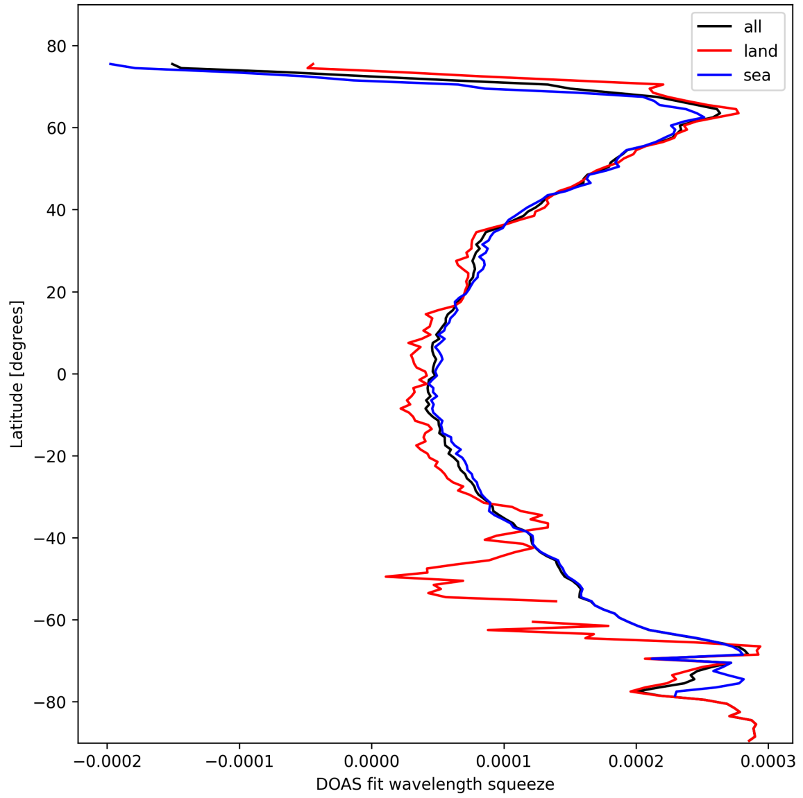
Figure 24: Zonal average of “DOAS fit wavelength squeeze” for 2025-10-28 to 2025-10-29.
