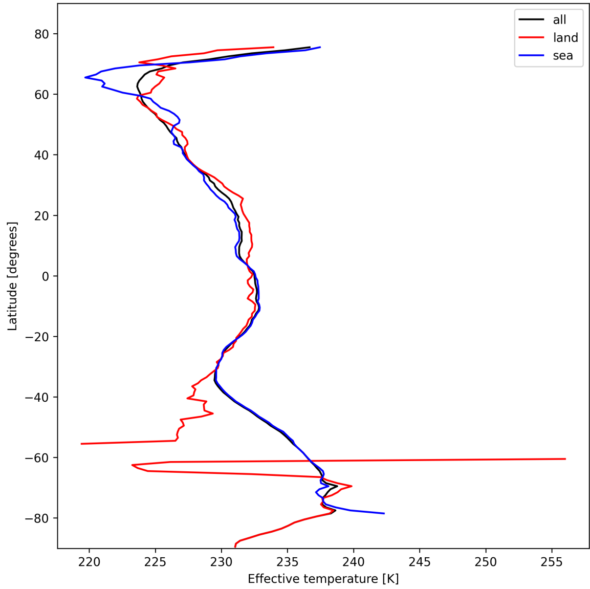
Figure 26: Zonal average of “Effective temperature” for 2025-10-28 to 2025-10-29.
