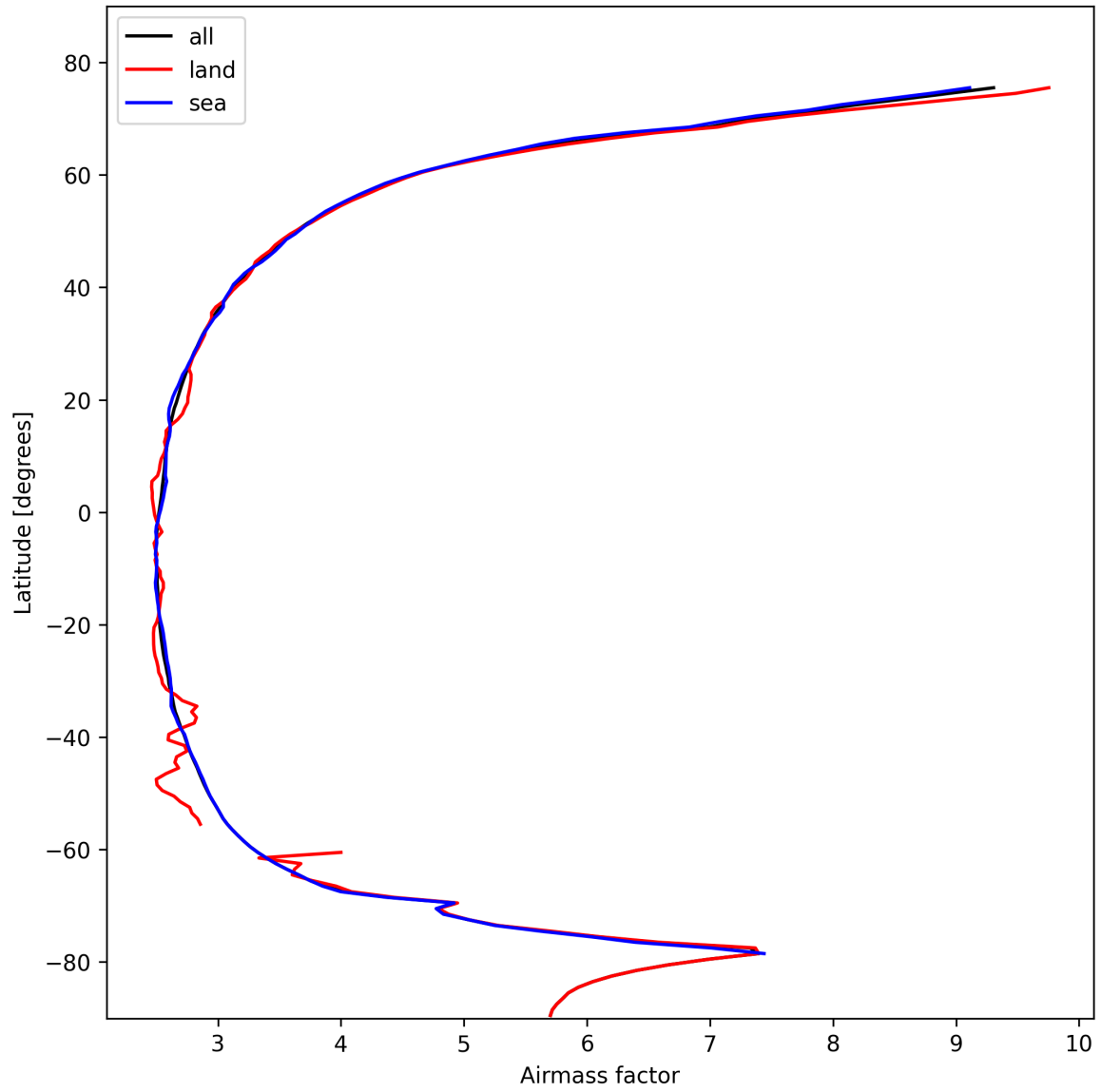
Figure 25: Zonal average of “Airmass factor” for 2025-10-28 to 2025-10-29.
