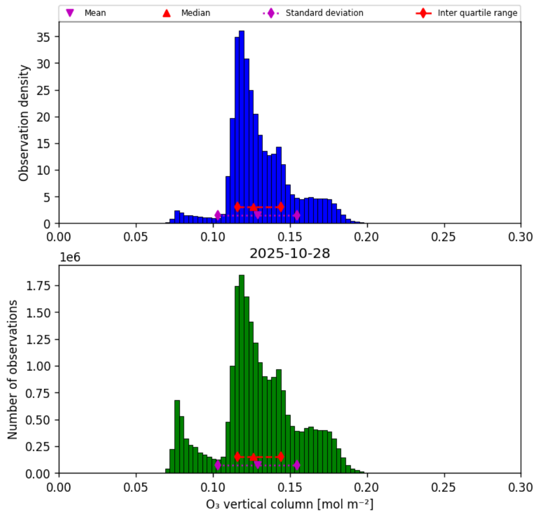
Figure 29: Histogram of “O 3 vertical column” for 2025-10-28 to 2025-10-29
