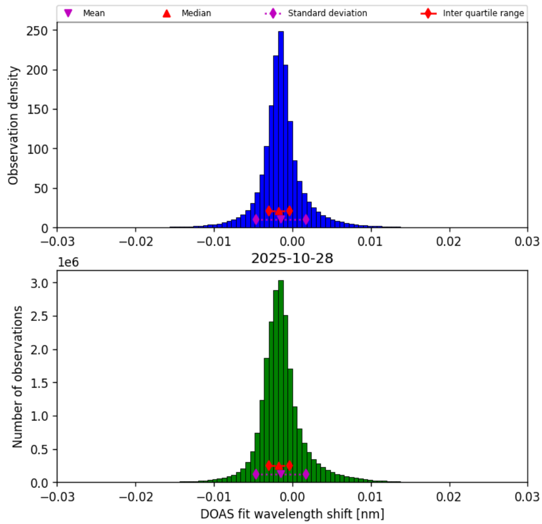
Figure 35: Histogram of “DOAS fit wavelength shift” for 2025-10-28 to 2025-10-29
