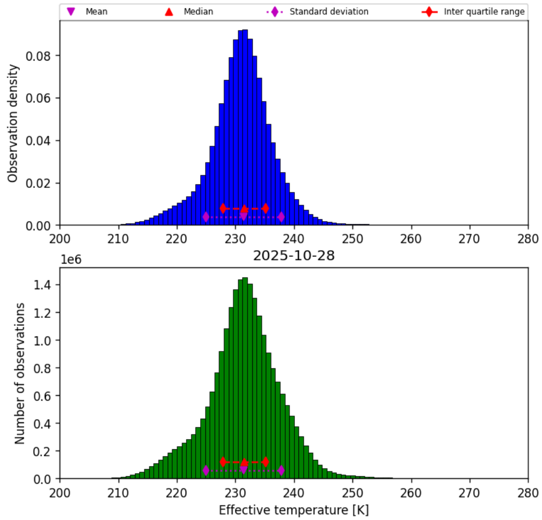
Figure 38: Histogram of “Effective temperature” for 2025-10-28 to 2025-10-29
