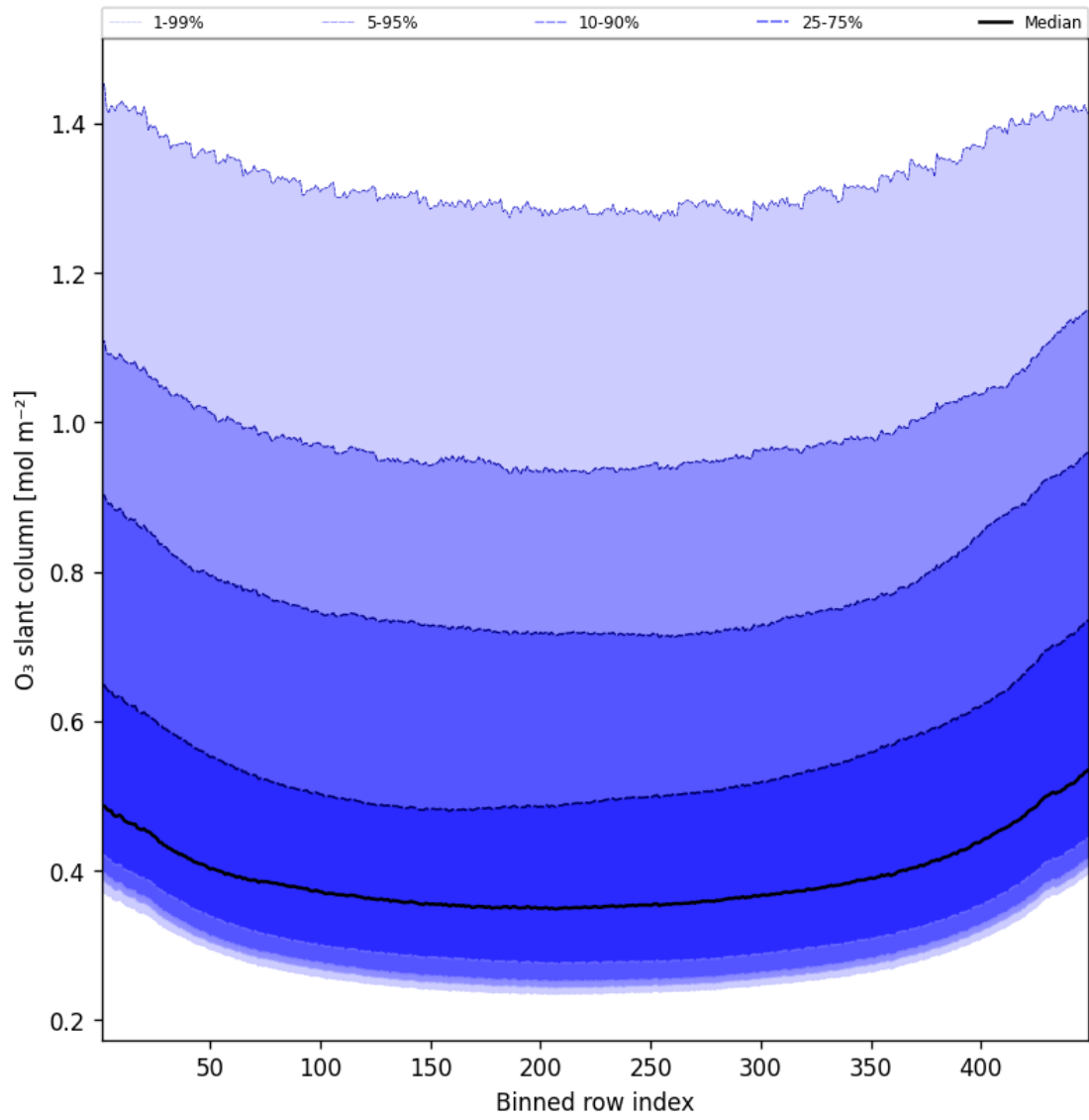
Figure 43: Along track statistics of “O 3 slant column” for 2025-10-30 to 2025-10-30
