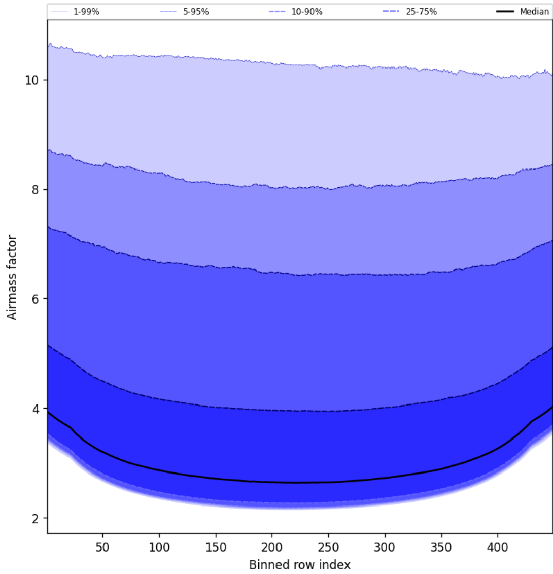
Figure 49: Along track statistics of “Airmass factor” for 2025-10-30 to 2025-10-30
