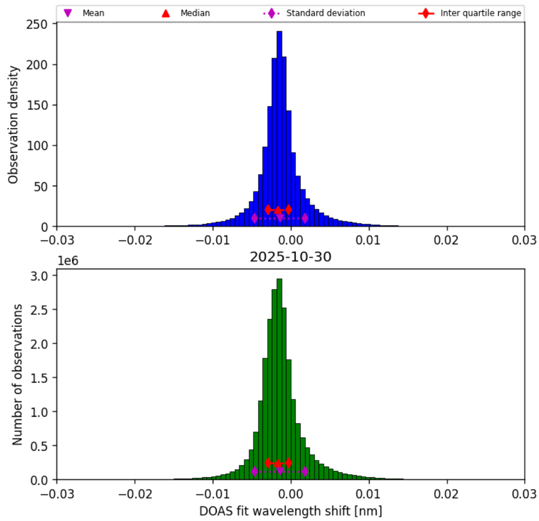
Figure 35: Histogram of “DOAS fit wavelength shift” for 2025-10-30 to 2025-10-30
