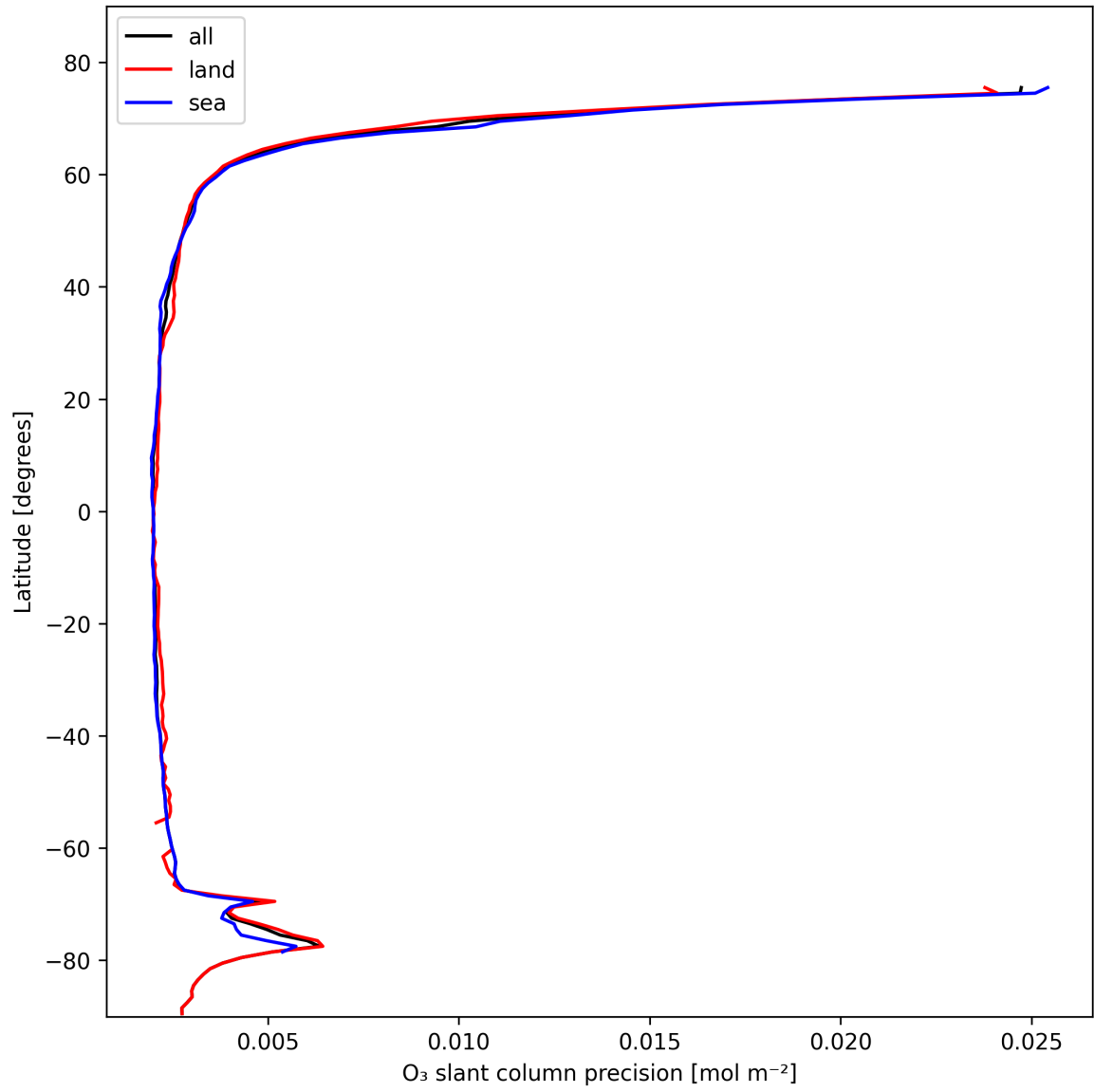
Figure 20: Zonal average of “O 3 slant column precision” for 2025-10-30 to 2025-10-30.
