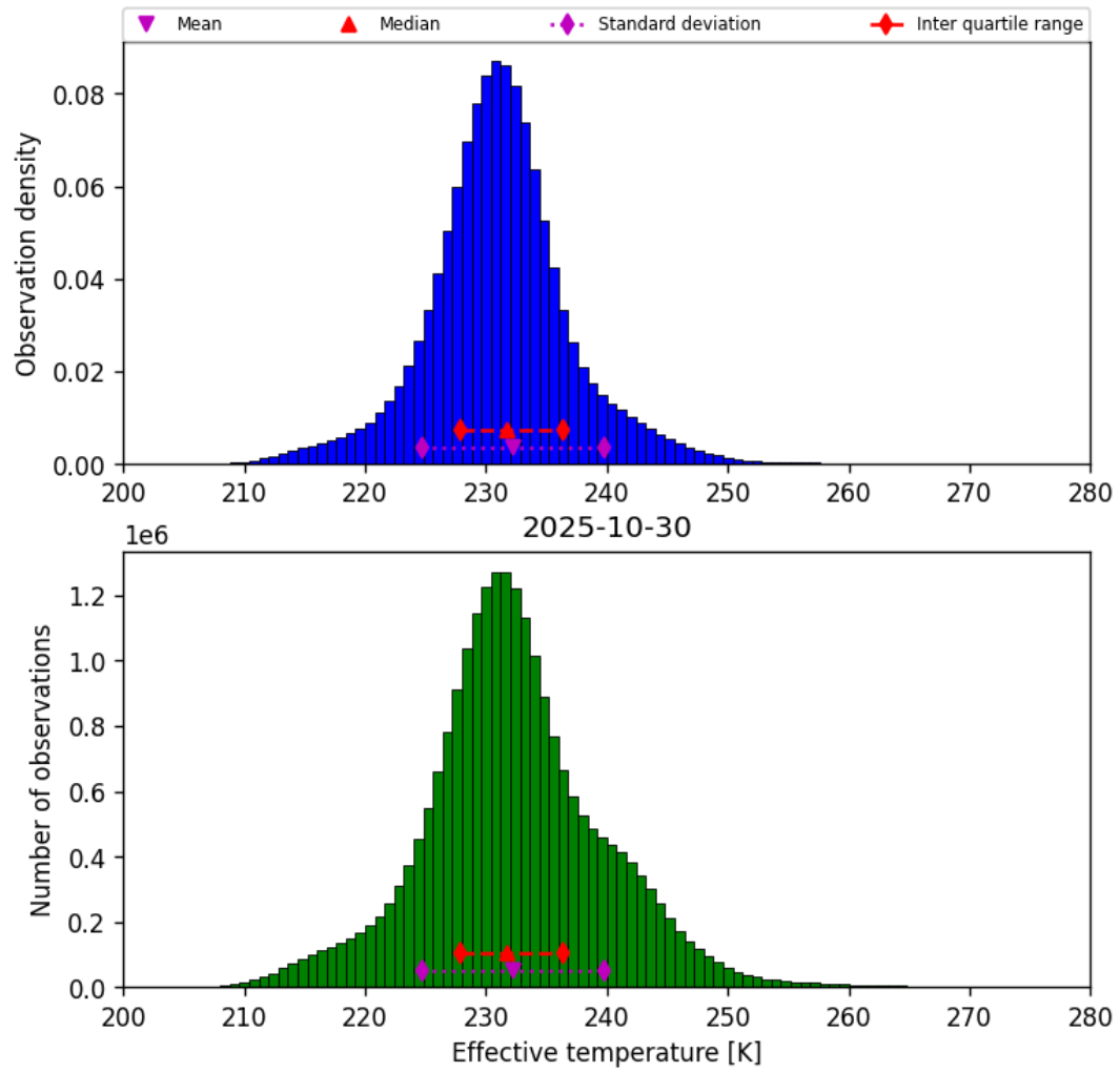
Figure 38: Histogram of “Effective temperature” for 2025-10-30 to 2025-10-30
