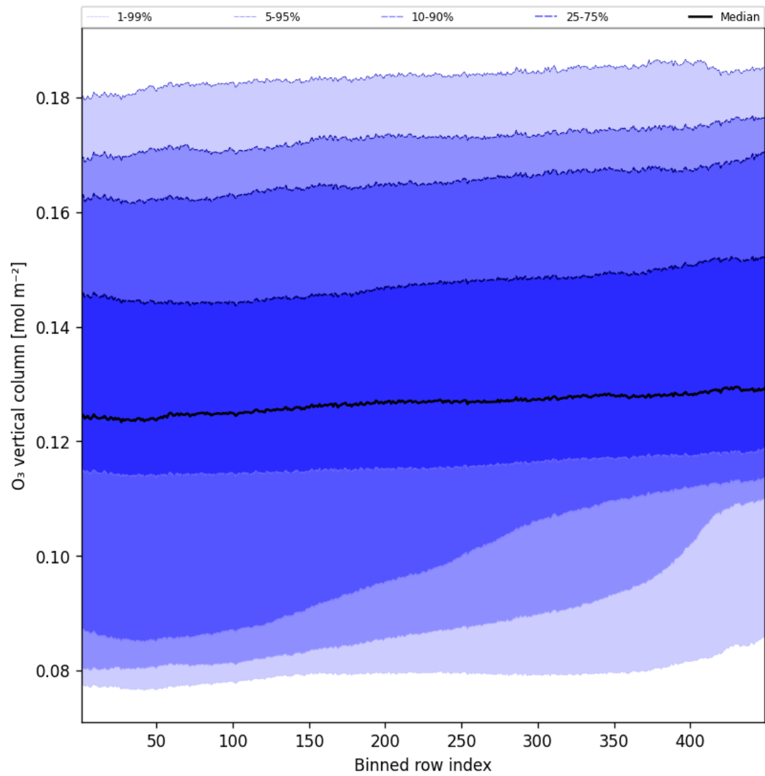
Figure 41: Along track statistics of “O 3 vertical column” for 2025-10-30 to 2025-10-30
