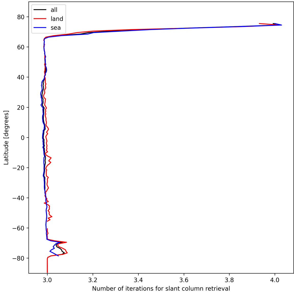
Figure 21: Zonal average of “Number of iterations for slant column retrieval” for 2025-10-30 to 2025-10-30.
