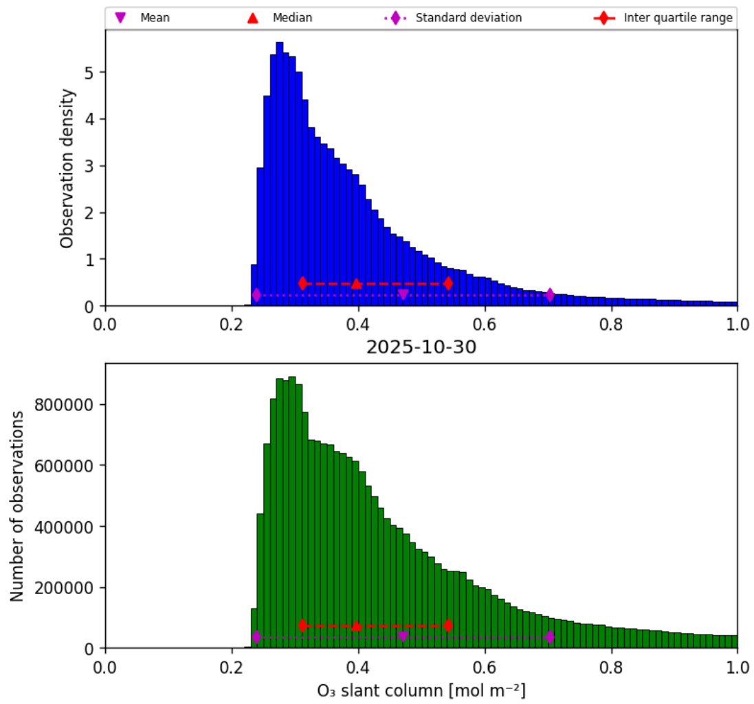
Figure 31: Histogram of “O 3 slant column” for 2025-10-30 to 2025-10-30
