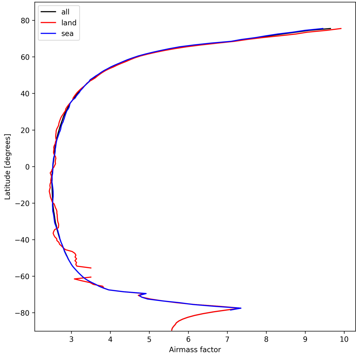
Figure 25: Zonal average of “Airmass factor” for 2025-10-30 to 2025-10-30.
