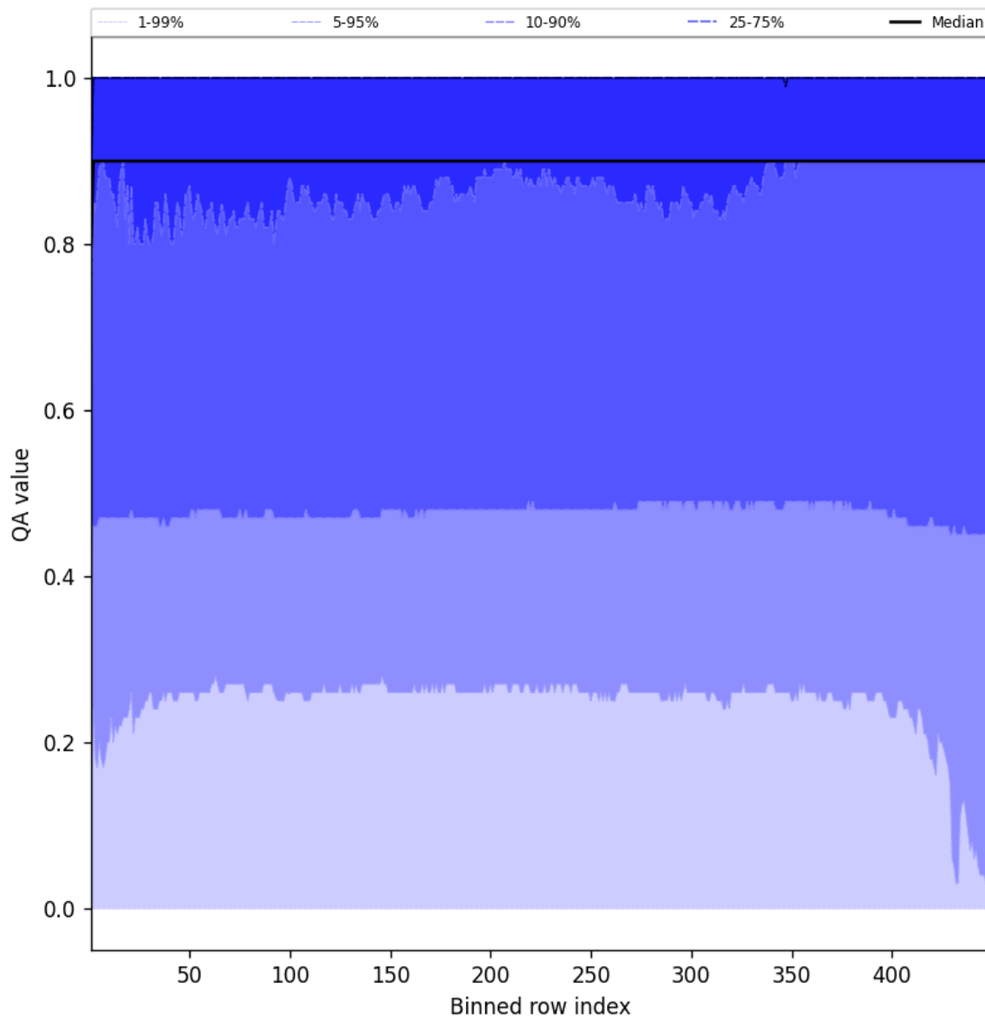
Figure 40: Along track statistics of “QA value” for 2025-10-30 to 2025-10-30
