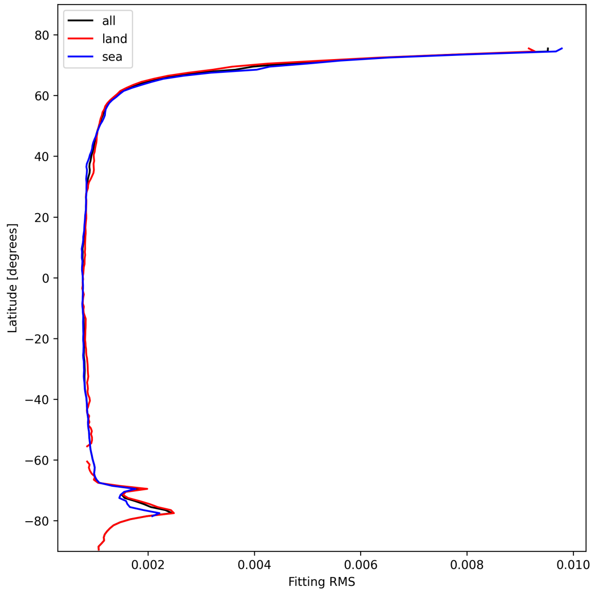
Figure 22: Zonal average of “Fitting RMS” for 2025-10-30 to 2025-10-30.
