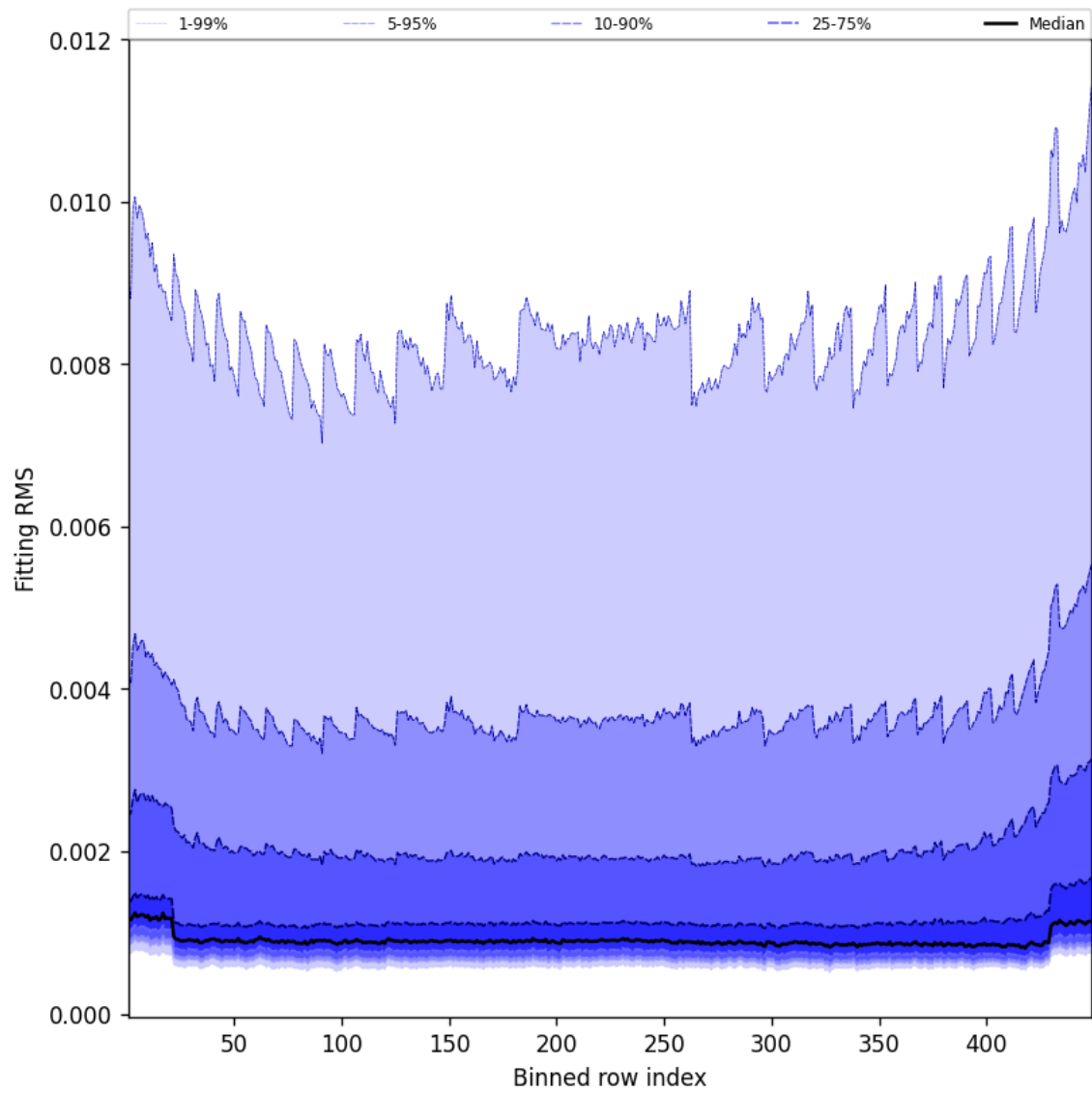
Figure 46: Along track statistics of “Fitting RMS” for 2025-10-30 to 2025-10-30
