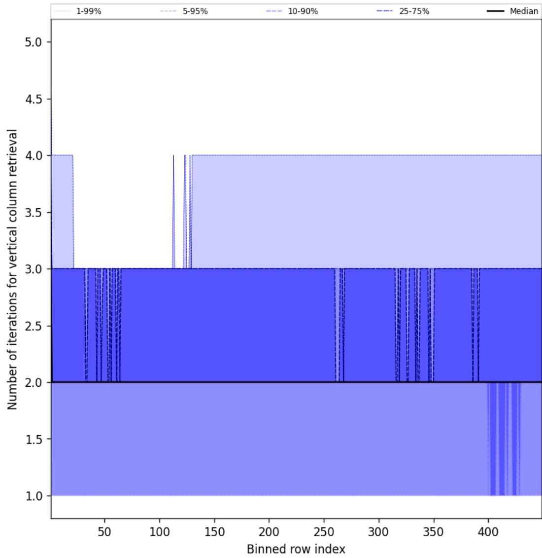
Figure 51: Along track statistics of “Number of iterations for vertical column retrieval” for 2025-10-30 to 2025-10-30
