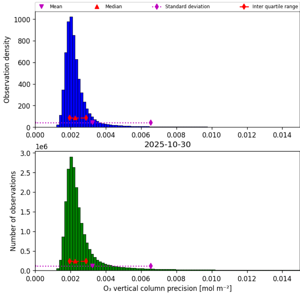
Figure 30: Histogram of “O 3 vertical column precision” for 2025-10-30 to 2025-10-30
