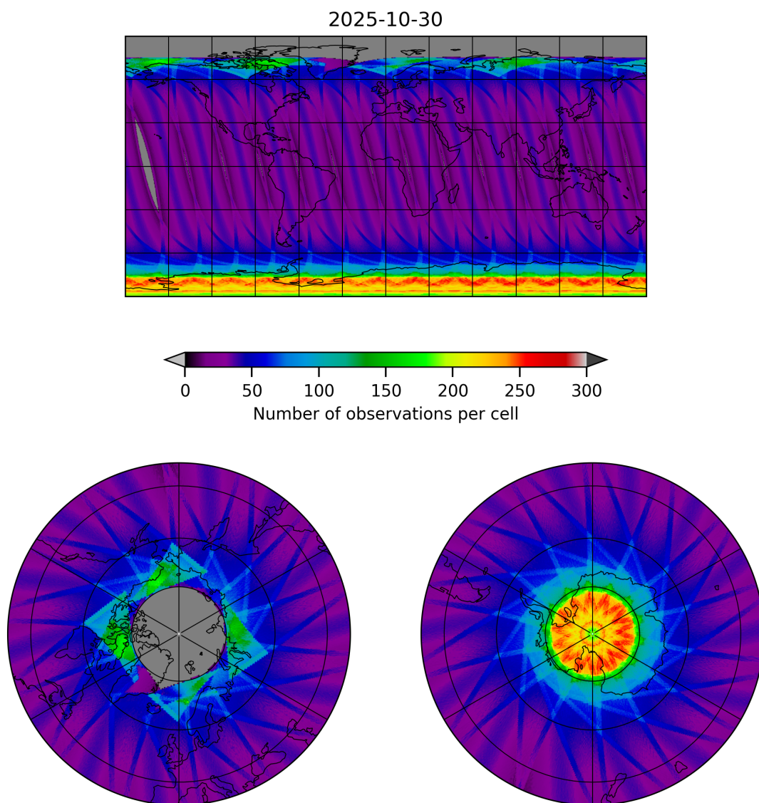
Figure 15: Map of the number of observations for 2025-10-30 to 2025-10-30
