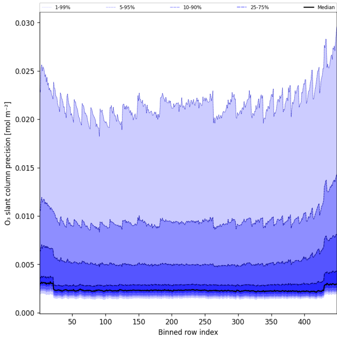
Figure 44: Along track statistics of “O 3 slant column precision” for 2025-10-30 to 2025-10-30
