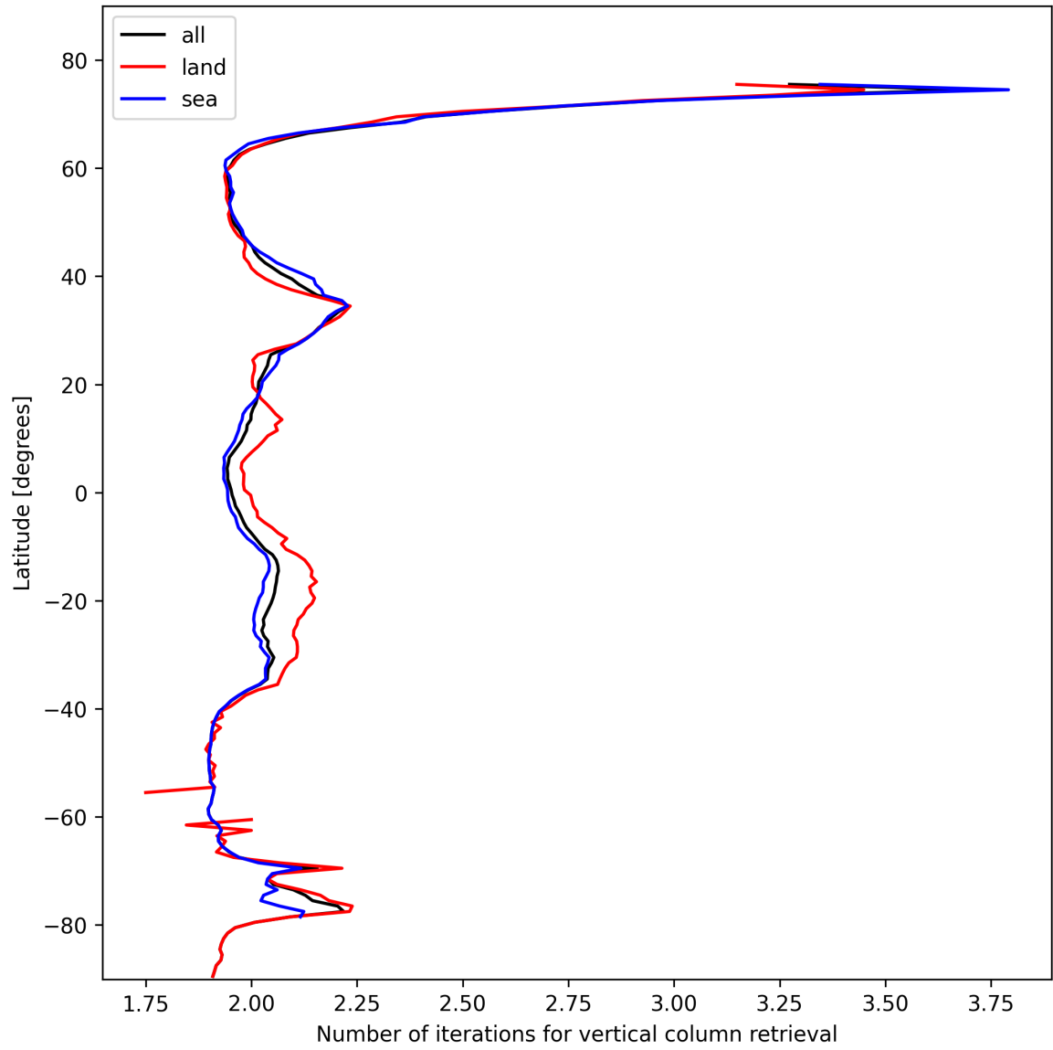
Figure 27: Zonal average of “Number of iterations for vertical column retrieval” for 2025-10-30 to 2025-10-30.
