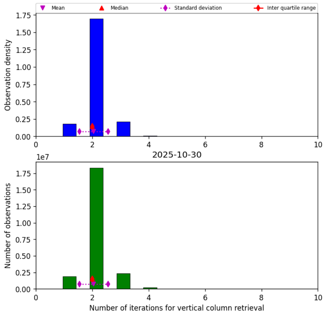
Figure 39: Histogram of “Number of iterations for vertical column retrieval” for 2025-10-30 to 2025-10-30
