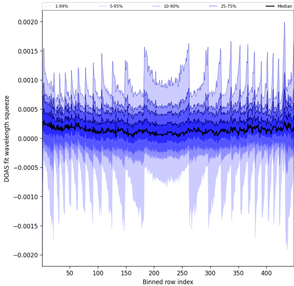
Figure 48: Along track statistics of “DOAS fit wavelength squeeze” for 2025-10-30 to 2025-10-30
