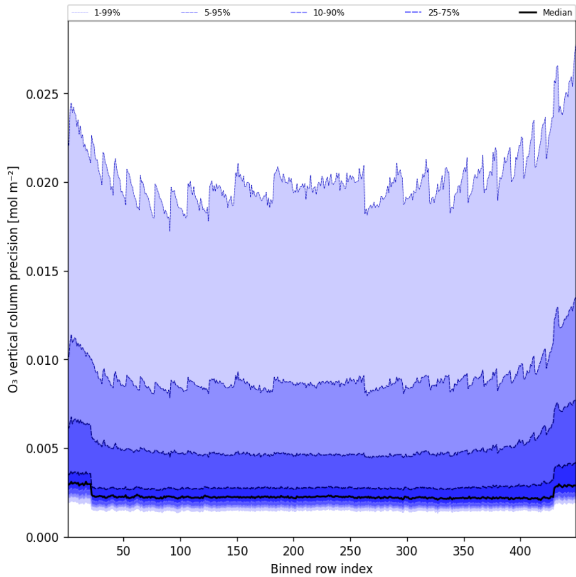
Figure 42: Along track statistics of “O 3 vertical column precision” for 2025-10-30 to 2025-10-30
