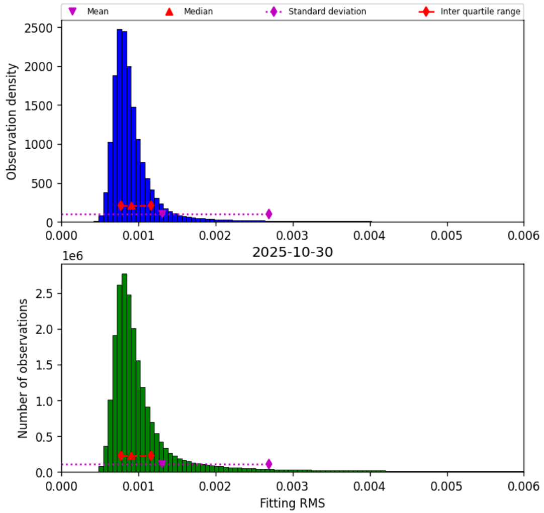
Figure 34: Histogram of “Fitting RMS” for 2025-10-30 to 2025-10-30
