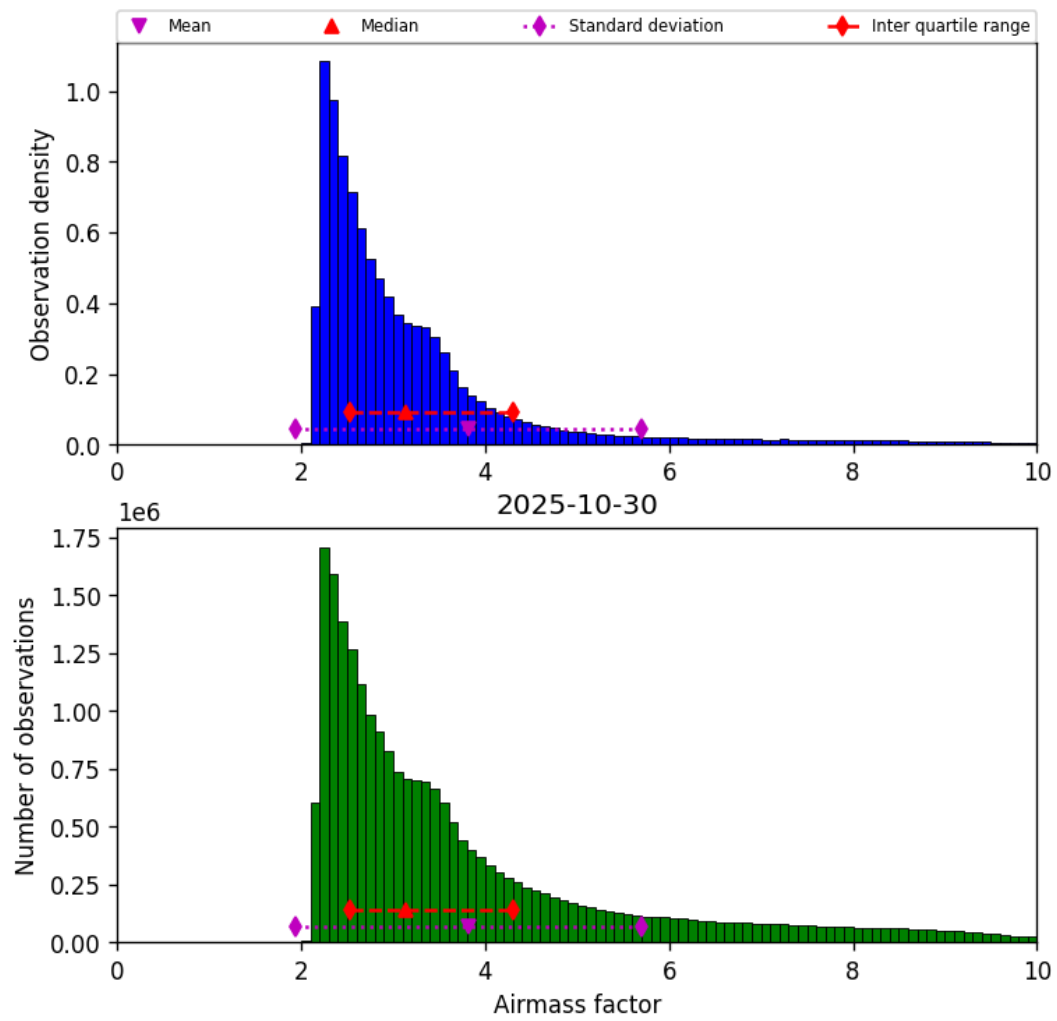
Figure 37: Histogram of “Airmass factor” for 2025-10-30 to 2025-10-30
