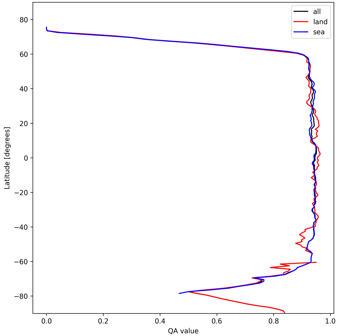
Figure 16: Zonal average of “QA value” for 2025-10-30 to 2025-10-30.
