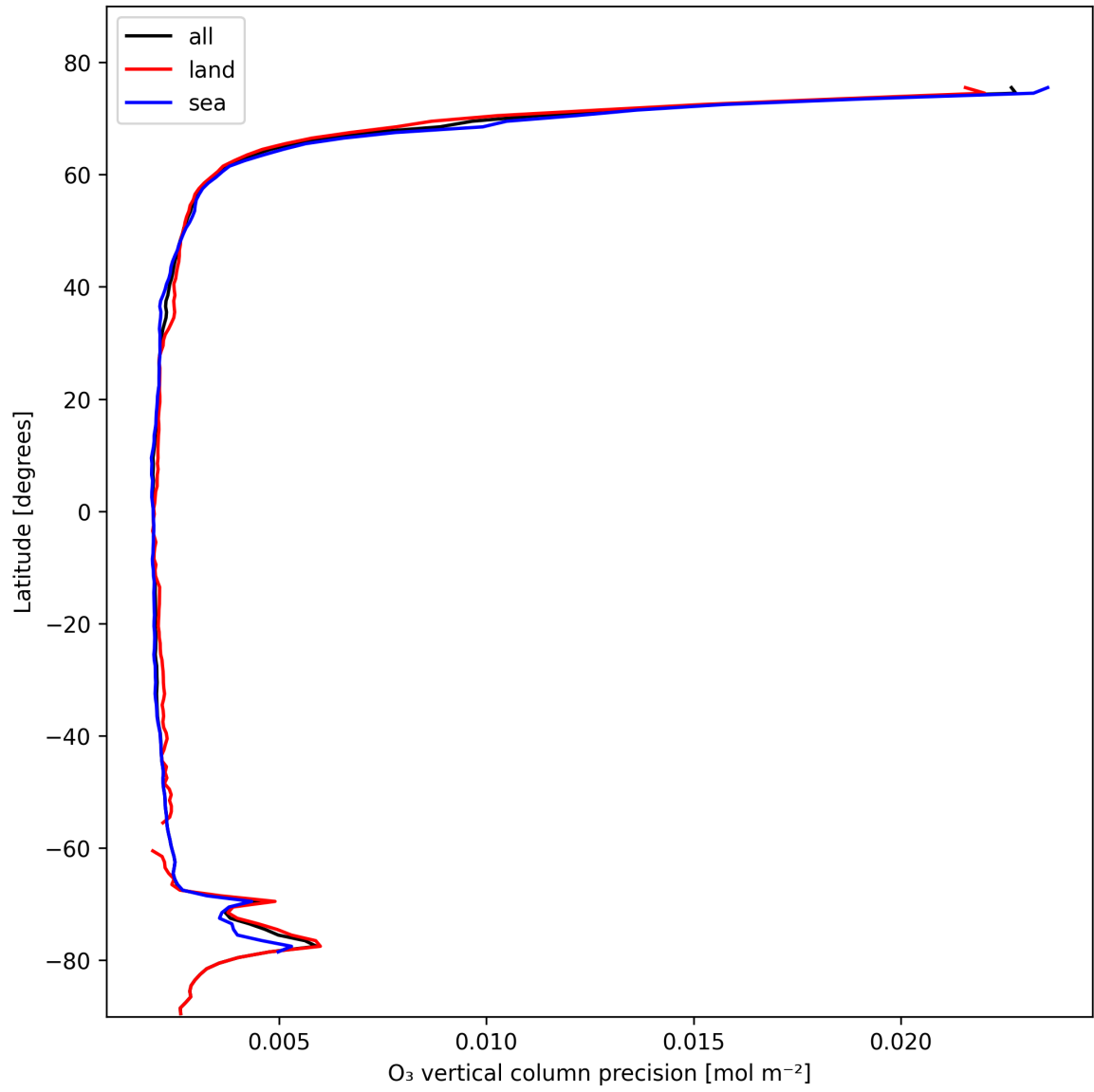
Figure 18: Zonal average of “O 3 vertical column precision” for 2025-10-30 to 2025-10-30.
