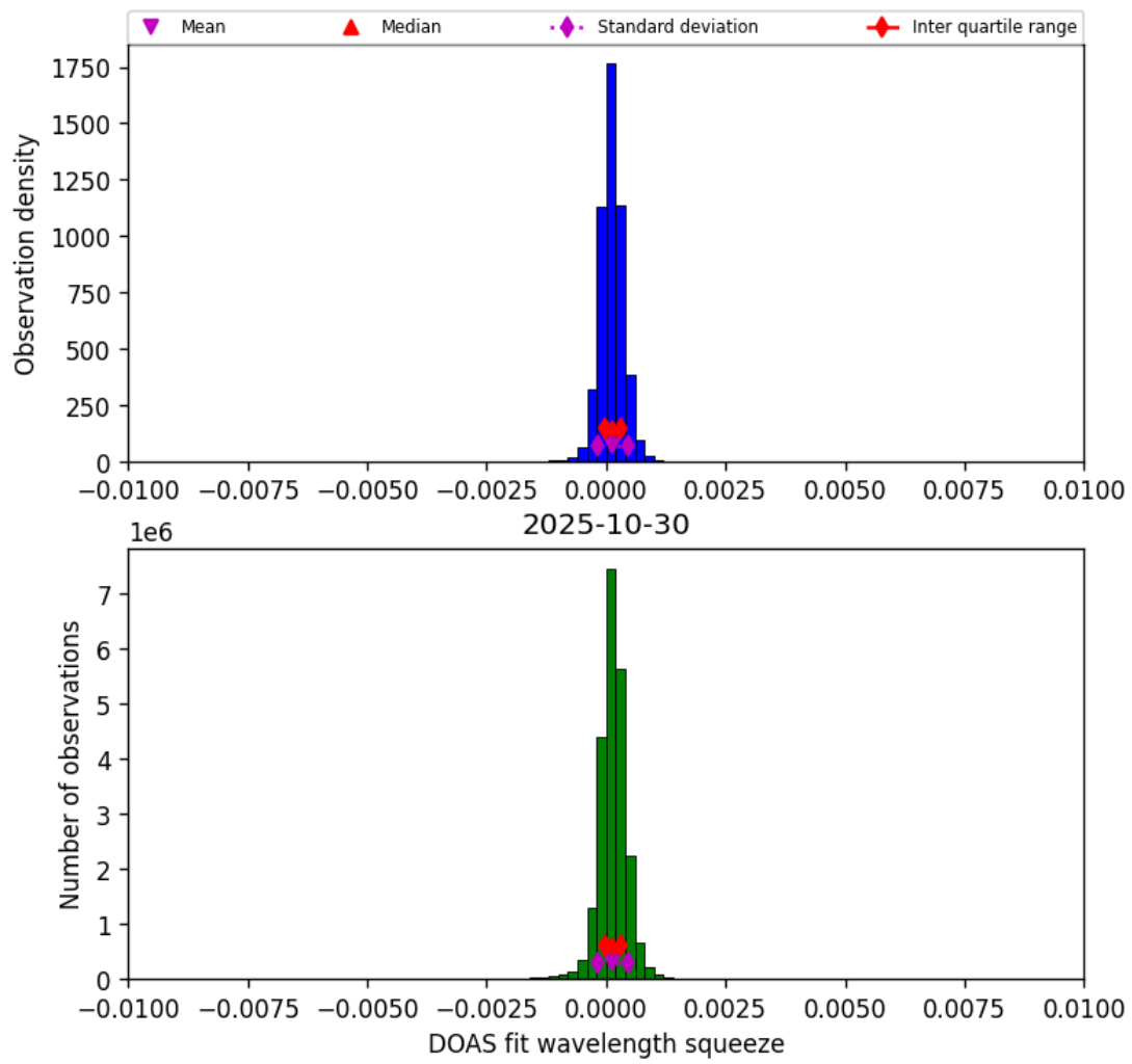
Figure 36: Histogram of “DOAS fit wavelength squeeze” for 2025-10-30 to 2025-10-30
