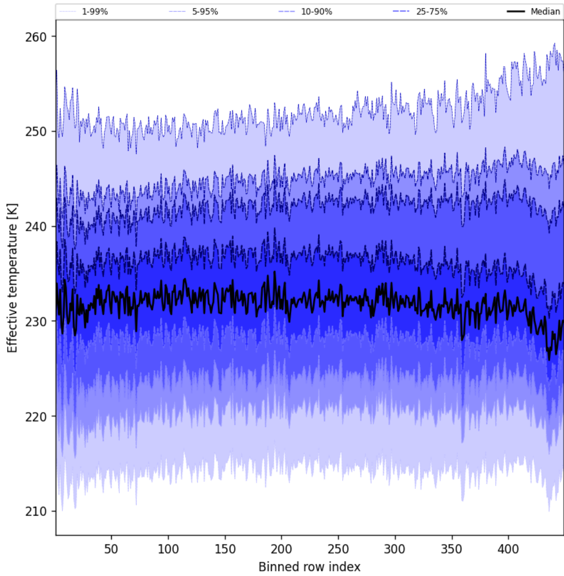
Figure 50: Along track statistics of “Effective temperature” for 2025-10-30 to 2025-10-30
