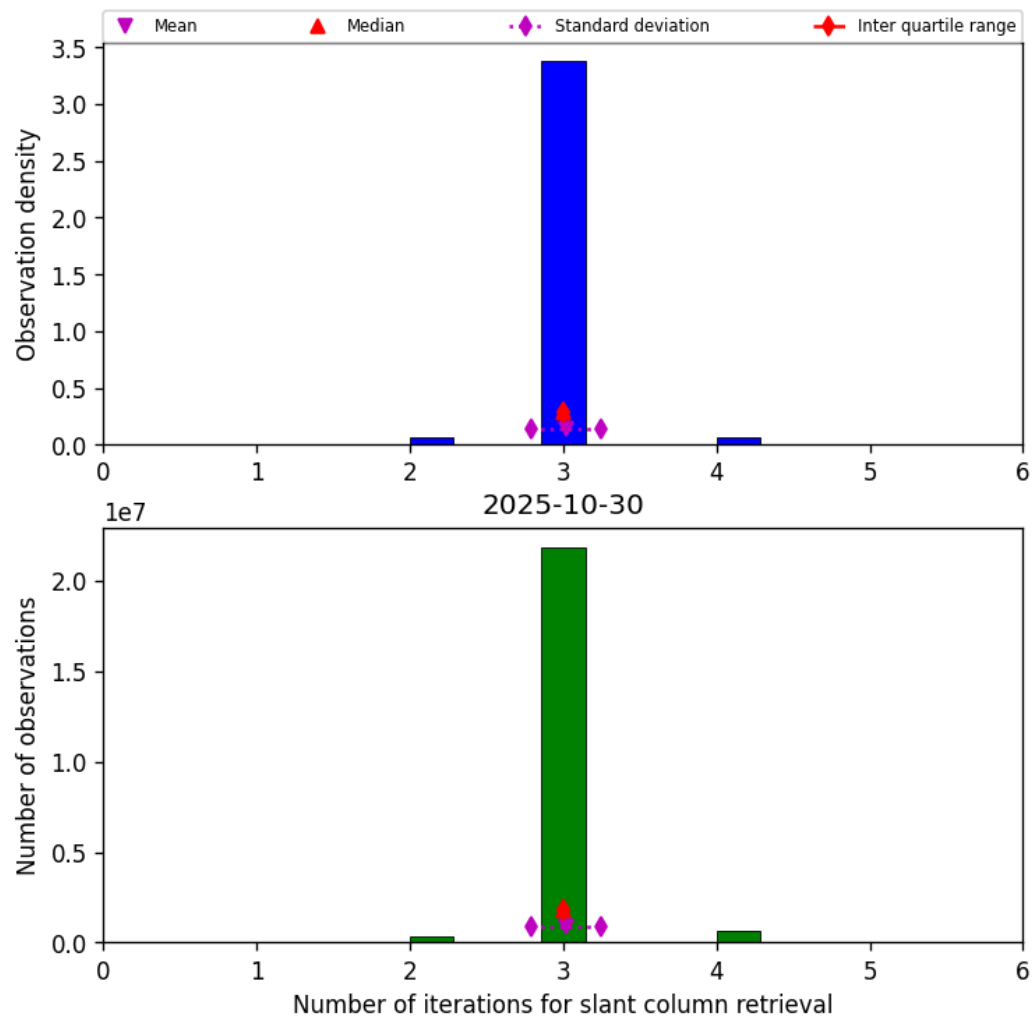
Figure 33: Histogram of “Number of iterations for slant column retrieval” for 2025-10-30 to 2025-10-30
