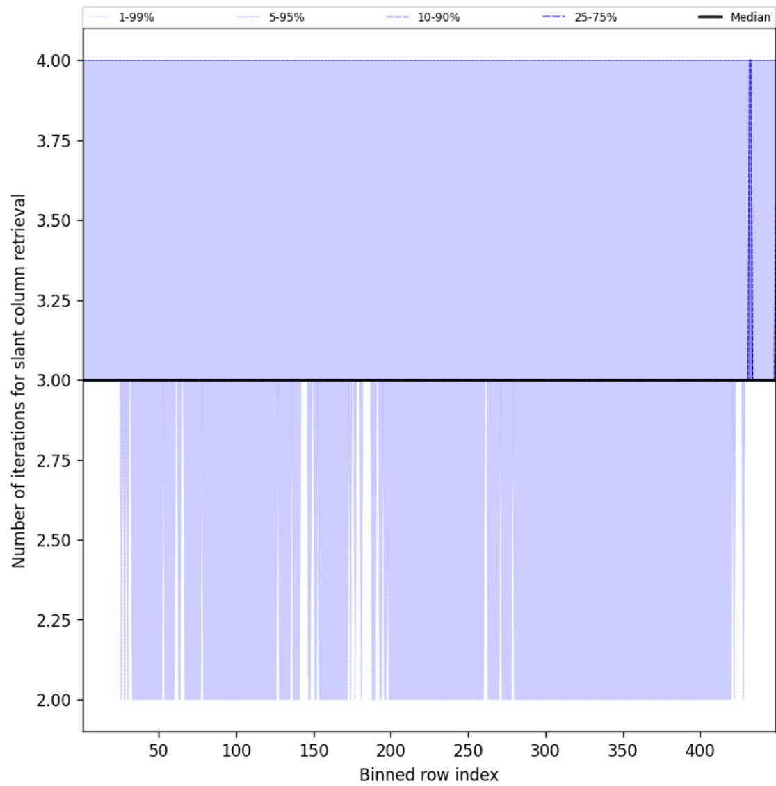
Figure 45: Along track statistics of “Number of iterations for slant column retrieval” for 2025-10-30 to 2025-10-30
