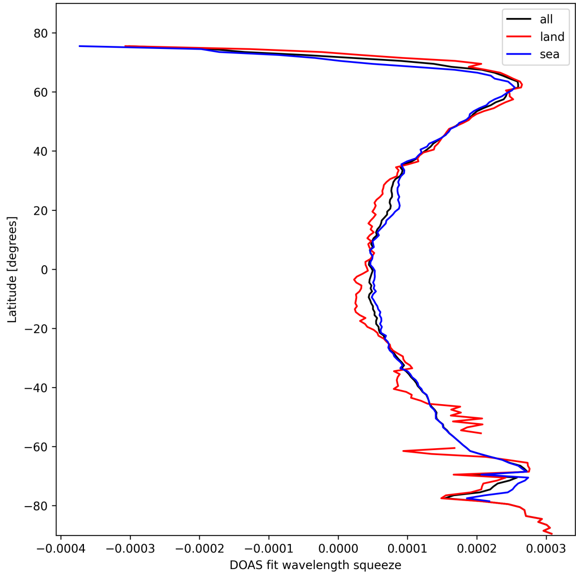
Figure 24: Zonal average of “DOAS fit wavelength squeeze” for 2025-10-30 to 2025-10-30.
