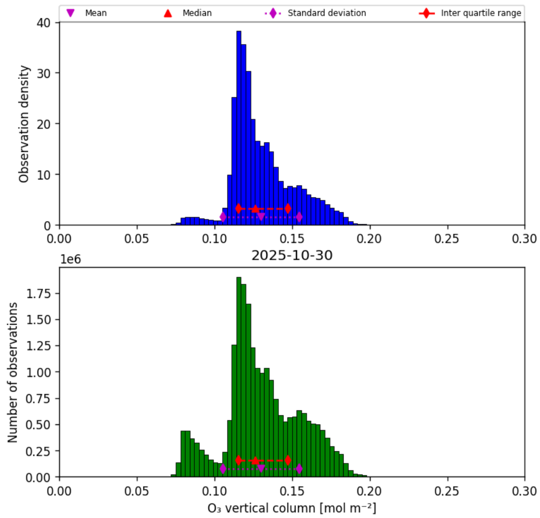
Figure 29: Histogram of “O 3 vertical column” for 2025-10-30 to 2025-10-30
