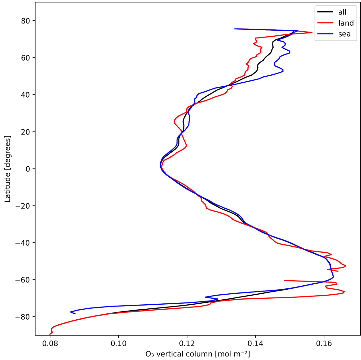
Figure 17: Zonal average of “O 3 vertical column” for 2025-10-30 to 2025-10-30.
