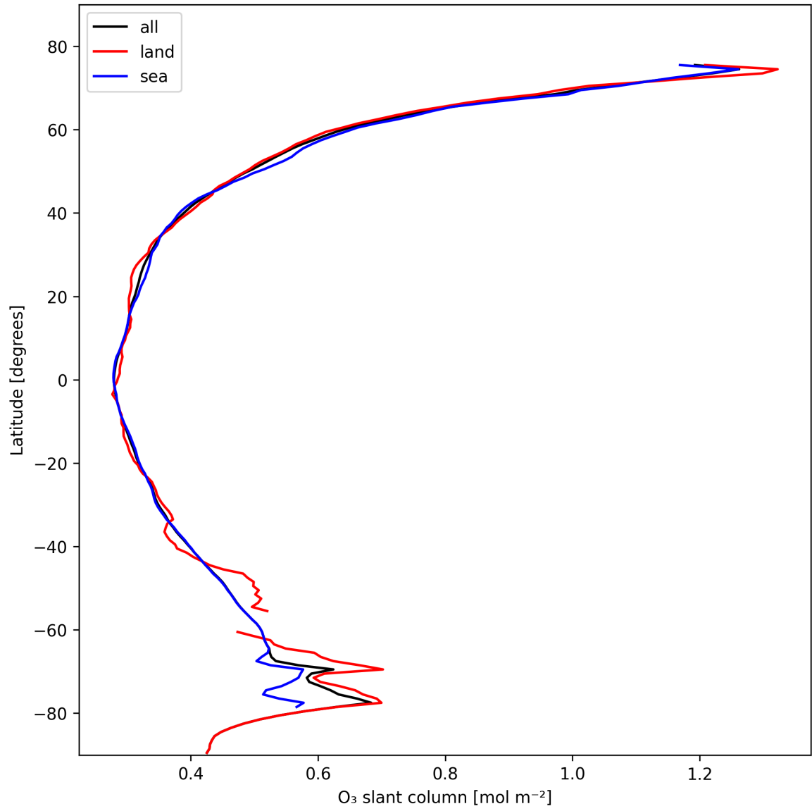
Figure 19: Zonal average of “O 3 slant column” for 2025-10-30 to 2025-10-30.
