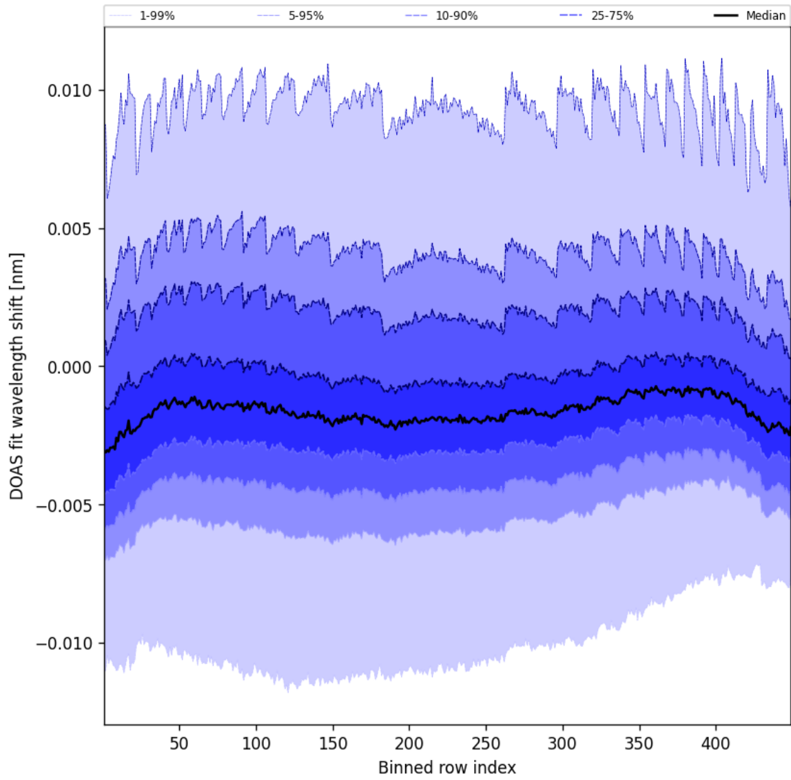
Figure 47: Along track statistics of “DOAS fit wavelength shift” for 2025-10-30 to 2025-10-30
