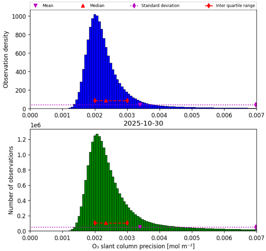
Figure 32: Histogram of “O 3 slant column precision” for 2025-10-30 to 2025-10-30
