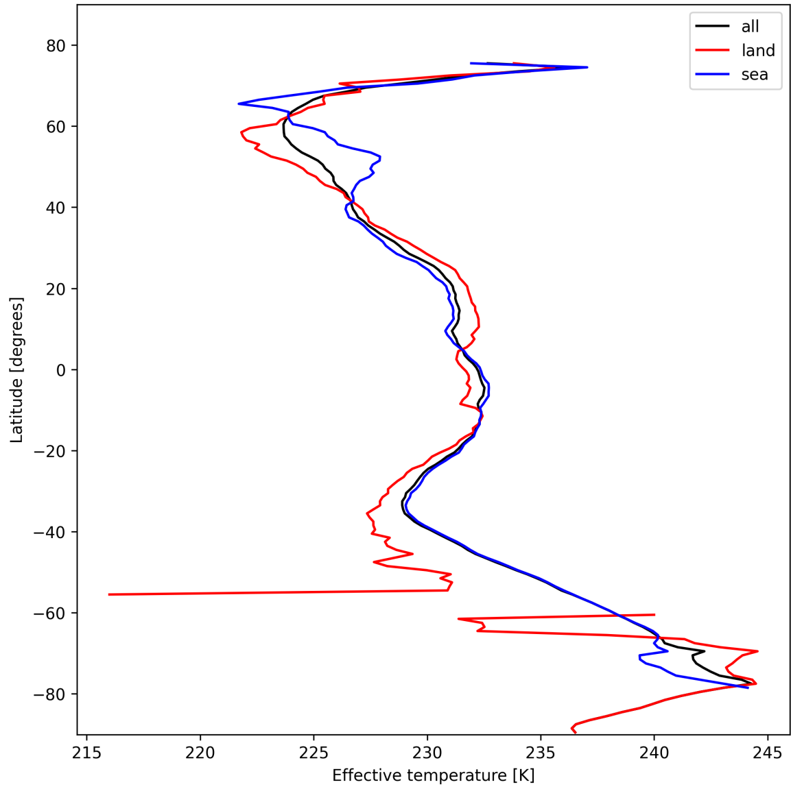
Figure 26: Zonal average of "Effective temperature" for 2025-10-30 to 2025-10-30.
