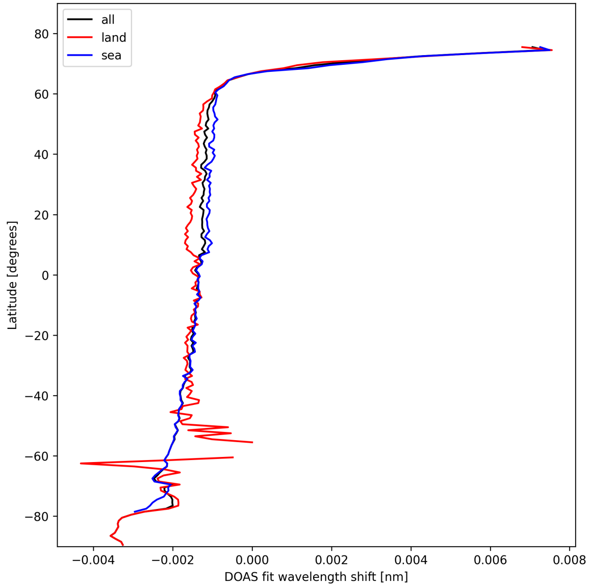
Figure 23: Zonal average of “DOAS fit wavelength shift” for 2025-10-30 to 2025-10-30.
