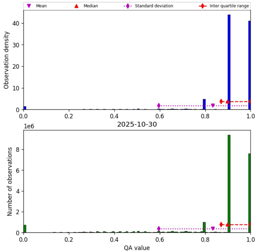
Figure 28: Histogram of “QA value” for 2025-10-30 to 2025-10-30
