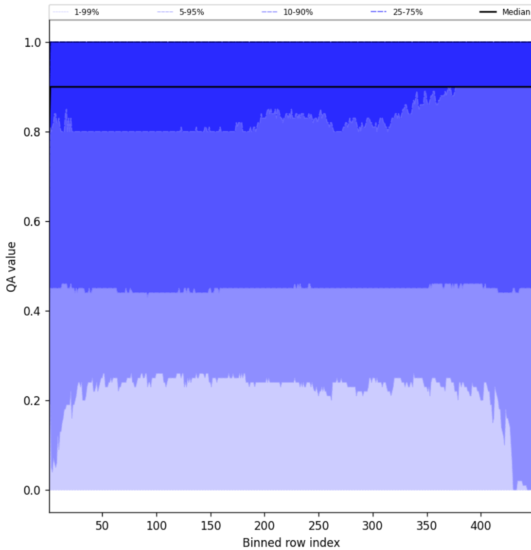
Figure 40: Along track statistics of “QA value” for 2025-10-31 to 2025-10-31
