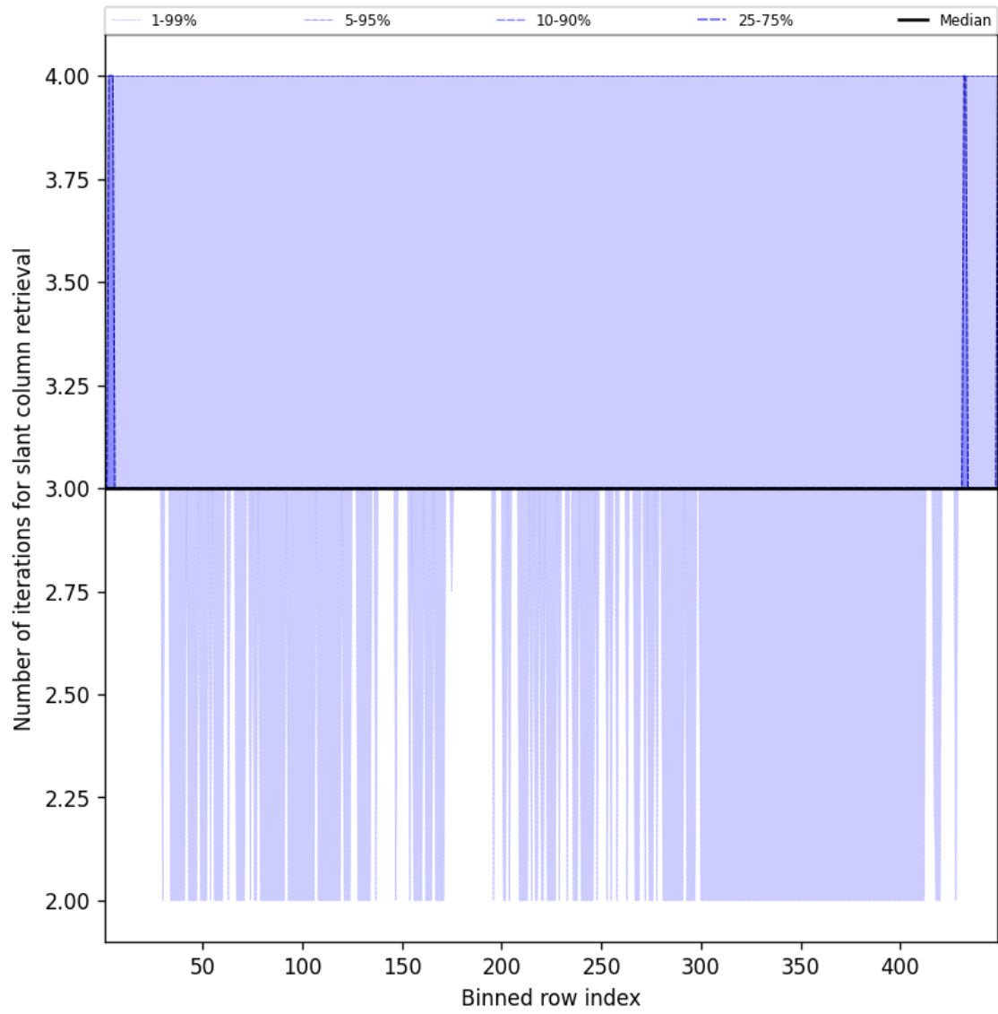
Figure 45: Along track statistics of “Number of iterations for slant column retrieval” for 2025-11-02 to 2025-11-03
