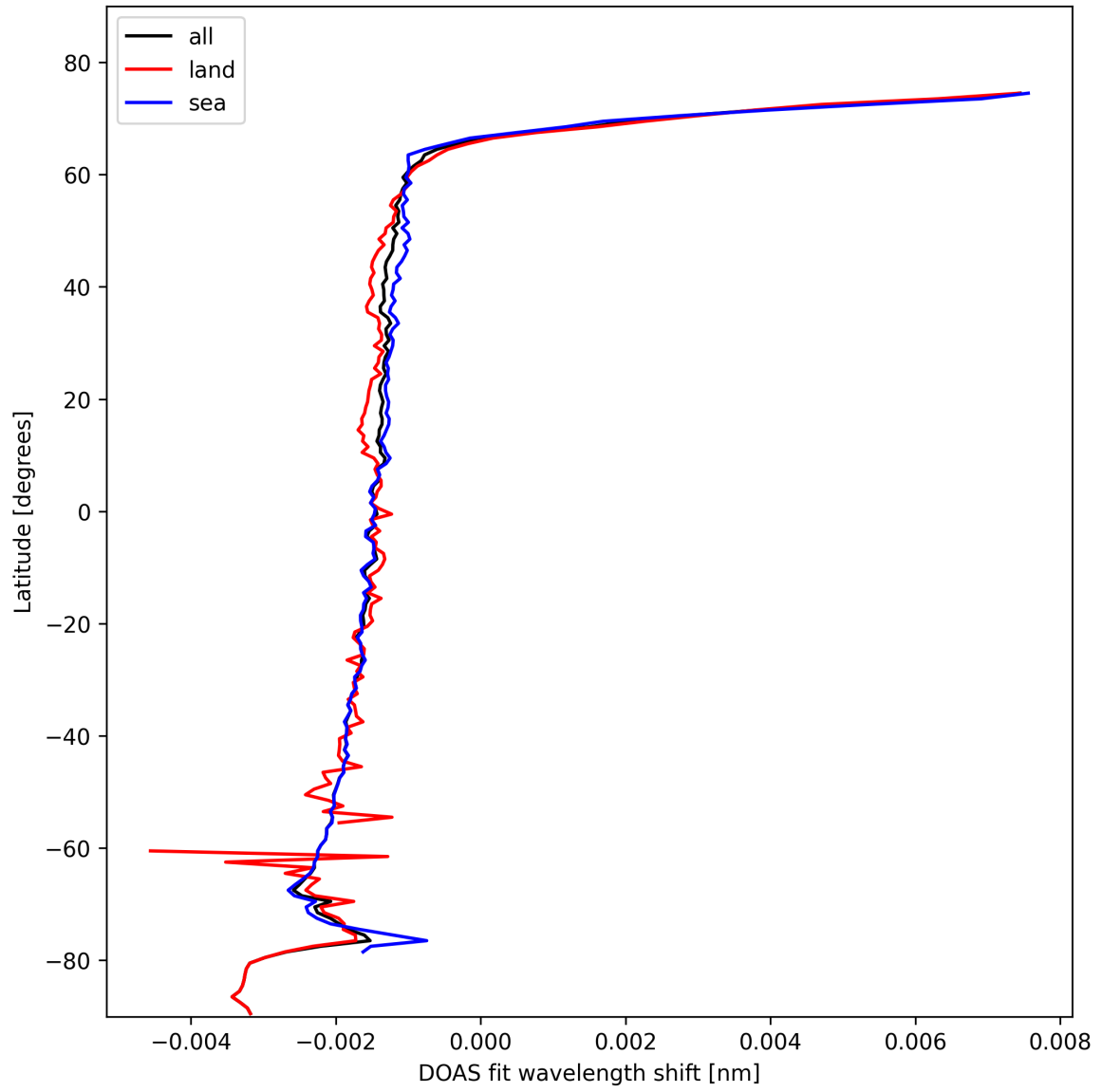
Figure 23: Zonal average of “DOAS fit wavelength shift” for 2025-11-02 to 2025-11-03.
