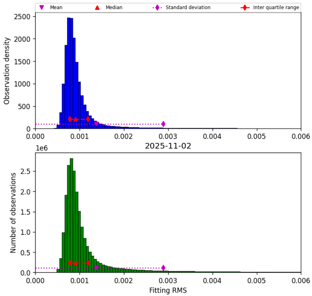
Figure 34: Histogram of “Fitting RMS” for 2025-11-02 to 2025-11-03
