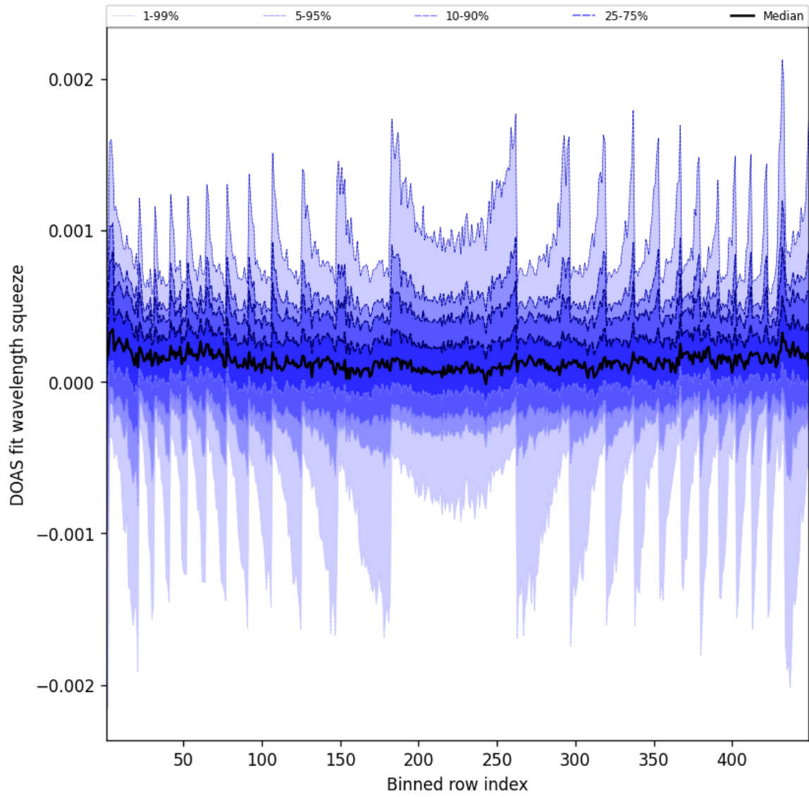
Figure 48: Along track statistics of “DOAS fit wavelength squeeze” for 2025-11-02 to 2025-11-03
