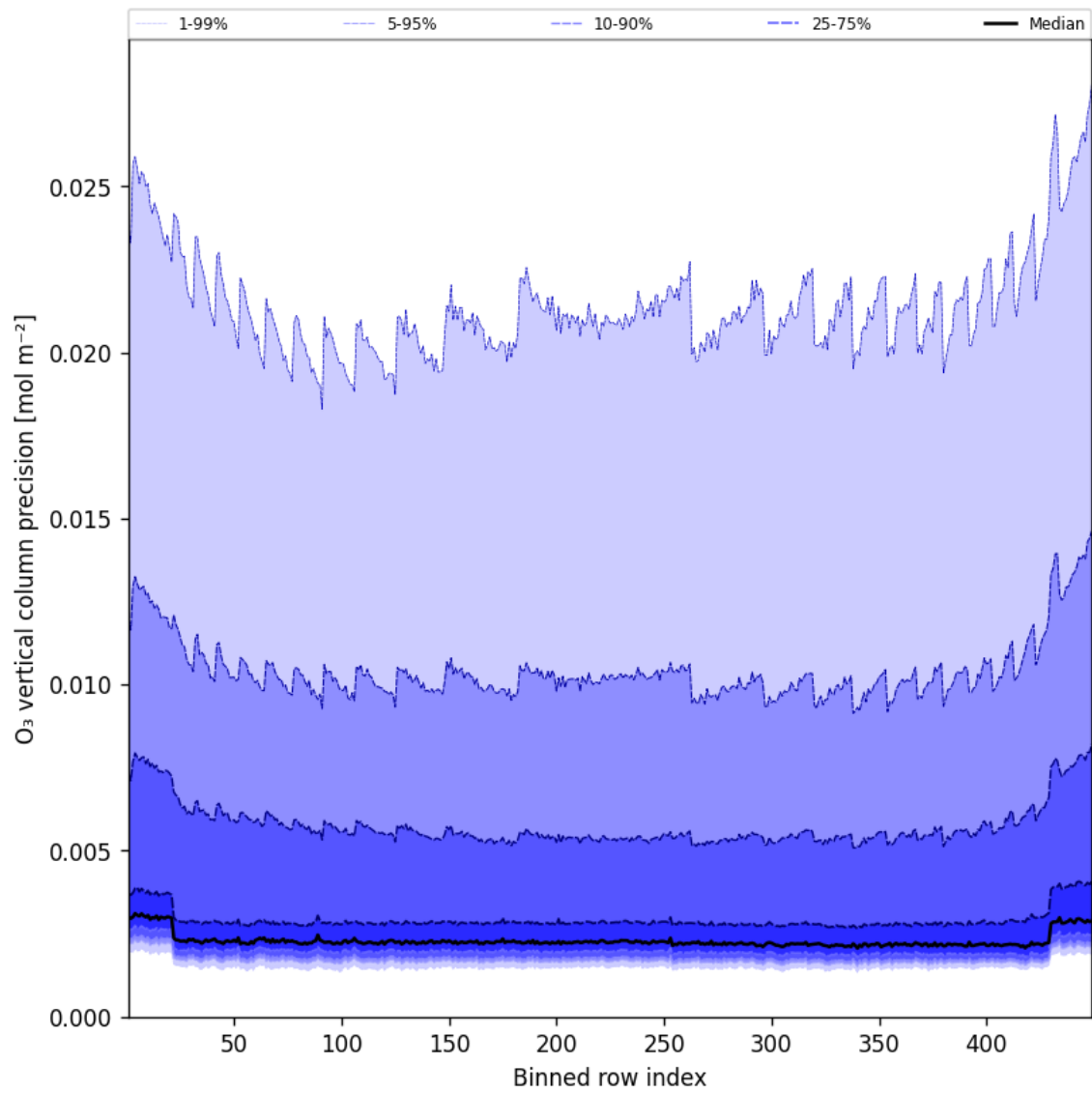
Figure 42: Along track statistics of “O 3 vertical column precision” for 2025-11-02 to 2025-11-03
