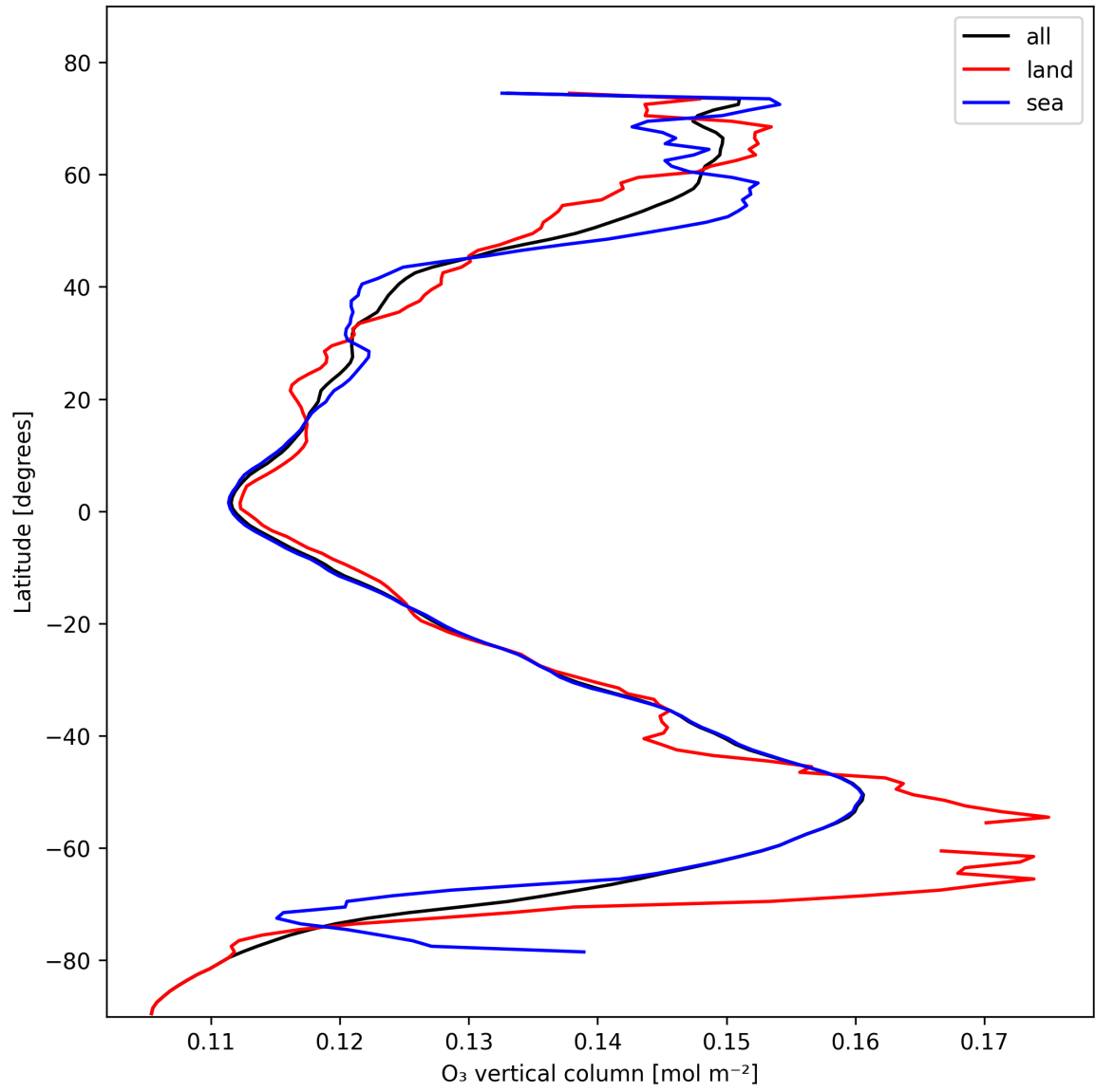
Figure 17: Zonal average of “O 3 vertical column” for 2025-11-02 to 2025-11-03.
