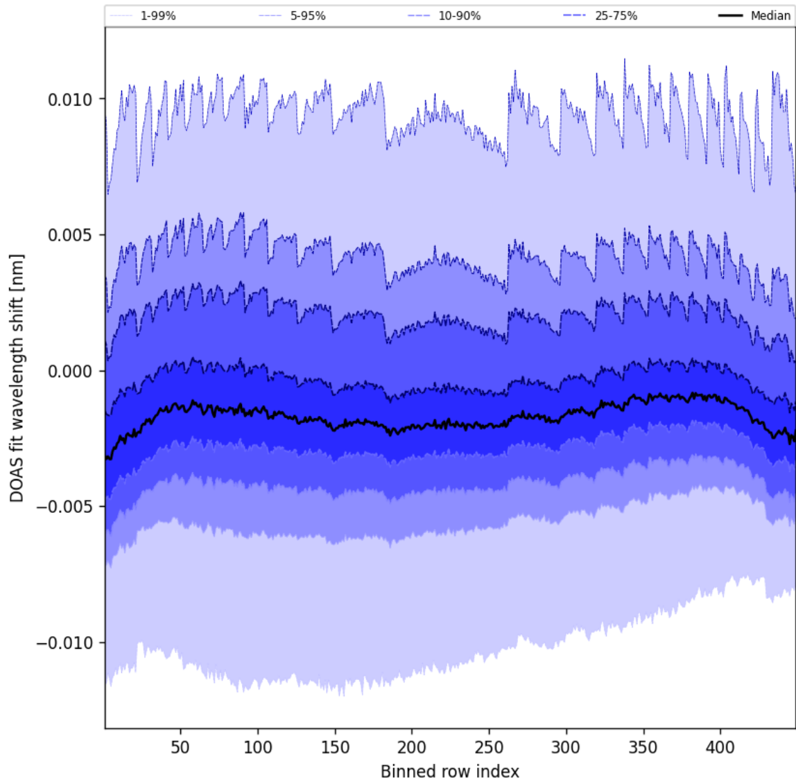
Figure 47: Along track statistics of “DOAS fit wavelength shift” for 2025-11-02 to 2025-11-03
