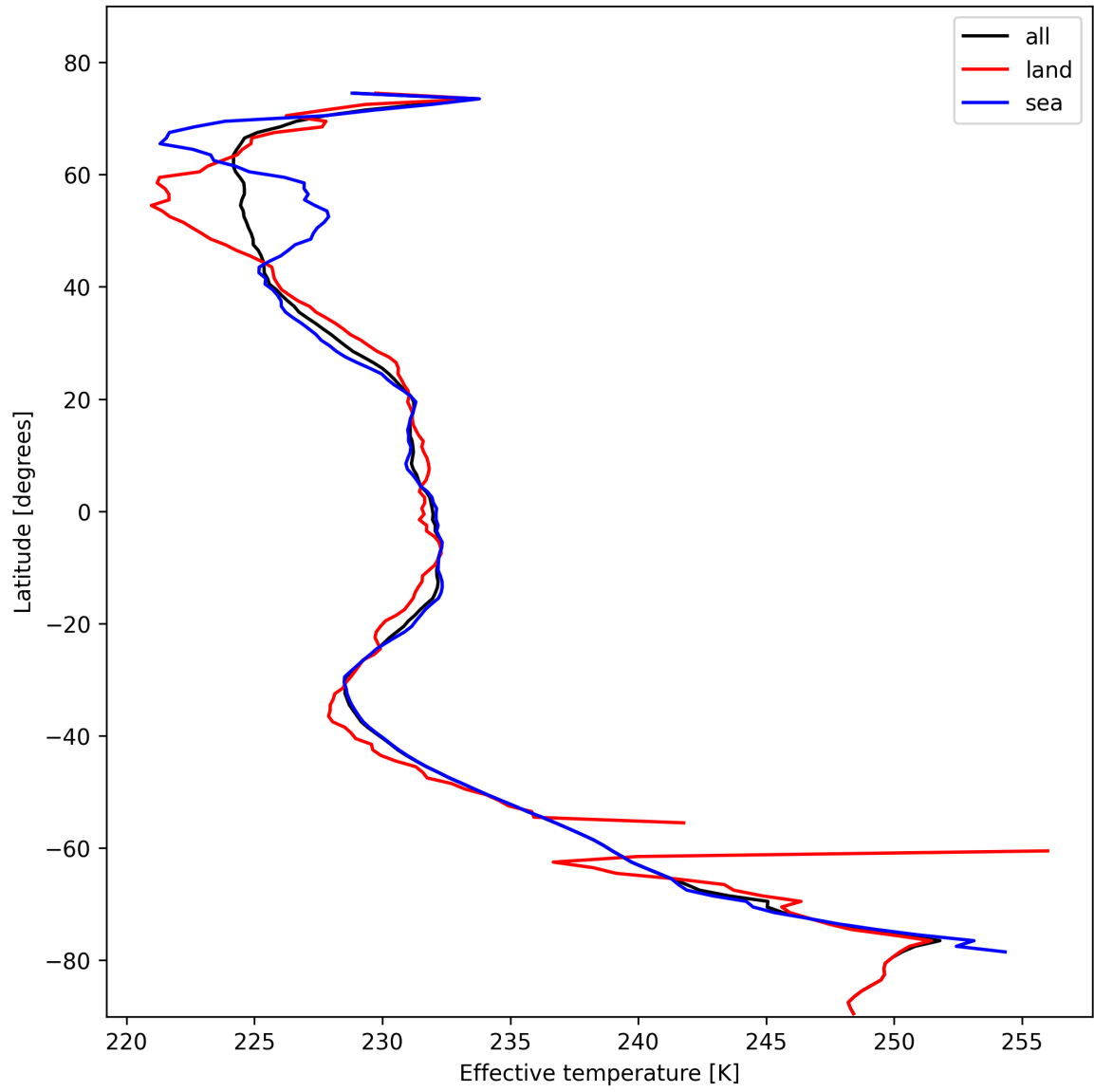
Figure 26: Zonal average of “Effective temperature” for 2025-11-02 to 2025-11-03.
