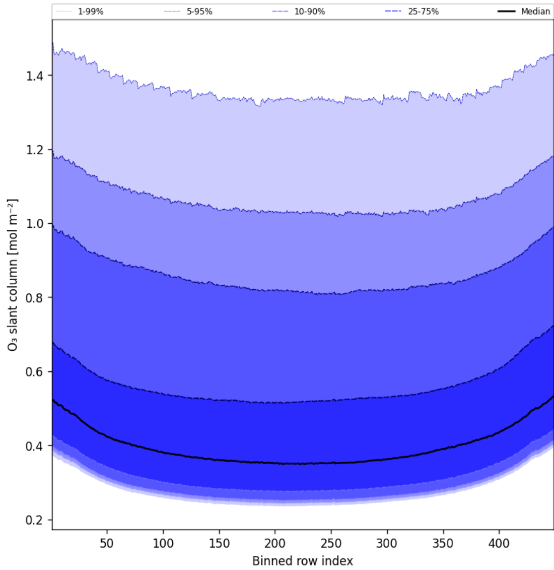
Figure 43: Along track statistics of “O 3 slant column” for 2025-11-02 to 2025-11-03
