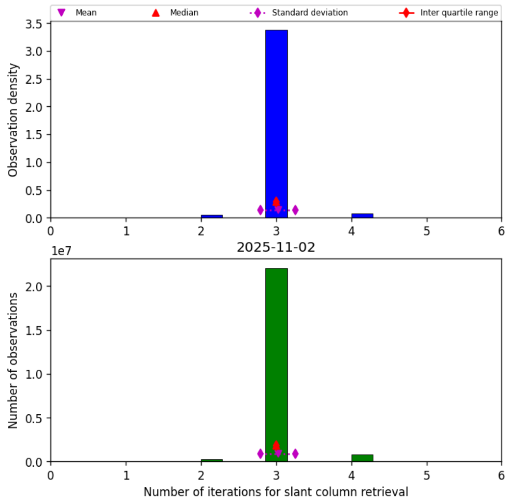
Figure 33: Histogram of “Number of iterations for slant column retrieval” for 2025-11-02 to 2025-11-03
