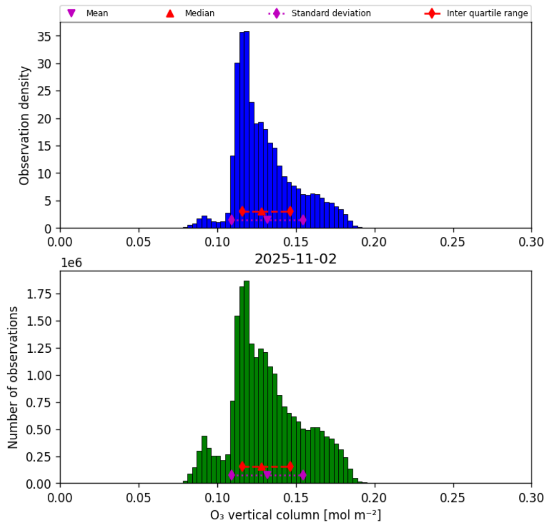
Figure 29: Histogram of “O 3 vertical column” for 2025-11-02 to 2025-11-03
