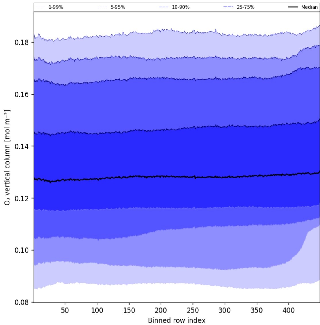
Figure 41: Along track statistics of “O 3 vertical column” for 2025-11-02 to 2025-11-03
