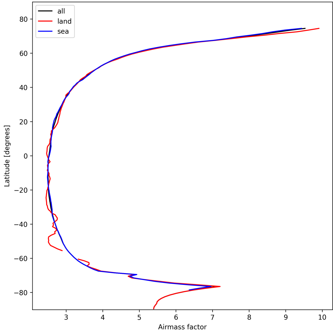
Figure 25: Zonal average of “Airmass factor” for 2025-11-02 to 2025-11-03.
