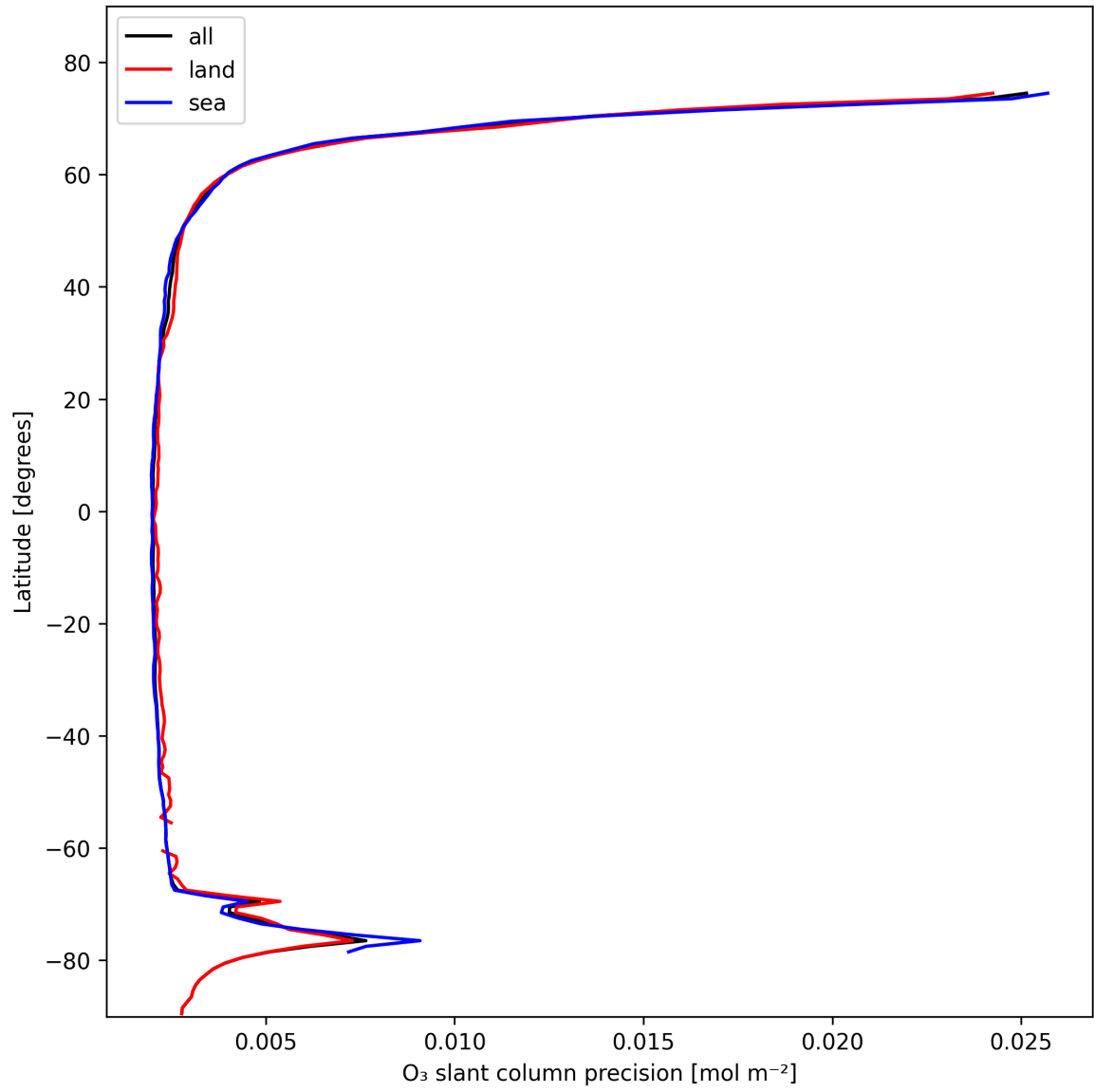
Figure 20: Zonal average of “O 3 slant column precision” for 2025-11-02 to 2025-11-03.
