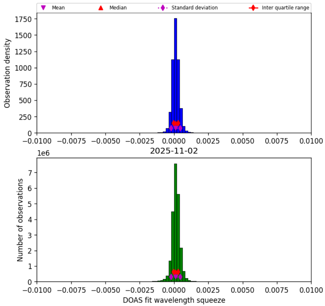
Figure 36: Histogram of “DOAS fit wavelength squeeze” for 2025-11-02 to 2025-11-03
