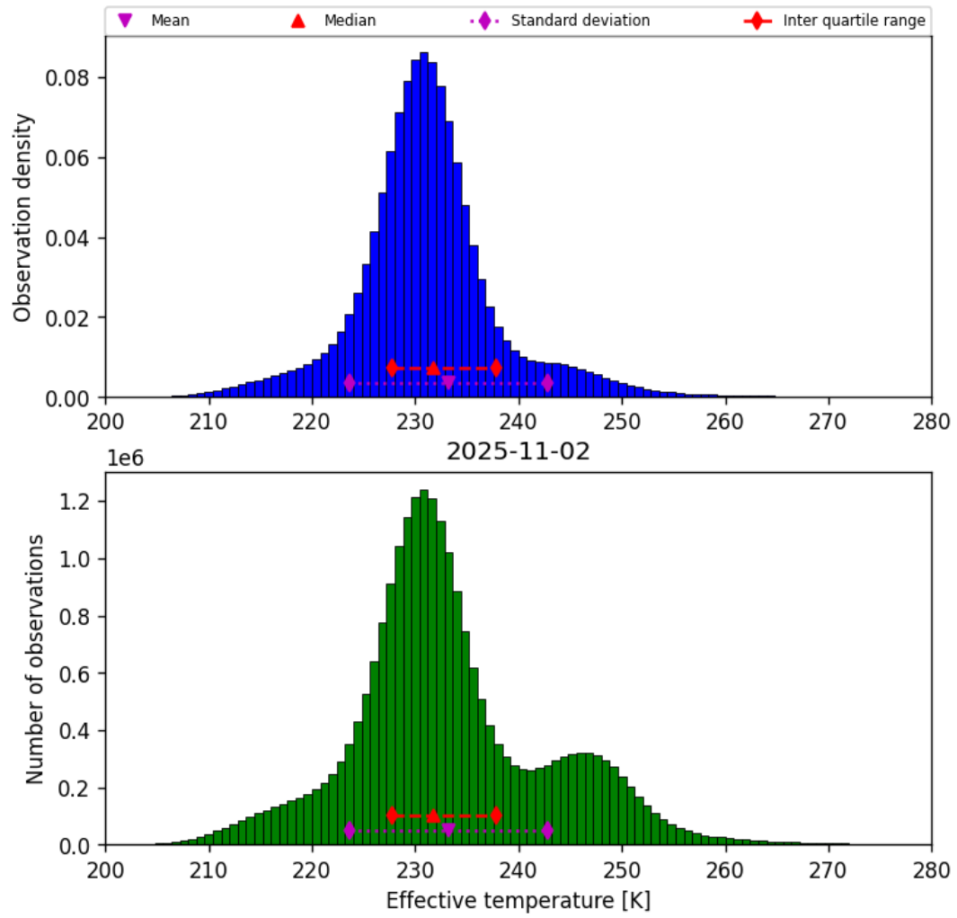
Figure 38: Histogram of “Effective temperature” for 2025-11-02 to 2025-11-03
