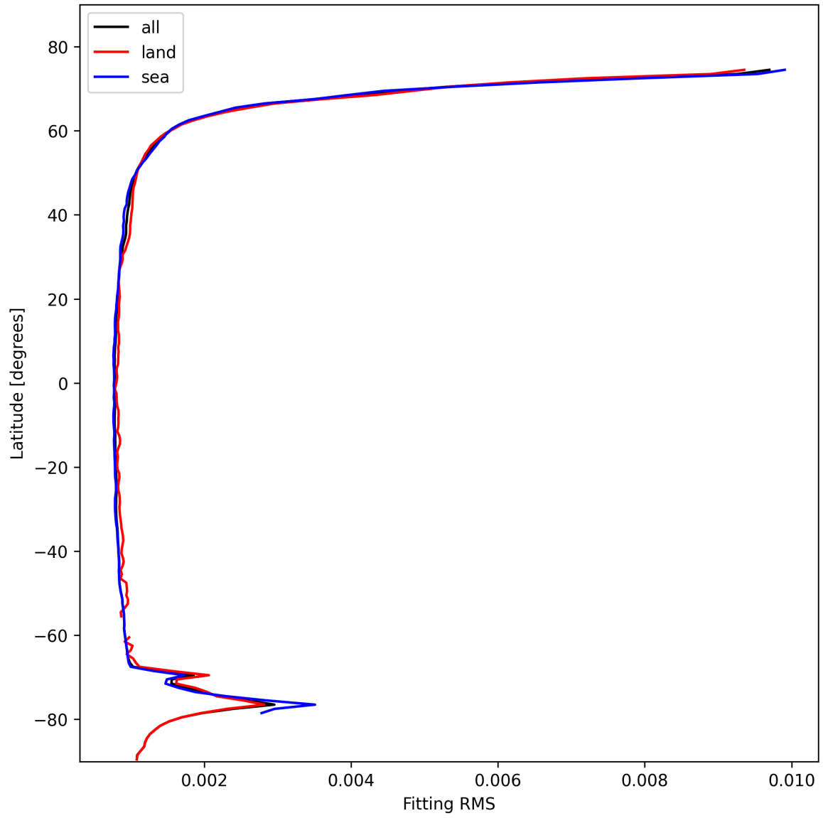
Figure 22: Zonal average of “Fitting RMS” for 2025-11-02 to 2025-11-03.
