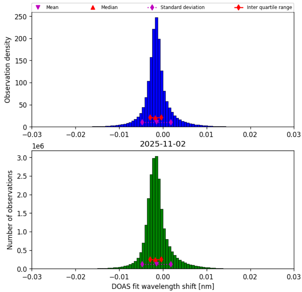
Figure 35: Histogram of “DOAS fit wavelength shift” for 2025-11-02 to 2025-11-03
