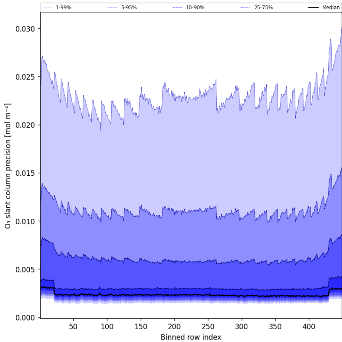
Figure 44: Along track statistics of “O 3 slant column precision” for 2025-11-02 to 2025-11-03
