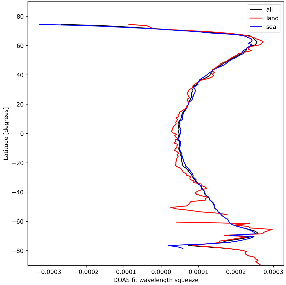
Figure 24: Zonal average of “DOAS fit wavelength squeeze” for 2025-11-02 to 2025-11-03.
