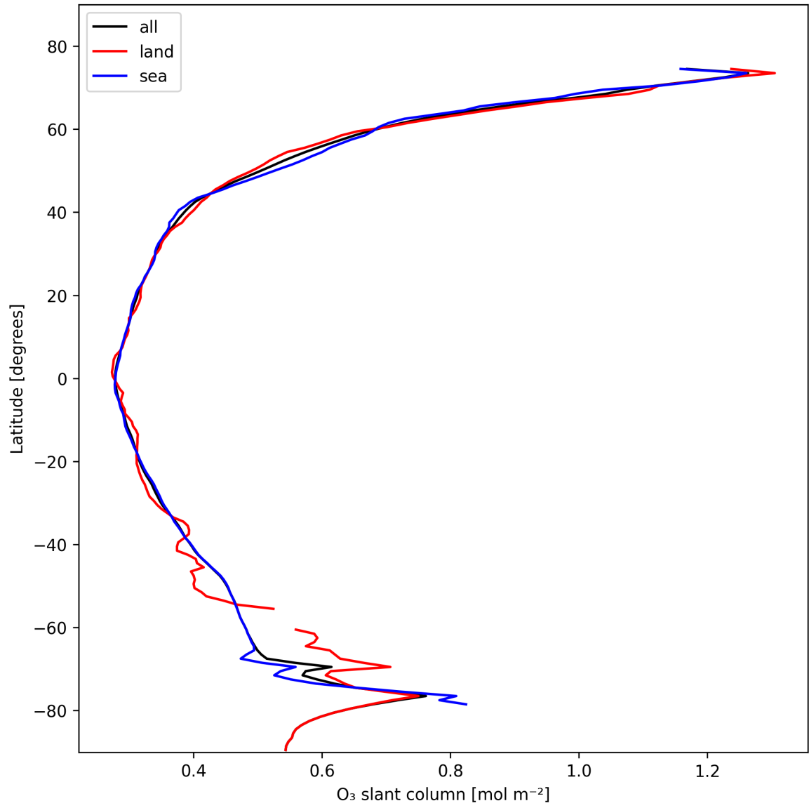
Figure 19: Zonal average of “O 3 slant column” for 2025-11-02 to 2025-11-03.
