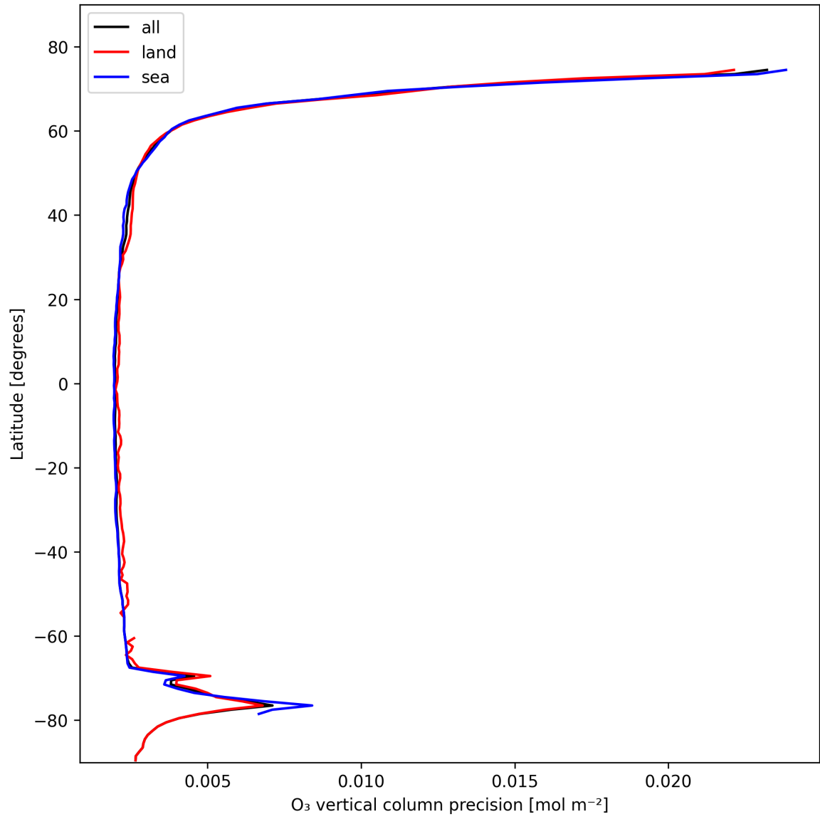
Figure 18: Zonal average of “O 3 vertical column precision” for 2025-11-02 to 2025-11-03.
