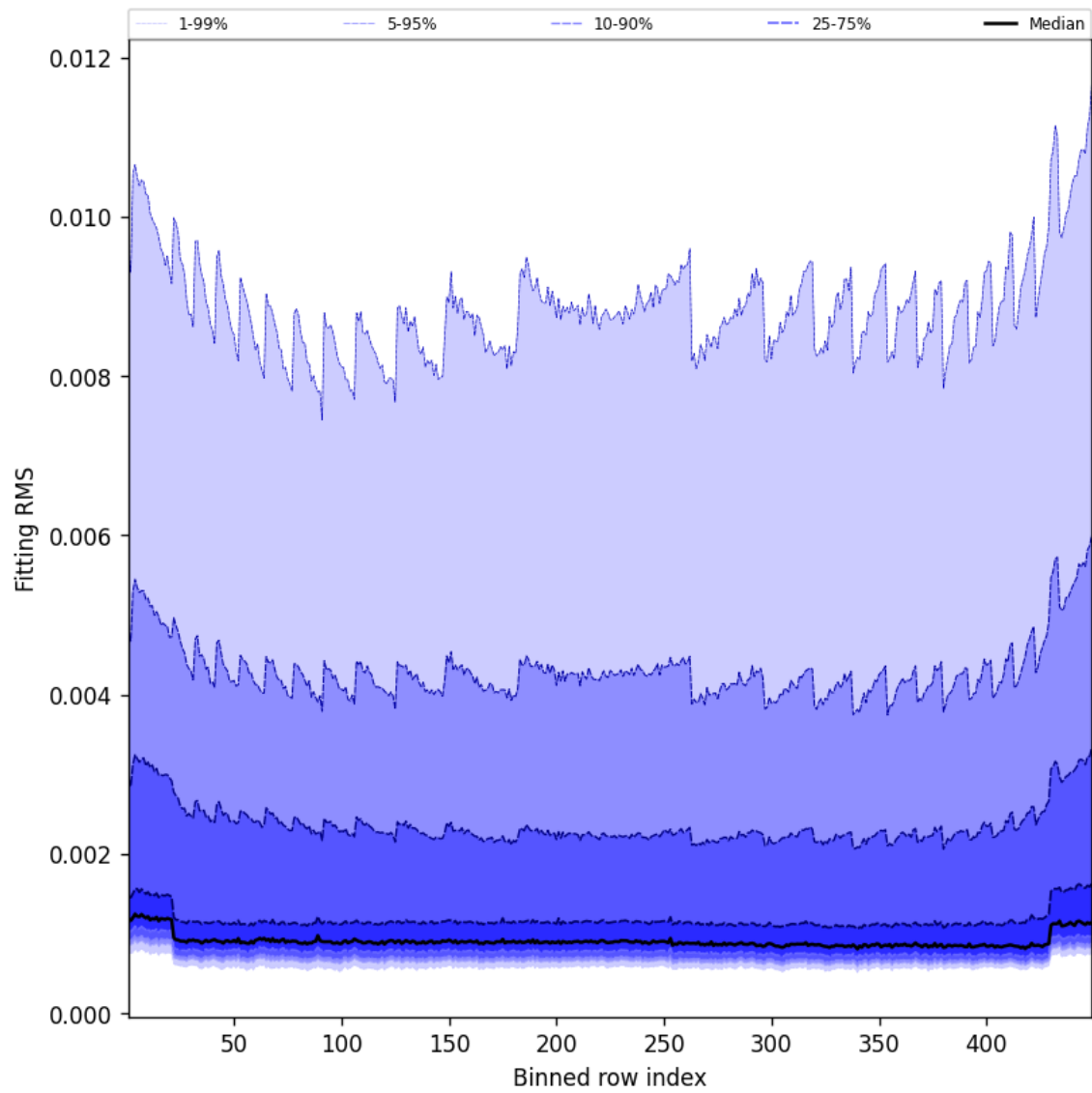
Figure 46: Along track statistics of “Fitting RMS” for 2025-11-02 to 2025-11-03
