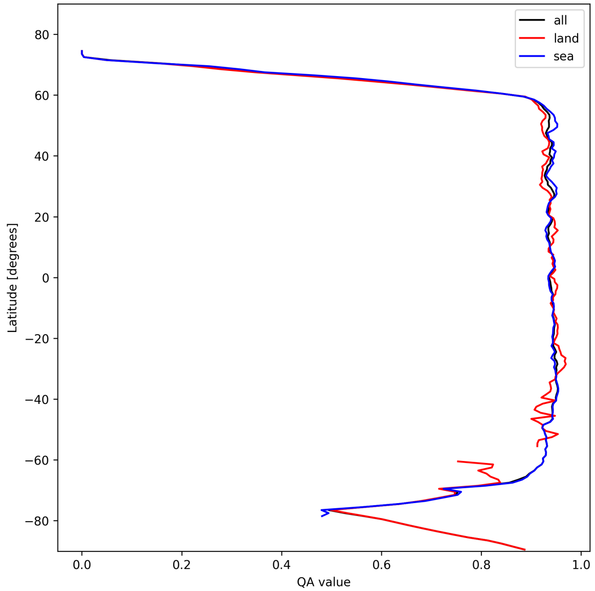
Figure 16: Zonal average of “QA value” for 2025-11-02 to 2025-11-03.
