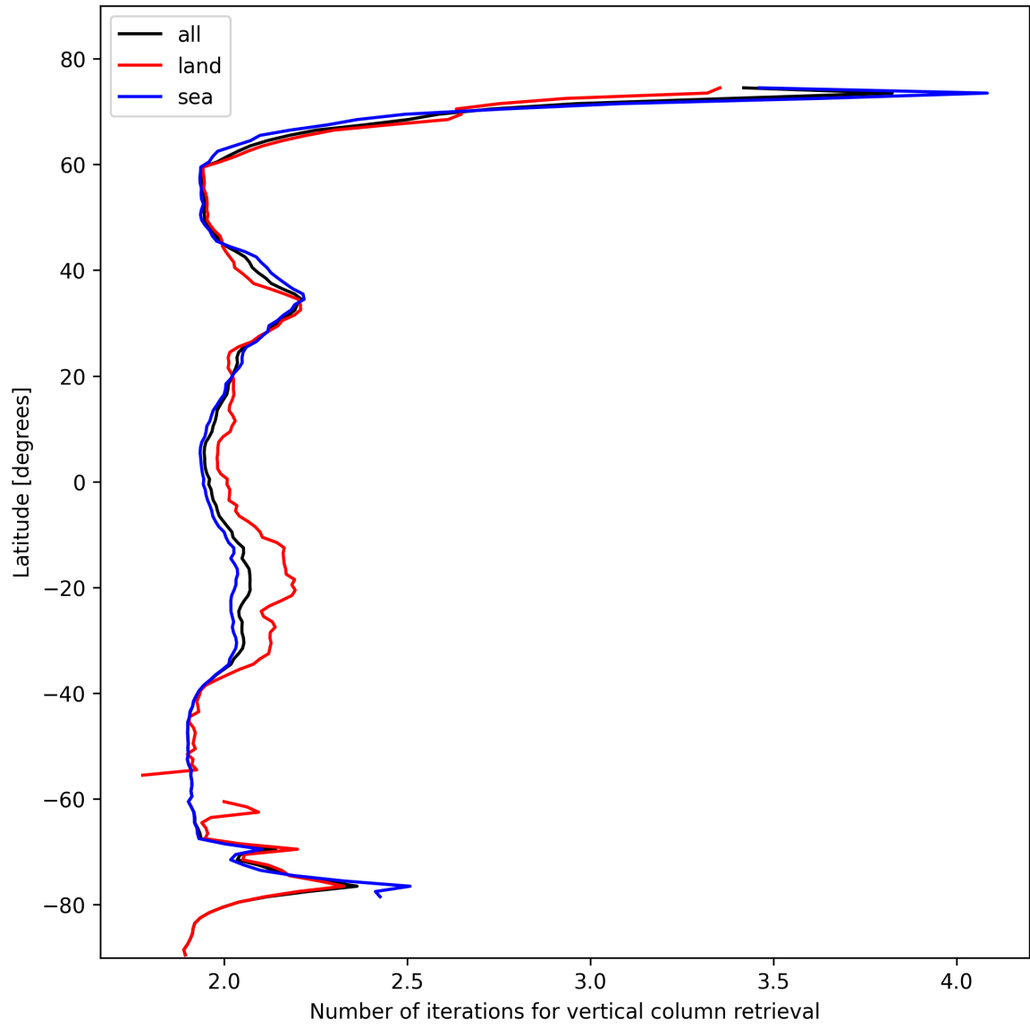
Figure 27: Zonal average of “Number of iterations for vertical column retrieval” for 2025-11-02 to 2025-11-03.
