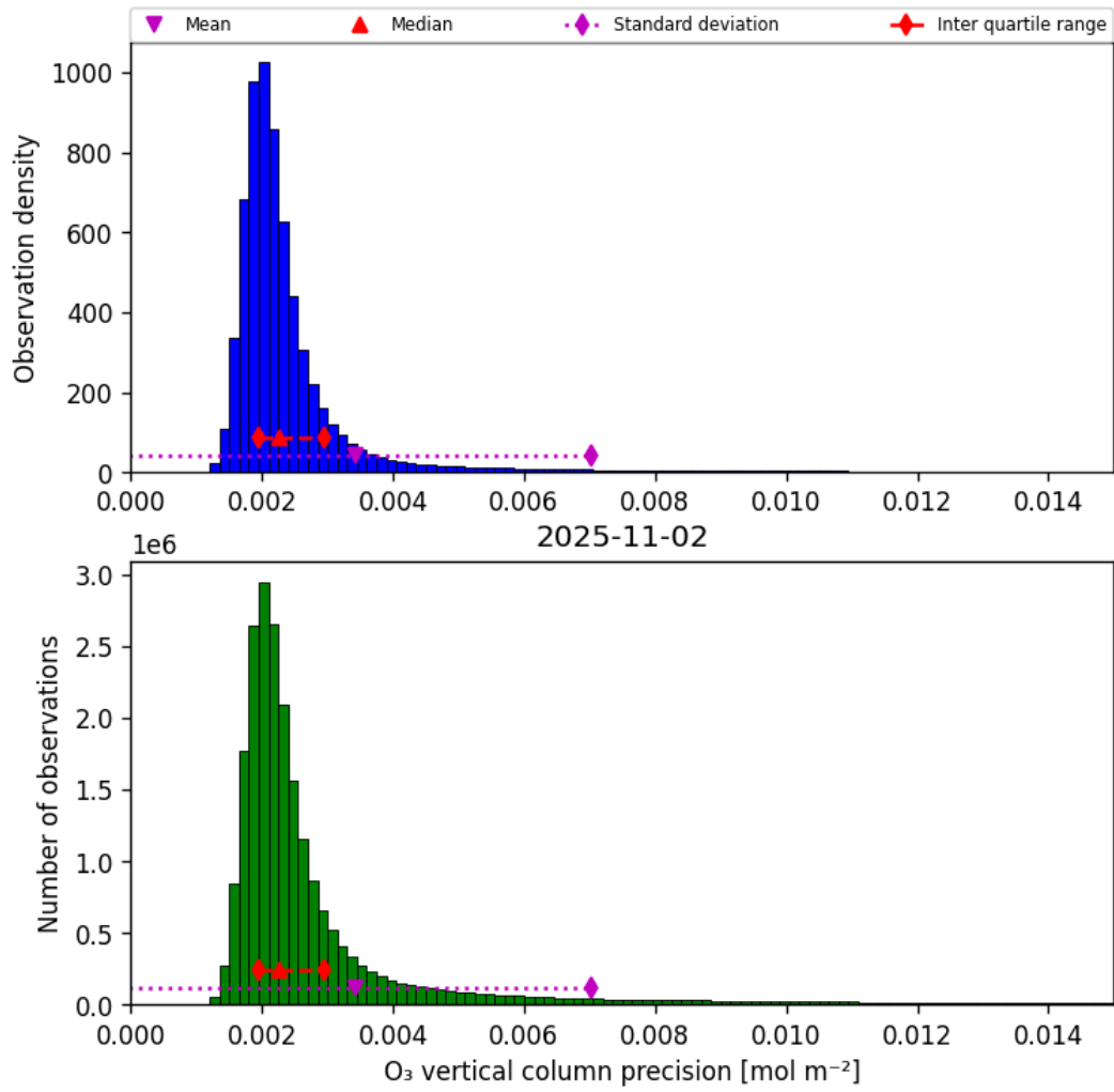
Figure 30: Histogram of “O 3 vertical column precision” for 2025-11-02 to 2025-11-03
