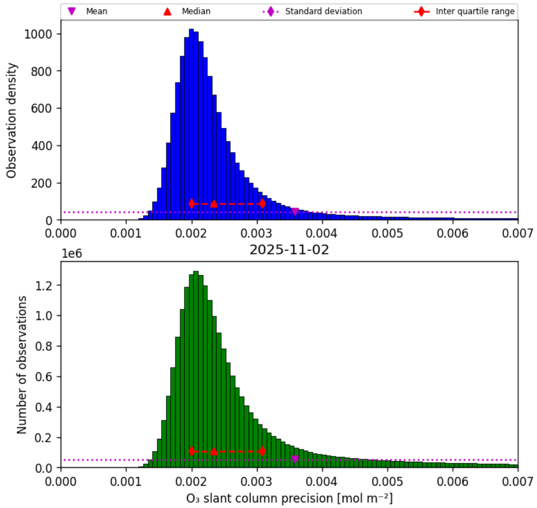
Figure 32: Histogram of “O 3 slant column precision” for 2025-11-02 to 2025-11-03
