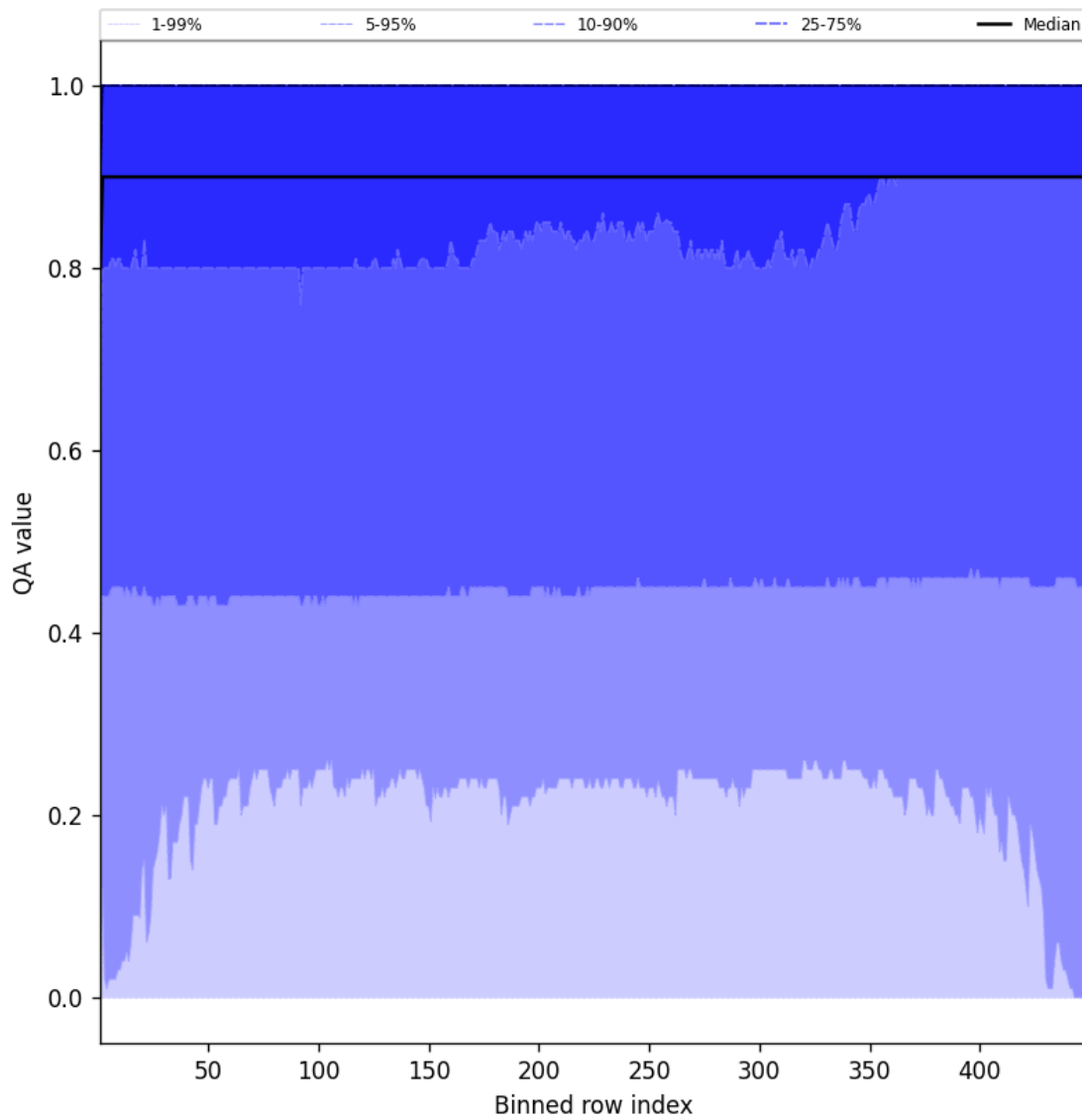
Figure 40: Along track statistics of “QA value” for 2025-11-02 to 2025-11-03
