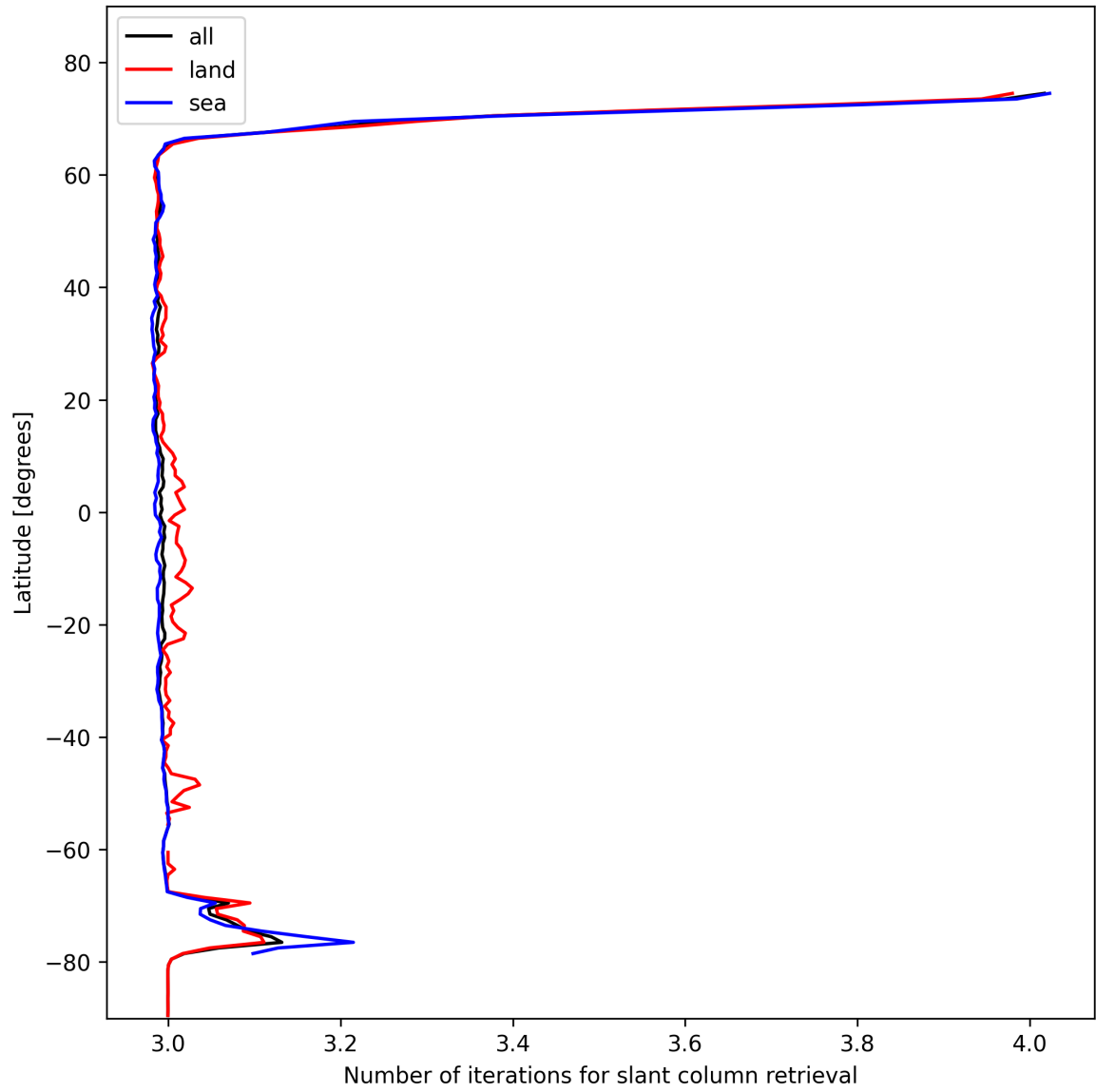
Figure 21: Zonal average of “Number of iterations for slant column retrieval” for 2025-11-02 to 2025-11-03.
