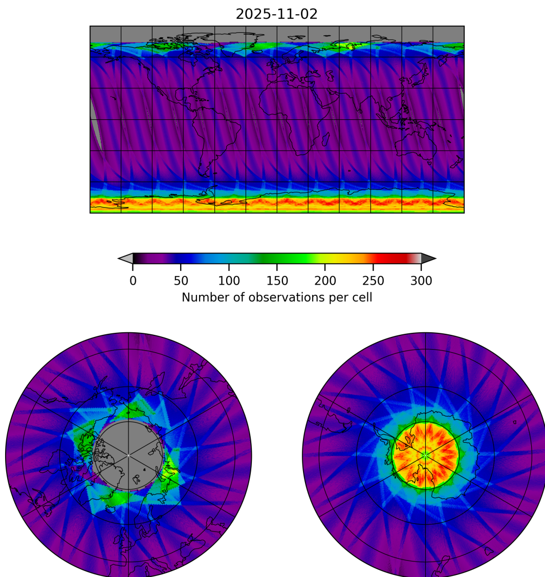
Figure 15: Map of the number of observations for 2025-11-02 to 2025-11-03
