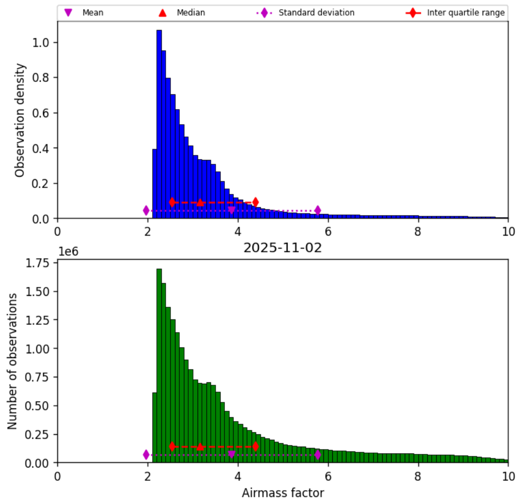
Figure 37: Histogram of “Airmass factor” for 2025-11-02 to 2025-11-03
