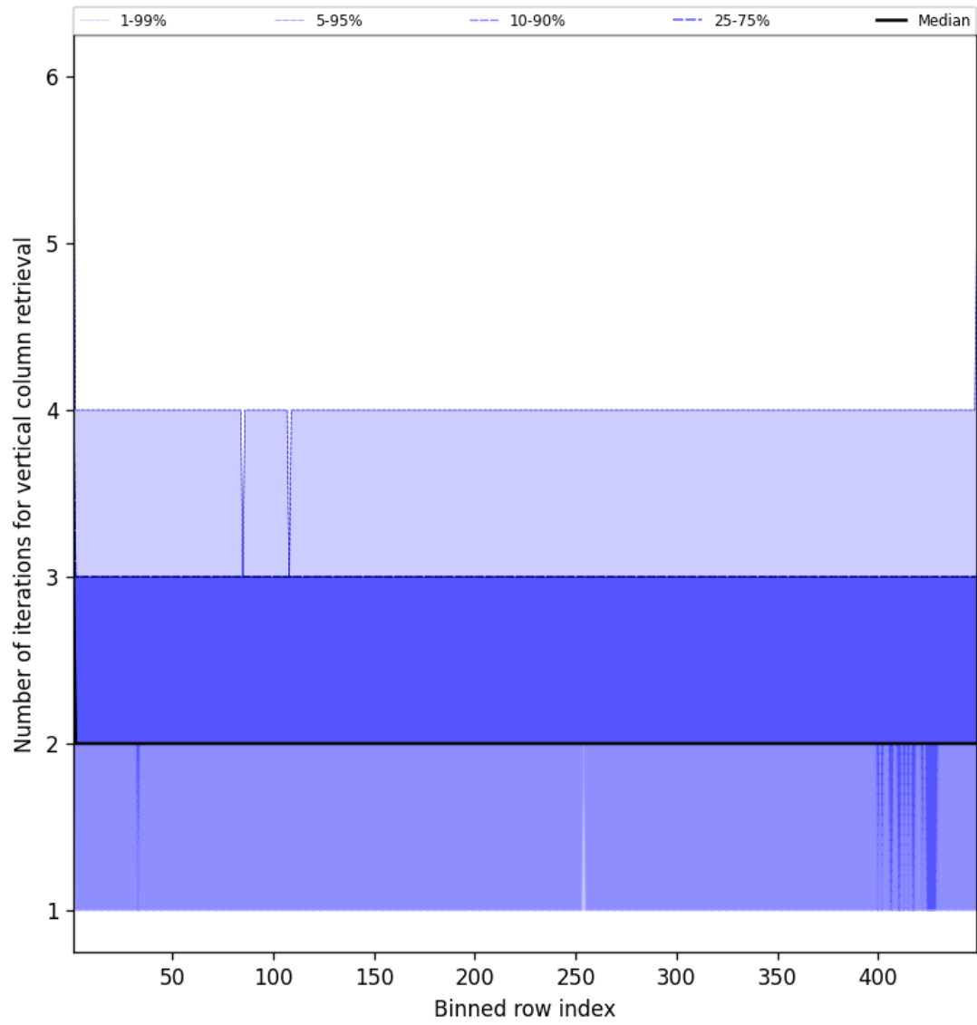
Figure 51: Along track statistics of “Number of iterations for vertical column retrieval” for 2025-11-02 to 2025-11-03
