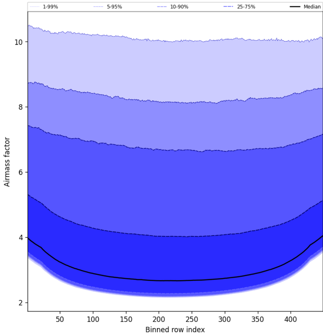
Figure 49: Along track statistics of “Airmass factor” for 2025-11-02 to 2025-11-03
