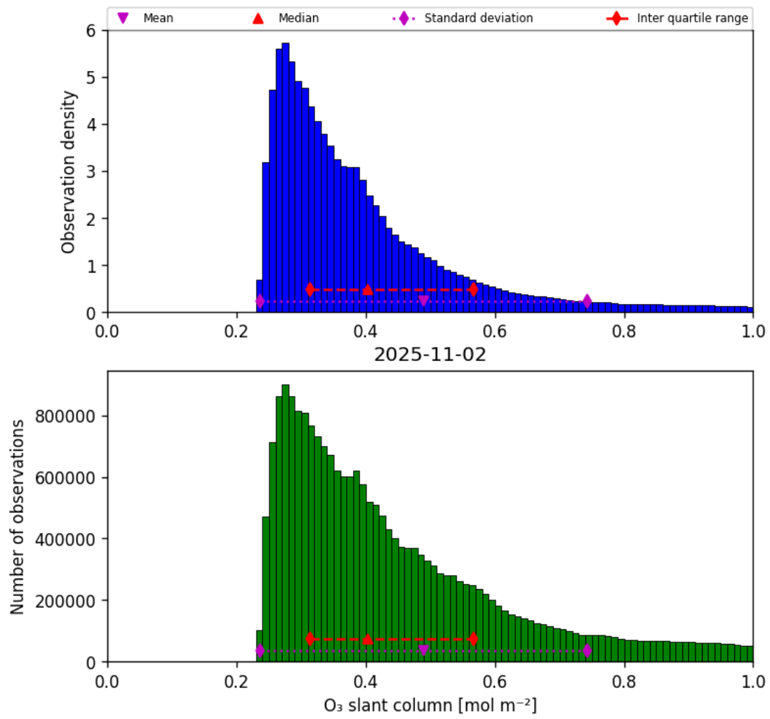
Figure 31: Histogram of “O 3 slant column” for 2025-11-02 to 2025-11-03
