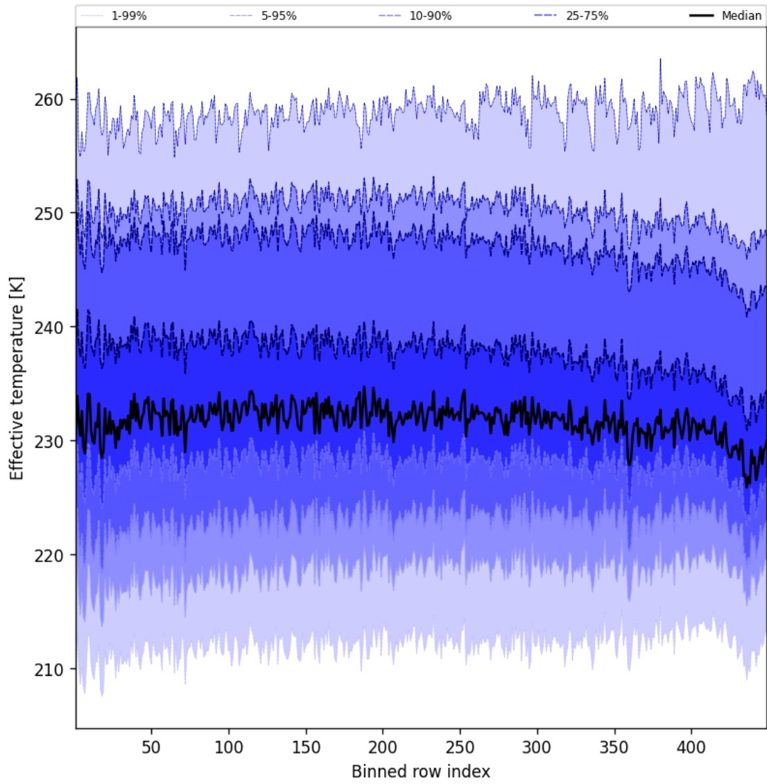
Figure 50: Along track statistics of “Effective temperature” for 2025-11-02 to 2025-11-03
