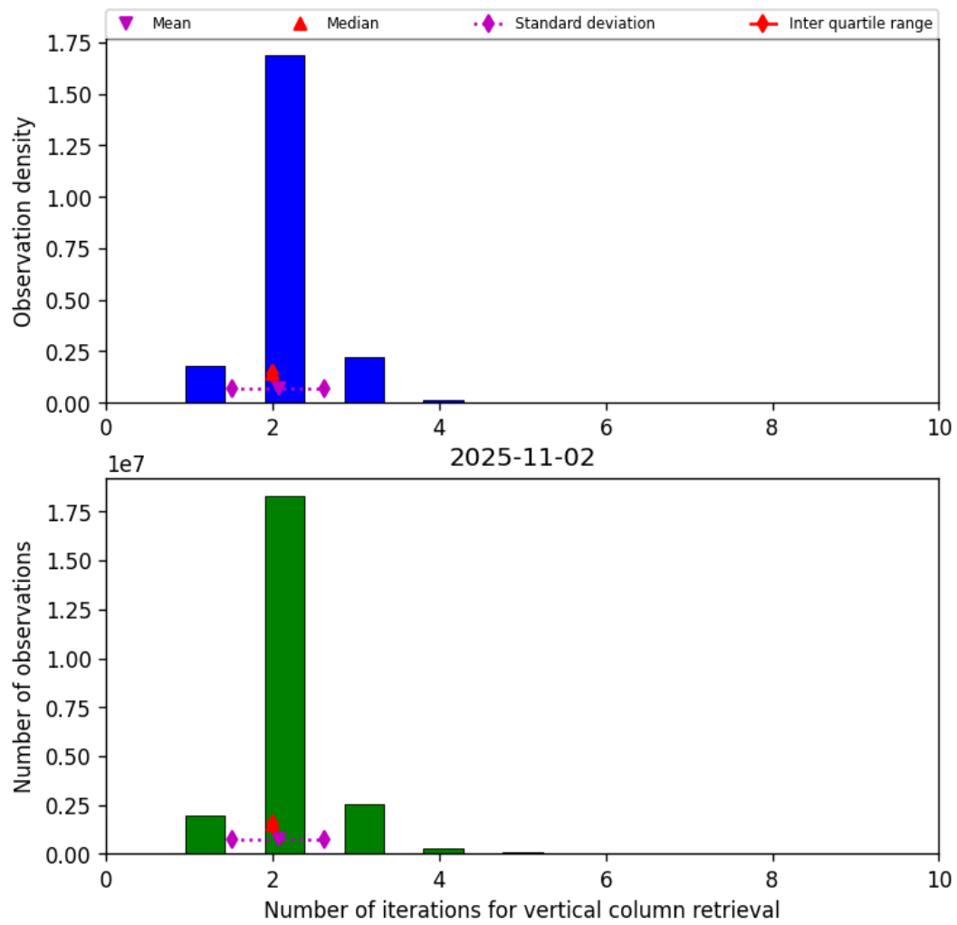
Figure 39: Histogram of “Number of iterations for vertical column retrieval” for 2025-11-02 to 2025-11-03
