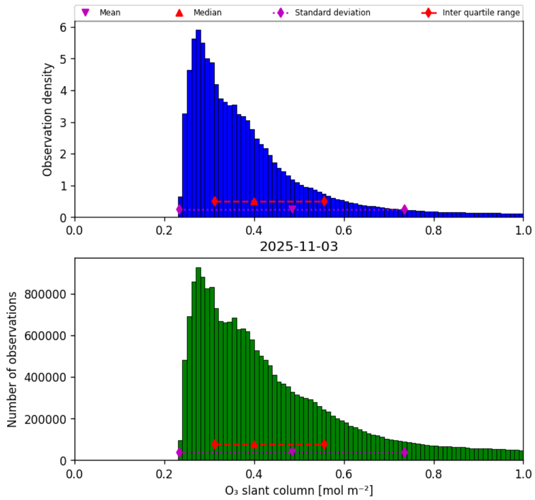
Figure 31: Histogram of “O 3 slant column” for 2025-11-03 to 2025-11-04
