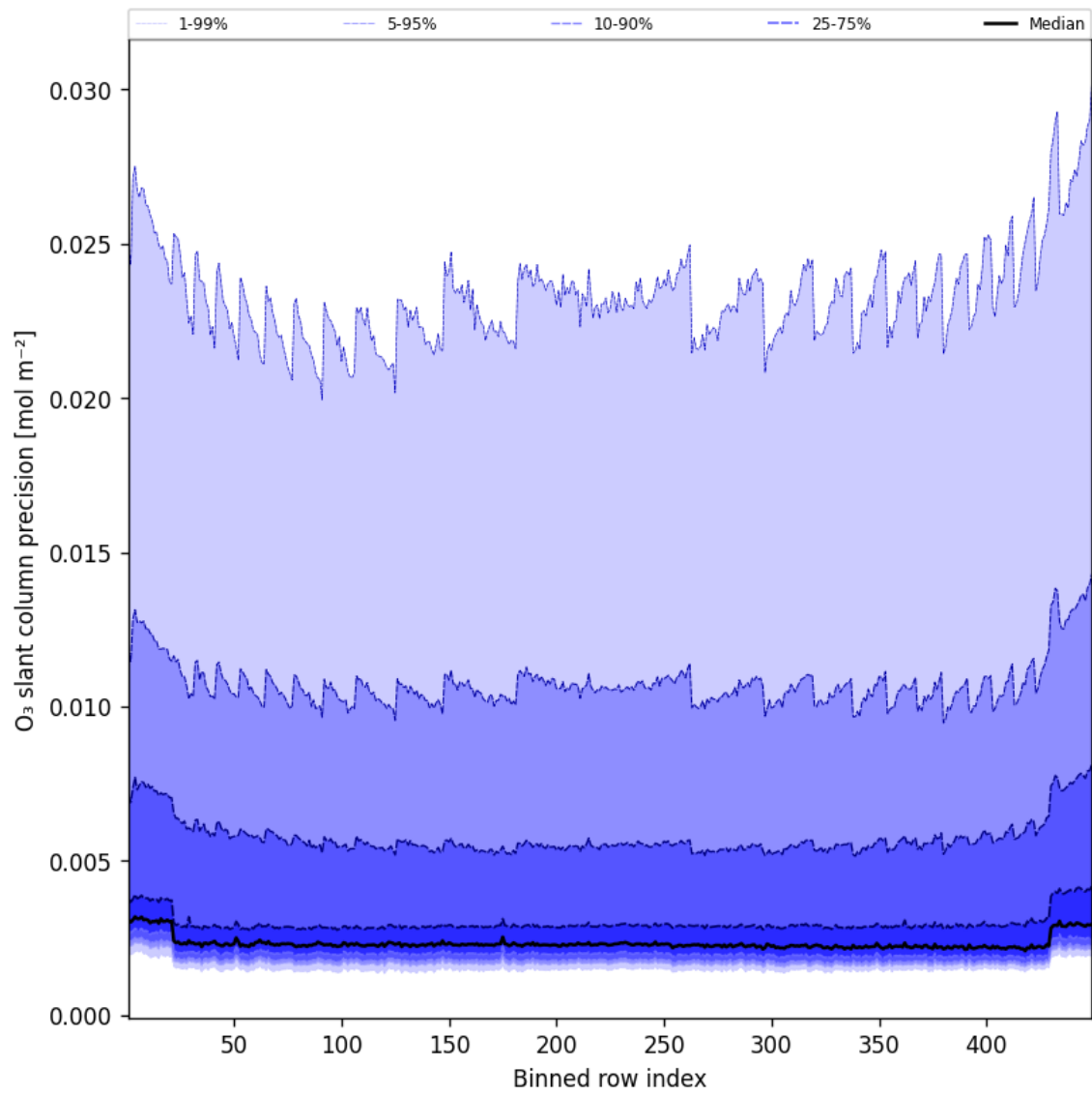
Figure 44: Along track statistics of “O 3 slant column precision” for 2025-11-03 to 2025-11-04
