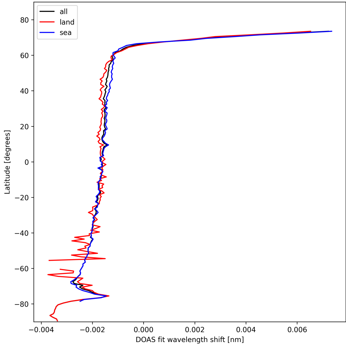
Figure 23: Zonal average of “DOAS fit wavelength shift” for 2025-11-03 to 2025-11-04.
