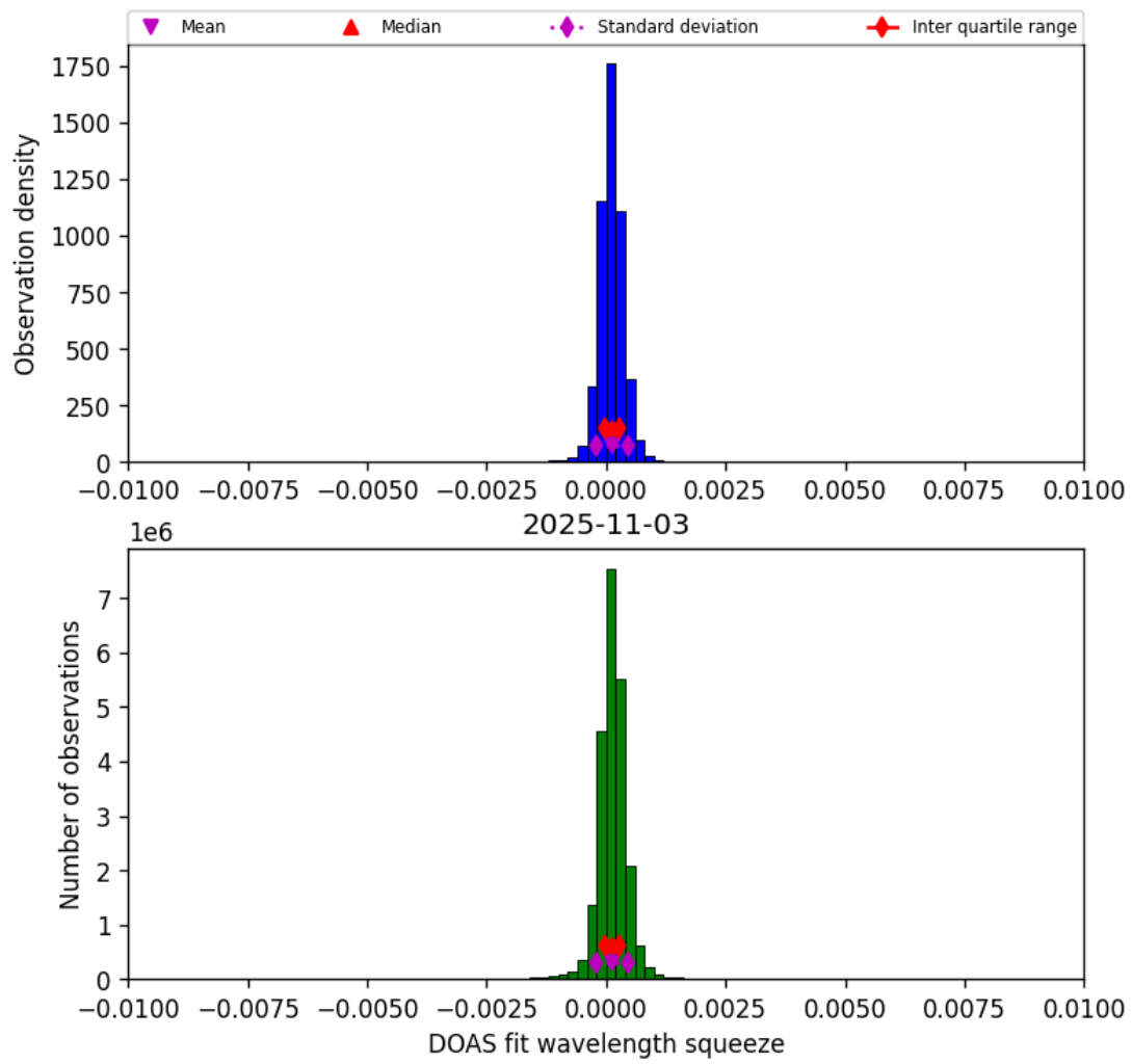
Figure 36: Histogram of “DOAS fit wavelength squeeze” for 2025-11-03 to 2025-11-04
