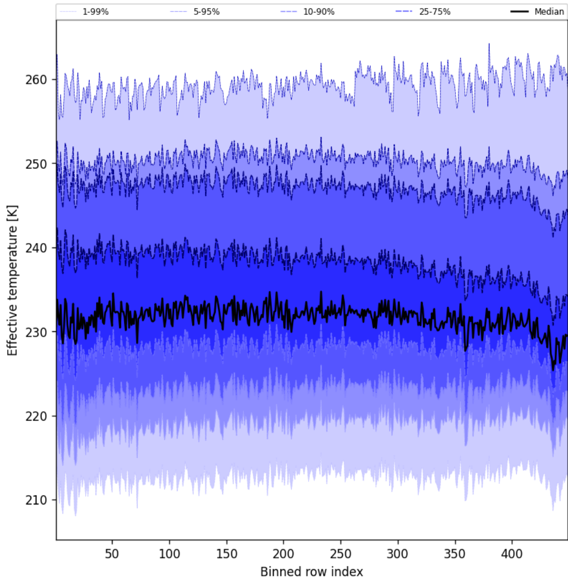
Figure 50: Along track statistics of “Effective temperature” for 2025-11-03 to 2025-11-04
