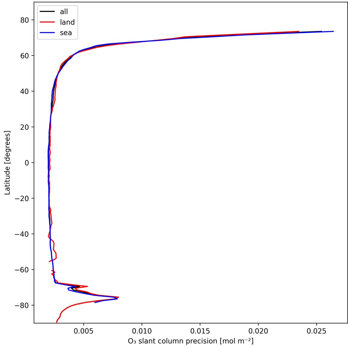
Figure 20: Zonal average of “O 3 slant column precision” for 2025-11-03 to 2025-11-04.
