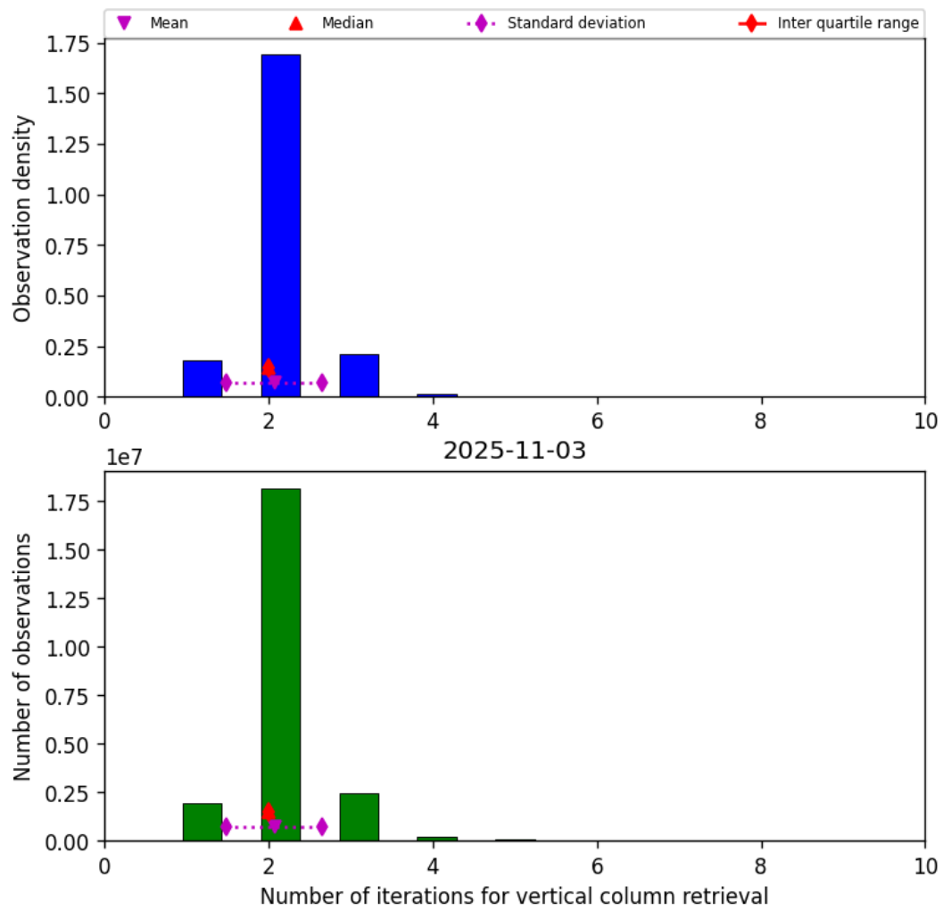
Figure 39: Histogram of “Number of iterations for vertical column retrieval” for 2025-11-03 to 2025-11-04
