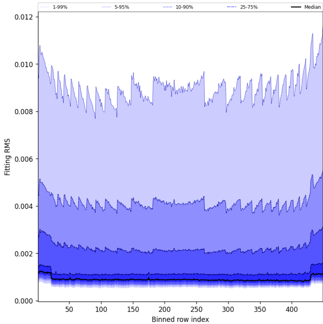
Figure 46: Along track statistics of “Fitting RMS” for 2025-11-03 to 2025-11-04
