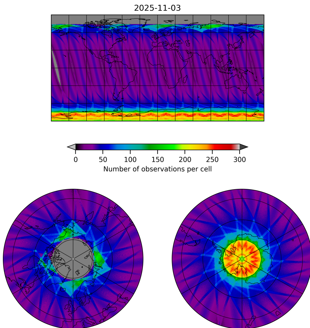
Figure 15: Map of the number of observations for 2025-11-03 to 2025-11-04
