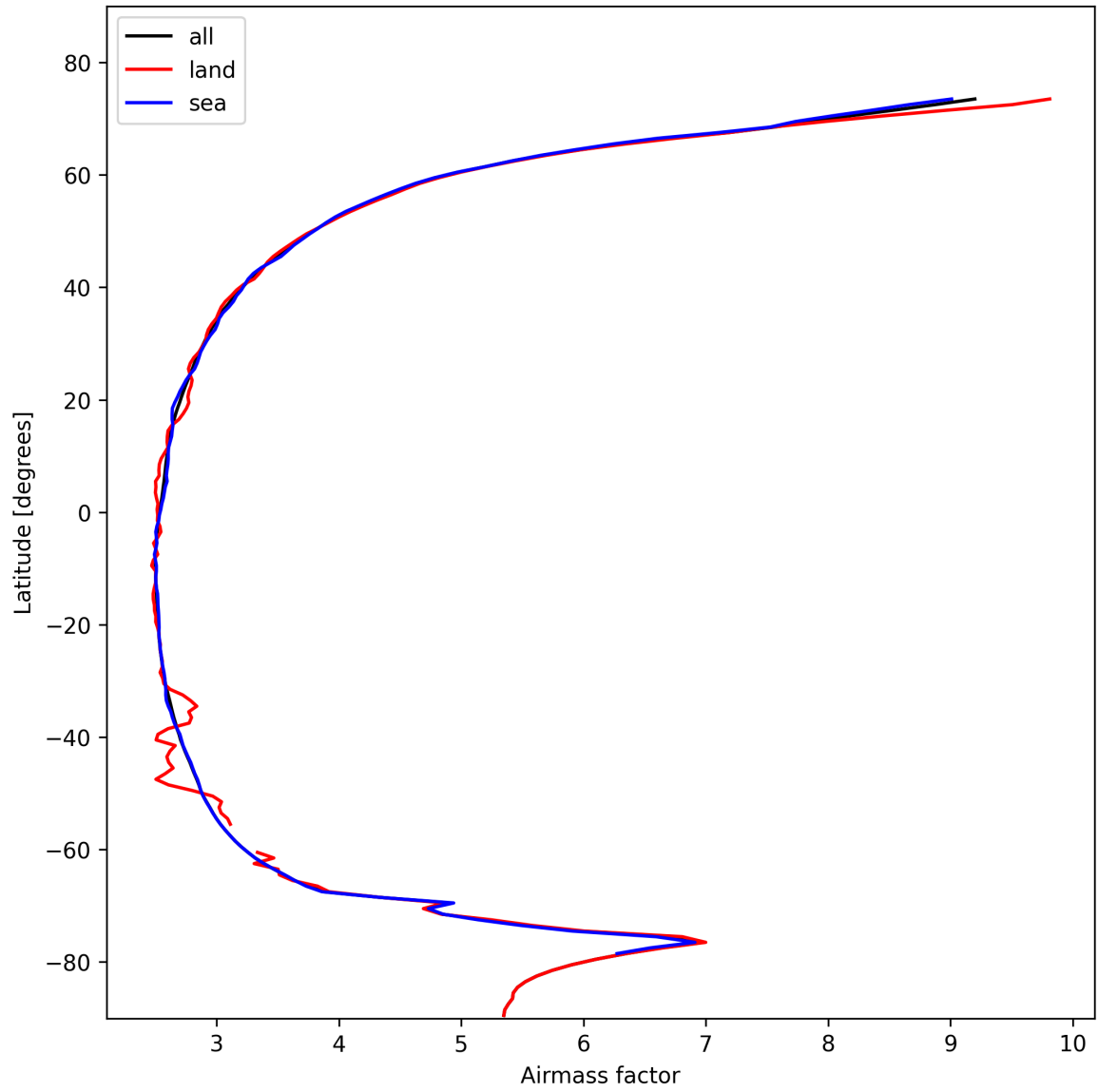
Figure 25: Zonal average of “Airmass factor” for 2025-11-03 to 2025-11-04.
