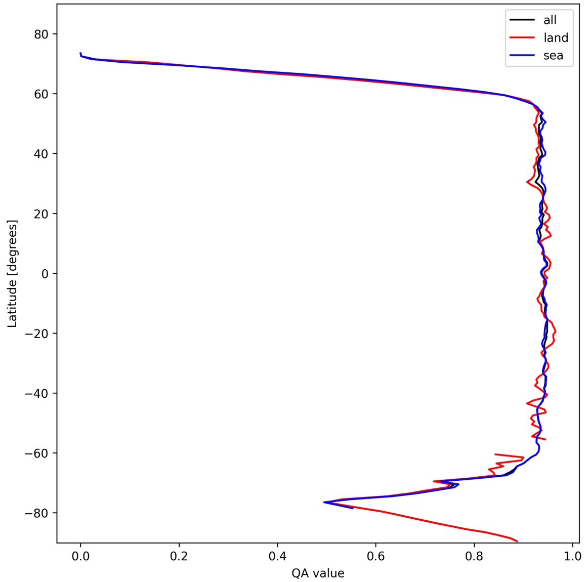
Figure 16: Zonal average of “QA value” for 2025-11-03 to 2025-11-04.
