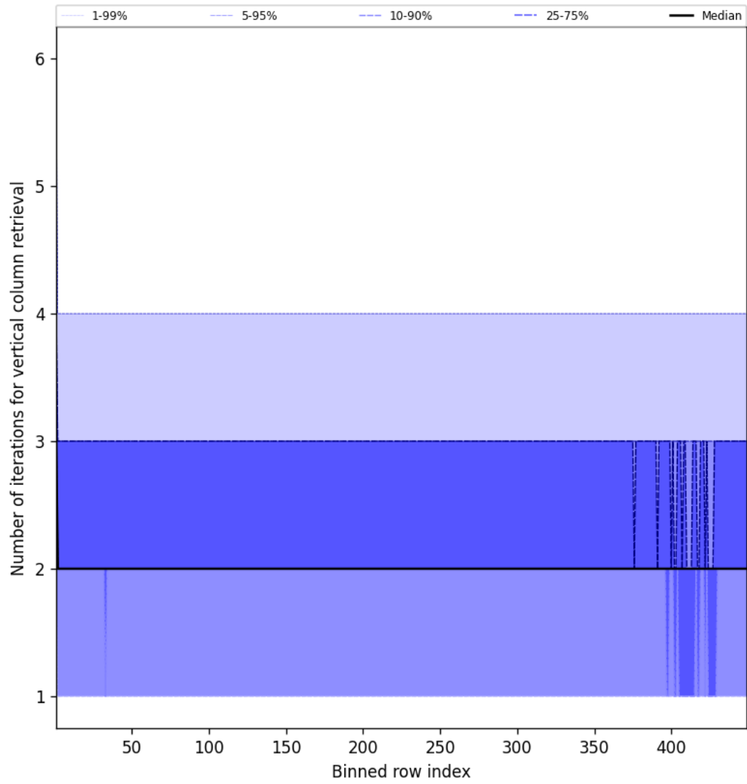
Figure 51: Along track statistics of “Number of iterations for vertical column retrieval” for 2025-11-03 to 2025-11-04
