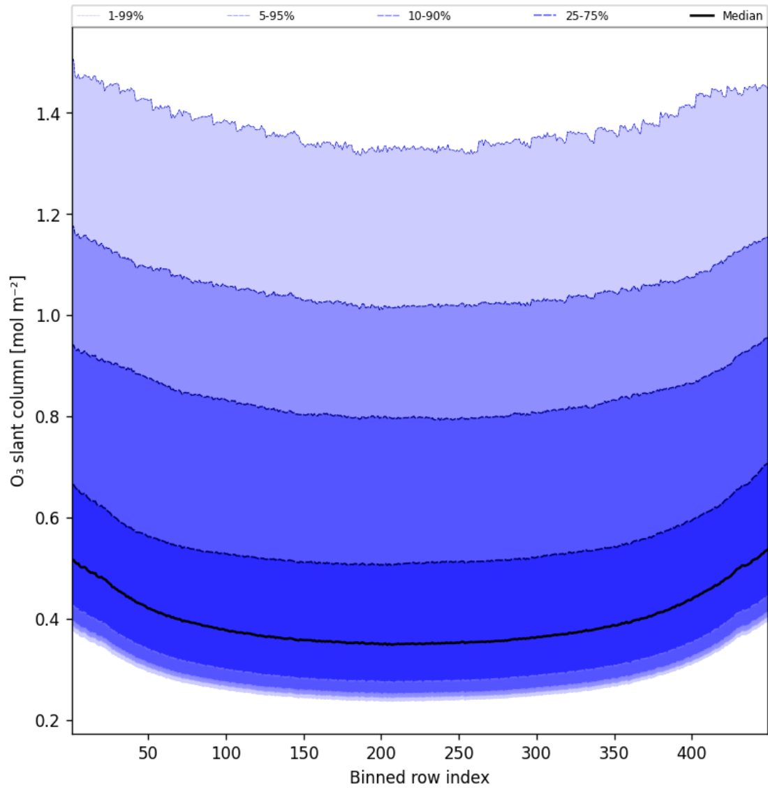
Figure 43: Along track statistics of “O 3 slant column” for 2025-11-03 to 2025-11-04
