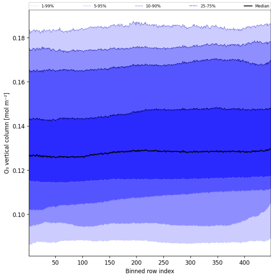
Figure 41: Along track statistics of “O 3 vertical column” for 2025-11-03 to 2025-11-04
