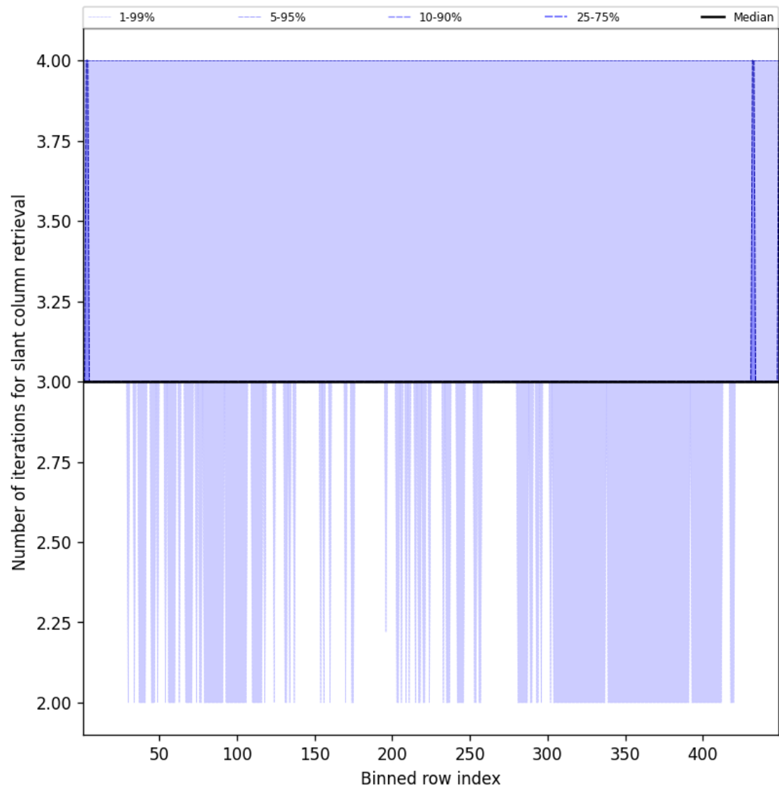
Figure 45: Along track statistics of “Number of iterations for slant column retrieval” for 2025-11-03 to 2025-11-04
