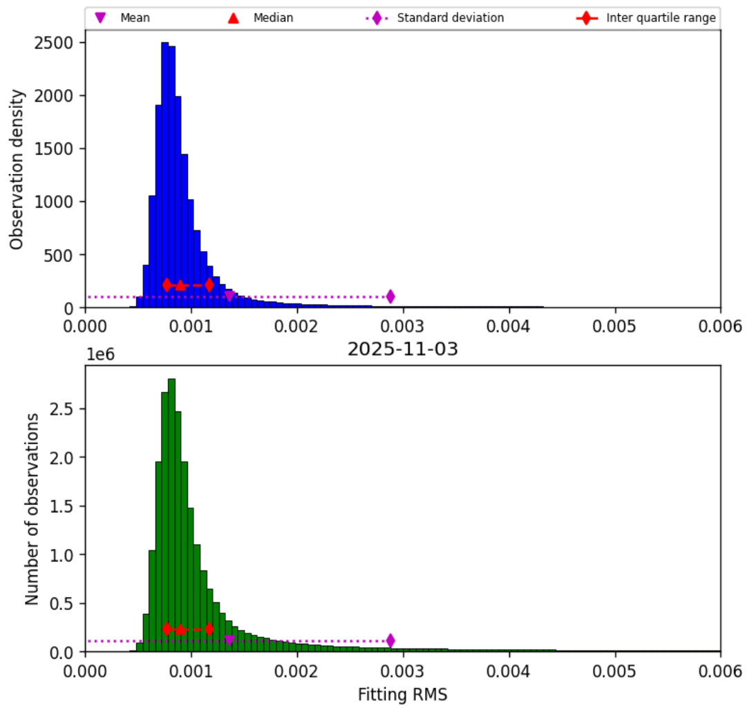
Figure 34: Histogram of “Fitting RMS” for 2025-11-03 to 2025-11-04
