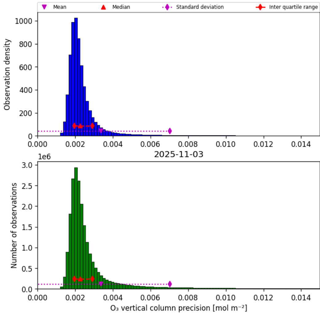
Figure 30: Histogram of “O 3 vertical column precision” for 2025-11-03 to 2025-11-04
