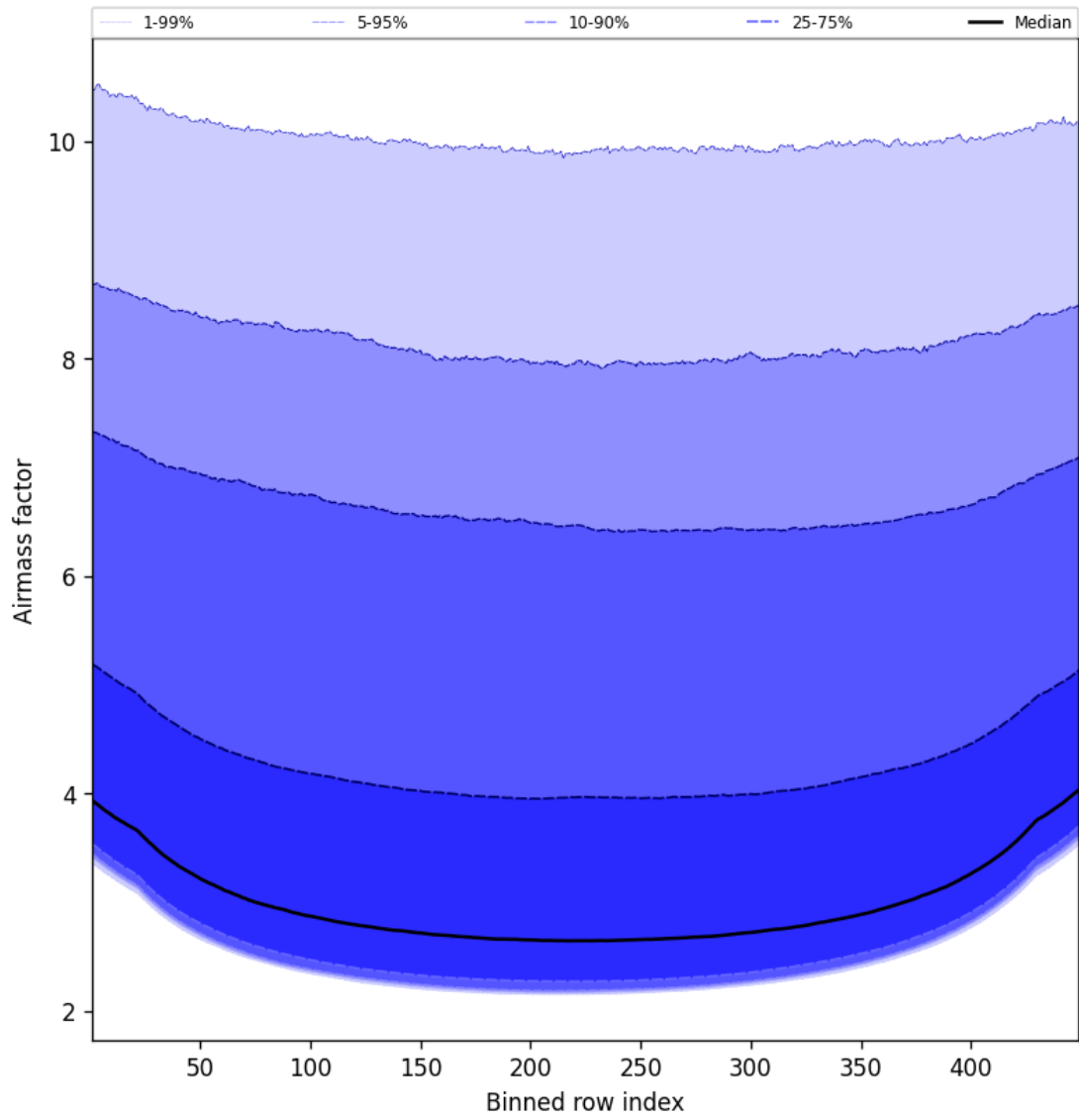
Figure 49: Along track statistics of “Airmass factor” for 2025-11-03 to 2025-11-04
