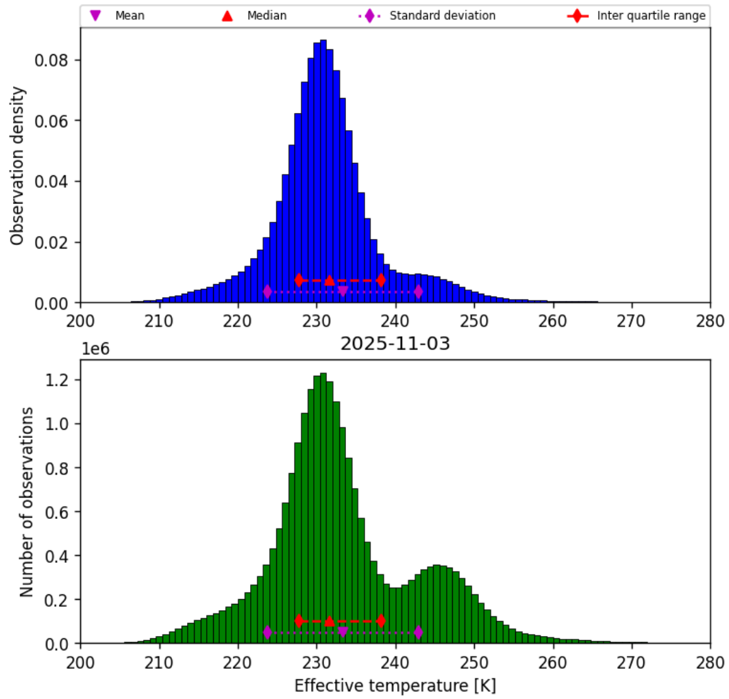
Figure 38: Histogram of “Effective temperature” for 2025-11-03 to 2025-11-04
