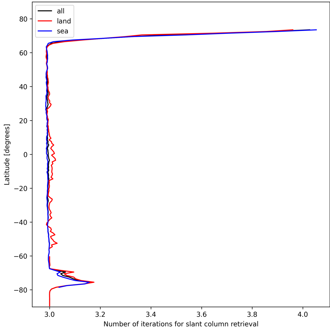
Figure 21: Zonal average of “Number of iterations for slant column retrieval” for 2025-11-03 to 2025-11-04.
