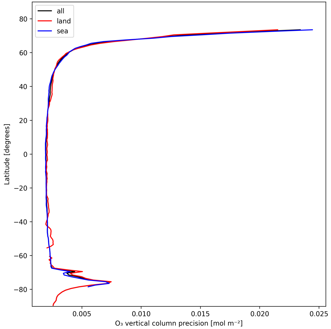
Figure 18: Zonal average of “O 3 vertical column precision” for 2025-11-03 to 2025-11-04.
