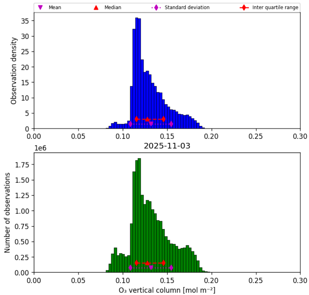
Figure 29: Histogram of “O 3 vertical column” for 2025-11-03 to 2025-11-04
