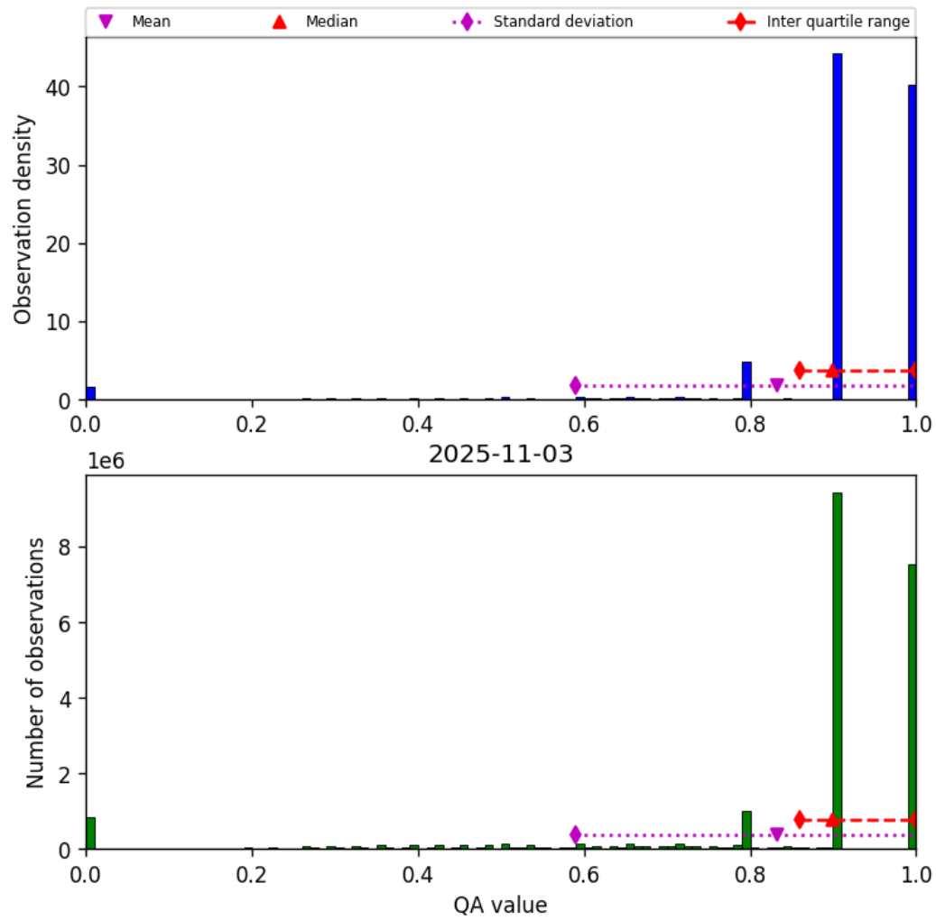
Figure 28: Histogram of “QA value” for 2025-11-03 to 2025-11-04
