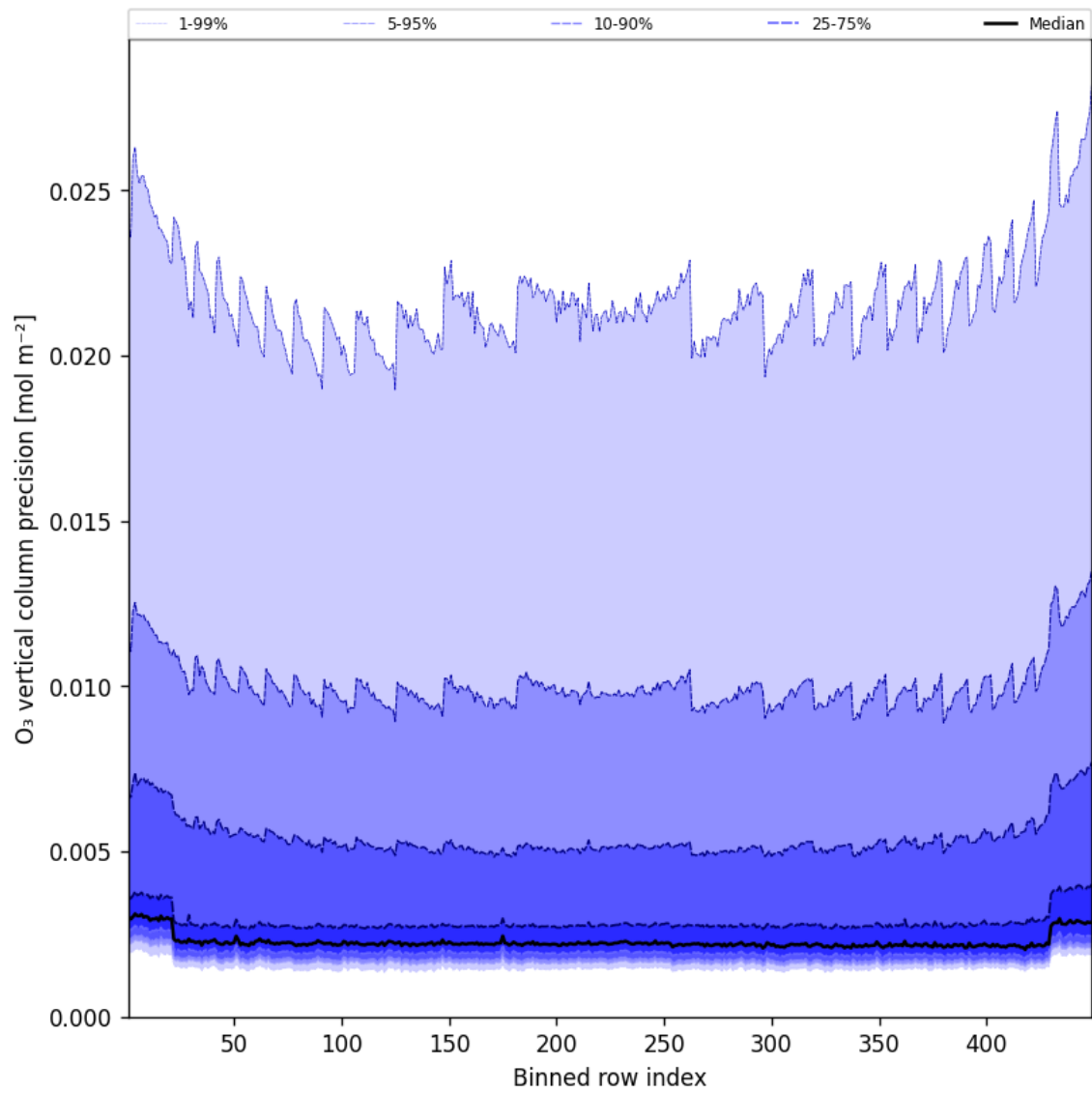
Figure 42: Along track statistics of “O 3 vertical column precision” for 2025-11-03 to 2025-11-04
