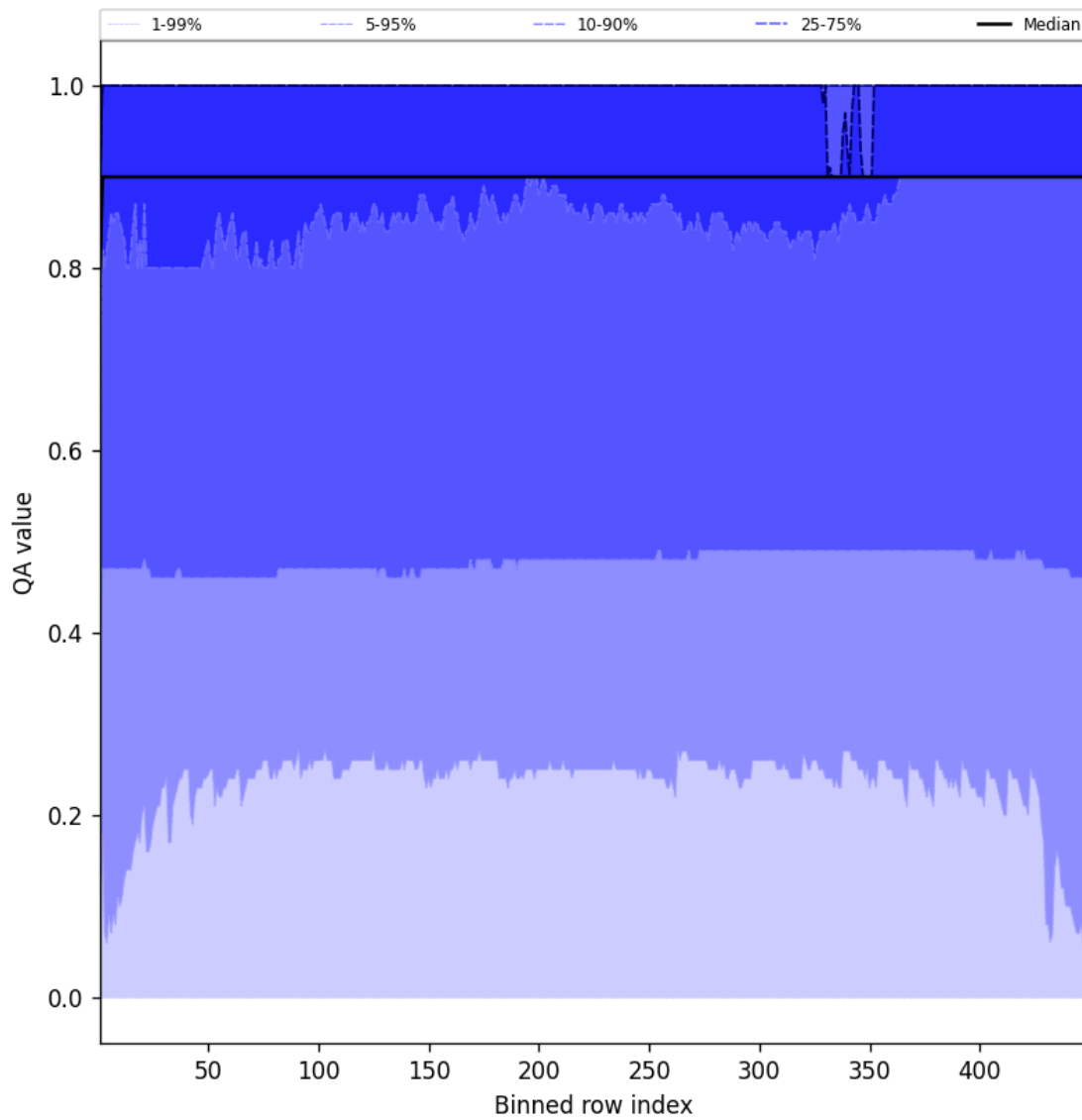
Figure 40: Along track statistics of “QA value” for 2025-11-03 to 2025-11-04
