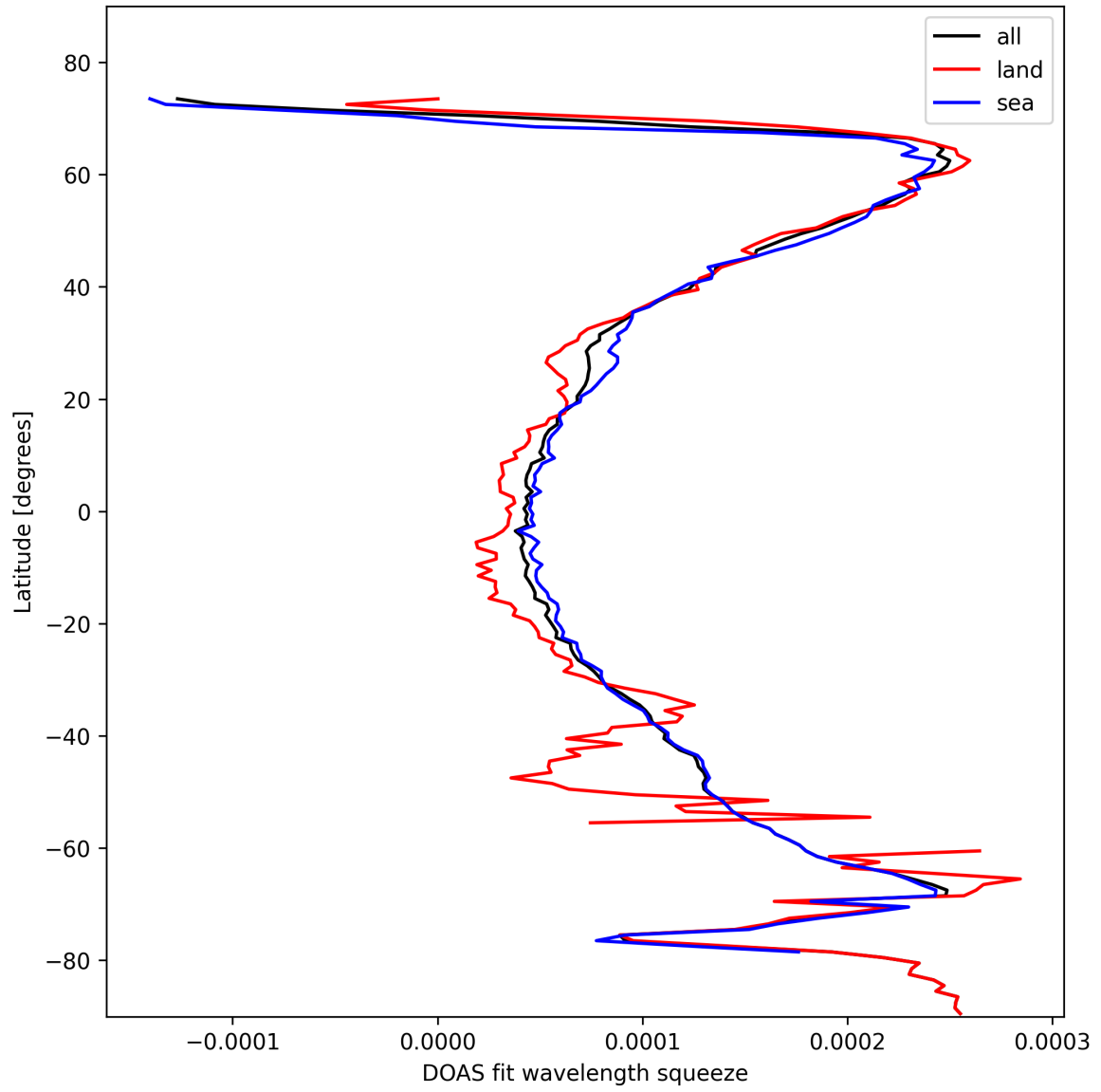
Figure 24: Zonal average of “DOAS fit wavelength squeeze” for 2025-11-03 to 2025-11-04.
