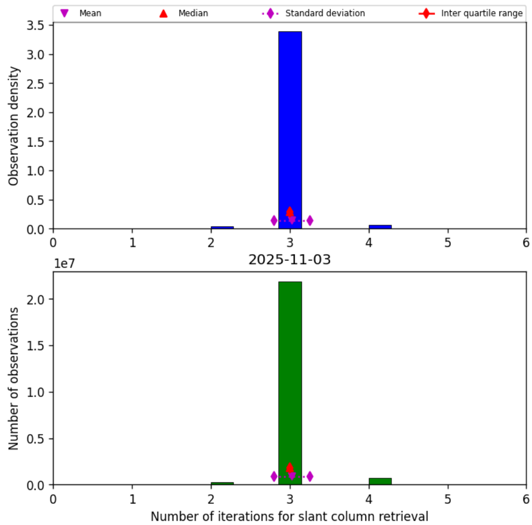
Figure 33: Histogram of “Number of iterations for slant column retrieval” for 2025-11-03 to 2025-11-04
