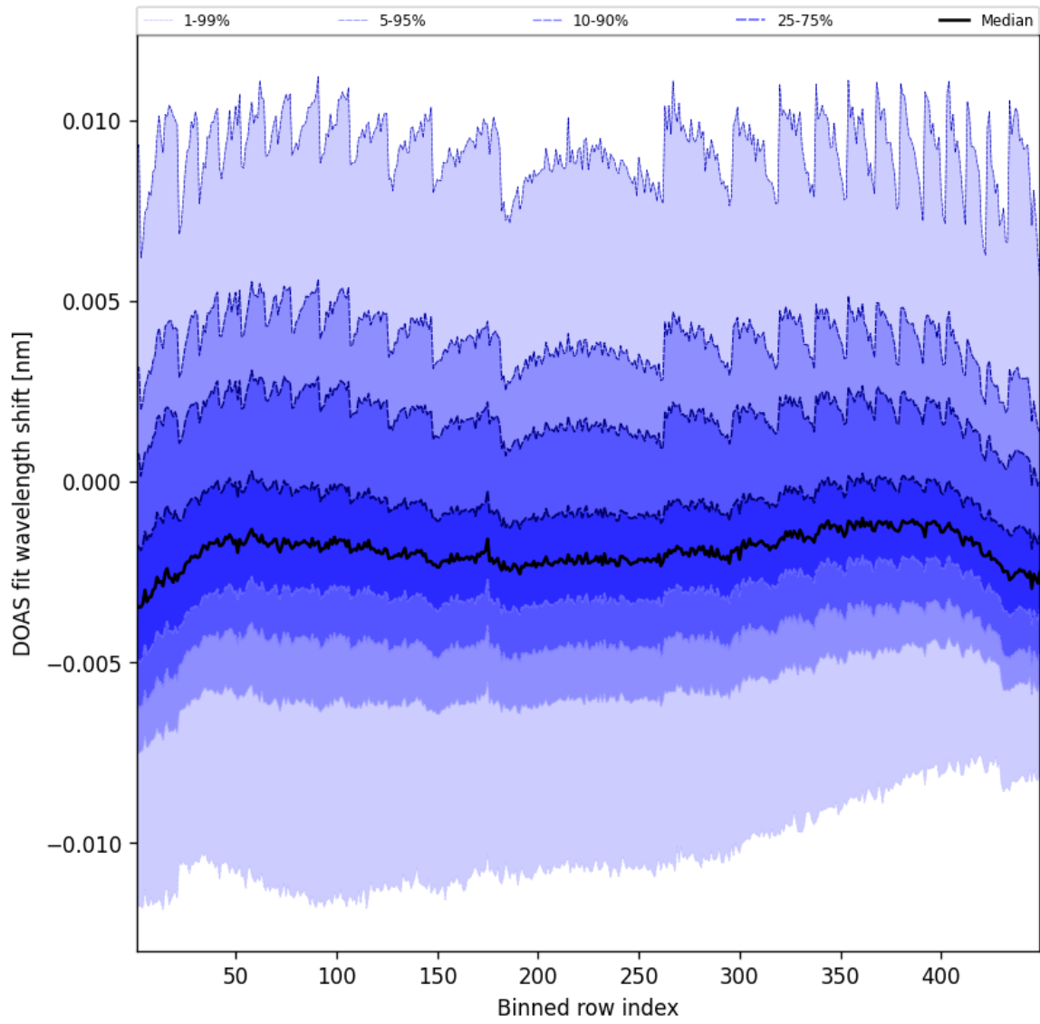
Figure 47: Along track statistics of “DOAS fit wavelength shift” for 2025-11-03 to 2025-11-04
