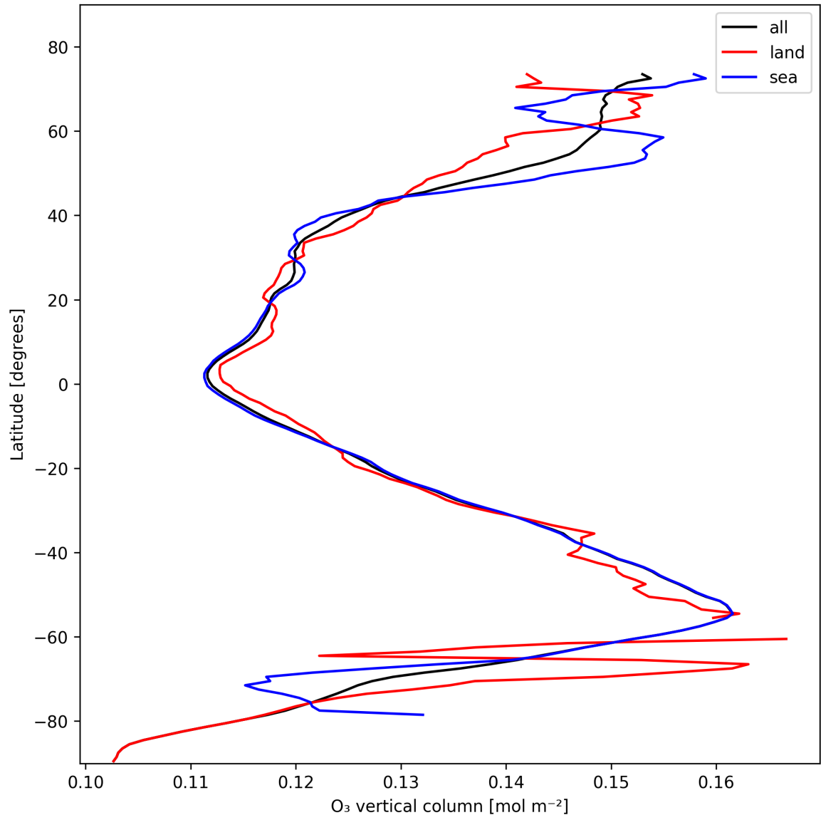
Figure 17: Zonal average of “O 3 vertical column” for 2025-11-03 to 2025-11-04.
