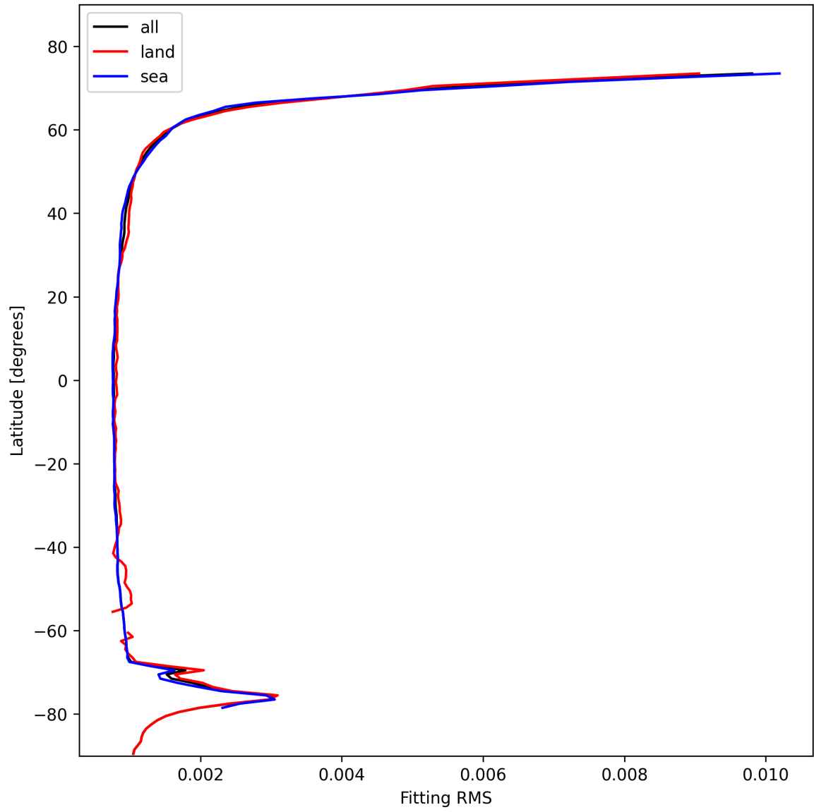
Figure 22: Zonal average of “Fitting RMS” for 2025-11-03 to 2025-11-04.
