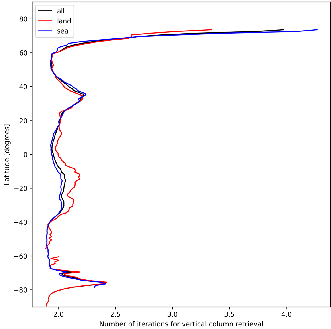
Figure 27: Zonal average of “Number of iterations for vertical column retrieval” for 2025-11-03 to 2025-11-04.
