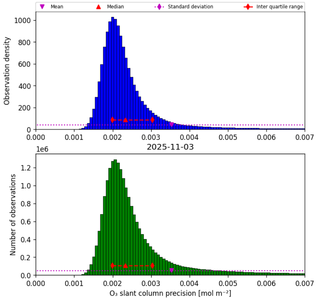
Figure 32: Histogram of “O 3 slant column precision” for 2025-11-03 to 2025-11-04
