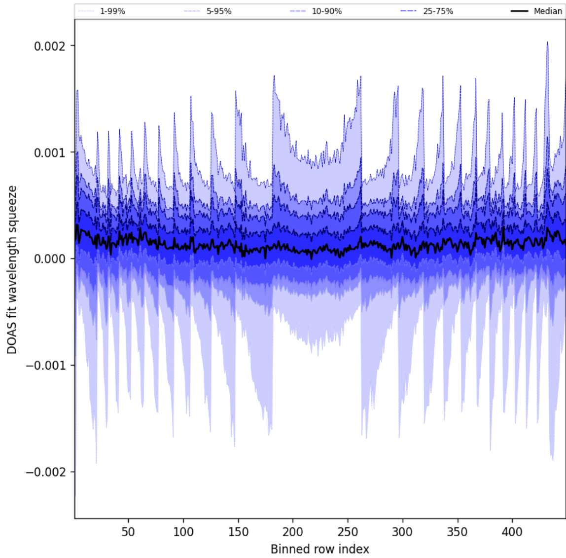
Figure 48: Along track statistics of “DOAS fit wavelength squeeze” for 2025-11-03 to 2025-11-04
