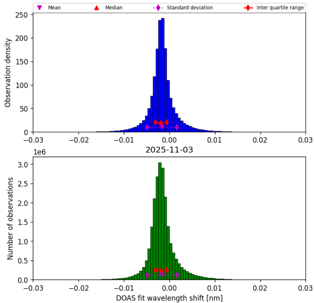
Figure 35: Histogram of “DOAS fit wavelength shift” for 2025-11-03 to 2025-11-04
