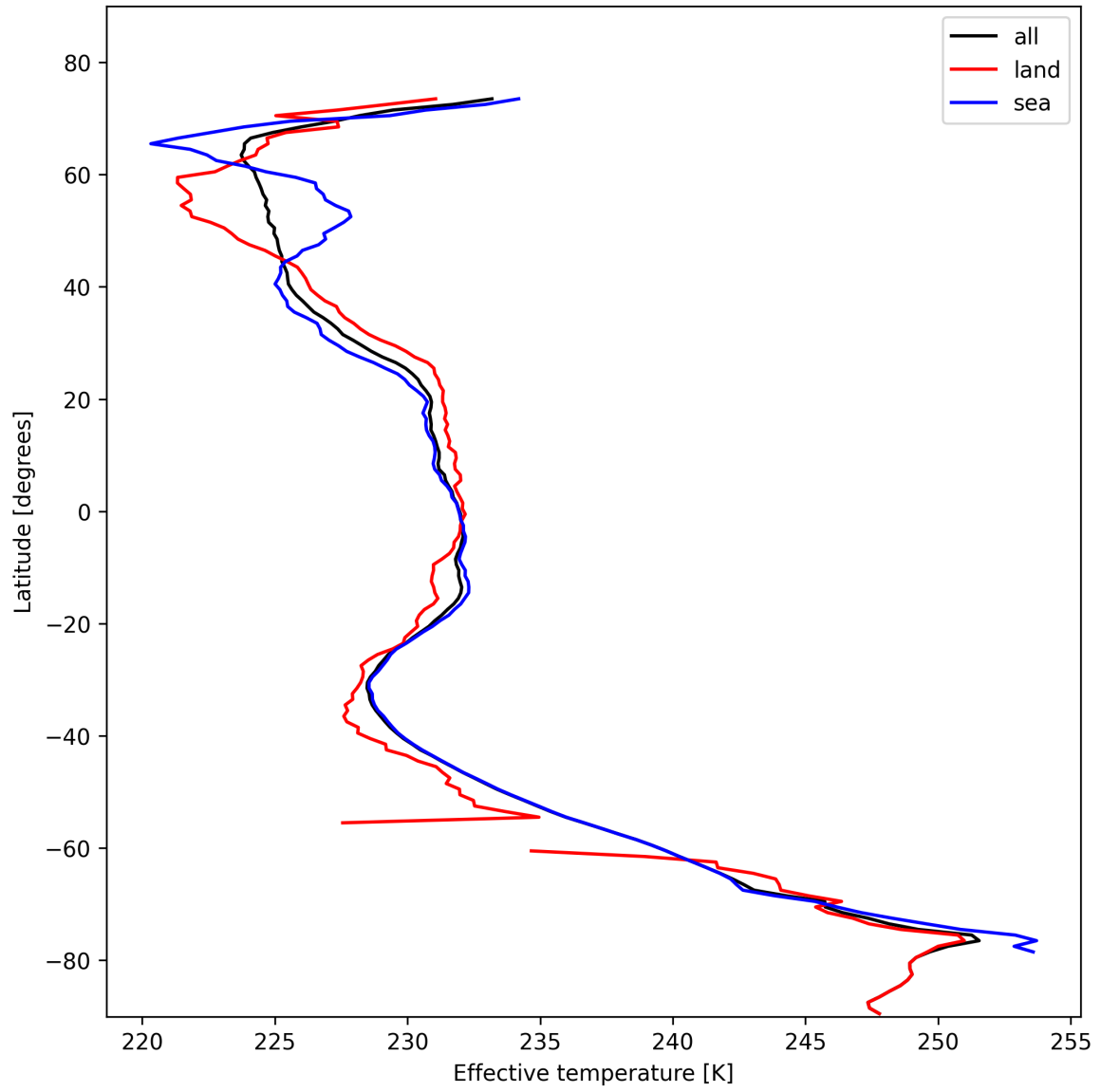
Figure 26: Zonal average of “Effective temperature” for 2025-11-03 to 2025-11-04.
