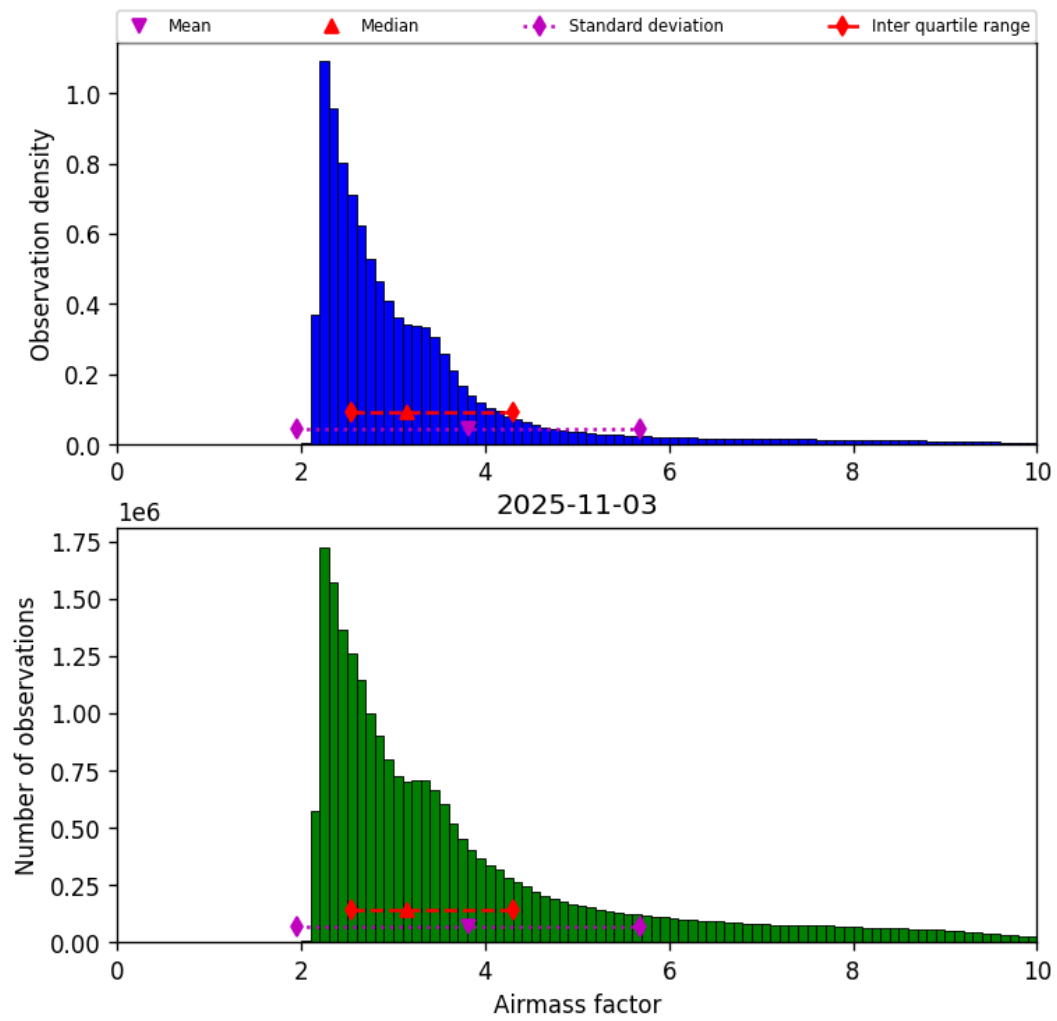
Figure 37: Histogram of “Airmass factor” for 2025-11-03 to 2025-11-04
