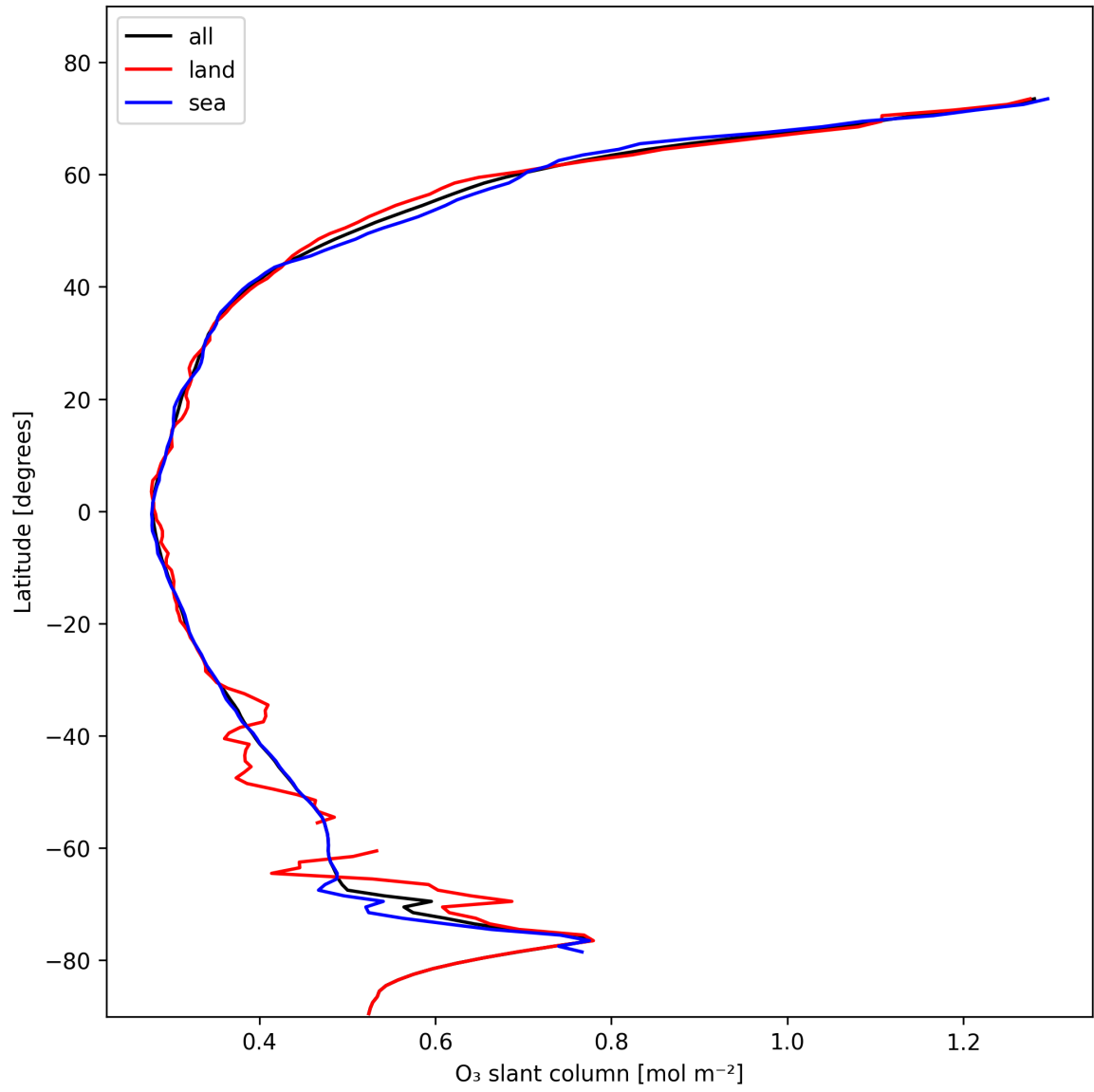
Figure 19: Zonal average of “O 3 slant column” for 2025-11-03 to 2025-11-04.
