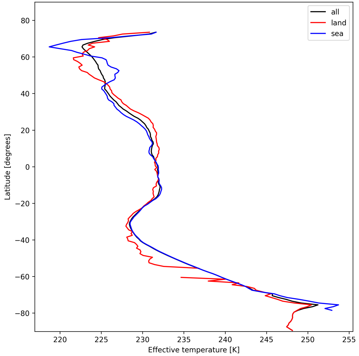
Figure 26: Zonal average of “Effective temperature” for 2025-11-04 to 2025-11-05.
