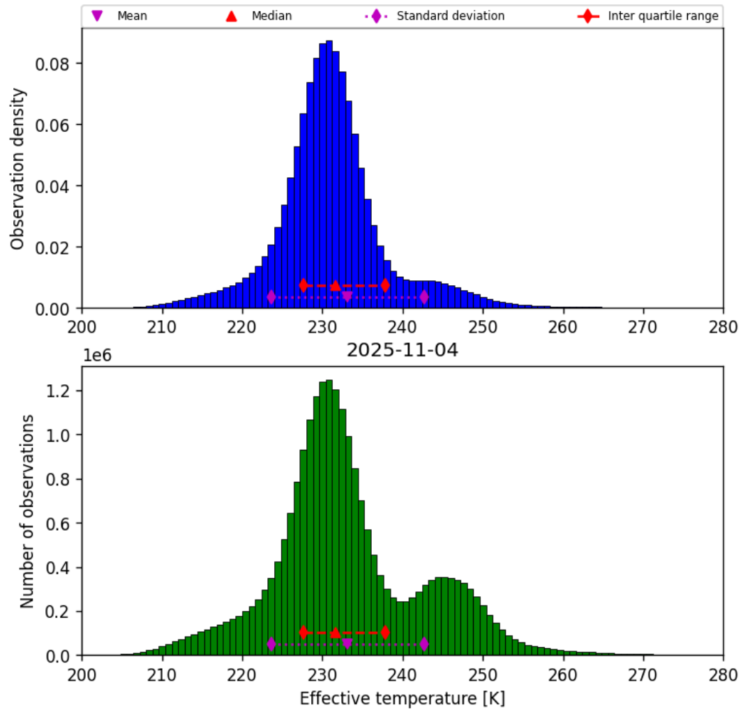
Figure 38: Histogram of “Effective temperature” for 2025-11-04 to 2025-11-05
