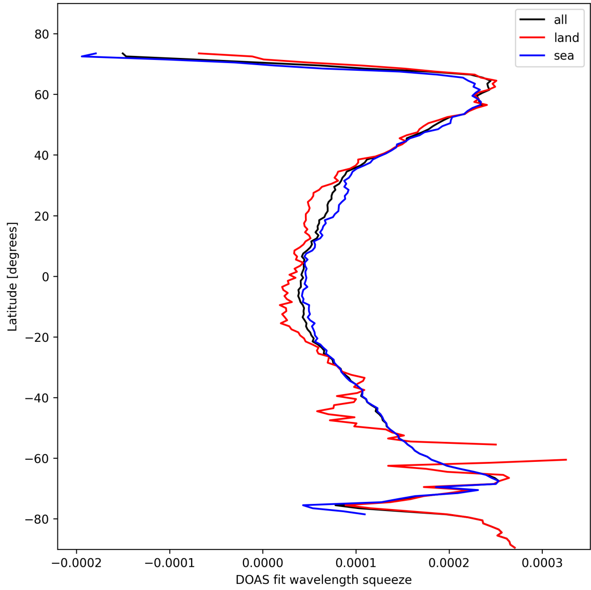
Figure 24: Zonal average of “DOAS fit wavelength squeeze” for 2025-11-04 to 2025-11-05.
