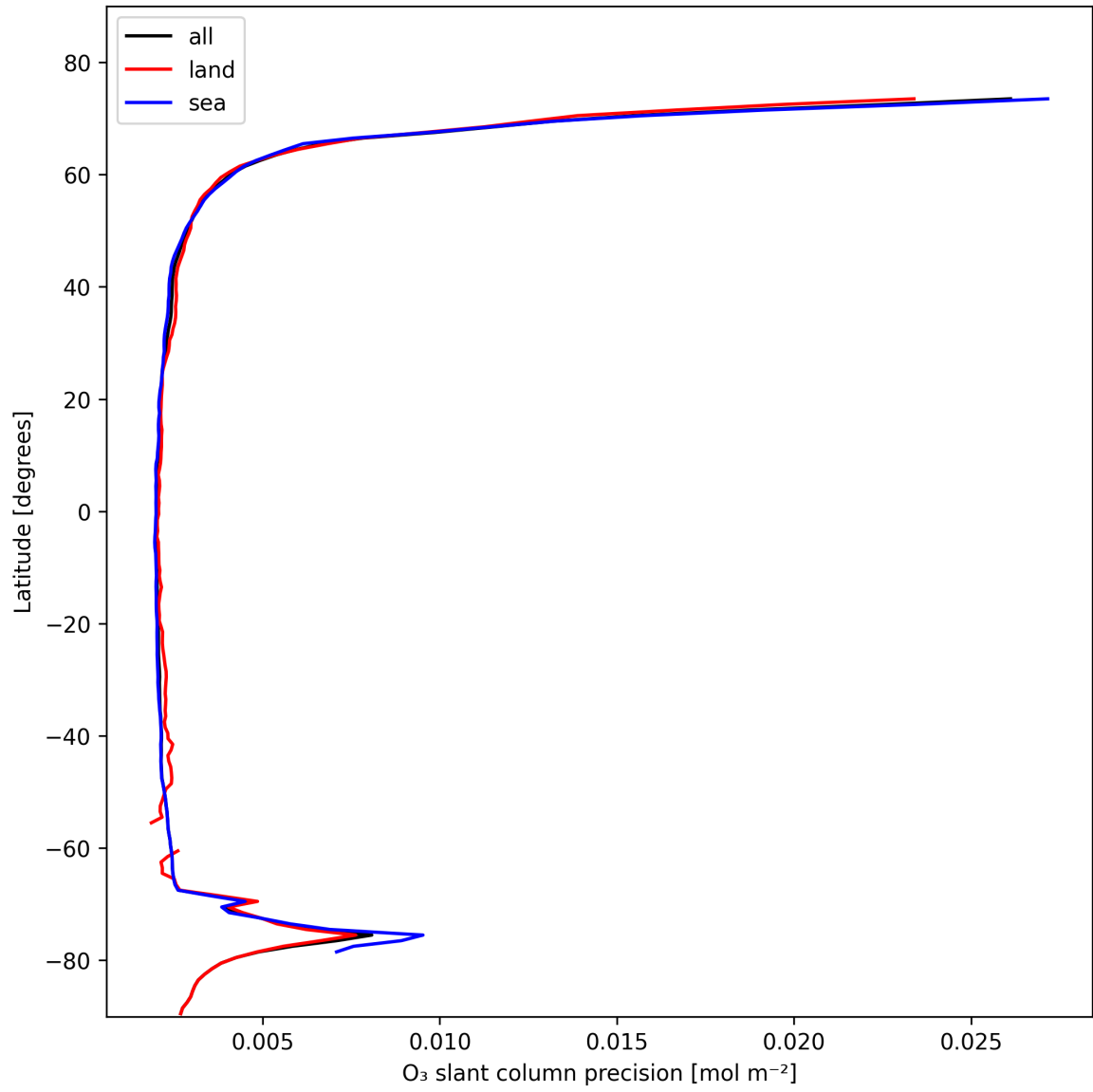
Figure 20: Zonal average of “O 3 slant column precision” for 2025-11-04 to 2025-11-05.
