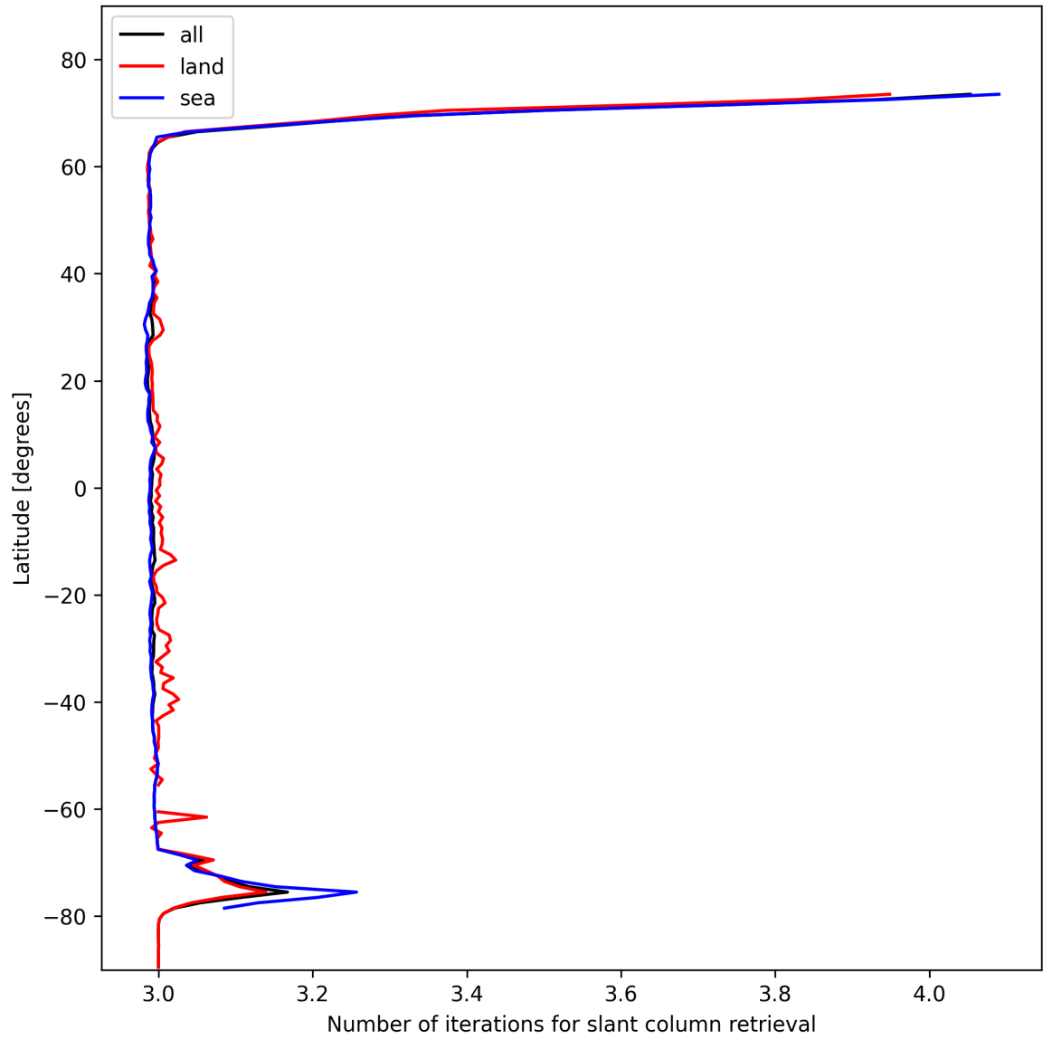
Figure 21: Zonal average of “Number of iterations for slant column retrieval” for 2025-11-04 to 2025-11-05.
