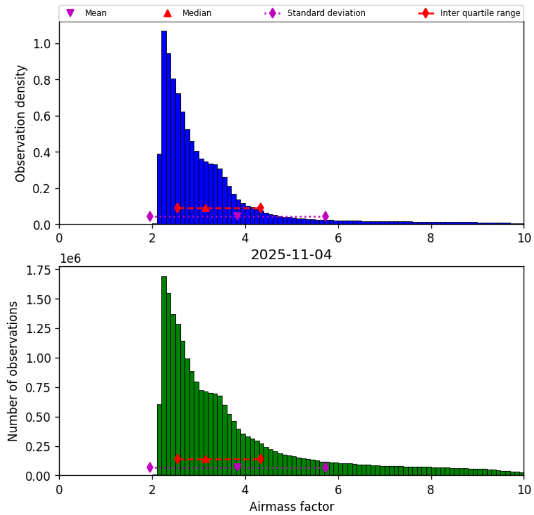
Figure 37: Histogram of “Airmass factor” for 2025-11-04 to 2025-11-05
