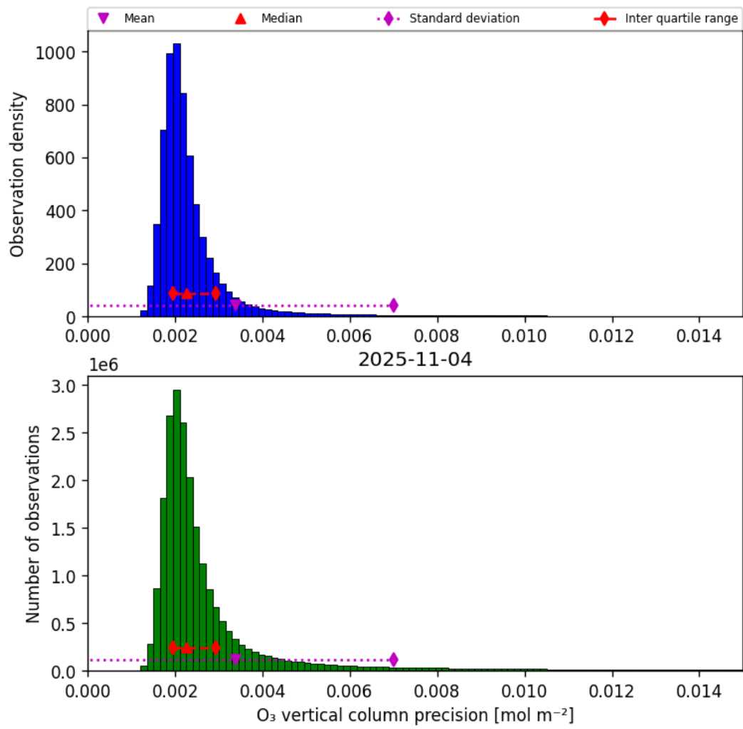
Figure 30: Histogram of “O 3 vertical column precision” for 2025-11-04 to 2025-11-05
