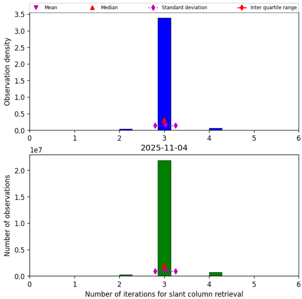
Figure 33: Histogram of “Number of iterations for slant column retrieval” for 2025-11-04 to 2025-11-05
