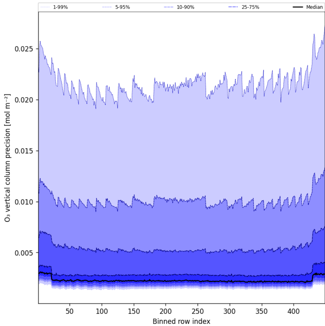
Figure 42: Along track statistics of “O 3 vertical column precision” for 2025-11-04 to 2025-11-05
