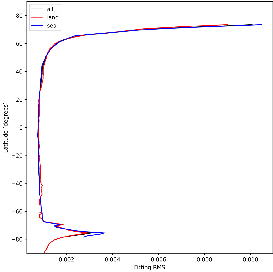
Figure 22: Zonal average of “Fitting RMS” for 2025-11-04 to 2025-11-05.
