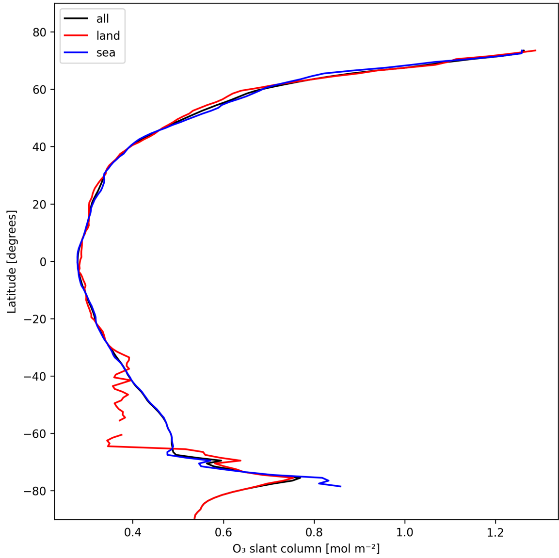
Figure 19: Zonal average of “O 3 slant column” for 2025-11-04 to 2025-11-05.
