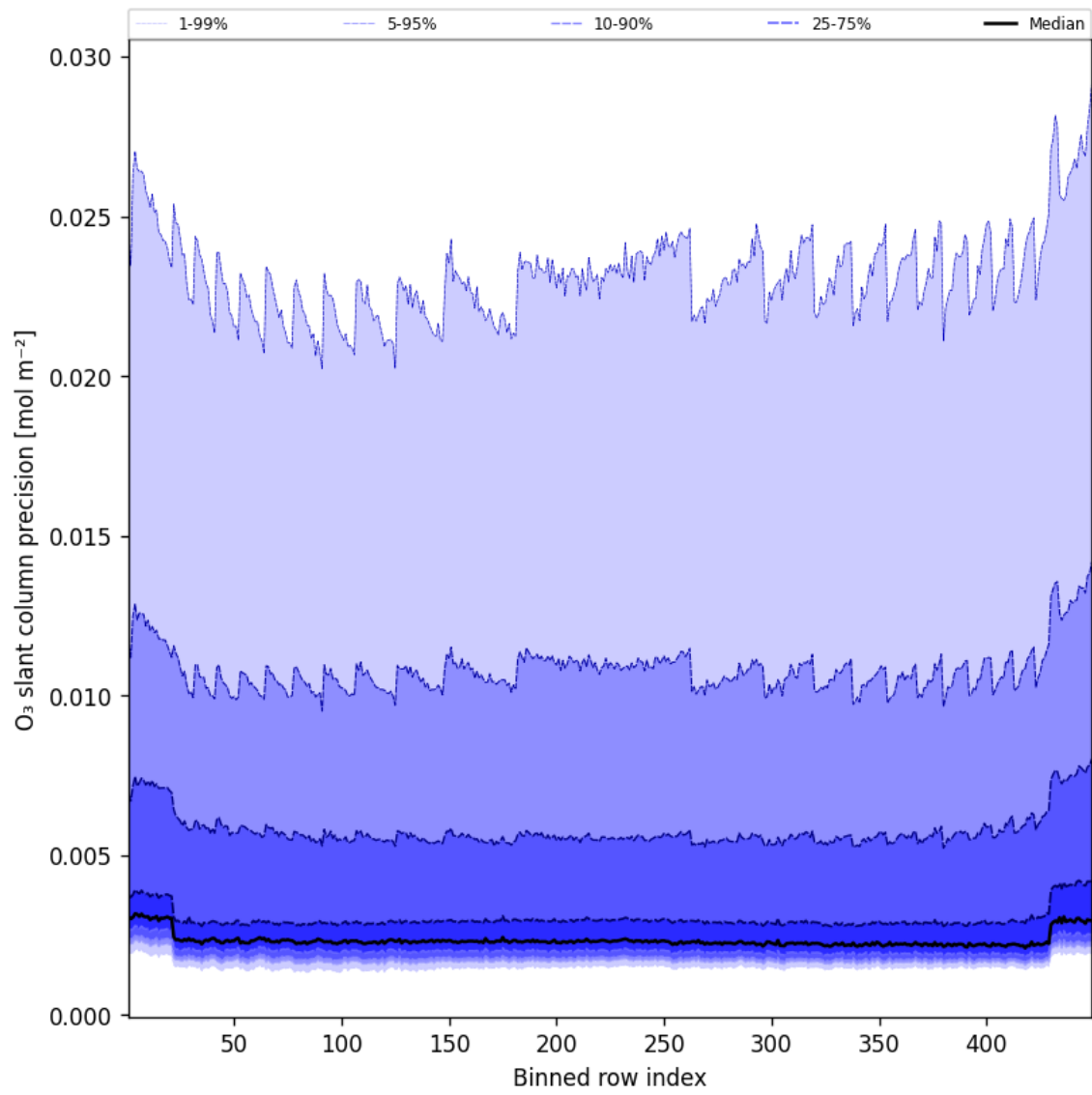
Figure 44: Along track statistics of “O 3 slant column precision” for 2025-11-04 to 2025-11-05
