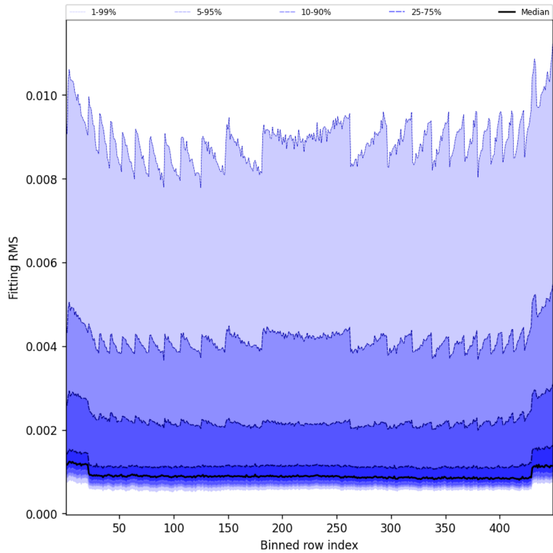
Figure 46: Along track statistics of “Fitting RMS” for 2025-11-04 to 2025-11-05
