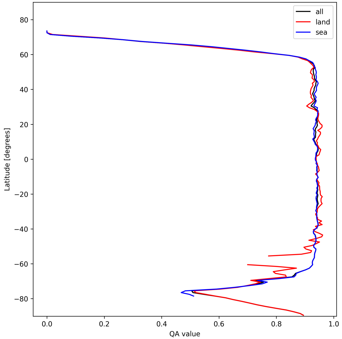
Figure 16: Zonal average of “QA value” for 2025-11-04 to 2025-11-05.
