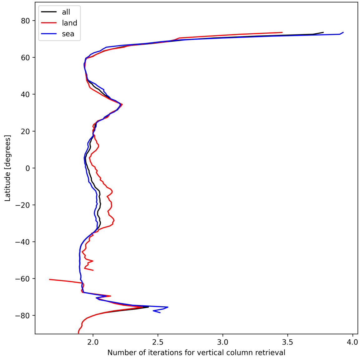
Figure 27: Zonal average of “Number of iterations for vertical column retrieval” for 2025-11-04 to 2025-11-05.
