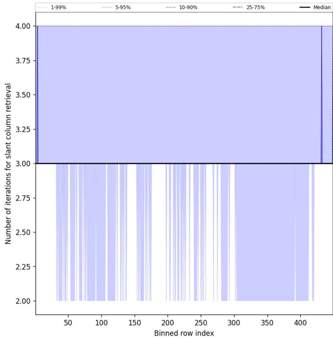
Figure 45: Along track statistics of “Number of iterations for slant column retrieval” for 2025-11-04 to 2025-11-05
