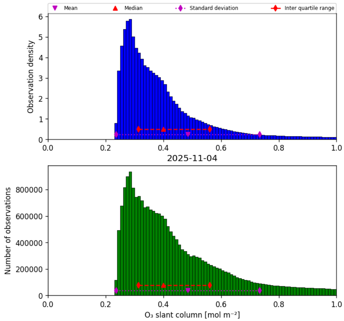
Figure 31: Histogram of “O 3 slant column” for 2025-11-04 to 2025-11-05
