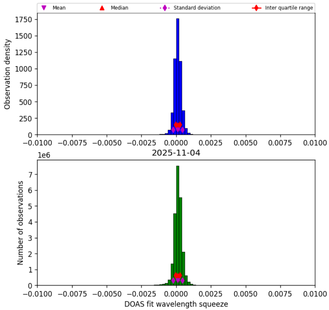
Figure 36: Histogram of “DOAS fit wavelength squeeze” for 2025-11-04 to 2025-11-05
