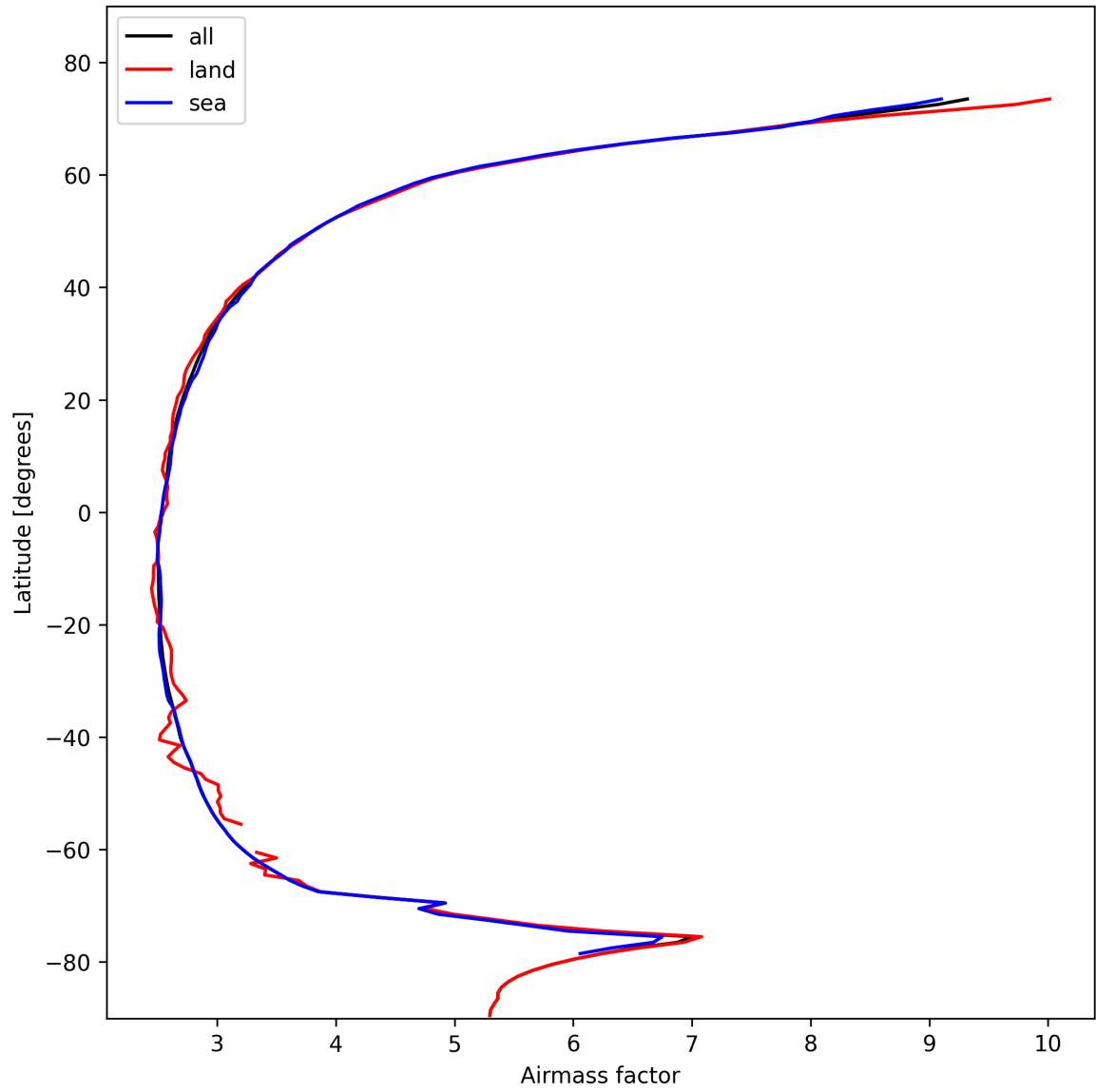
Figure 25: Zonal average of “Airmass factor” for 2025-11-04 to 2025-11-05.
