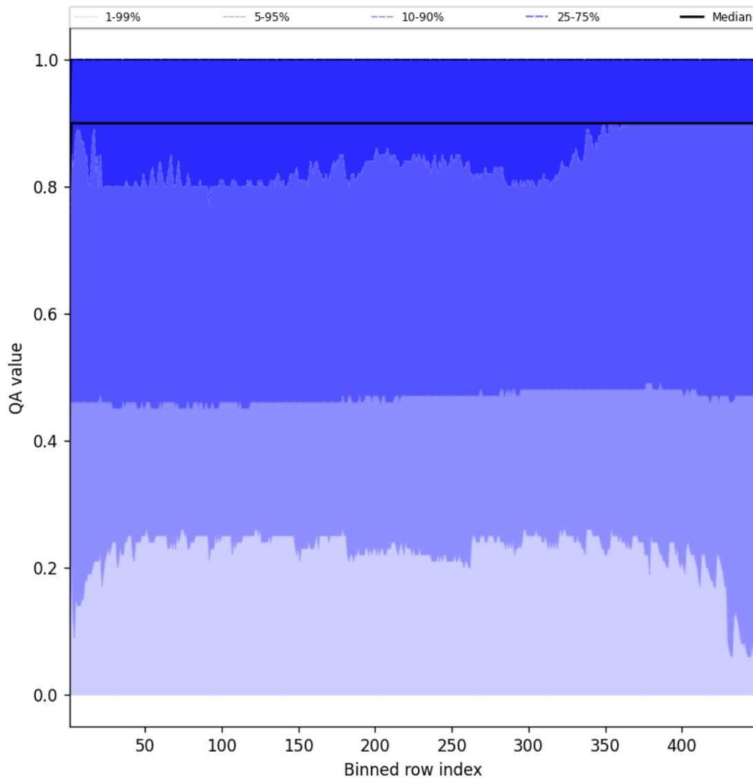
Figure 40: Along track statistics of “QA value” for 2025-11-04 to 2025-11-05
