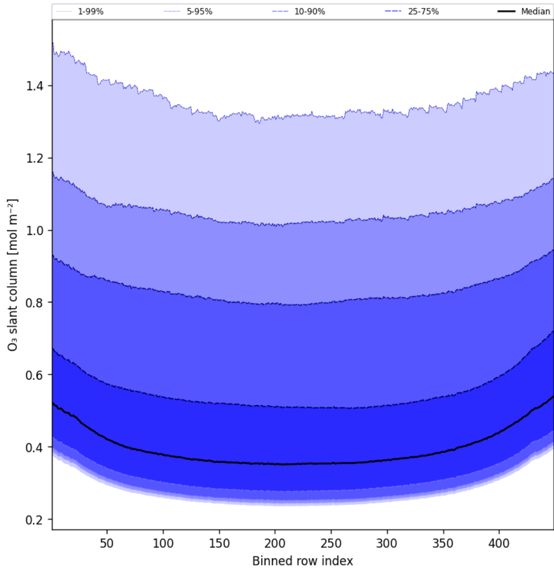
Figure 43: Along track statistics of “O 3 slant column” for 2025-11-04 to 2025-11-05
