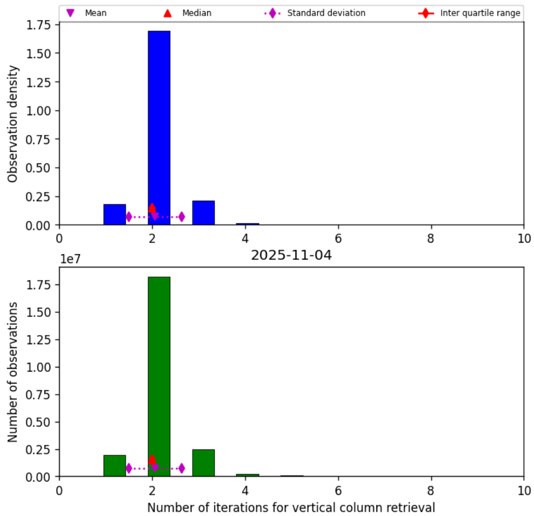
Figure 39: Histogram of “Number of iterations for vertical column retrieval” for 2025-11-04 to 2025-11-05
