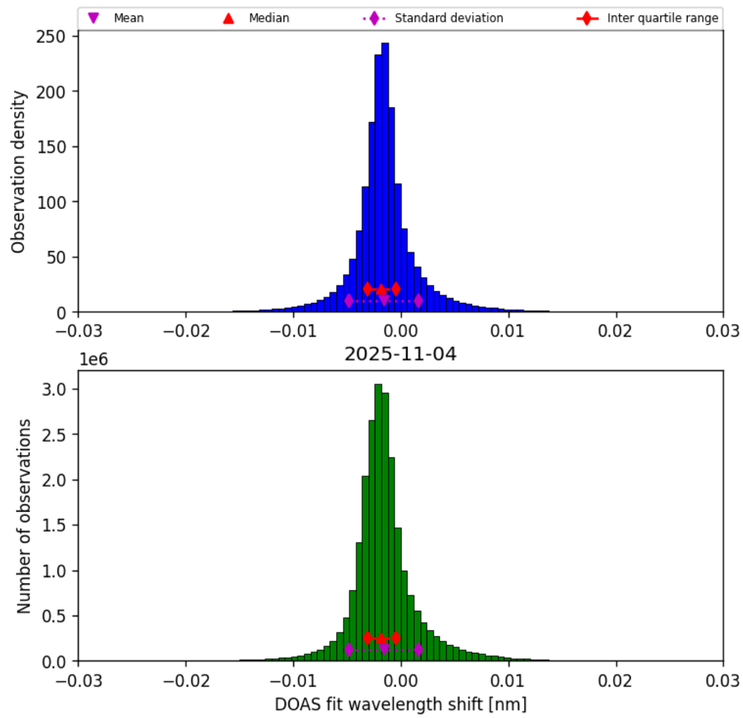
Figure 35: Histogram of “DOAS fit wavelength shift” for 2025-11-04 to 2025-11-05
