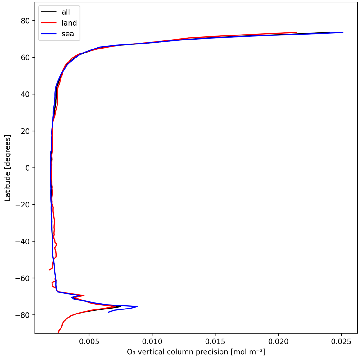
Figure 18: Zonal average of “O 3 vertical column precision” for 2025-11-04 to 2025-11-05.
