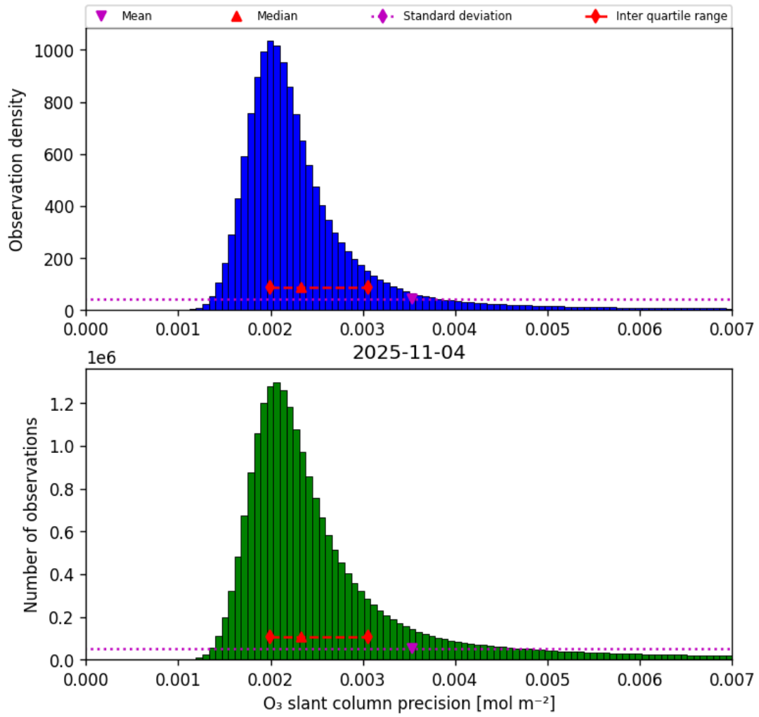
Figure 32: Histogram of “O 3 slant column precision” for 2025-11-04 to 2025-11-05
