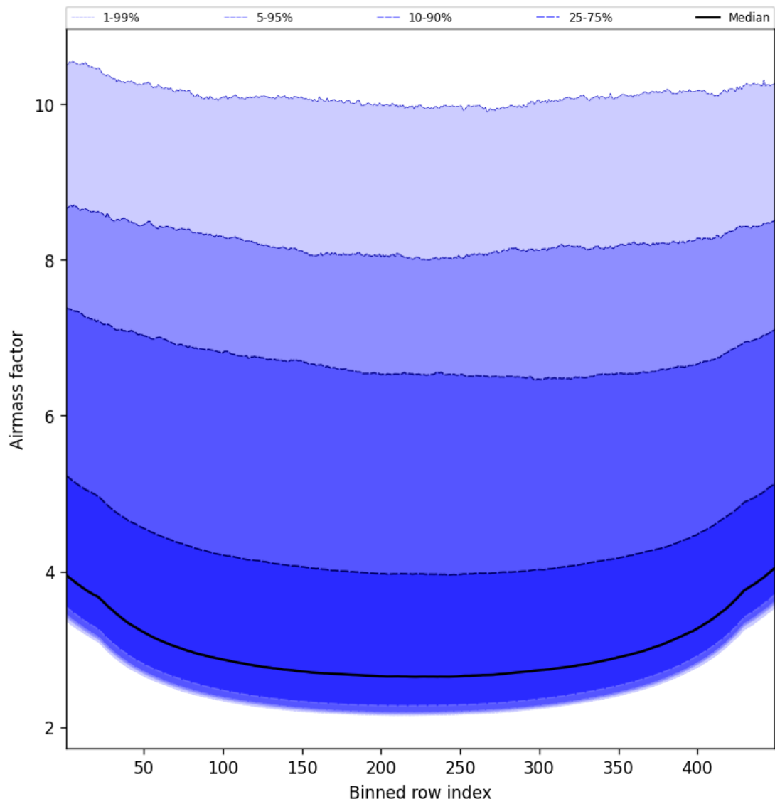
Figure 49: Along track statistics of “Airmass factor” for 2025-11-04 to 2025-11-05
