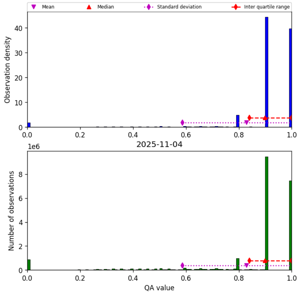
Figure 28: Histogram of “QA value” for 2025-11-04 to 2025-11-05
