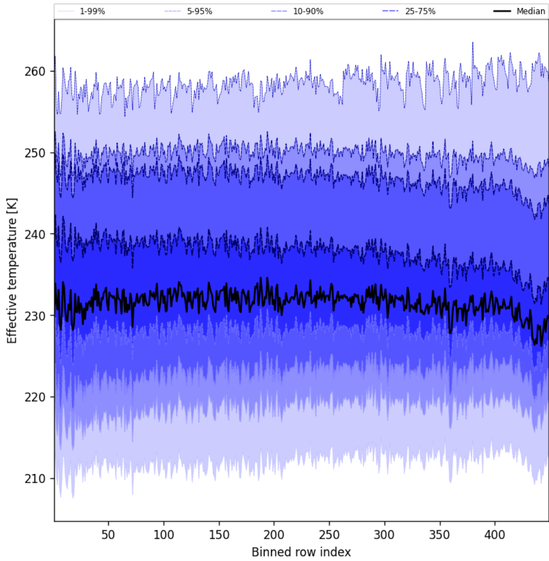
Figure 50: Along track statistics of “Effective temperature” for 2025-11-04 to 2025-11-05
