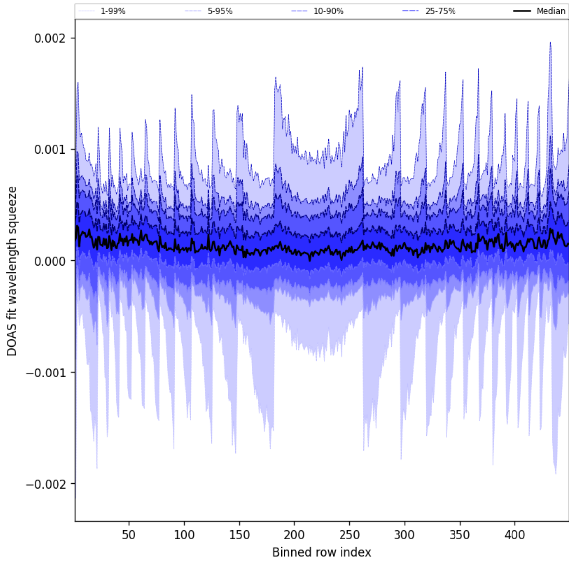
Figure 48: Along track statistics of “DOAS fit wavelength squeeze” for 2025-11-04 to 2025-11-05
