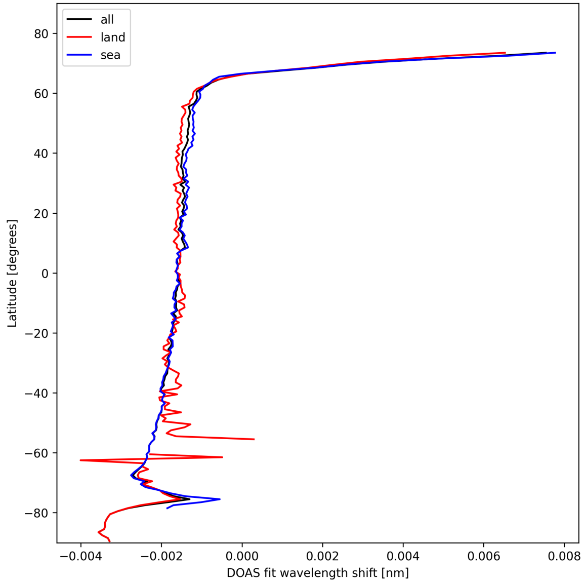
Figure 23: Zonal average of “DOAS fit wavelength shift” for 2025-11-04 to 2025-11-05.
