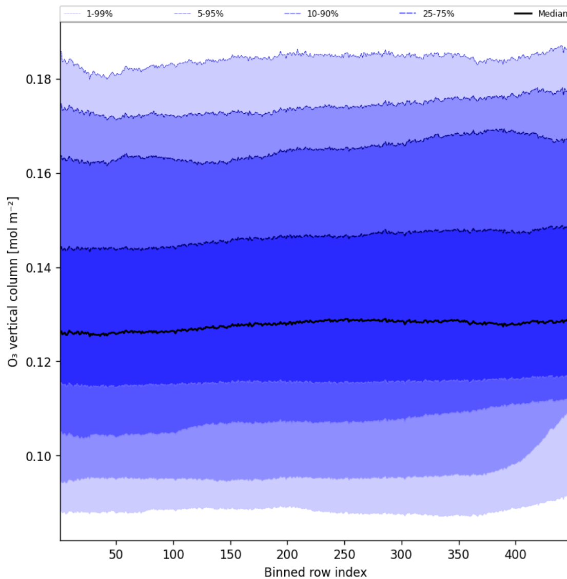
Figure 41: Along track statistics of “O 3 vertical column” for 2025-11-04 to 2025-11-05
