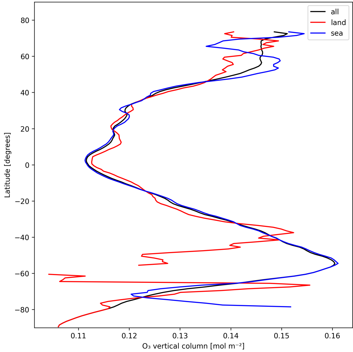
Figure 17: Zonal average of “O 3 vertical column” for 2025-11-04 to 2025-11-05.
