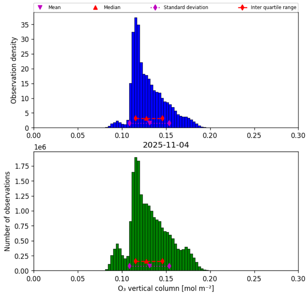
Figure 29: Histogram of “O 3 vertical column” for 2025-11-04 to 2025-11-05
