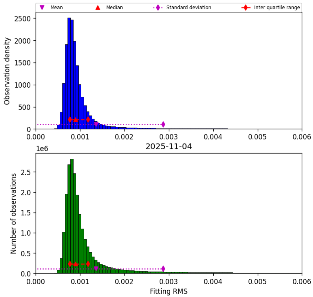
Figure 34: Histogram of “Fitting RMS” for 2025-11-04 to 2025-11-05
