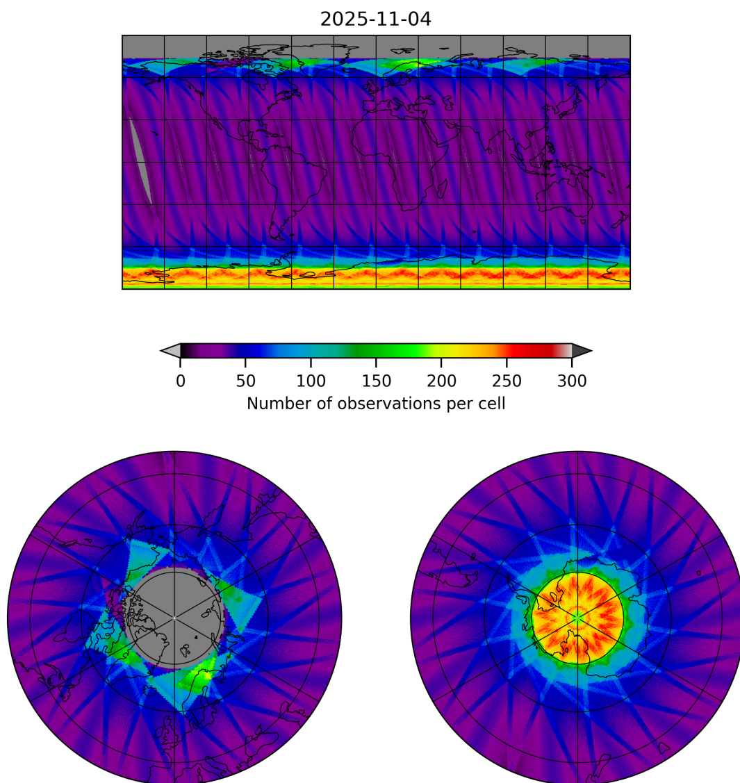
Figure 15: Map of the number of observations for 2025-11-04 to 2025-11-05
