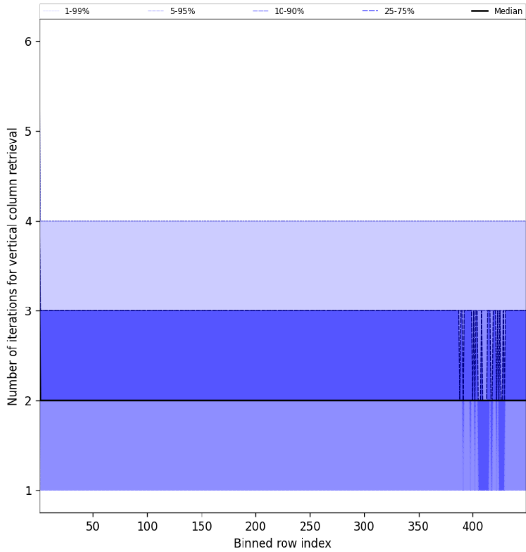
Figure 51: Along track statistics of “Number of iterations for vertical column retrieval” for 2025-11-04 to 2025-11-05
