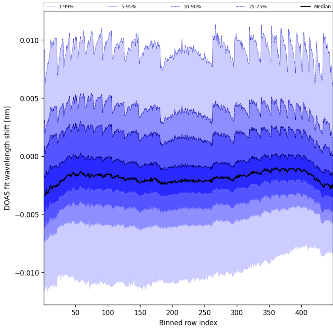
Figure 47: Along track statistics of “DOAS fit wavelength shift” for 2025-11-04 to 2025-11-05
