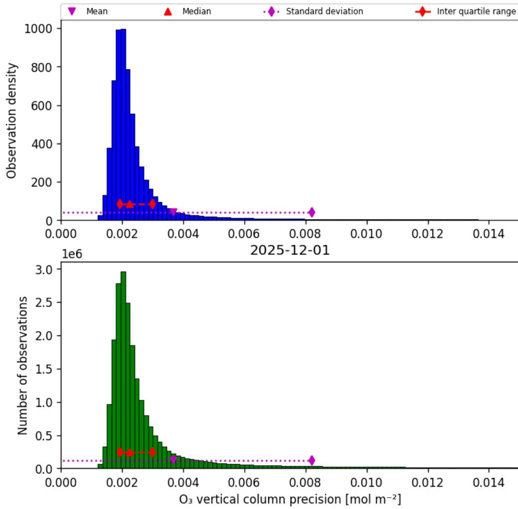
Figure 30: Histogram of “O 3 vertical column precision” for 2025-12-01 to 2025-12-01
