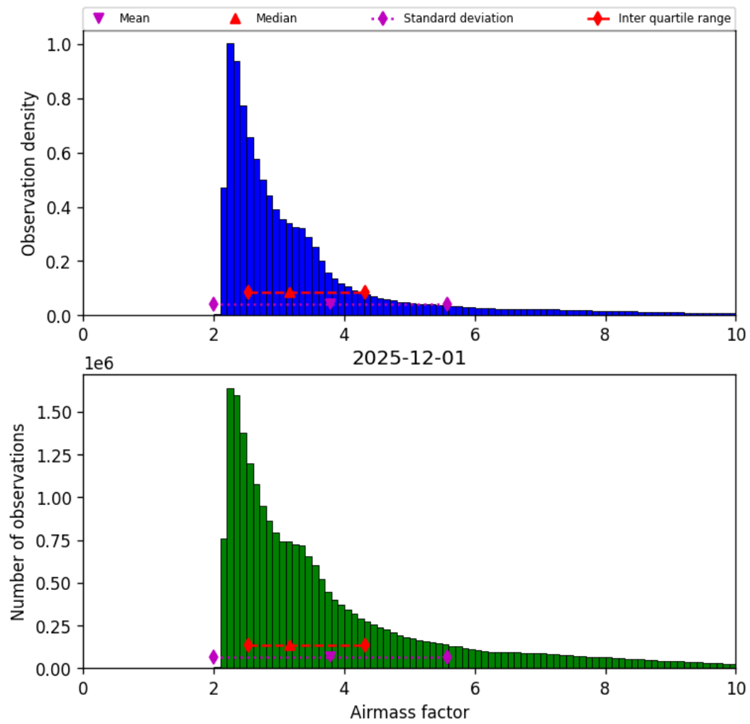
Figure 37: Histogram of “Airmass factor” for 2025-12-01 to 2025-12-01
