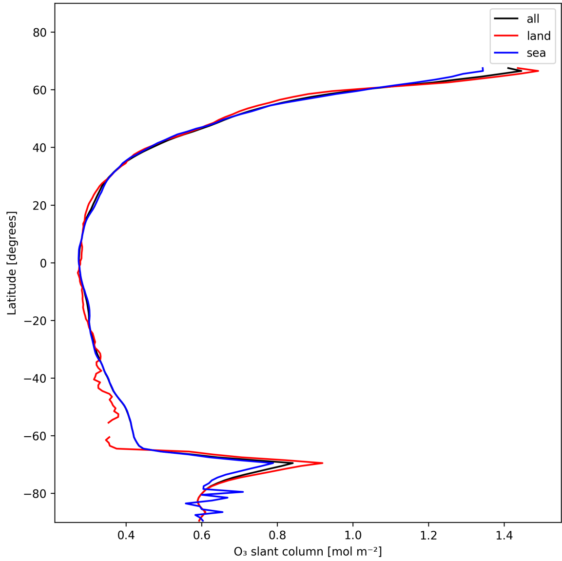
Figure 19: Zonal average of “O 3 slant column” for 2025-12-01 to 2025-12-01.
