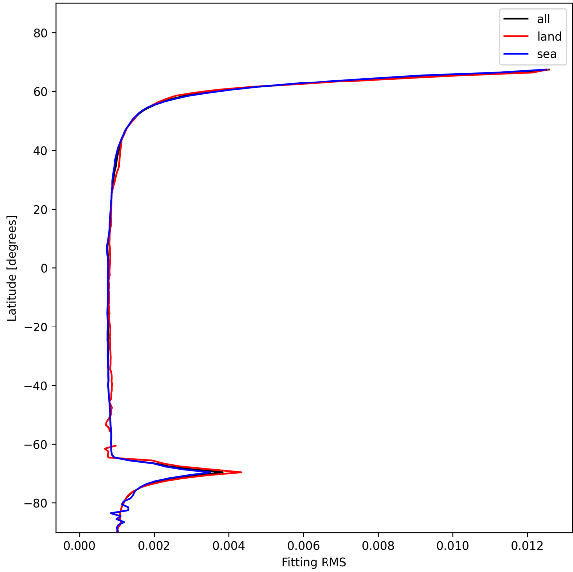
Figure 22: Zonal average of “Fitting RMS” for 2025-12-01 to 2025-12-01.
