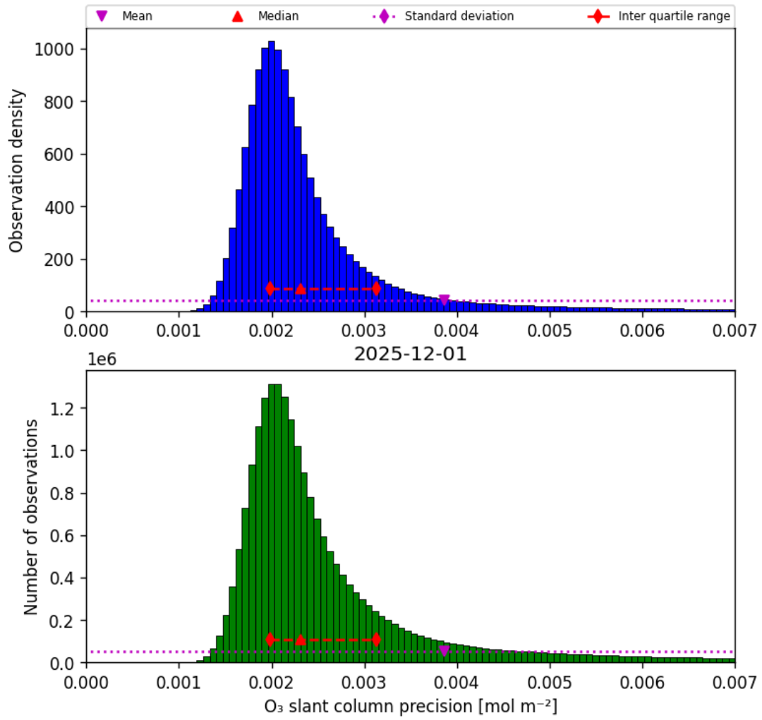
Figure 32: Histogram of “O 3 slant column precision” for 2025-12-01 to 2025-12-01
