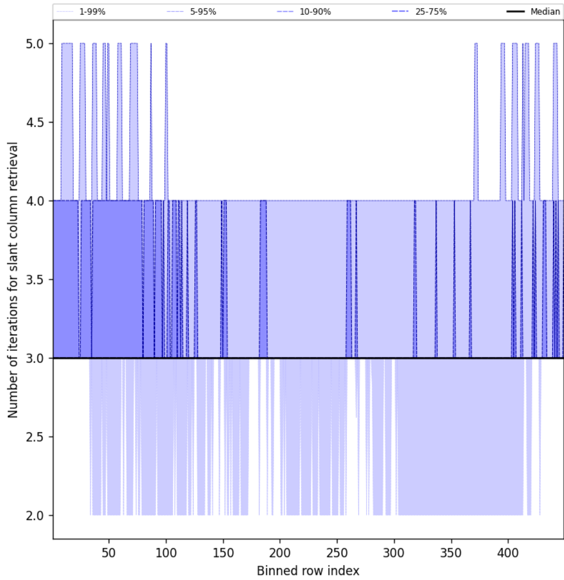
Figure 45: Along track statistics of “Number of iterations for slant column retrieval” for 2025-12-01 to 2025-12-01
