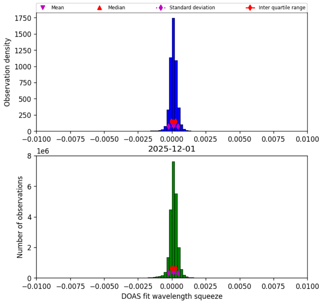
Figure 36: Histogram of “DOAS fit wavelength squeeze” for 2025-12-01 to 2025-12-01
