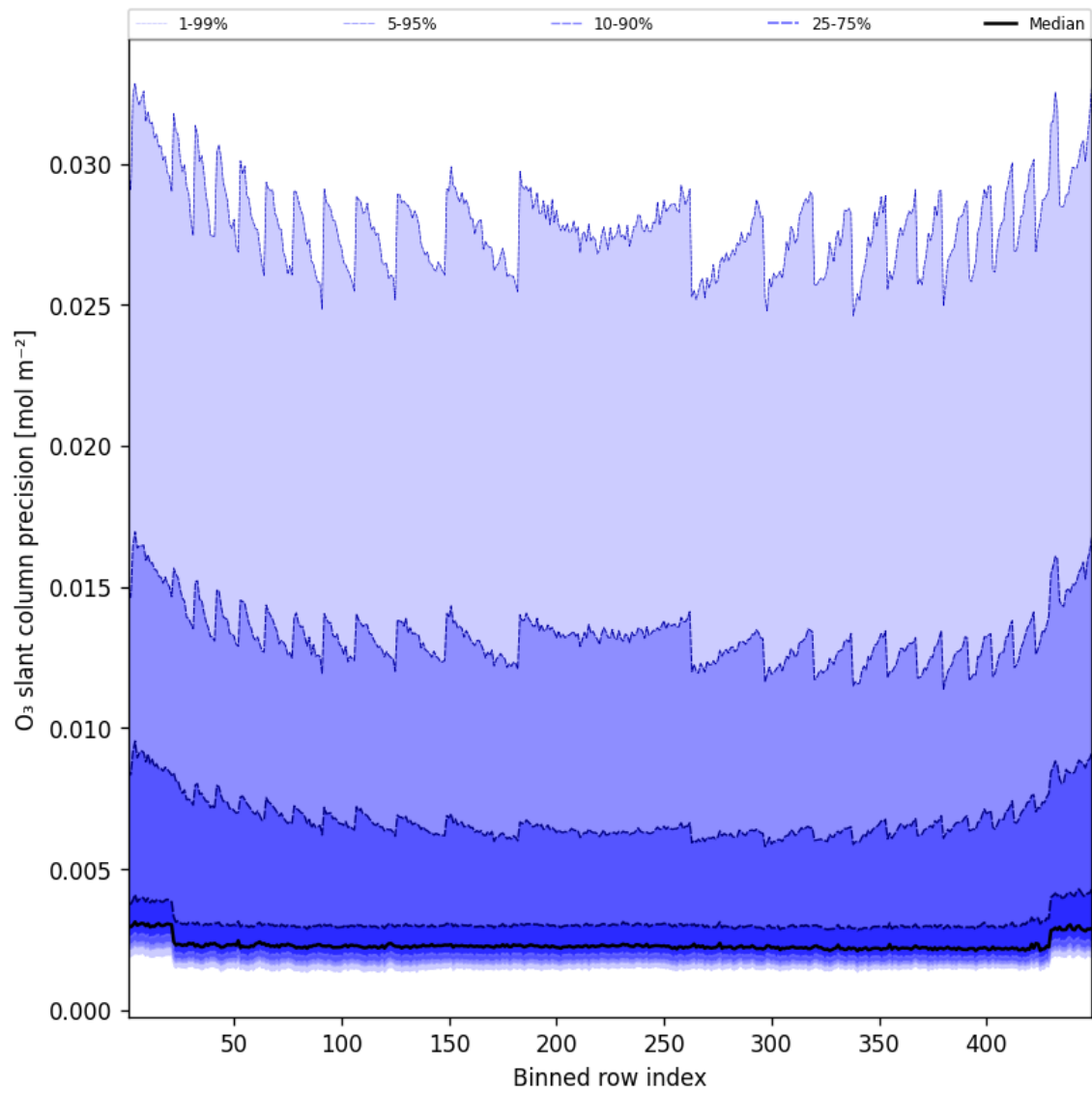
Figure 44: Along track statistics of “O 3 slant column precision” for 2025-12-01 to 2025-12-01
