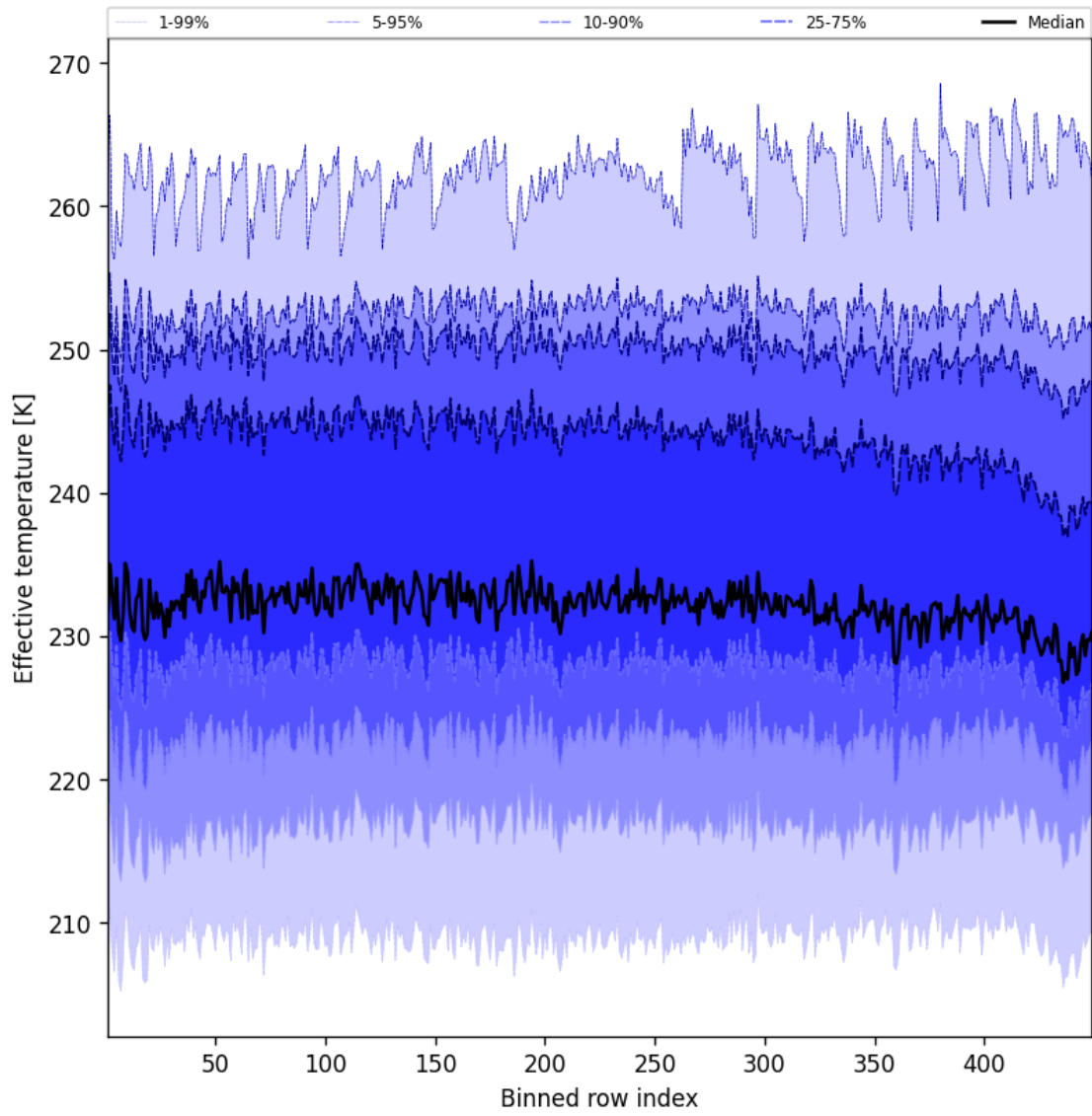
Figure 50: Along track statistics of “Effective temperature” for 2025-12-01 to 2025-12-01
