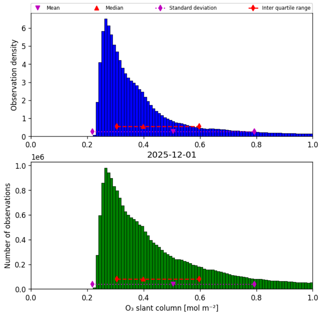
Figure 31: Histogram of “O 3 slant column” for 2025-12-01 to 2025-12-01
