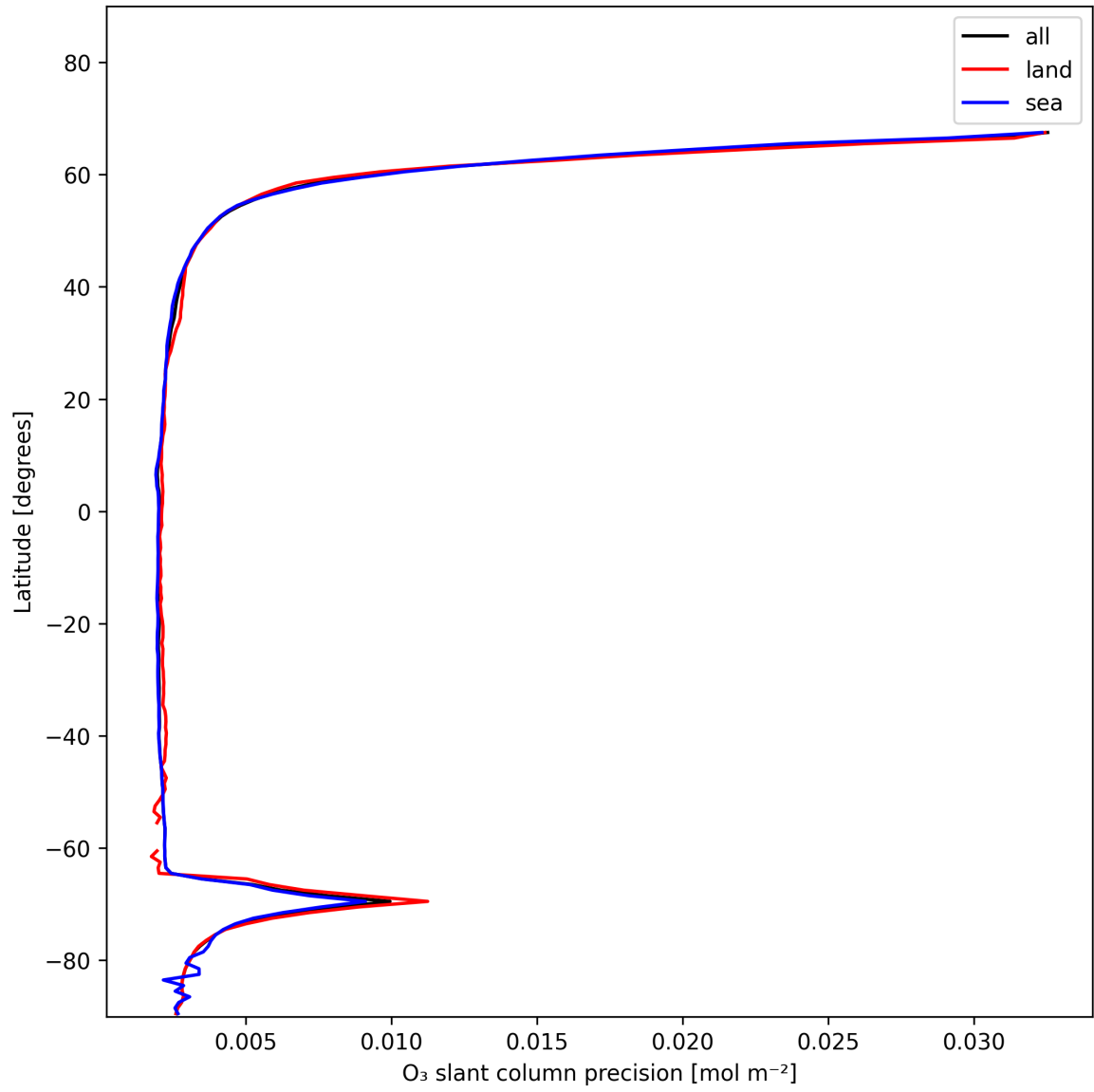
Figure 20: Zonal average of “O 3 slant column precision” for 2025-12-01 to 2025-12-01.
