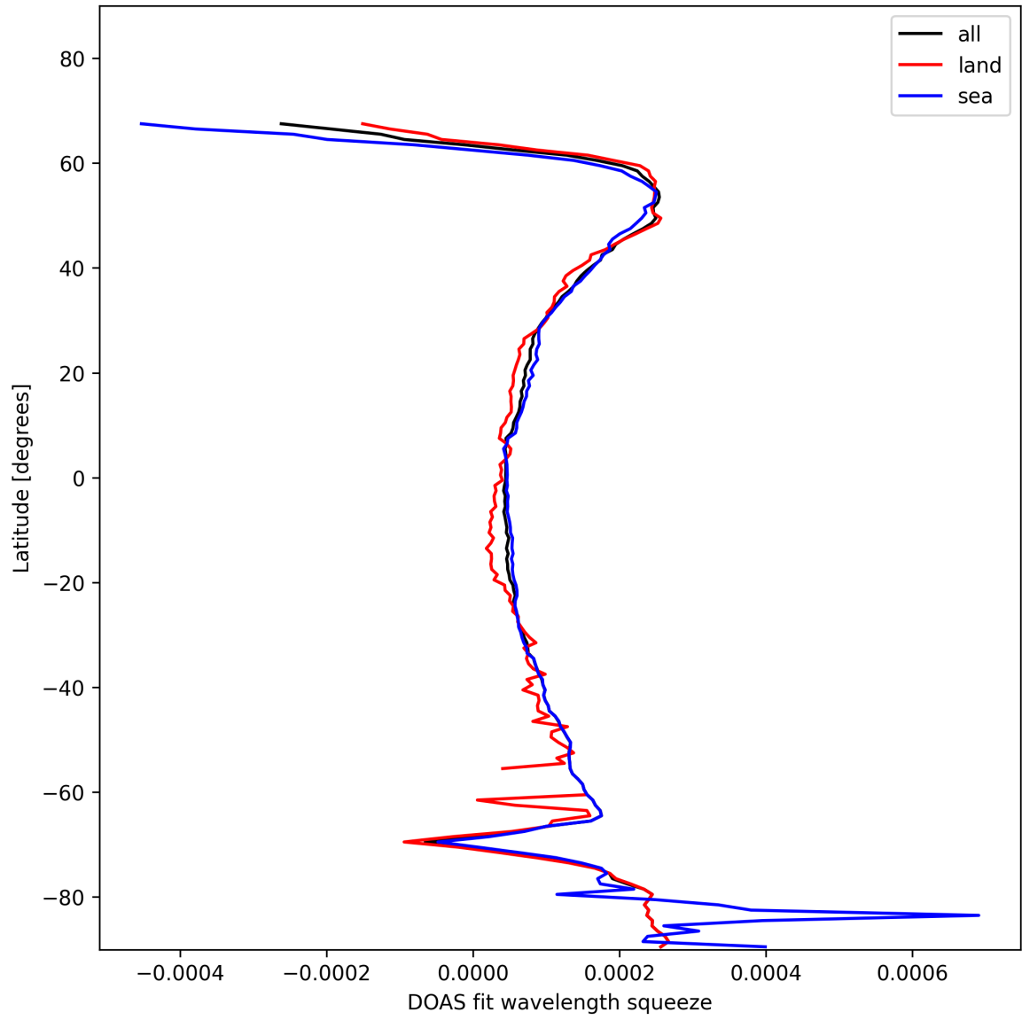
Figure 24: Zonal average of “DOAS fit wavelength squeeze” for 2025-12-01 to 2025-12-01.
