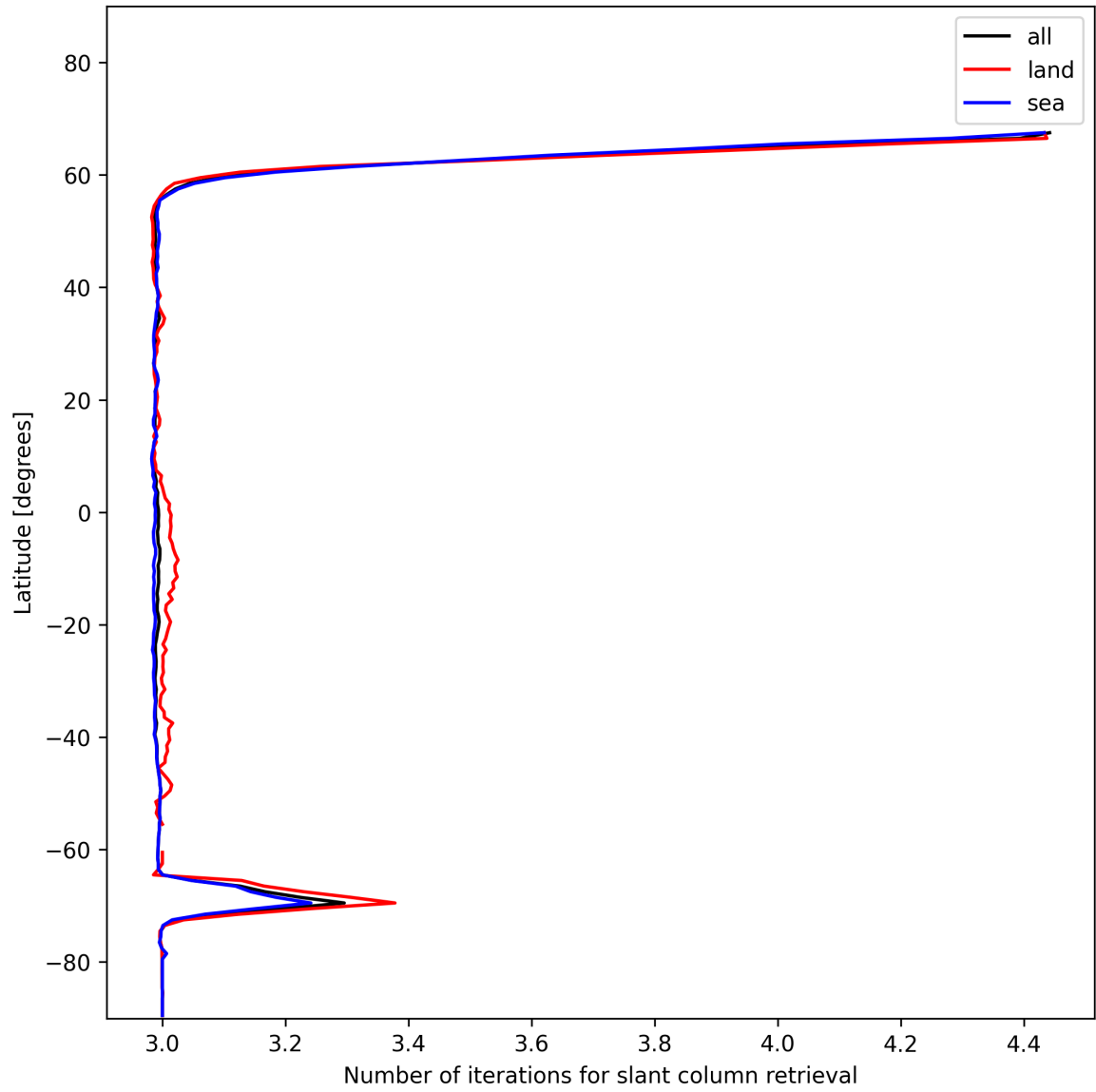
Figure 21: Zonal average of “Number of iterations for slant column retrieval” for 2025-12-01 to 2025-12-01.
