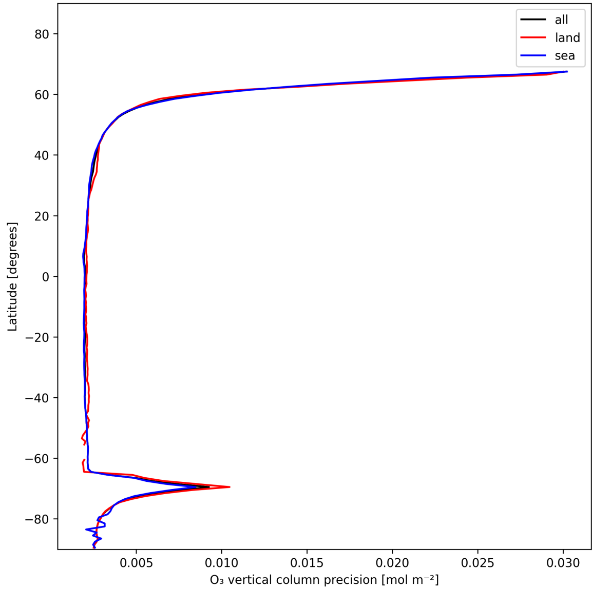
Figure 18: Zonal average of “O 3 vertical column precision” for 2025-12-01 to 2025-12-01.
