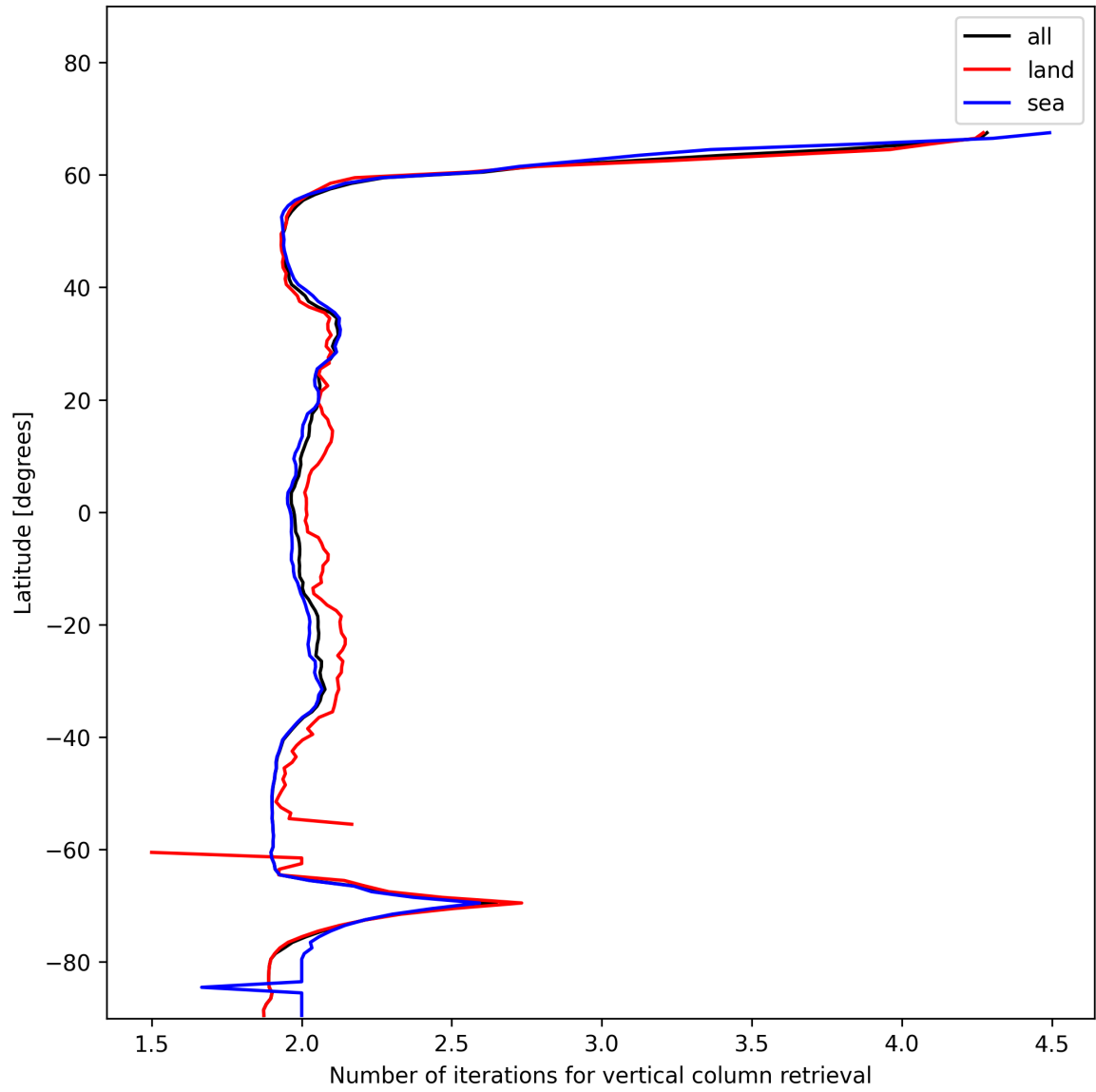
Figure 27: Zonal average of “Number of iterations for vertical column retrieval” for 2025-12-01 to 2025-12-01.
