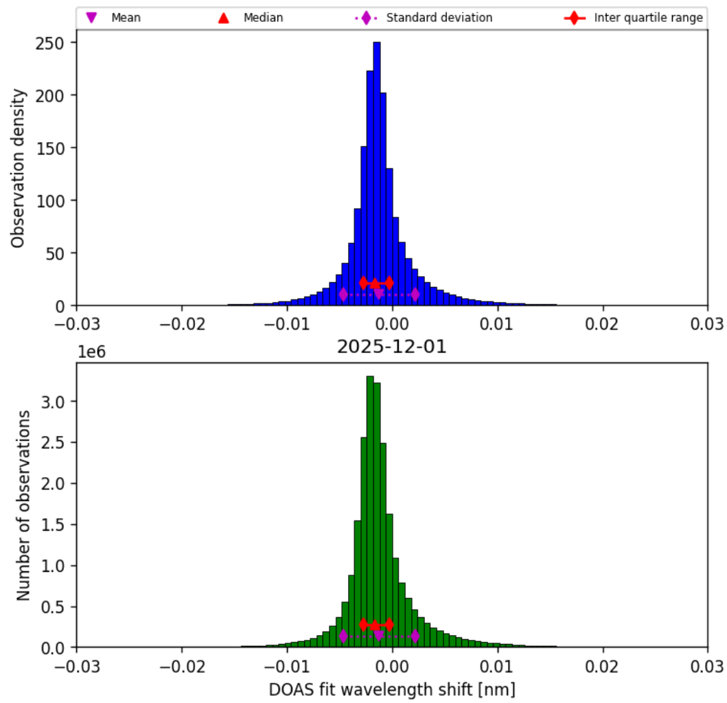
Figure 35: Histogram of “DOAS fit wavelength shift” for 2025-12-01 to 2025-12-01
