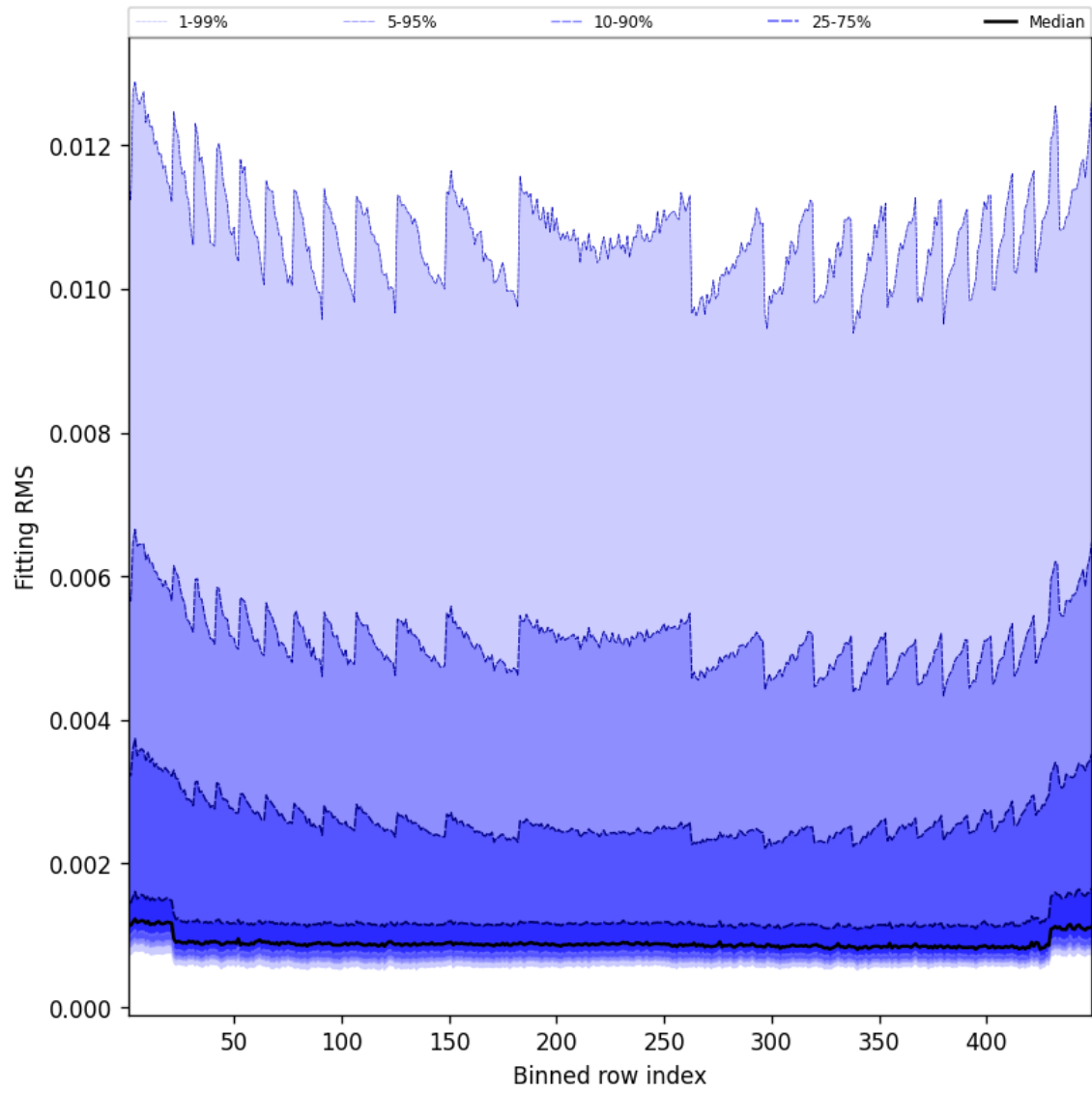
Figure 46: Along track statistics of “Fitting RMS” for 2025-12-01 to 2025-12-01
