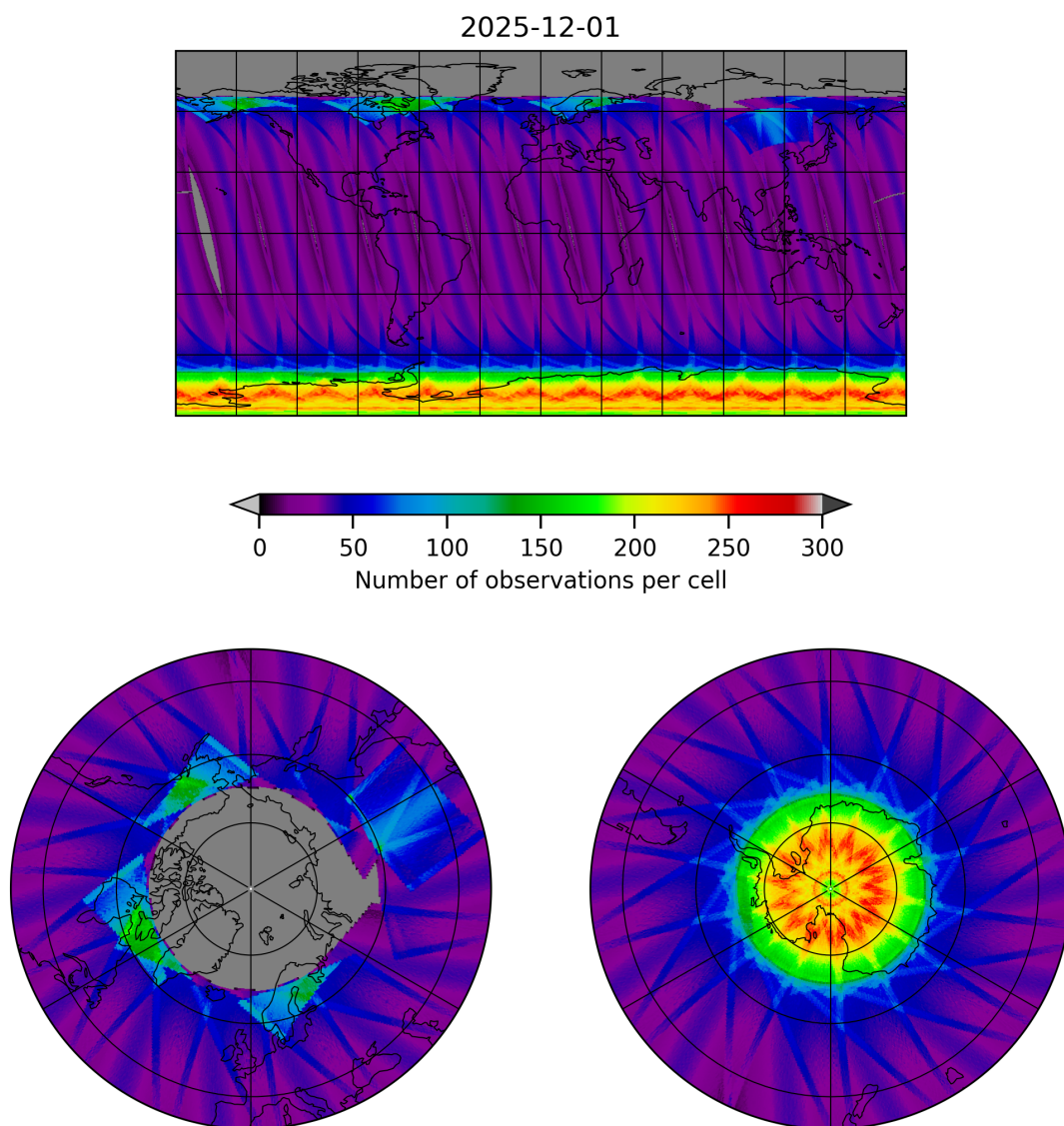
Figure 15: Map of the number of observations for 2025-12-01 to 2025-12-01
