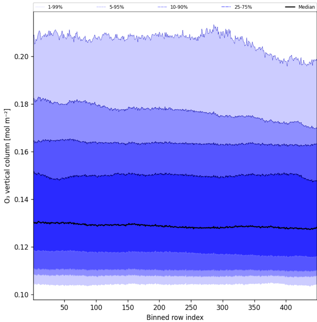
Figure 41: Along track statistics of “O 3 vertical column” for 2025-12-01 to 2025-12-01
