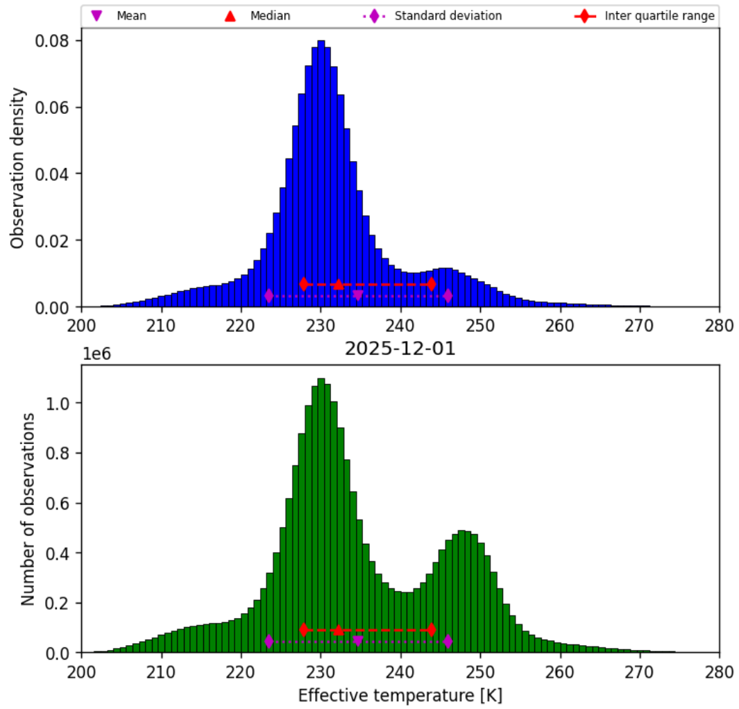
Figure 38: Histogram of “Effective temperature” for 2025-12-01 to 2025-12-01
