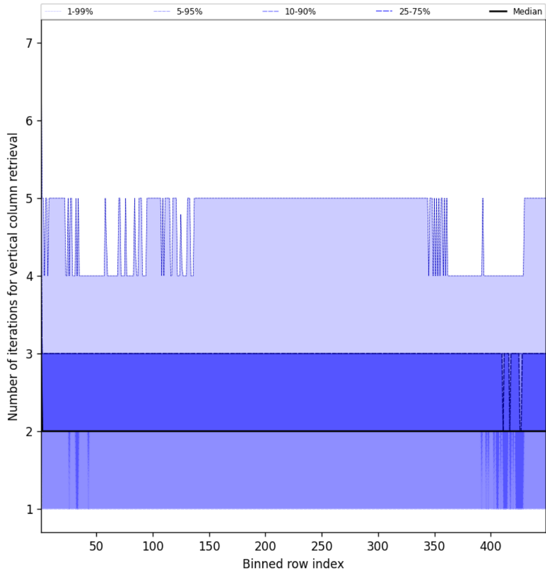
Figure 51: Along track statistics of “Number of iterations for vertical column retrieval” for 2025-12-01 to 2025-12-01
