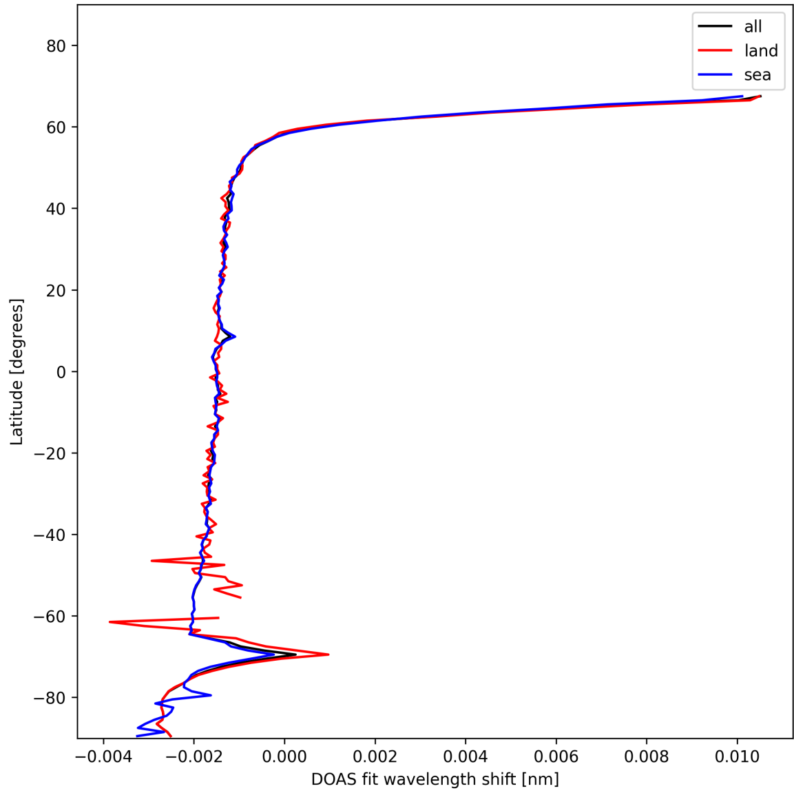
Figure 23: Zonal average of “DOAS fit wavelength shift” for 2025-12-01 to 2025-12-01.
