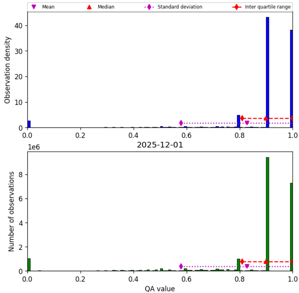
Figure 28: Histogram of “QA value” for 2025-12-01 to 2025-12-01
