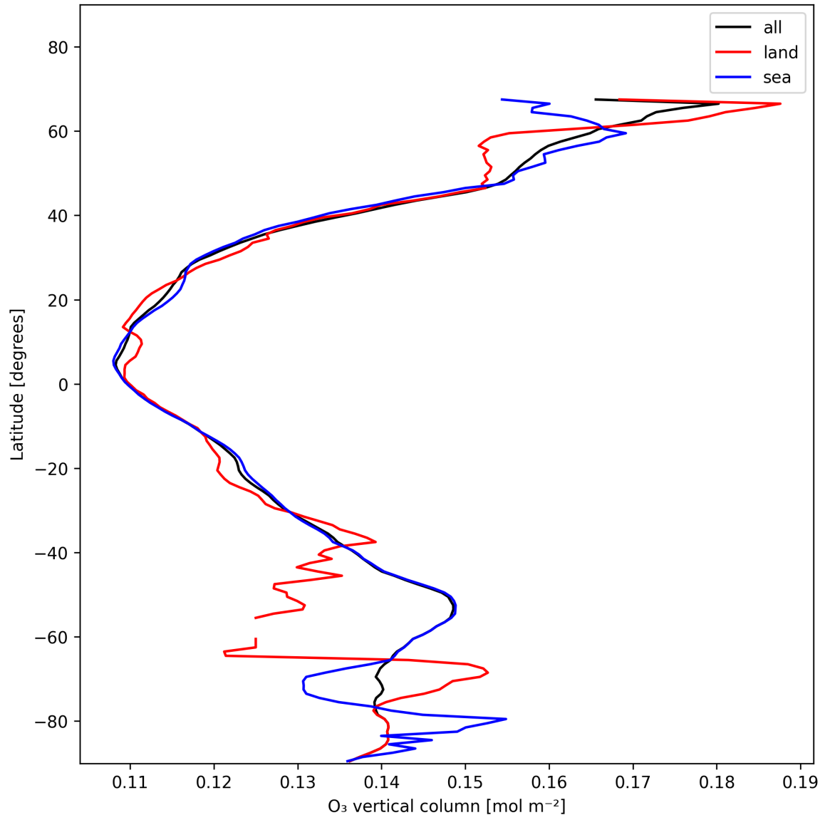
Figure 17: Zonal average of “O 3 vertical column” for 2025-12-01 to 2025-12-01.
