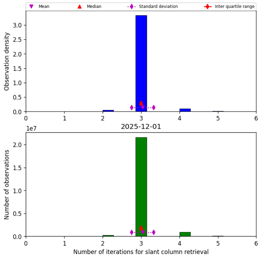
Figure 33: Histogram of “Number of iterations for slant column retrieval” for 2025-12-01 to 2025-12-01
