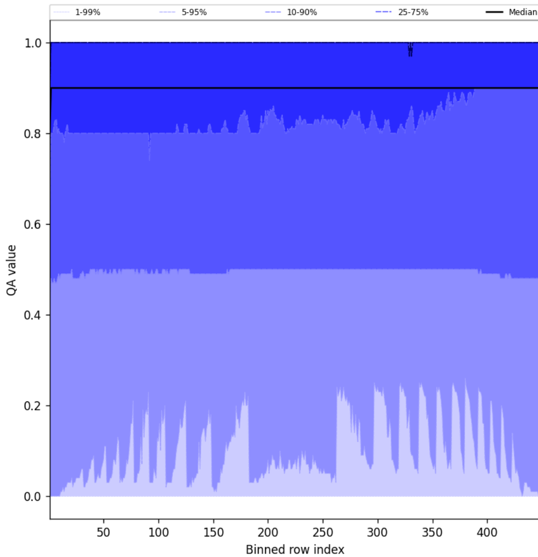
Figure 40: Along track statistics of “QA value” for 2025-12-01 to 2025-12-01
