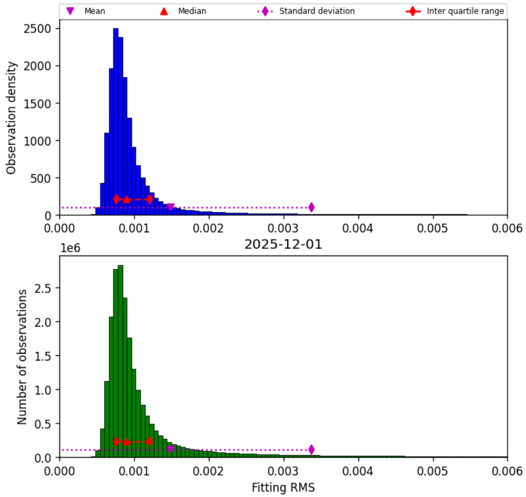
Figure 34: Histogram of “Fitting RMS” for 2025-12-01 to 2025-12-01
