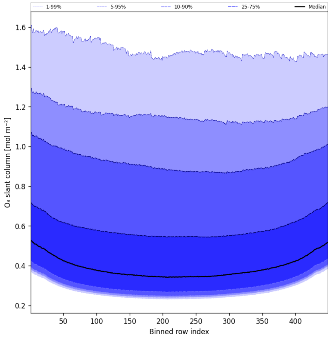
Figure 43: Along track statistics of “O 3 slant column” for 2025-12-01 to 2025-12-01
