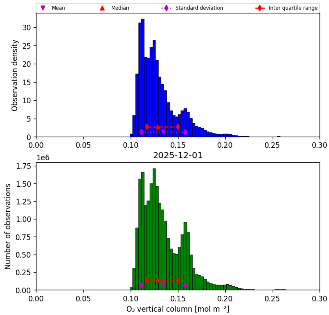
Figure 29: Histogram of “O 3 vertical column” for 2025-12-01 to 2025-12-01
