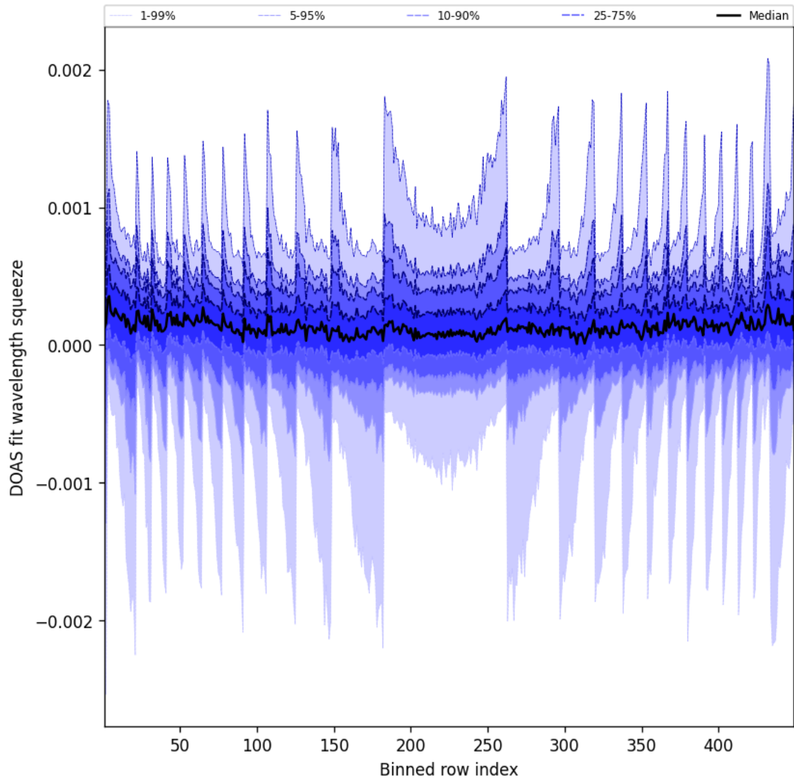
Figure 48: Along track statistics of “DOAS fit wavelength squeeze” for 2025-12-01 to 2025-12-01
