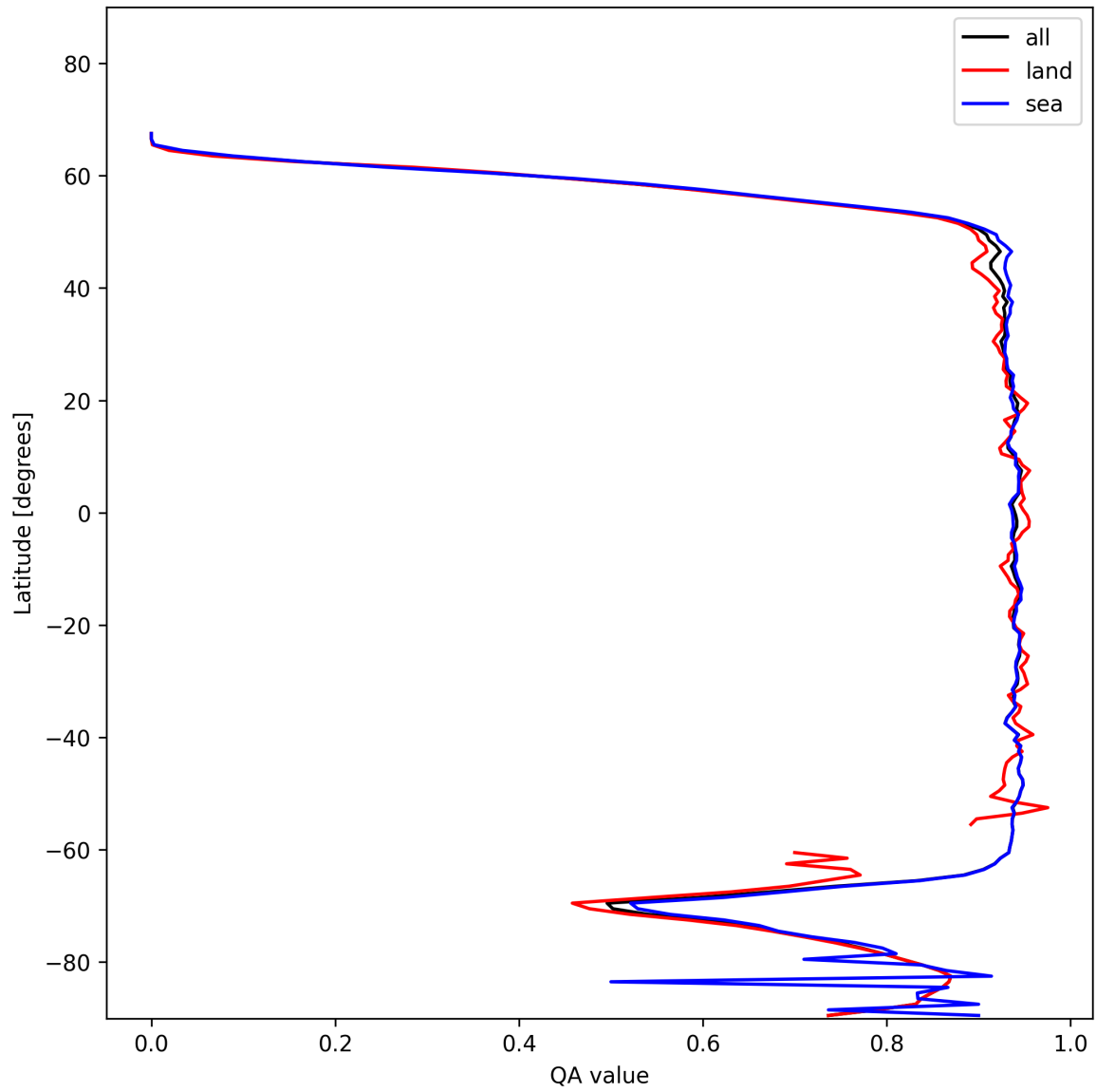
Figure 16: Zonal average of "QA value" for 2025-12-01 to 2025-12-01.
