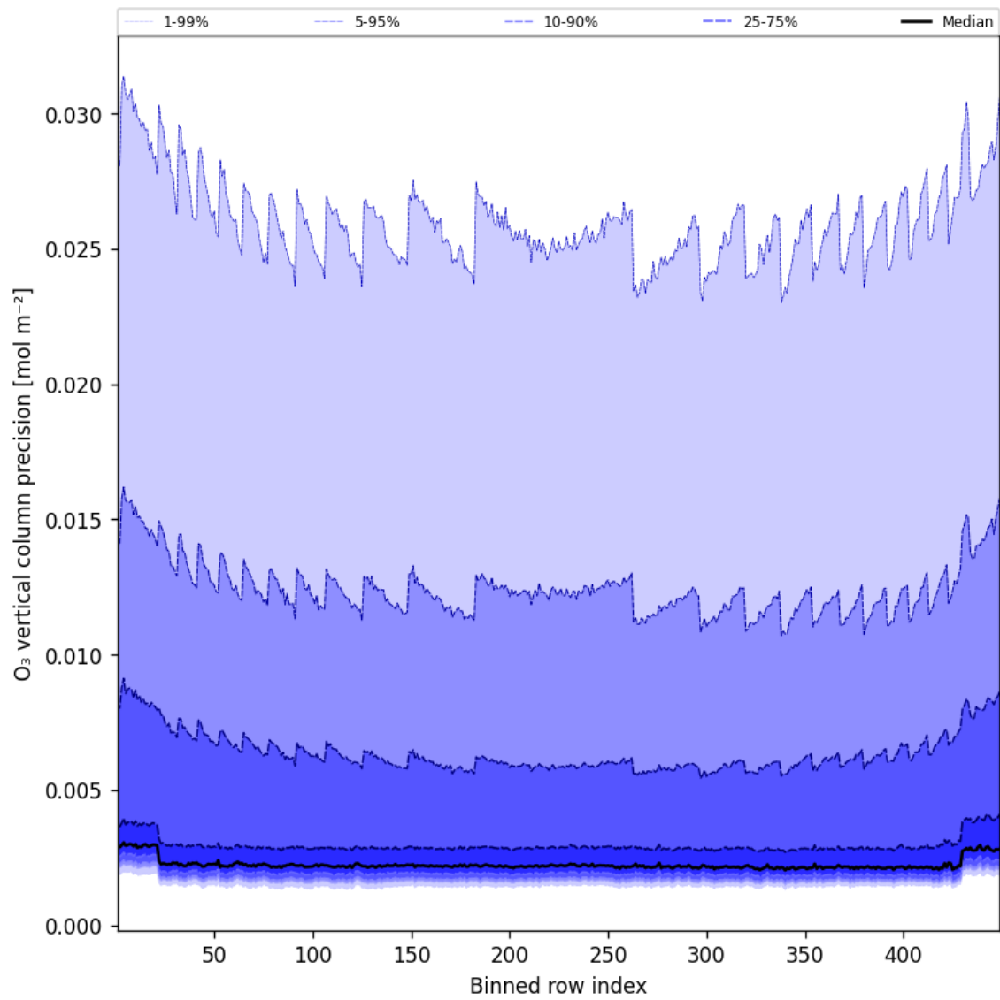
Figure 42: Along track statistics of “O 3 vertical column precision” for 2025-12-01 to 2025-12-01
