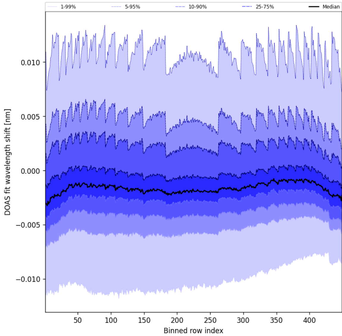
Figure 47: Along track statistics of “DOAS fit wavelength shift” for 2025-12-01 to 2025-12-01
