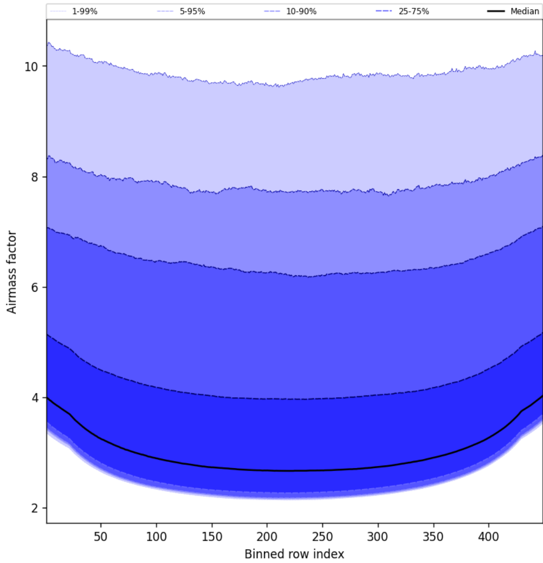
Figure 49: Along track statistics of “Airmass factor” for 2025-12-01 to 2025-12-01
