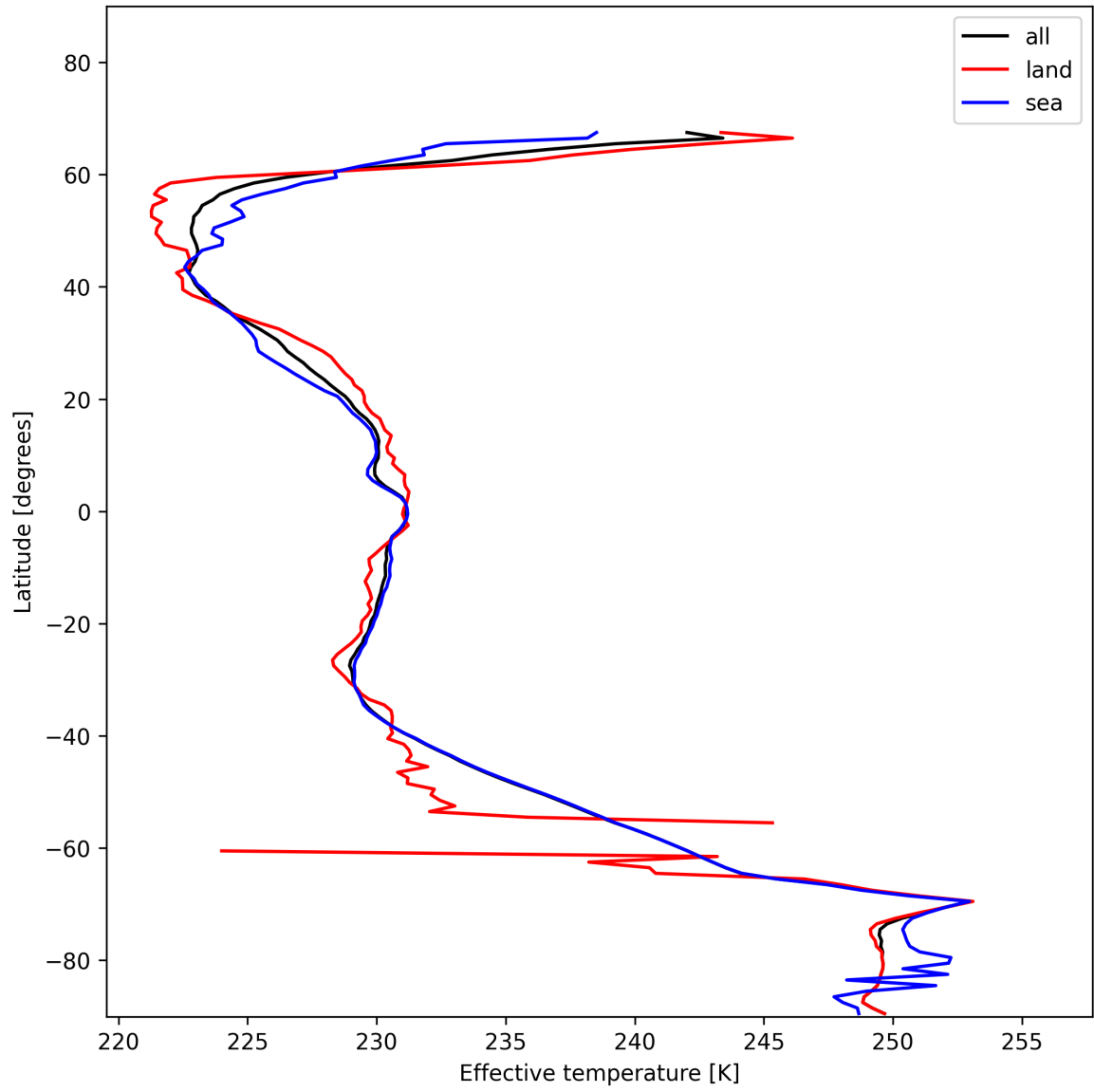
Figure 26: Zonal average of “Effective temperature” for 2025-12-01 to 2025-12-01.
