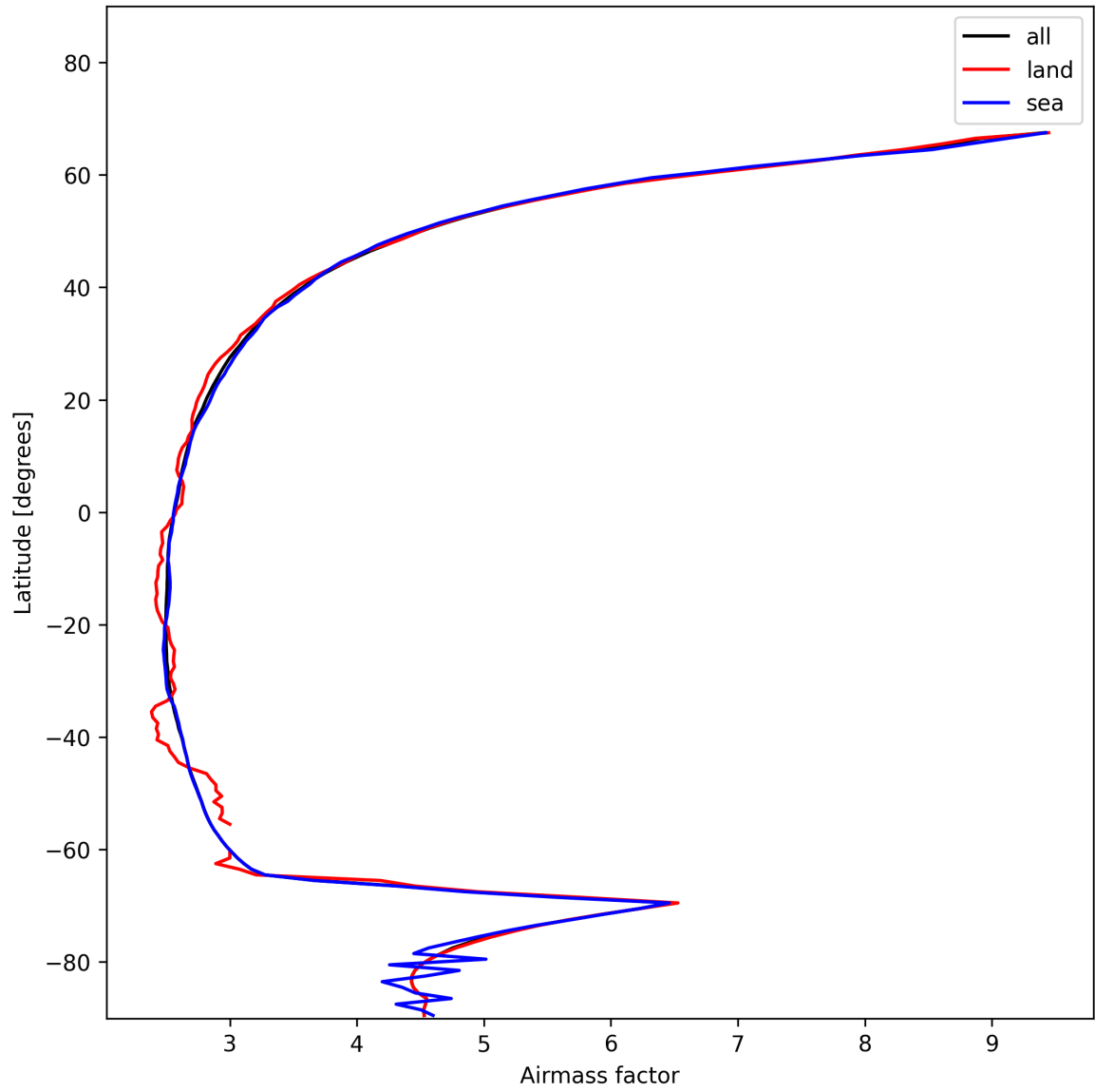
Figure 25: Zonal average of “Airmass factor” for 2025-12-01 to 2025-12-01.
