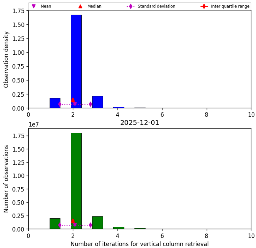
Figure 39: Histogram of “Number of iterations for vertical column retrieval” for 2025-12-01 to 2025-12-01
