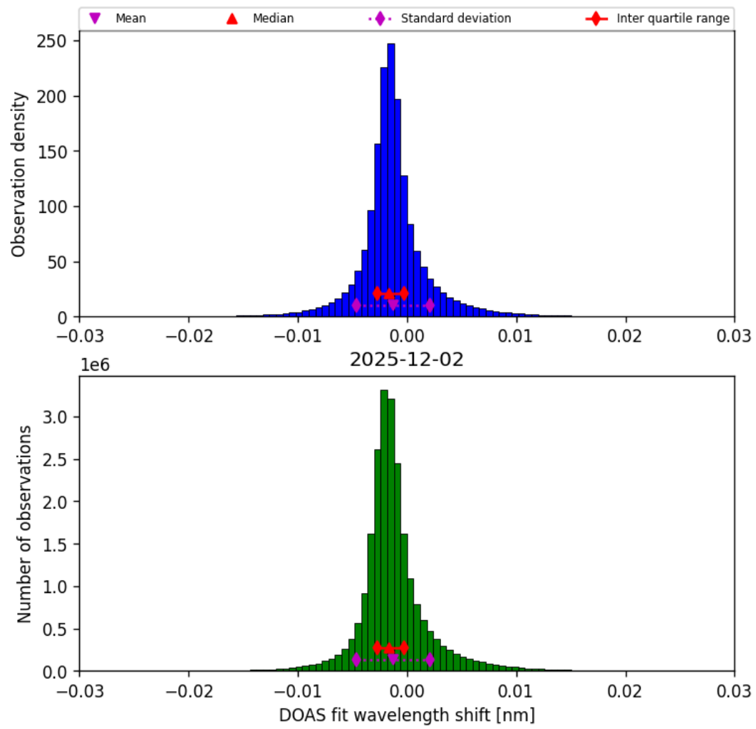
Figure 35: Histogram of “DOAS fit wavelength shift” for 2025-12-02 to 2025-12-02
