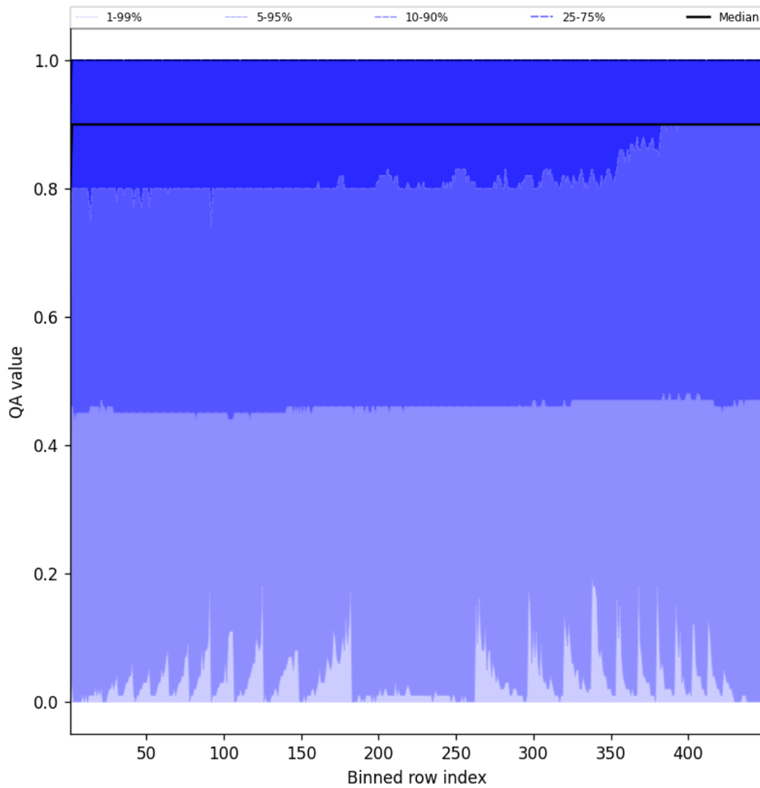
Figure 40: Along track statistics of “QA value” for 2025-12-02 to 2025-12-02
