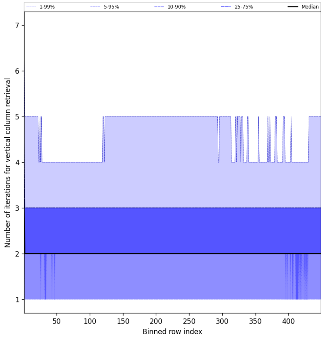
Figure 51: Along track statistics of “Number of iterations for vertical column retrieval” for 2025-12-02 to 2025-12-02
