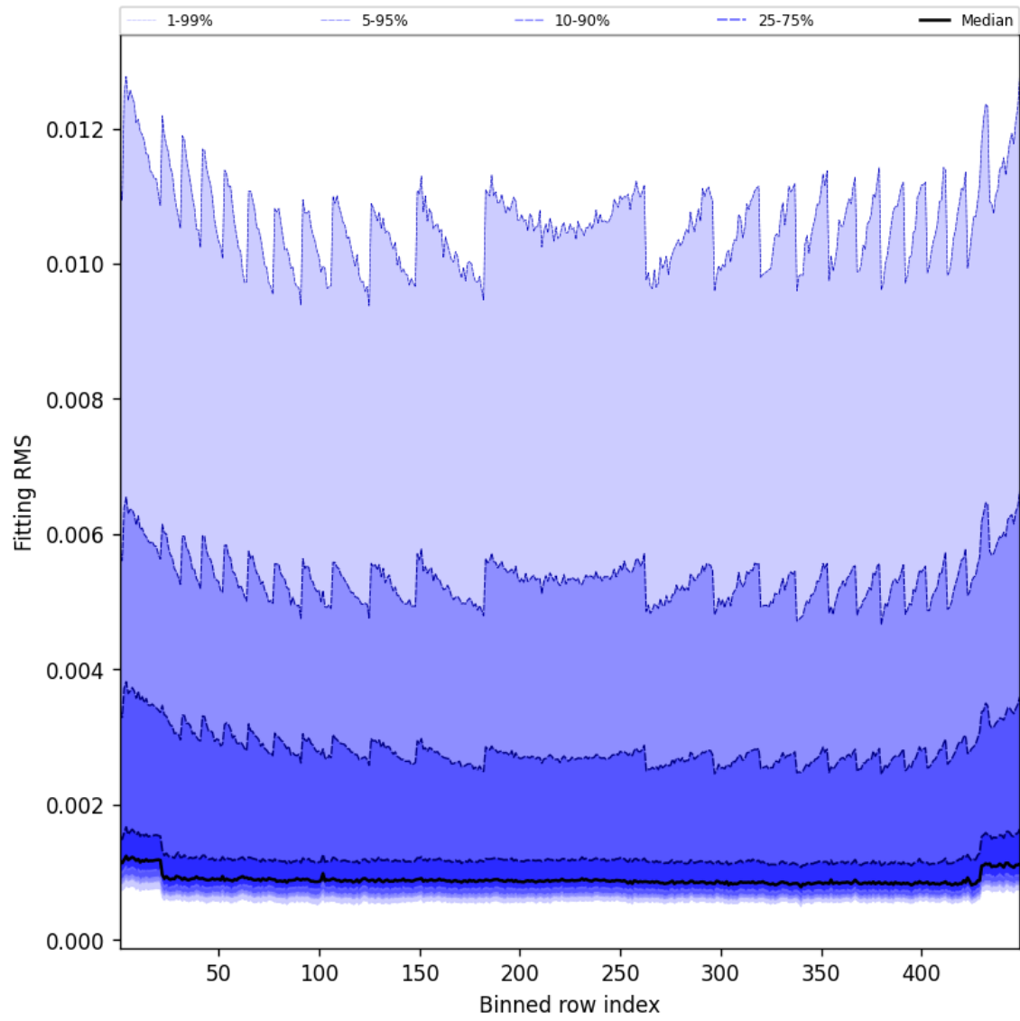
Figure 46: Along track statistics of “Fitting RMS” for 2025-12-02 to 2025-12-02
