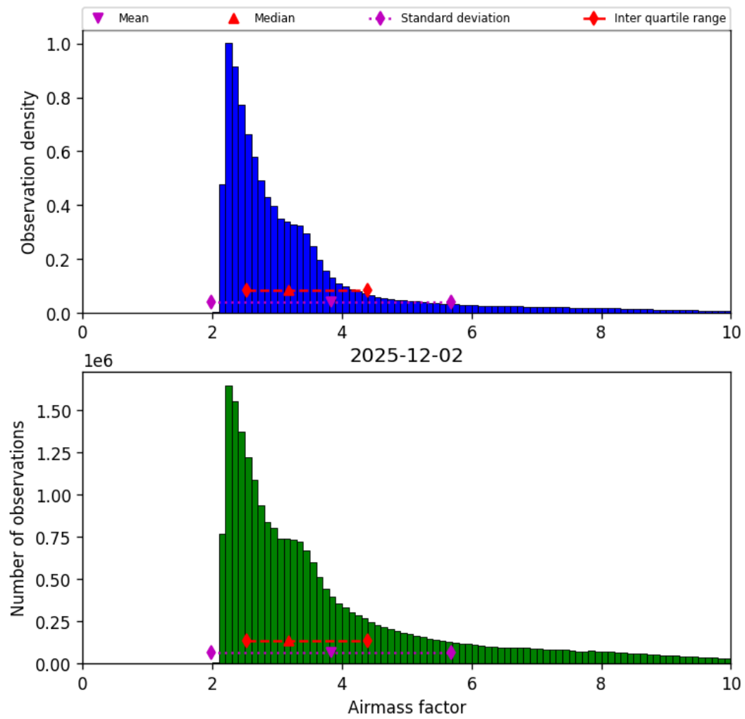
Figure 37: Histogram of “Airmass factor” for 2025-12-02 to 2025-12-02
