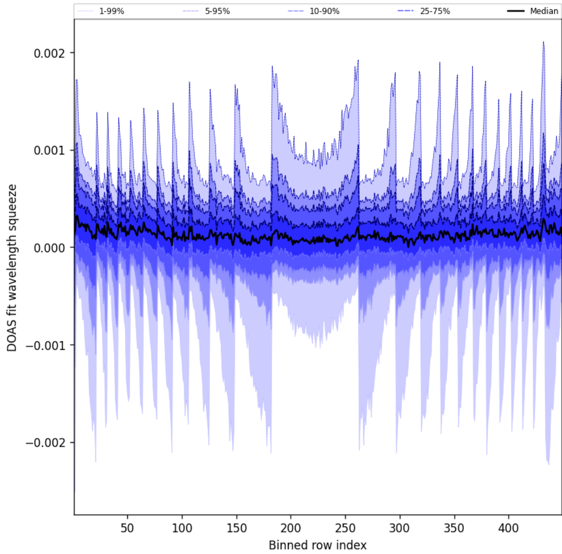
Figure 48: Along track statistics of “DOAS fit wavelength squeeze” for 2025-12-02 to 2025-12-02
