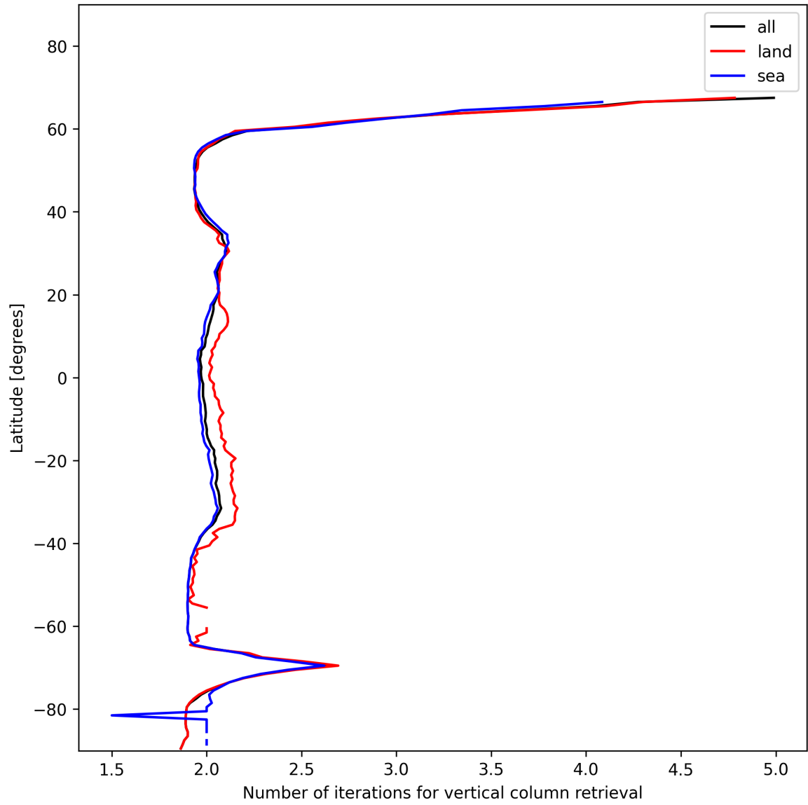
Figure 27: Zonal average of “Number of iterations for vertical column retrieval” for 2025-12-02 to 2025-12-02.
