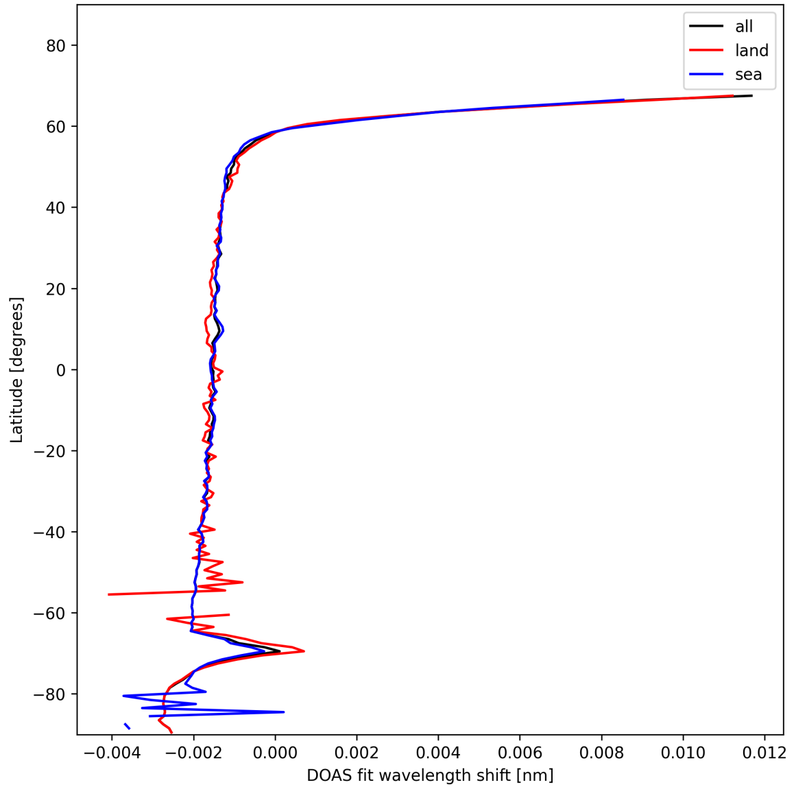
Figure 23: Zonal average of “DOAS fit wavelength shift” for 2025-12-02 to 2025-12-02.
