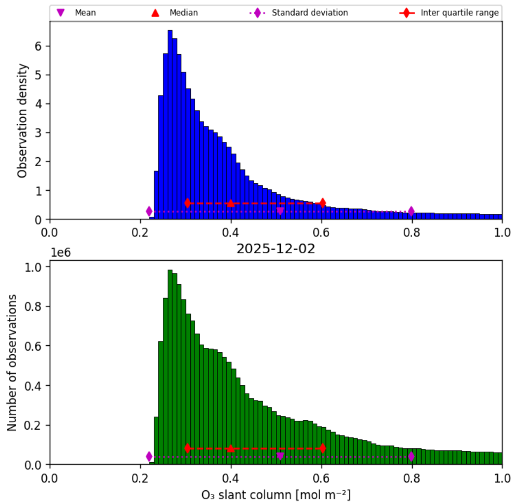
Figure 31: Histogram of “O 3 slant column” for 2025-12-02 to 2025-12-02
