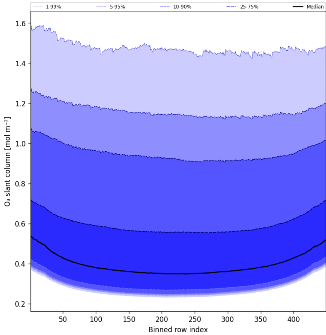
Figure 43: Along track statistics of “O 3 slant column” for 2025-12-02 to 2025-12-02
