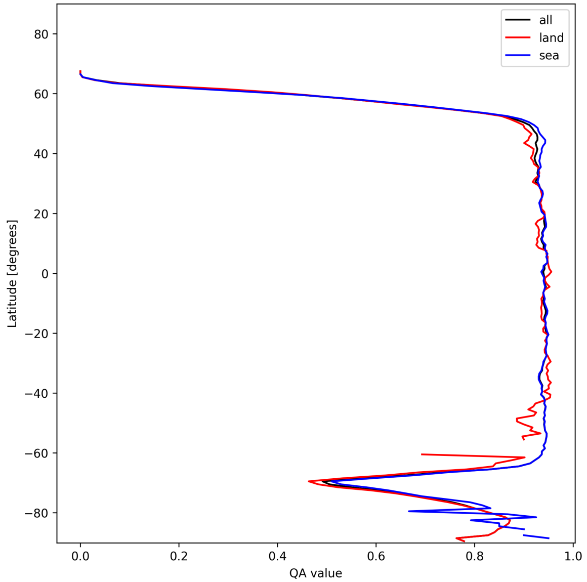
Figure 16: Zonal average of “QA value” for 2025-12-02 to 2025-12-02.
