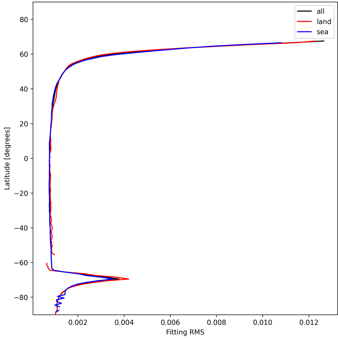
Figure 22: Zonal average of “Fitting RMS” for 2025-12-02 to 2025-12-02.
