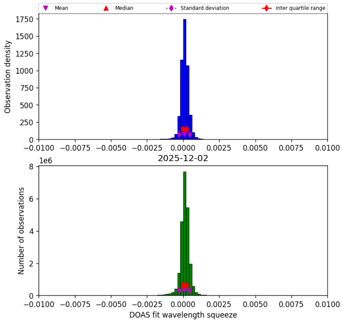
Figure 36: Histogram of “DOAS fit wavelength squeeze” for 2025-12-02 to 2025-12-02
