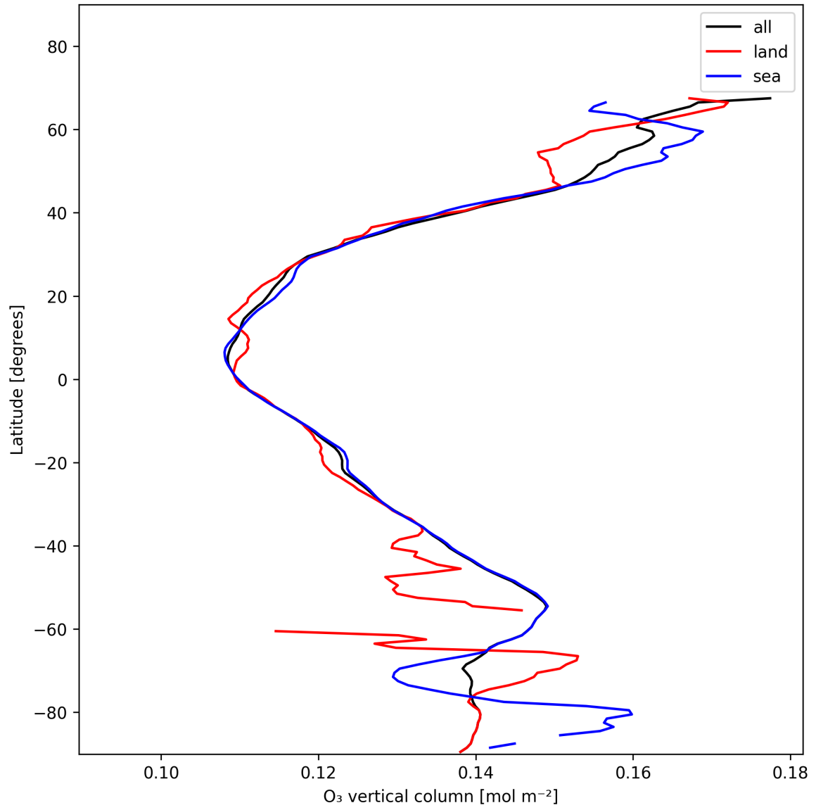
Figure 17: Zonal average of “O 3 vertical column” for 2025-12-02 to 2025-12-02.
