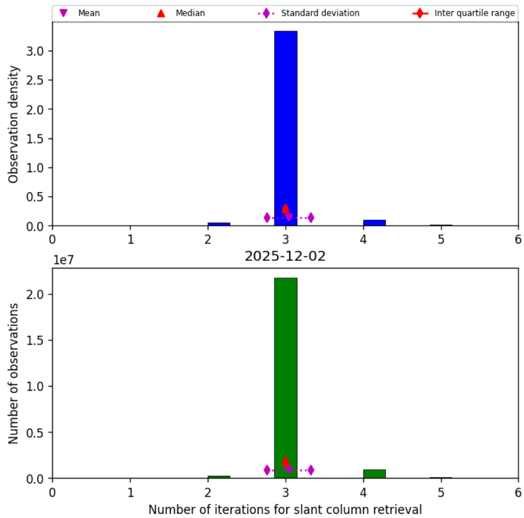
Figure 33: Histogram of “Number of iterations for slant column retrieval” for 2025-12-02 to 2025-12-02
