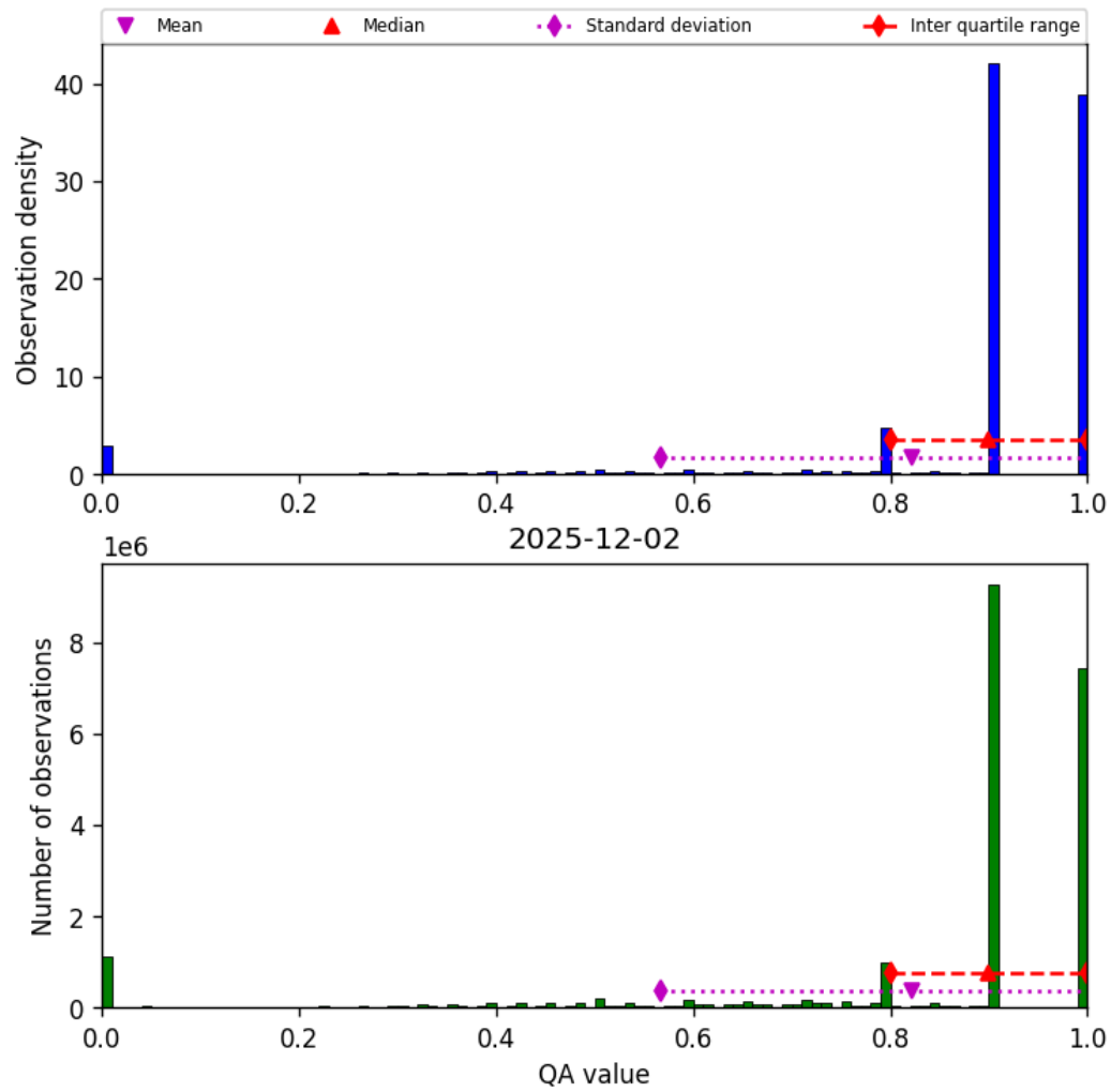
Figure 28: Histogram of “QA value” for 2025-12-02 to 2025-12-02
