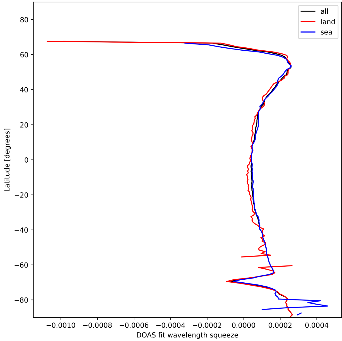
Figure 24: Zonal average of “DOAS fit wavelength squeeze” for 2025-12-02 to 2025-12-02.
