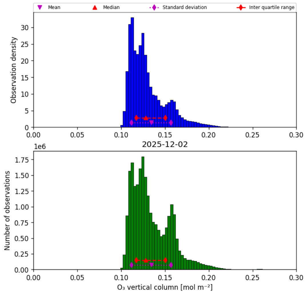
Figure 29: Histogram of “O 3 vertical column” for 2025-12-02 to 2025-12-02
