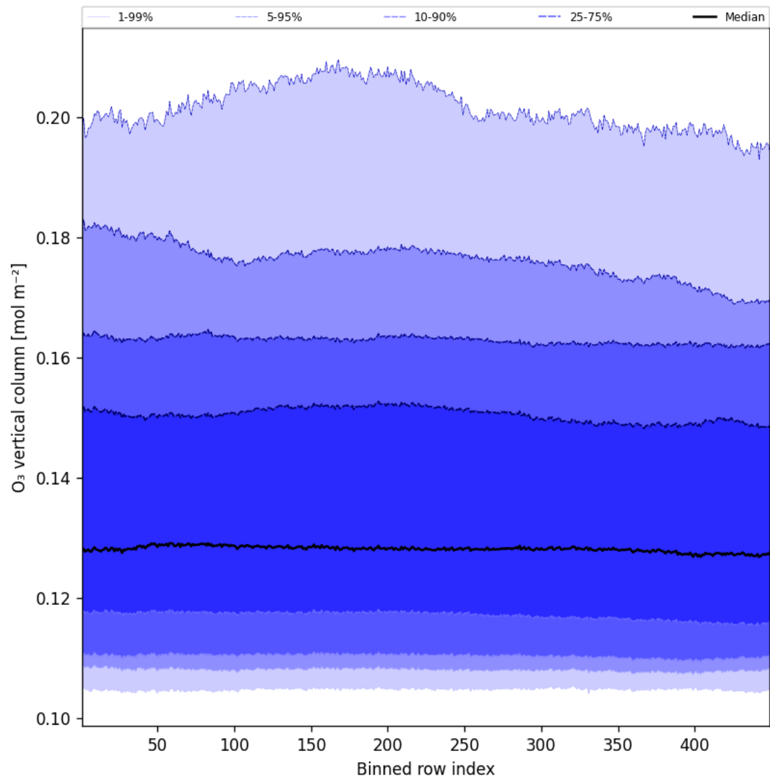
Figure 41: Along track statistics of “O 3 vertical column” for 2025-12-02 to 2025-12-02
