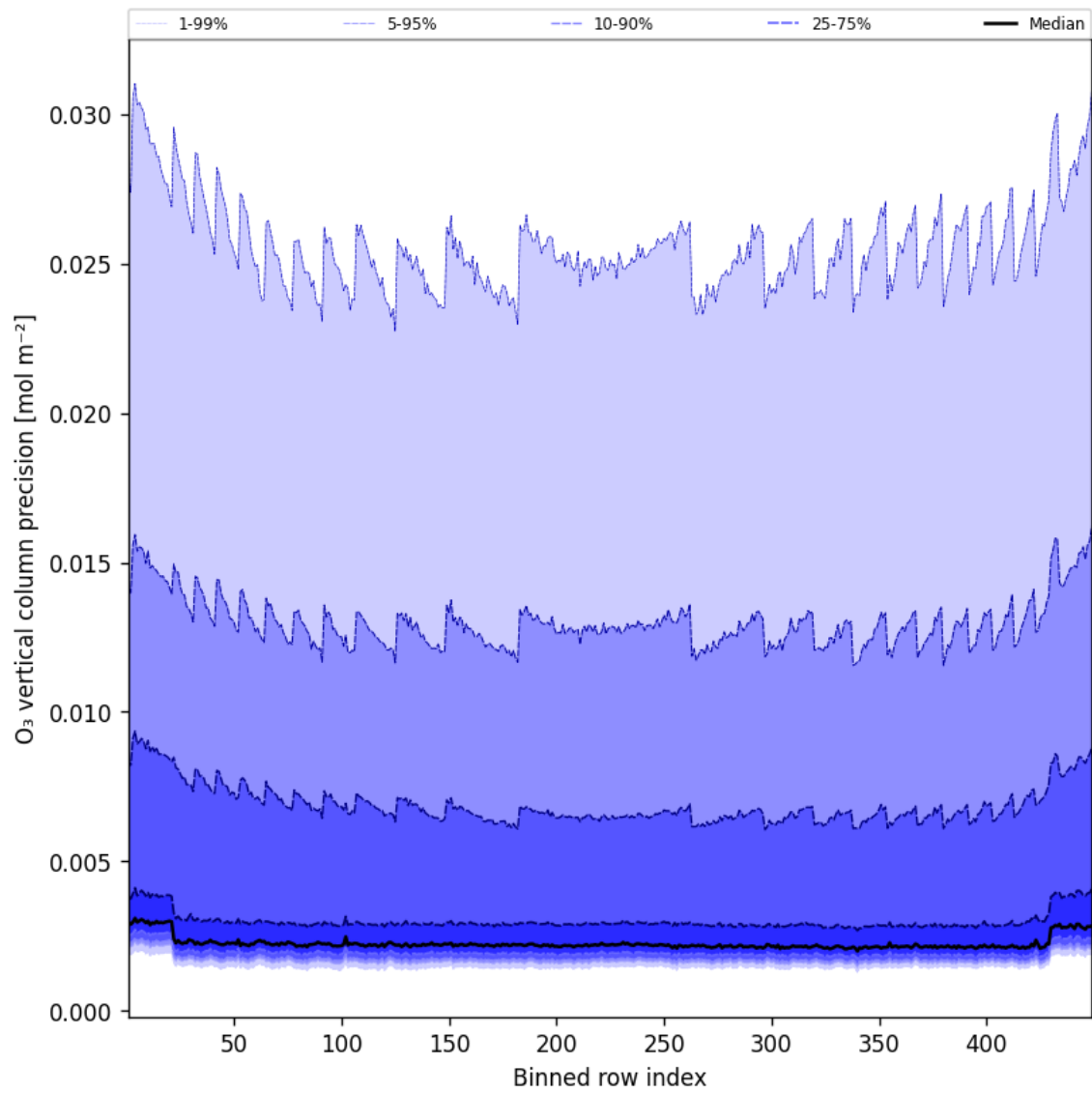
Figure 42: Along track statistics of “O 3 vertical column precision” for 2025-12-02 to 2025-12-02
