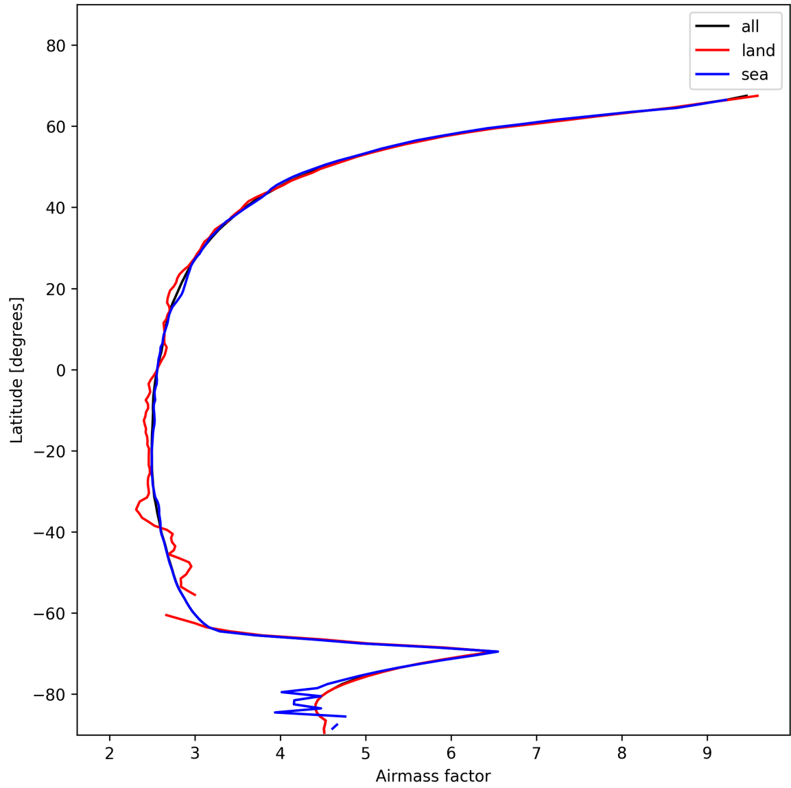
Figure 25: Zonal average of “Airmass factor” for 2025-12-02 to 2025-12-02.
