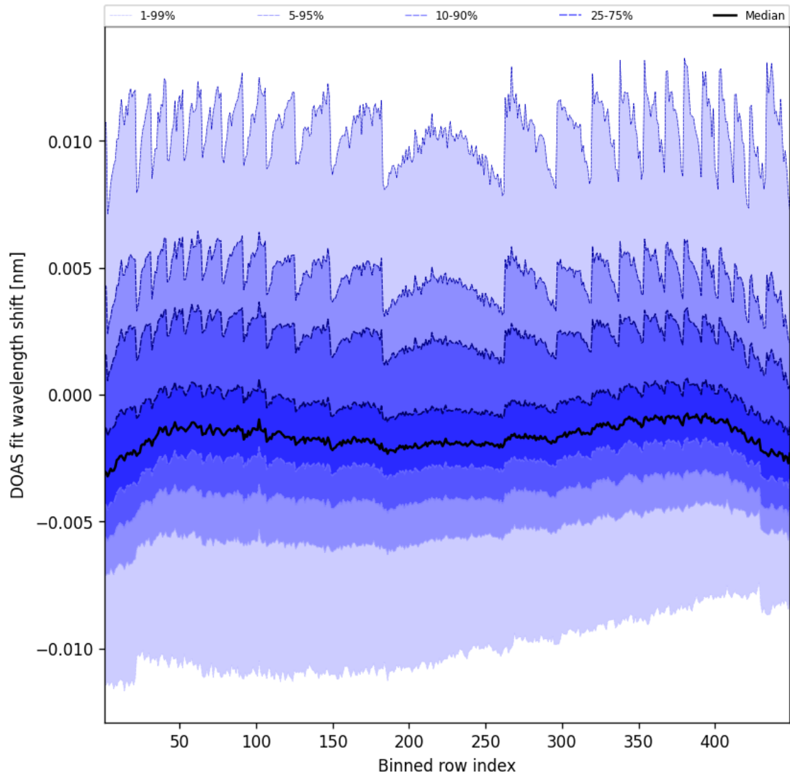
Figure 47: Along track statistics of “DOAS fit wavelength shift” for 2025-12-02 to 2025-12-02
