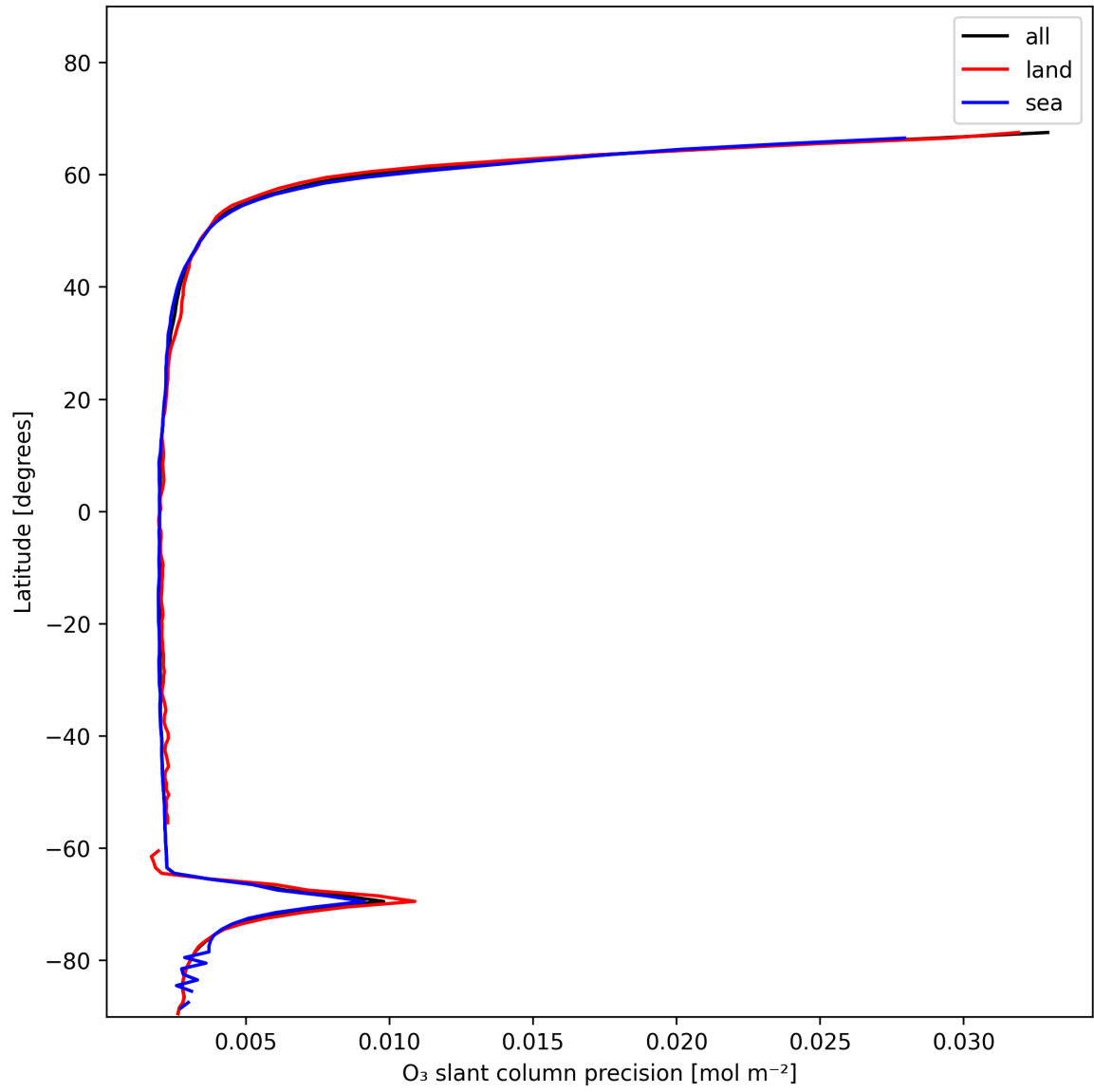
Figure 20: Zonal average of “O 3 slant column precision” for 2025-12-02 to 2025-12-02.
