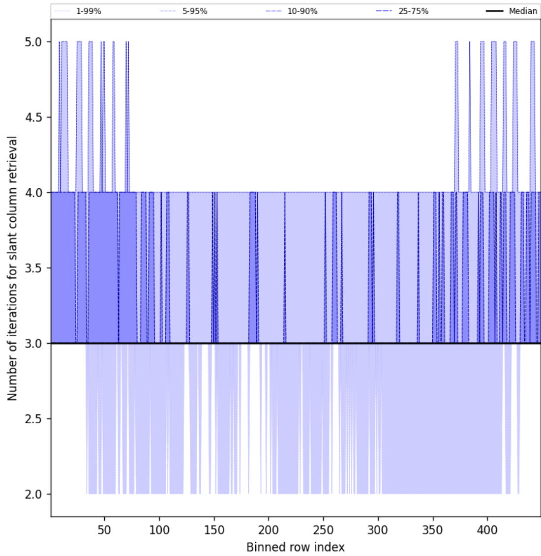
Figure 45: Along track statistics of “Number of iterations for slant column retrieval” for 2025-12-02 to 2025-12-02
