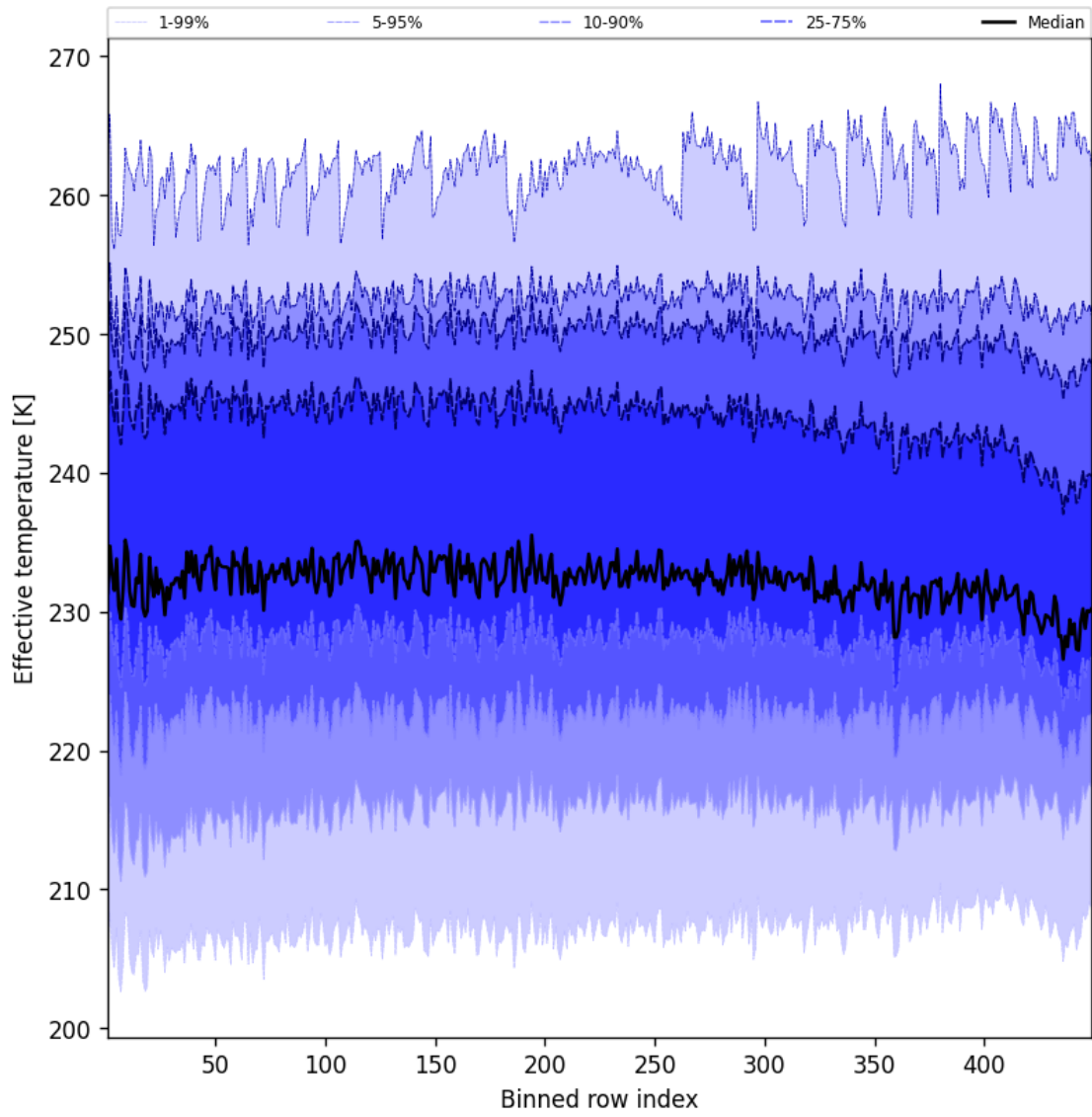
Figure 50: Along track statistics of “Effective temperature” for 2025-12-02 to 2025-12-02
