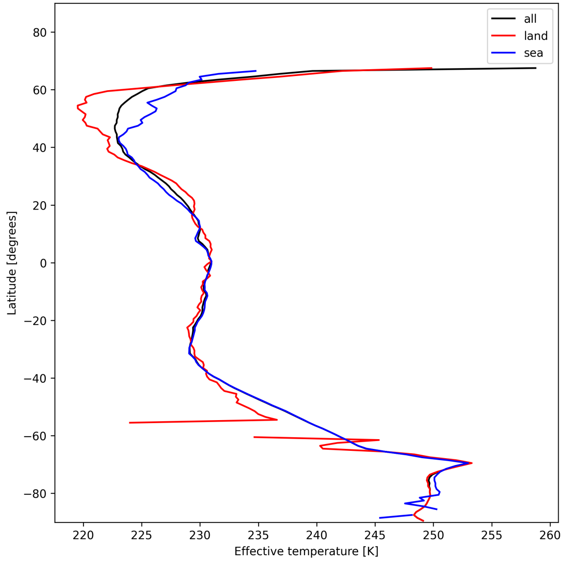
Figure 26: Zonal average of “Effective temperature” for 2025-12-02 to 2025-12-02.
