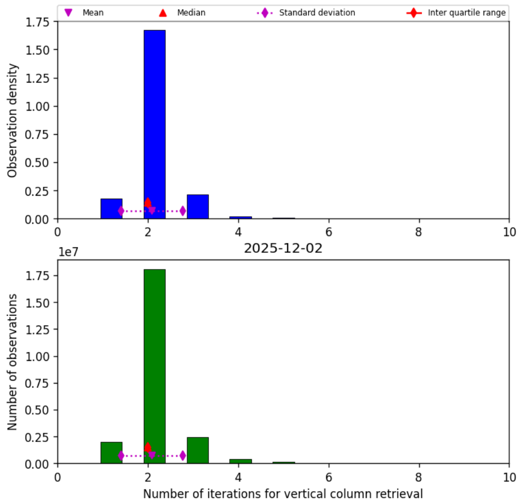
Figure 39: Histogram of “Number of iterations for vertical column retrieval” for 2025-12-02 to 2025-12-02
