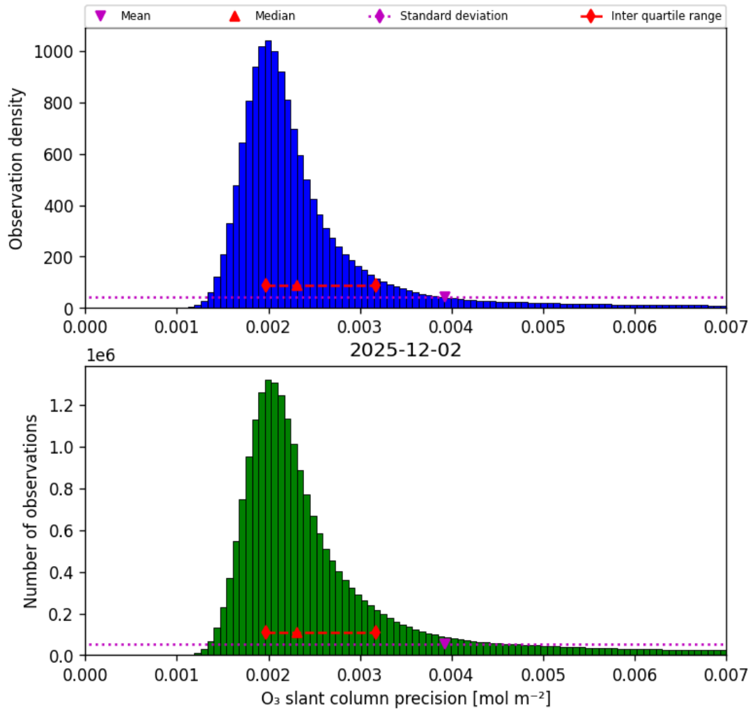
Figure 32: Histogram of “O 3 slant column precision” for 2025-12-02 to 2025-12-02
