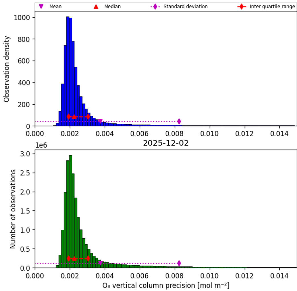
Figure 30: Histogram of “O 3 vertical column precision” for 2025-12-02 to 2025-12-02
