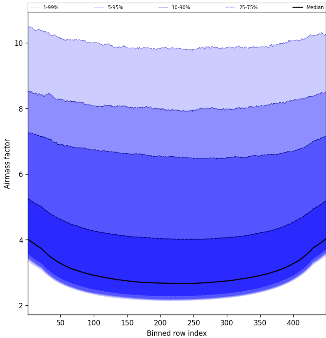
Figure 49: Along track statistics of “Airmass factor” for 2025-12-02 to 2025-12-02
