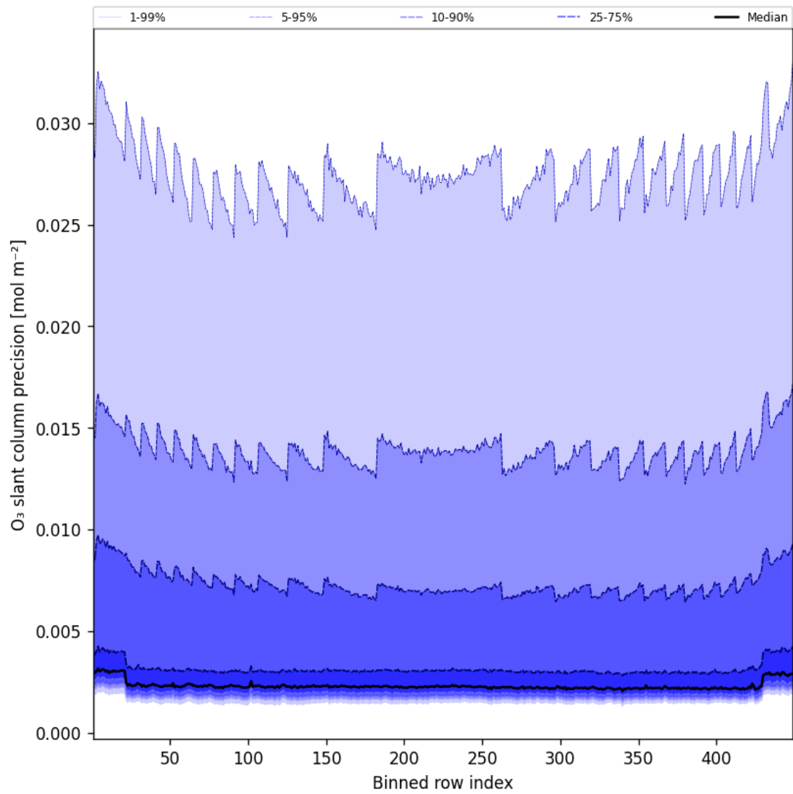
Figure 44: Along track statistics of “O 3 slant column precision” for 2025-12-02 to 2025-12-02
