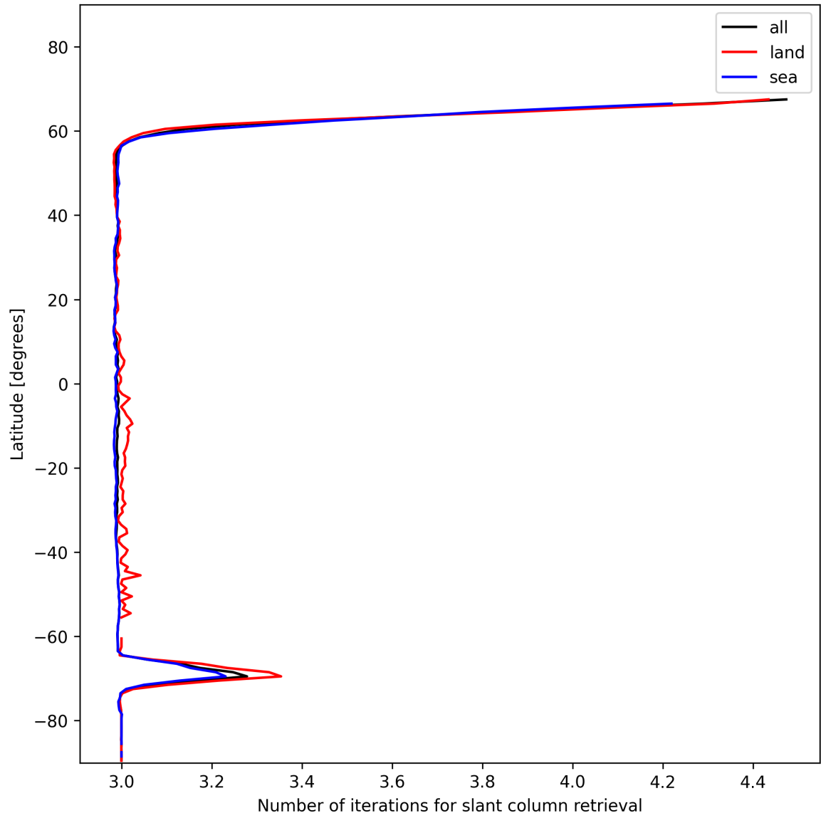
Figure 21: Zonal average of “Number of iterations for slant column retrieval” for 2025-12-02 to 2025-12-02.
