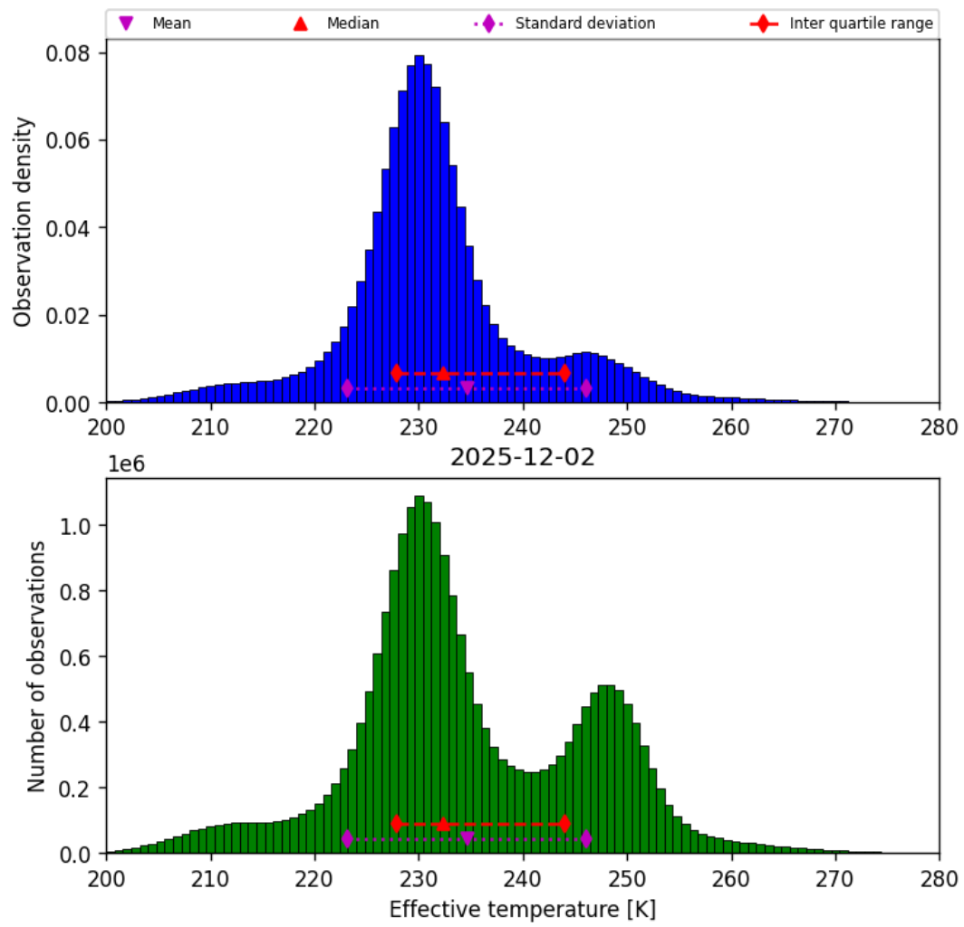
Figure 38: Histogram of “Effective temperature” for 2025-12-02 to 2025-12-02
