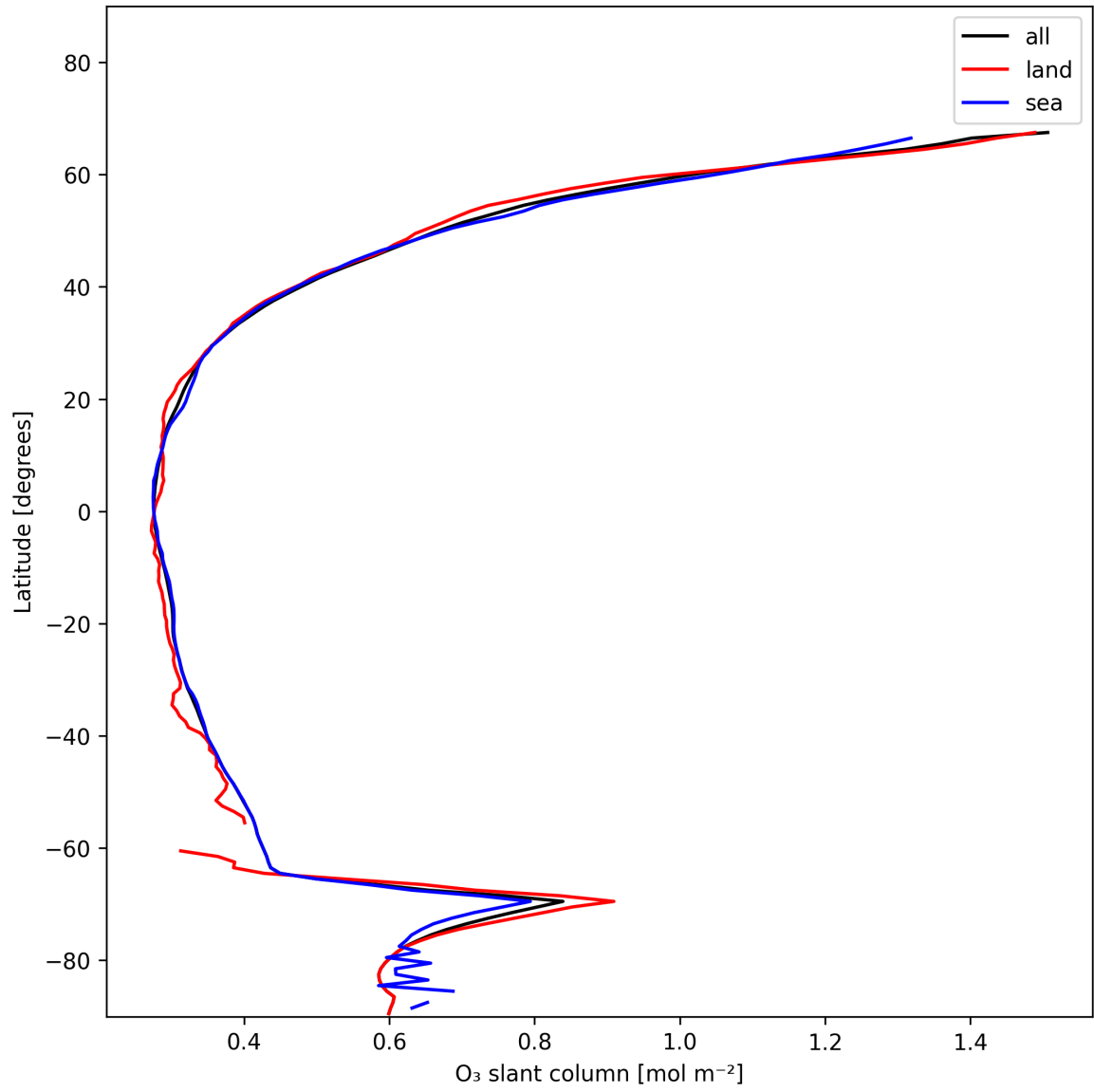
Figure 19: Zonal average of “O 3 slant column” for 2025-12-02 to 2025-12-02.
