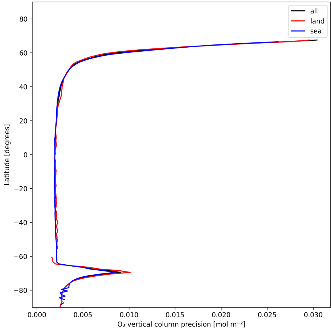
Figure 18: Zonal average of “O 3 vertical column precision” for 2025-12-02 to 2025-12-02.
