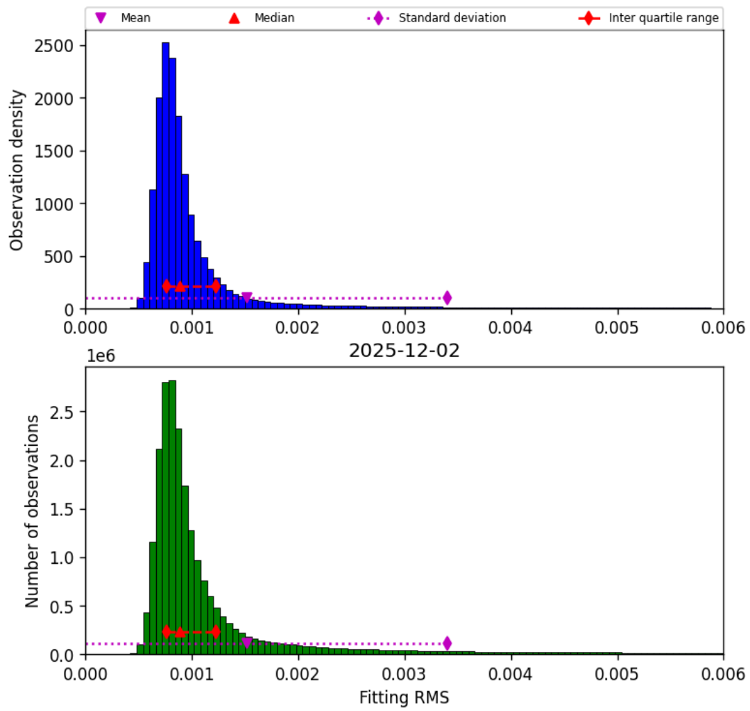
Figure 34: Histogram of “Fitting RMS” for 2025-12-02 to 2025-12-02
