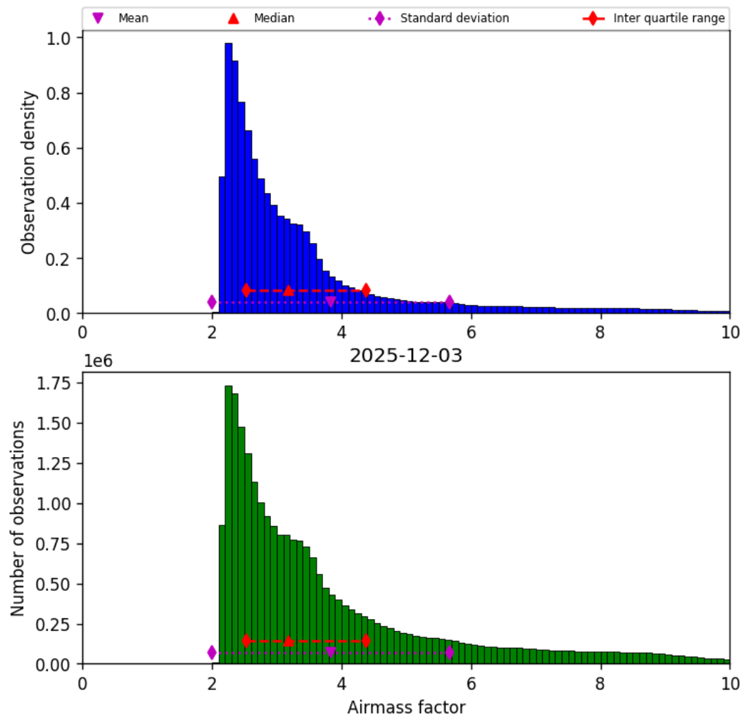
Figure 37: Histogram of “Airmass factor” for 2025-12-03 to 2025-12-04
