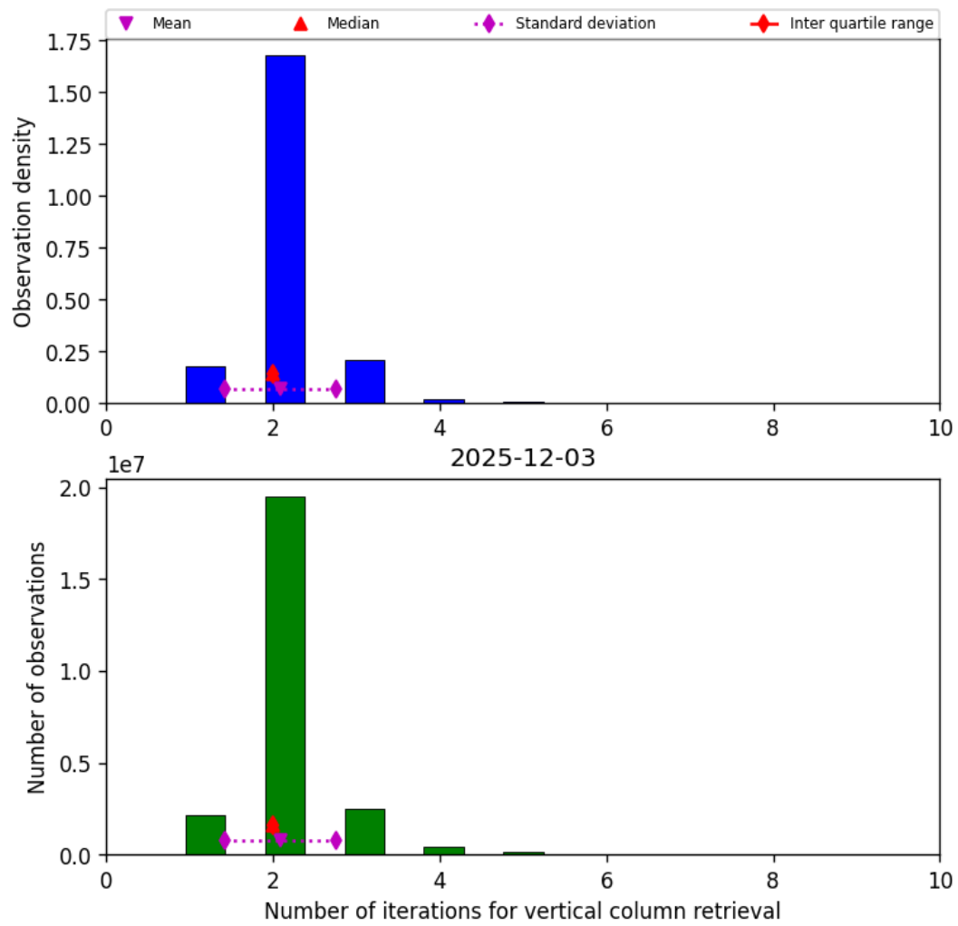
Figure 39: Histogram of “Number of iterations for vertical column retrieval” for 2025-12-03 to 2025-12-04
