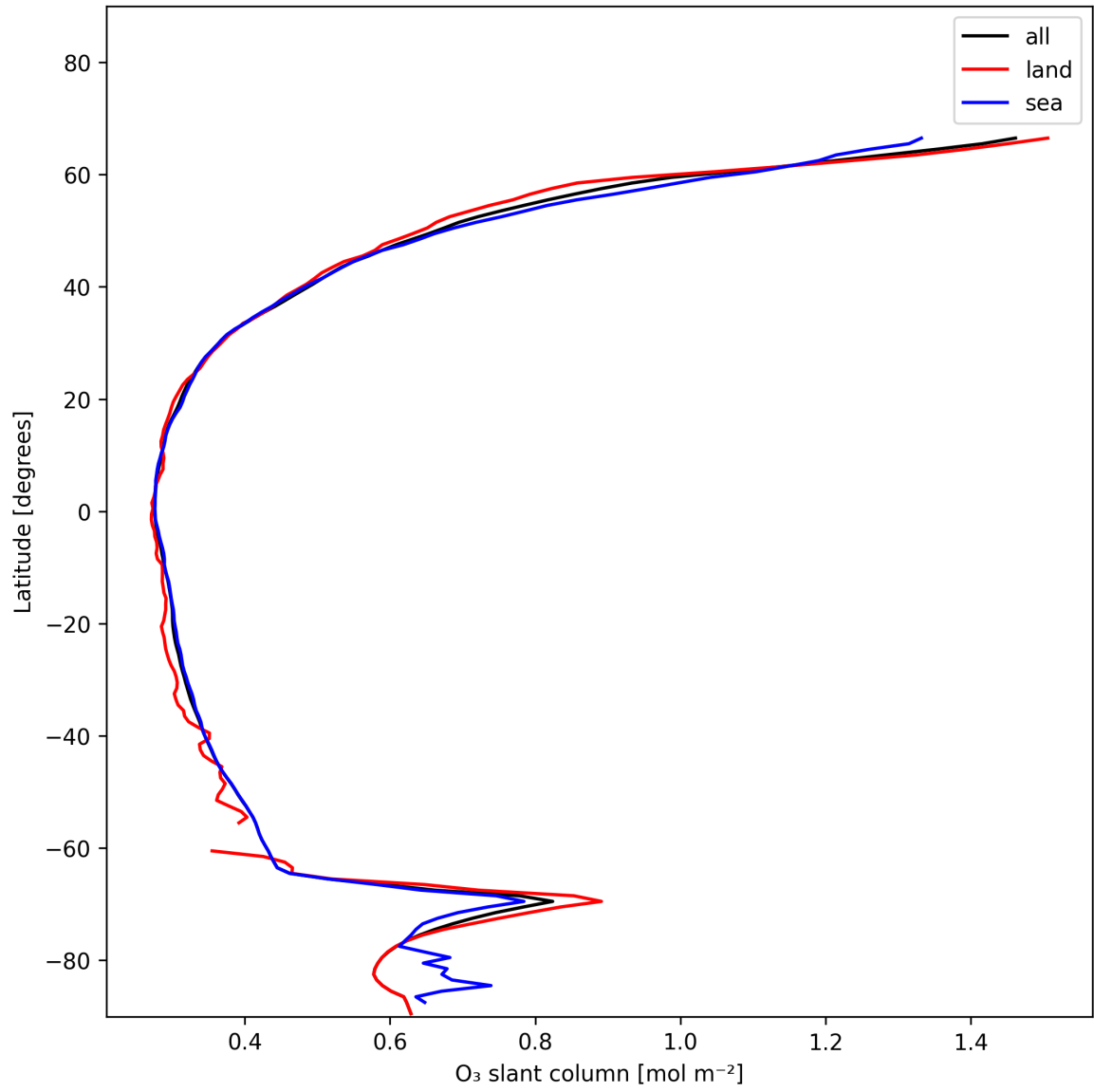
Figure 19: Zonal average of “O 3 slant column” for 2025-12-03 to 2025-12-04.
