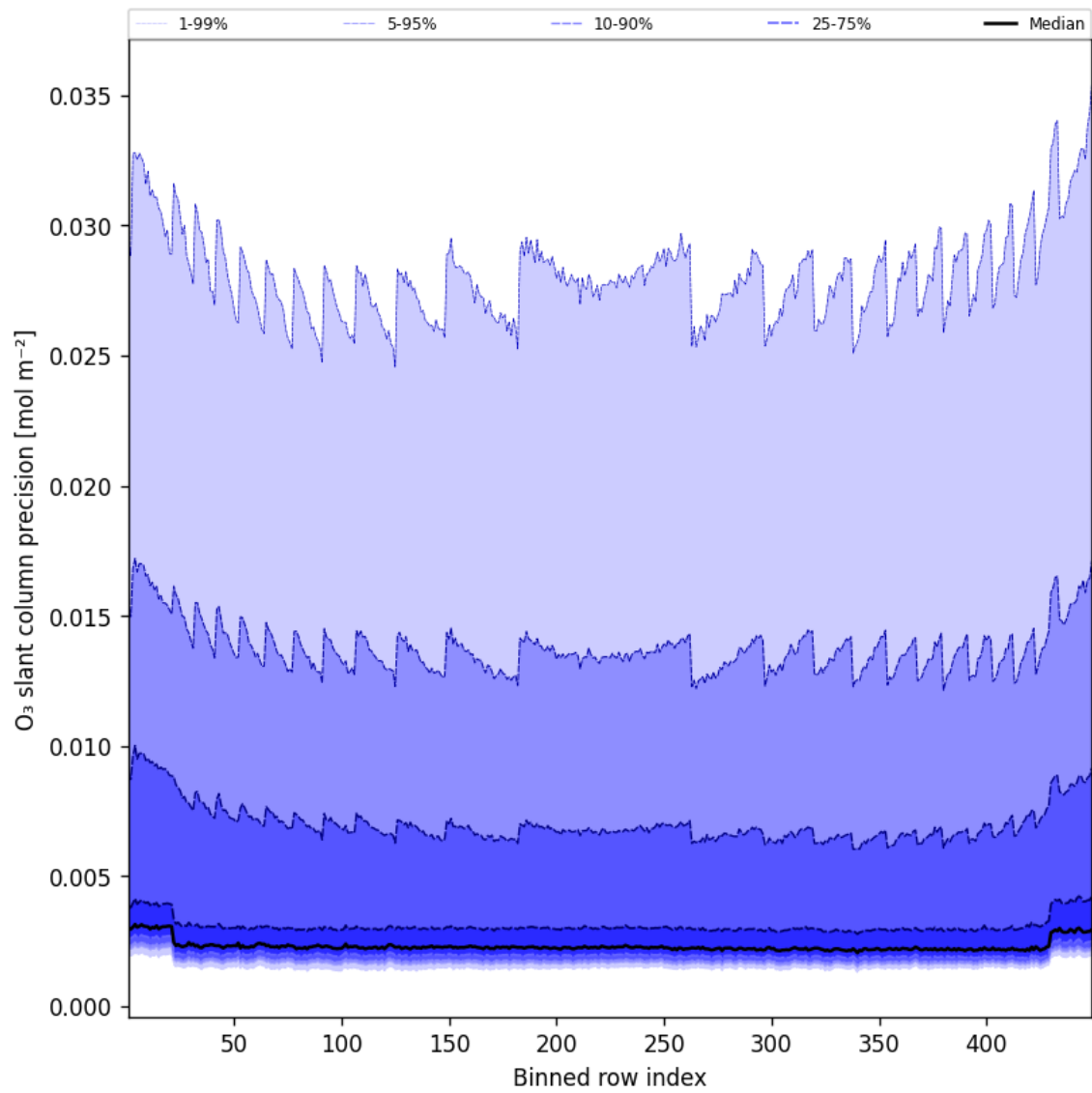
Figure 44: Along track statistics of “O 3 slant column precision” for 2025-12-03 to 2025-12-04
