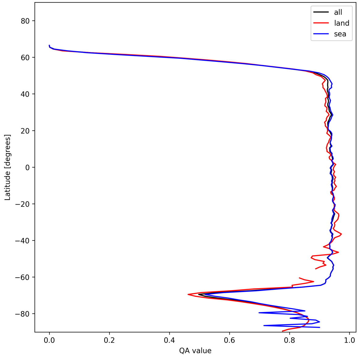
Figure 16: Zonal average of “QA value” for 2025-12-03 to 2025-12-04.
