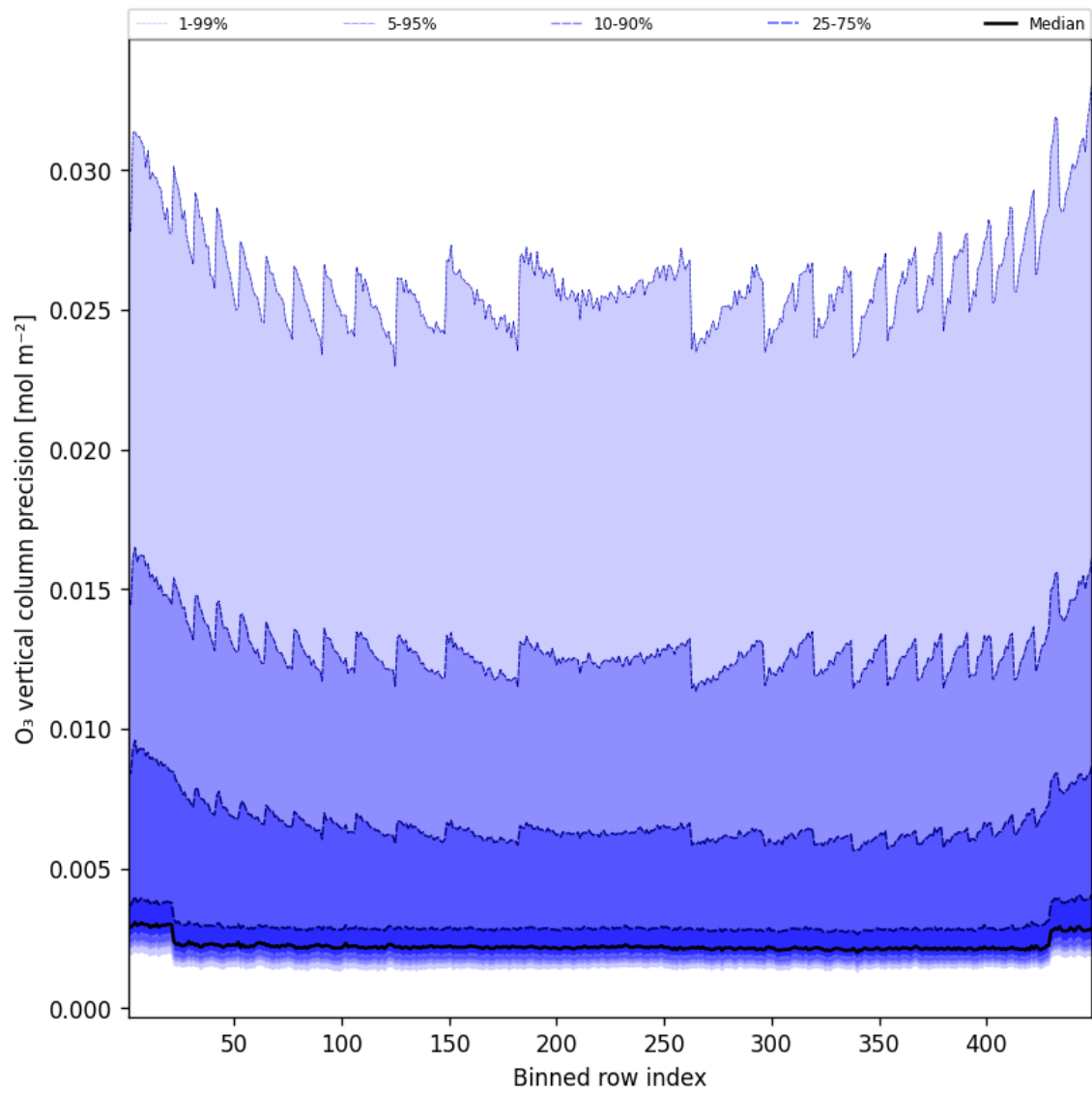
Figure 42: Along track statistics of “O 3 vertical column precision” for 2025-12-03 to 2025-12-04
