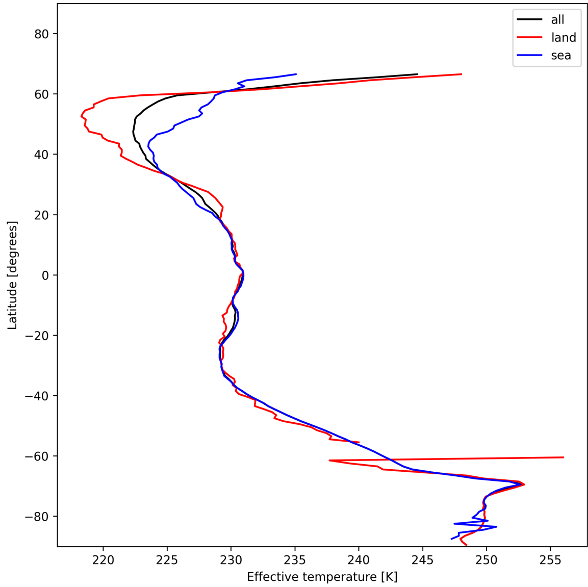
Figure 26: Zonal average of “Effective temperature” for 2025-12-03 to 2025-12-04.
