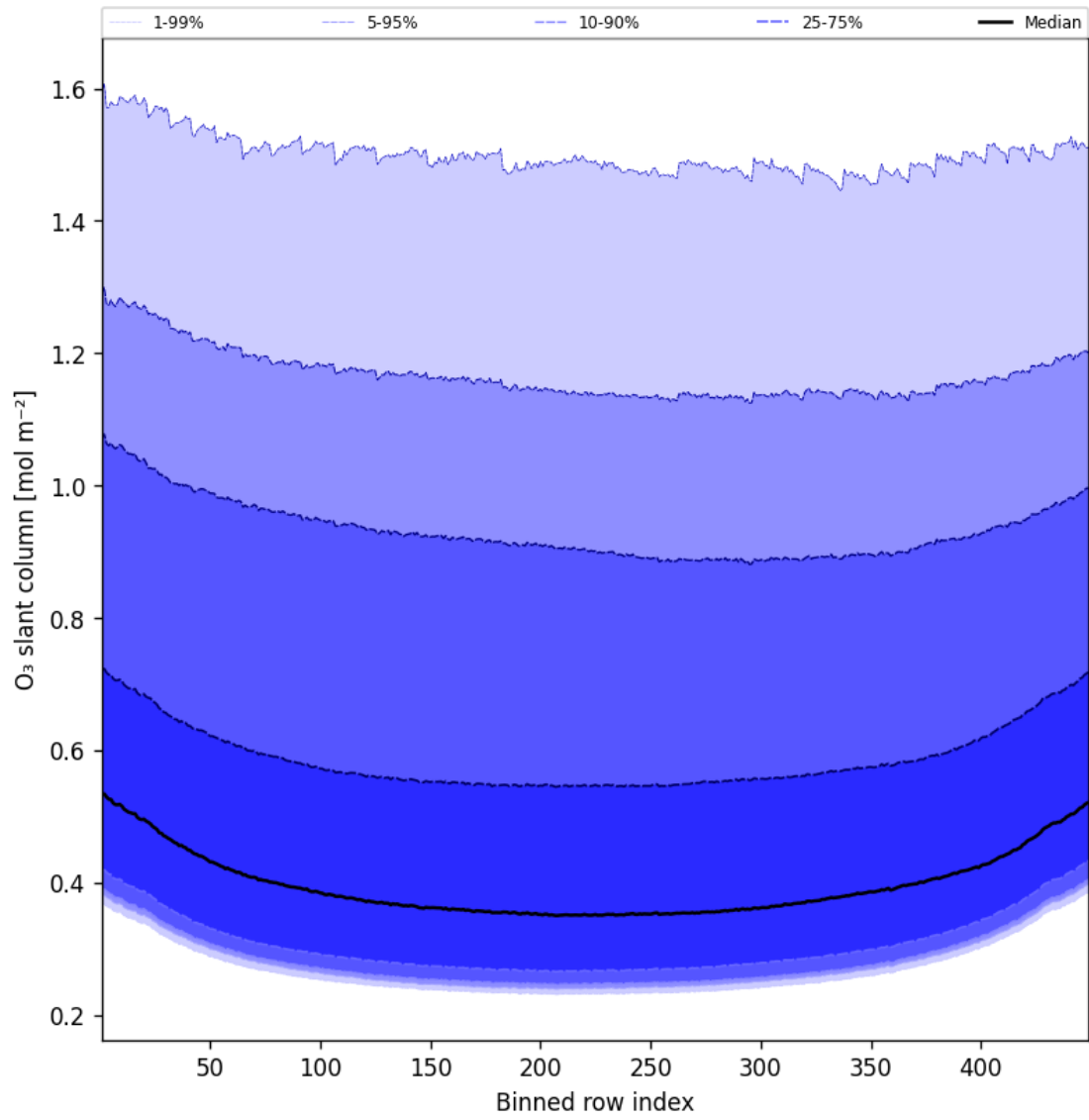
Figure 43: Along track statistics of “O 3 slant column” for 2025-12-03 to 2025-12-04
