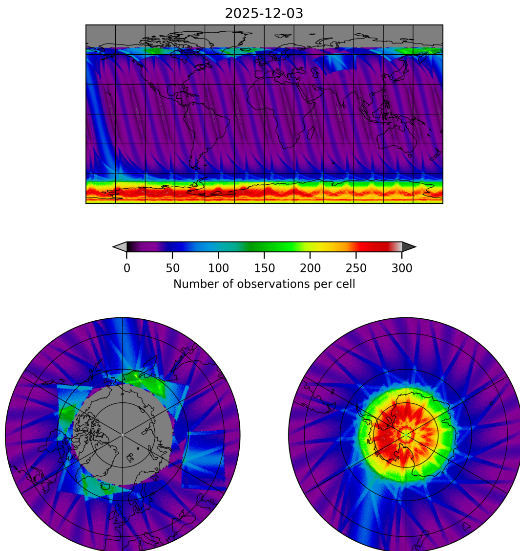
Figure 15: Map of the number of observations for 2025-12-03 to 2025-12-04
