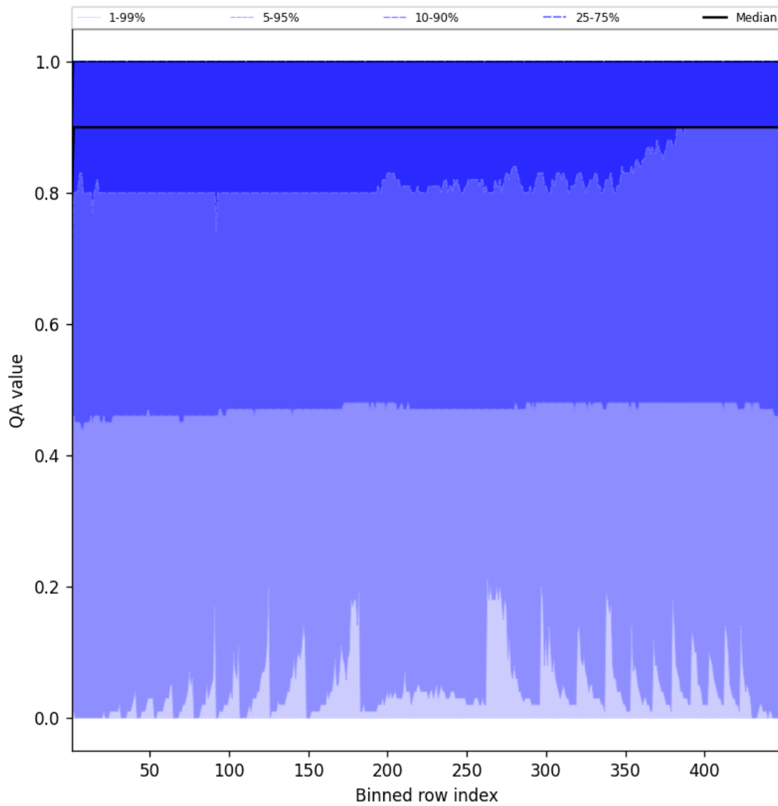
Figure 40: Along track statistics of “QA value” for 2025-12-03 to 2025-12-04
