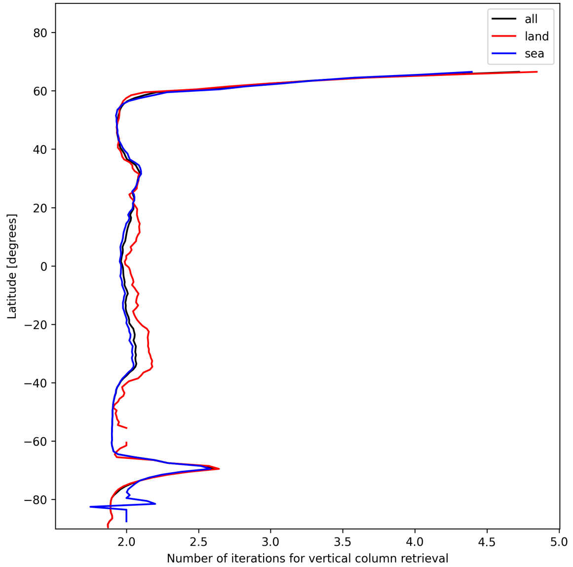
Figure 27: Zonal average of “Number of iterations for vertical column retrieval” for 2025-12-03 to 2025-12-04.
