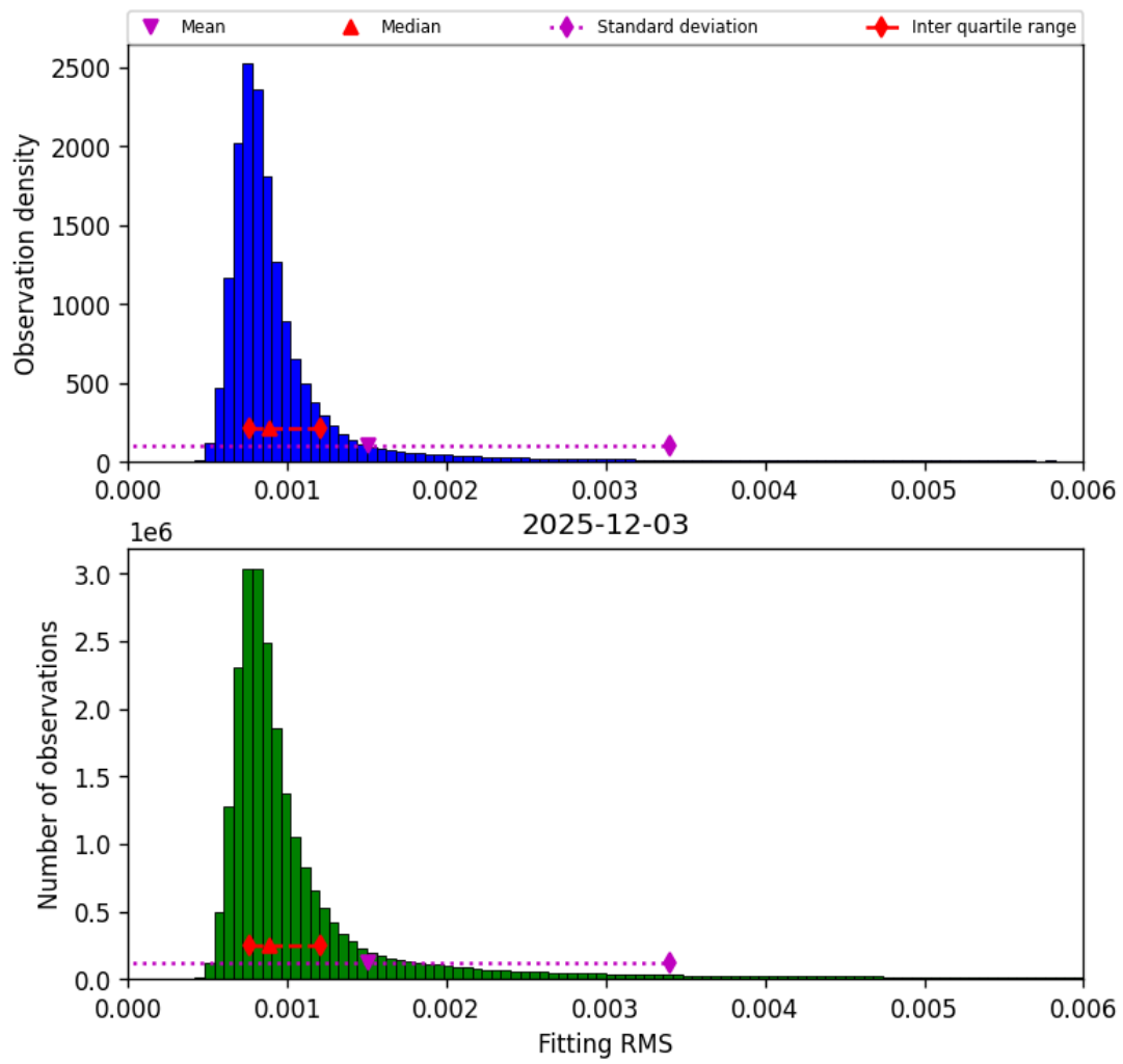
Figure 34: Histogram of “Fitting RMS” for 2025-12-03 to 2025-12-04
