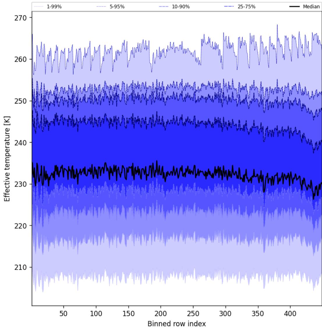
Figure 50: Along track statistics of “Effective temperature” for 2025-12-03 to 2025-12-04
