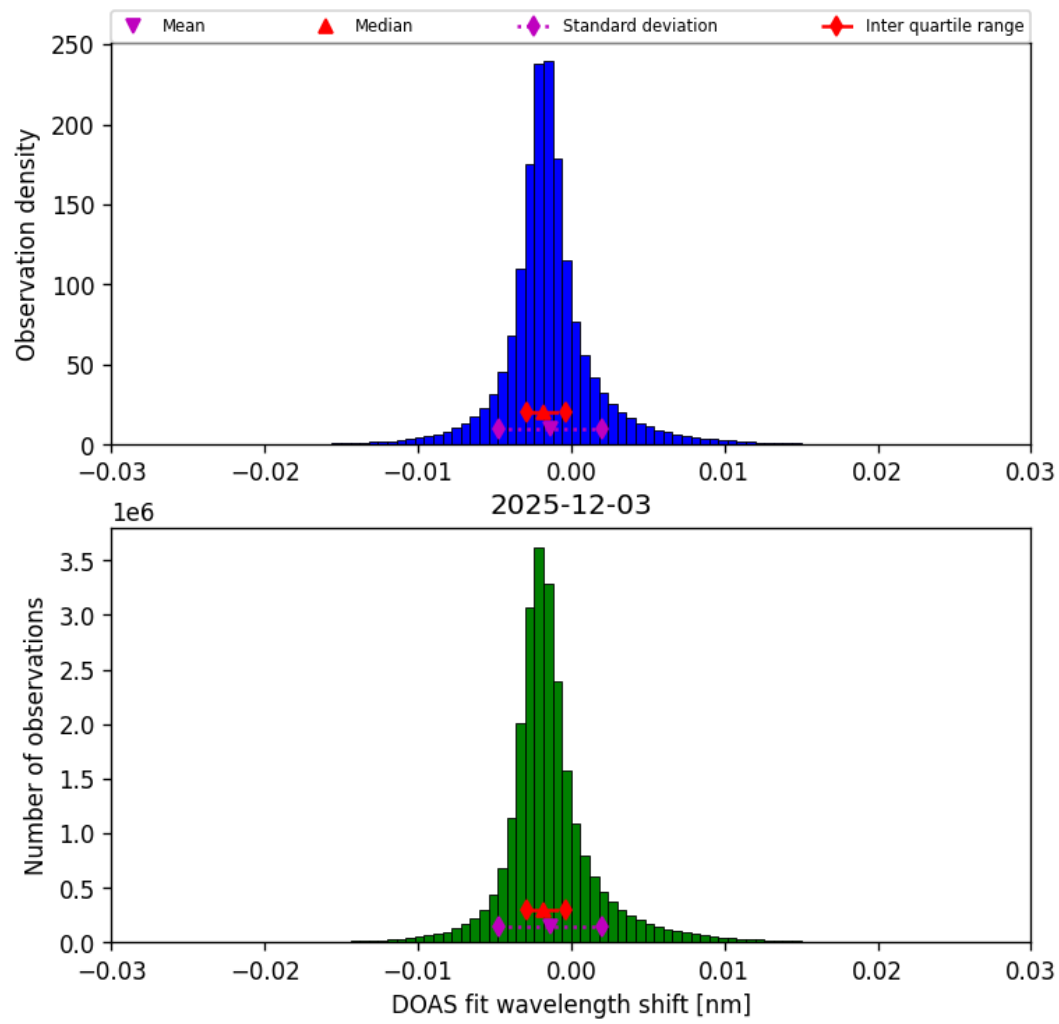
Figure 35: Histogram of “DOAS fit wavelength shift” for 2025-12-03 to 2025-12-04
