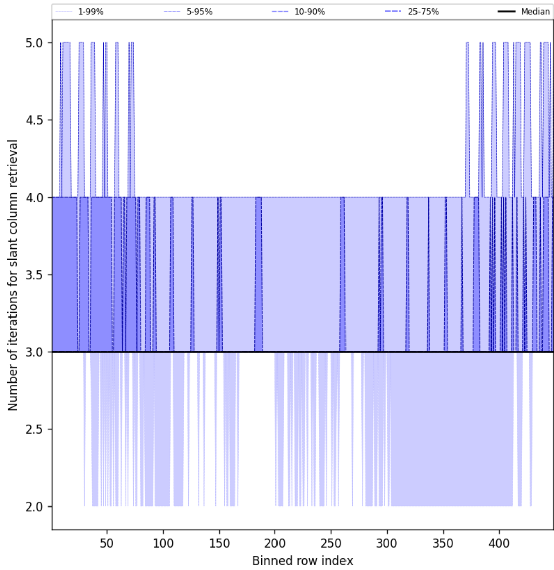
Figure 45: Along track statistics of “Number of iterations for slant column retrieval” for 2025-12-03 to 2025-12-04
