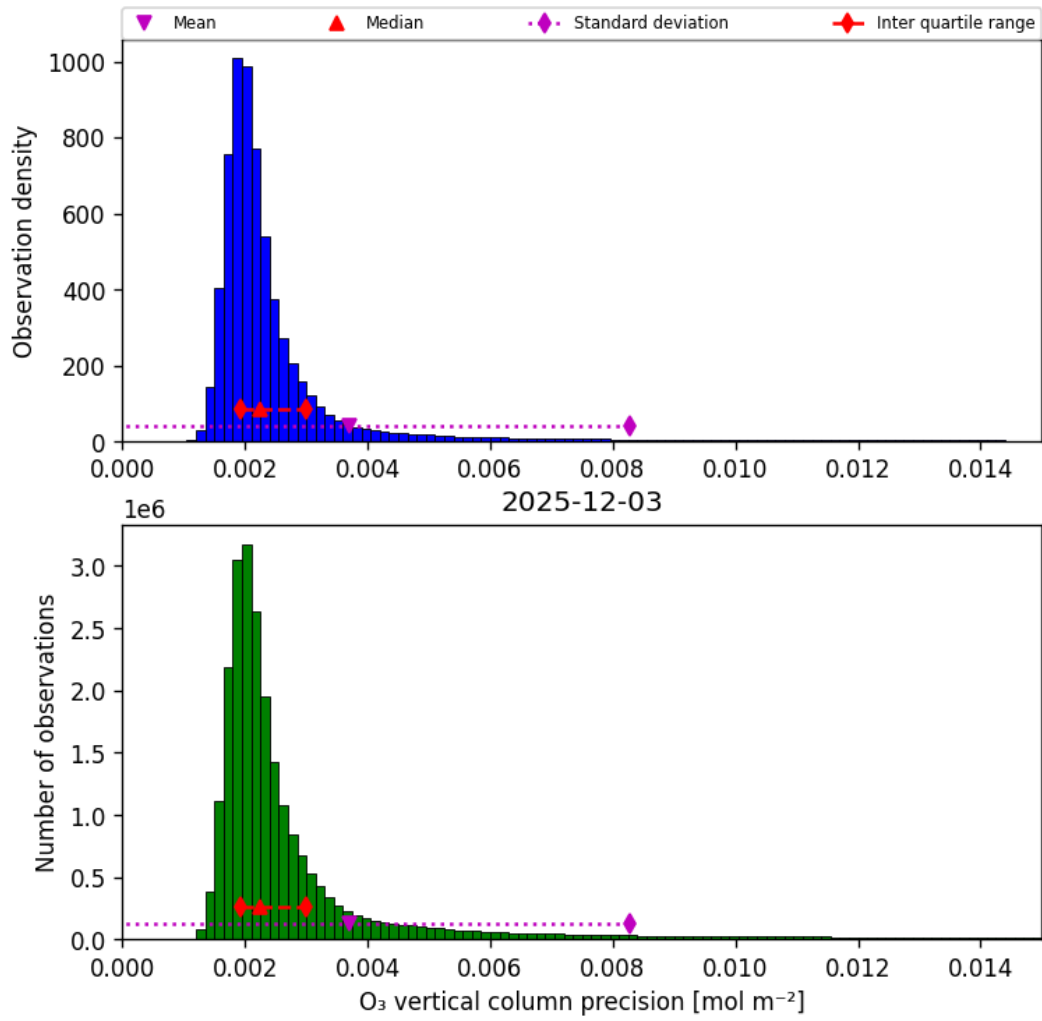
Figure 30: Histogram of "O 3 vertical column precision" for 2025-12-03 to 2025-12-04
