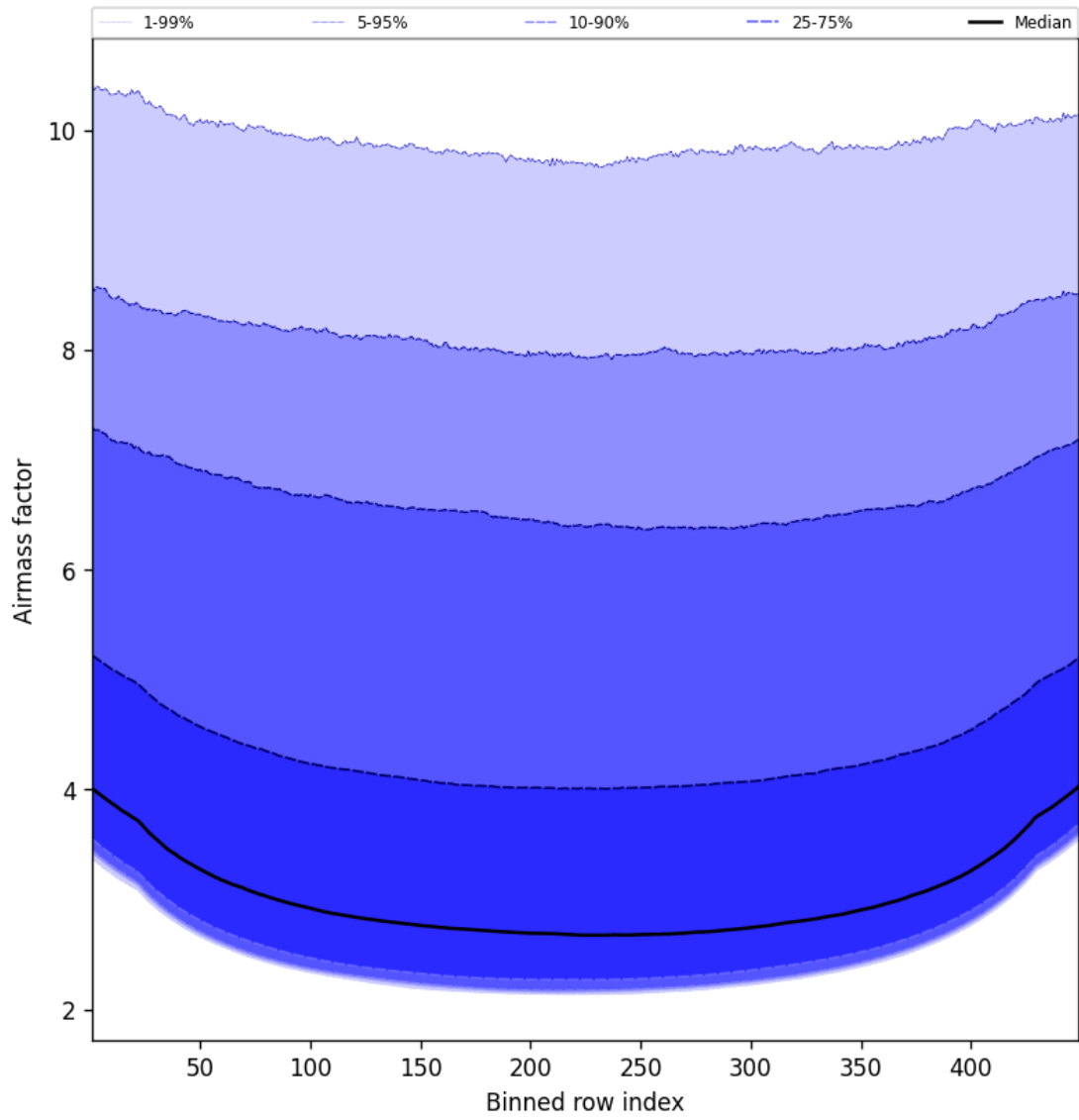
Figure 49: Along track statistics of “Airmass factor” for 2025-12-03 to 2025-12-04
