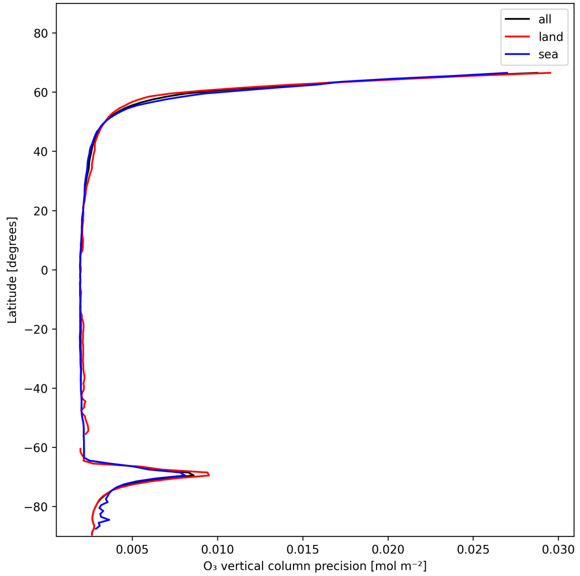
Figure 18: Zonal average of “O 3 vertical column precision” for 2025-12-03 to 2025-12-04.
