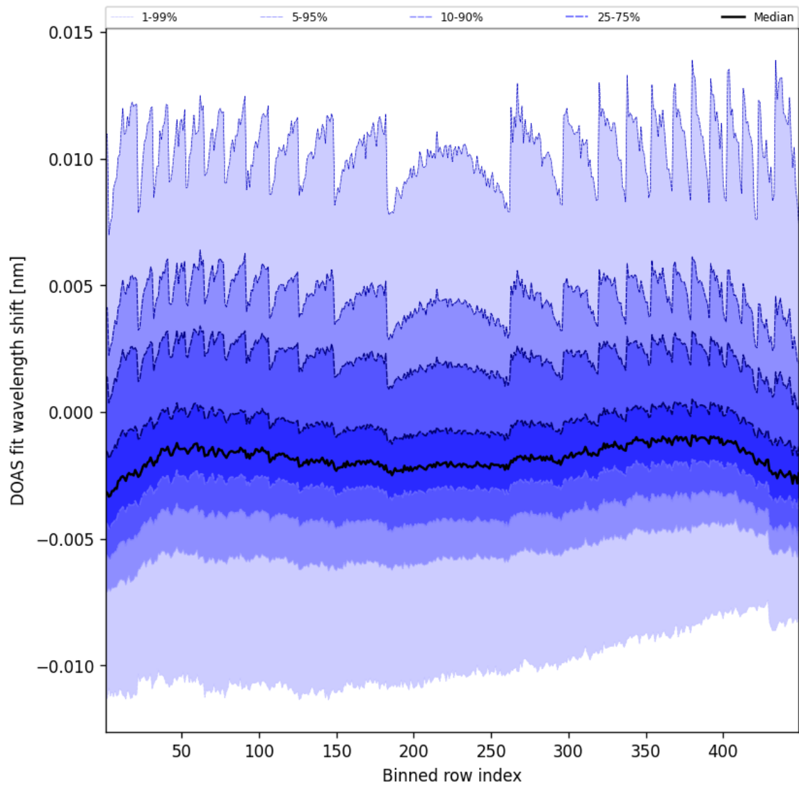
Figure 47: Along track statistics of “DOAS fit wavelength shift” for 2025-12-03 to 2025-12-04
