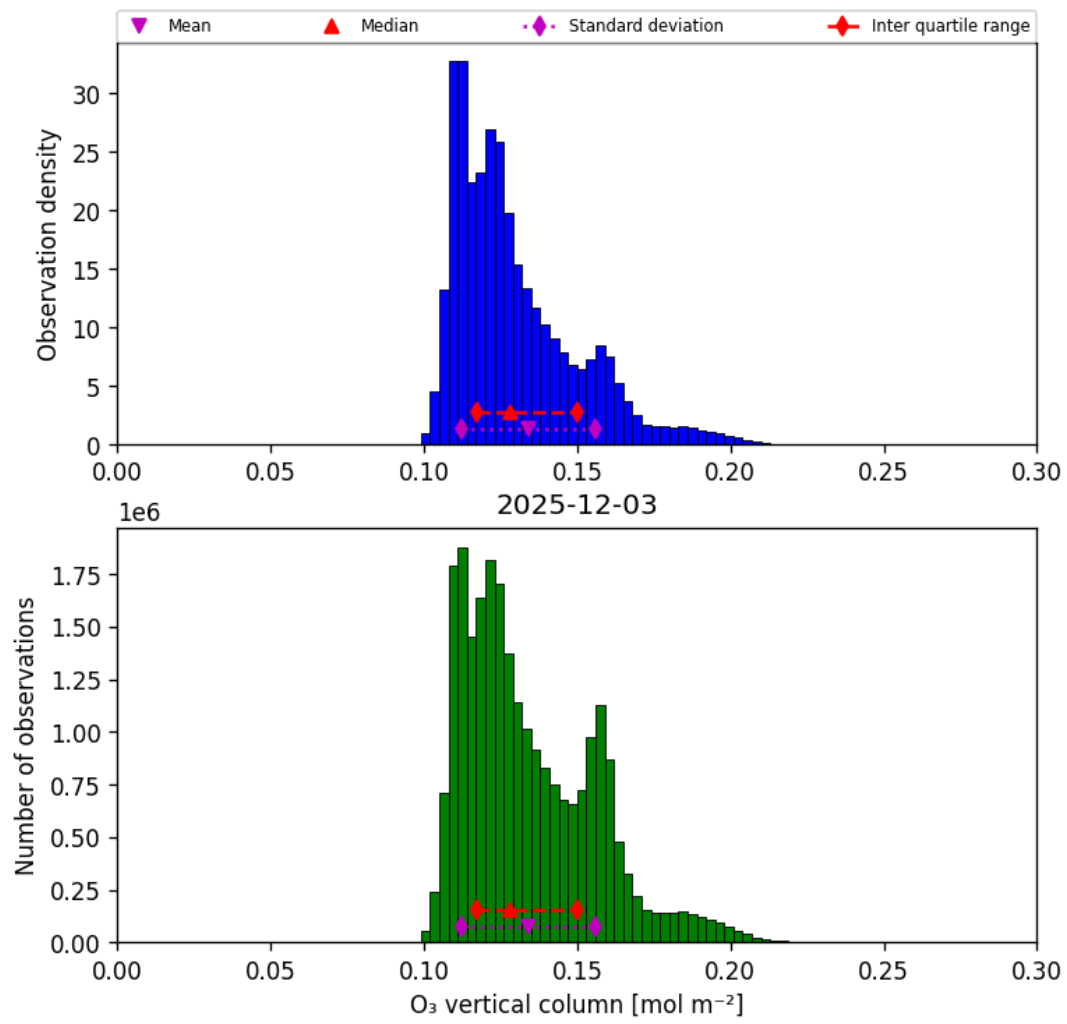
Figure 29: Histogram of “O 3 vertical column” for 2025-12-03 to 2025-12-04
