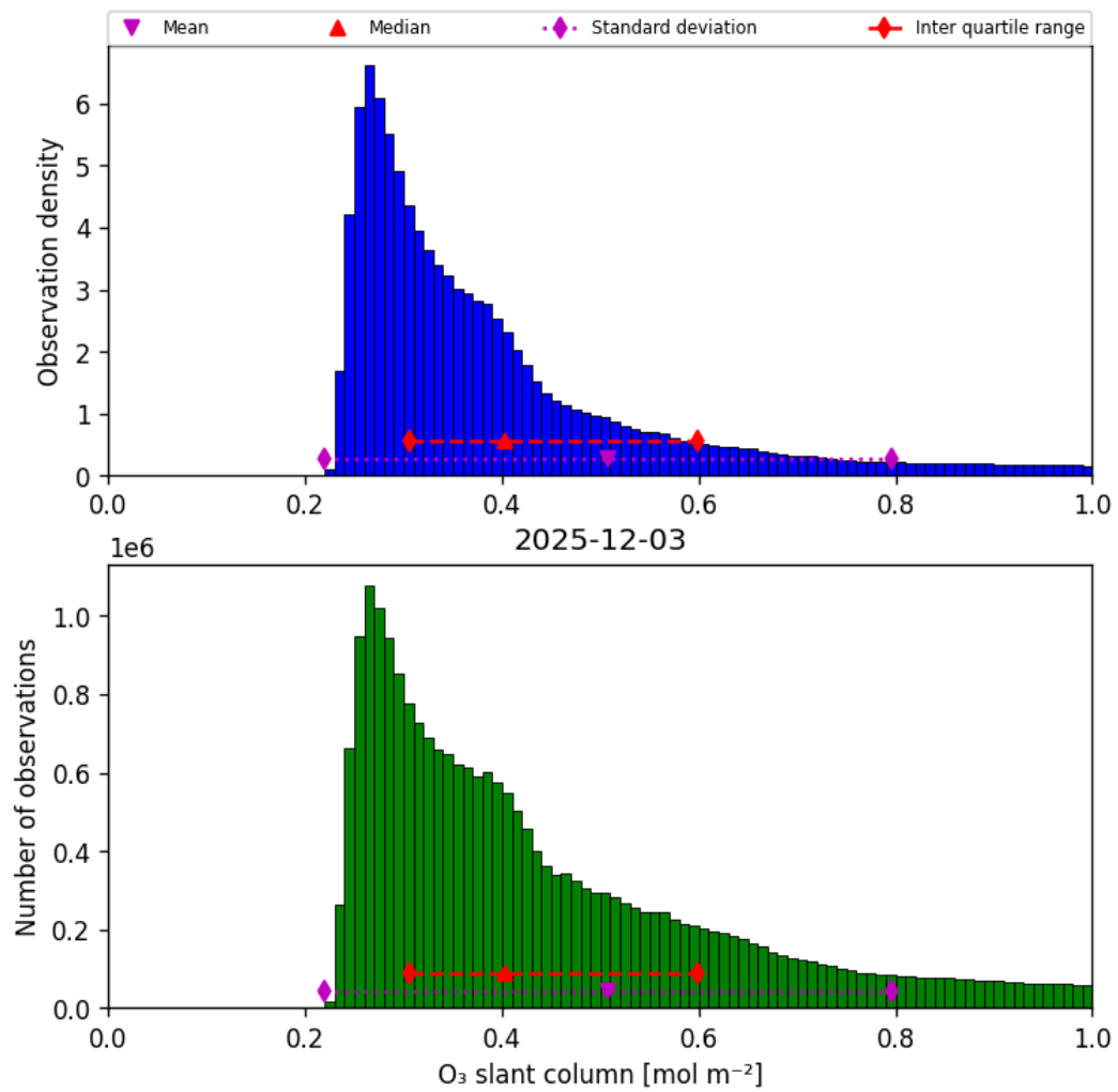
Figure 31: Histogram of “O 3 slant column” for 2025-12-03 to 2025-12-04
