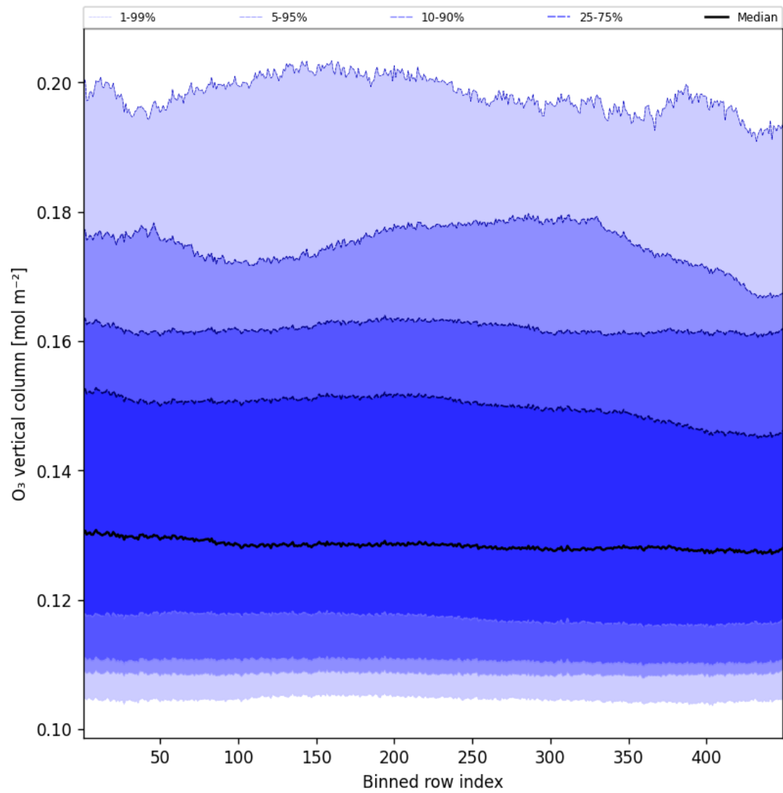
Figure 41: Along track statistics of “ \text{O}_3 vertical column” for 2025-12-03 to 2025-12-04
