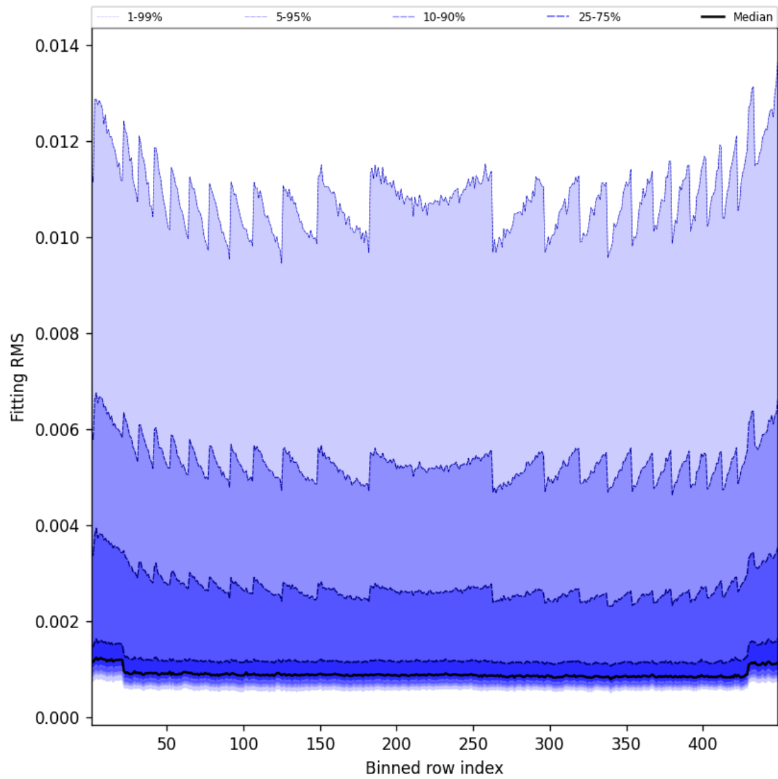
Figure 46: Along track statistics of “Fitting RMS” for 2025-12-03 to 2025-12-04
