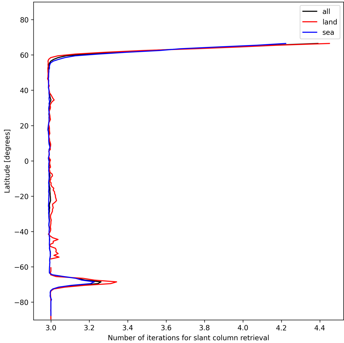
Figure 21: Zonal average of “Number of iterations for slant column retrieval” for 2025-12-03 to 2025-12-04.
