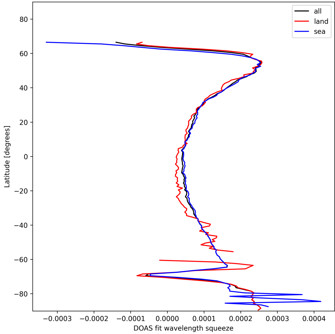
Figure 24: Zonal average of “DOAS fit wavelength squeeze” for 2025-12-03 to 2025-12-04.
