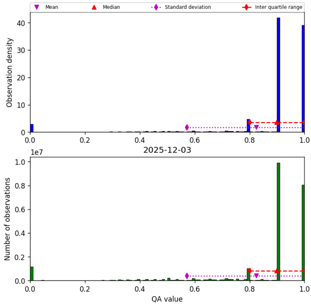
Figure 28: Histogram of “QA value” for 2025-12-03 to 2025-12-04
