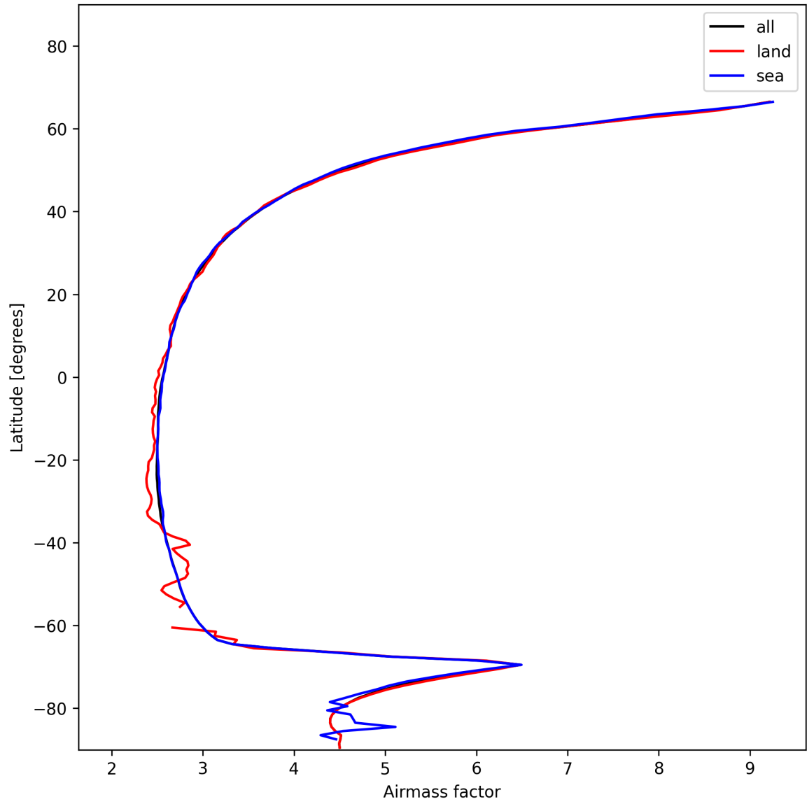
Figure 25: Zonal average of “Airmass factor” for 2025-12-03 to 2025-12-04.
