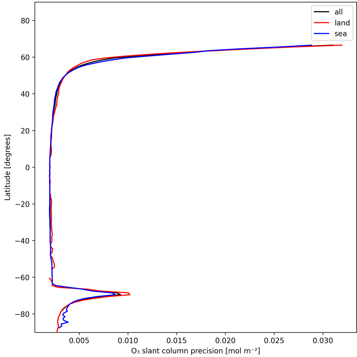
Figure 20: Zonal average of “O 3 slant column precision” for 2025-12-03 to 2025-12-04.
