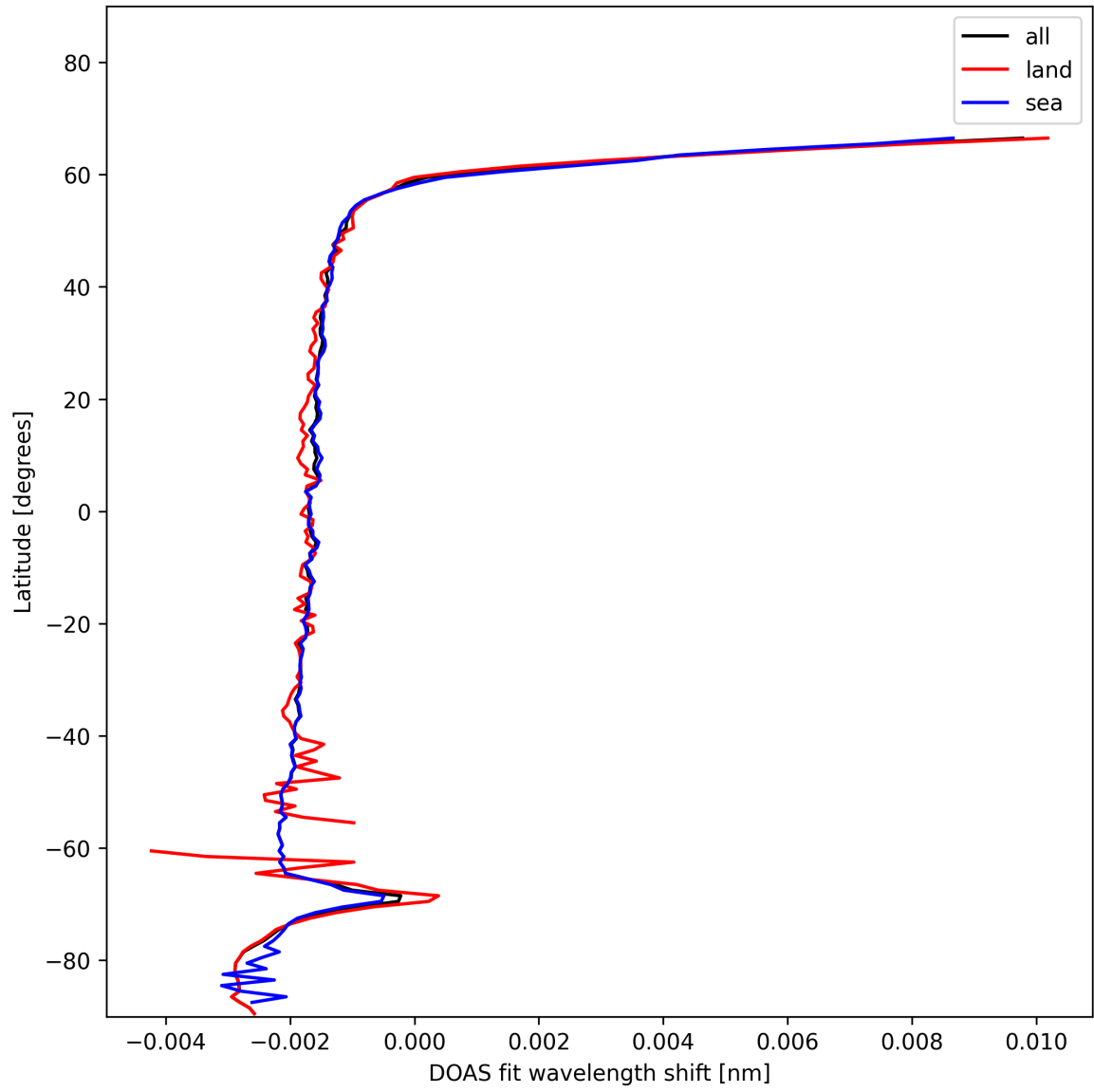
Figure 23: Zonal average of “DOAS fit wavelength shift” for 2025-12-03 to 2025-12-04.
