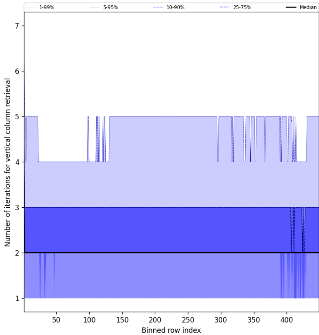
Figure 51: Along track statistics of “Number of iterations for vertical column retrieval” for 2025-12-03 to 2025-12-04
