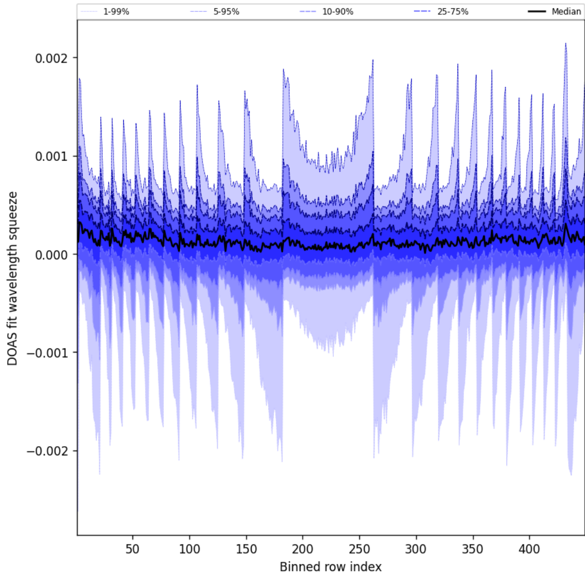
Figure 48: Along track statistics of “DOAS fit wavelength squeeze” for 2025-12-03 to 2025-12-04
