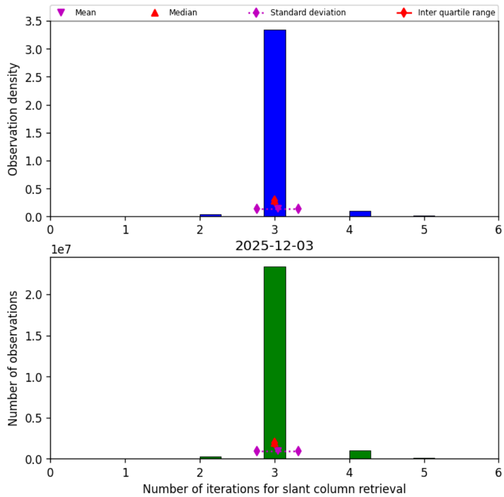
Figure 33: Histogram of “Number of iterations for slant column retrieval” for 2025-12-03 to 2025-12-04
