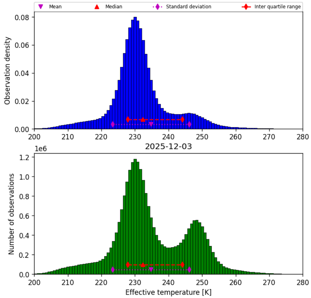
Figure 38: Histogram of “Effective temperature” for 2025-12-03 to 2025-12-04
