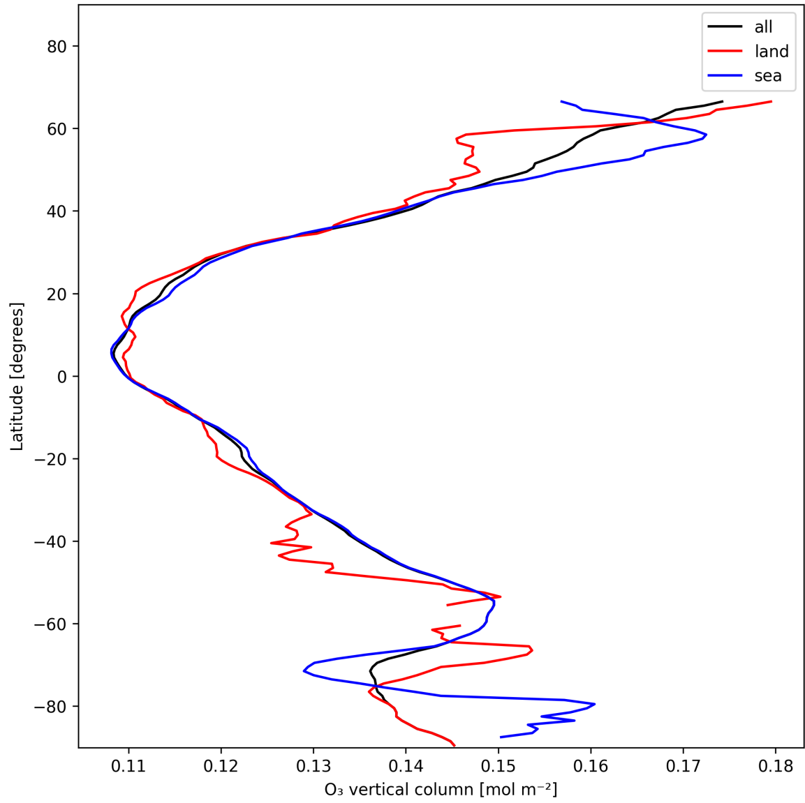
Figure 17: Zonal average of “O 3 vertical column” for 2025-12-03 to 2025-12-04.
