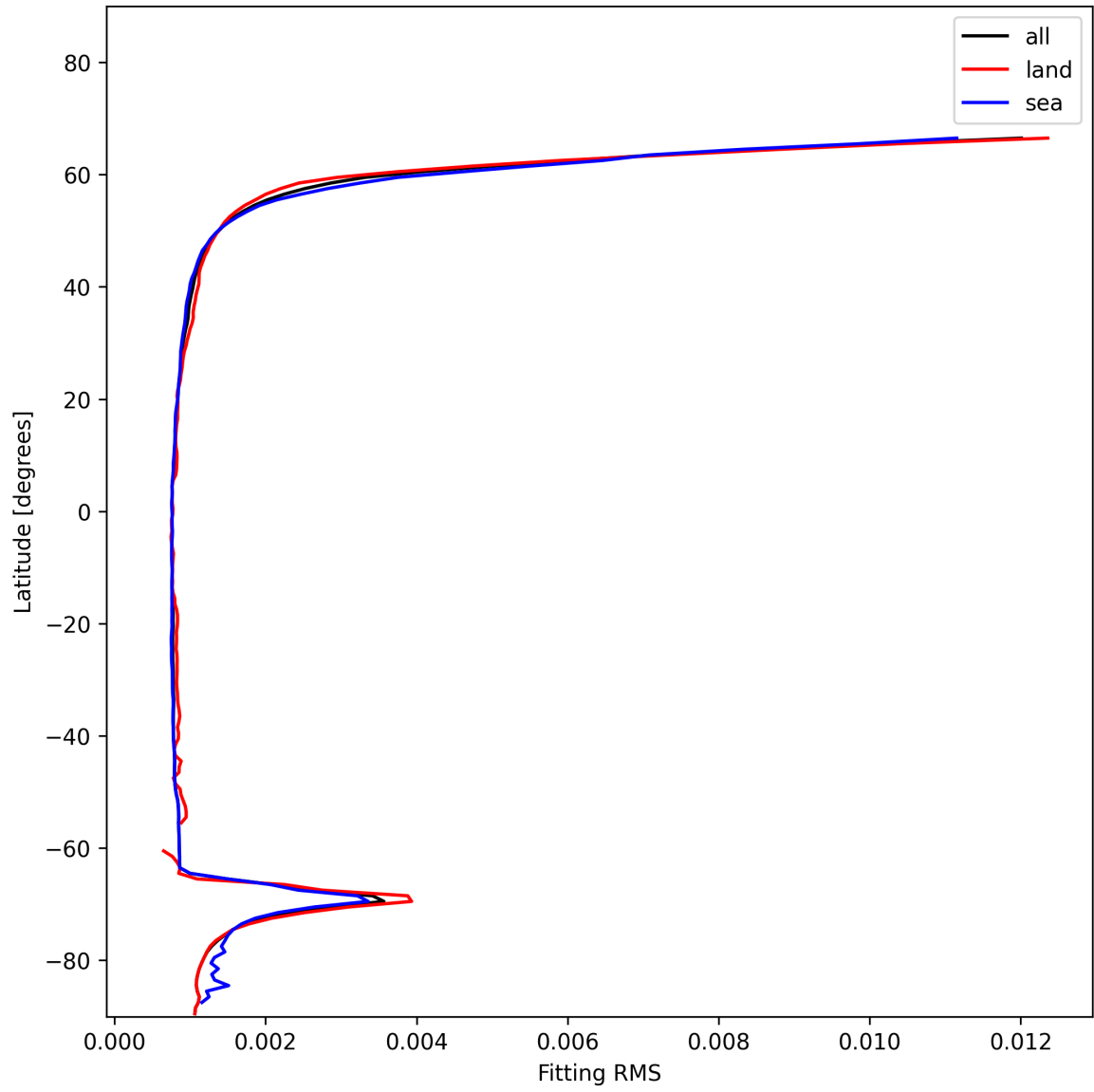
Figure 22: Zonal average of “Fitting RMS” for 2025-12-03 to 2025-12-04.
