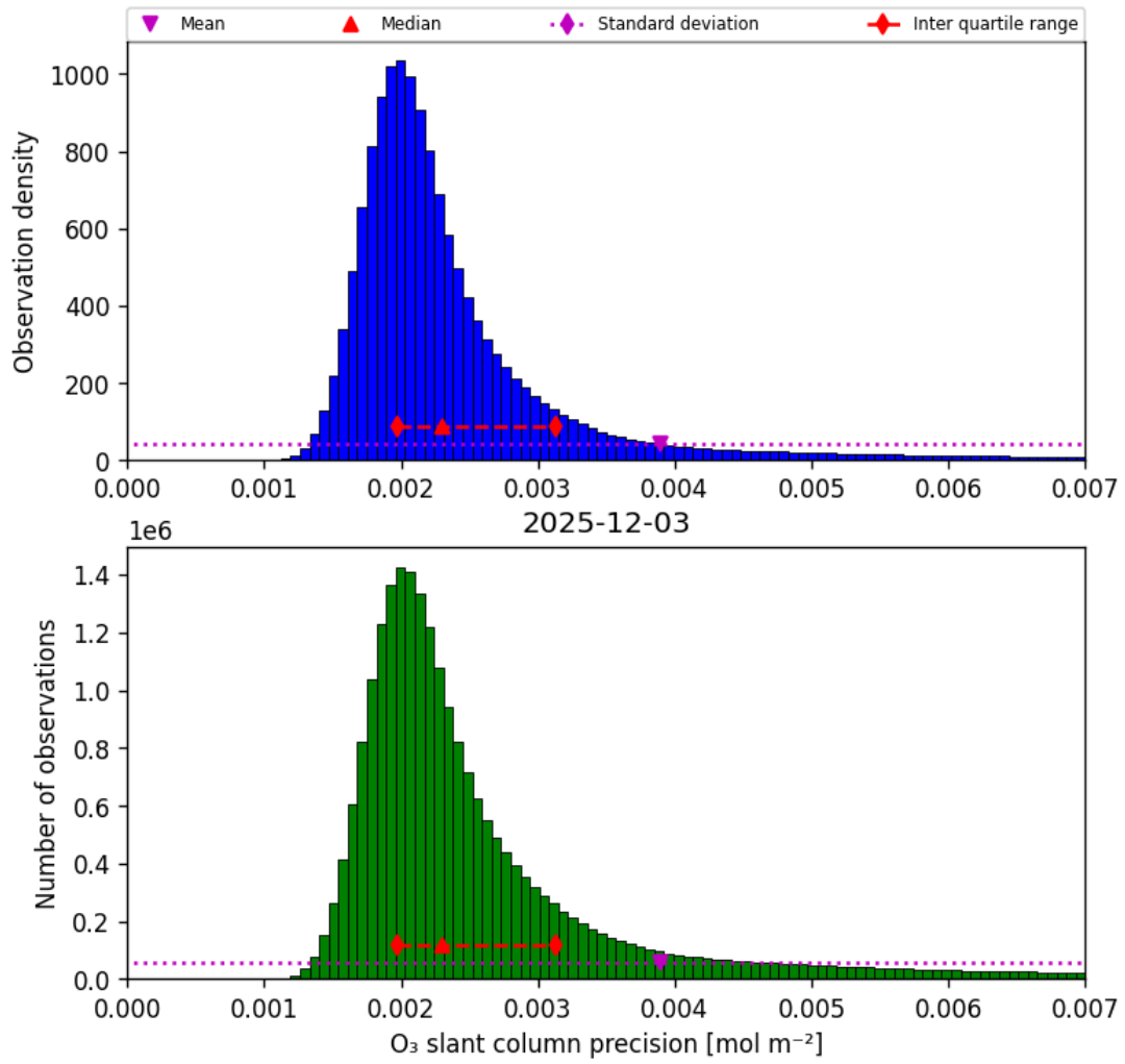
Figure 32: Histogram of “O 3 slant column precision” for 2025-12-03 to 2025-12-04
