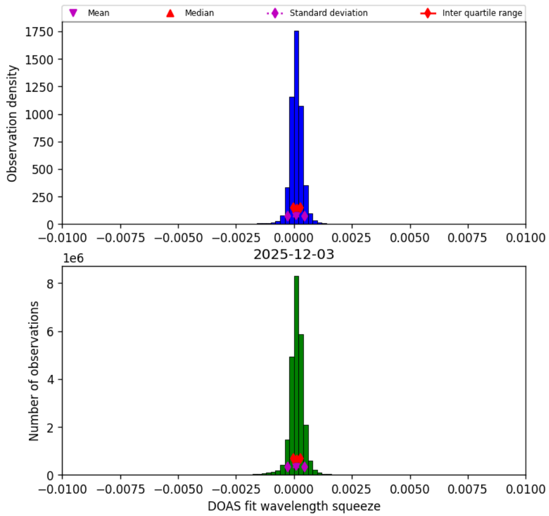
Figure 36: Histogram of “DOAS fit wavelength squeeze” for 2025-12-03 to 2025-12-04
