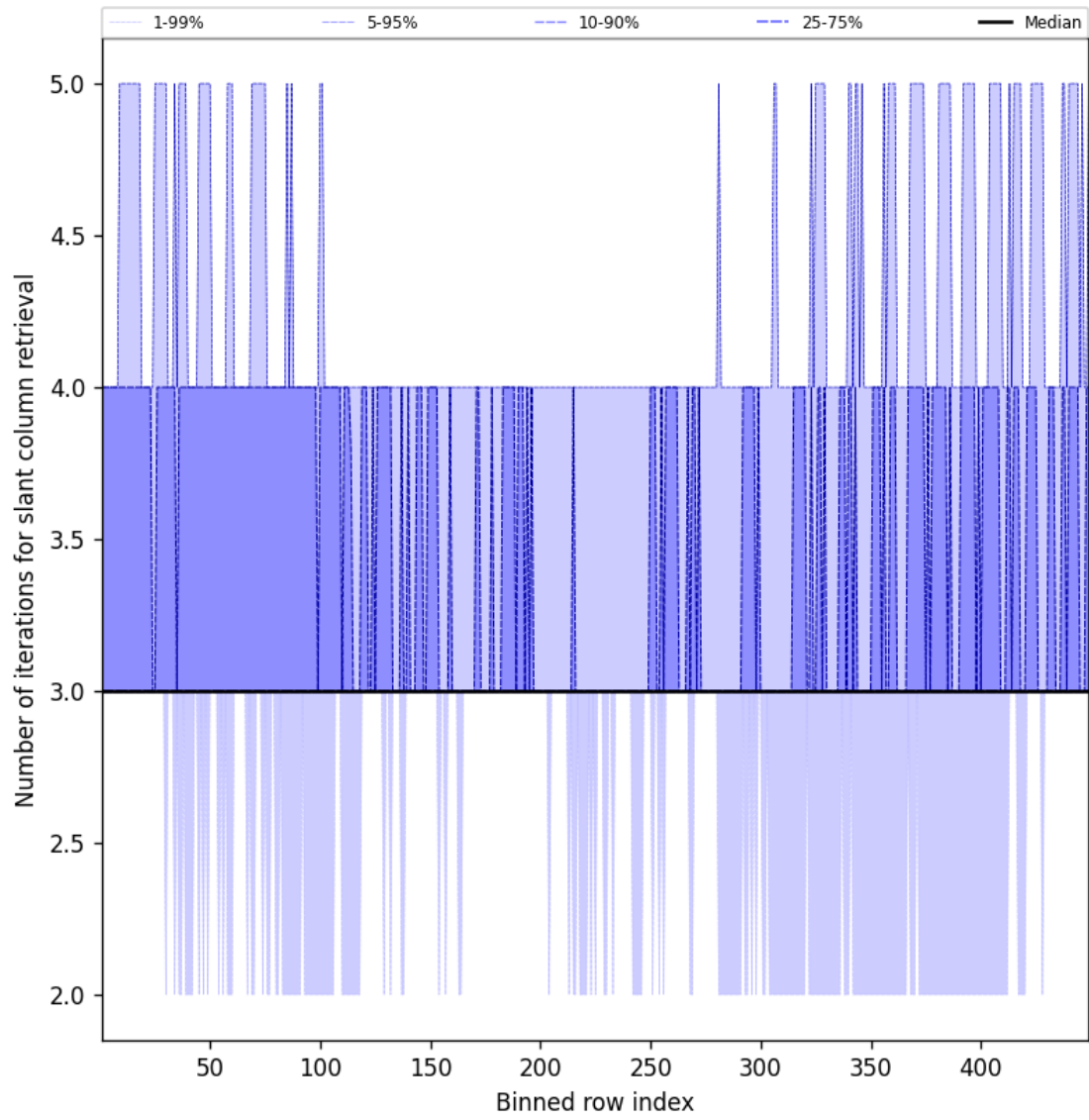
Figure 45: Along track statistics of “Number of iterations for slant column retrieval” for 2025-12-04 to 2025-12-05
