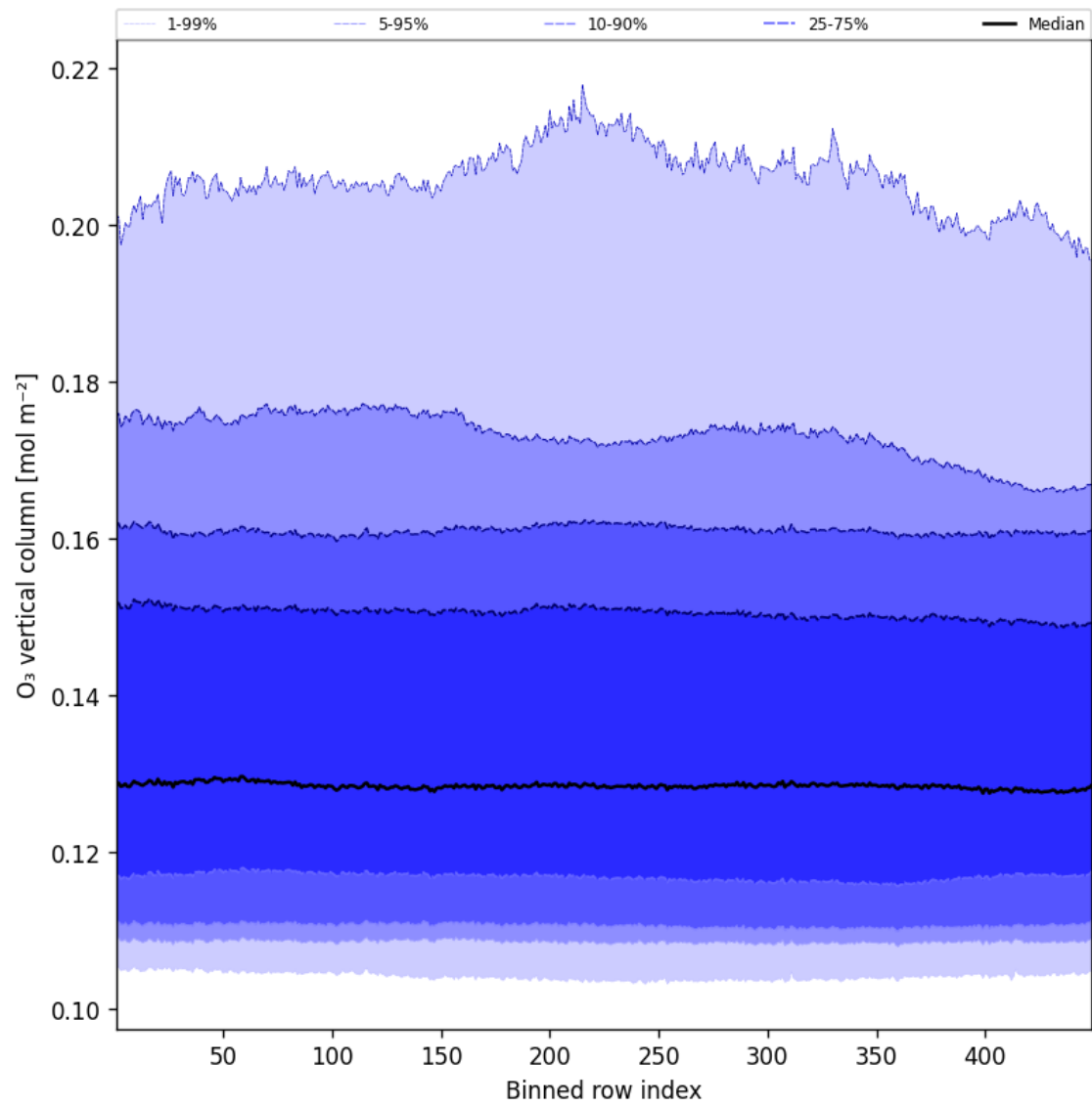
Figure 41: Along track statistics of “O 3 vertical column” for 2025-12-04 to 2025-12-05
