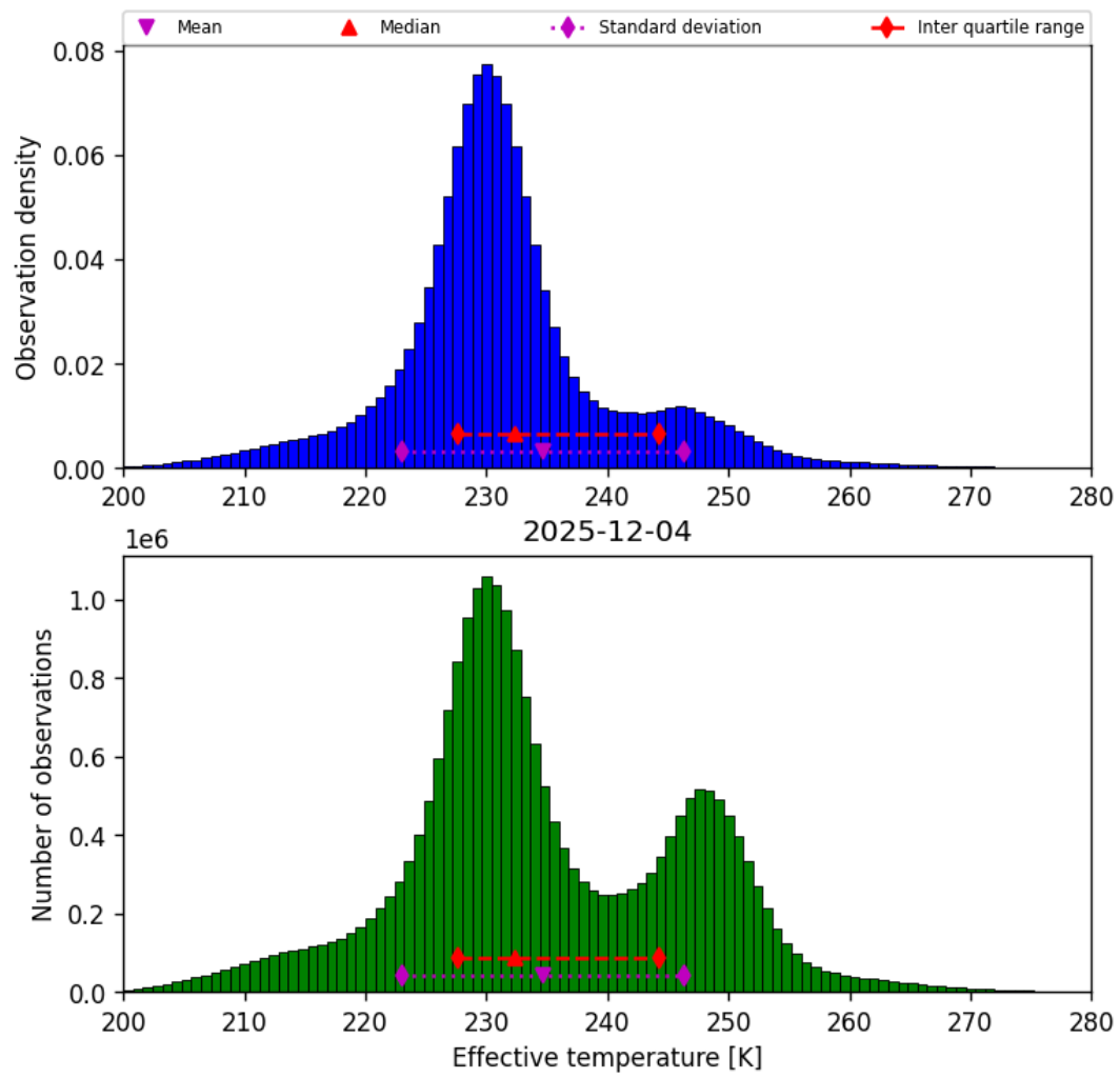
Figure 38: Histogram of “Effective temperature” for 2025-12-04 to 2025-12-05
