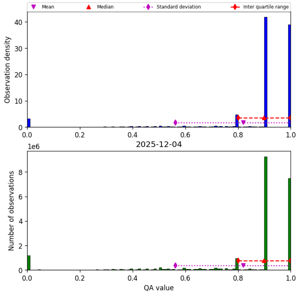
Figure 28: Histogram of “QA value” for 2025-12-04 to 2025-12-05
