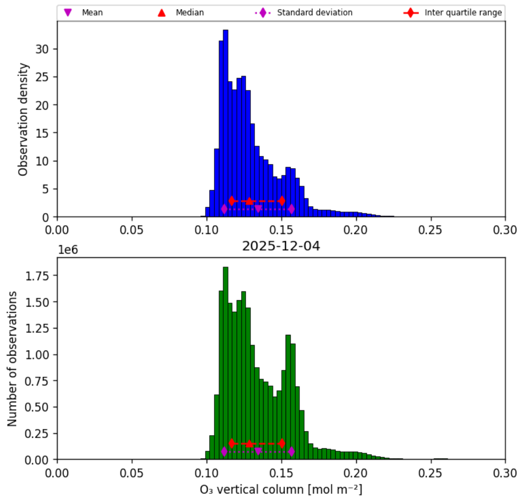
Figure 29: Histogram of “O 3 vertical column” for 2025-12-04 to 2025-12-05
