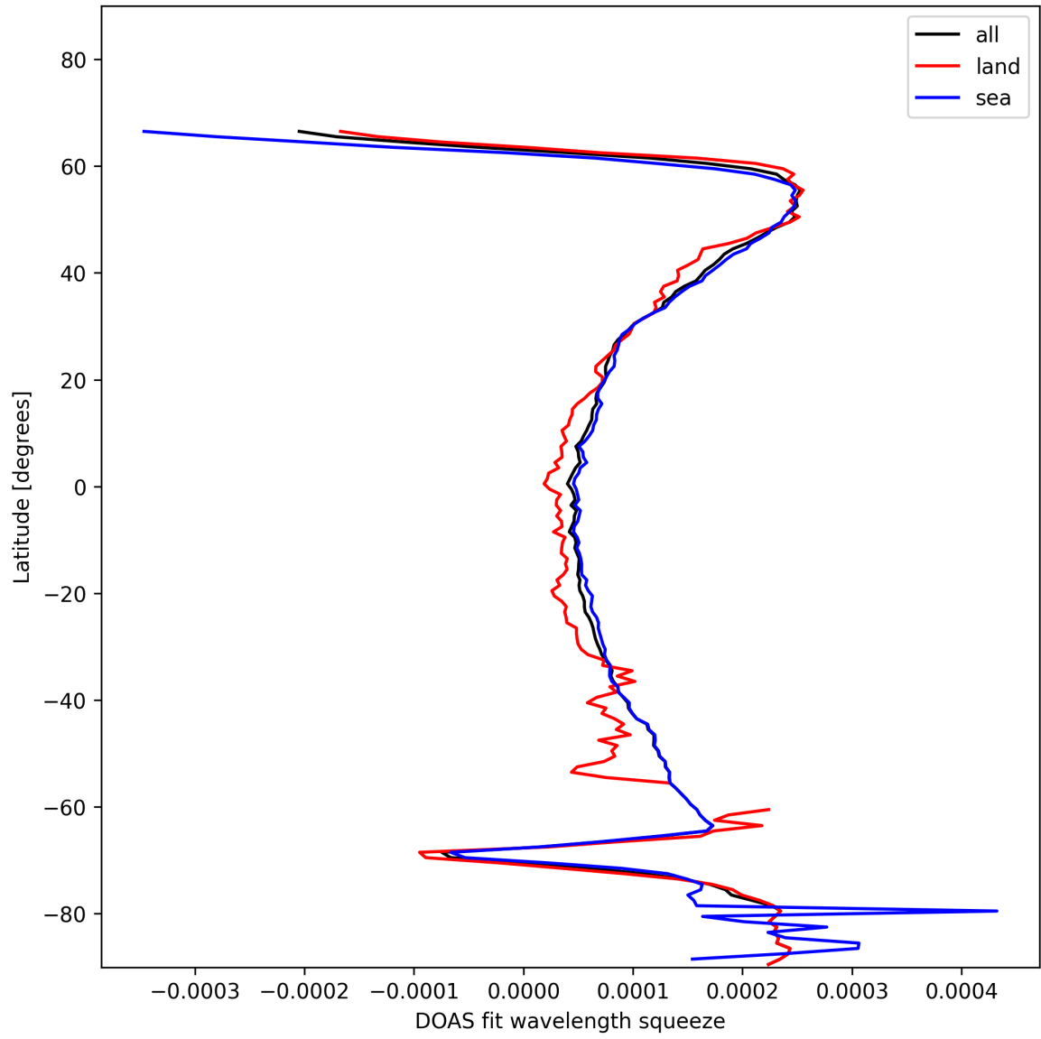
Figure 24: Zonal average of “DOAS fit wavelength squeeze” for 2025-12-04 to 2025-12-05.
