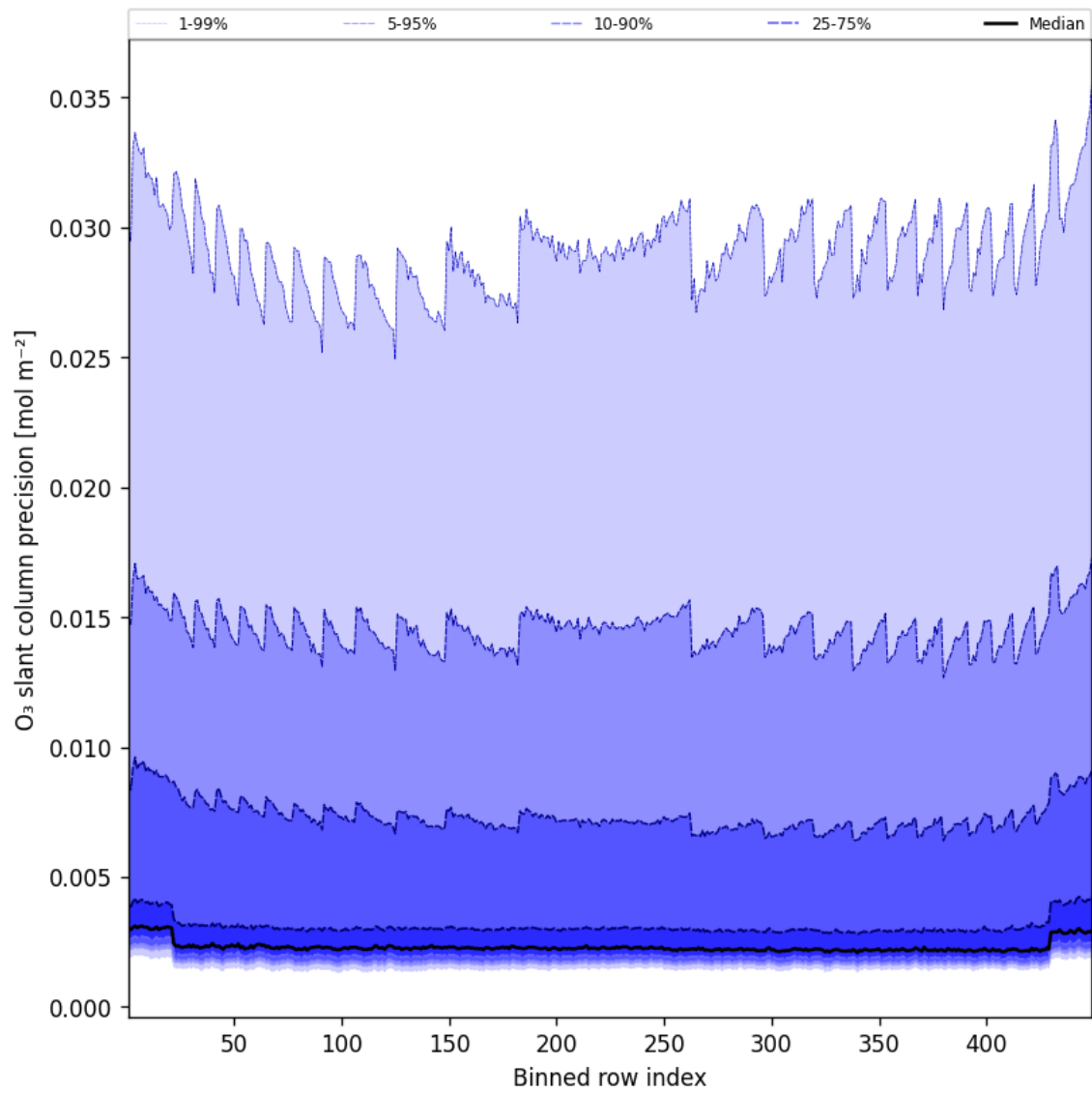
Figure 44: Along track statistics of “O 3 slant column precision” for 2025-12-04 to 2025-12-05
