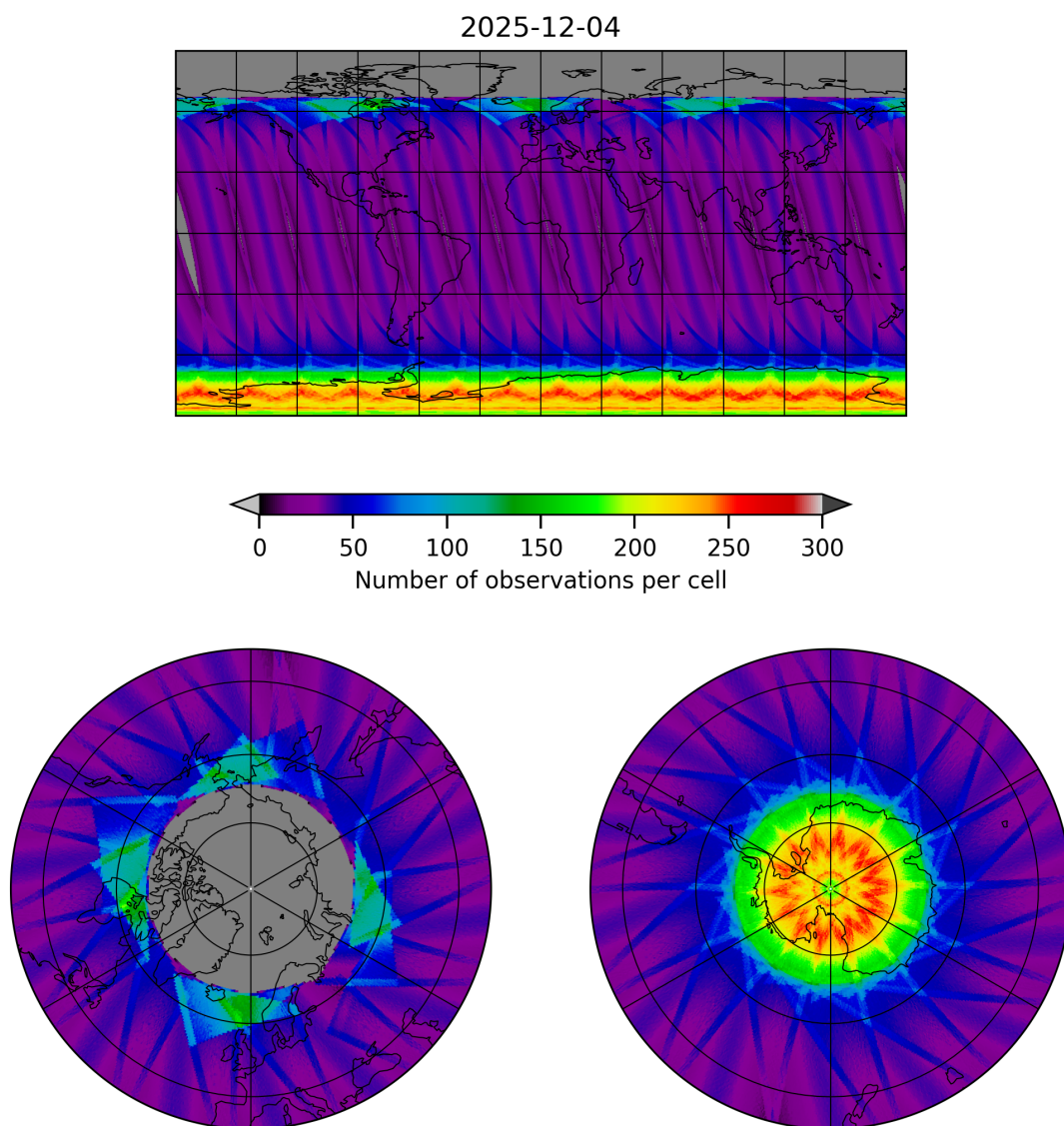
Figure 15: Map of the number of observations for 2025-12-04 to 2025-12-05
