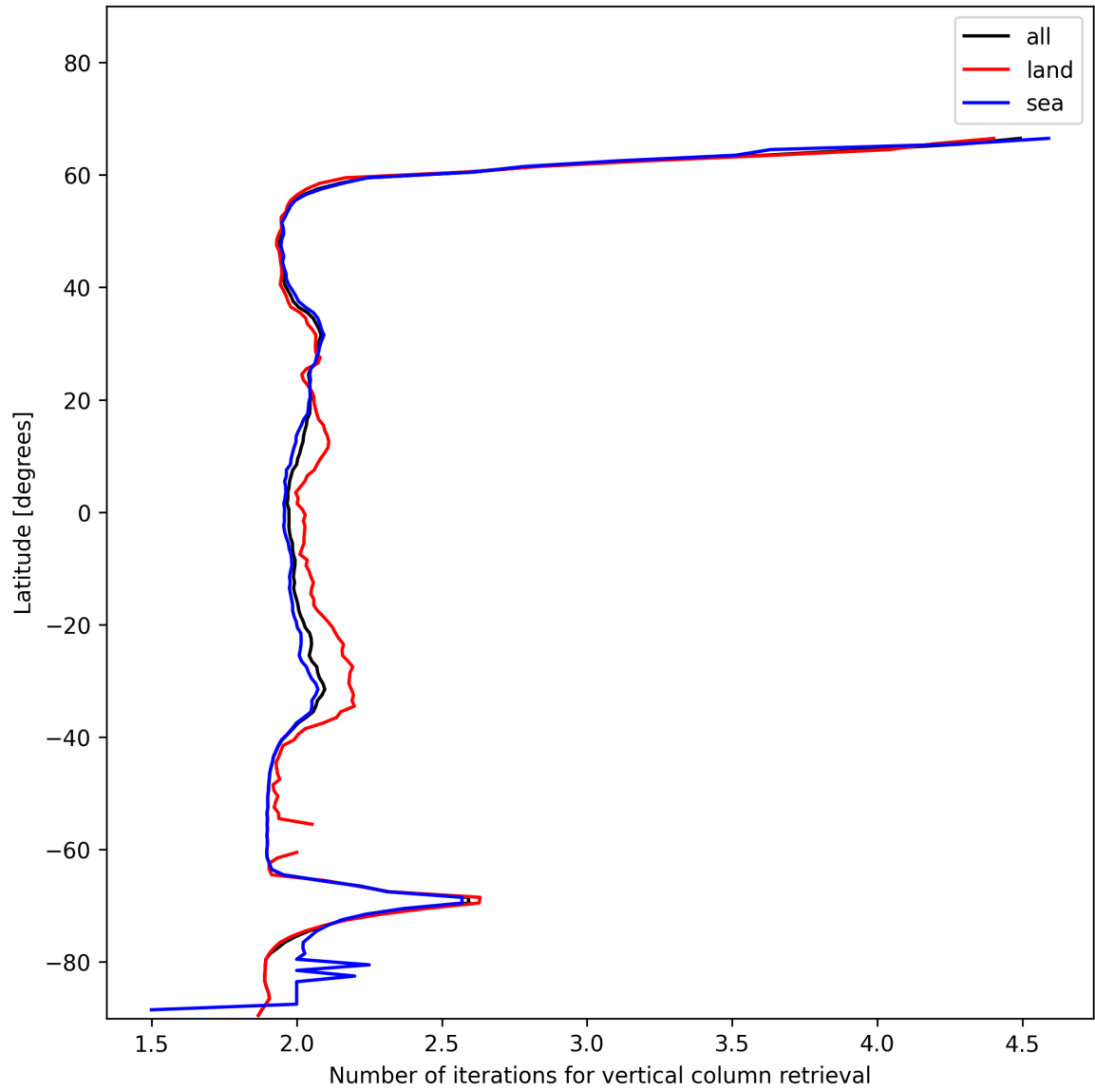
Figure 27: Zonal average of “Number of iterations for vertical column retrieval” for 2025-12-04 to 2025-12-05.
