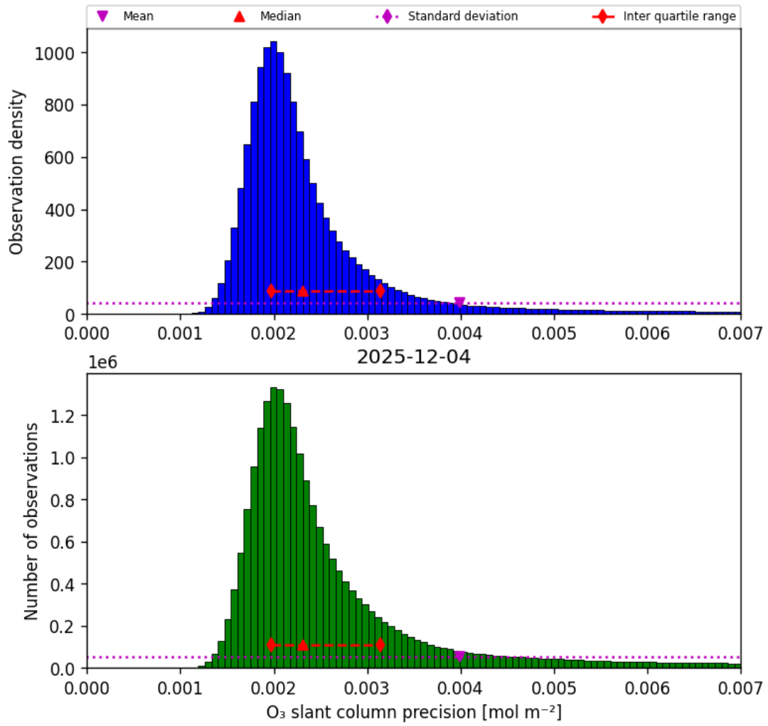
Figure 32: Histogram of “O 3 slant column precision” for 2025-12-04 to 2025-12-05
