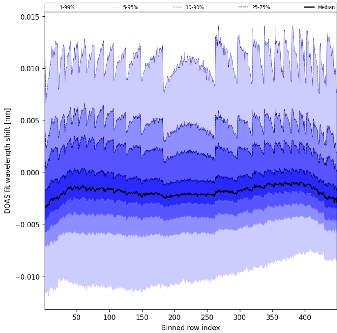
Figure 47: Along track statistics of “DOAS fit wavelength shift” for 2025-12-04 to 2025-12-05
