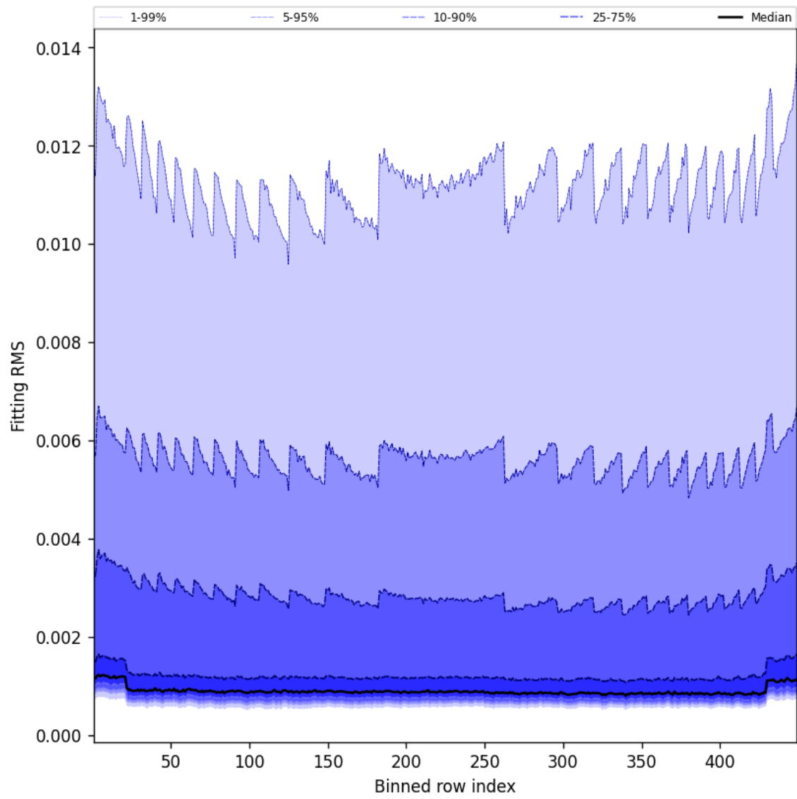
Figure 46: Along track statistics of “Fitting RMS” for 2025-12-04 to 2025-12-05
