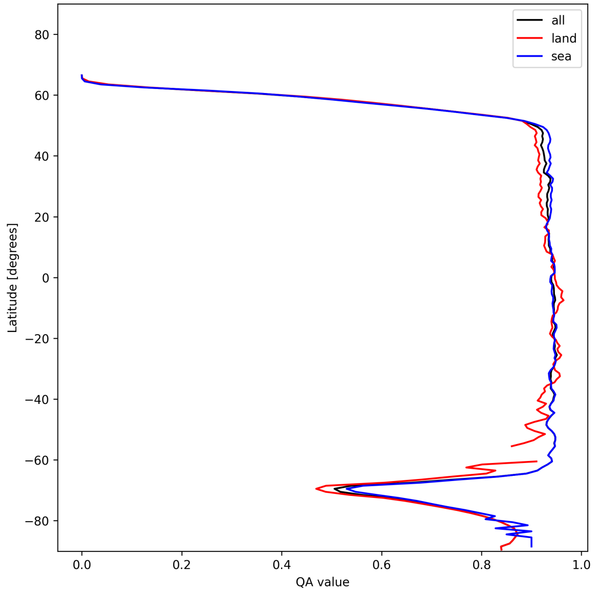
Figure 16: Zonal average of “QA value” for 2025-12-04 to 2025-12-05.
