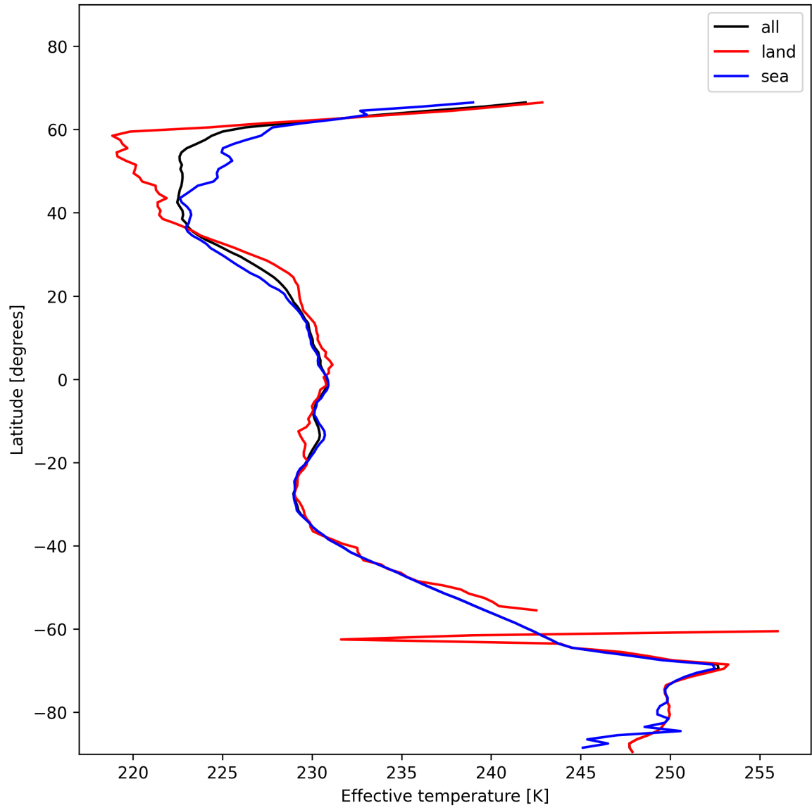
Figure 26: Zonal average of “Effective temperature” for 2025-12-04 to 2025-12-05.
