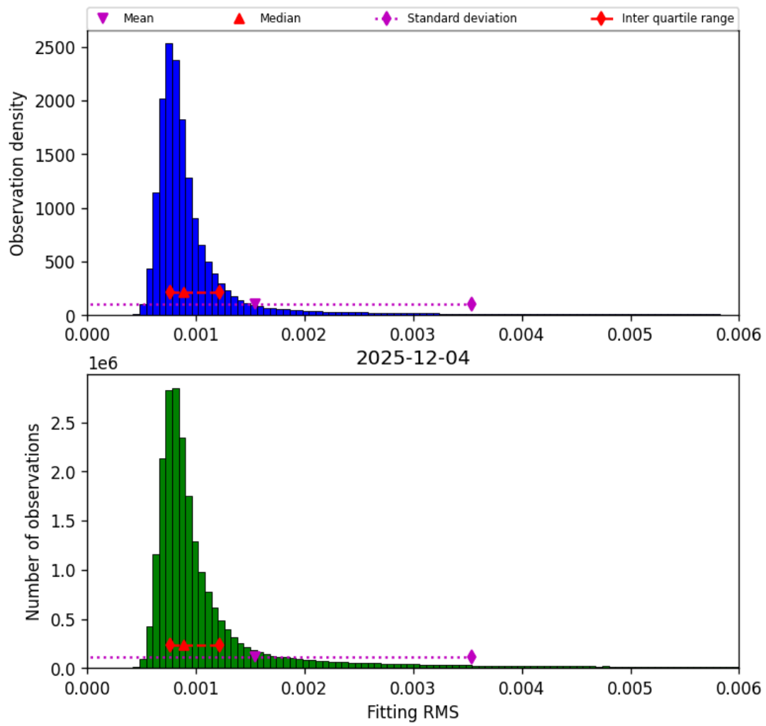
Figure 34: Histogram of “Fitting RMS” for 2025-12-04 to 2025-12-05
