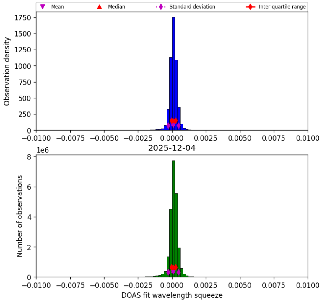
Figure 36: Histogram of “DOAS fit wavelength squeeze” for 2025-12-04 to 2025-12-05
