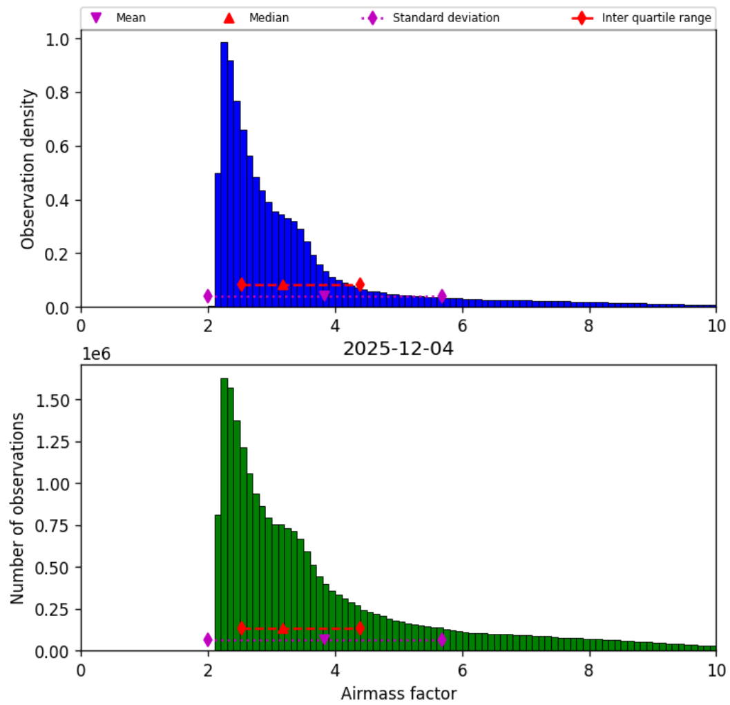
Figure 37: Histogram of “Airmass factor” for 2025-12-04 to 2025-12-05
