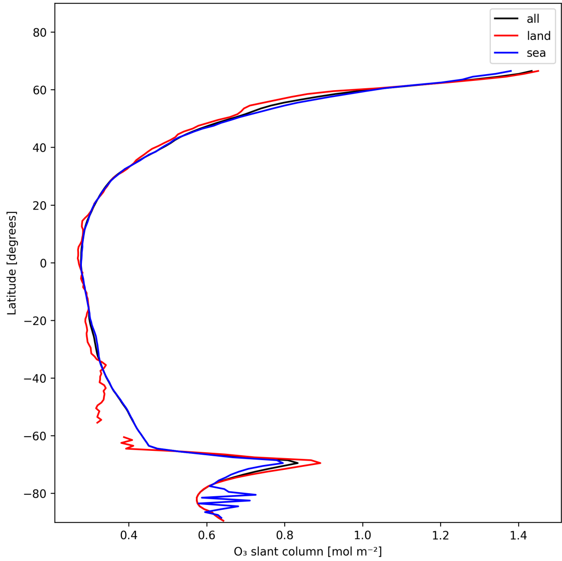
Figure 19: Zonal average of “O 3 slant column” for 2025-12-04 to 2025-12-05.
