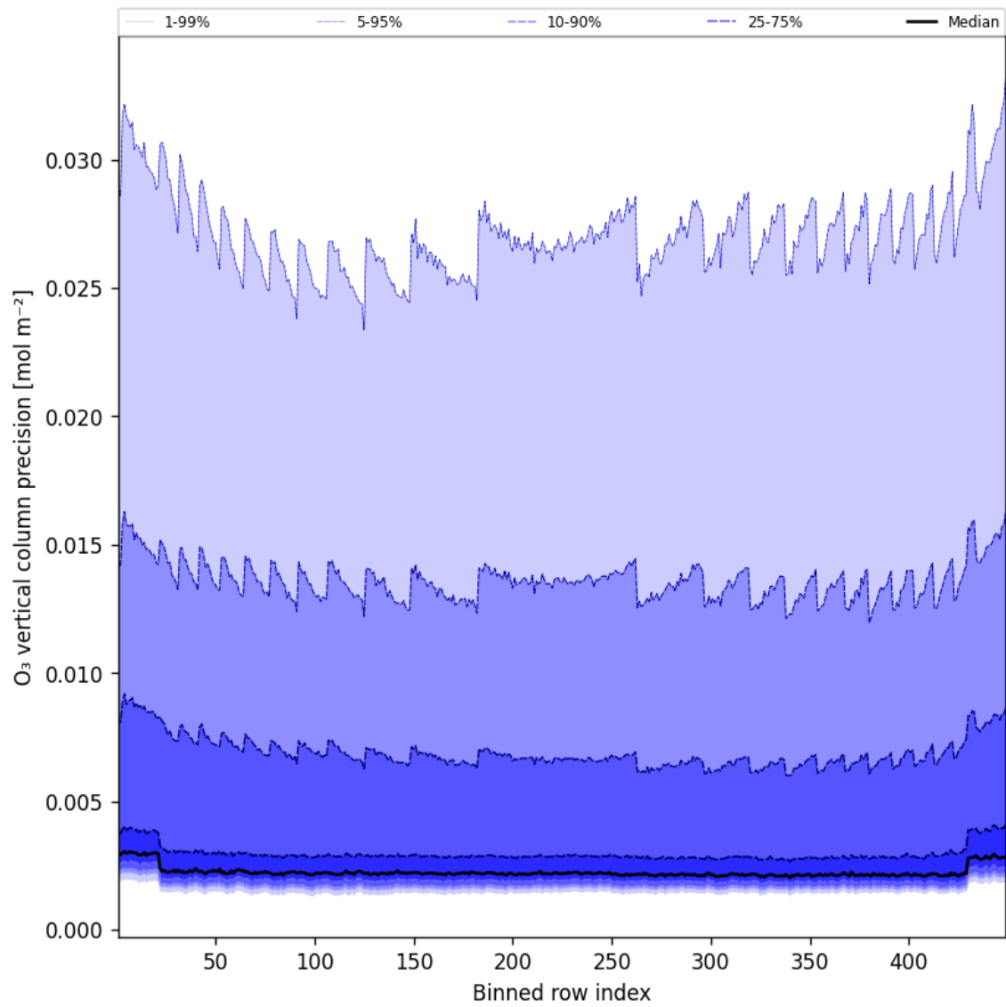
Figure 42: Along track statistics of “O 3 vertical column precision” for 2025-12-04 to 2025-12-05
