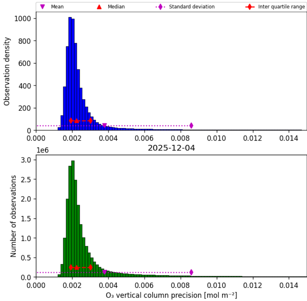
Figure 30: Histogram of “O 3 vertical column precision” for 2025-12-04 to 2025-12-05
