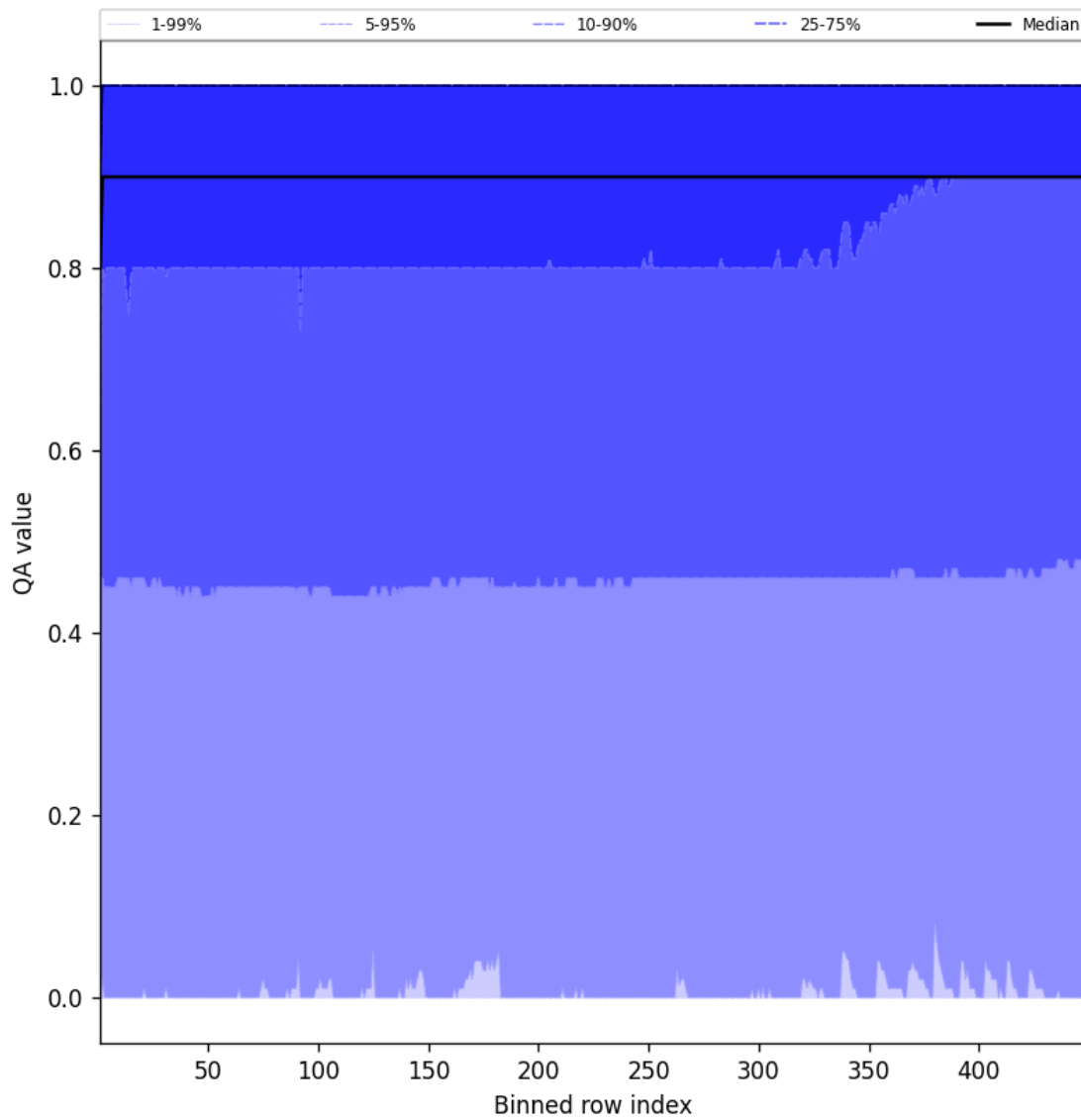
Figure 40: Along track statistics of “QA value” for 2025-12-04 to 2025-12-05
