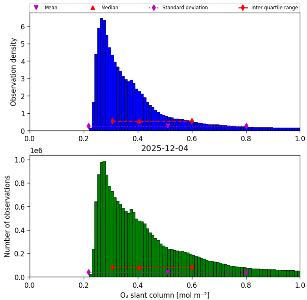
Figure 31: Histogram of “O 3 slant column” for 2025-12-04 to 2025-12-05
