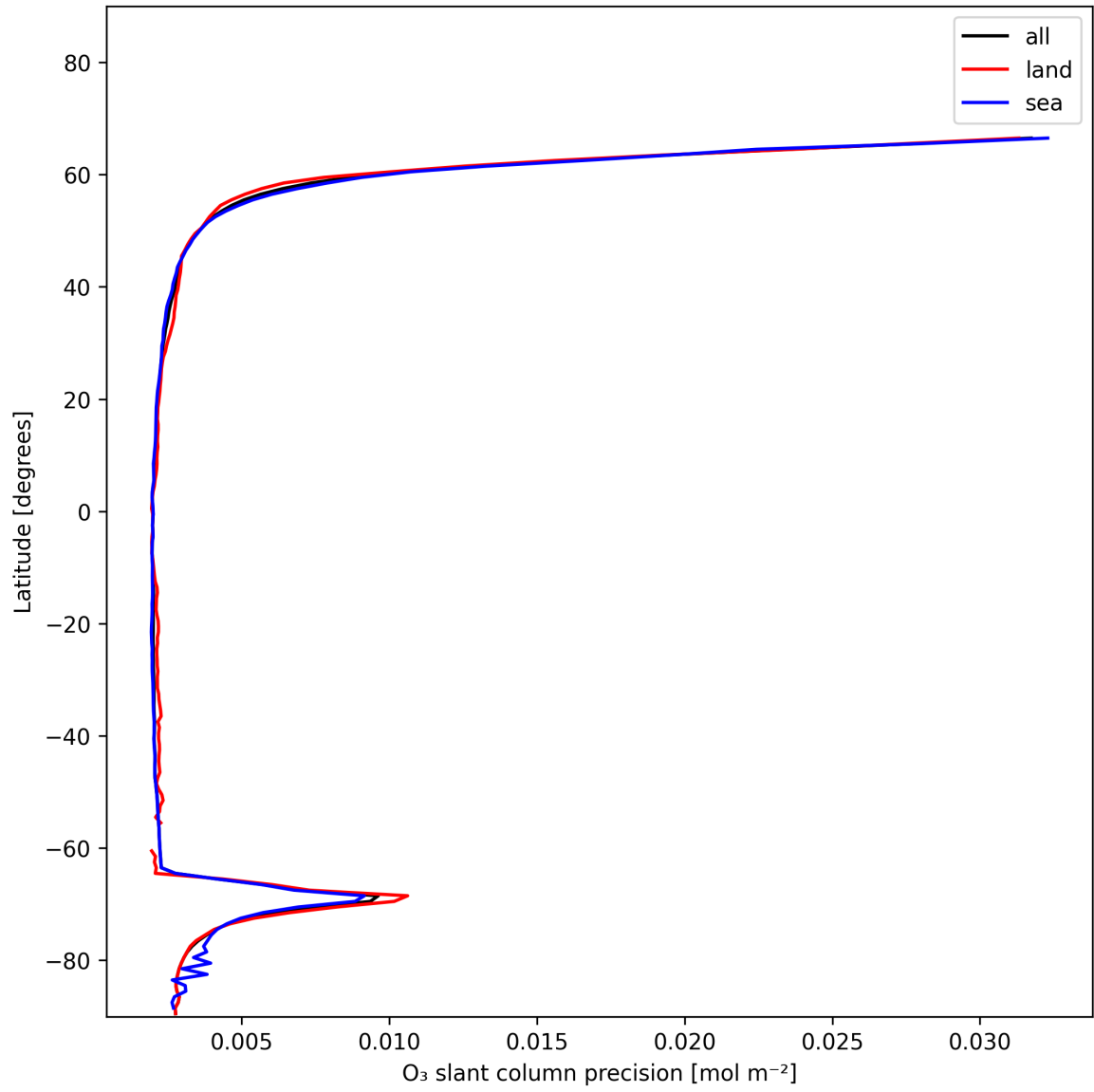
Figure 20: Zonal average of “O 3 slant column precision” for 2025-12-04 to 2025-12-05.
