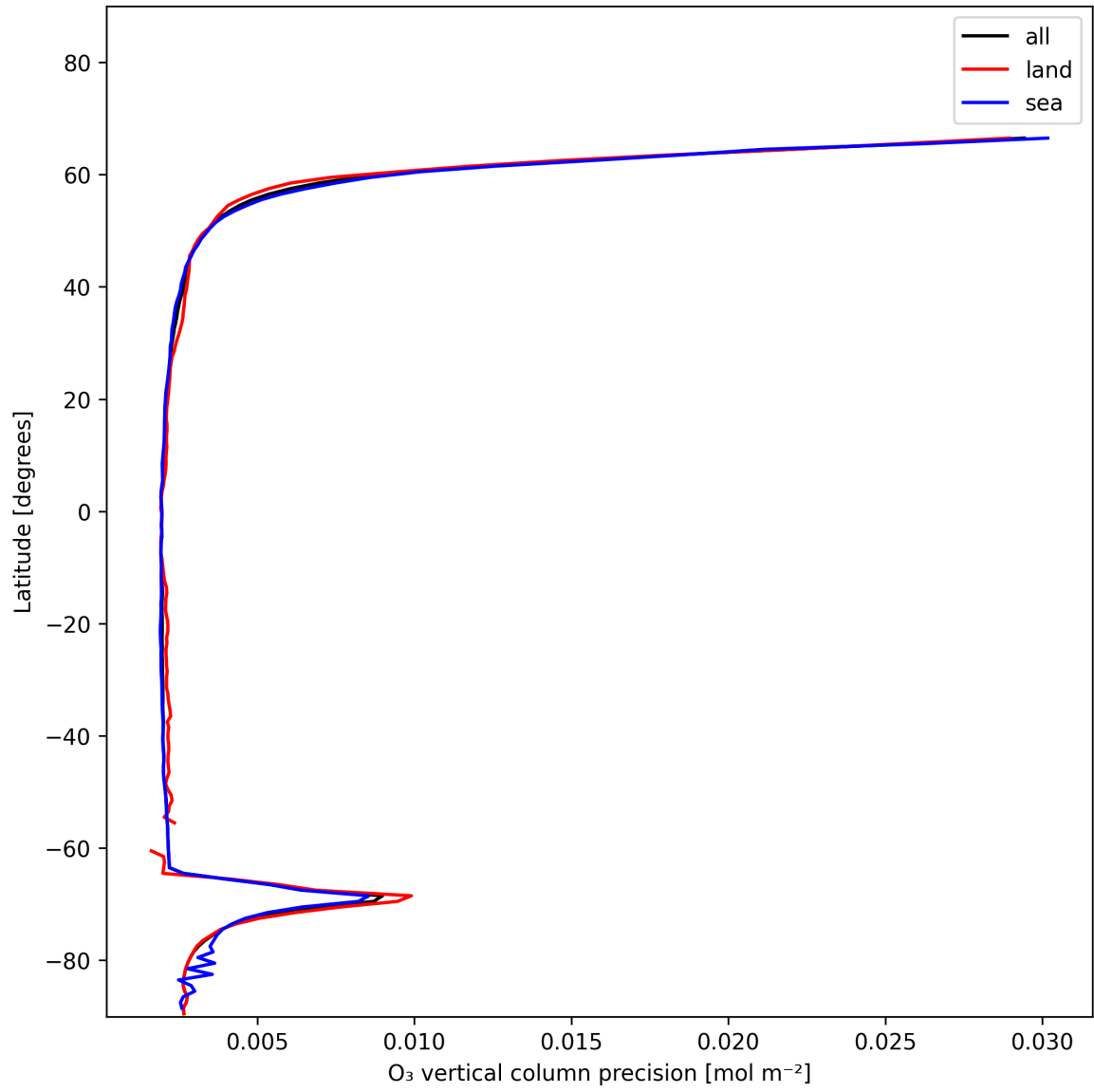
Figure 18: Zonal average of “O 3 vertical column precision” for 2025-12-04 to 2025-12-05.
