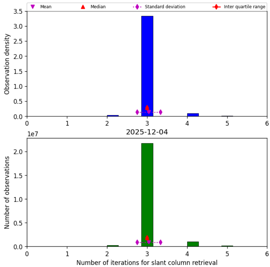
Figure 33: Histogram of “Number of iterations for slant column retrieval” for 2025-12-04 to 2025-12-05
