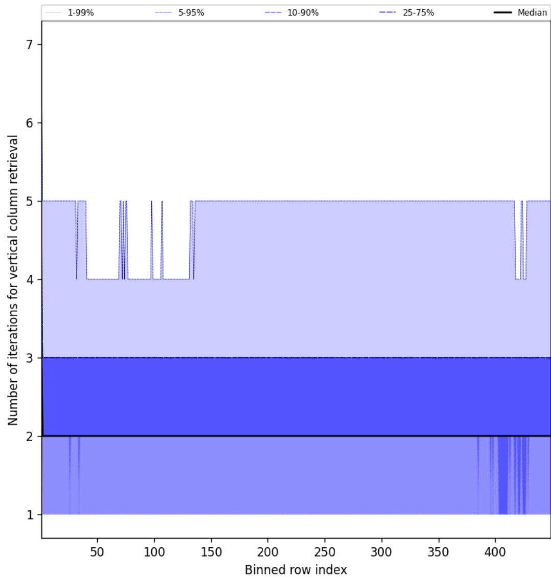
Figure 51: Along track statistics of “Number of iterations for vertical column retrieval” for 2025-12-04 to 2025-12-05
