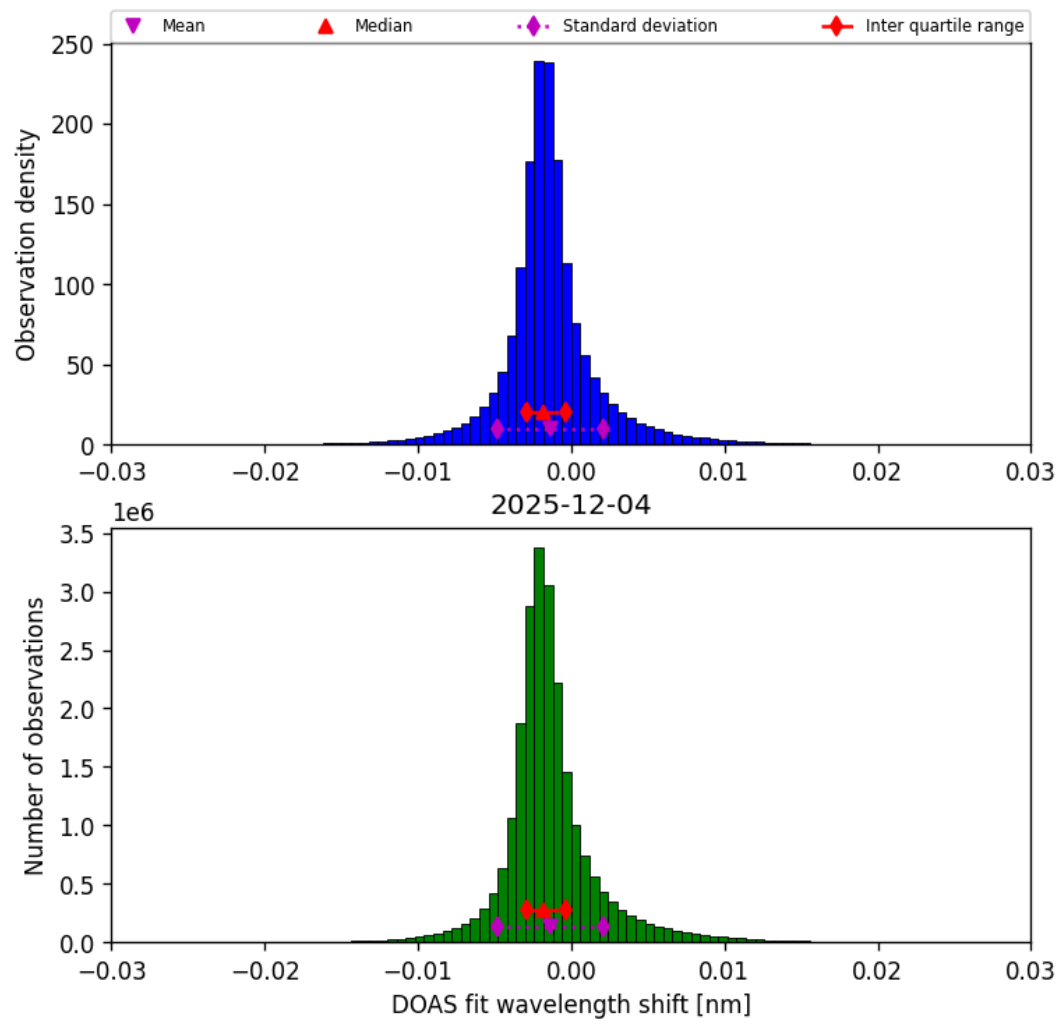
Figure 35: Histogram of “DOAS fit wavelength shift” for 2025-12-04 to 2025-12-05
