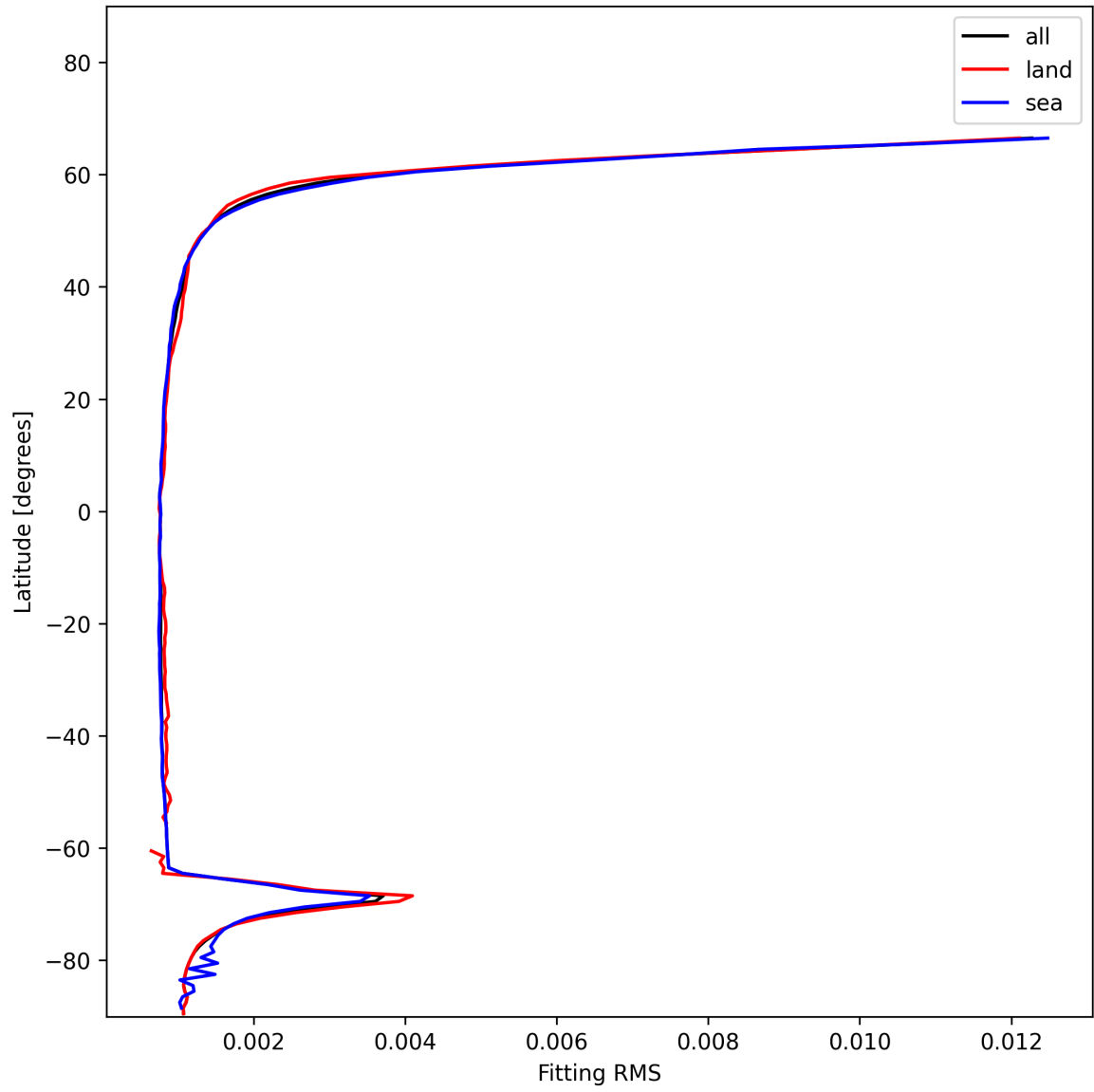
Figure 22: Zonal average of “Fitting RMS” for 2025-12-04 to 2025-12-05.
