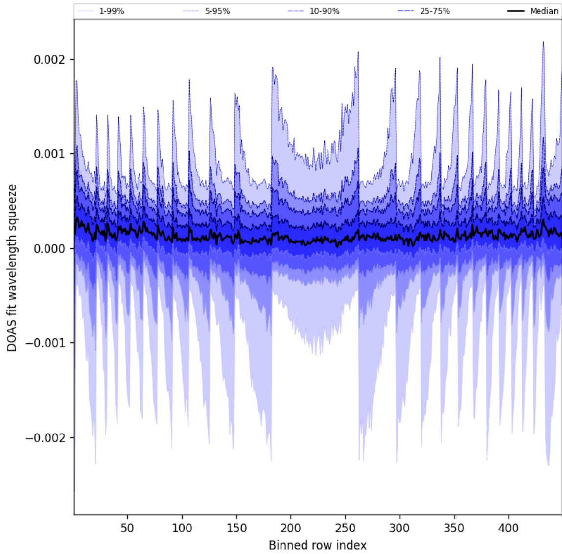
Figure 48: Along track statistics of “DOAS fit wavelength squeeze” for 2025-12-04 to 2025-12-05
