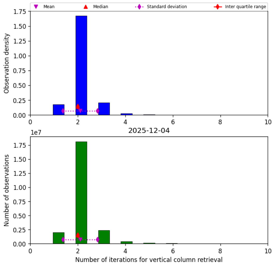
Figure 39: Histogram of “Number of iterations for vertical column retrieval” for 2025-12-04 to 2025-12-05
