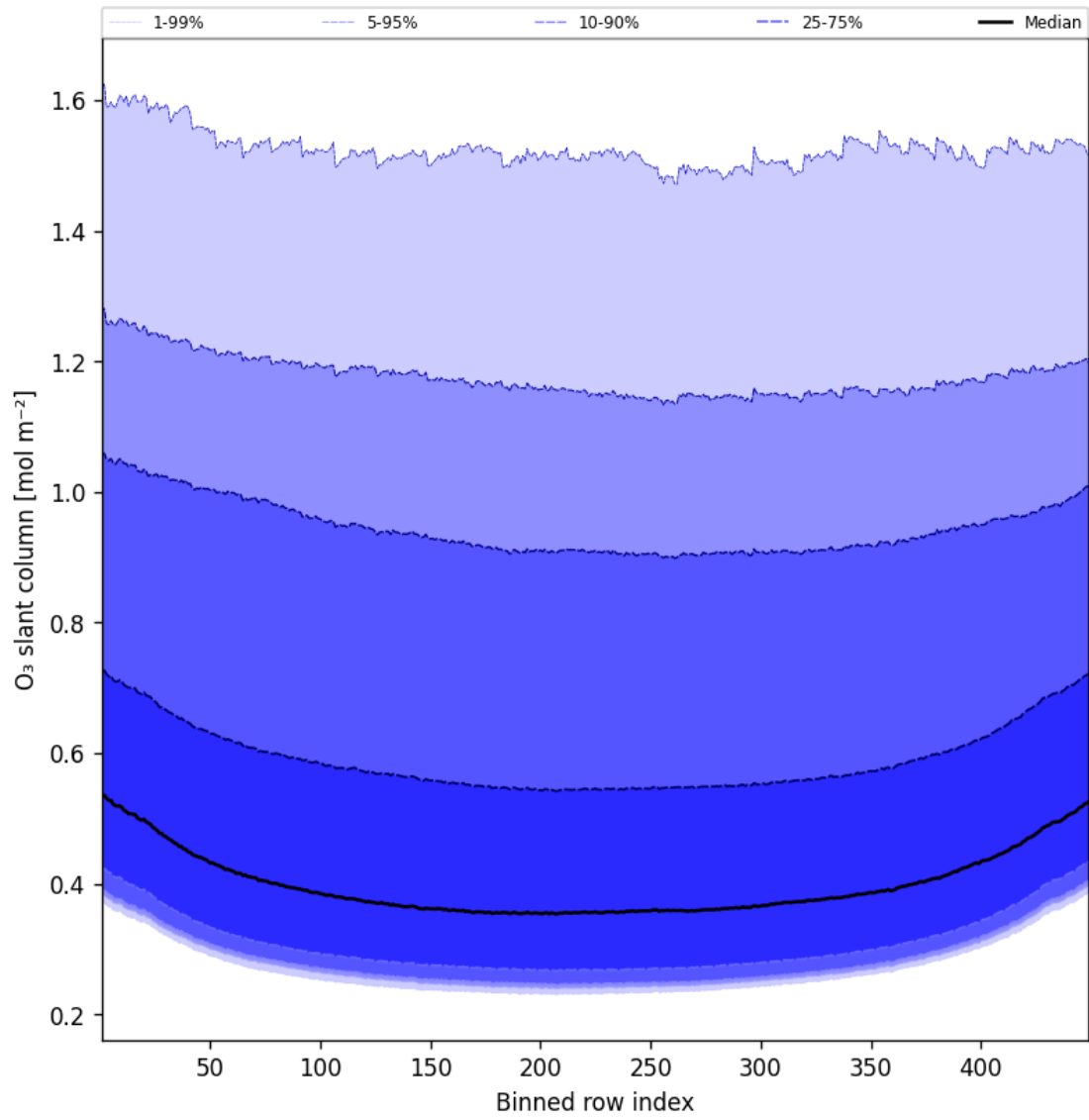
Figure 43: Along track statistics of “O 3 slant column” for 2025-12-04 to 2025-12-05
