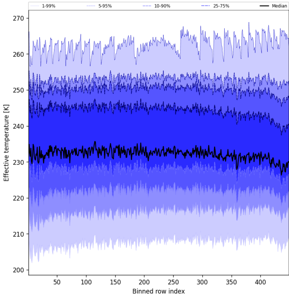
Figure 50: Along track statistics of “Effective temperature” for 2025-12-04 to 2025-12-05
