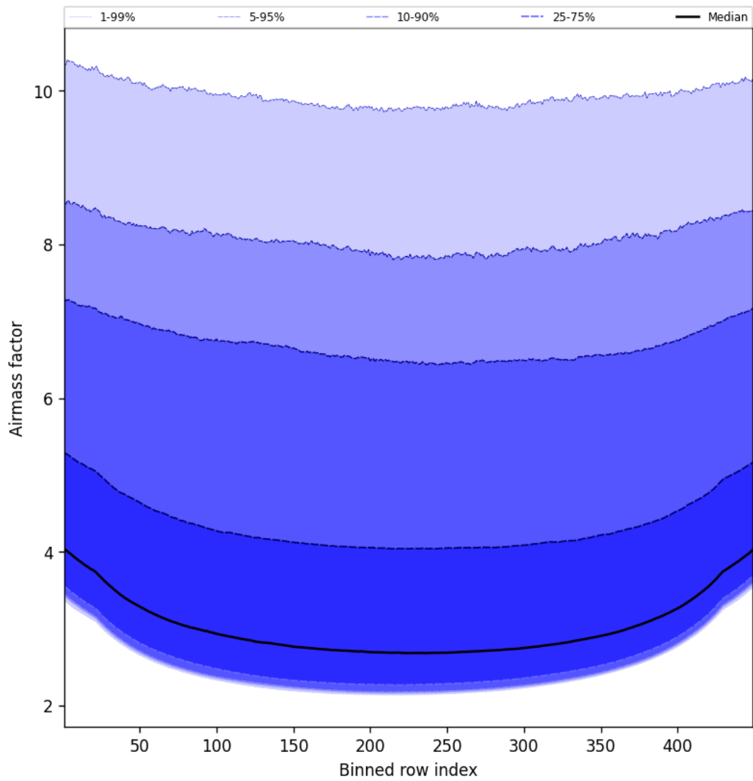
Figure 49: Along track statistics of “Airmass factor” for 2025-12-04 to 2025-12-05
