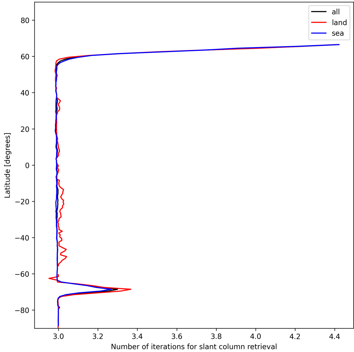
Figure 21: Zonal average of “Number of iterations for slant column retrieval” for 2025-12-04 to 2025-12-05.
