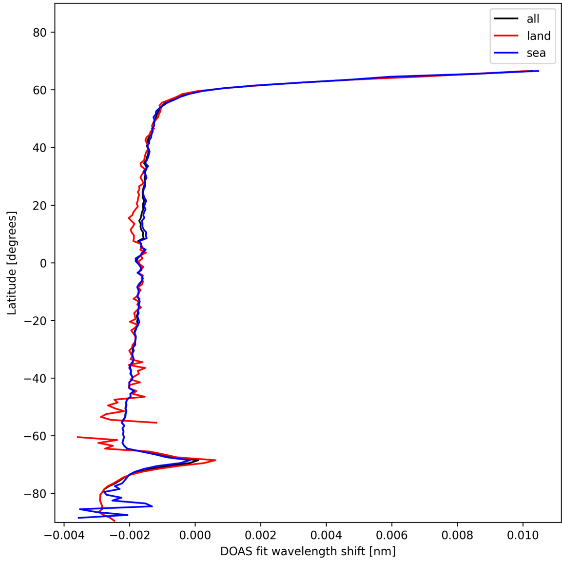
Figure 23: Zonal average of “DOAS fit wavelength shift” for 2025-12-04 to 2025-12-05.
