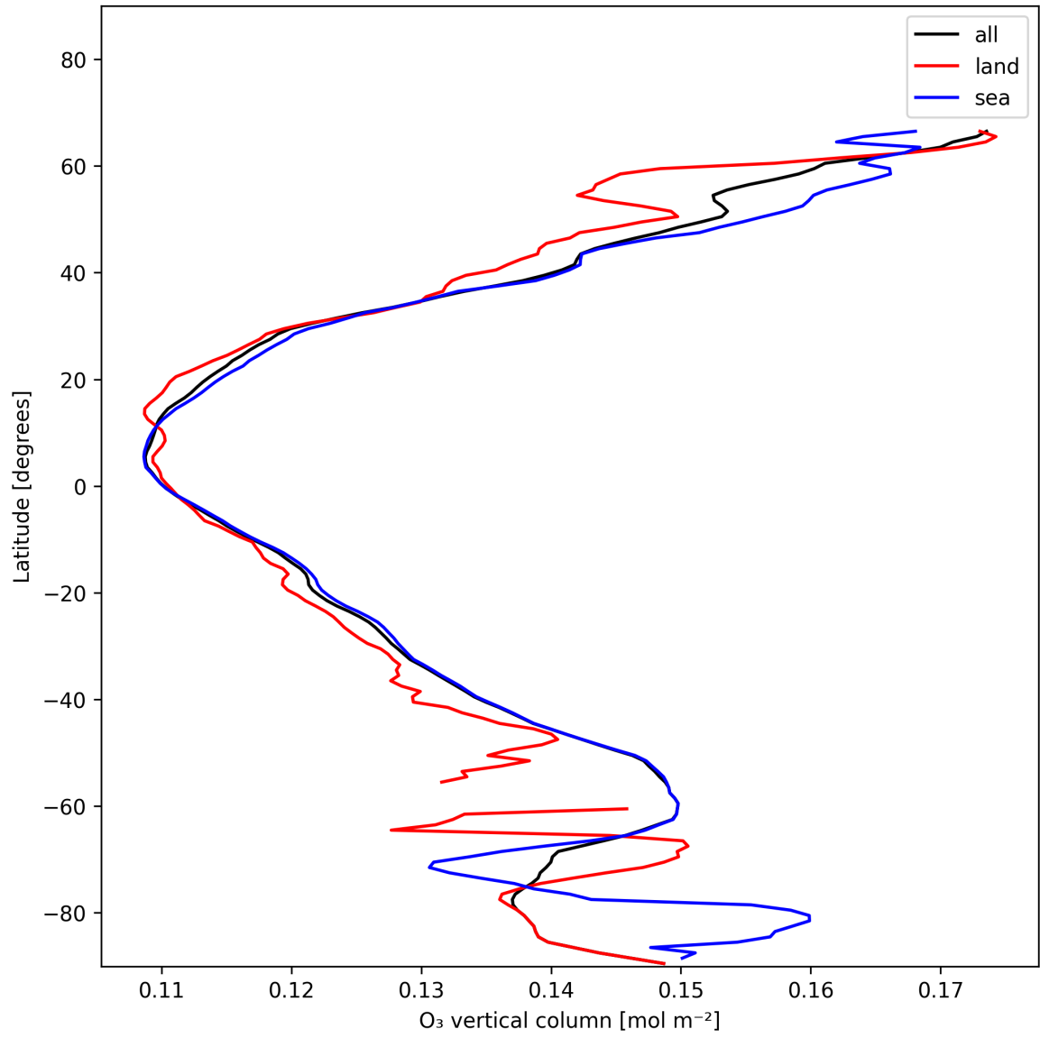
Figure 17: Zonal average of “O 3 vertical column” for 2025-12-04 to 2025-12-05.
