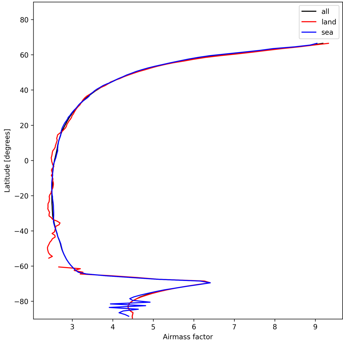
Figure 25: Zonal average of “Airmass factor” for 2025-12-04 to 2025-12-05.
