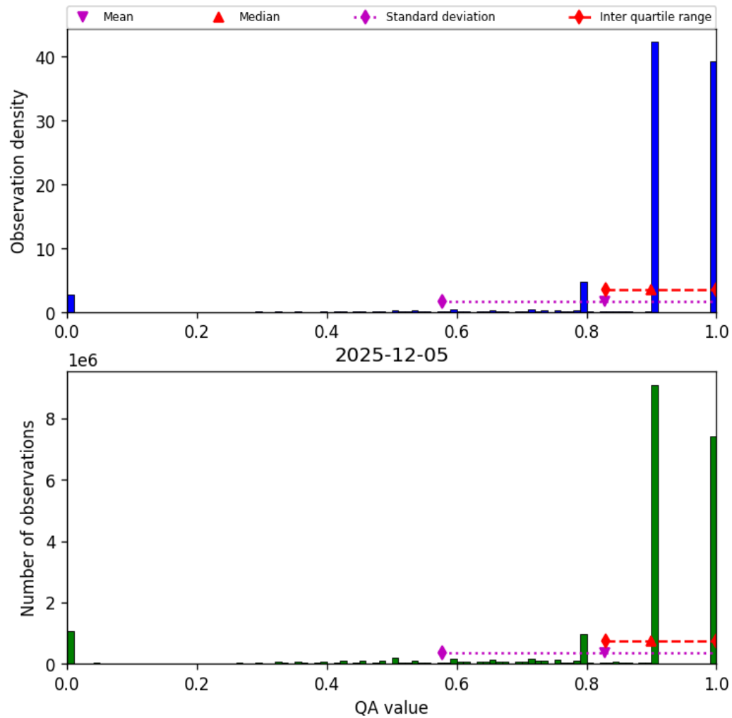
Figure 28: Histogram of “QA value” for 2025-12-05 to 2025-12-06
