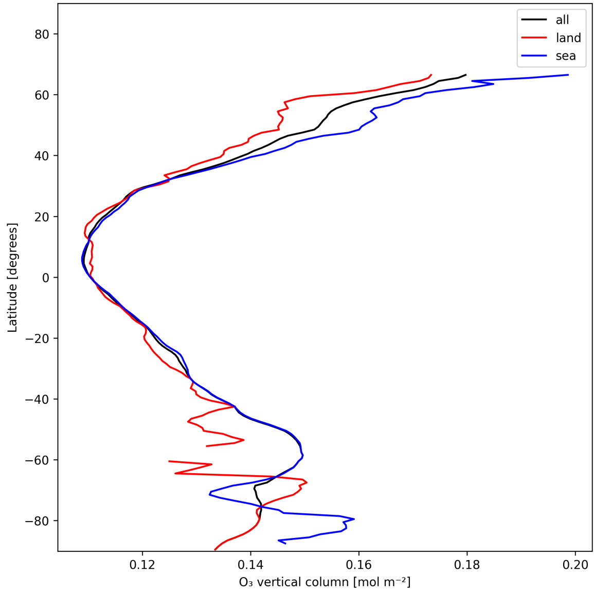
Figure 17: Zonal average of “O 3 vertical column” for 2025-12-05 to 2025-12-06.
