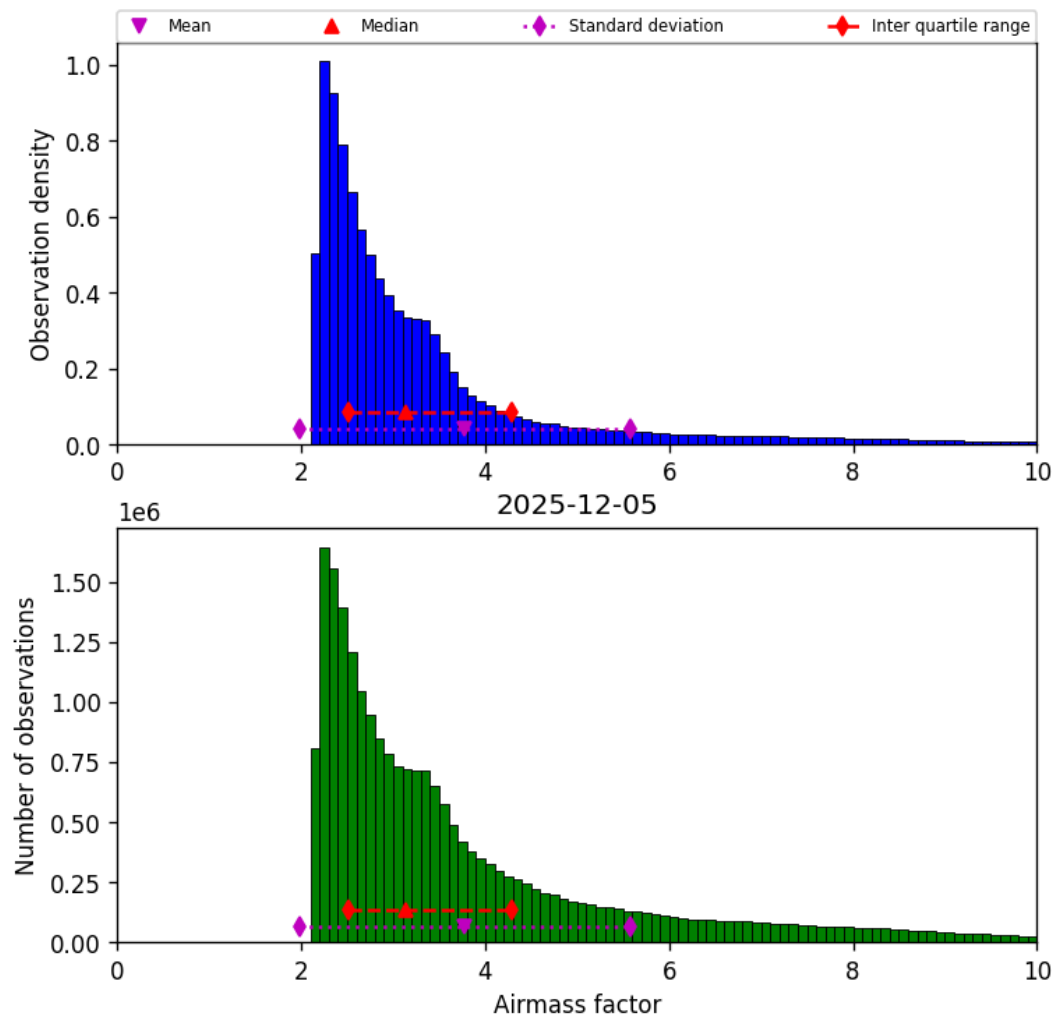
Figure 37: Histogram of “Airmass factor” for 2025-12-05 to 2025-12-06
