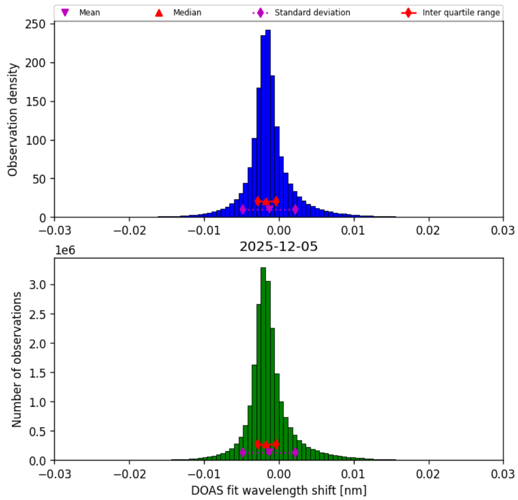
Figure 35: Histogram of “DOAS fit wavelength shift” for 2025-12-05 to 2025-12-06
