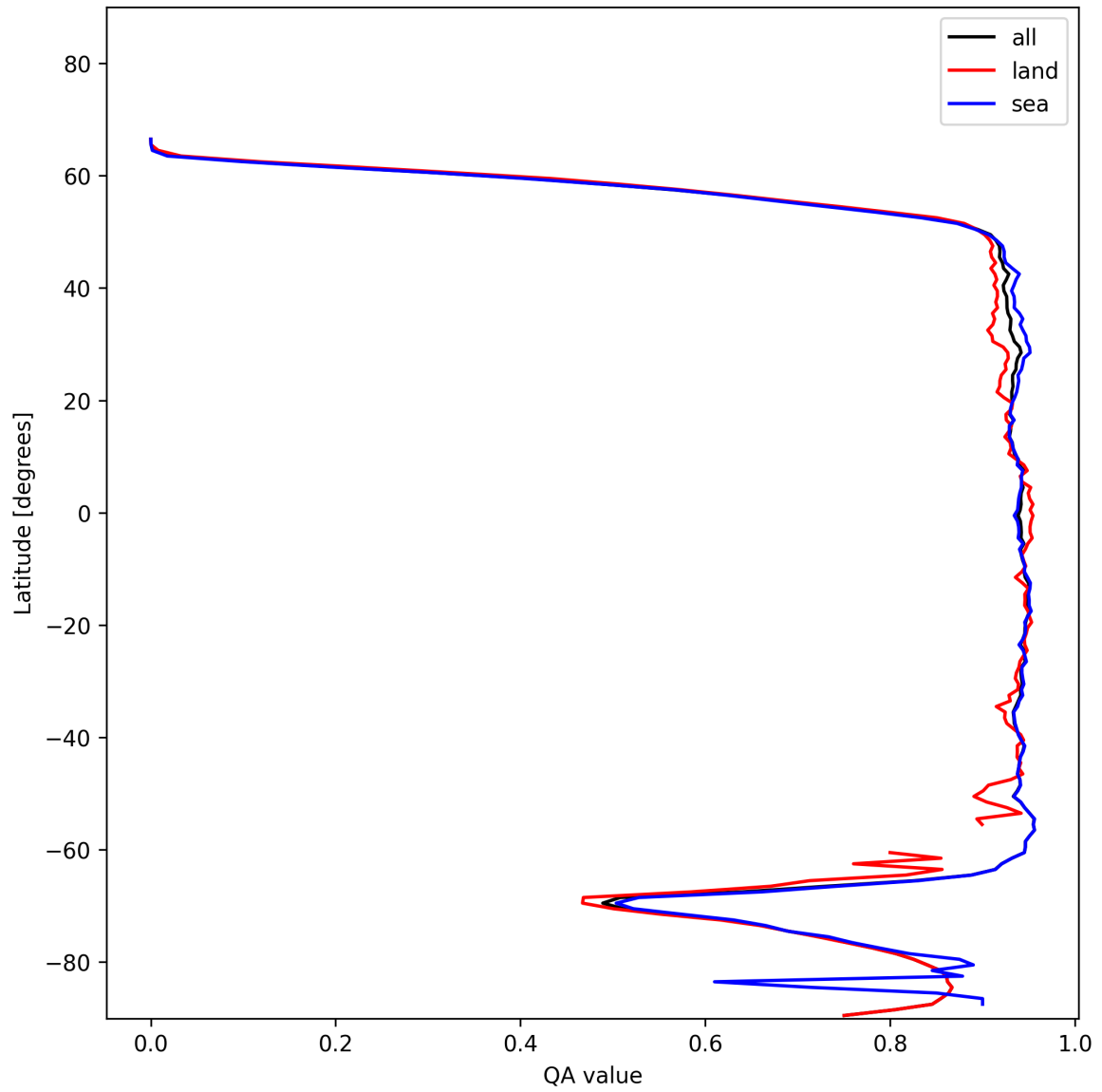
Figure 16: Zonal average of “QA value” for 2025-12-05 to 2025-12-06.
