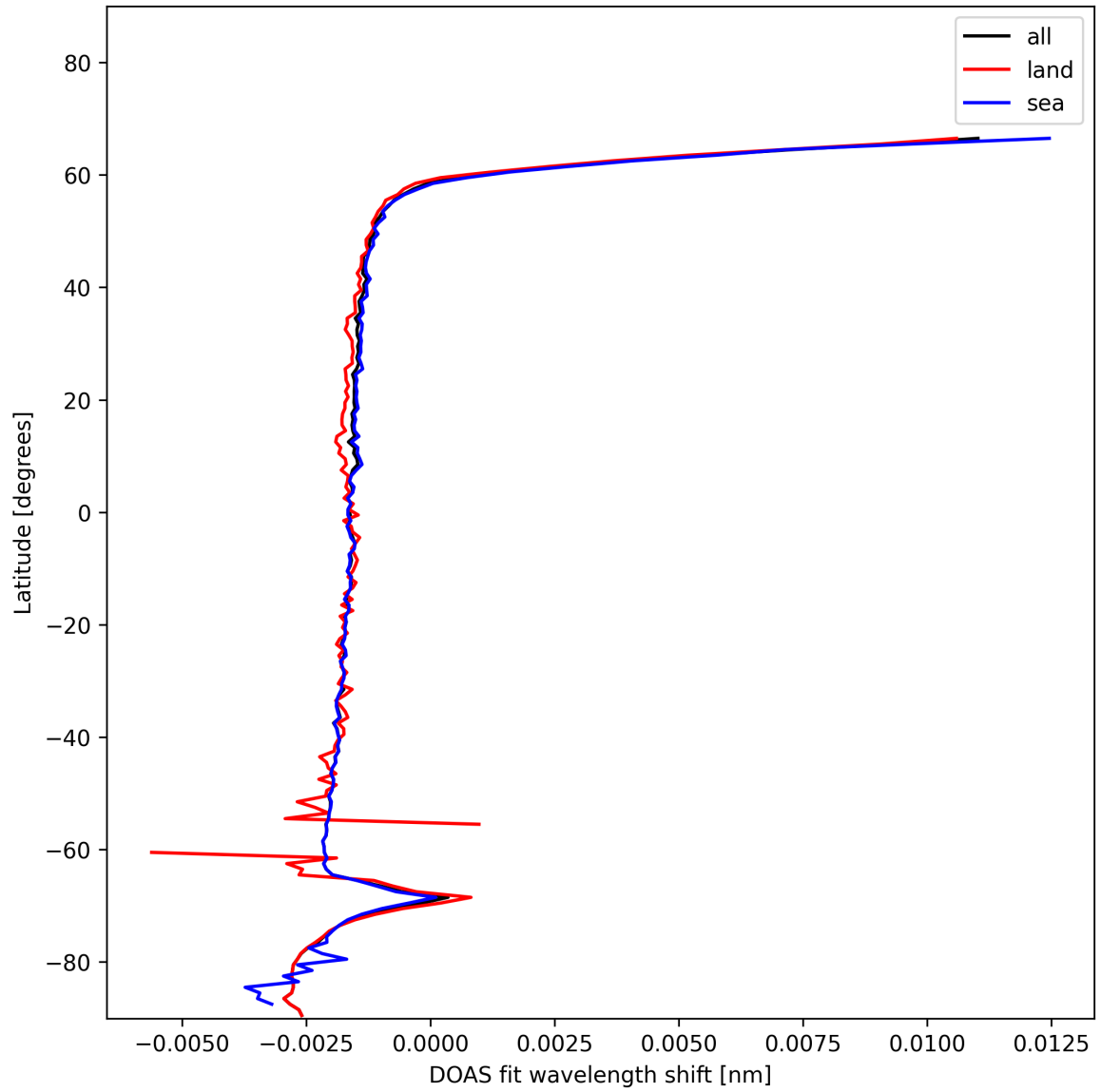
Figure 23: Zonal average of “DOAS fit wavelength shift” for 2025-12-05 to 2025-12-06.
