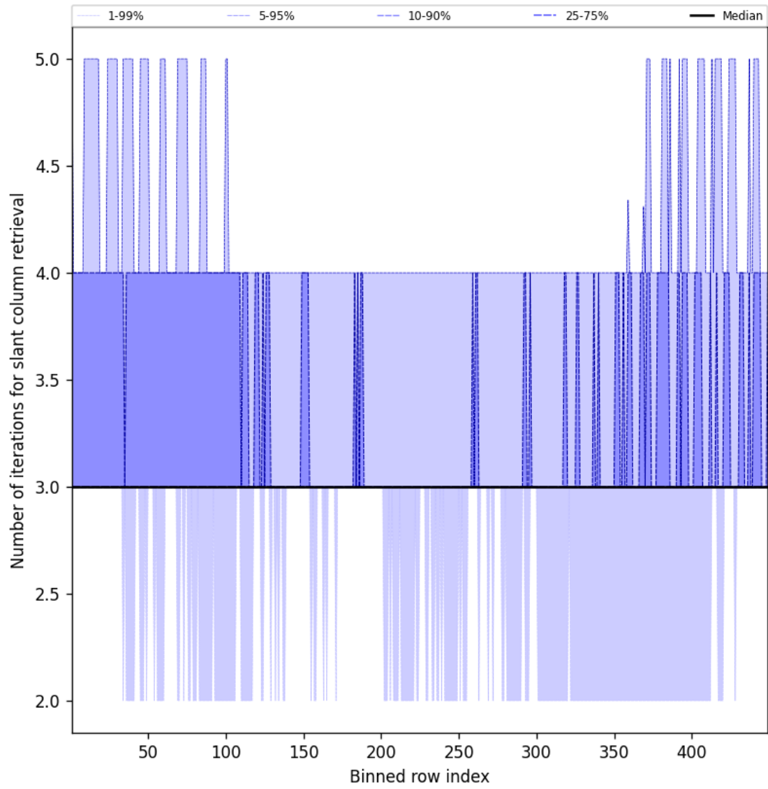
Figure 45: Along track statistics of “Number of iterations for slant column retrieval” for 2025-12-05 to 2025-12-06
