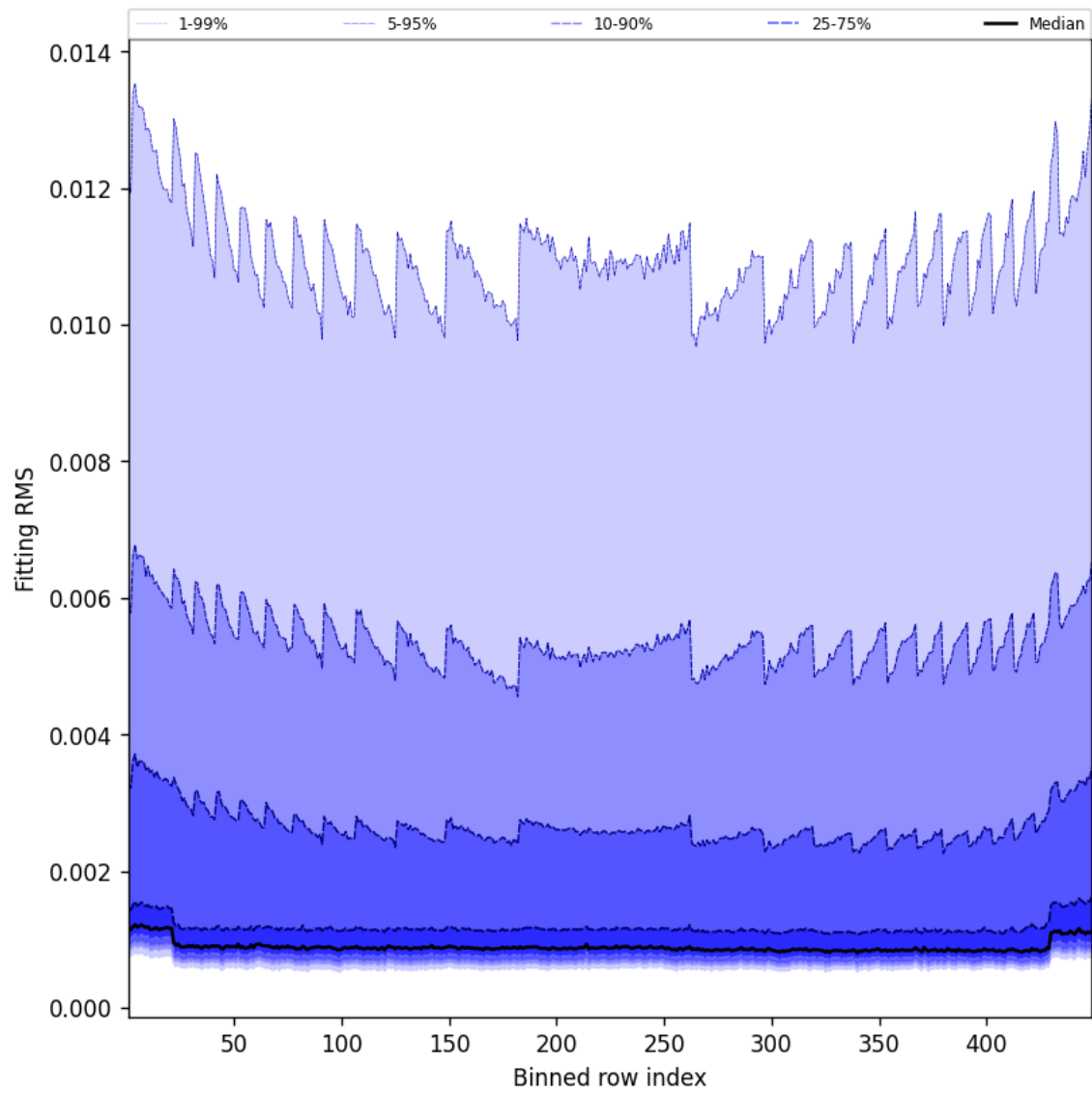
Figure 46: Along track statistics of “Fitting RMS” for 2025-12-05 to 2025-12-06
