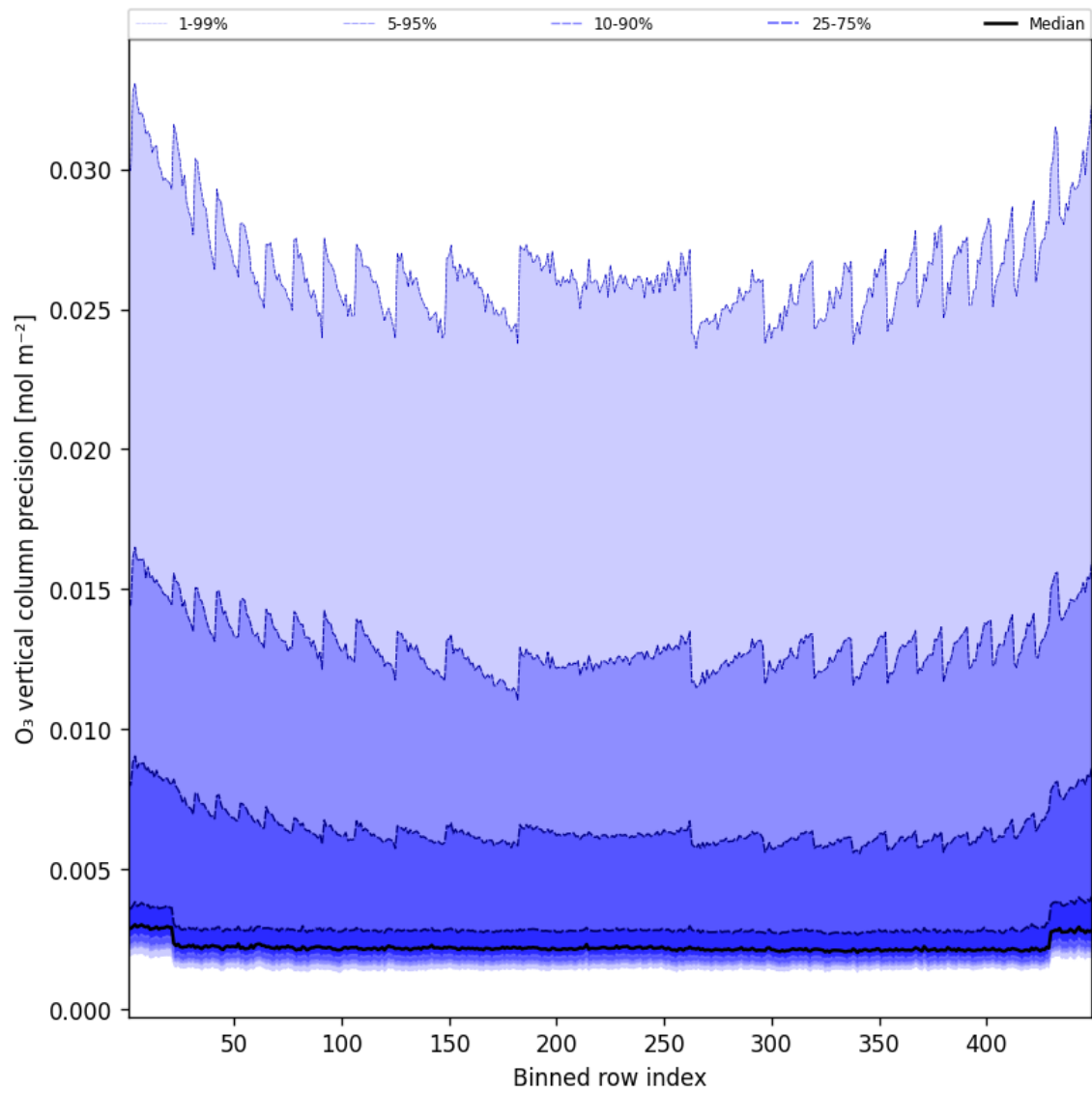
Figure 42: Along track statistics of “O 3 vertical column precision” for 2025-12-05 to 2025-12-06
