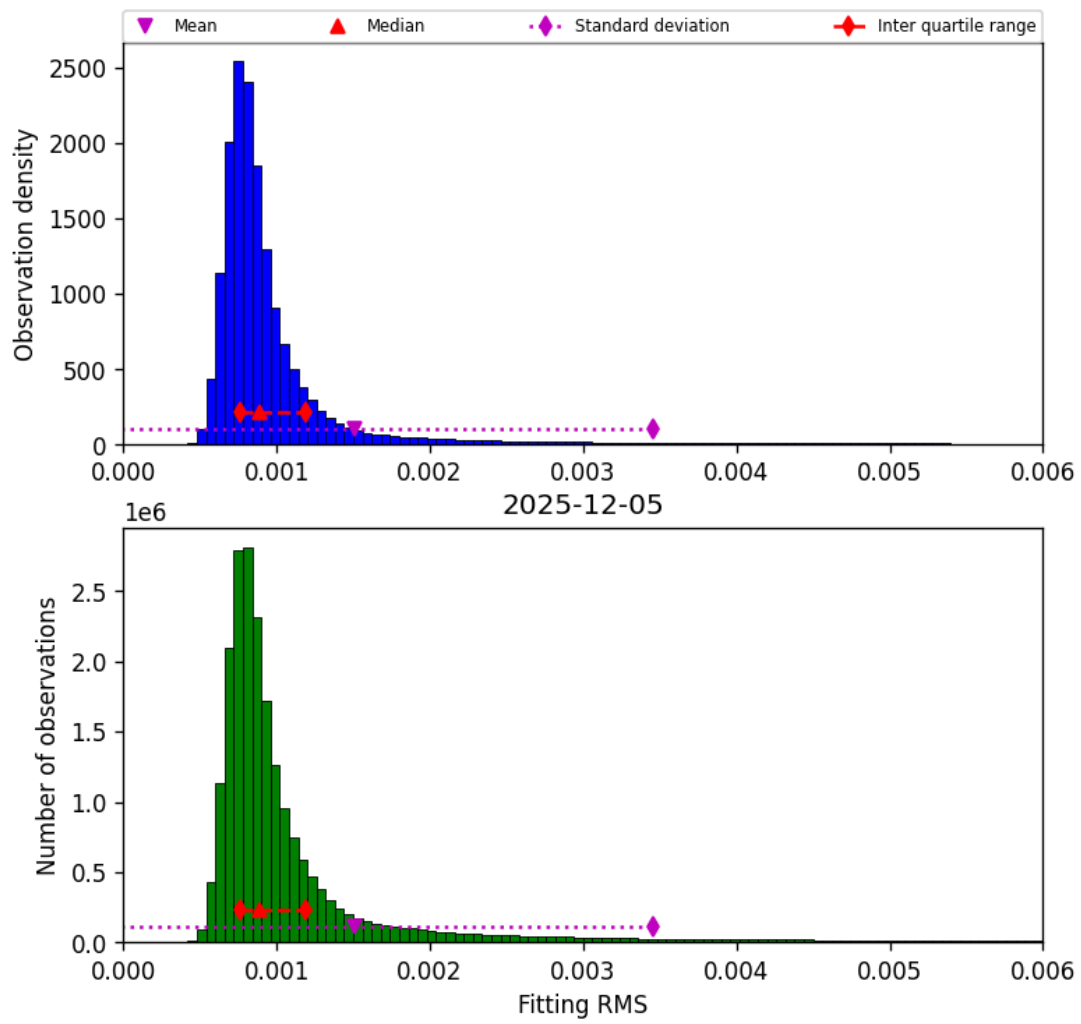
Figure 34: Histogram of “Fitting RMS” for 2025-12-05 to 2025-12-06
