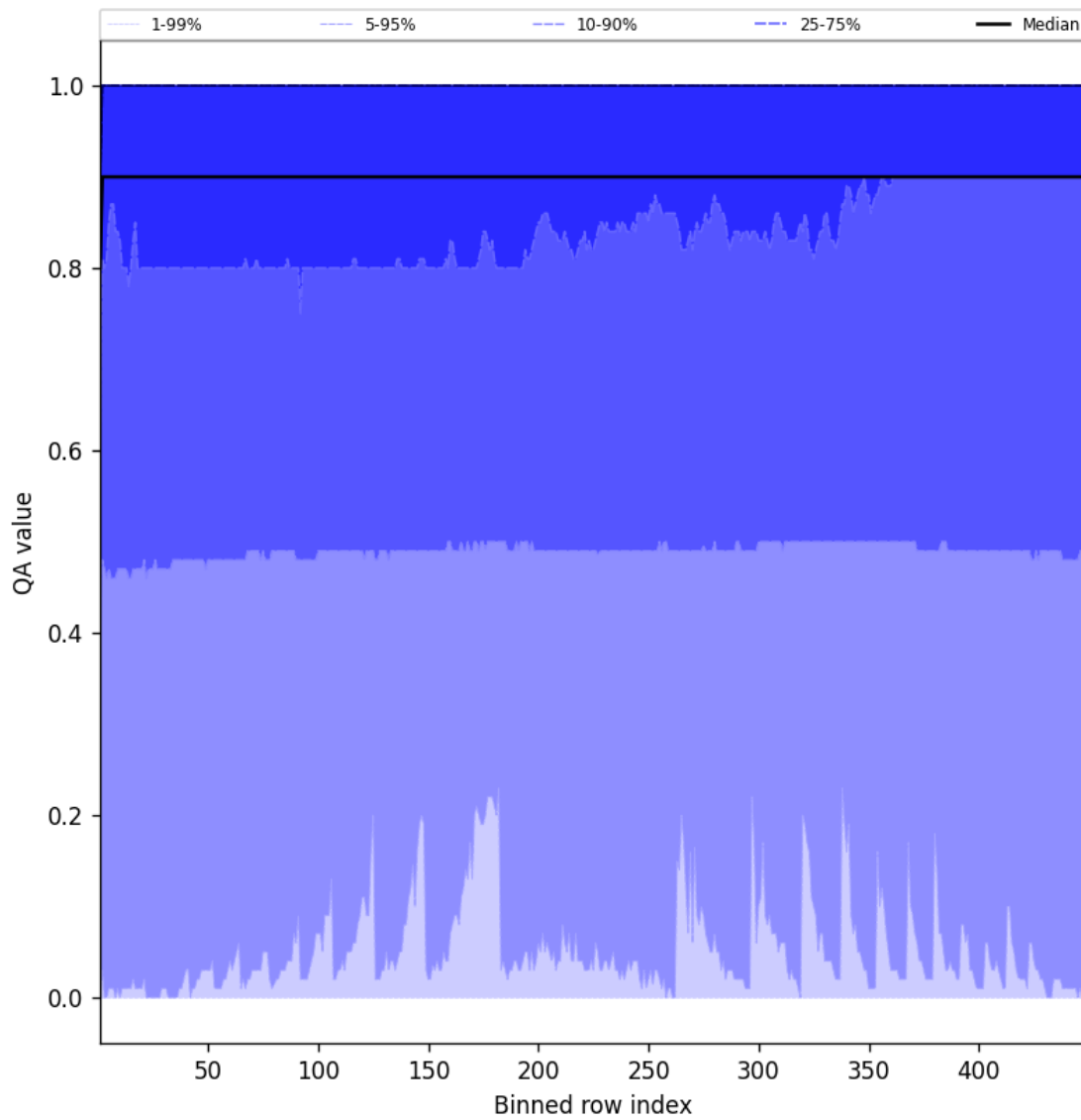
Figure 40: Along track statistics of “QA value” for 2025-12-05 to 2025-12-06
