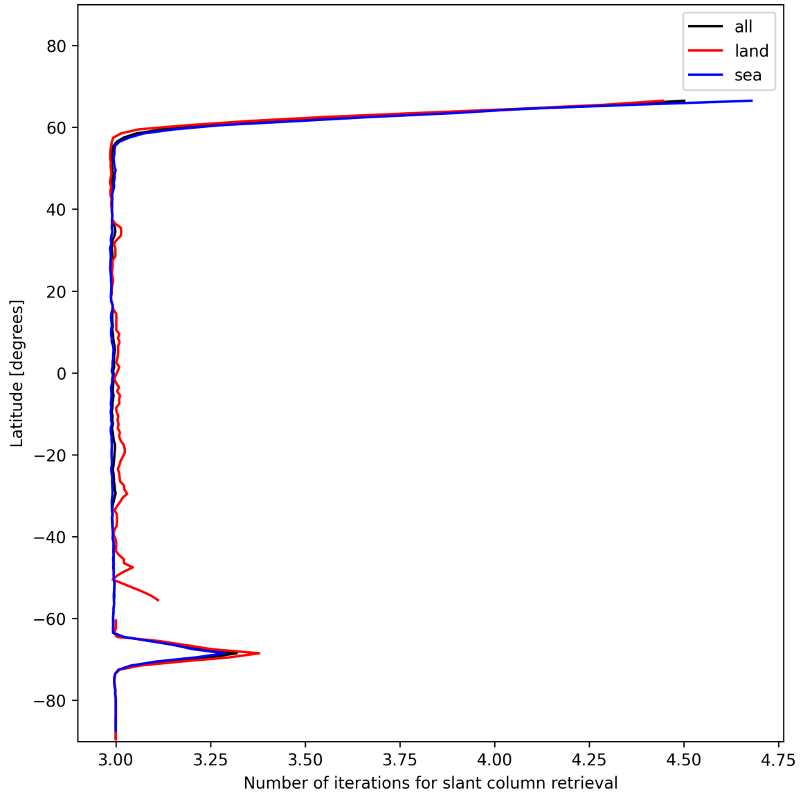
Figure 21: Zonal average of “Number of iterations for slant column retrieval” for 2025-12-05 to 2025-12-06.
