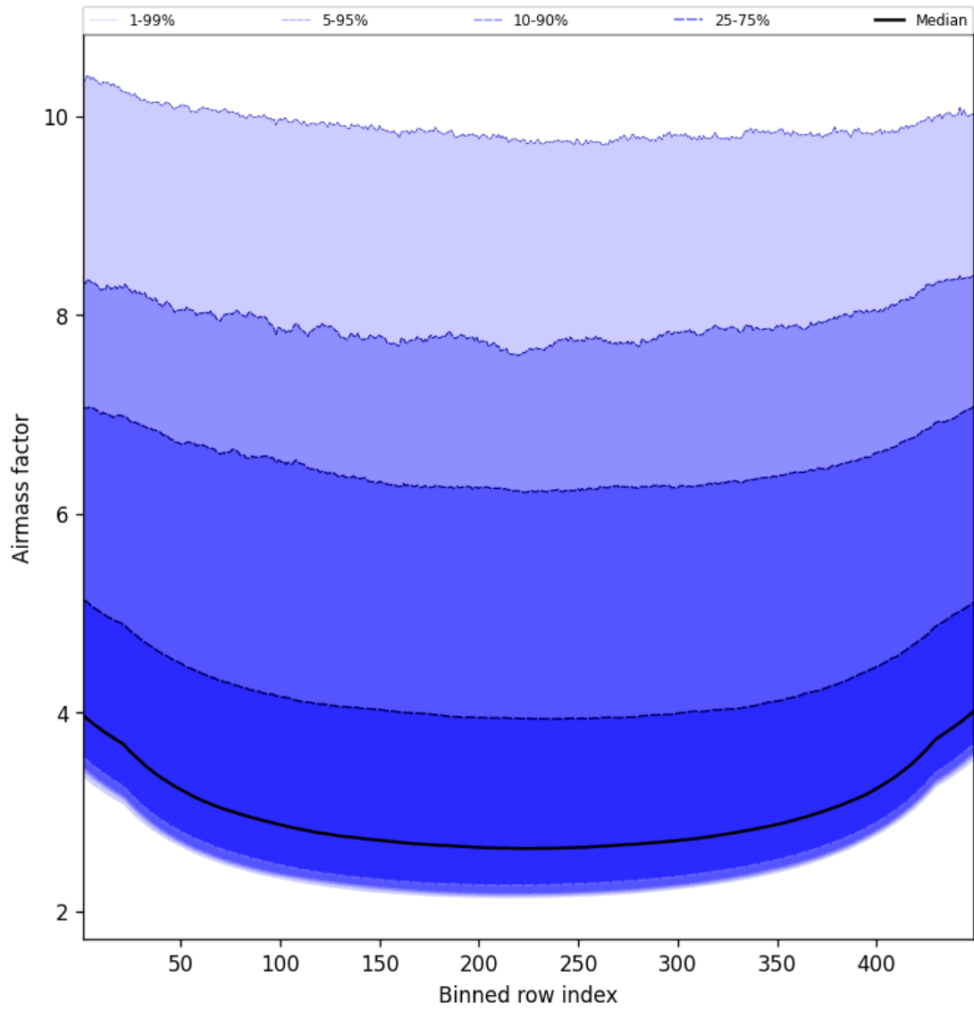
Figure 49: Along track statistics of “Airmass factor” for 2025-12-05 to 2025-12-06
