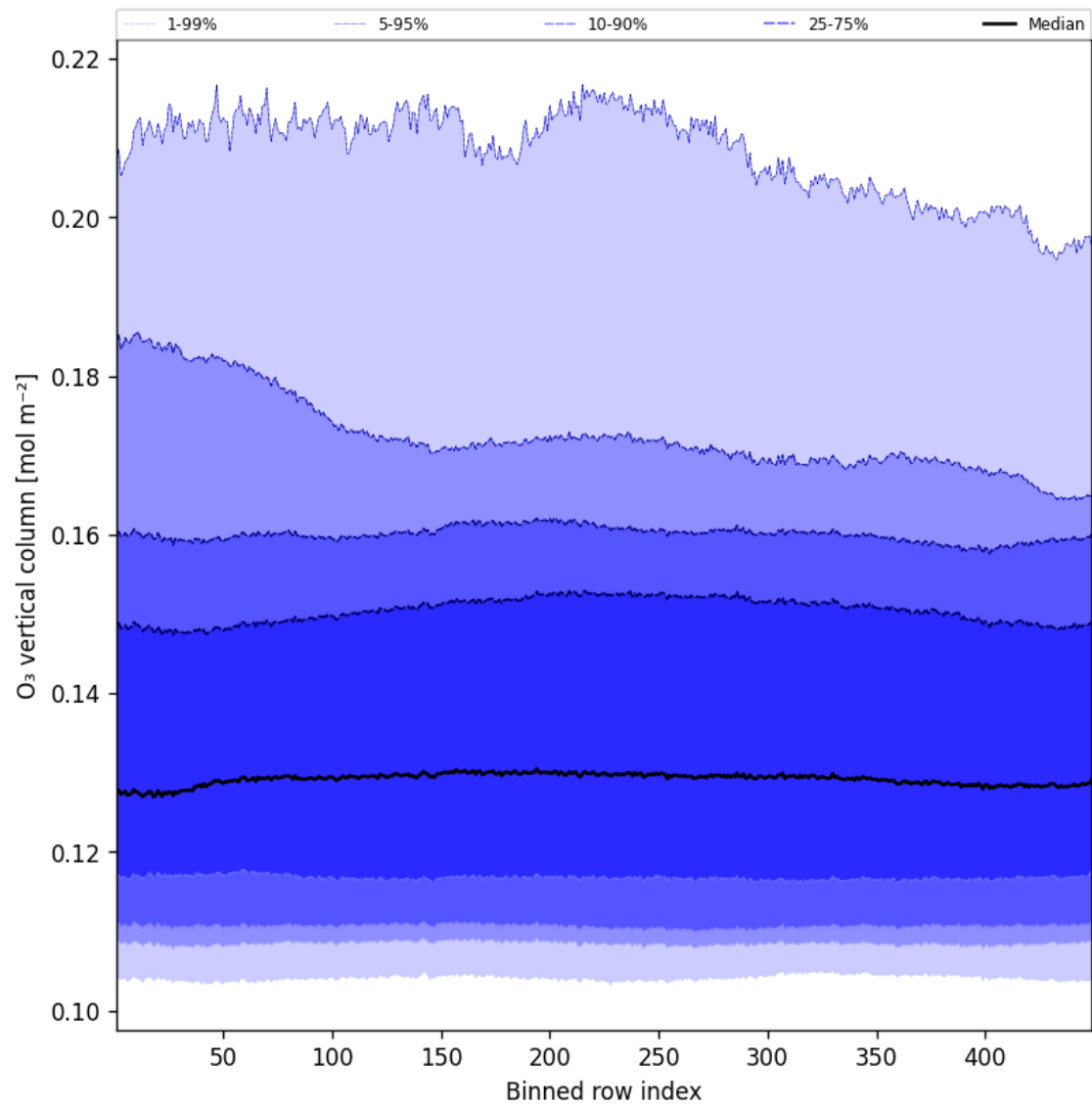
Figure 41: Along track statistics of “O 3 vertical column” for 2025-12-05 to 2025-12-06
