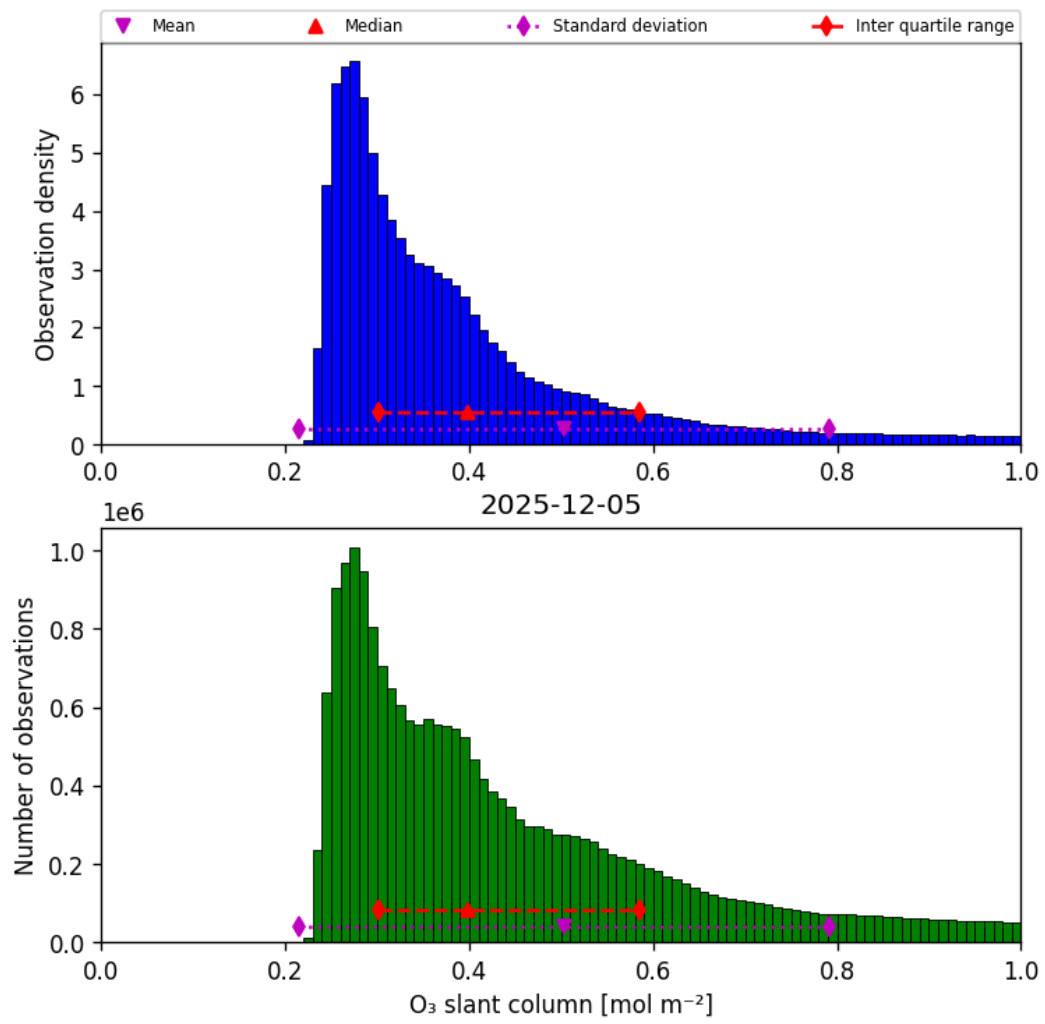
Figure 31: Histogram of “O 3 slant column” for 2025-12-05 to 2025-12-06
