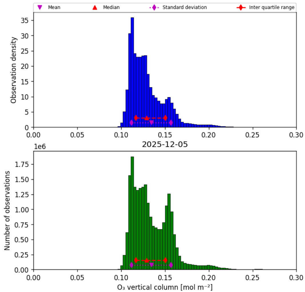
Figure 29: Histogram of “O 3 vertical column” for 2025-12-05 to 2025-12-06
