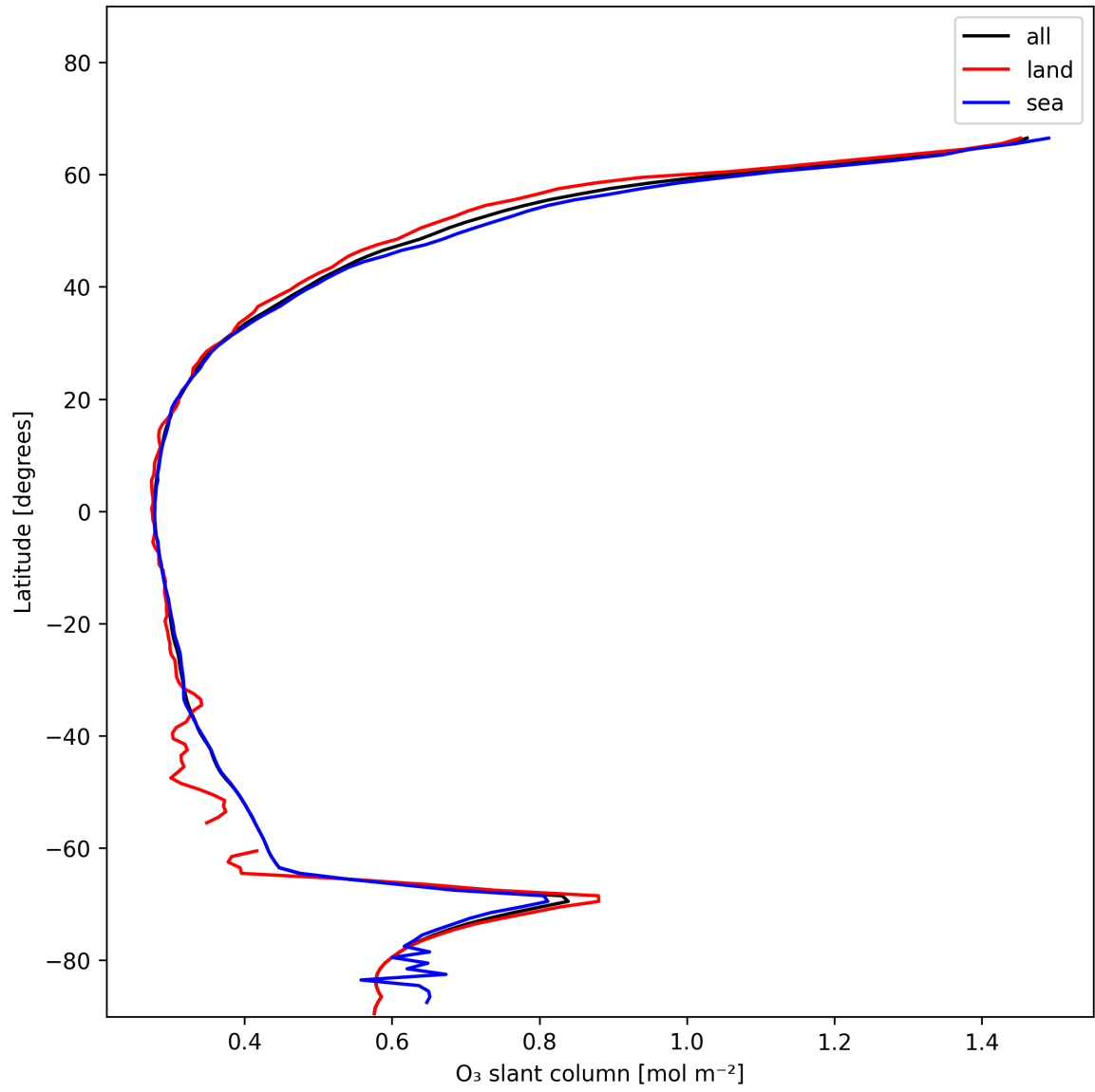
Figure 19: Zonal average of “O 3 slant column” for 2025-12-05 to 2025-12-06.
