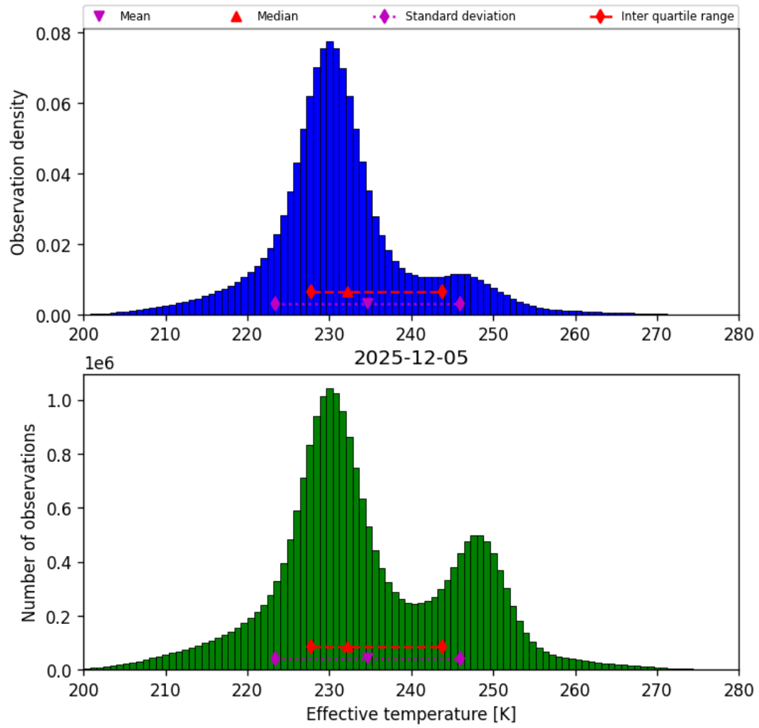
Figure 38: Histogram of “Effective temperature” for 2025-12-05 to 2025-12-06
