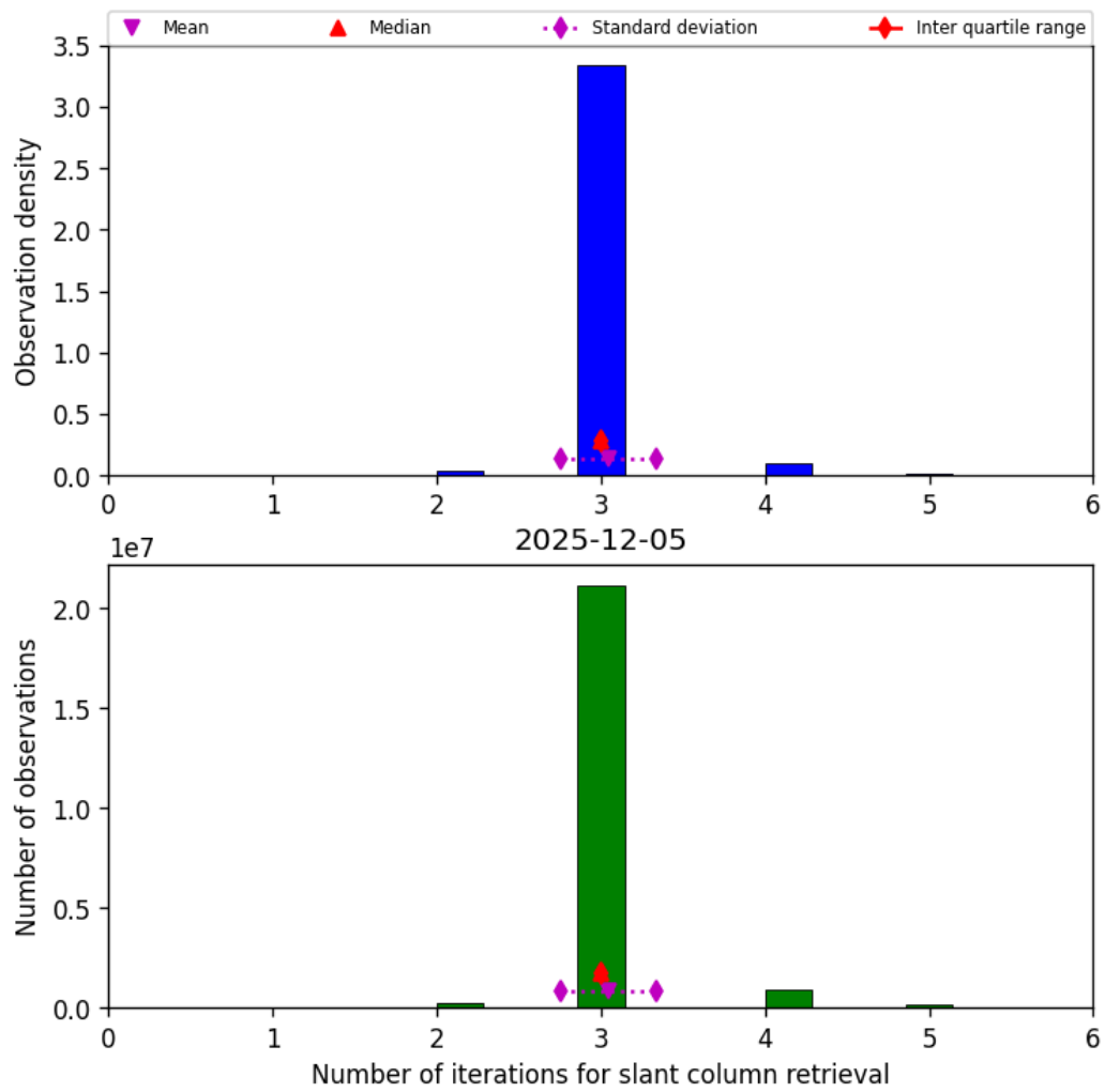
Figure 33: Histogram of “Number of iterations for slant column retrieval” for 2025-12-05 to 2025-12-06
