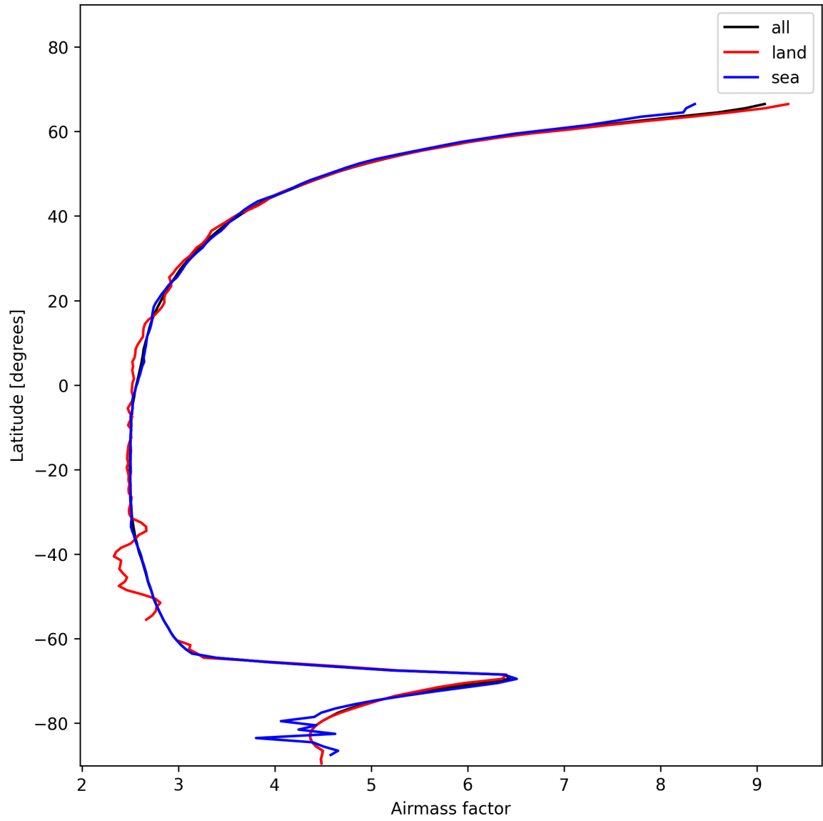
Figure 25: Zonal average of “Airmass factor” for 2025-12-05 to 2025-12-06.
