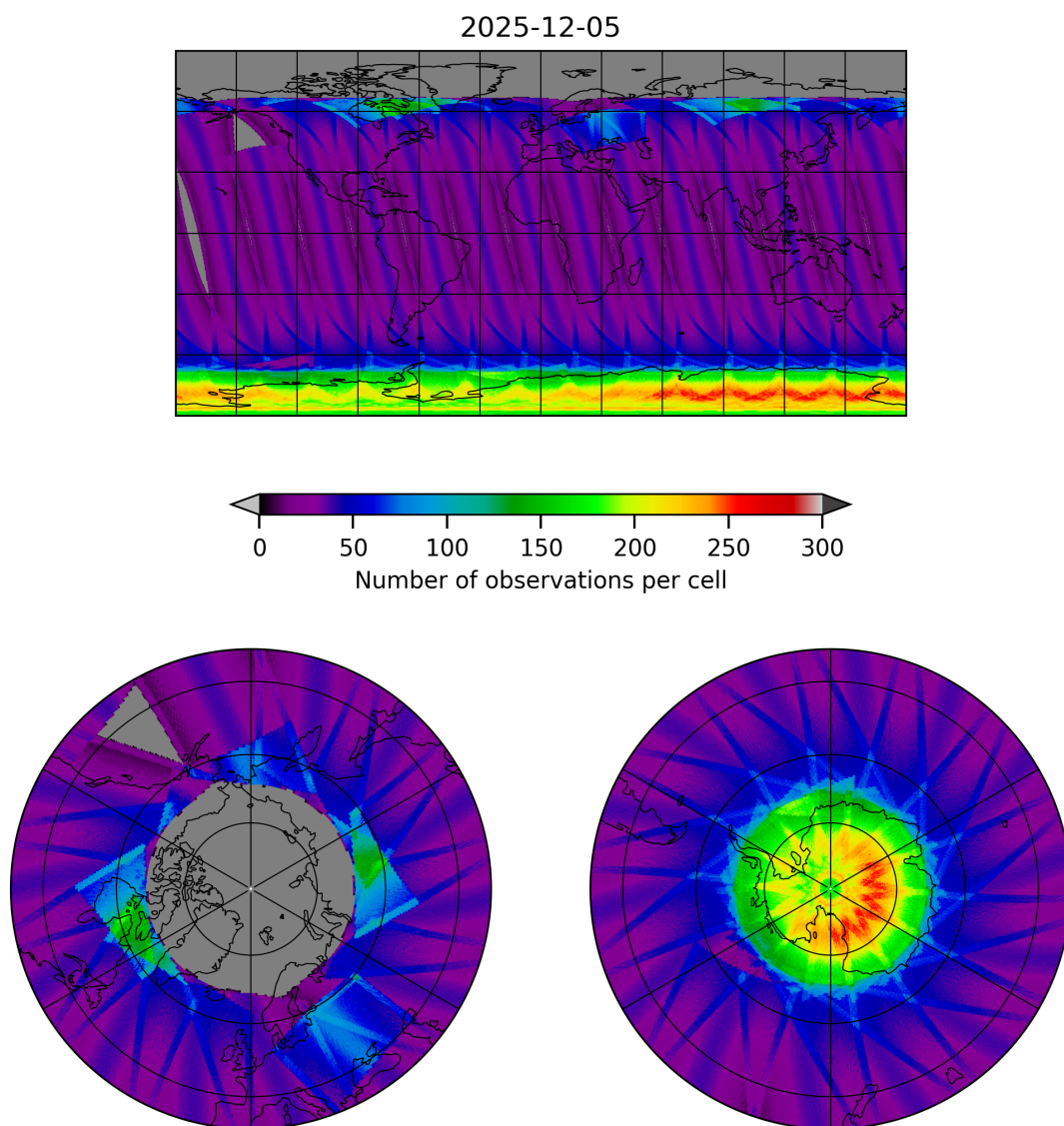
Figure 15: Map of the number of observations for 2025-12-05 to 2025-12-06
