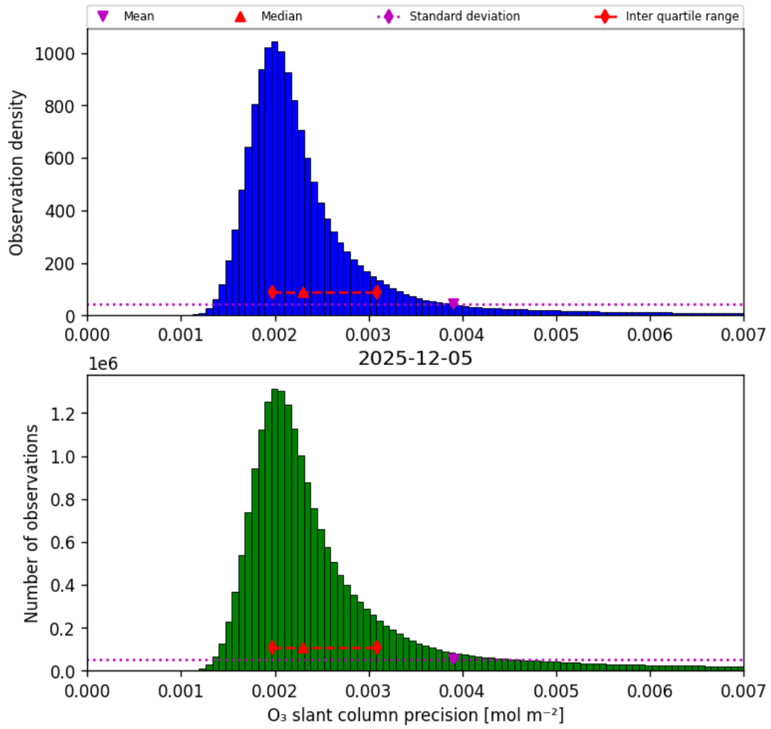
Figure 32: Histogram of “O 3 slant column precision” for 2025-12-05 to 2025-12-06
