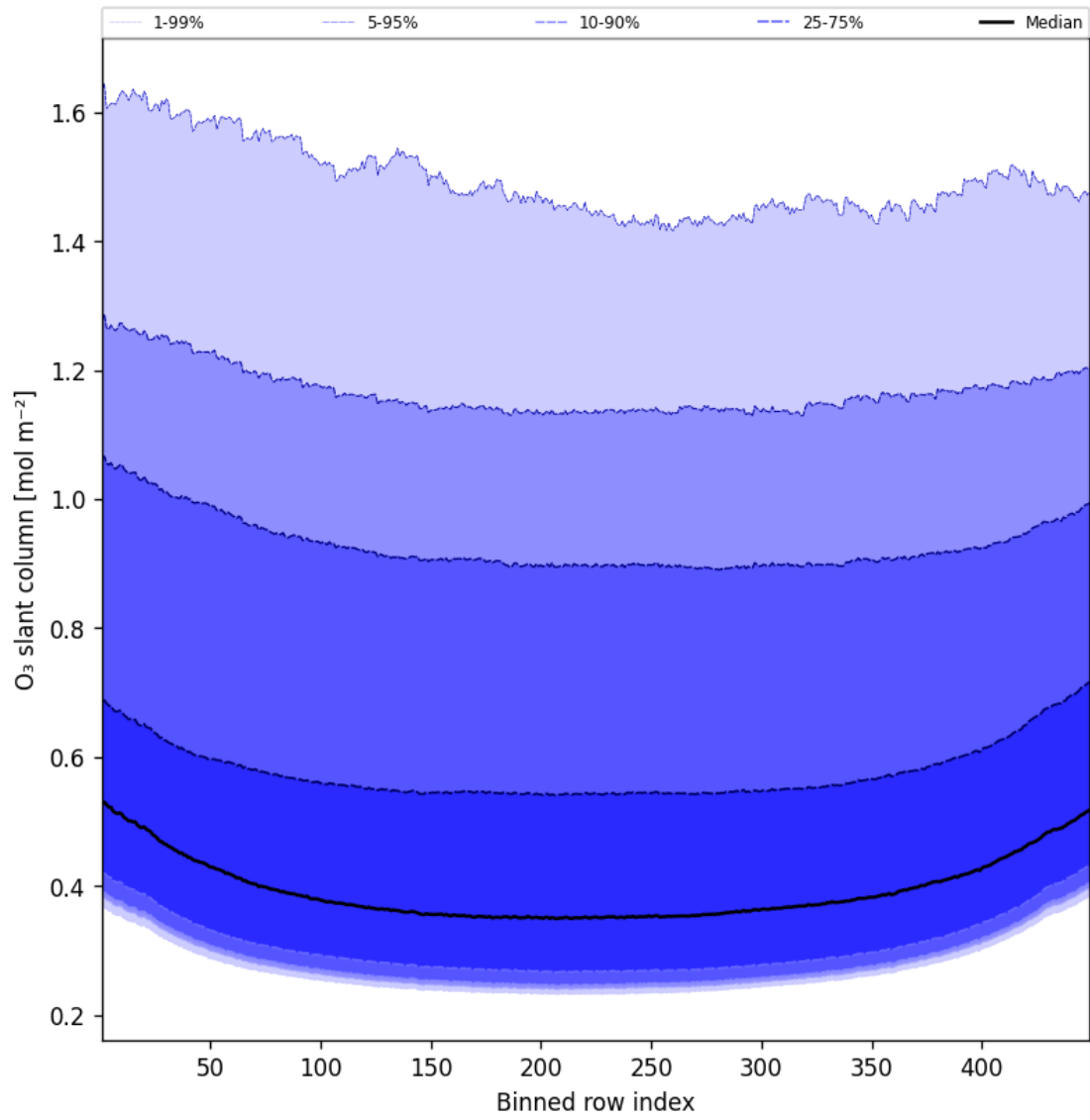
Figure 43: Along track statistics of “O 3 slant column” for 2025-12-05 to 2025-12-06
