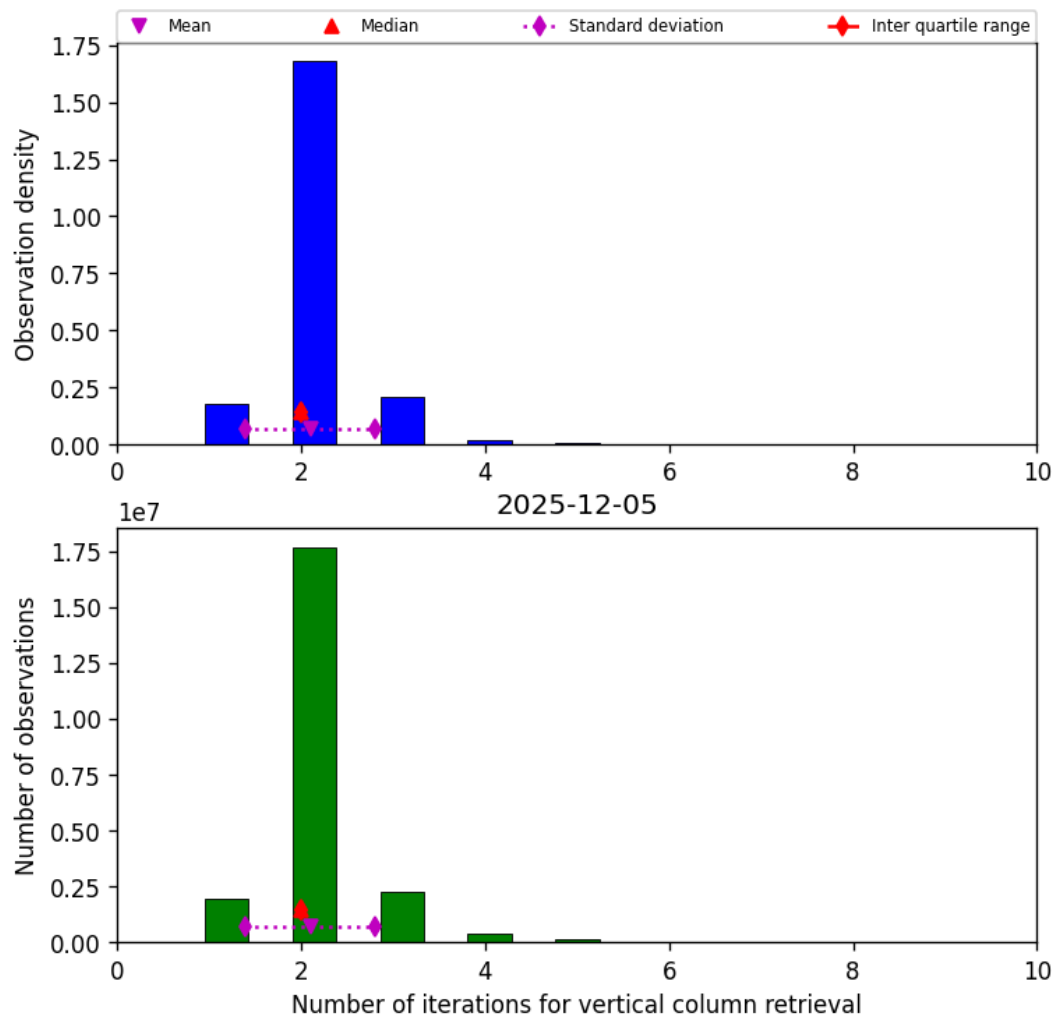
Figure 39: Histogram of “Number of iterations for vertical column retrieval” for 2025-12-05 to 2025-12-06
