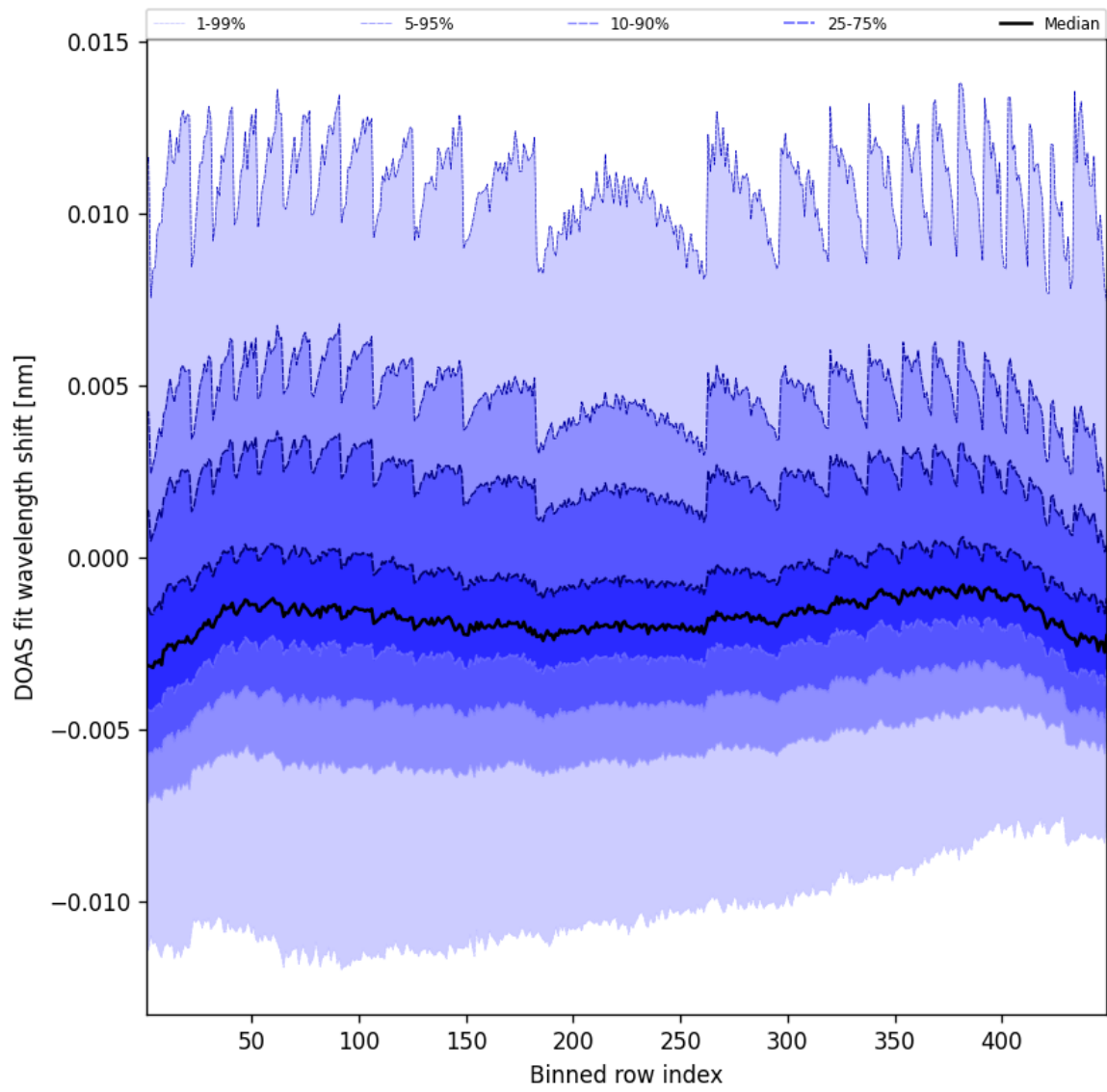
Figure 47: Along track statistics of “DOAS fit wavelength shift” for 2025-12-05 to 2025-12-06
