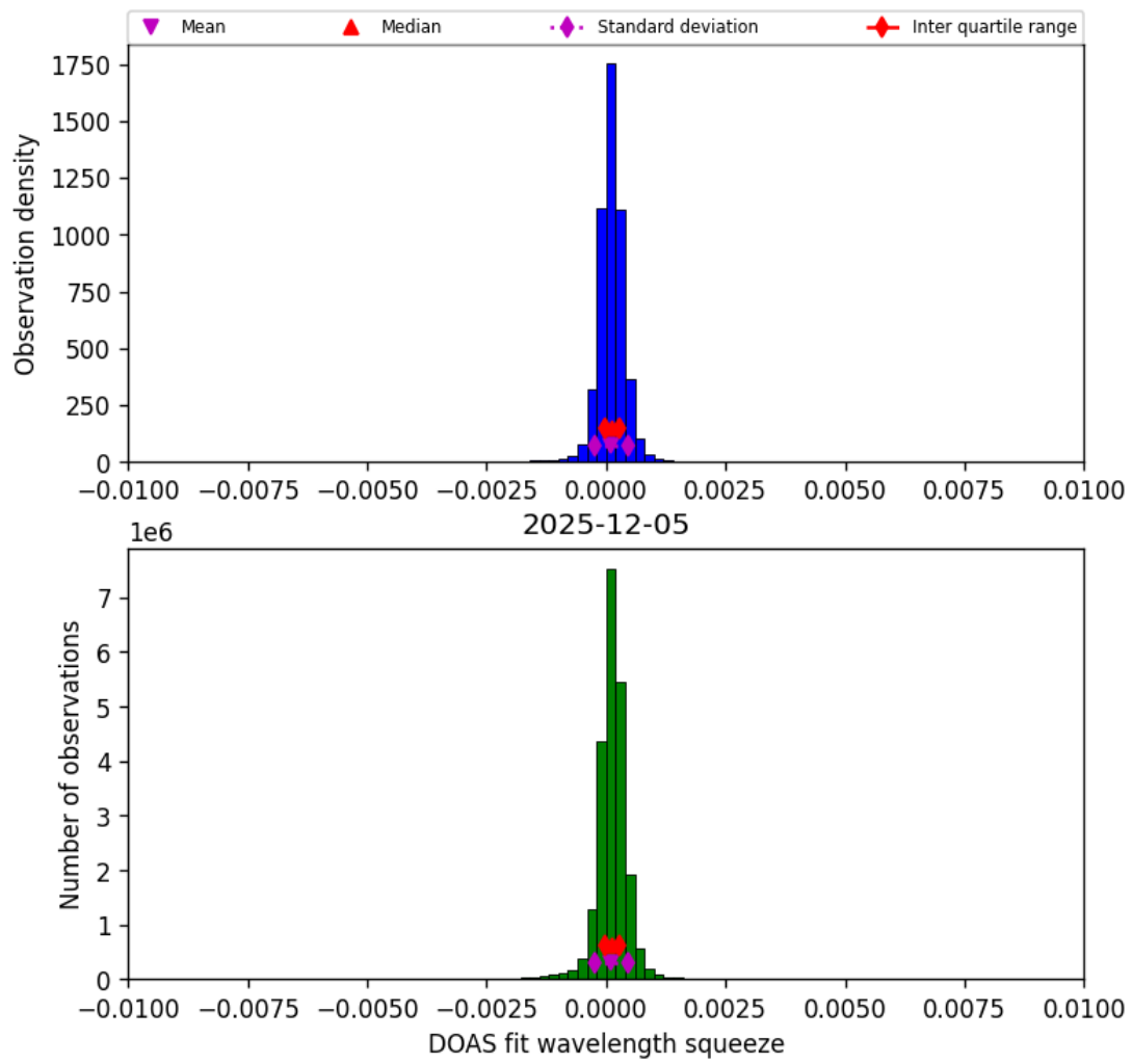
Figure 36: Histogram of “DOAS fit wavelength squeeze” for 2025-12-05 to 2025-12-06
