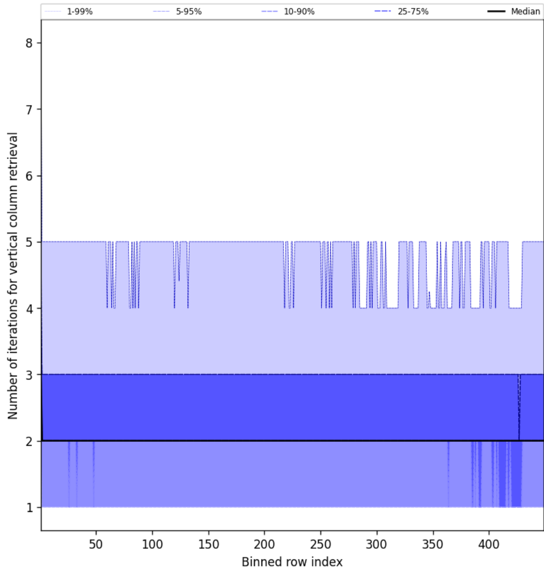
Figure 51: Along track statistics of “Number of iterations for vertical column retrieval” for 2025-12-05 to 2025-12-06
