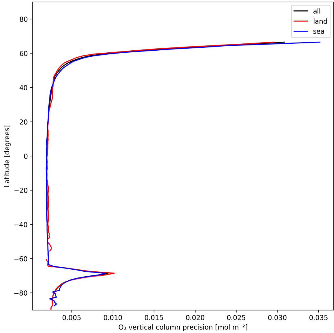
Figure 18: Zonal average of “O 3 vertical column precision” for 2025-12-05 to 2025-12-06.
