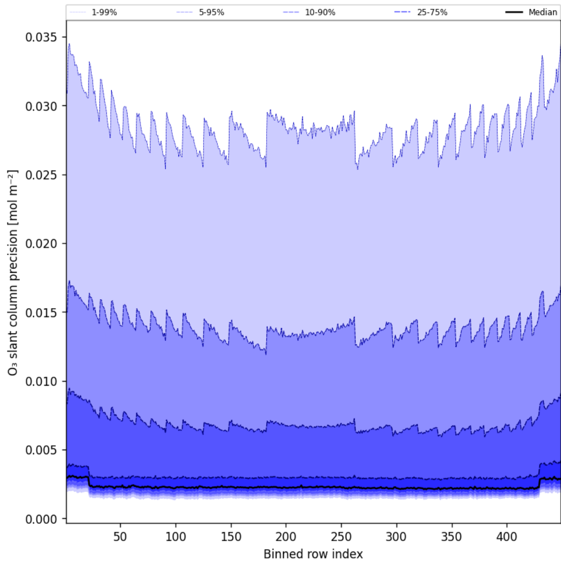
Figure 44: Along track statistics of “O 3 slant column precision” for 2025-12-05 to 2025-12-06
