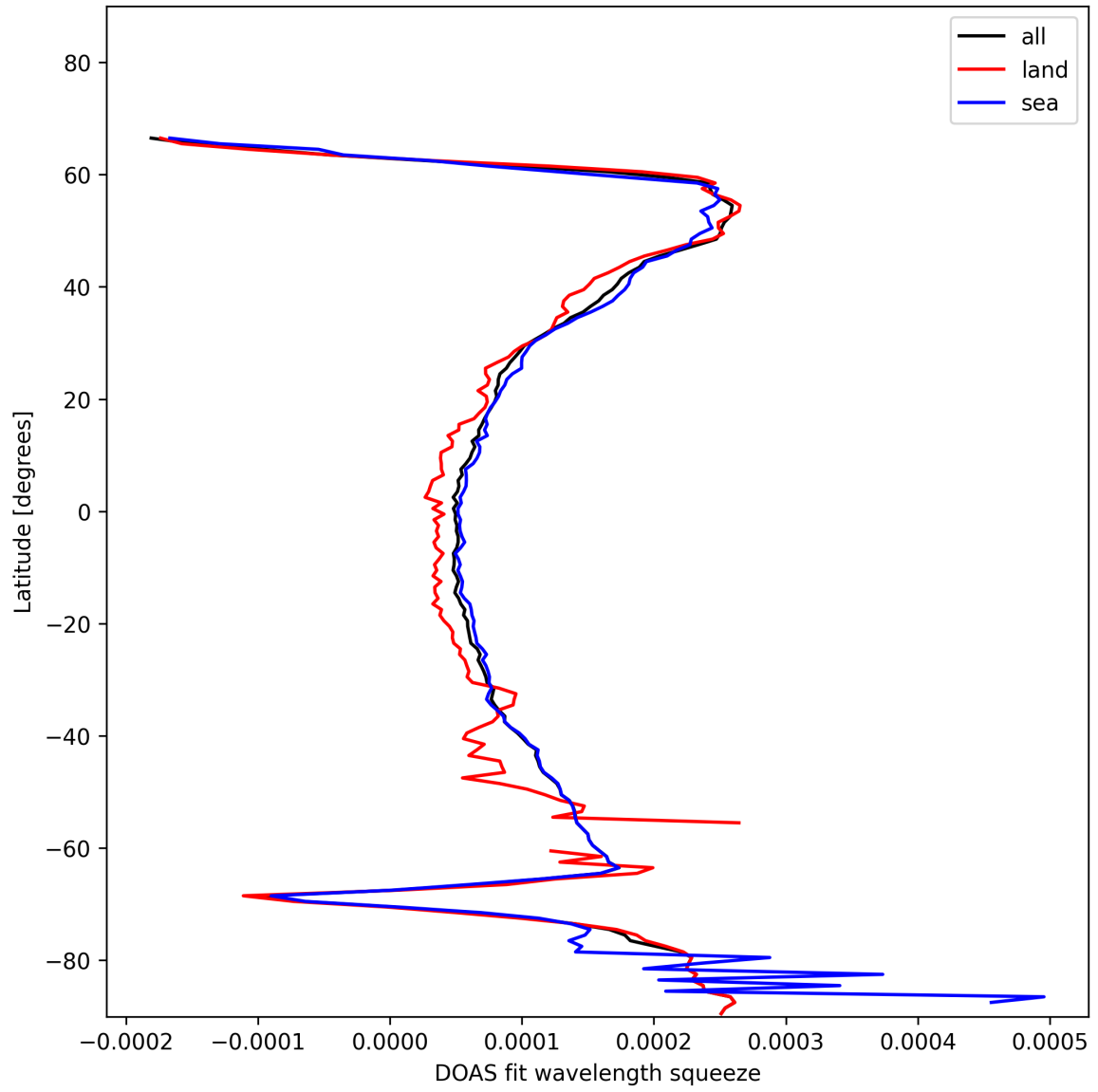
Figure 24: Zonal average of “DOAS fit wavelength squeeze” for 2025-12-05 to 2025-12-06.
