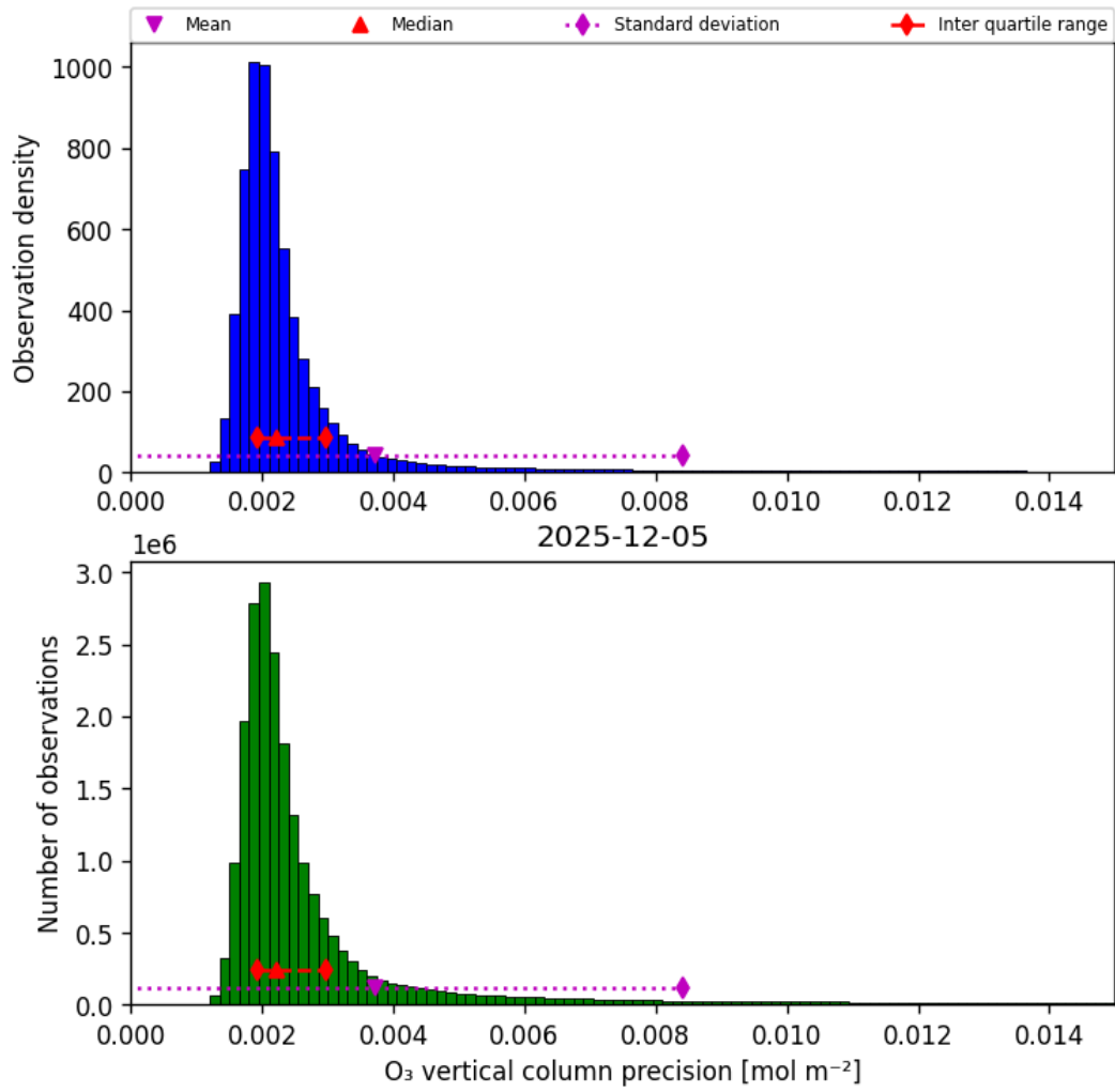
Figure 30: Histogram of “O 3 vertical column precision” for 2025-12-05 to 2025-12-06
