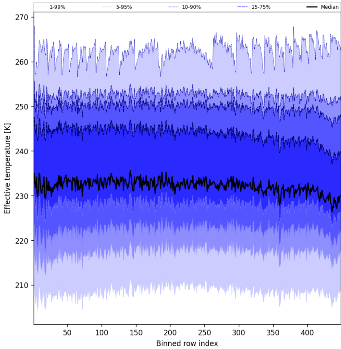
Figure 50: Along track statistics of “Effective temperature” for 2025-12-05 to 2025-12-06
