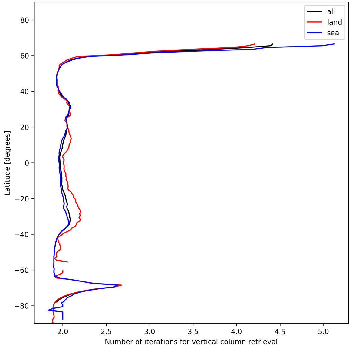
Figure 27: Zonal average of “Number of iterations for vertical column retrieval” for 2025-12-05 to 2025-12-06.
