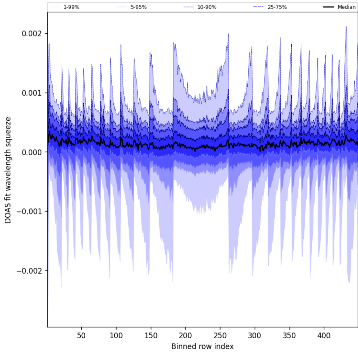
Figure 48: Along track statistics of “DOAS fit wavelength squeeze” for 2025-12-05 to 2025-12-06
