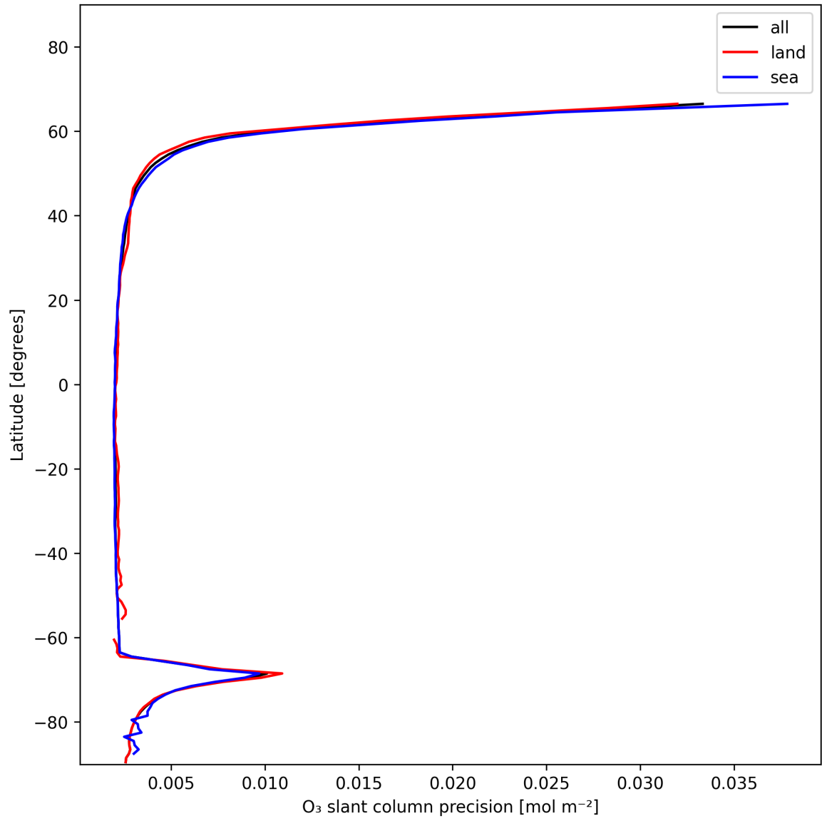
Figure 20: Zonal average of “O 3 slant column precision” for 2025-12-05 to 2025-12-06.
