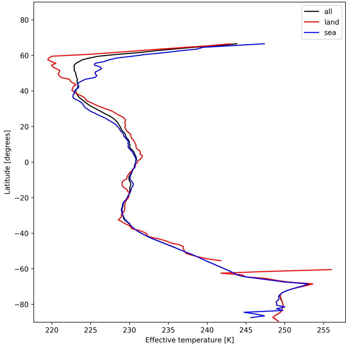
Figure 26: Zonal average of “Effective temperature” for 2025-12-05 to 2025-12-06.
