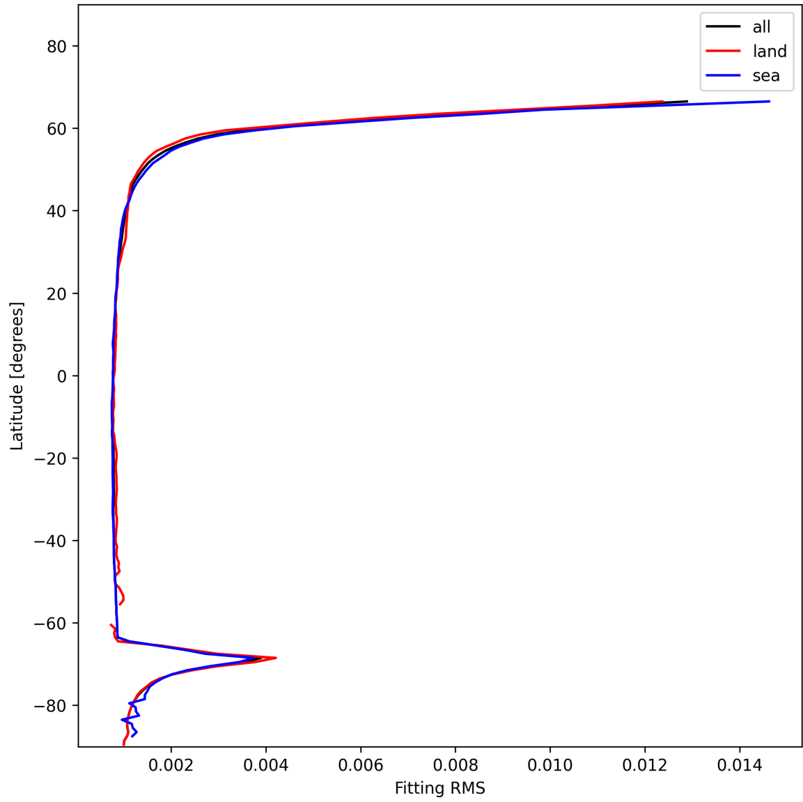
Figure 22: Zonal average of “Fitting RMS” for 2025-12-05 to 2025-12-06.
