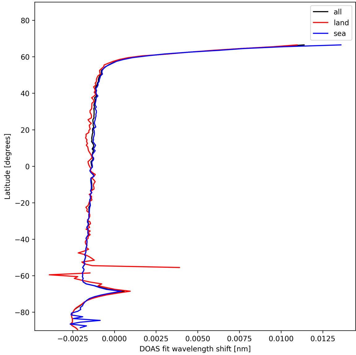
Figure 23: Zonal average of “DOAS fit wavelength shift” for 2025-12-06 to 2025-12-07.
