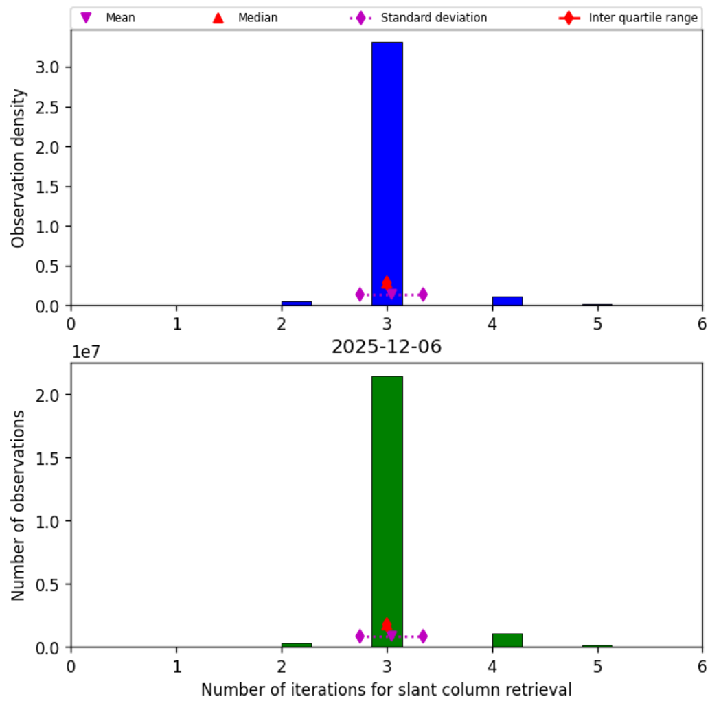
Figure 33: Histogram of "Number of iterations for slant column retrieval" for 2025-12-06 to 2025-12-07
