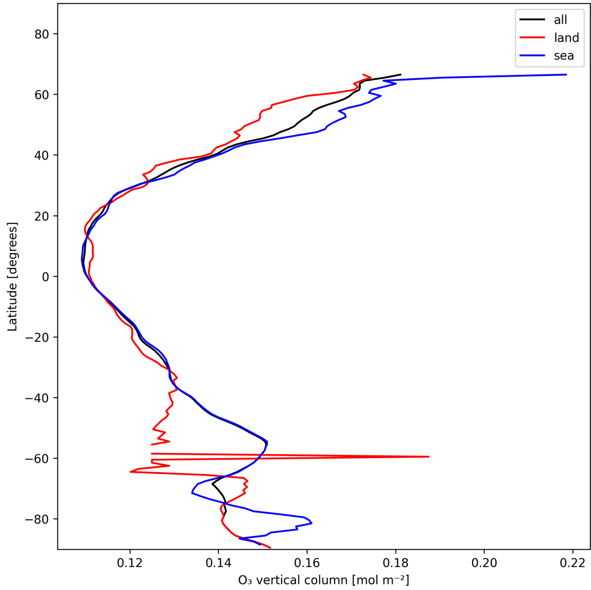
Figure 17: Zonal average of “O 3 vertical column” for 2025-12-06 to 2025-12-07.
