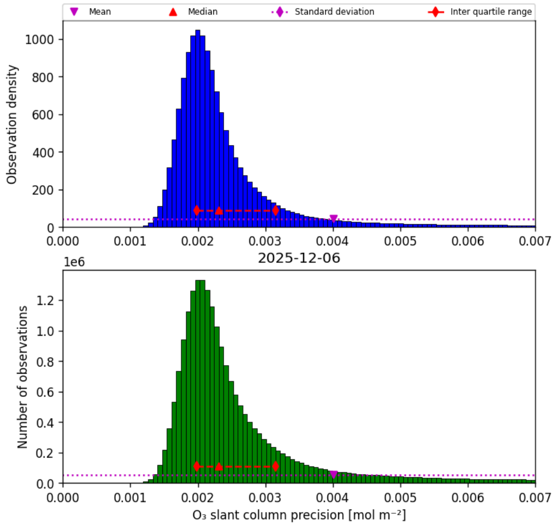
Figure 32: Histogram of “O 3 slant column precision” for 2025-12-06 to 2025-12-07
