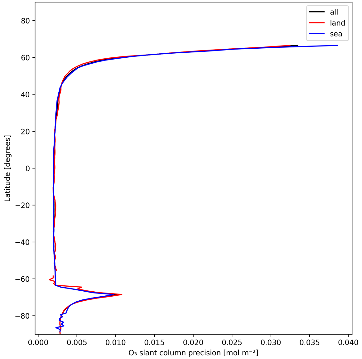
Figure 20: Zonal average of “O 3 slant column precision” for 2025-12-06 to 2025-12-07.
