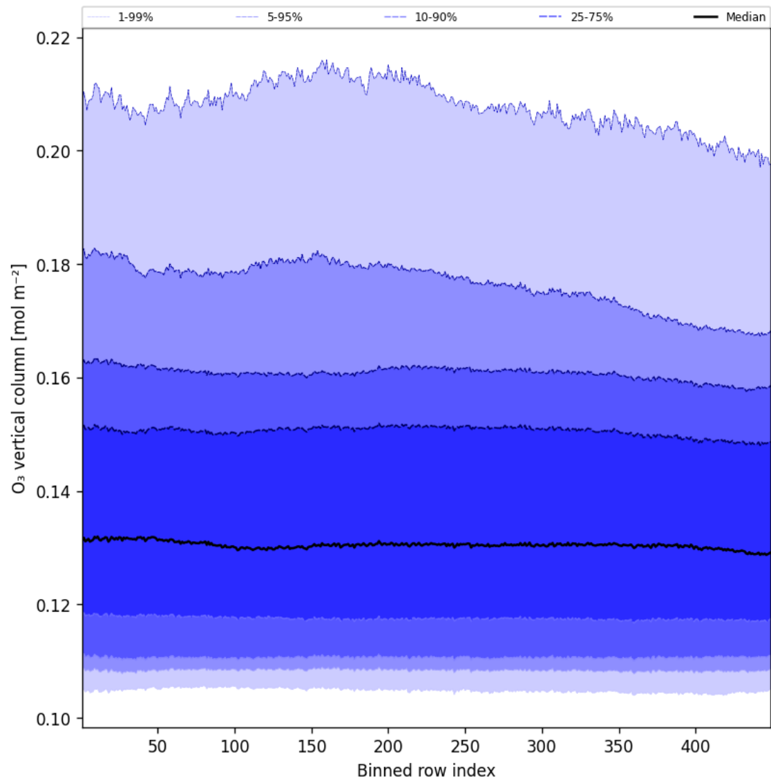
Figure 41: Along track statistics of “O 3 vertical column” for 2025-12-06 to 2025-12-07
