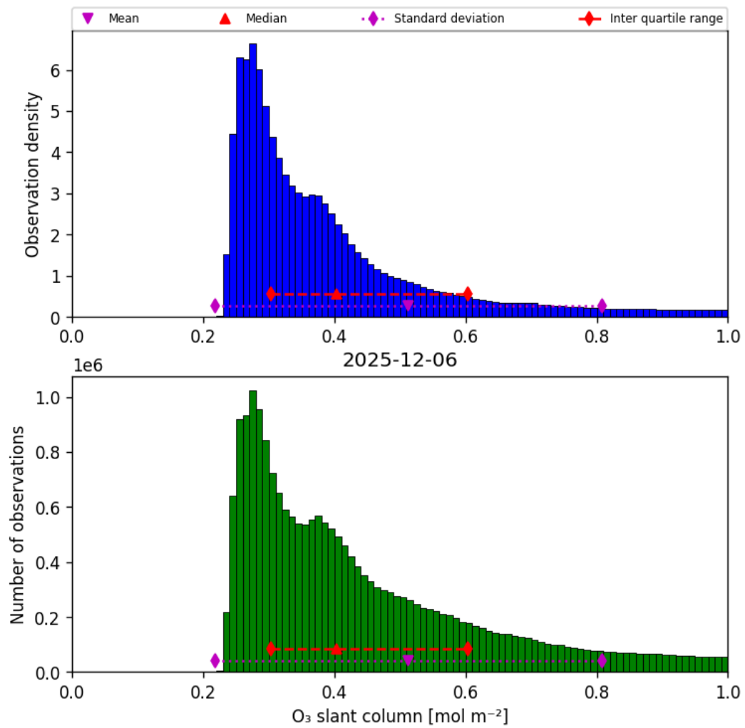
Figure 31: Histogram of “O 3 slant column” for 2025-12-06 to 2025-12-07
