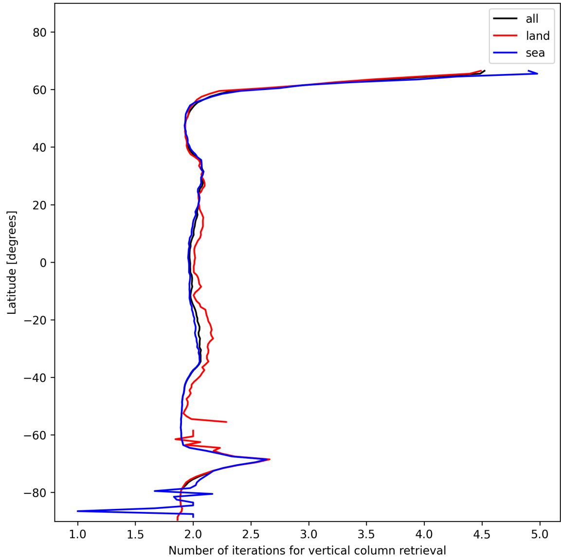
Figure 27: Zonal average of “Number of iterations for vertical column retrieval” for 2025-12-06 to 2025-12-07.
