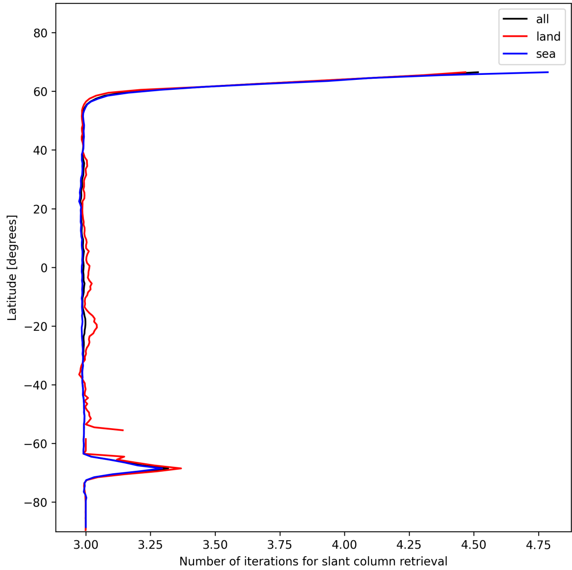
Figure 21: Zonal average of “Number of iterations for slant column retrieval” for 2025-12-06 to 2025-12-07.
