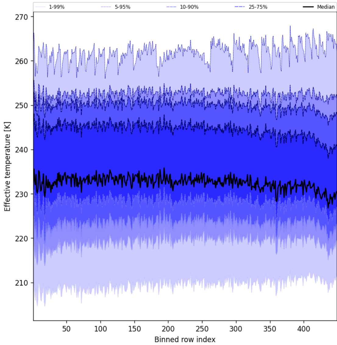
Figure 50: Along track statistics of “Effective temperature” for 2025-12-06 to 2025-12-07
