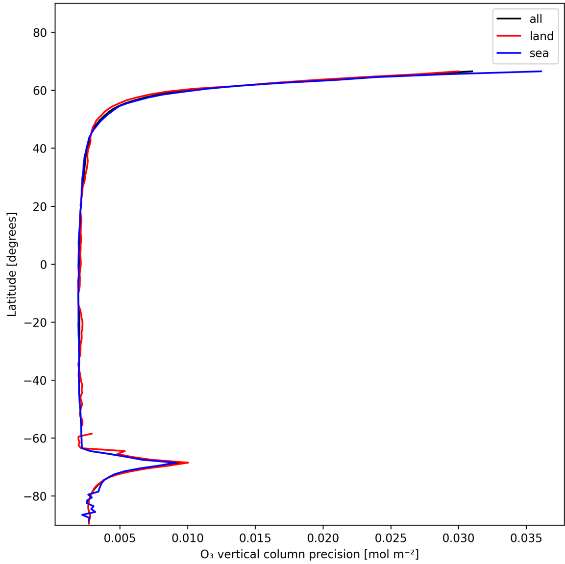
Figure 18: Zonal average of “O 3 vertical column precision” for 2025-12-06 to 2025-12-07.
