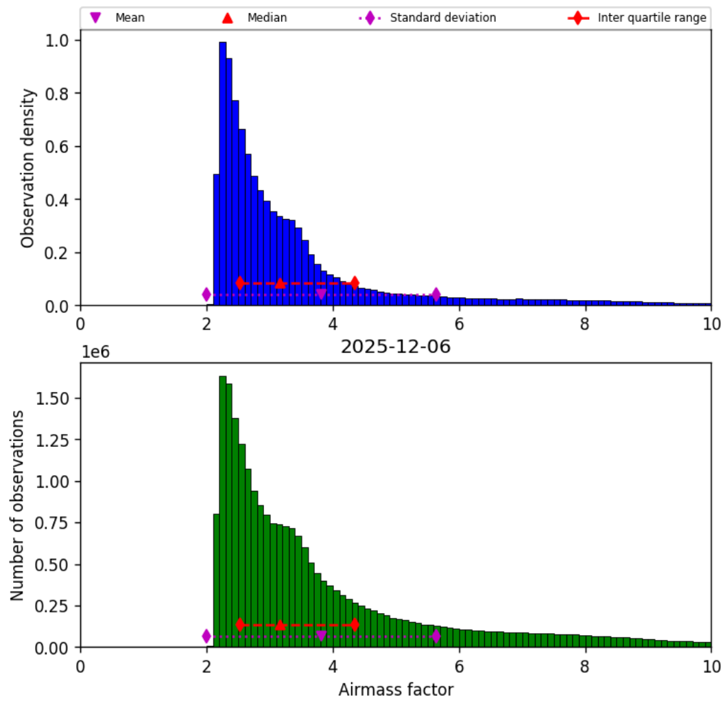
Figure 37: Histogram of “Airmass factor” for 2025-12-06 to 2025-12-07
