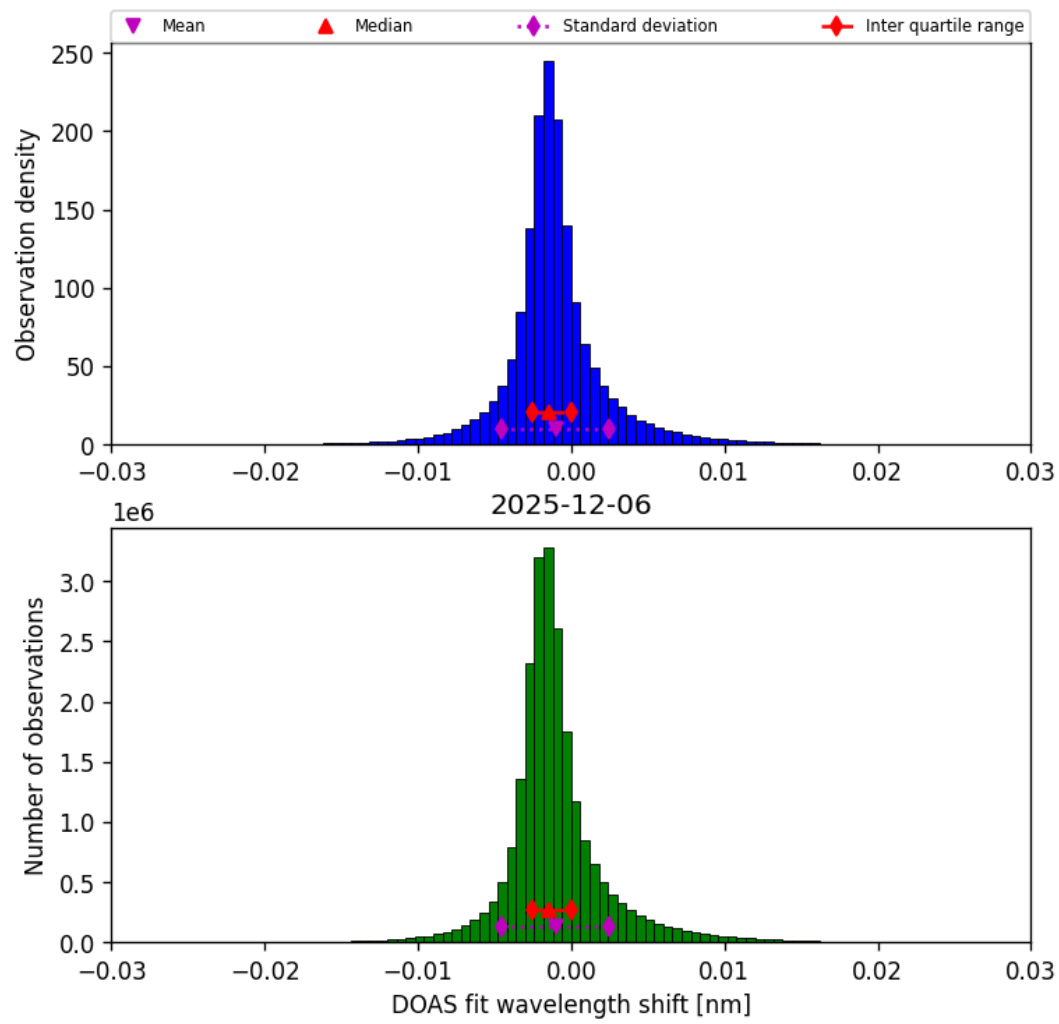
Figure 35: Histogram of “DOAS fit wavelength shift” for 2025-12-06 to 2025-12-07
