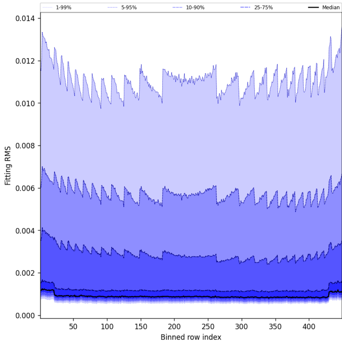
Figure 46: Along track statistics of “Fitting RMS” for 2025-12-06 to 2025-12-07
