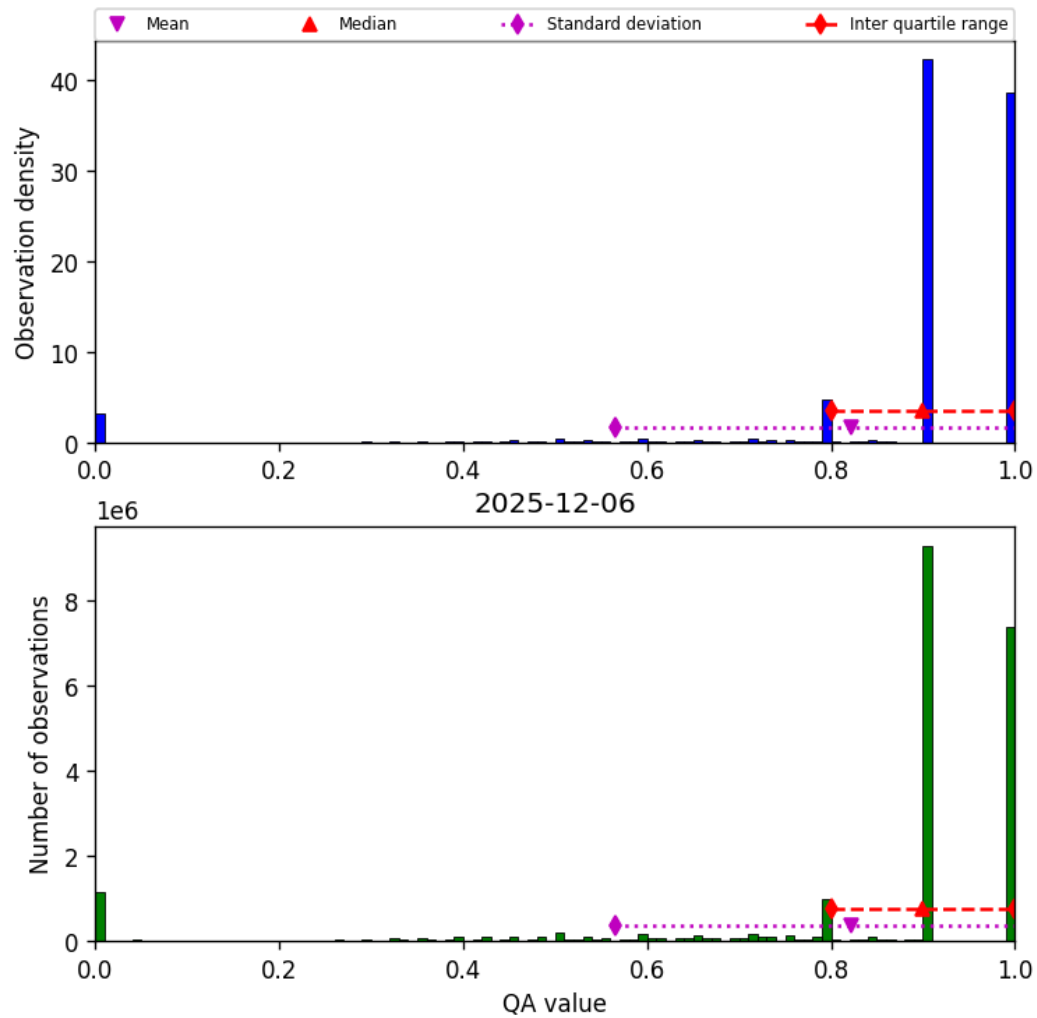
Figure 28: Histogram of “QA value” for 2025-12-06 to 2025-12-07
