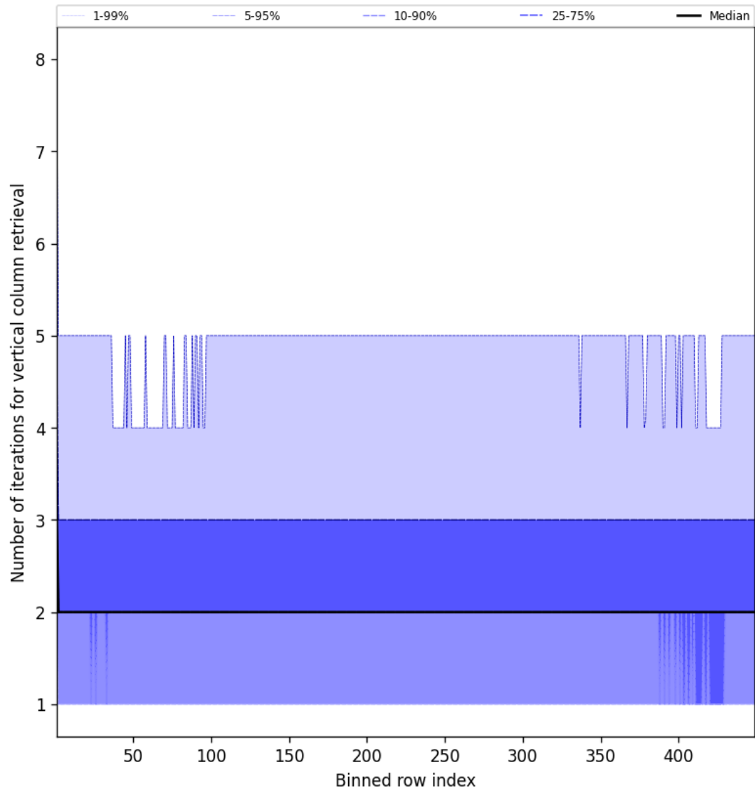
Figure 51: Along track statistics of “Number of iterations for vertical column retrieval” for 2025-12-06 to 2025-12-07
