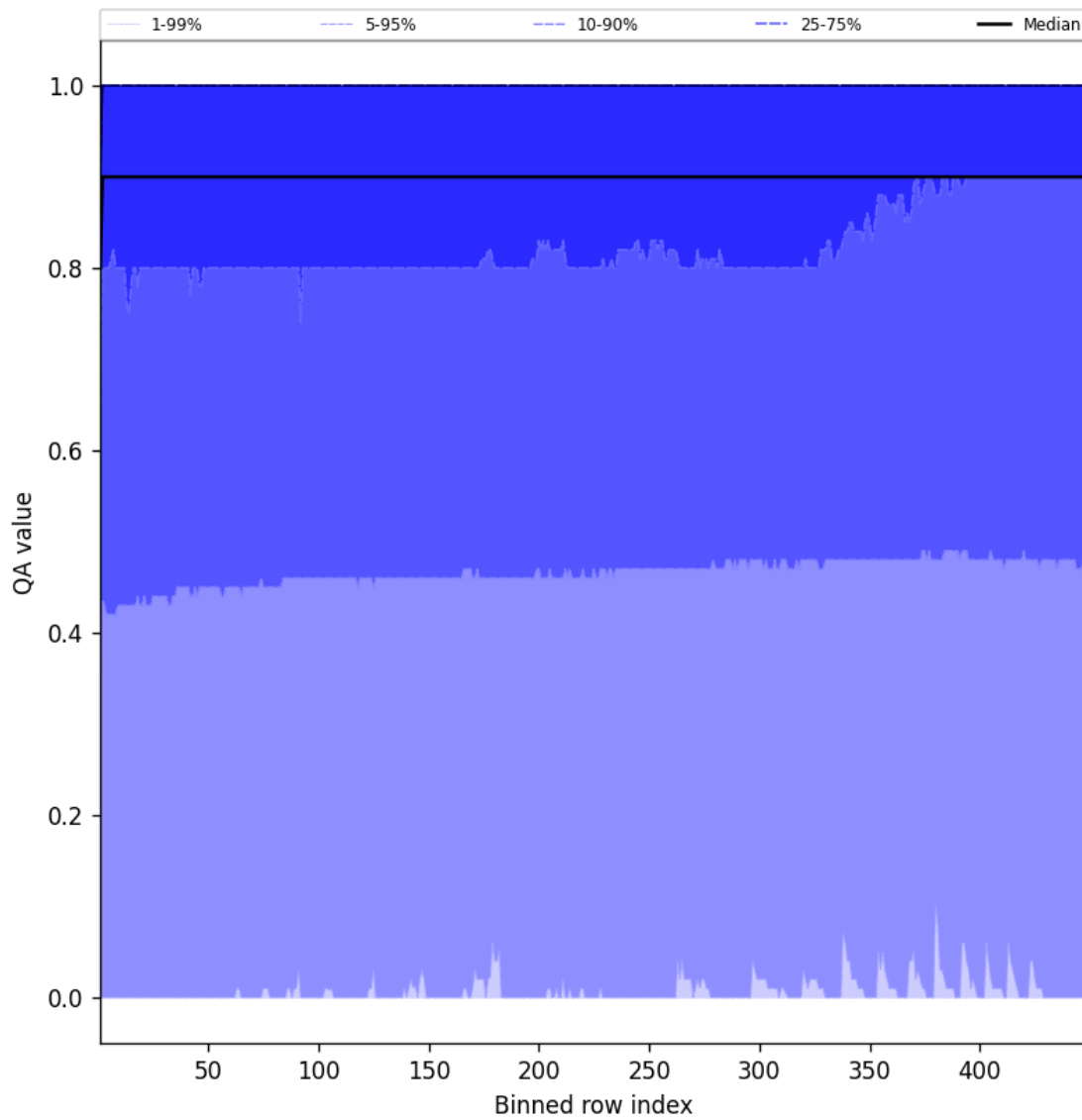
Figure 40: Along track statistics of “QA value” for 2025-12-06 to 2025-12-07
