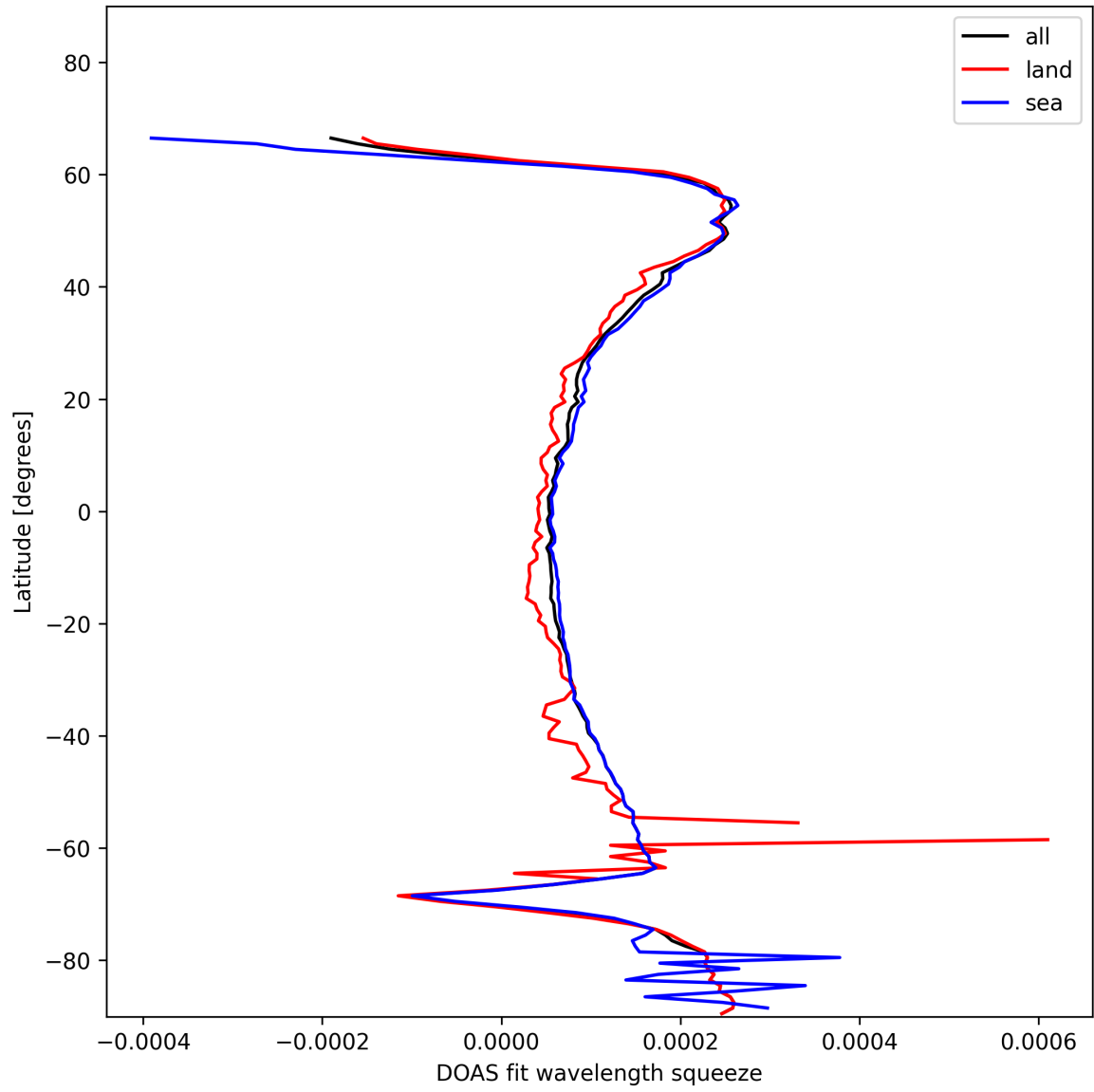
Figure 24: Zonal average of “DOAS fit wavelength squeeze” for 2025-12-06 to 2025-12-07.
