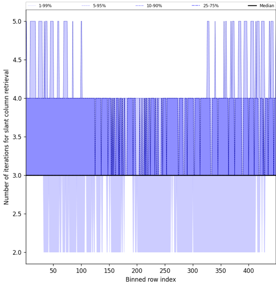
Figure 45: Along track statistics of “Number of iterations for slant column retrieval” for 2025-12-06 to 2025-12-07
