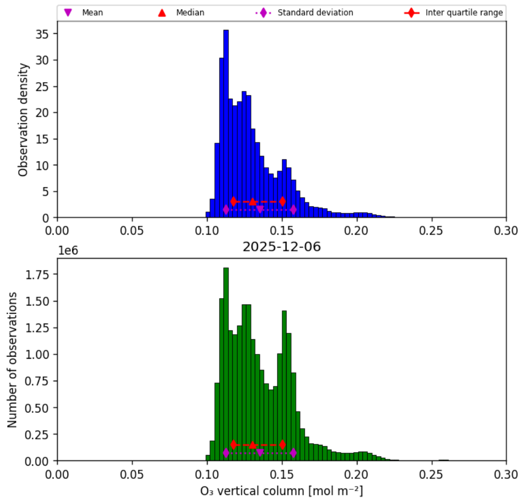
Figure 29: Histogram of “O 3 vertical column” for 2025-12-06 to 2025-12-07
