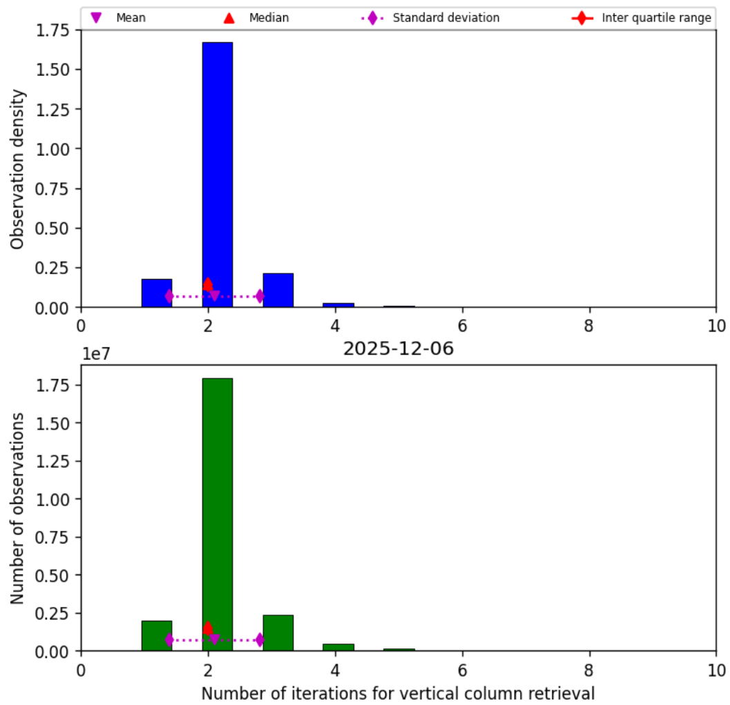
Figure 39: Histogram of “Number of iterations for vertical column retrieval” for 2025-12-06 to 2025-12-07
