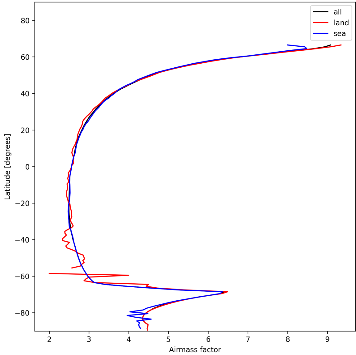
Figure 25: Zonal average of “Airmass factor” for 2025-12-06 to 2025-12-07.
