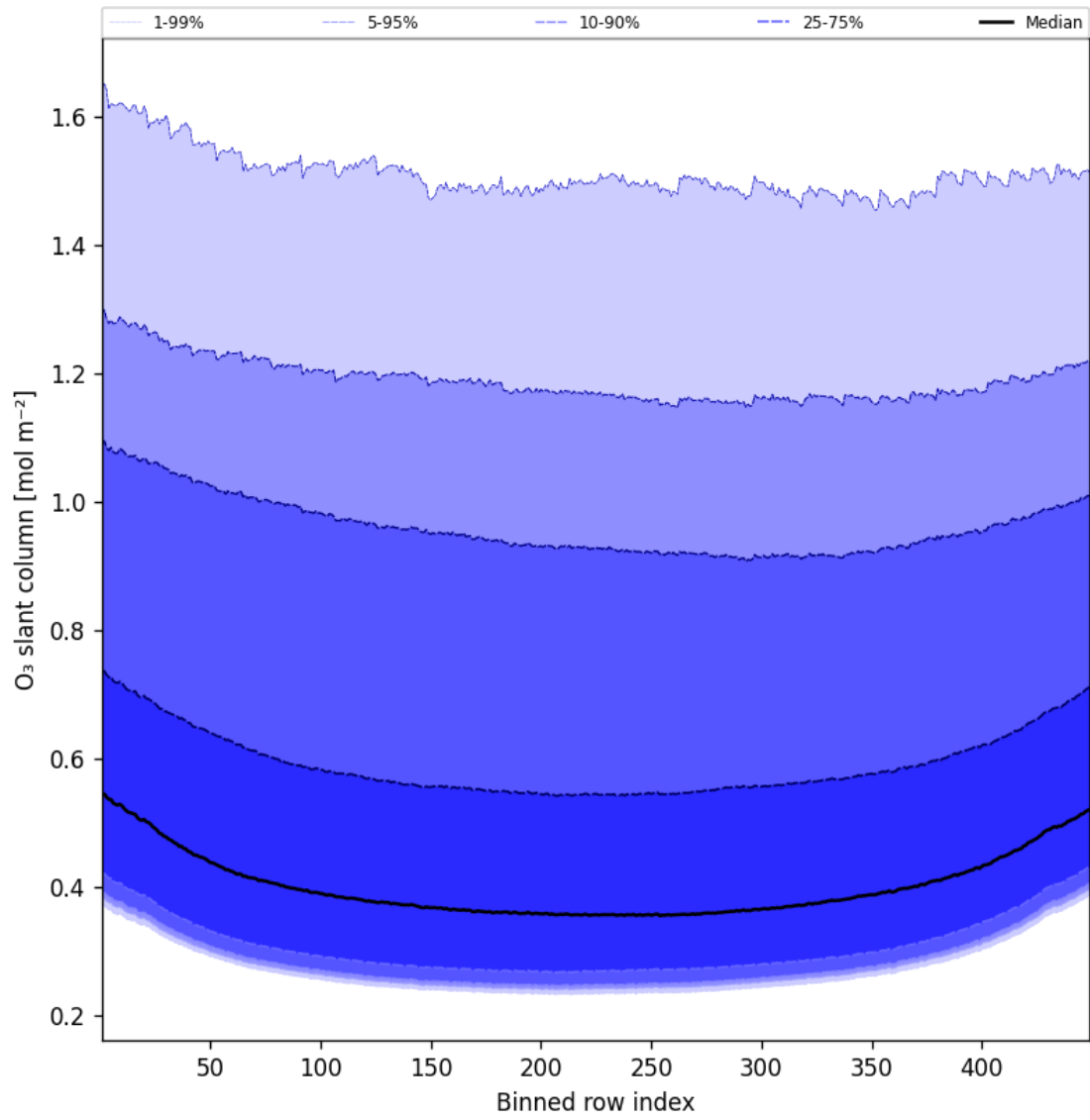
Figure 43: Along track statistics of “O 3 slant column” for 2025-12-06 to 2025-12-07
