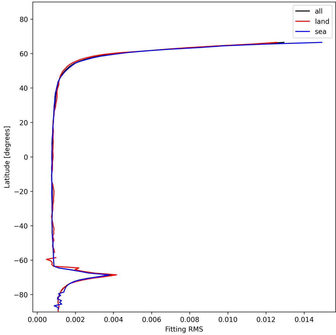
Figure 22: Zonal average of “Fitting RMS” for 2025-12-06 to 2025-12-07.
