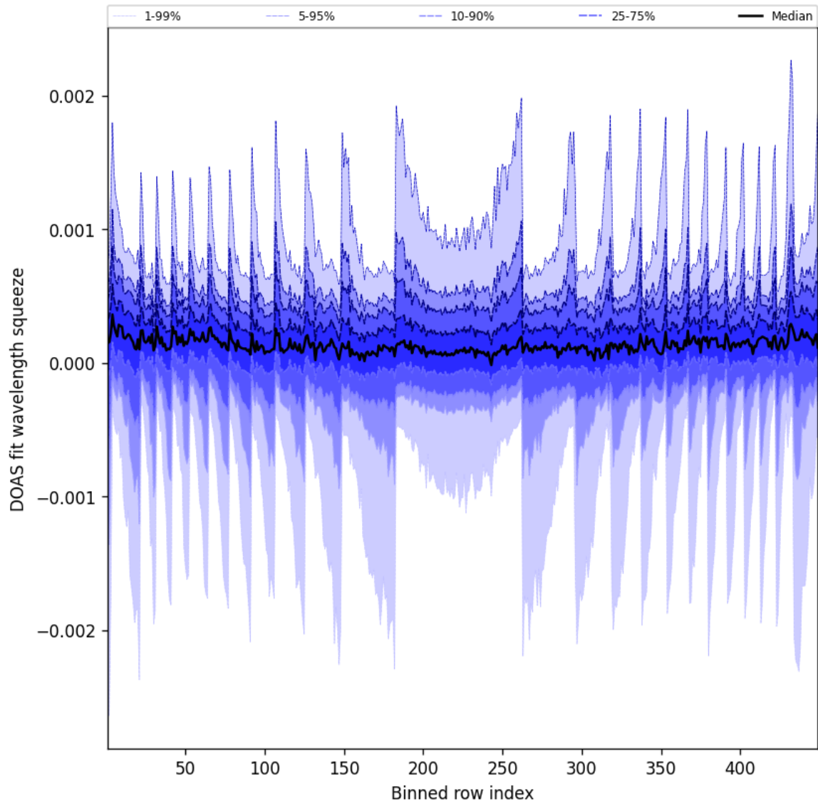
Figure 48: Along track statistics of “DOAS fit wavelength squeeze” for 2025-12-06 to 2025-12-07
