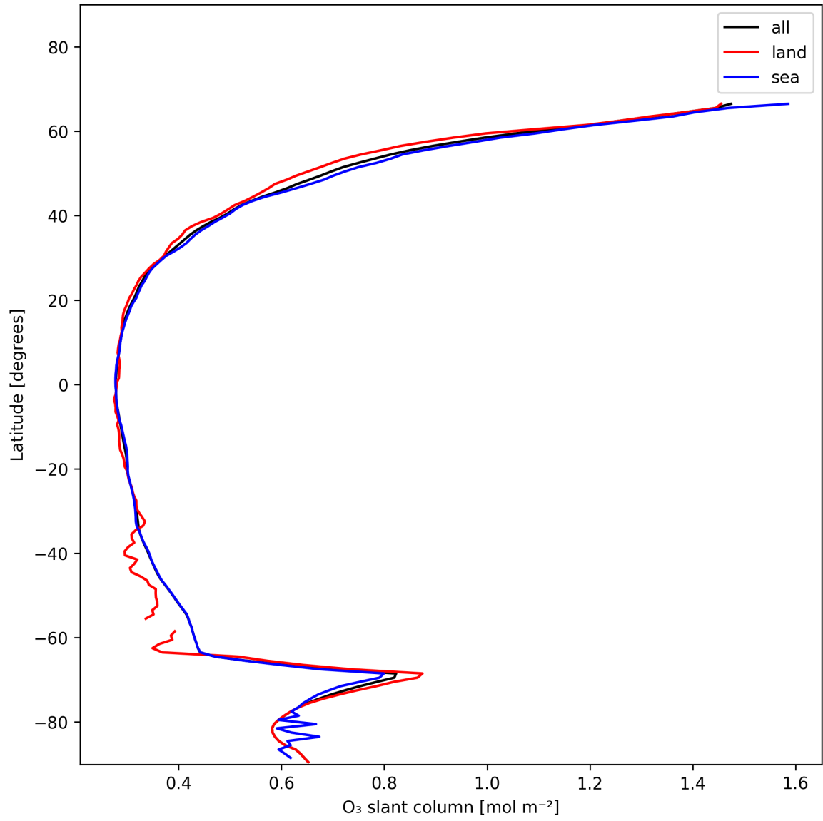
Figure 19: Zonal average of “O 3 slant column” for 2025-12-06 to 2025-12-07.
