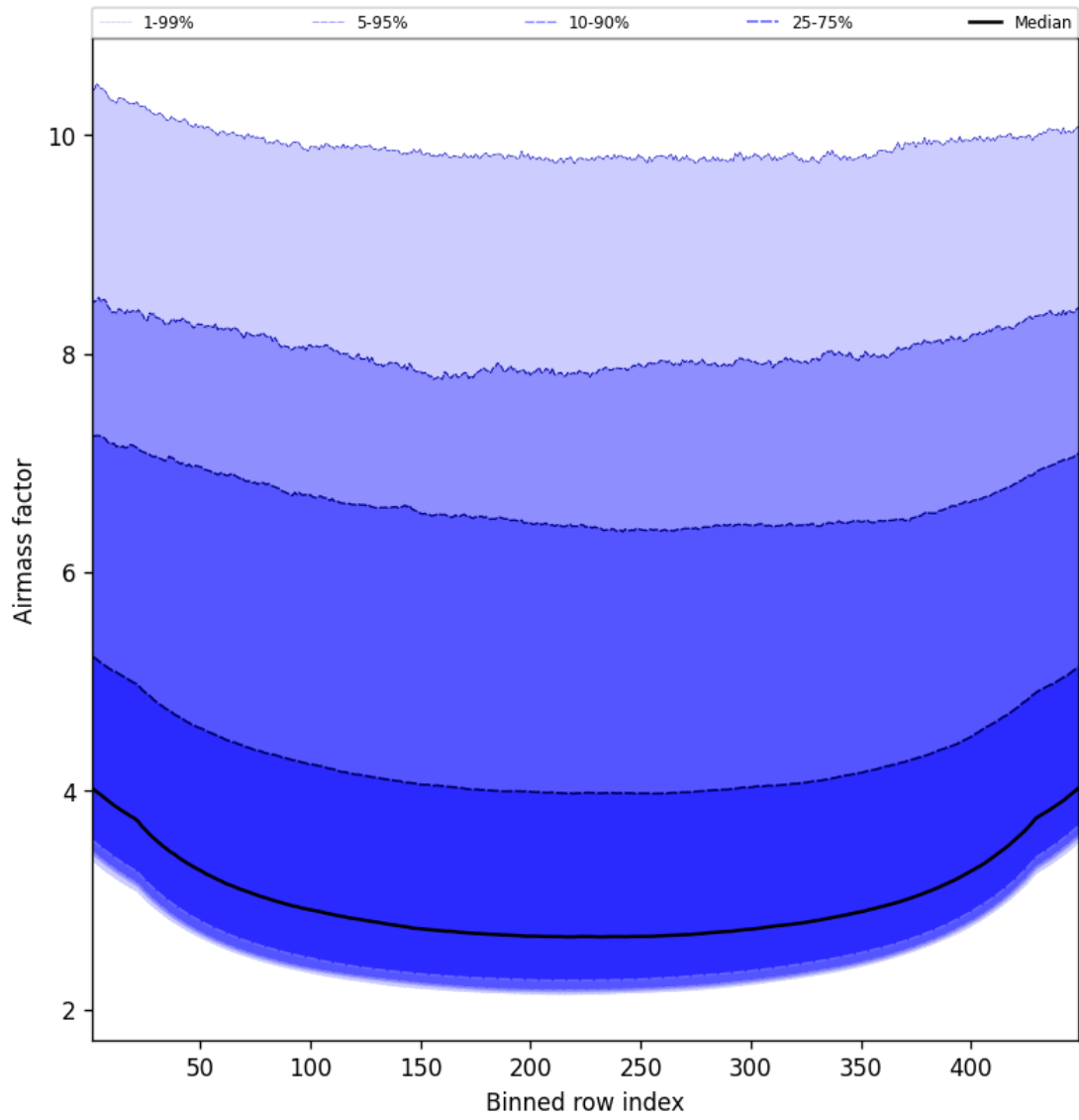
Figure 49: Along track statistics of “Airmass factor” for 2025-12-06 to 2025-12-07
