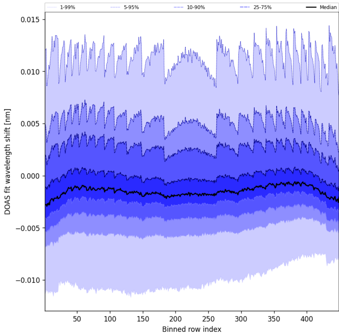
Figure 47: Along track statistics of “DOAS fit wavelength shift” for 2025-12-06 to 2025-12-07
