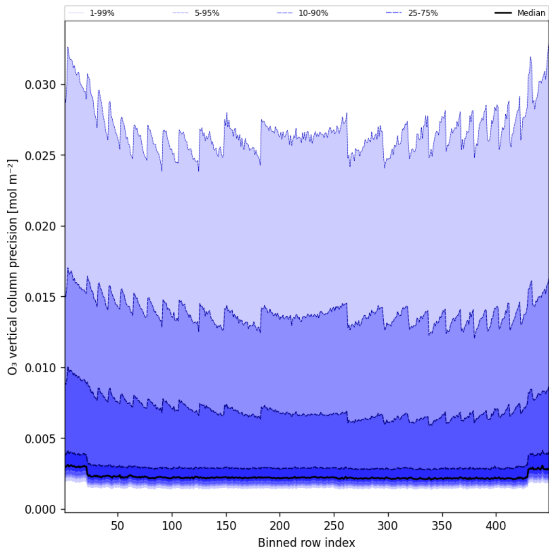
Figure 42: Along track statistics of “O 3 vertical column precision” for 2025-12-06 to 2025-12-07
