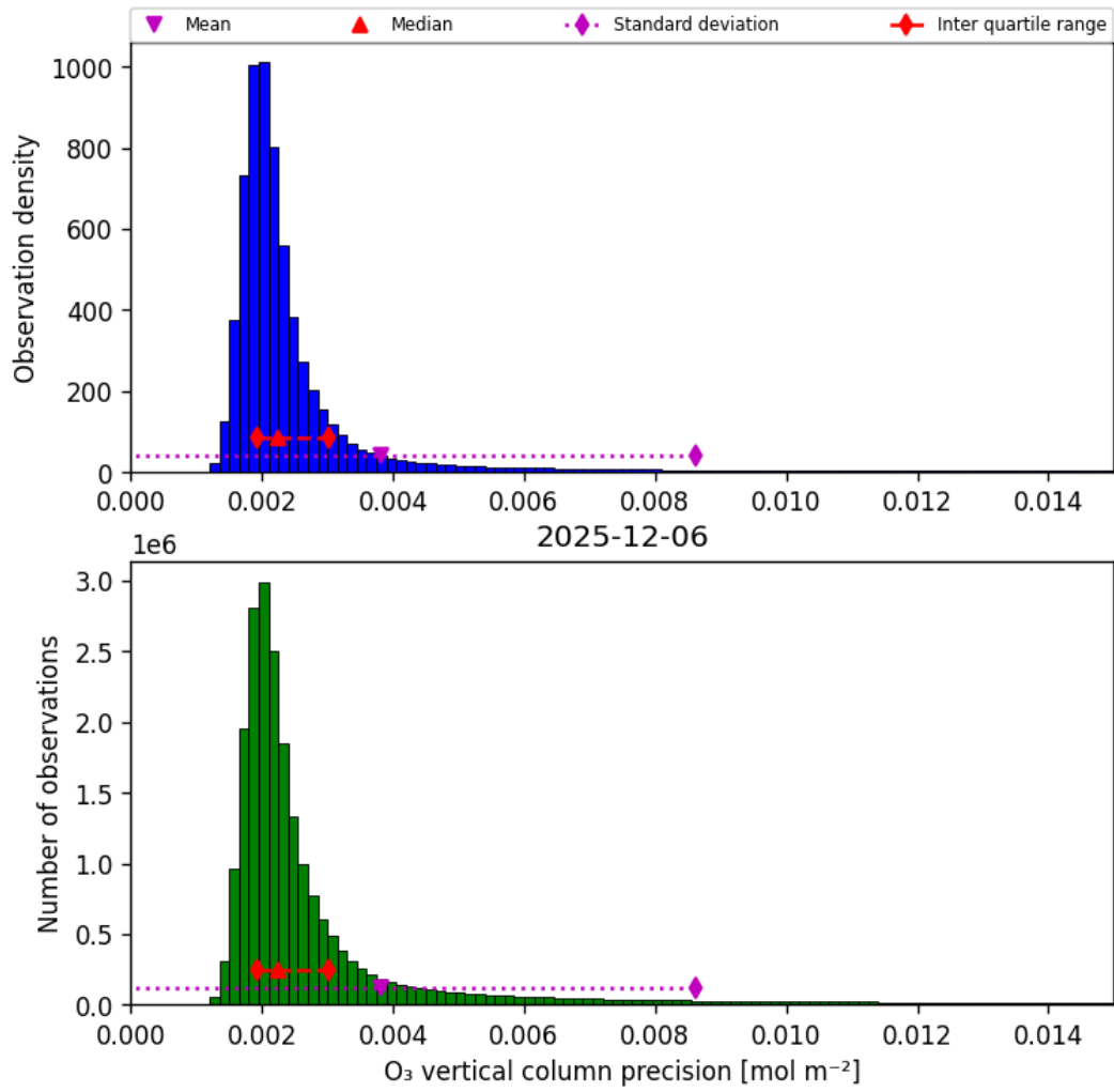
Figure 30: Histogram of “O 3 vertical column precision” for 2025-12-06 to 2025-12-07
