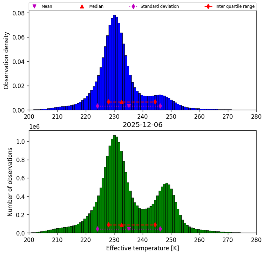
Figure 38: Histogram of “Effective temperature” for 2025-12-06 to 2025-12-07
