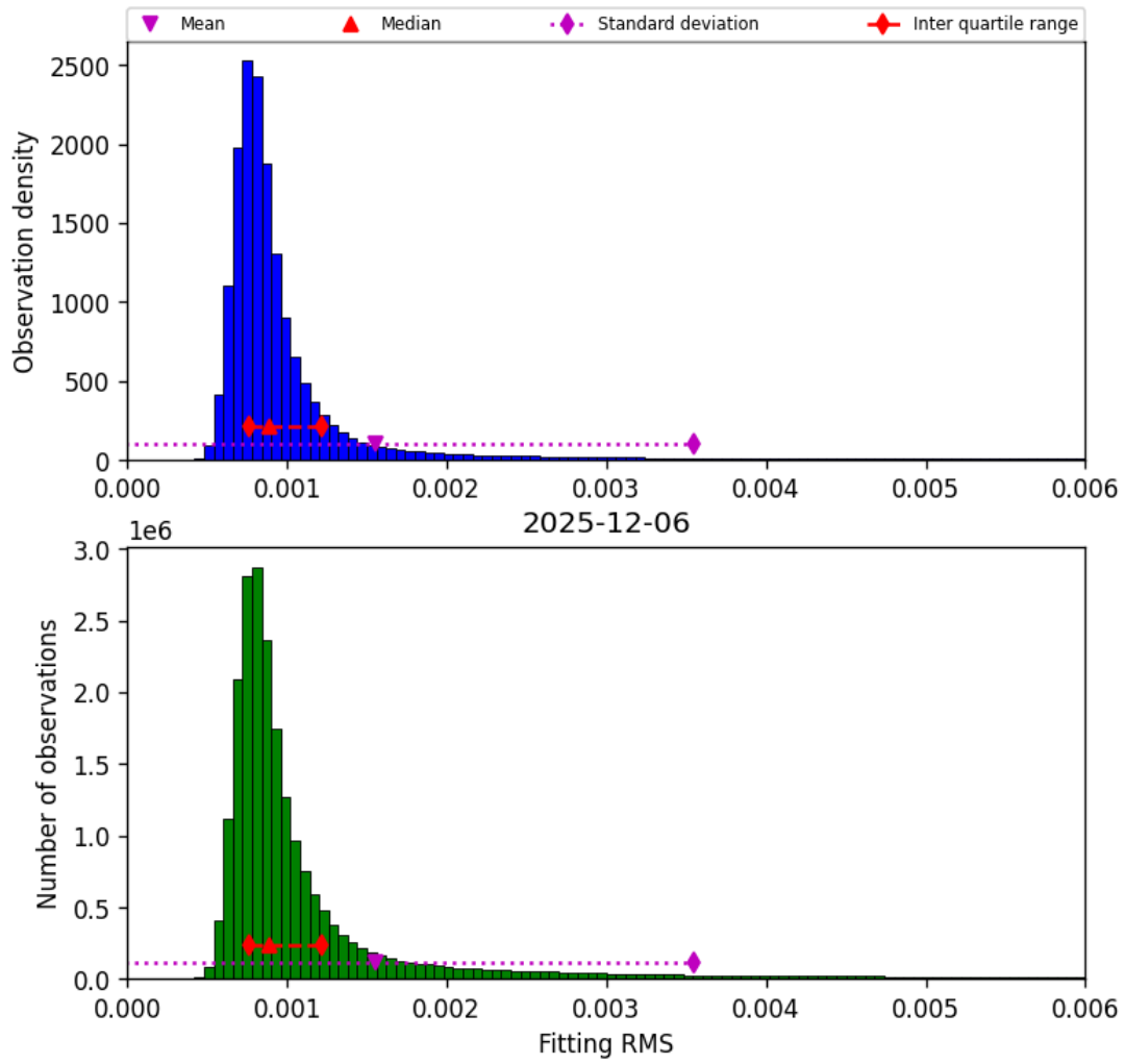
Figure 34: Histogram of “Fitting RMS” for 2025-12-06 to 2025-12-07
