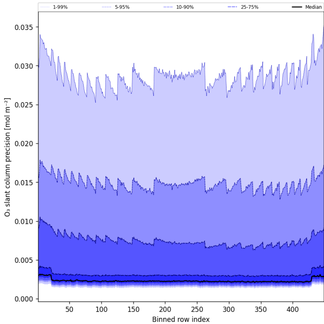
Figure 44: Along track statistics of “O 3 slant column precision” for 2025-12-06 to 2025-12-07
