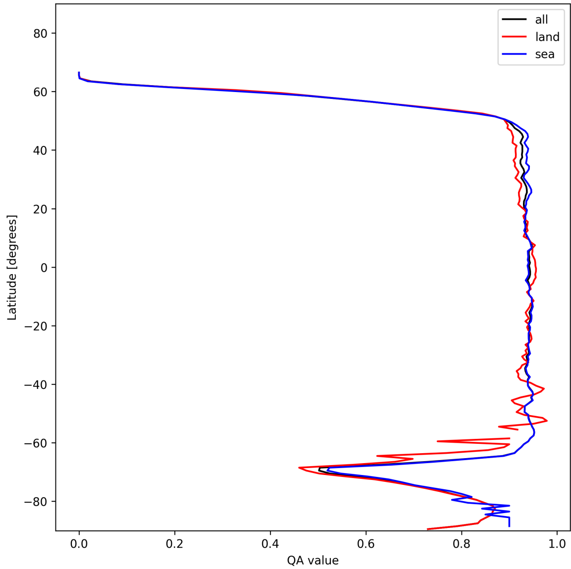
Figure 16: Zonal average of “QA value” for 2025-12-06 to 2025-12-07.
