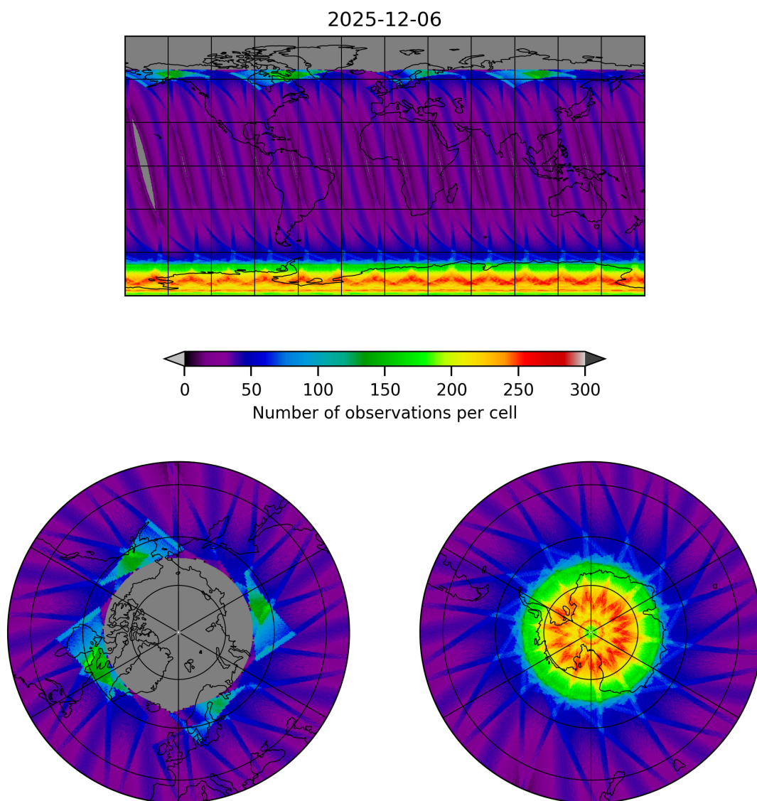
Figure 15: Map of the number of observations for 2025-12-06 to 2025-12-07
