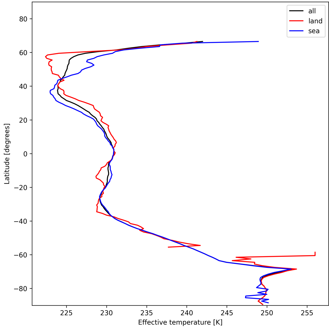
Figure 26: Zonal average of "Effective temperature" for 2025-12-06 to 2025-12-07.
