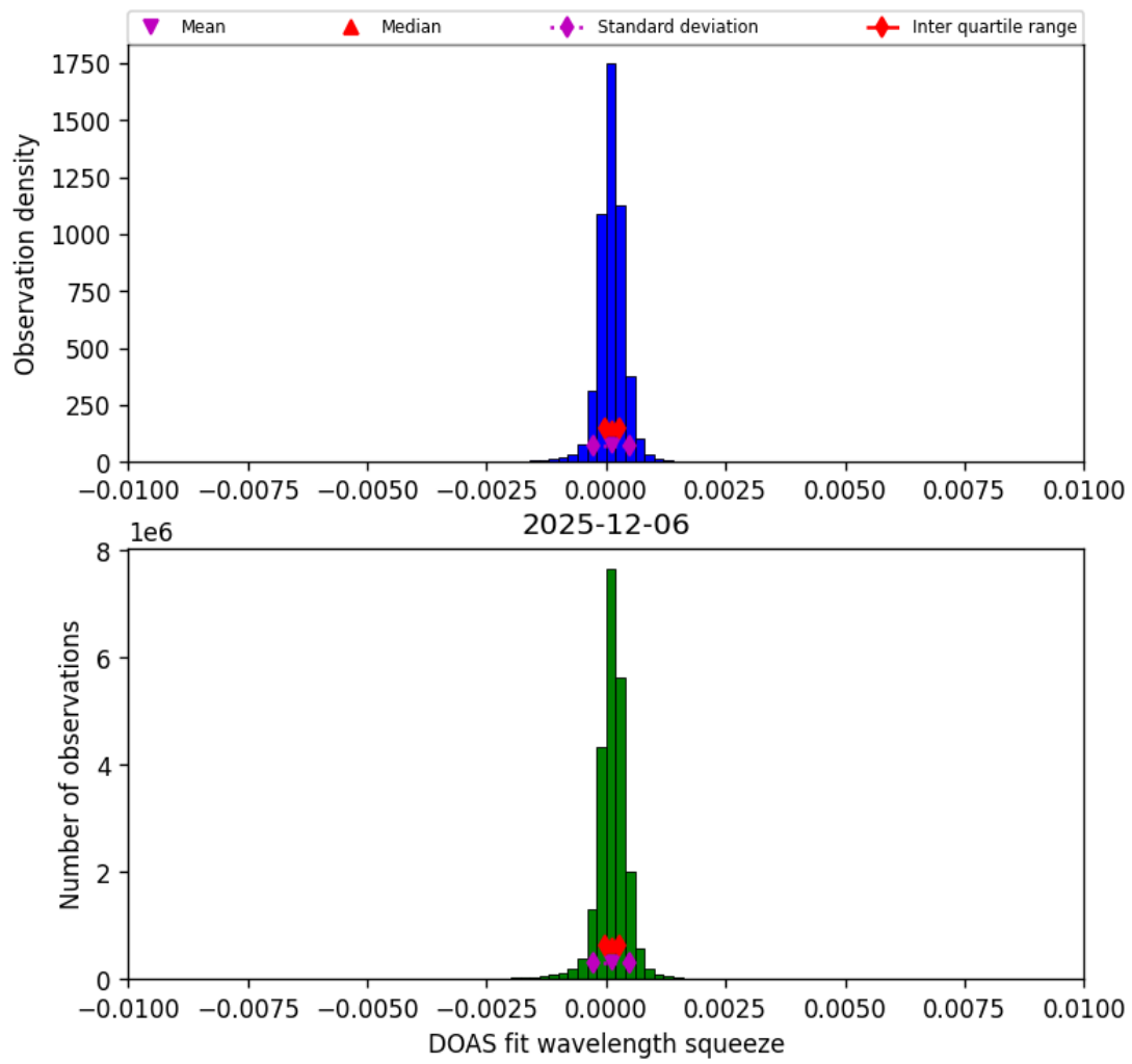
Figure 36: Histogram of “DOAS fit wavelength squeeze” for 2025-12-06 to 2025-12-07
