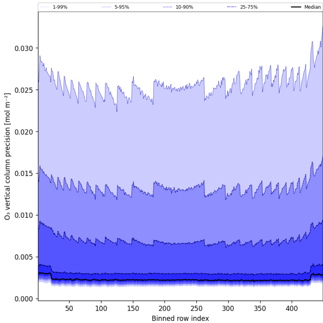
Figure 42: Along track statistics of “O 3 vertical column precision” for 2025-12-07 to 2025-12-07
