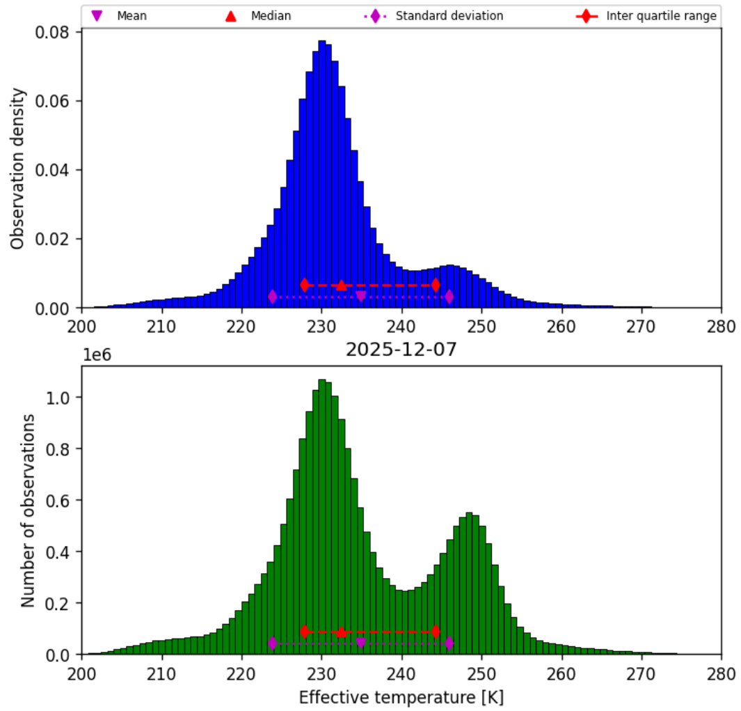
Figure 38: Histogram of “Effective temperature” for 2025-12-07 to 2025-12-07
