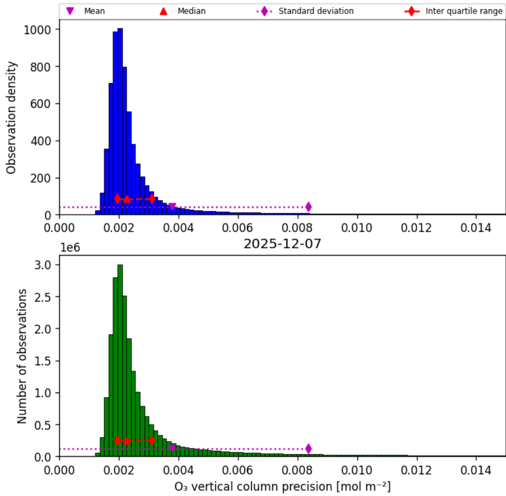
Figure 30: Histogram of “O 3 vertical column precision” for 2025-12-07 to 2025-12-07
