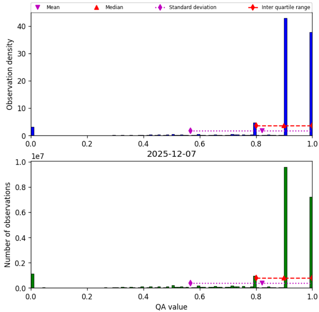
Figure 28: Histogram of “QA value” for 2025-12-07 to 2025-12-07
