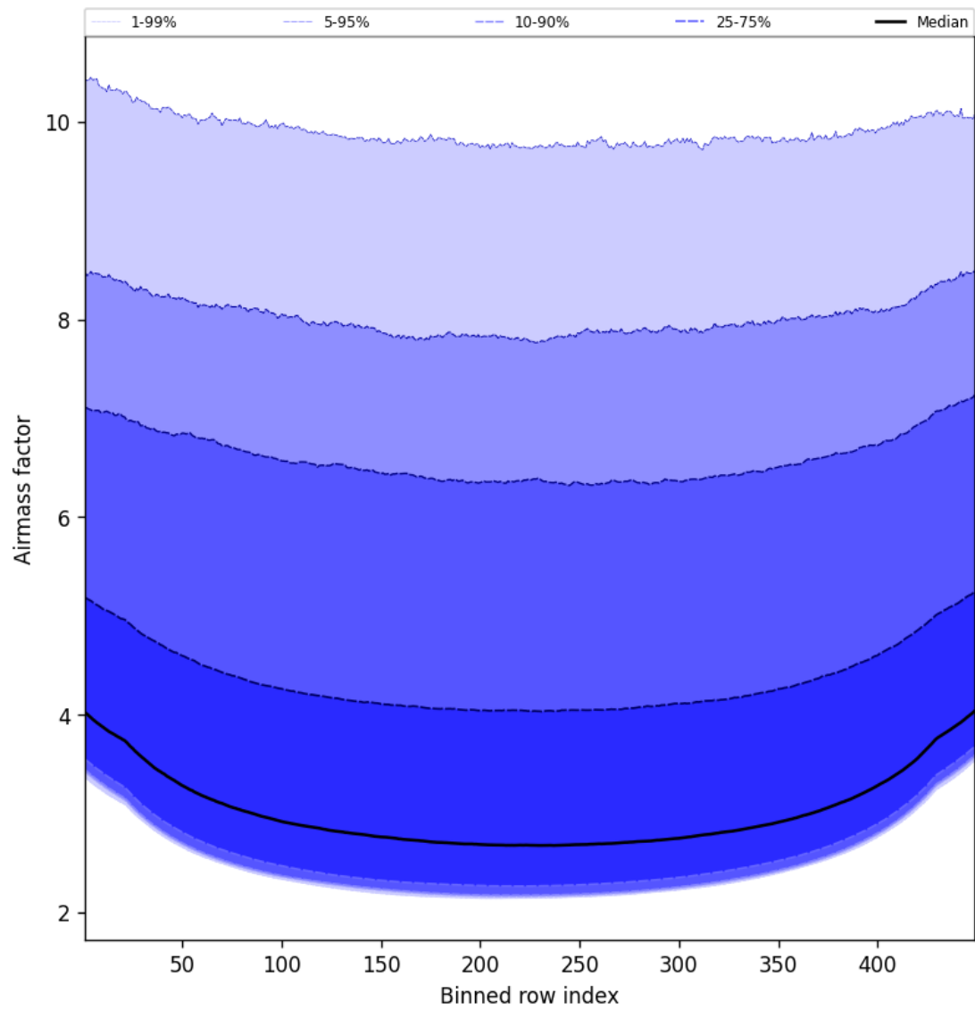
Figure 49: Along track statistics of “Airmass factor” for 2025-12-07 to 2025-12-07
