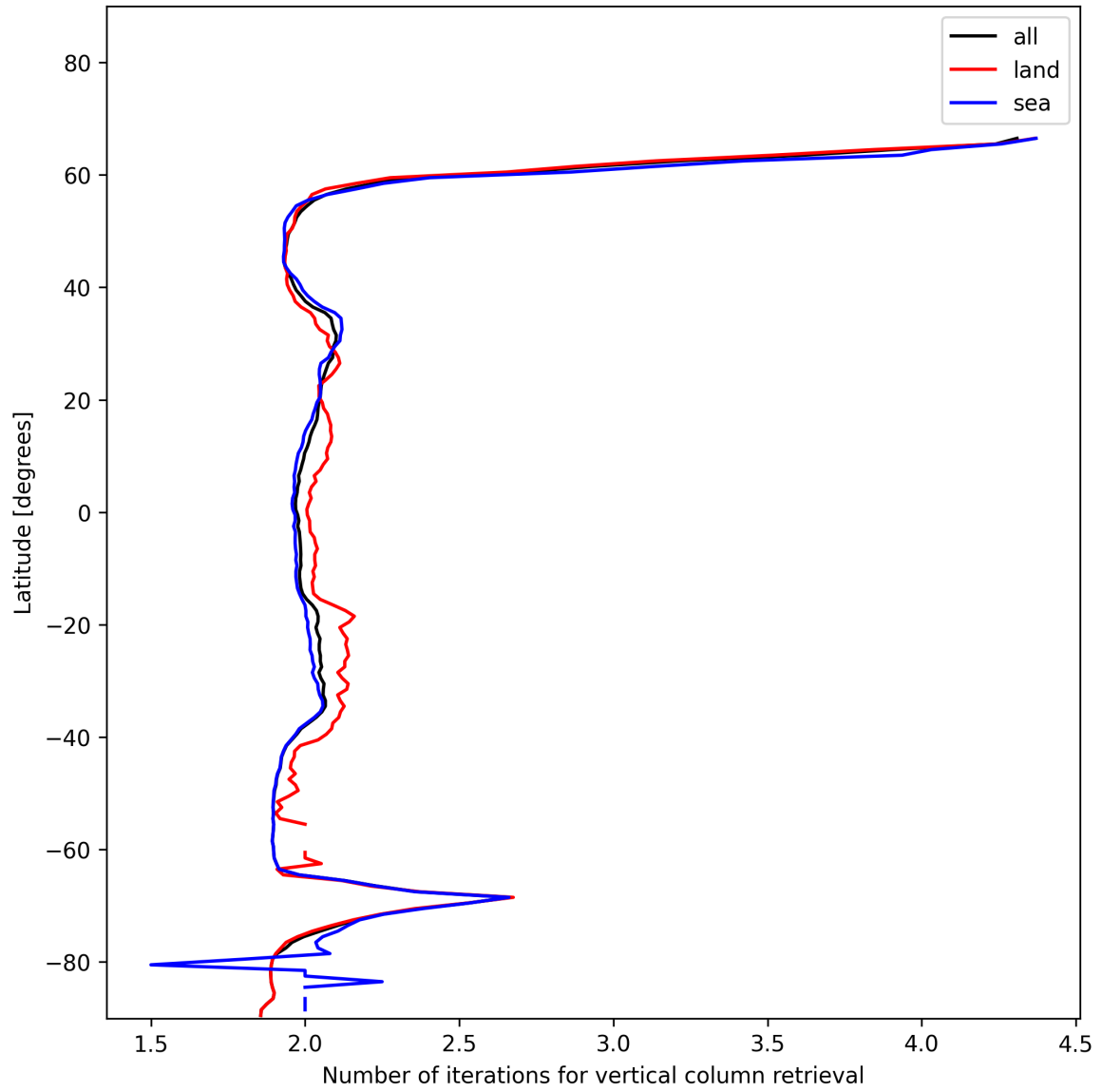
Figure 27: Zonal average of “Number of iterations for vertical column retrieval” for 2025-12-07 to 2025-12-07.
