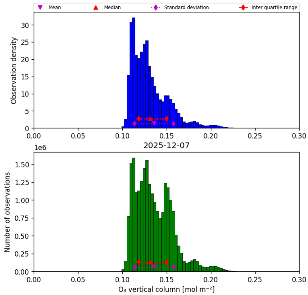
Figure 29: Histogram of “O 3 vertical column” for 2025-12-07 to 2025-12-07
