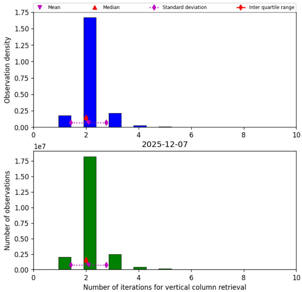
Figure 39: Histogram of “Number of iterations for vertical column retrieval” for 2025-12-07 to 2025-12-07
