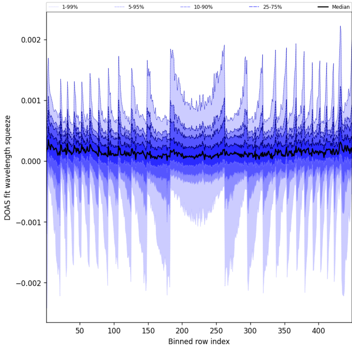
Figure 48: Along track statistics of “DOAS fit wavelength squeeze” for 2025-12-07 to 2025-12-07
