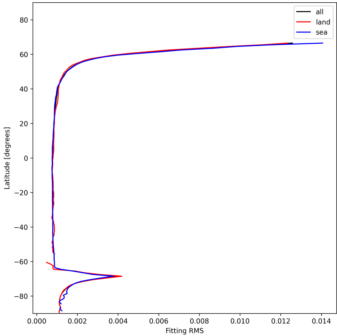
Figure 22: Zonal average of “Fitting RMS” for 2025-12-07 to 2025-12-07.
