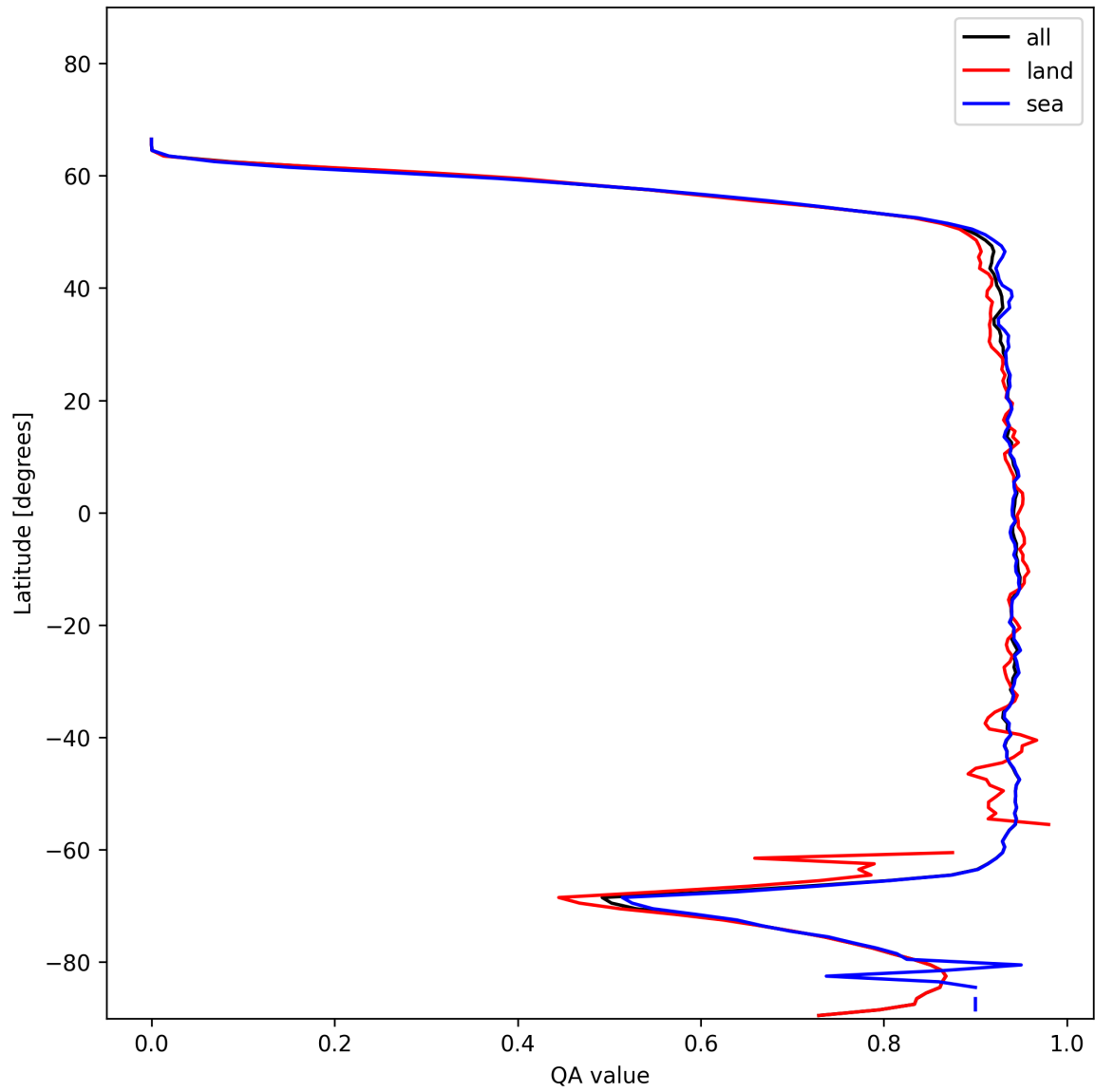
Figure 16: Zonal average of “QA value” for 2025-12-07 to 2025-12-07.
