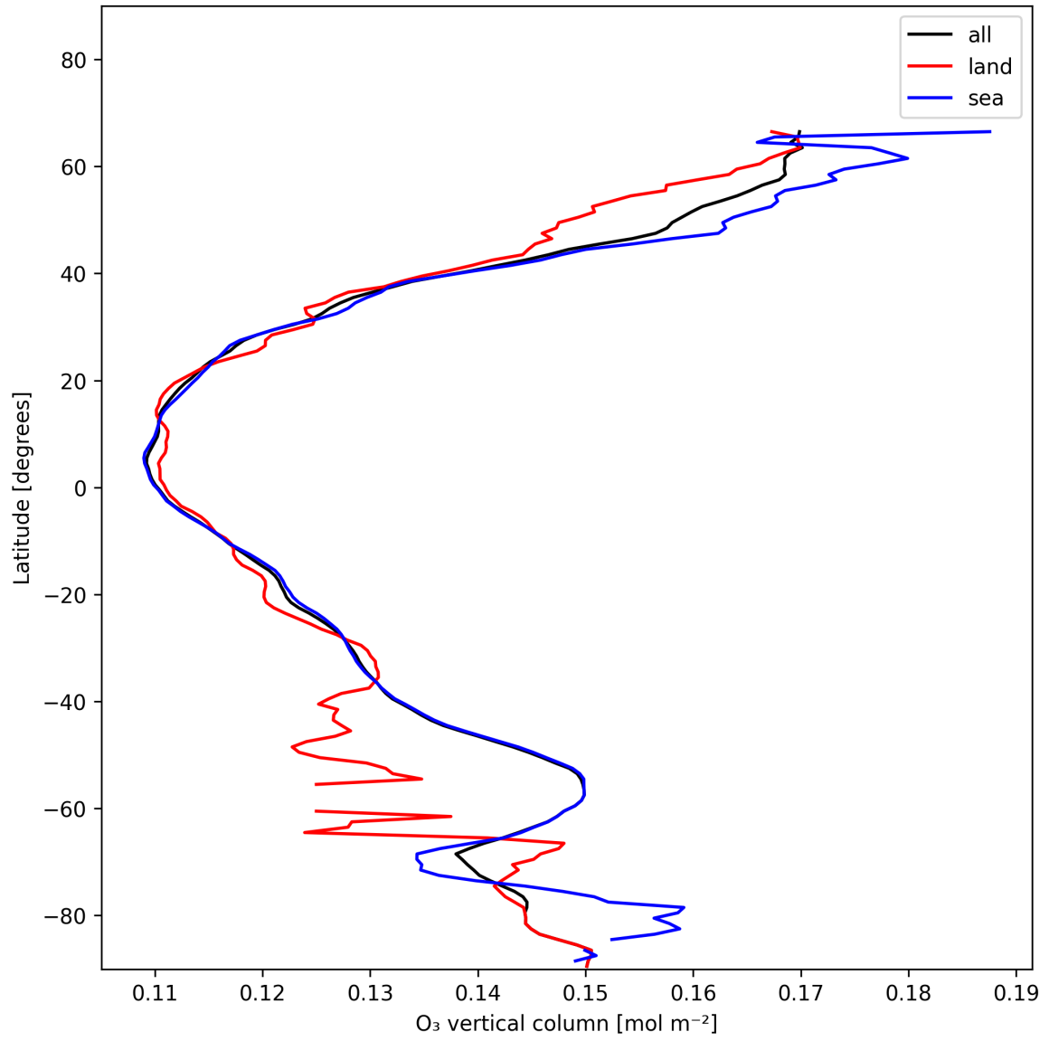
Figure 17: Zonal average of “O 3 vertical column” for 2025-12-07 to 2025-12-07.
