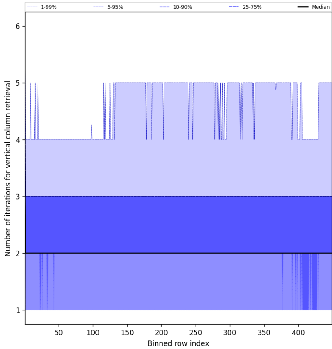
Figure 51: Along track statistics of “Number of iterations for vertical column retrieval” for 2025-12-07 to 2025-12-07
