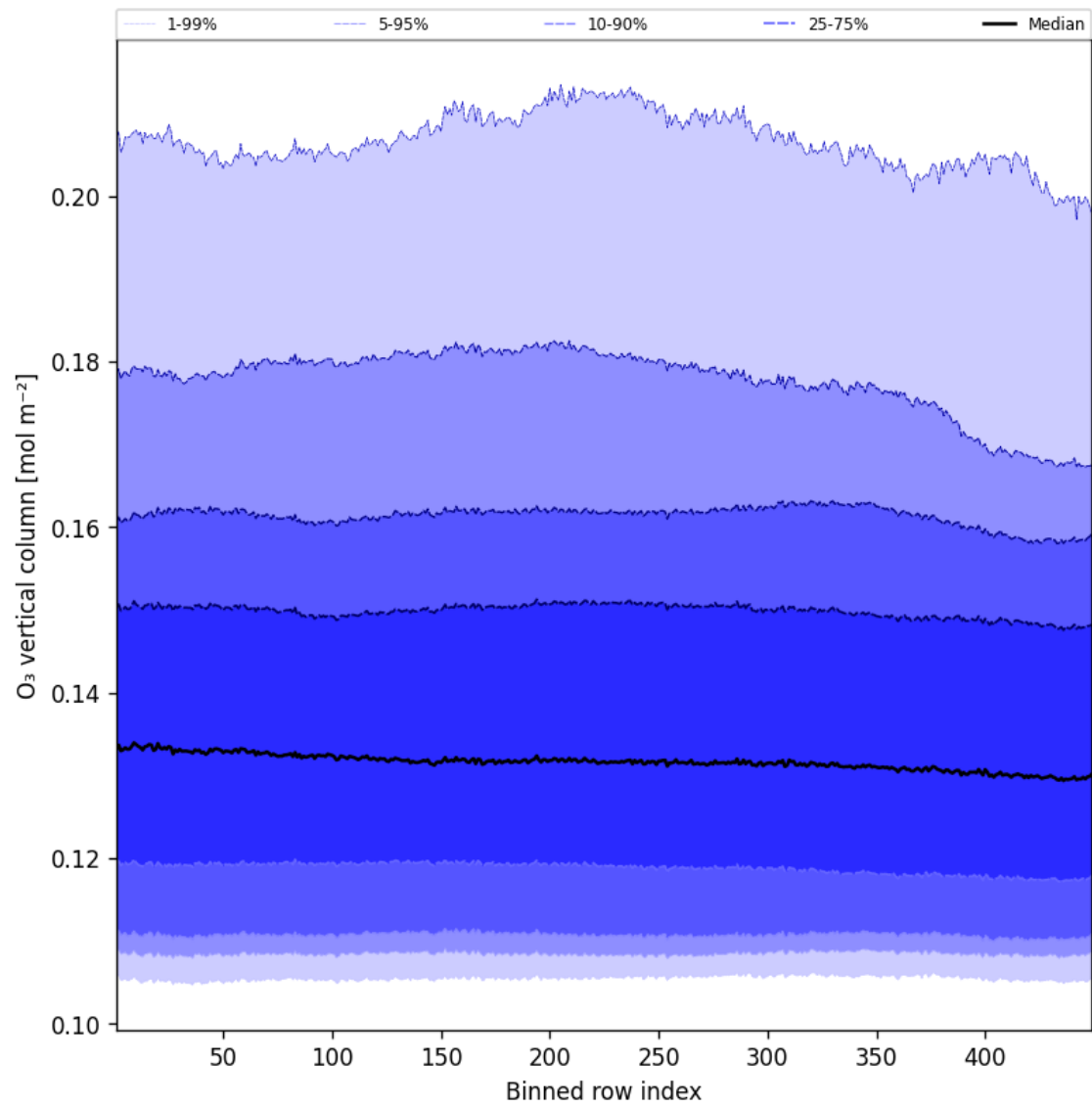
Figure 41: Along track statistics of “O 3 vertical column” for 2025-12-07 to 2025-12-07
