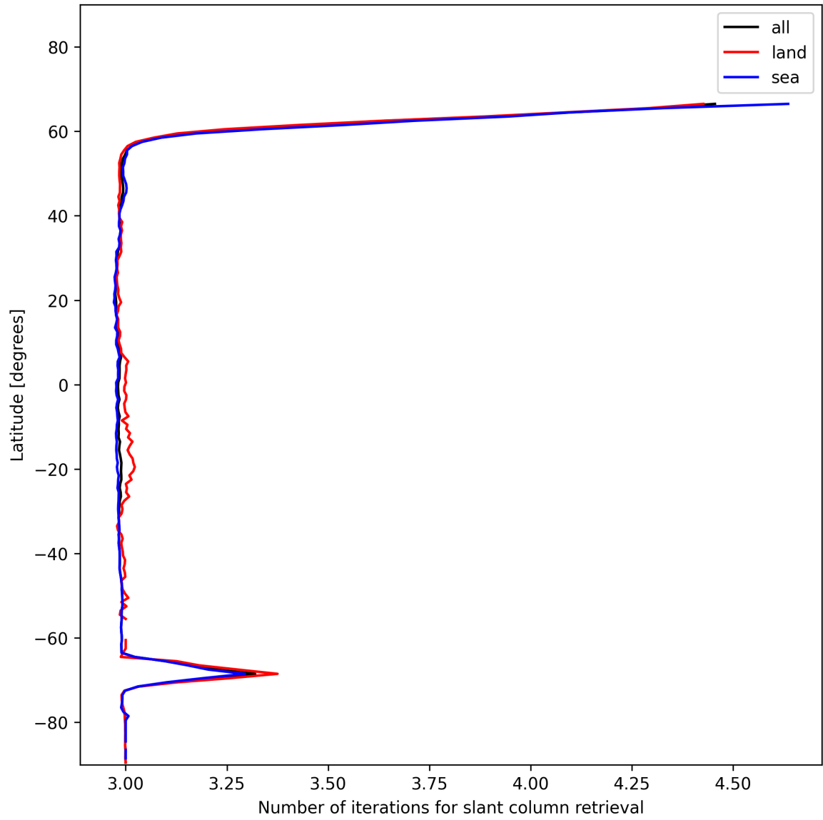
Figure 21: Zonal average of “Number of iterations for slant column retrieval” for 2025-12-07 to 2025-12-07.
