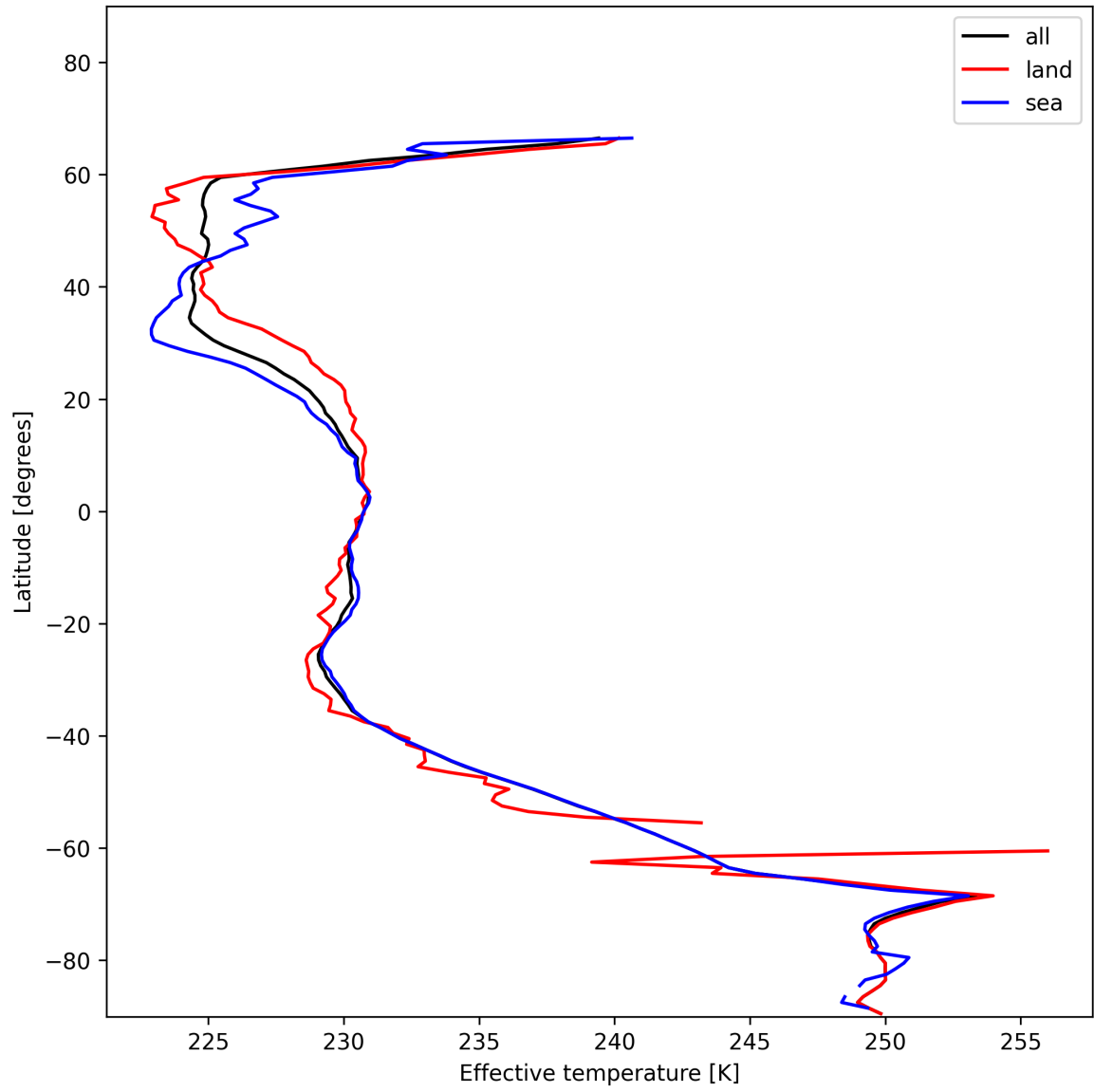
Figure 26: Zonal average of “Effective temperature” for 2025-12-07 to 2025-12-07.
