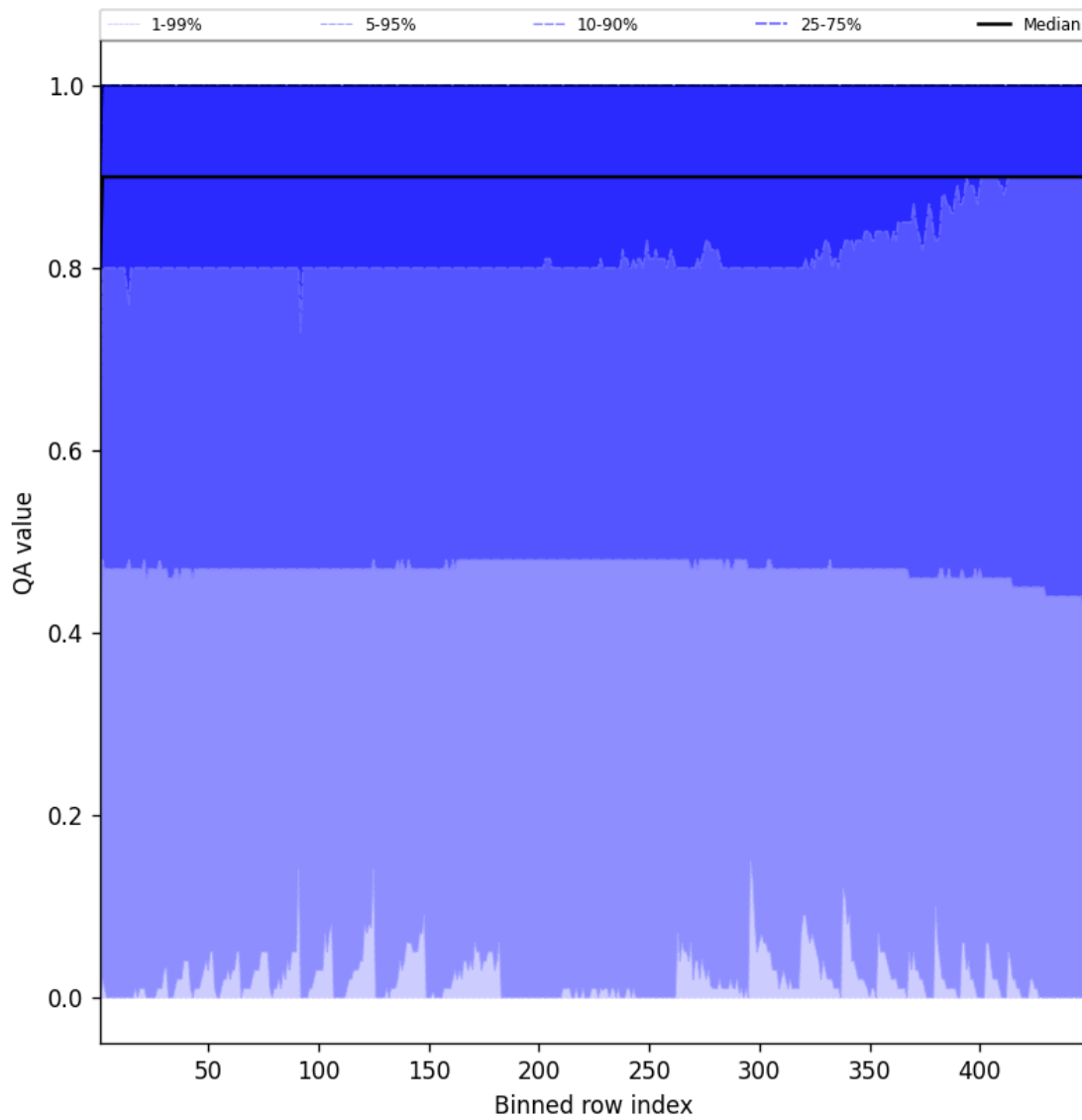
Figure 40: Along track statistics of “QA value” for 2025-12-07 to 2025-12-07
