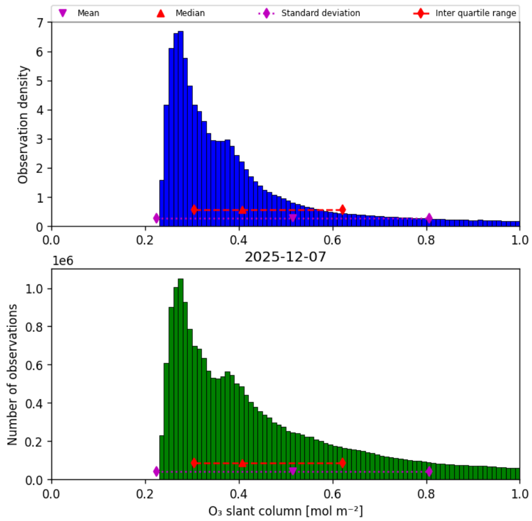
Figure 31: Histogram of “O 3 slant column” for 2025-12-07 to 2025-12-07
