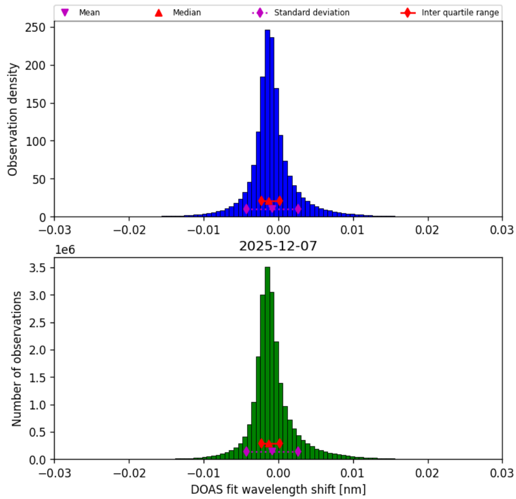
Figure 35: Histogram of “DOAS fit wavelength shift” for 2025-12-07 to 2025-12-07
