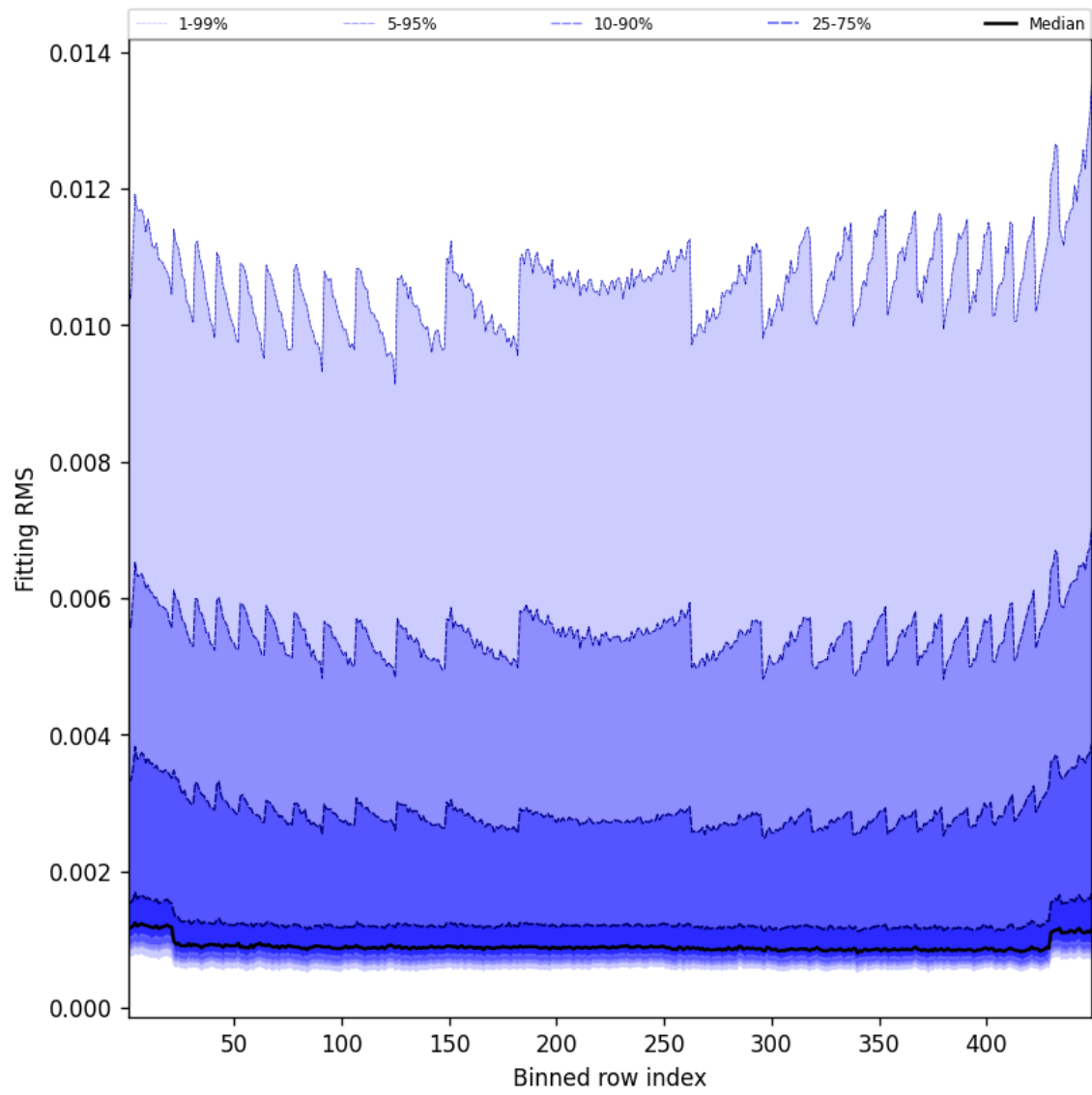
Figure 46: Along track statistics of “Fitting RMS” for 2025-12-07 to 2025-12-07
