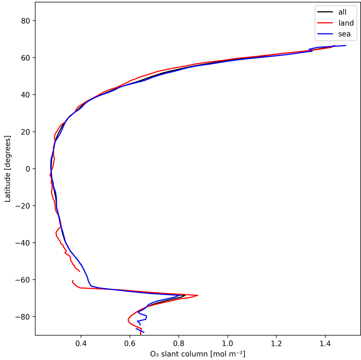
Figure 19: Zonal average of “O 3 slant column” for 2025-12-07 to 2025-12-07.
