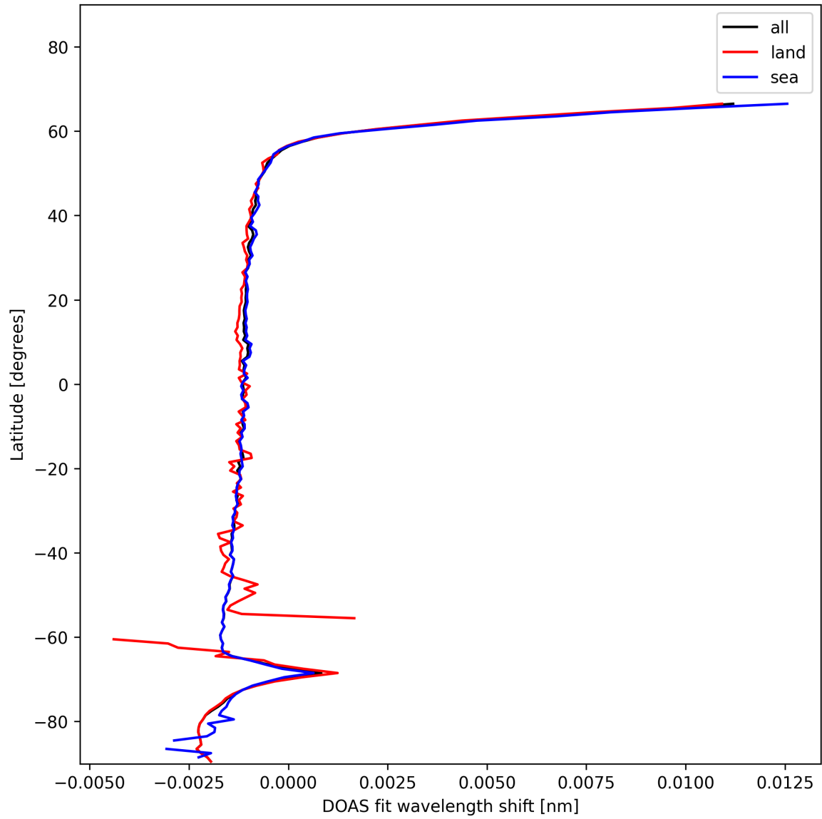
Figure 23: Zonal average of “DOAS fit wavelength shift” for 2025-12-07 to 2025-12-07.
