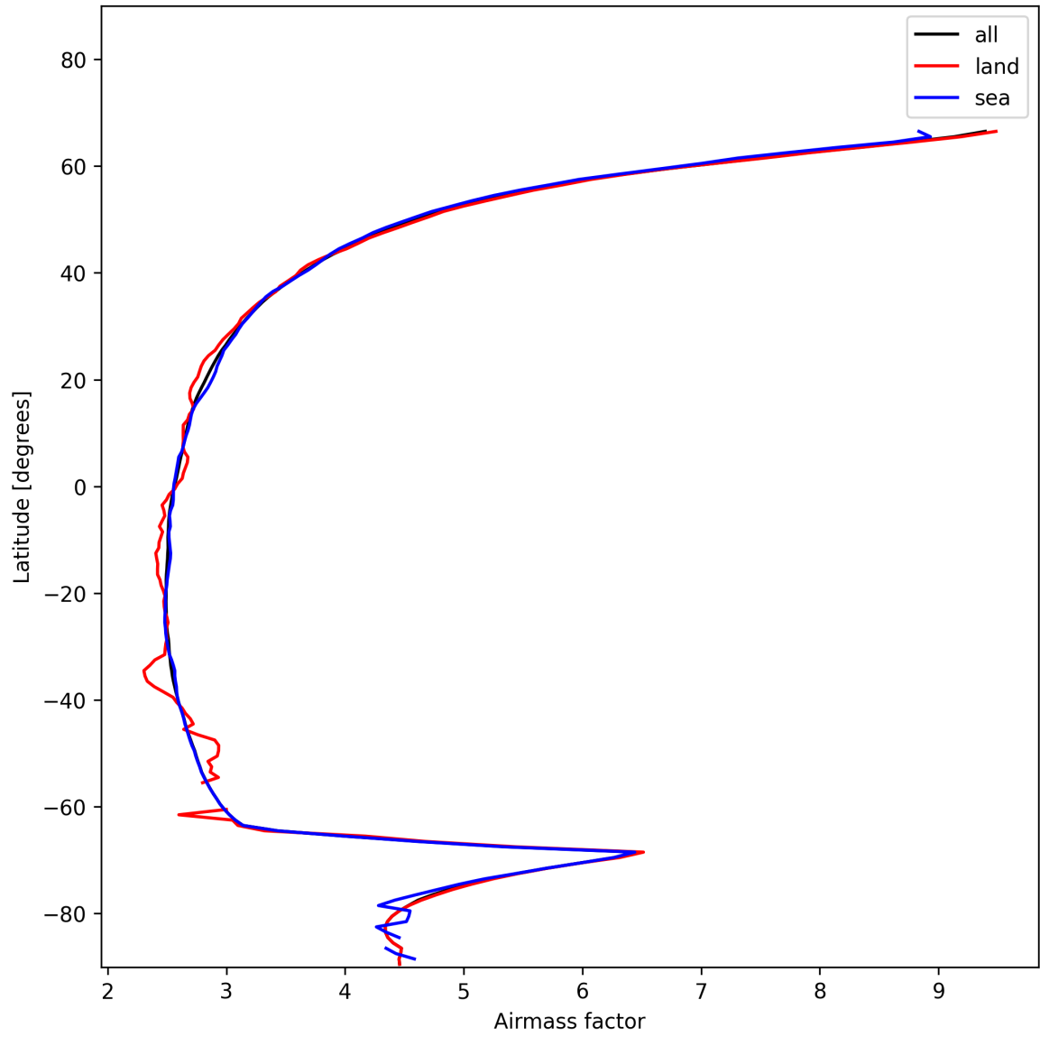
Figure 25: Zonal average of “Airmass factor” for 2025-12-07 to 2025-12-07.
