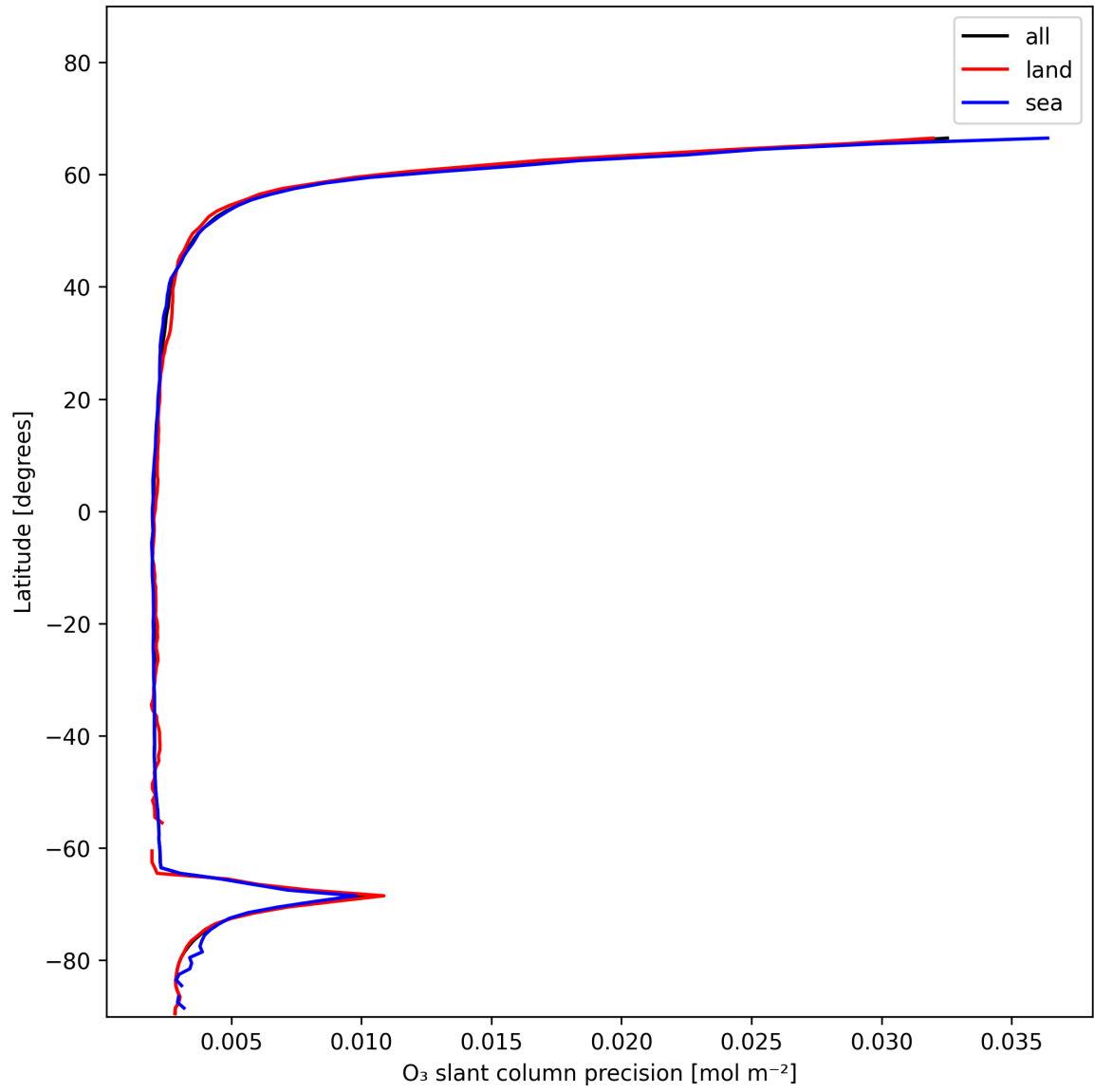
Figure 20: Zonal average of “O 3 slant column precision” for 2025-12-07 to 2025-12-07.
