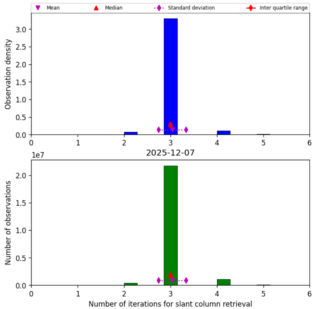
Figure 33: Histogram of "Number of iterations for slant column retrieval" for 2025-12-07 to 2025-12-07
