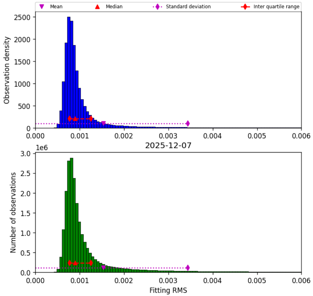
Figure 34: Histogram of “Fitting RMS” for 2025-12-07 to 2025-12-07
