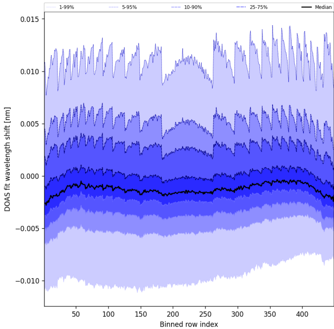
Figure 47: Along track statistics of “DOAS fit wavelength shift” for 2025-12-07 to 2025-12-07
