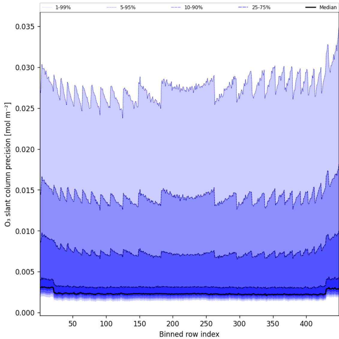
Figure 44: Along track statistics of “O 3 slant column precision” for 2025-12-07 to 2025-12-07
