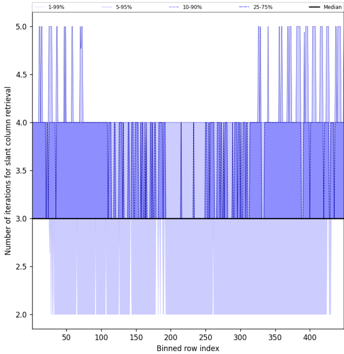
Figure 45: Along track statistics of “Number of iterations for slant column retrieval” for 2025-12-07 to 2025-12-07
