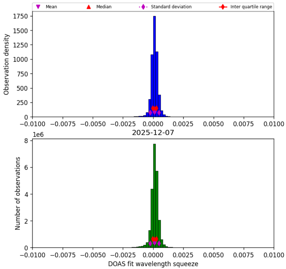
Figure 36: Histogram of “DOAS fit wavelength squeeze” for 2025-12-07 to 2025-12-07
