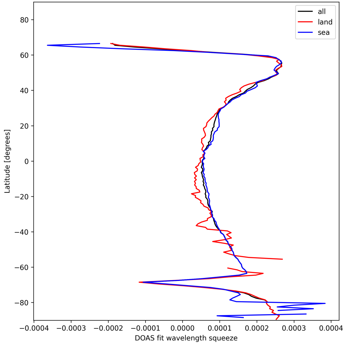
Figure 24: Zonal average of “DOAS fit wavelength squeeze” for 2025-12-07 to 2025-12-07.
