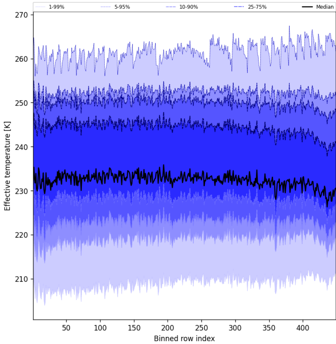
Figure 50: Along track statistics of “Effective temperature” for 2025-12-07 to 2025-12-07
