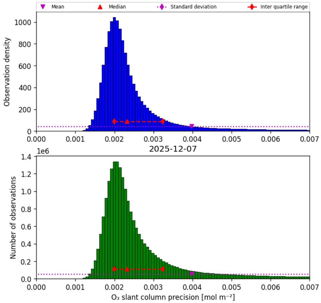
Figure 32: Histogram of “O 3 slant column precision” for 2025-12-07 to 2025-12-07
