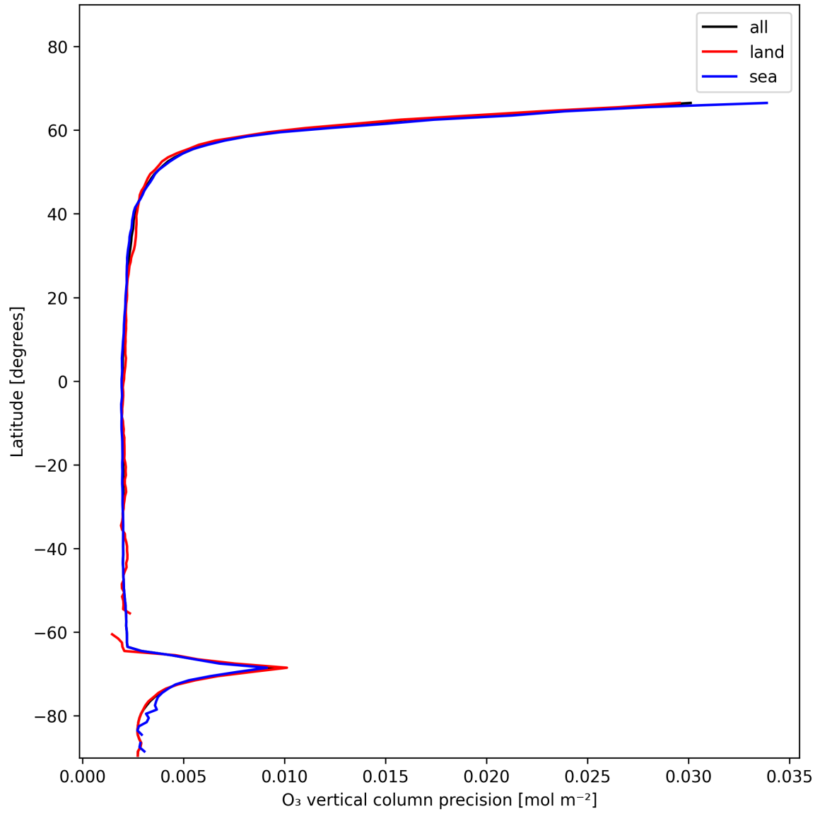
Figure 18: Zonal average of “O 3 vertical column precision” for 2025-12-07 to 2025-12-07.
