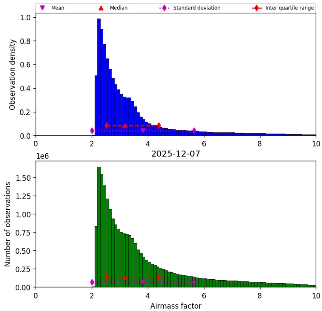
Figure 37: Histogram of "Airmass factor" for 2025-12-07 to 2025-12-07
