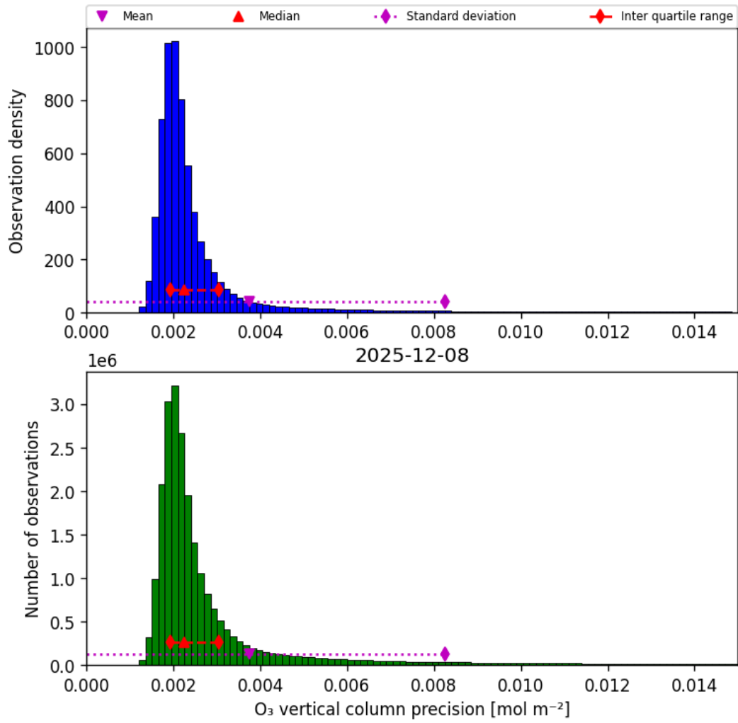
Figure 30: Histogram of “O 3 vertical column precision” for 2025-12-08 to 2025-12-09
