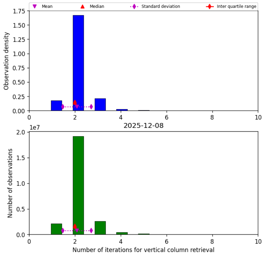
Figure 39: Histogram of “Number of iterations for vertical column retrieval” for 2025-12-08 to 2025-12-09
