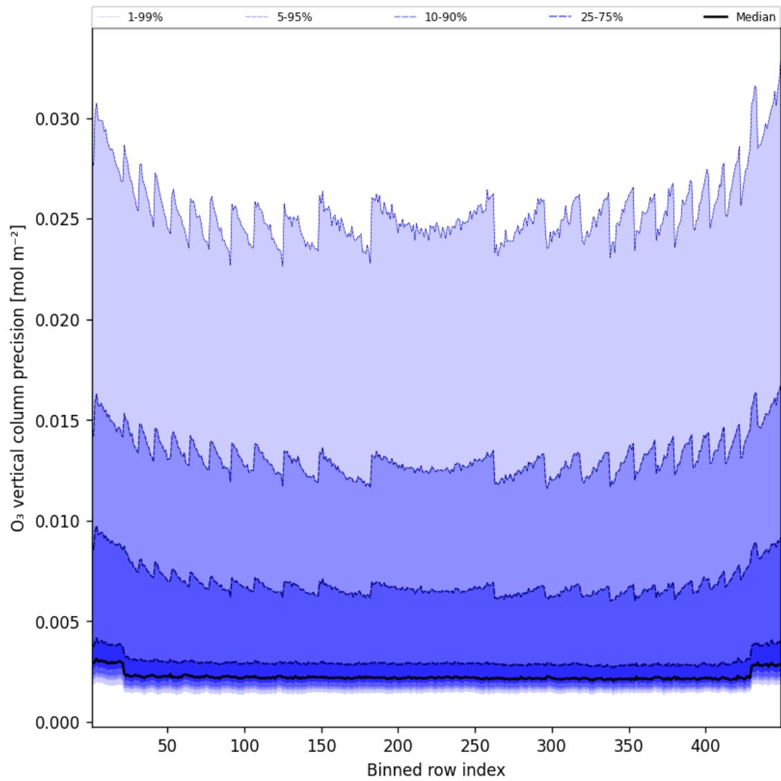
Figure 42: Along track statistics of “O 3 vertical column precision” for 2025-12-08 to 2025-12-09
