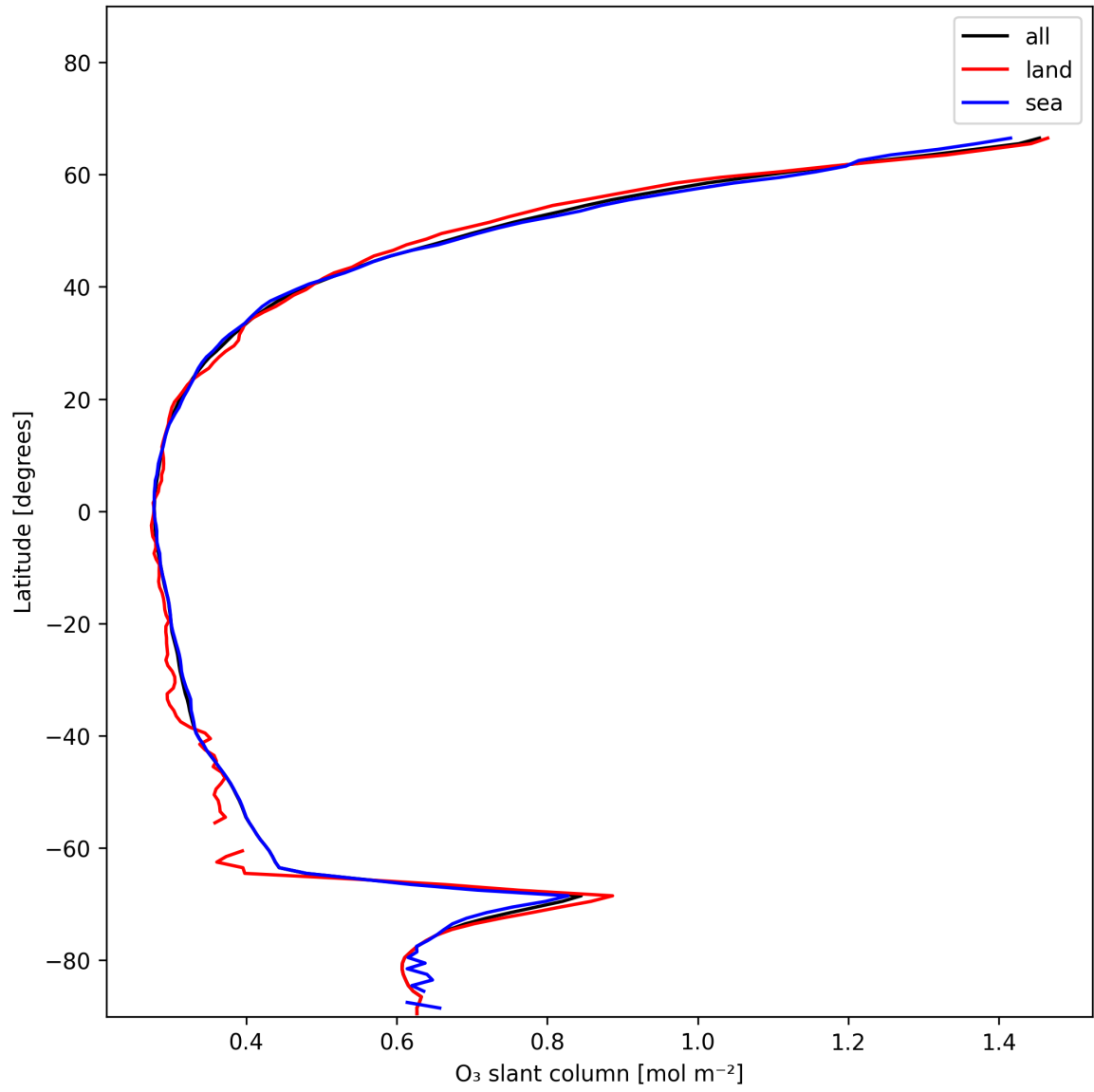
Figure 19: Zonal average of “O 3 slant column” for 2025-12-08 to 2025-12-09.
