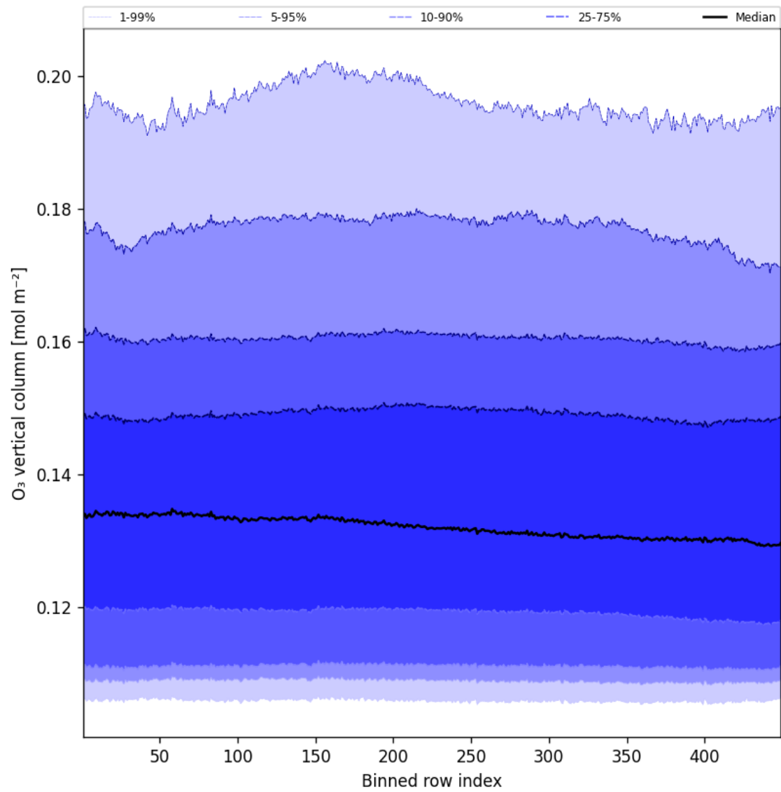
Figure 41: Along track statistics of “O 3 vertical column” for 2025-12-08 to 2025-12-09
