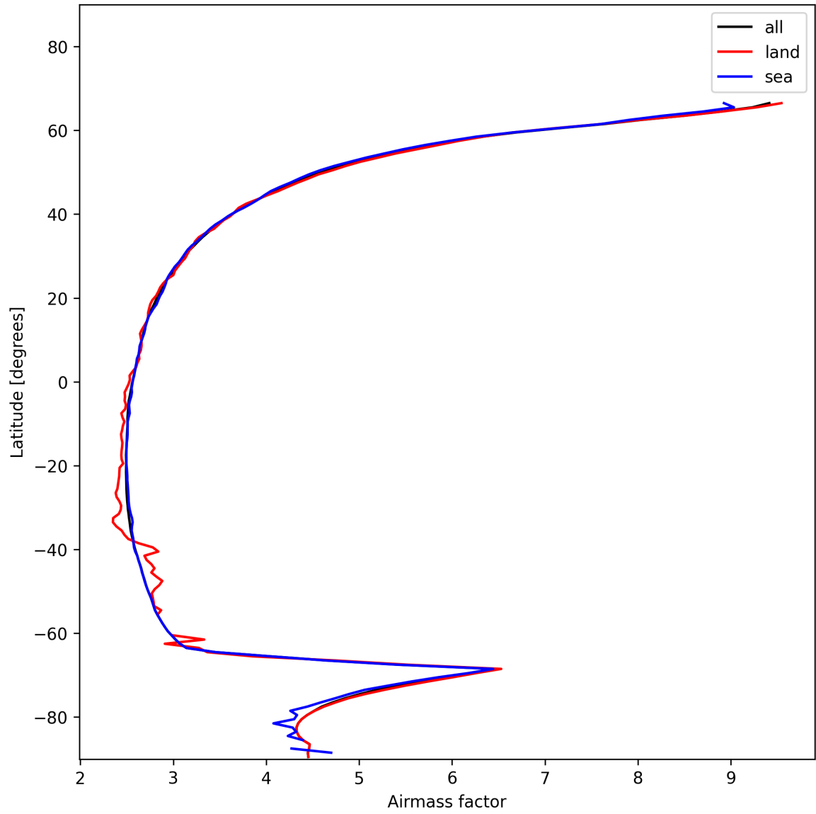
Figure 25: Zonal average of “Airmass factor” for 2025-12-08 to 2025-12-09.
