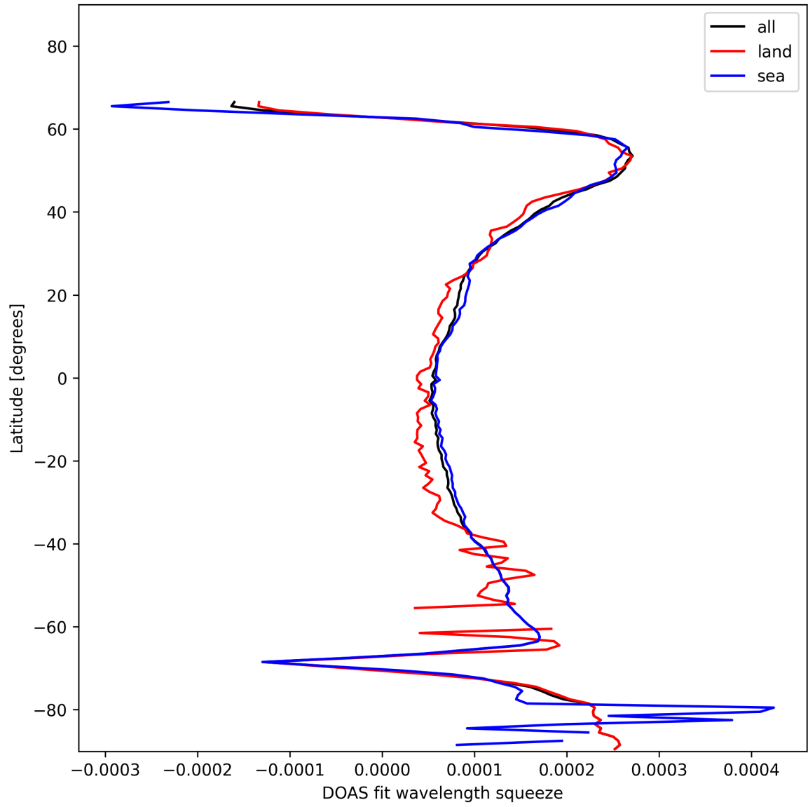
Figure 24: Zonal average of “DOAS fit wavelength squeeze” for 2025-12-08 to 2025-12-09.
