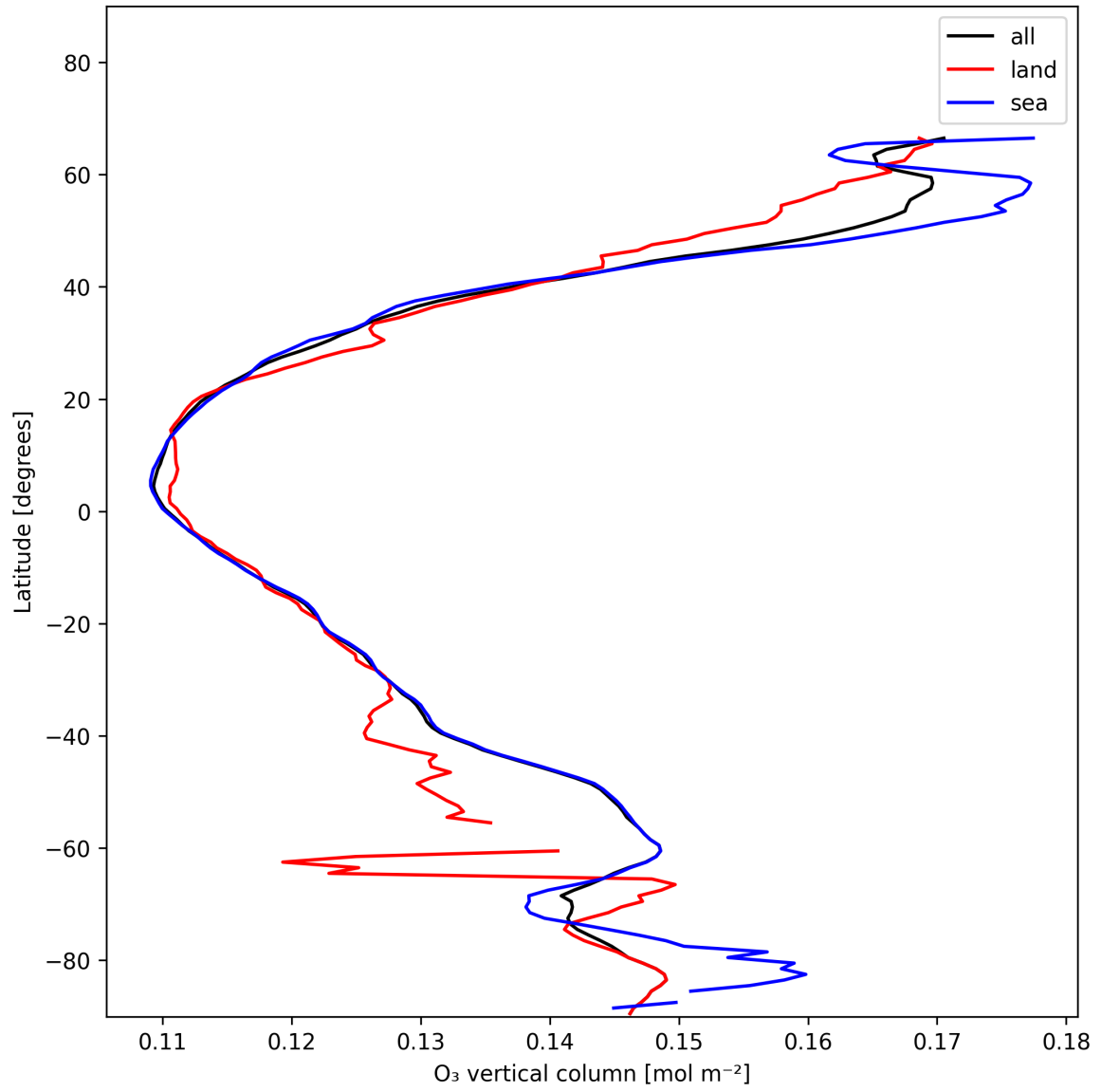
Figure 17: Zonal average of “O 3 vertical column” for 2025-12-08 to 2025-12-09.
