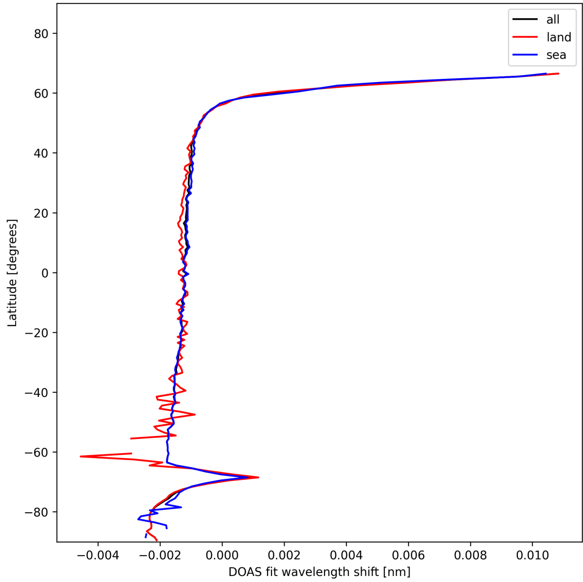
Figure 23: Zonal average of "DOAS fit wavelength shift" for 2025-12-08 to 2025-12-09.
