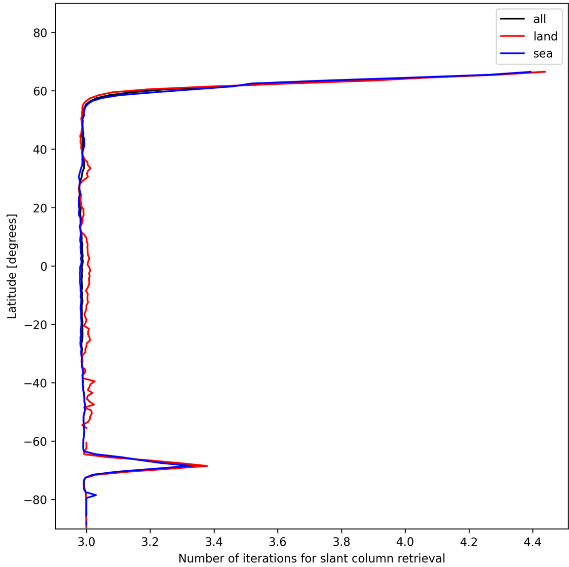
Figure 21: Zonal average of “Number of iterations for slant column retrieval” for 2025-12-08 to 2025-12-09.
