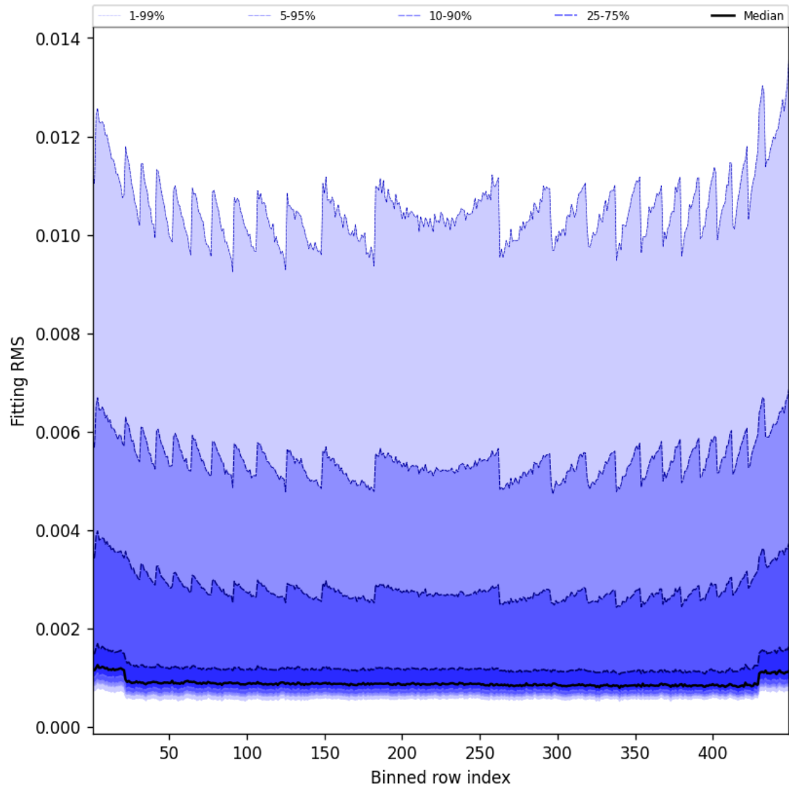
Figure 46: Along track statistics of “Fitting RMS” for 2025-12-08 to 2025-12-09
