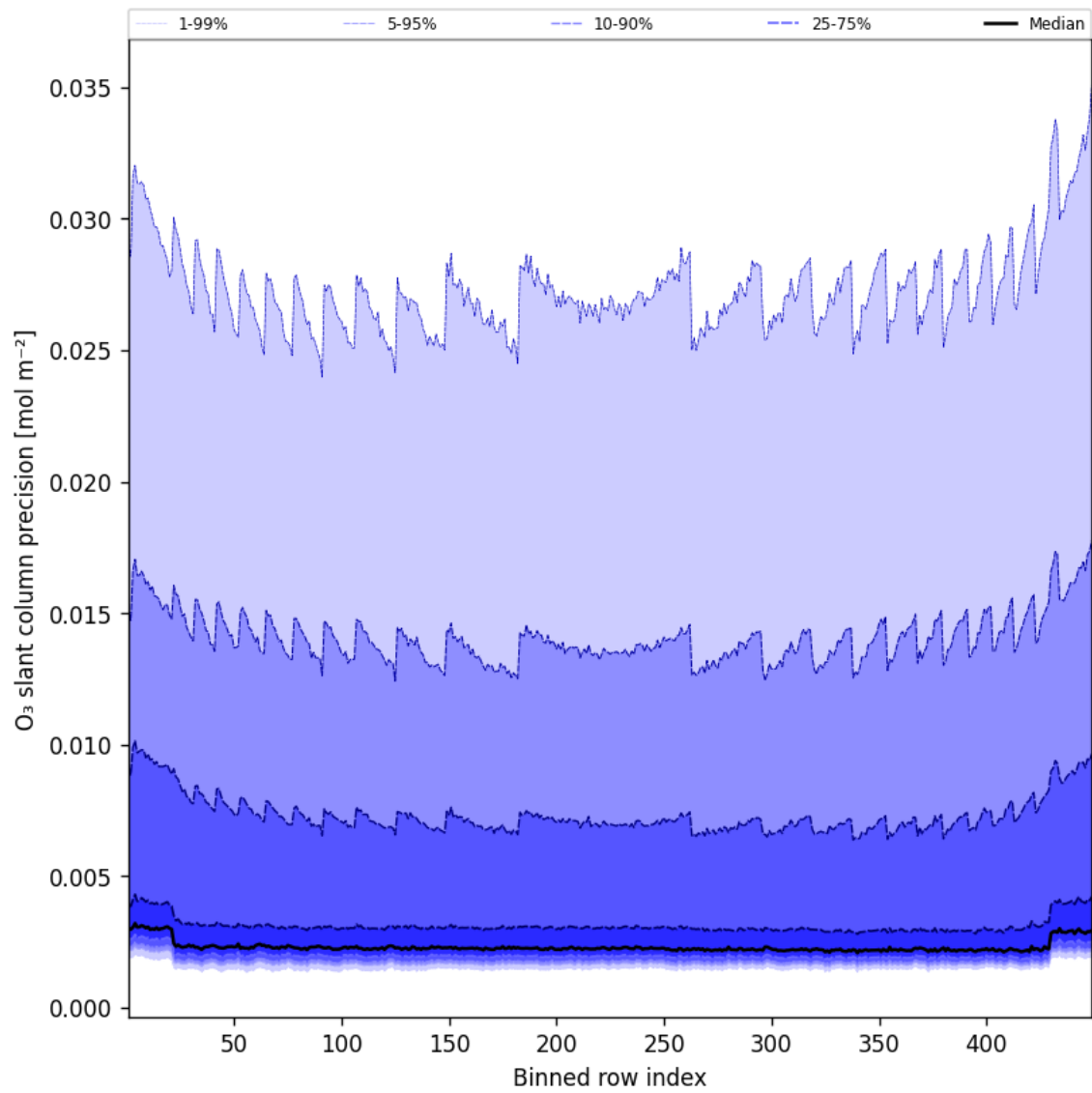
Figure 44: Along track statistics of “O 3 slant column precision” for 2025-12-08 to 2025-12-09
