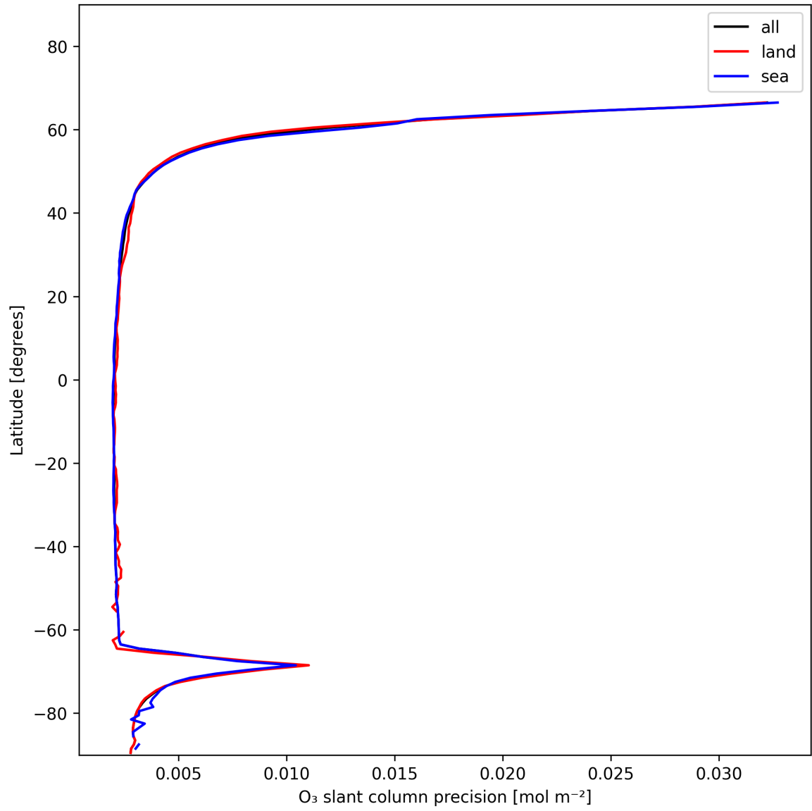
Figure 20: Zonal average of “O 3 slant column precision” for 2025-12-08 to 2025-12-09.
