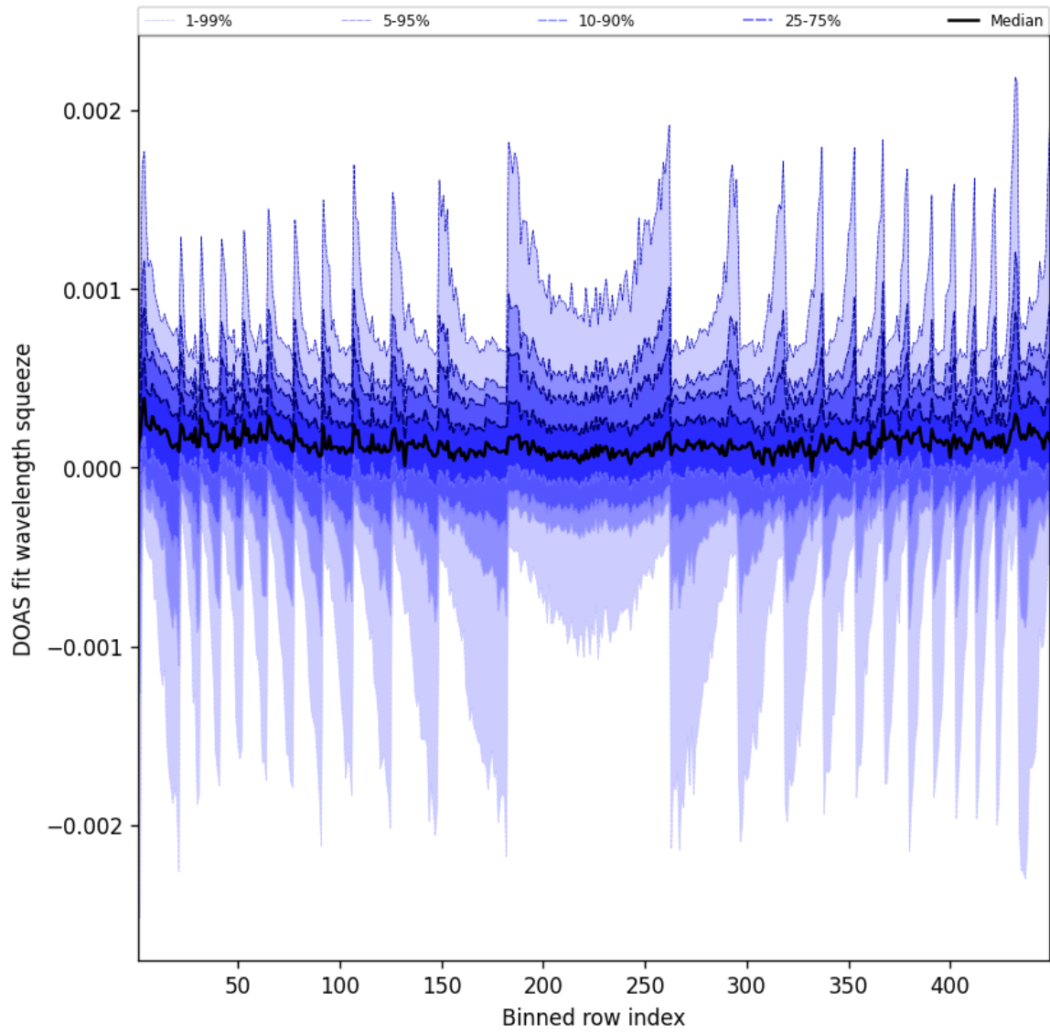
Figure 48: Along track statistics of “DOAS fit wavelength squeeze” for 2025-12-08 to 2025-12-09
