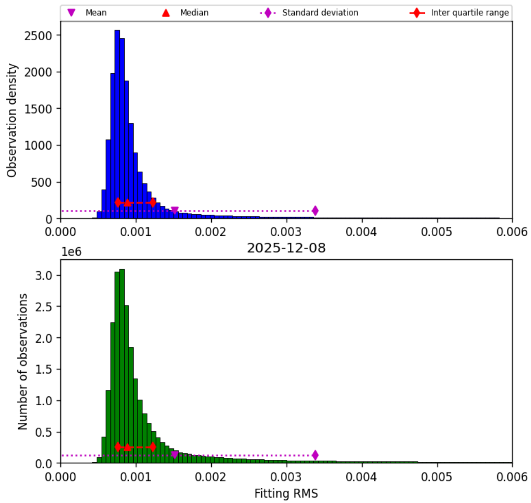
Figure 34: Histogram of “Fitting RMS” for 2025-12-08 to 2025-12-09
