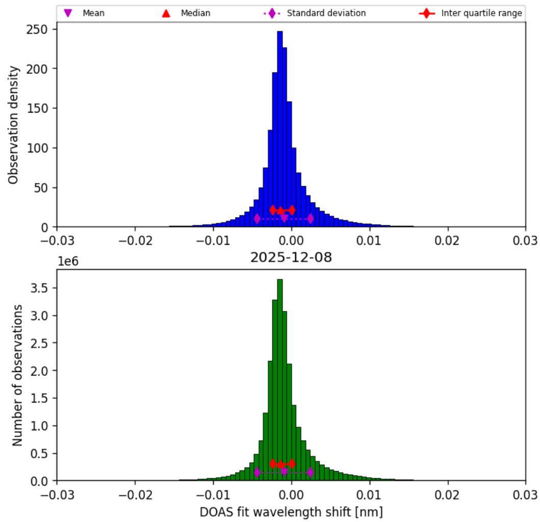
Figure 35: Histogram of “DOAS fit wavelength shift” for 2025-12-08 to 2025-12-09
