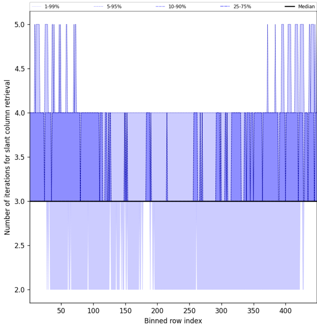
Figure 45: Along track statistics of “Number of iterations for slant column retrieval” for 2025-12-08 to 2025-12-09
