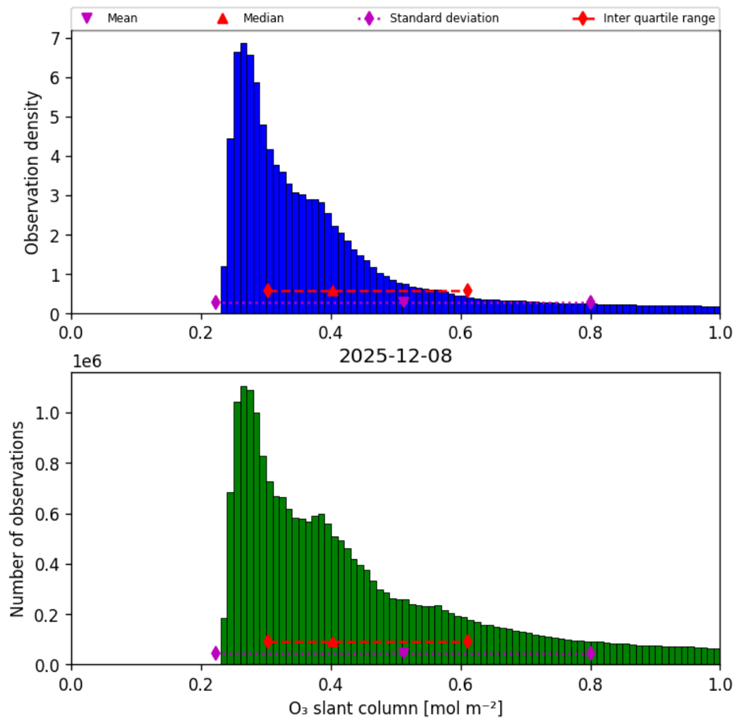
Figure 31: Histogram of “O 3 slant column” for 2025-12-08 to 2025-12-09
