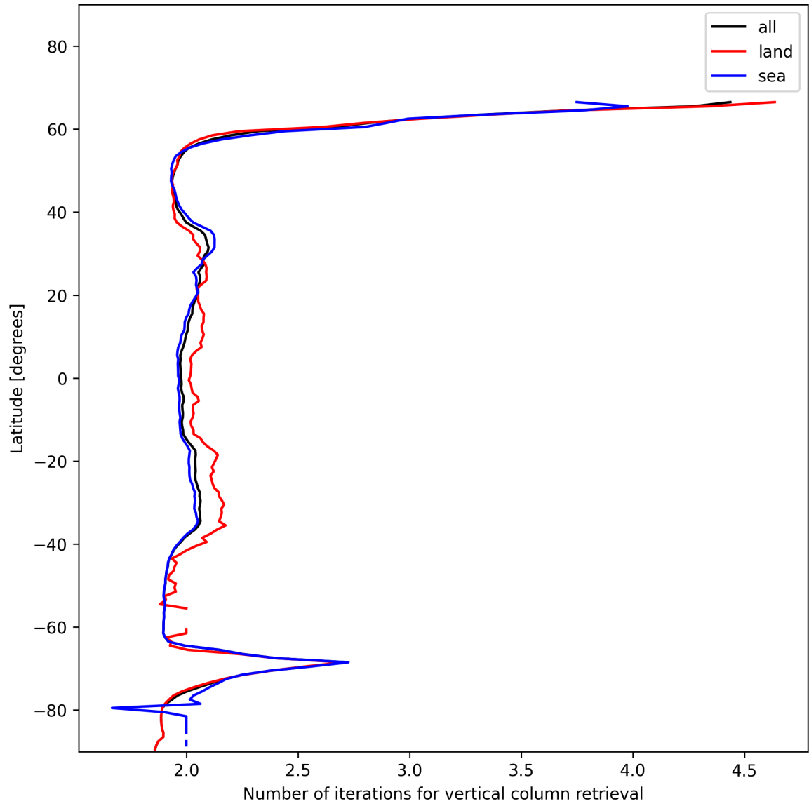
Figure 27: Zonal average of “Number of iterations for vertical column retrieval” for 2025-12-08 to 2025-12-09.
