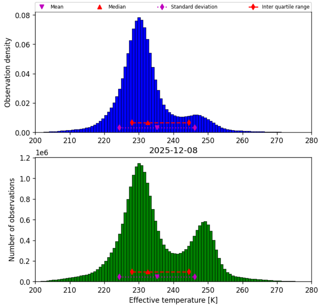
Figure 38: Histogram of “Effective temperature” for 2025-12-08 to 2025-12-09
