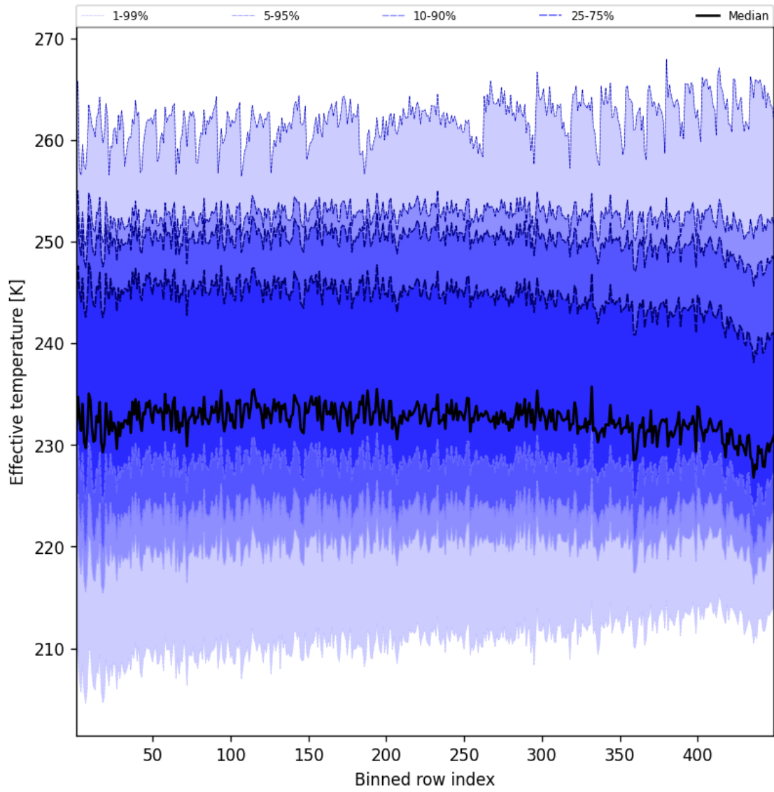
Figure 50: Along track statistics of “Effective temperature” for 2025-12-08 to 2025-12-09
