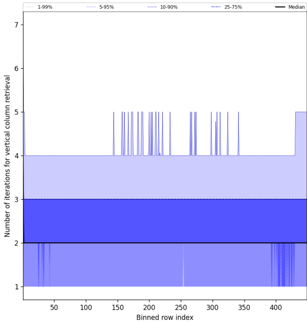
Figure 51: Along track statistics of “Number of iterations for vertical column retrieval” for 2025-12-08 to 2025-12-09
