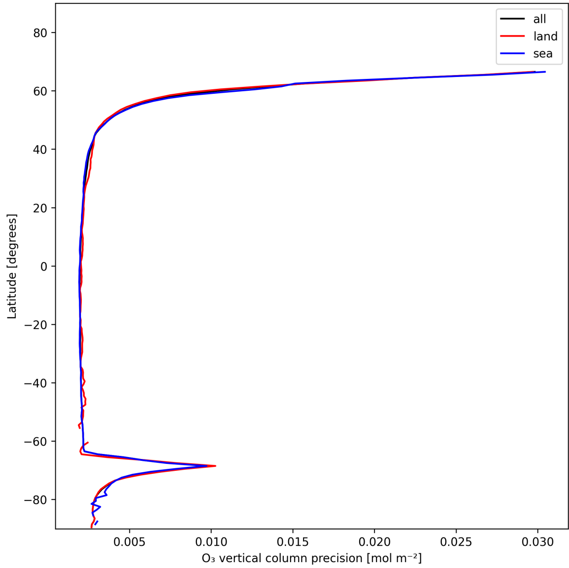
Figure 18: Zonal average of “O 3 vertical column precision” for 2025-12-08 to 2025-12-09.
