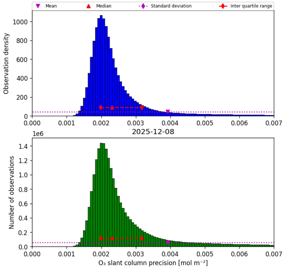
Figure 32: Histogram of “O 3 slant column precision” for 2025-12-08 to 2025-12-09
