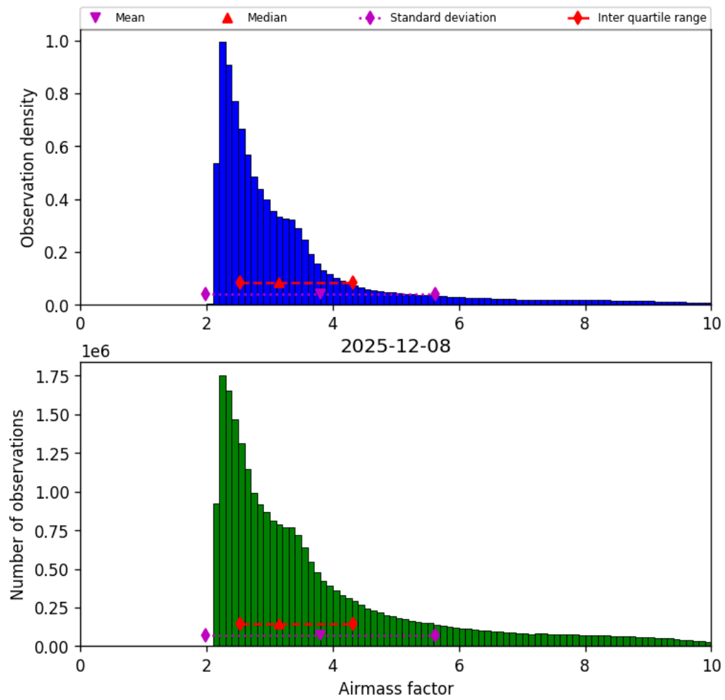
Figure 37: Histogram of “Airmass factor” for 2025-12-08 to 2025-12-09
