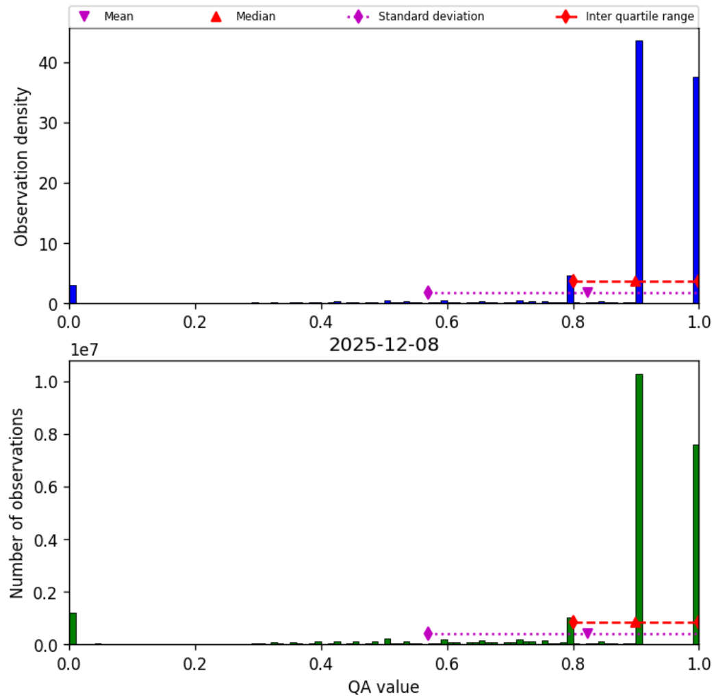
Figure 28: Histogram of “QA value” for 2025-12-08 to 2025-12-09
