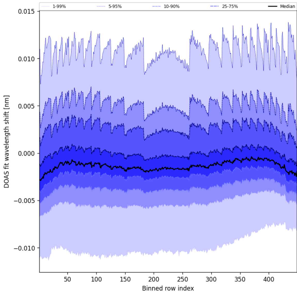
Figure 47: Along track statistics of "DOAS fit wavelength shift" for 2025-12-08 to 2025-12-09
