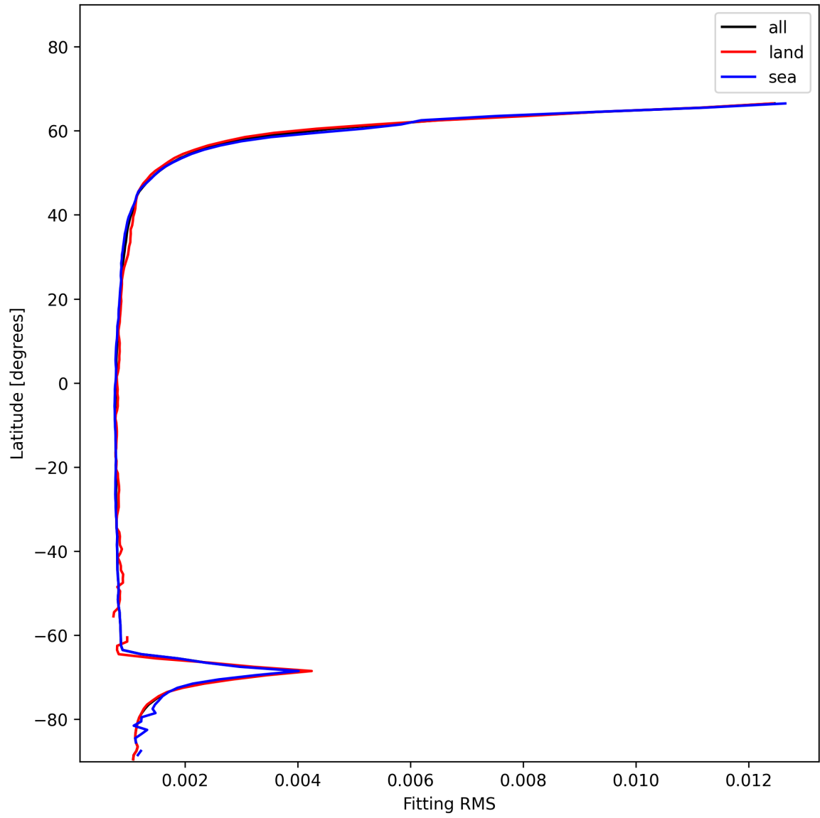
Figure 22: Zonal average of “Fitting RMS” for 2025-12-08 to 2025-12-09.
