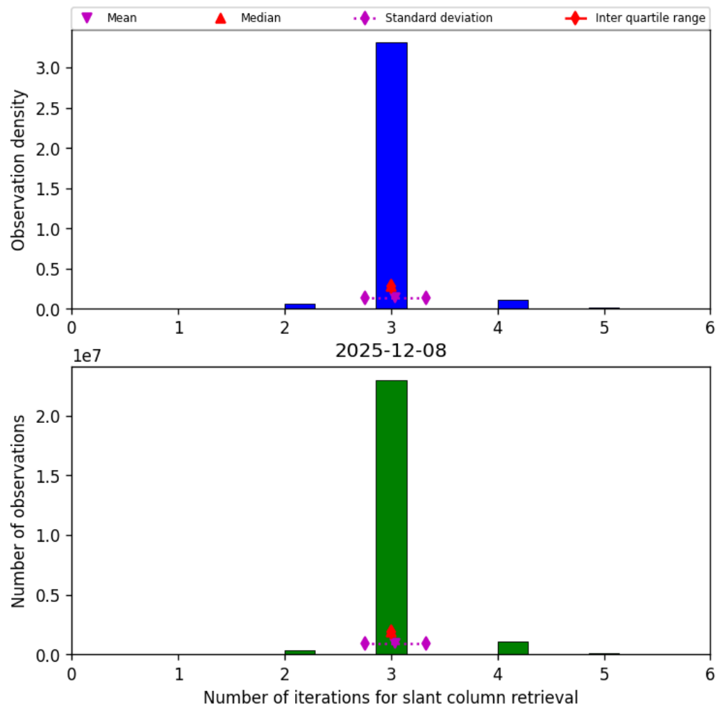
Figure 33: Histogram of “Number of iterations for slant column retrieval” for 2025-12-08 to 2025-12-09
