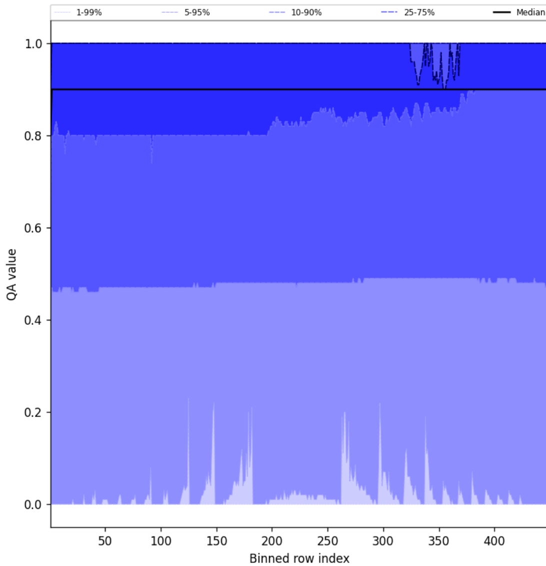
Figure 40: Along track statistics of “QA value” for 2025-12-08 to 2025-12-09
