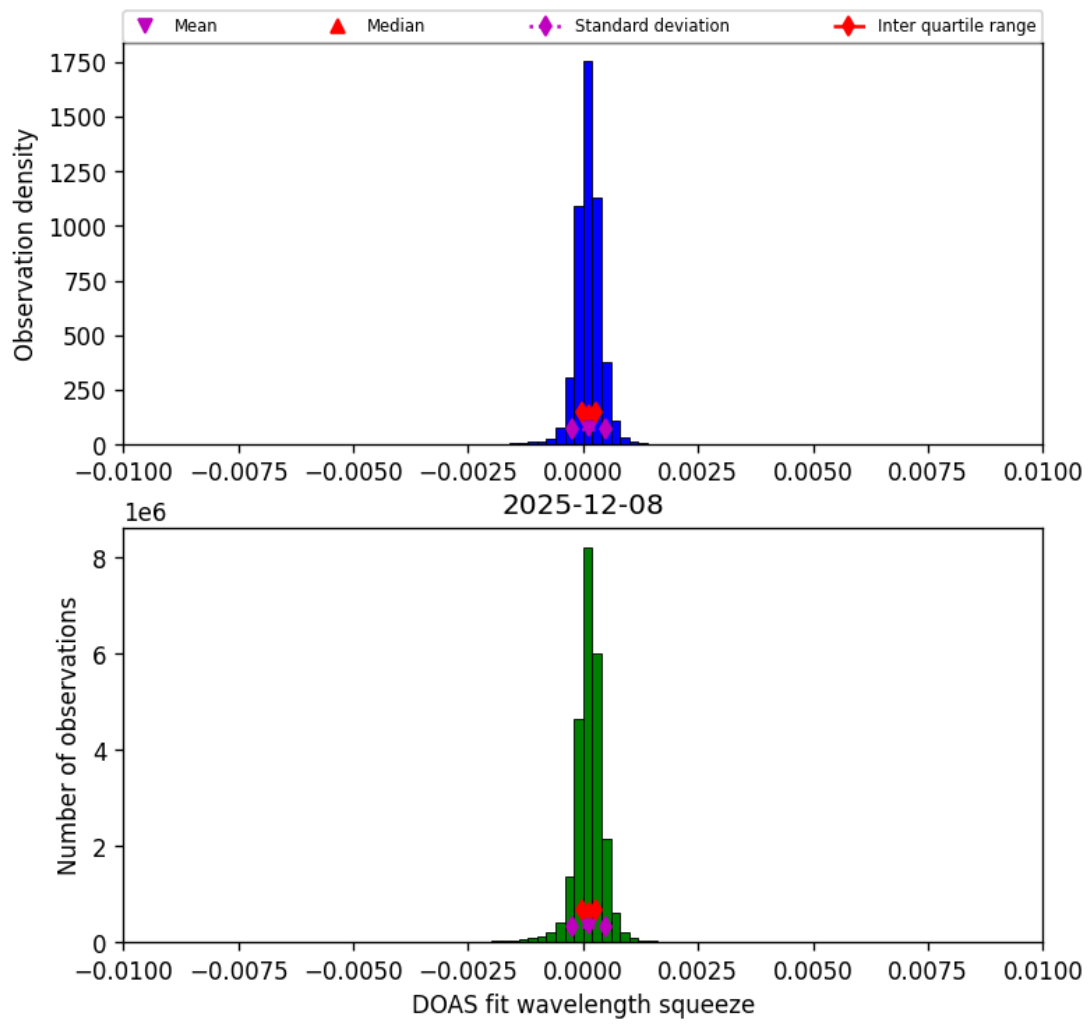
Figure 36: Histogram of “DOAS fit wavelength squeeze” for 2025-12-08 to 2025-12-09
