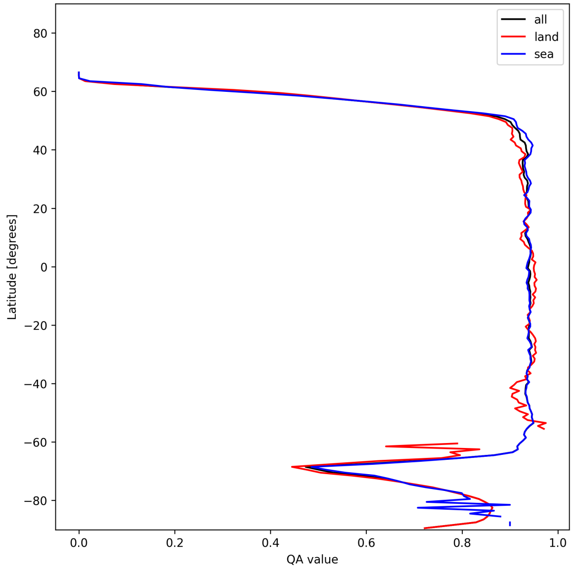
Figure 16: Zonal average of “QA value” for 2025-12-08 to 2025-12-09.
