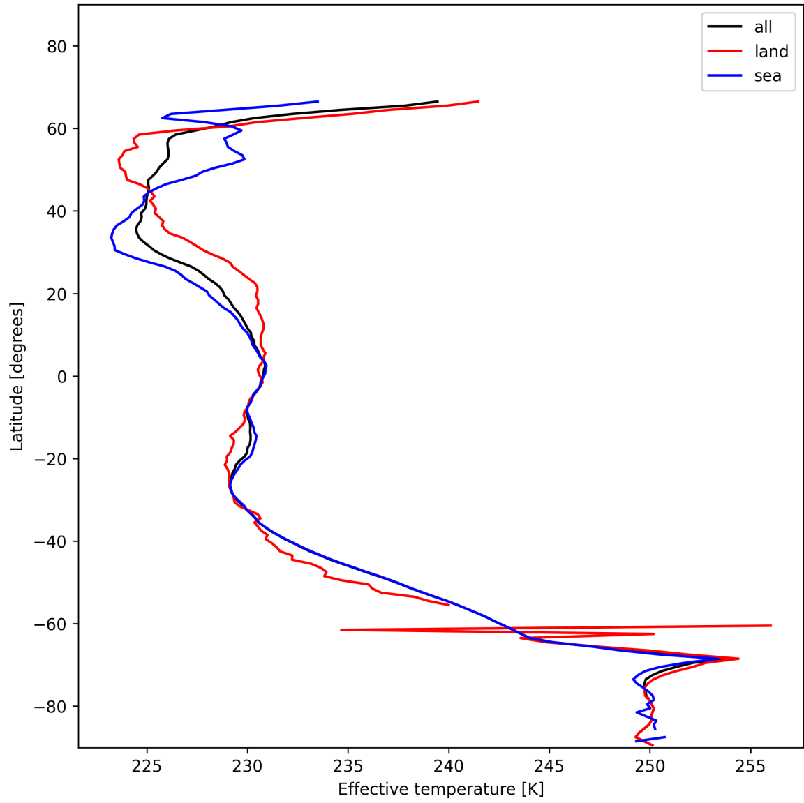
Figure 26: Zonal average of “Effective temperature” for 2025-12-08 to 2025-12-09.
