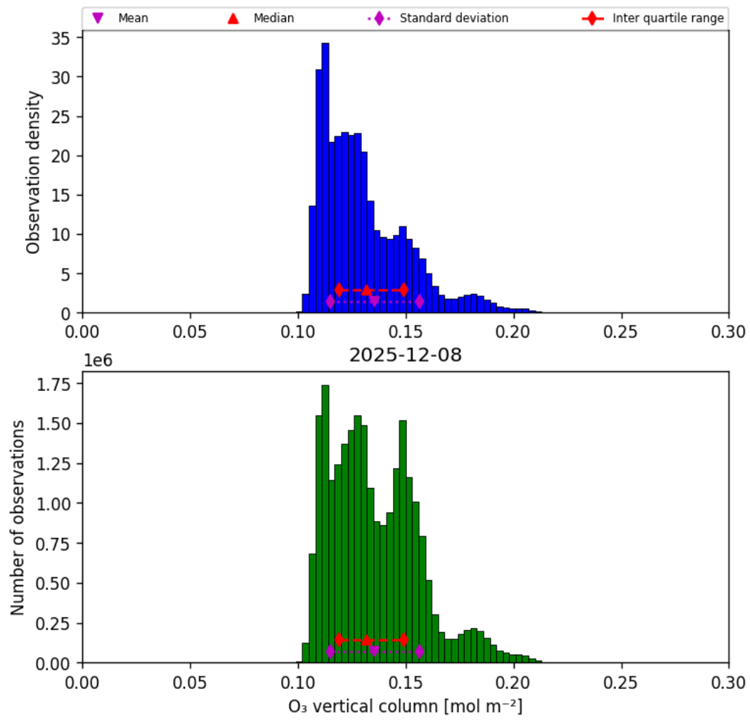
Figure 29: Histogram of “O 3 vertical column” for 2025-12-08 to 2025-12-09
