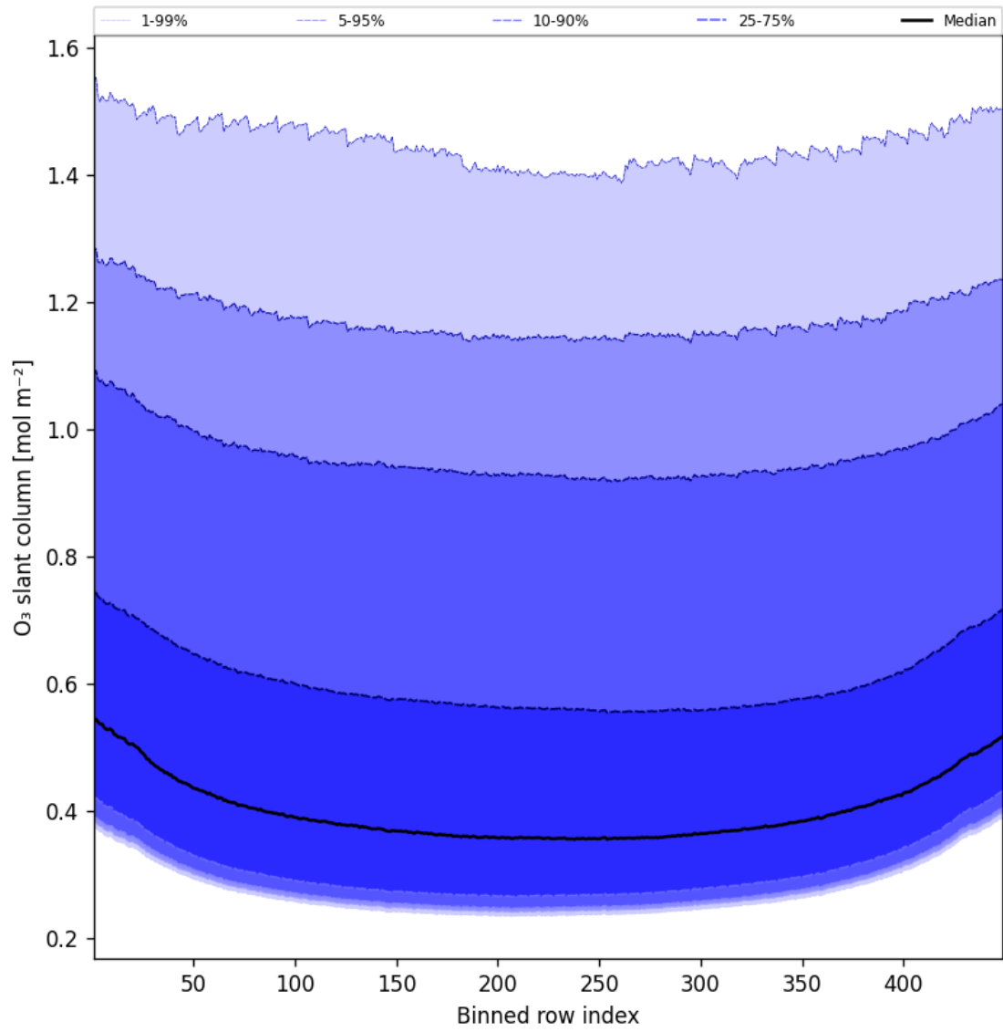
Figure 43: Along track statistics of “O 3 slant column” for 2025-12-08 to 2025-12-09
