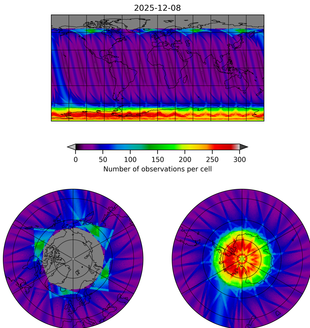
Figure 15: Map of the number of observations for 2025-12-08 to 2025-12-09
