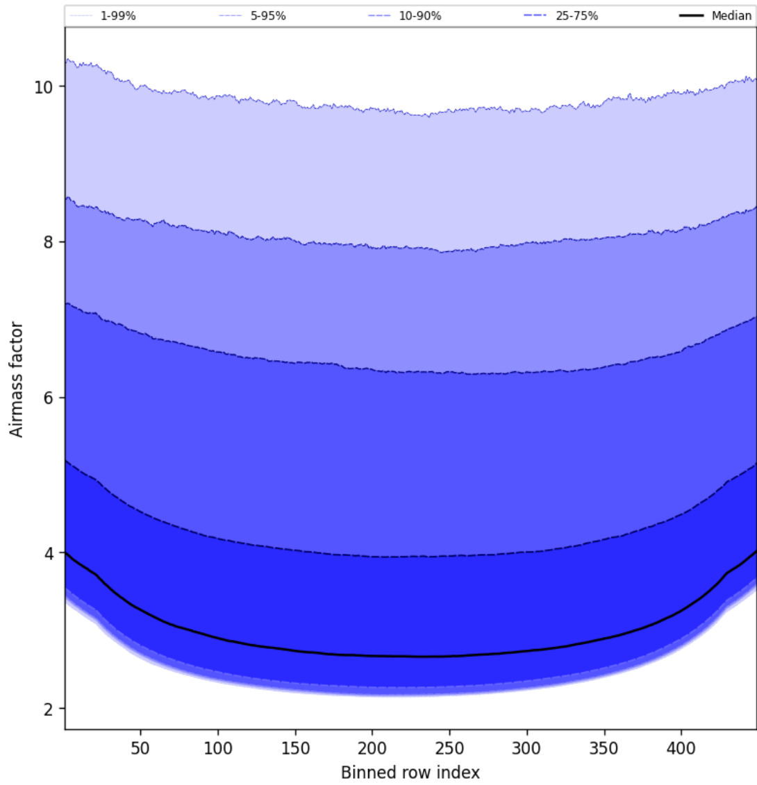
Figure 49: Along track statistics of “Airmass factor” for 2025-12-08 to 2025-12-09
