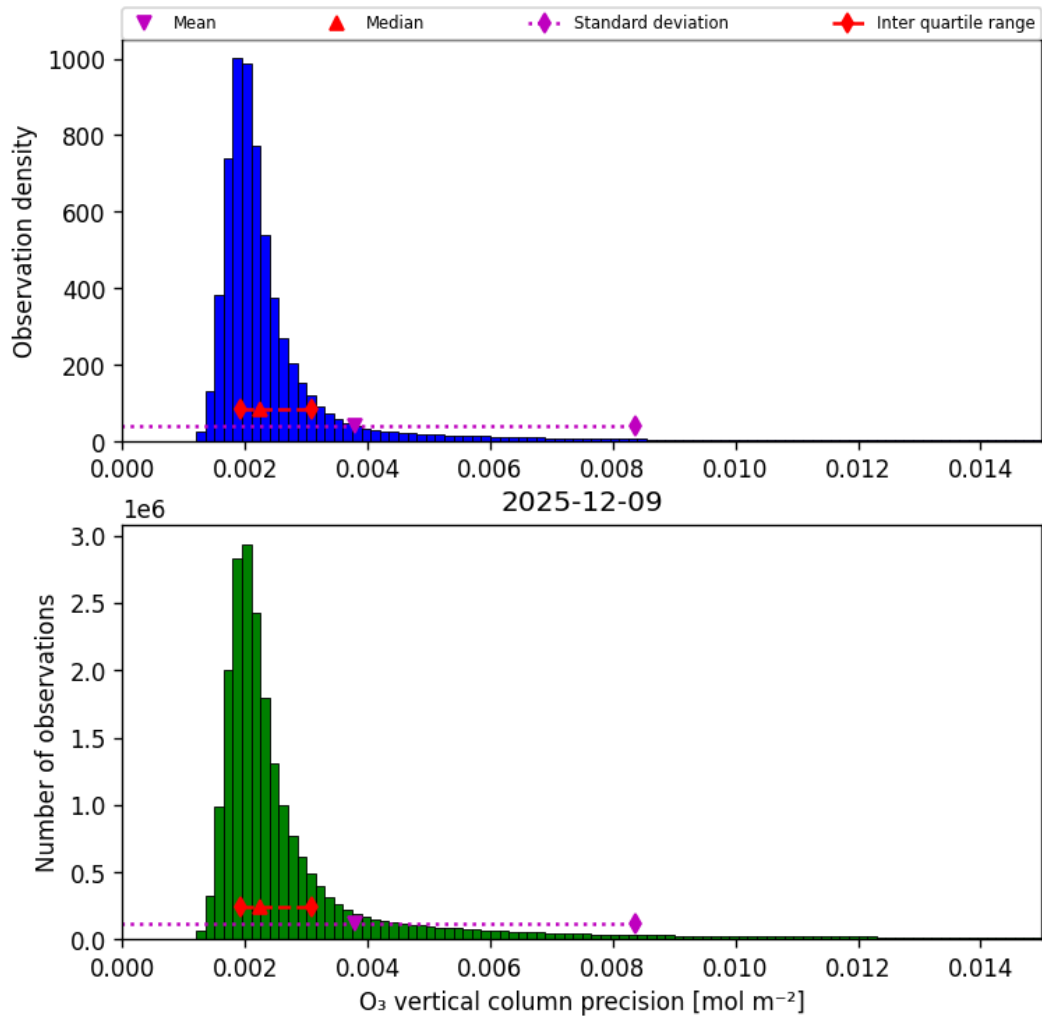
Figure 30: Histogram of “O 3 vertical column precision” for 2025-12-09 to 2025-12-10
