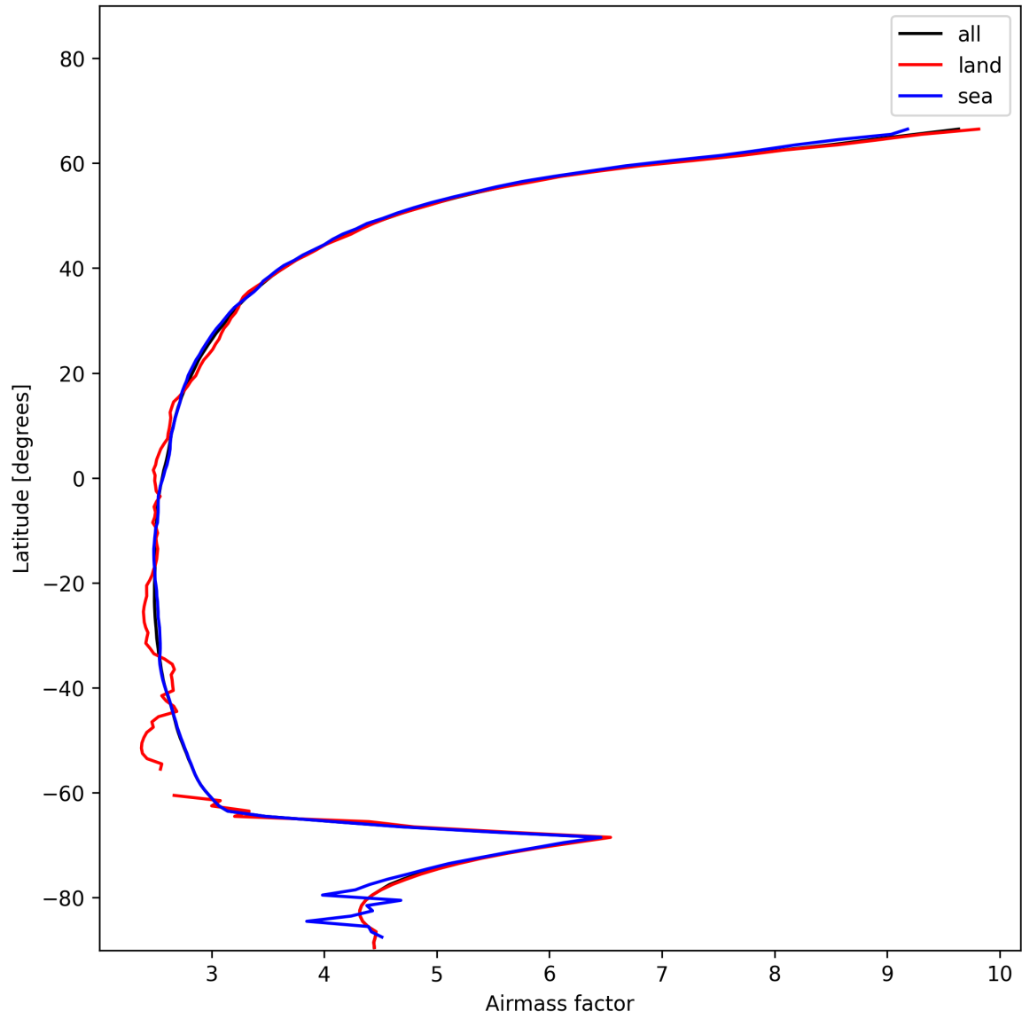
Figure 25: Zonal average of “Airmass factor” for 2025-12-09 to 2025-12-10.
