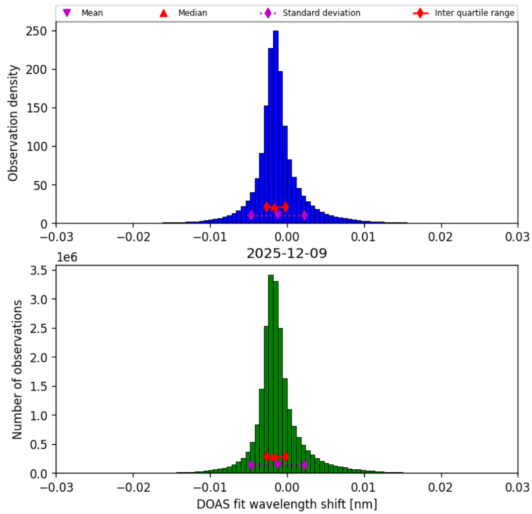
Figure 35: Histogram of “DOAS fit wavelength shift” for 2025-12-09 to 2025-12-10
