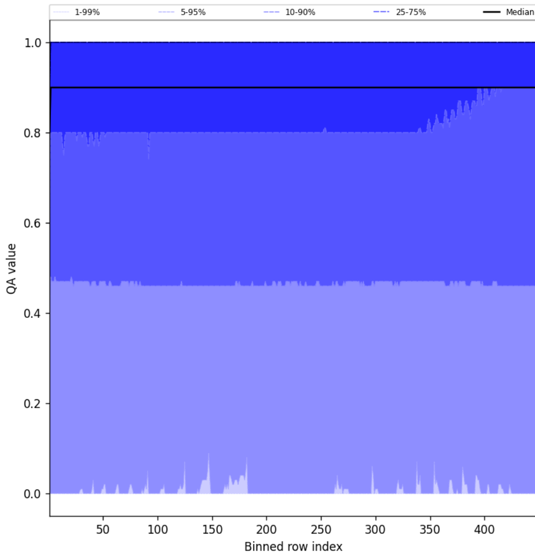
Figure 40: Along track statistics of “QA value” for 2025-12-09 to 2025-12-10
