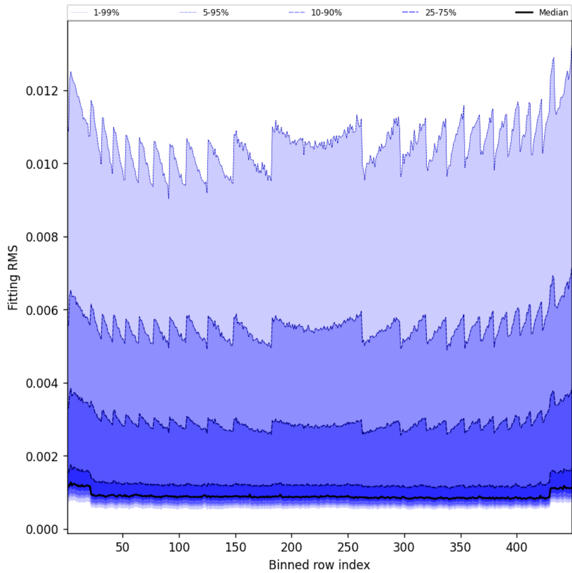
Figure 46: Along track statistics of “Fitting RMS” for 2025-12-09 to 2025-12-10
