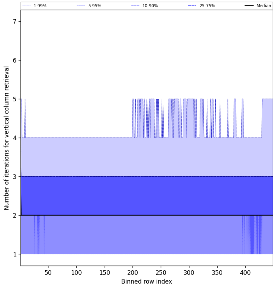
Figure 51: Along track statistics of “Number of iterations for vertical column retrieval” for 2025-12-09 to 2025-12-10
