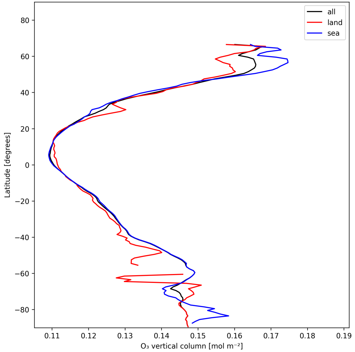
Figure 17: Zonal average of “O 3 vertical column” for 2025-12-09 to 2025-12-10.
