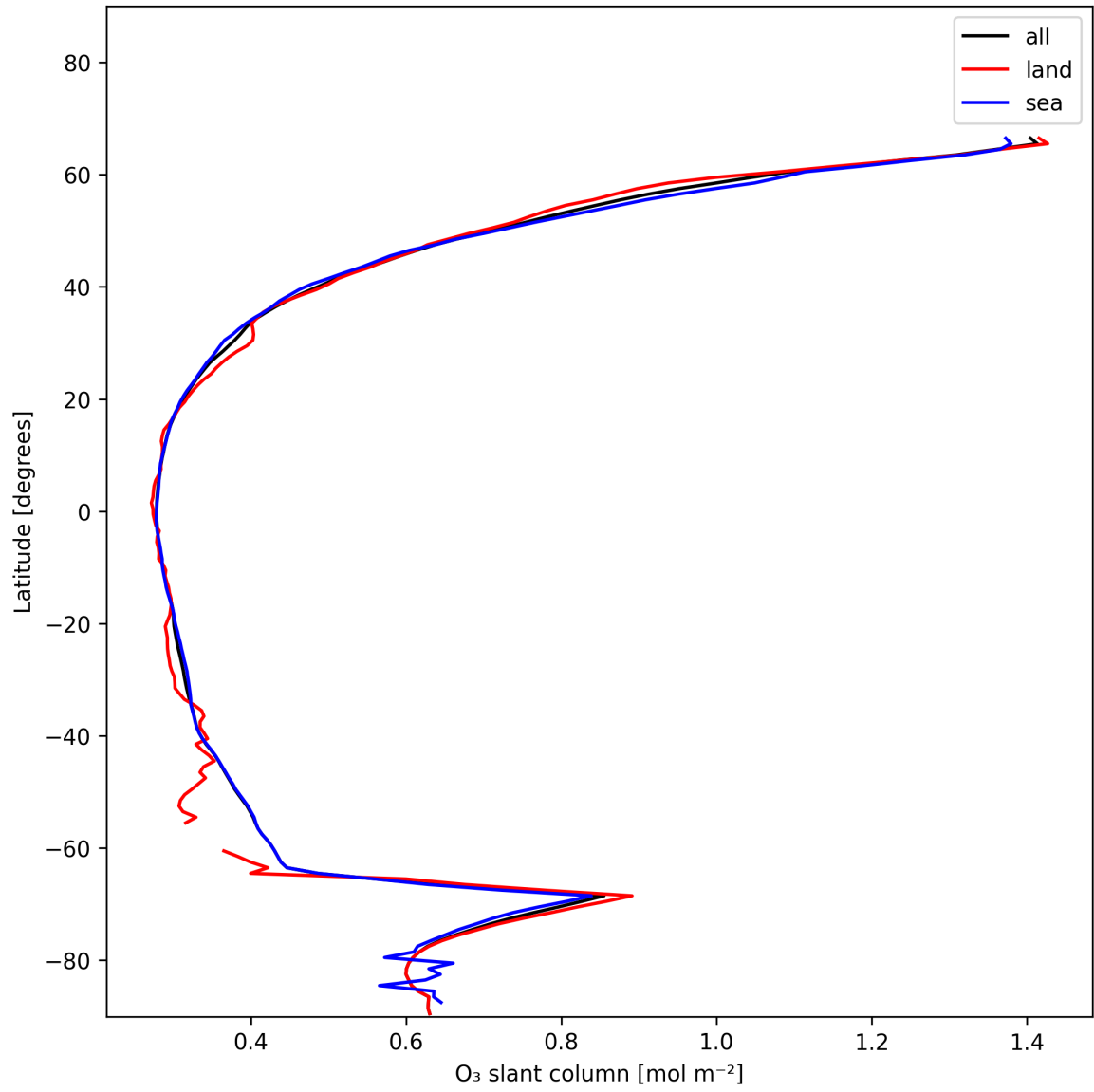
Figure 19: Zonal average of “O 3 slant column” for 2025-12-09 to 2025-12-10.
