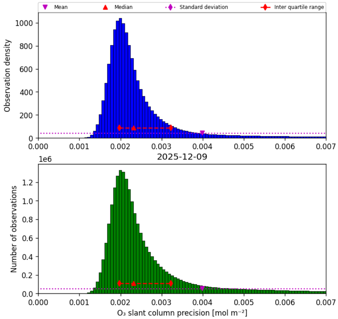
Figure 32: Histogram of “O 3 slant column precision” for 2025-12-09 to 2025-12-10
