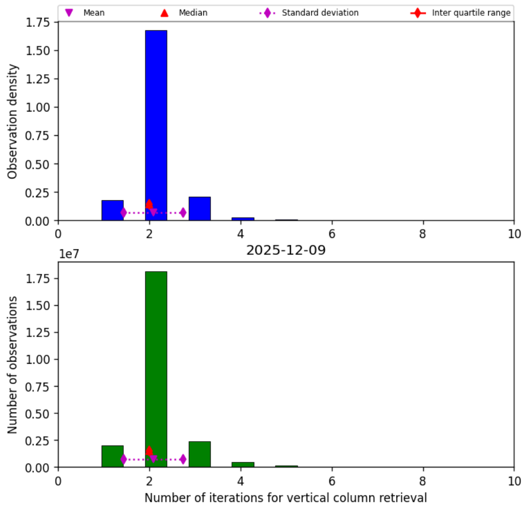
Figure 39: Histogram of “Number of iterations for vertical column retrieval” for 2025-12-09 to 2025-12-10
