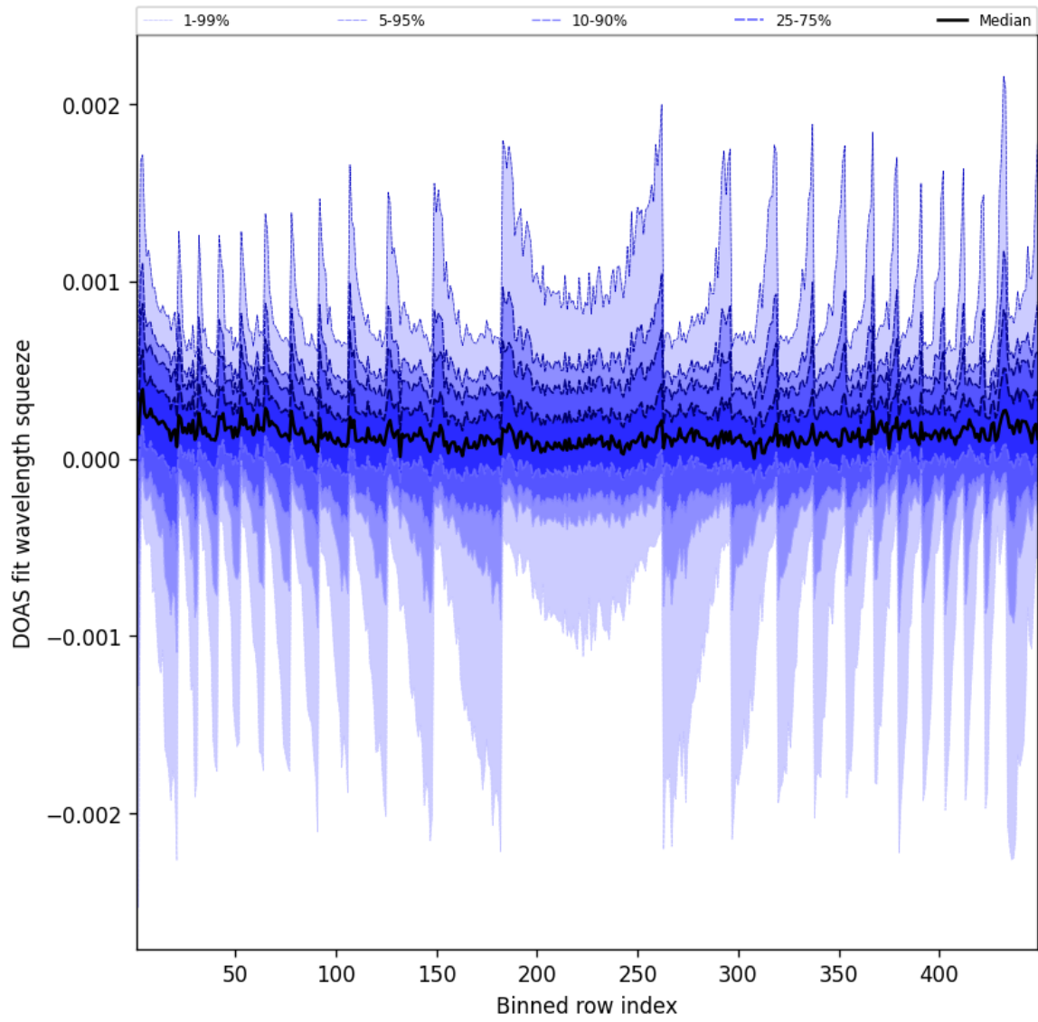
Figure 48: Along track statistics of “DOAS fit wavelength squeeze” for 2025-12-09 to 2025-12-10
