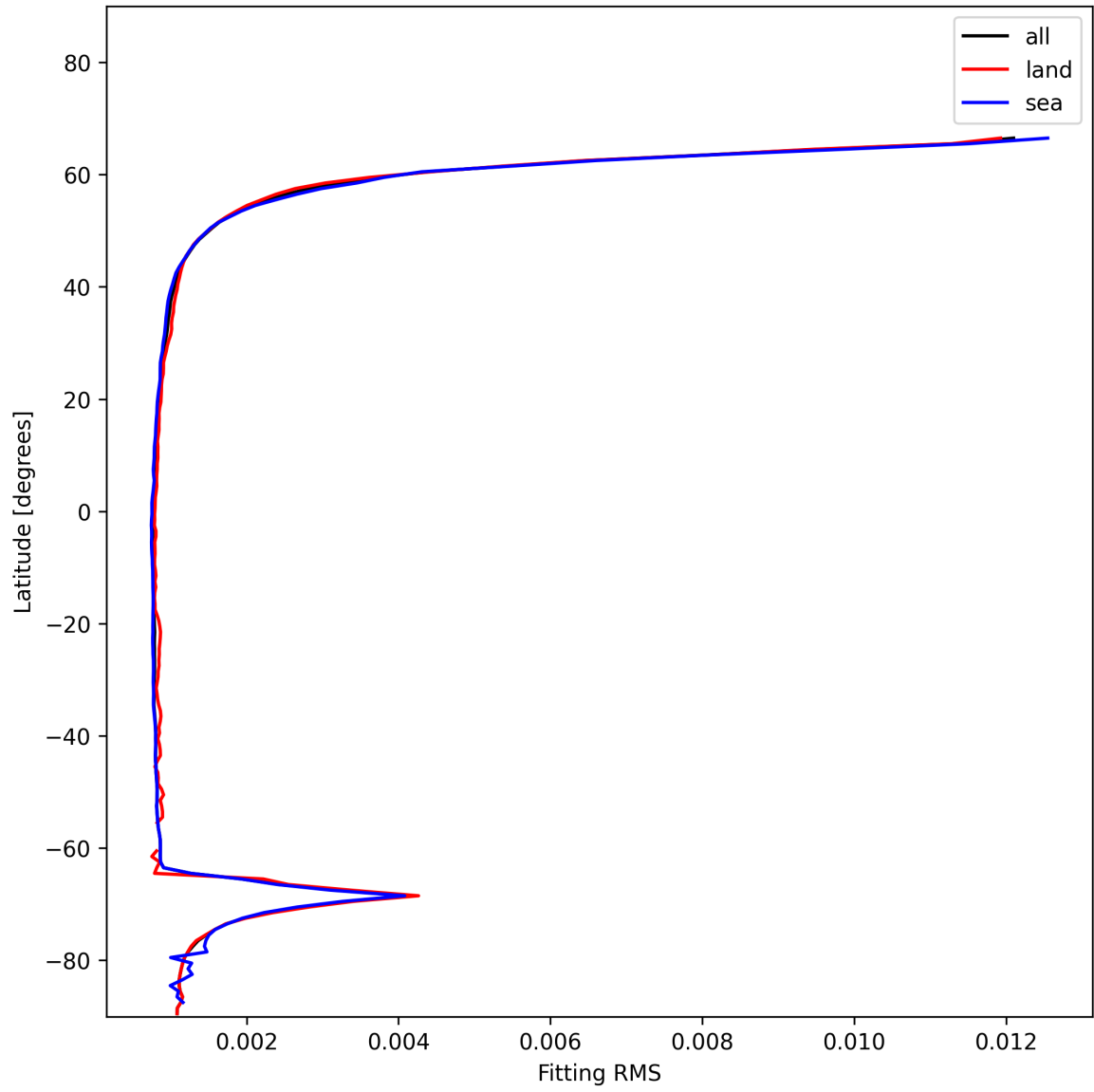
Figure 22: Zonal average of “Fitting RMS” for 2025-12-09 to 2025-12-10.
