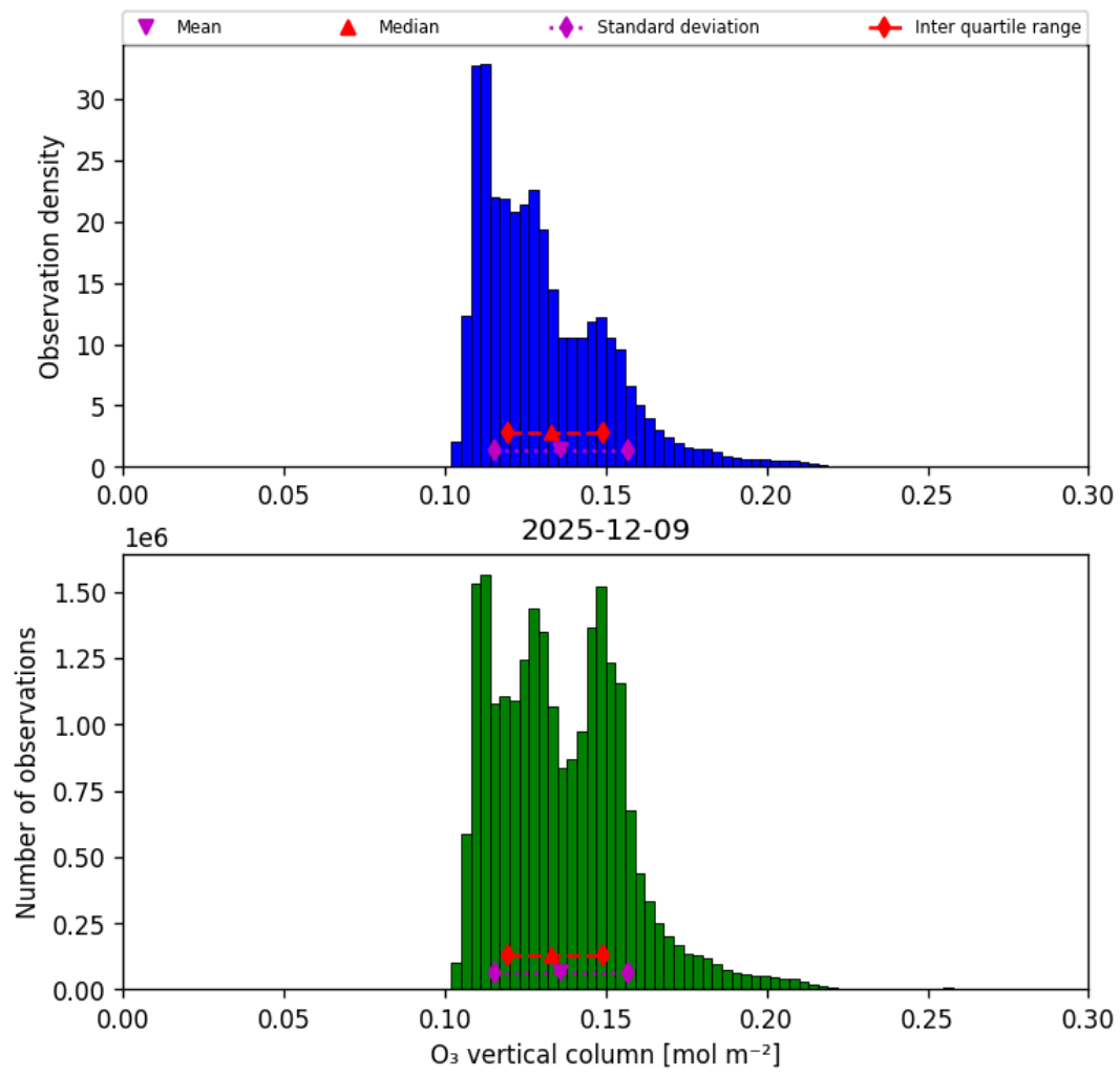
Figure 29: Histogram of “O 3 vertical column” for 2025-12-09 to 2025-12-10
