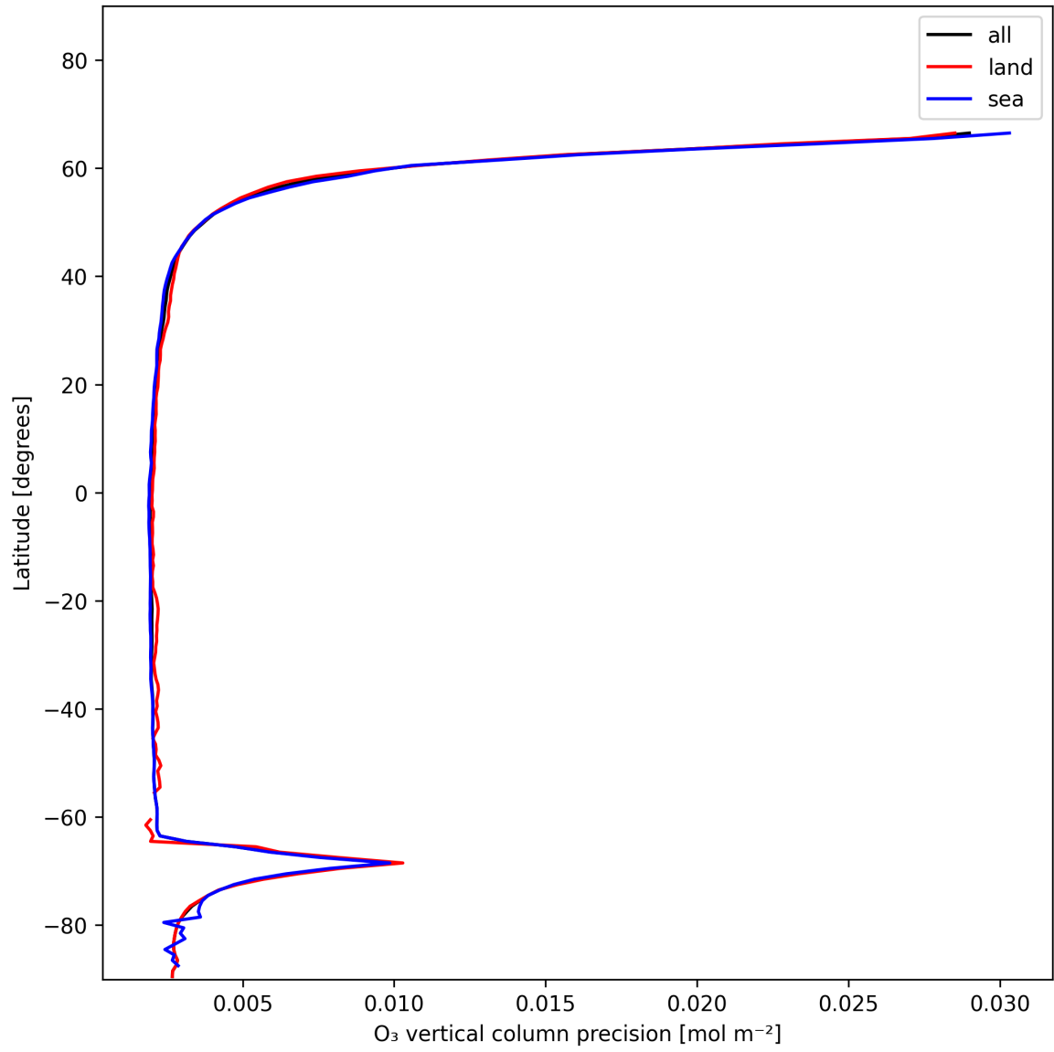
Figure 18: Zonal average of “O 3 vertical column precision” for 2025-12-09 to 2025-12-10.
