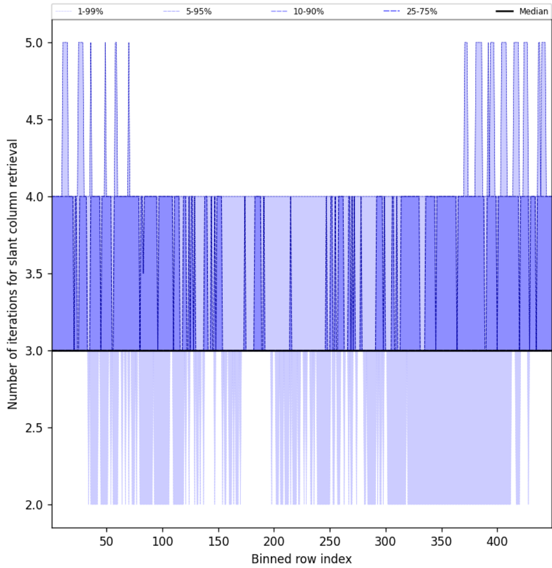
Figure 45: Along track statistics of “Number of iterations for slant column retrieval” for 2025-12-09 to 2025-12-10
