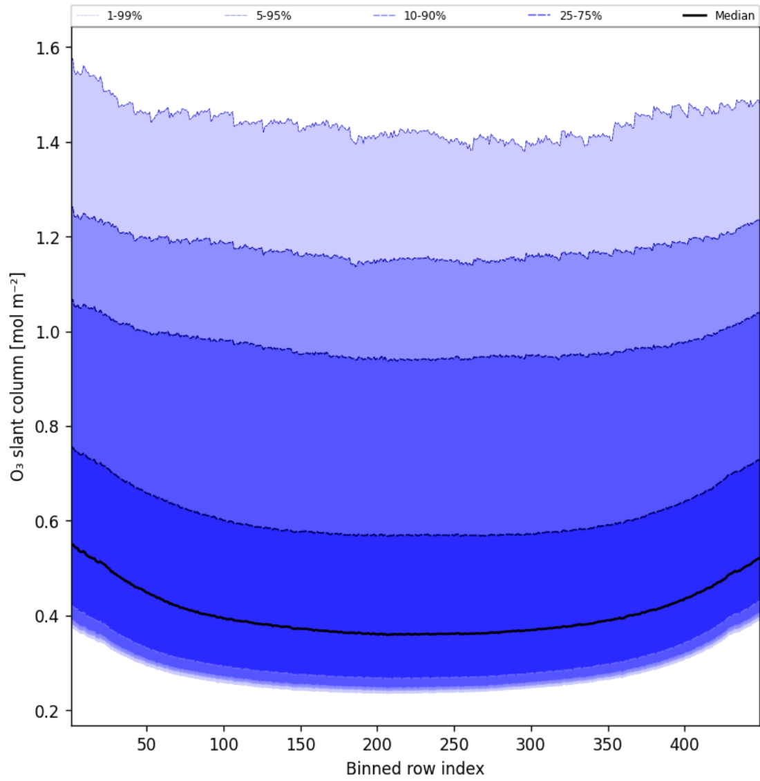
Figure 43: Along track statistics of “O 3 slant column” for 2025-12-09 to 2025-12-10
