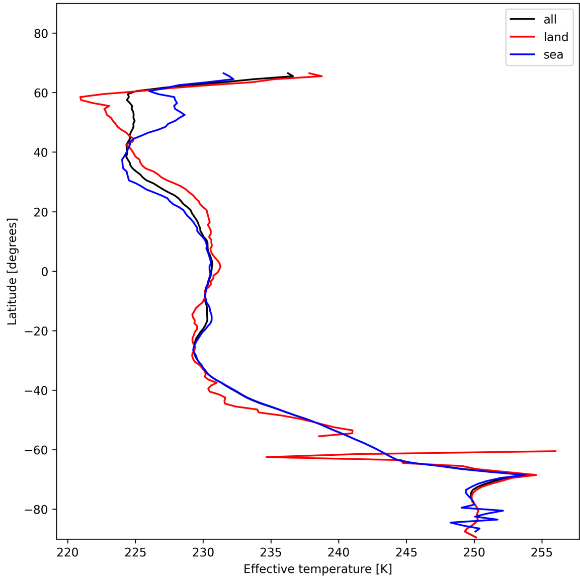
Figure 26: Zonal average of “Effective temperature” for 2025-12-09 to 2025-12-10.
