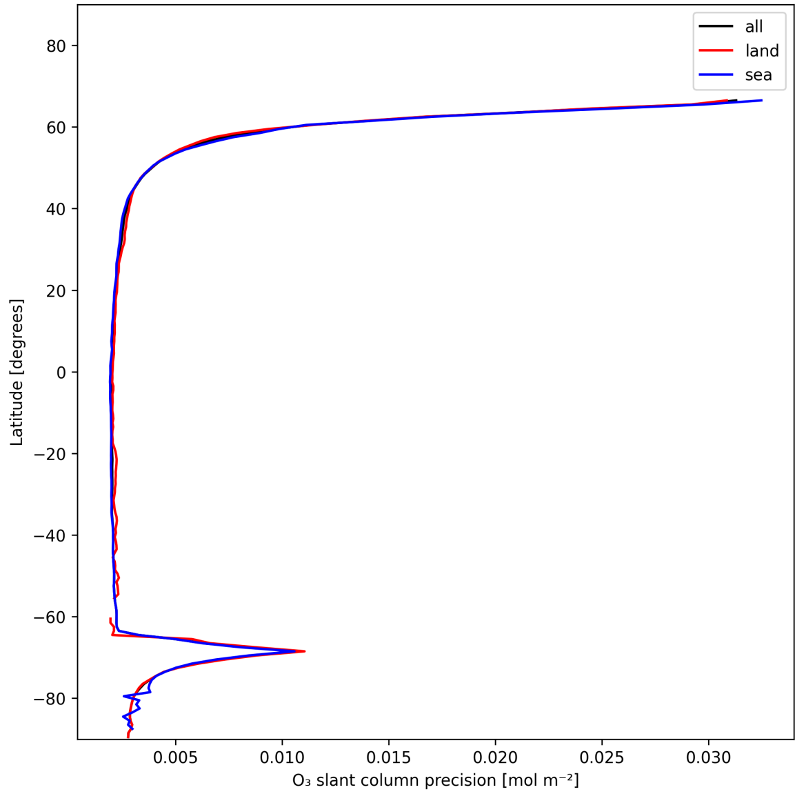
Figure 20: Zonal average of “O 3 slant column precision” for 2025-12-09 to 2025-12-10.
