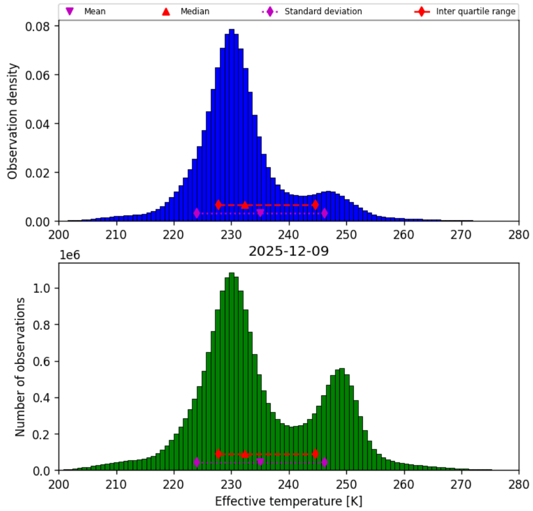
Figure 38: Histogram of “Effective temperature” for 2025-12-09 to 2025-12-10
