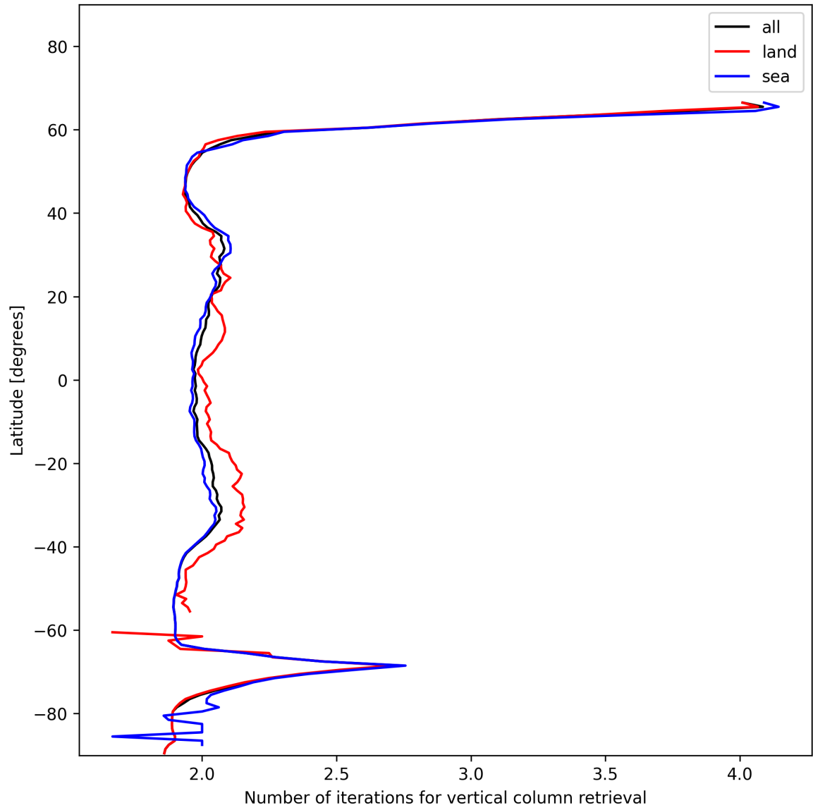
Figure 27: Zonal average of “Number of iterations for vertical column retrieval” for 2025-12-09 to 2025-12-10.
