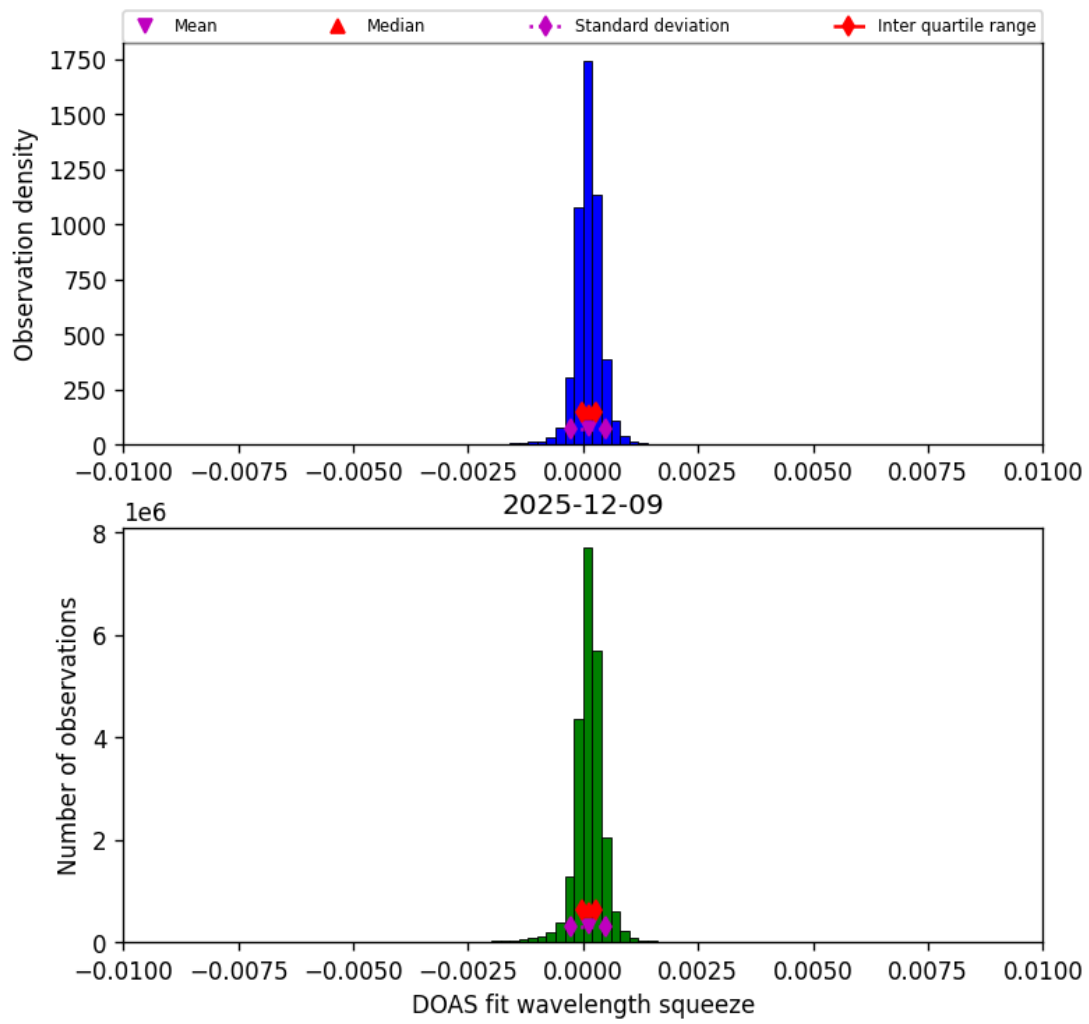
Figure 36: Histogram of “DOAS fit wavelength squeeze” for 2025-12-09 to 2025-12-10
