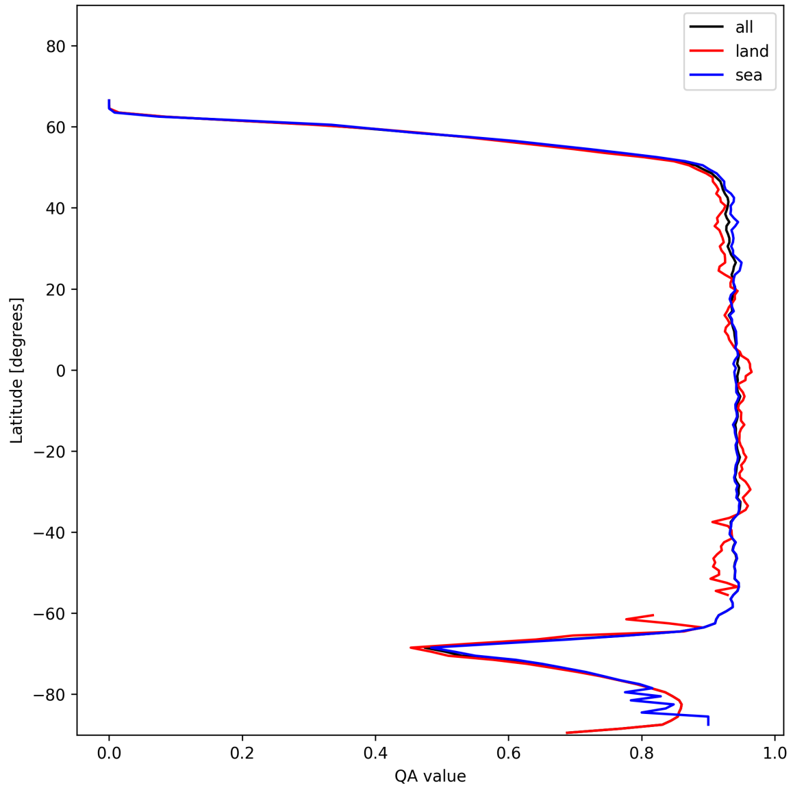
Figure 16: Zonal average of “QA value” for 2025-12-09 to 2025-12-10.
