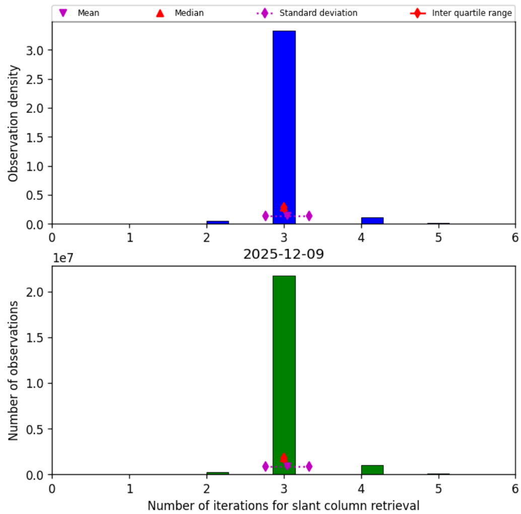
Figure 33: Histogram of "Number of iterations for slant column retrieval" for 2025-12-09 to 2025-12-10
