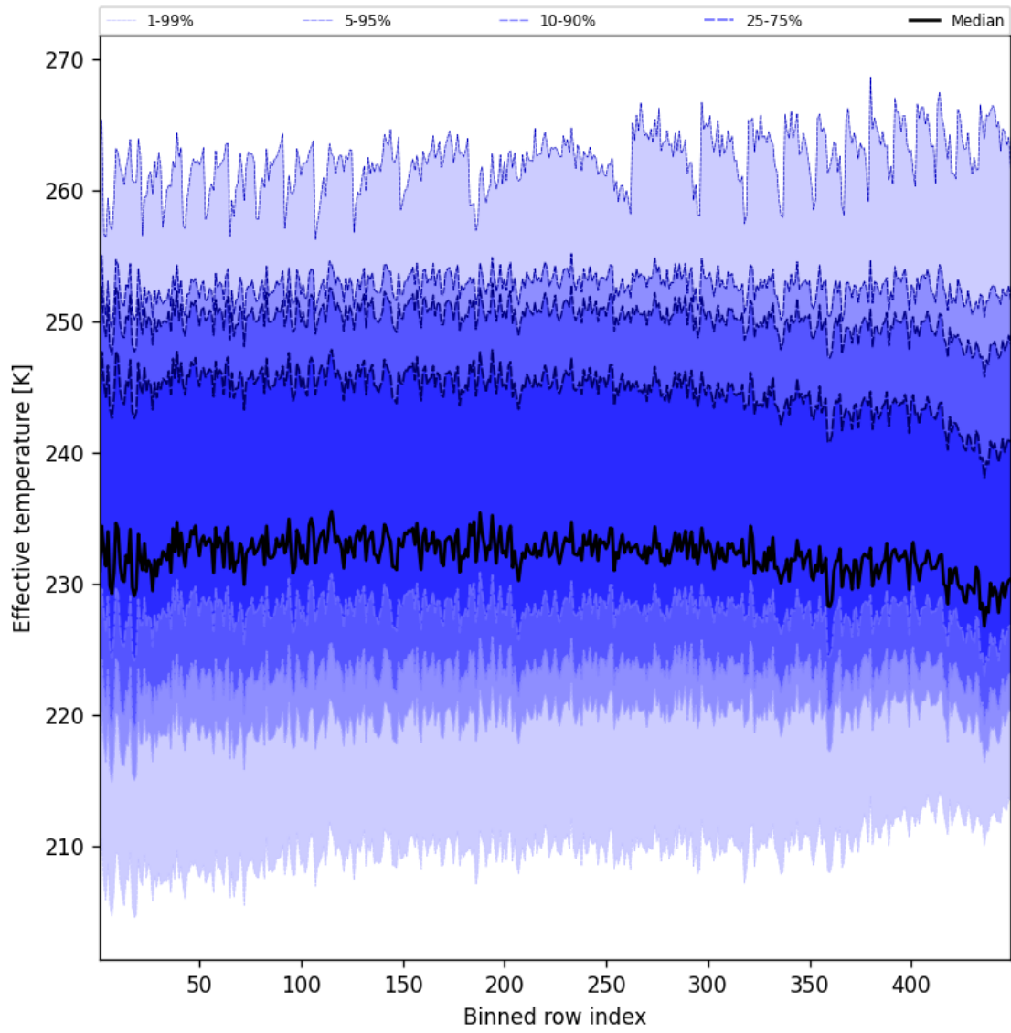
Figure 50: Along track statistics of “Effective temperature” for 2025-12-09 to 2025-12-10
