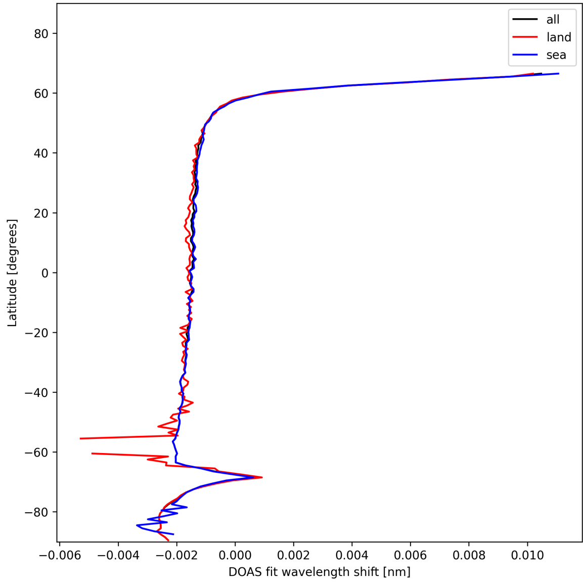
Figure 23: Zonal average of “DOAS fit wavelength shift” for 2025-12-09 to 2025-12-10.
