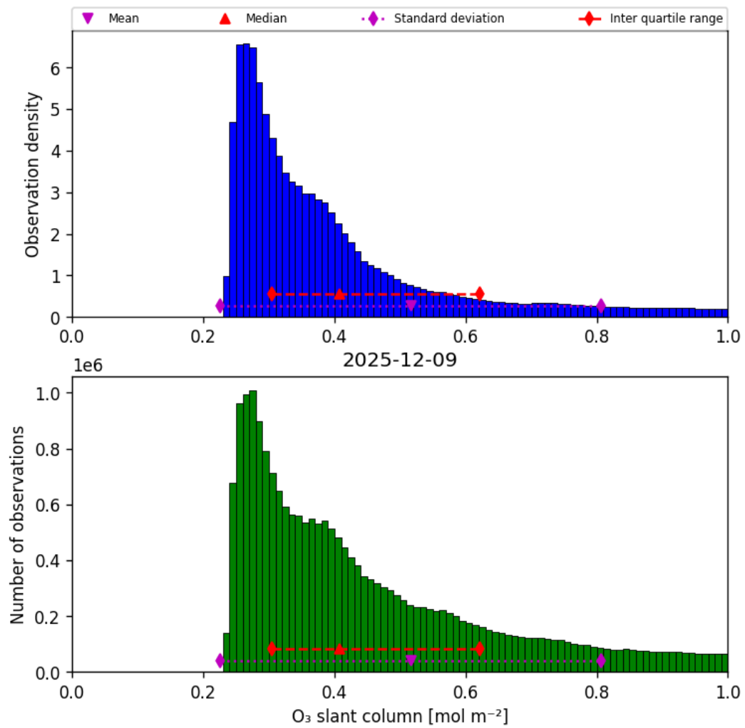
Figure 31: Histogram of “O 3 slant column” for 2025-12-09 to 2025-12-10
