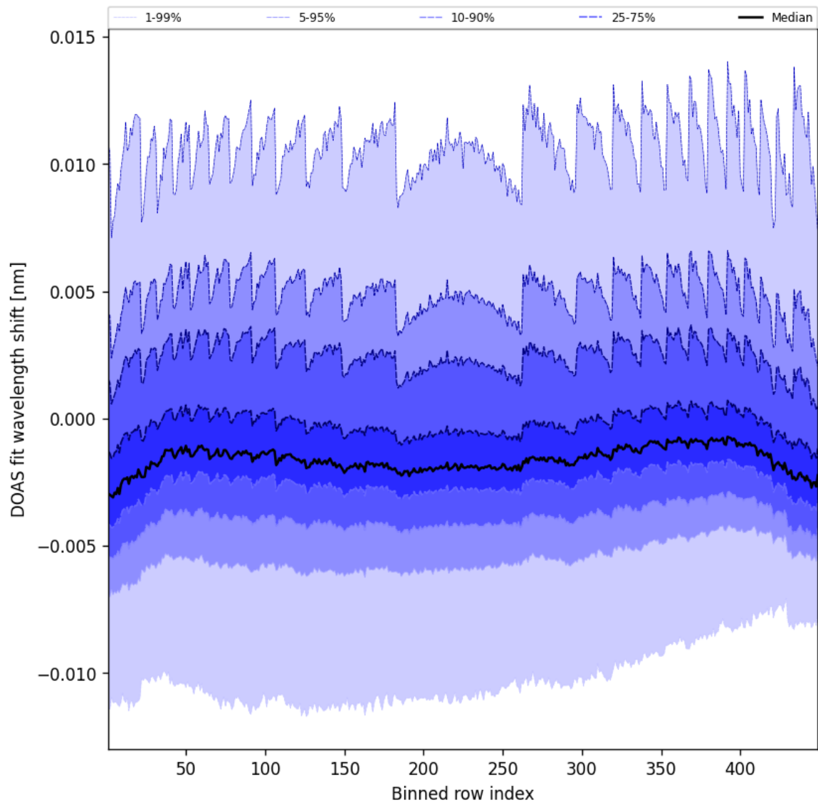
Figure 47: Along track statistics of “DOAS fit wavelength shift” for 2025-12-09 to 2025-12-10
