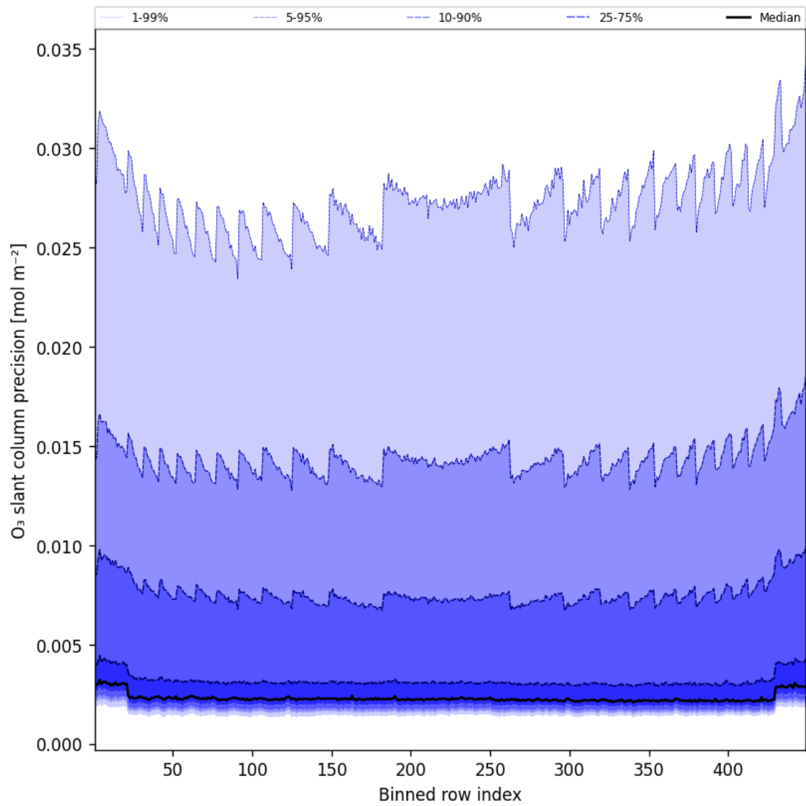
Figure 44: Along track statistics of “O 3 slant column precision” for 2025-12-09 to 2025-12-10
