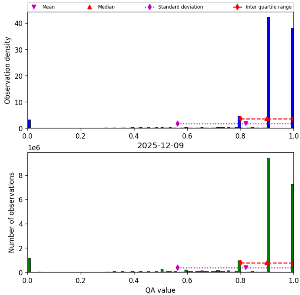
Figure 28: Histogram of “QA value” for 2025-12-09 to 2025-12-10
