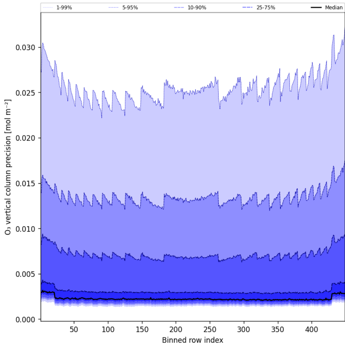
Figure 42: Along track statistics of “O 3 vertical column precision” for 2025-12-09 to 2025-12-10
