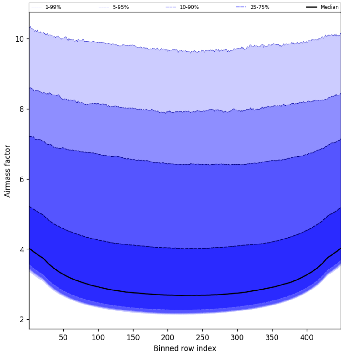
Figure 49: Along track statistics of “Airmass factor” for 2025-12-09 to 2025-12-10
