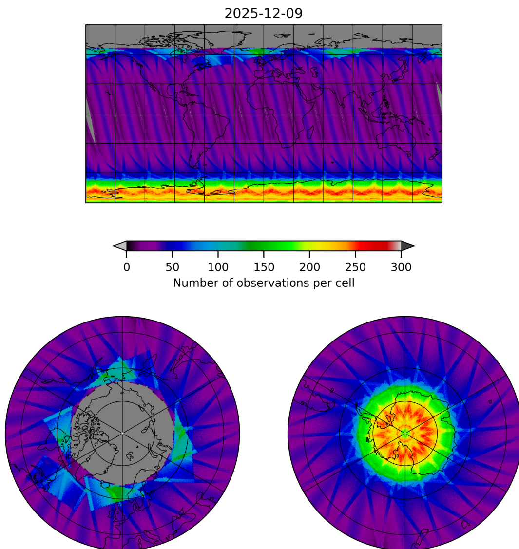
Figure 15: Map of the number of observations for 2025-12-09 to 2025-12-10
