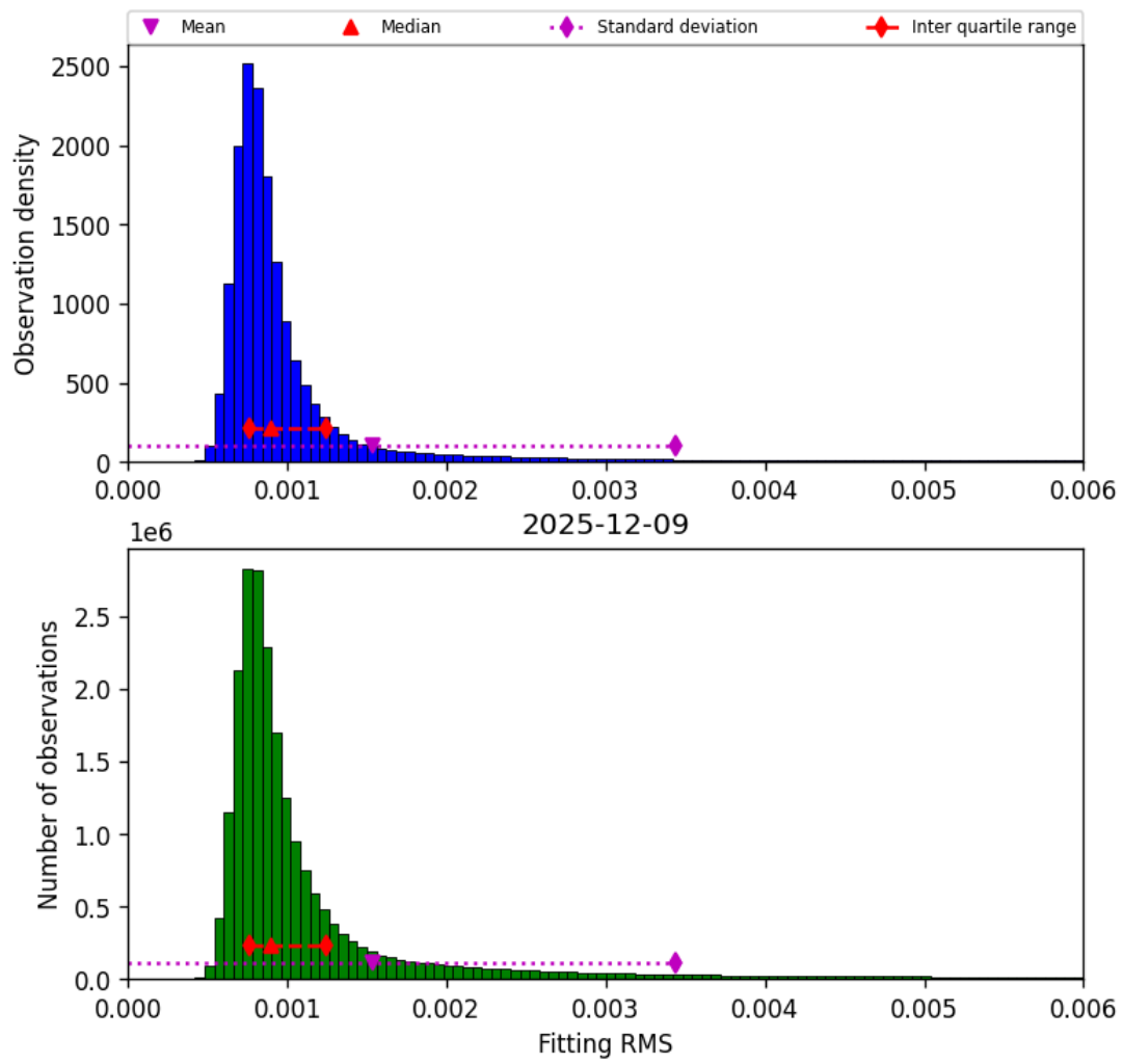
Figure 34: Histogram of “Fitting RMS” for 2025-12-09 to 2025-12-10
