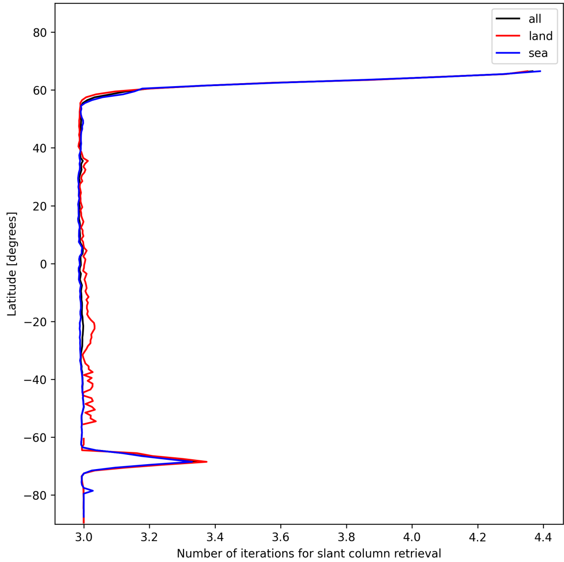
Figure 21: Zonal average of “Number of iterations for slant column retrieval” for 2025-12-09 to 2025-12-10.
