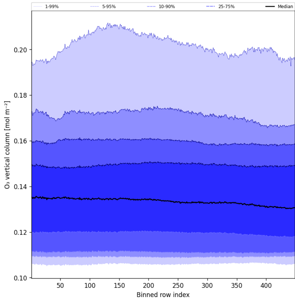
Figure 41: Along track statistics of “O 3 vertical column” for 2025-12-09 to 2025-12-10
