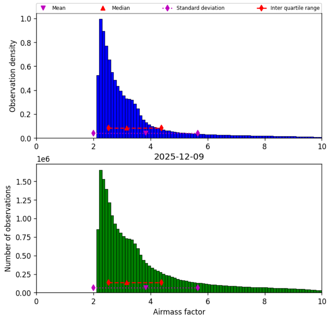
Figure 37: Histogram of “Airmass factor” for 2025-12-09 to 2025-12-10
