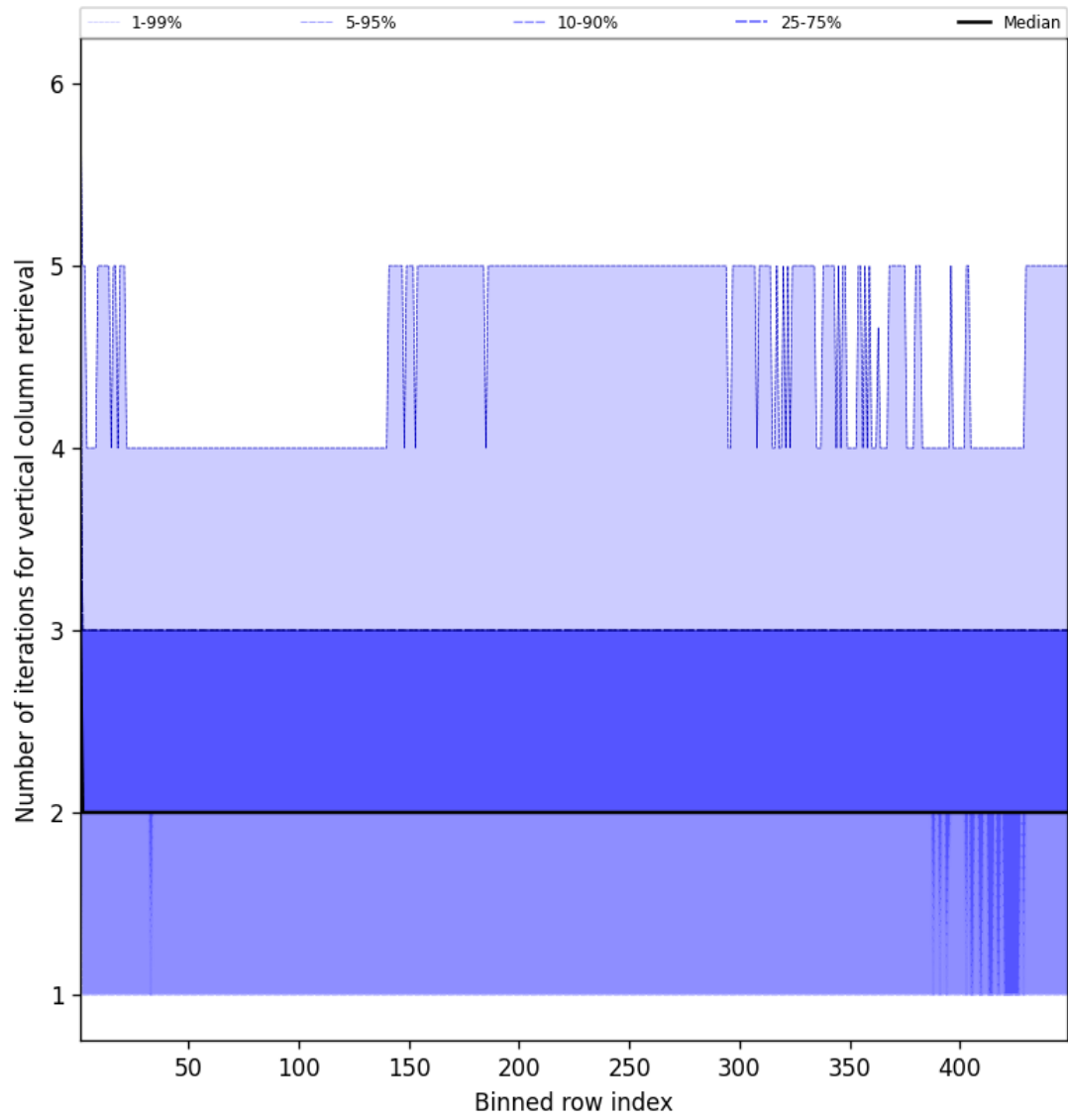
Figure 51: Along track statistics of “Number of iterations for vertical column retrieval” for 2025-12-10 to 2025-12-11
