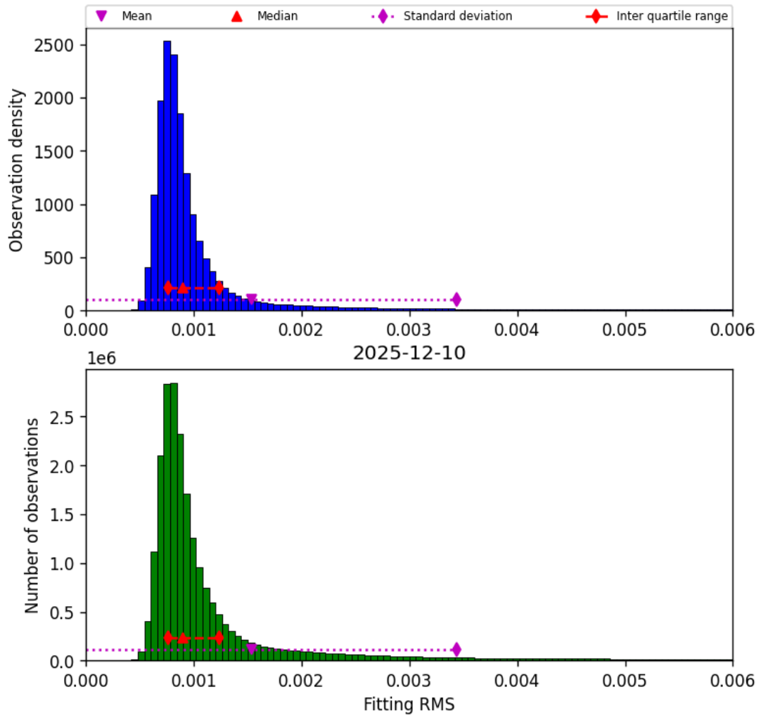
Figure 34: Histogram of “Fitting RMS” for 2025-12-10 to 2025-12-11
