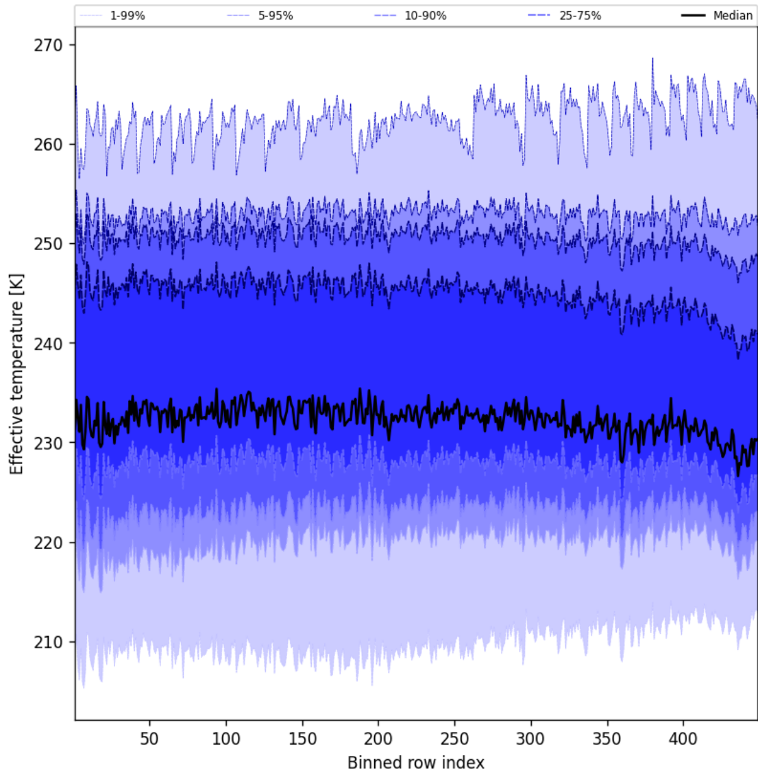
Figure 50: Along track statistics of “Effective temperature” for 2025-12-10 to 2025-12-11
