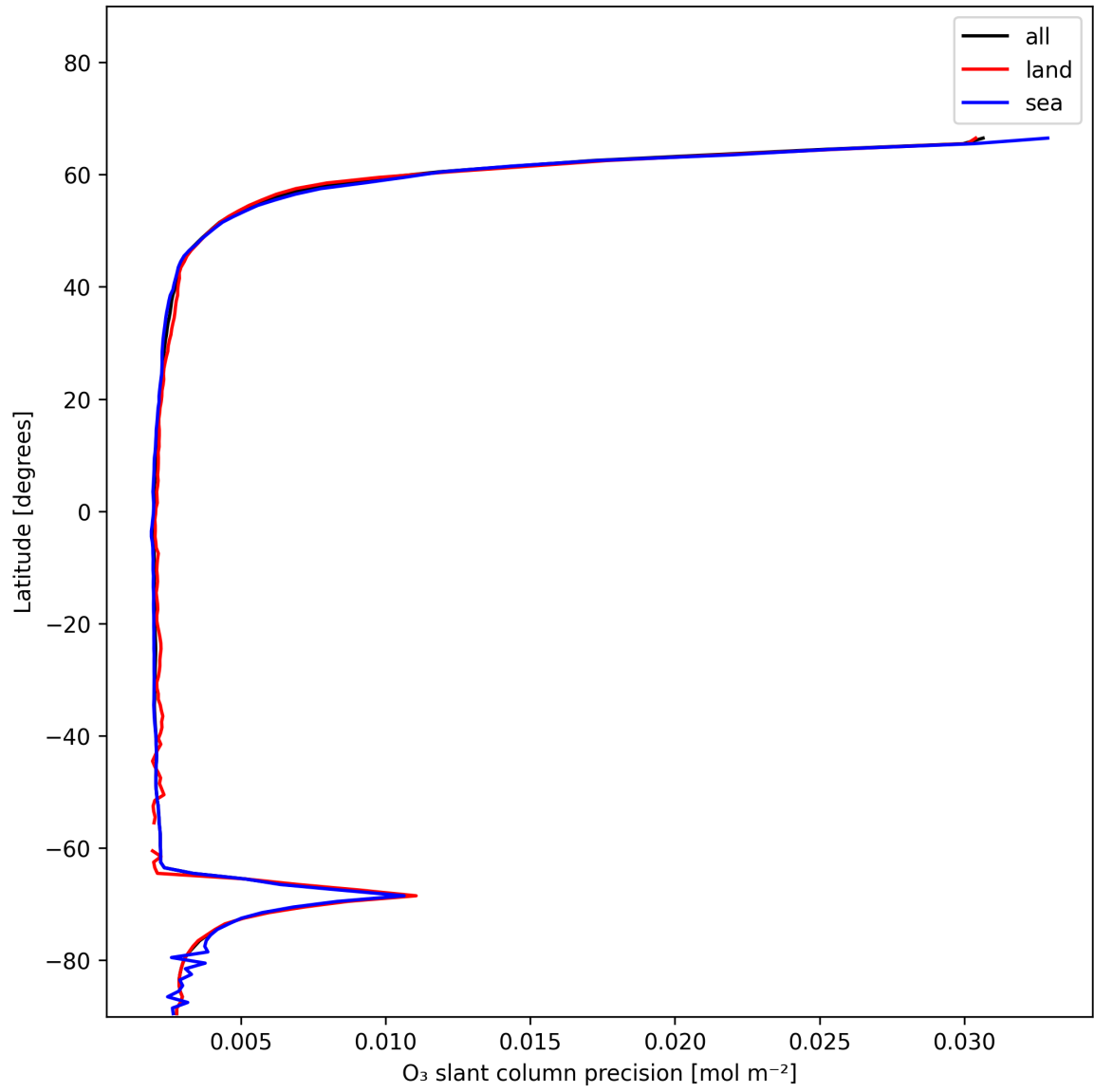
Figure 20: Zonal average of “O 3 slant column precision” for 2025-12-10 to 2025-12-11.
