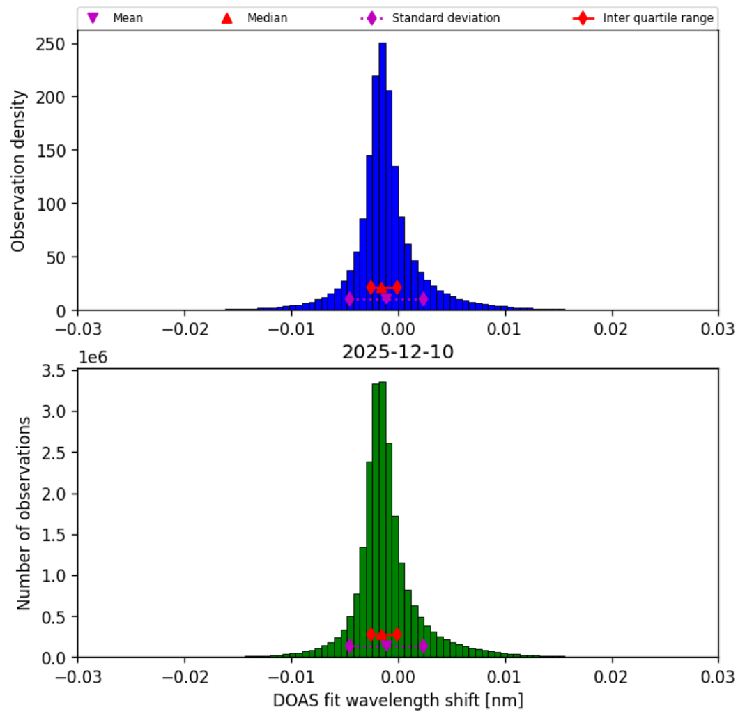
Figure 35: Histogram of “DOAS fit wavelength shift” for 2025-12-10 to 2025-12-11
