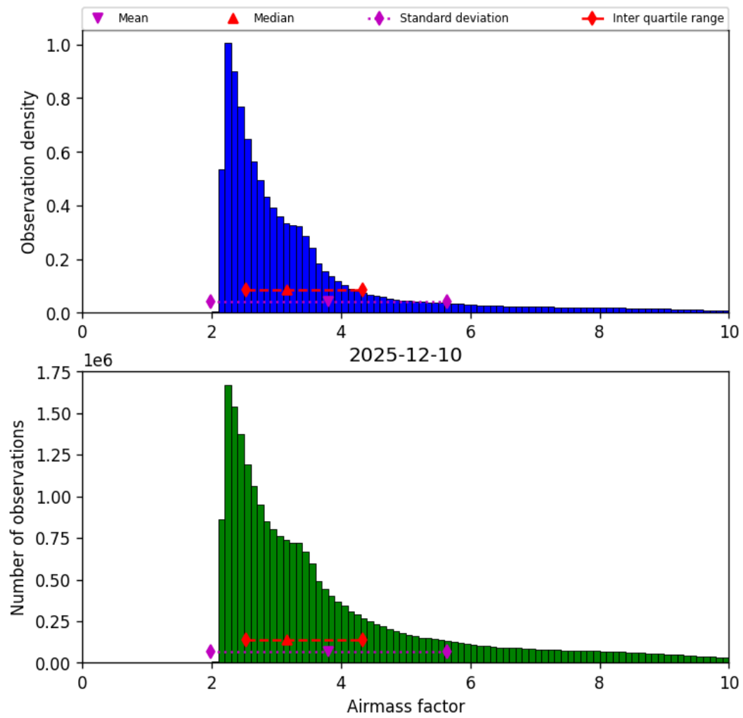
Figure 37: Histogram of “Airmass factor” for 2025-12-10 to 2025-12-11
