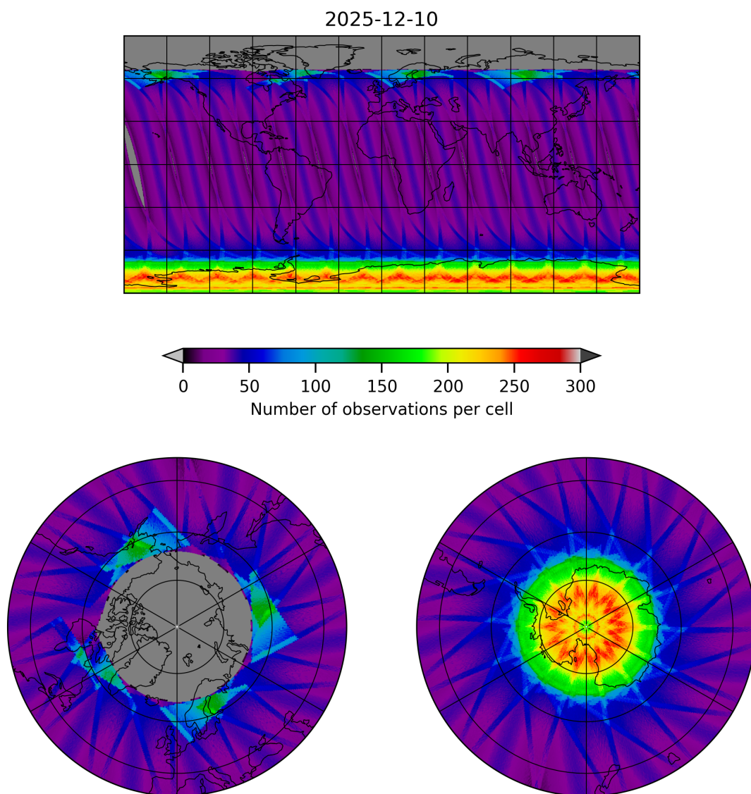
Figure 15: Map of the number of observations for 2025-12-10 to 2025-12-11
