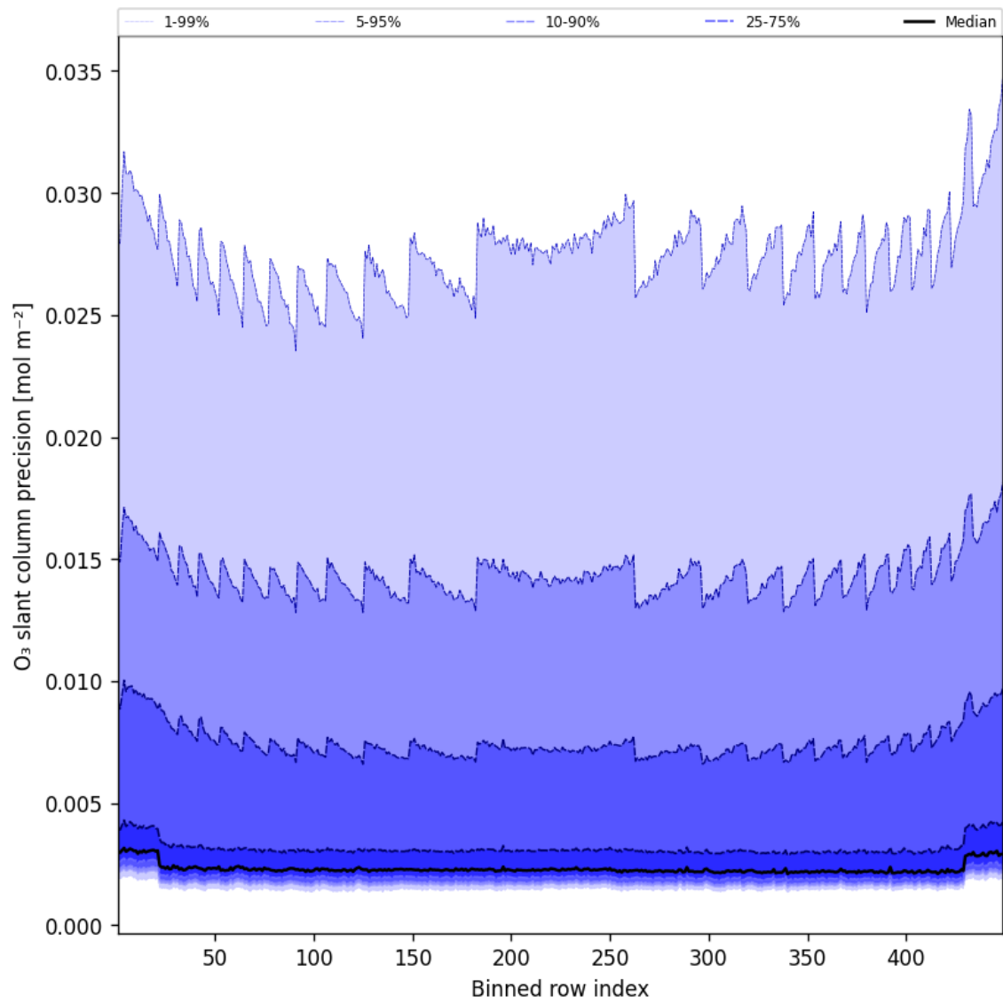
Figure 44: Along track statistics of “O 3 slant column precision” for 2025-12-10 to 2025-12-11
