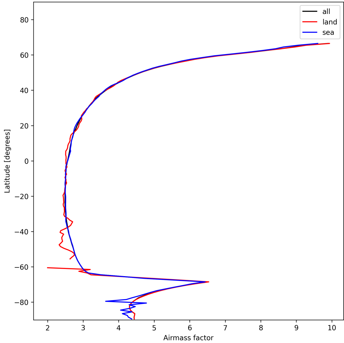
Figure 25: Zonal average of “Airmass factor” for 2025-12-10 to 2025-12-11.
