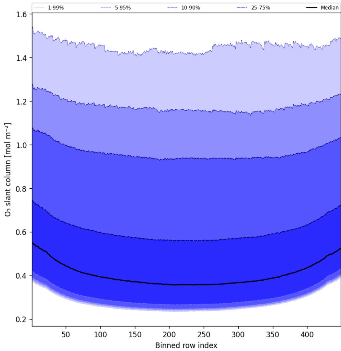
Figure 43: Along track statistics of “O 3 slant column” for 2025-12-10 to 2025-12-11
