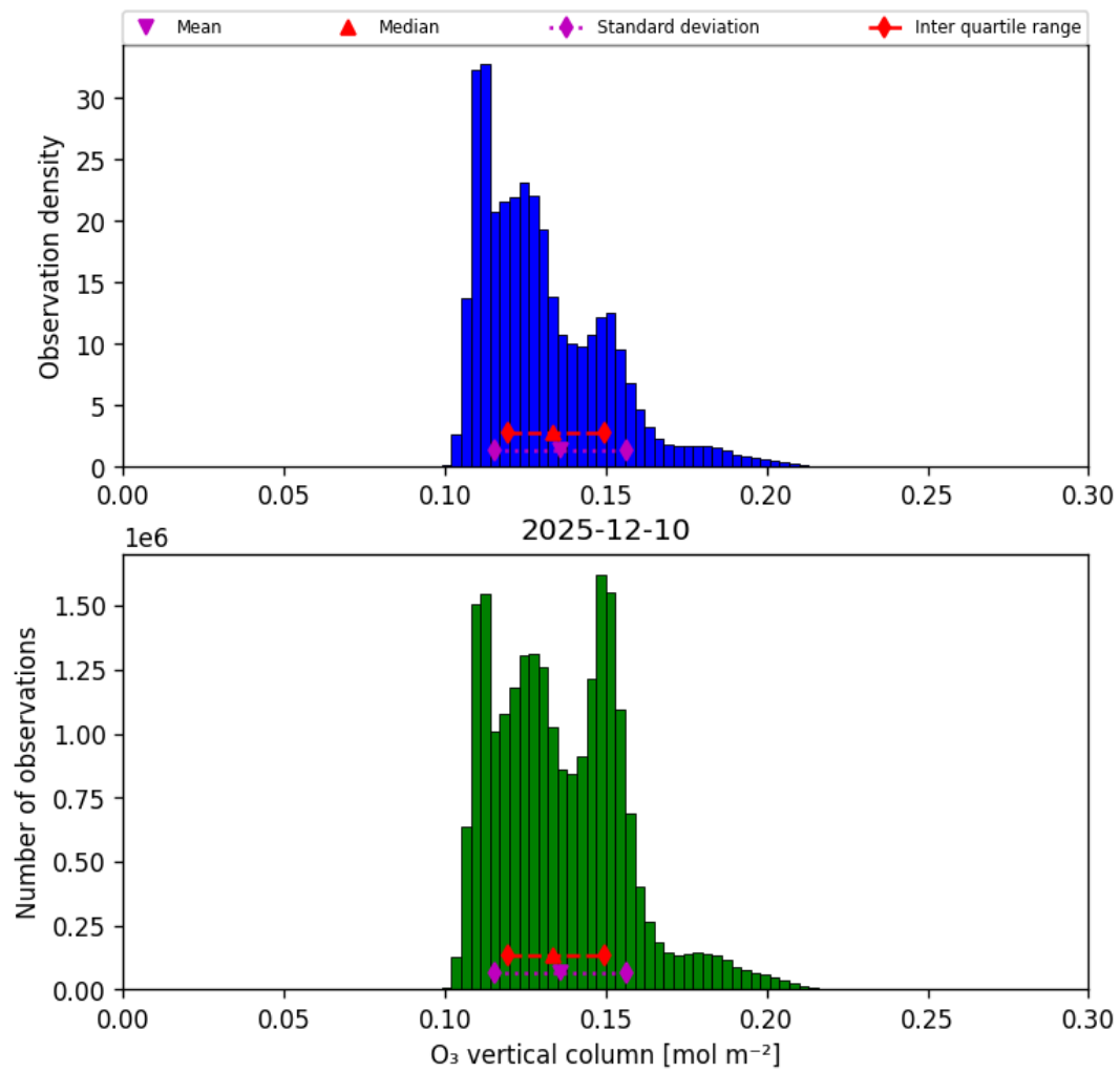
Figure 29: Histogram of “O 3 vertical column” for 2025-12-10 to 2025-12-11
