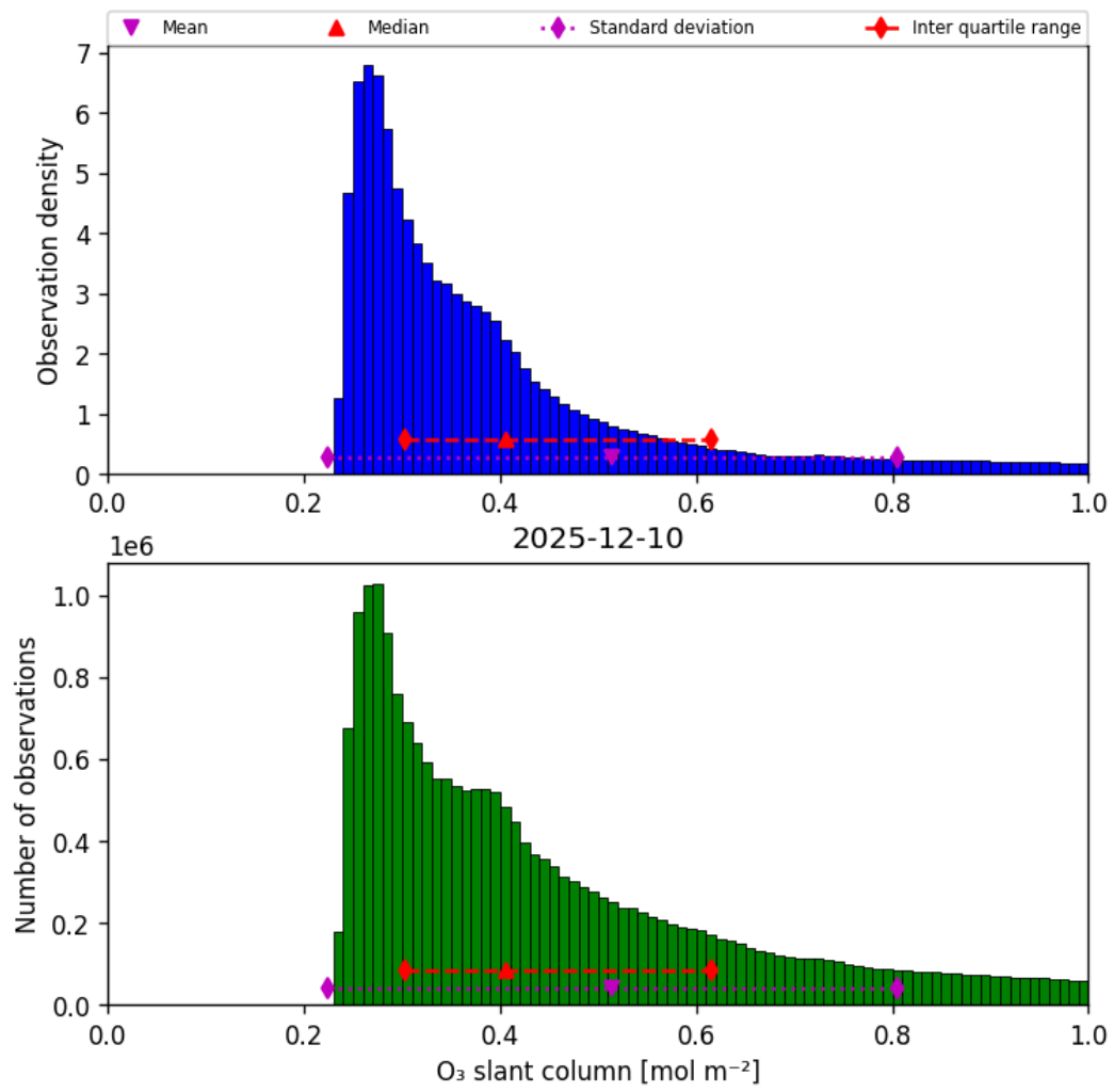
Figure 31: Histogram of “O 3 slant column” for 2025-12-10 to 2025-12-11
