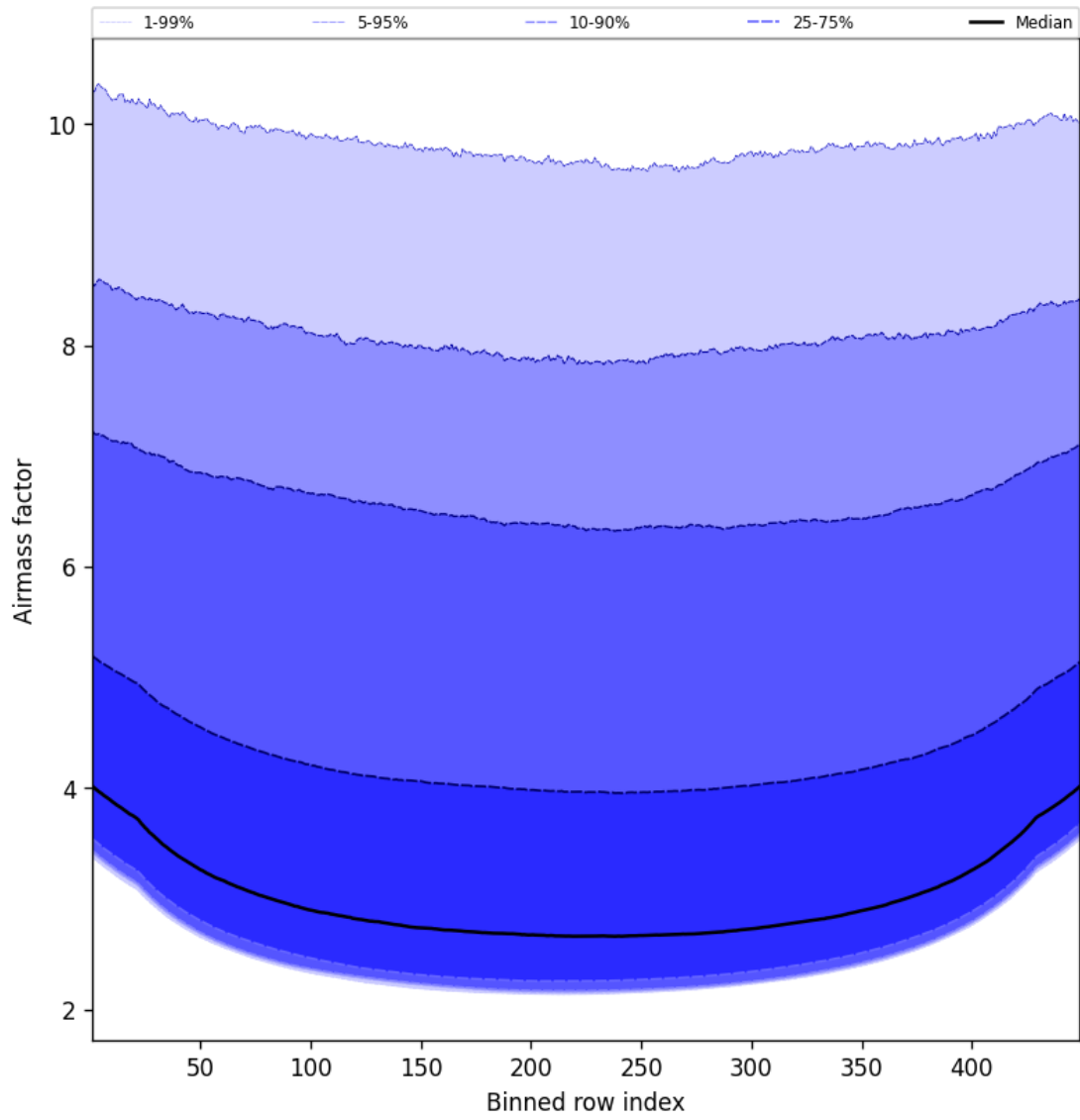
Figure 49: Along track statistics of “Airmass factor” for 2025-12-10 to 2025-12-11
