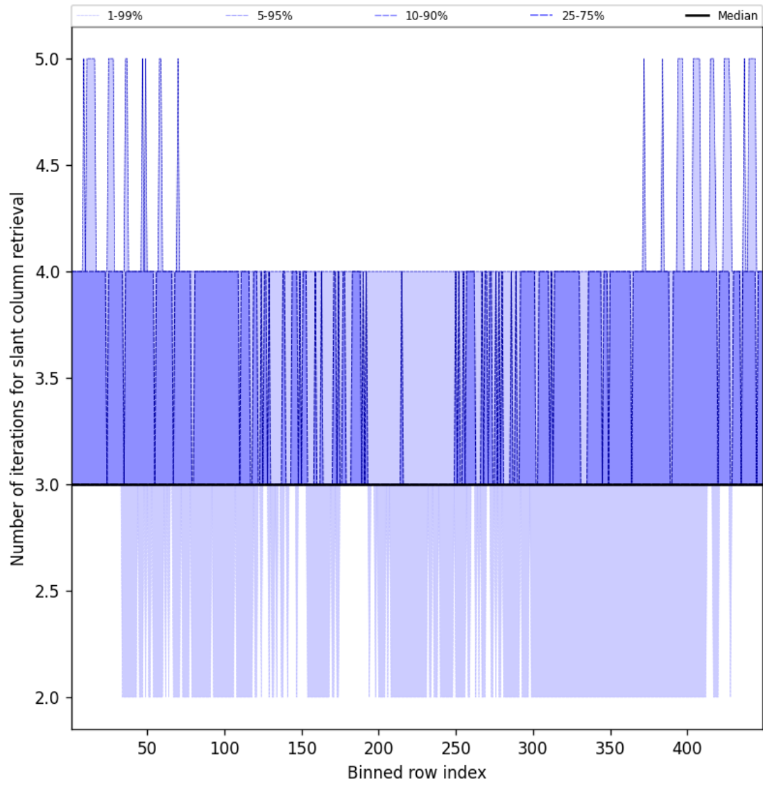
Figure 45: Along track statistics of “Number of iterations for slant column retrieval” for 2025-12-10 to 2025-12-11
