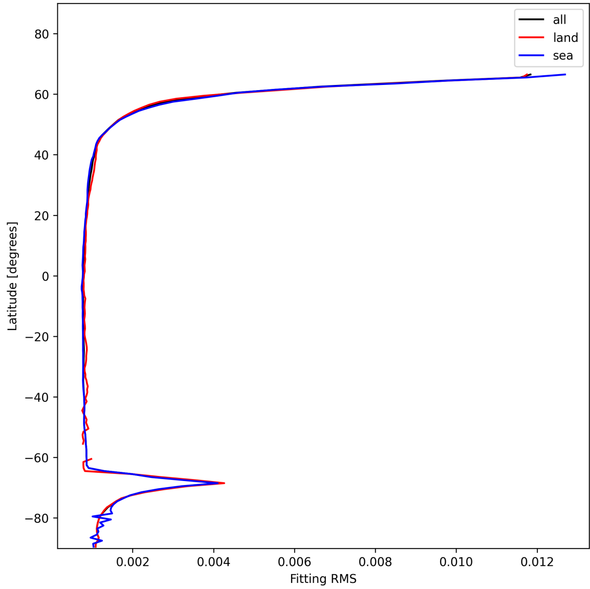
Figure 22: Zonal average of “Fitting RMS” for 2025-12-10 to 2025-12-11.
