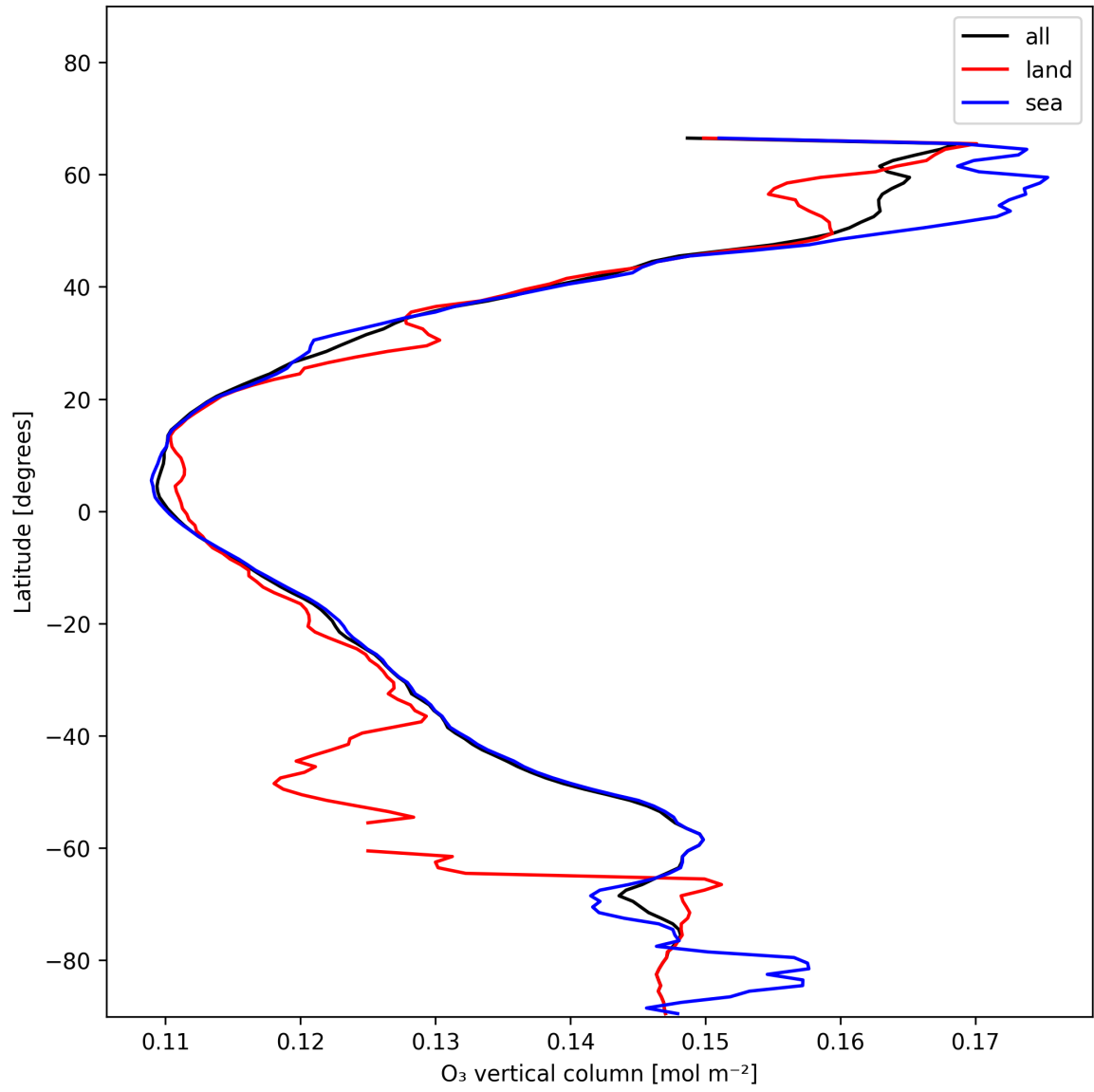
Figure 17: Zonal average of “O 3 vertical column” for 2025-12-10 to 2025-12-11.
