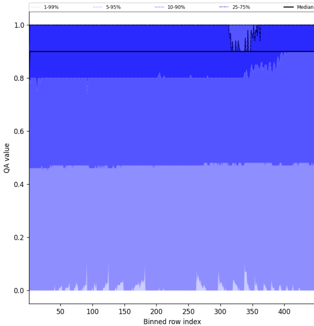
Figure 40: Along track statistics of “QA value” for 2025-12-10 to 2025-12-11
