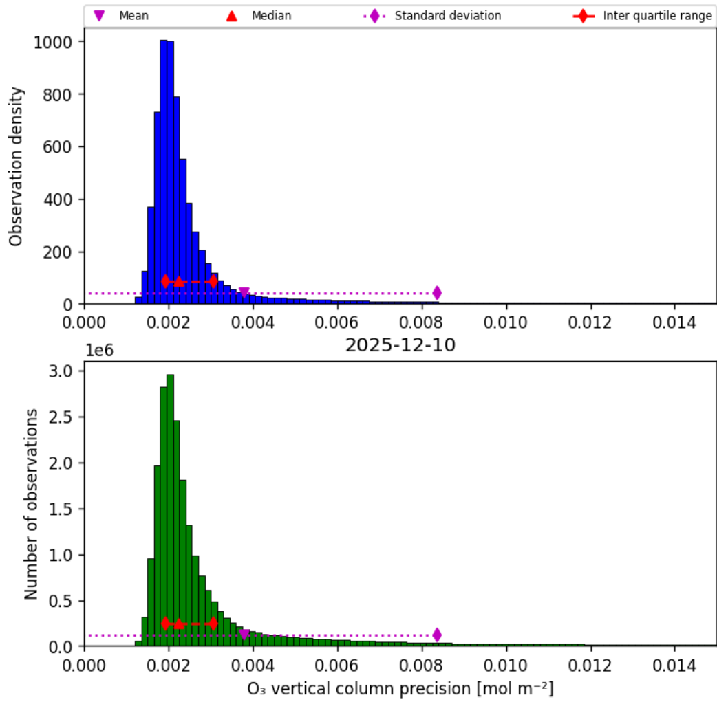
Figure 30: Histogram of “O 3 vertical column precision” for 2025-12-10 to 2025-12-11
