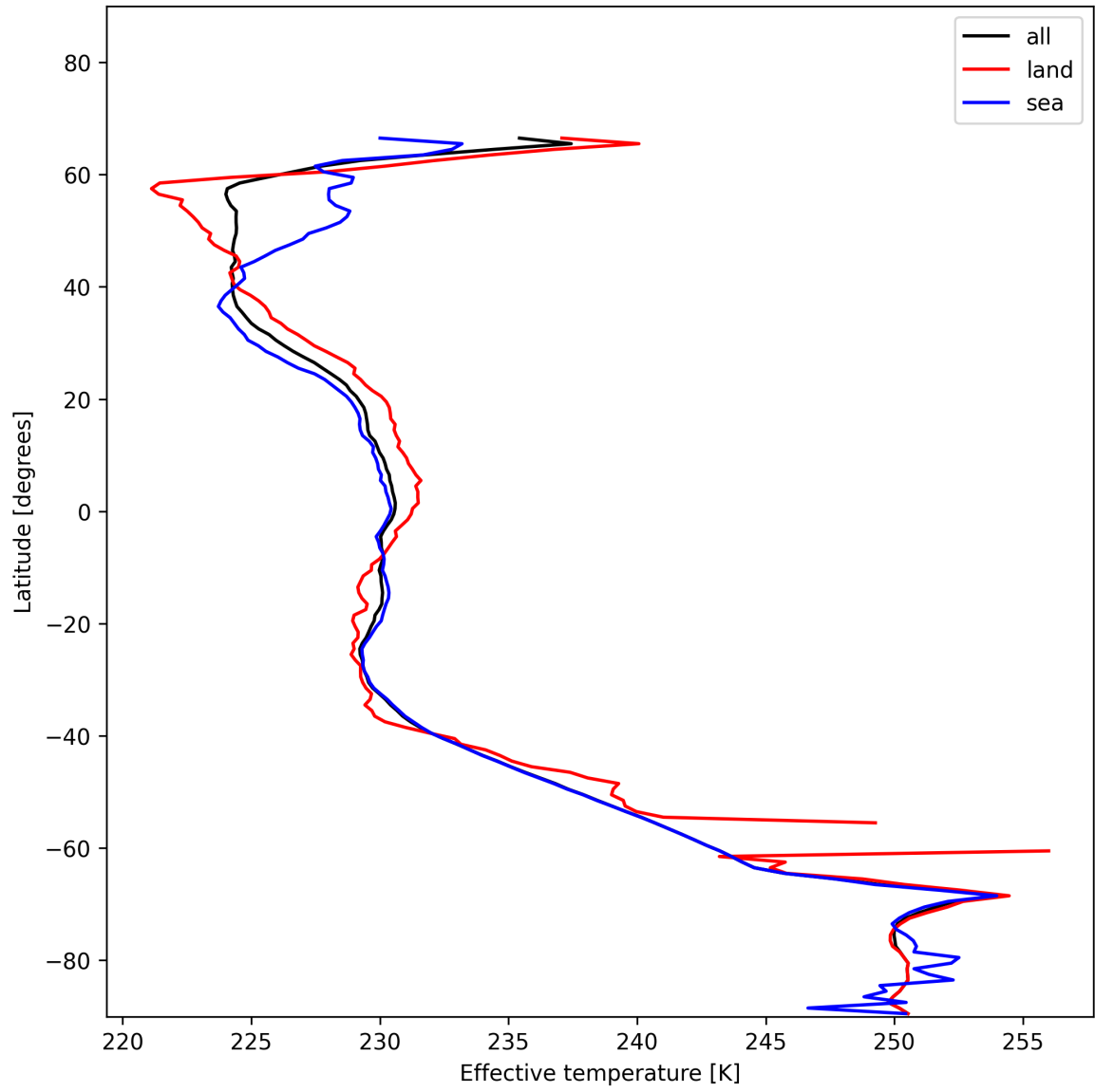
Figure 26: Zonal average of “Effective temperature” for 2025-12-10 to 2025-12-11.
