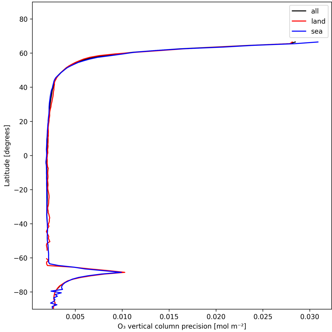
Figure 18: Zonal average of “O 3 vertical column precision” for 2025-12-10 to 2025-12-11.
