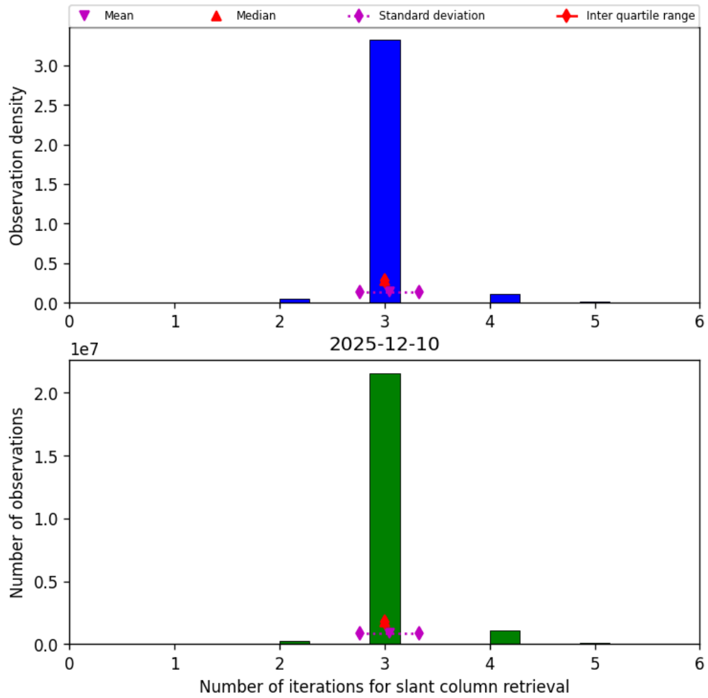
Figure 33: Histogram of “Number of iterations for slant column retrieval” for 2025-12-10 to 2025-12-11
