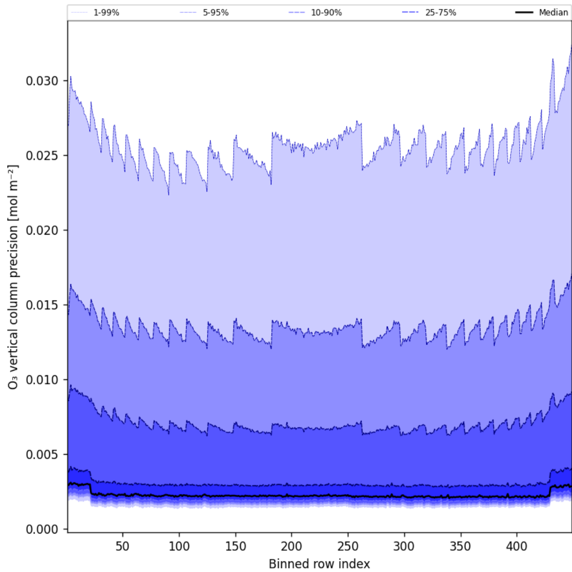
Figure 42: Along track statistics of “O 3 vertical column precision” for 2025-12-10 to 2025-12-11
