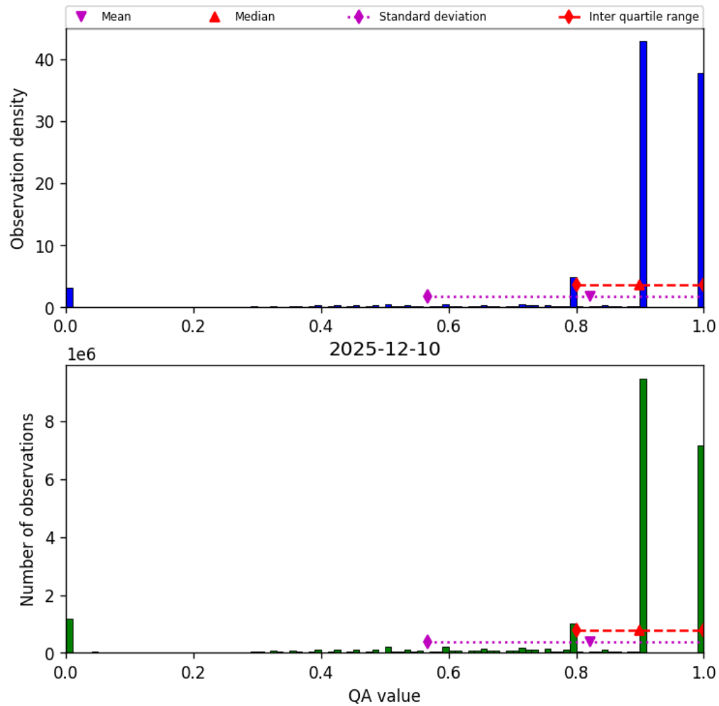
Figure 28: Histogram of “QA value” for 2025-12-10 to 2025-12-11
