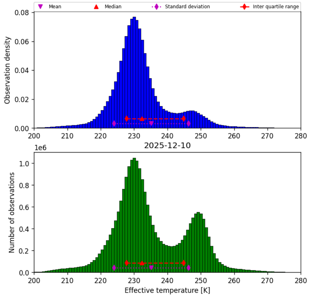
Figure 38: Histogram of “Effective temperature” for 2025-12-10 to 2025-12-11
