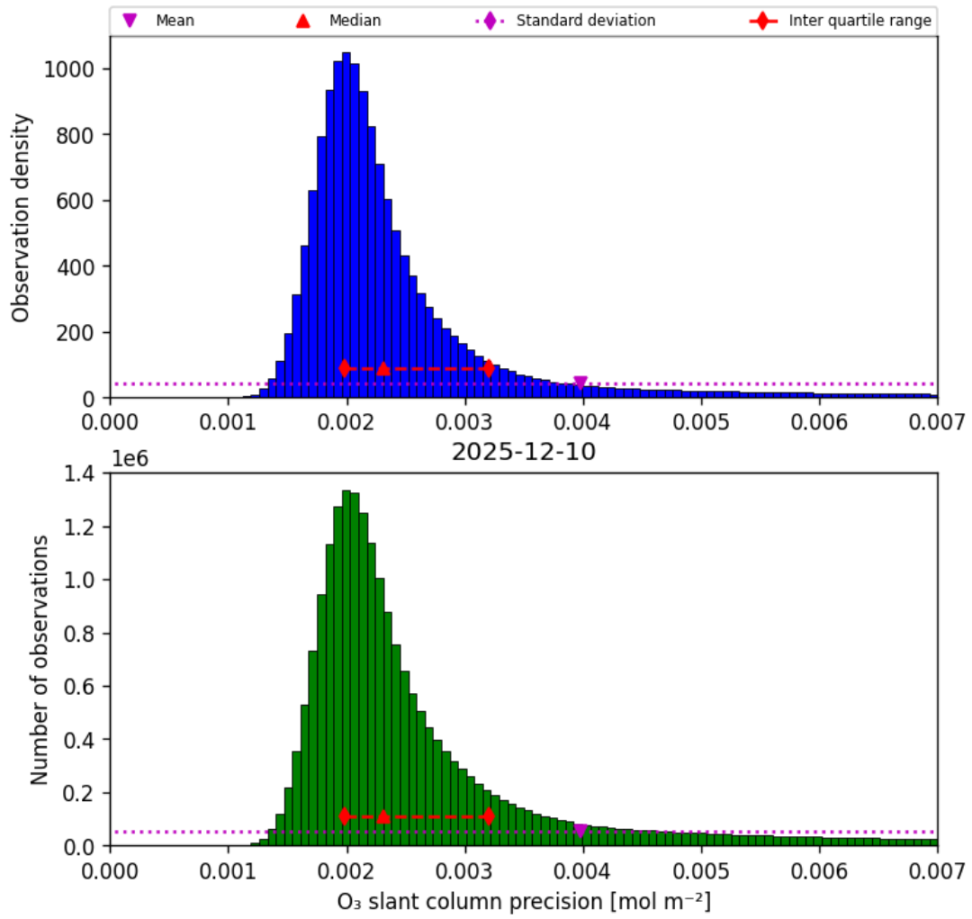
Figure 32: Histogram of “O 3 slant column precision” for 2025-12-10 to 2025-12-11
