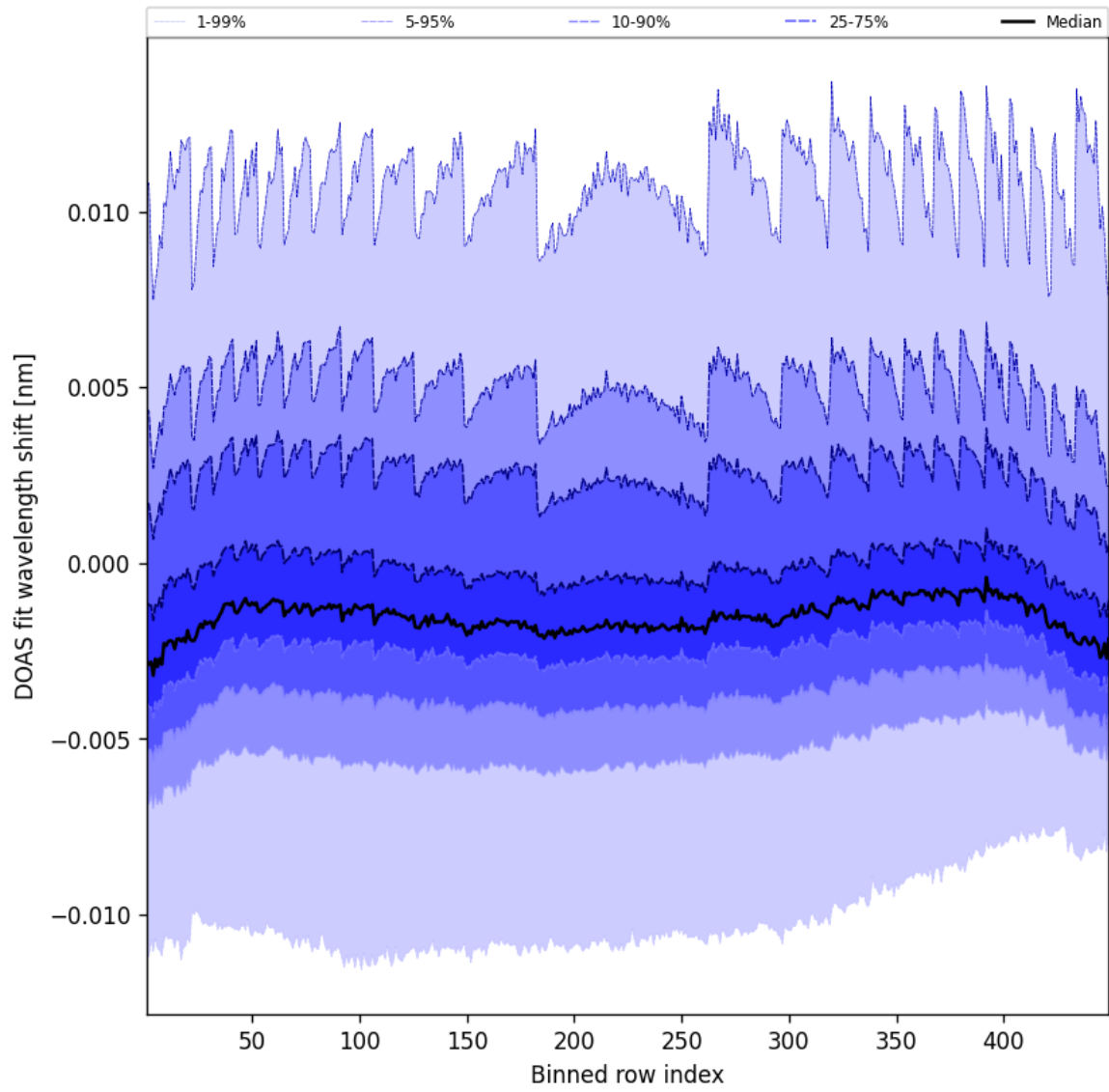
Figure 47: Along track statistics of “DOAS fit wavelength shift” for 2025-12-10 to 2025-12-11
