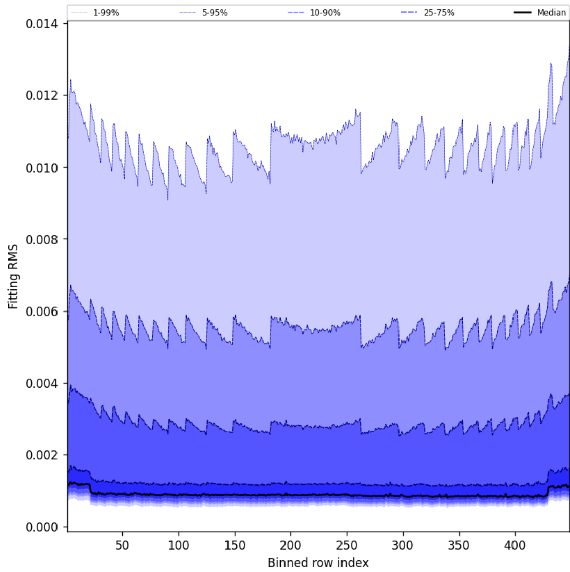
Figure 46: Along track statistics of “Fitting RMS” for 2025-12-10 to 2025-12-11
