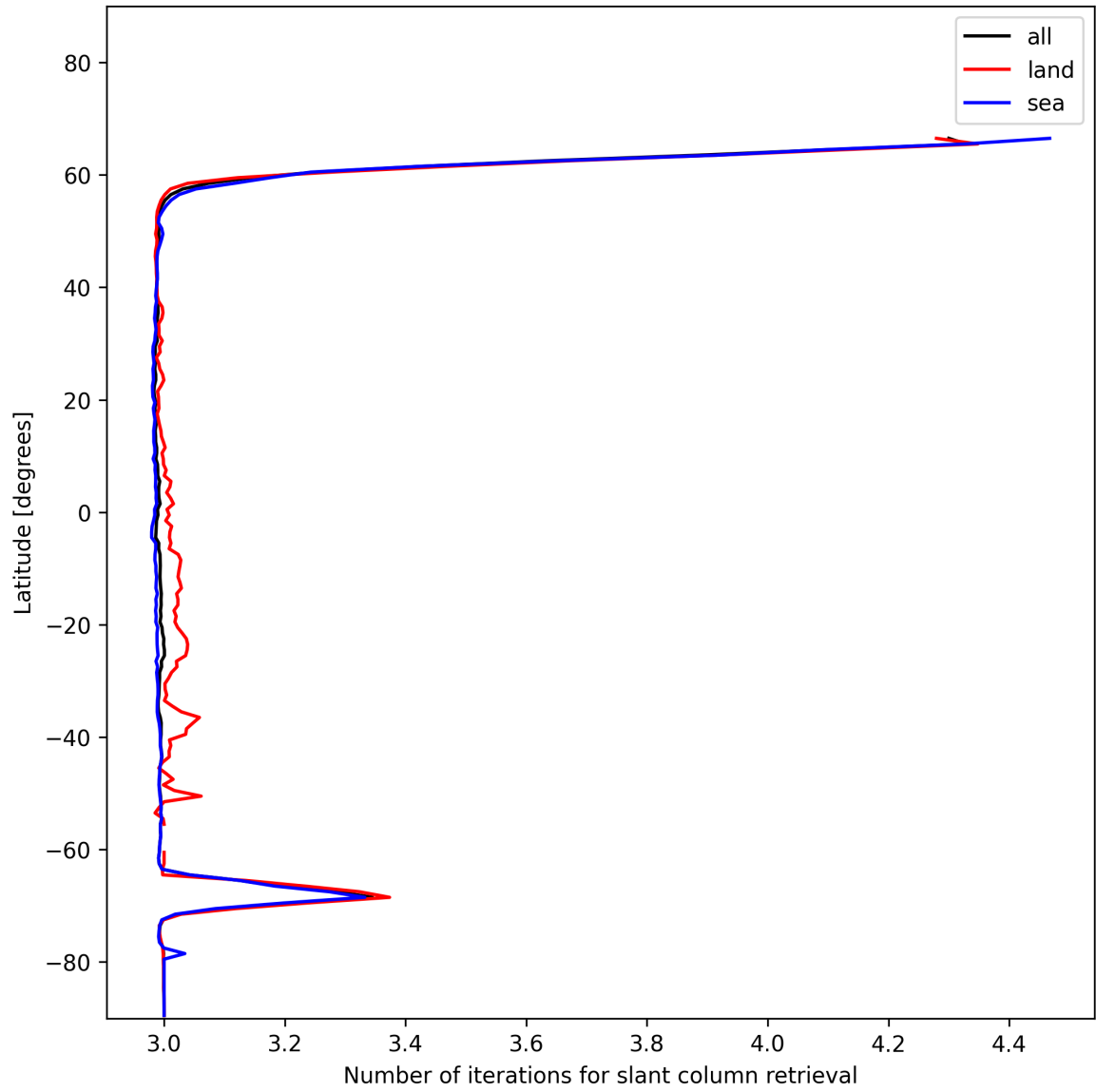
Figure 21: Zonal average of “Number of iterations for slant column retrieval” for 2025-12-10 to 2025-12-11.
