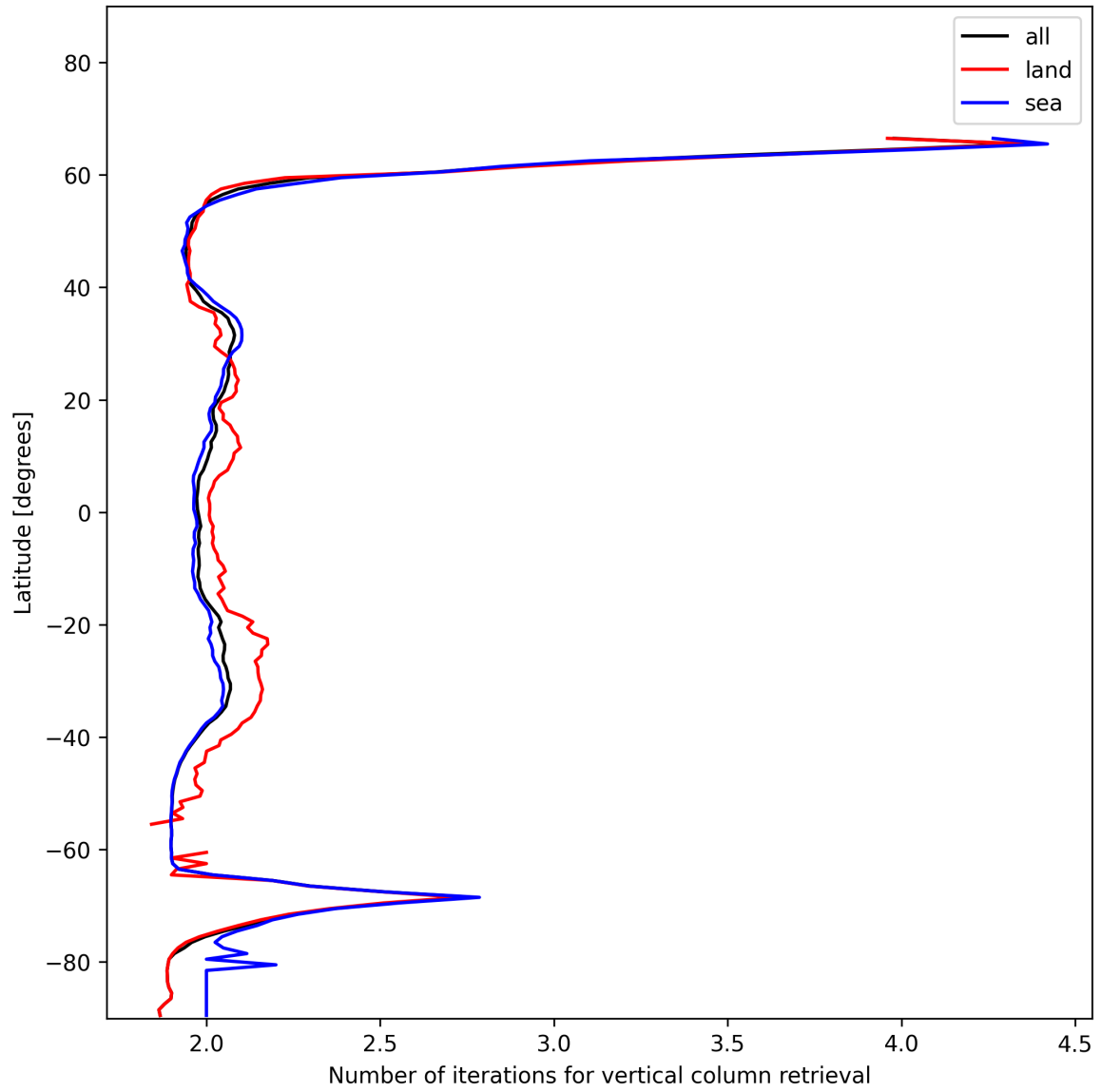
Figure 27: Zonal average of “Number of iterations for vertical column retrieval” for 2025-12-10 to 2025-12-11.
