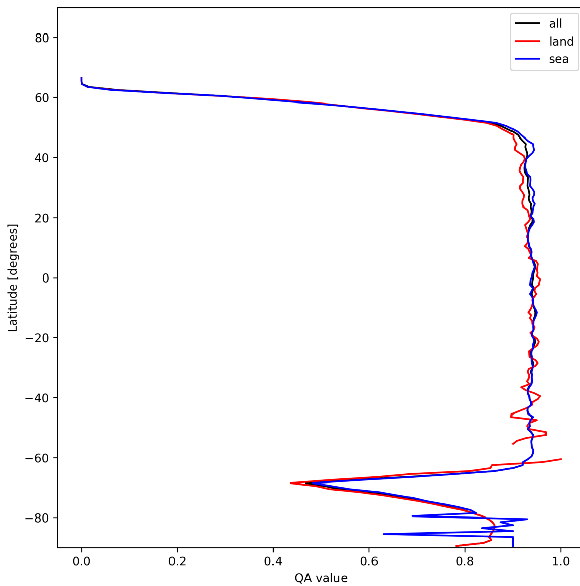
Figure 16: Zonal average of “QA value” for 2025-12-10 to 2025-12-11.
