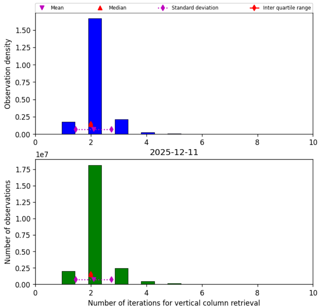
Figure 39: Histogram of “Number of iterations for vertical column retrieval” for 2025-12-11 to 2025-12-12
