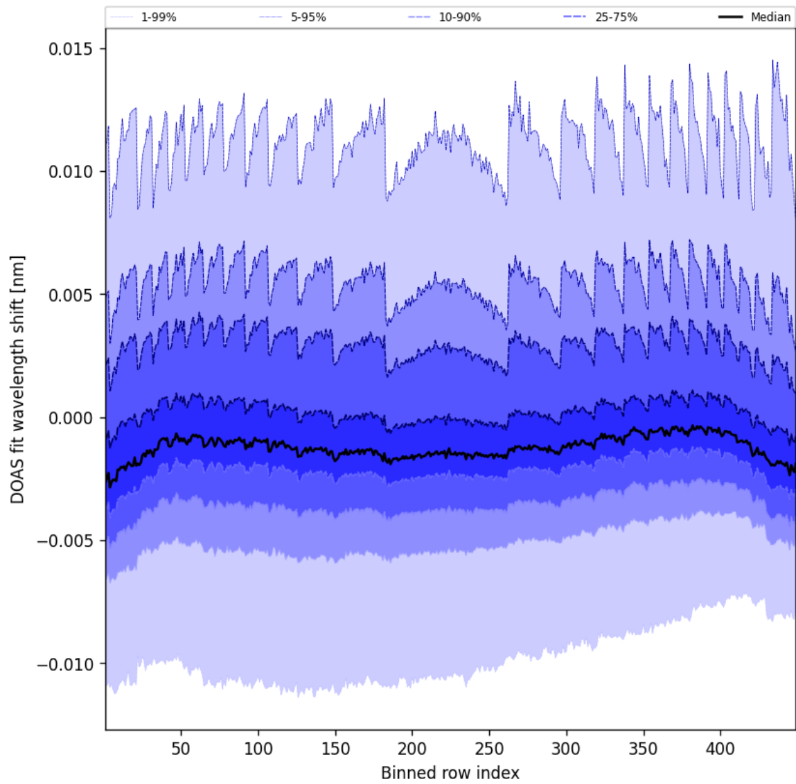
Figure 47: Along track statistics of “DOAS fit wavelength shift” for 2025-12-11 to 2025-12-12
