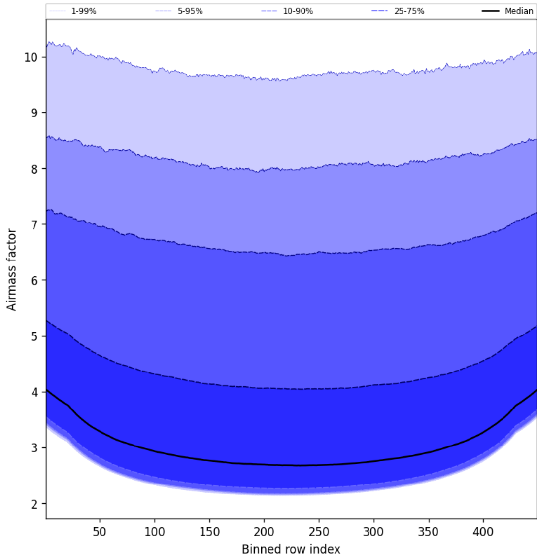
Figure 49: Along track statistics of “Airmass factor” for 2025-12-11 to 2025-12-12
