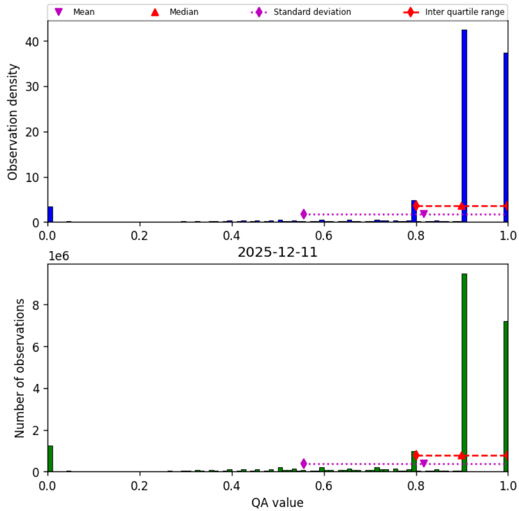
Figure 28: Histogram of “QA value” for 2025-12-11 to 2025-12-12
