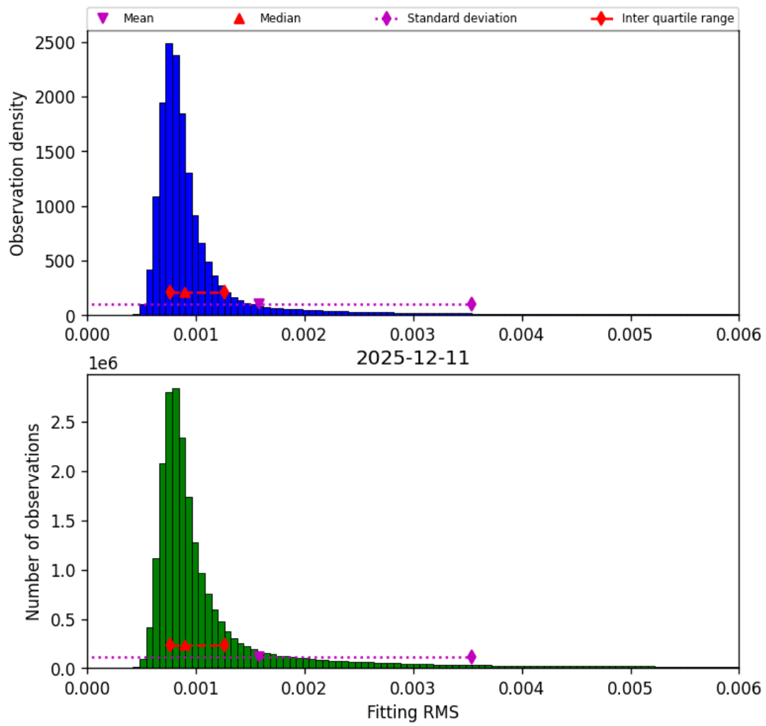
Figure 34: Histogram of “Fitting RMS” for 2025-12-11 to 2025-12-12
