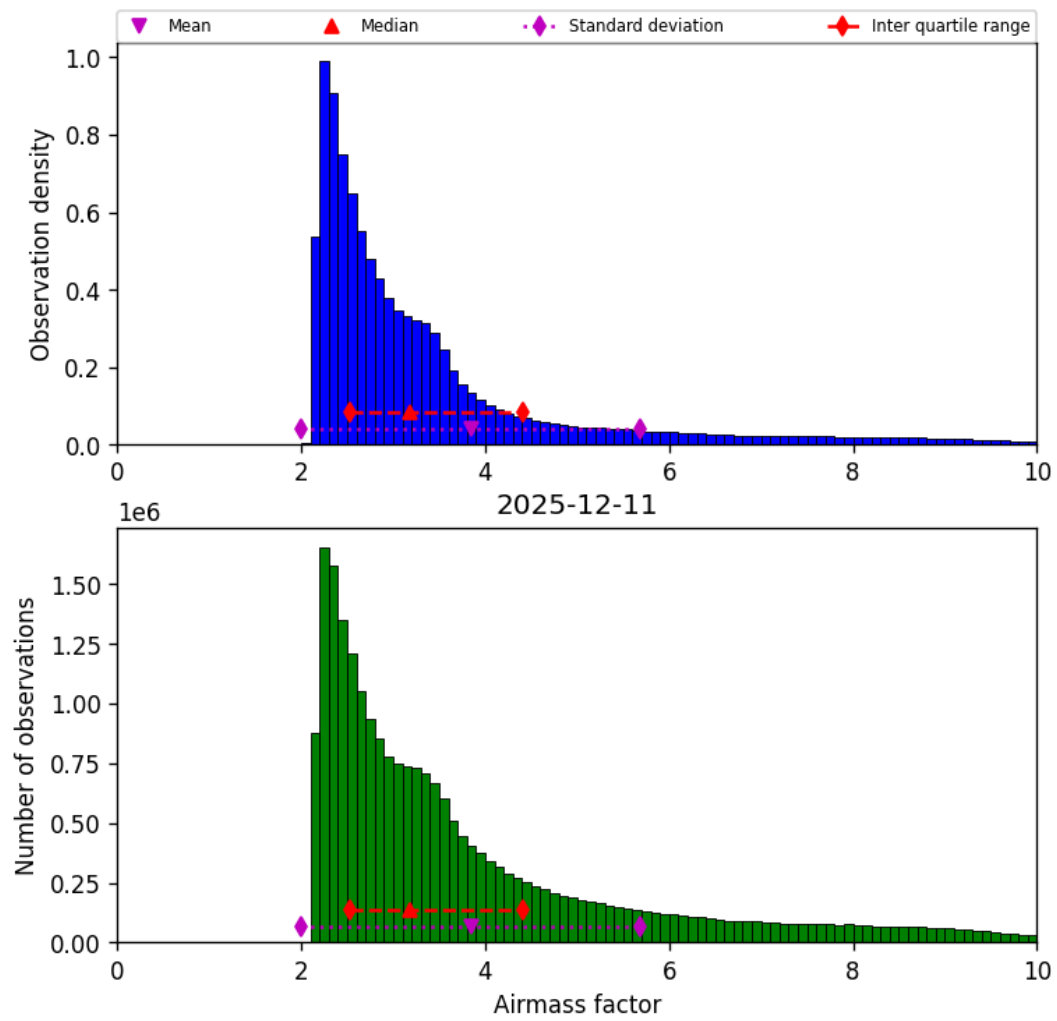
Figure 37: Histogram of “Airmass factor” for 2025-12-11 to 2025-12-12
