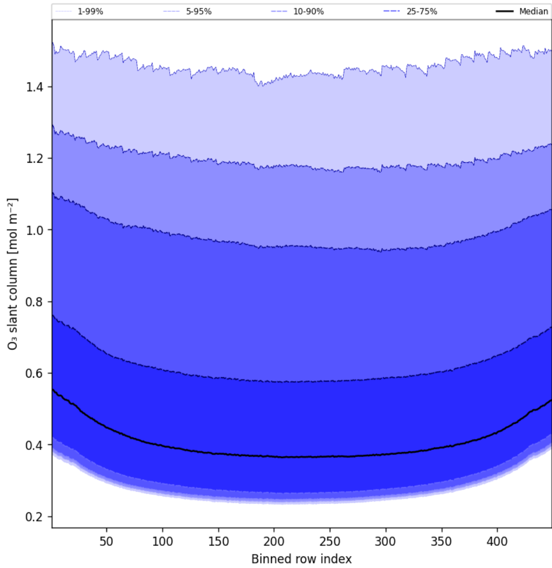
Figure 43: Along track statistics of “O 3 slant column” for 2025-12-11 to 2025-12-12
