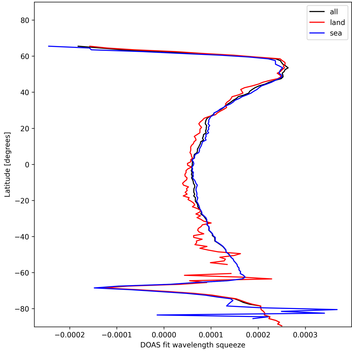
Figure 24: Zonal average of “DOAS fit wavelength squeeze” for 2025-12-11 to 2025-12-12.
