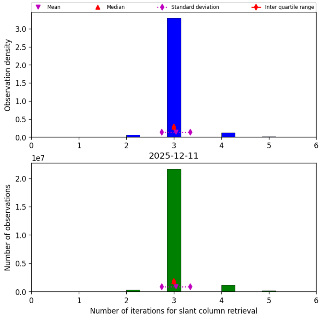
Figure 33: Histogram of “Number of iterations for slant column retrieval” for 2025-12-11 to 2025-12-12
