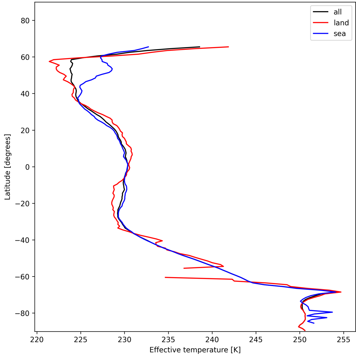
Figure 26: Zonal average of “Effective temperature” for 2025-12-11 to 2025-12-12.
