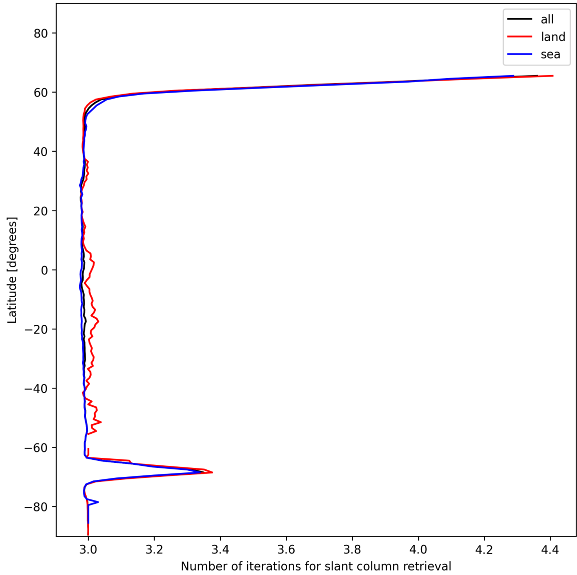
Figure 21: Zonal average of “Number of iterations for slant column retrieval” for 2025-12-11 to 2025-12-12.
