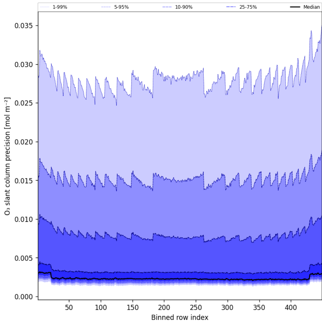
Figure 44: Along track statistics of “O 3 slant column precision” for 2025-12-11 to 2025-12-12
