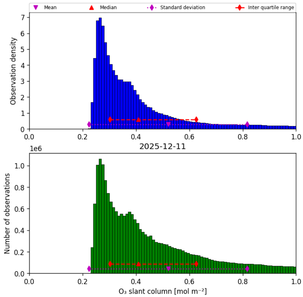
Figure 31: Histogram of “O 3 slant column” for 2025-12-11 to 2025-12-12
