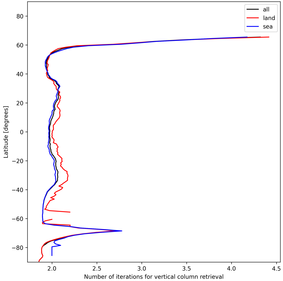
Figure 27: Zonal average of “Number of iterations for vertical column retrieval” for 2025-12-11 to 2025-12-12.
