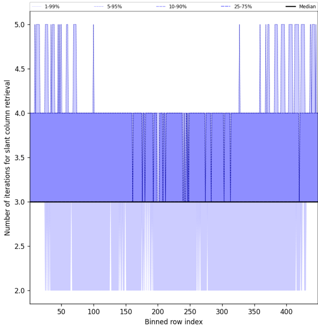
Figure 45: Along track statistics of “Number of iterations for slant column retrieval” for 2025-12-11 to 2025-12-12
