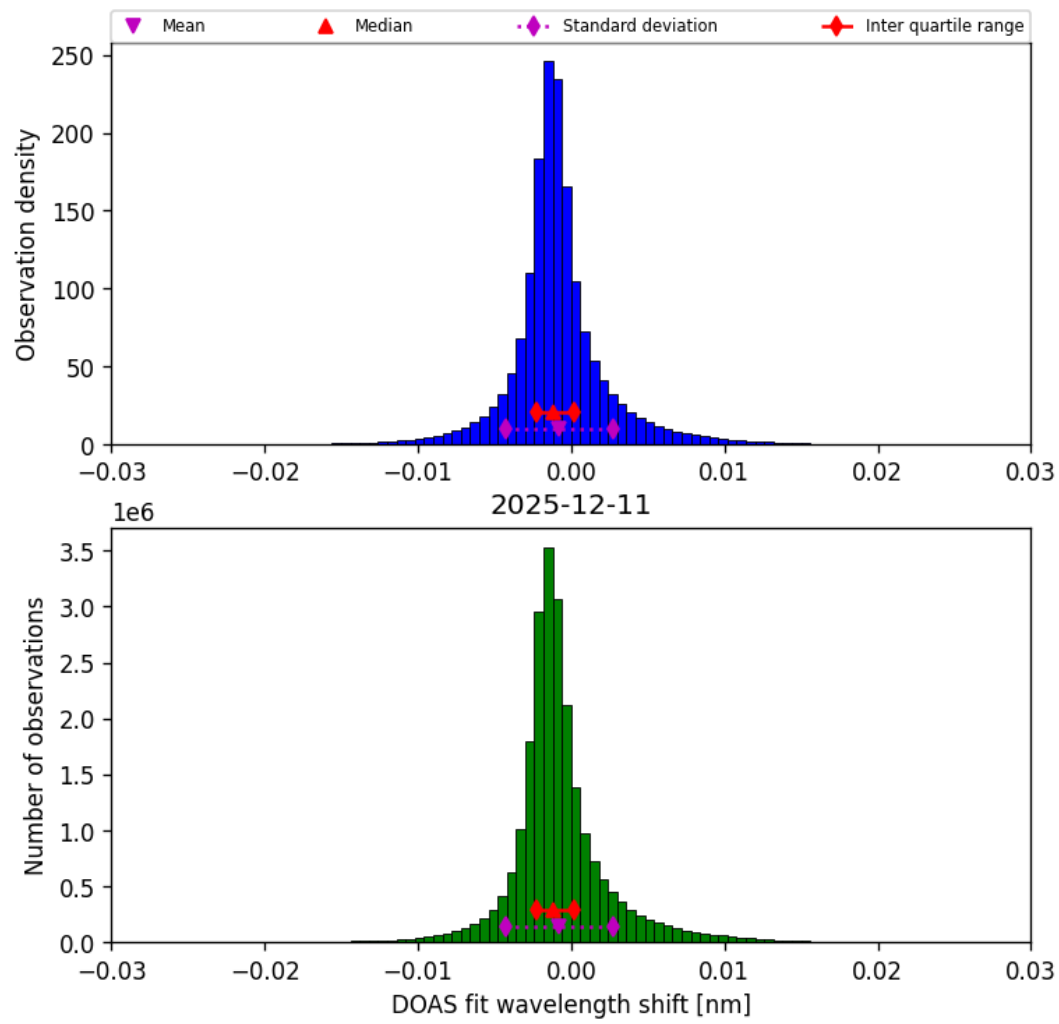
Figure 35: Histogram of “DOAS fit wavelength shift” for 2025-12-11 to 2025-12-12
