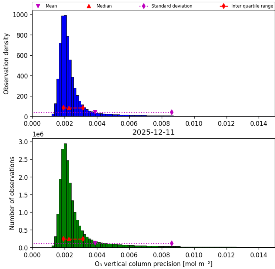
Figure 30: Histogram of “O 3 vertical column precision” for 2025-12-11 to 2025-12-12
