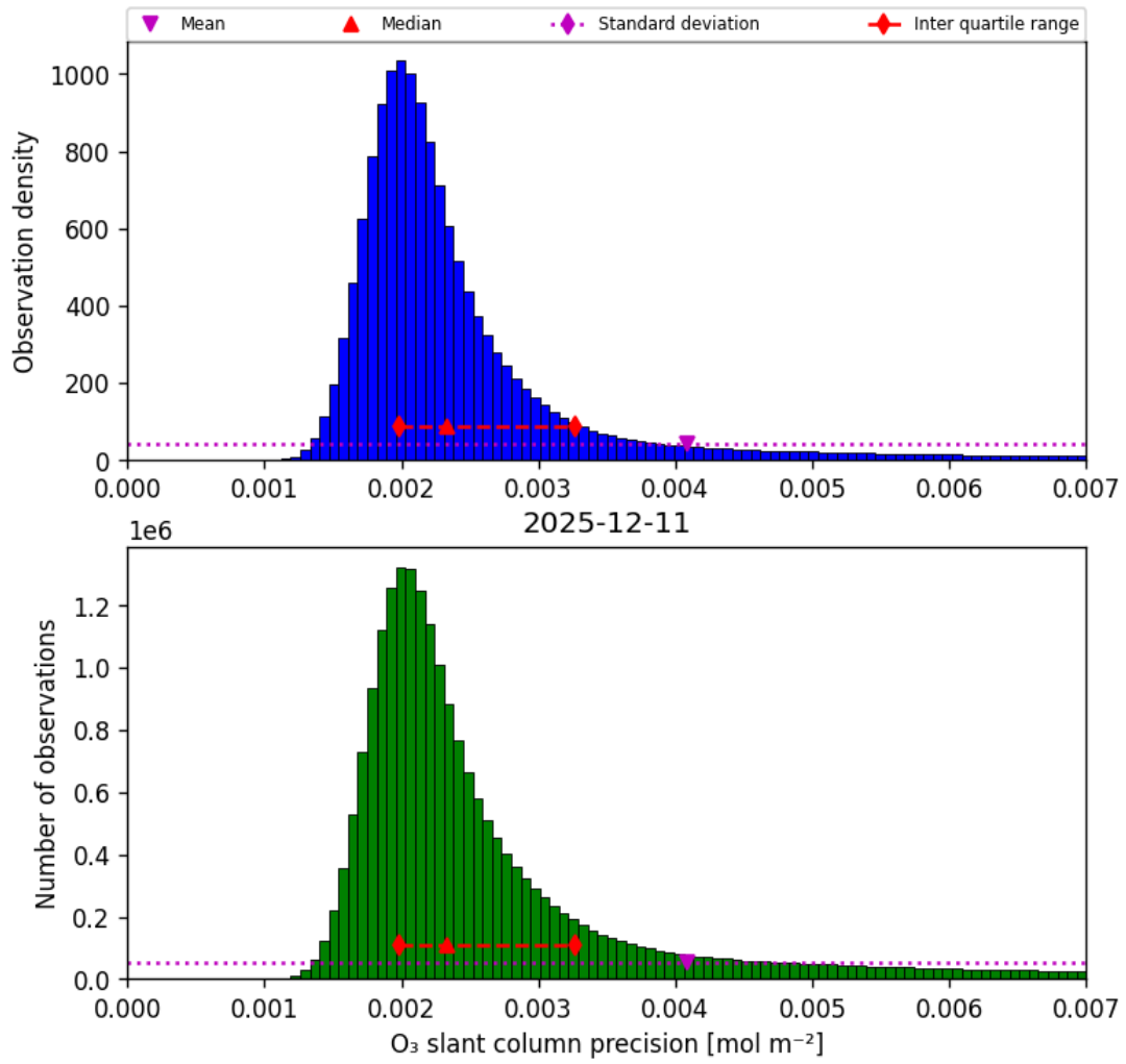
Figure 32: Histogram of “O 3 slant column precision” for 2025-12-11 to 2025-12-12
