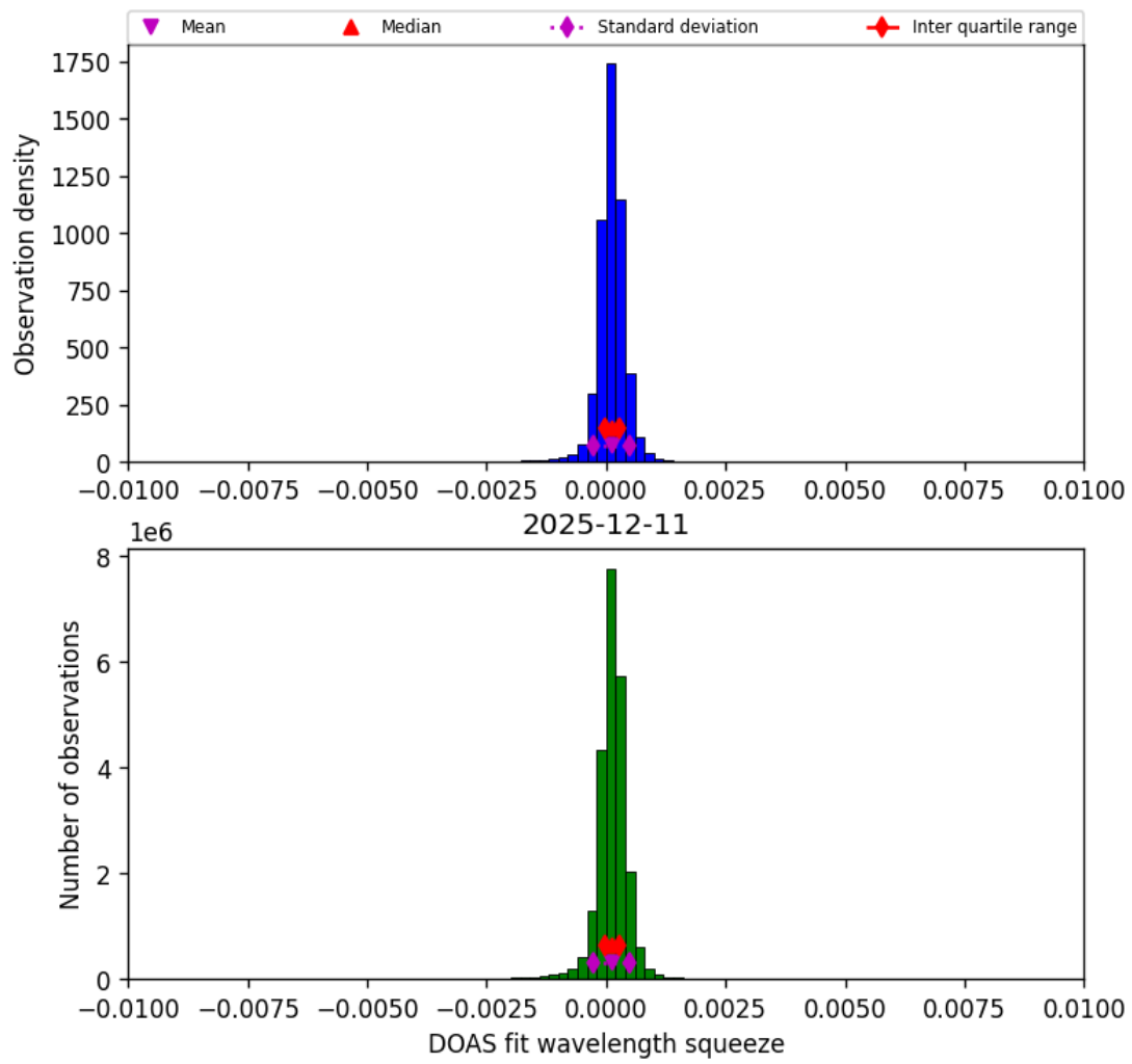
Figure 36: Histogram of “DOAS fit wavelength squeeze” for 2025-12-11 to 2025-12-12
