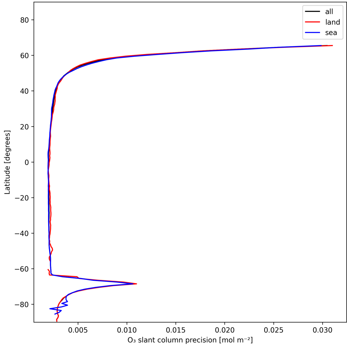
Figure 20: Zonal average of “O 3 slant column precision” for 2025-12-11 to 2025-12-12.
