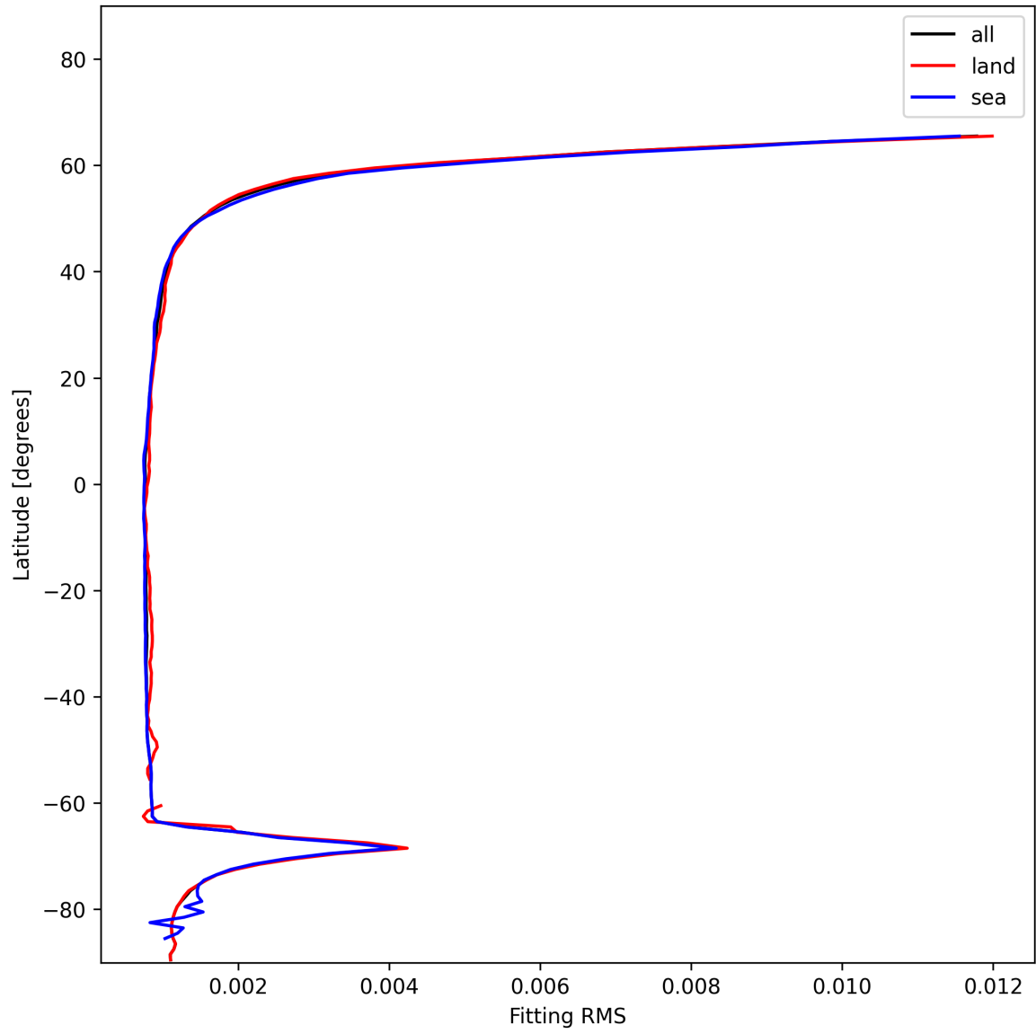
Figure 22: Zonal average of “Fitting RMS” for 2025-12-11 to 2025-12-12.
