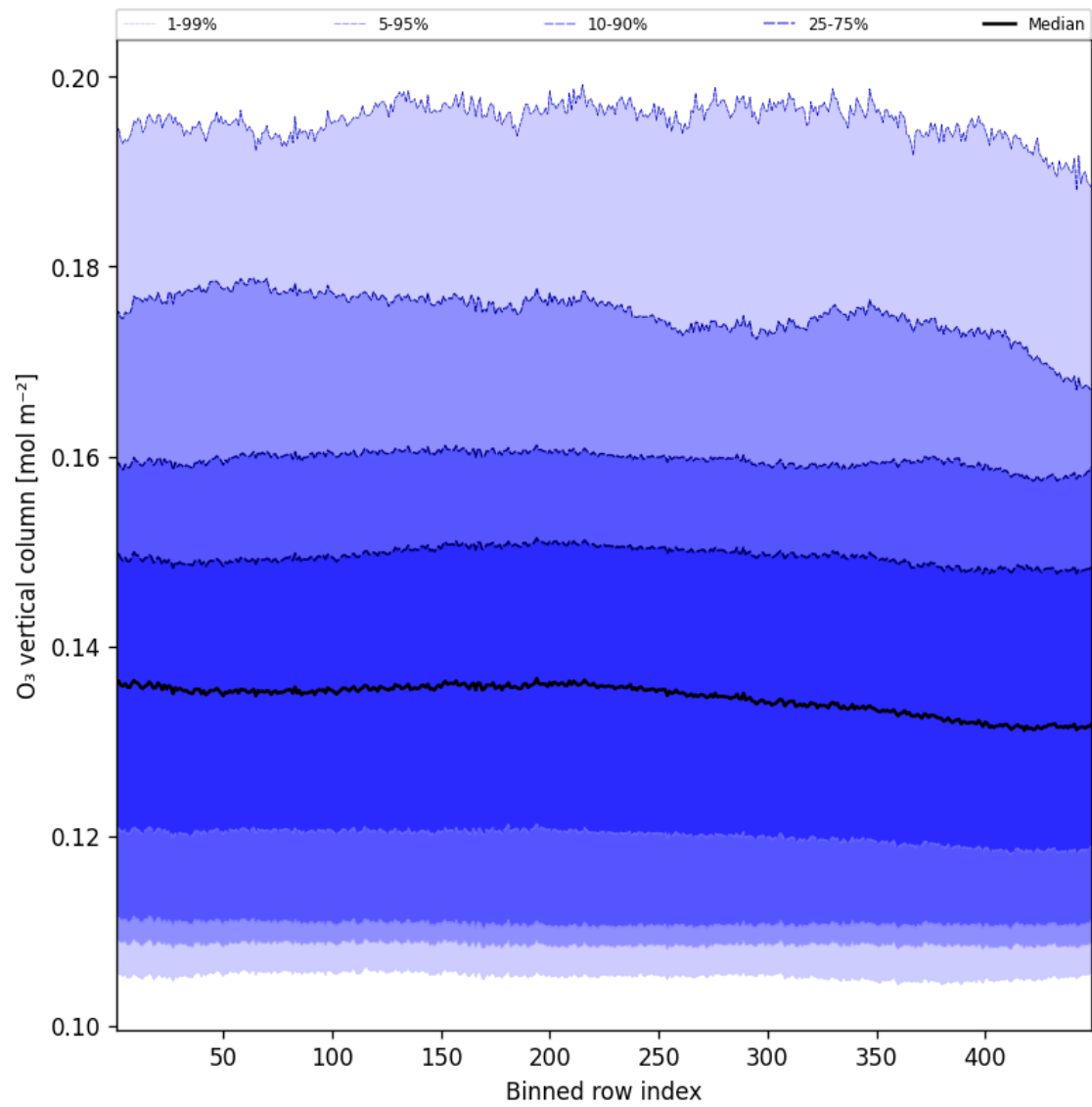
Figure 41: Along track statistics of “O 3 vertical column” for 2025-12-11 to 2025-12-12
