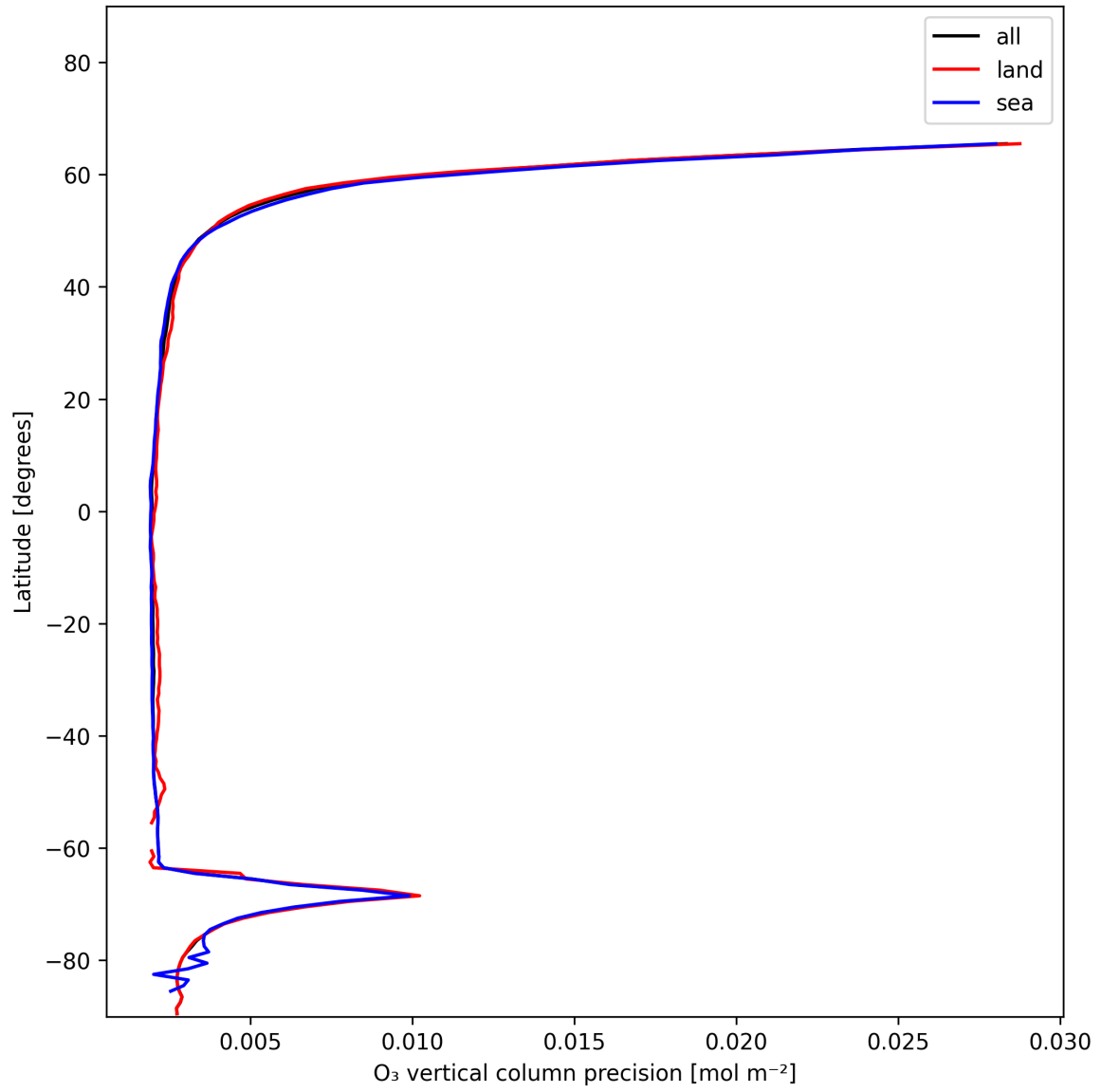
Figure 18: Zonal average of “O 3 vertical column precision” for 2025-12-11 to 2025-12-12.
