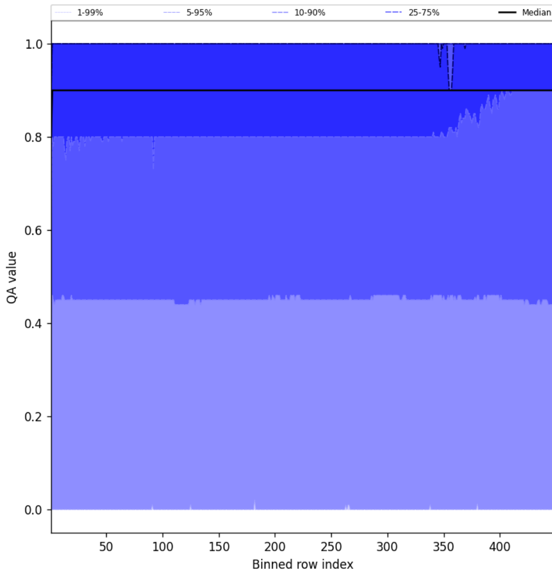
Figure 40: Along track statistics of “QA value” for 2025-12-11 to 2025-12-12
