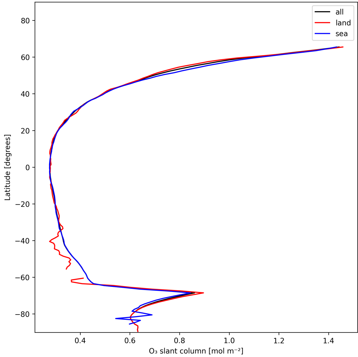
Figure 19: Zonal average of “O 3 slant column” for 2025-12-11 to 2025-12-12.
