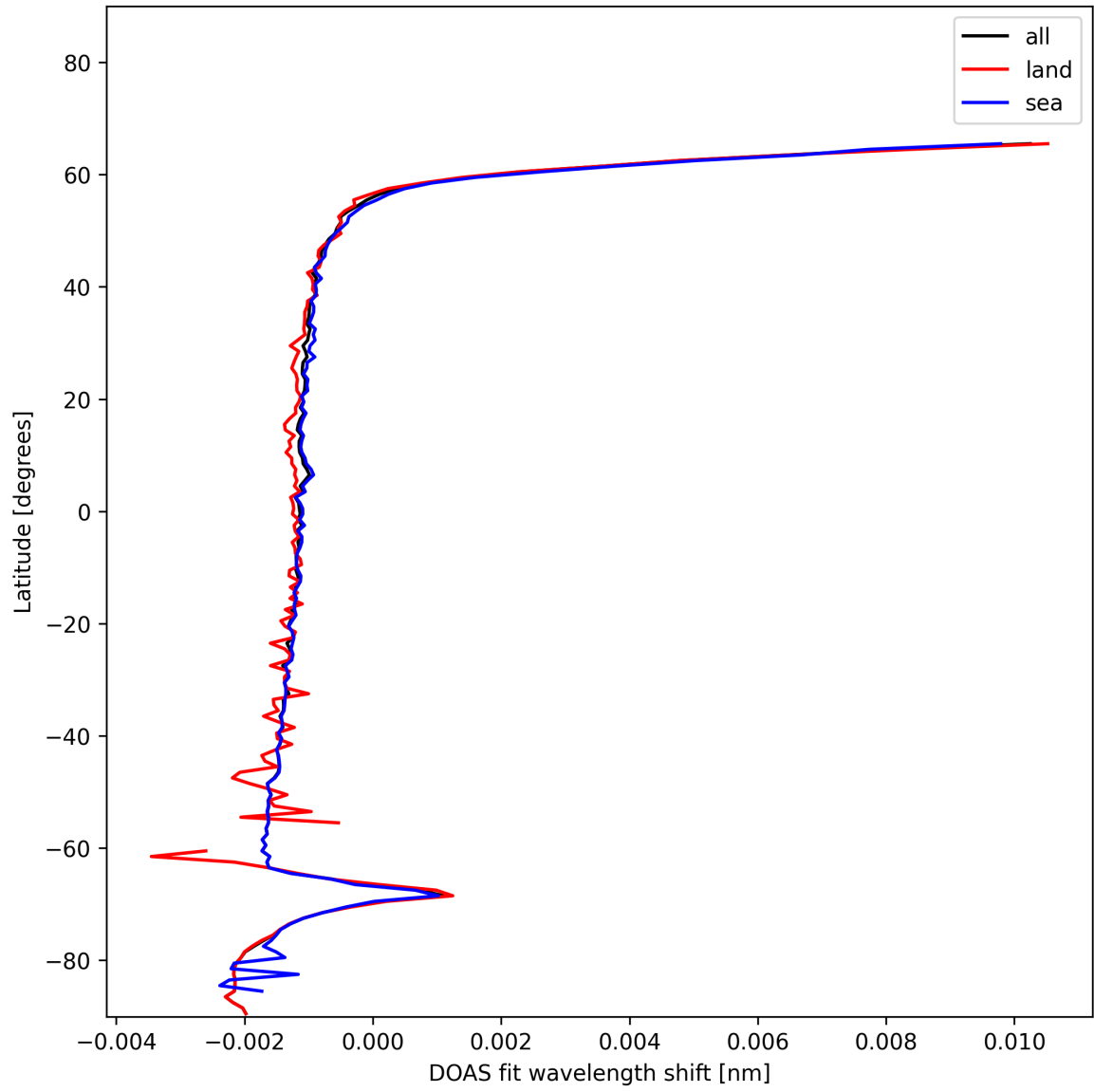
Figure 23: Zonal average of “DOAS fit wavelength shift” for 2025-12-11 to 2025-12-12.
