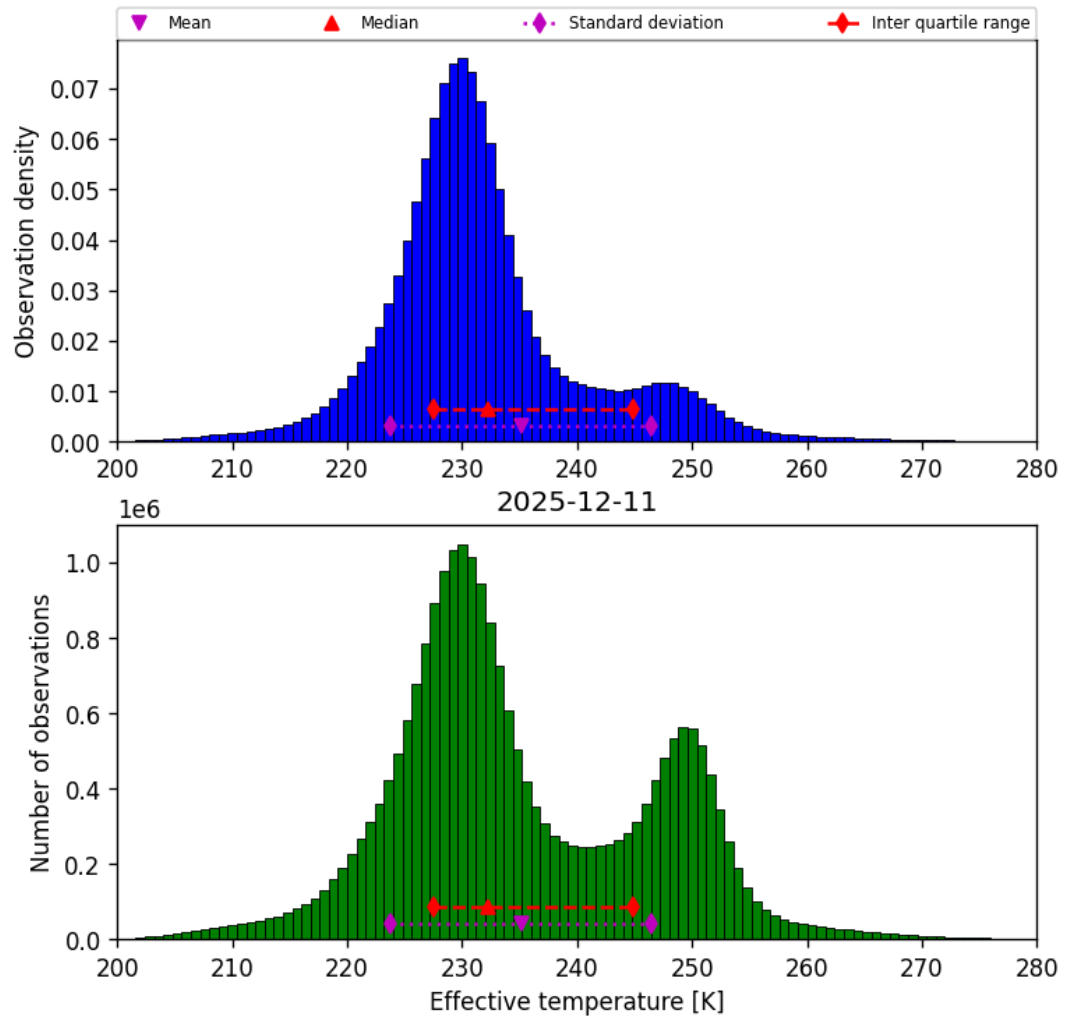
Figure 38: Histogram of “Effective temperature” for 2025-12-11 to 2025-12-12
