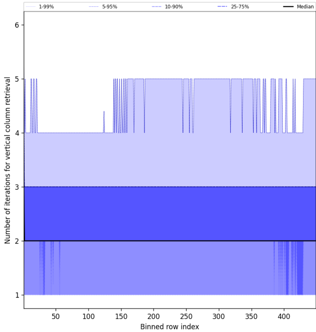
Figure 51: Along track statistics of “Number of iterations for vertical column retrieval” for 2025-12-11 to 2025-12-12
