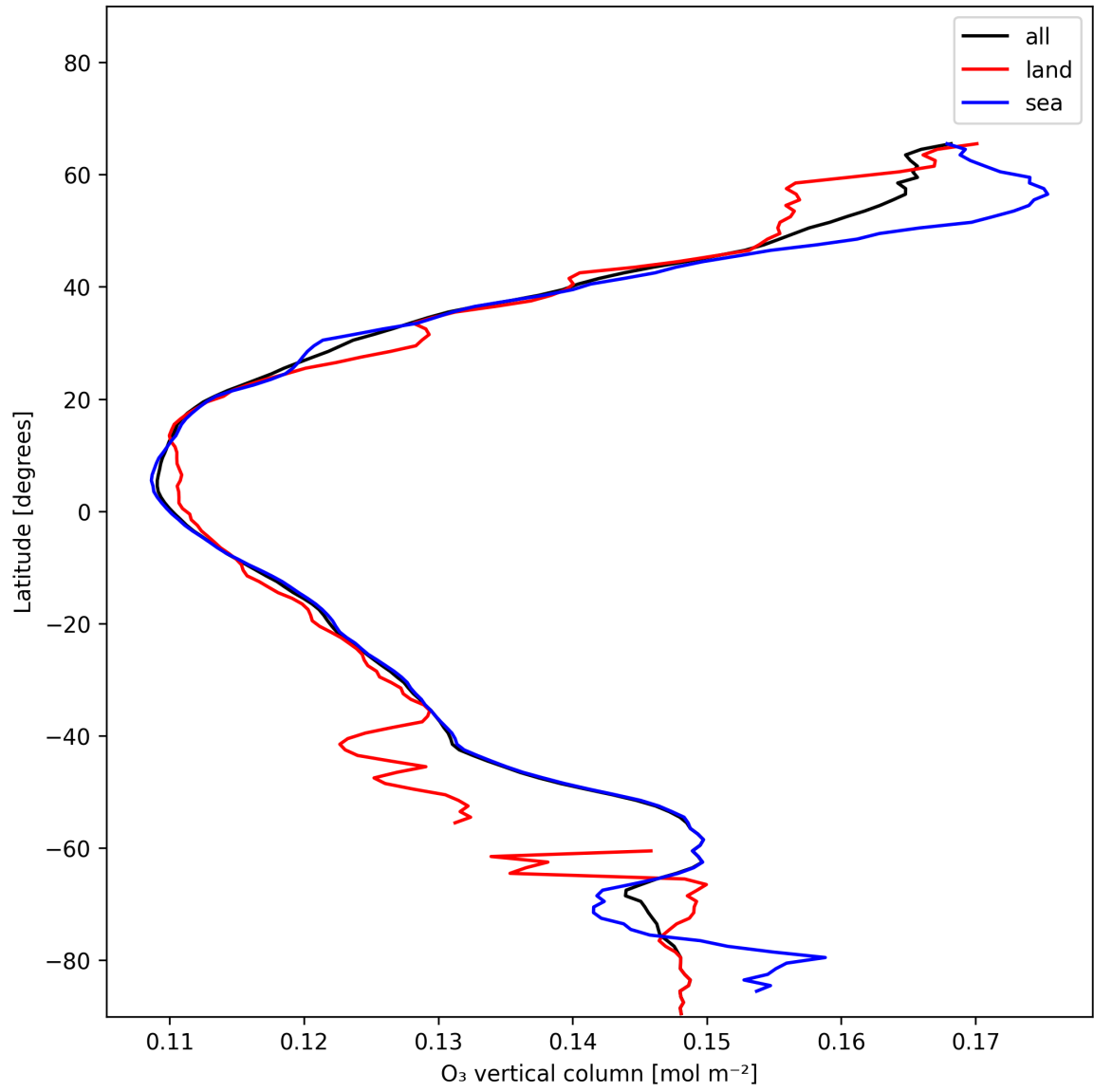
Figure 17: Zonal average of “O 3 vertical column” for 2025-12-11 to 2025-12-12.
