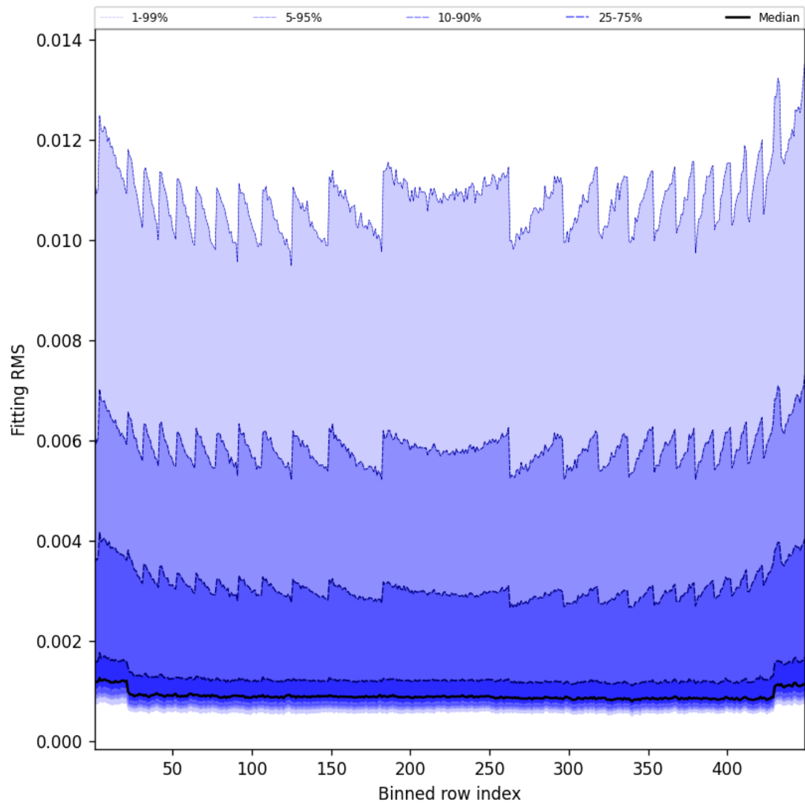
Figure 46: Along track statistics of “Fitting RMS” for 2025-12-11 to 2025-12-12
