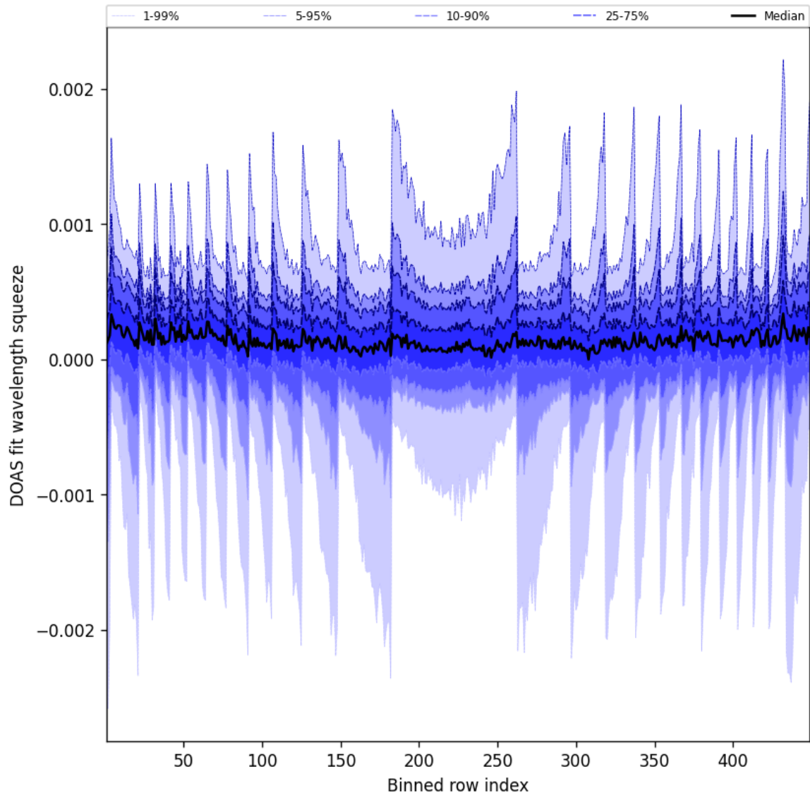
Figure 48: Along track statistics of “DOAS fit wavelength squeeze” for 2025-12-11 to 2025-12-12
