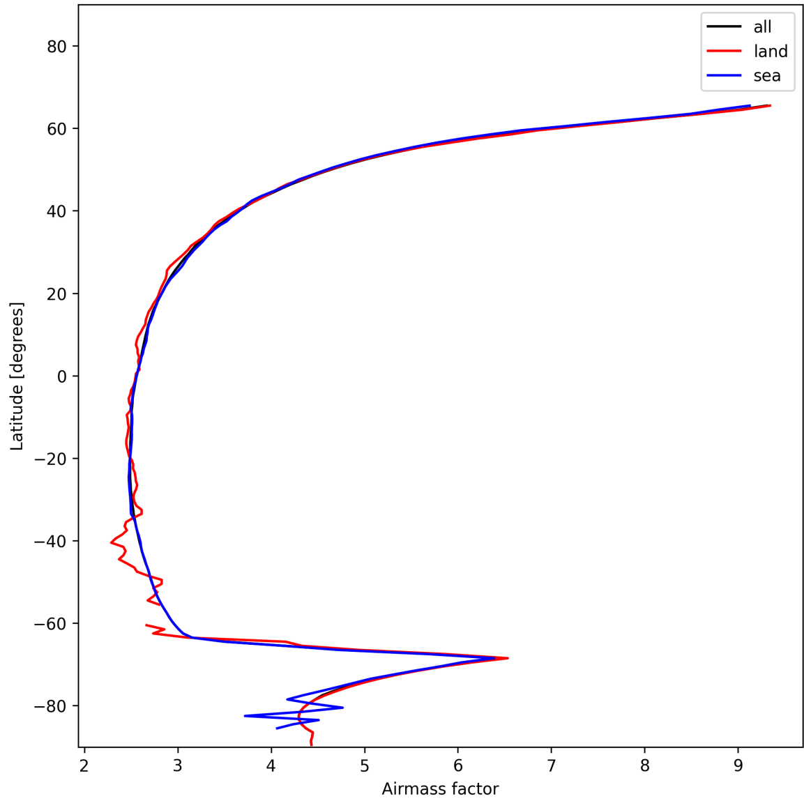
Figure 25: Zonal average of “Airmass factor” for 2025-12-11 to 2025-12-12.
