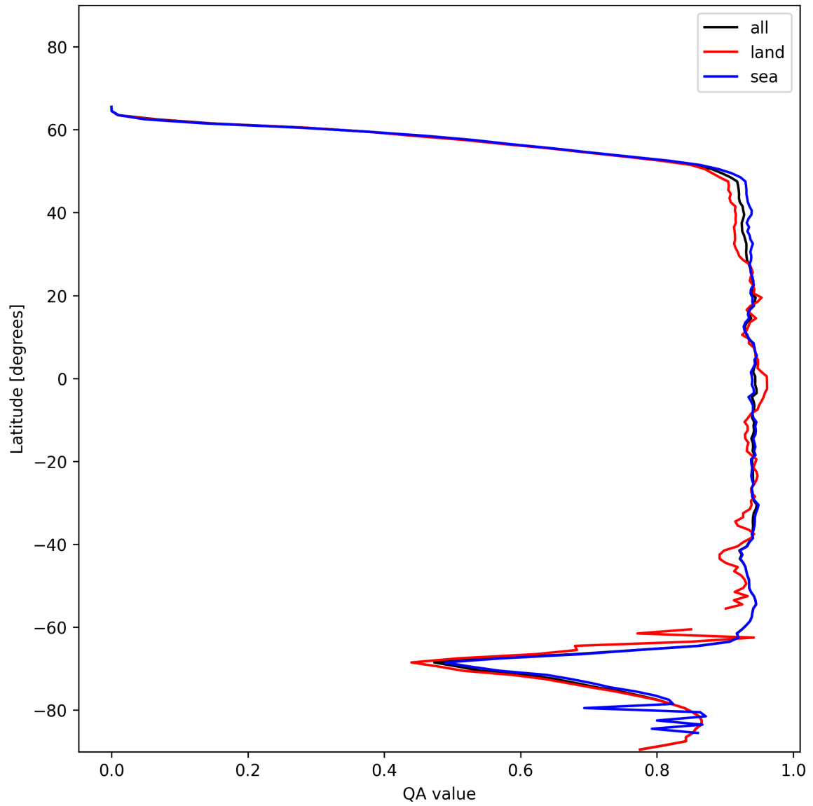
Figure 16: Zonal average of “QA value” for 2025-12-11 to 2025-12-12.
