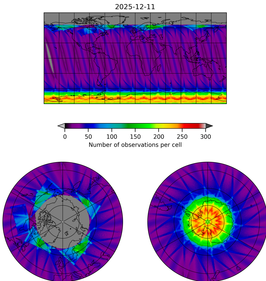
Figure 15: Map of the number of observations for 2025-12-11 to 2025-12-12
