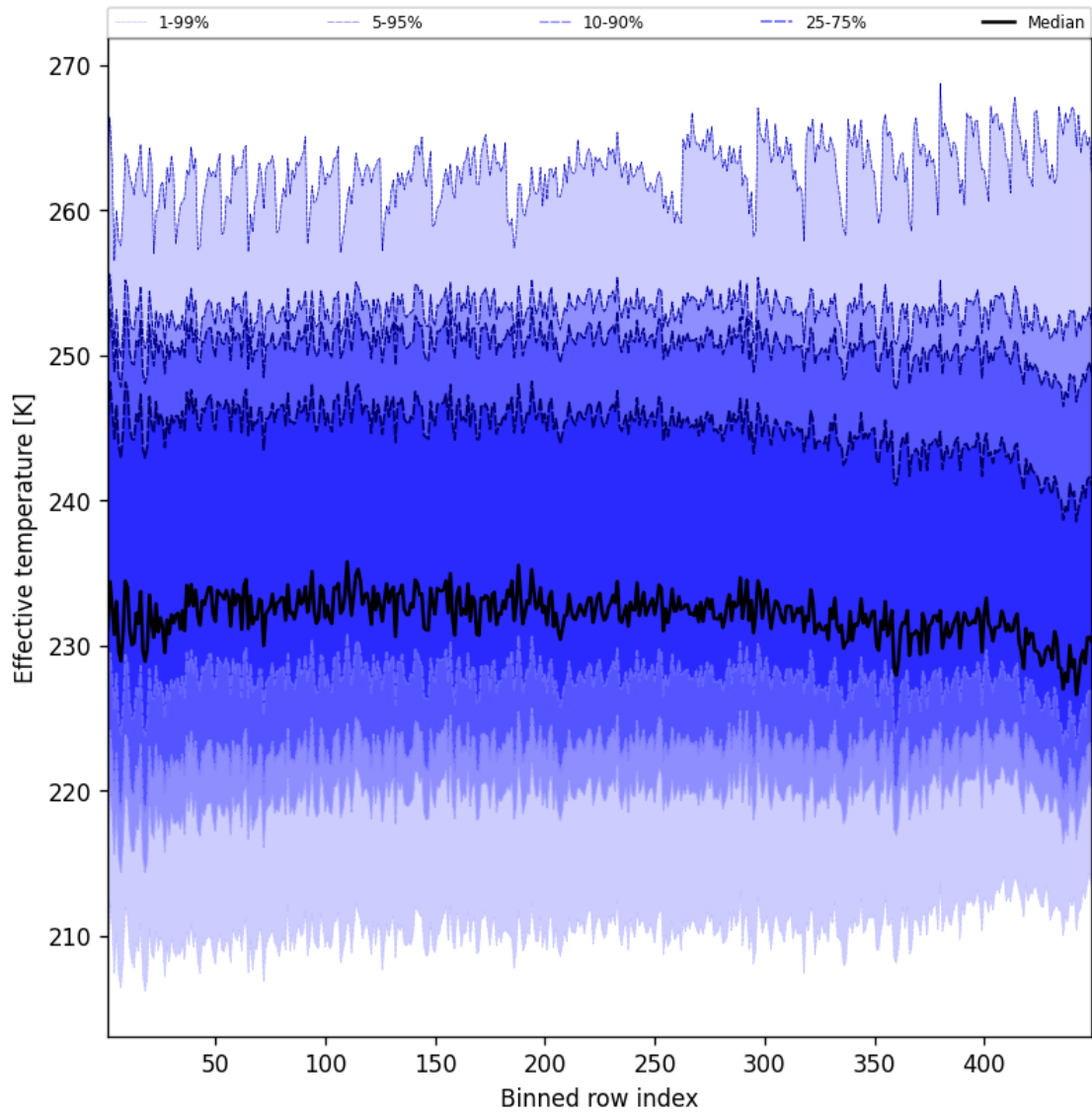
Figure 50: Along track statistics of “Effective temperature” for 2025-12-11 to 2025-12-12
