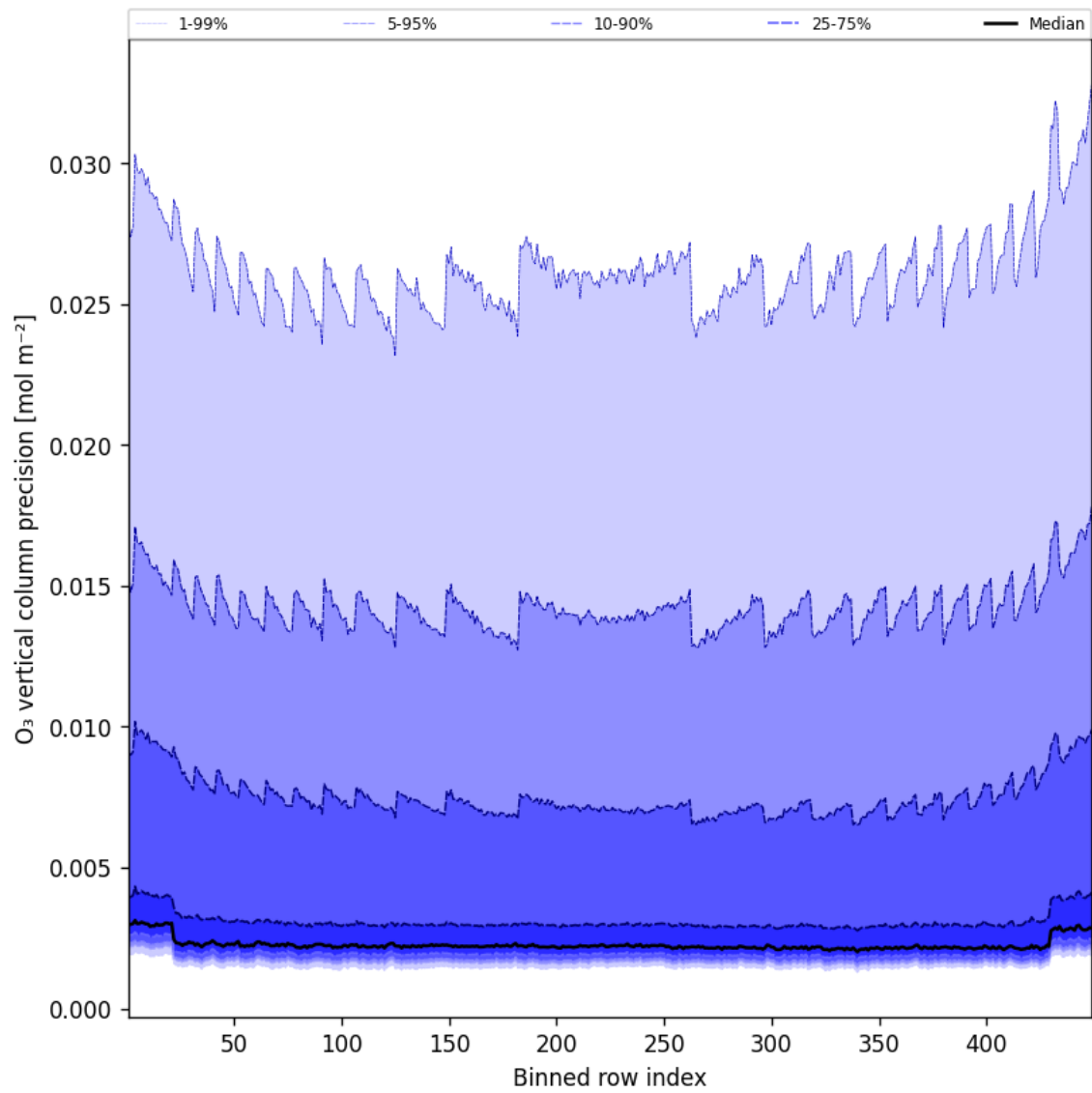
Figure 42: Along track statistics of “O 3 vertical column precision” for 2025-12-11 to 2025-12-12
