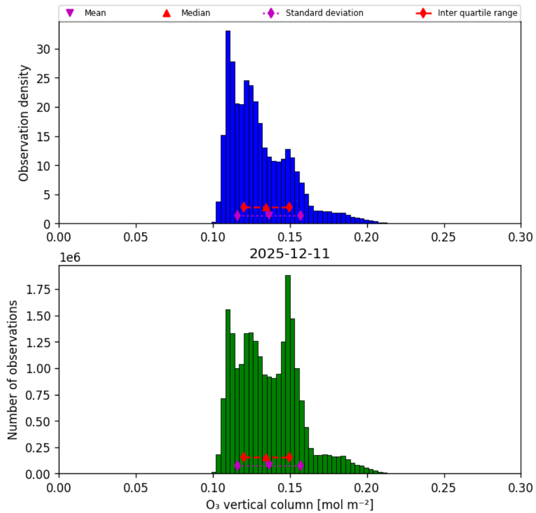
Figure 29: Histogram of “O 3 vertical column” for 2025-12-11 to 2025-12-12
