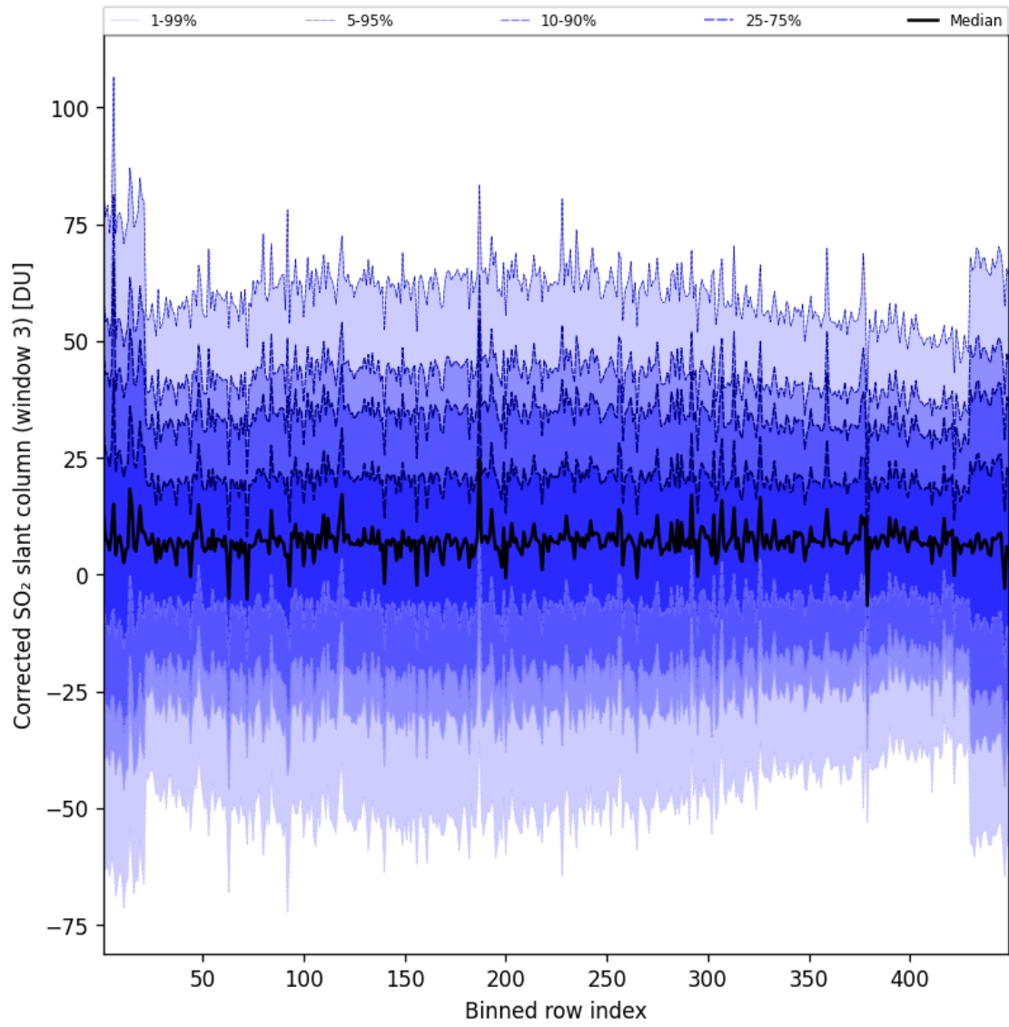
Figure 100: Along track statistics of “Corrected SO 2 slant column (window 3)” for 2024-12-02 to 2024-12-03
