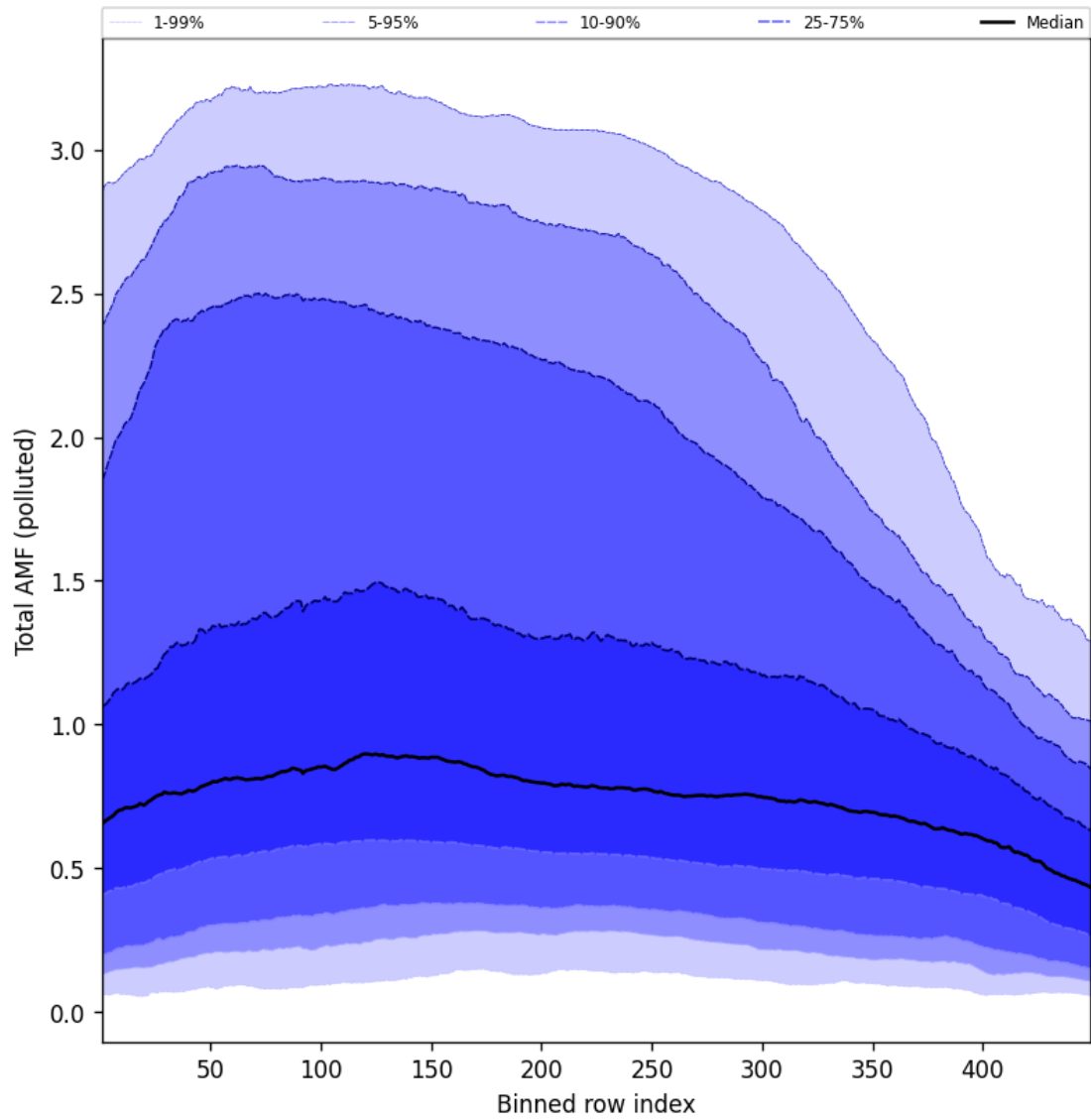
Figure 107: Along track statistics of “Total AMF (polluted)” for 2024-12-02 to 2024-12-03
