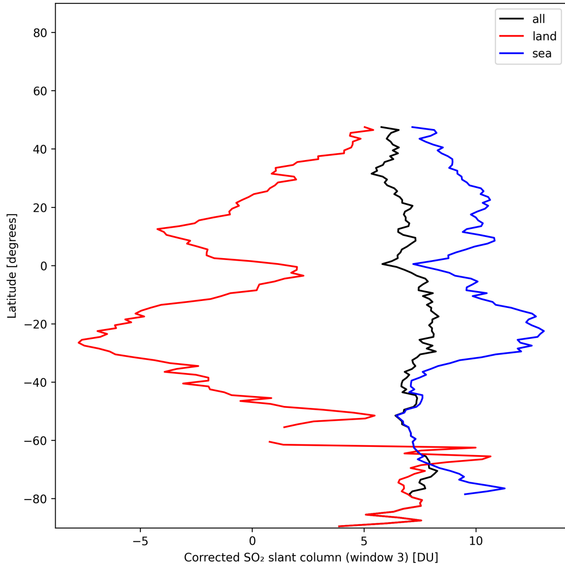
Figure 46: Zonal average of “Corrected SO 2 slant column (window 3)” for 2024-12-02 to 2024-12-03.
