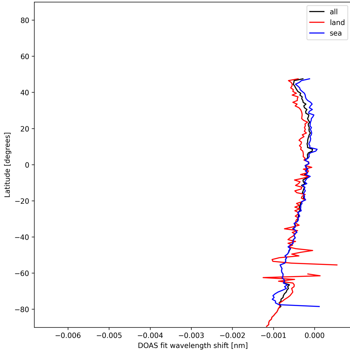
Figure 50: Zonal average of “DOAS fit wavelength shift” for 2024-12-02 to 2024-12-03.
