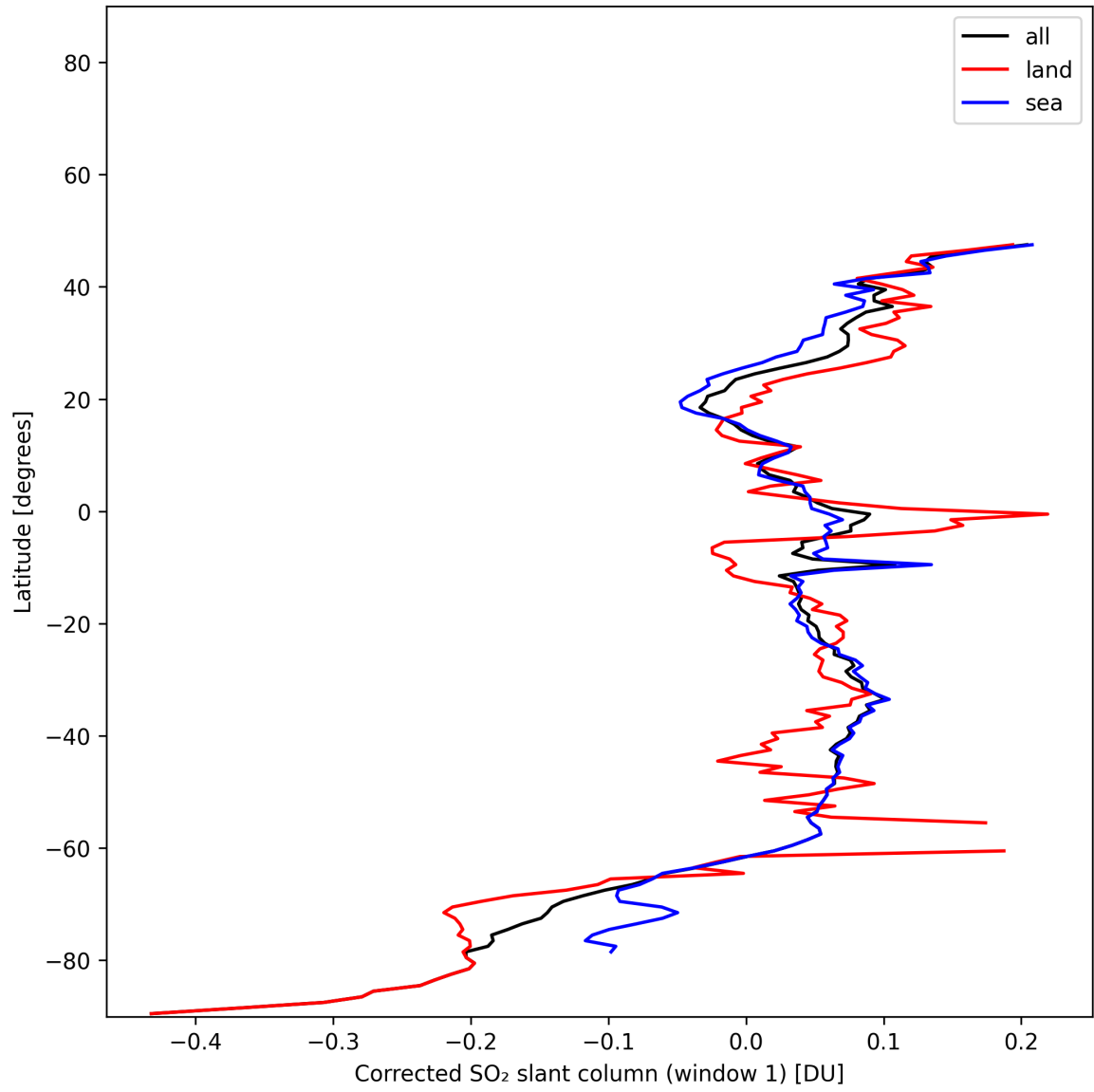
Figure 38: Zonal average of “Corrected SO 2 slant column (window 1)” for 2024-12-02 to 2024-12-03.
