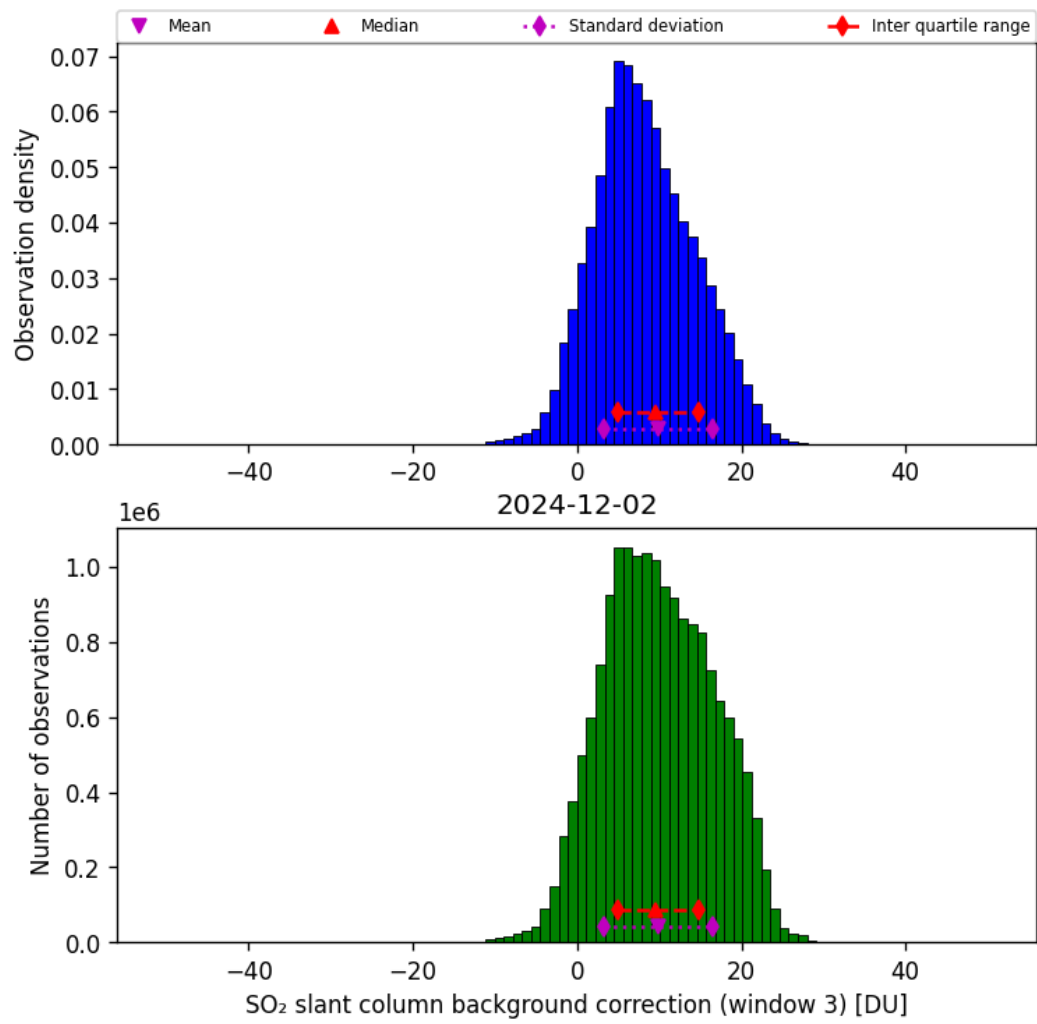
Figure 74: Histogram of “SO 2 slant column background correction (window 3)” for 2024-12-02 to 2024-12-03
