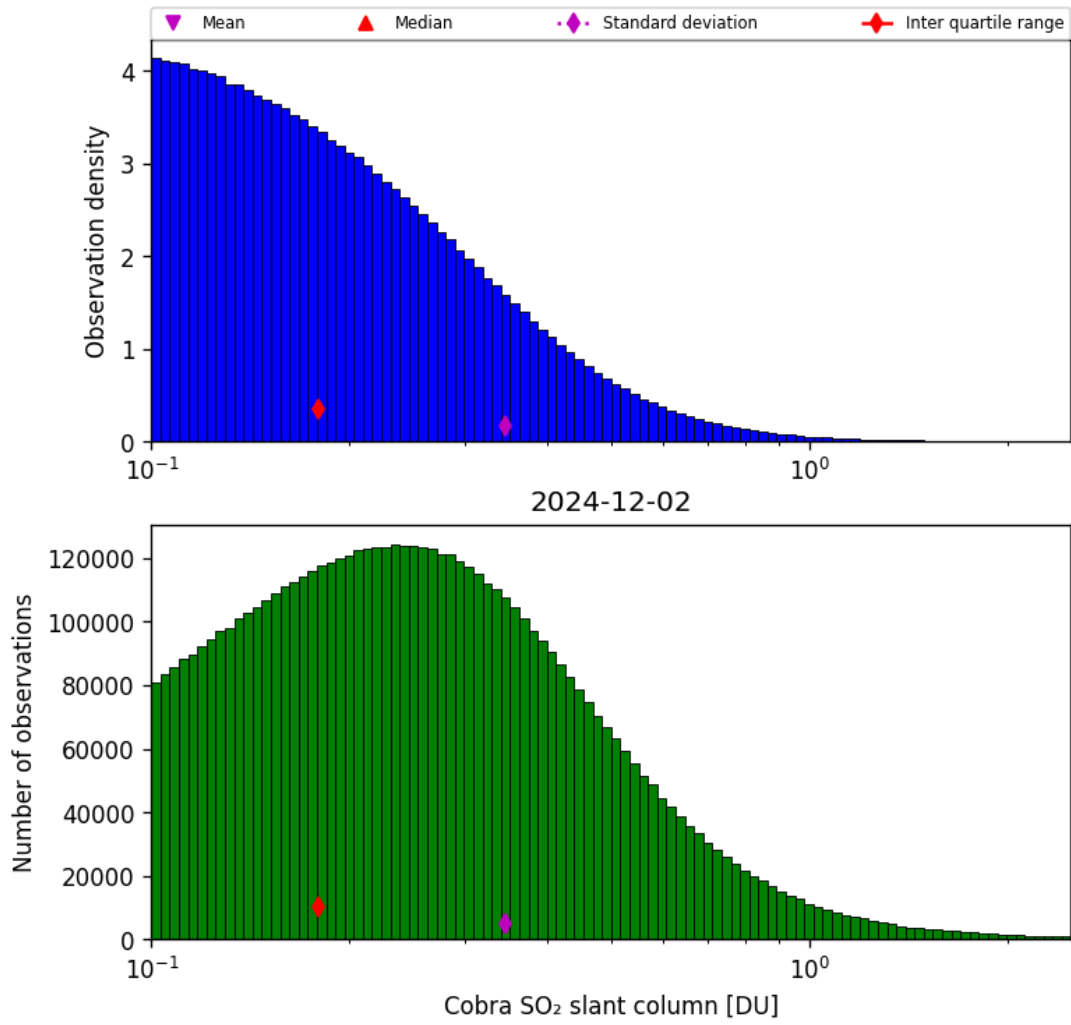
Figure 61: Histogram of “Cobra SO 2 slant column” for 2024-12-02 to 2024-12-03
