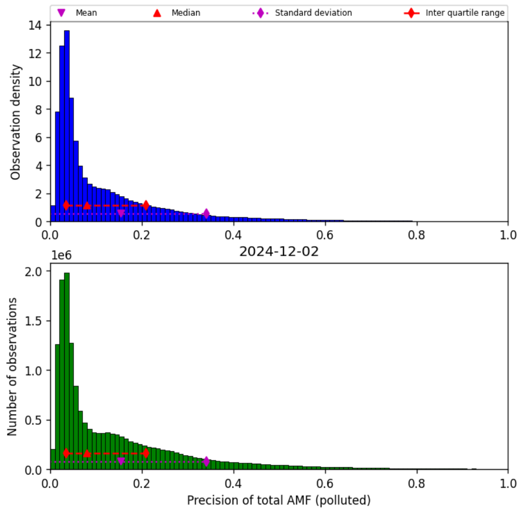
Figure 81: Histogram of “Precision of total AMF (polluted)” for 2024-12-02 to 2024-12-03
