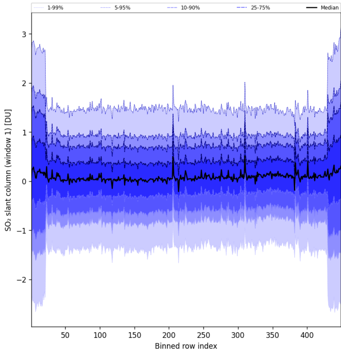
Figure 90: Along track statistics of “SO 2 slant column (window 1)” for 2024-12-02 to 2024-12-03
