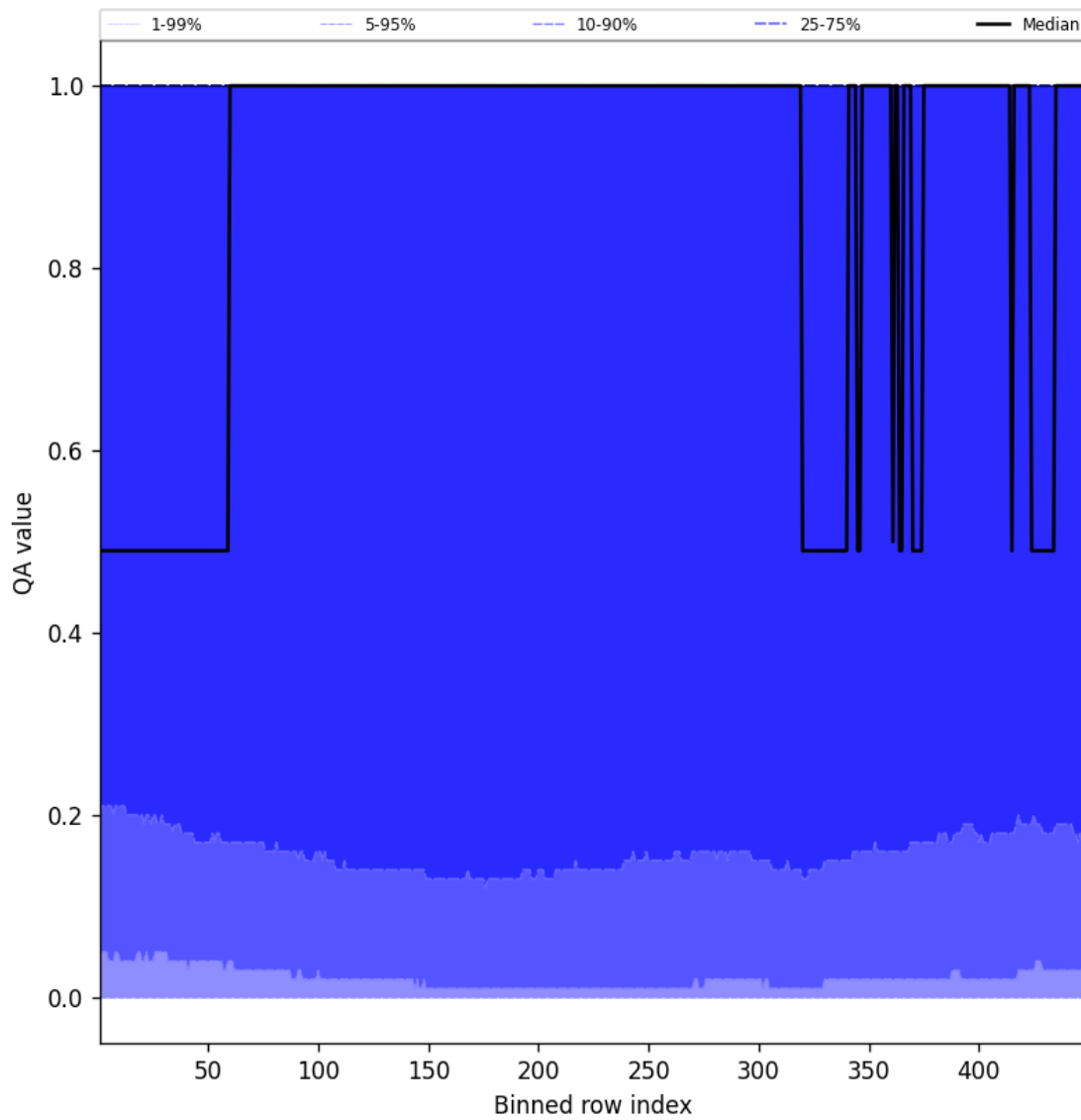
Figure 84: Along track statistics of “QA value” for 2024-12-02 to 2024-12-03
