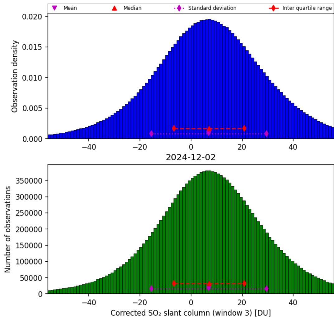
Figure 73: Histogram of “Corrected SO 2 slant column (window 3)” for 2024-12-02 to 2024-12-03
