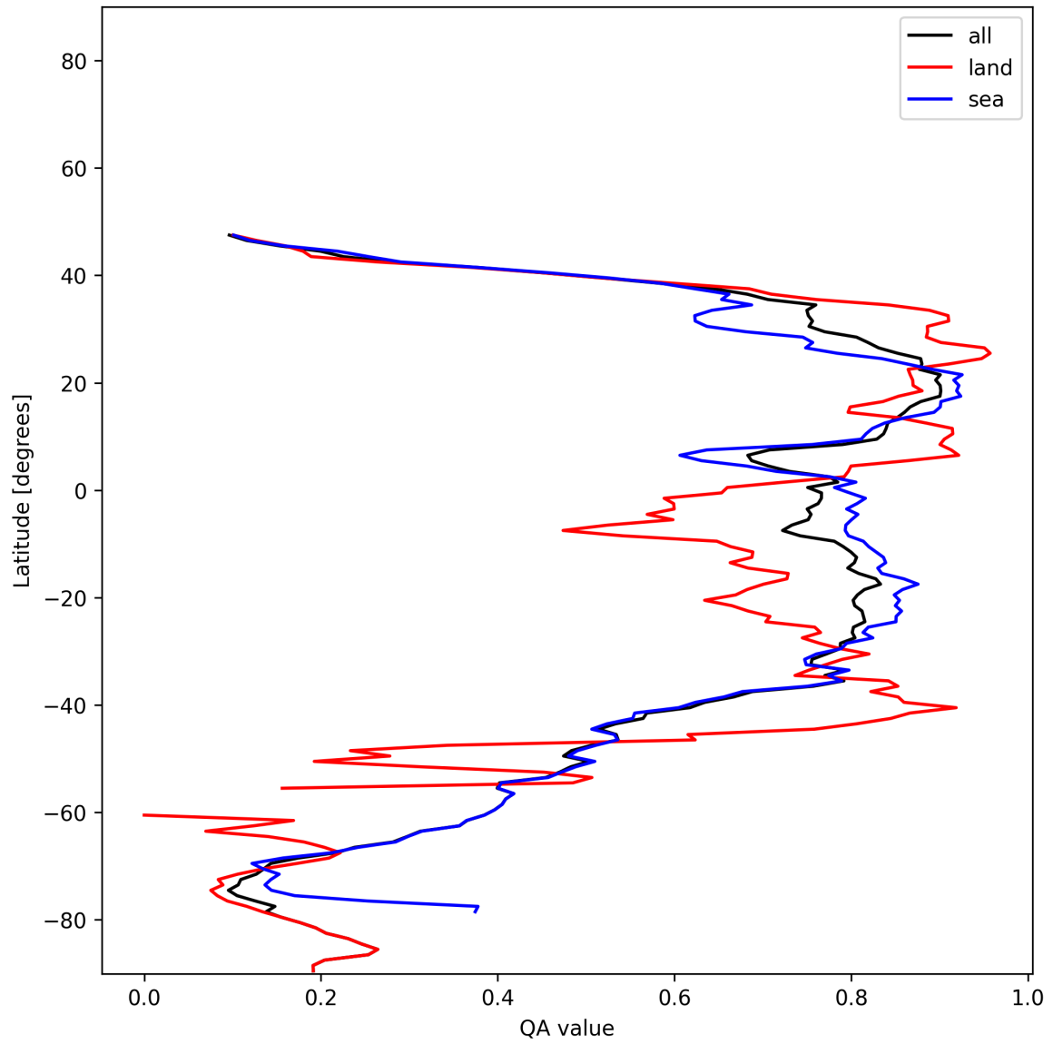
Figure 30: Zonal average of “QA value” for 2024-12-02 to 2024-12-03.
