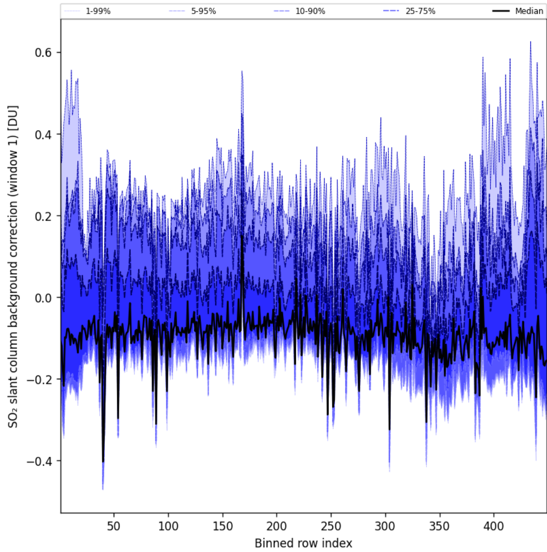
Figure 93: Along track statistics of “SO 2 slant column background correction (window 1)” for 2024-12-02 to 2024-12-03
