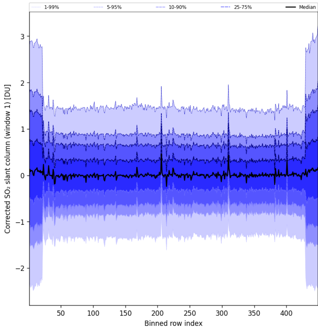
Figure 92: Along track statistics of “Corrected SO 2 slant column (window 1)” for 2024-12-02 to 2024-12-03
