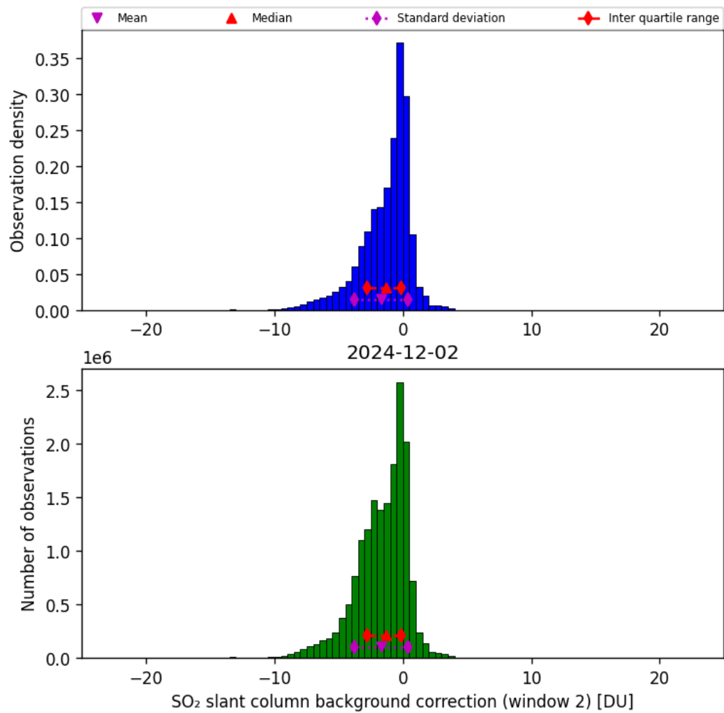
Figure 70: Histogram of “SO 2 slant column background correction (window 2)” for 2024-12-02 to 2024-12-03
