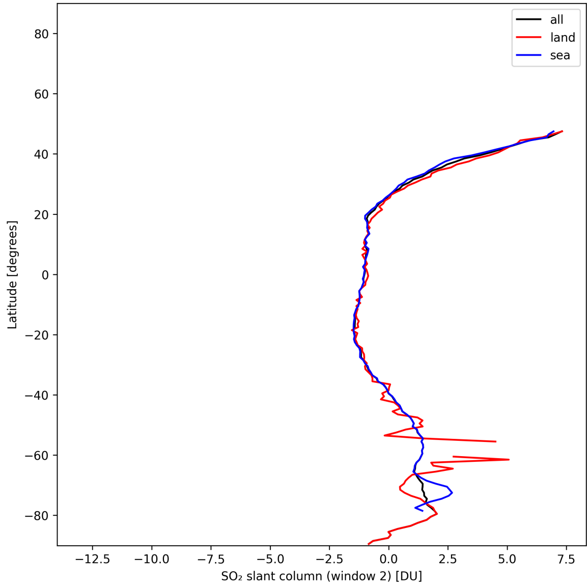
Figure 40: Zonal average of “SO 2 slant column (window 2)” for 2024-12-02 to 2024-12-03.
