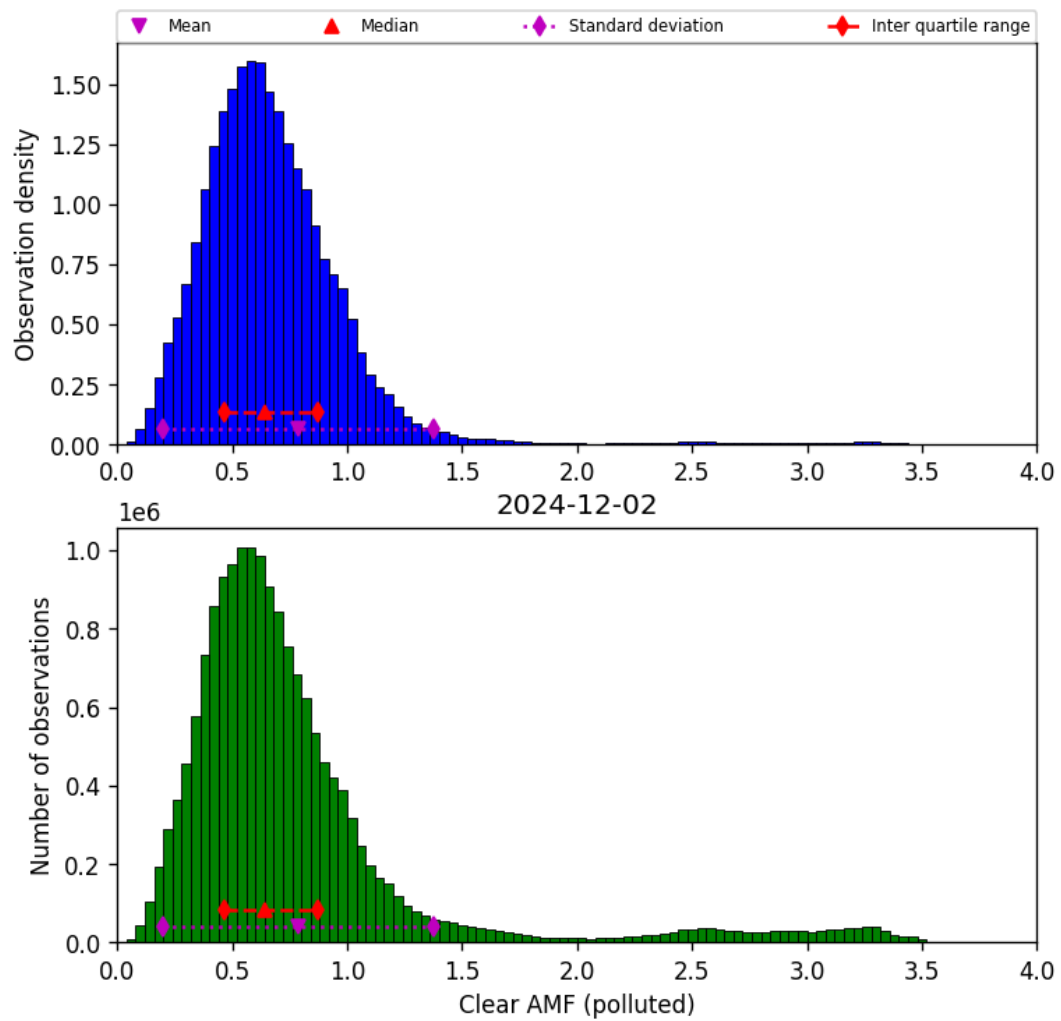
Figure 82: Histogram of “Clear AMF (polluted)” for 2024-12-02 to 2024-12-03
