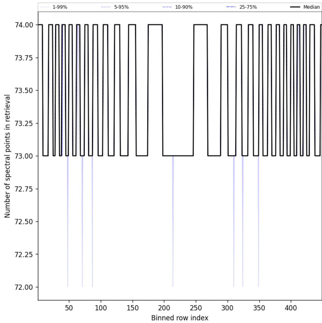
Figure 110: Along track statistics of “Number of spectral points in retrieval” for 2024-12-02 to 2024-12-03
