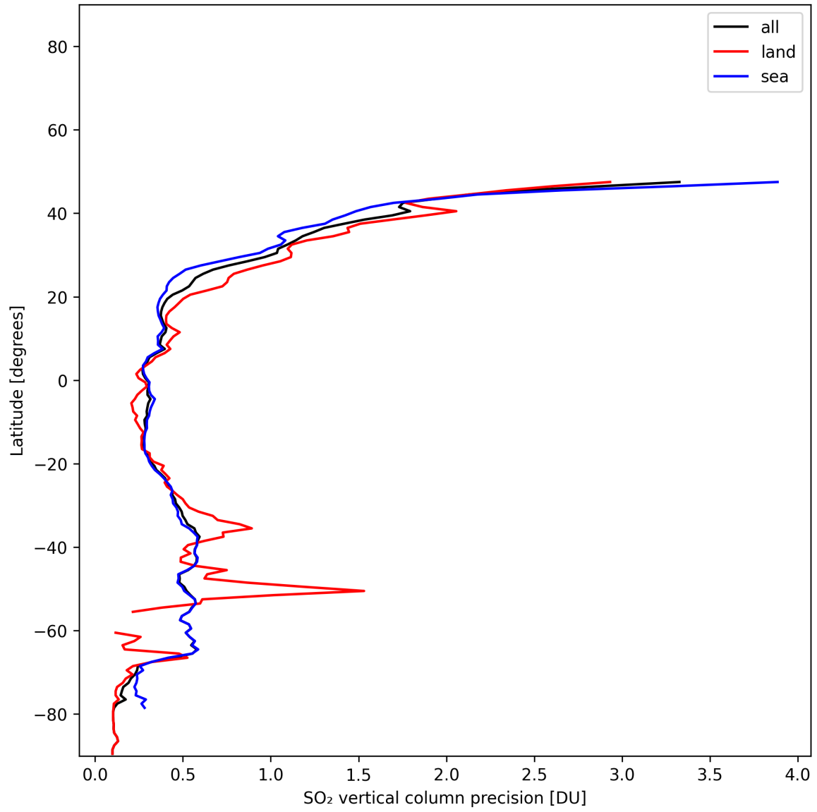
Figure 32: Zonal average of “SO 2 vertical column precision” for 2024-12-02 to 2024-12-03.
