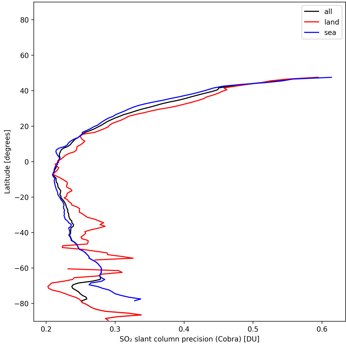
Figure 35: Zonal average of “SO 2 slant column precision (Cobra)” for 2024-12-02 to 2024-12-03.
