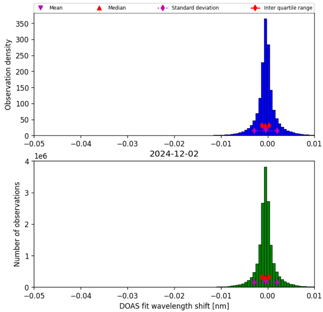
Figure 77: Histogram of “DOAS fit wavelength shift” for 2024-12-02 to 2024-12-03
