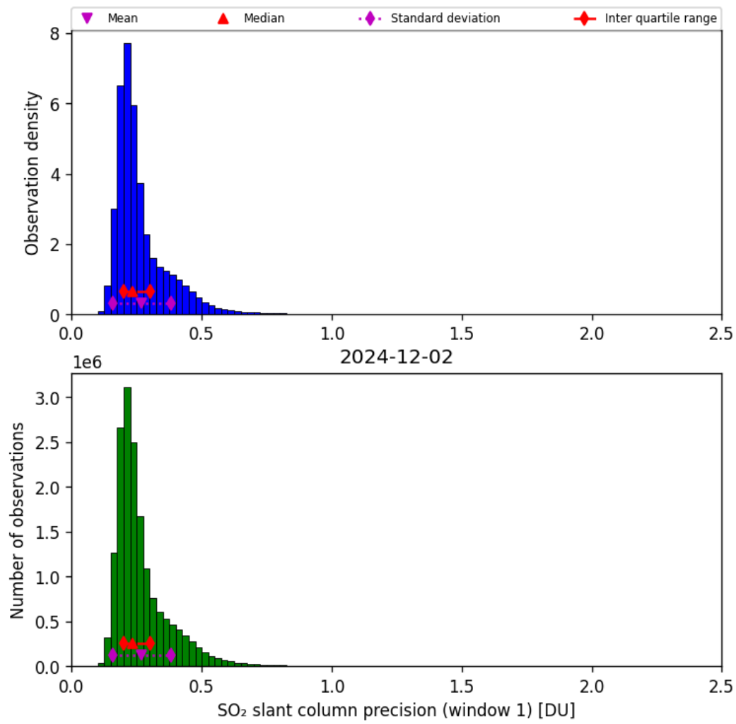
Figure 64: Histogram of “SO 2 slant column precision (window 1)” for 2024-12-02 to 2024-12-03
