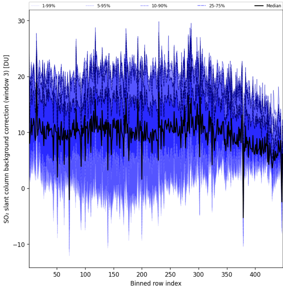
Figure 101: Along track statistics of “SO 2 slant column background correction (window 3)” for 2024-12-02 to 2024-12-03
