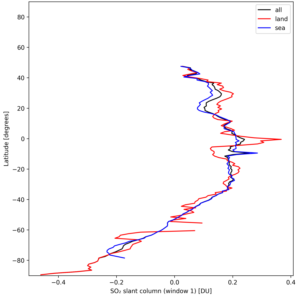
Figure 36: Zonal average of “SO 2 slant column (window 1)” for 2024-12-02 to 2024-12-03.
