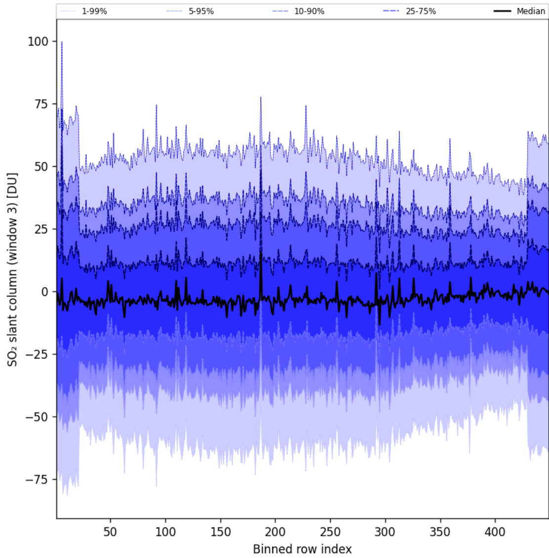
Figure 98: Along track statistics of “SO 2 slant column (window 3)” for 2024-12-02 to 2024-12-03
