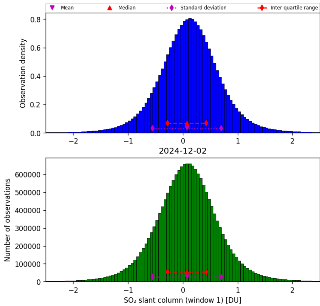
Figure 63: Histogram of “SO 2 slant column (window 1)” for 2024-12-02 to 2024-12-03
