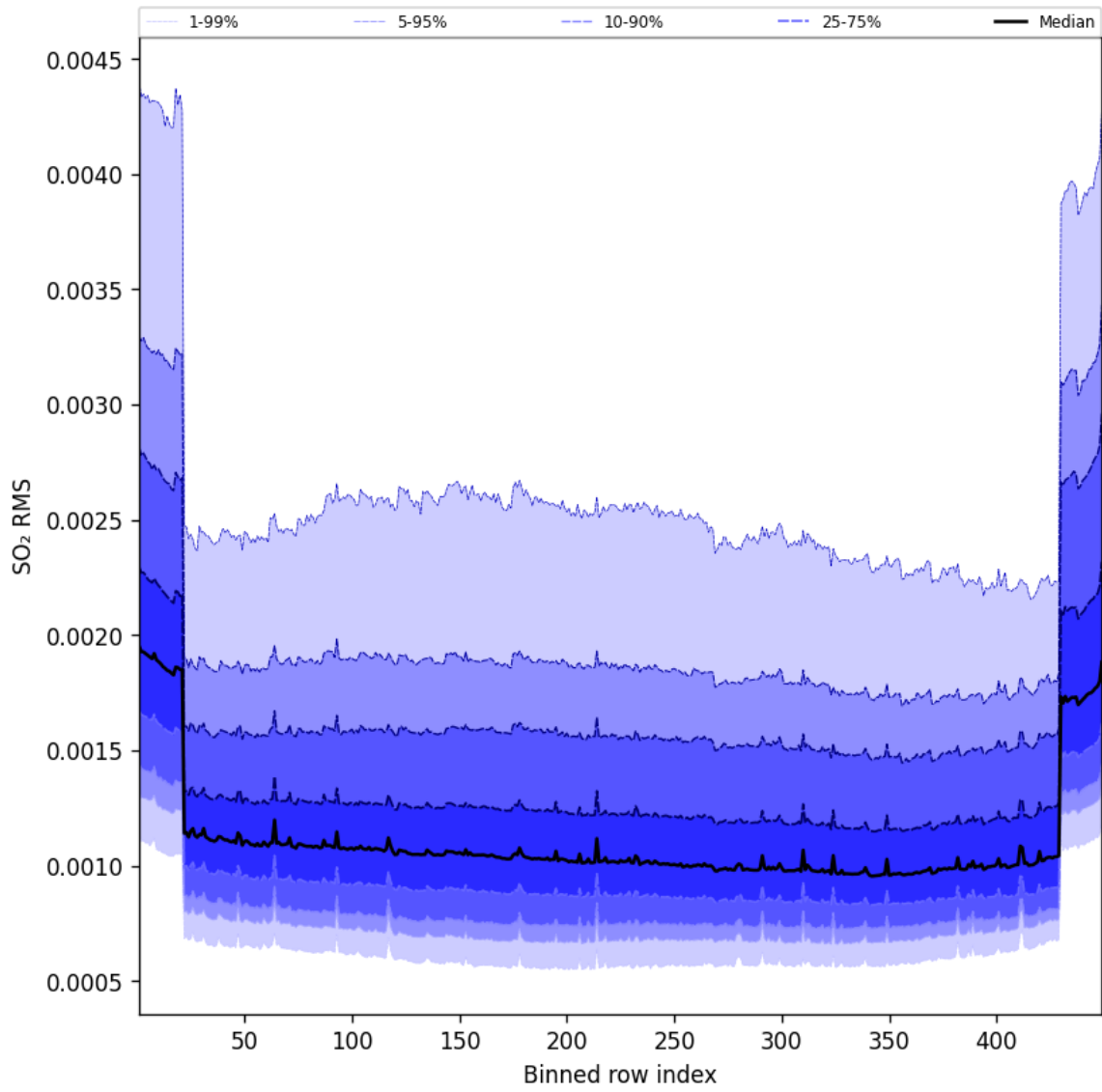
Figure 106: Along track statistics of “SO 2 RMS” for 2024-12-02 to 2024-12-03
