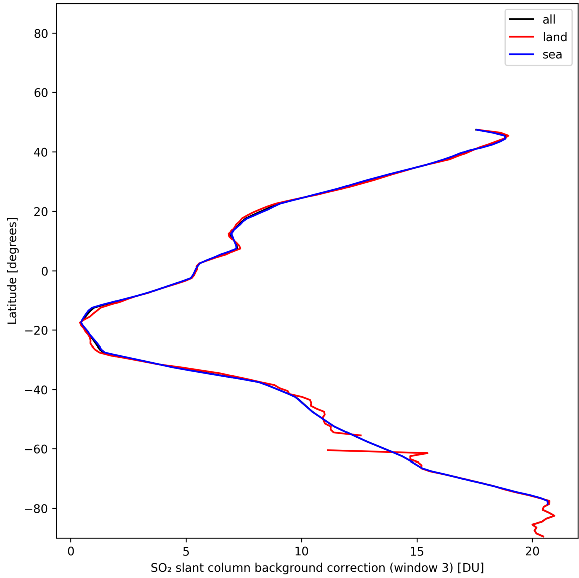
Figure 47: Zonal average of “SO 2 slant column background correction (window 3)” for 2024-12-02 to 2024-12-03.
