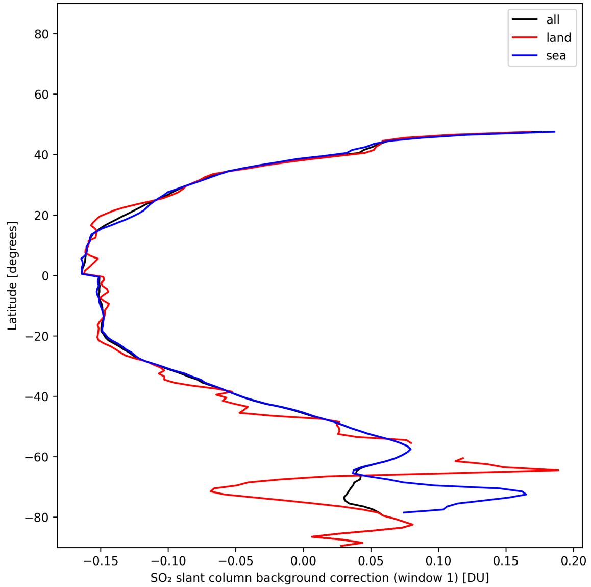
Figure 39: Zonal average of “SO 2 slant column background correction (window 1)” for 2024-12-02 to 2024-12-03.
