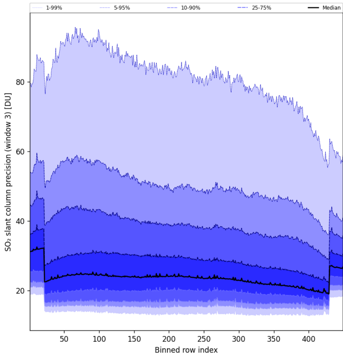
Figure 99: Along track statistics of “SO 2 slant column precision (window 3)” for 2024-12-02 to 2024-12-03
