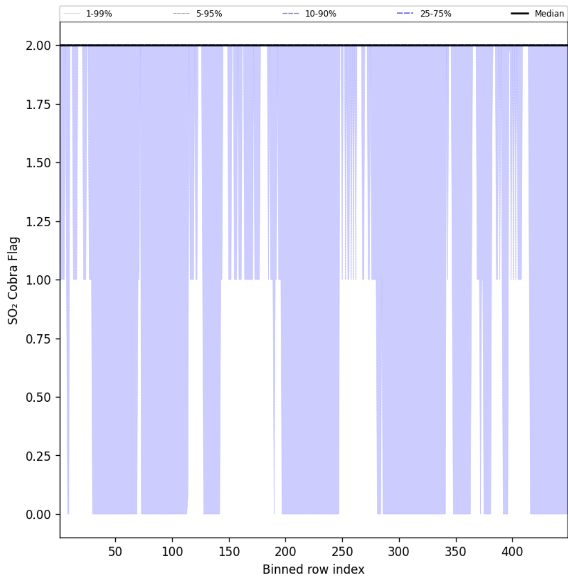
Figure 102: Along track statistics of "SO 2 Cobra Flag" for 2024-12-02 to 2024-12-03
