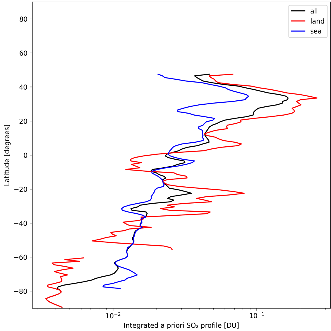
Figure 49: Zonal average of “Integrated a priori SO 2 profile” for 2024-12-02 to 2024-12-03.
