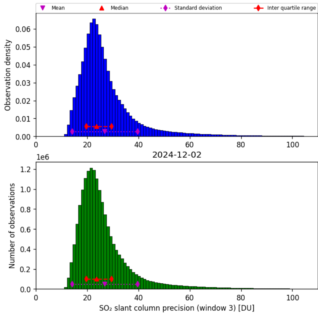
Figure 72: Histogram of “SO 2 slant column precision (window 3)” for 2024-12-02 to 2024-12-03
