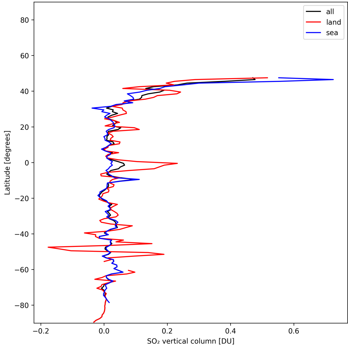
Figure 31: Zonal average of “SO 2 vertical column” for 2024-12-02 to 2024-12-03.
