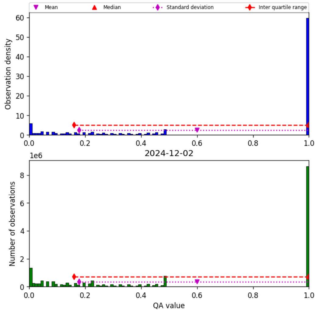
Figure 57: Histogram of “QA value” for 2024-12-02 to 2024-12-03
