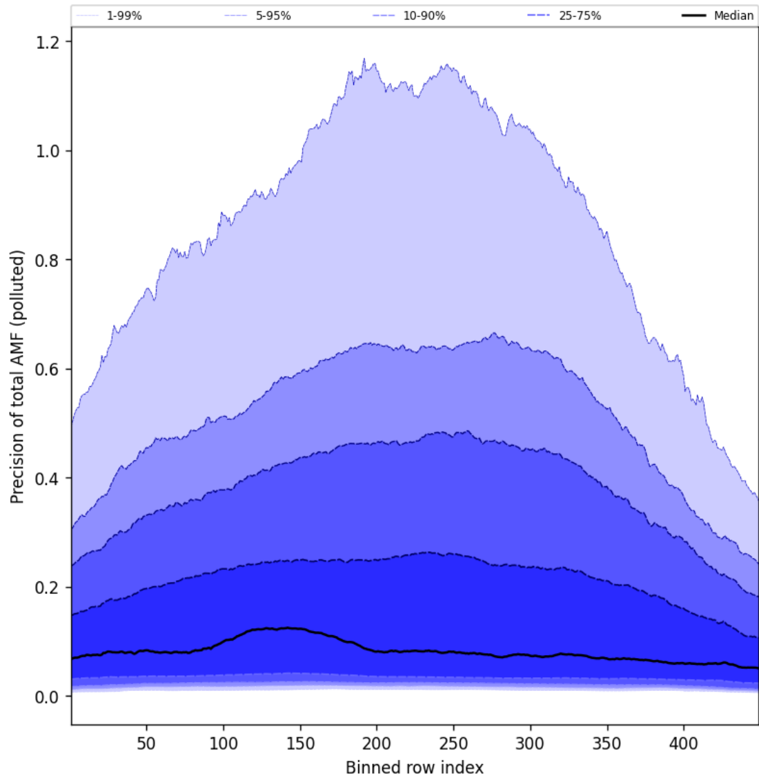
Figure 108: Along track statistics of “Precision of total AMF (polluted)” for 2024-12-02 to 2024-12-03
