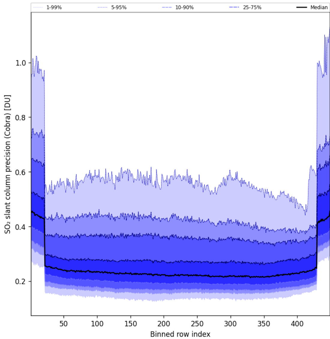
Figure 89: Along track statistics of “SO 2 slant column precision (Cobra)” for 2024-12-02 to 2024-12-03
