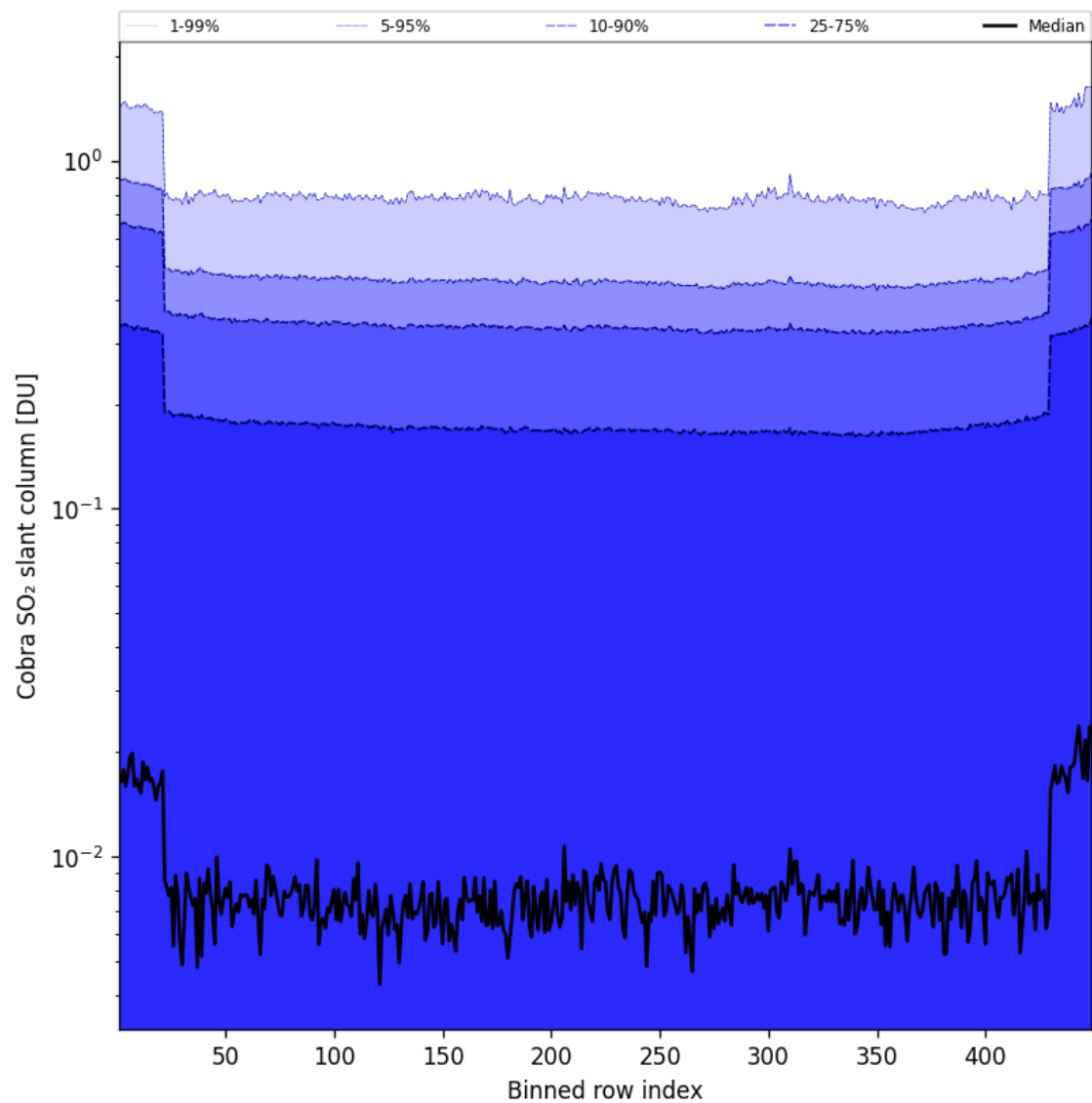
Figure 88: Along track statistics of “Cobra SO 2 slant column” for 2024-12-02 to 2024-12-03
