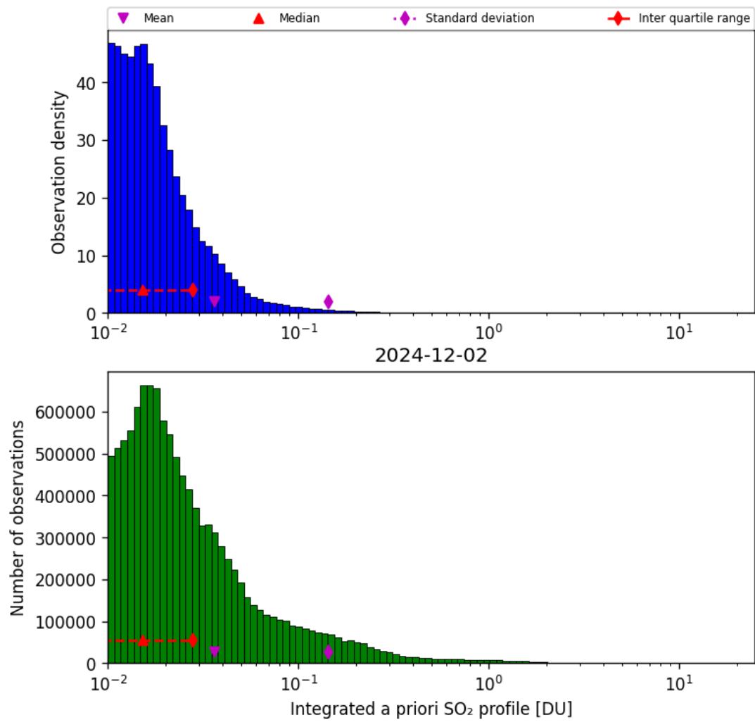
Figure 76: Histogram of “Integrated a priori SO 2 profile” for 2024-12-02 to 2024-12-03
