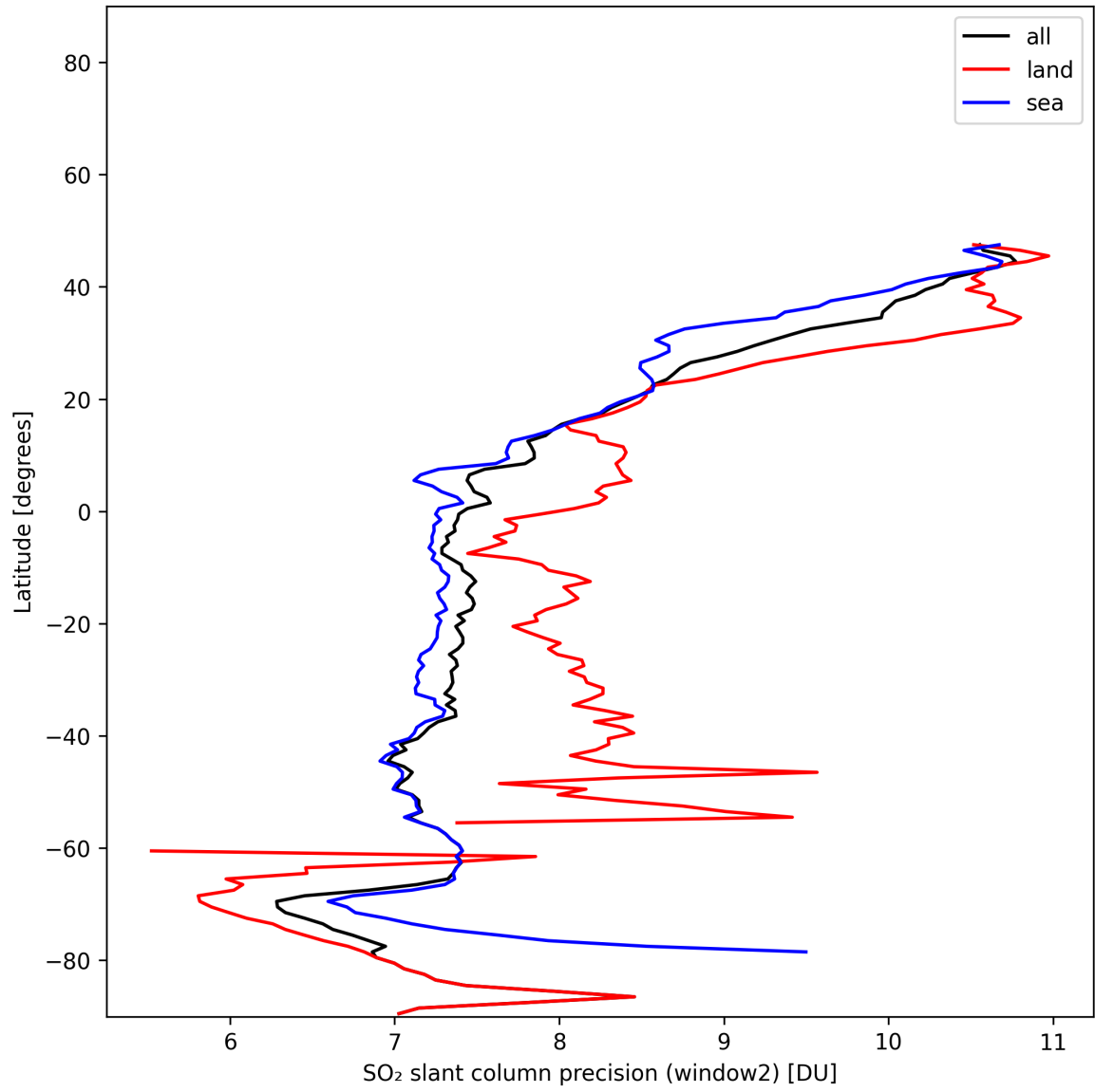
Figure 41: Zonal average of “SO 2 slant column precision (window2)” for 2024-12-02 to 2024-12-03.
