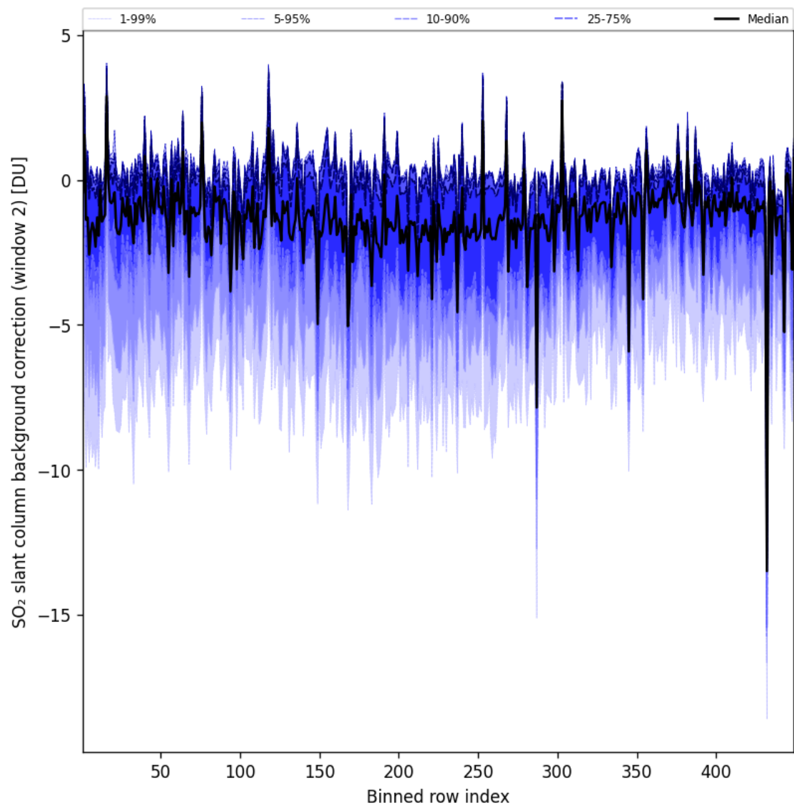
Figure 97: Along track statistics of “SO 2 slant column background correction (window 2)” for 2024-12-02 to 2024-12-03
