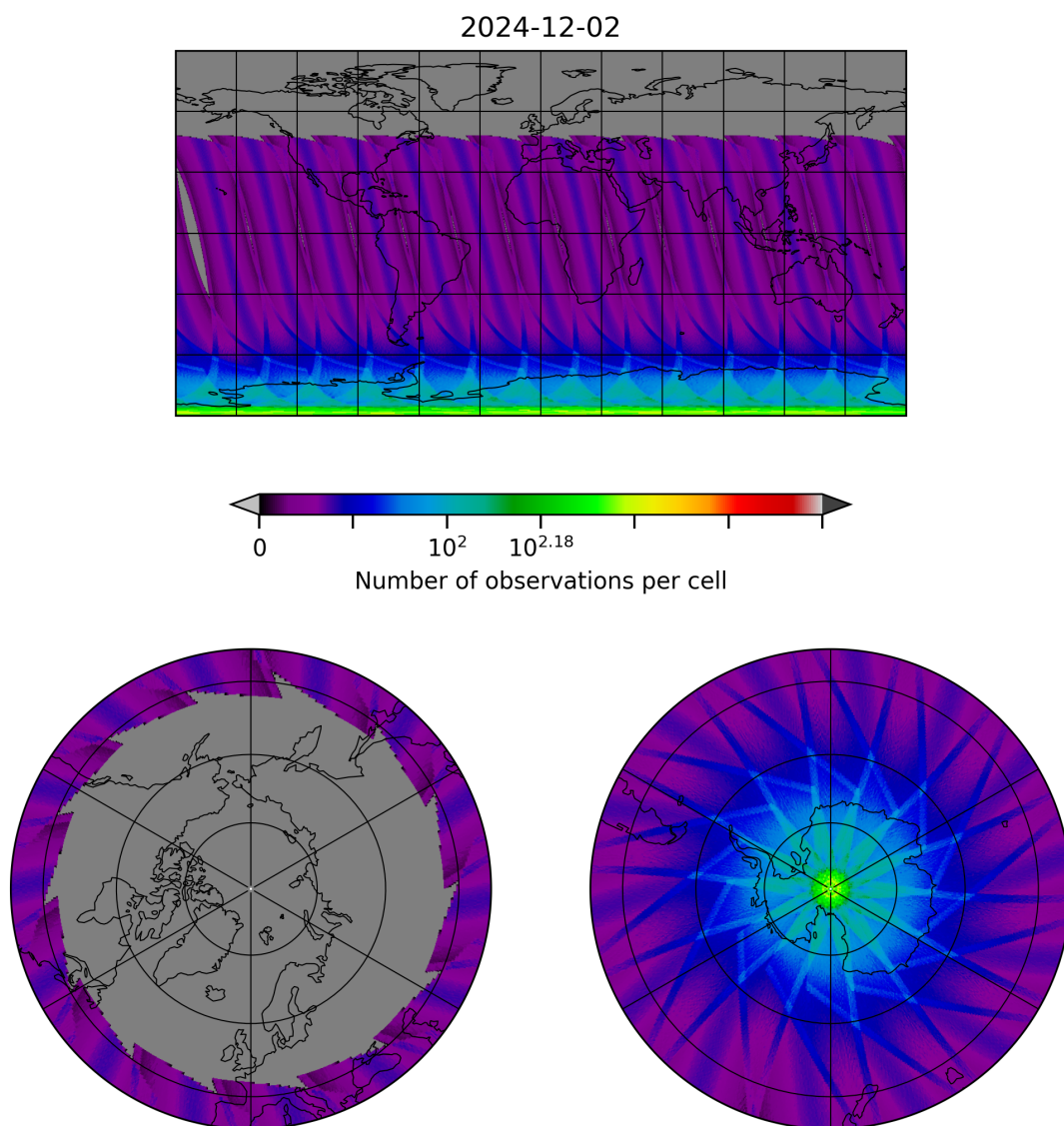
Figure 29: Map of the number of observations for 2024-12-02 to 2024-12-03
