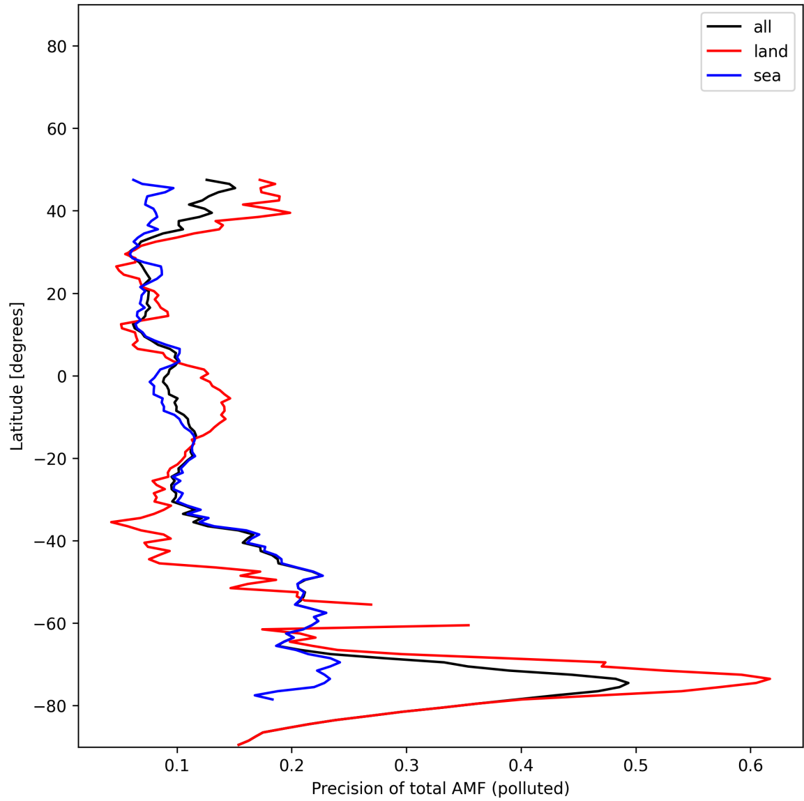
Figure 54: Zonal average of “Precision of total AMF (polluted)” for 2024-12-02 to 2024-12-03.
