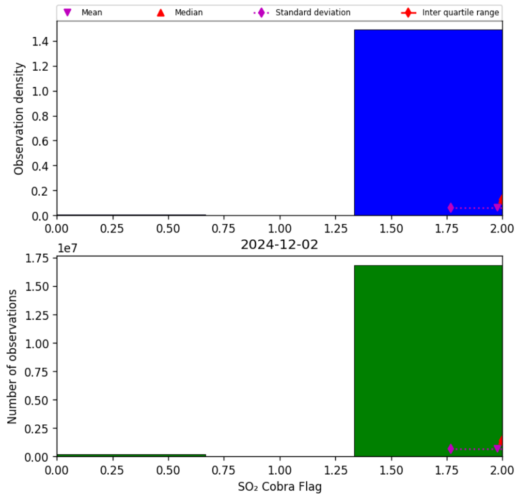
Figure 75: Histogram of "SO 2 Cobra Flag" for 2024-12-02 to 2024-12-03
