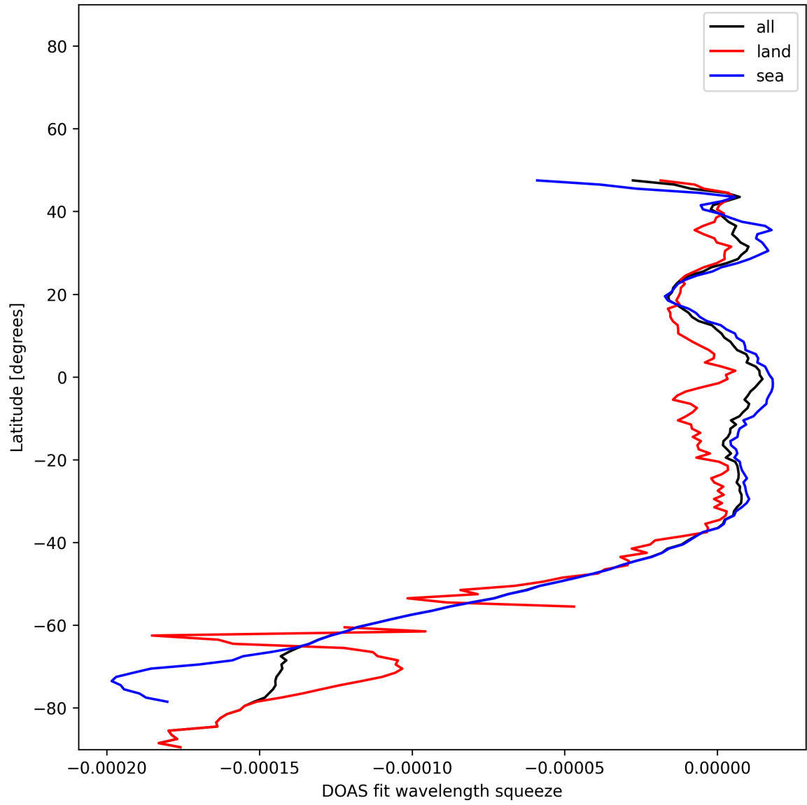
Figure 51: Zonal average of “DOAS fit wavelength squeeze” for 2024-12-02 to 2024-12-03.
