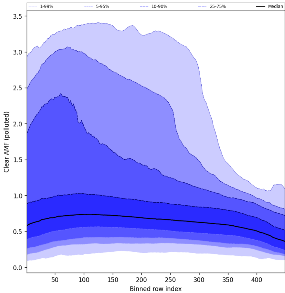
Figure 109: Along track statistics of “Clear AMF (polluted)” for 2024-12-02 to 2024-12-03
