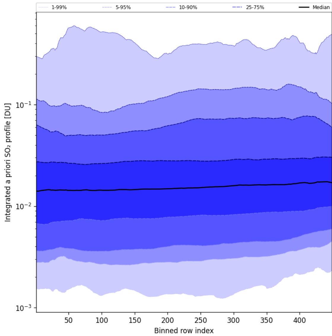
Figure 103: Along track statistics of “Integrated a priori SO 2 profile” for 2024-12-02 to 2024-12-03
