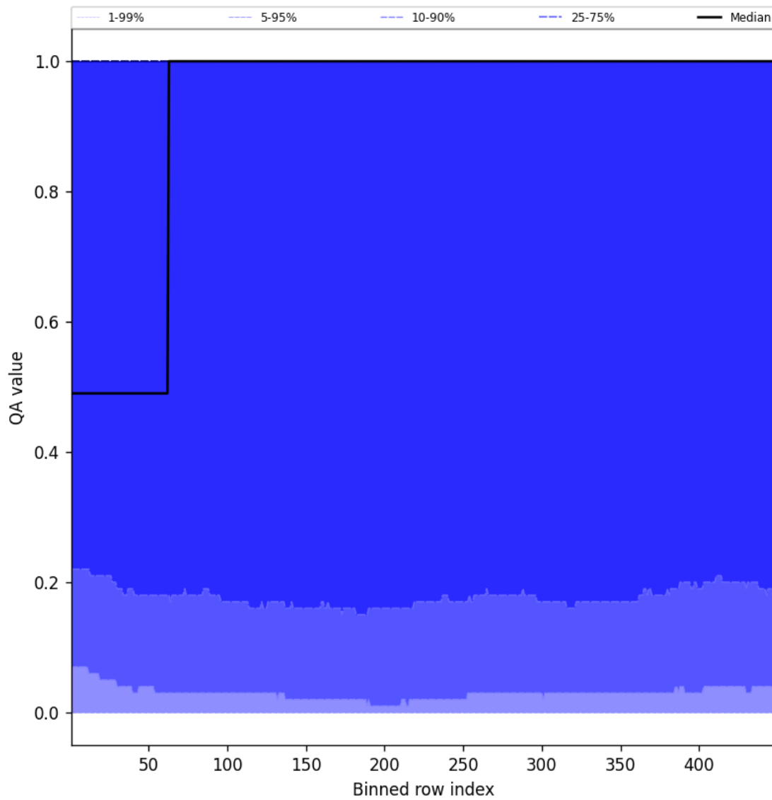
Figure 84: Along track statistics of “QA value” for 2024-12-28 to 2024-12-29
