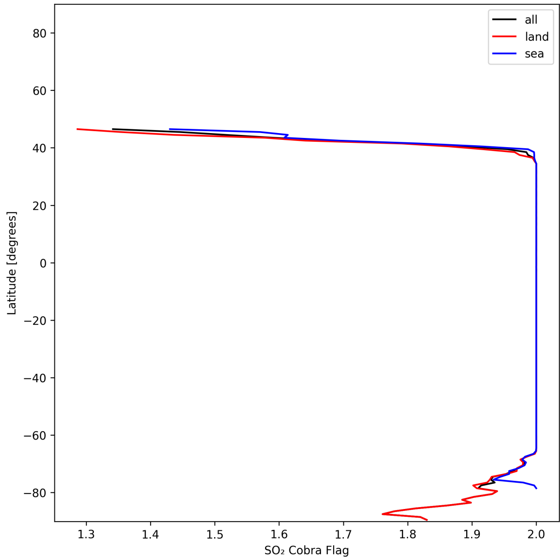
Figure 48: Zonal average of "SO 2 Cobra Flag" for 2024-12-28 to 2024-12-29.
