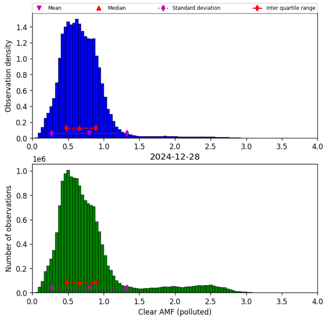
Figure 82: Histogram of "Clear AMF (polluted)" for 2024-12-28 to 2024-12-29
