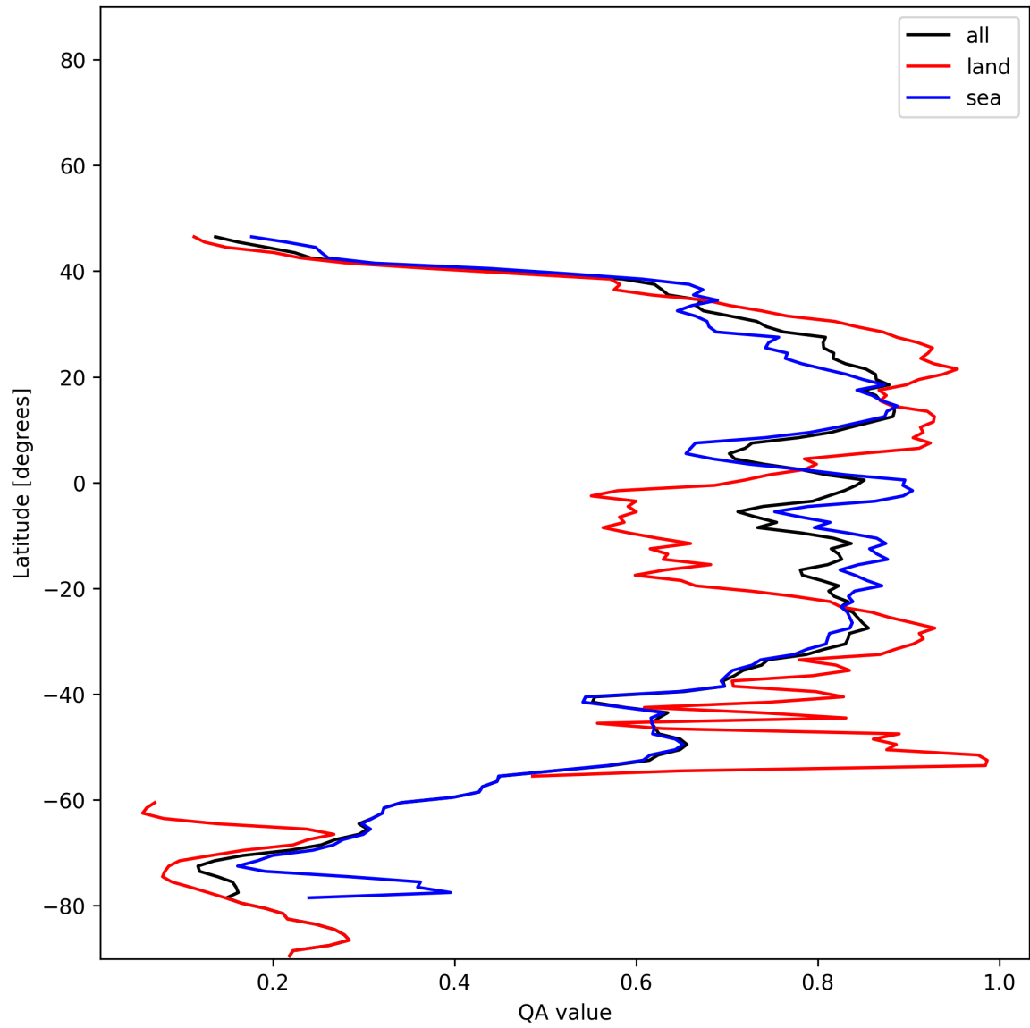
Figure 30: Zonal average of “QA value” for 2024-12-28 to 2024-12-29.
