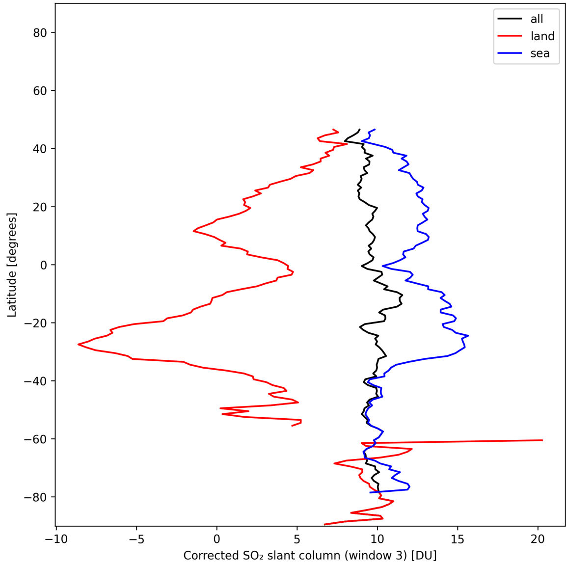
Figure 46: Zonal average of “Corrected SO 2 slant column (window 3)” for 2024-12-28 to 2024-12-29.
