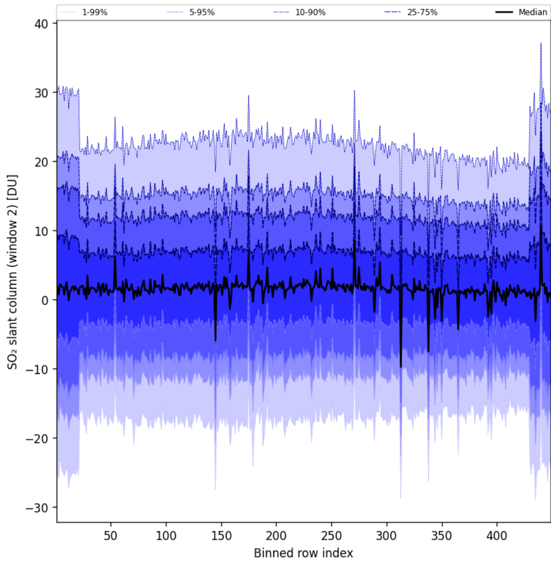
Figure 94: Along track statistics of “SO 2 slant column (window 2)” for 2024-12-28 to 2024-12-29
