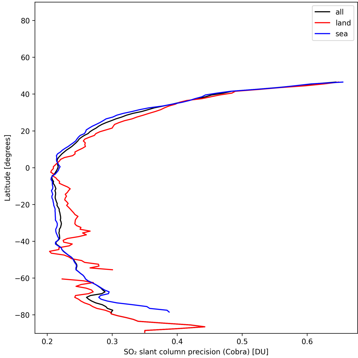
Figure 35: Zonal average of “SO 2 slant column precision (Cobra)” for 2024-12-28 to 2024-12-29.
