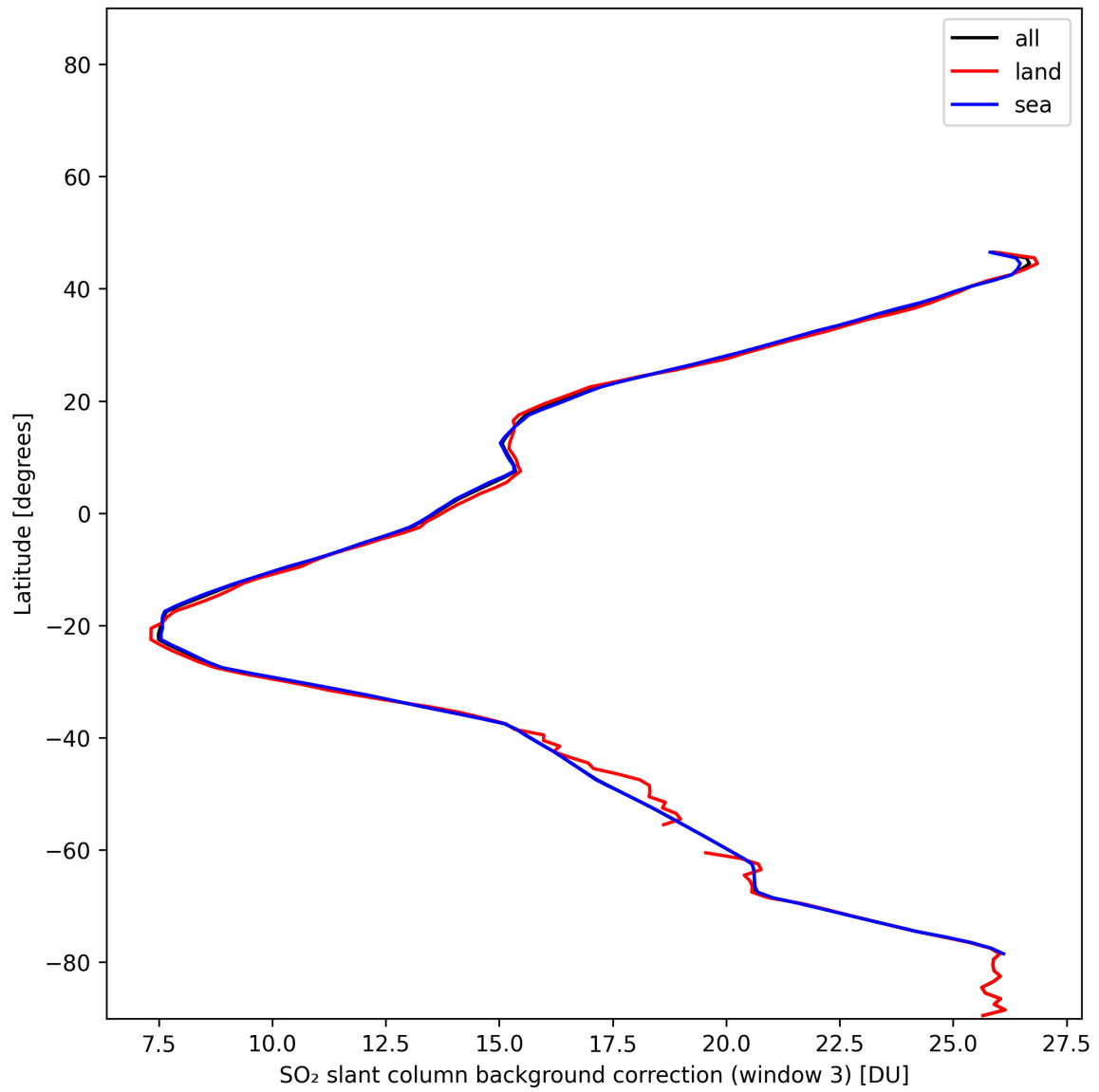
Figure 47: Zonal average of “SO 2 slant column background correction (window 3)” for 2024-12-28 to 2024-12-29.
