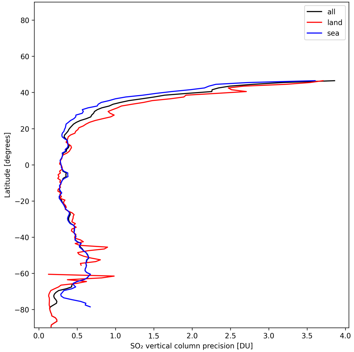
Figure 32: Zonal average of “SO 2 vertical column precision” for 2024-12-28 to 2024-12-29.
