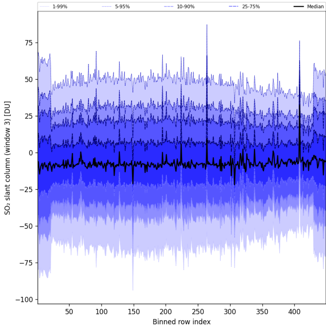
Figure 98: Along track statistics of “SO 2 slant column (window 3)” for 2024-12-28 to 2024-12-29
