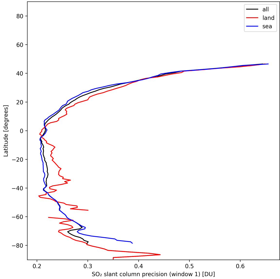
Figure 37: Zonal average of “SO 2 slant column precision (window 1)” for 2024-12-28 to 2024-12-29.
