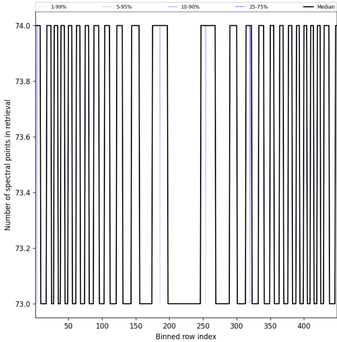
Figure 110: Along track statistics of “Number of spectral points in retrieval” for 2024-12-28 to 2024-12-29
