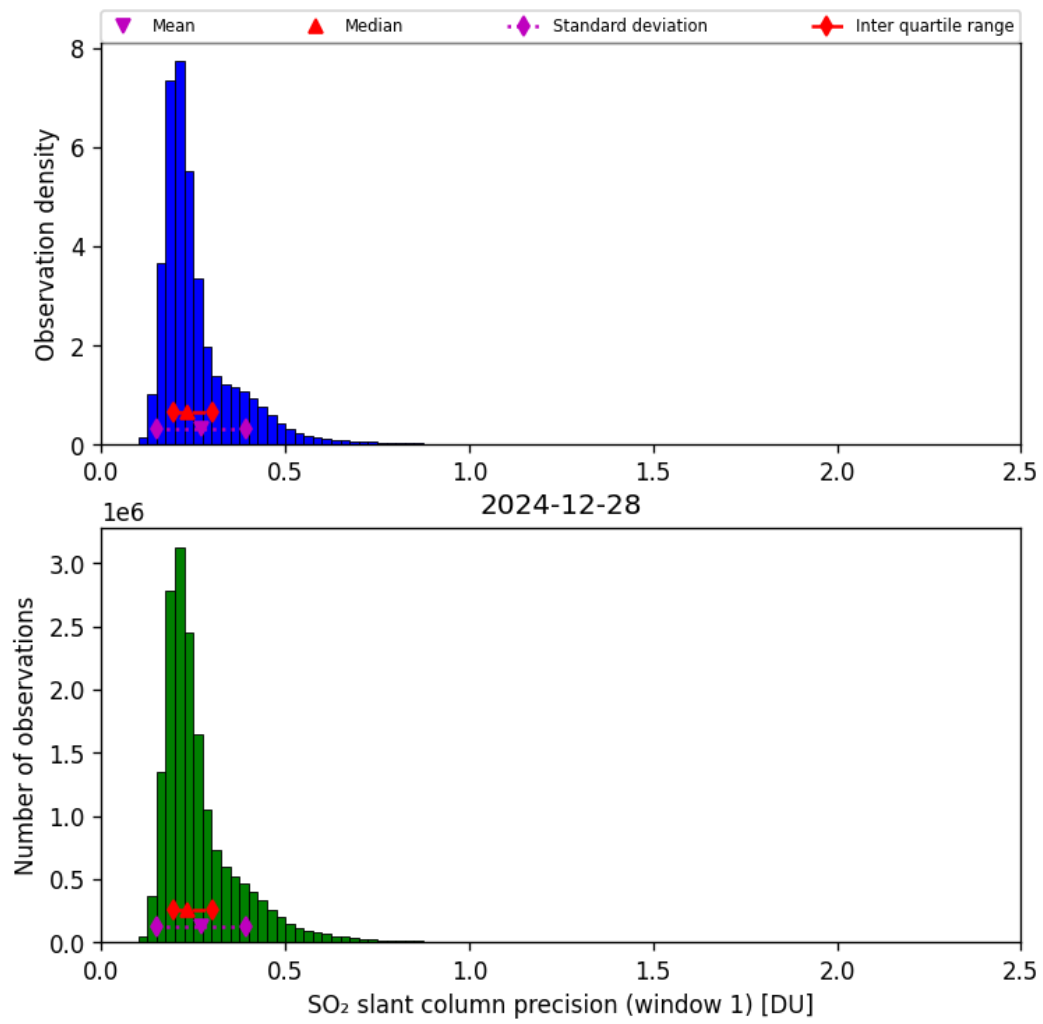
Figure 64: Histogram of “SO 2 slant column precision (window 1)” for 2024-12-28 to 2024-12-29
