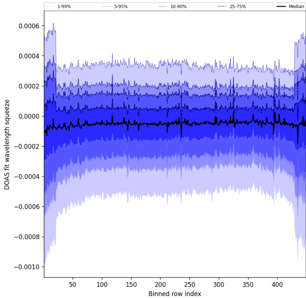
Figure 105: Along track statistics of “DOAS fit wavelength squeeze” for 2024-12-28 to 2024-12-29
