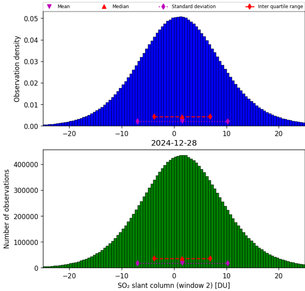
Figure 67: Histogram of “SO 2 slant column (window 2)” for 2024-12-28 to 2024-12-29
