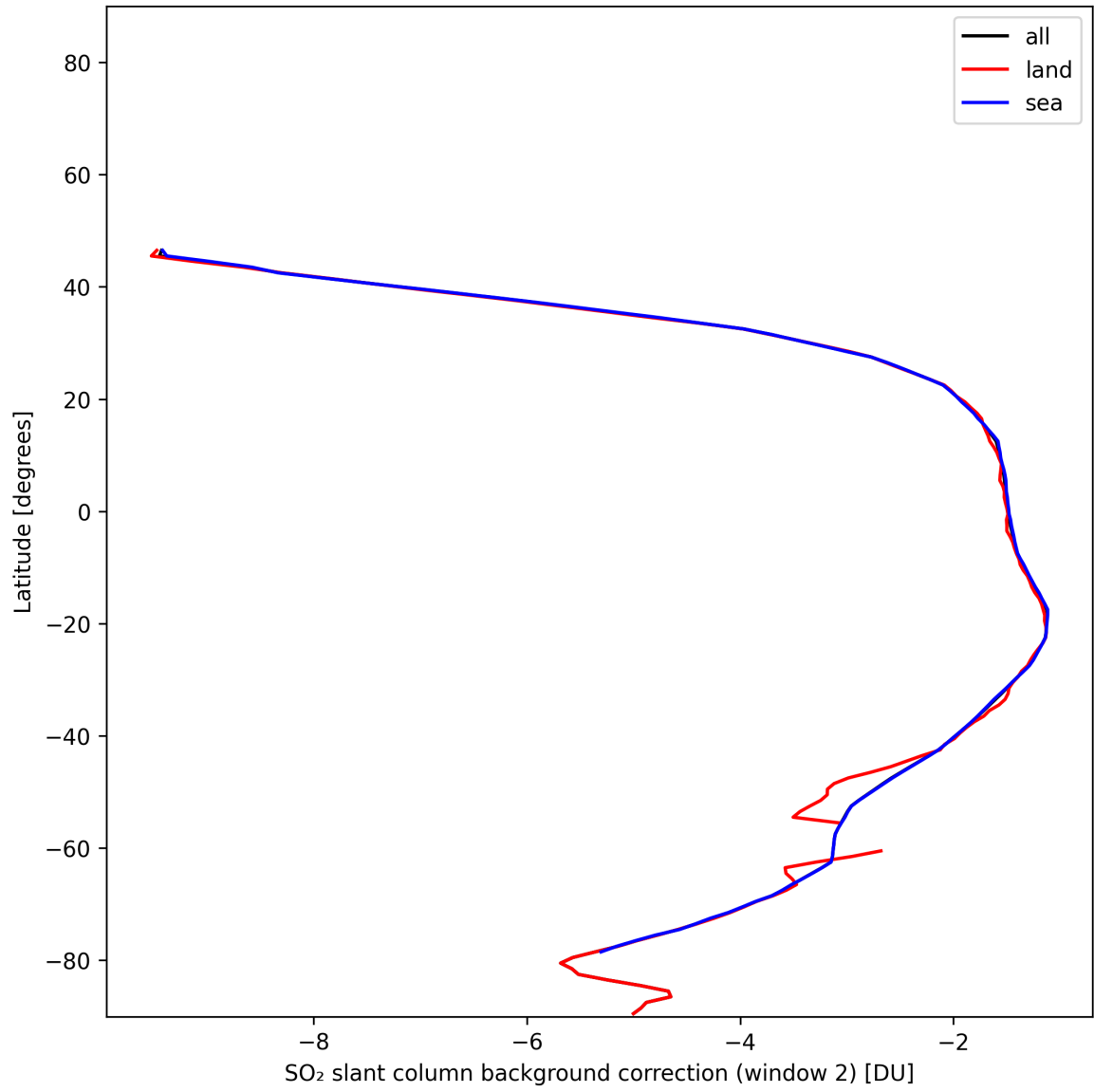
Figure 43: Zonal average of “SO 2 slant column background correction (window 2)” for 2024-12-28 to 2024-12-29.
