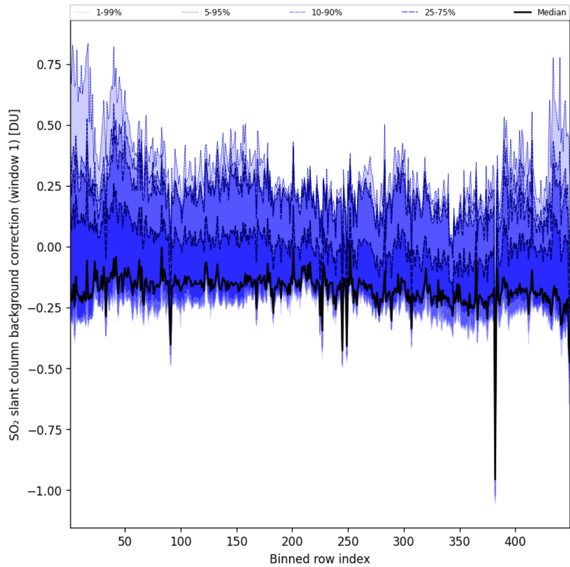
Figure 93: Along track statistics of “SO 2 slant column background correction (window 1)” for 2024-12-28 to 2024-12-29
