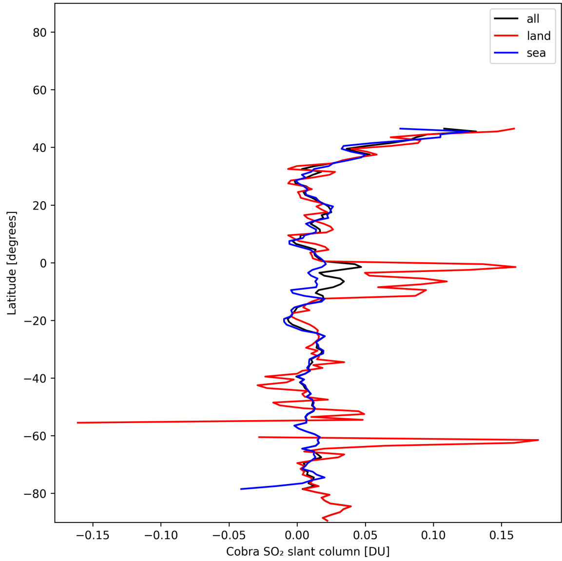
Figure 34: Zonal average of “Cobra SO 2 slant column” for 2024-12-28 to 2024-12-29.
