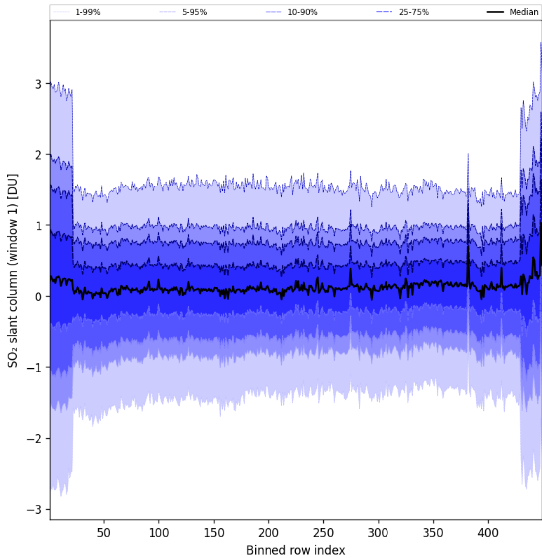
Figure 90: Along track statistics of “SO 2 slant column (window 1)” for 2024-12-28 to 2024-12-29
