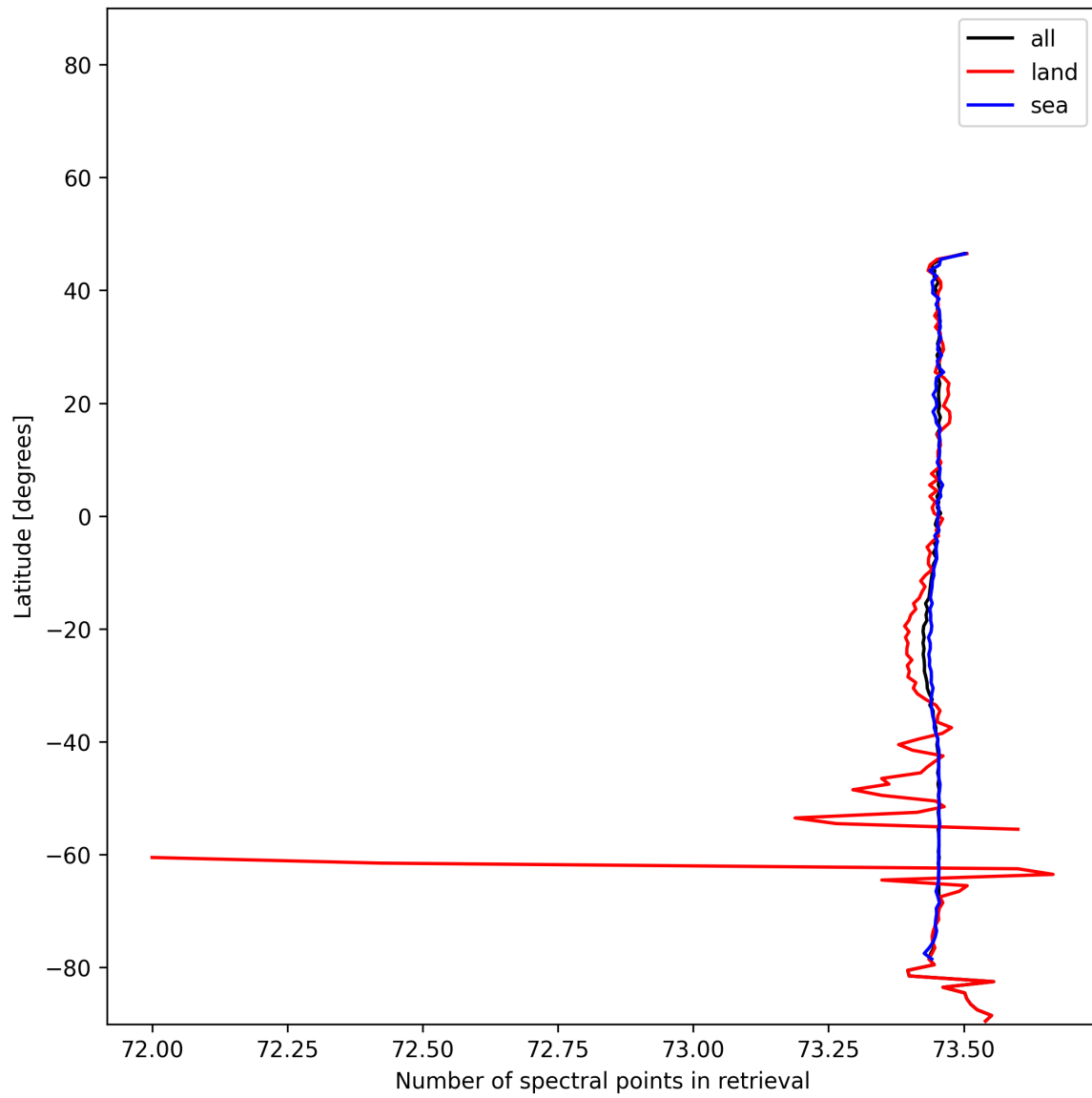
Figure 56: Zonal average of “Number of spectral points in retrieval” for 2024-12-28 to 2024-12-29.
