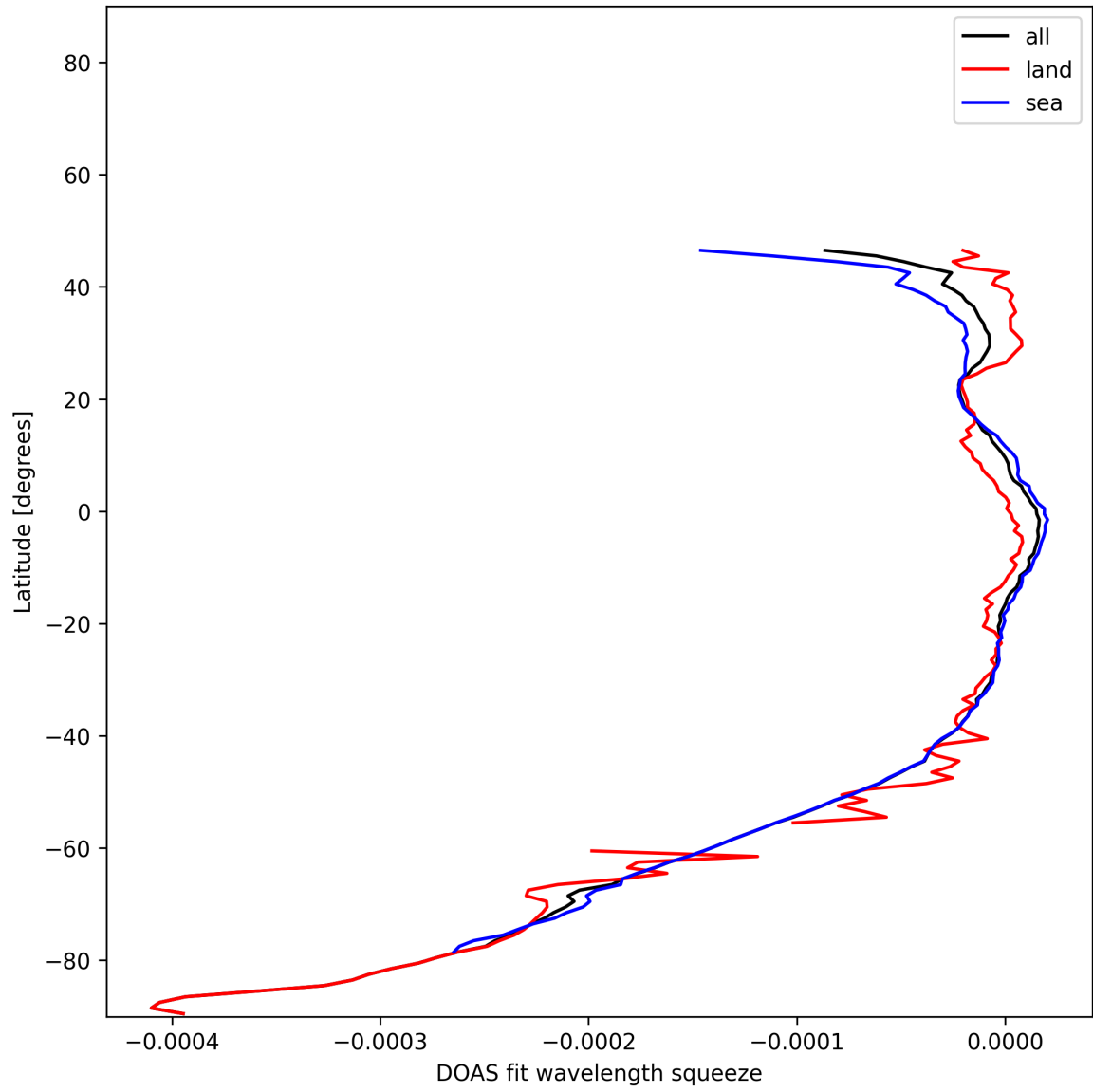
Figure 51: Zonal average of “DOAS fit wavelength squeeze” for 2024-12-28 to 2024-12-29.
