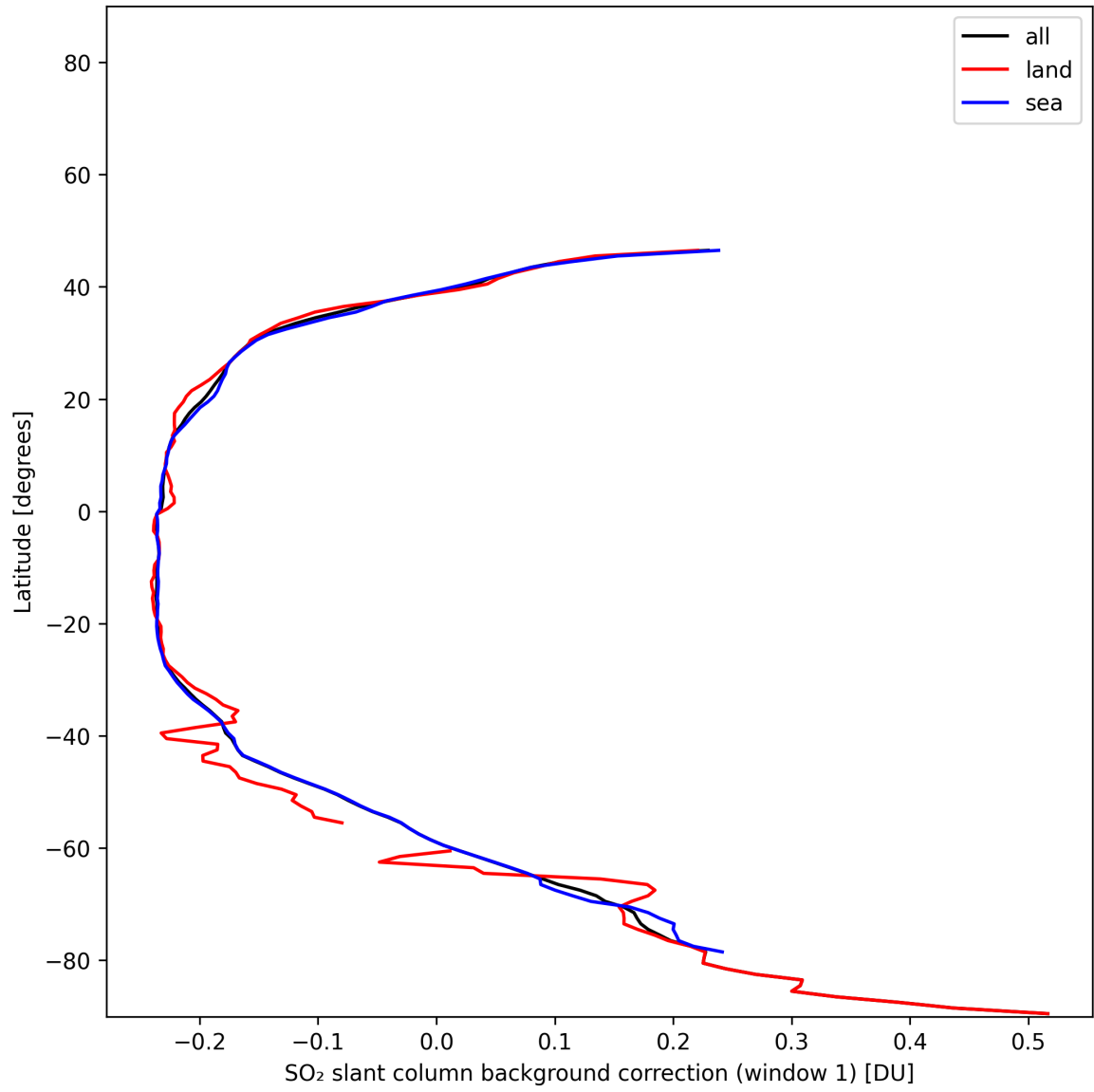
Figure 39: Zonal average of “SO 2 slant column background correction (window 1)” for 2024-12-28 to 2024-12-29.
