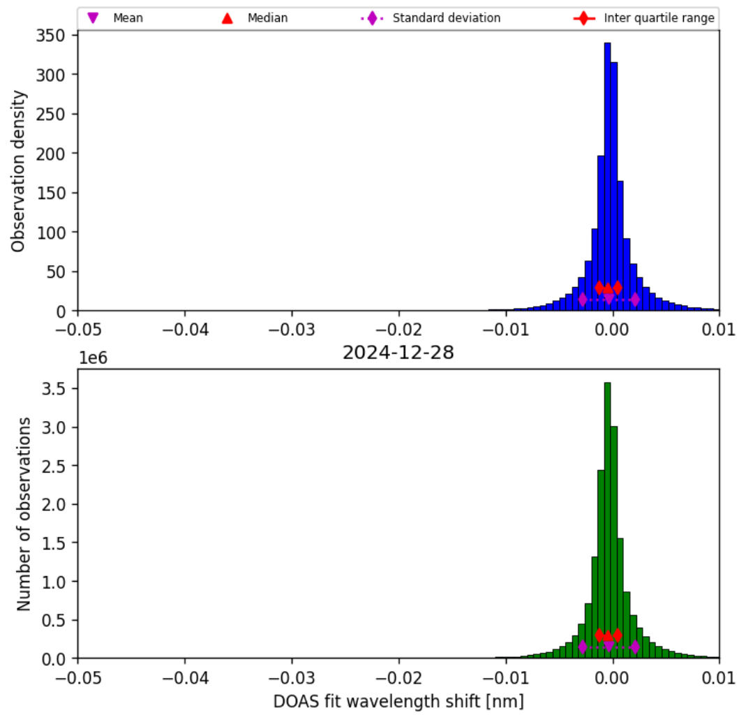
Figure 77: Histogram of “DOAS fit wavelength shift” for 2024-12-28 to 2024-12-29
