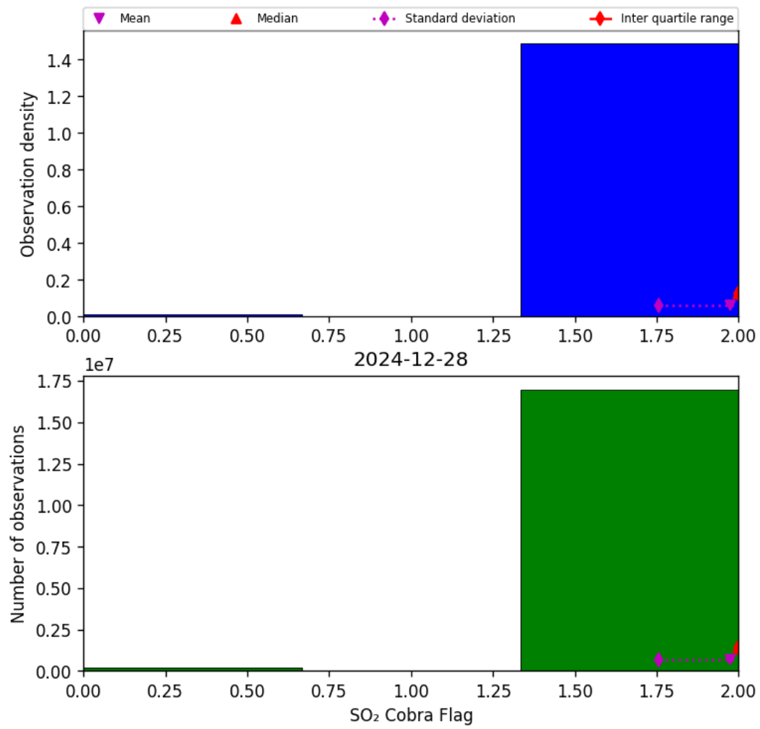
Figure 75: Histogram of “SO 2 Cobra Flag” for 2024-12-28 to 2024-12-29
