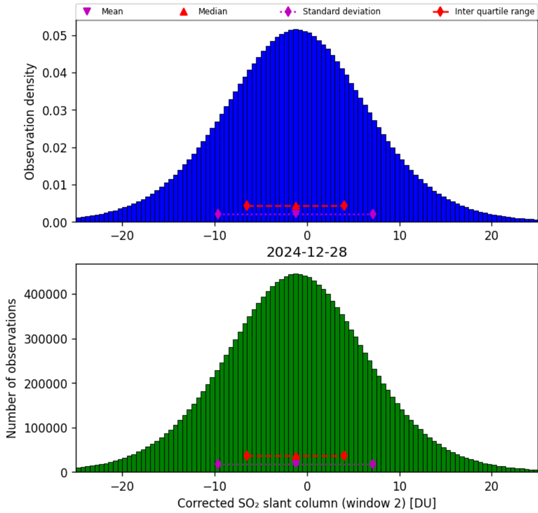
Figure 69: Histogram of “Corrected SO 2 slant column (window 2)” for 2024-12-28 to 2024-12-29
