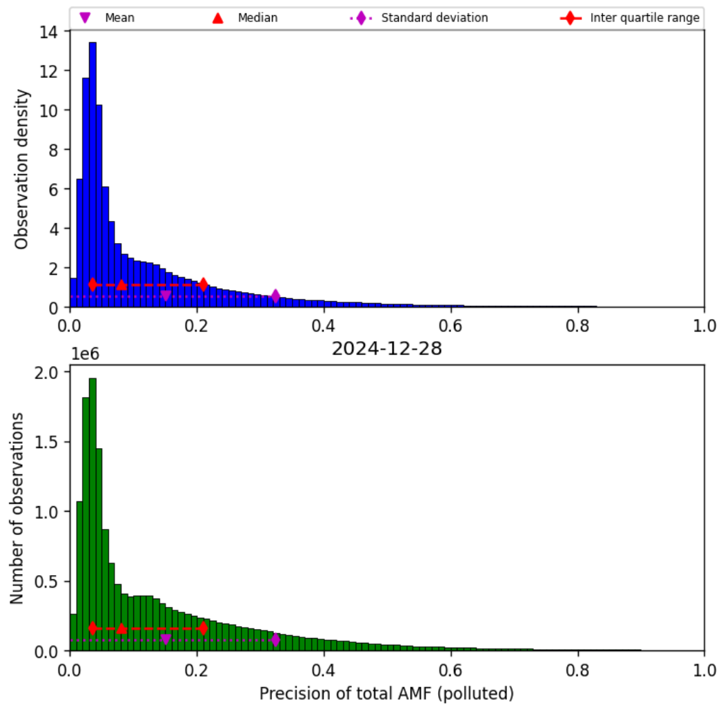
Figure 81: Histogram of “Precision of total AMF (polluted)” for 2024-12-28 to 2024-12-29
