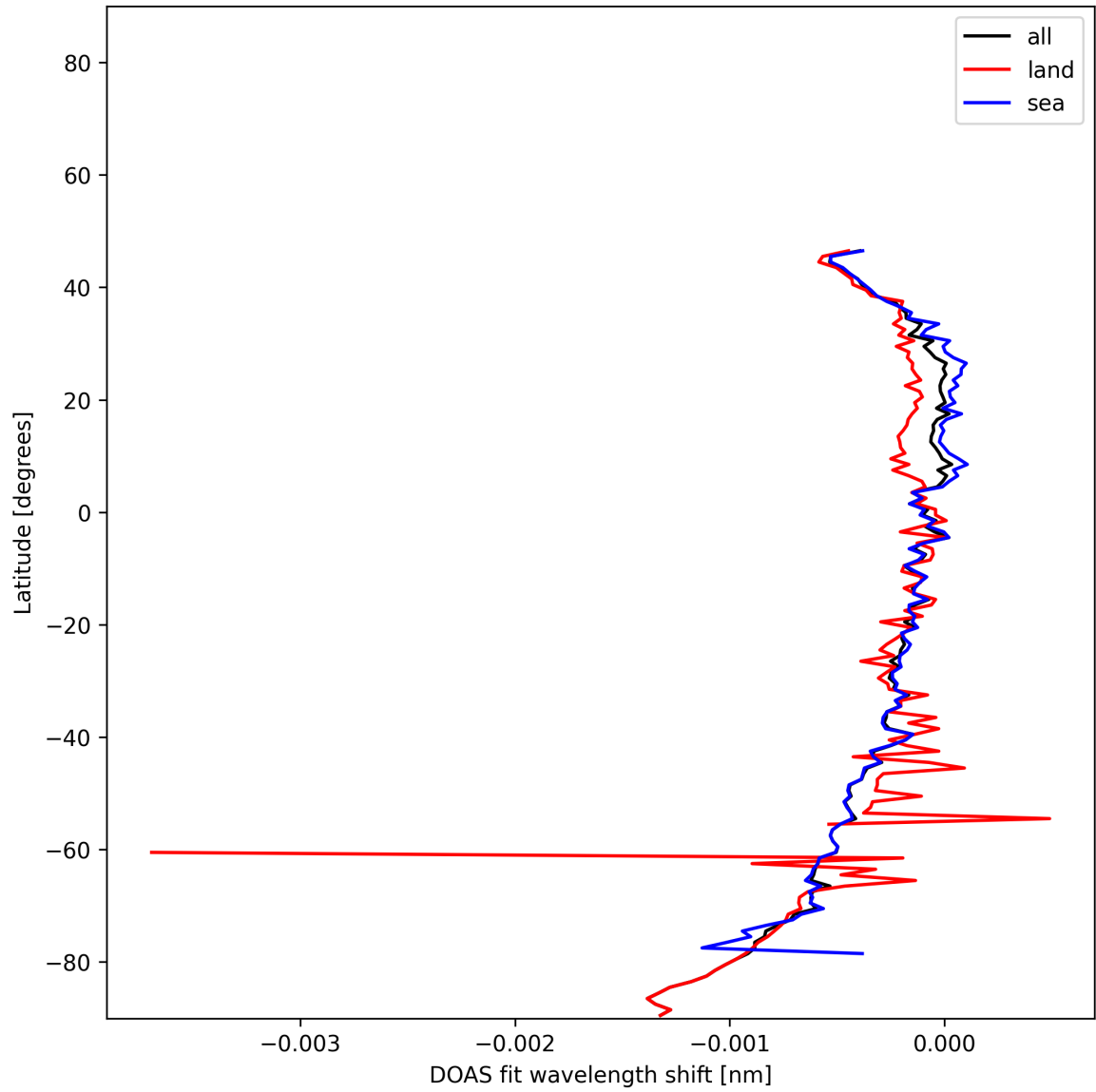
Figure 50: Zonal average of "DOAS fit wavelength shift" for 2024-12-28 to 2024-12-29.
