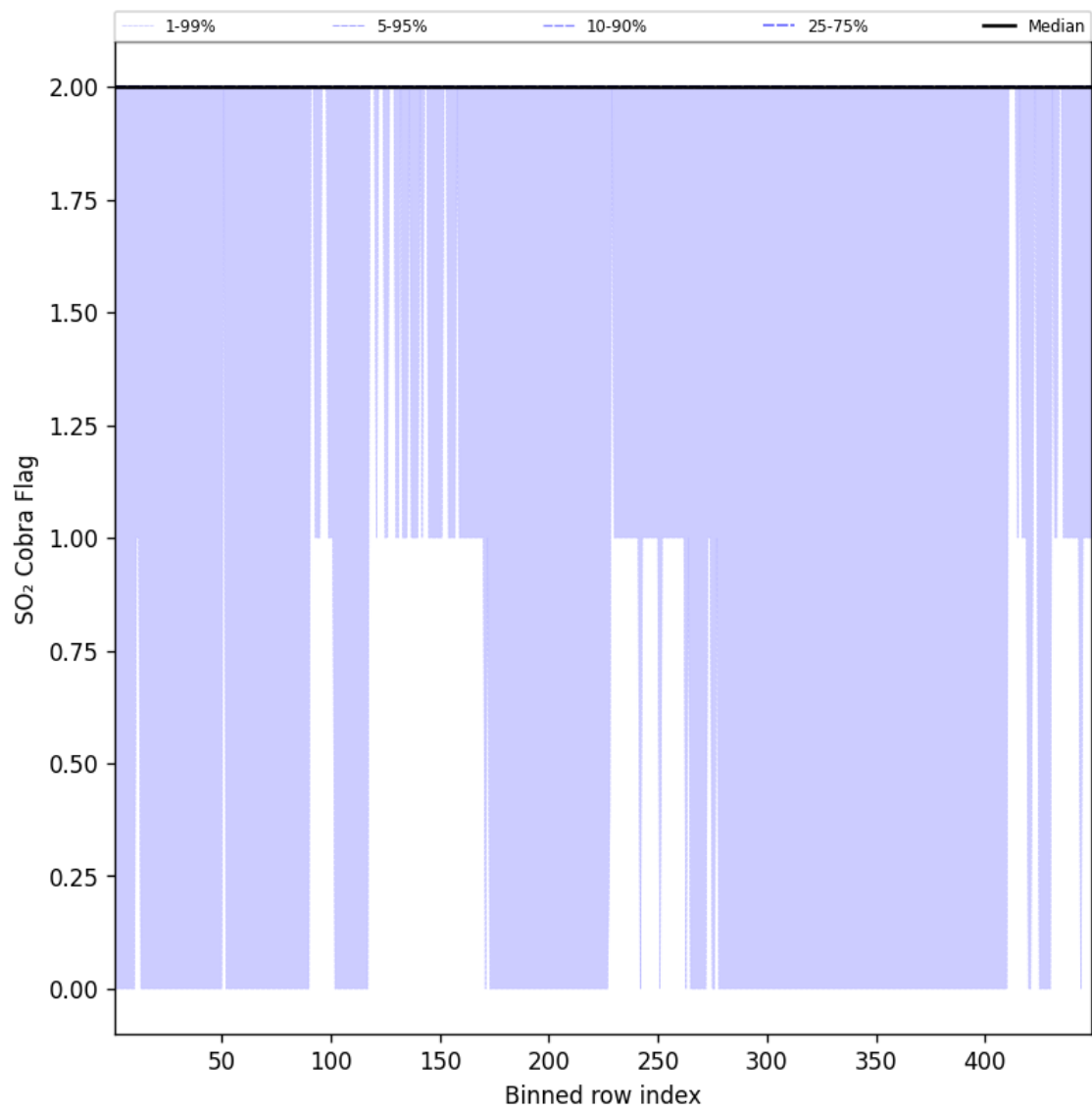
Figure 102: Along track statistics of “SO 2 Cobra Flag” for 2024-12-28 to 2024-12-29
