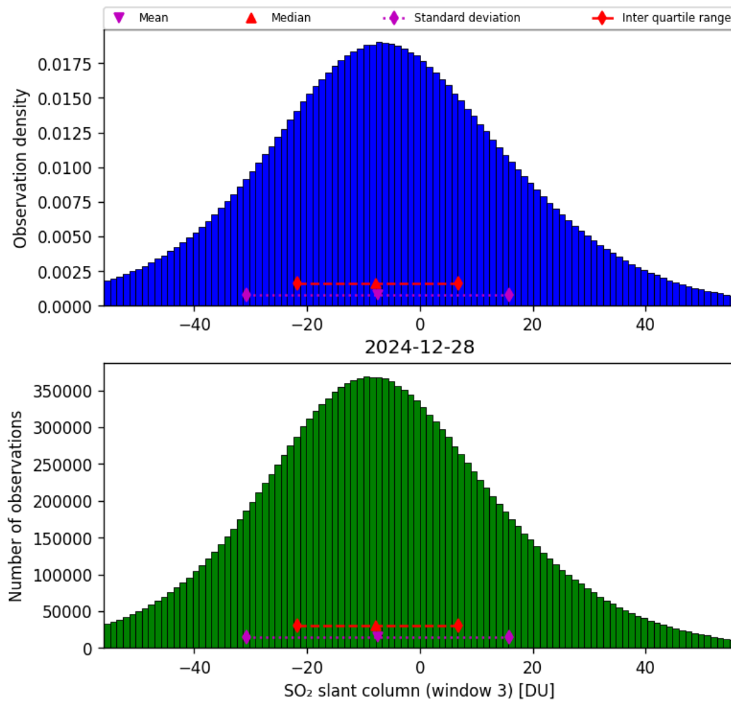
Figure 71: Histogram of “SO 2 slant column (window 3)” for 2024-12-28 to 2024-12-29
