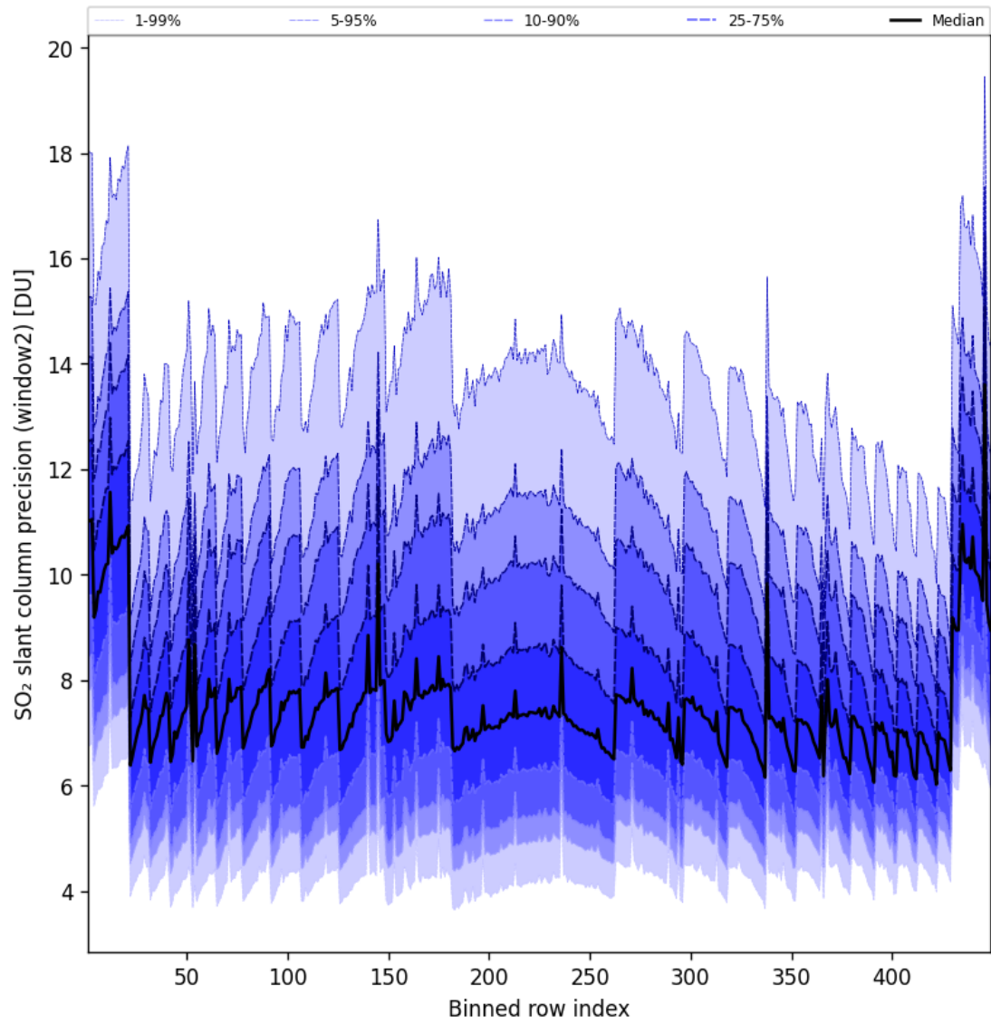
Figure 95: Along track statistics of “SO 2 slant column precision (window2)” for 2024-12-28 to 2024-12-29
