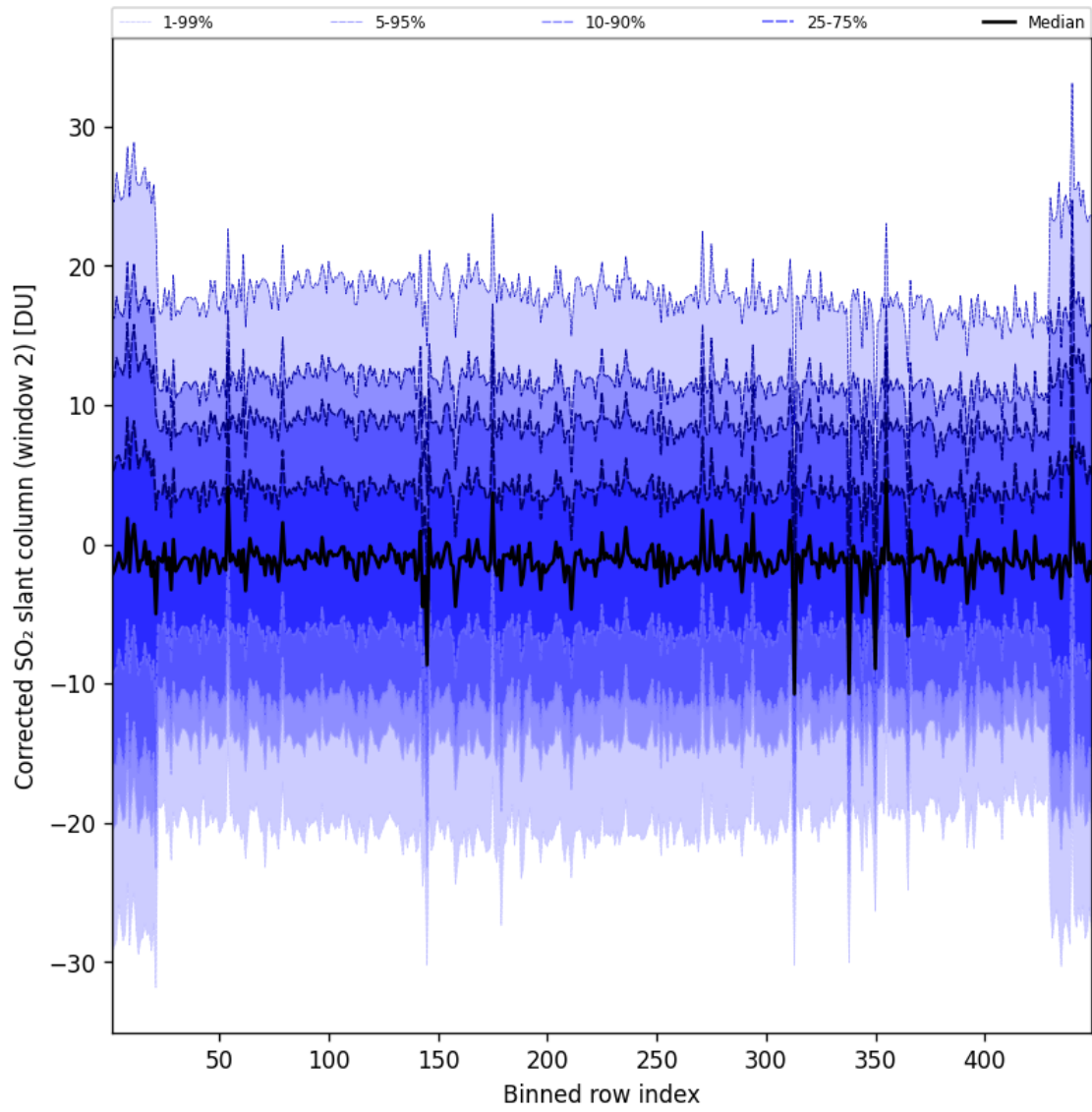
Figure 96: Along track statistics of “Corrected SO 2 slant column (window 2)” for 2024-12-28 to 2024-12-29
