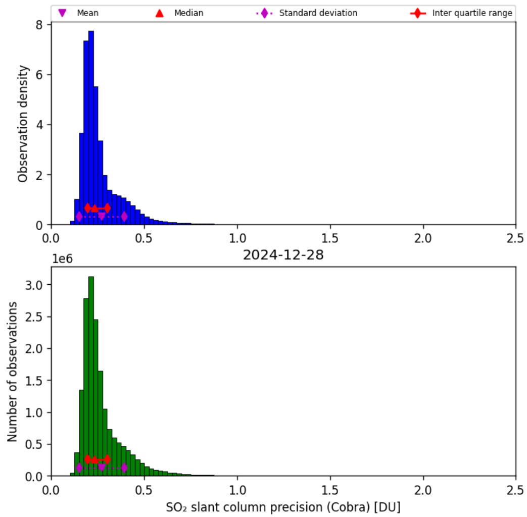
Figure 62: Histogram of “SO 2 slant column precision (Cobra)” for 2024-12-28 to 2024-12-29
