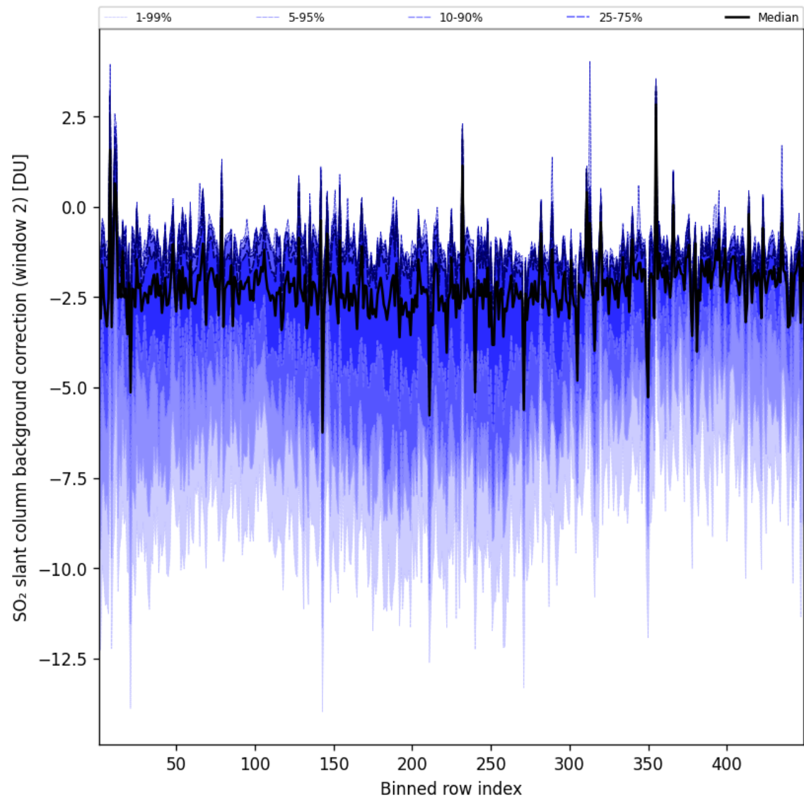
Figure 97: Along track statistics of “SO 2 slant column background correction (window 2)” for 2024-12-28 to 2024-12-29
