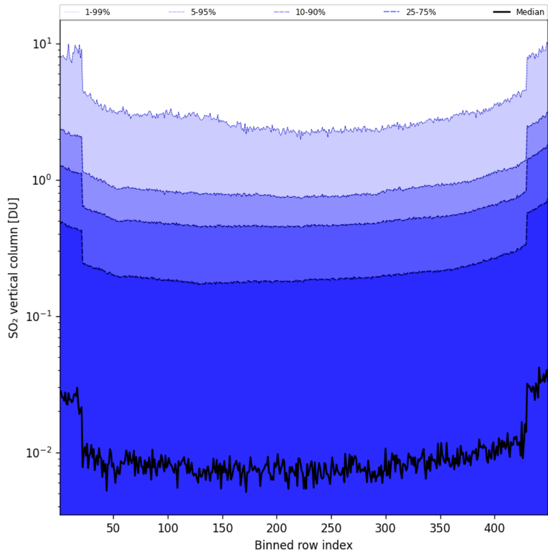
Figure 85: Along track statistics of “SO 2 vertical column” for 2024-12-28 to 2024-12-29
