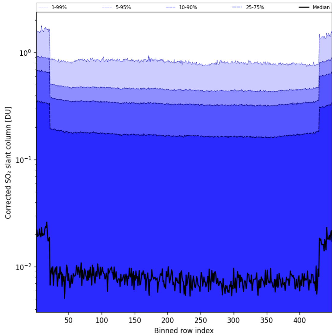
Figure 87: Along track statistics of “Corrected SO 2 slant column” for 2024-12-28 to 2024-12-29
