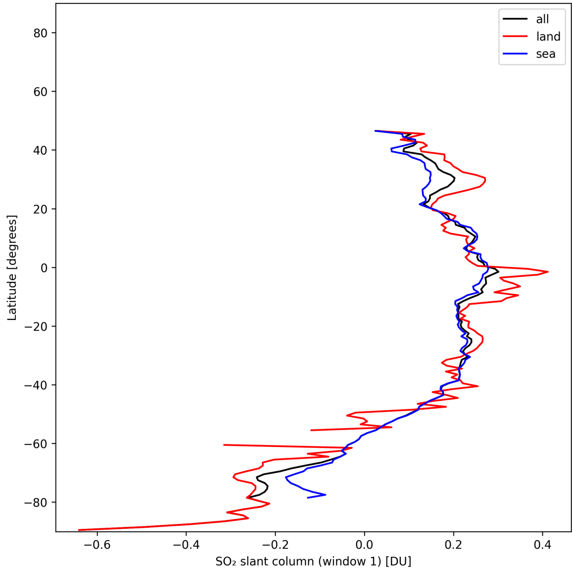
Figure 36: Zonal average of “SO 2 slant column (window 1)” for 2024-12-28 to 2024-12-29.
