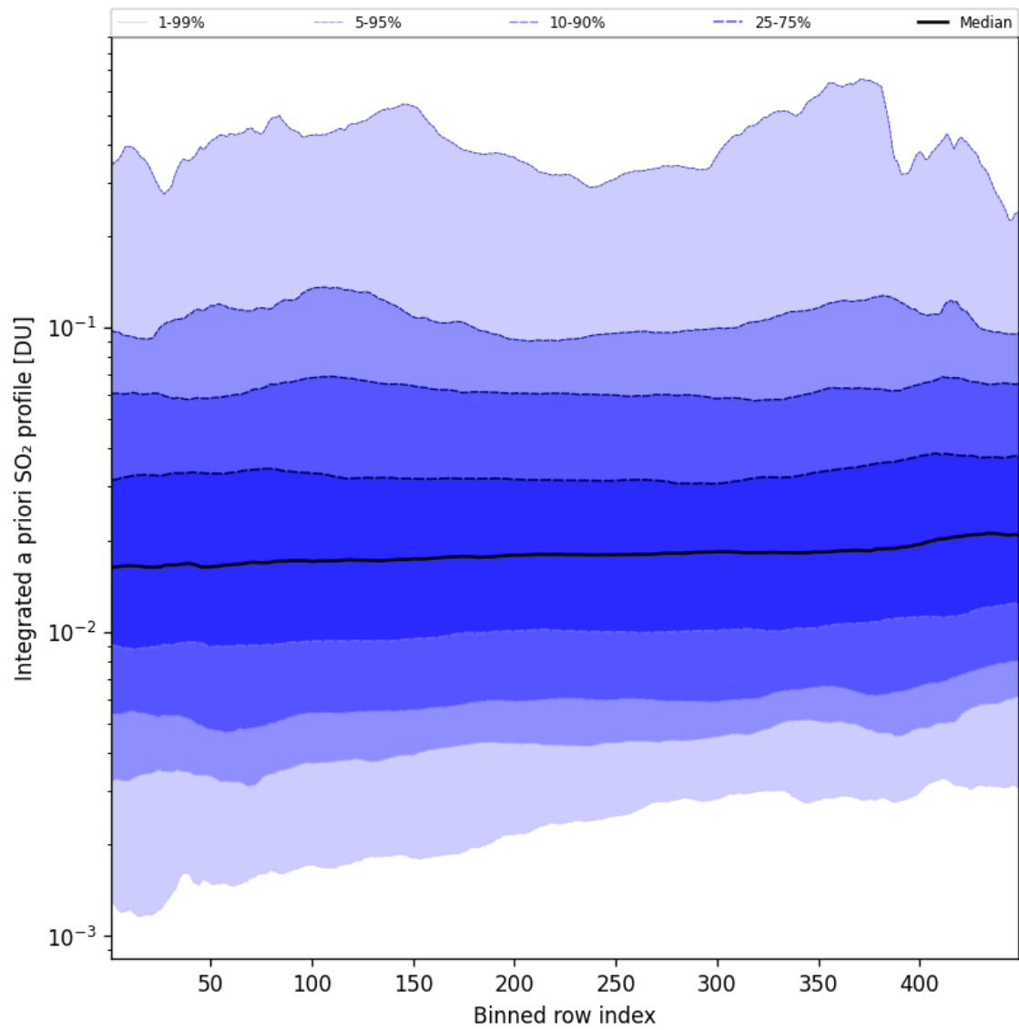
Figure 103: Along track statistics of “Integrated a priori SO 2 profile” for 2024-12-28 to 2024-12-29
