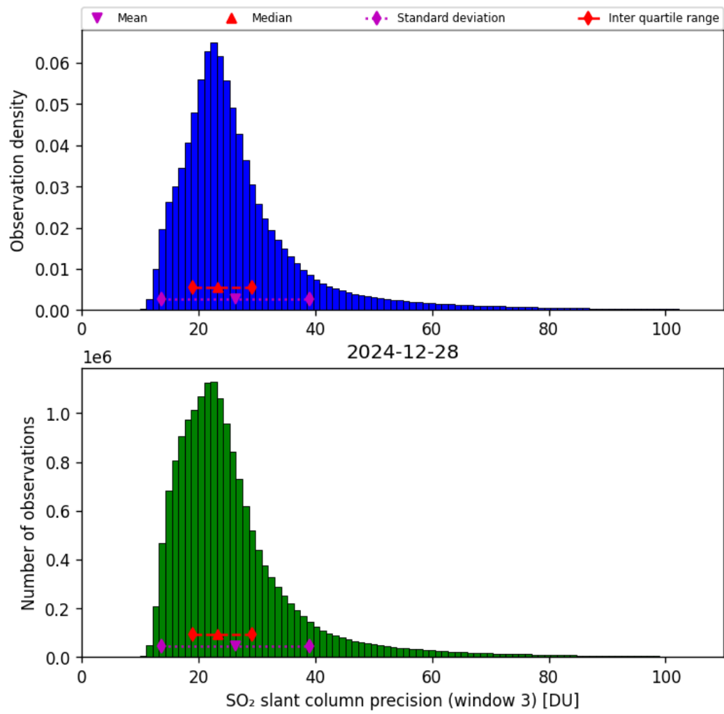
Figure 72: Histogram of “SO 2 slant column precision (window 3)” for 2024-12-28 to 2024-12-29
