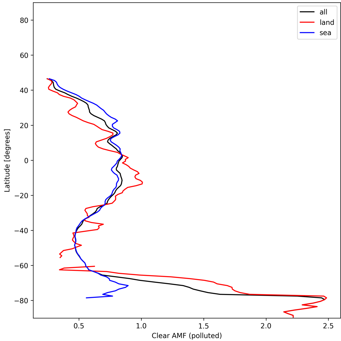
Figure 55: Zonal average of “Clear AMF (polluted)” for 2024-12-28 to 2024-12-29.
