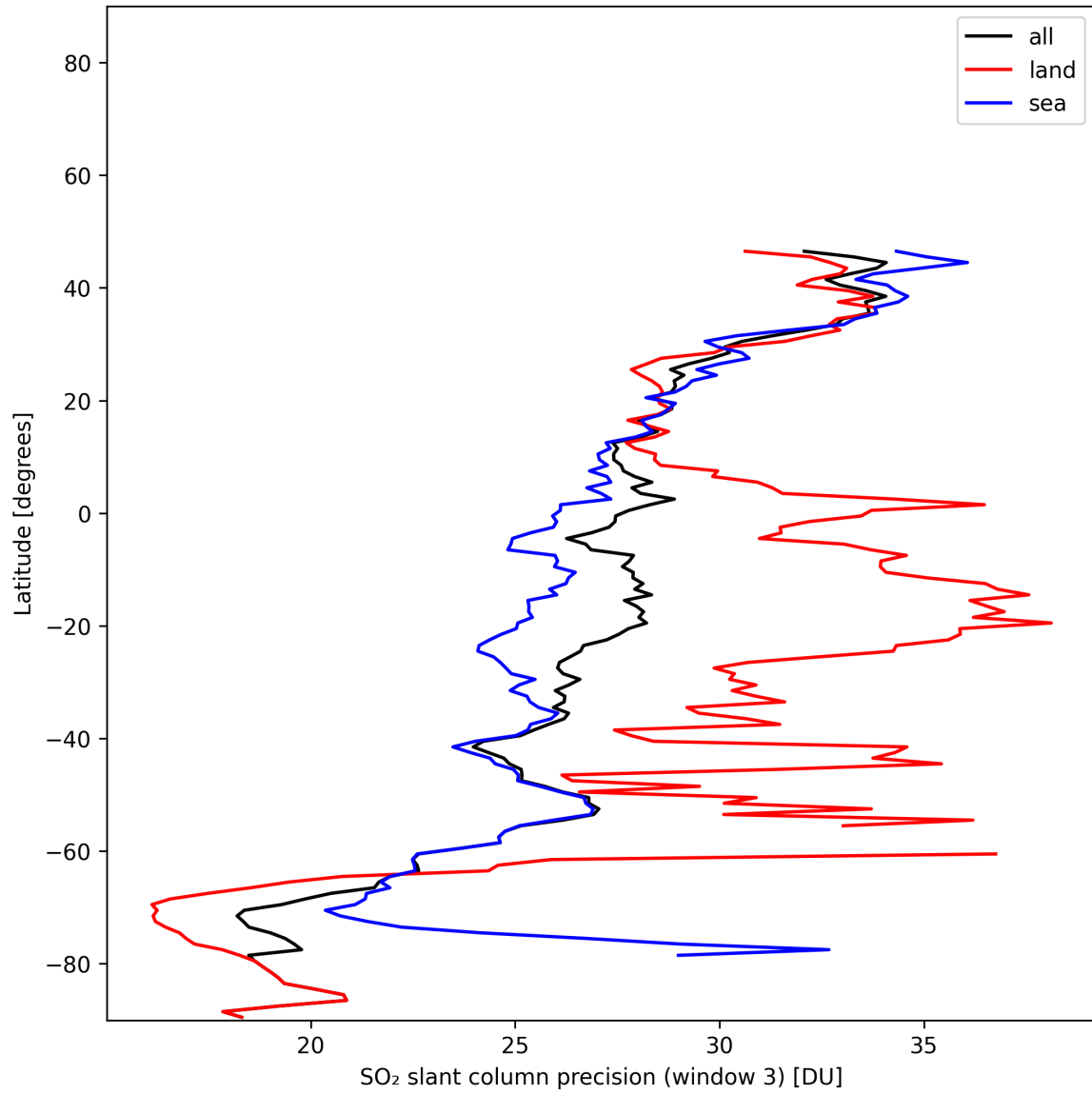
Figure 45: Zonal average of “SO 2 slant column precision (window 3)” for 2024-12-28 to 2024-12-29.
