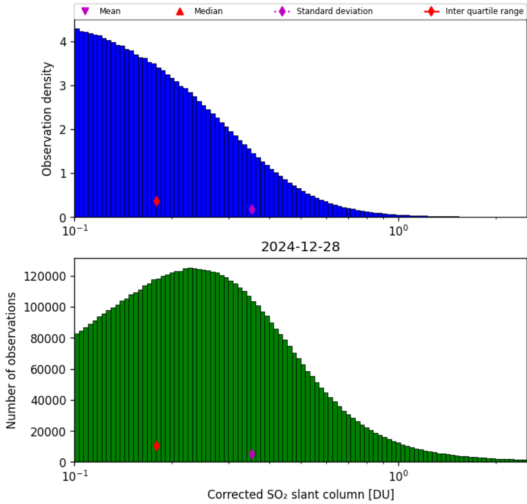
Figure 60: Histogram of “Corrected SO 2 slant column” for 2024-12-28 to 2024-12-29
