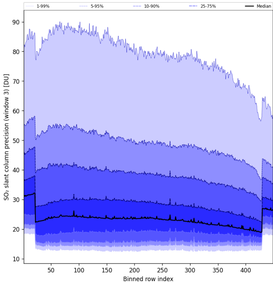
Figure 99: Along track statistics of “SO 2 slant column precision (window 3)” for 2024-12-28 to 2024-12-29
