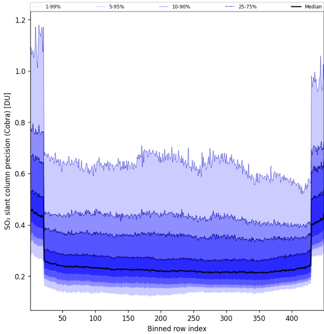
Figure 89: Along track statistics of “SO 2 slant column precision (Cobra)” for 2024-12-28 to 2024-12-29
