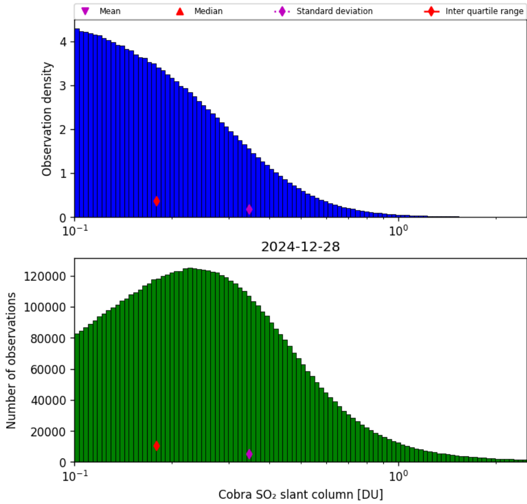
Figure 61: Histogram of “Cobra SO 2 slant column” for 2024-12-28 to 2024-12-29
