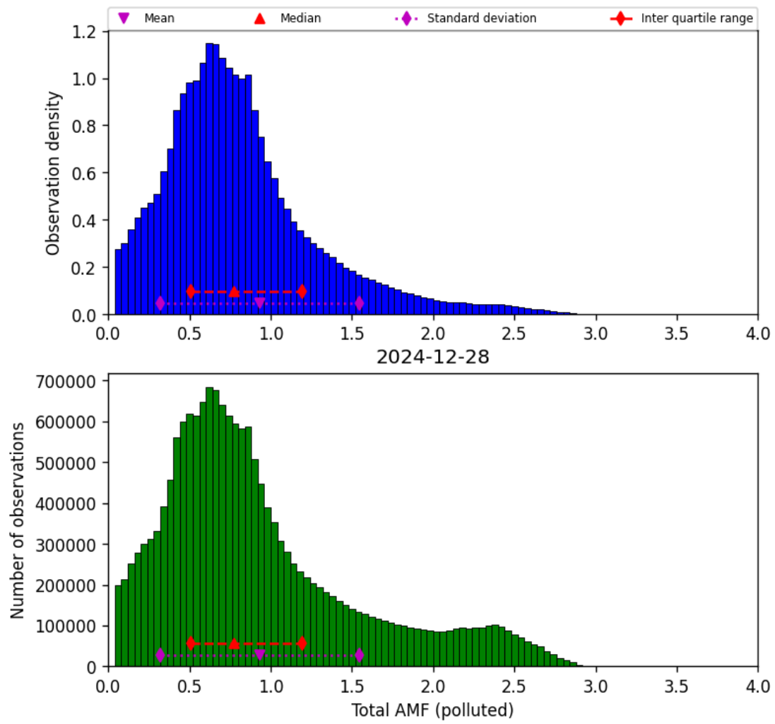
Figure 80: Histogram of “Total AMF (polluted)” for 2024-12-28 to 2024-12-29
