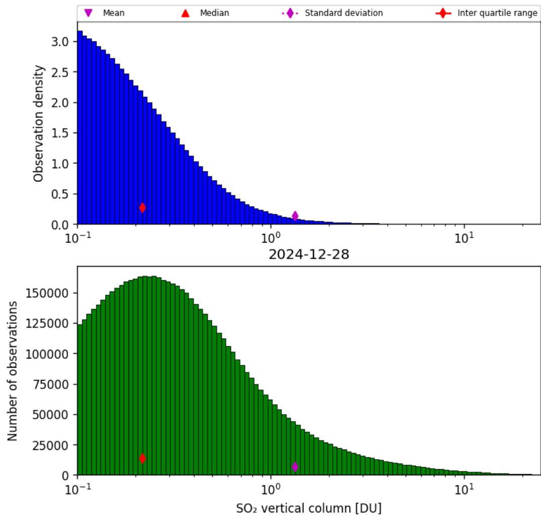
Figure 58: Histogram of “SO 2 vertical column” for 2024-12-28 to 2024-12-29
