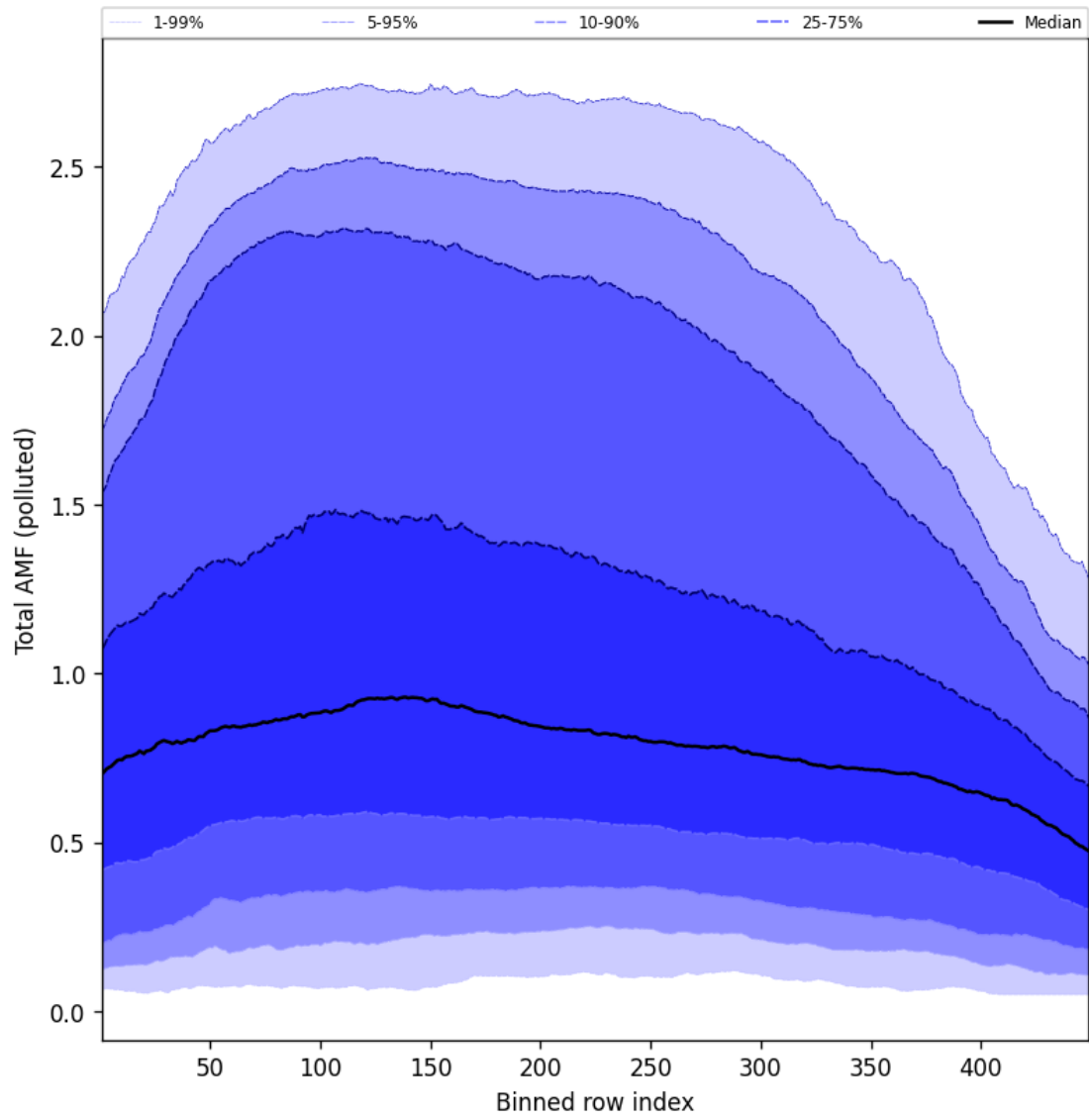
Figure 107: Along track statistics of “Total AMF (polluted)” for 2024-12-28 to 2024-12-29
