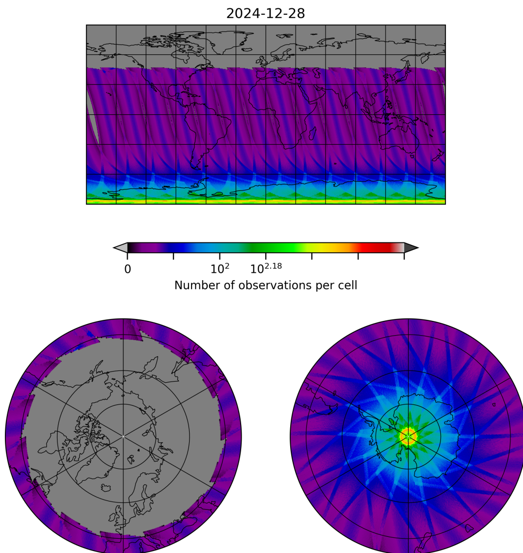
Figure 29: Map of the number of observations for 2024-12-28 to 2024-12-29
