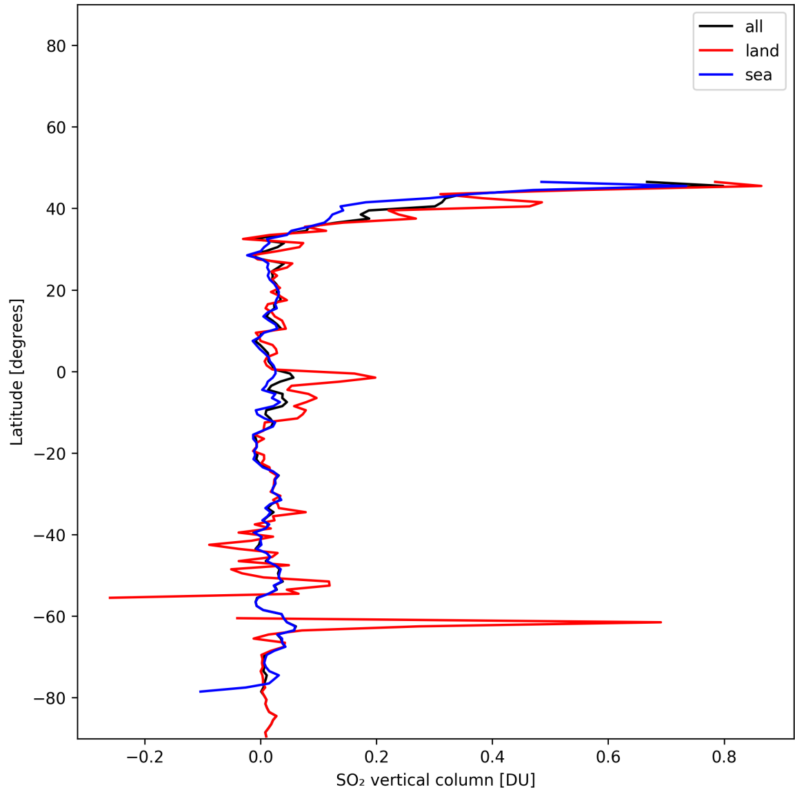
Figure 31: Zonal average of “SO 2 vertical column” for 2024-12-28 to 2024-12-29.
