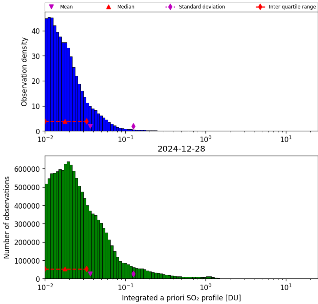
Figure 76: Histogram of “Integrated a priori SO 2 profile” for 2024-12-28 to 2024-12-29
