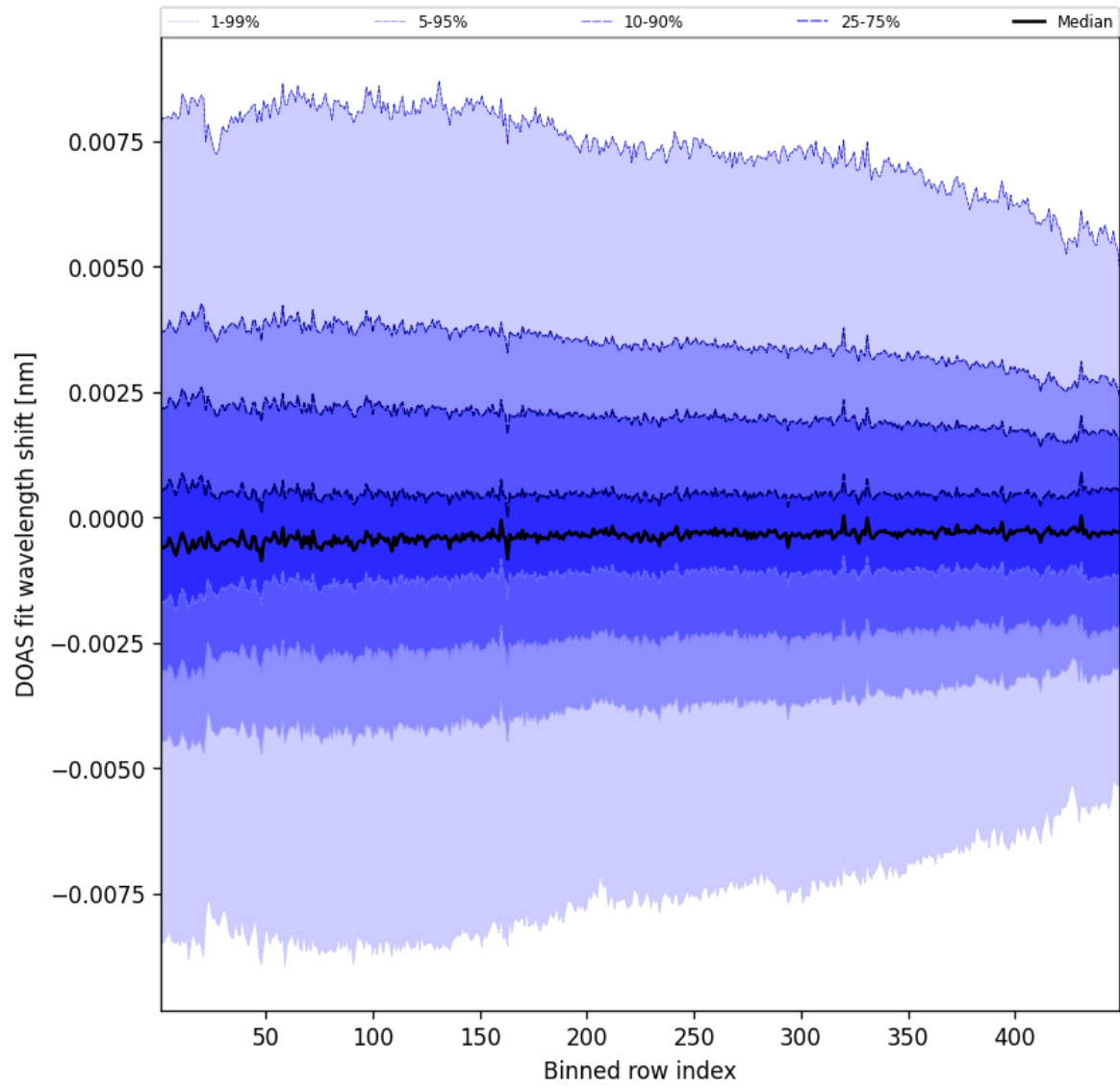
Figure 104: Along track statistics of “DOAS fit wavelength shift” for 2024-12-28 to 2024-12-29
