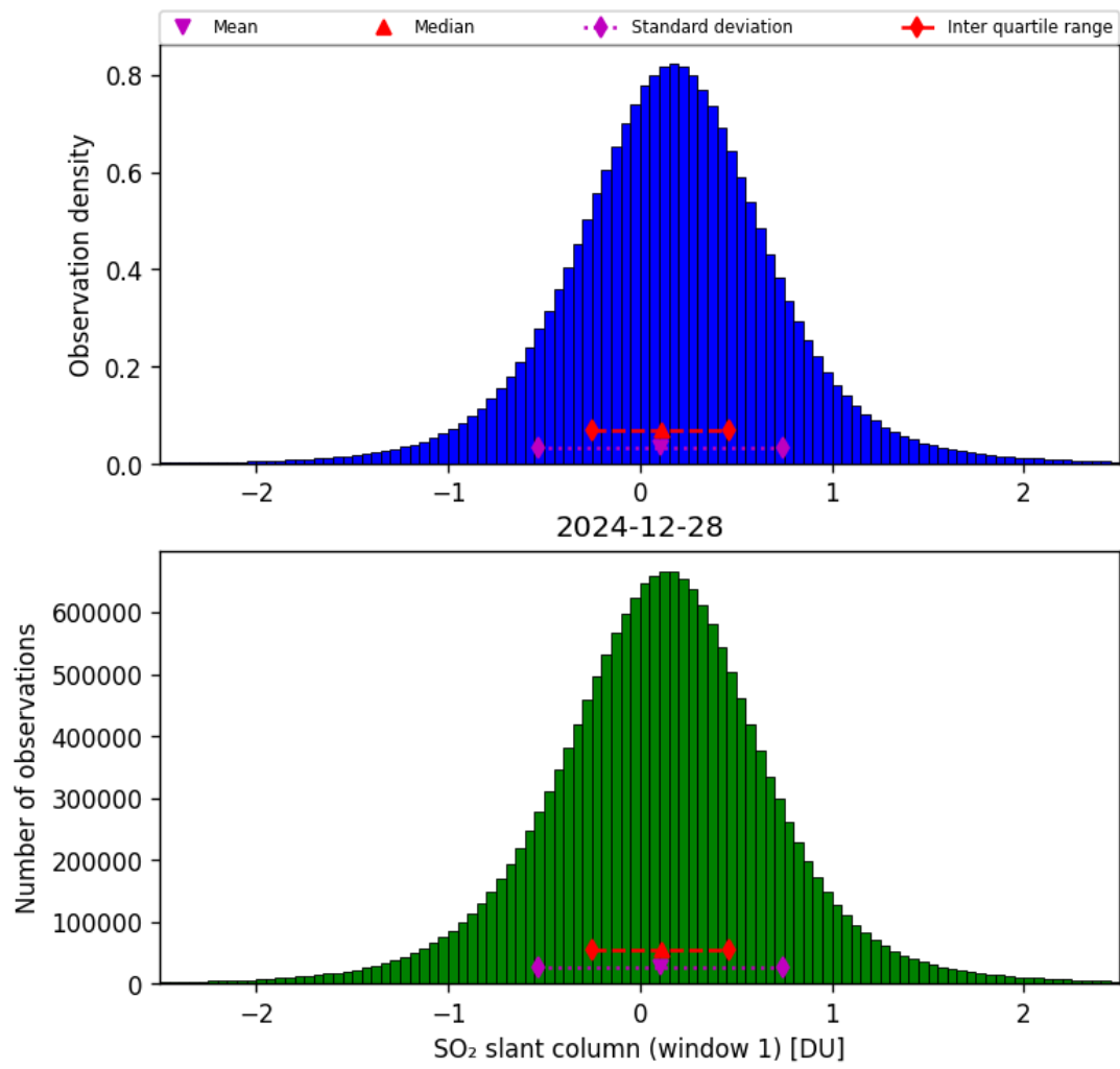
Figure 63: Histogram of “SO 2 slant column (window 1)” for 2024-12-28 to 2024-12-29
