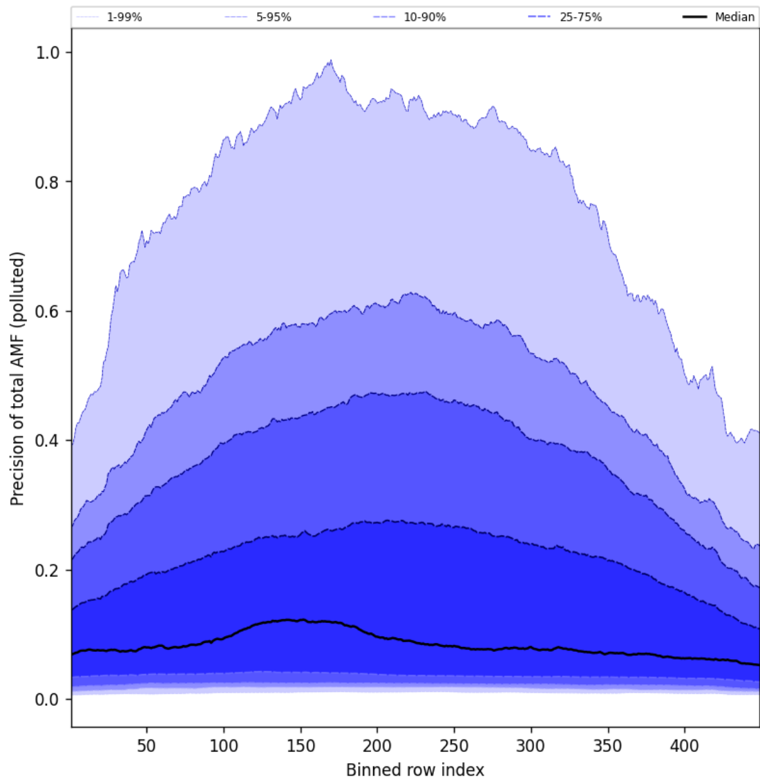
Figure 108: Along track statistics of “Precision of total AMF (polluted)” for 2024-12-28 to 2024-12-29
