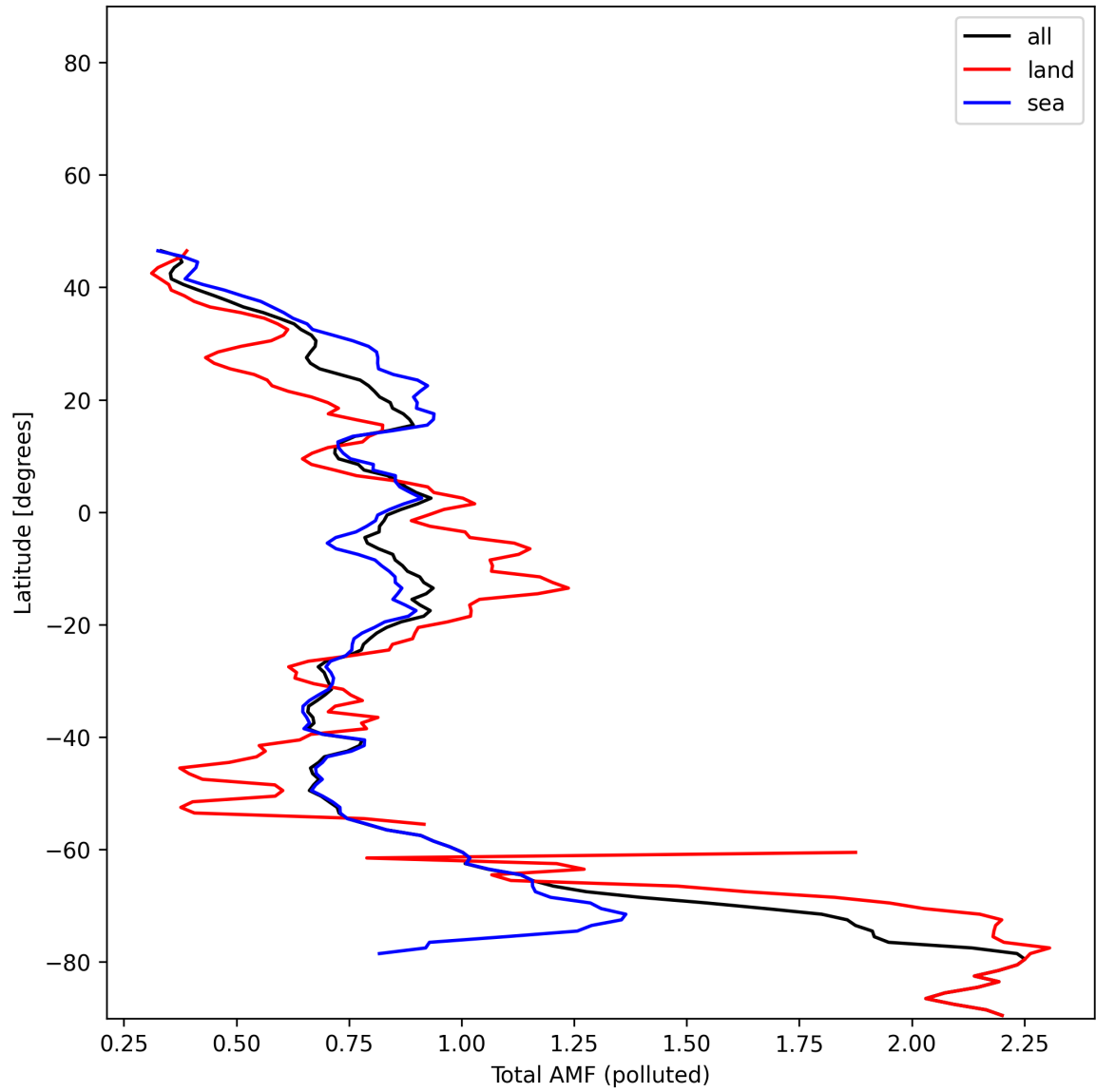
Figure 53: Zonal average of “Total AMF (polluted)” for 2024-12-28 to 2024-12-29.
