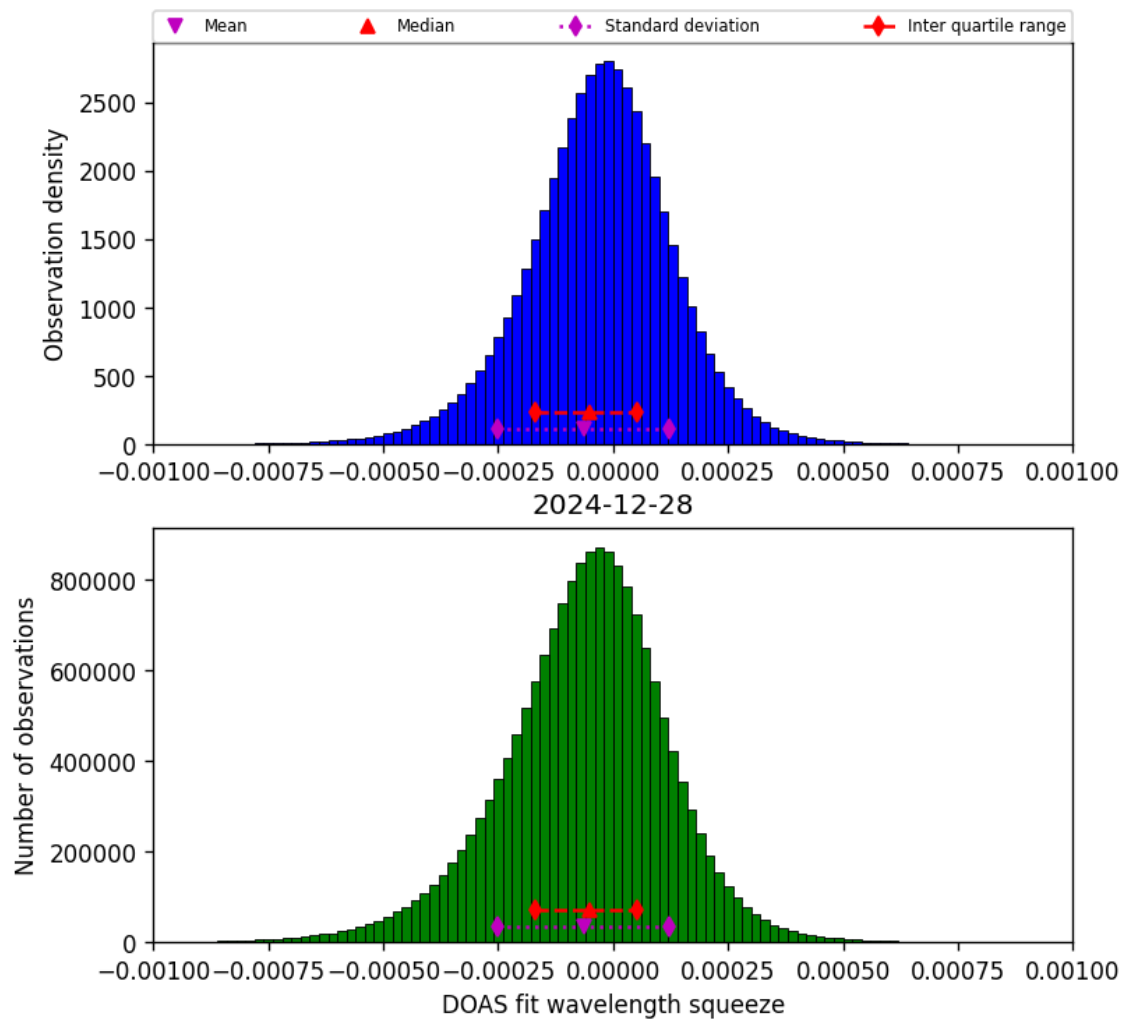
Figure 78: Histogram of “DOAS fit wavelength squeeze” for 2024-12-28 to 2024-12-29
