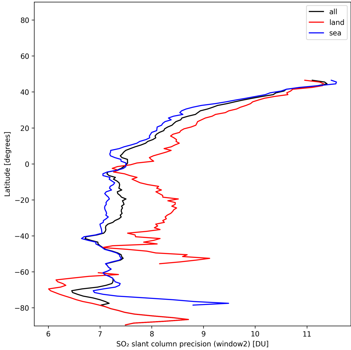
Figure 41: Zonal average of “SO 2 slant column precision (window2)” for 2024-12-28 to 2024-12-29.
