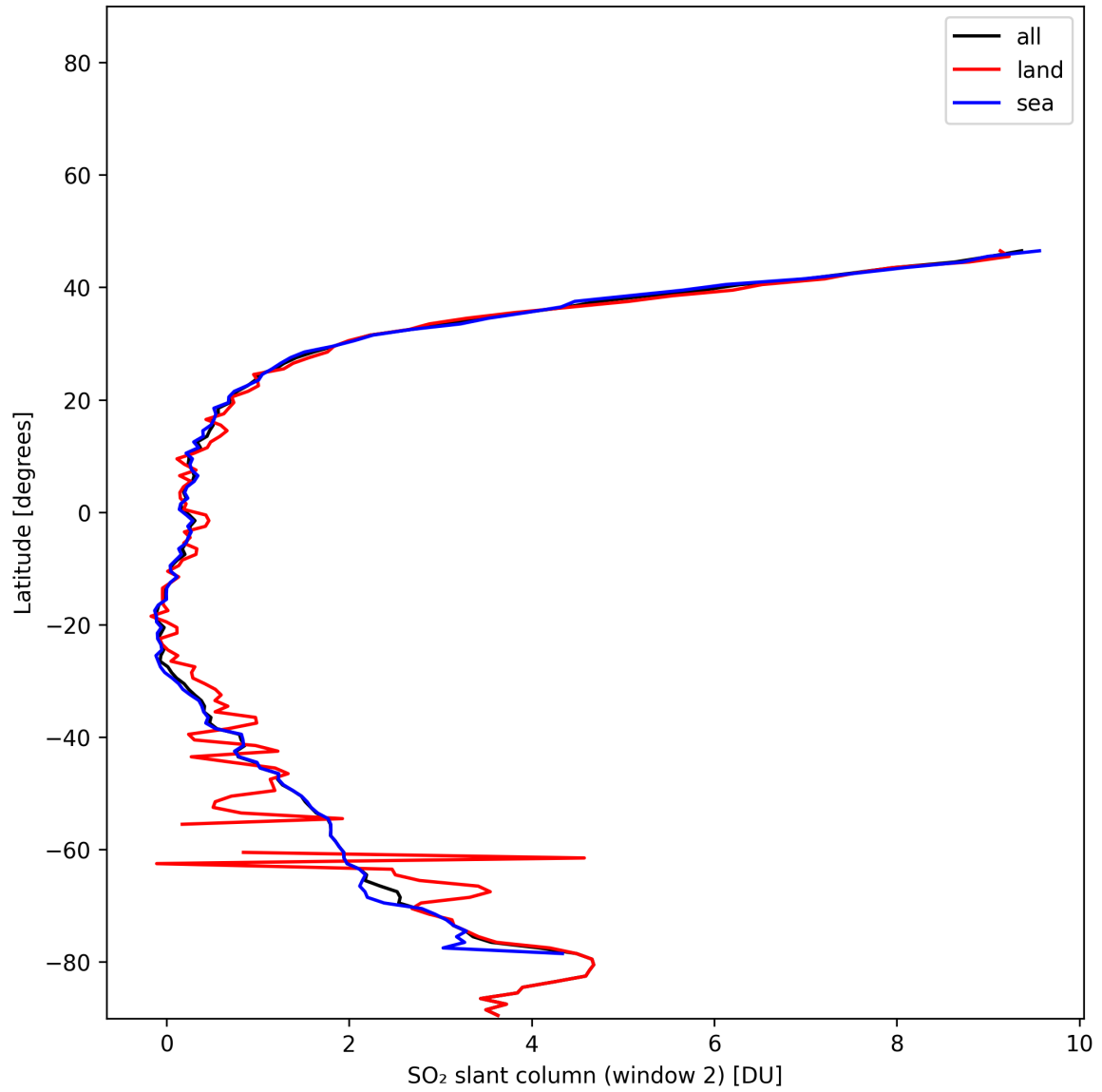
Figure 40: Zonal average of “SO 2 slant column (window 2)” for 2024-12-28 to 2024-12-29.
