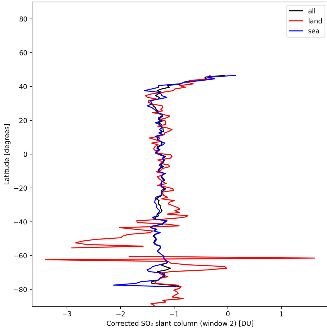
Figure 42: Zonal average of “Corrected SO 2 slant column (window 2)” for 2024-12-28 to 2024-12-29.
