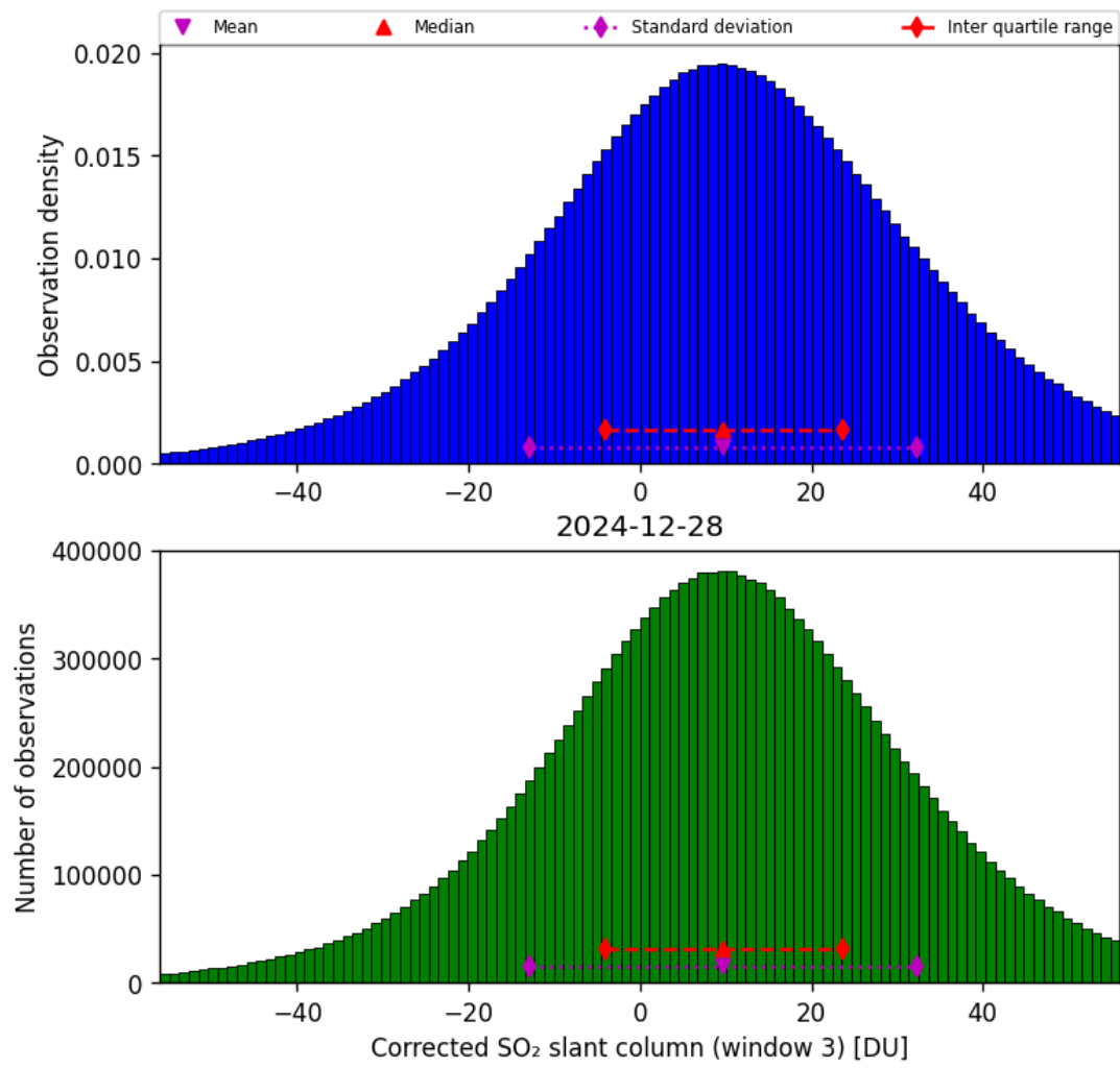
Figure 73: Histogram of “Corrected SO 2 slant column (window 3)” for 2024-12-28 to 2024-12-29
