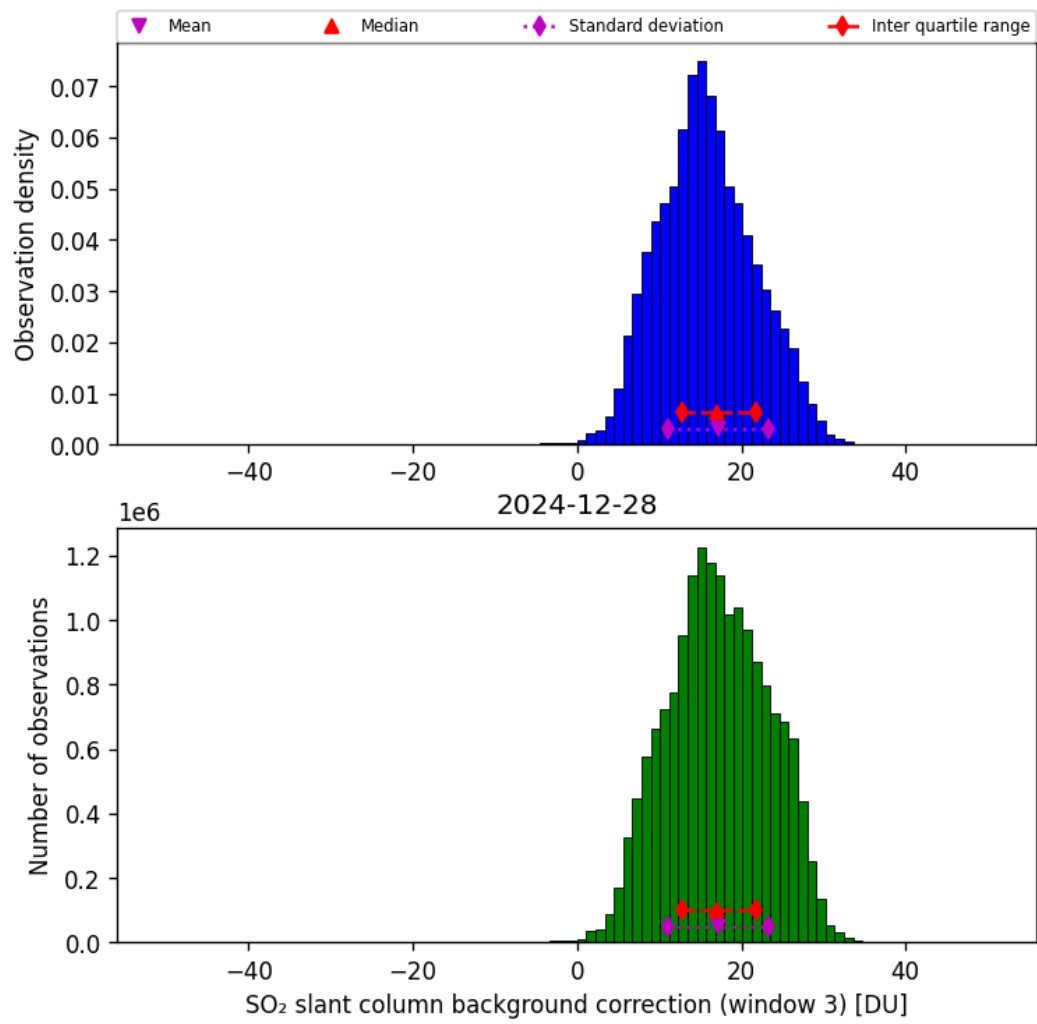
Figure 74: Histogram of “SO 2 slant column background correction (window 3)” for 2024-12-28 to 2024-12-29
