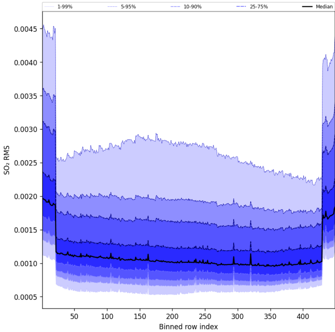
Figure 106: Along track statistics of “SO 2 RMS” for 2024-12-28 to 2024-12-29
