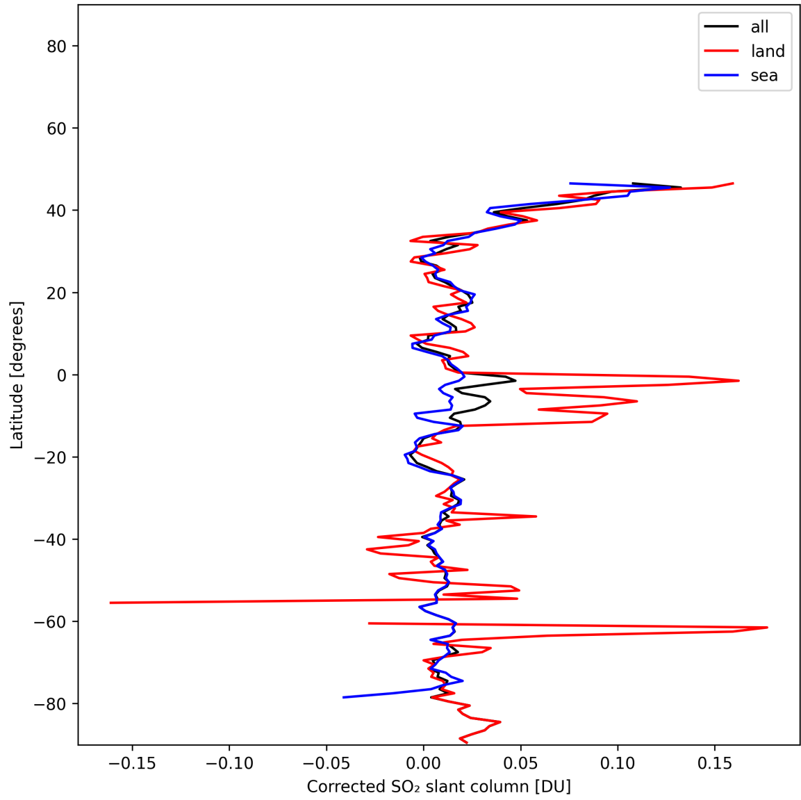
Figure 33: Zonal average of “Corrected SO 2 slant column” for 2024-12-28 to 2024-12-29.
