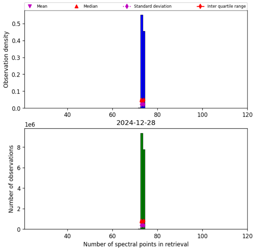
Figure 83: Histogram of “Number of spectral points in retrieval” for 2024-12-28 to 2024-12-29
