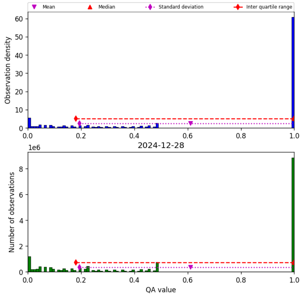
Figure 57: Histogram of “QA value” for 2024-12-28 to 2024-12-29
