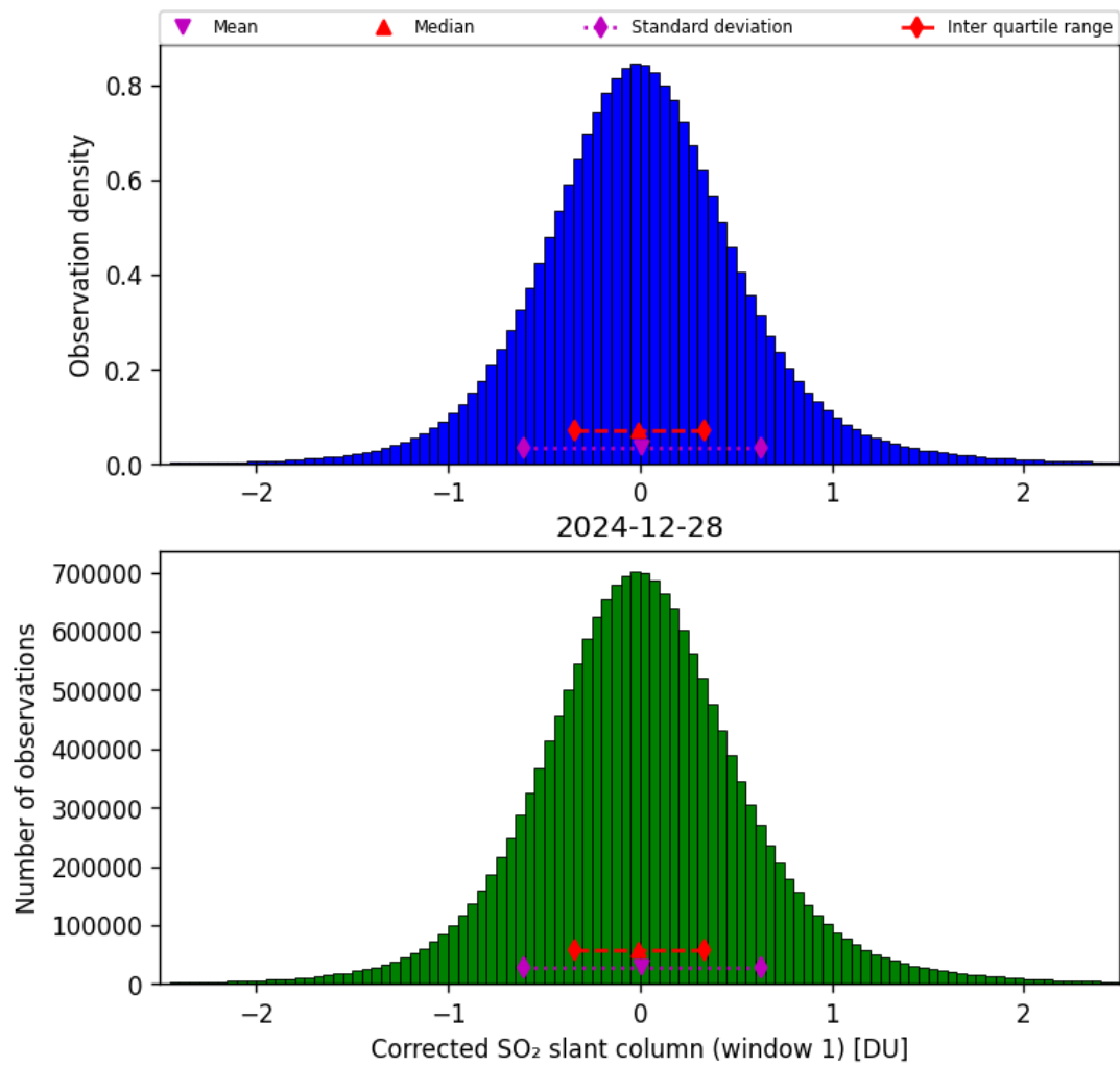
Figure 65: Histogram of “Corrected SO 2 slant column (window 1)” for 2024-12-28 to 2024-12-29
