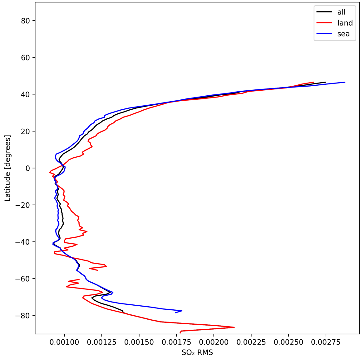
Figure 52: Zonal average of “SO 2 RMS” for 2024-12-28 to 2024-12-29.
