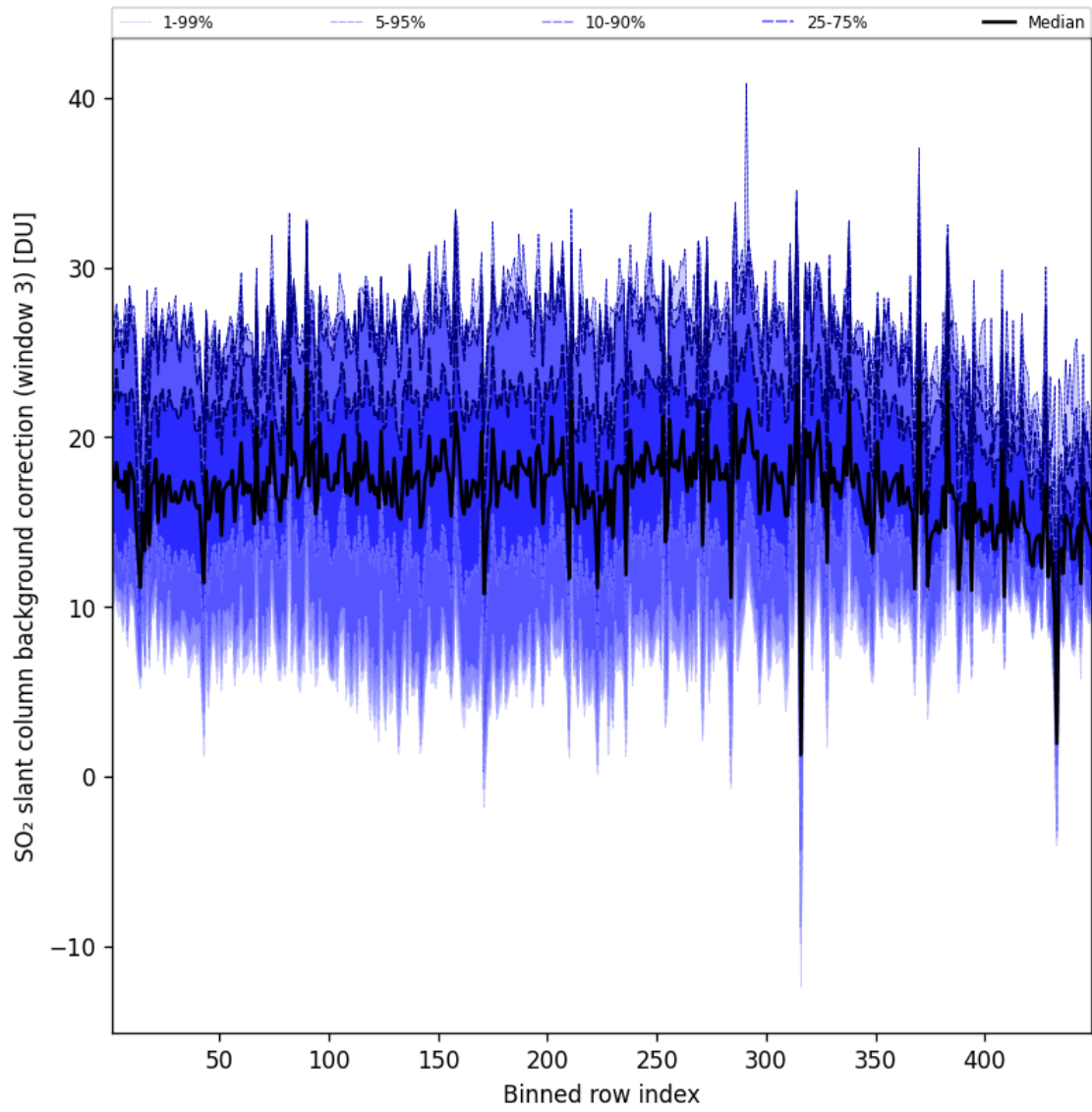
Figure 101: Along track statistics of “SO 2 slant column background correction (window 3)” for 2024-12-28 to 2024-12-29
