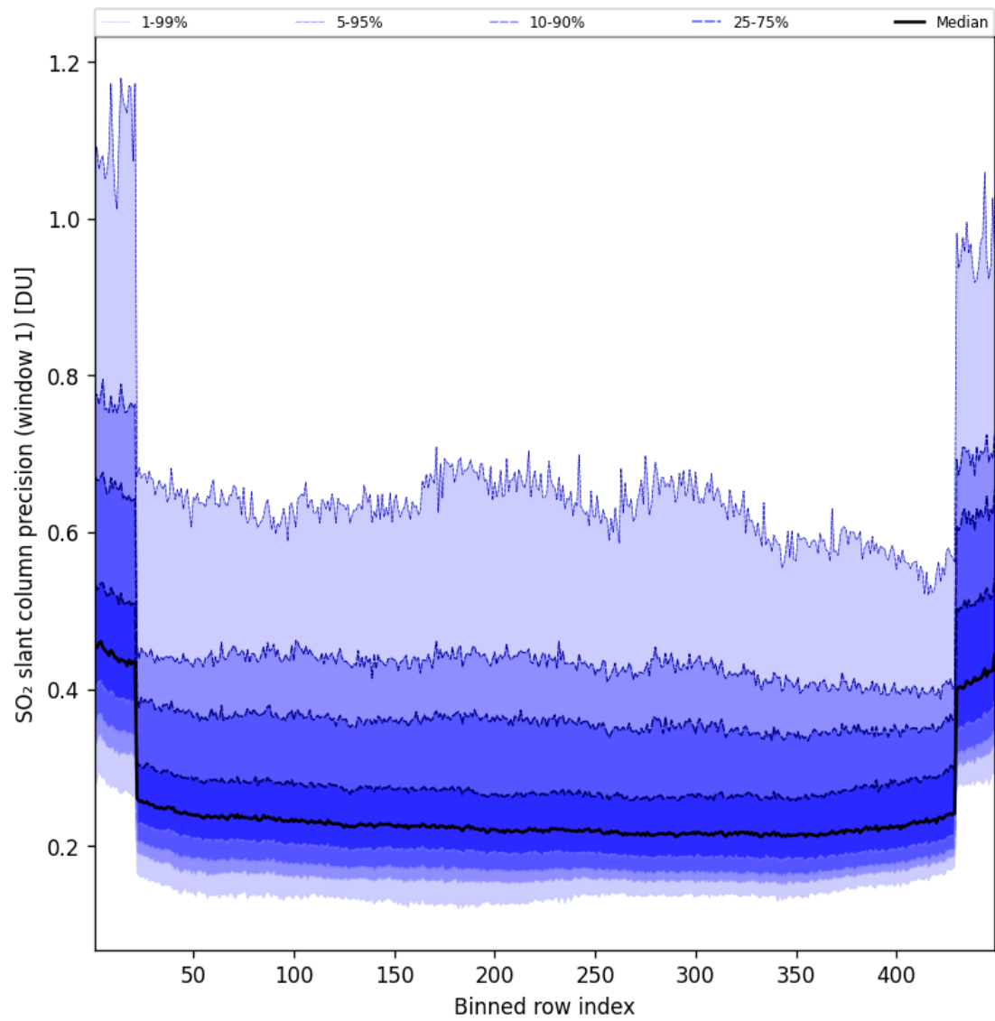
Figure 91: Along track statistics of “SO 2 slant column precision (window 1)” for 2024-12-28 to 2024-12-29
