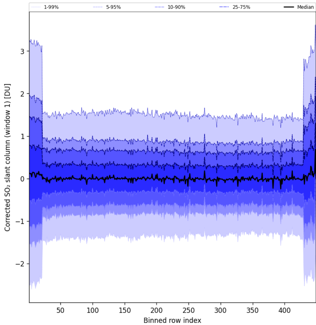
Figure 92: Along track statistics of “Corrected SO 2 slant column (window 1)” for 2024-12-28 to 2024-12-29
