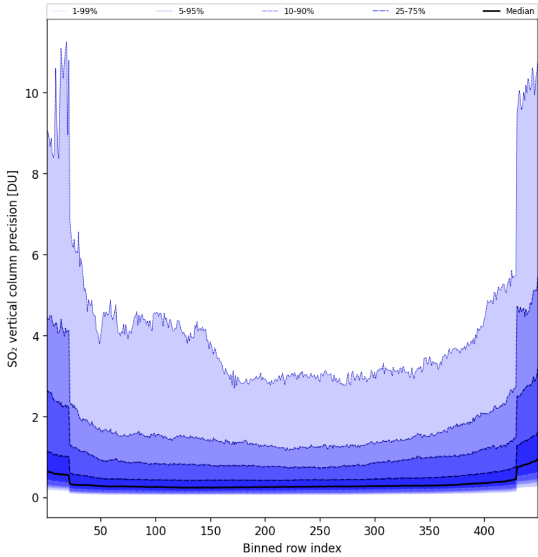
Figure 86: Along track statistics of “SO 2 vertical column precision” for 2024-12-28 to 2024-12-29
