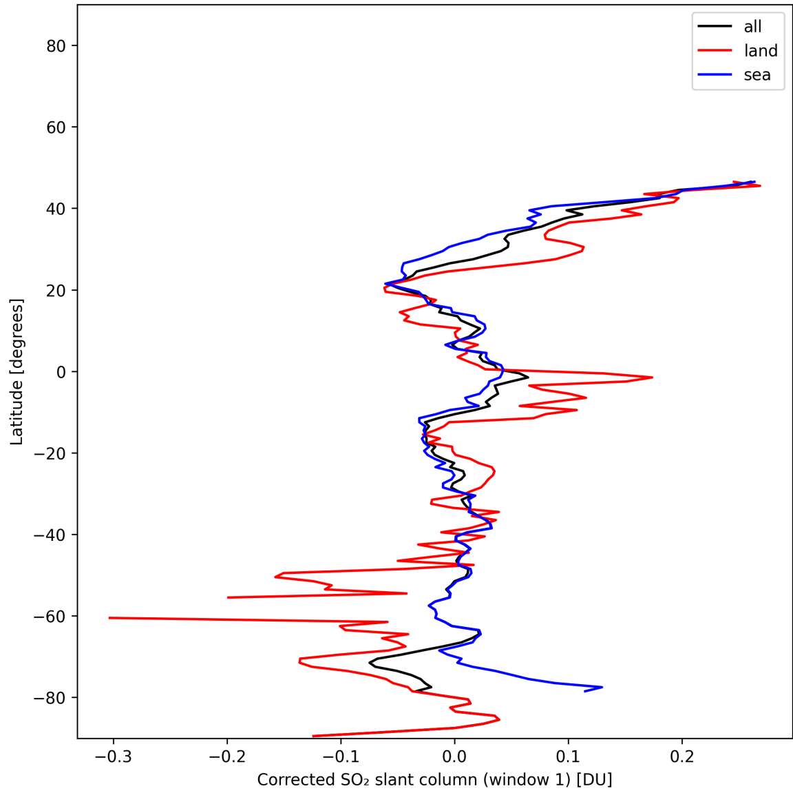
Figure 38: Zonal average of “Corrected SO 2 slant column (window 1)” for 2024-12-28 to 2024-12-29.
