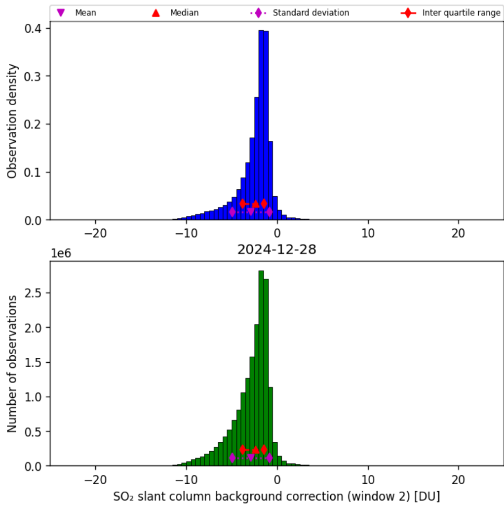
Figure 70: Histogram of “SO 2 slant column background correction (window 2)” for 2024-12-28 to 2024-12-29
