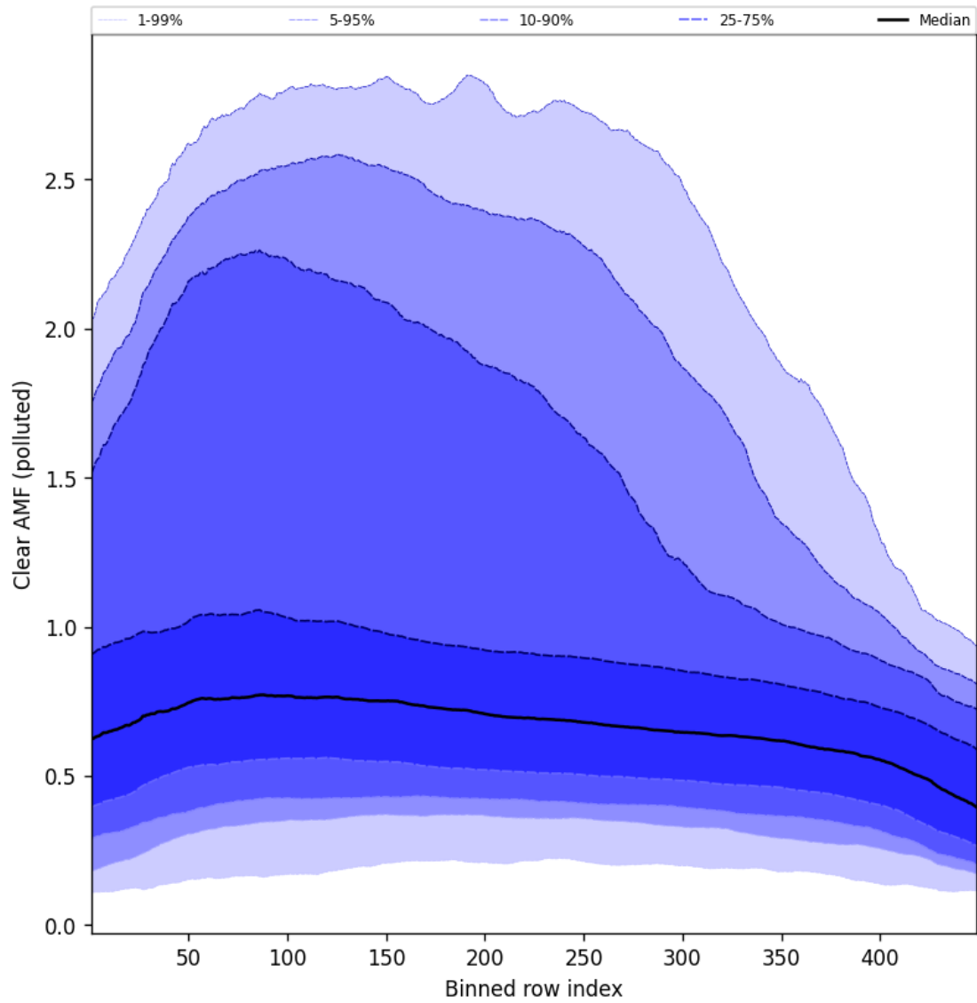
Figure 109: Along track statistics of “Clear AMF (polluted)” for 2024-12-28 to 2024-12-29
