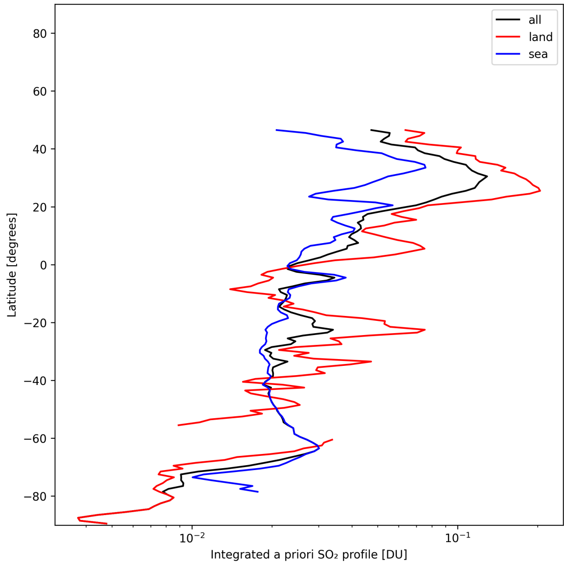
Figure 49: Zonal average of “Integrated a priori SO 2 profile” for 2024-12-28 to 2024-12-29.
