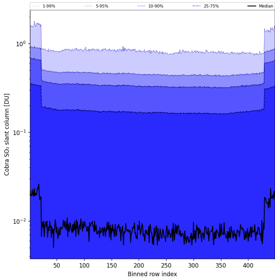
Figure 88: Along track statistics of "Cobra SO 2 slant column" for 2024-12-28 to 2024-12-29
