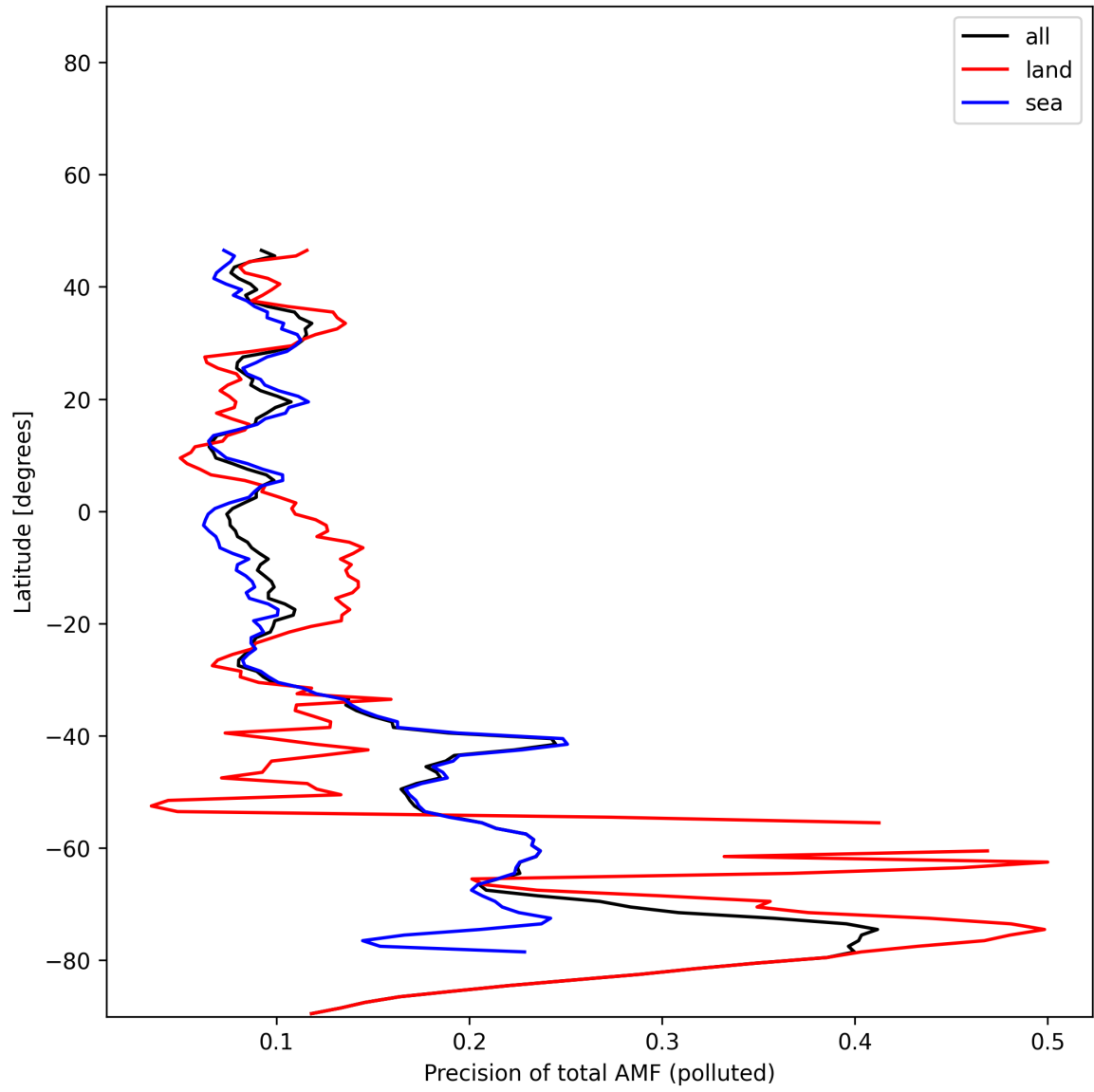
Figure 54: Zonal average of “Precision of total AMF (polluted)” for 2024-12-28 to 2024-12-29.
