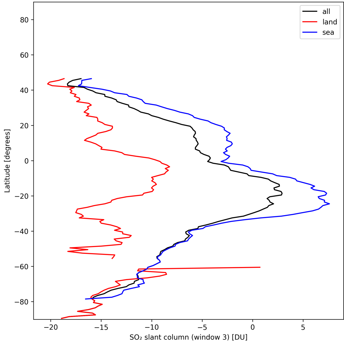
Figure 44: Zonal average of “SO 2 slant column (window 3)” for 2024-12-28 to 2024-12-29.
