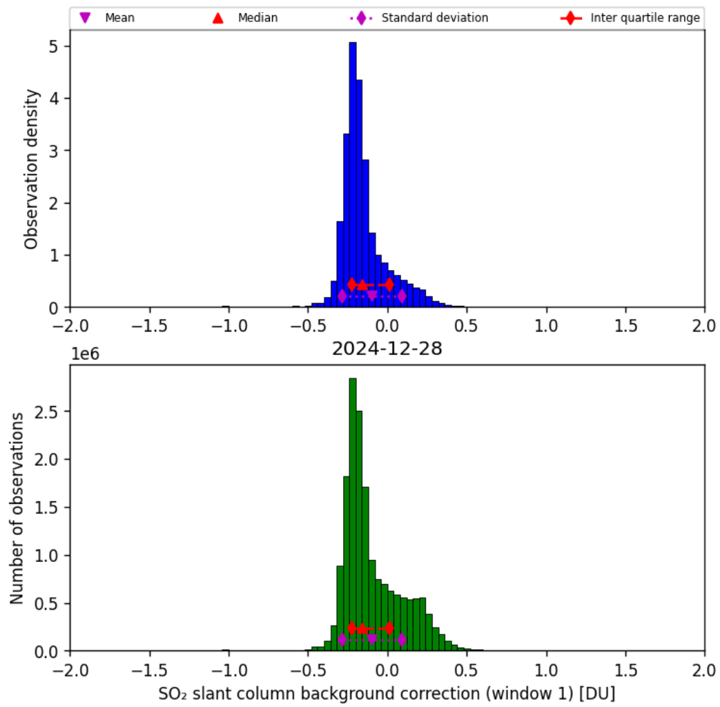
Figure 66: Histogram of “SO 2 slant column background correction (window 1)” for 2024-12-28 to 2024-12-29
