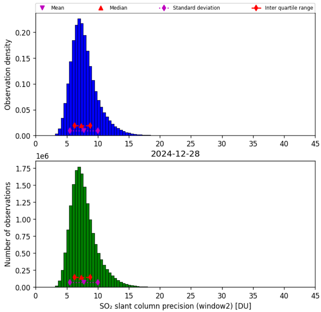
Figure 68: Histogram of “SO 2 slant column precision (window2)” for 2024-12-28 to 2024-12-29
