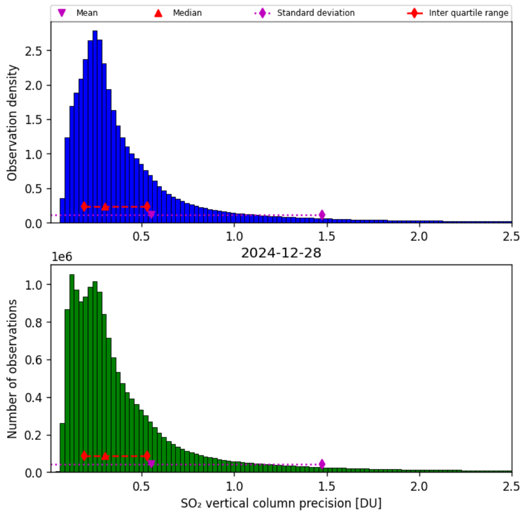
Figure 59: Histogram of “SO 2 vertical column precision” for 2024-12-28 to 2024-12-29
