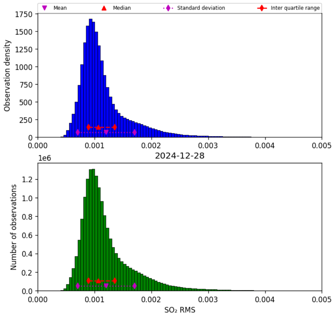
Figure 79: Histogram of “SO 2 RMS” for 2024-12-28 to 2024-12-29
