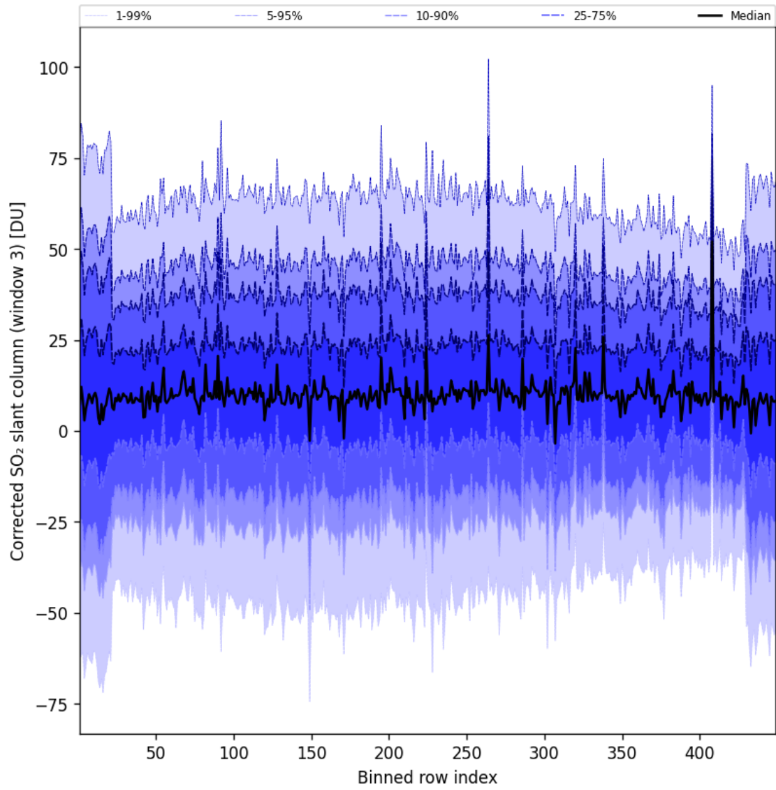
Figure 100: Along track statistics of “Corrected SO 2 slant column (window 3)” for 2024-12-28 to 2024-12-29
