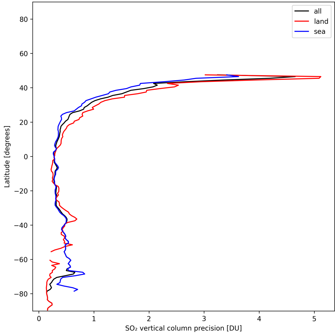
Figure 32: Zonal average of “SO 2 vertical column precision” for 2025-01-02 to 2025-01-03.
