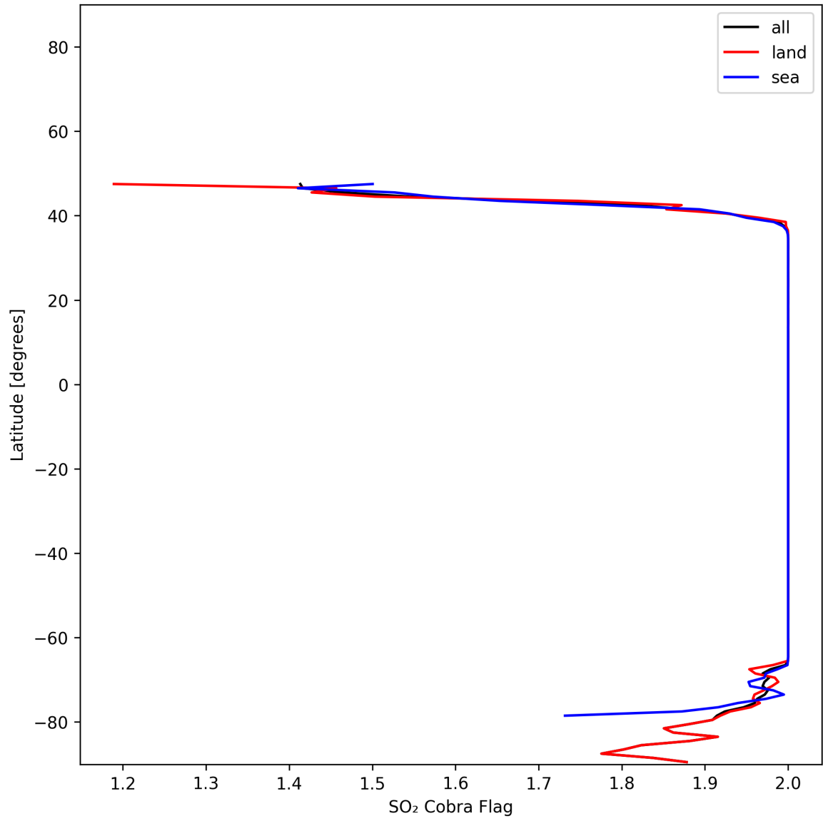
Figure 48: Zonal average of “SO 2 Cobra Flag” for 2025-01-02 to 2025-01-03.
