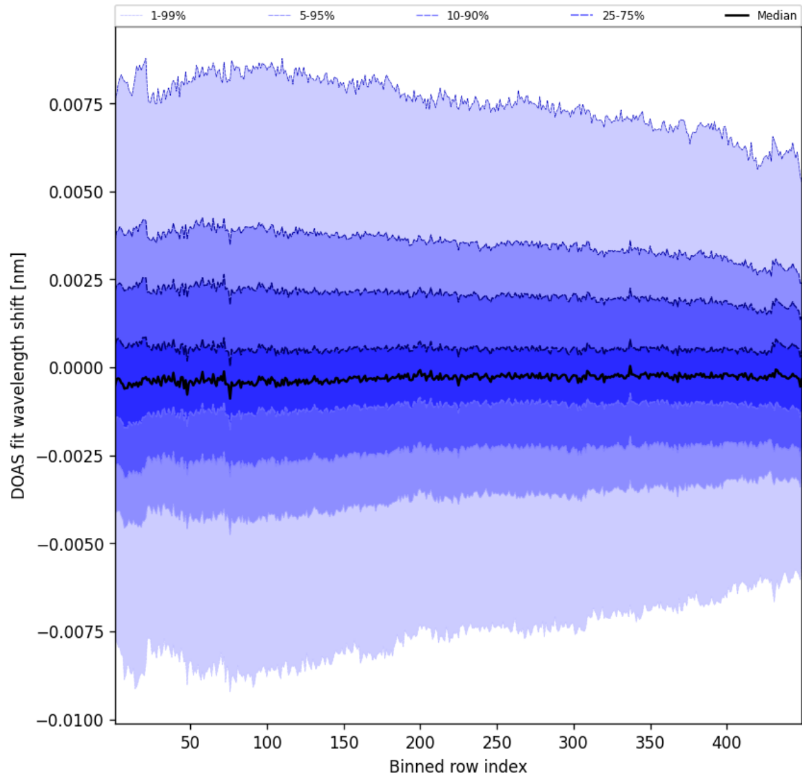
Figure 104: Along track statistics of “DOAS fit wavelength shift” for 2025-01-02 to 2025-01-03
