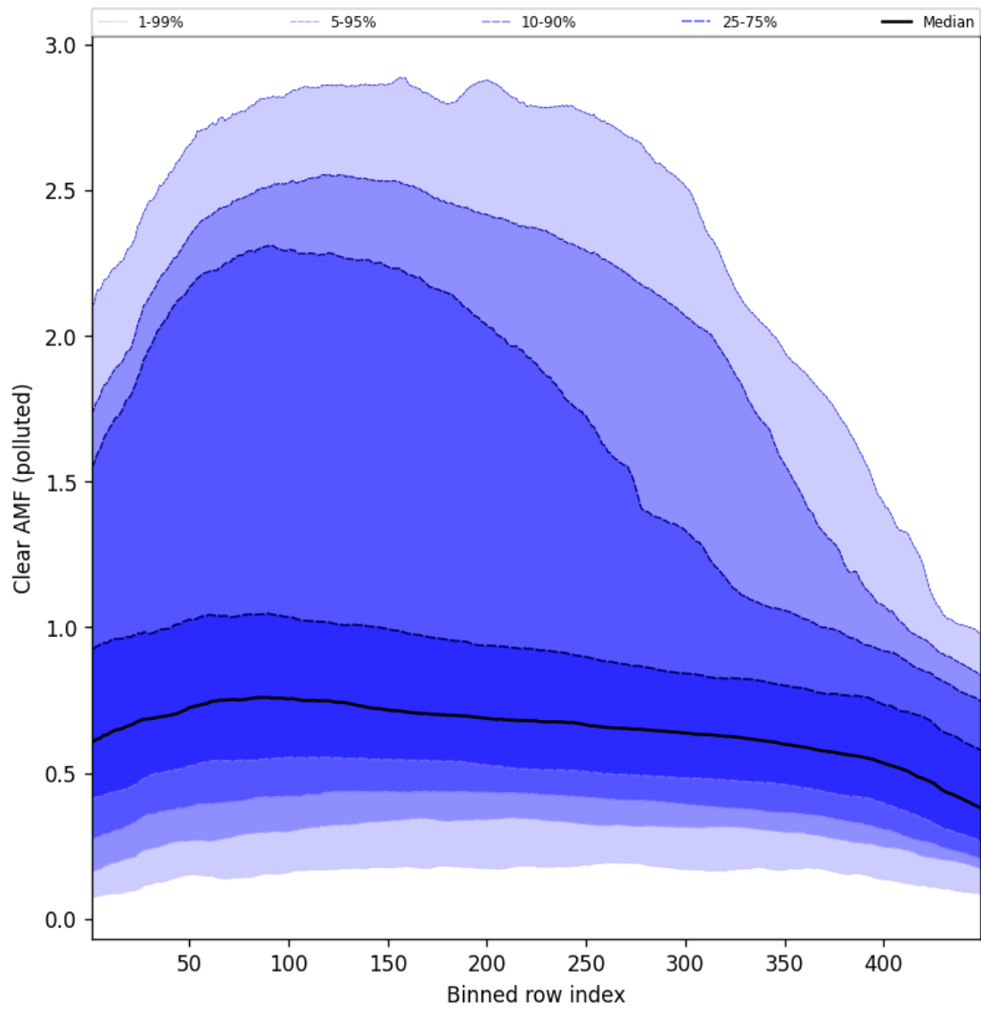
Figure 109: Along track statistics of “Clear AMF (polluted)” for 2025-01-02 to 2025-01-03
