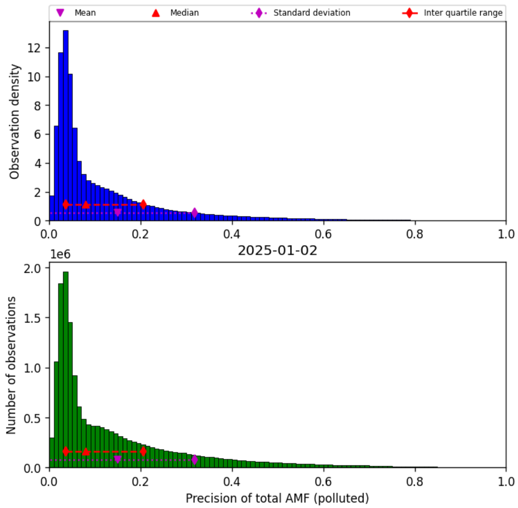
Figure 81: Histogram of “Precision of total AMF (polluted)” for 2025-01-02 to 2025-01-03
