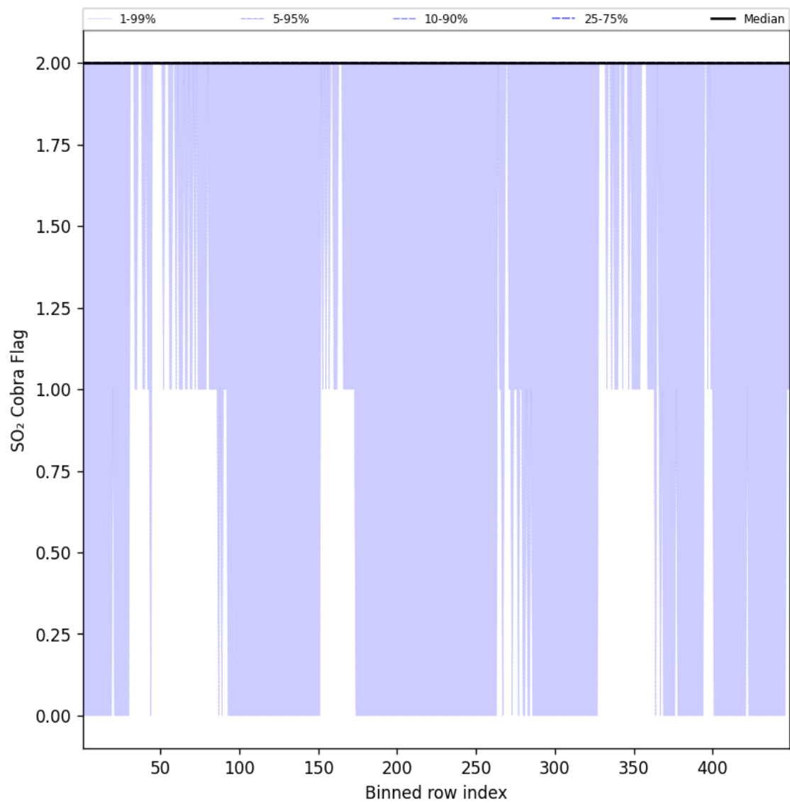
Figure 102: Along track statistics of “SO 2 Cobra Flag” for 2025-01-02 to 2025-01-03
