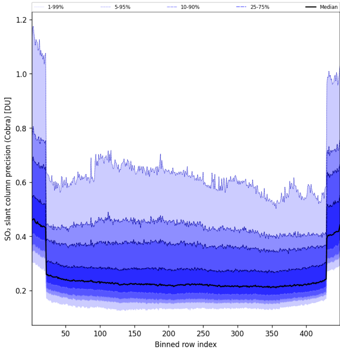
Figure 89: Along track statistics of “SO 2 slant column precision (Cobra)” for 2025-01-02 to 2025-01-03
