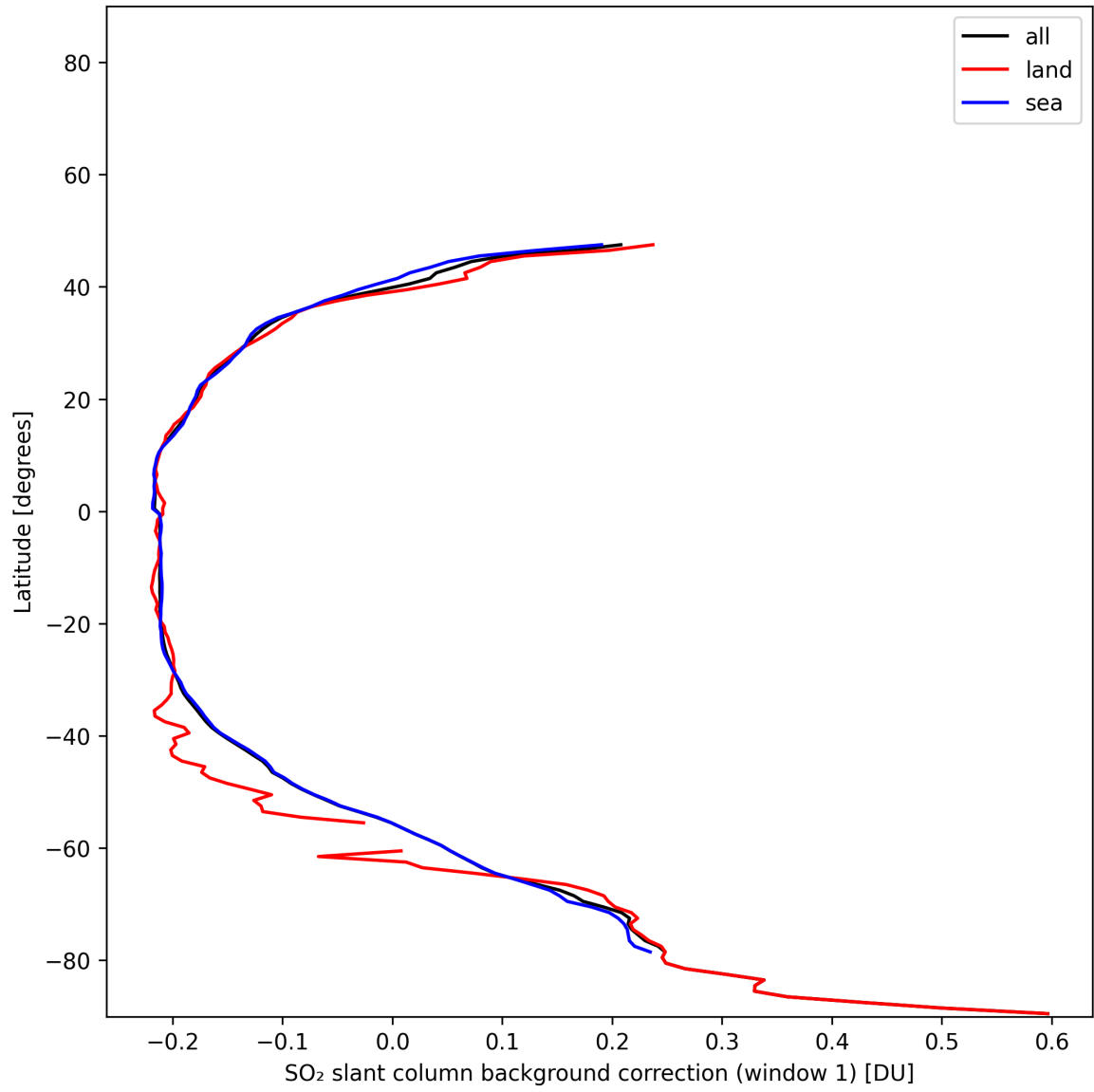
Figure 39: Zonal average of “SO 2 slant column background correction (window 1)” for 2025-01-02 to 2025-01-03.
