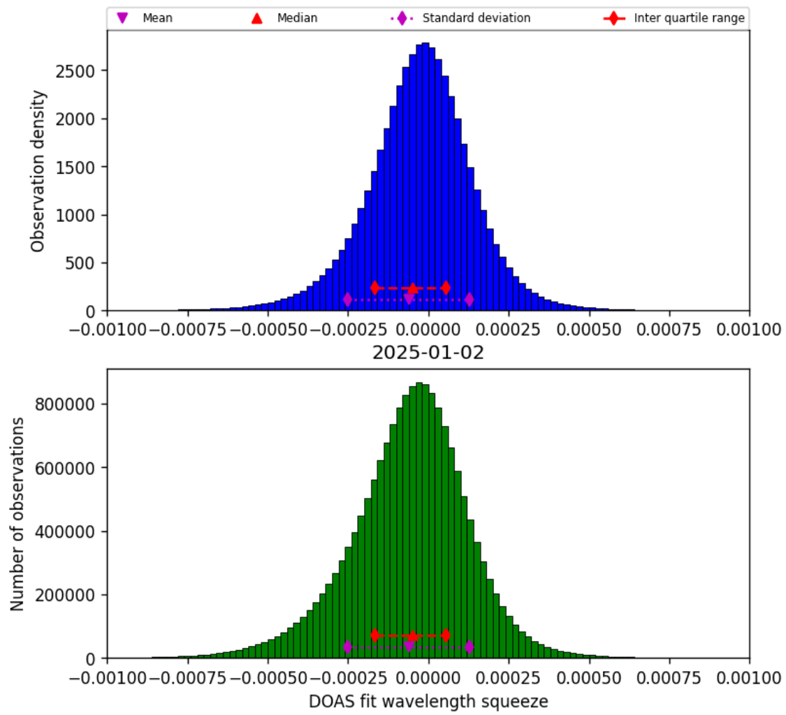
Figure 78: Histogram of “DOAS fit wavelength squeeze” for 2025-01-02 to 2025-01-03
