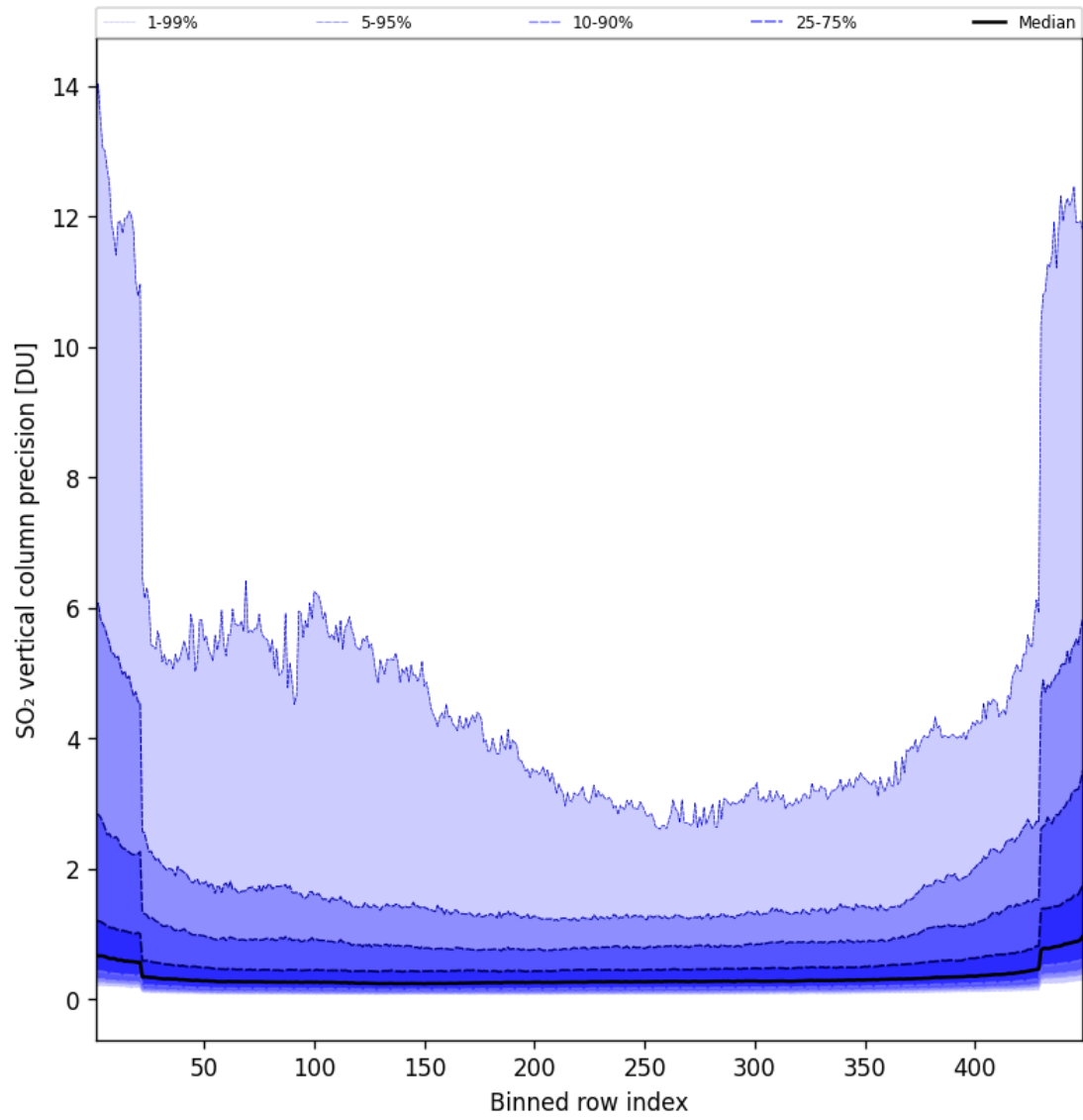
Figure 86: Along track statistics of “SO 2 vertical column precision” for 2025-01-02 to 2025-01-03
