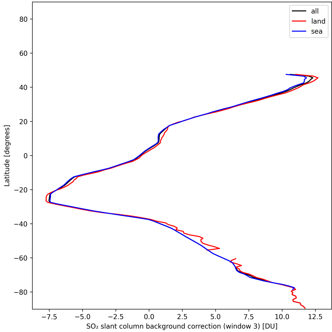
Figure 47: Zonal average of “SO 2 slant column background correction (window 3)” for 2025-01-02 to 2025-01-03.
