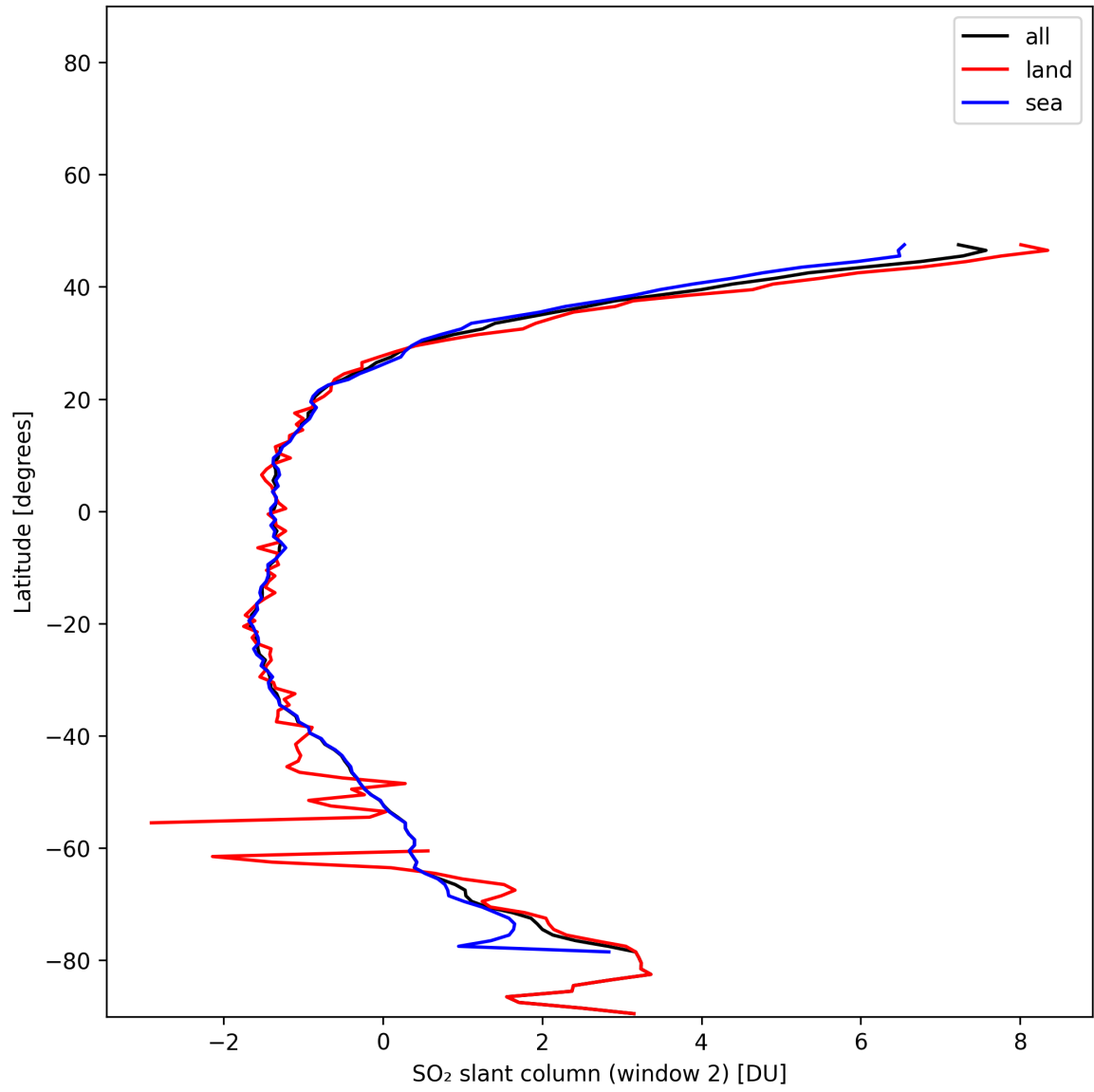
Figure 40: Zonal average of “SO 2 slant column (window 2)” for 2025-01-02 to 2025-01-03.
