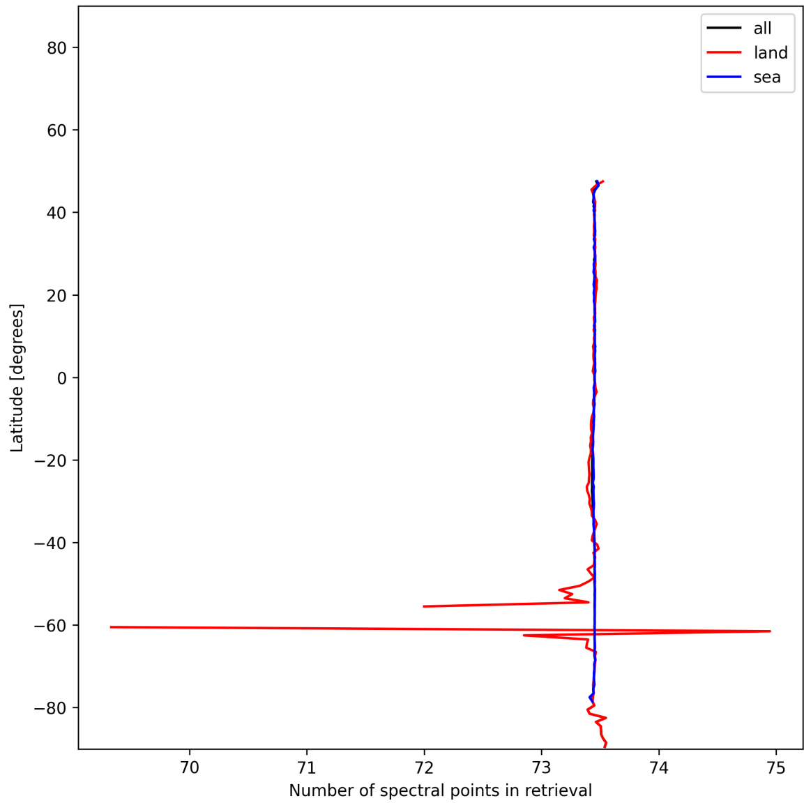
Figure 56: Zonal average of “Number of spectral points in retrieval” for 2025-01-02 to 2025-01-03.
