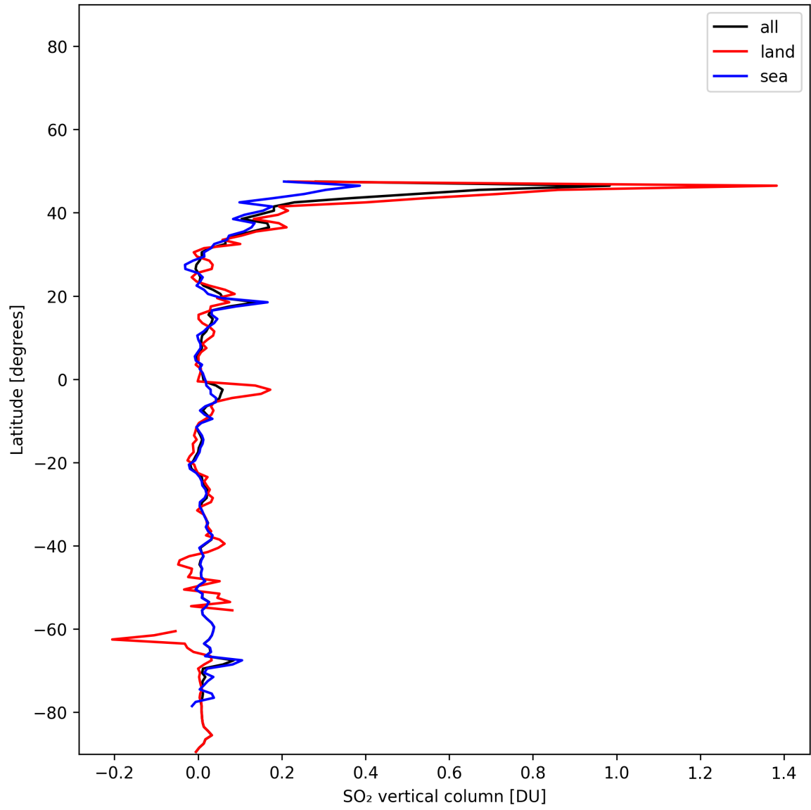
Figure 31: Zonal average of “SO 2 vertical column” for 2025-01-02 to 2025-01-03.
