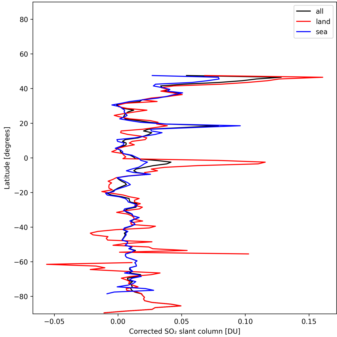
Figure 33: Zonal average of “Corrected SO 2 slant column” for 2025-01-02 to 2025-01-03.
