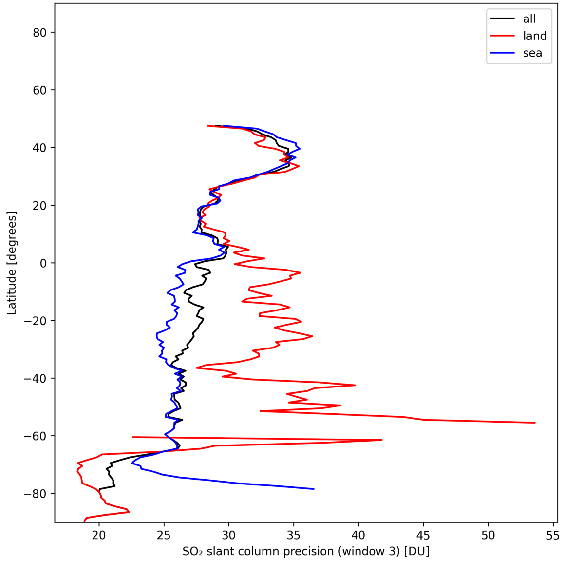
Figure 45: Zonal average of “SO 2 slant column precision (window 3)” for 2025-01-02 to 2025-01-03.
