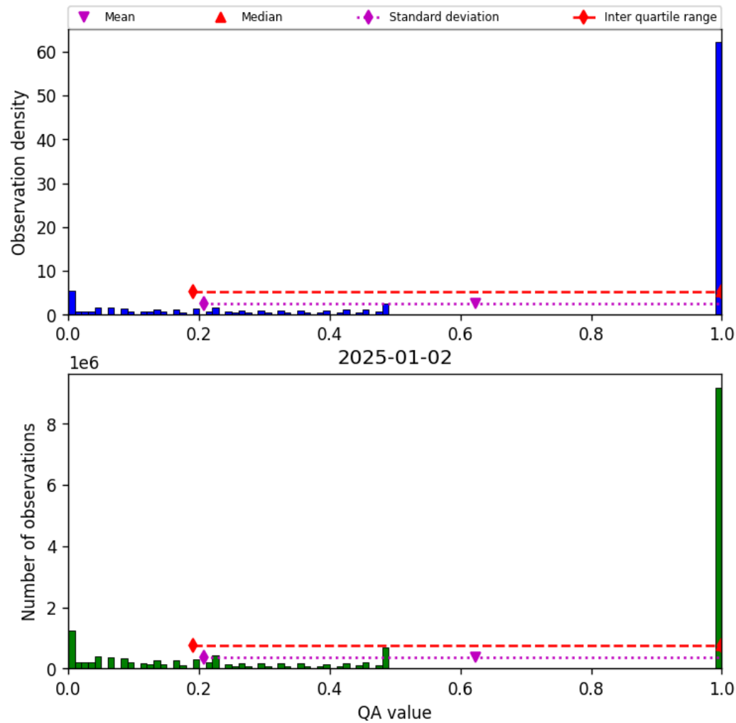
Figure 57: Histogram of “QA value” for 2025-01-02 to 2025-01-03
