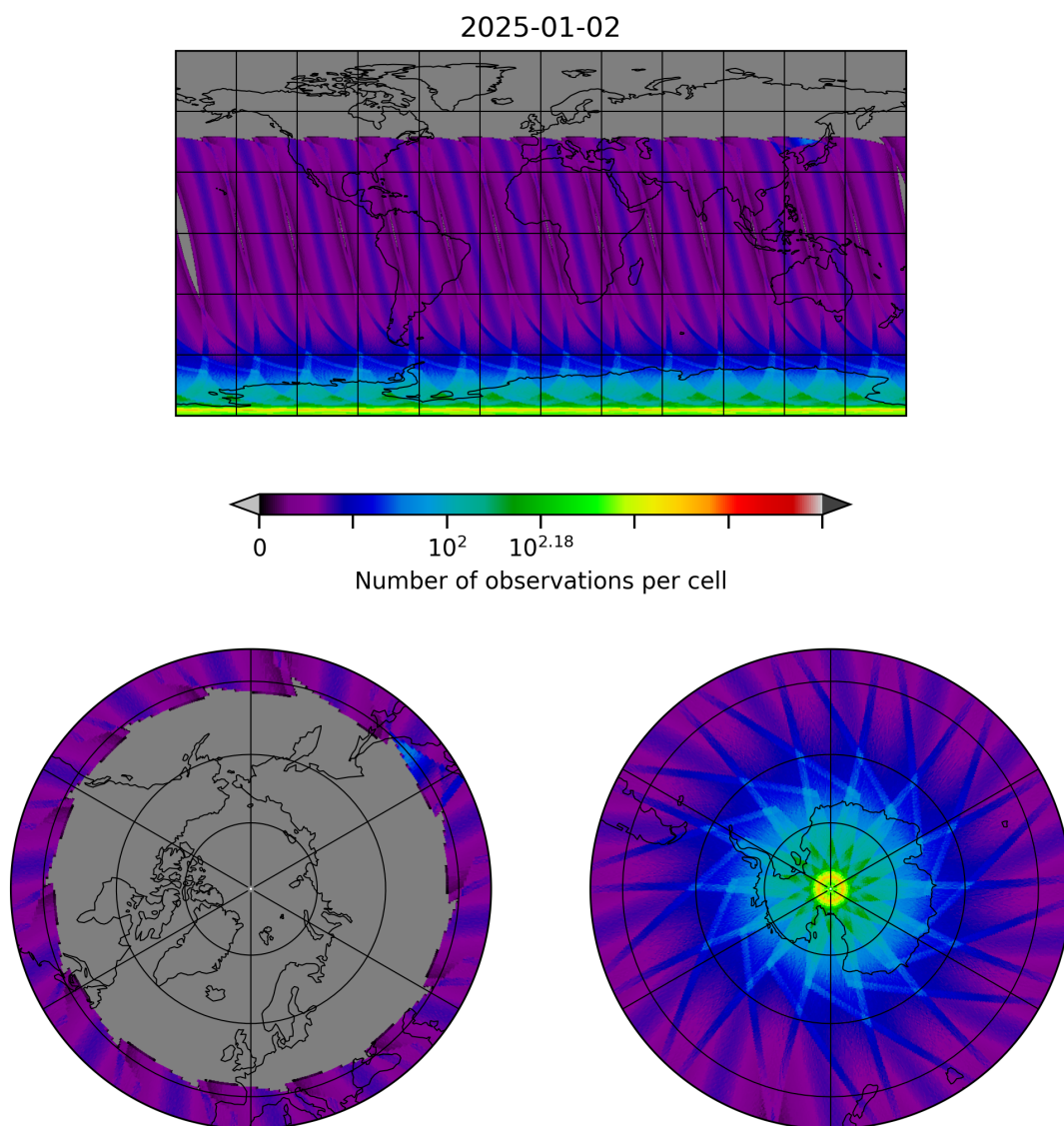
Figure 29: Map of the number of observations for 2025-01-02 to 2025-01-03
