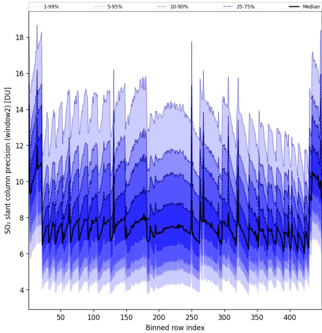
Figure 95: Along track statistics of “SO 2 slant column precision (window2)” for 2025-01-02 to 2025-01-03
