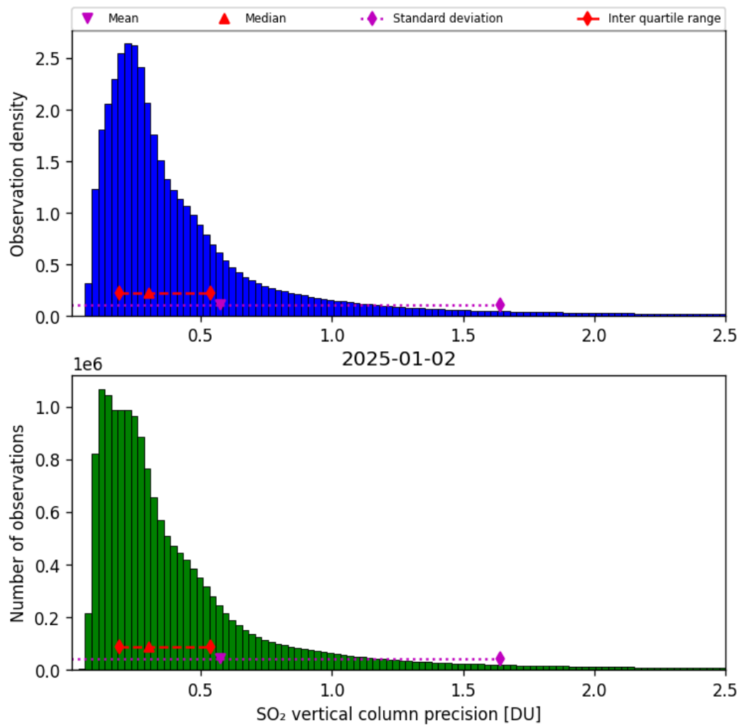
Figure 59: Histogram of “SO 2 vertical column precision” for 2025-01-02 to 2025-01-03
