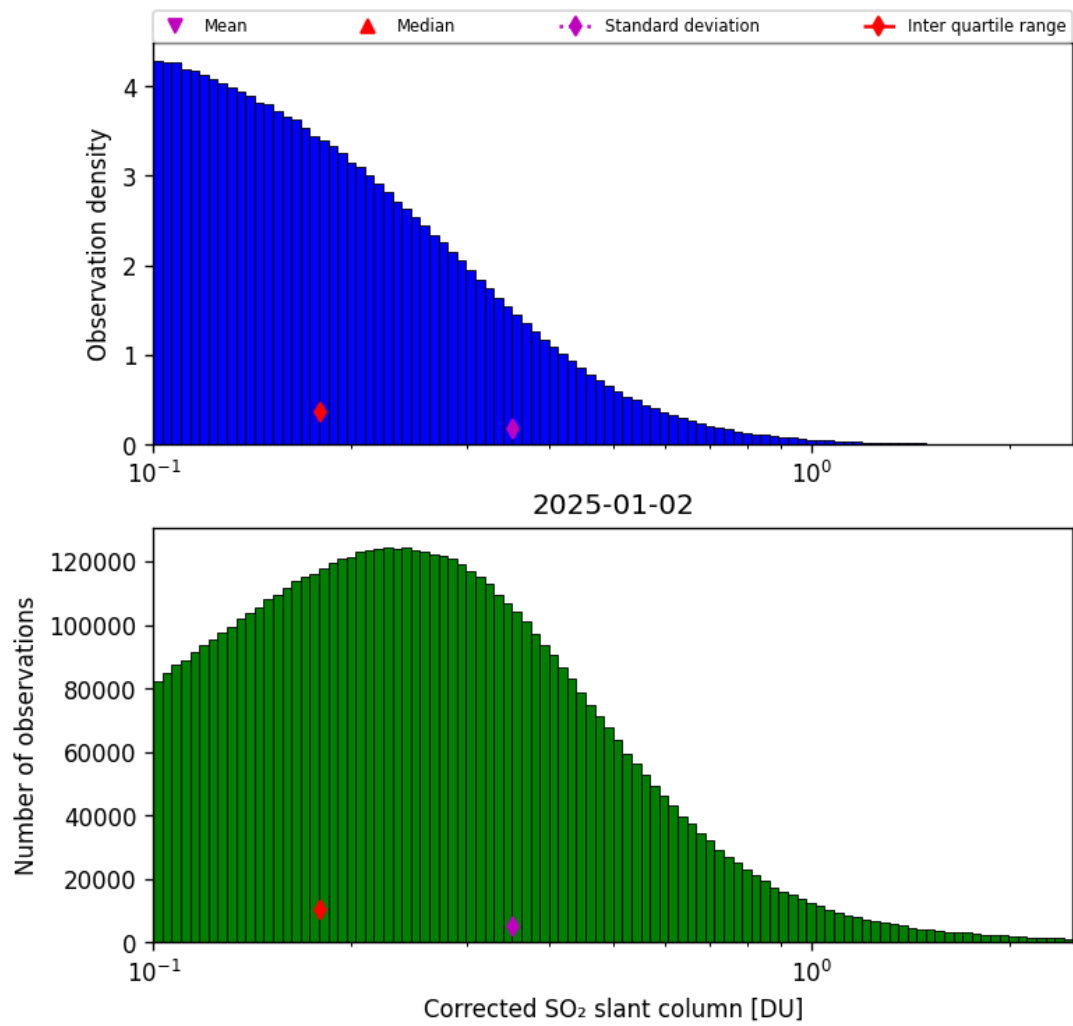
Figure 60: Histogram of “Corrected SO 2 slant column” for 2025-01-02 to 2025-01-03
