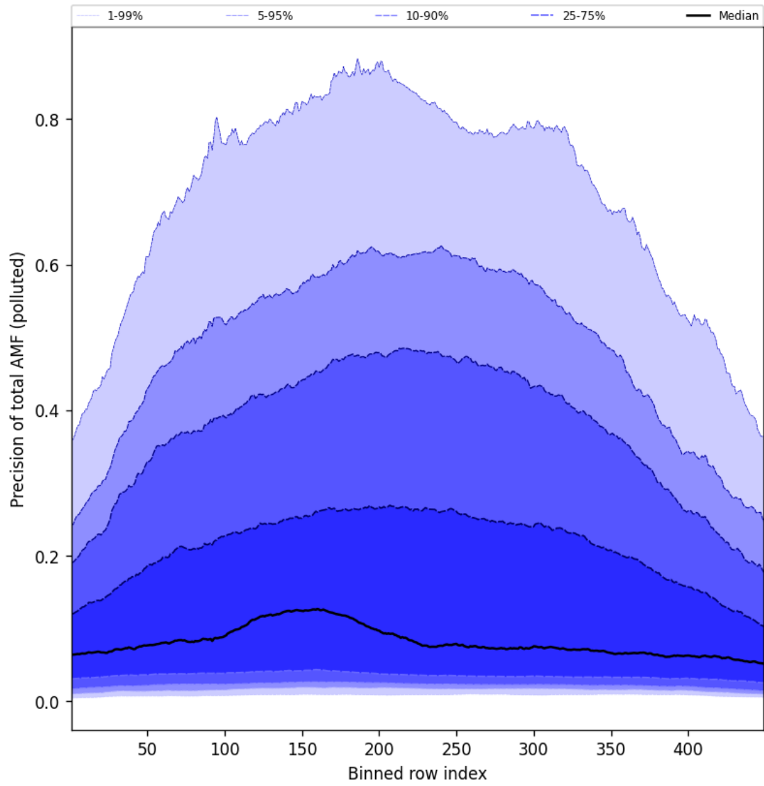
Figure 108: Along track statistics of “Precision of total AMF (polluted)” for 2025-01-02 to 2025-01-03
