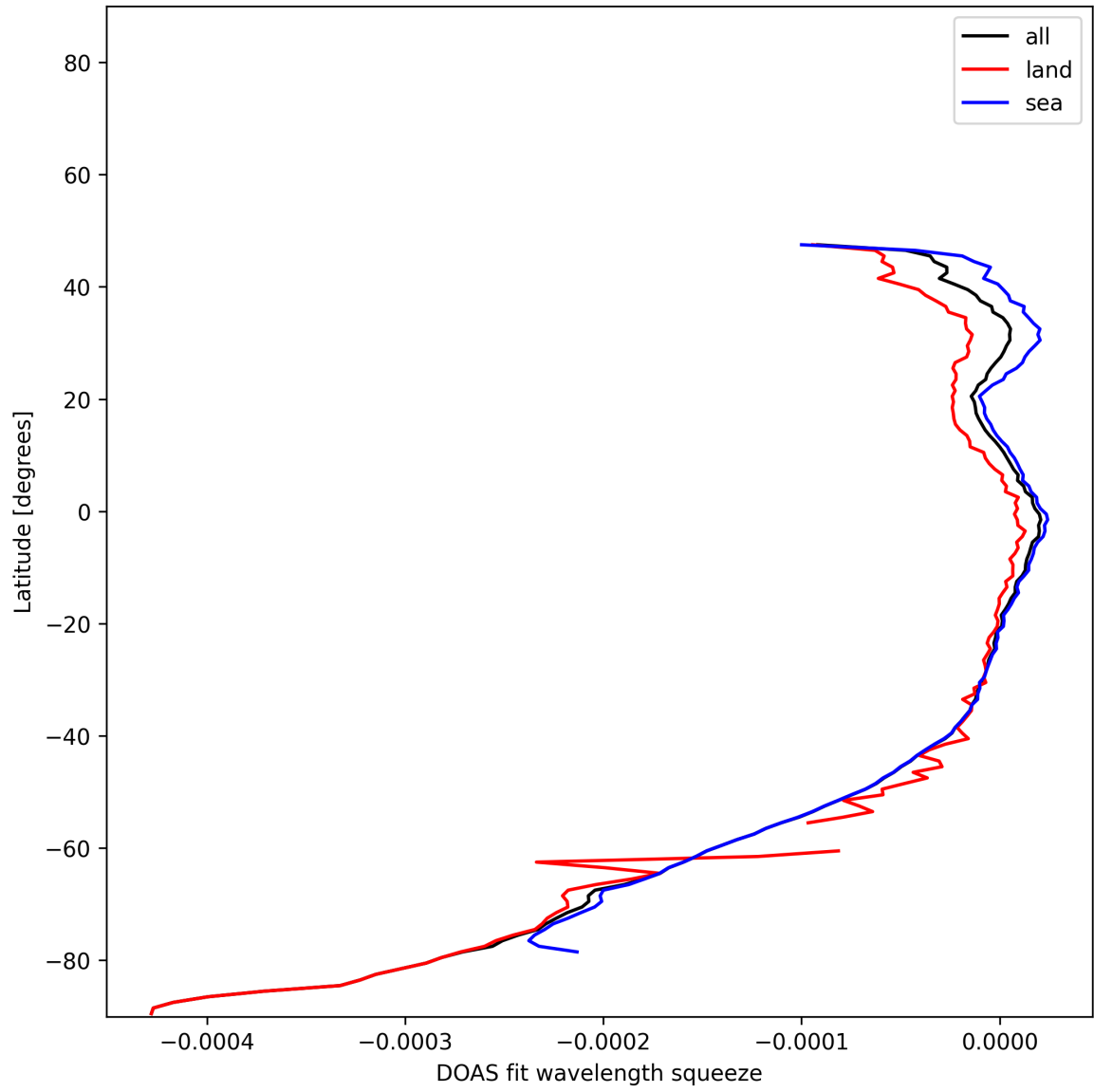
Figure 51: Zonal average of “DOAS fit wavelength squeeze” for 2025-01-02 to 2025-01-03.
