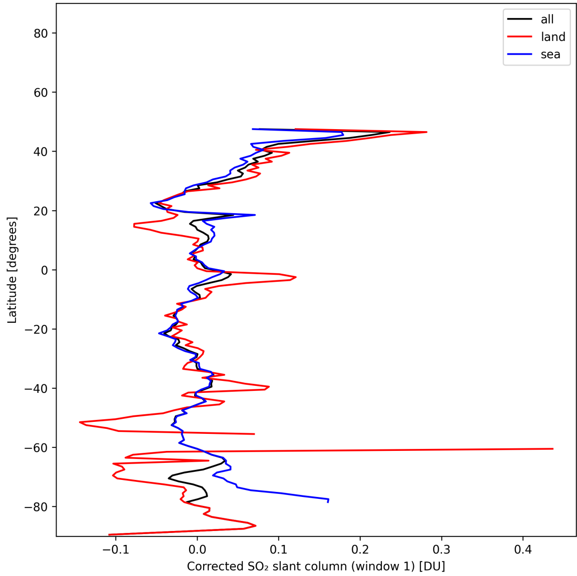
Figure 38: Zonal average of “Corrected SO 2 slant column (window 1)” for 2025-01-02 to 2025-01-03.
