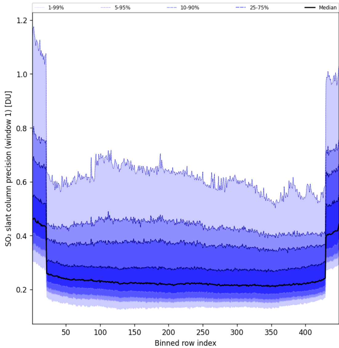
Figure 91: Along track statistics of “SO 2 slant column precision (window 1)” for 2025-01-02 to 2025-01-03
