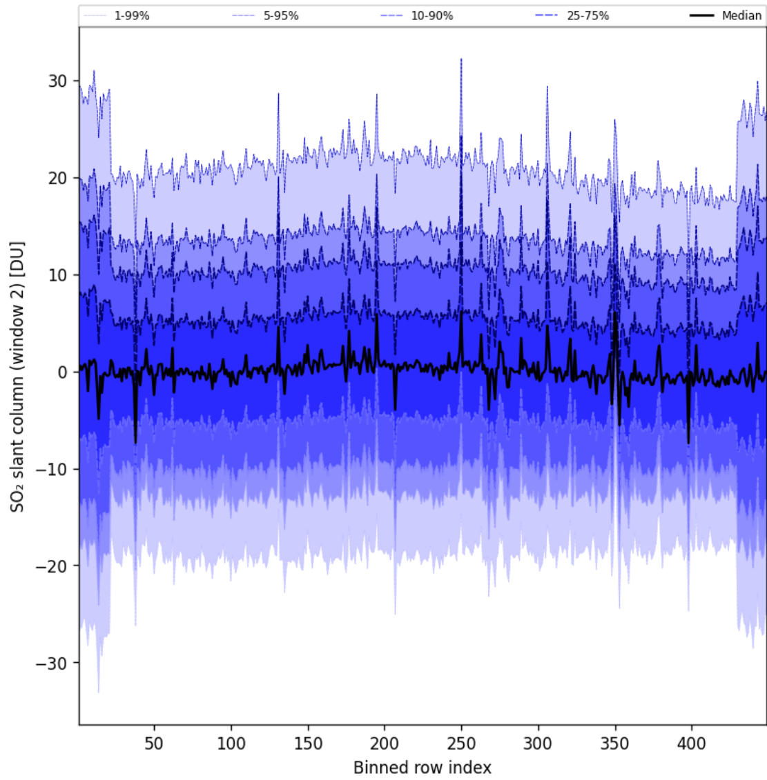
Figure 94: Along track statistics of “SO 2 slant column (window 2)” for 2025-01-02 to 2025-01-03
