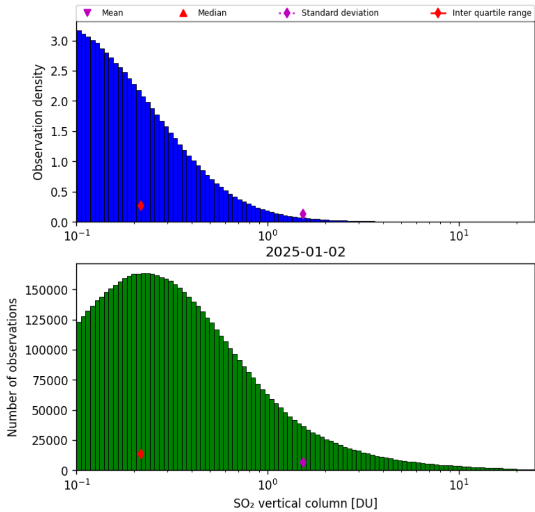
Figure 58: Histogram of “SO 2 vertical column” for 2025-01-02 to 2025-01-03
