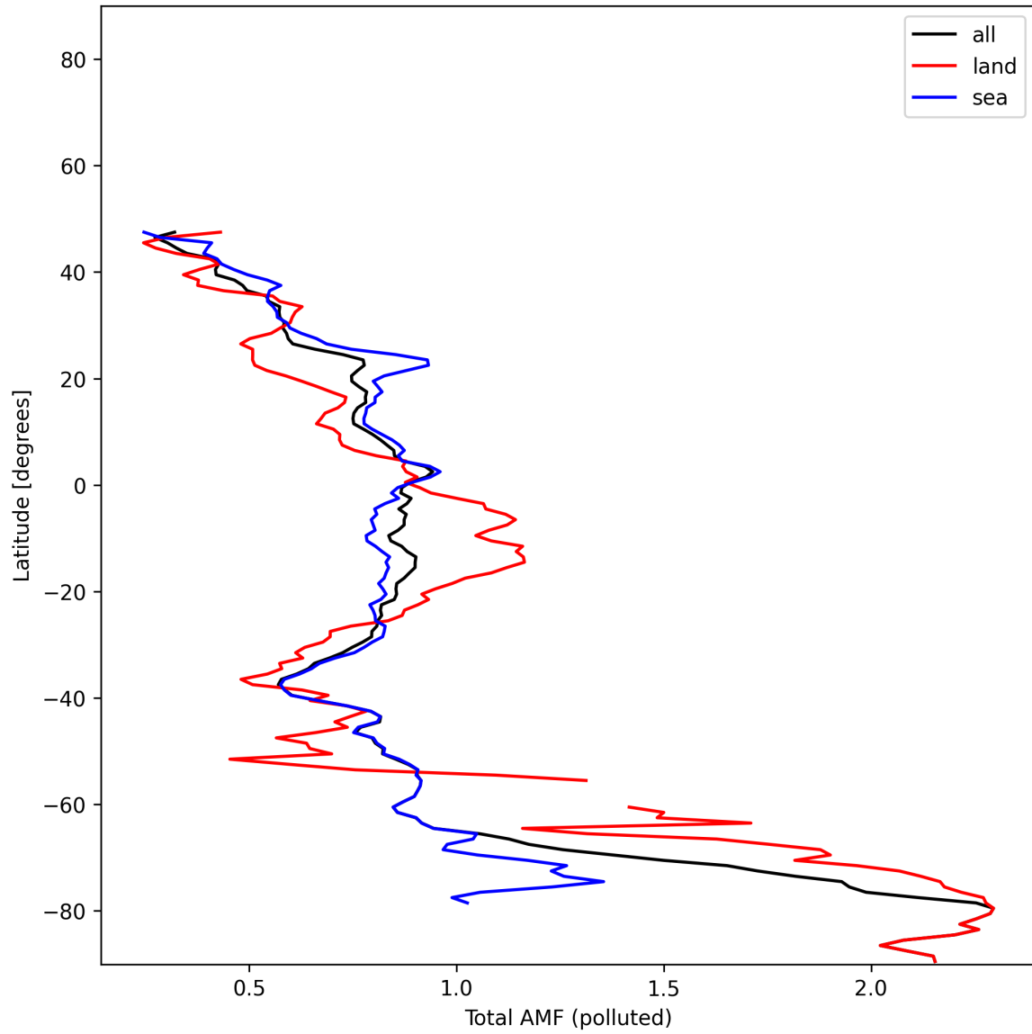
Figure 53: Zonal average of “Total AMF (polluted)” for 2025-01-02 to 2025-01-03.
