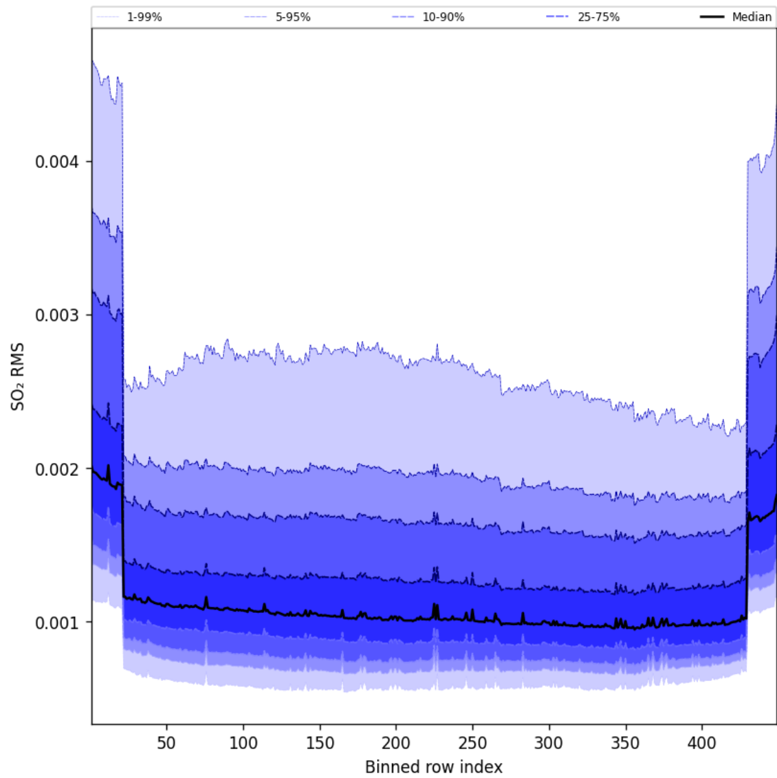
Figure 106: Along track statistics of “SO 2 RMS” for 2025-01-02 to 2025-01-03
