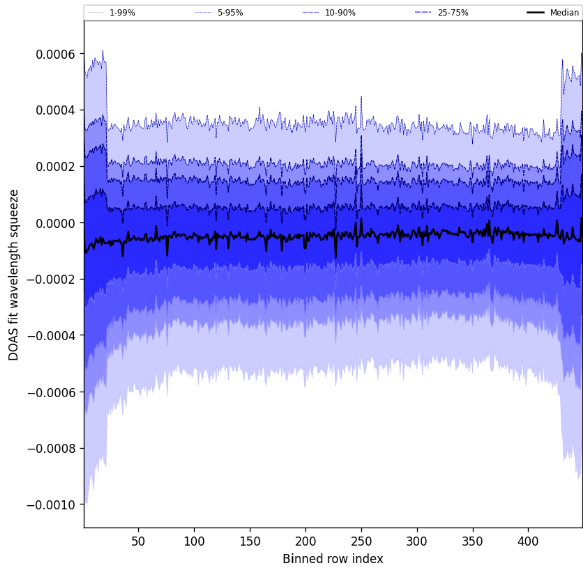
Figure 105: Along track statistics of “DOAS fit wavelength squeeze” for 2025-01-02 to 2025-01-03
