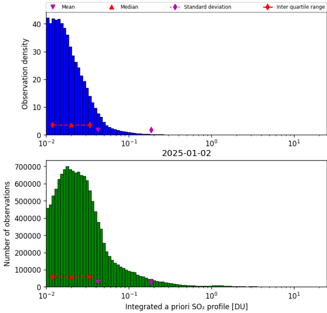
Figure 76: Histogram of “Integrated a priori SO 2 profile” for 2025-01-02 to 2025-01-03
