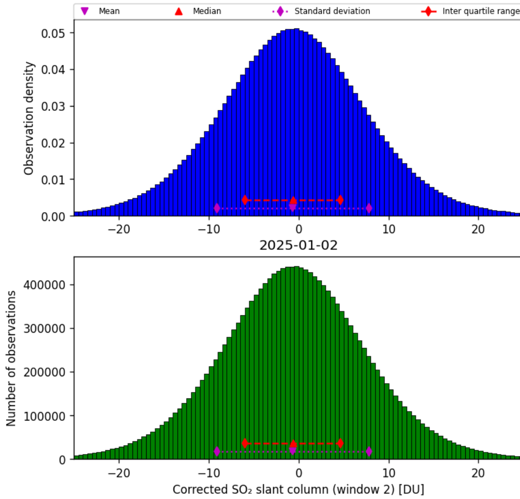
Figure 69: Histogram of “Corrected SO 2 slant column (window 2)” for 2025-01-02 to 2025-01-03
