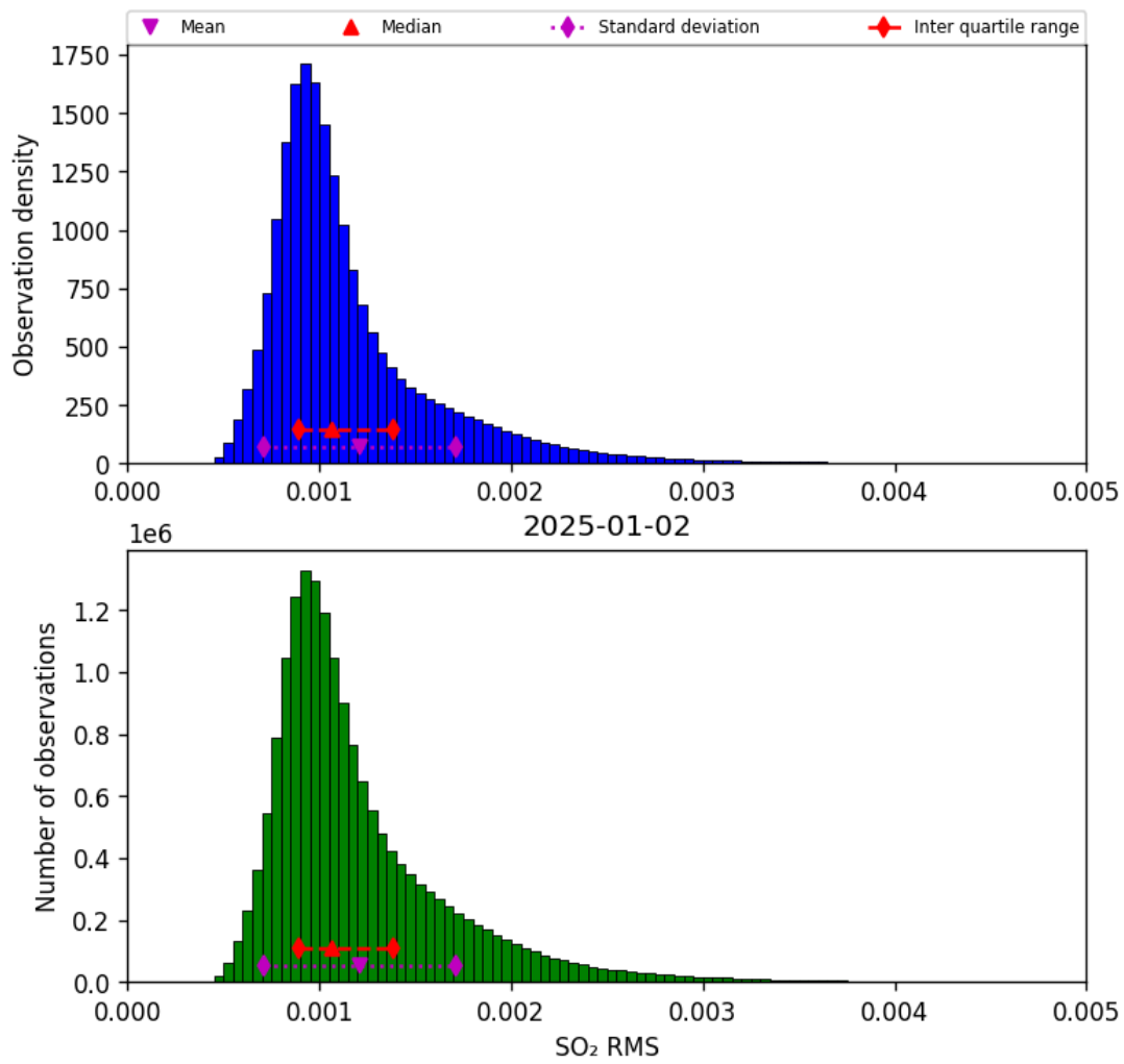
Figure 79: Histogram of “SO 2 RMS” for 2025-01-02 to 2025-01-03
