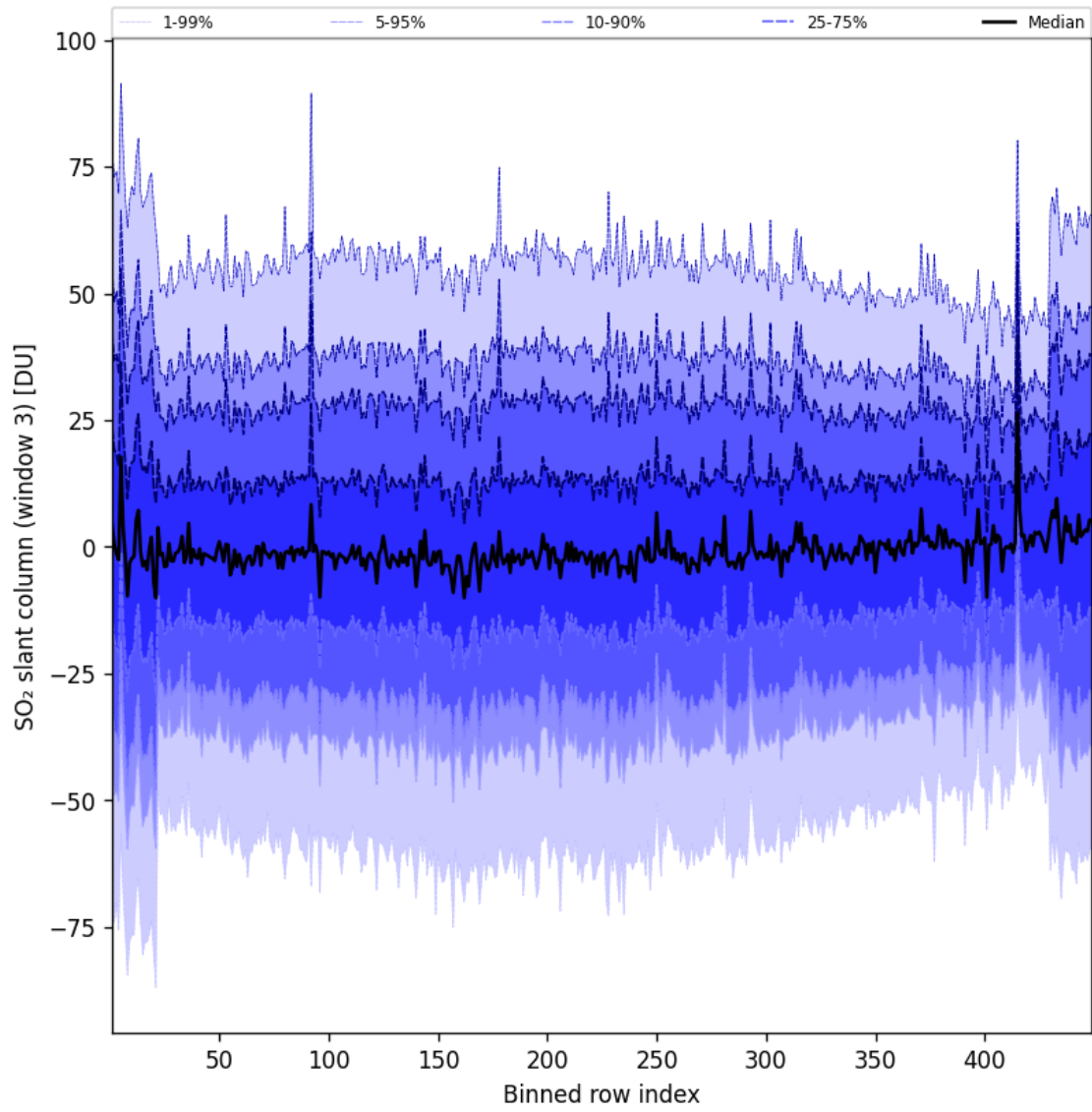
Figure 98: Along track statistics of “SO 2 slant column (window 3)” for 2025-01-02 to 2025-01-03
