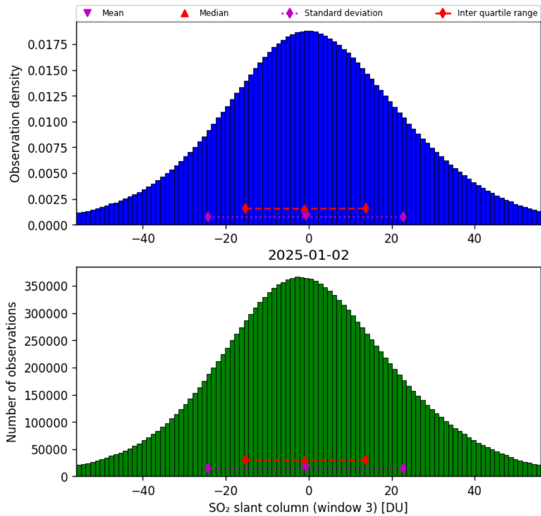
Figure 71: Histogram of “SO 2 slant column (window 3)” for 2025-01-02 to 2025-01-03
