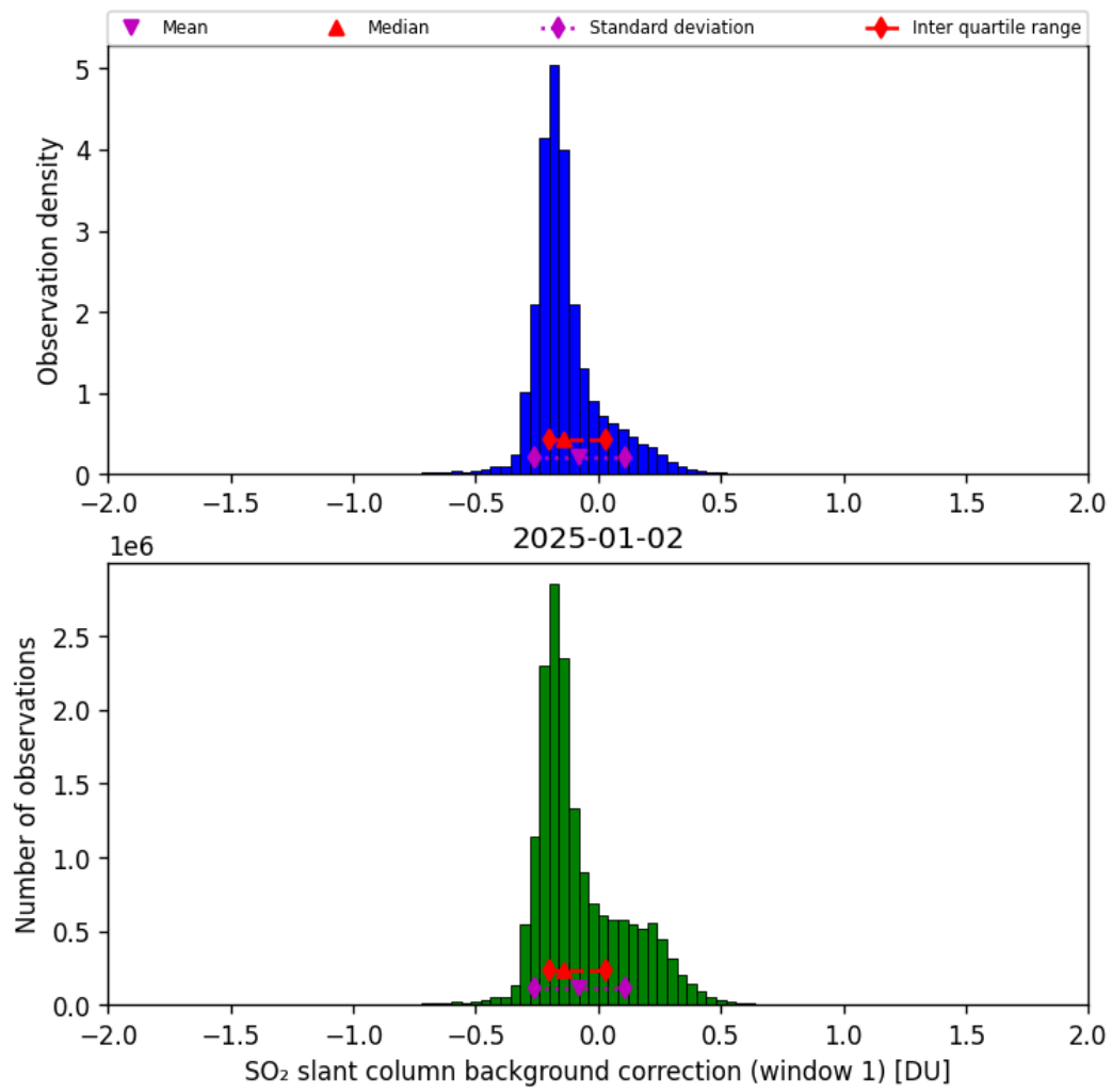
Figure 66: Histogram of “SO 2 slant column background correction (window 1)” for 2025-01-02 to 2025-01-03
