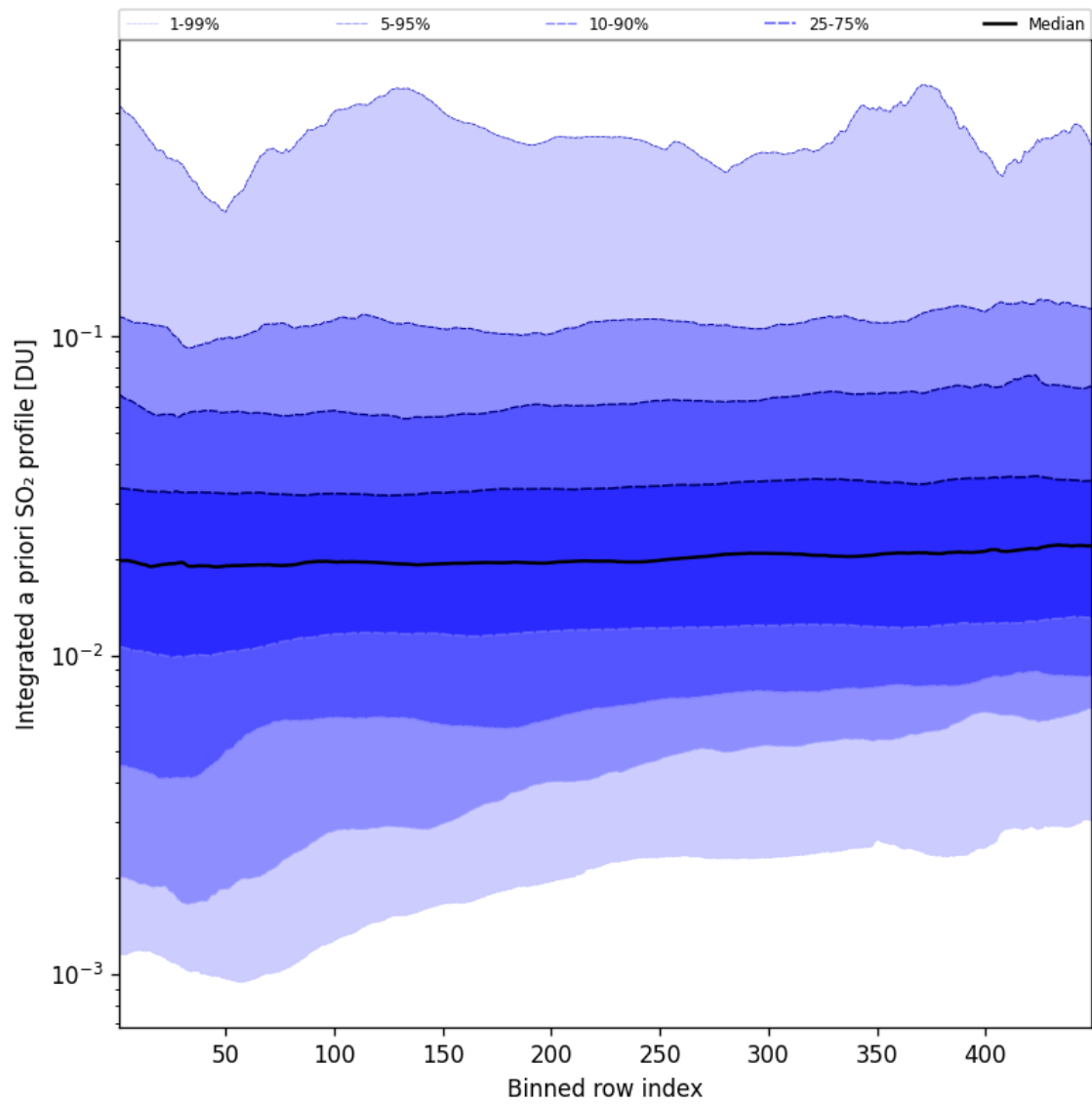
Figure 103: Along track statistics of “Integrated a priori SO 2 profile” for 2025-01-02 to 2025-01-03
