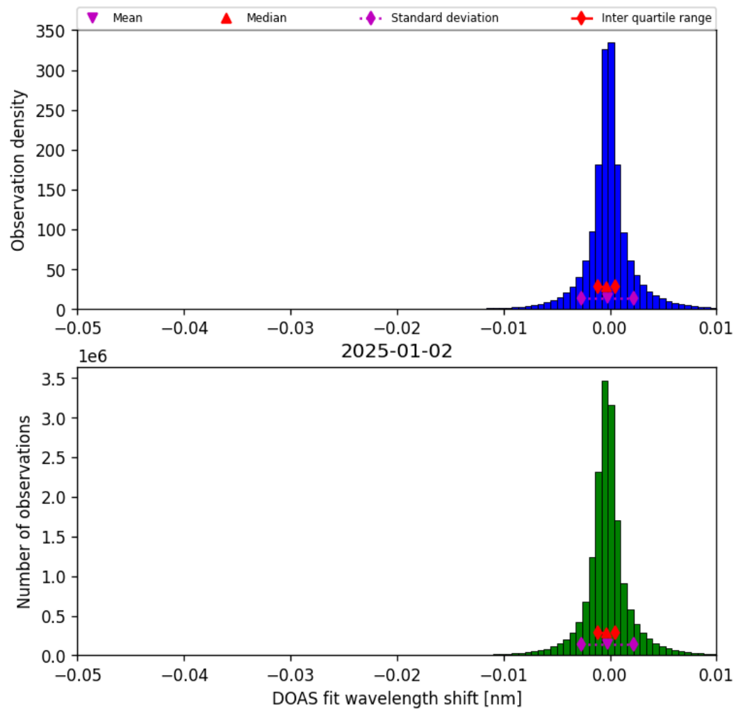
Figure 77: Histogram of “DOAS fit wavelength shift” for 2025-01-02 to 2025-01-03
