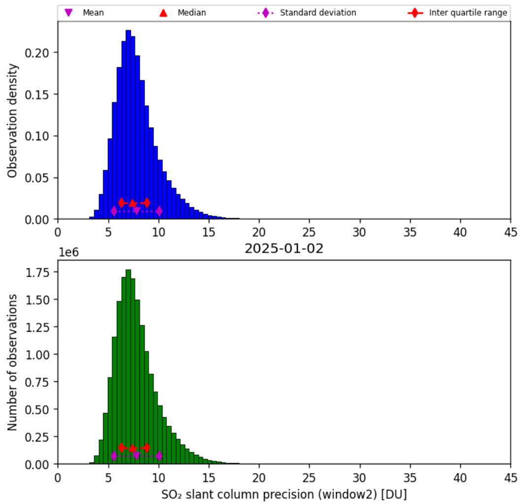
Figure 68: Histogram of “SO 2 slant column precision (window2)” for 2025-01-02 to 2025-01-03
