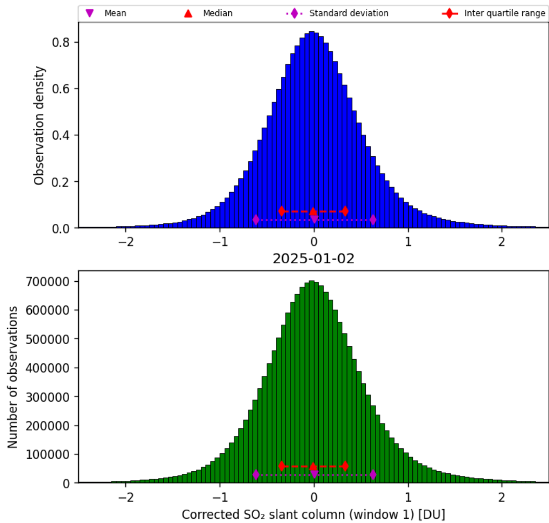
Figure 65: Histogram of “Corrected SO 2 slant column (window 1)” for 2025-01-02 to 2025-01-03
