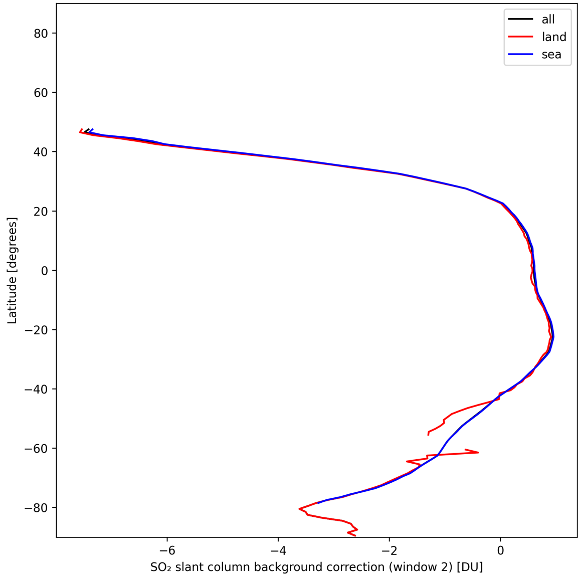
Figure 43: Zonal average of “SO 2 slant column background correction (window 2)” for 2025-01-02 to 2025-01-03.
