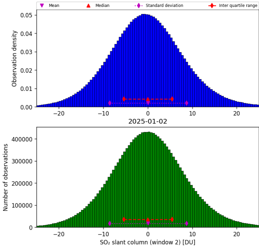
Figure 67: Histogram of “SO 2 slant column (window 2)” for 2025-01-02 to 2025-01-03
