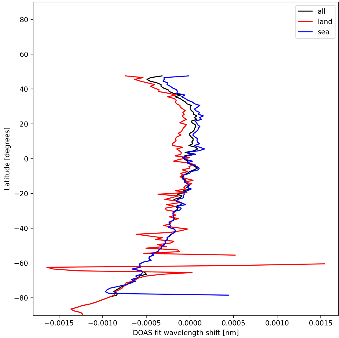
Figure 50: Zonal average of “DOAS fit wavelength shift” for 2025-01-02 to 2025-01-03.
