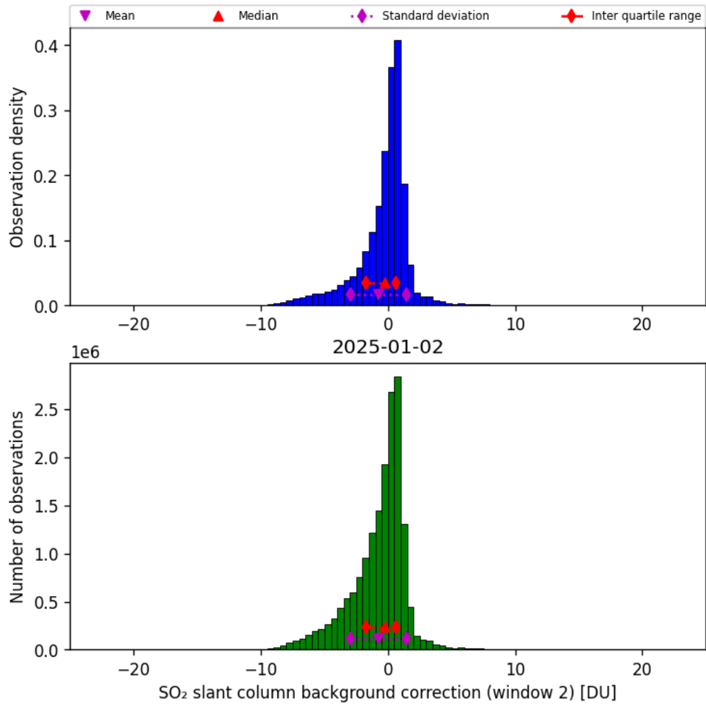
Figure 70: Histogram of “SO 2 slant column background correction (window 2)” for 2025-01-02 to 2025-01-03
