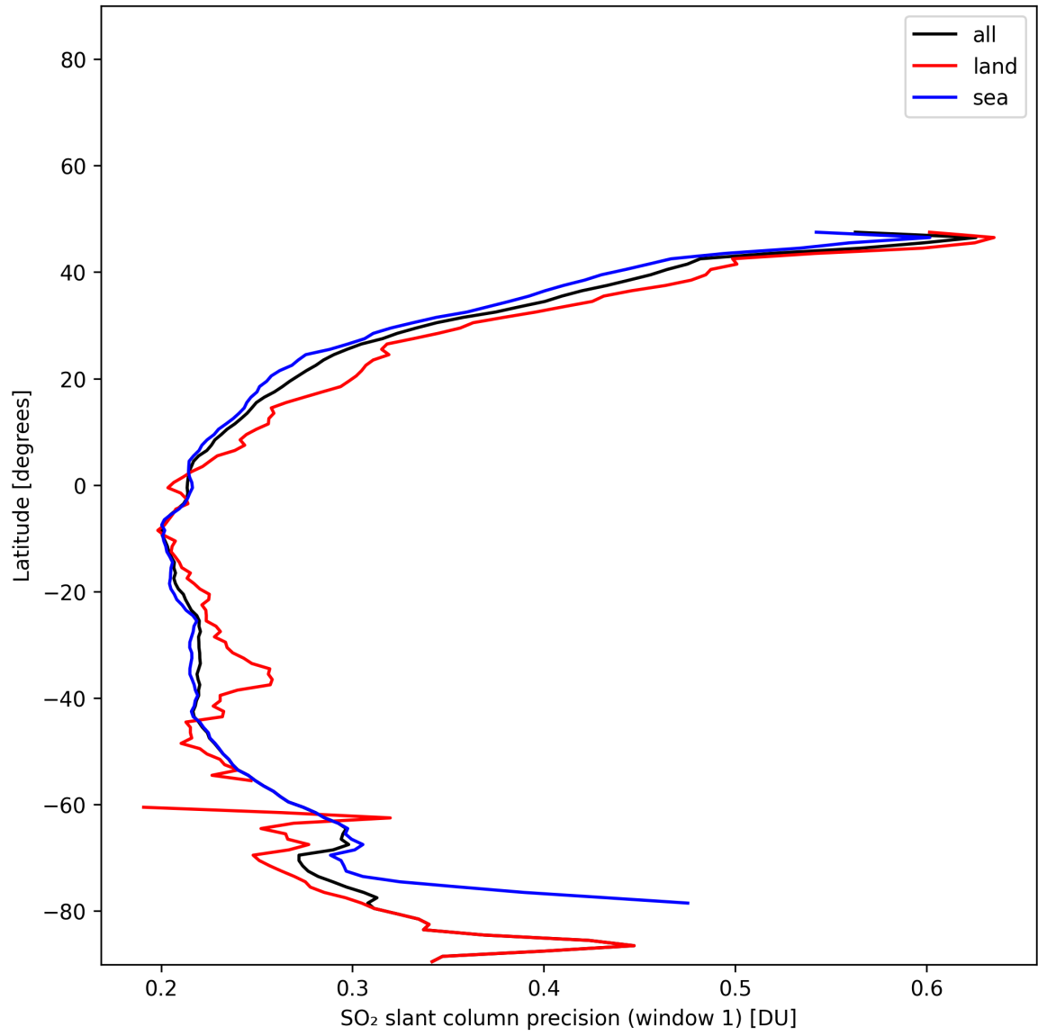
Figure 37: Zonal average of “SO 2 slant column precision (window 1)” for 2025-01-02 to 2025-01-03.
