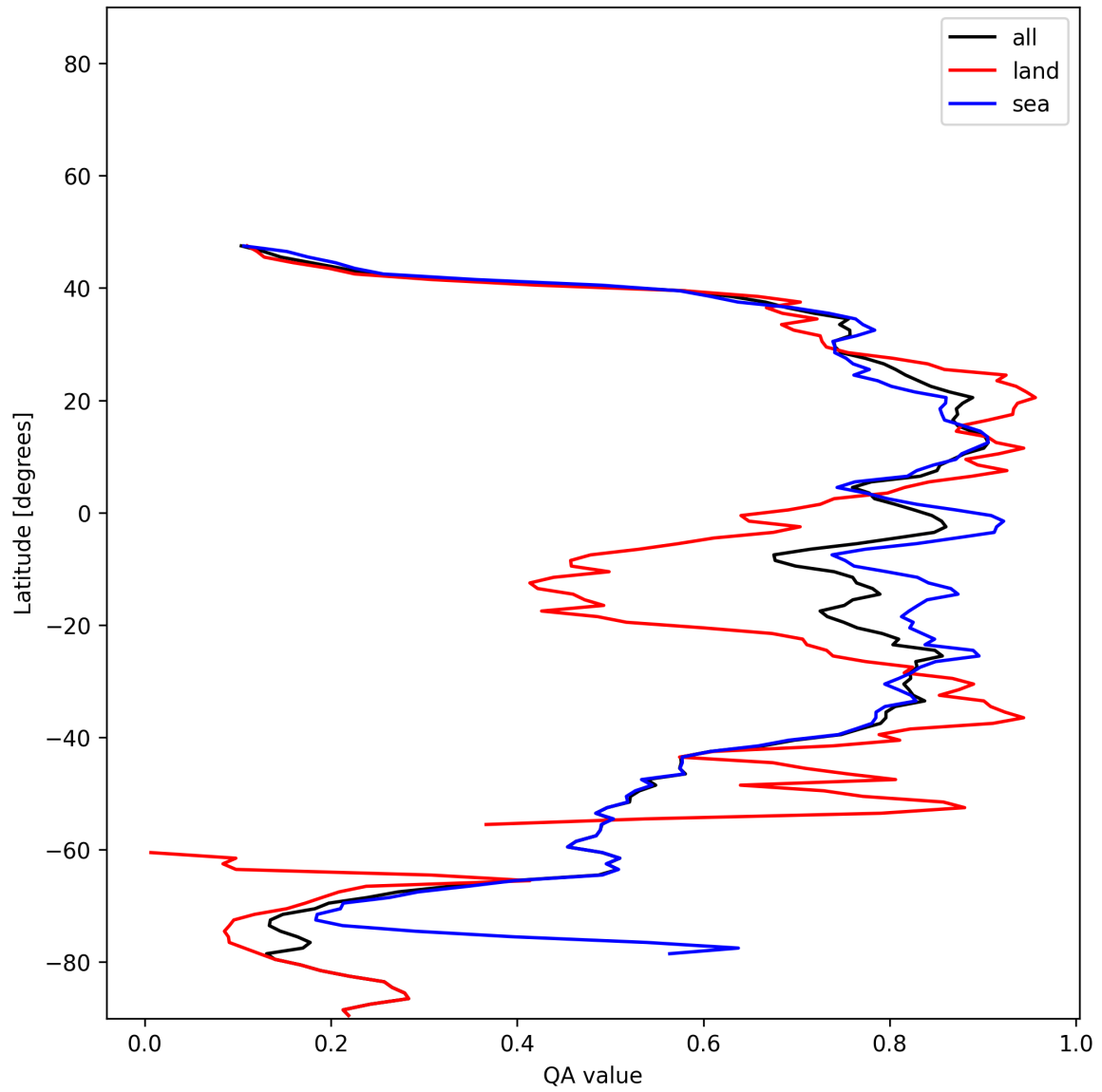
Figure 30: Zonal average of “QA value” for 2025-01-02 to 2025-01-03.
