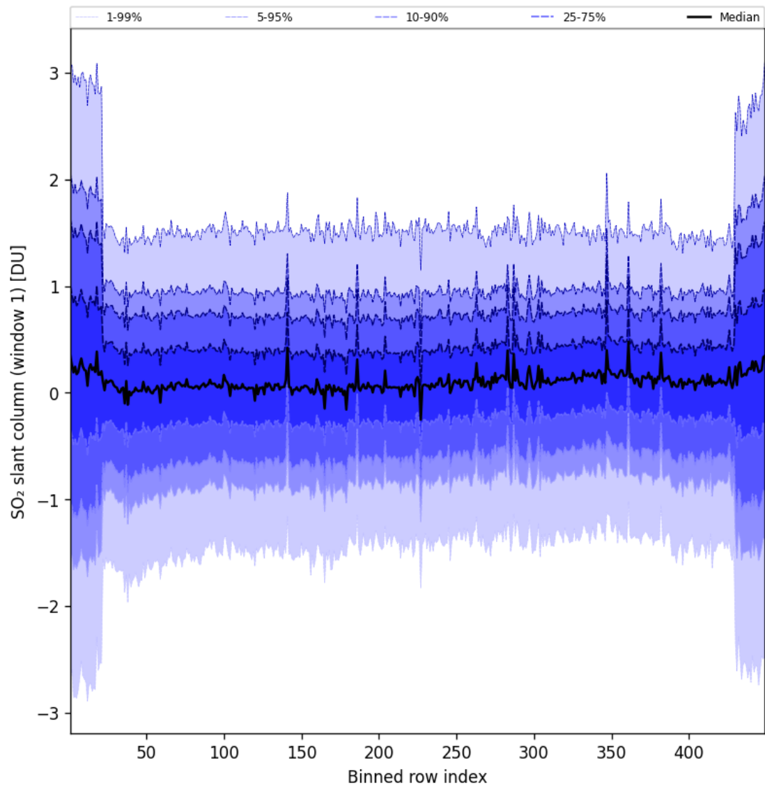
Figure 90: Along track statistics of “SO 2 slant column (window 1)” for 2025-01-02 to 2025-01-03
