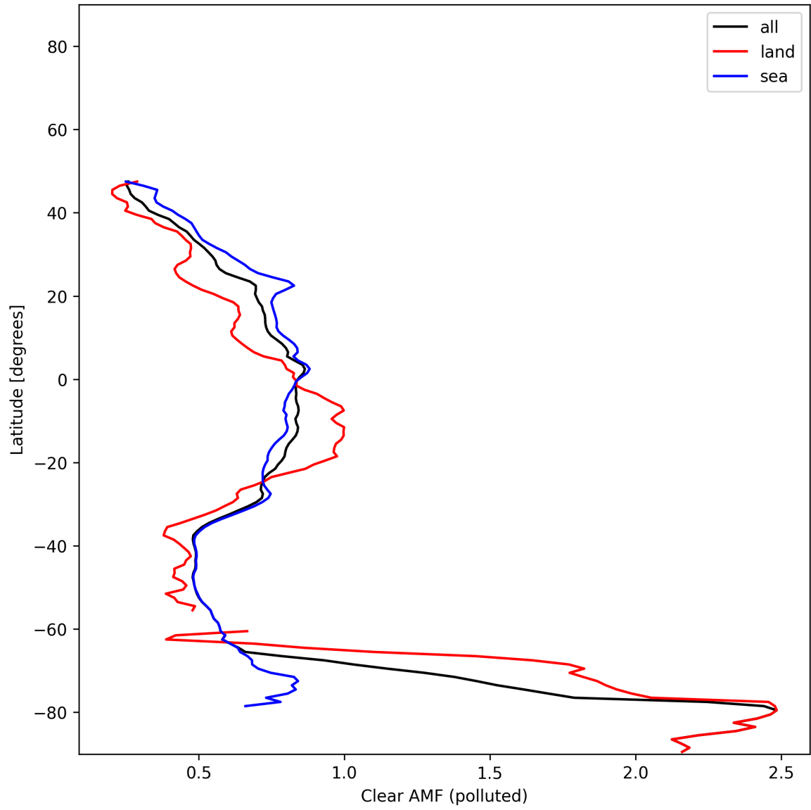
Figure 55: Zonal average of “Clear AMF (polluted)” for 2025-01-02 to 2025-01-03.
