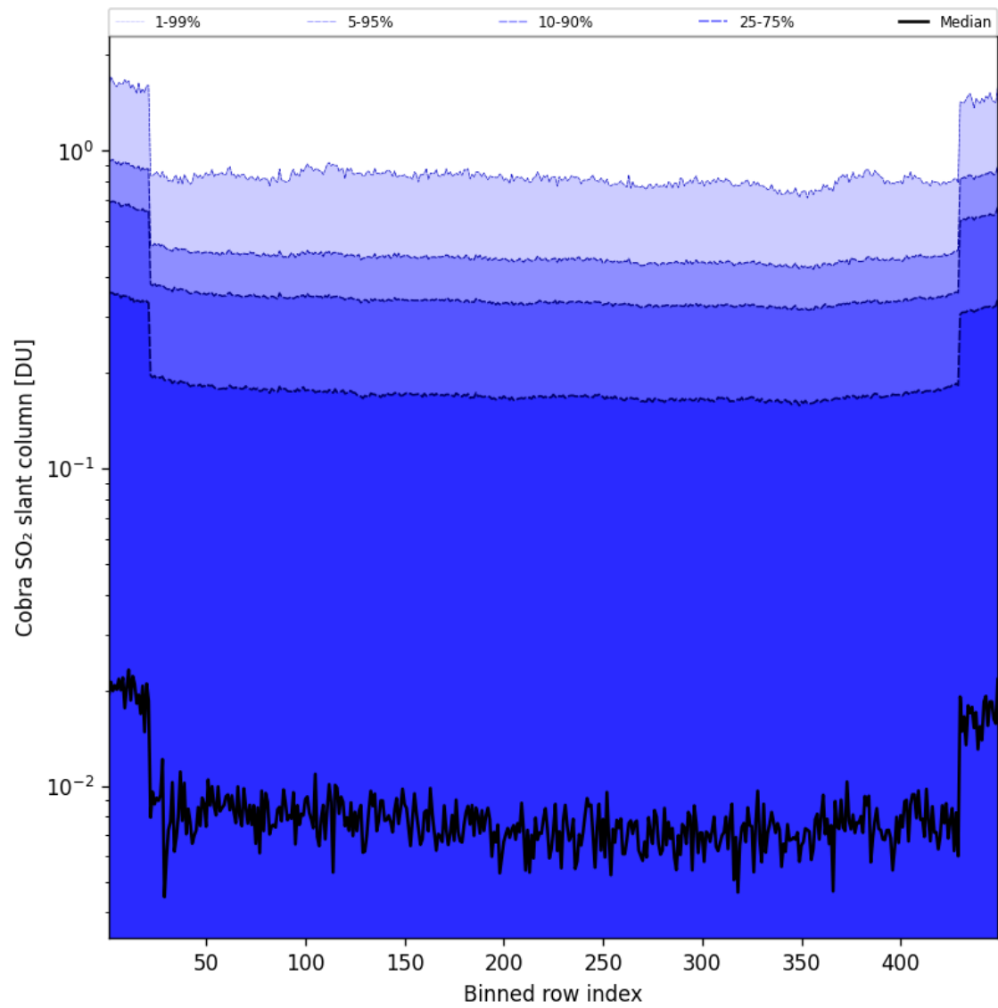
Figure 88: Along track statistics of “Cobra SO 2 slant column” for 2025-01-02 to 2025-01-03
