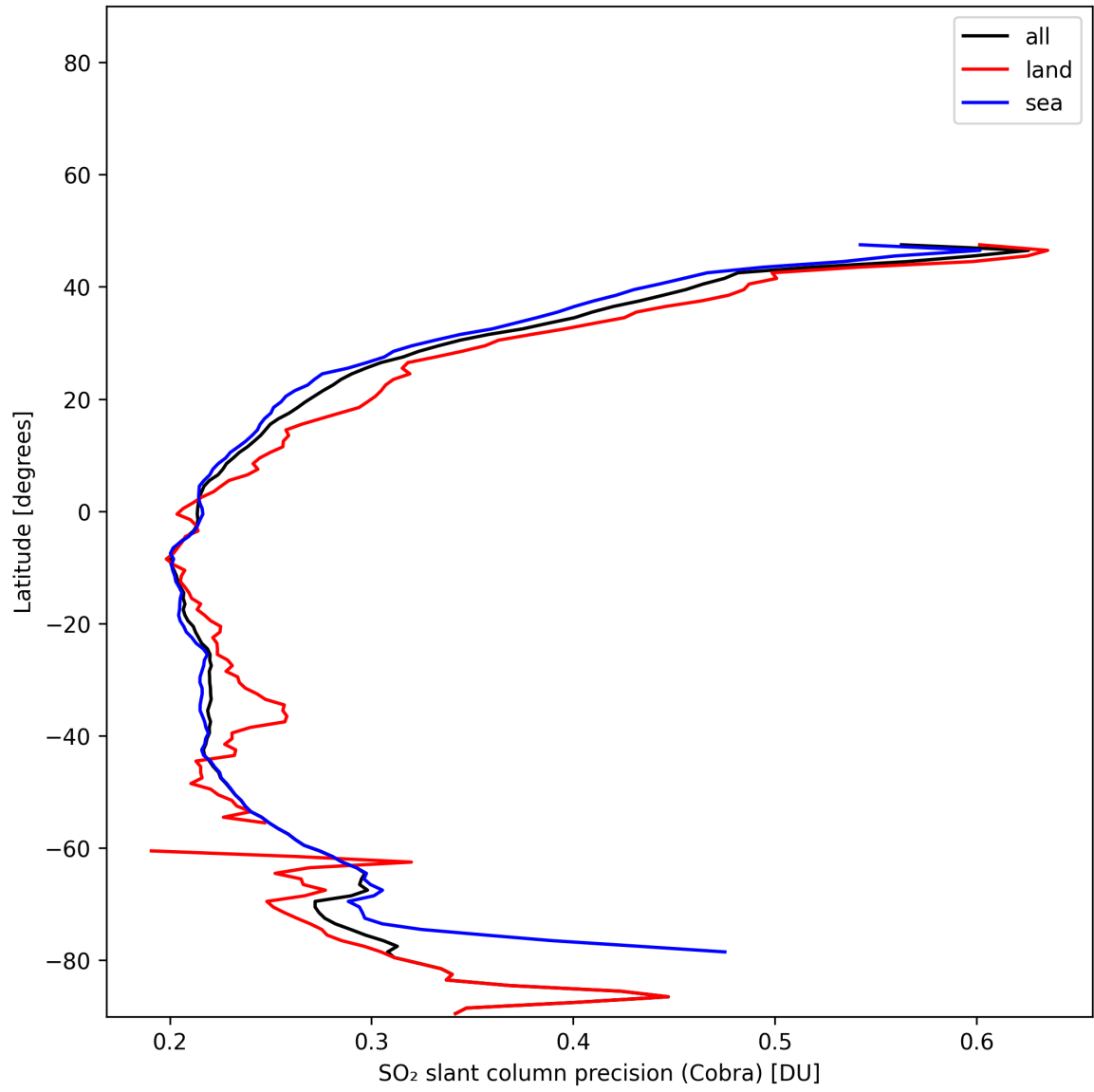
Figure 35: Zonal average of “SO 2 slant column precision (Cobra)” for 2025-01-02 to 2025-01-03.
