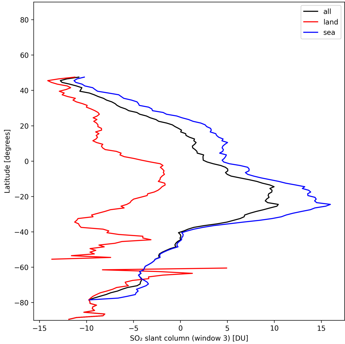
Figure 44: Zonal average of “SO 2 slant column (window 3)” for 2025-01-02 to 2025-01-03.
