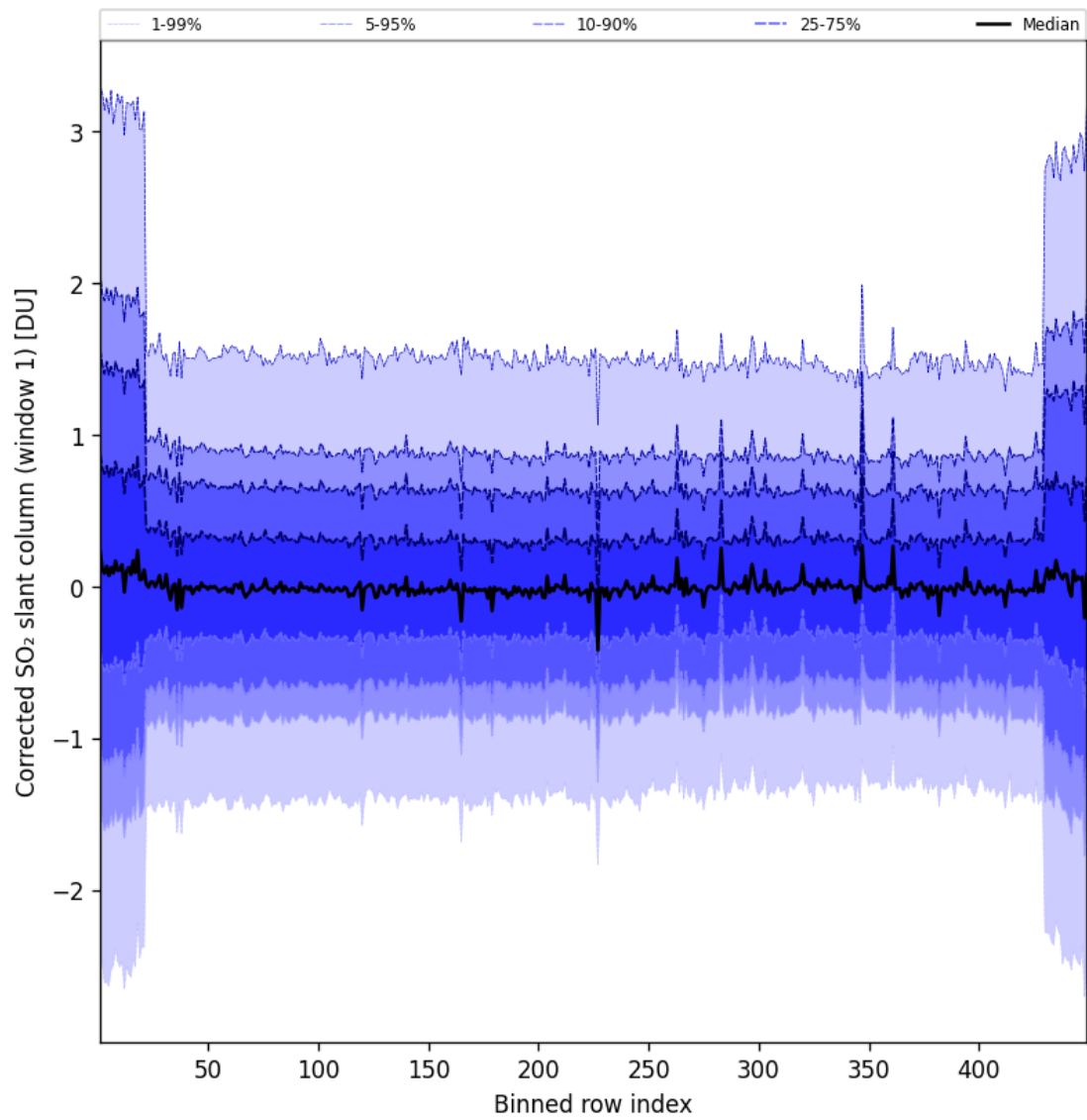
Figure 92: Along track statistics of “Corrected SO 2 slant column (window 1)” for 2025-01-02 to 2025-01-03
