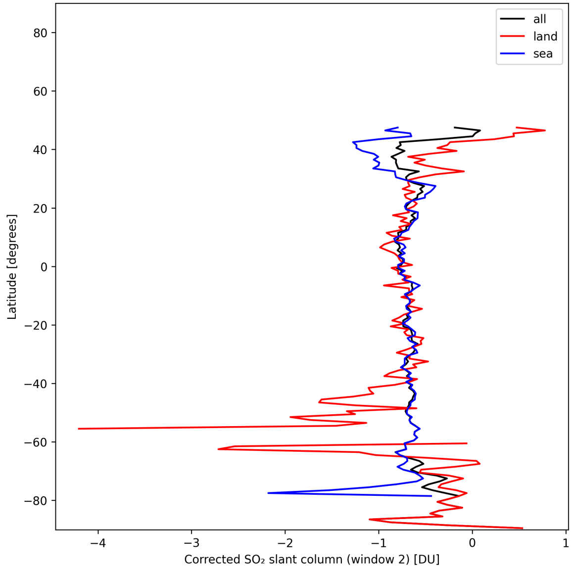
Figure 42: Zonal average of “Corrected SO 2 slant column (window 2)” for 2025-01-02 to 2025-01-03.
