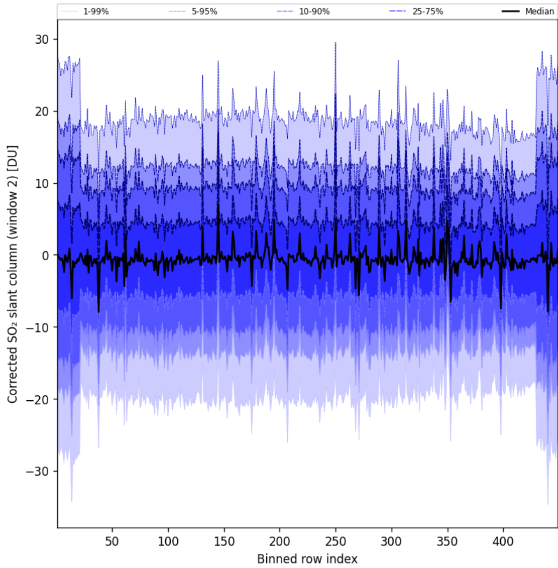
Figure 96: Along track statistics of “Corrected SO 2 slant column (window 2)” for 2025-01-02 to 2025-01-03
