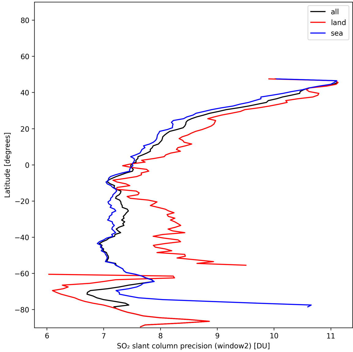
Figure 41: Zonal average of “SO 2 slant column precision (window2)” for 2025-01-02 to 2025-01-03.
