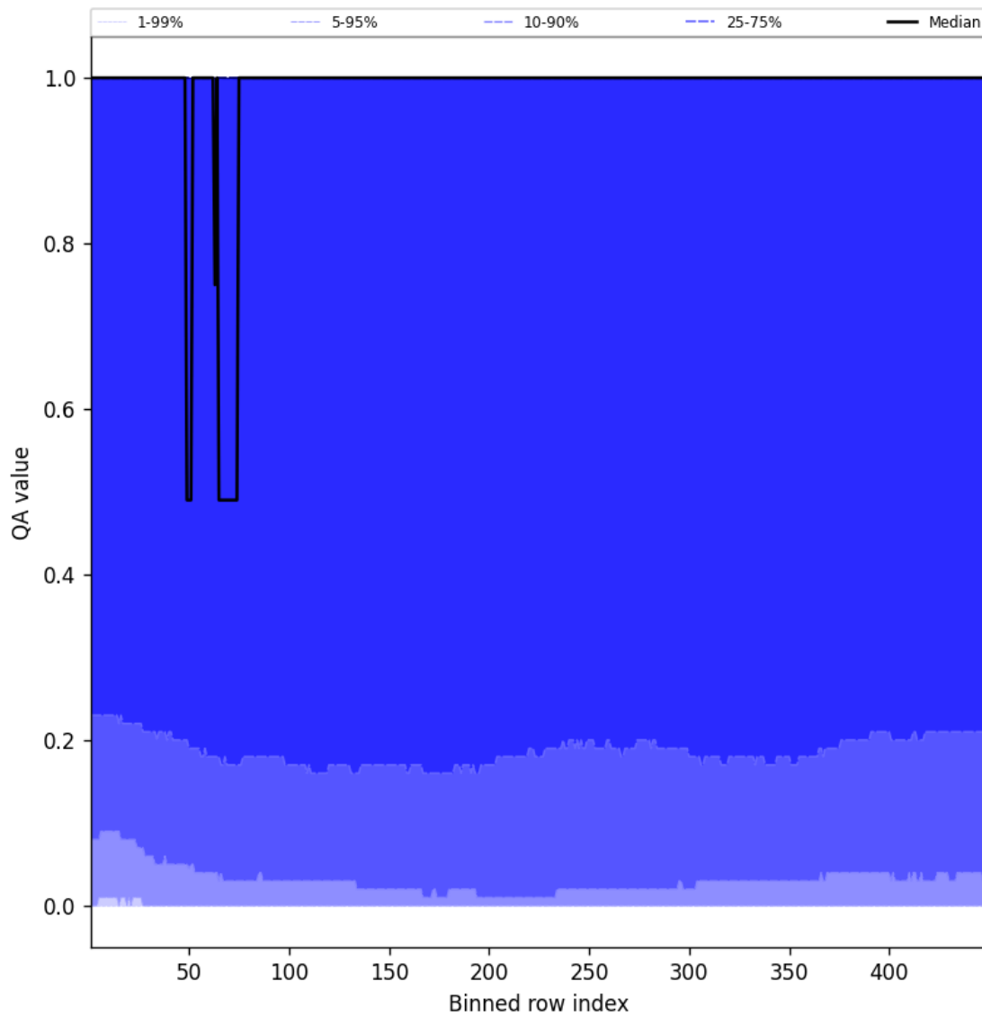
Figure 84: Along track statistics of “QA value” for 2025-01-02 to 2025-01-03
