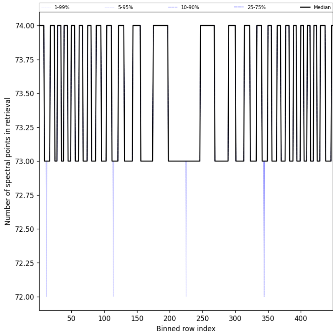
Figure 110: Along track statistics of “Number of spectral points in retrieval” for 2025-01-02 to 2025-01-03
