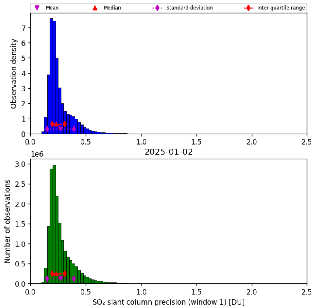
Figure 64: Histogram of “SO 2 slant column precision (window 1)” for 2025-01-02 to 2025-01-03
