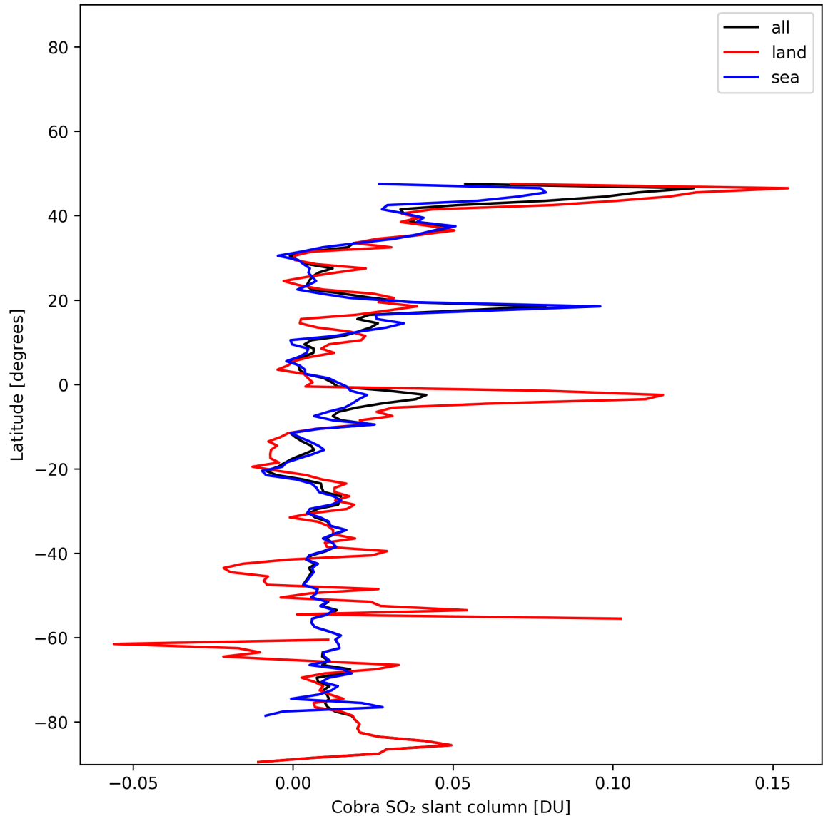
Figure 34: Zonal average of “Cobra SO 2 slant column” for 2025-01-02 to 2025-01-03.
