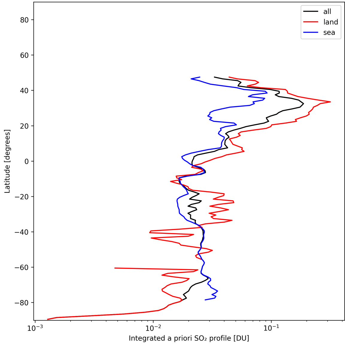
Figure 49: Zonal average of “Integrated a priori SO 2 profile” for 2025-01-02 to 2025-01-03.
