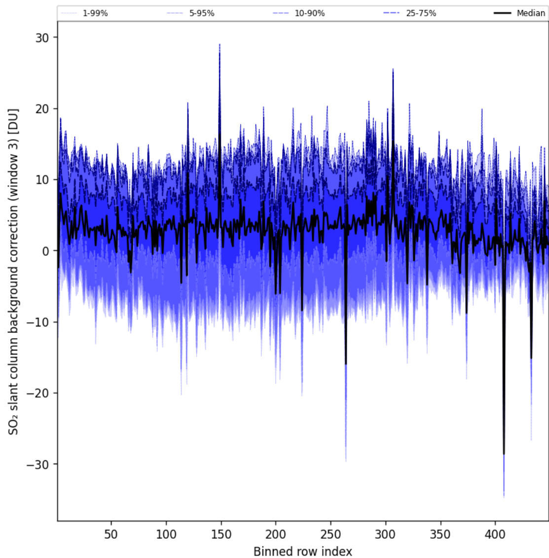
Figure 101: Along track statistics of “SO 2 slant column background correction (window 3)” for 2025-01-02 to 2025-01-03
