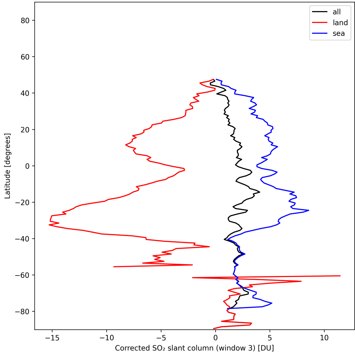
Figure 46: Zonal average of “Corrected SO 2 slant column (window 3)” for 2025-01-02 to 2025-01-03.
