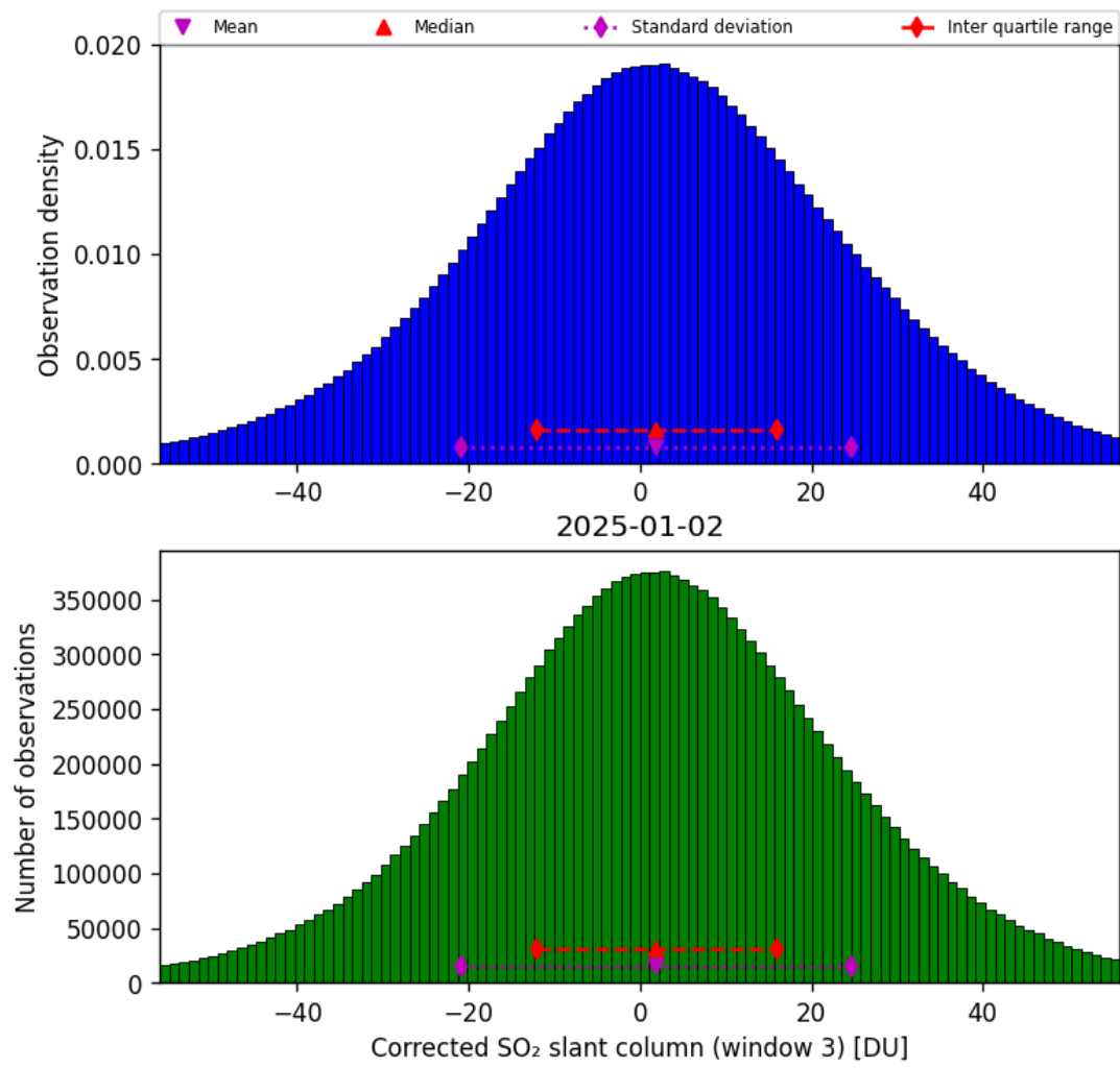
Figure 73: Histogram of “Corrected SO 2 slant column (window 3)” for 2025-01-02 to 2025-01-03
