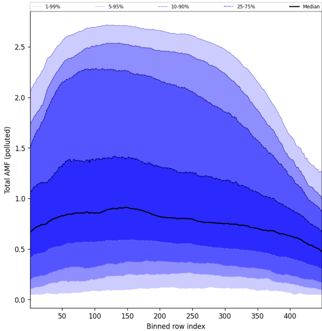
Figure 107: Along track statistics of “Total AMF (polluted)” for 2025-01-02 to 2025-01-03
