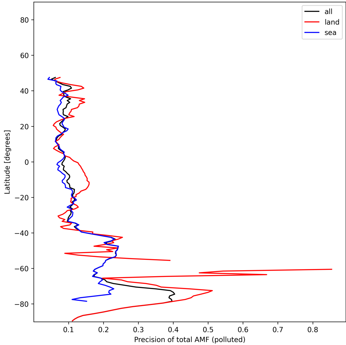
Figure 54: Zonal average of “Precision of total AMF (polluted)” for 2025-01-02 to 2025-01-03.
