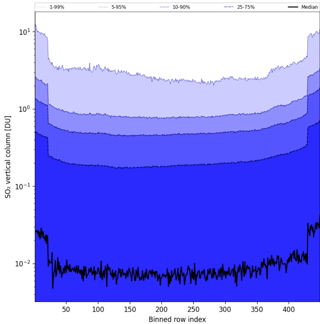
Figure 85: Along track statistics of “SO 2 vertical column” for 2025-01-02 to 2025-01-03
