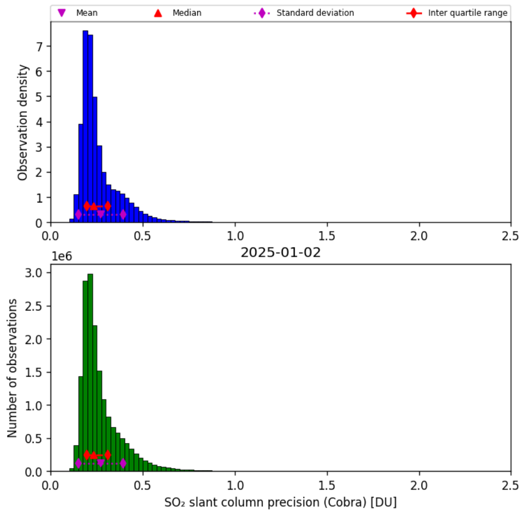
Figure 62: Histogram of “SO 2 slant column precision (Cobra)” for 2025-01-02 to 2025-01-03
