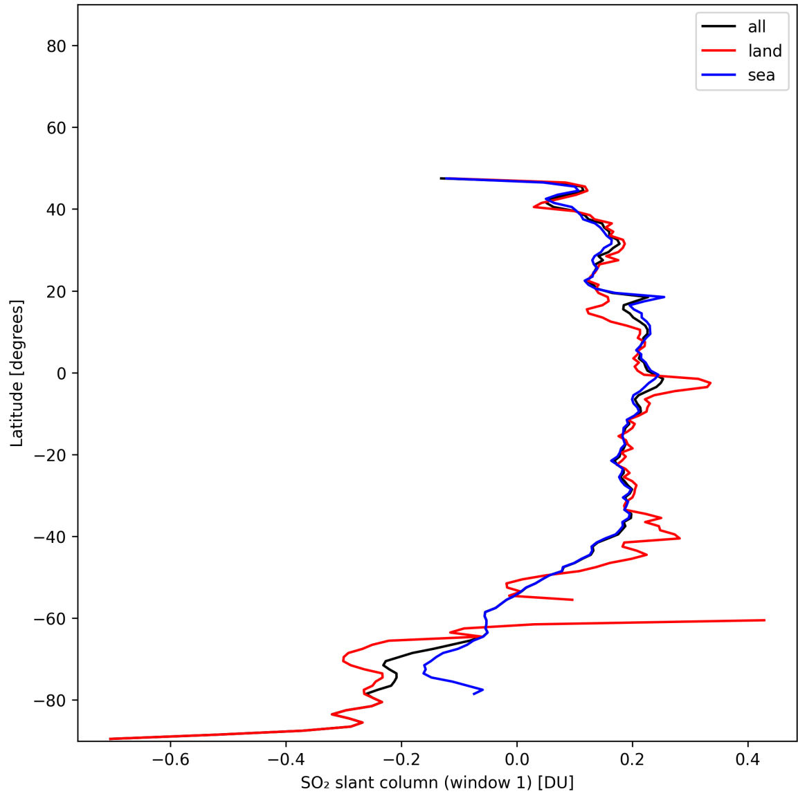
Figure 36: Zonal average of “SO 2 slant column (window 1)” for 2025-01-02 to 2025-01-03.
