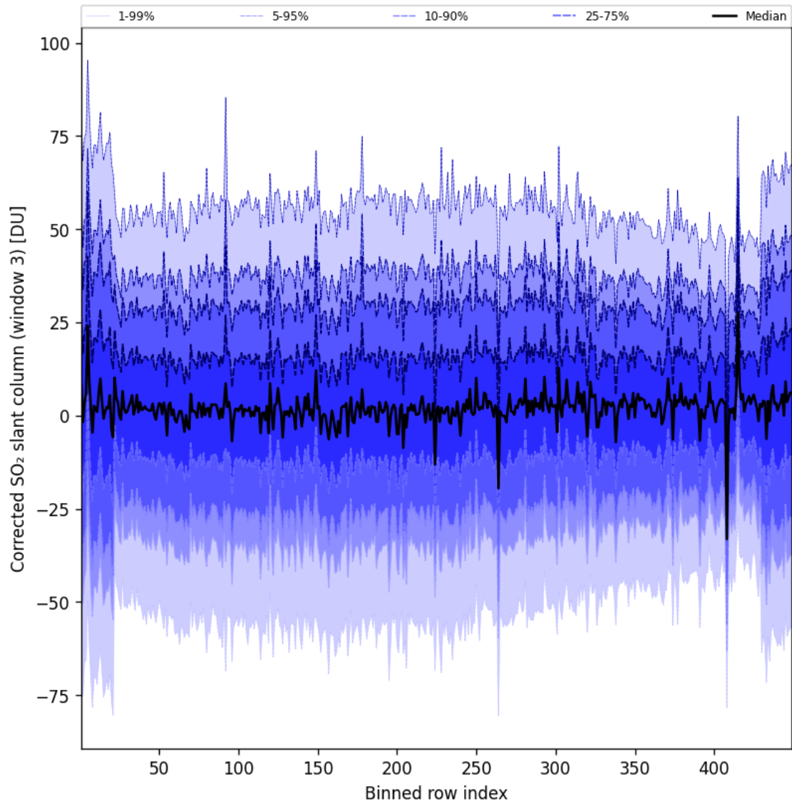
Figure 100: Along track statistics of "Corrected SO 2 slant column (window 3)" for 2025-01-02 to 2025-01-03
