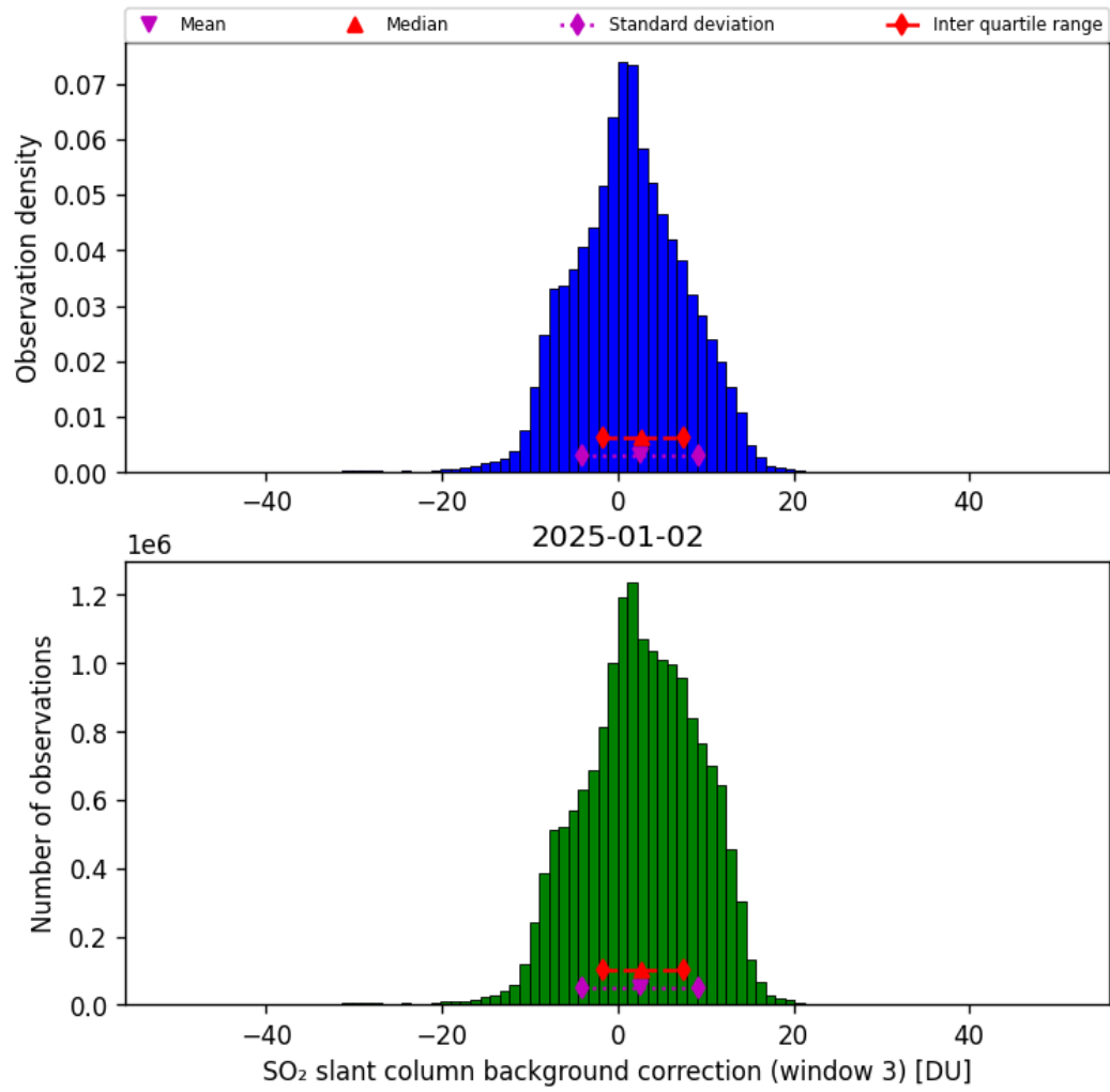
Figure 74: Histogram of “SO 2 slant column background correction (window 3)” for 2025-01-02 to 2025-01-03
