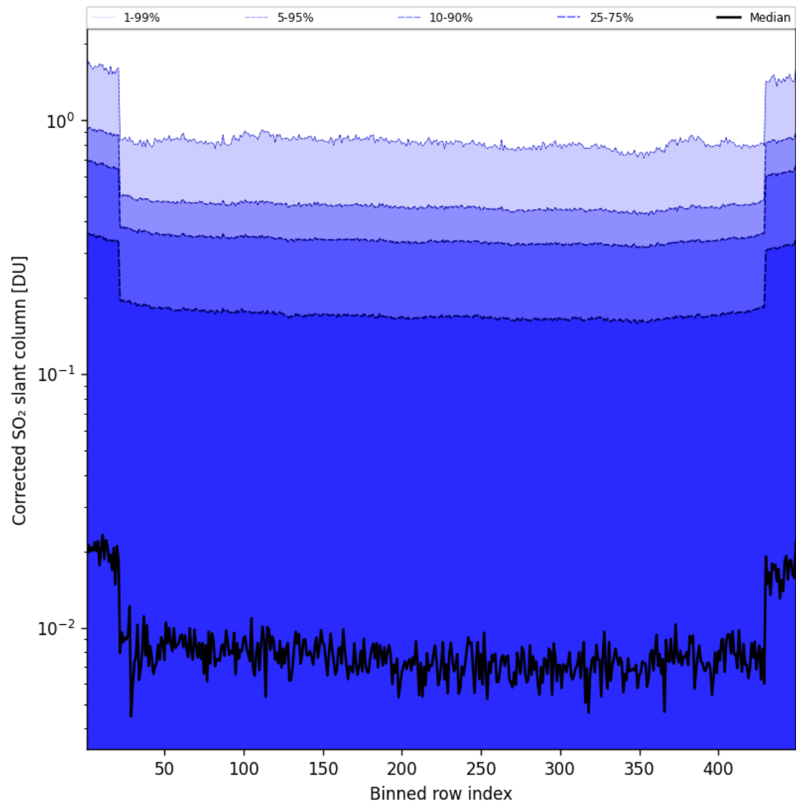
Figure 87: Along track statistics of “Corrected SO 2 slant column” for 2025-01-02 to 2025-01-03
