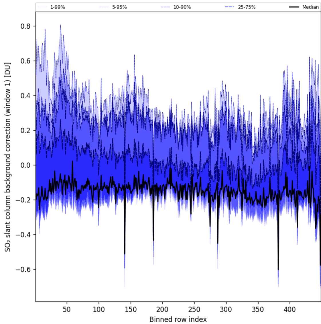
Figure 93: Along track statistics of “SO 2 slant column background correction (window 1)” for 2025-01-02 to 2025-01-03
