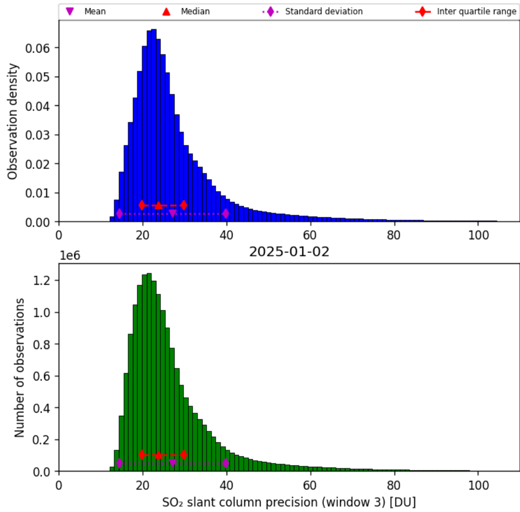
Figure 72: Histogram of “SO 2 slant column precision (window 3)” for 2025-01-02 to 2025-01-03
