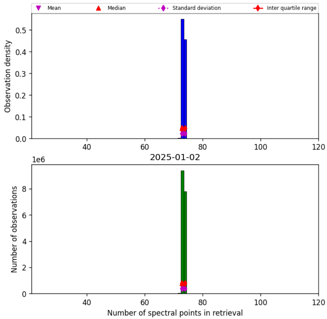
Figure 83: Histogram of “Number of spectral points in retrieval” for 2025-01-02 to 2025-01-03
