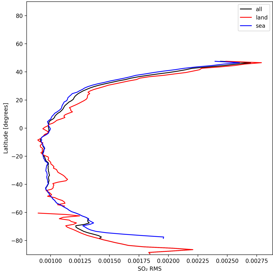
Figure 52: Zonal average of “SO 2 RMS” for 2025-01-02 to 2025-01-03.
