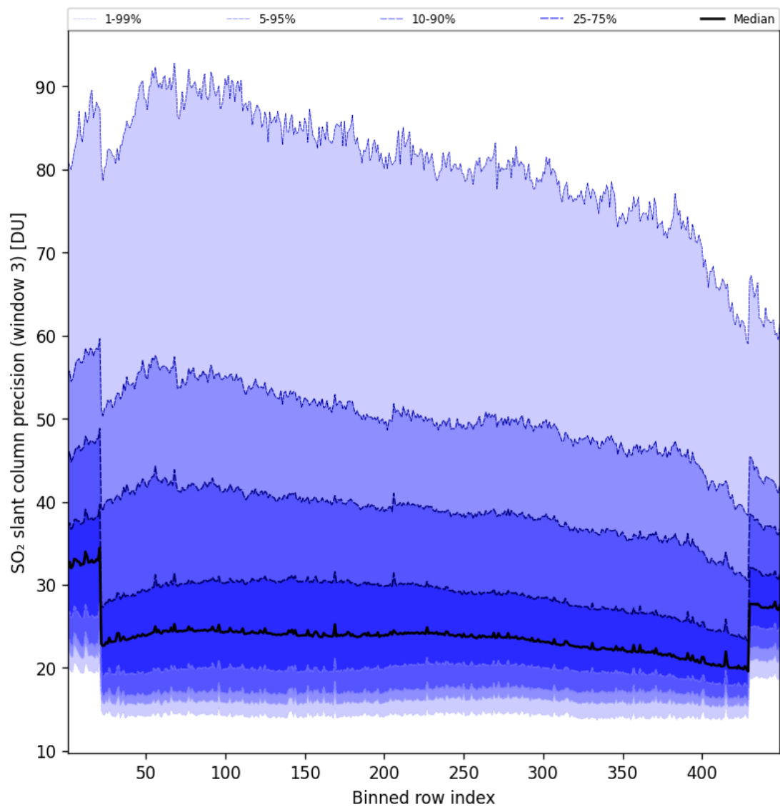
Figure 99: Along track statistics of “SO 2 slant column precision (window 3)” for 2025-01-02 to 2025-01-03
