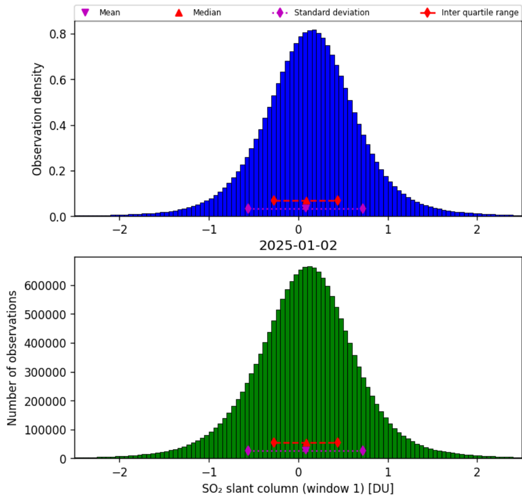
Figure 63: Histogram of “SO 2 slant column (window 1)” for 2025-01-02 to 2025-01-03
