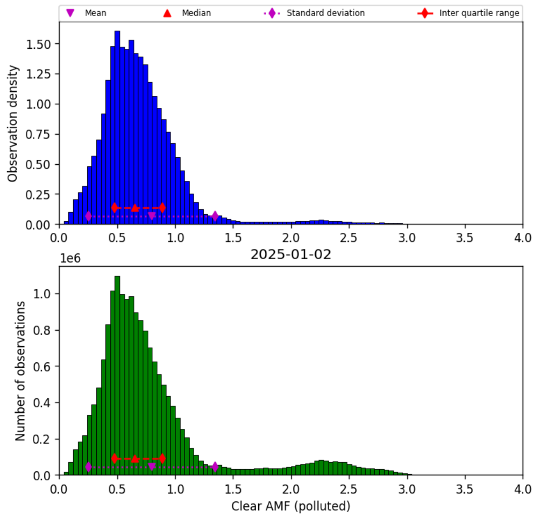
Figure 82: Histogram of “Clear AMF (polluted)” for 2025-01-02 to 2025-01-03
