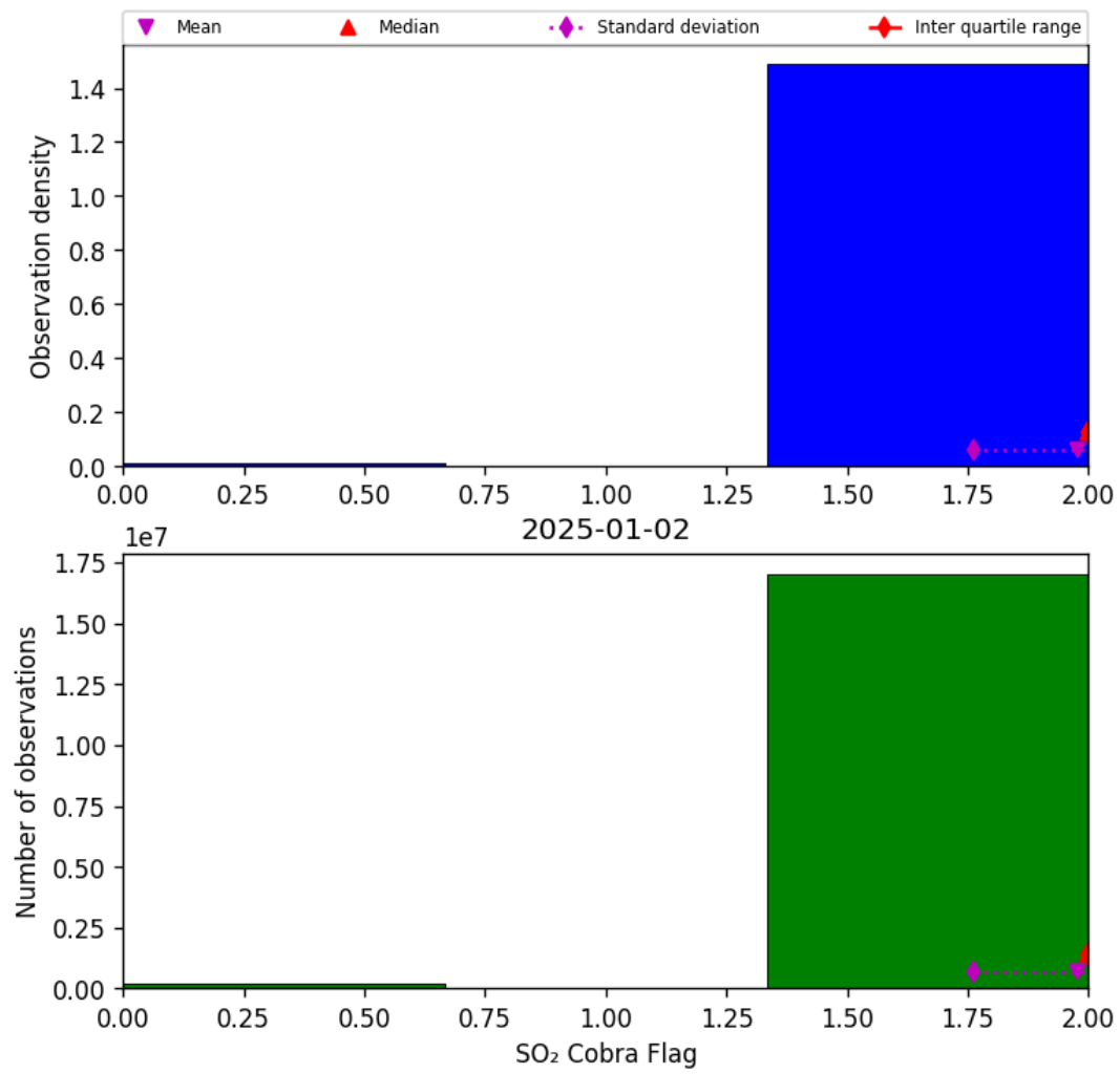
Figure 75: Histogram of “SO 2 Cobra Flag” for 2025-01-02 to 2025-01-03
