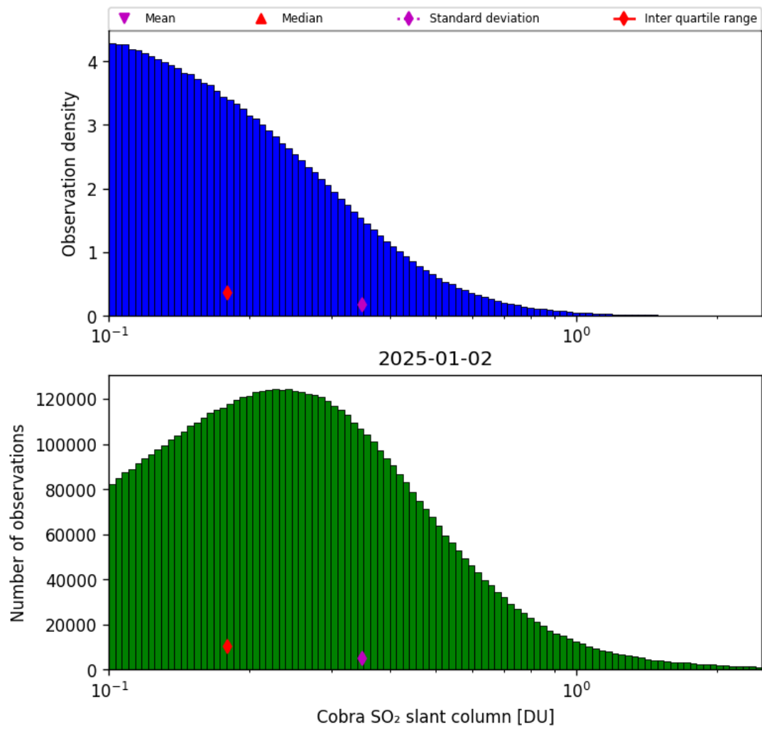
Figure 61: Histogram of “Cobra SO 2 slant column” for 2025-01-02 to 2025-01-03
