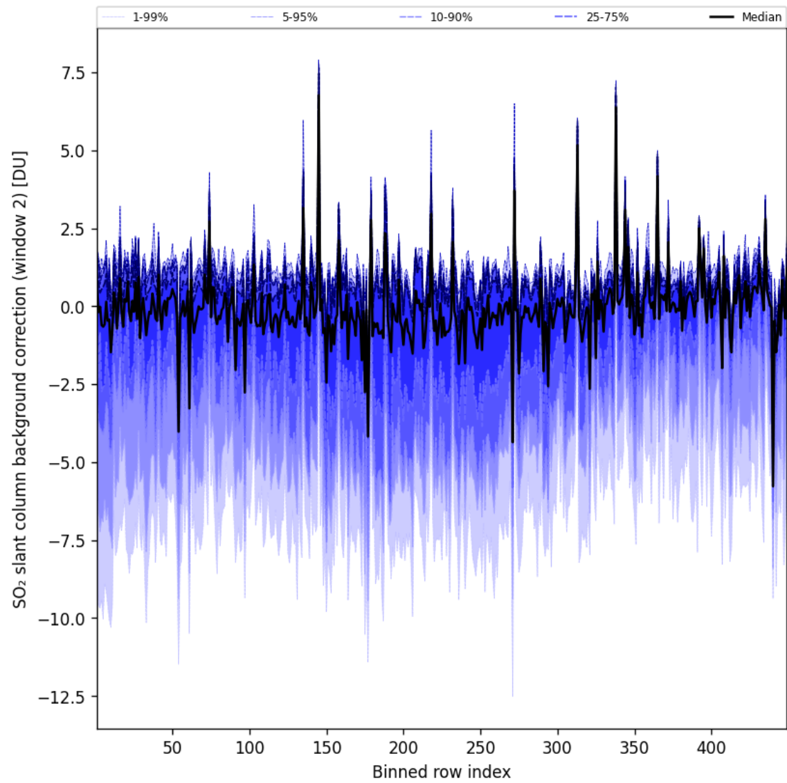
Figure 97: Along track statistics of “SO 2 slant column background correction (window 2)” for 2025-01-02 to 2025-01-03
