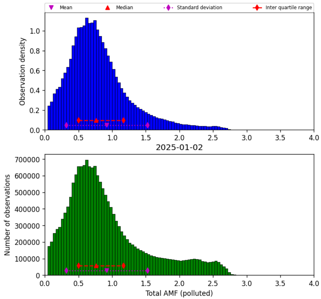
Figure 80: Histogram of “Total AMF (polluted)” for 2025-01-02 to 2025-01-03
