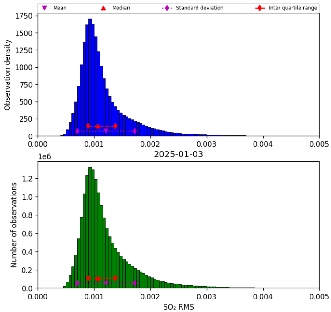
Figure 79: Histogram of “SO 2 RMS” for 2025-01-03 to 2025-01-04
