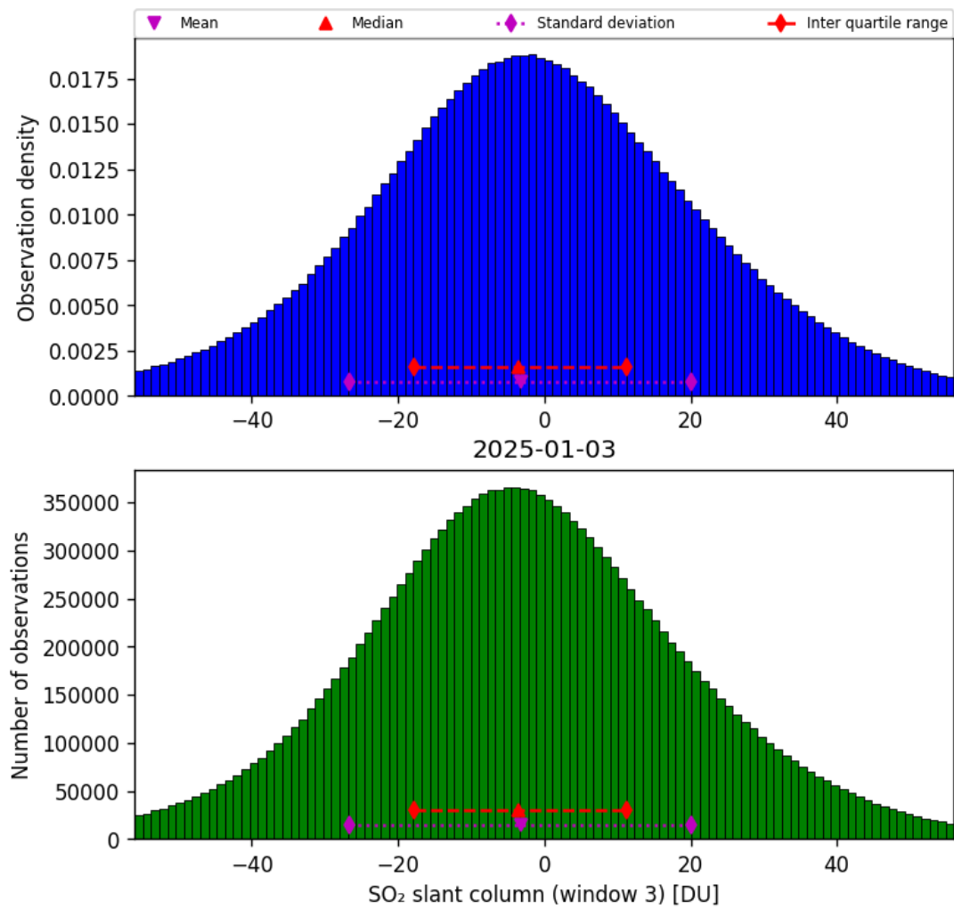
Figure 71: Histogram of “SO 2 slant column (window 3)” for 2025-01-03 to 2025-01-04
