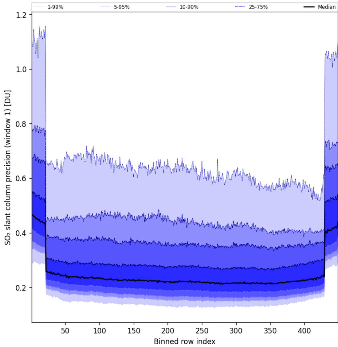
Figure 91: Along track statistics of “SO 2 slant column precision (window 1)” for 2025-01-03 to 2025-01-04
