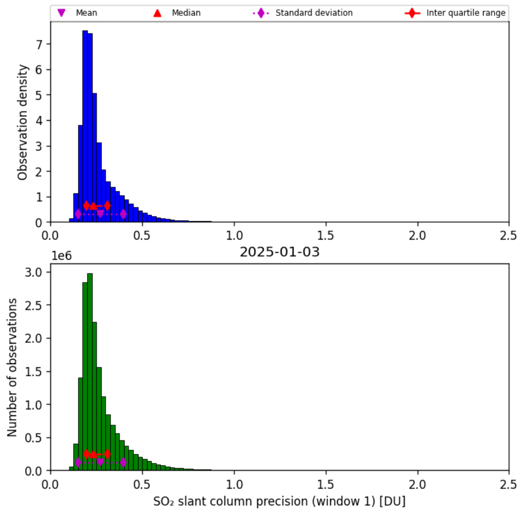
Figure 64: Histogram of “SO 2 slant column precision (window 1)” for 2025-01-03 to 2025-01-04
