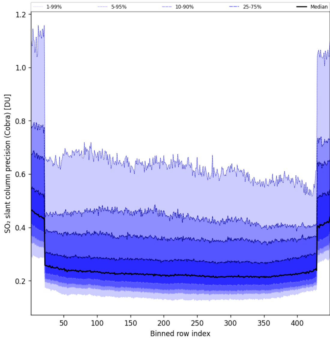
Figure 89: Along track statistics of “SO 2 slant column precision (Cobra)” for 2025-01-03 to 2025-01-04
