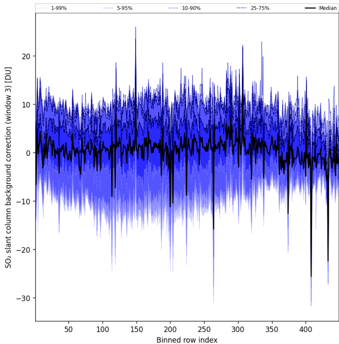
Figure 101: Along track statistics of “SO 2 slant column background correction (window 3)” for 2025-01-03 to 2025-01-04
