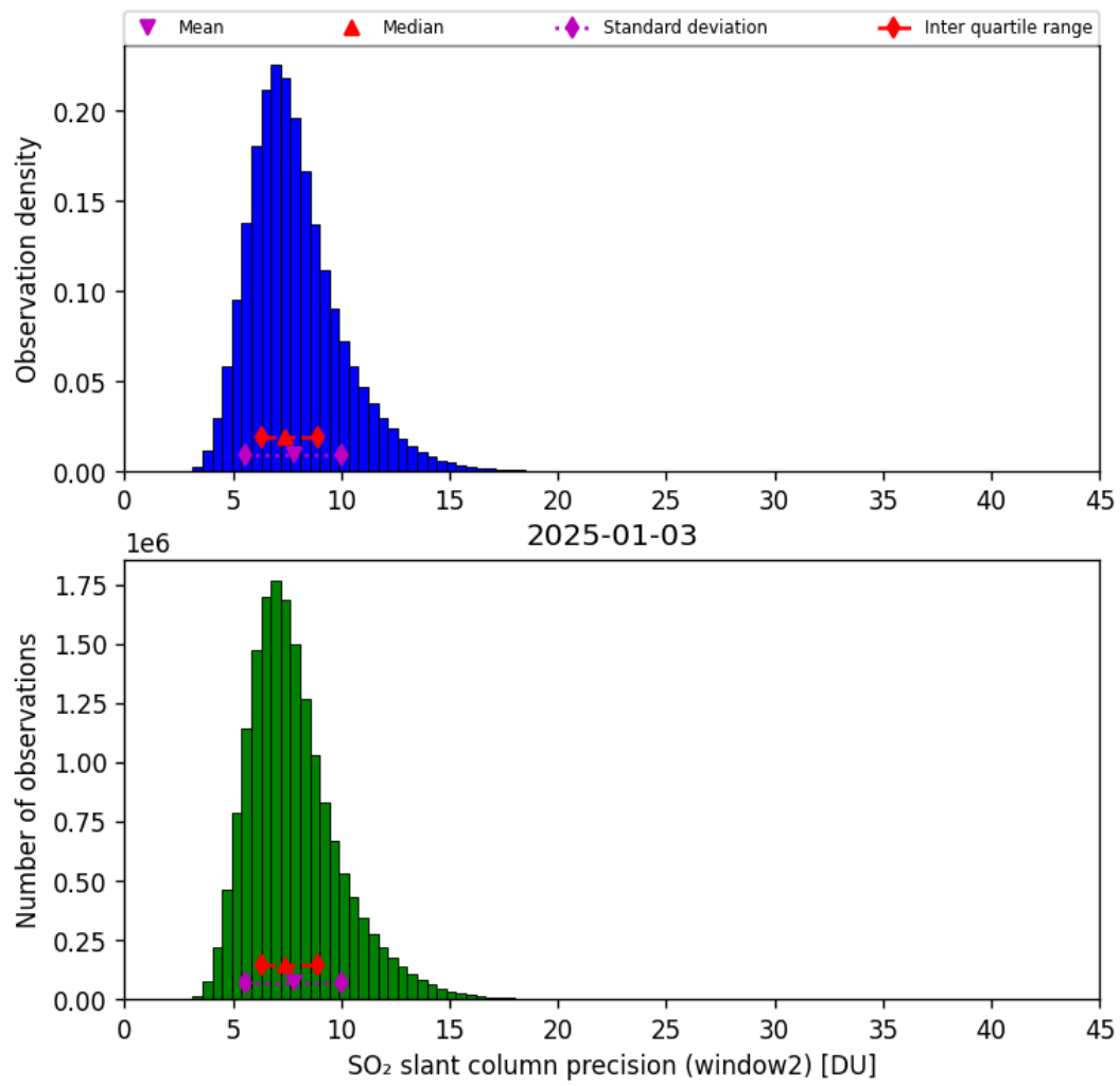
Figure 68: Histogram of “SO 2 slant column precision (window2)” for 2025-01-03 to 2025-01-04
