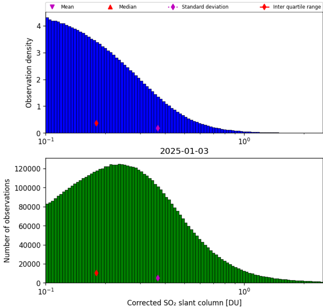
Figure 60: Histogram of “Corrected SO 2 slant column” for 2025-01-03 to 2025-01-04
