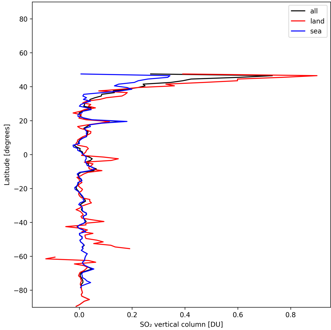
Figure 31: Zonal average of “SO 2 vertical column” for 2025-01-03 to 2025-01-04.
