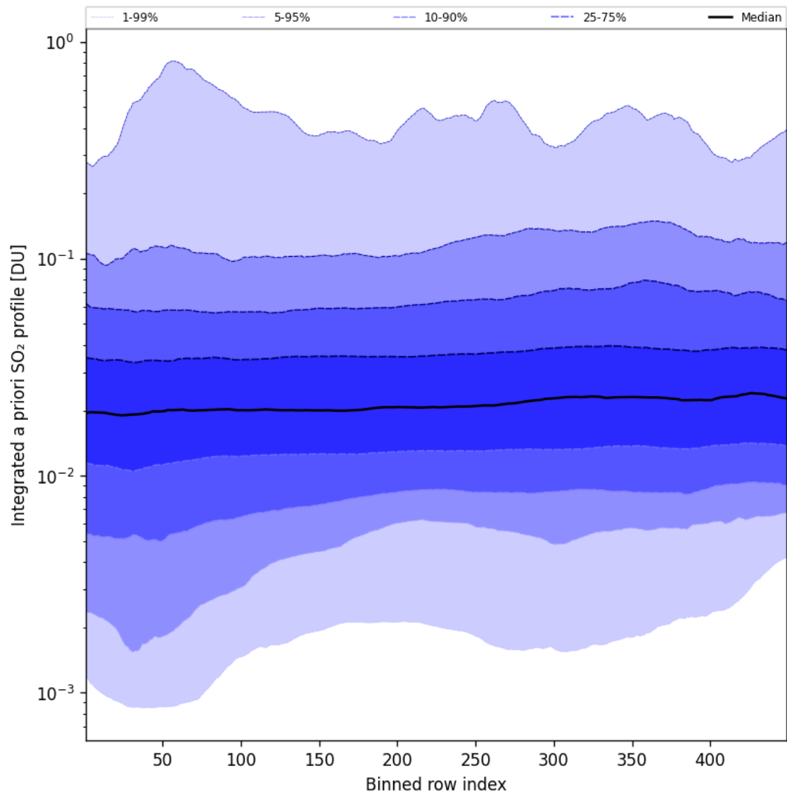
Figure 103: Along track statistics of “Integrated a priori SO 2 profile” for 2025-01-03 to 2025-01-04
