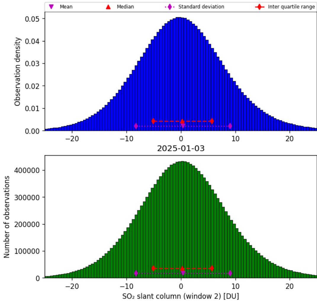
Figure 67: Histogram of “SO 2 slant column (window 2)” for 2025-01-03 to 2025-01-04
