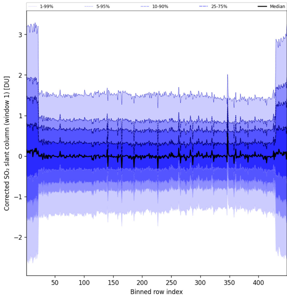
Figure 92: Along track statistics of “Corrected SO 2 slant column (window 1)” for 2025-01-03 to 2025-01-04
