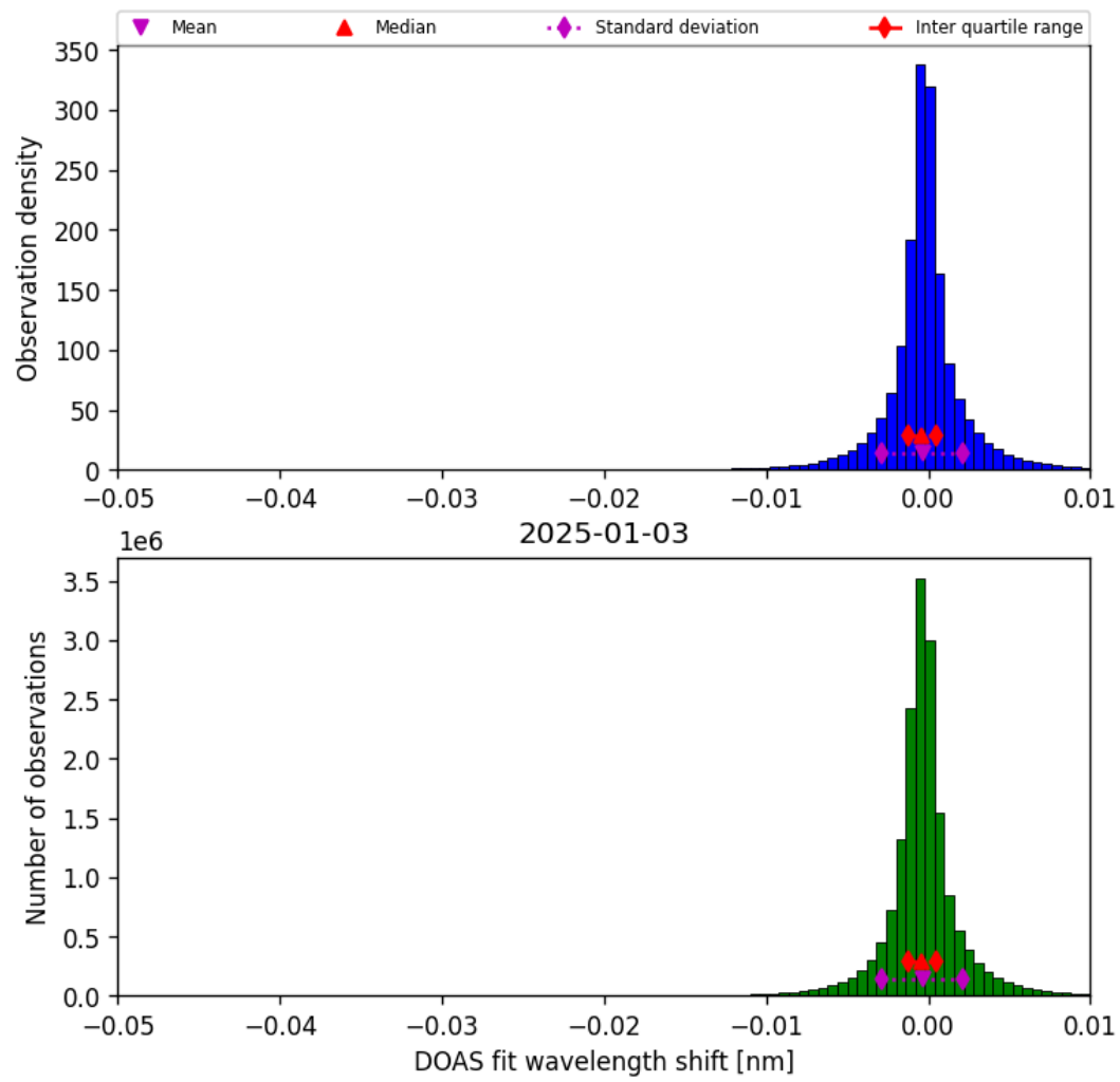
Figure 77: Histogram of “DOAS fit wavelength shift” for 2025-01-03 to 2025-01-04
