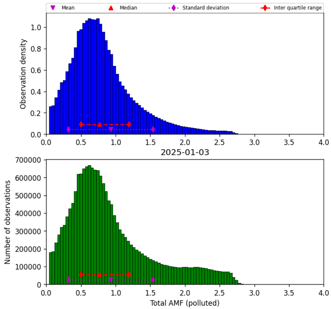
Figure 80: Histogram of “Total AMF (polluted)” for 2025-01-03 to 2025-01-04
