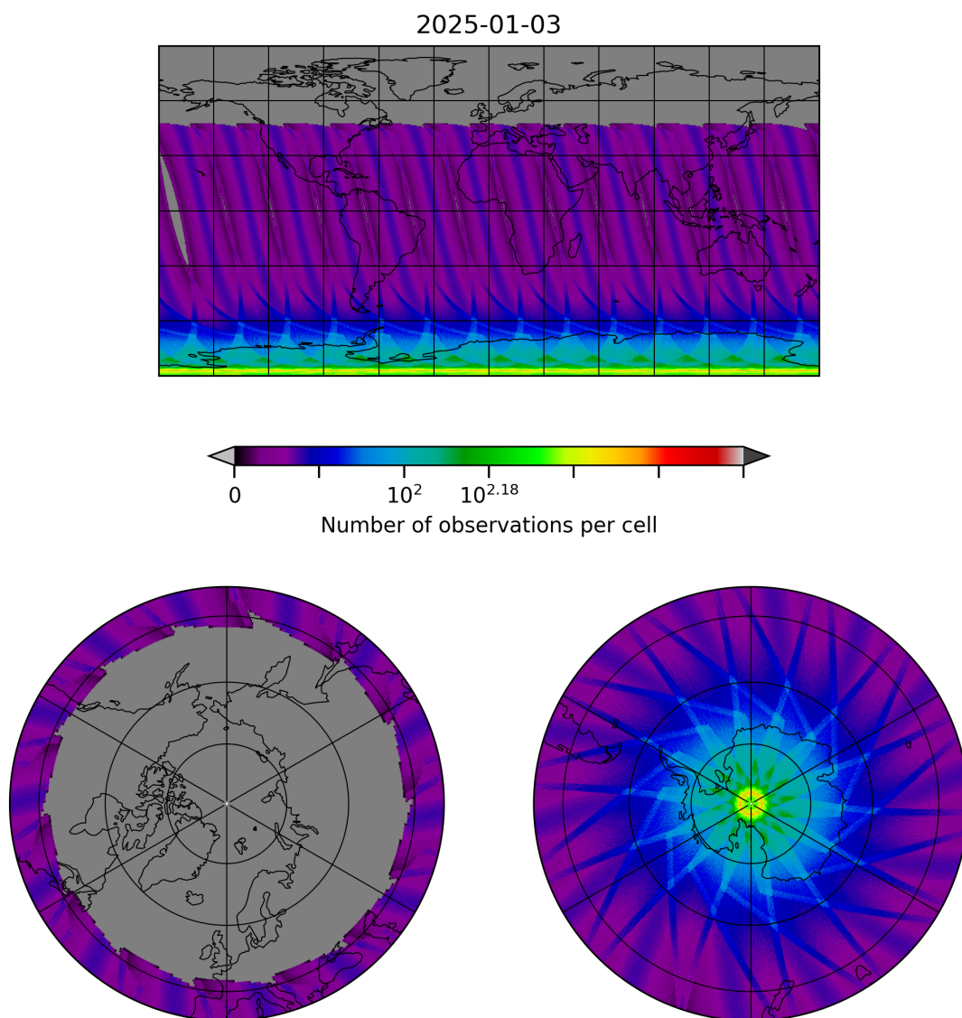
Figure 29: Map of the number of observations for 2025-01-03 to 2025-01-04
