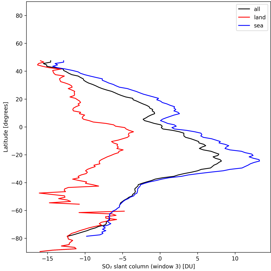
Figure 44: Zonal average of “SO 2 slant column (window 3)” for 2025-01-03 to 2025-01-04.
