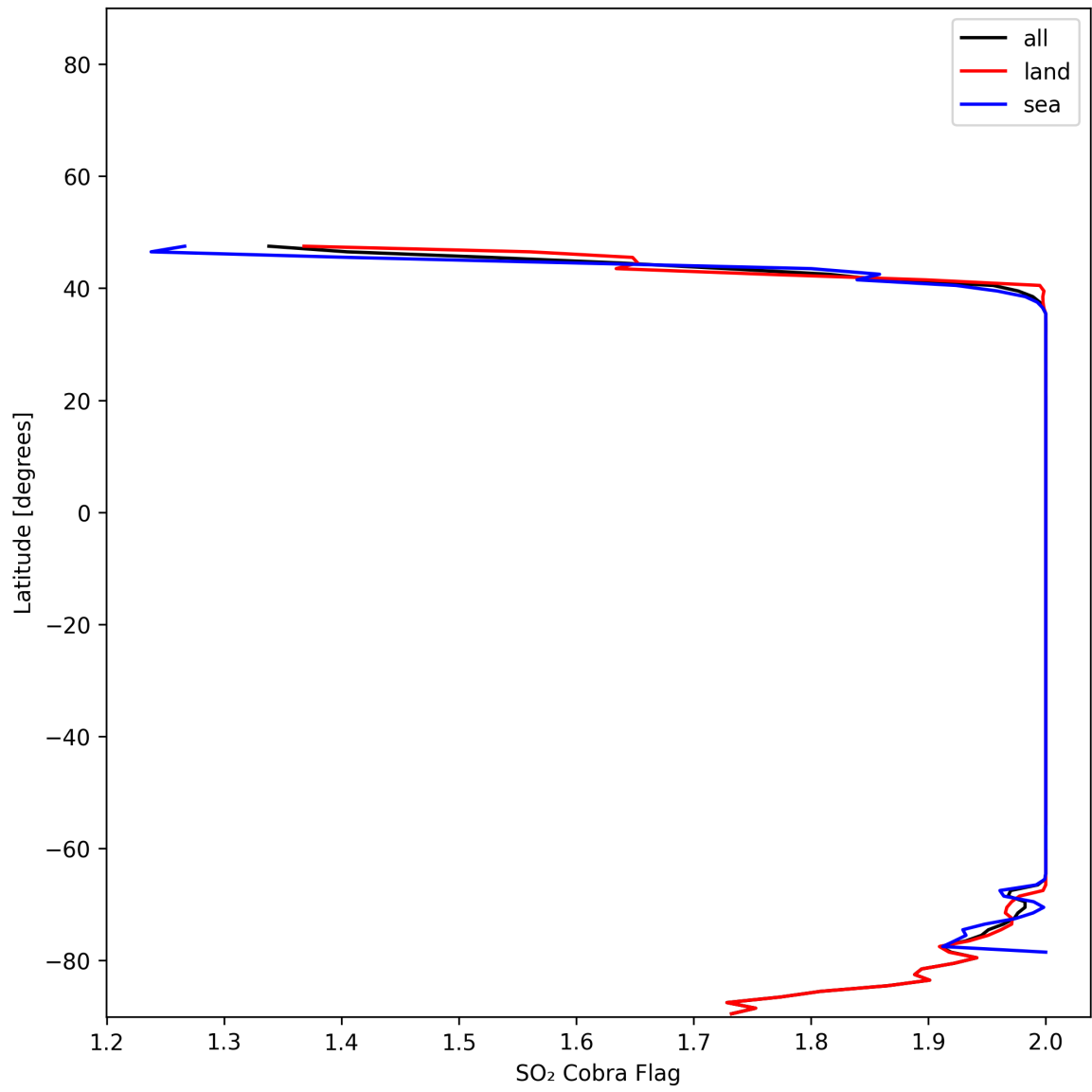
Figure 48: Zonal average of "SO 2 Cobra Flag" for 2025-01-03 to 2025-01-04.
