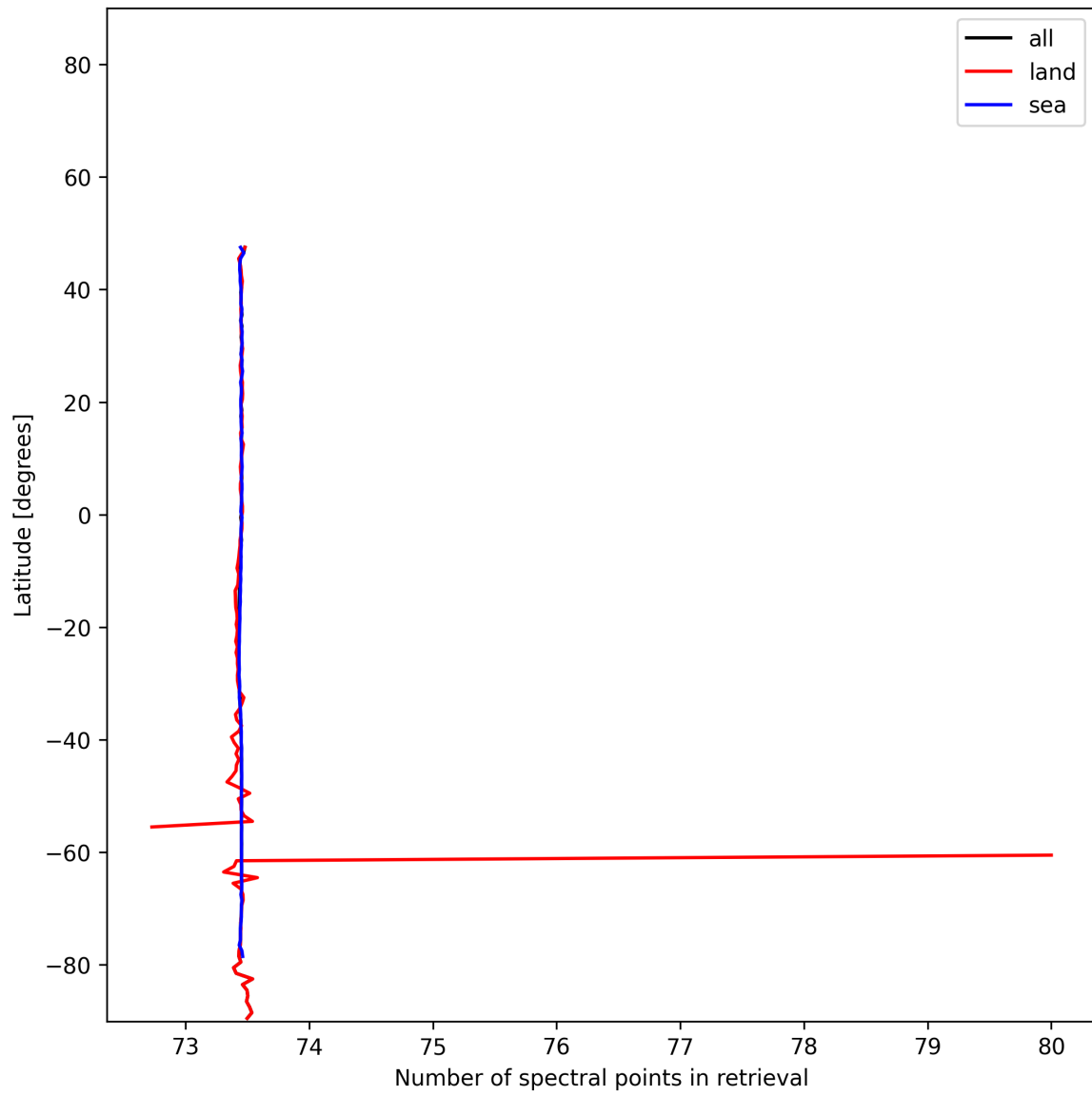
Figure 56: Zonal average of “Number of spectral points in retrieval” for 2025-01-03 to 2025-01-04.
