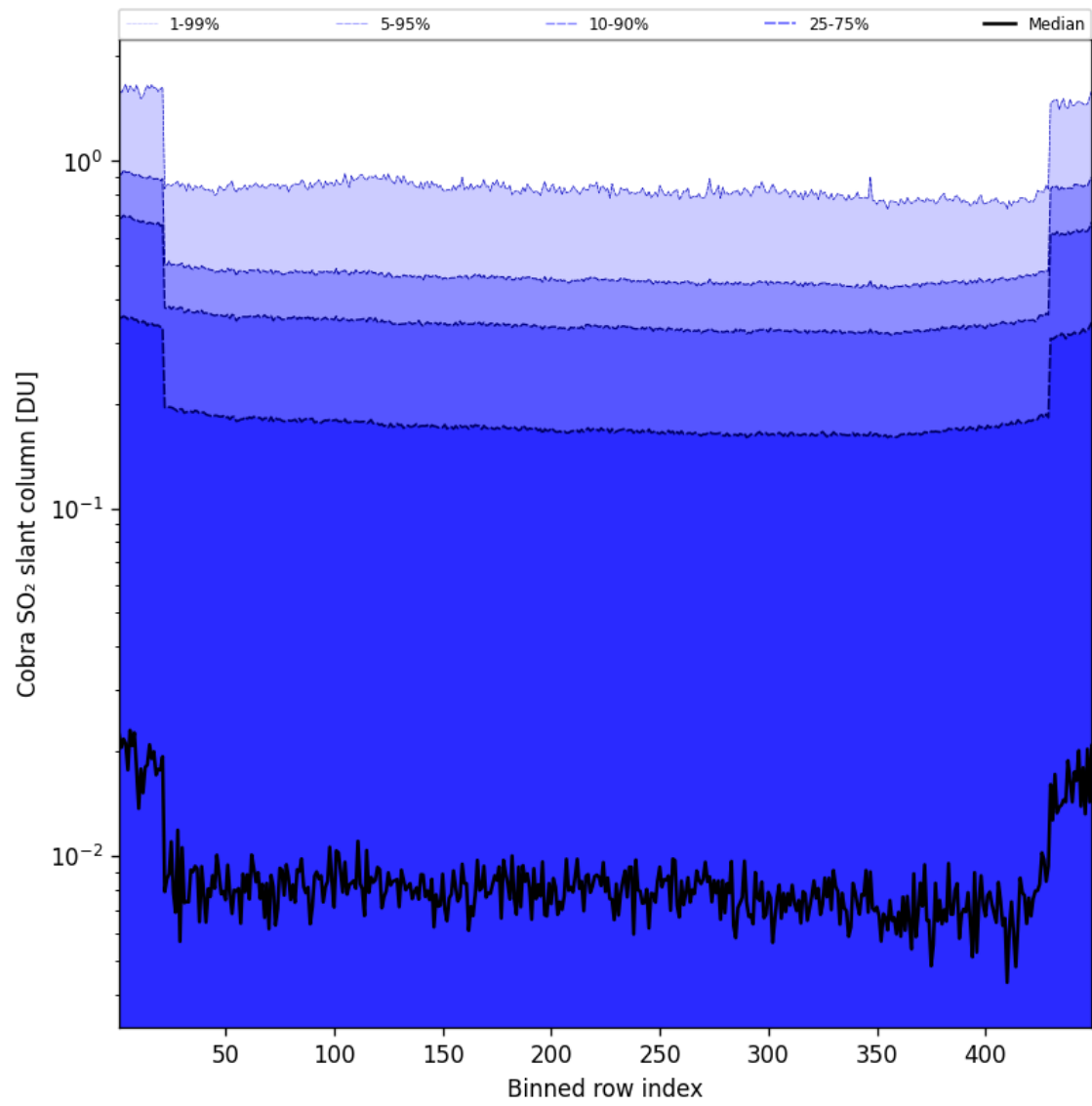
Figure 88: Along track statistics of “Cobra SO 2 slant column” for 2025-01-03 to 2025-01-04
