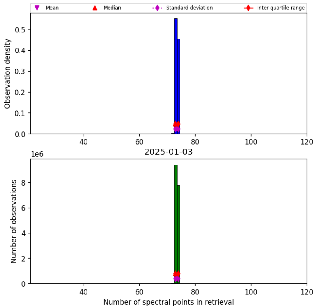
Figure 83: Histogram of “Number of spectral points in retrieval” for 2025-01-03 to 2025-01-04
