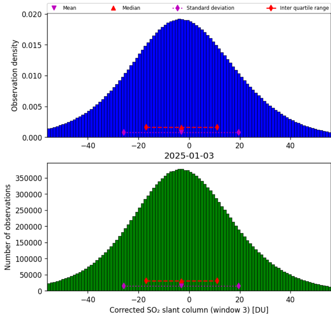
Figure 73: Histogram of “Corrected SO 2 slant column (window 3)” for 2025-01-03 to 2025-01-04
