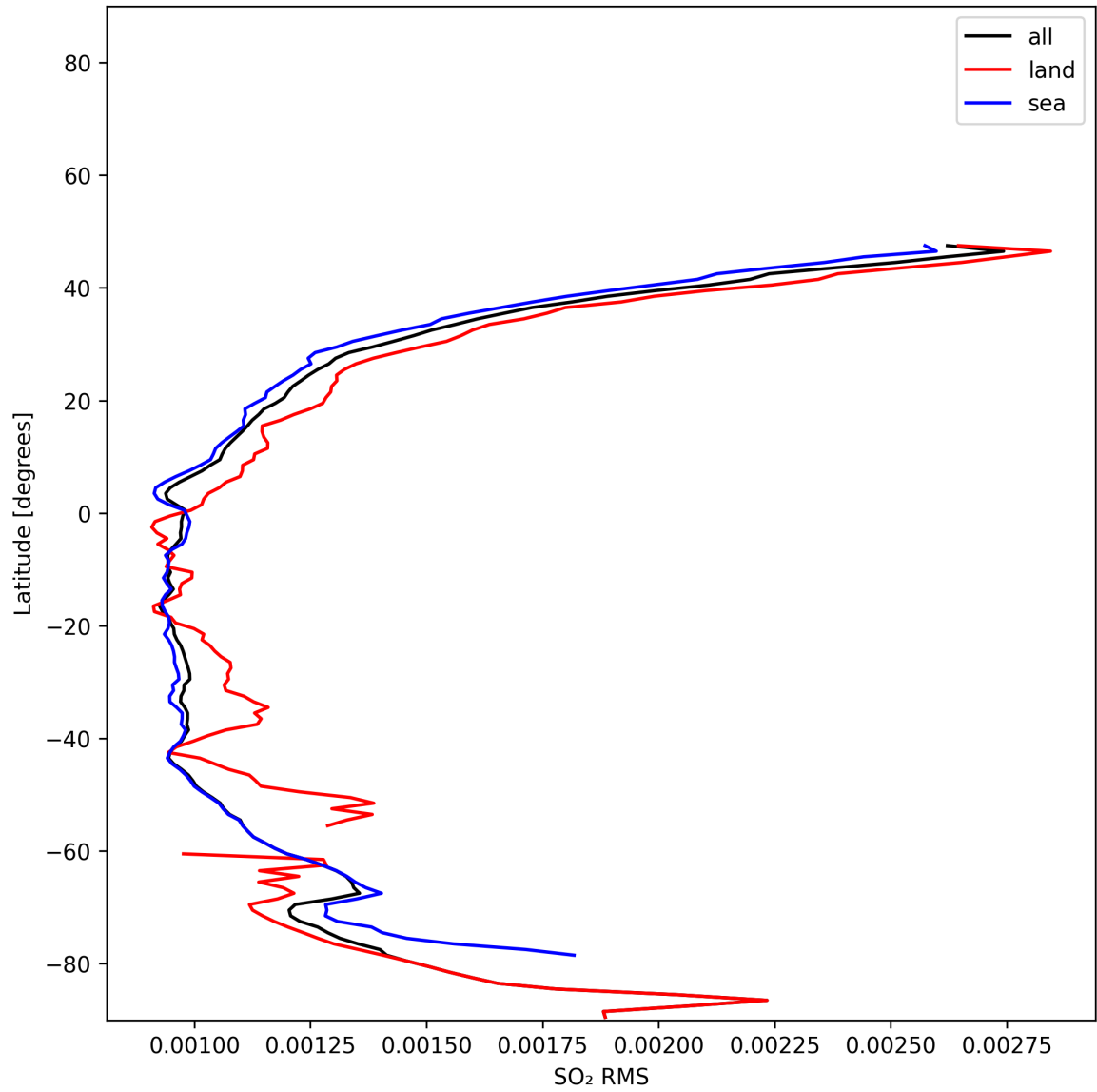
Figure 52: Zonal average of “SO 2 RMS” for 2025-01-03 to 2025-01-04.
