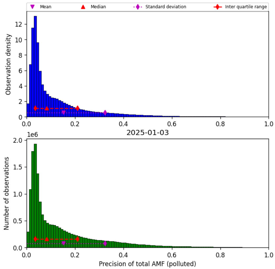
Figure 81: Histogram of “Precision of total AMF (polluted)” for 2025-01-03 to 2025-01-04
