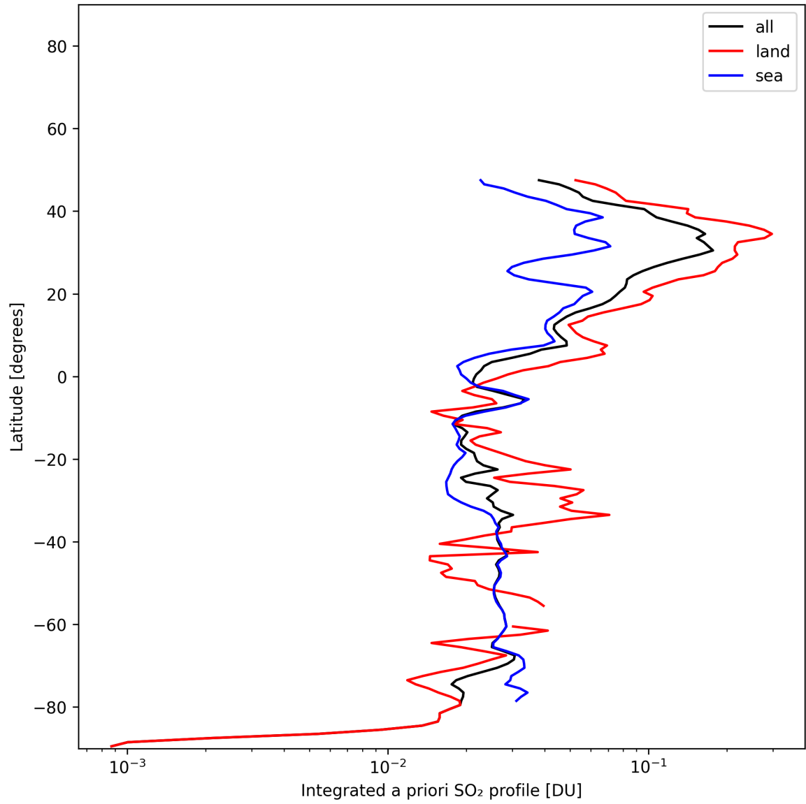
Figure 49: Zonal average of “Integrated a priori SO 2 profile” for 2025-01-03 to 2025-01-04.
