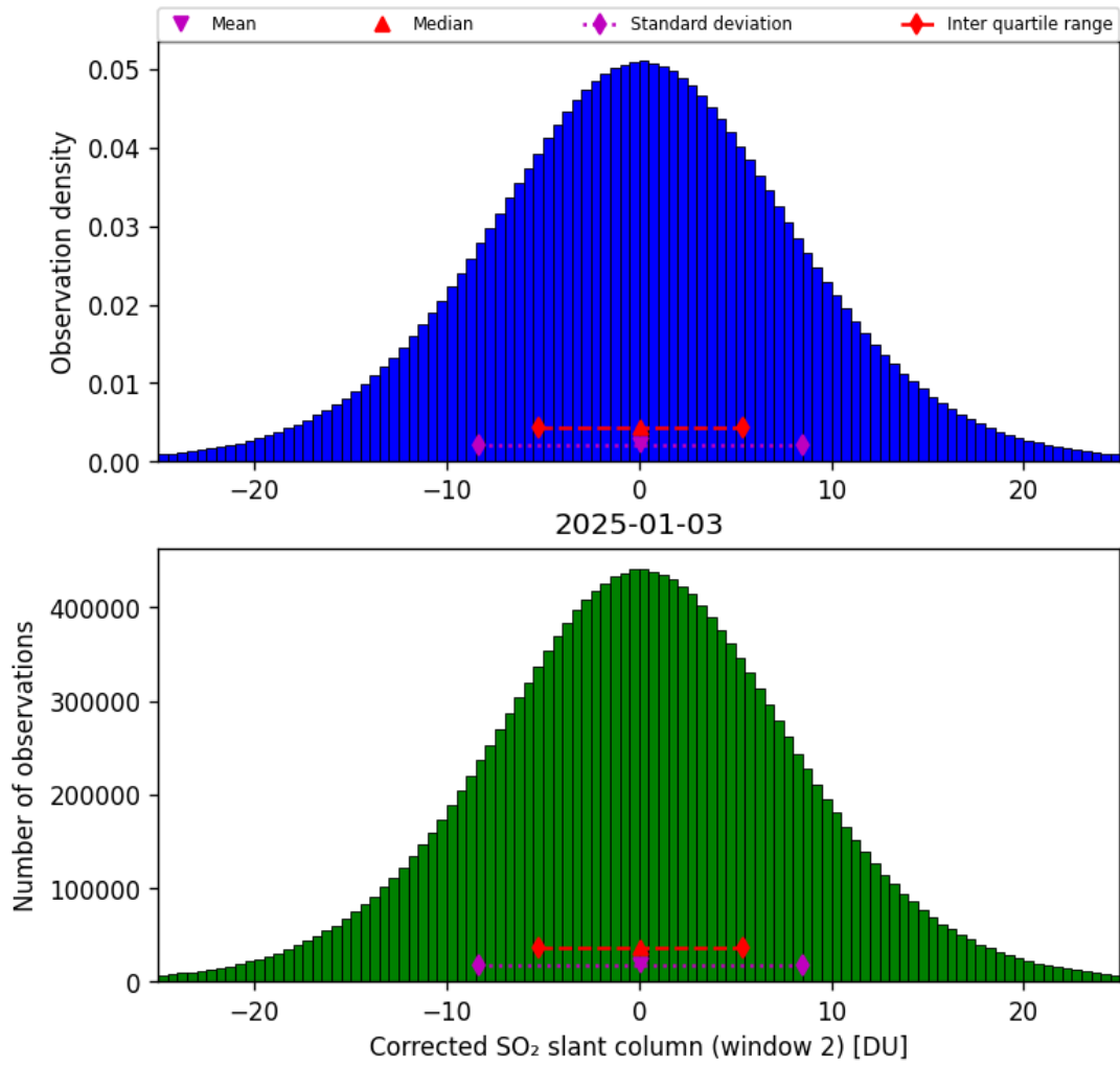
Figure 69: Histogram of “Corrected SO 2 slant column (window 2)” for 2025-01-03 to 2025-01-04
