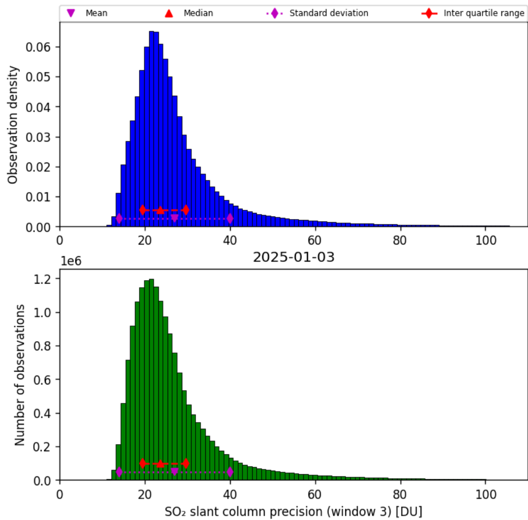
Figure 72: Histogram of “SO 2 slant column precision (window 3)” for 2025-01-03 to 2025-01-04
