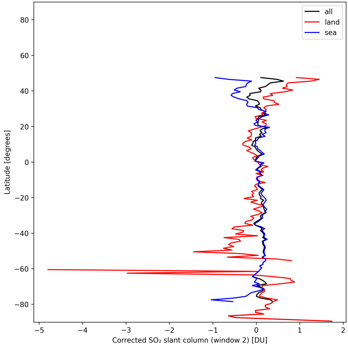
Figure 42: Zonal average of “Corrected SO 2 slant column (window 2)” for 2025-01-03 to 2025-01-04.
