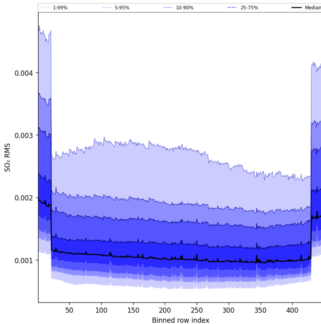
Figure 106: Along track statistics of “SO 2 RMS” for 2025-01-03 to 2025-01-04
