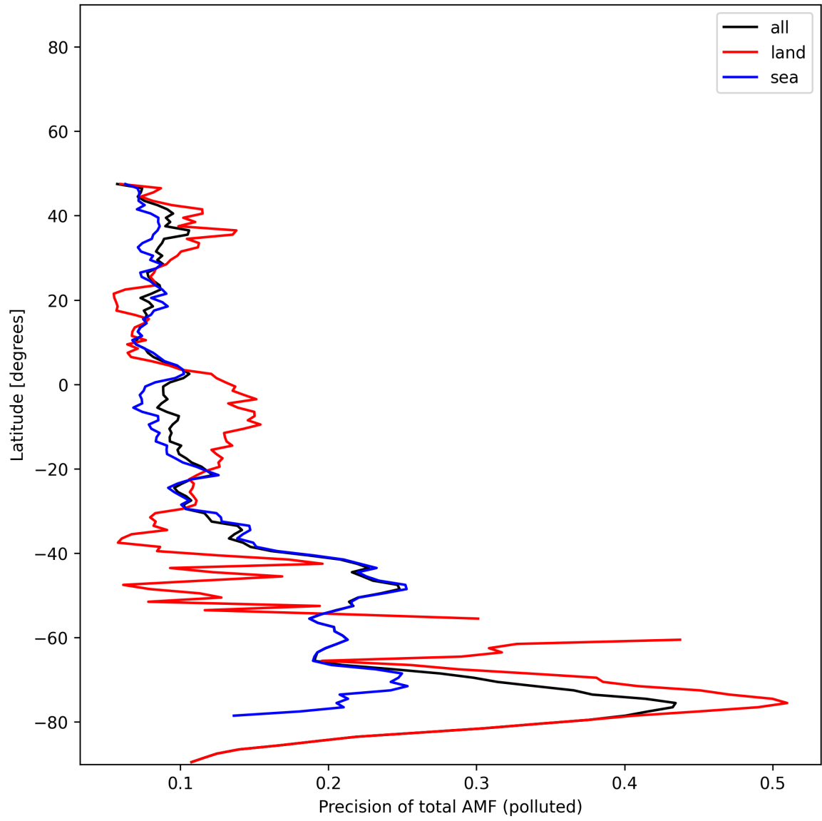
Figure 54: Zonal average of “Precision of total AMF (polluted)” for 2025-01-03 to 2025-01-04.
