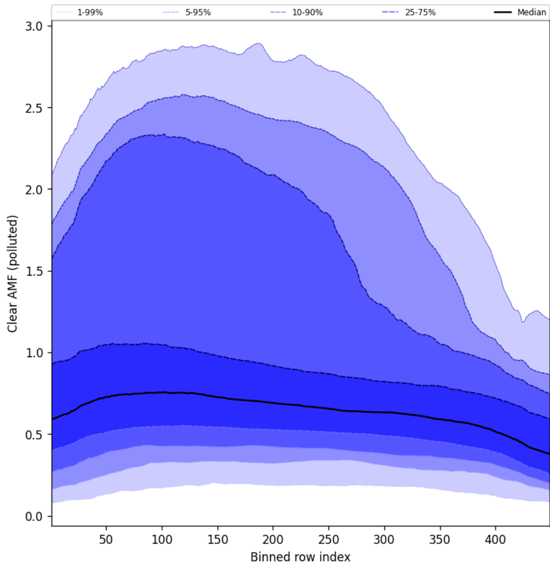
Figure 109: Along track statistics of “Clear AMF (polluted)” for 2025-01-03 to 2025-01-04
