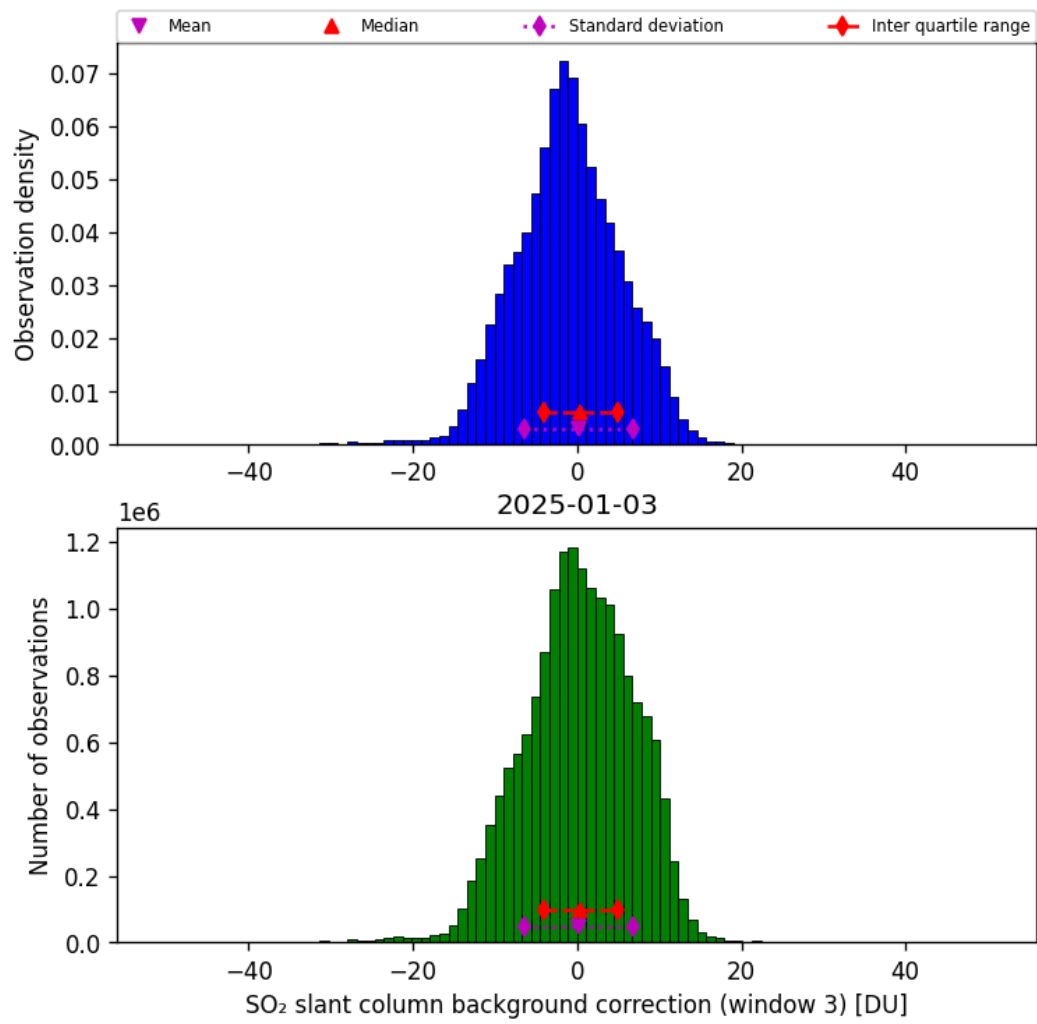
Figure 74: Histogram of “SO 2 slant column background correction (window 3)” for 2025-01-03 to 2025-01-04
