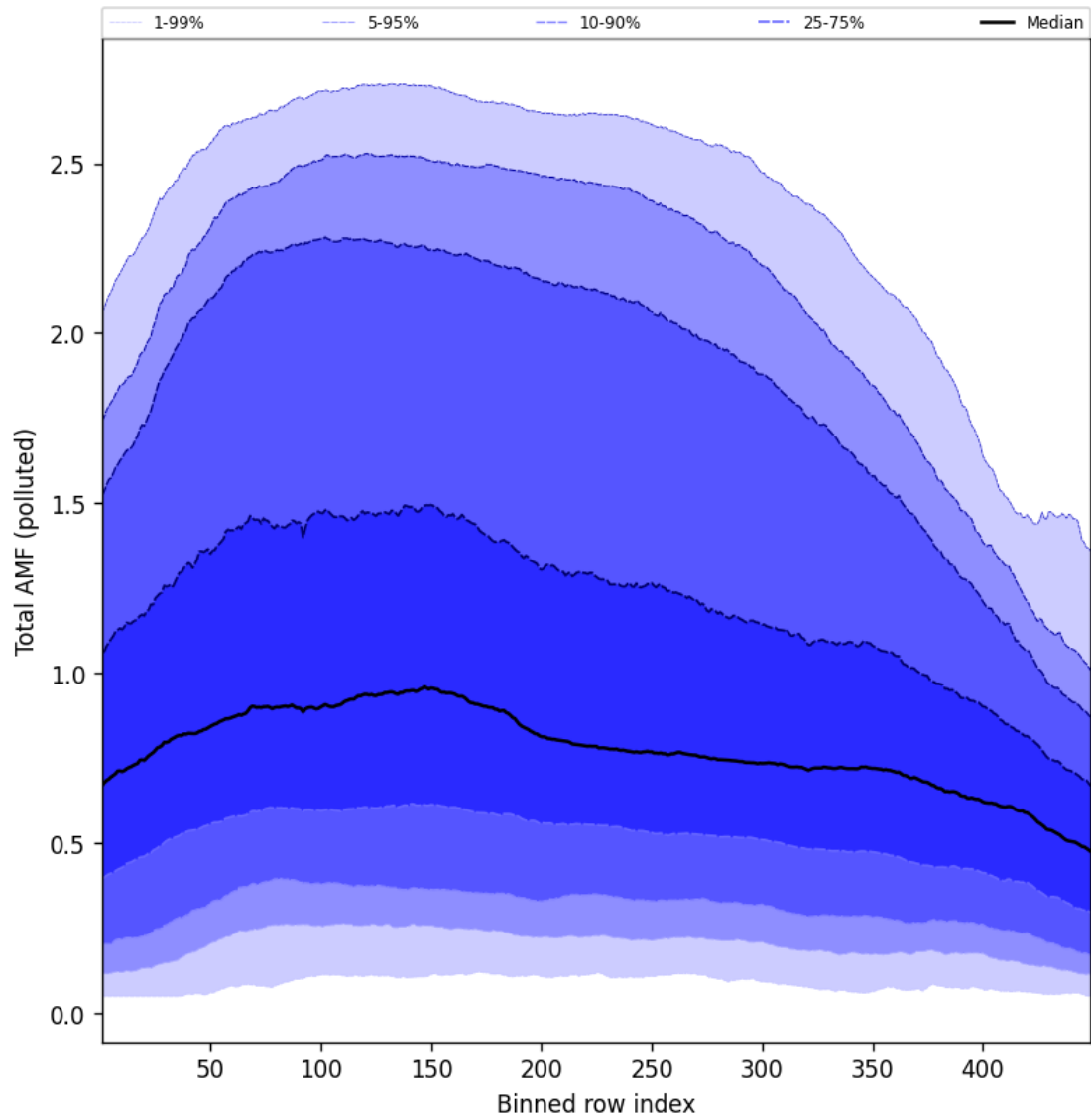
Figure 107: Along track statistics of “Total AMF (polluted)” for 2025-01-03 to 2025-01-04
