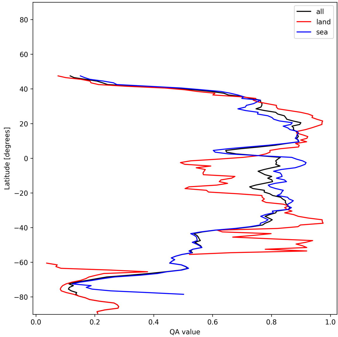
Figure 30: Zonal average of “QA value” for 2025-01-03 to 2025-01-04.
