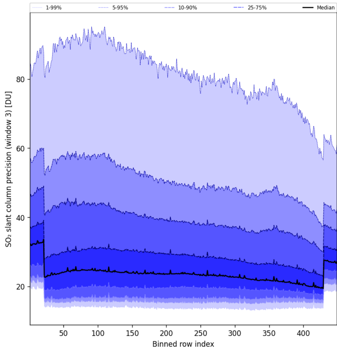
Figure 99: Along track statistics of “SO 2 slant column precision (window 3)” for 2025-01-03 to 2025-01-04
