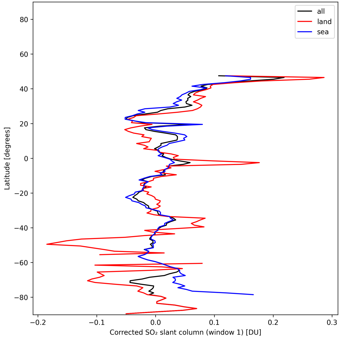
Figure 38: Zonal average of “Corrected SO 2 slant column (window 1)” for 2025-01-03 to 2025-01-04.
