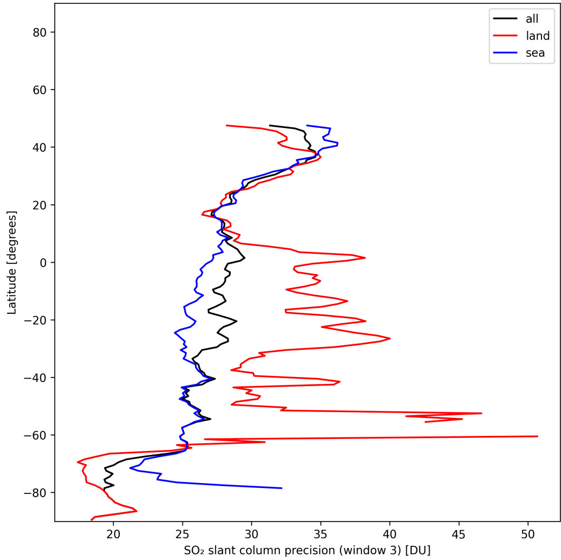
Figure 45: Zonal average of “SO 2 slant column precision (window 3)” for 2025-01-03 to 2025-01-04.
