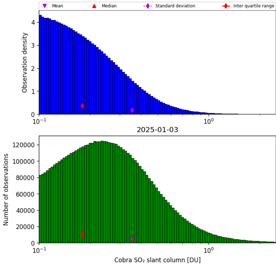
Figure 61: Histogram of “Cobra SO 2 slant column” for 2025-01-03 to 2025-01-04
