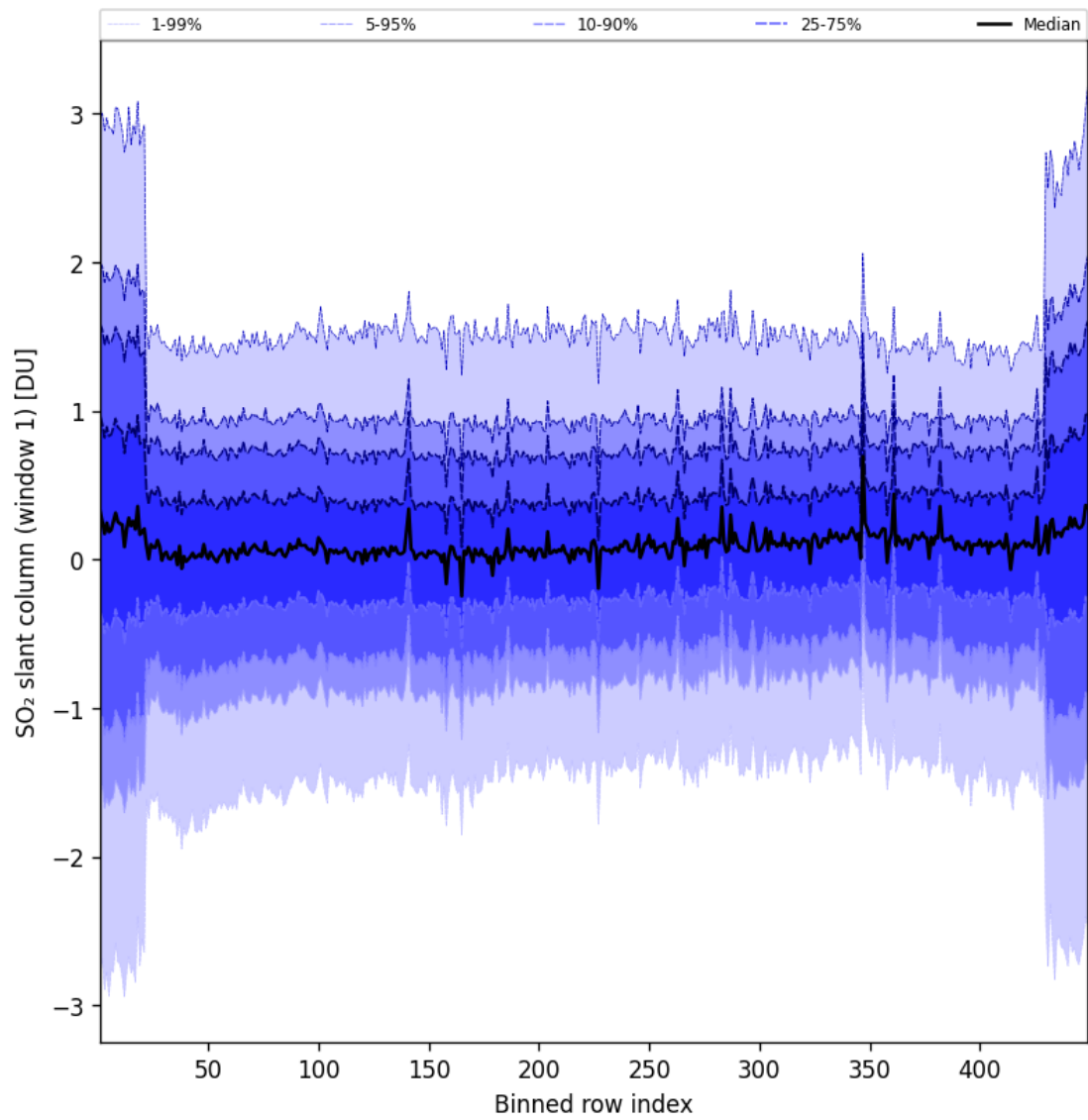
Figure 90: Along track statistics of “SO 2 slant column (window 1)” for 2025-01-03 to 2025-01-04
