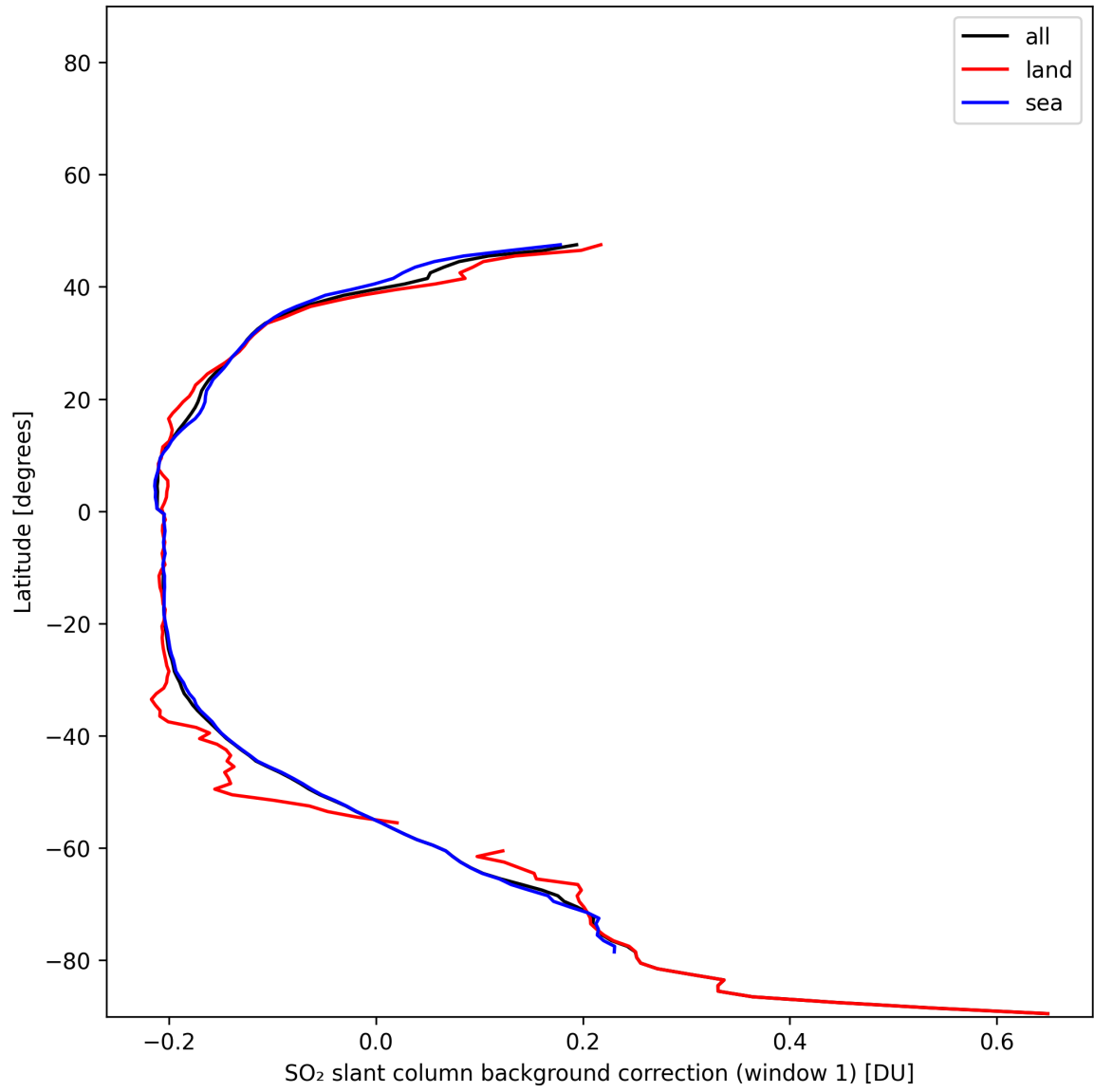
Figure 39: Zonal average of “SO 2 slant column background correction (window 1)” for 2025-01-03 to 2025-01-04.
