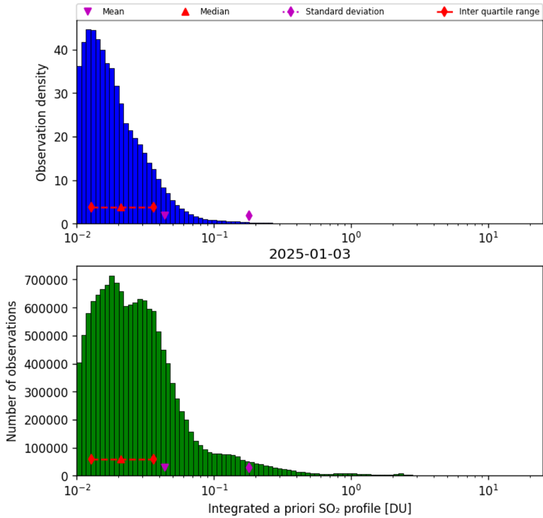
Figure 76: Histogram of “Integrated a priori SO 2 profile” for 2025-01-03 to 2025-01-04
