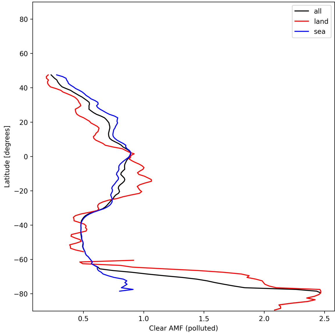
Figure 55: Zonal average of “Clear AMF (polluted)” for 2025-01-03 to 2025-01-04.
