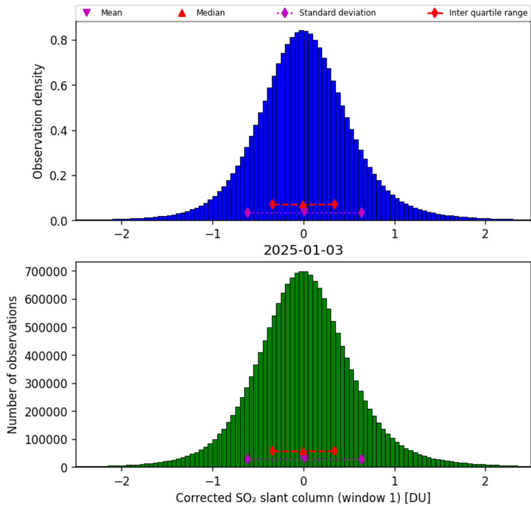
Figure 65: Histogram of “Corrected SO 2 slant column (window 1)” for 2025-01-03 to 2025-01-04
