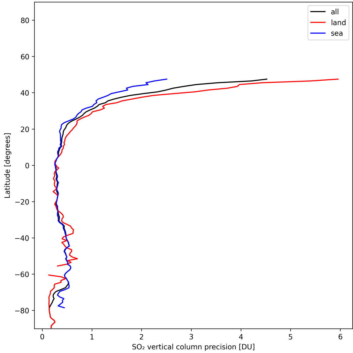
Figure 32: Zonal average of “SO 2 vertical column precision” for 2025-01-03 to 2025-01-04.
