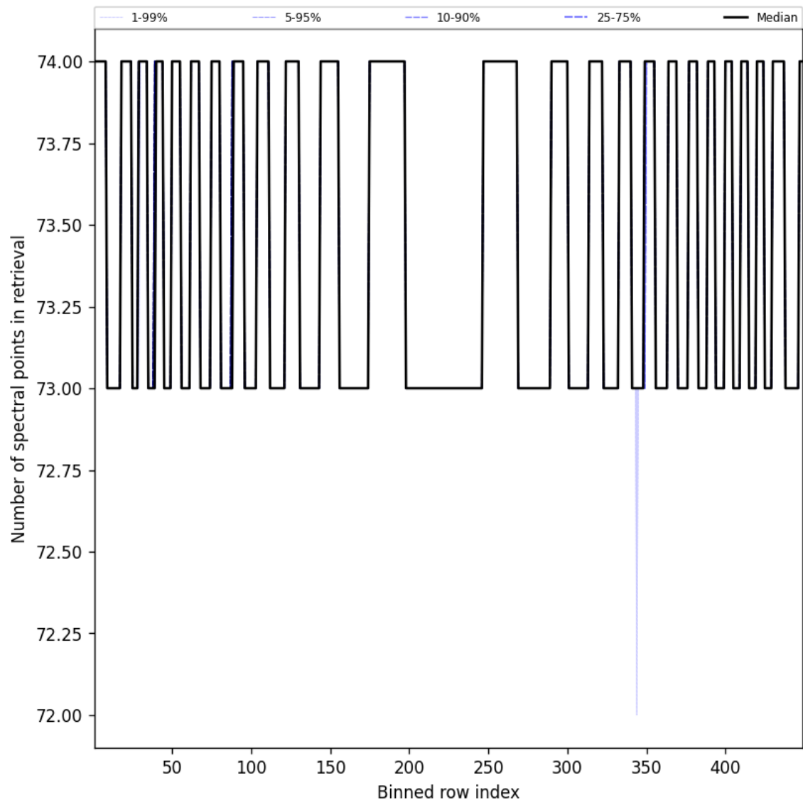
Figure 110: Along track statistics of “Number of spectral points in retrieval” for 2025-01-03 to 2025-01-04
