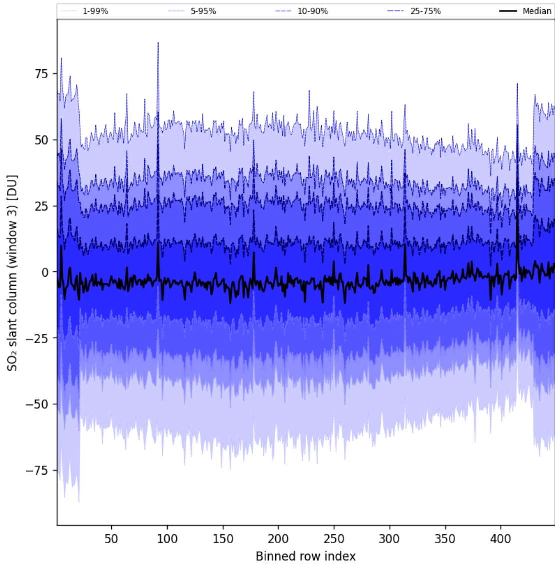
Figure 98: Along track statistics of “SO 2 slant column (window 3)” for 2025-01-03 to 2025-01-04
