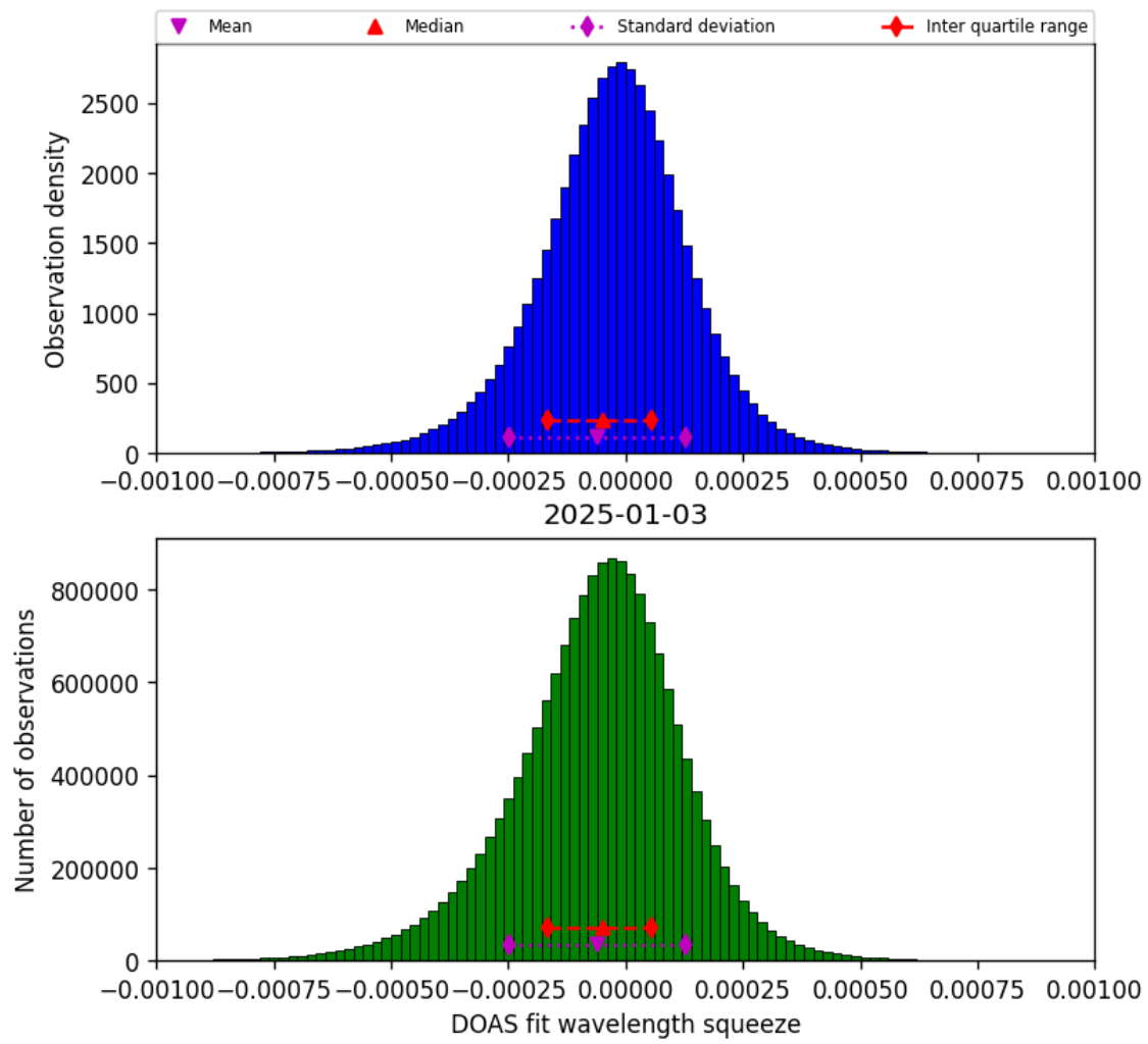
Figure 78: Histogram of “DOAS fit wavelength squeeze” for 2025-01-03 to 2025-01-04
