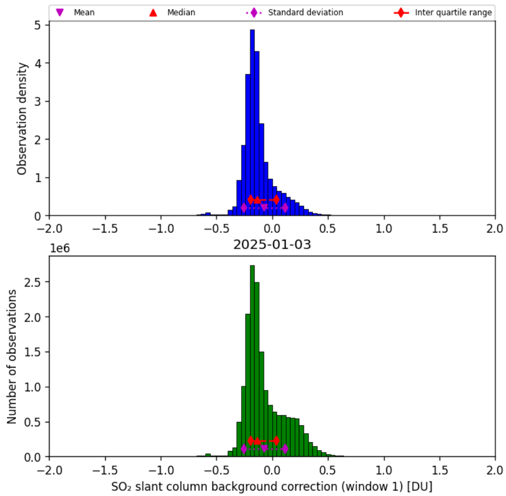
Figure 66: Histogram of “SO 2 slant column background correction (window 1)” for 2025-01-03 to 2025-01-04
