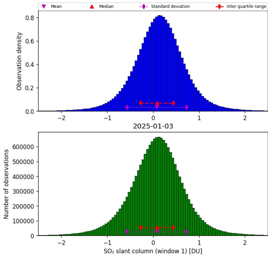
Figure 63: Histogram of “SO 2 slant column (window 1)” for 2025-01-03 to 2025-01-04
