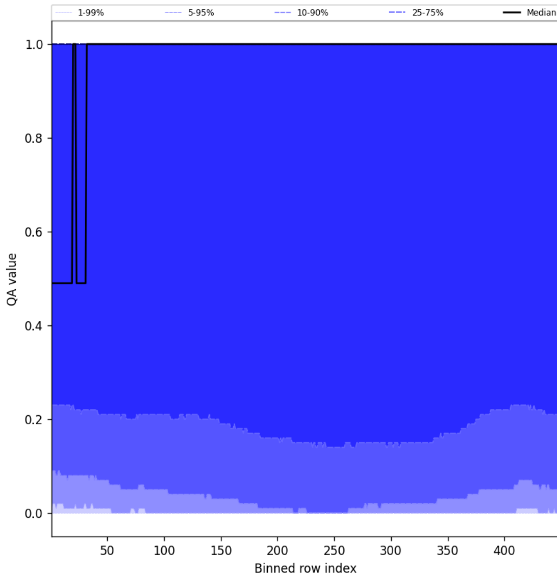
Figure 84: Along track statistics of “QA value” for 2025-01-03 to 2025-01-04
