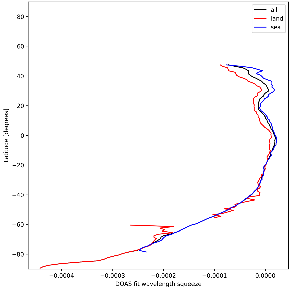
Figure 51: Zonal average of “DOAS fit wavelength squeeze” for 2025-01-03 to 2025-01-04.
