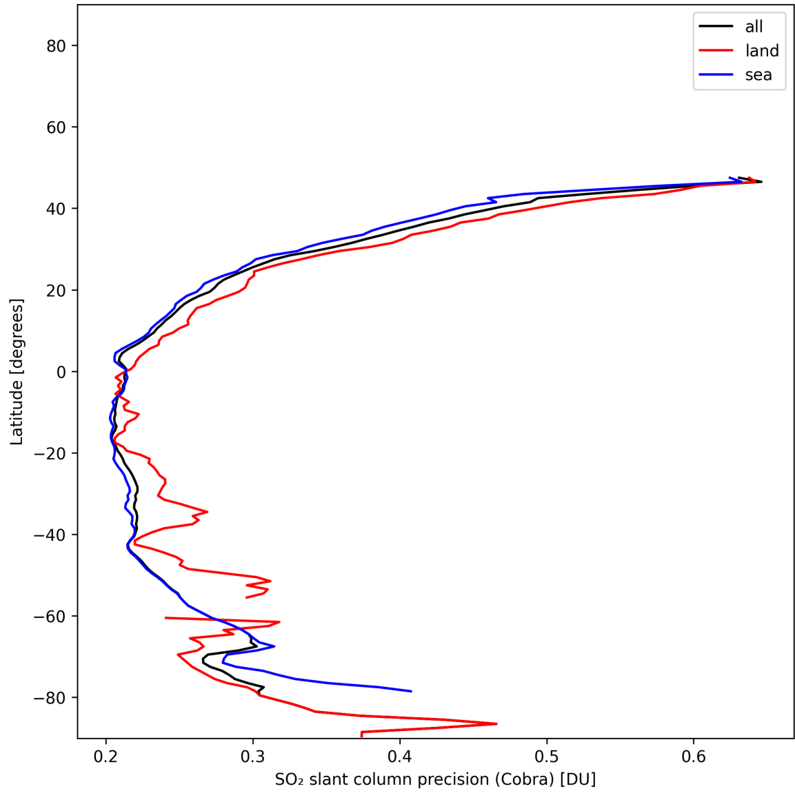
Figure 35: Zonal average of “SO 2 slant column precision (Cobra)” for 2025-01-03 to 2025-01-04.
