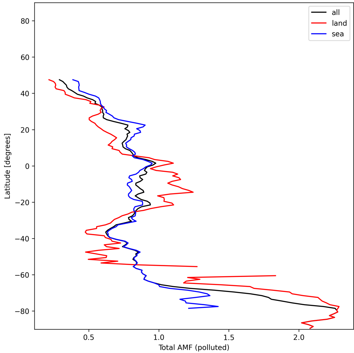
Figure 53: Zonal average of “Total AMF (polluted)” for 2025-01-03 to 2025-01-04.
