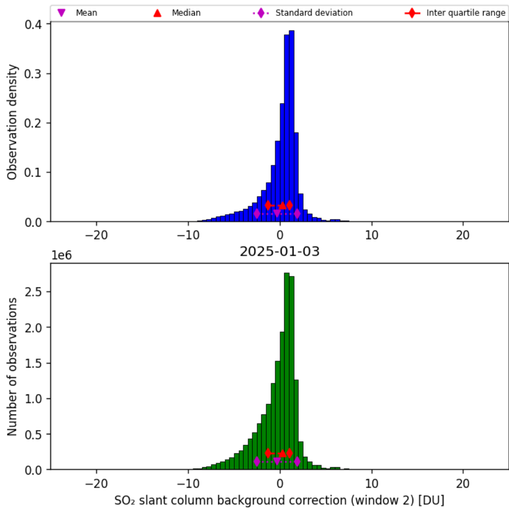
Figure 70: Histogram of “SO 2 slant column background correction (window 2)” for 2025-01-03 to 2025-01-04
