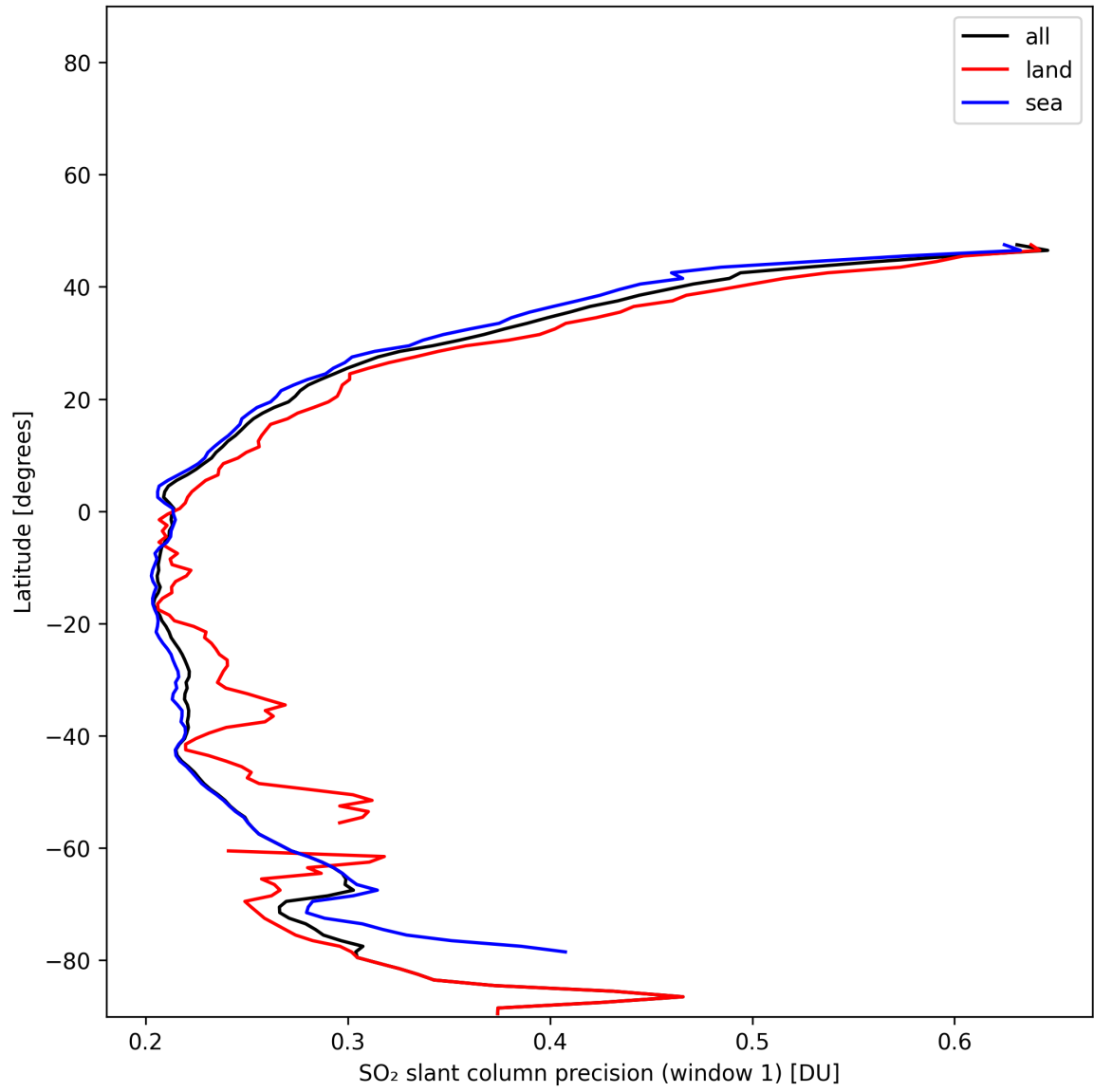
Figure 37: Zonal average of “SO 2 slant column precision (window 1)” for 2025-01-03 to 2025-01-04.
