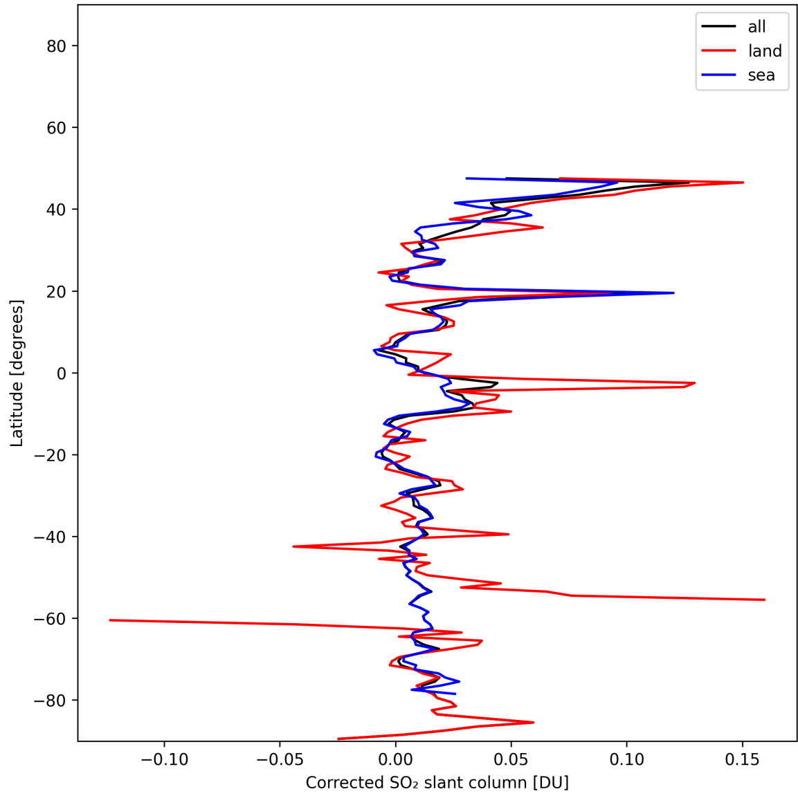
Figure 33: Zonal average of “Corrected SO 2 slant column” for 2025-01-03 to 2025-01-04.
