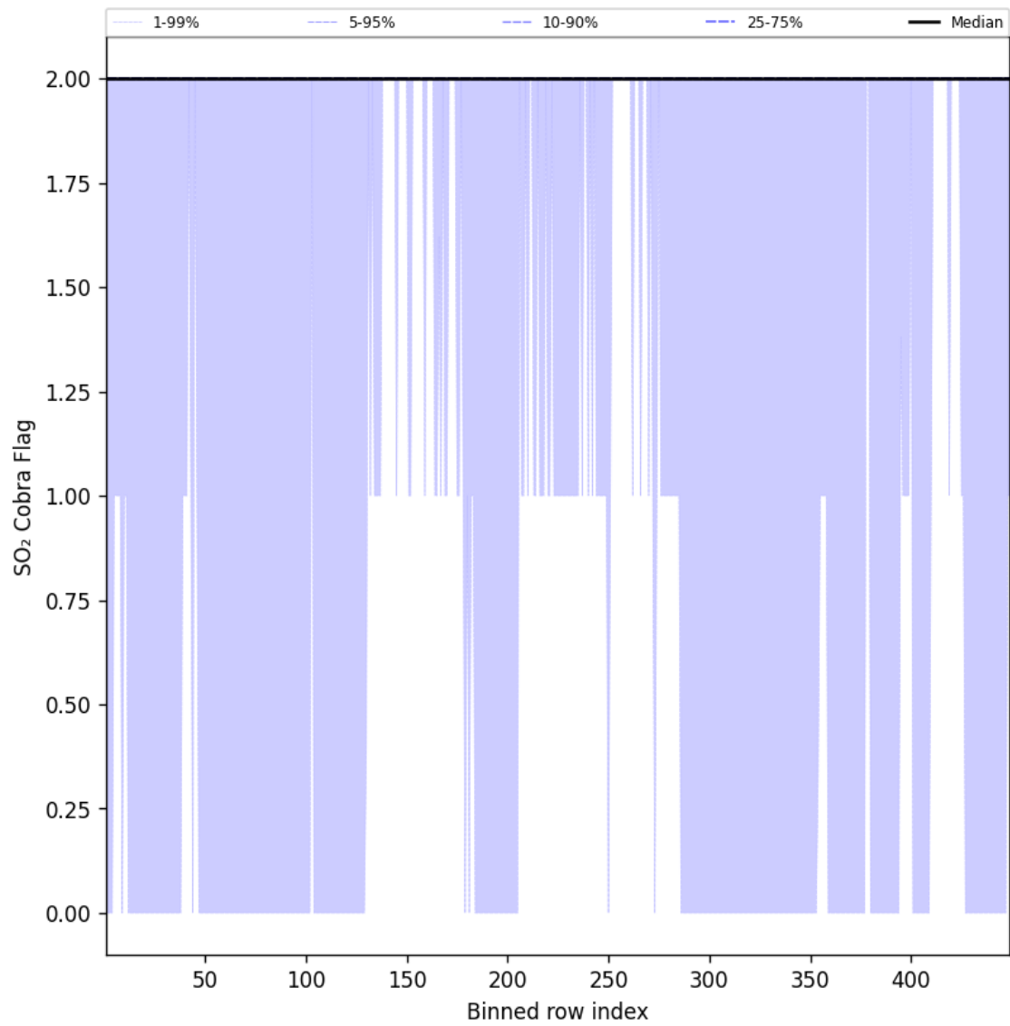
Figure 102: Along track statistics of “SO 2 Cobra Flag” for 2025-01-03 to 2025-01-04
