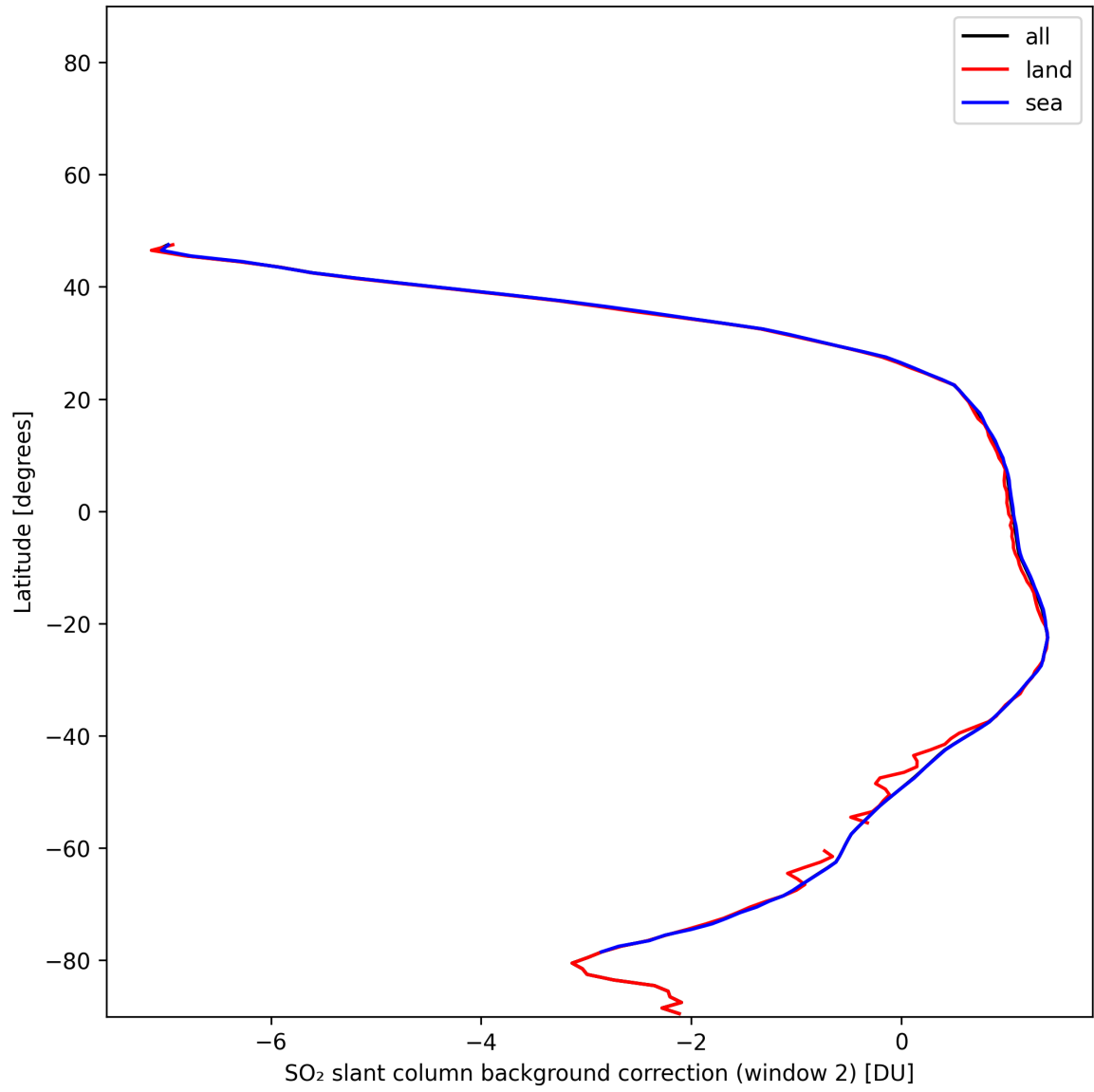
Figure 43: Zonal average of “SO 2 slant column background correction (window 2)” for 2025-01-03 to 2025-01-04.
