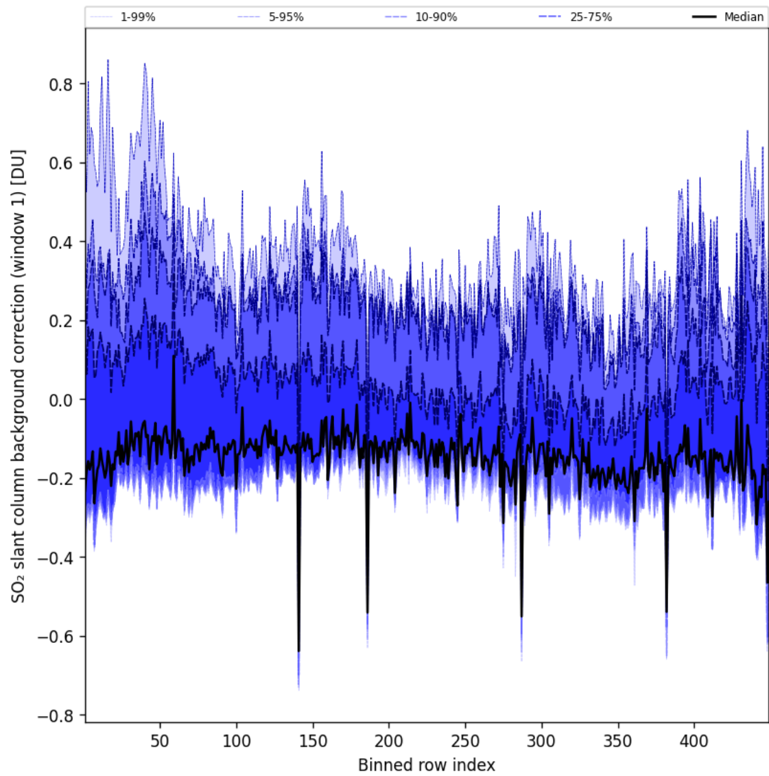
Figure 93: Along track statistics of “SO 2 slant column background correction (window 1)” for 2025-01-03 to 2025-01-04
