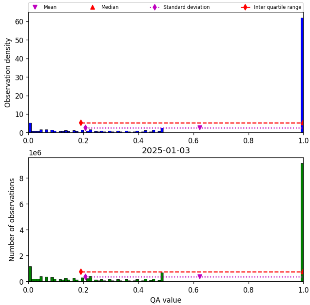
Figure 57: Histogram of “QA value” for 2025-01-03 to 2025-01-04
