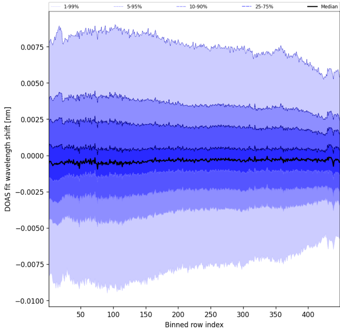
Figure 104: Along track statistics of “DOAS fit wavelength shift” for 2025-01-03 to 2025-01-04
