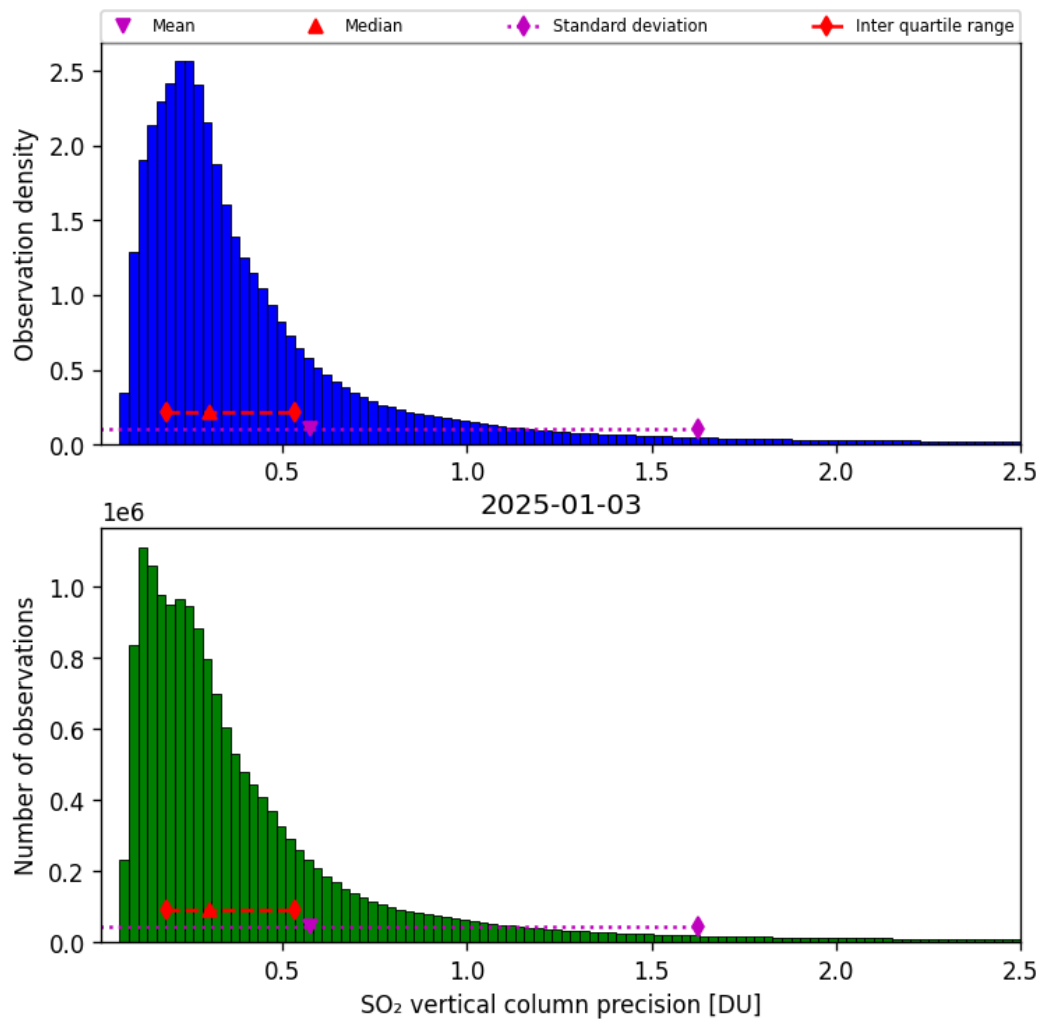
Figure 59: Histogram of "SO 2 vertical column precision" for 2025-01-03 to 2025-01-04
