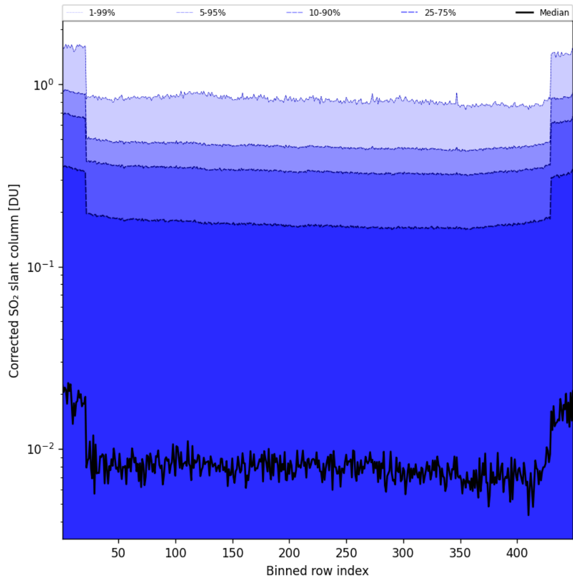
Figure 87: Along track statistics of “Corrected SO 2 slant column” for 2025-01-03 to 2025-01-04
