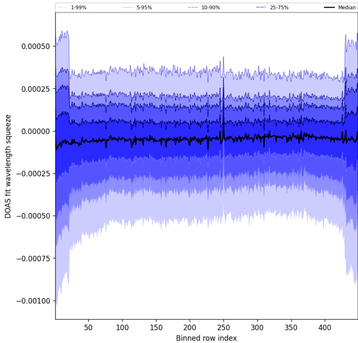
Figure 105: Along track statistics of “DOAS fit wavelength squeeze” for 2025-01-03 to 2025-01-04
