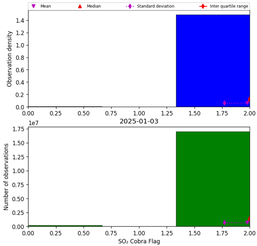
Figure 75: Histogram of “SO 2 Cobra Flag” for 2025-01-03 to 2025-01-04
