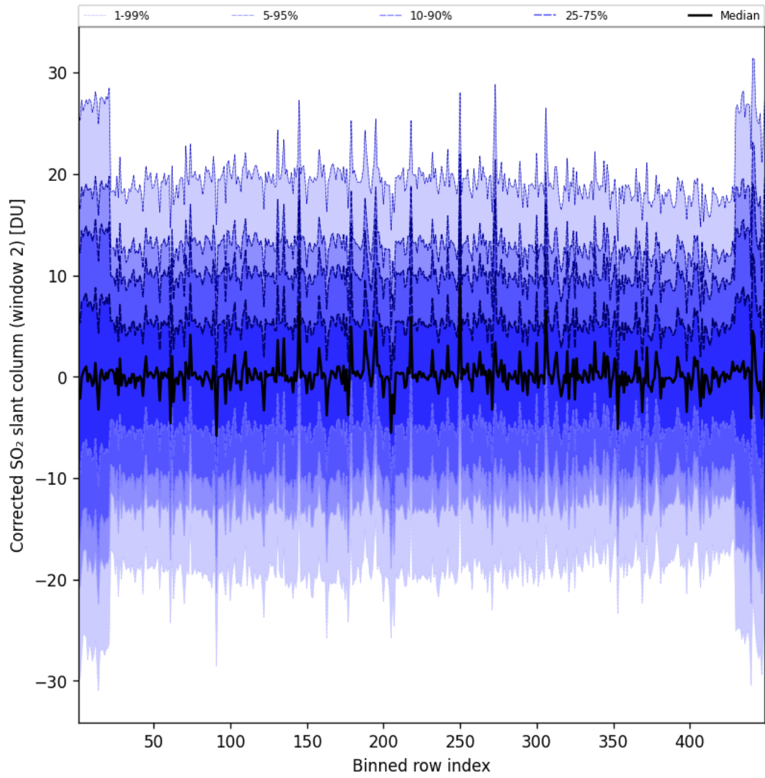
Figure 96: Along track statistics of “Corrected SO 2 slant column (window 2)” for 2025-01-03 to 2025-01-04
