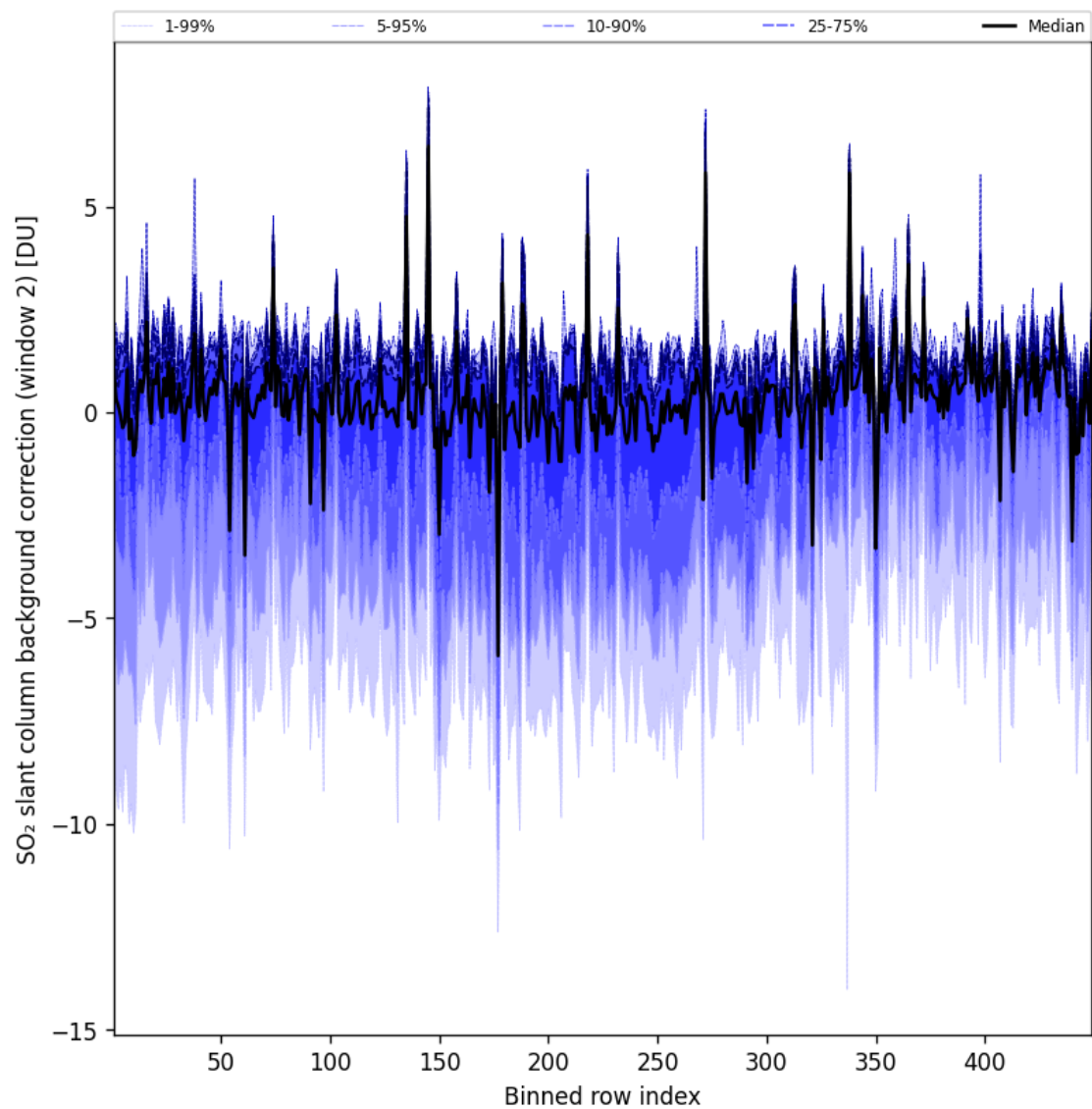
Figure 97: Along track statistics of “SO 2 slant column background correction (window 2)” for 2025-01-03 to 2025-01-04
