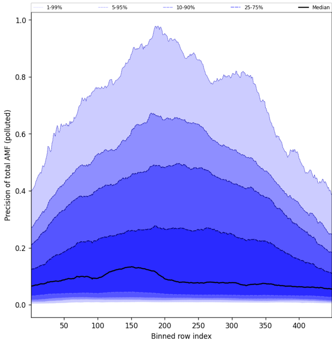
Figure 108: Along track statistics of “Precision of total AMF (polluted)” for 2025-01-03 to 2025-01-04
