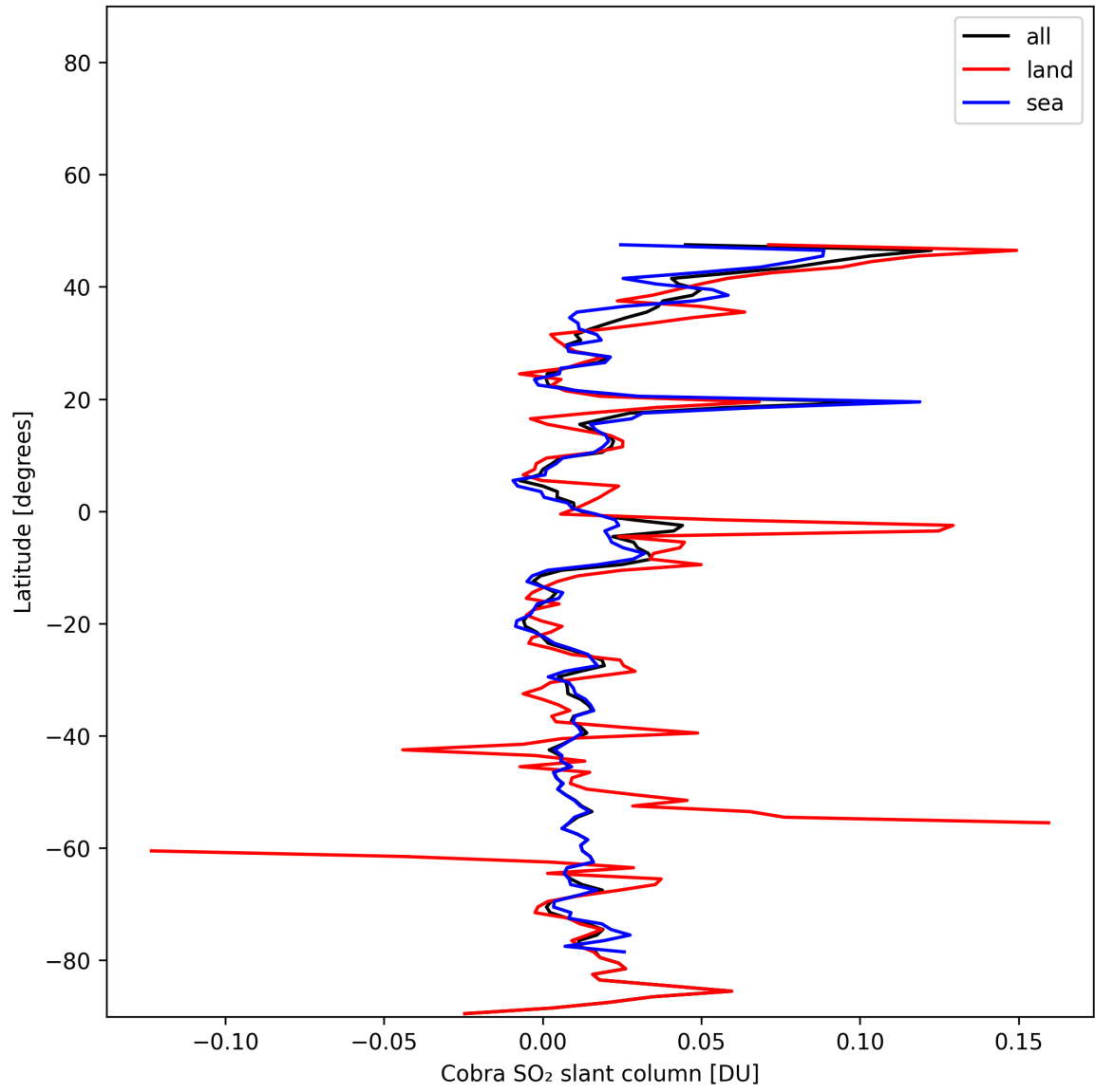
Figure 34: Zonal average of “Cobra SO 2 slant column” for 2025-01-03 to 2025-01-04.
