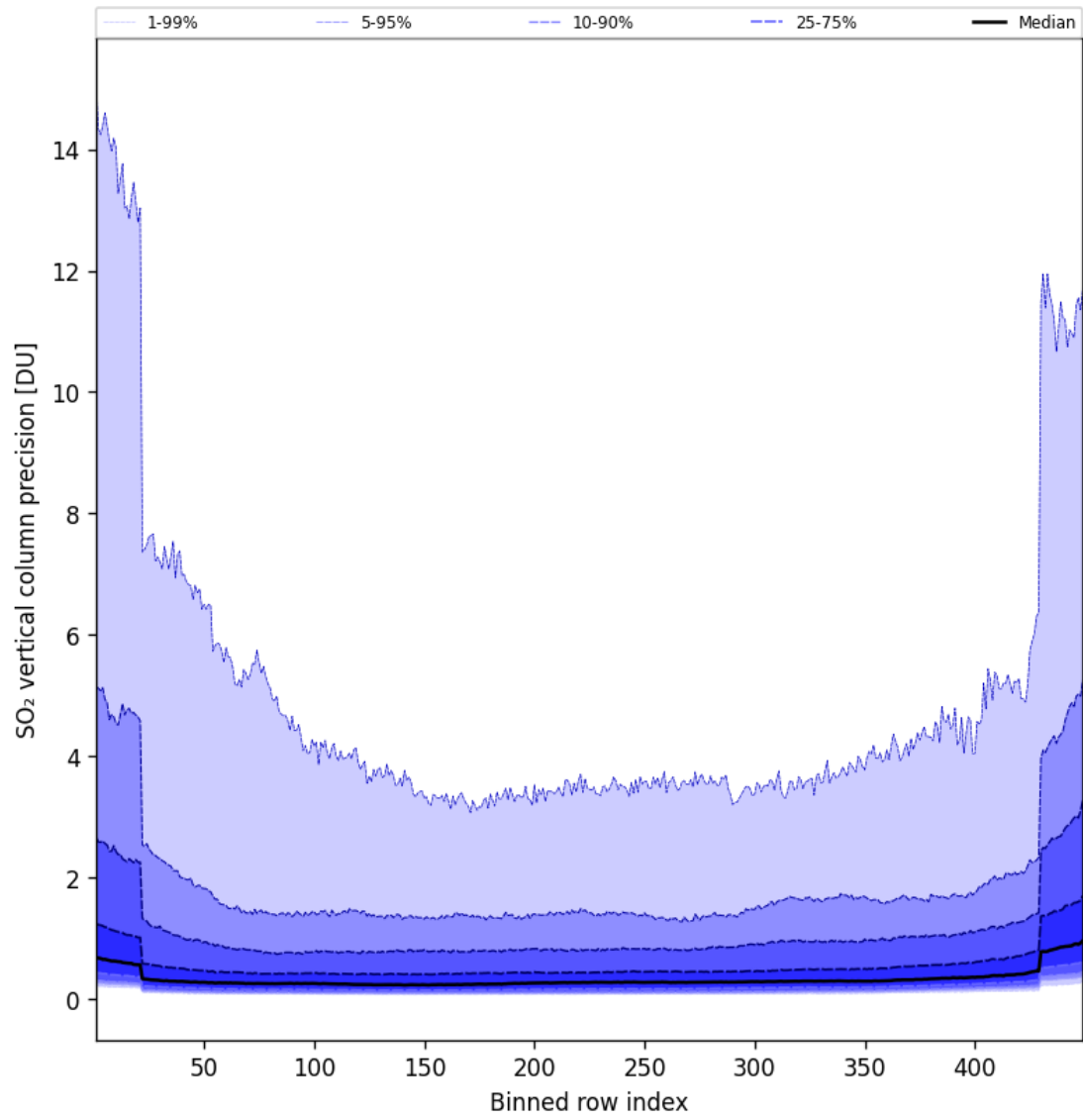
Figure 86: Along track statistics of “SO 2 vertical column precision” for 2025-01-03 to 2025-01-04
