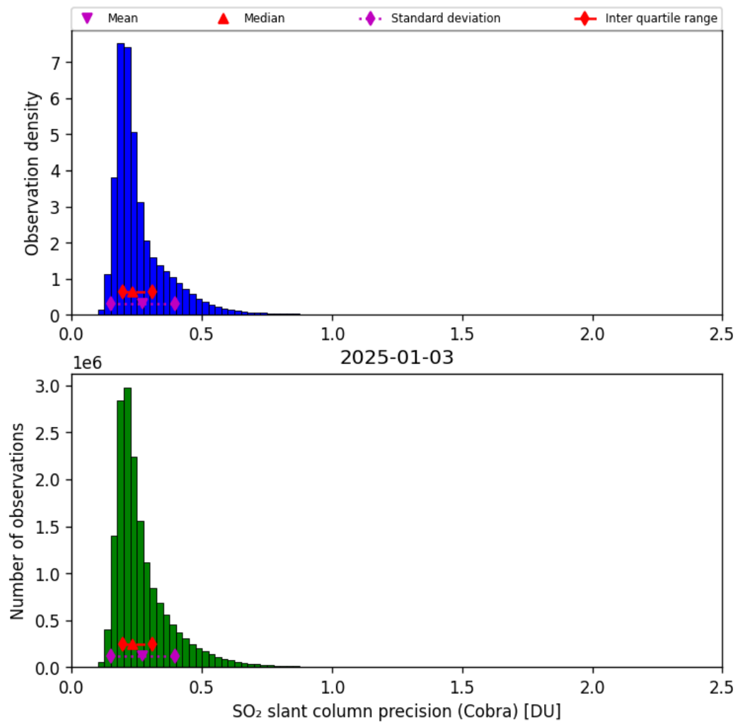
Figure 62: Histogram of “SO 2 slant column precision (Cobra)” for 2025-01-03 to 2025-01-04
