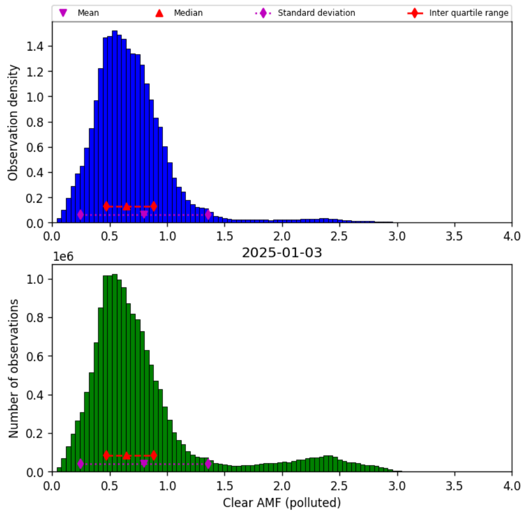
Figure 82: Histogram of “Clear AMF (polluted)” for 2025-01-03 to 2025-01-04
