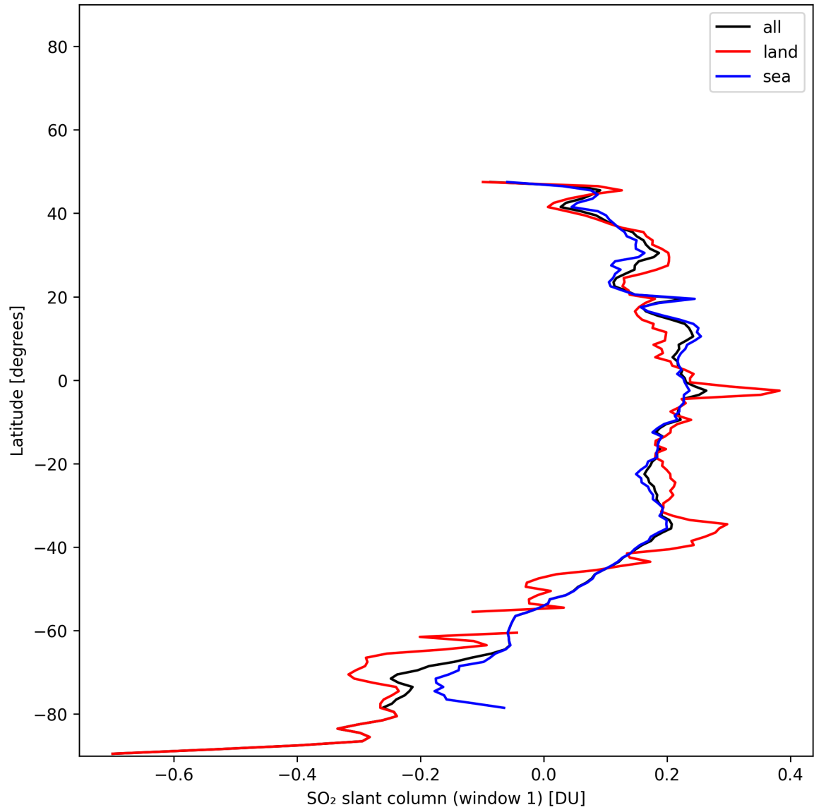
Figure 36: Zonal average of “SO 2 slant column (window 1)” for 2025-01-03 to 2025-01-04.
