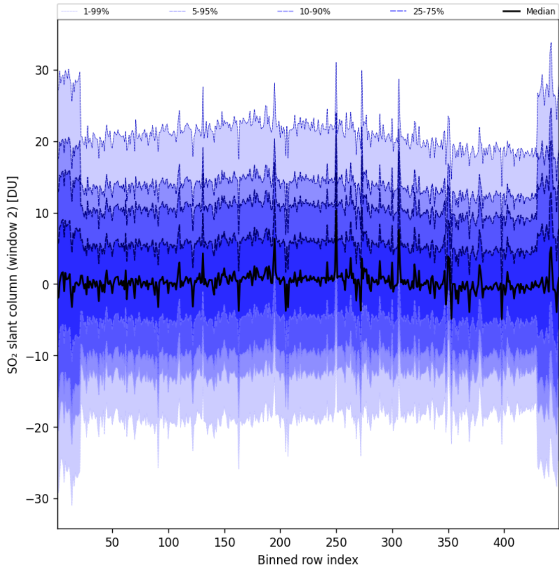
Figure 94: Along track statistics of “SO 2 slant column (window 2)” for 2025-01-03 to 2025-01-04
