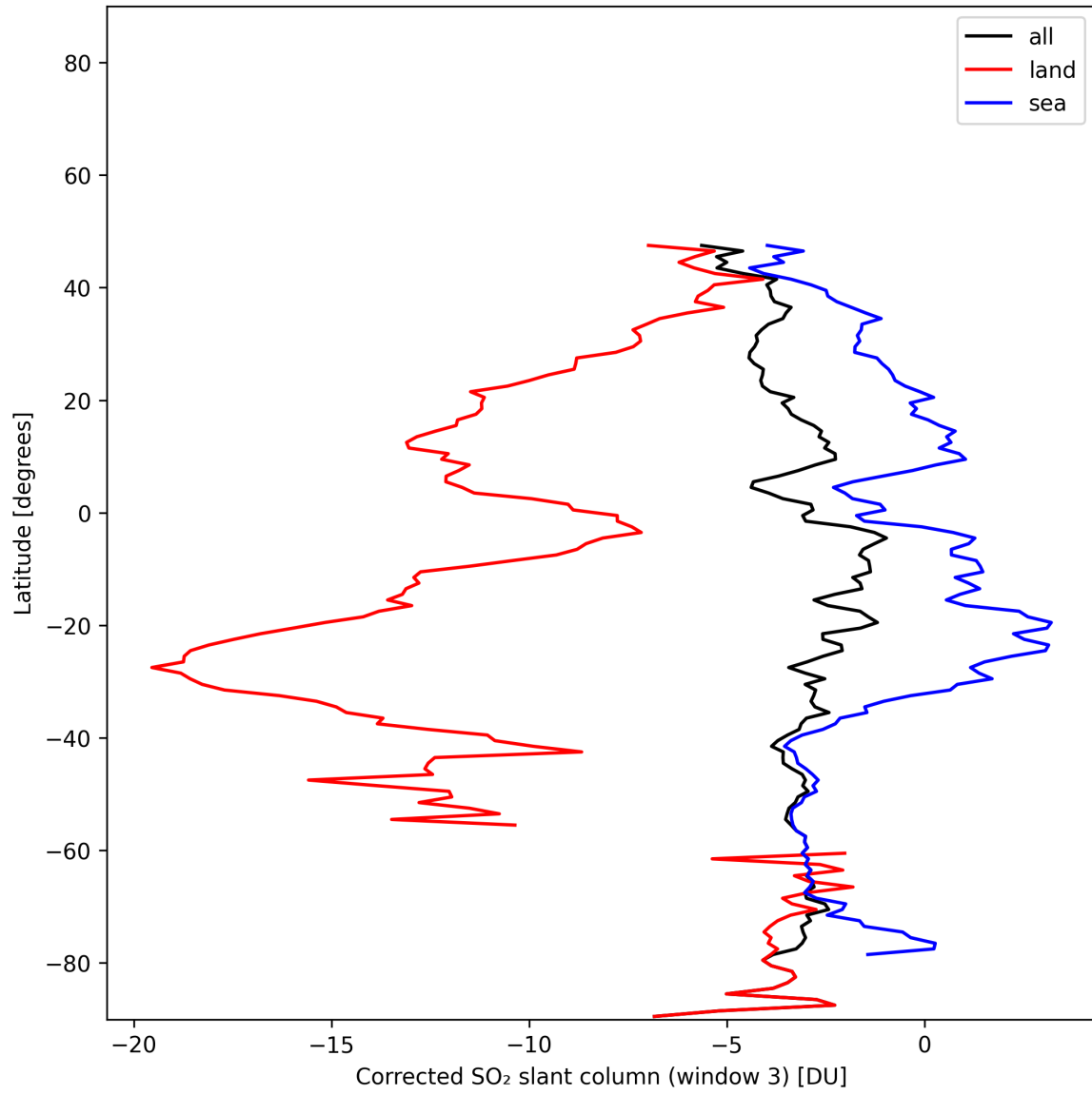
Figure 46: Zonal average of “Corrected SO 2 slant column (window 3)” for 2025-01-03 to 2025-01-04.
