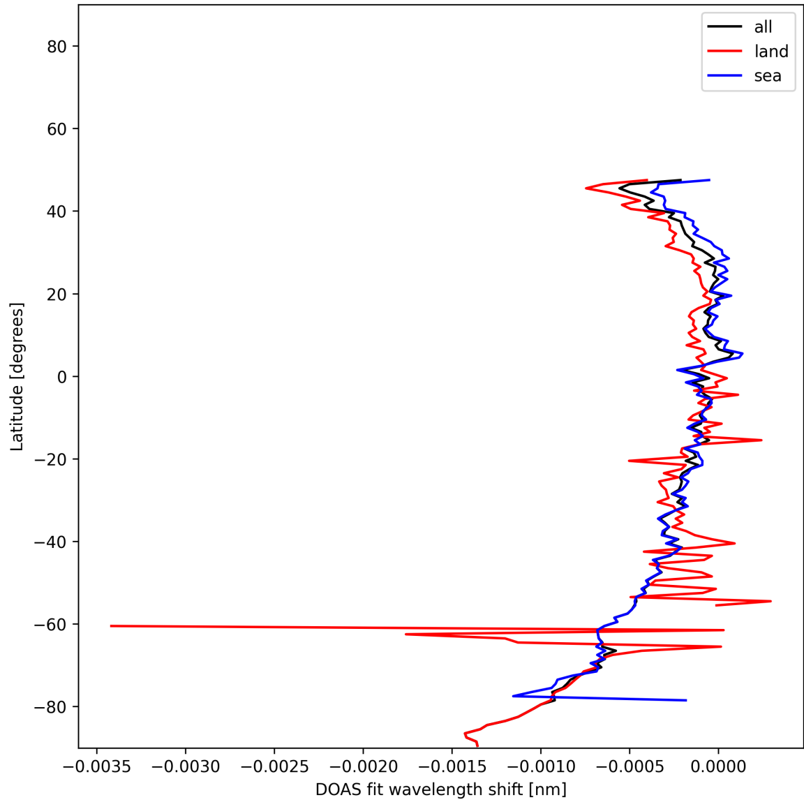
Figure 50: Zonal average of “DOAS fit wavelength shift” for 2025-01-03 to 2025-01-04.
