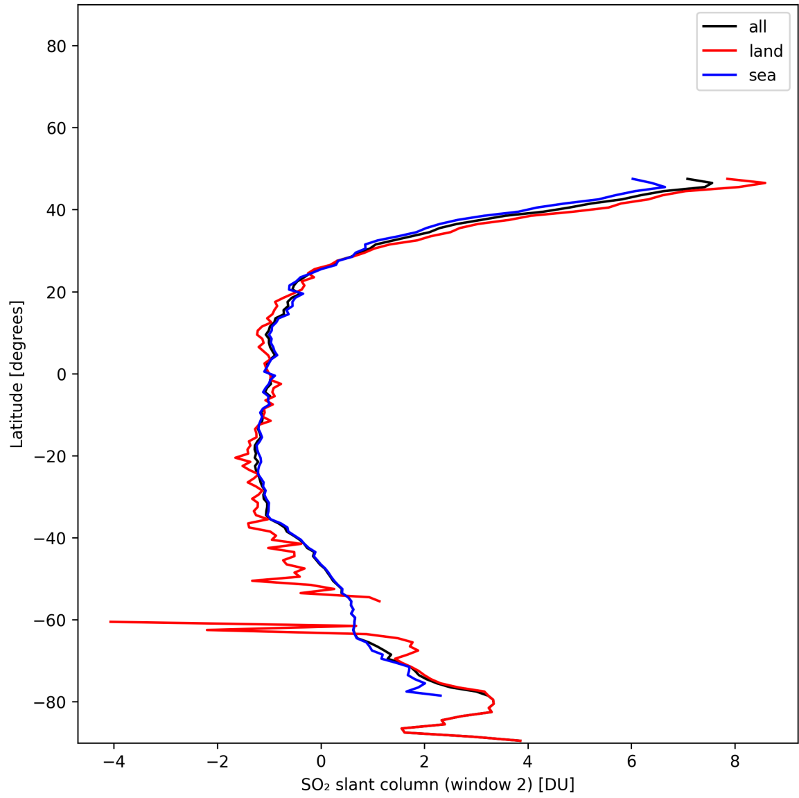
Figure 40: Zonal average of “SO 2 slant column (window 2)” for 2025-01-03 to 2025-01-04.
