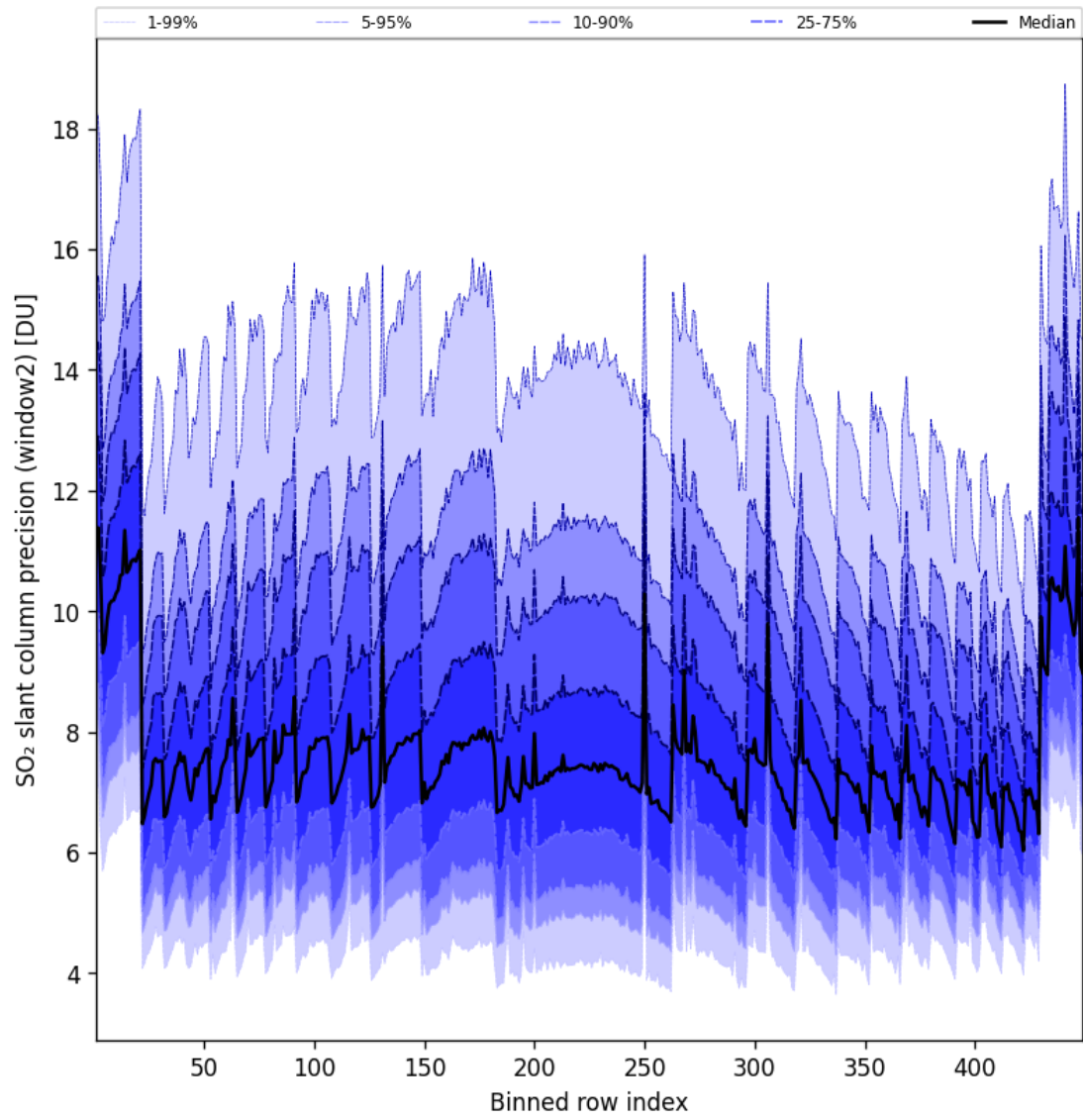
Figure 95: Along track statistics of “SO 2 slant column precision (window2)” for 2025-01-03 to 2025-01-04
