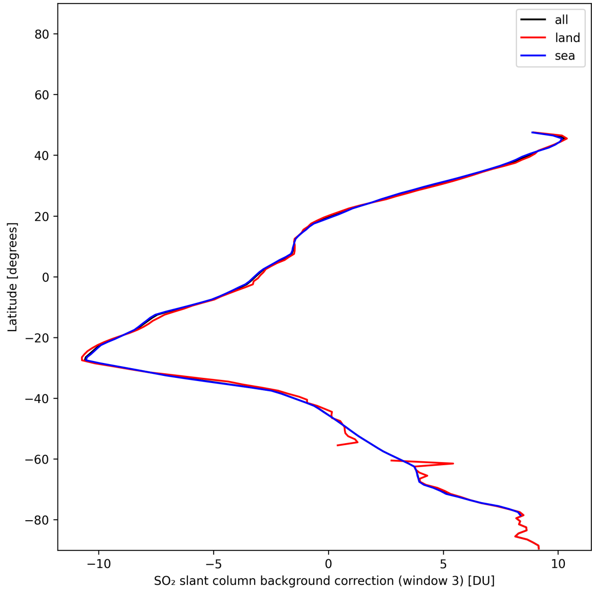
Figure 47: Zonal average of “SO 2 slant column background correction (window 3)” for 2025-01-03 to 2025-01-04.
