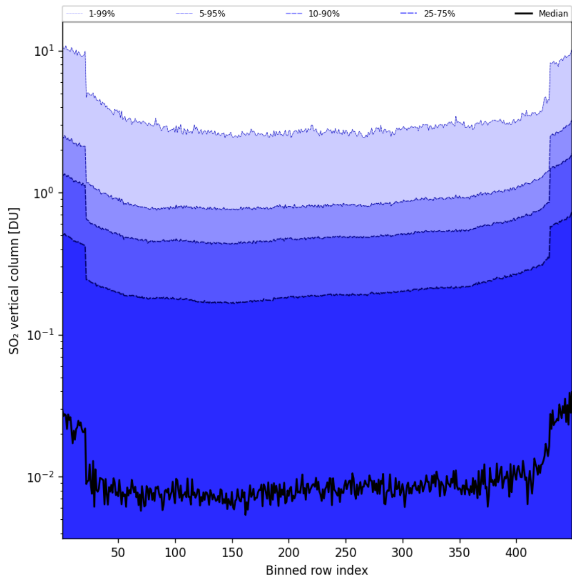
Figure 85: Along track statistics of “SO 2 vertical column” for 2025-01-03 to 2025-01-04
