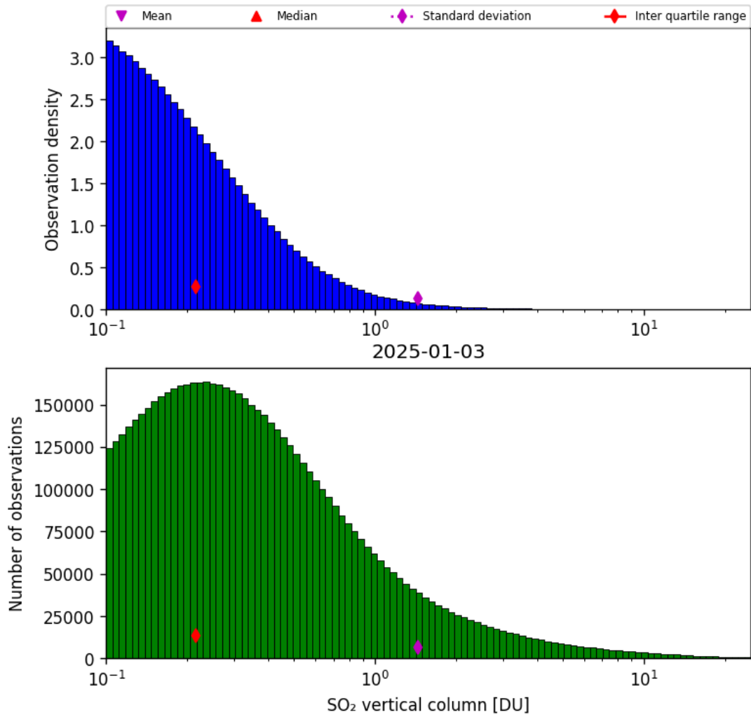
Figure 58: Histogram of “SO 2 vertical column” for 2025-01-03 to 2025-01-04
