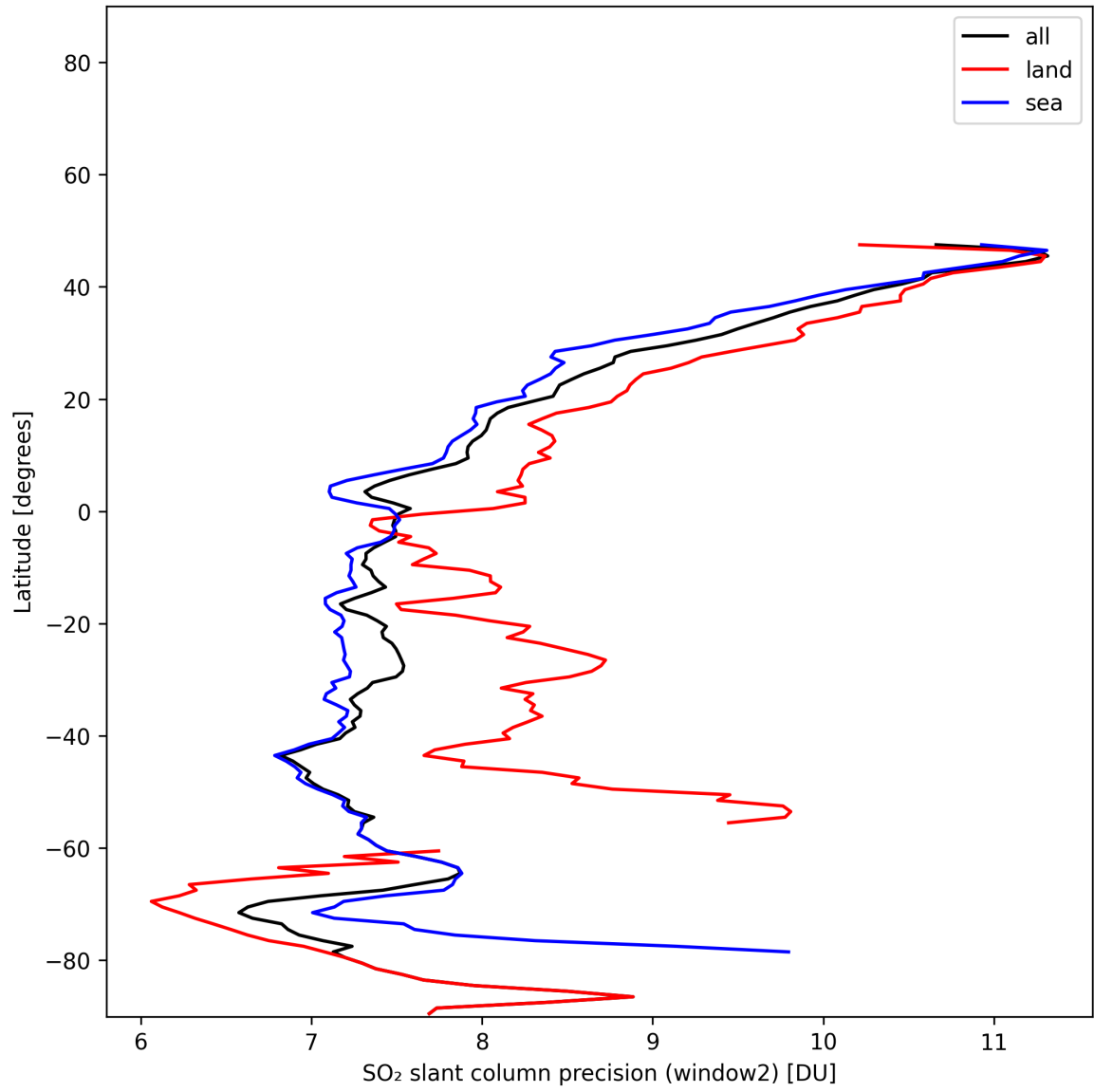
Figure 41: Zonal average of “SO 2 slant column precision (window2)” for 2025-01-03 to 2025-01-04.
