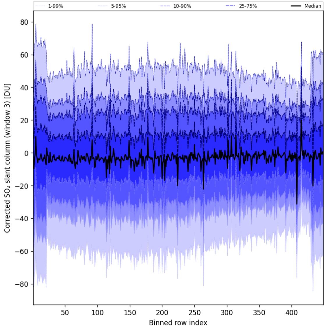
Figure 100: Along track statistics of “Corrected SO 2 slant column (window 3)” for 2025-01-03 to 2025-01-04
