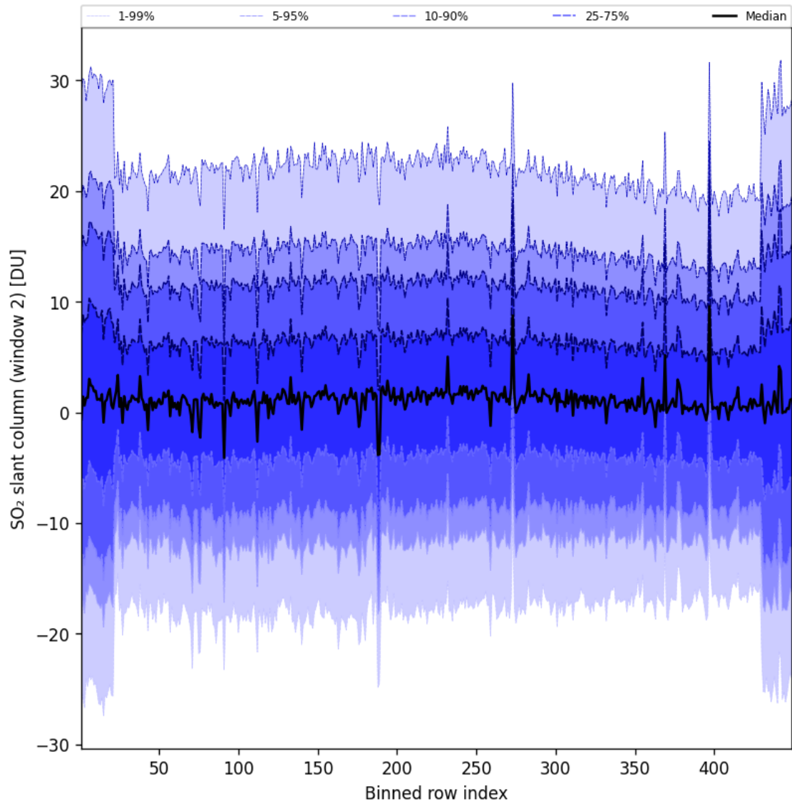
Figure 94: Along track statistics of “SO 2 slant column (window 2)” for 2025-01-05 to 2025-01-05
