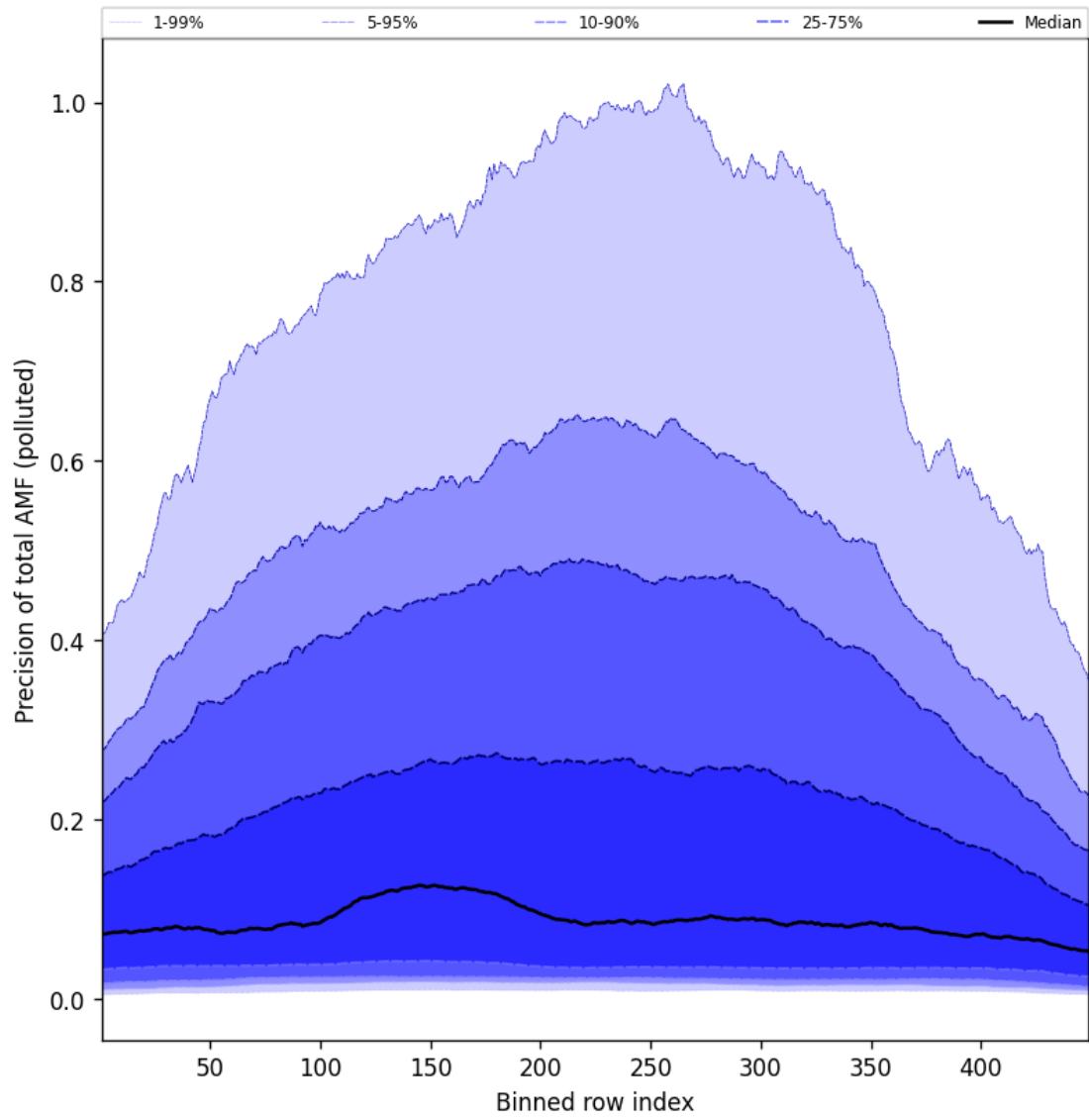
Figure 108: Along track statistics of “Precision of total AMF (polluted)” for 2025-01-05 to 2025-01-05
