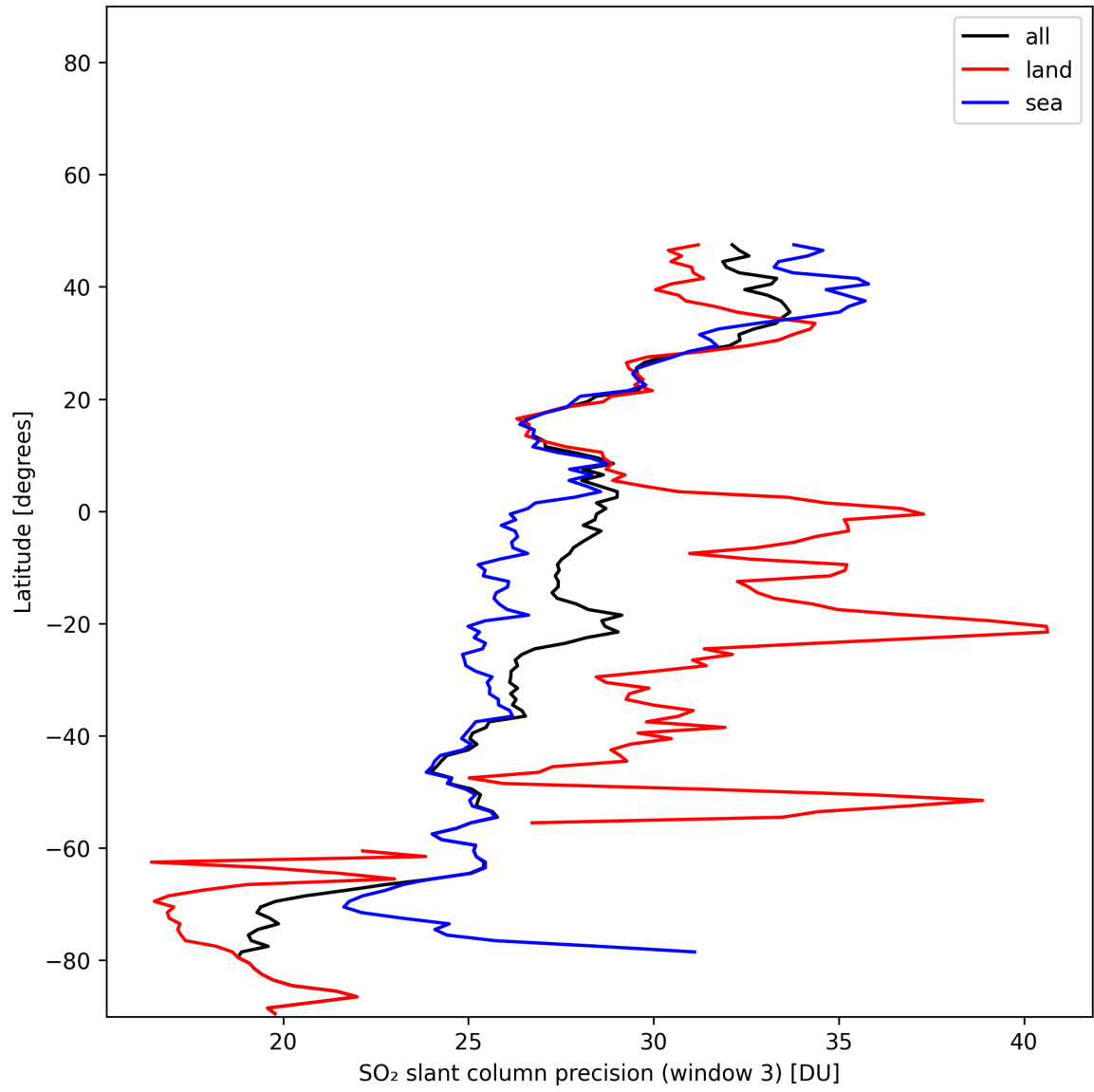
Figure 45: Zonal average of “SO 2 slant column precision (window 3)” for 2025-01-05 to 2025-01-05.
