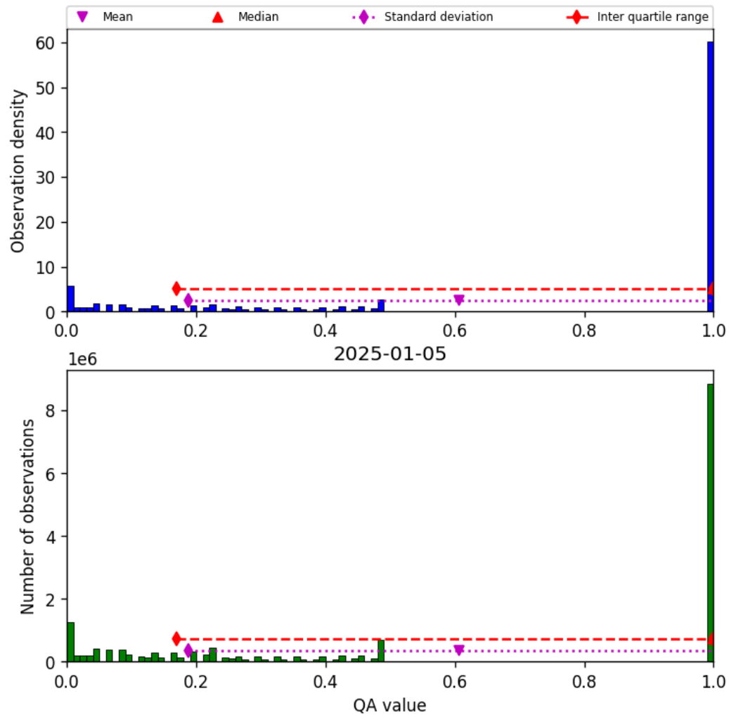
Figure 57: Histogram of “QA value” for 2025-01-05 to 2025-01-05
