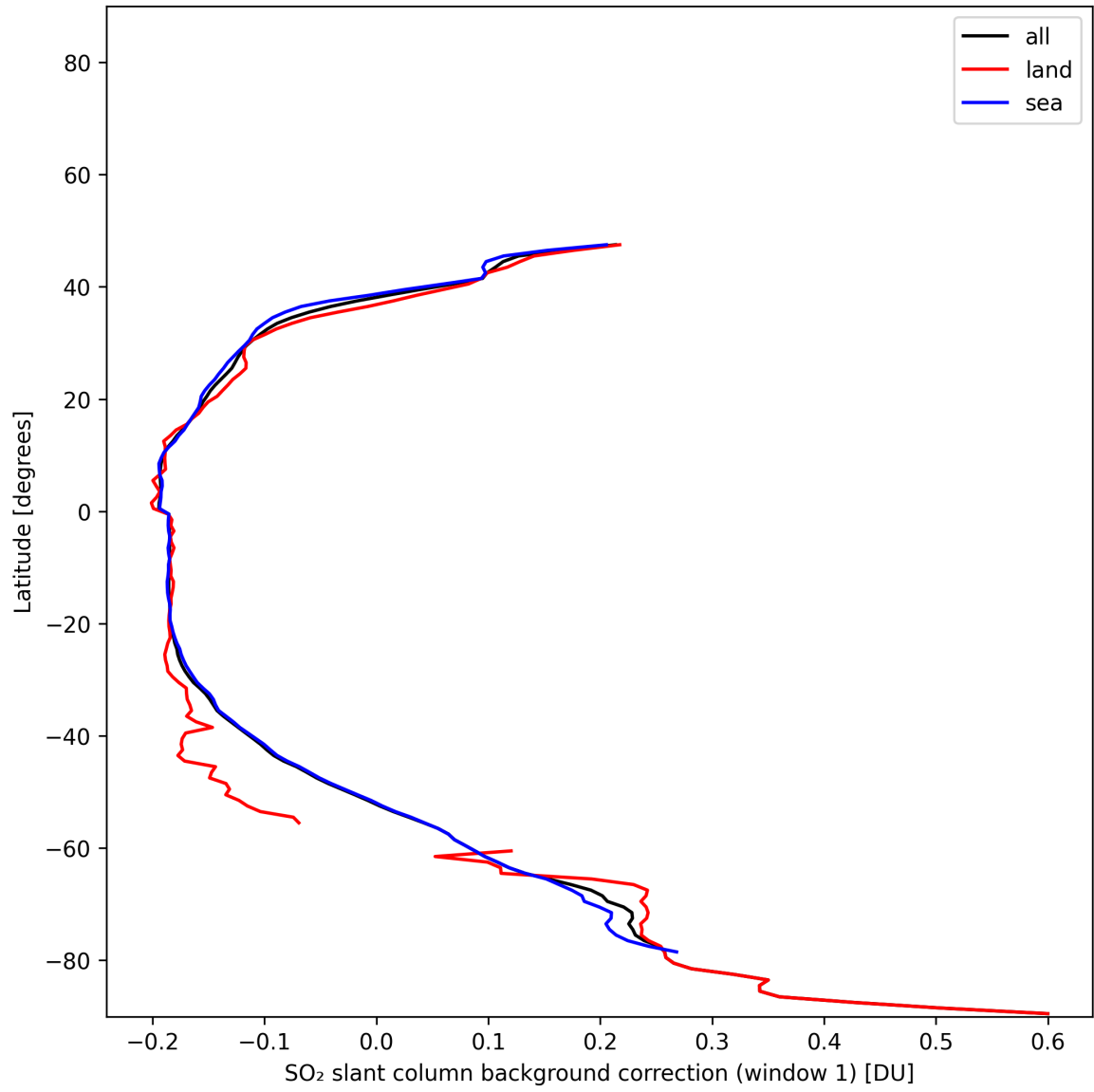
Figure 39: Zonal average of “SO 2 slant column background correction (window 1)” for 2025-01-05 to 2025-01-05.
