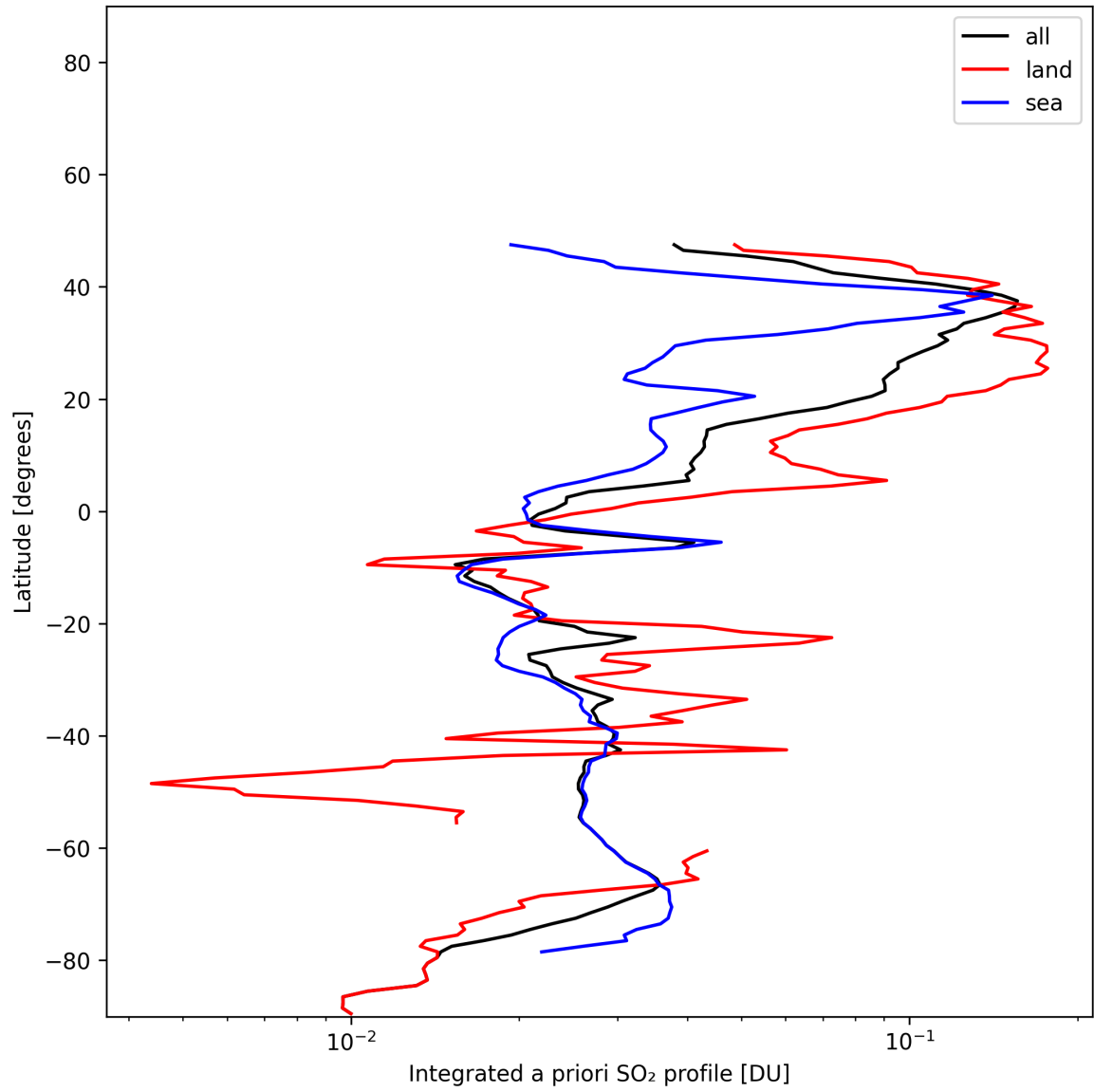
Figure 49: Zonal average of “Integrated a priori SO 2 profile” for 2025-01-05 to 2025-01-05.
