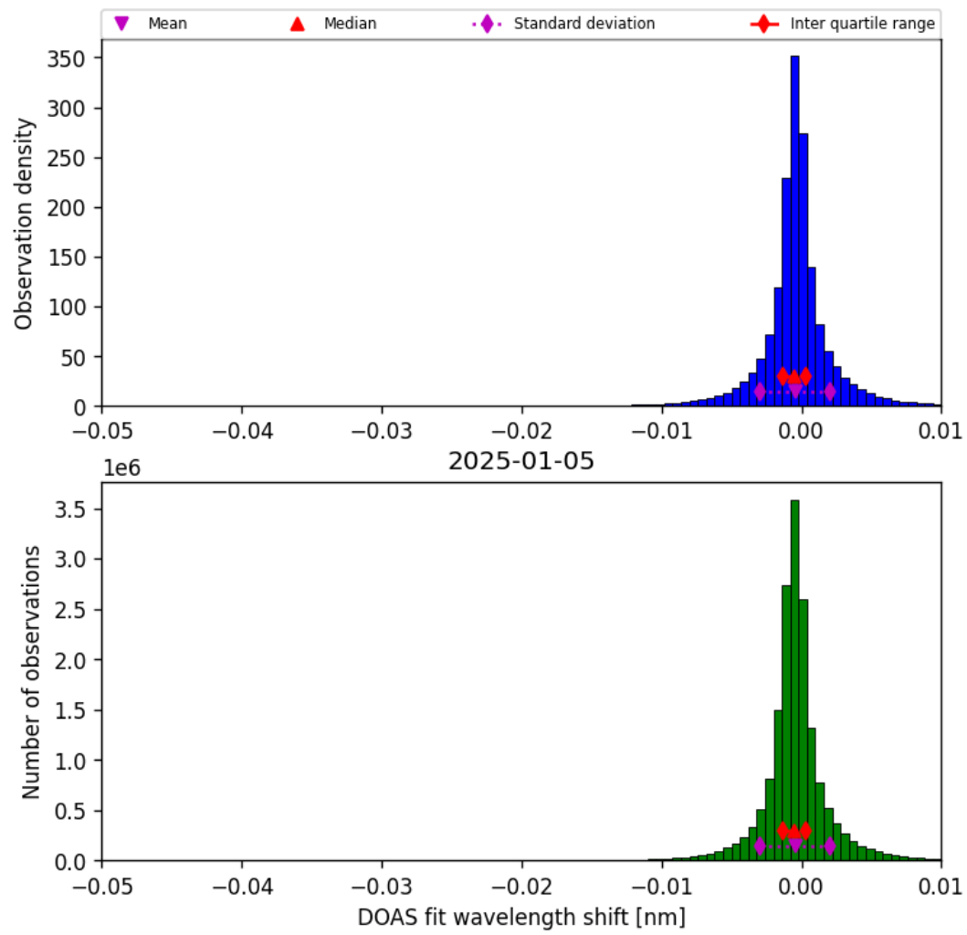
Figure 77: Histogram of “DOAS fit wavelength shift” for 2025-01-05 to 2025-01-05
