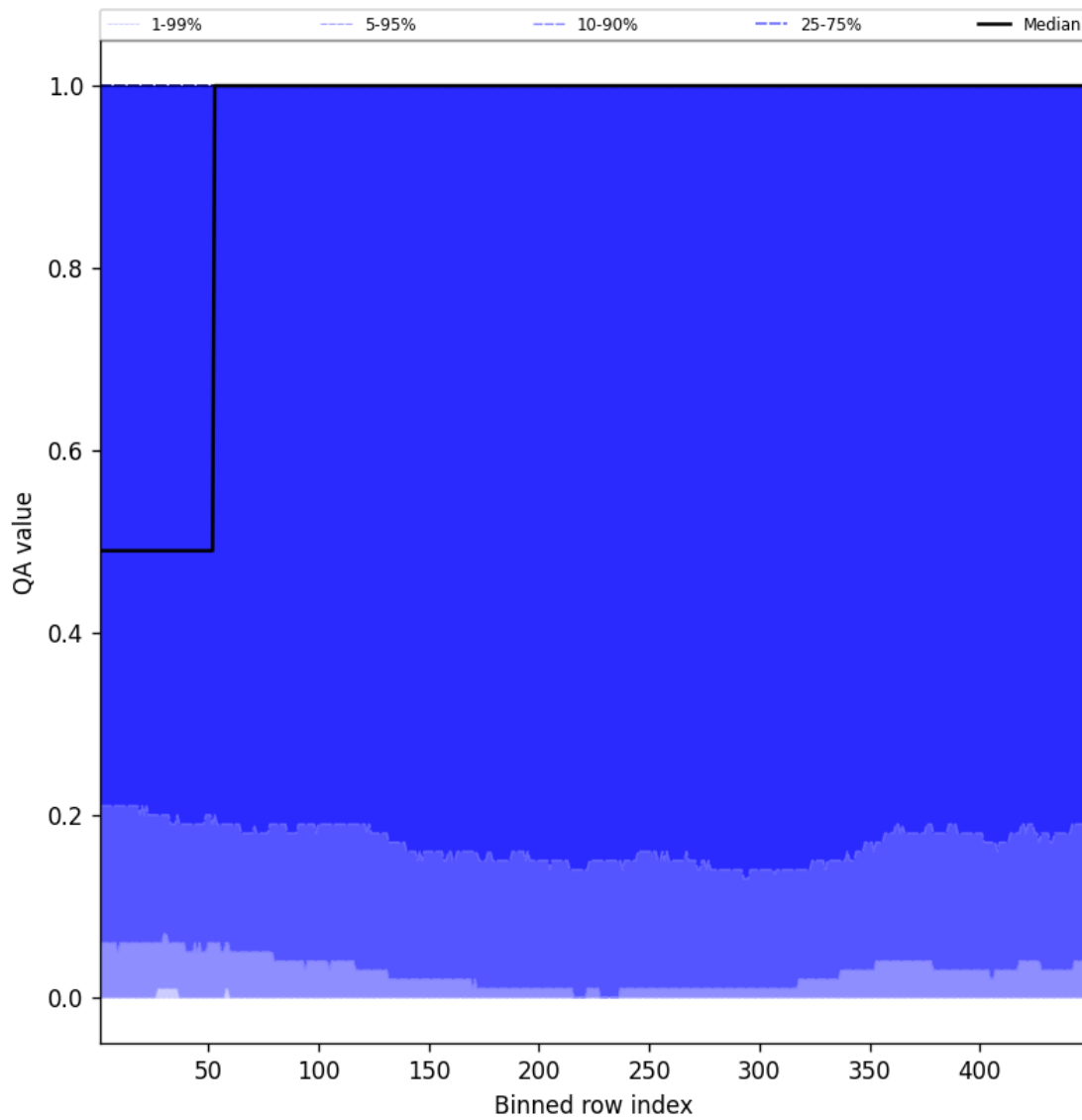
Figure 84: Along track statistics of “QA value” for 2025-01-05 to 2025-01-05
