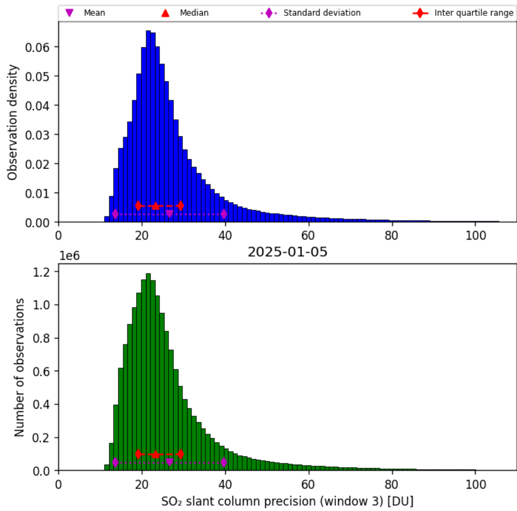
Figure 72: Histogram of “SO 2 slant column precision (window 3)” for 2025-01-05 to 2025-01-05
