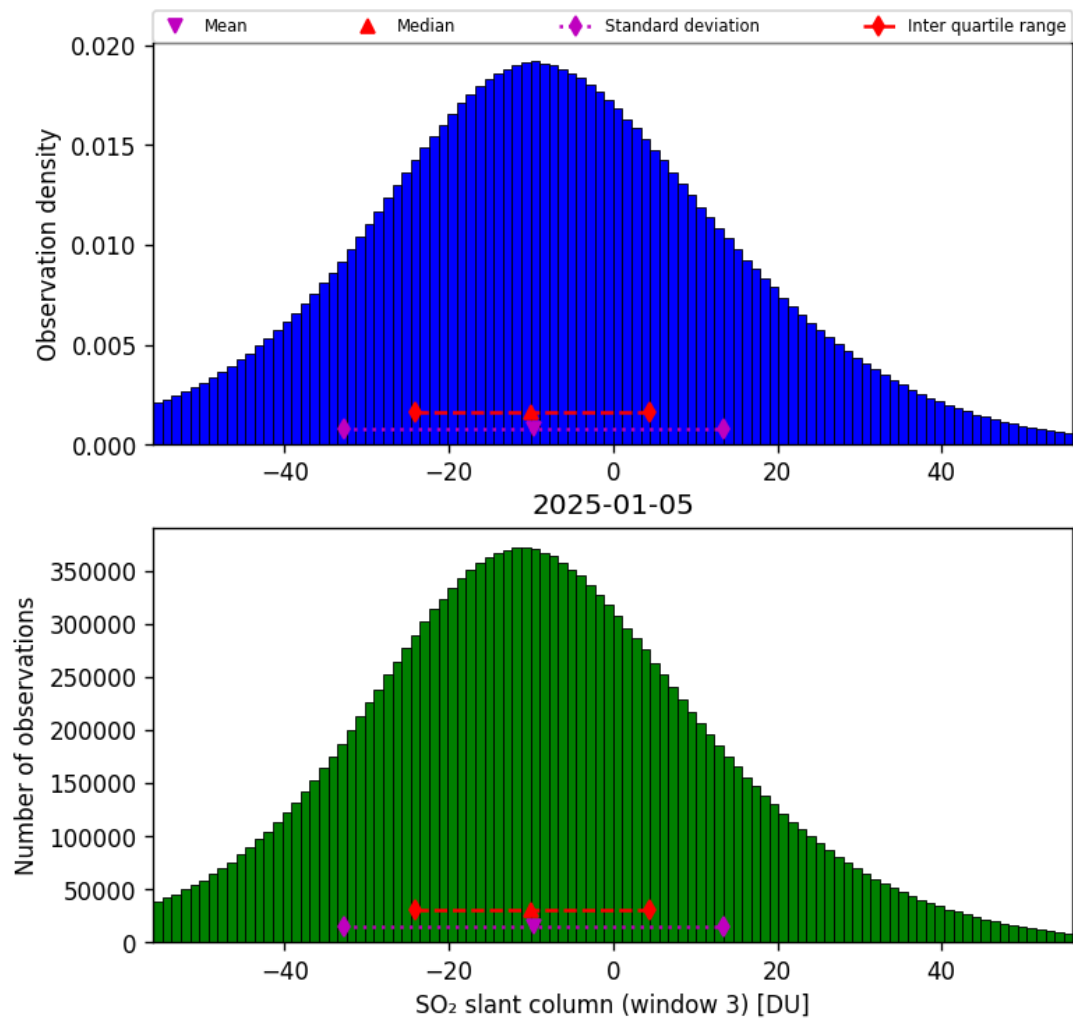
Figure 71: Histogram of “SO 2 slant column (window 3)” for 2025-01-05 to 2025-01-05
