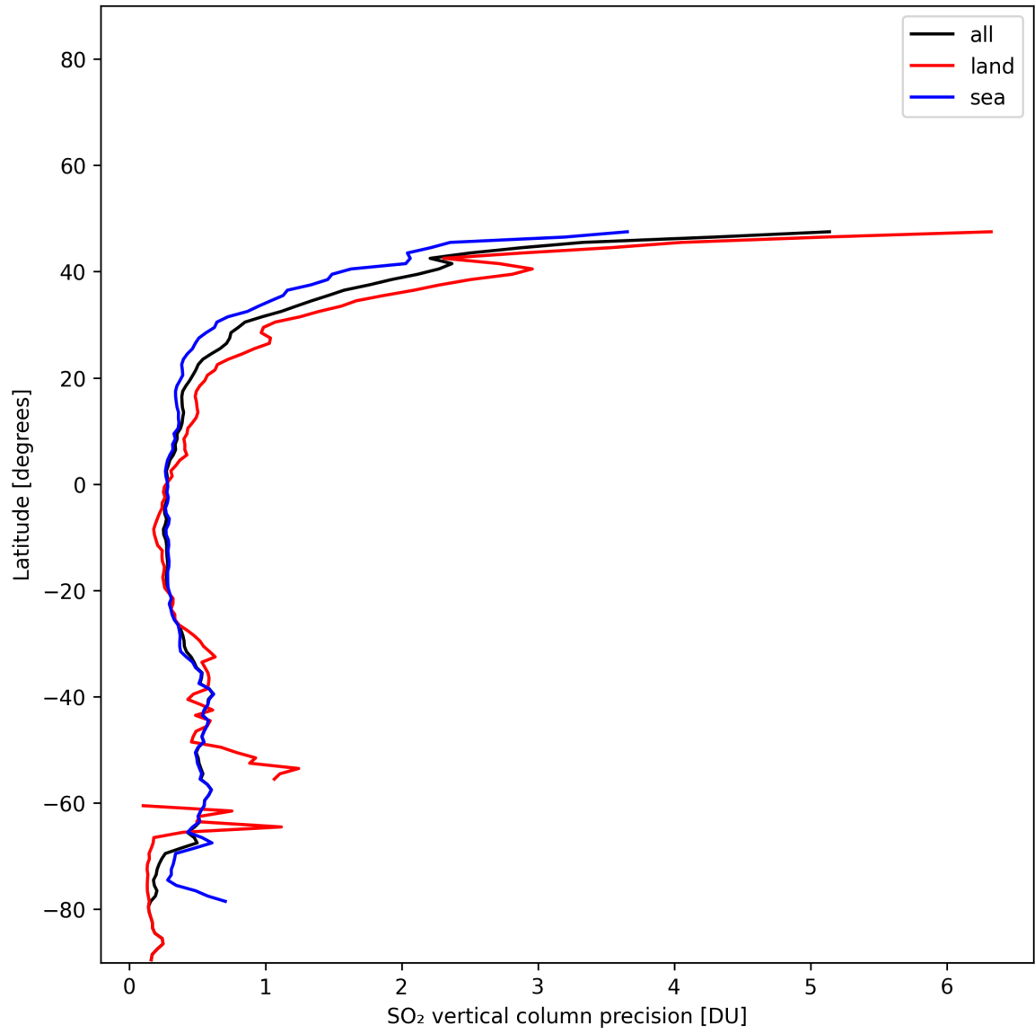
Figure 32: Zonal average of “SO 2 vertical column precision” for 2025-01-05 to 2025-01-05.
