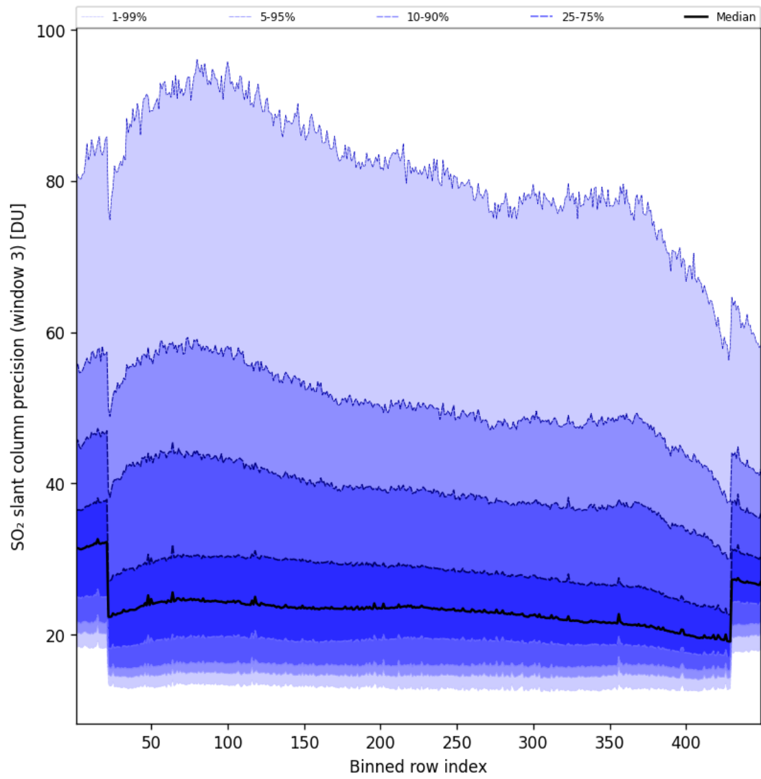
Figure 99: Along track statistics of “SO 2 slant column precision (window 3)” for 2025-01-05 to 2025-01-05
