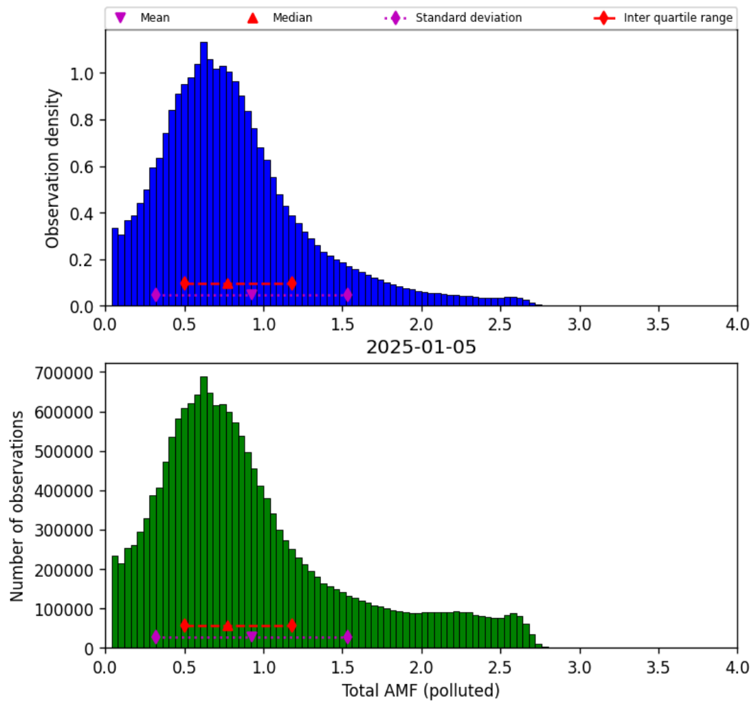
Figure 80: Histogram of “Total AMF (polluted)” for 2025-01-05 to 2025-01-05
