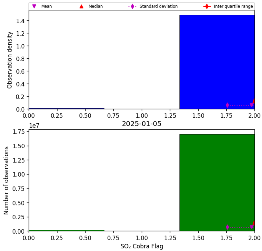
Figure 75: Histogram of “SO 2 Cobra Flag” for 2025-01-05 to 2025-01-05
