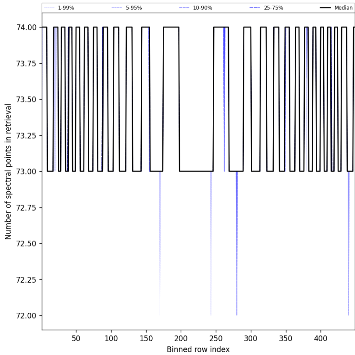
Figure 110: Along track statistics of “Number of spectral points in retrieval” for 2025-01-05 to 2025-01-05
