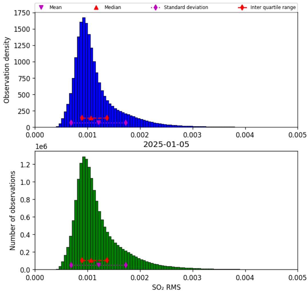
Figure 79: Histogram of “SO 2 RMS” for 2025-01-05 to 2025-01-05
