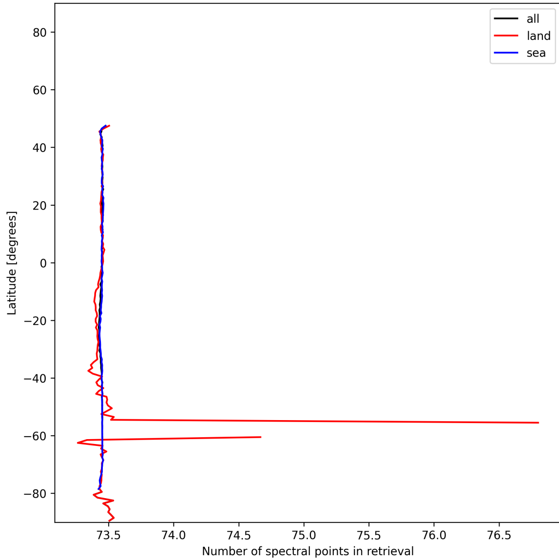
Figure 56: Zonal average of “Number of spectral points in retrieval” for 2025-01-05 to 2025-01-05.
