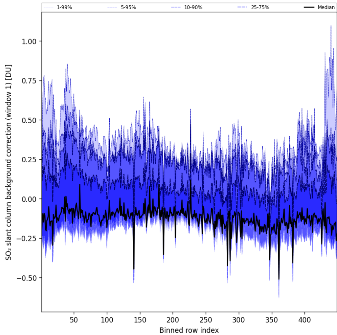
Figure 93: Along track statistics of “SO 2 slant column background correction (window 1)” for 2025-01-05 to 2025-01-05
