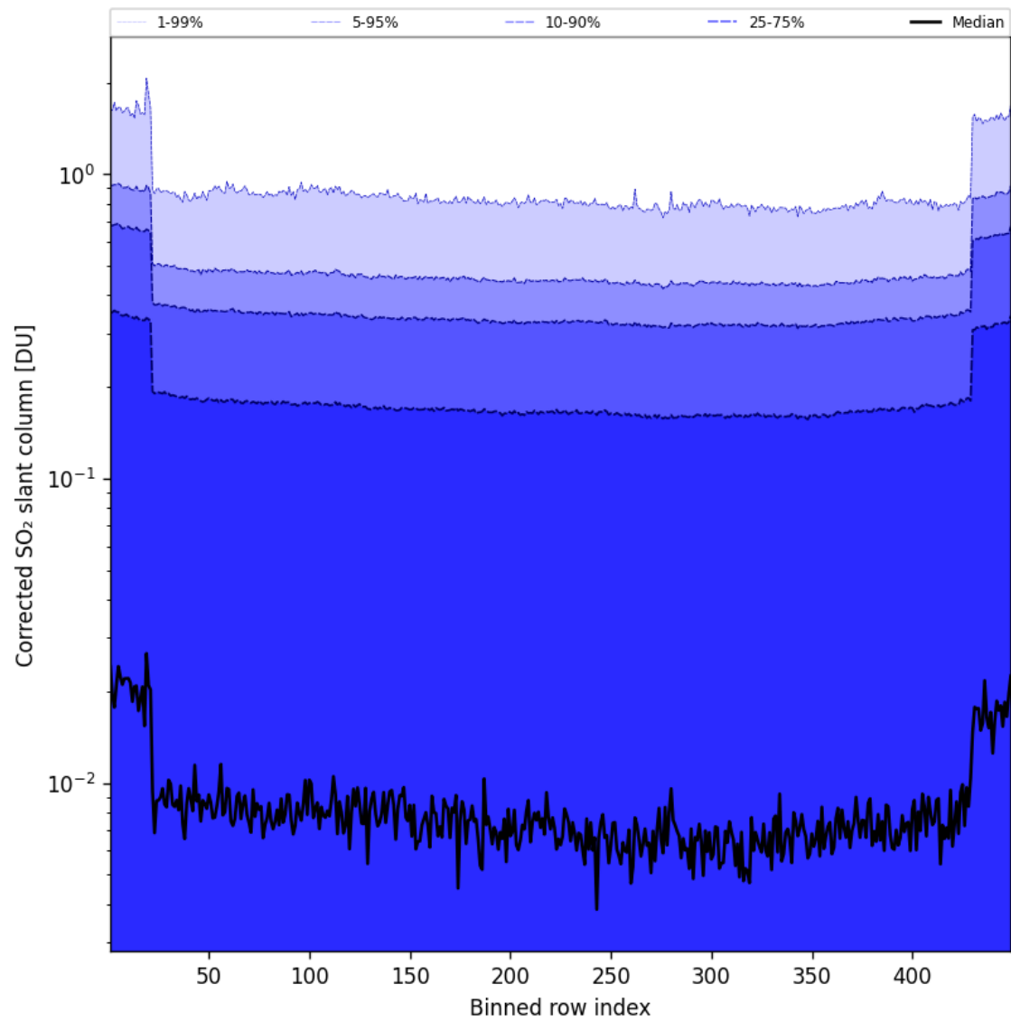
Figure 87: Along track statistics of “Corrected SO 2 slant column” for 2025-01-05 to 2025-01-05
