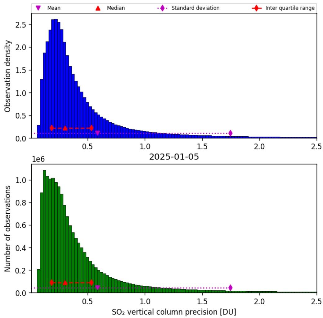
Figure 59: Histogram of “SO 2 vertical column precision” for 2025-01-05 to 2025-01-05
