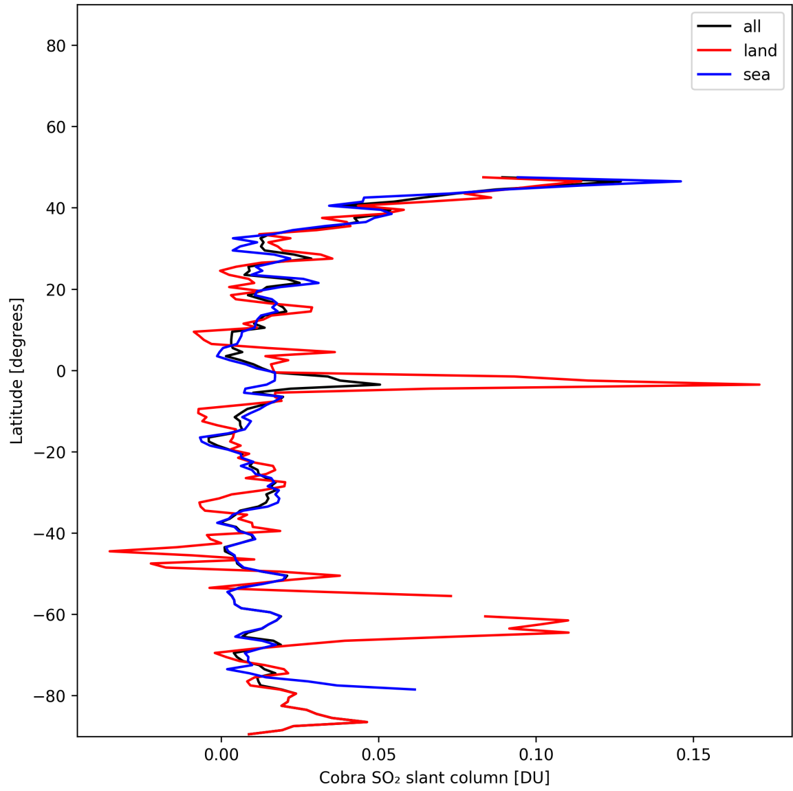
Figure 34: Zonal average of “Cobra SO 2 slant column” for 2025-01-05 to 2025-01-05.
