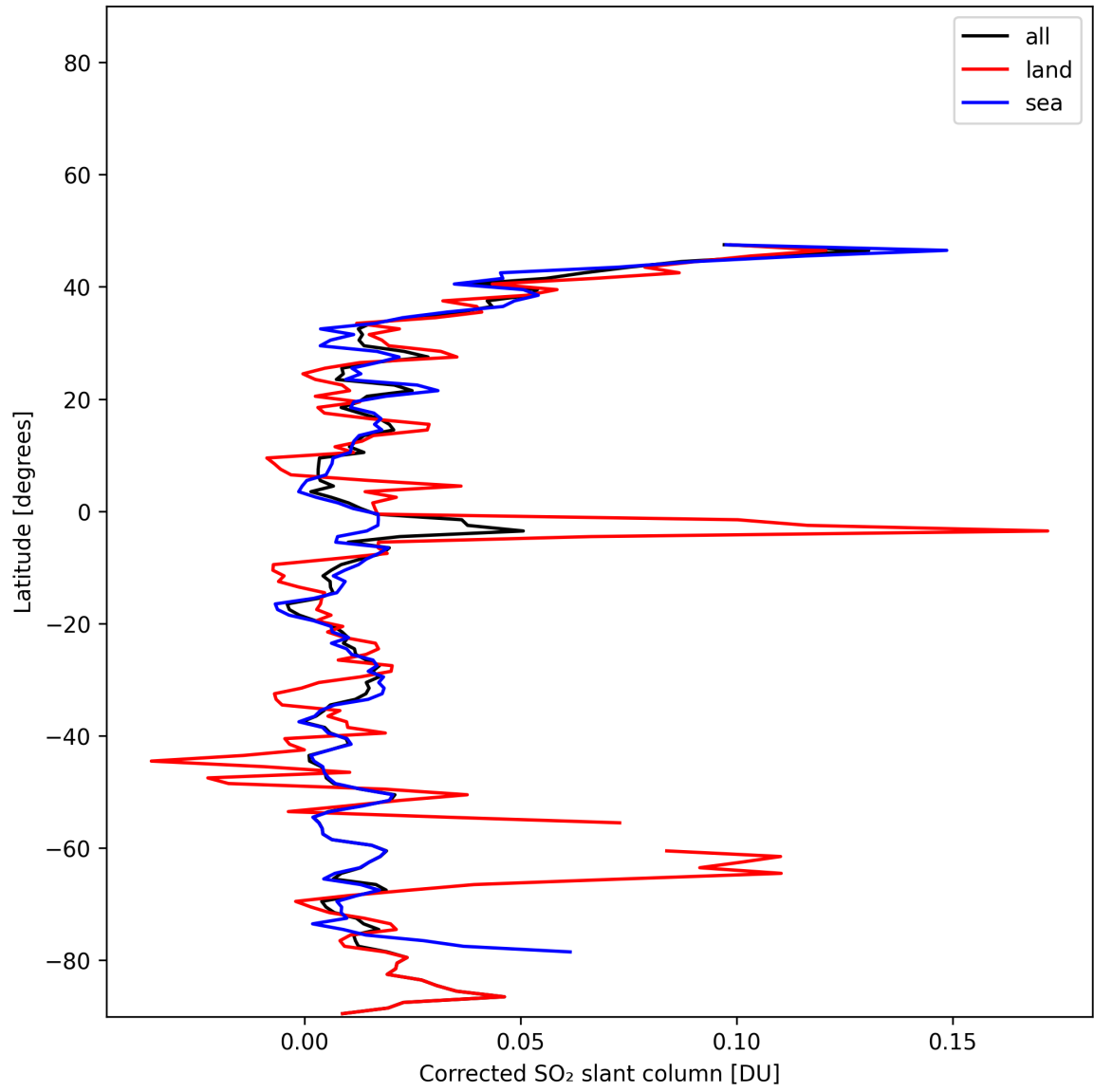
Figure 33: Zonal average of “Corrected SO 2 slant column” for 2025-01-05 to 2025-01-05.
