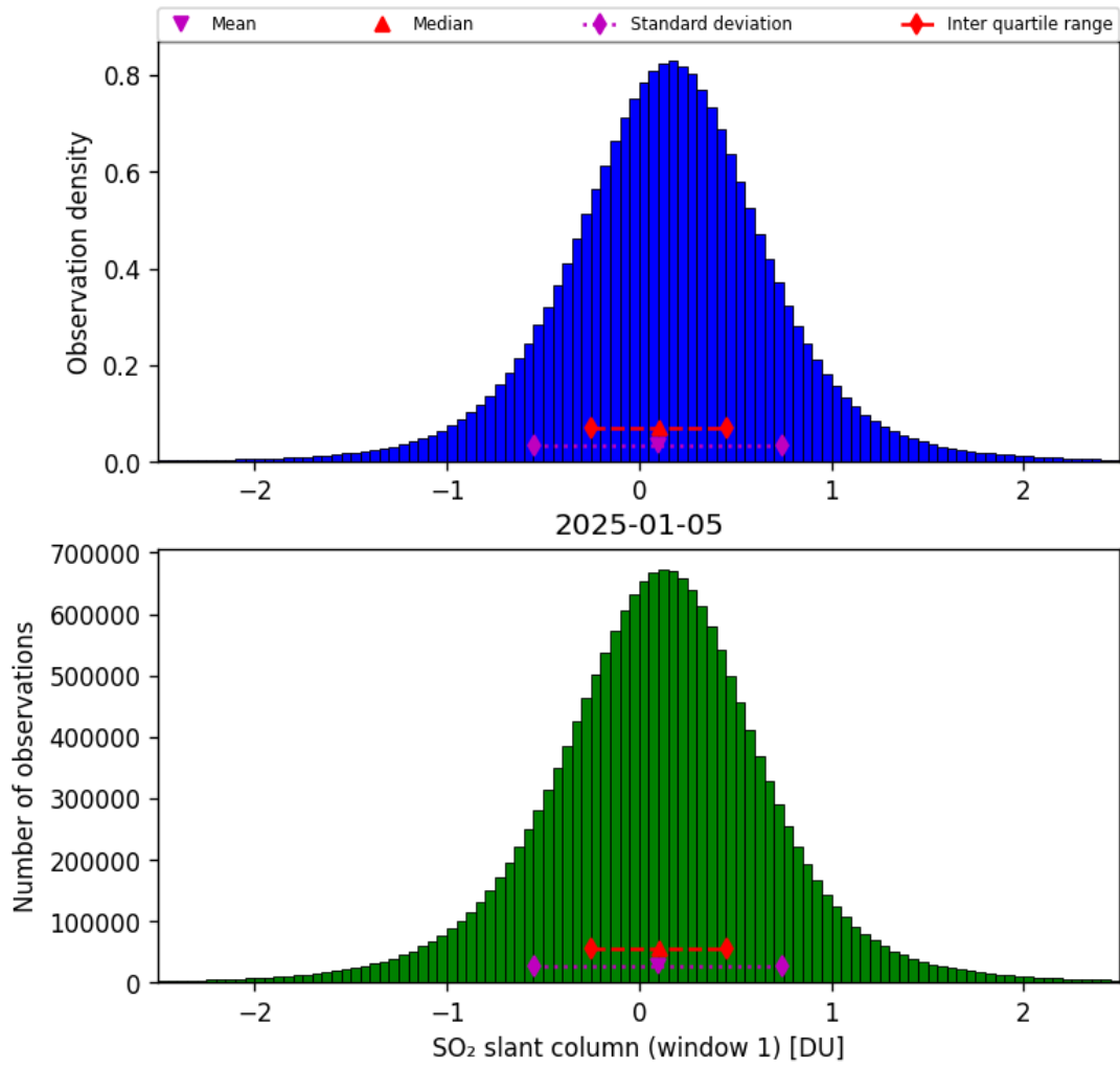
Figure 63: Histogram of “SO 2 slant column (window 1)” for 2025-01-05 to 2025-01-05
