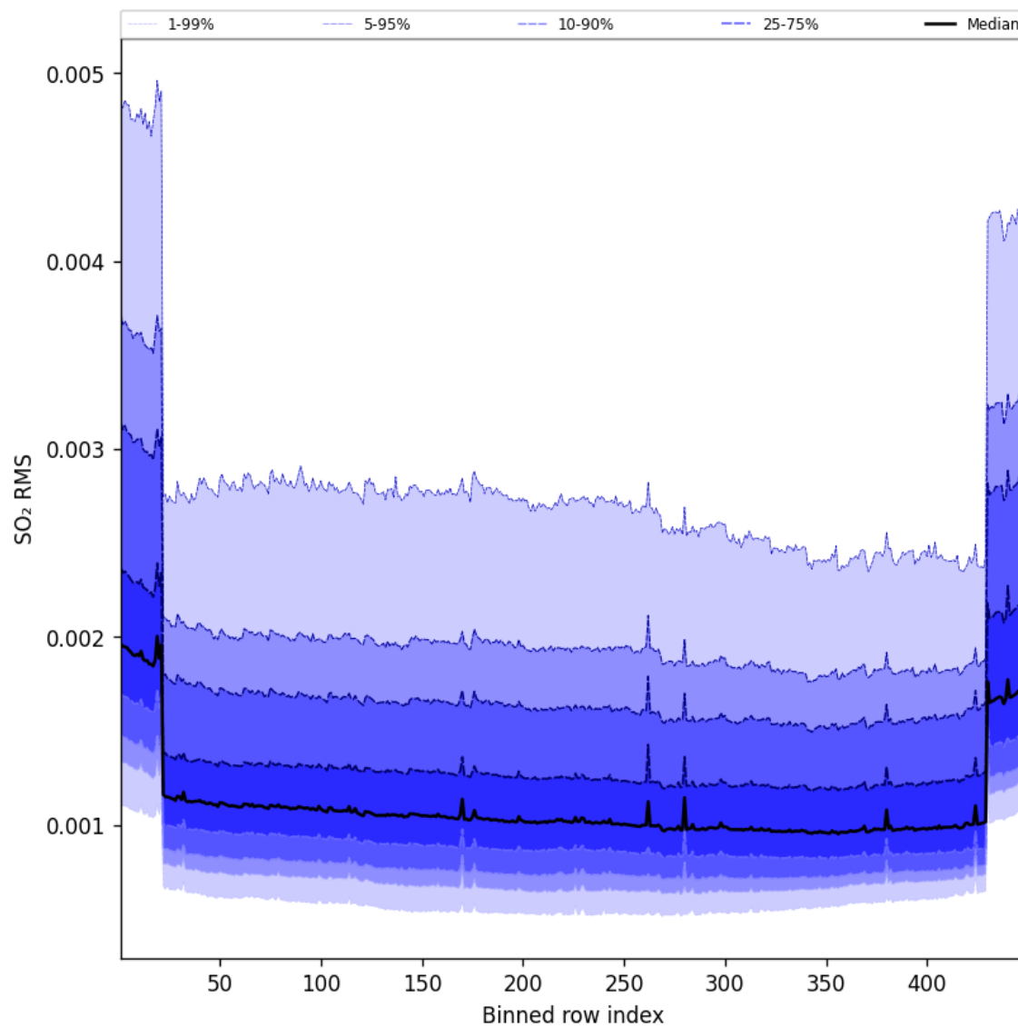
Figure 106: Along track statistics of “SO 2 RMS” for 2025-01-05 to 2025-01-05
