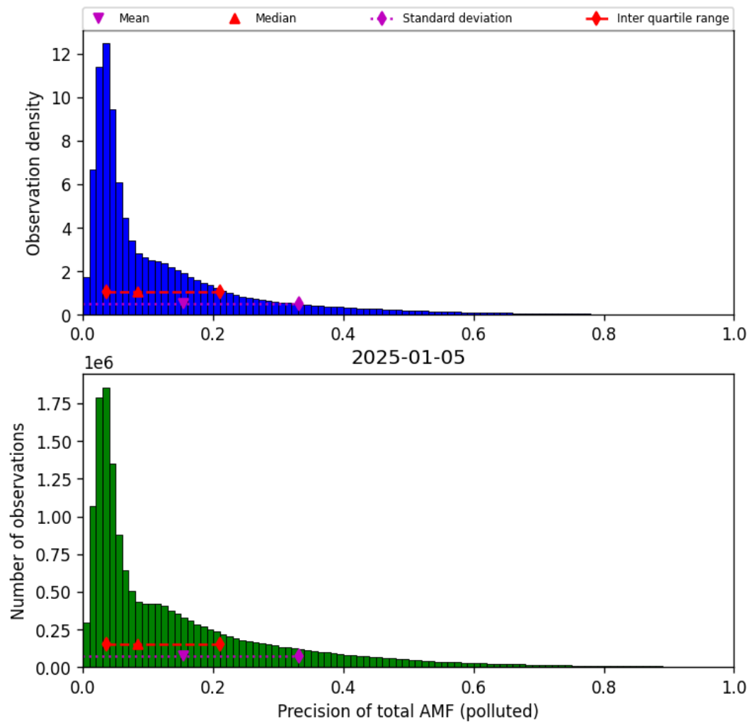
Figure 81: Histogram of “Precision of total AMF (polluted)” for 2025-01-05 to 2025-01-05
