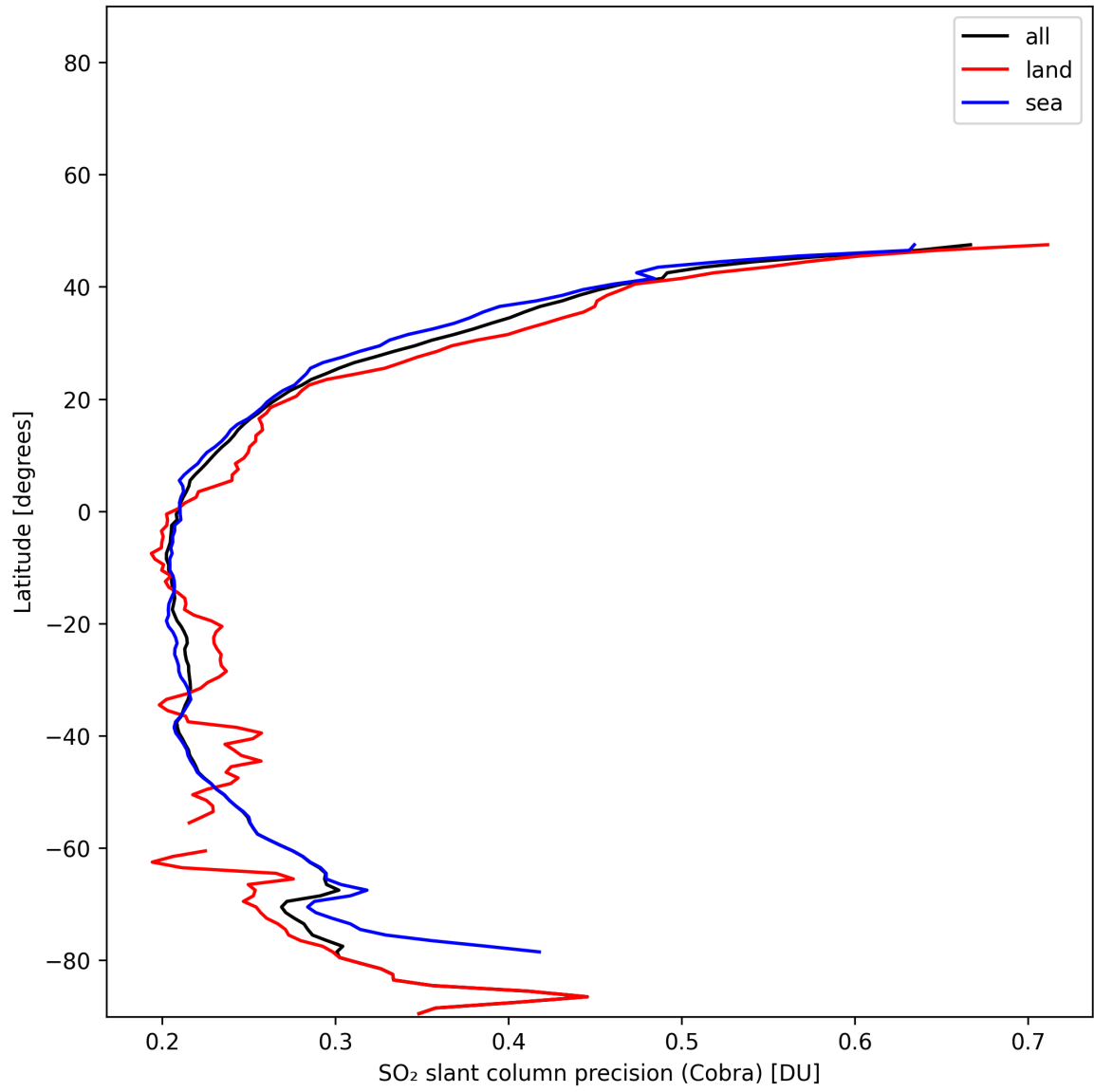
Figure 35: Zonal average of “SO 2 slant column precision (Cobra)” for 2025-01-05 to 2025-01-05.
