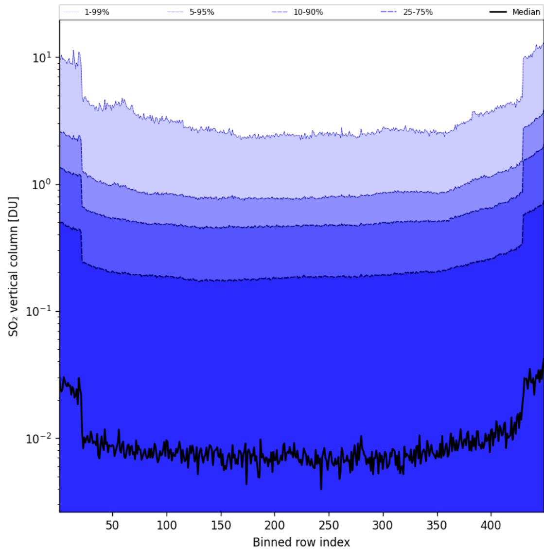
Figure 85: Along track statistics of “SO 2 vertical column” for 2025-01-05 to 2025-01-05
