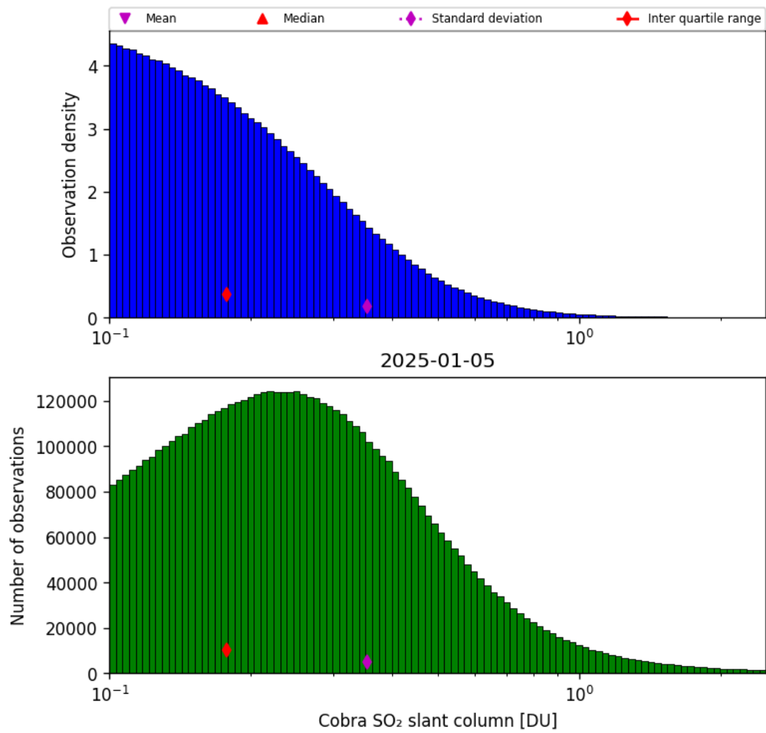
Figure 61: Histogram of “Cobra SO 2 slant column” for 2025-01-05 to 2025-01-05
