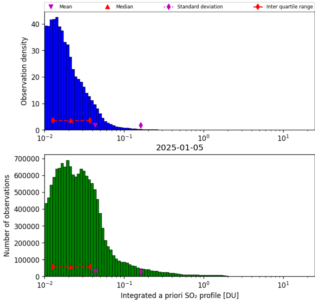
Figure 76: Histogram of “Integrated a priori SO 2 profile” for 2025-01-05 to 2025-01-05
