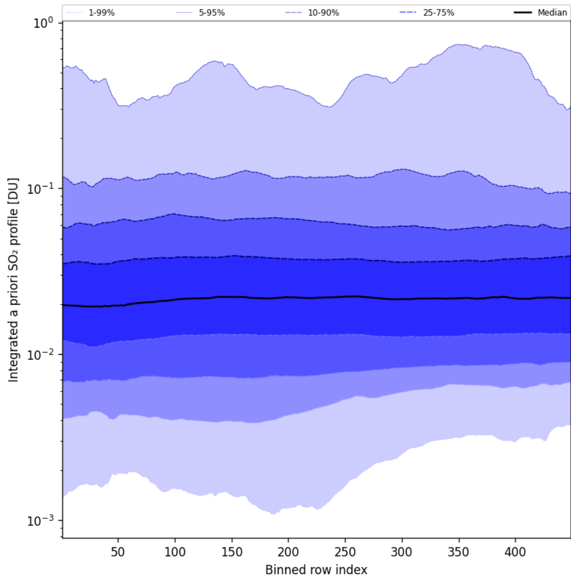
Figure 103: Along track statistics of “Integrated a priori SO 2 profile” for 2025-01-05 to 2025-01-05
