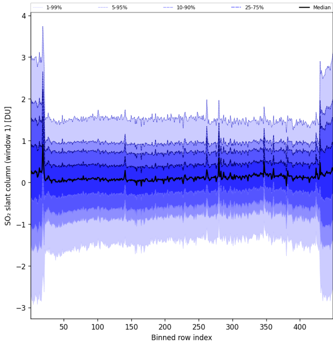
Figure 90: Along track statistics of “SO 2 slant column (window 1)” for 2025-01-05 to 2025-01-05
