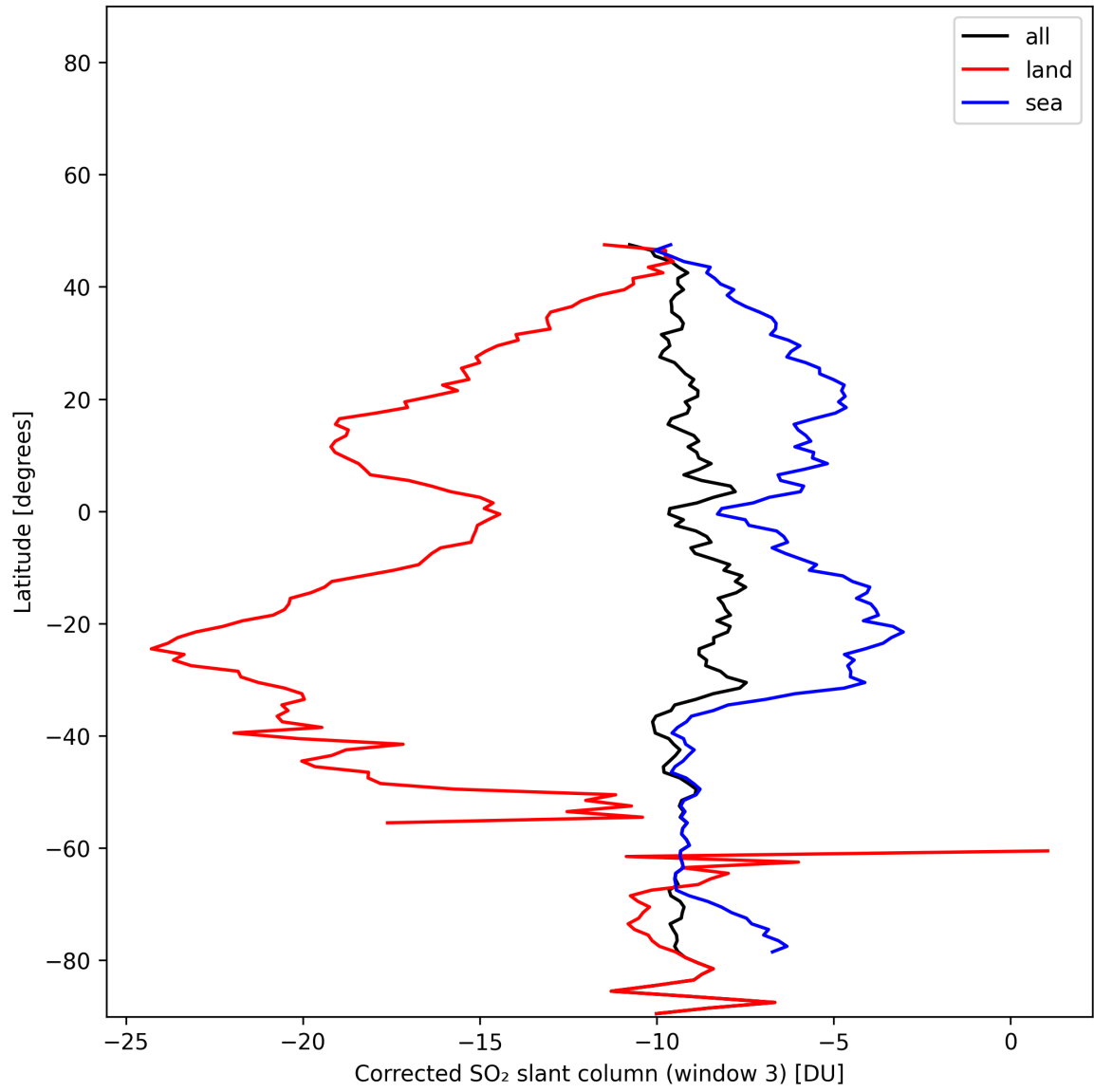
Figure 46: Zonal average of “Corrected SO 2 slant column (window 3)” for 2025-01-05 to 2025-01-05.
