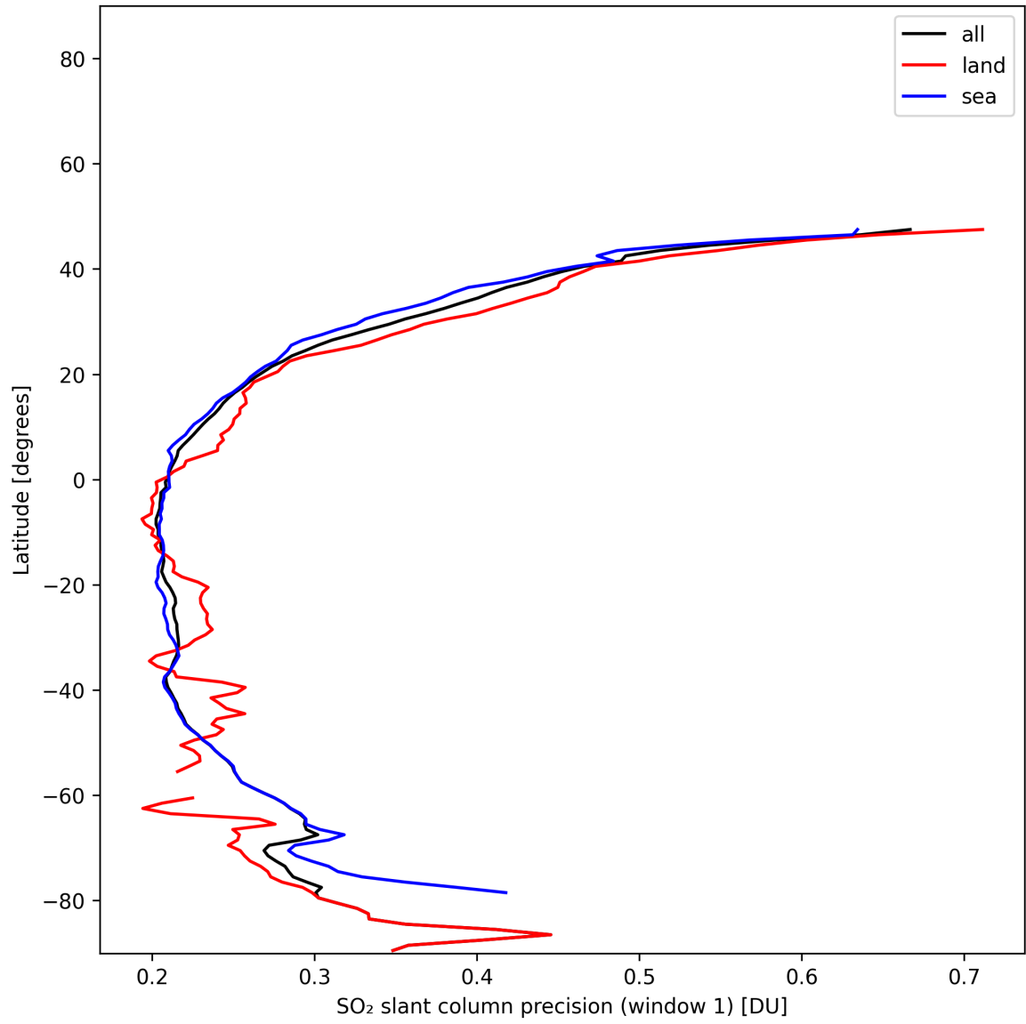
Figure 37: Zonal average of "SO 2 slant column precision (window 1)" for 2025-01-05 to 2025-01-05.
