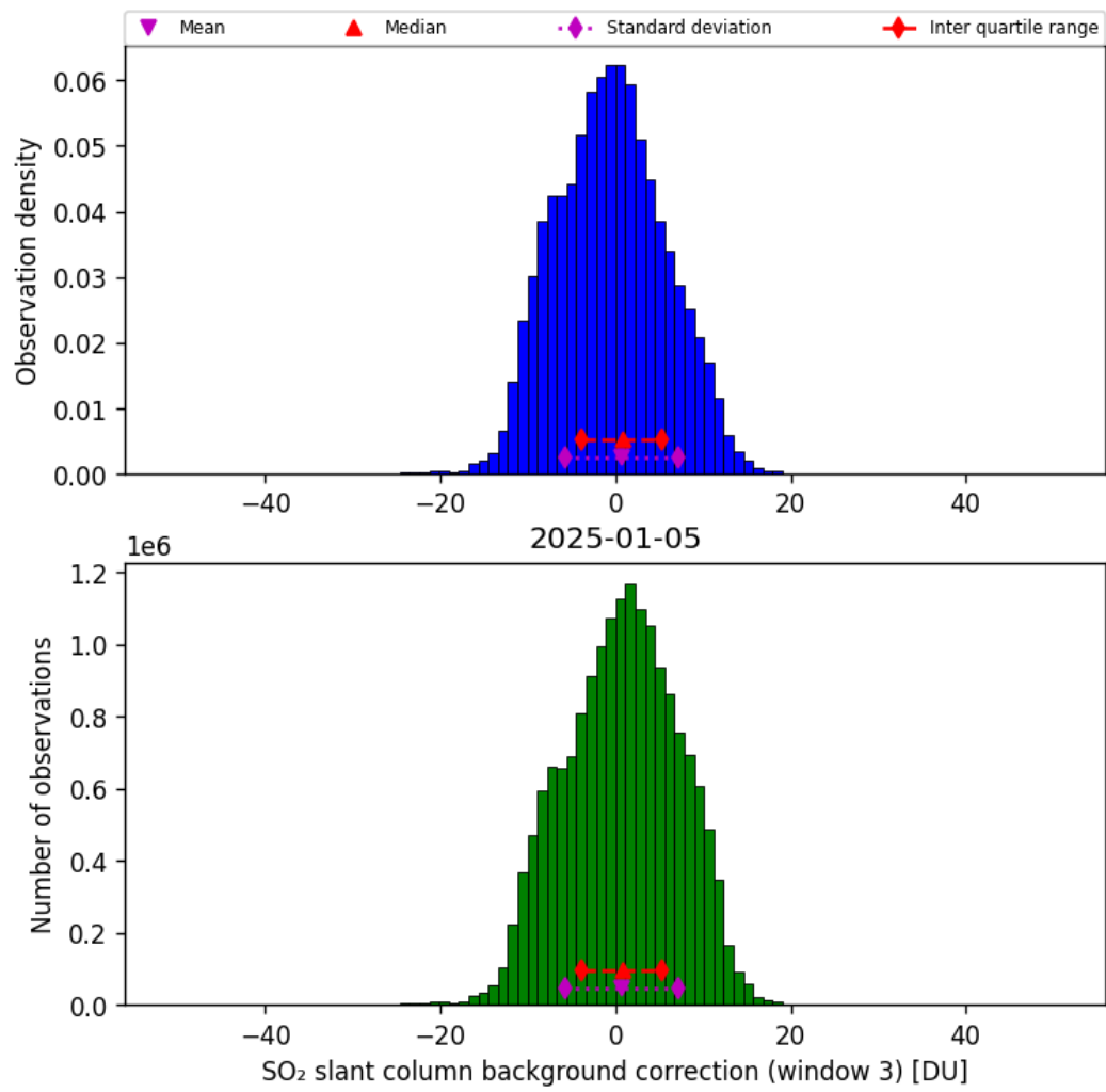
Figure 74: Histogram of “SO 2 slant column background correction (window 3)” for 2025-01-05 to 2025-01-05
