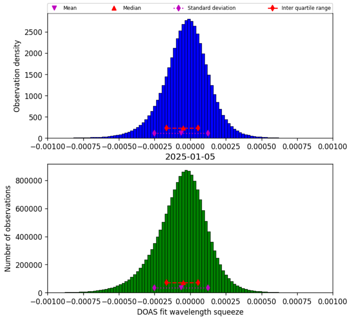
Figure 78: Histogram of “DOAS fit wavelength squeeze” for 2025-01-05 to 2025-01-05
