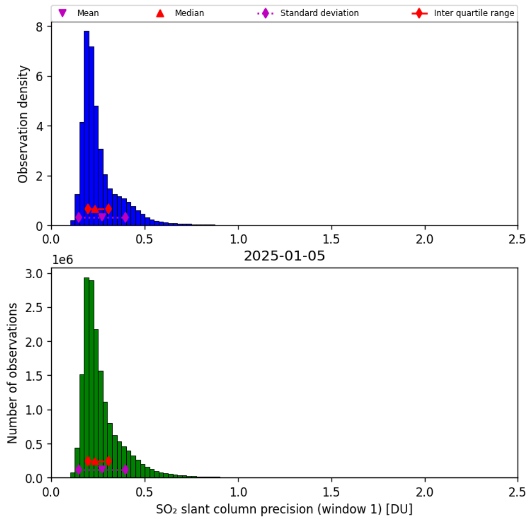
Figure 64: Histogram of “SO 2 slant column precision (window 1)” for 2025-01-05 to 2025-01-05
