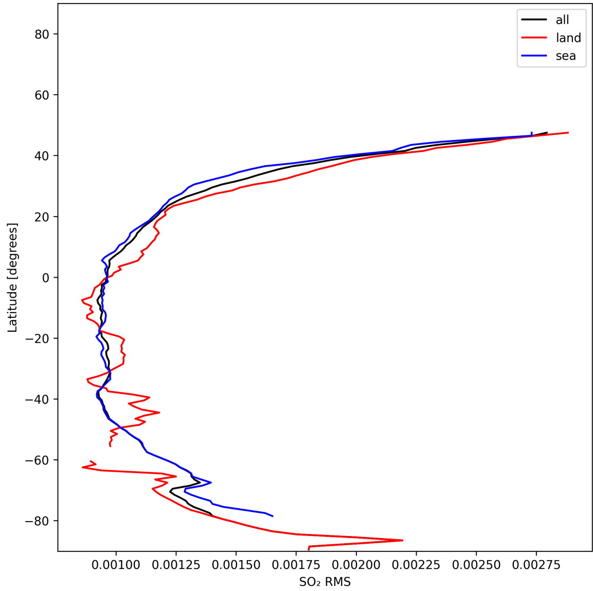
Figure 52: Zonal average of “SO 2 RMS” for 2025-01-05 to 2025-01-05.
