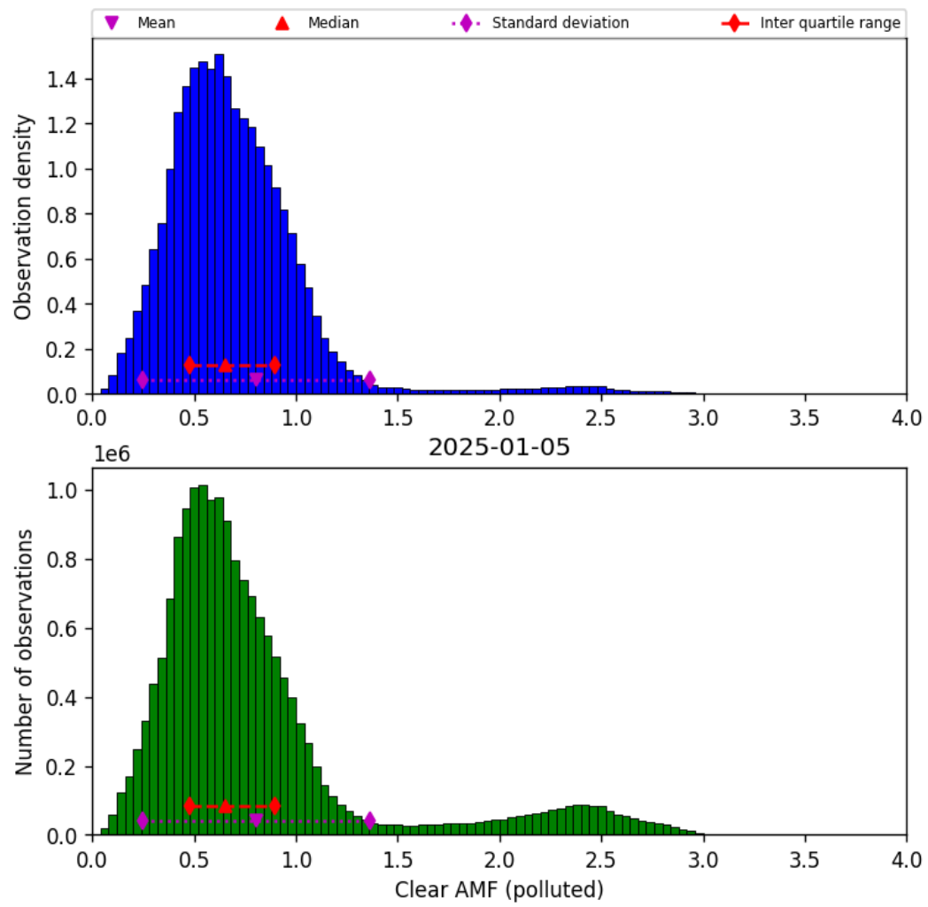
Figure 82: Histogram of “Clear AMF (polluted)” for 2025-01-05 to 2025-01-05
