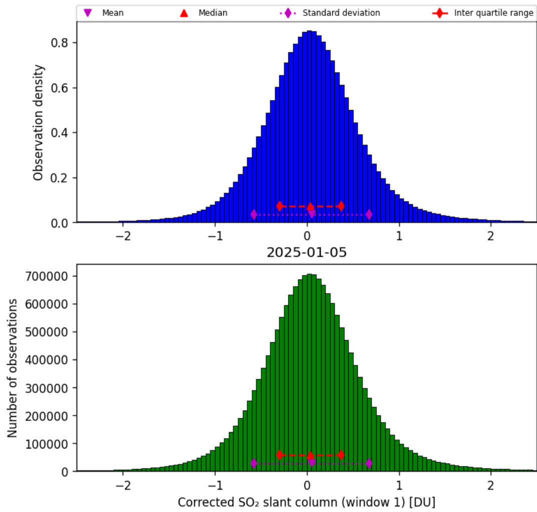
Figure 65: Histogram of “Corrected SO 2 slant column (window 1)” for 2025-01-05 to 2025-01-05
