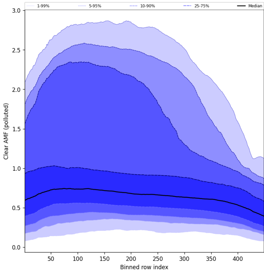
Figure 109: Along track statistics of “Clear AMF (polluted)” for 2025-01-05 to 2025-01-05
