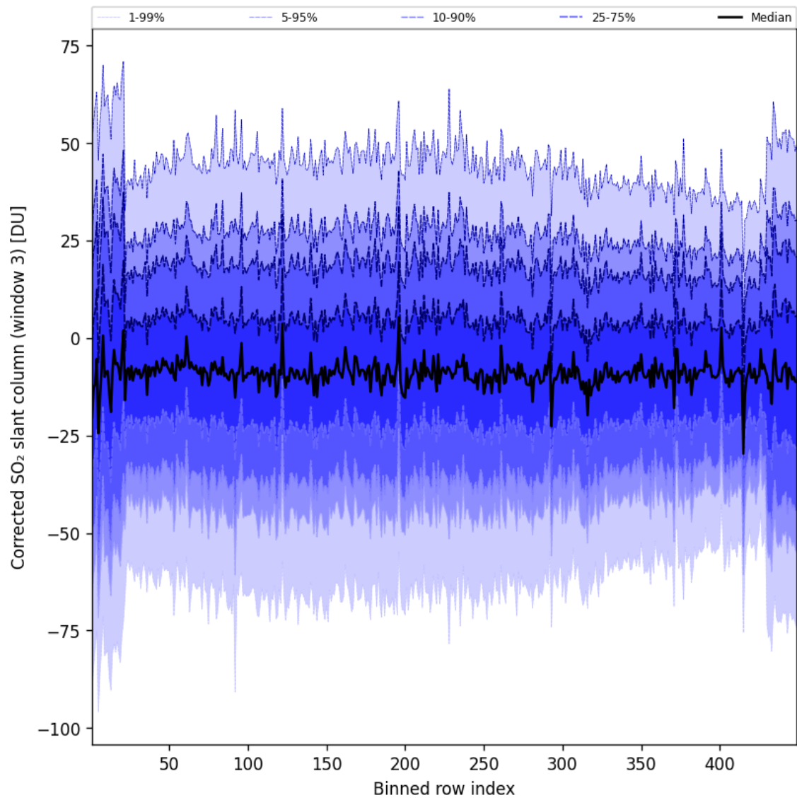
Figure 100: Along track statistics of “Corrected SO 2 slant column (window 3)” for 2025-01-05 to 2025-01-05
