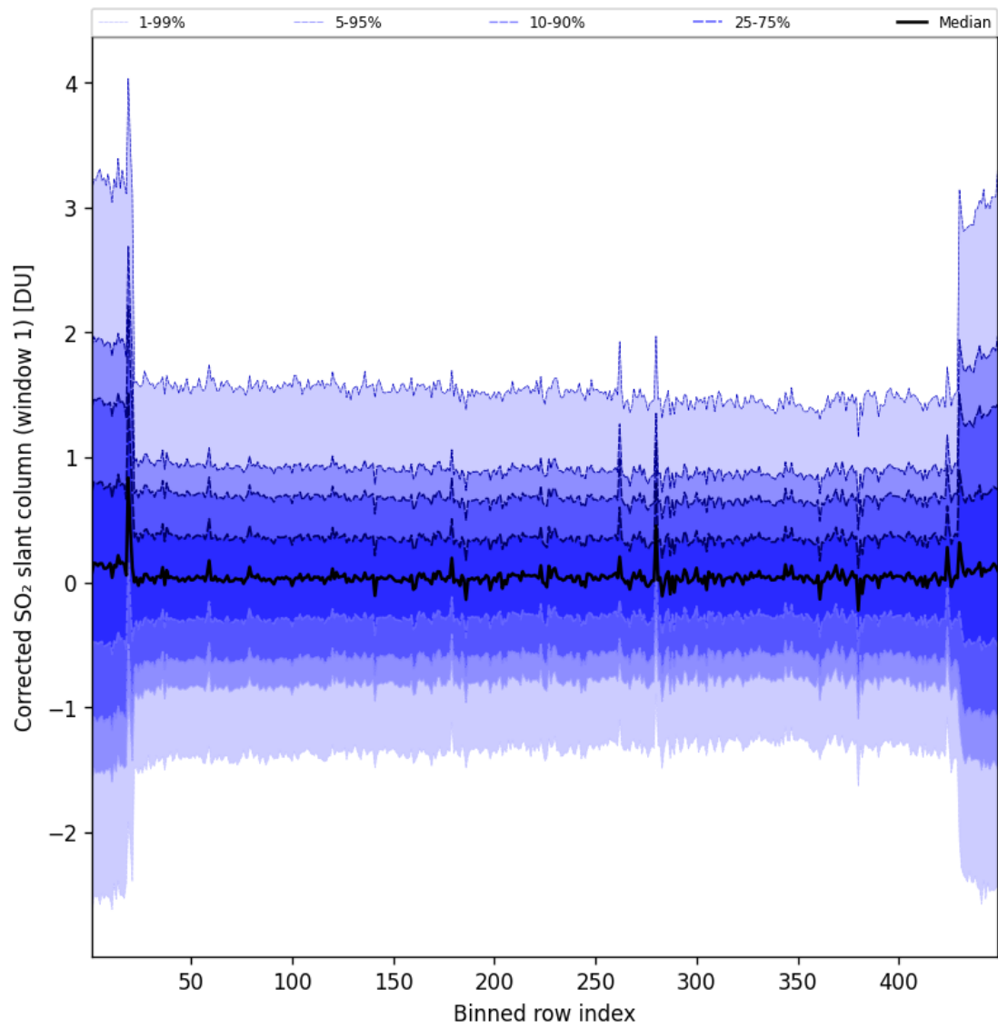
Figure 92: Along track statistics of “Corrected SO 2 slant column (window 1)” for 2025-01-05 to 2025-01-05
