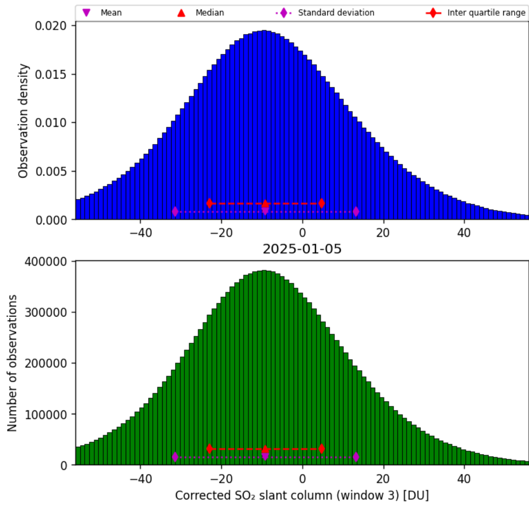
Figure 73: Histogram of “Corrected SO 2 slant column (window 3)” for 2025-01-05 to 2025-01-05
