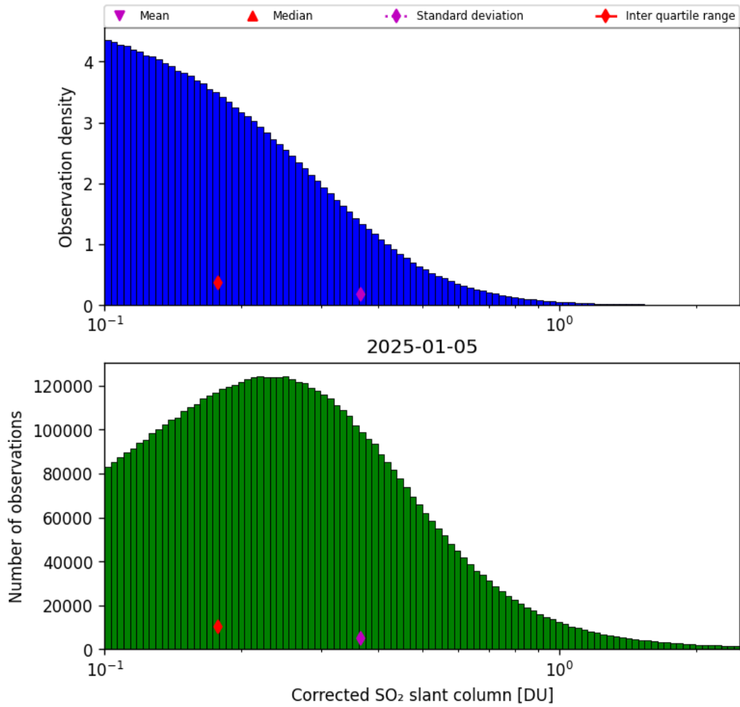
Figure 60: Histogram of “Corrected SO 2 slant column” for 2025-01-05 to 2025-01-05
