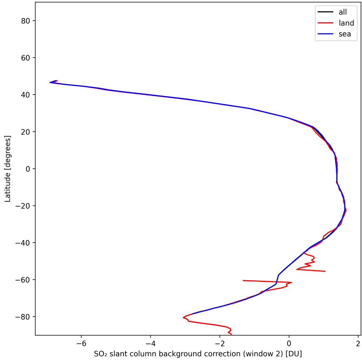
Figure 43: Zonal average of “SO 2 slant column background correction (window 2)” for 2025-01-05 to 2025-01-05.
