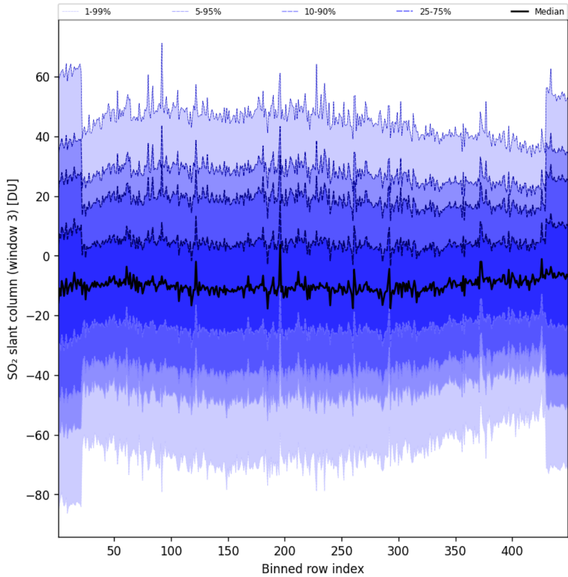
Figure 98: Along track statistics of “SO 2 slant column (window 3)” for 2025-01-05 to 2025-01-05
