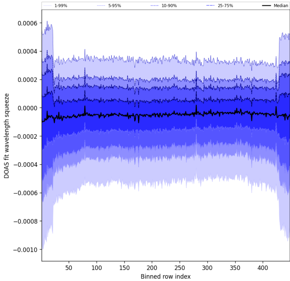
Figure 105: Along track statistics of “DOAS fit wavelength squeeze” for 2025-01-05 to 2025-01-05
