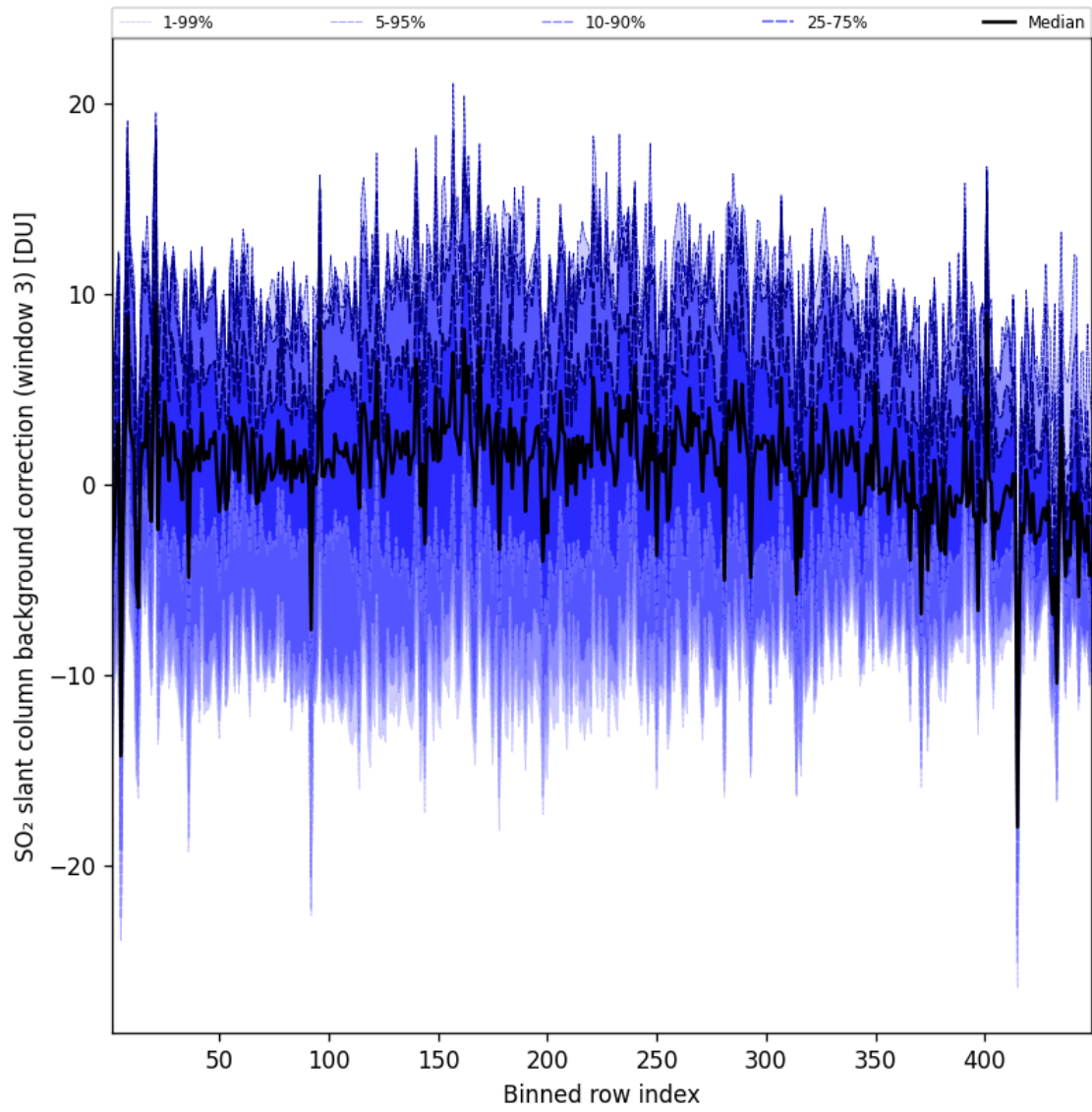
Figure 101: Along track statistics of “SO 2 slant column background correction (window 3)” for 2025-01-05 to 2025-01-05
