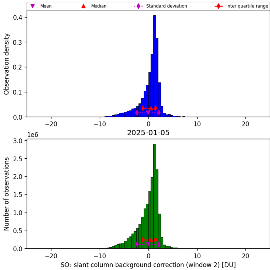
Figure 70: Histogram of “SO 2 slant column background correction (window 2)” for 2025-01-05 to 2025-01-05
