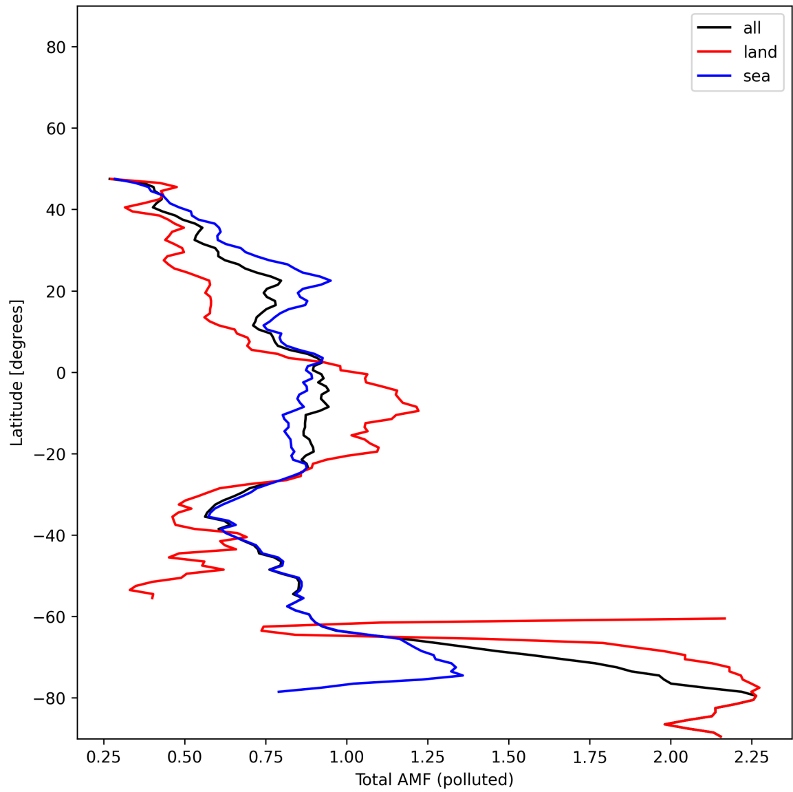
Figure 53: Zonal average of “Total AMF (polluted)” for 2025-01-05 to 2025-01-05.
