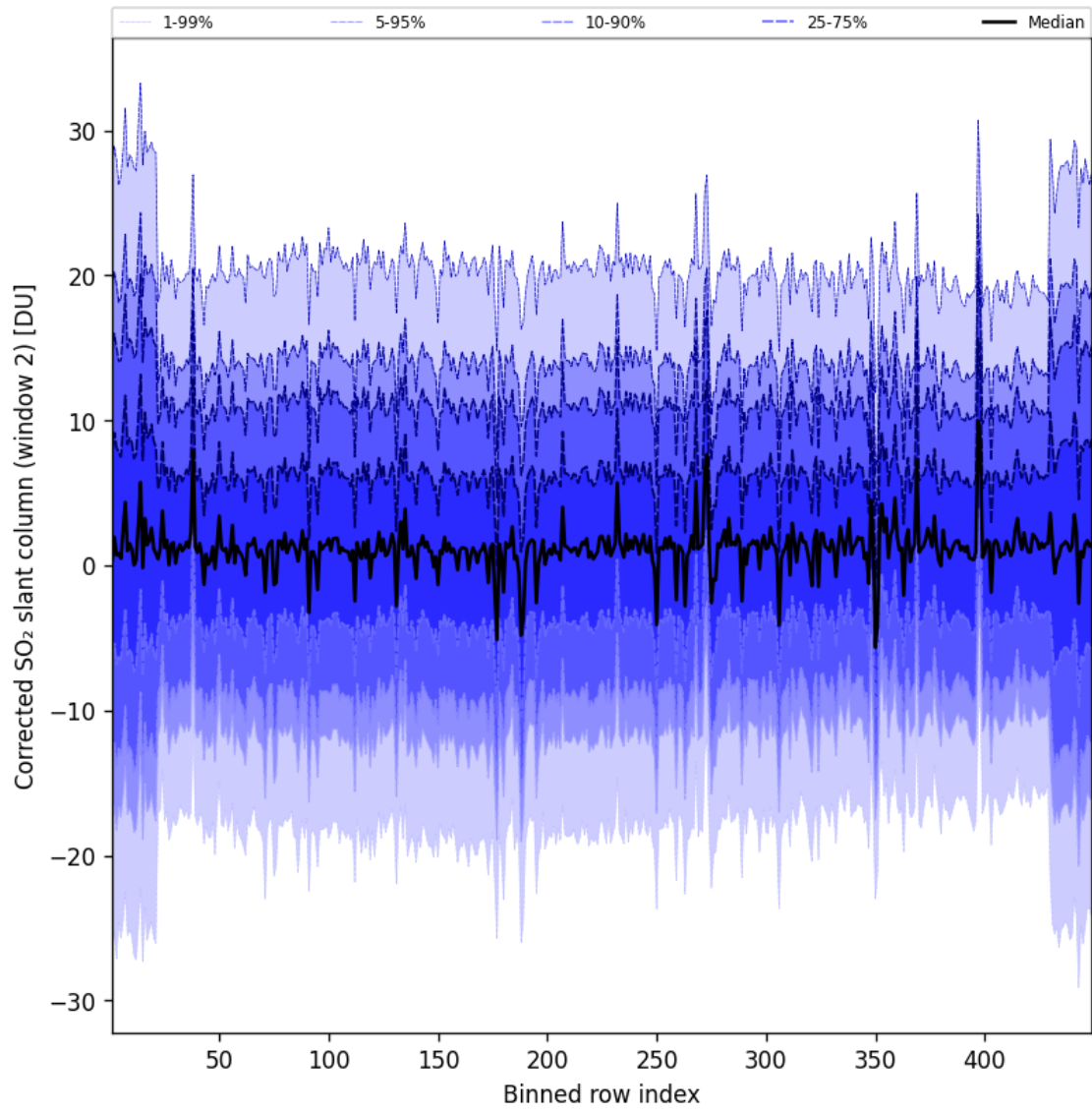
Figure 96: Along track statistics of “Corrected SO 2 slant column (window 2)” for 2025-01-05 to 2025-01-05
