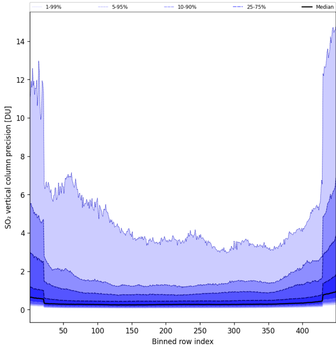
Figure 86: Along track statistics of "SO 2 vertical column precision" for 2025-01-05 to 2025-01-05
