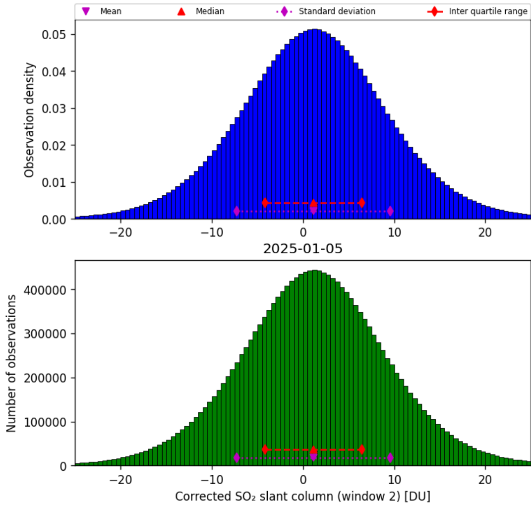
Figure 69: Histogram of “Corrected SO 2 slant column (window 2)” for 2025-01-05 to 2025-01-05
