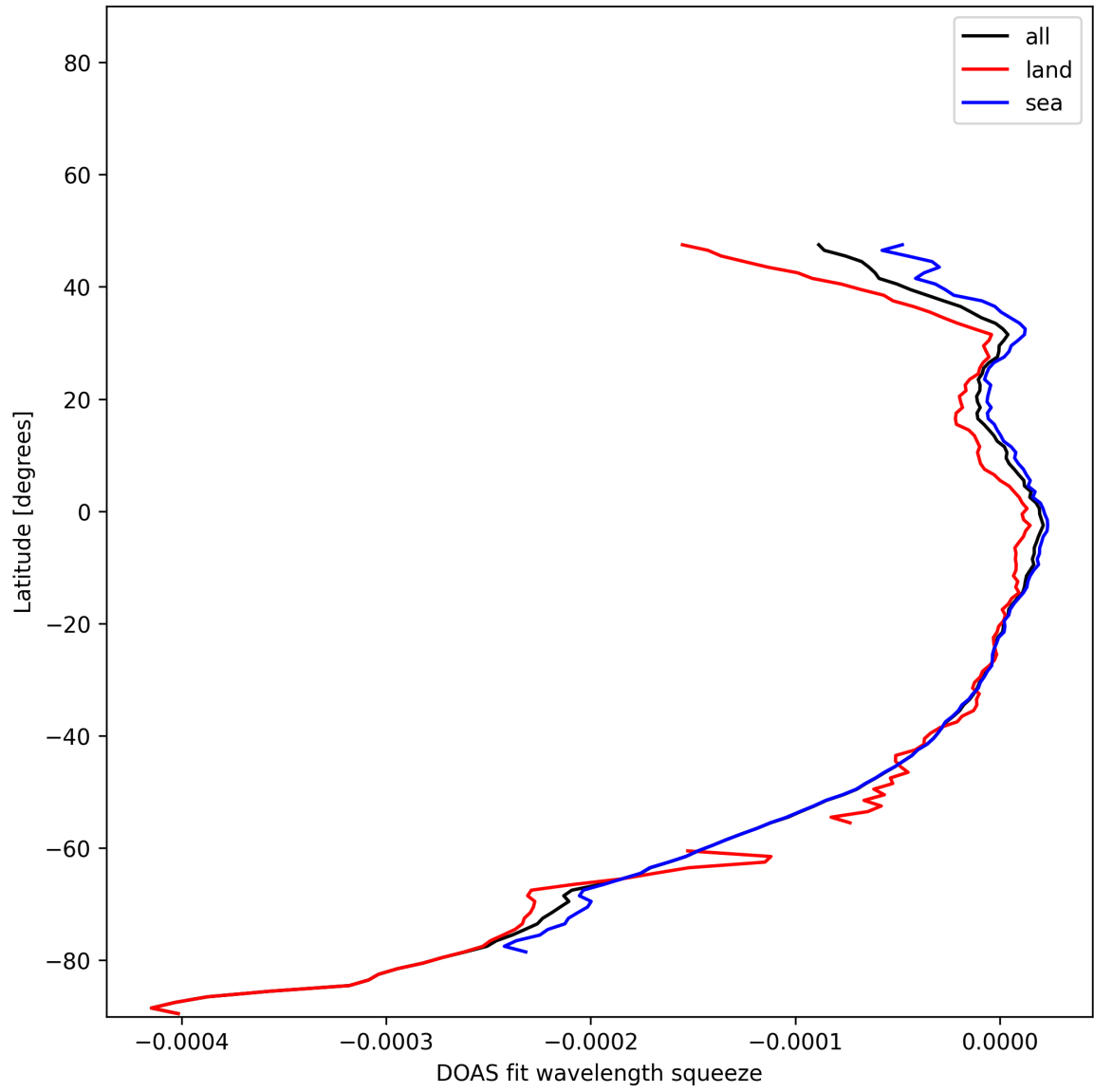
Figure 51: Zonal average of “DOAS fit wavelength squeeze” for 2025-01-05 to 2025-01-05.
