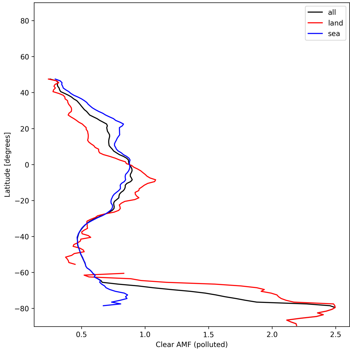
Figure 55: Zonal average of “Clear AMF (polluted)” for 2025-01-05 to 2025-01-05.
