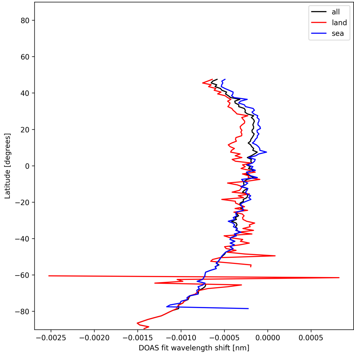
Figure 50: Zonal average of "DOAS fit wavelength shift" for 2025-01-05 to 2025-01-05.
