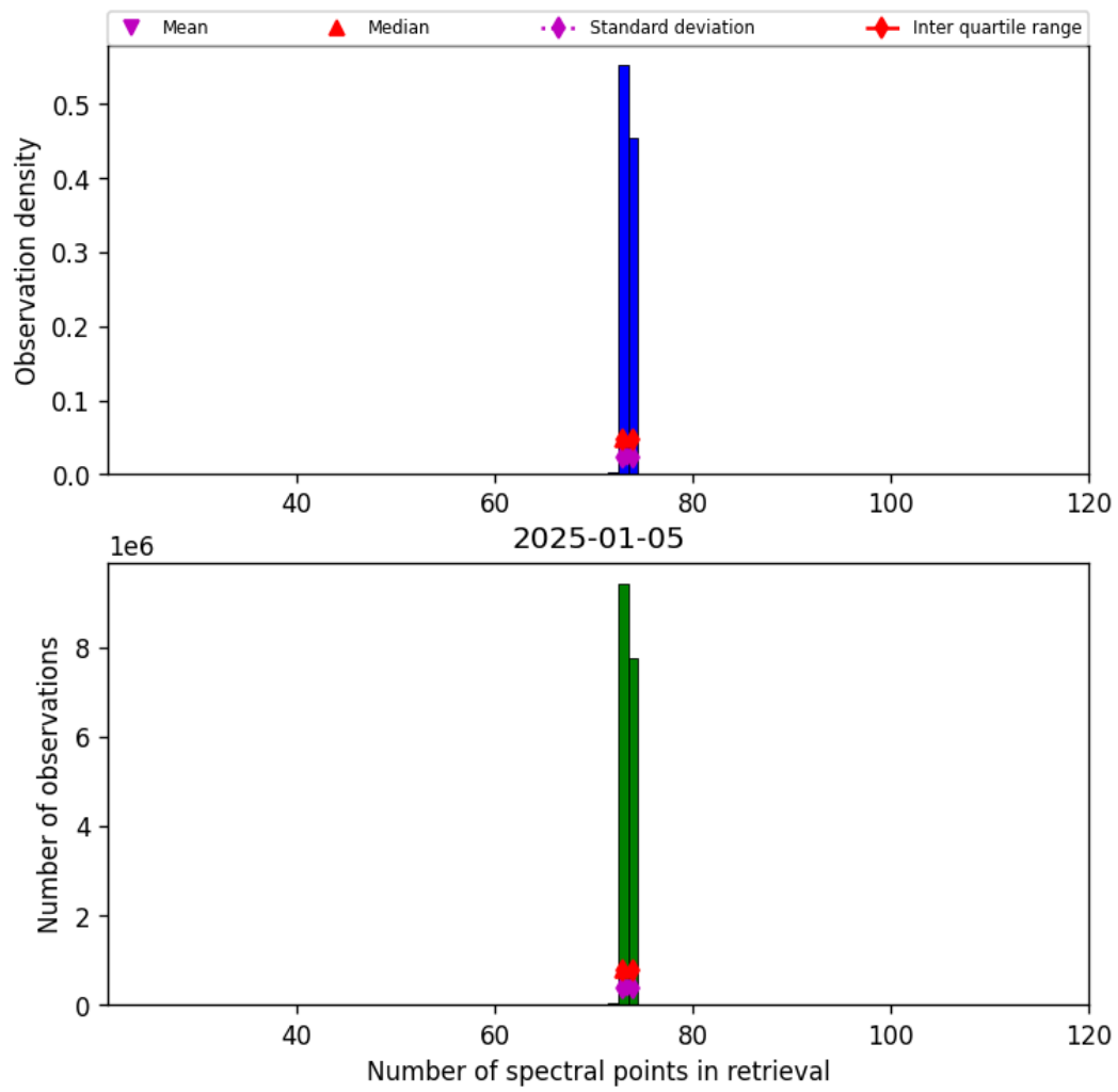
Figure 83: Histogram of “Number of spectral points in retrieval” for 2025-01-05 to 2025-01-05
