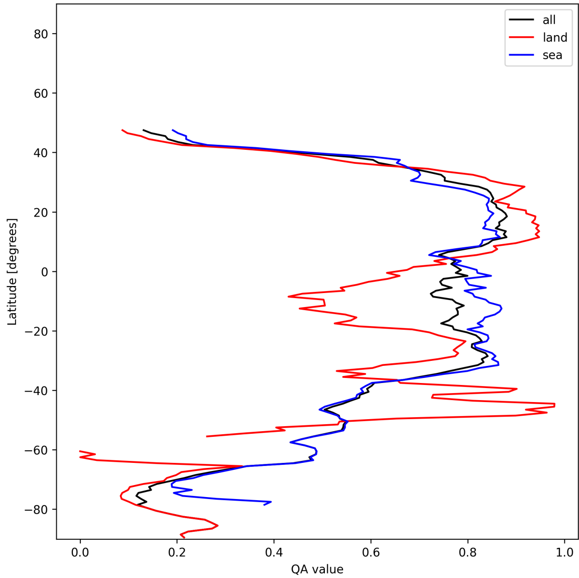
Figure 30: Zonal average of “QA value” for 2025-01-05 to 2025-01-05.
