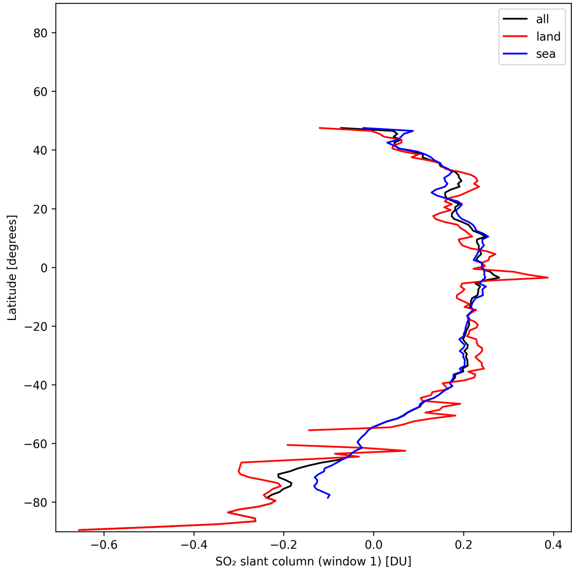
Figure 36: Zonal average of “SO 2 slant column (window 1)” for 2025-01-05 to 2025-01-05.
