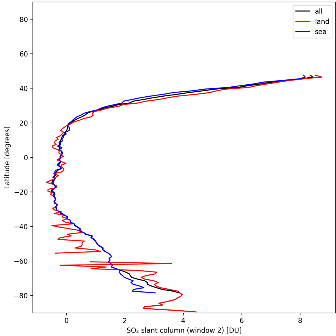
Figure 40: Zonal average of “SO 2 slant column (window 2)” for 2025-01-05 to 2025-01-05.
