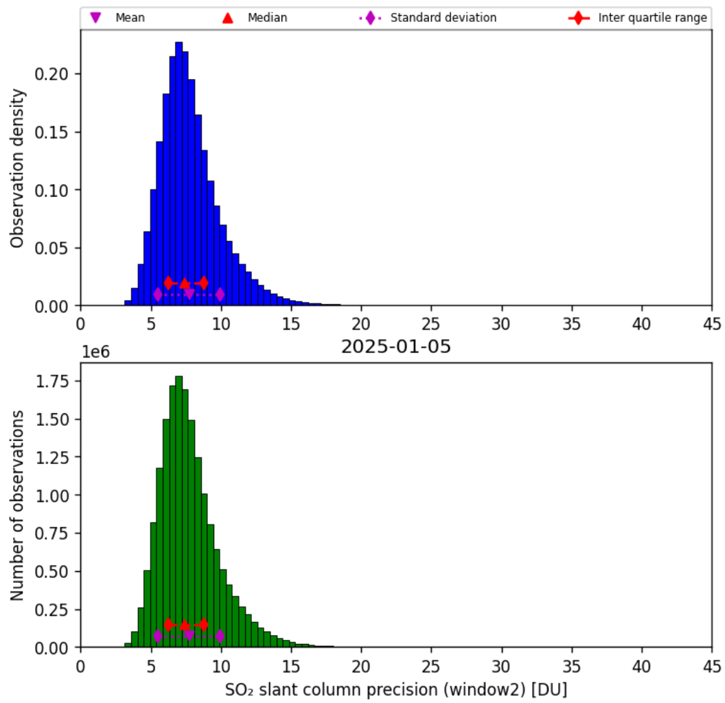
Figure 68: Histogram of “SO 2 slant column precision (window2)” for 2025-01-05 to 2025-01-05
