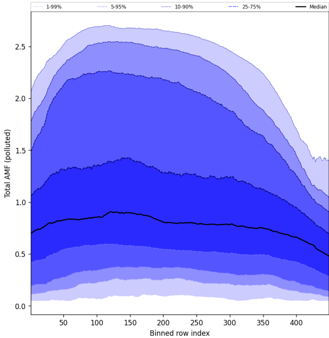
Figure 107: Along track statistics of “Total AMF (polluted)” for 2025-01-05 to 2025-01-05
