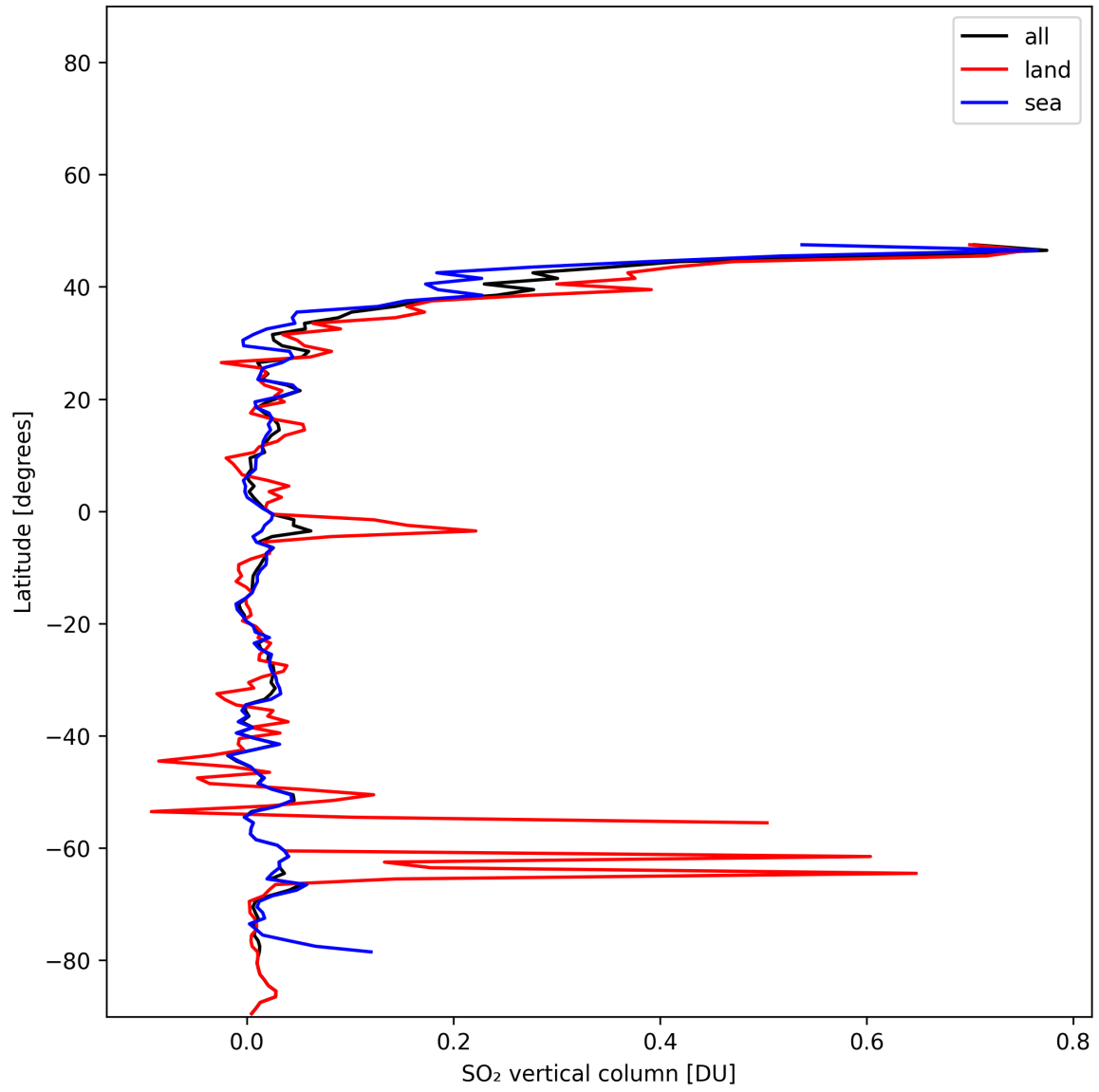
Figure 31: Zonal average of “SO 2 vertical column” for 2025-01-05 to 2025-01-05.
