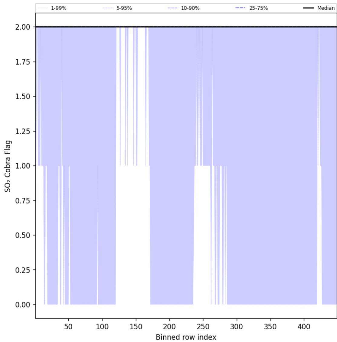
Figure 102: Along track statistics of "SO 2 Cobra Flag" for 2025-01-05 to 2025-01-05
