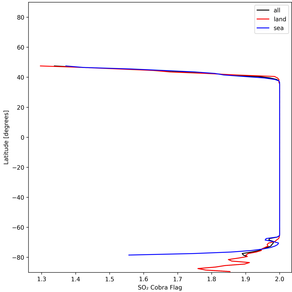
Figure 48: Zonal average of “SO 2 Cobra Flag” for 2025-01-05 to 2025-01-05.
