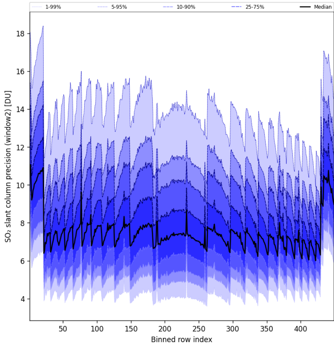
Figure 95: Along track statistics of “SO 2 slant column precision (window2)” for 2025-01-05 to 2025-01-05
