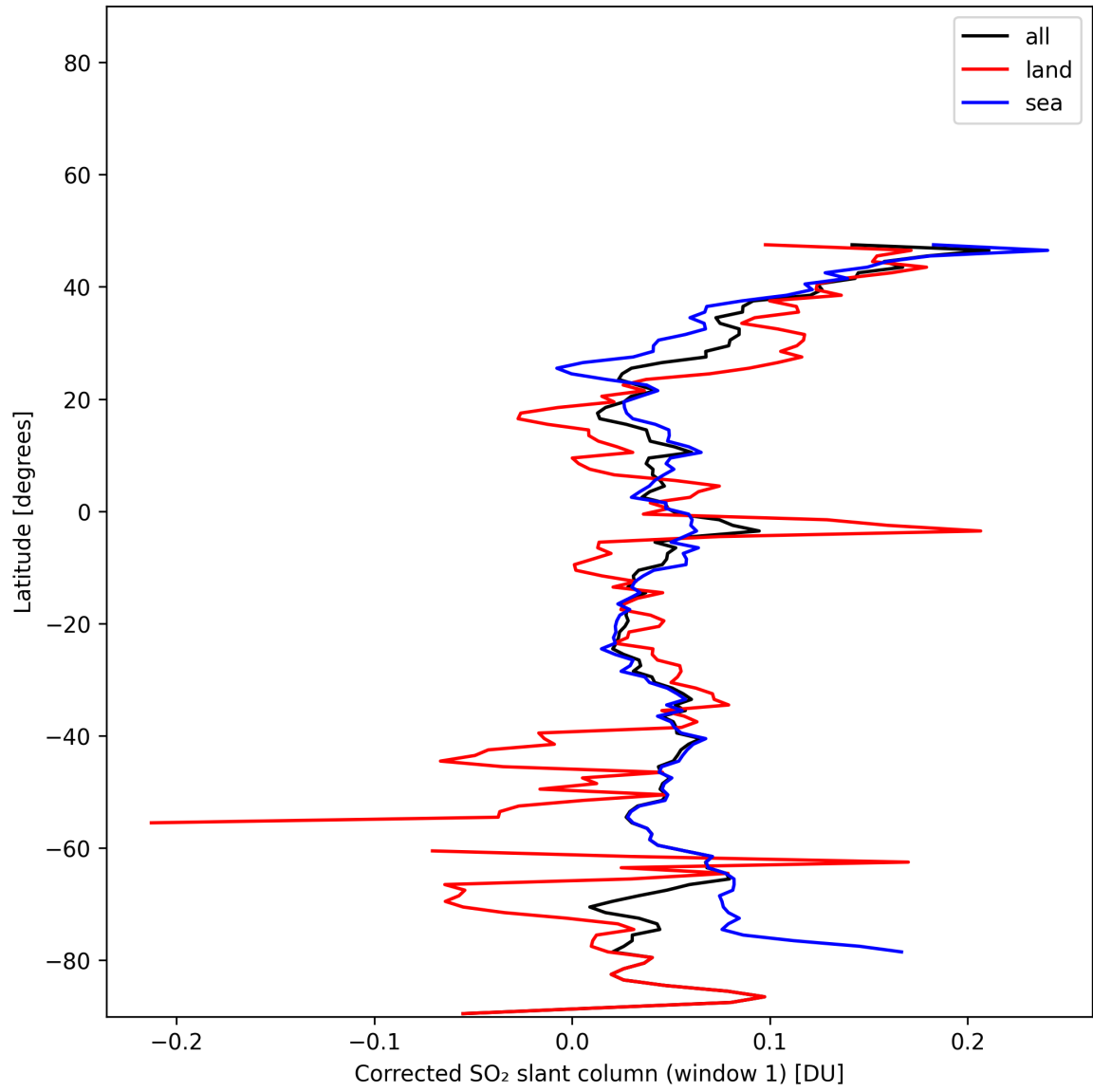
Figure 38: Zonal average of “Corrected SO 2 slant column (window 1)” for 2025-01-05 to 2025-01-05.
