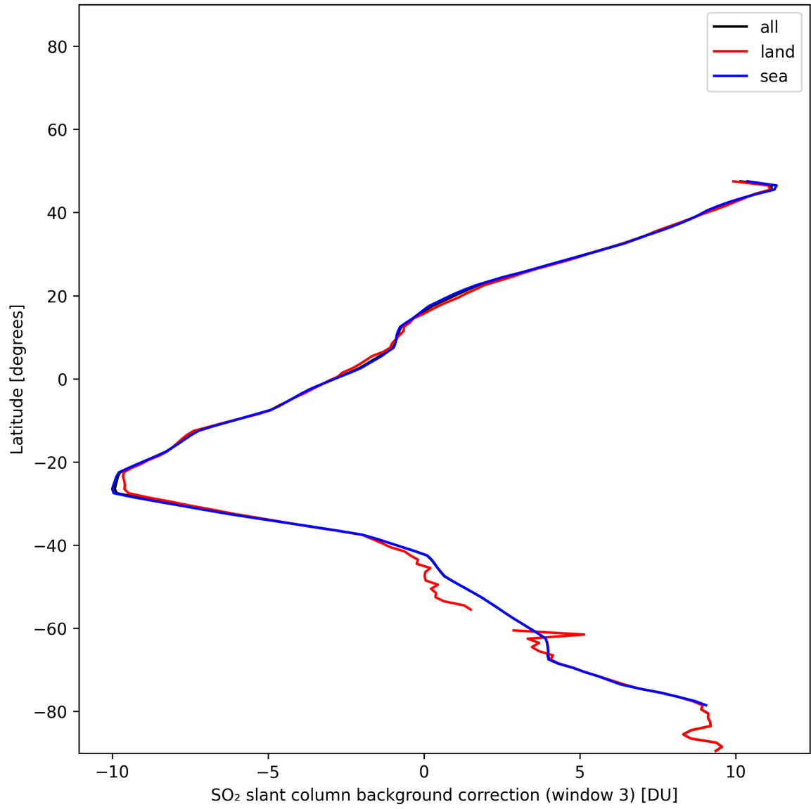
Figure 47: Zonal average of “SO 2 slant column background correction (window 3)” for 2025-01-05 to 2025-01-05.
