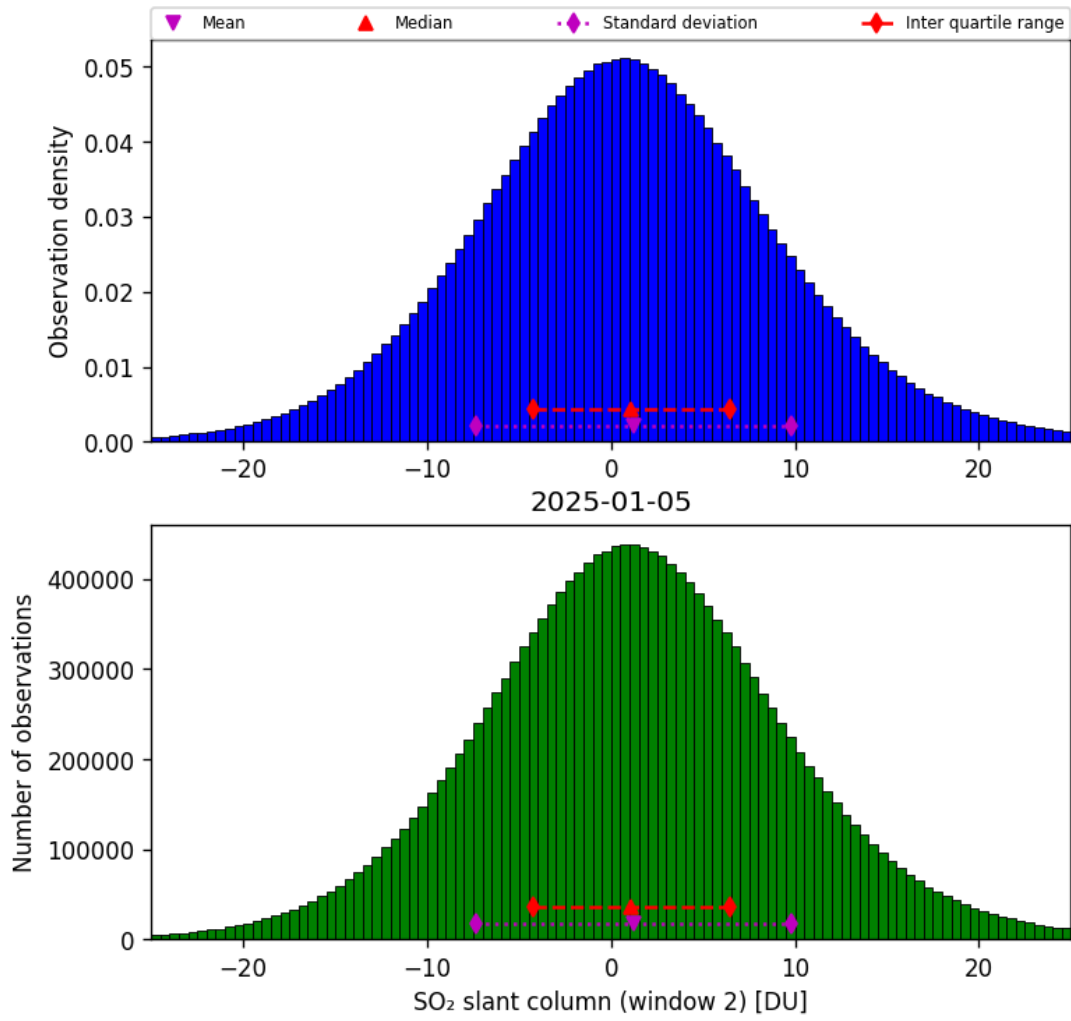
Figure 67: Histogram of “SO 2 slant column (window 2)” for 2025-01-05 to 2025-01-05
