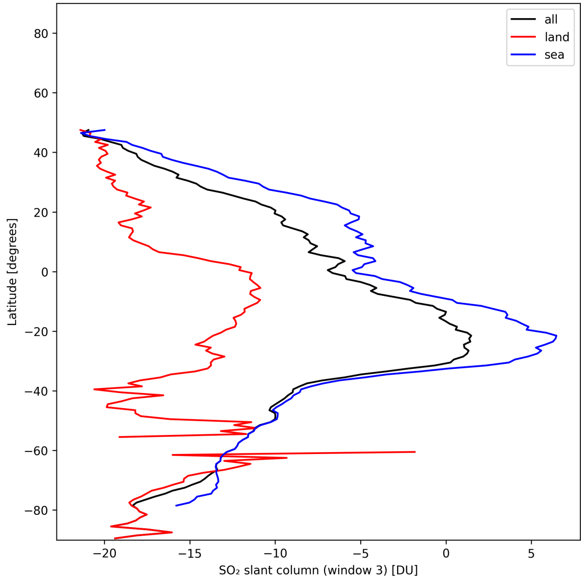
Figure 44: Zonal average of “SO 2 slant column (window 3)” for 2025-01-05 to 2025-01-05.
