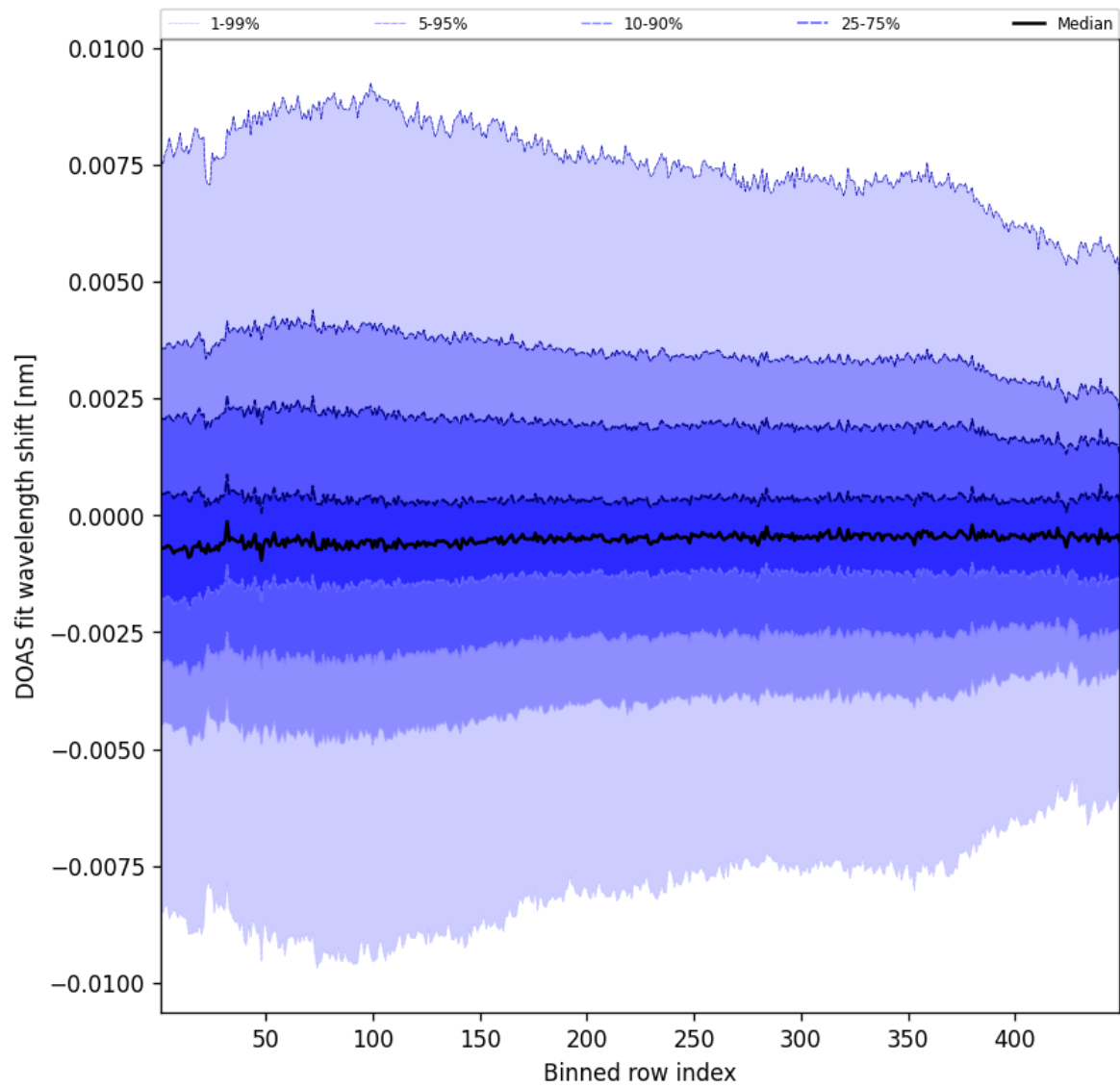
Figure 104: Along track statistics of “DOAS fit wavelength shift” for 2025-01-05 to 2025-01-05
