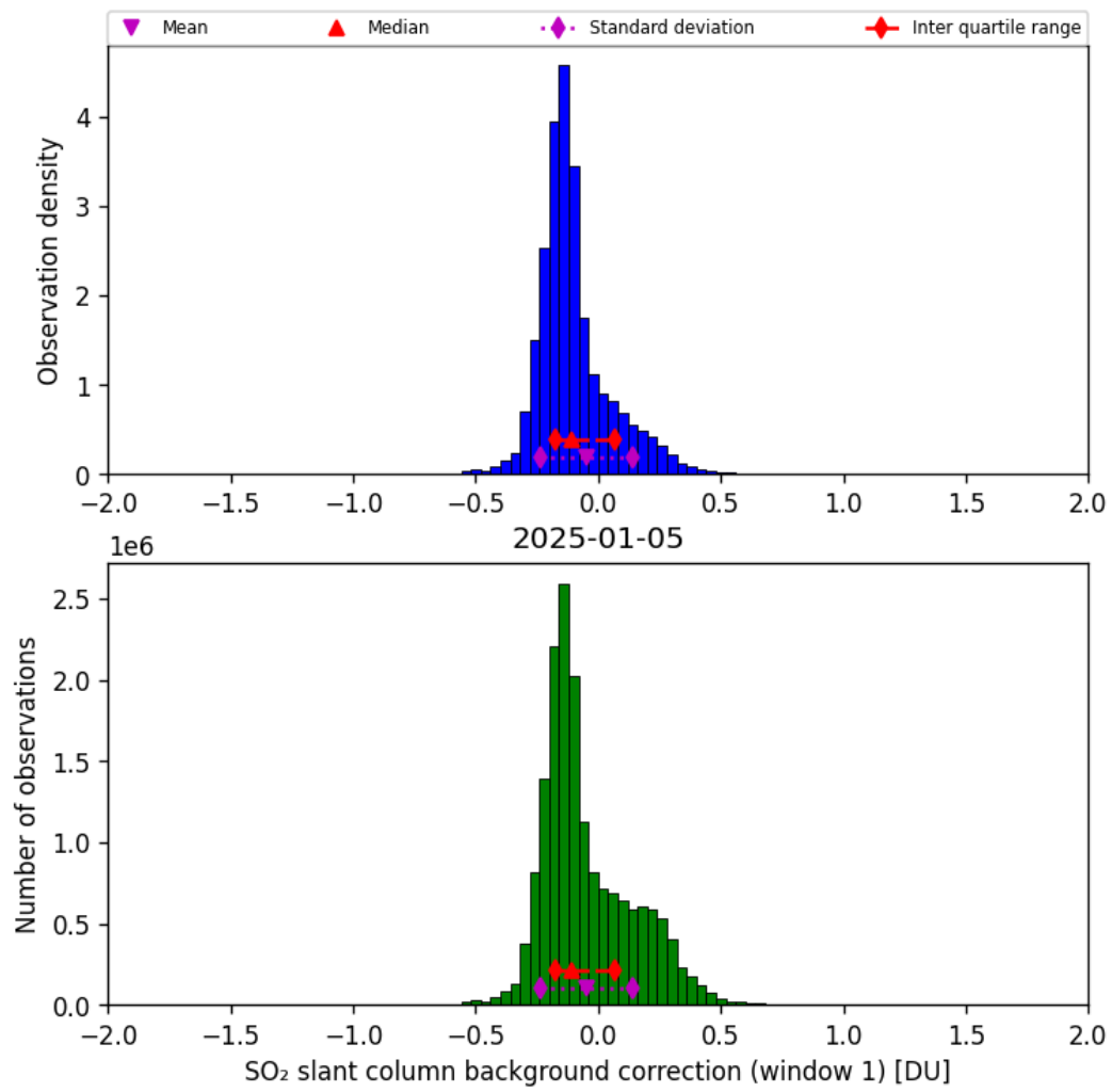
Figure 66: Histogram of “SO 2 slant column background correction (window 1)” for 2025-01-05 to 2025-01-05
