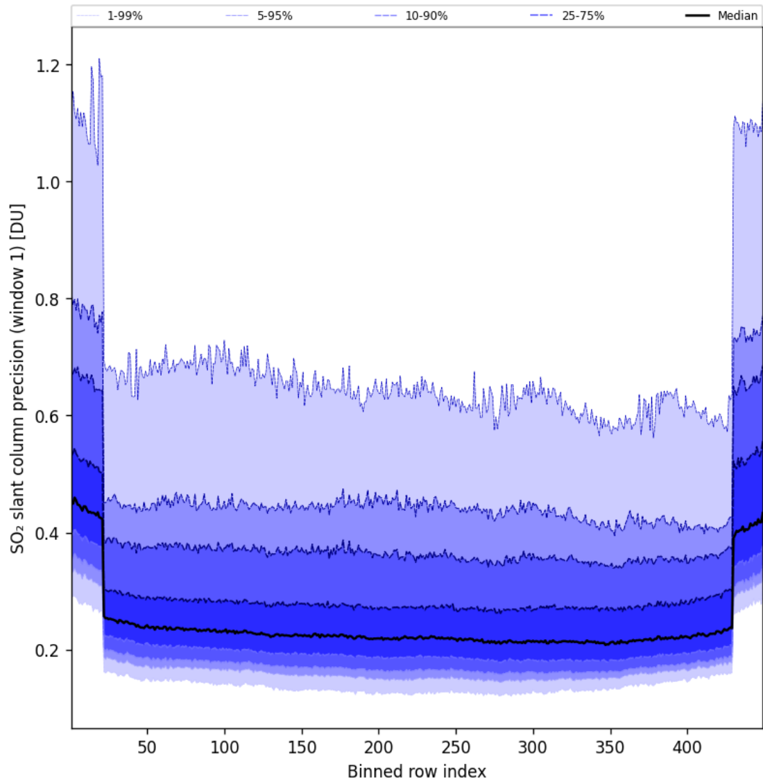
Figure 91: Along track statistics of “SO 2 slant column precision (window 1)” for 2025-01-05 to 2025-01-05
