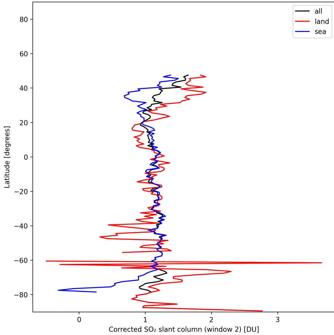
Figure 42: Zonal average of “Corrected SO 2 slant column (window 2)” for 2025-01-05 to 2025-01-05.
