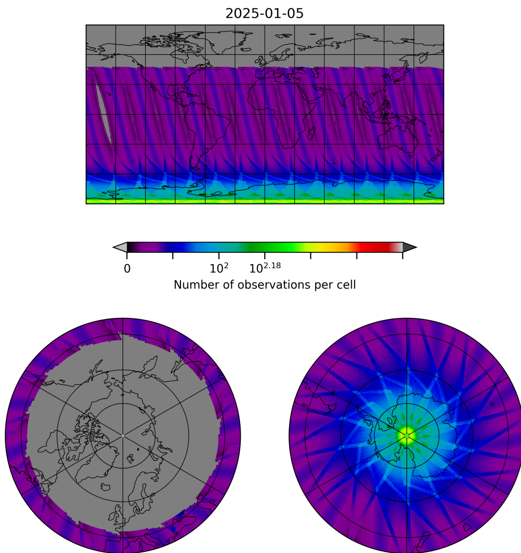
Figure 29: Map of the number of observations for 2025-01-05 to 2025-01-05
