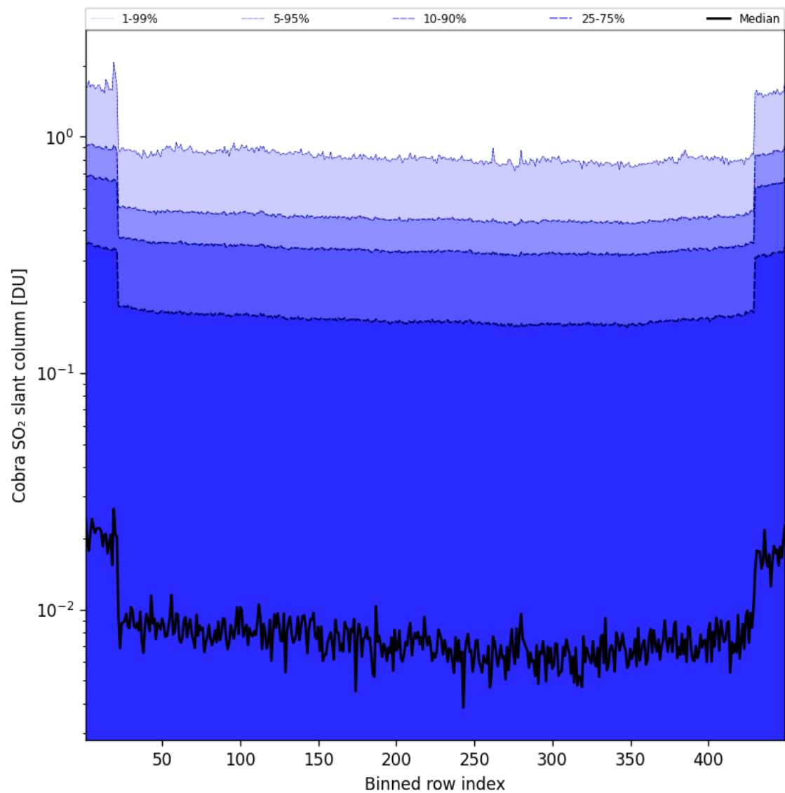
Figure 88: Along track statistics of “Cobra SO 2 slant column” for 2025-01-05 to 2025-01-05
