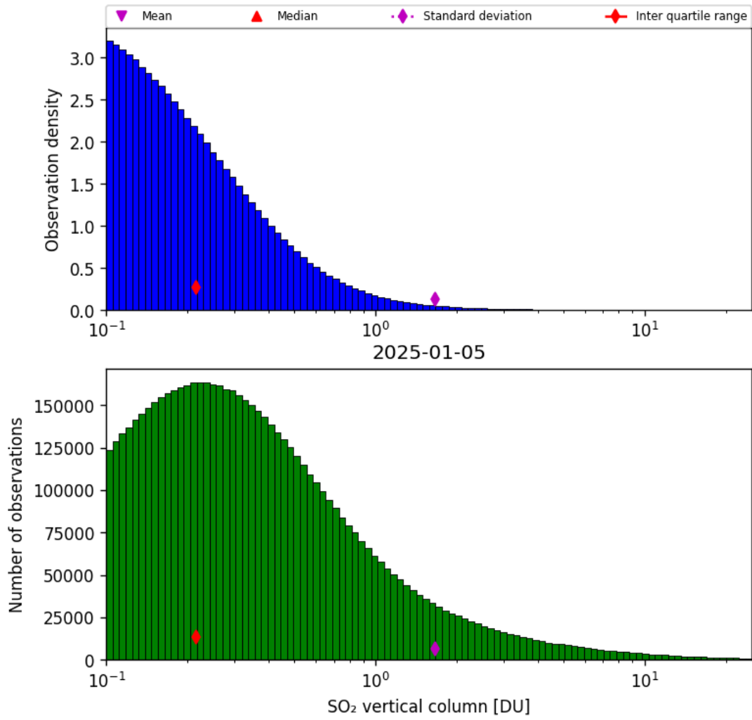
Figure 58: Histogram of “SO 2 vertical column” for 2025-01-05 to 2025-01-05
