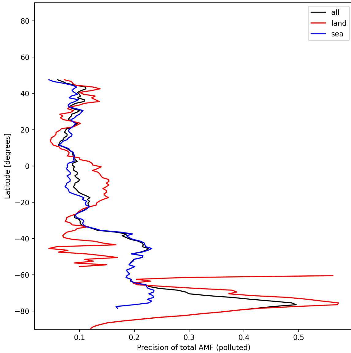
Figure 54: Zonal average of “Precision of total AMF (polluted)” for 2025-01-05 to 2025-01-05.
