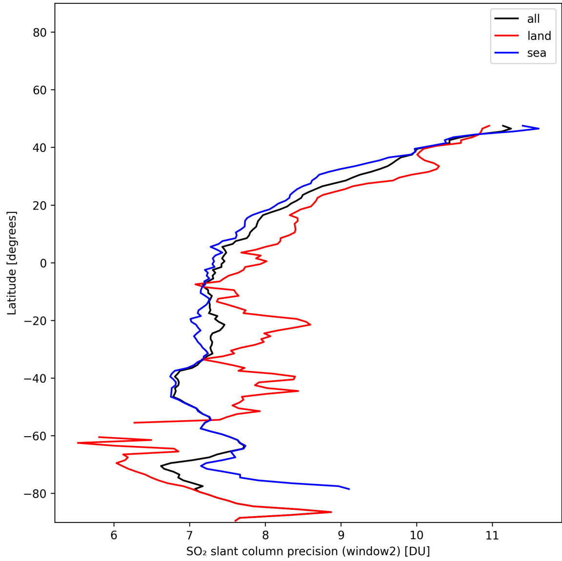
Figure 41: Zonal average of “SO 2 slant column precision (window2)” for 2025-01-05 to 2025-01-05.
