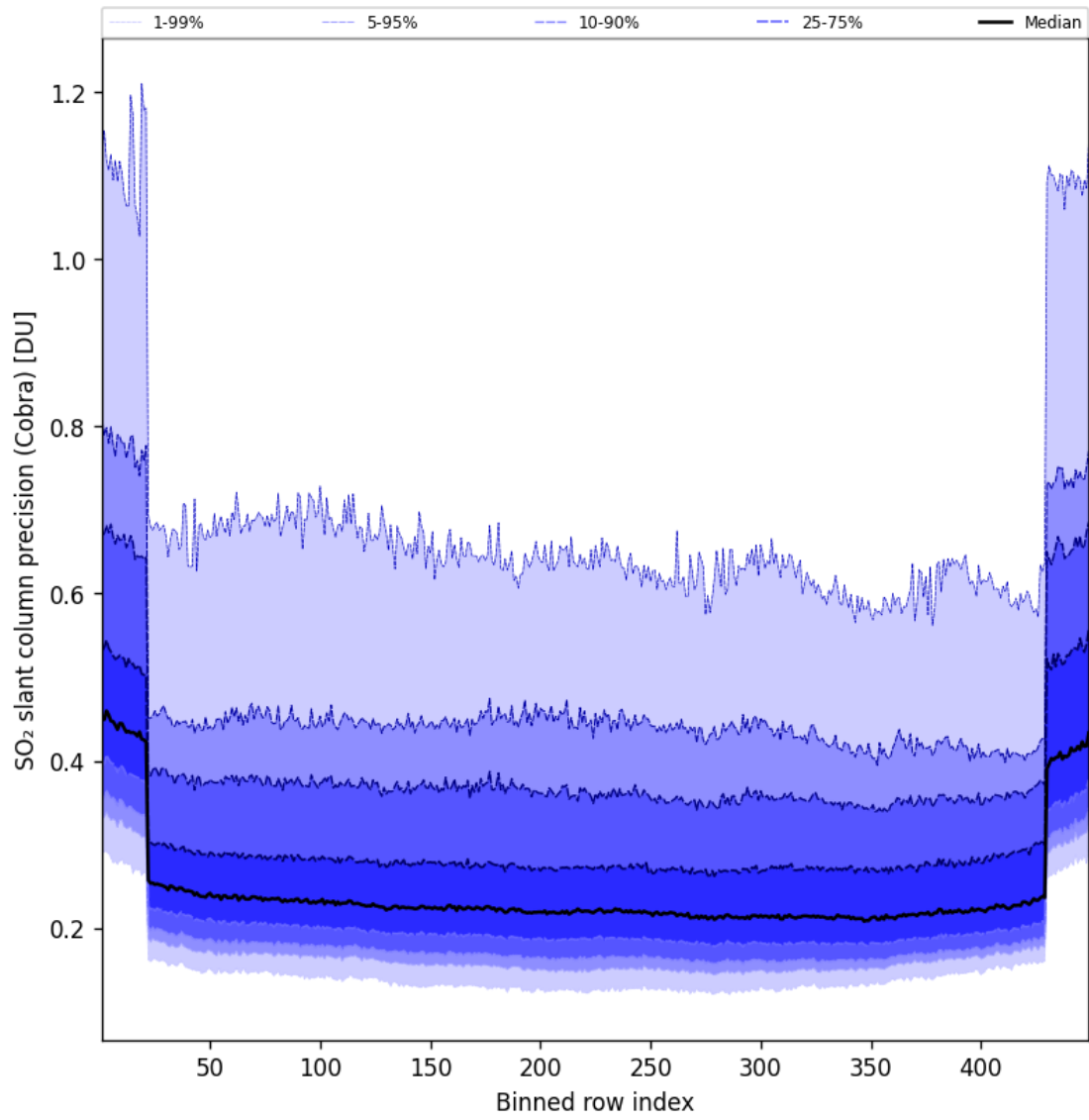
Figure 89: Along track statistics of “SO 2 slant column precision (Cobra)” for 2025-01-05 to 2025-01-05
