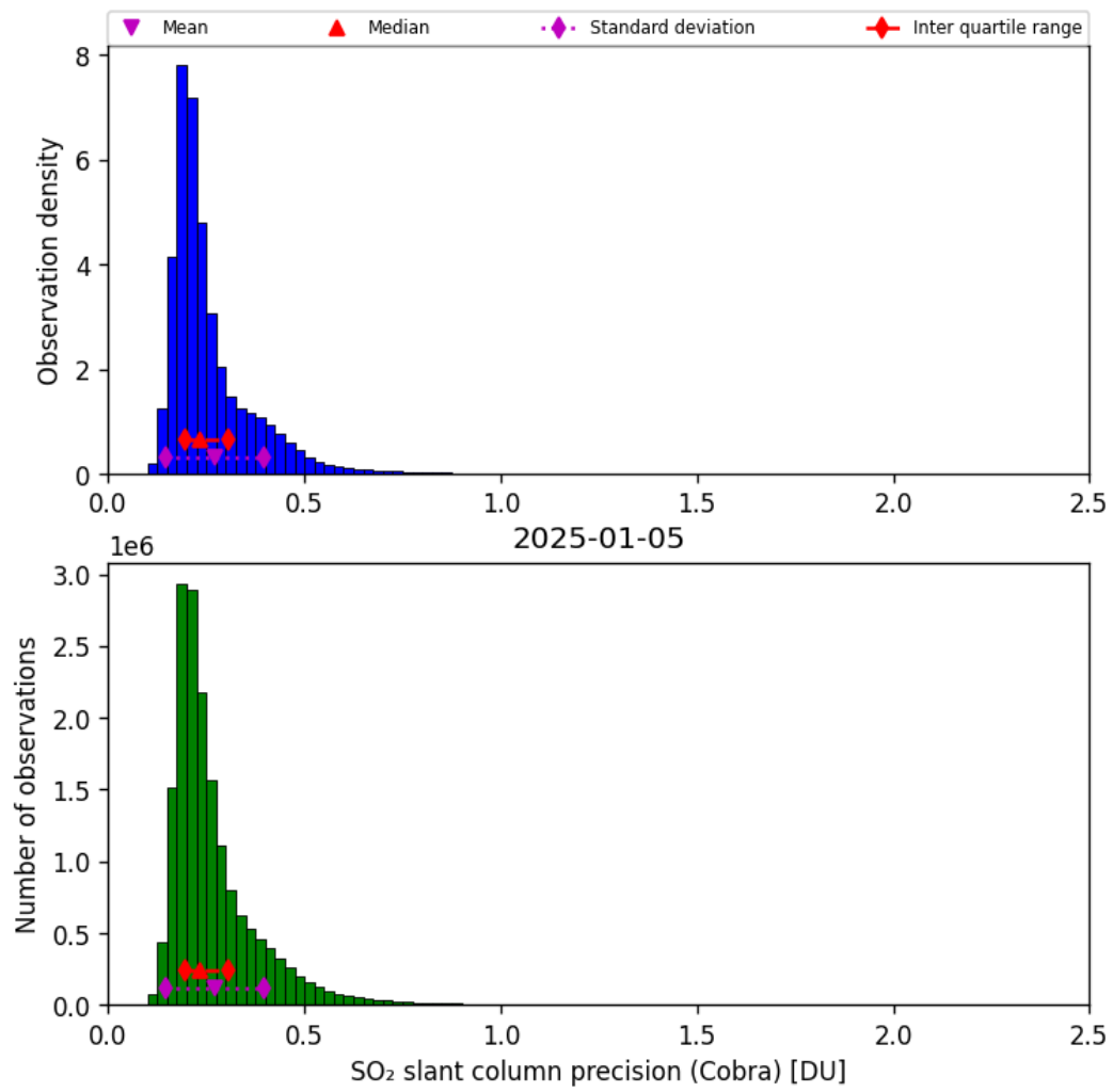
Figure 62: Histogram of “SO 2 slant column precision (Cobra)” for 2025-01-05 to 2025-01-05
