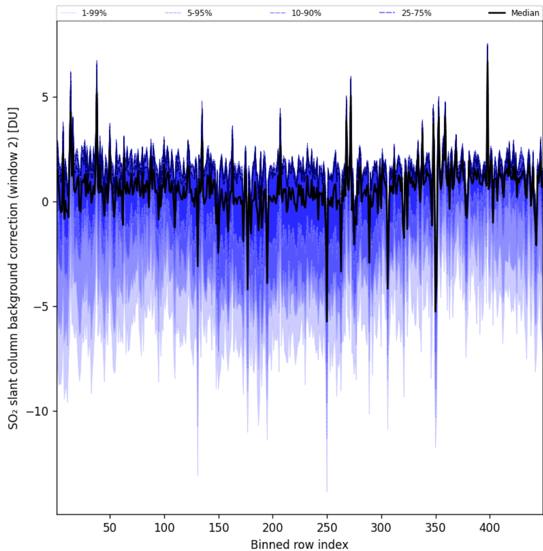
Figure 97: Along track statistics of “SO 2 slant column background correction (window 2)” for 2025-01-05 to 2025-01-05
