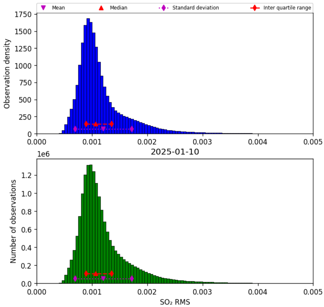
Figure 79: Histogram of “SO 2 RMS” for 2025-01-10 to 2025-01-10
