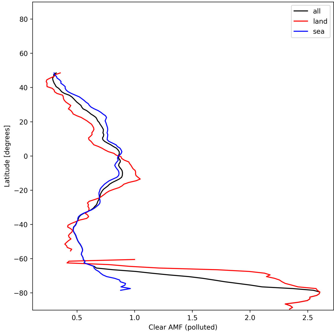
Figure 55: Zonal average of “Clear AMF (polluted)” for 2025-01-10 to 2025-01-10.
