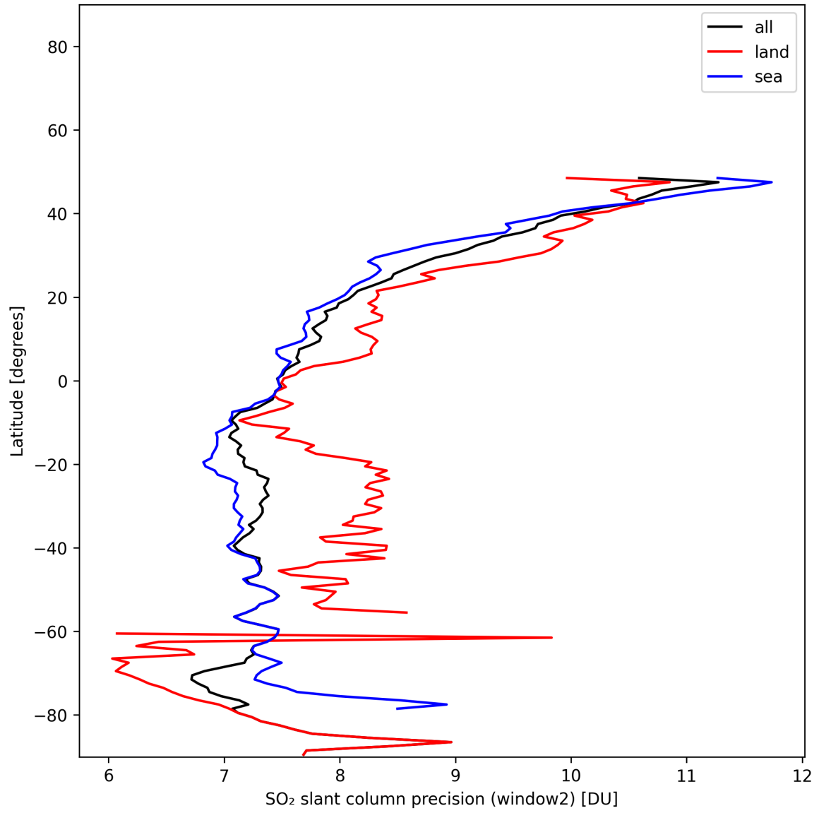
Figure 41: Zonal average of “SO 2 slant column precision (window2)” for 2025-01-10 to 2025-01-10.
