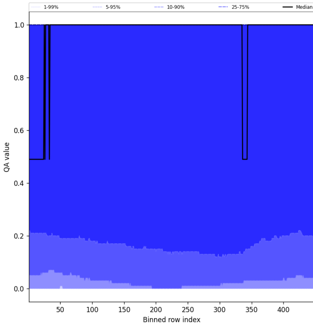
Figure 84: Along track statistics of “QA value” for 2025-01-10 to 2025-01-10
