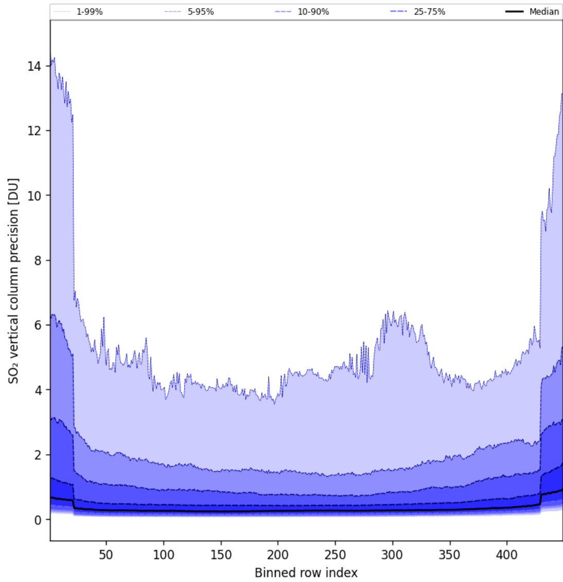
Figure 86: Along track statistics of “SO 2 vertical column precision” for 2025-01-10 to 2025-01-10
