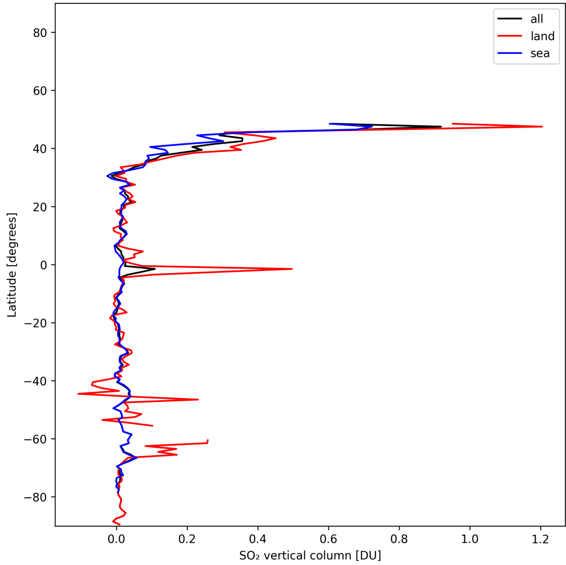
Figure 31: Zonal average of “SO 2 vertical column” for 2025-01-10 to 2025-01-10.
