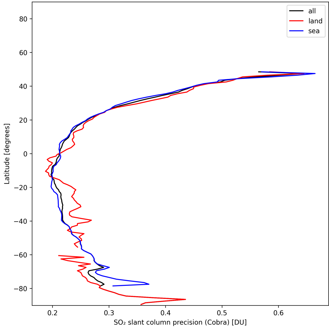
Figure 35: Zonal average of “SO 2 slant column precision (Cobra)” for 2025-01-10 to 2025-01-10.
