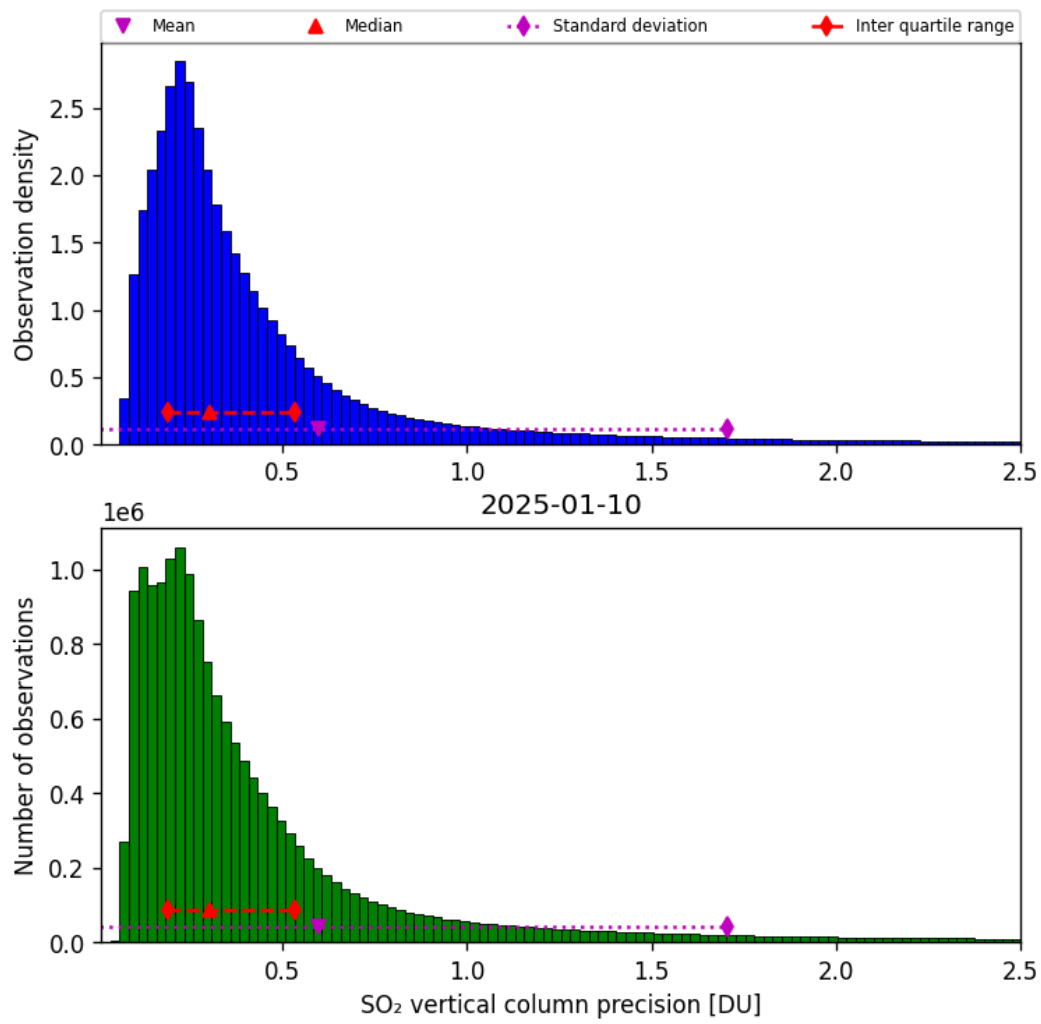
Figure 59: Histogram of "SO 2 vertical column precision" for 2025-01-10 to 2025-01-10
