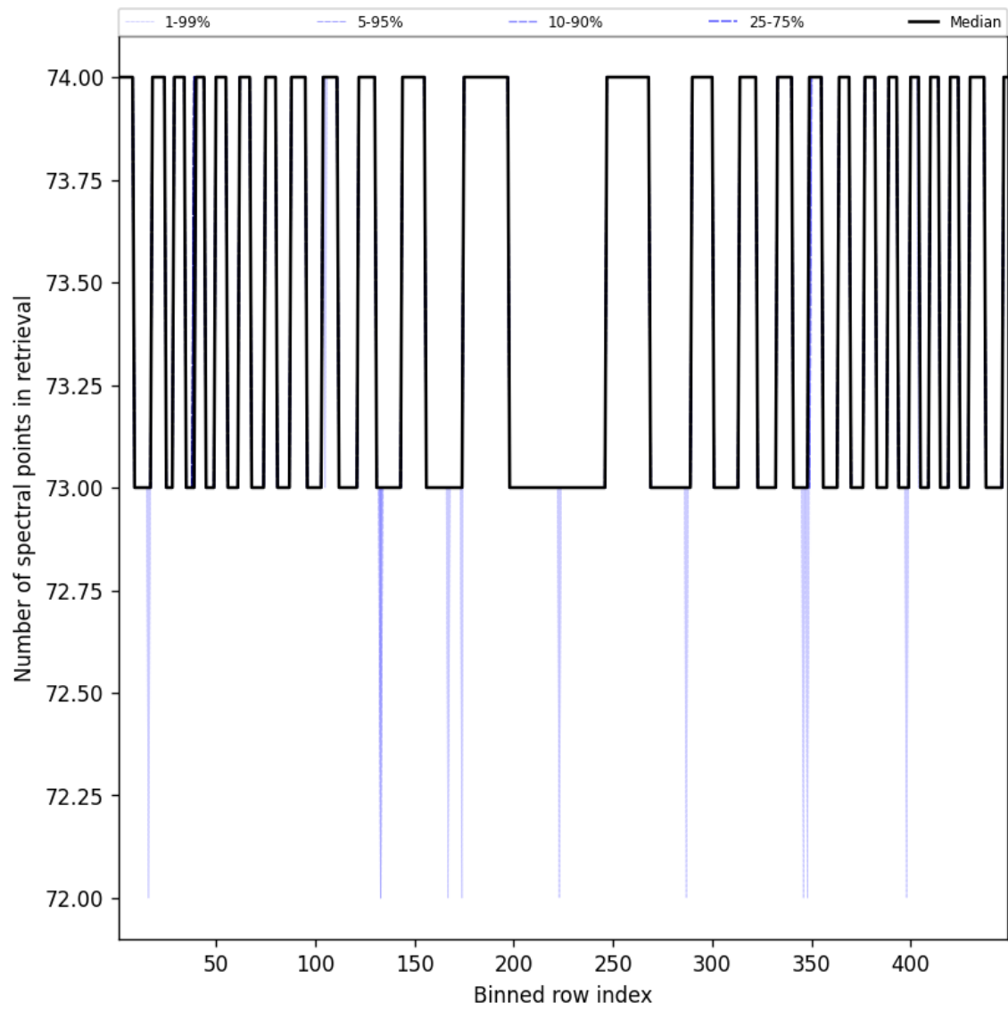
Figure 110: Along track statistics of “Number of spectral points in retrieval” for 2025-01-10 to 2025-01-10
