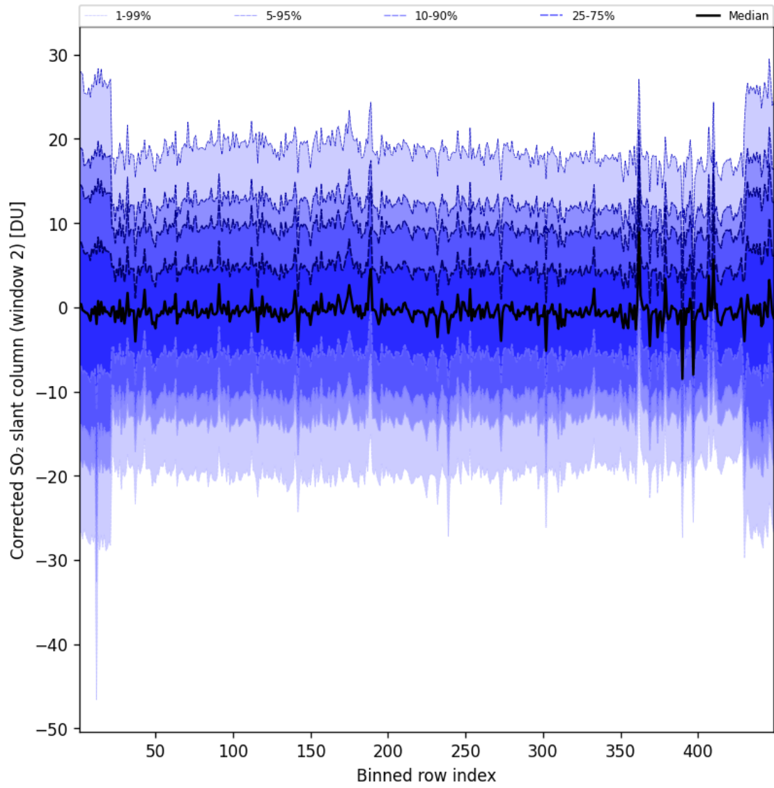
Figure 96: Along track statistics of “Corrected SO 2 slant column (window 2)” for 2025-01-10 to 2025-01-10
