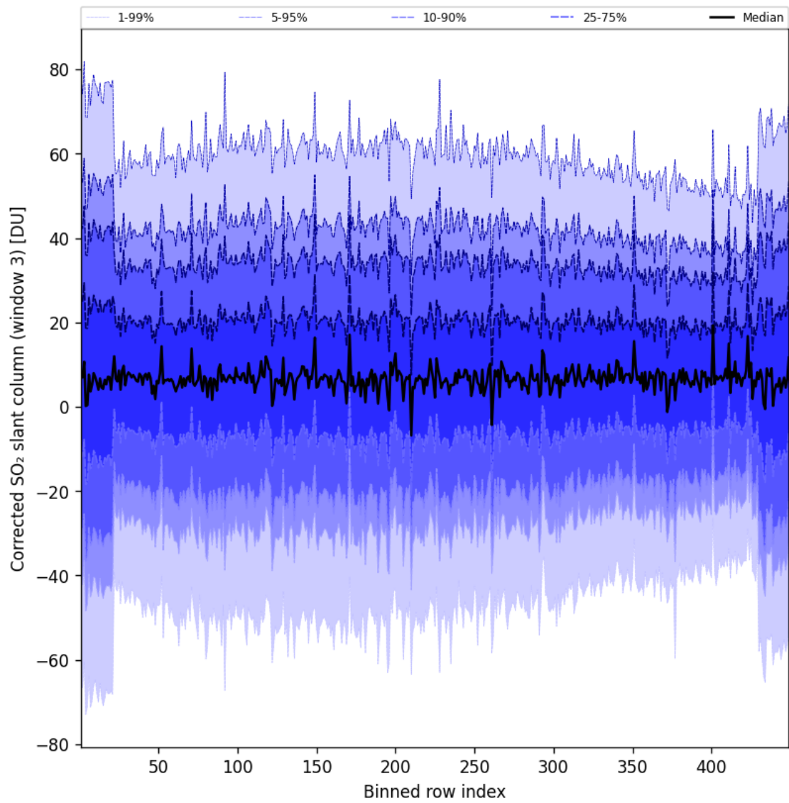
Figure 100: Along track statistics of “Corrected SO 2 slant column (window 3)” for 2025-01-10 to 2025-01-10
