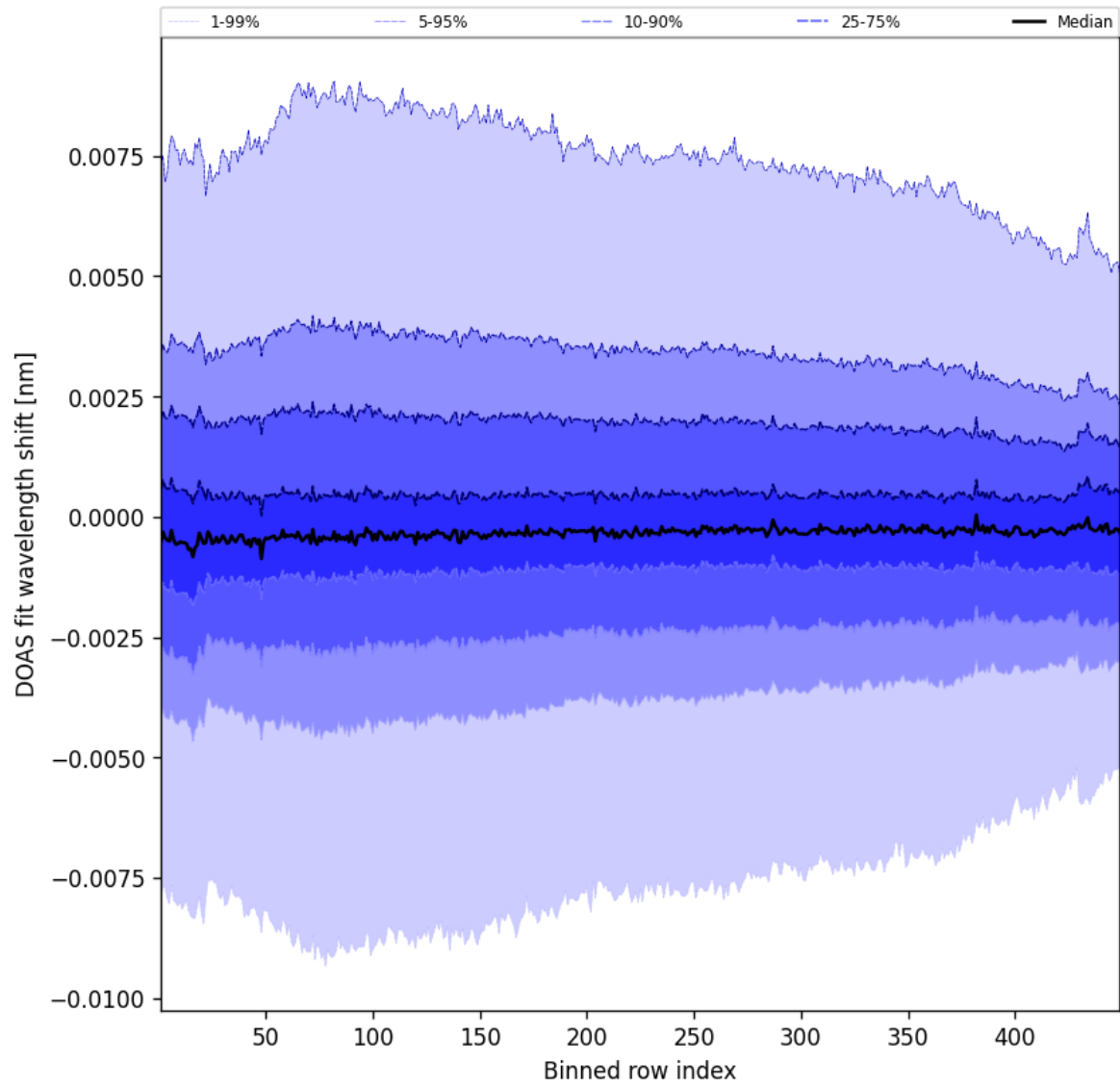
Figure 104: Along track statistics of “DOAS fit wavelength shift” for 2025-01-10 to 2025-01-10
