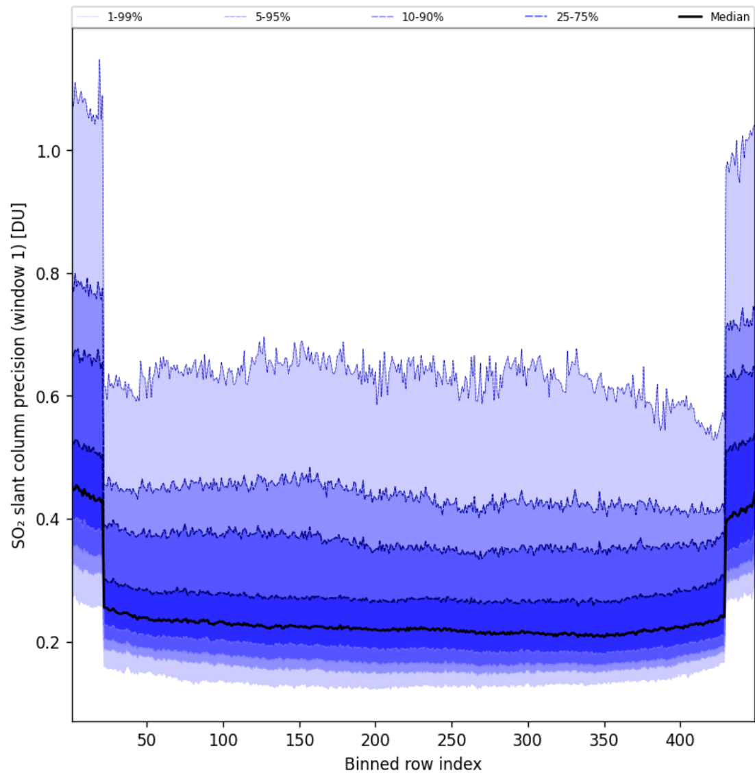
Figure 91: Along track statistics of “SO 2 slant column precision (window 1)” for 2025-01-10 to 2025-01-10
