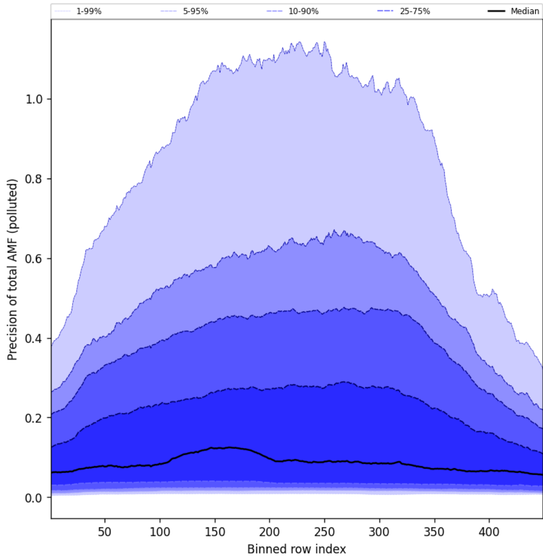
Figure 108: Along track statistics of “Precision of total AMF (polluted)” for 2025-01-10 to 2025-01-10
