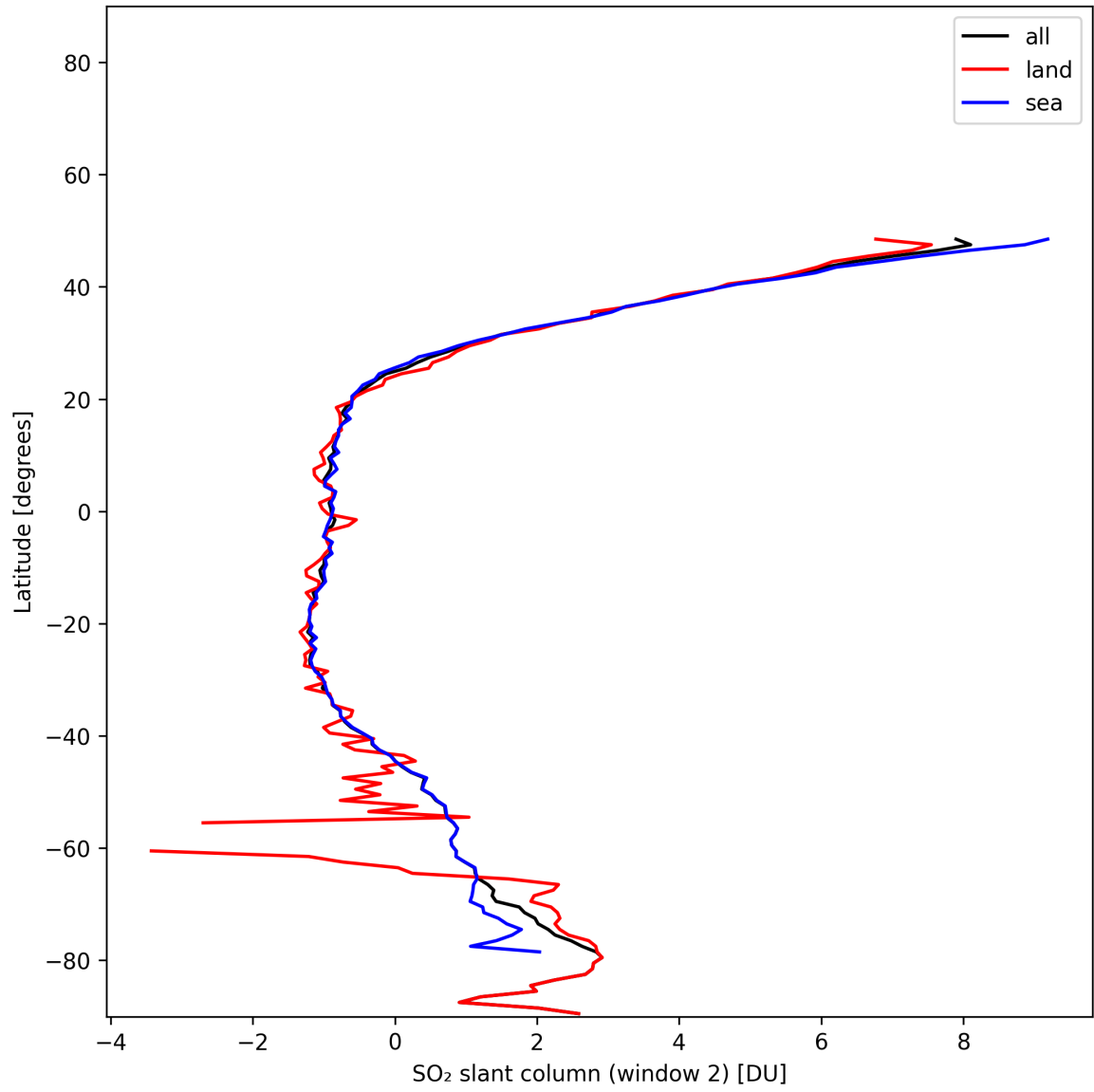
Figure 40: Zonal average of “SO 2 slant column (window 2)” for 2025-01-10 to 2025-01-10.
