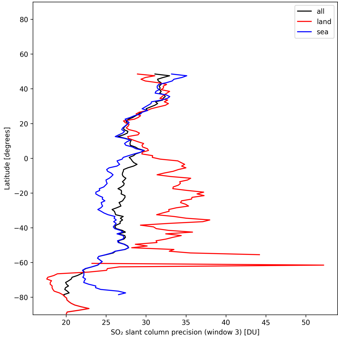
Figure 45: Zonal average of “SO 2 slant column precision (window 3)” for 2025-01-10 to 2025-01-10.
