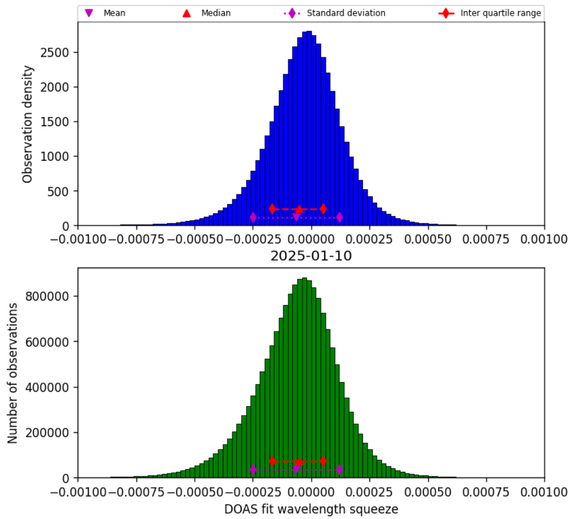
Figure 78: Histogram of “DOAS fit wavelength squeeze” for 2025-01-10 to 2025-01-10
