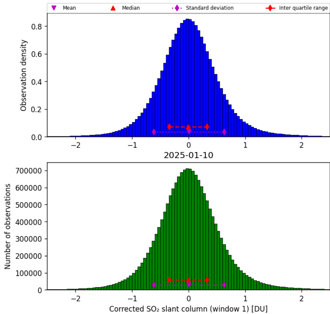
Figure 65: Histogram of “Corrected SO 2 slant column (window 1)” for 2025-01-10 to 2025-01-10
