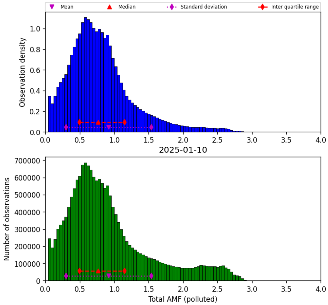
Figure 80: Histogram of “Total AMF (polluted)” for 2025-01-10 to 2025-01-10
