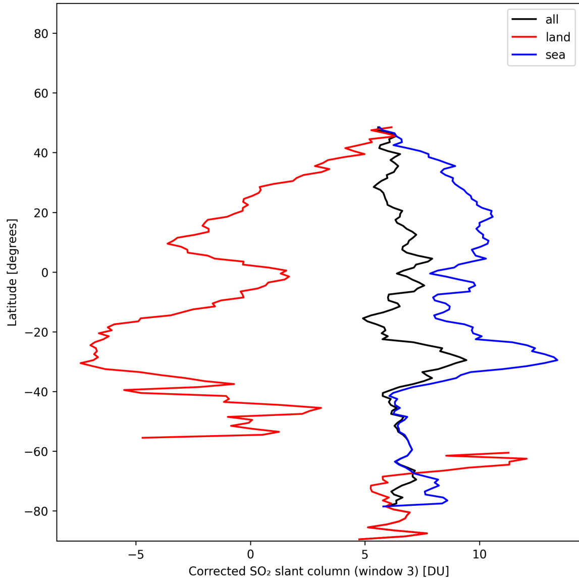
Figure 46: Zonal average of “Corrected SO 2 slant column (window 3)” for 2025-01-10 to 2025-01-10.
