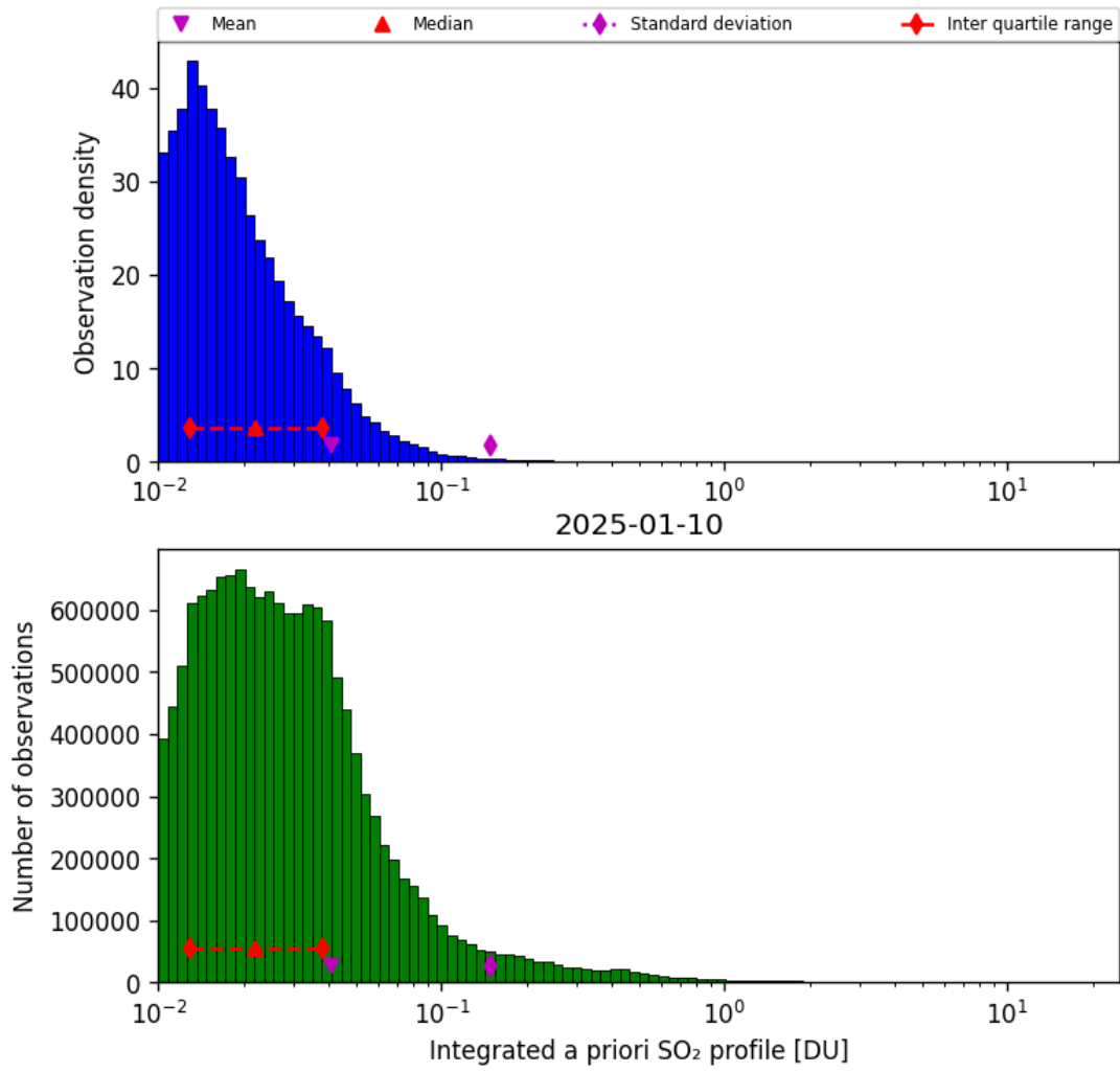
Figure 76: Histogram of “Integrated a priori SO 2 profile” for 2025-01-10 to 2025-01-10
