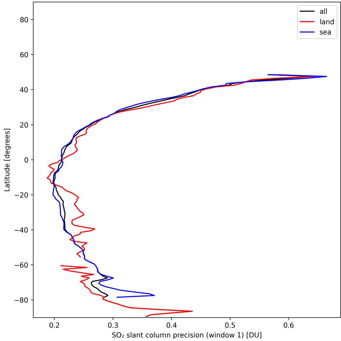
Figure 37: Zonal average of “SO 2 slant column precision (window 1)” for 2025-01-10 to 2025-01-10.
