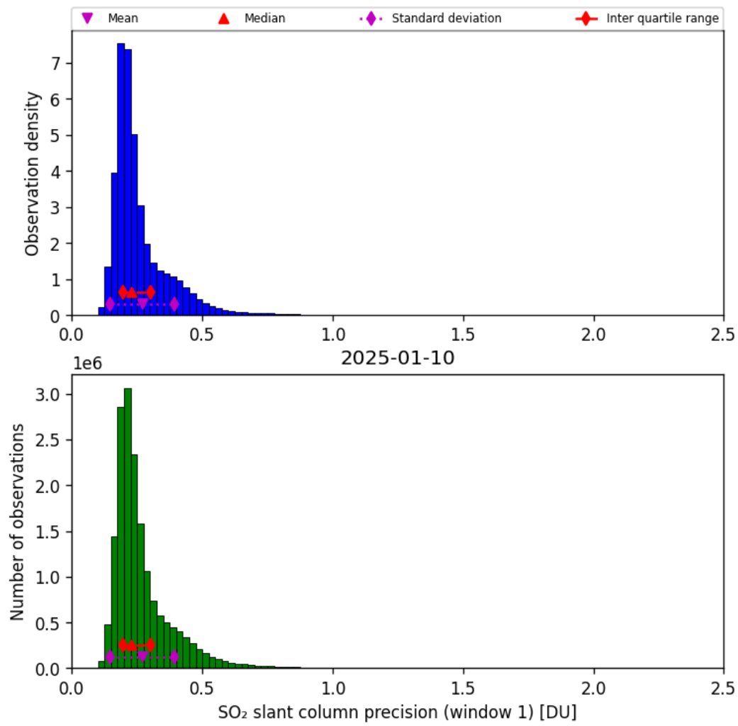
Figure 64: Histogram of “SO 2 slant column precision (window 1)” for 2025-01-10 to 2025-01-10
