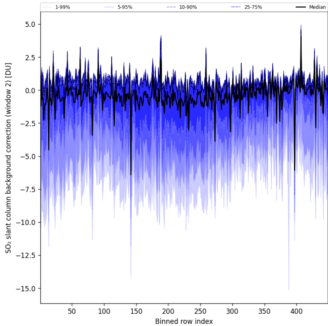
Figure 97: Along track statistics of “SO 2 slant column background correction (window 2)” for 2025-01-10 to 2025-01-10
