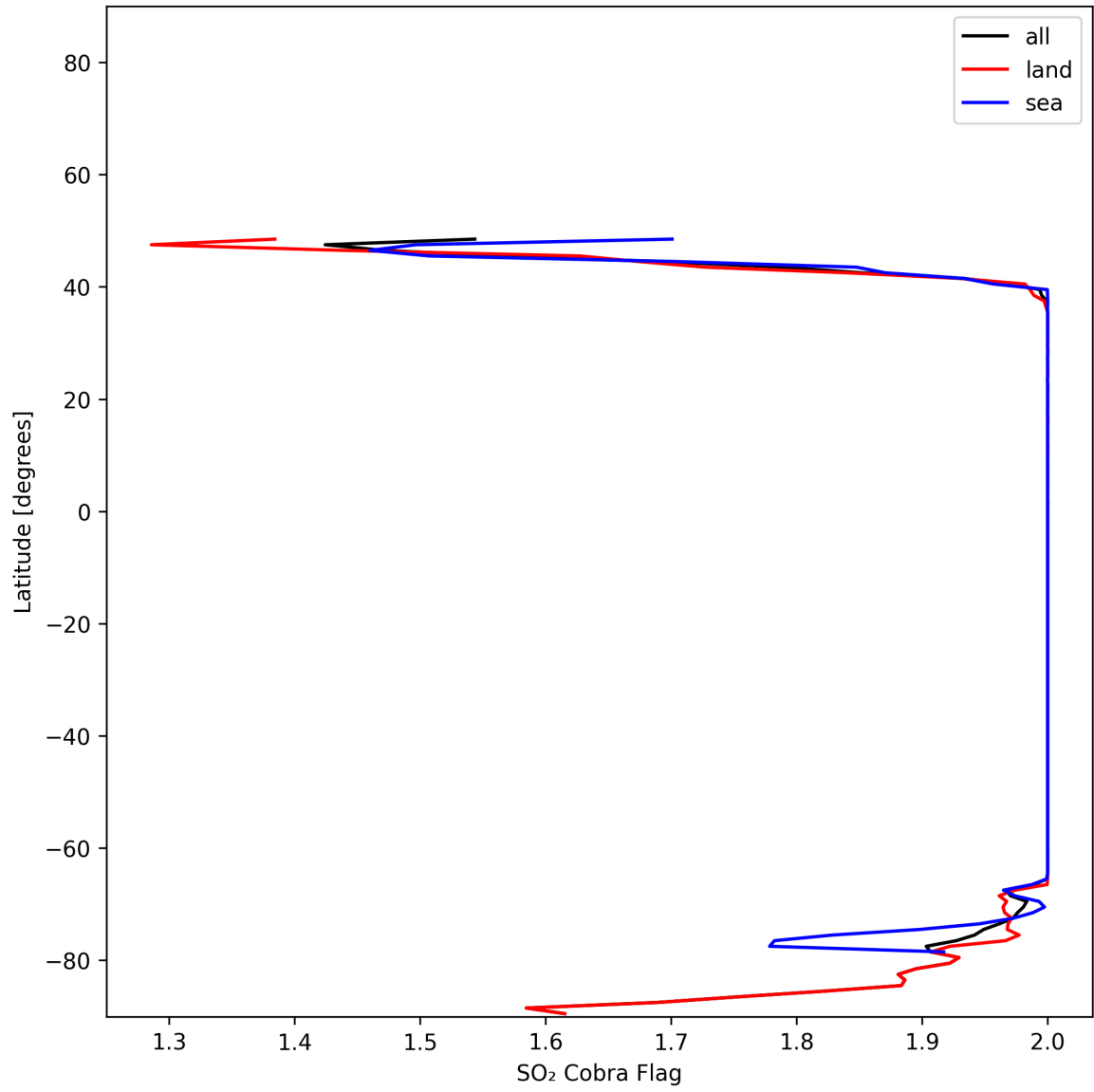
Figure 48: Zonal average of "SO 2 Cobra Flag" for 2025-01-10 to 2025-01-10.
