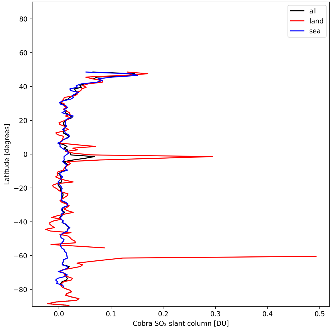
Figure 34: Zonal average of “Cobra SO 2 slant column” for 2025-01-10 to 2025-01-10.
