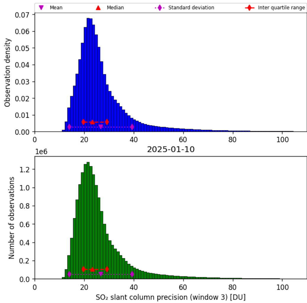
Figure 72: Histogram of “SO 2 slant column precision (window 3)” for 2025-01-10 to 2025-01-10
