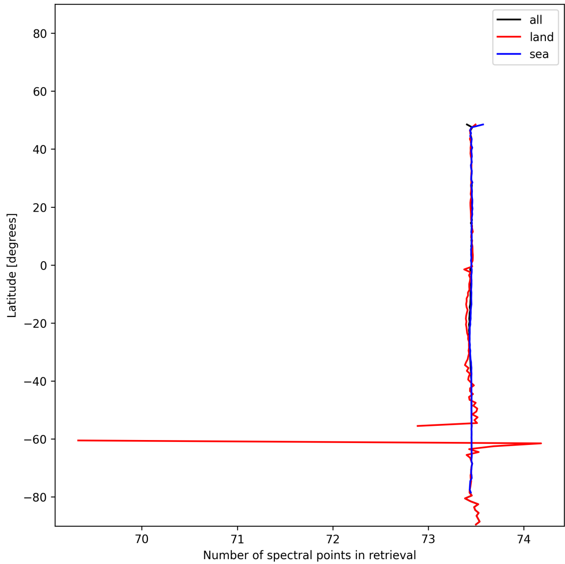
Figure 56: Zonal average of “Number of spectral points in retrieval” for 2025-01-10 to 2025-01-10.
