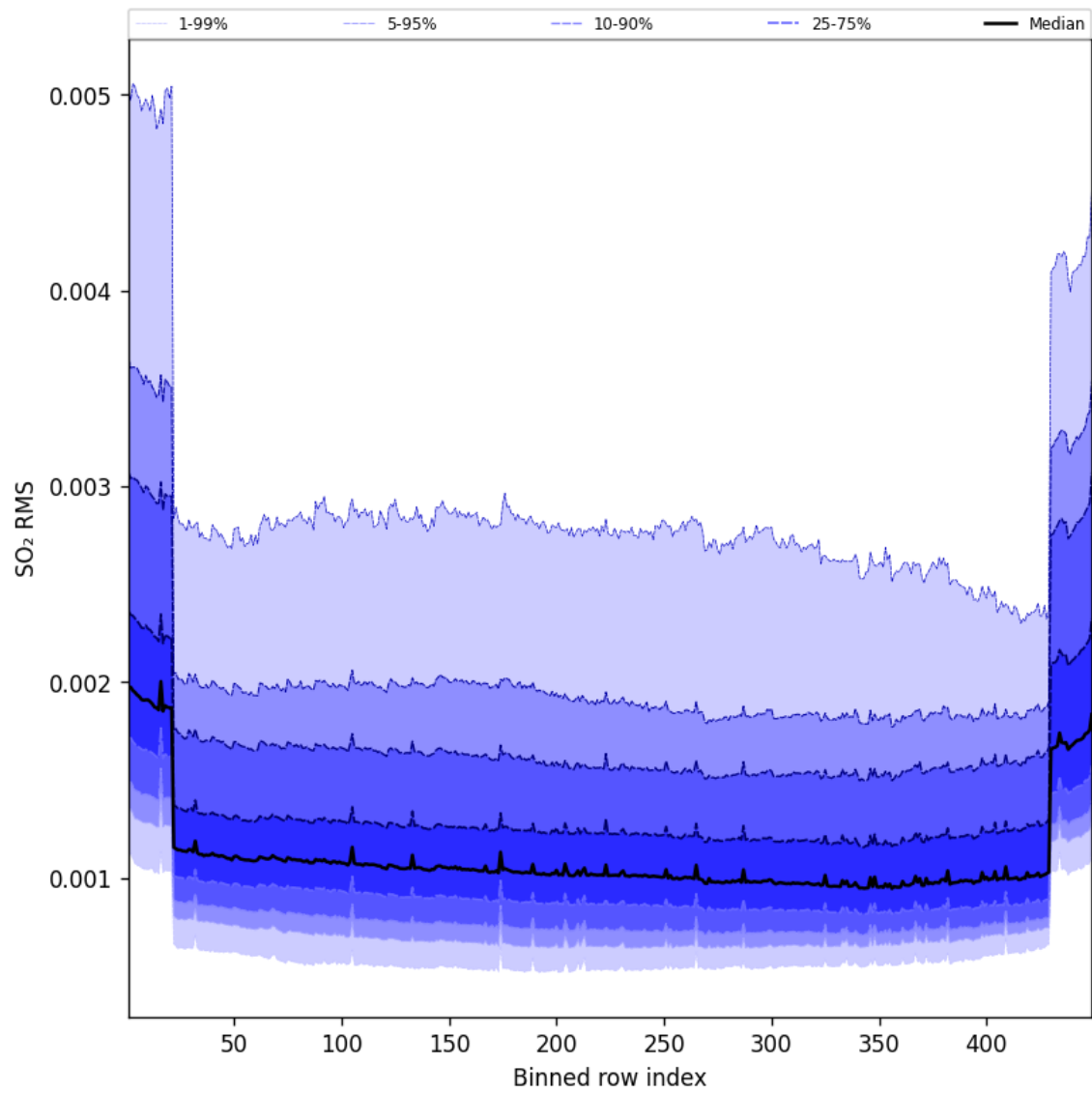
Figure 106: Along track statistics of “SO 2 RMS” for 2025-01-10 to 2025-01-10
