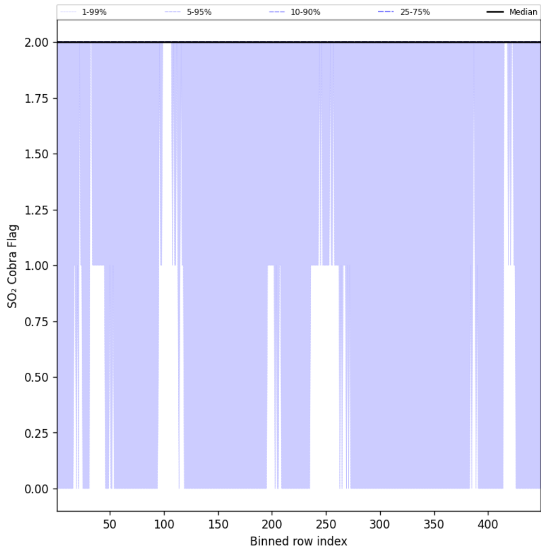
Figure 102: Along track statistics of “SO 2 Cobra Flag” for 2025-01-10 to 2025-01-10
