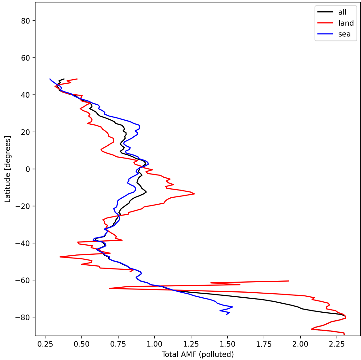
Figure 53: Zonal average of “Total AMF (polluted)” for 2025-01-10 to 2025-01-10.
