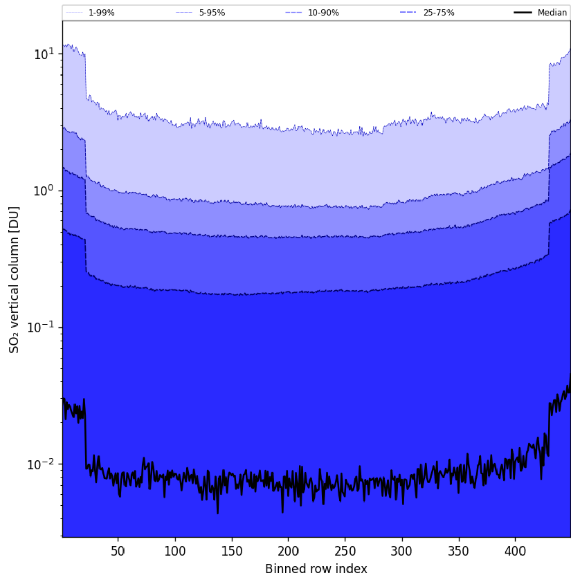
Figure 85: Along track statistics of “SO 2 vertical column” for 2025-01-10 to 2025-01-10
