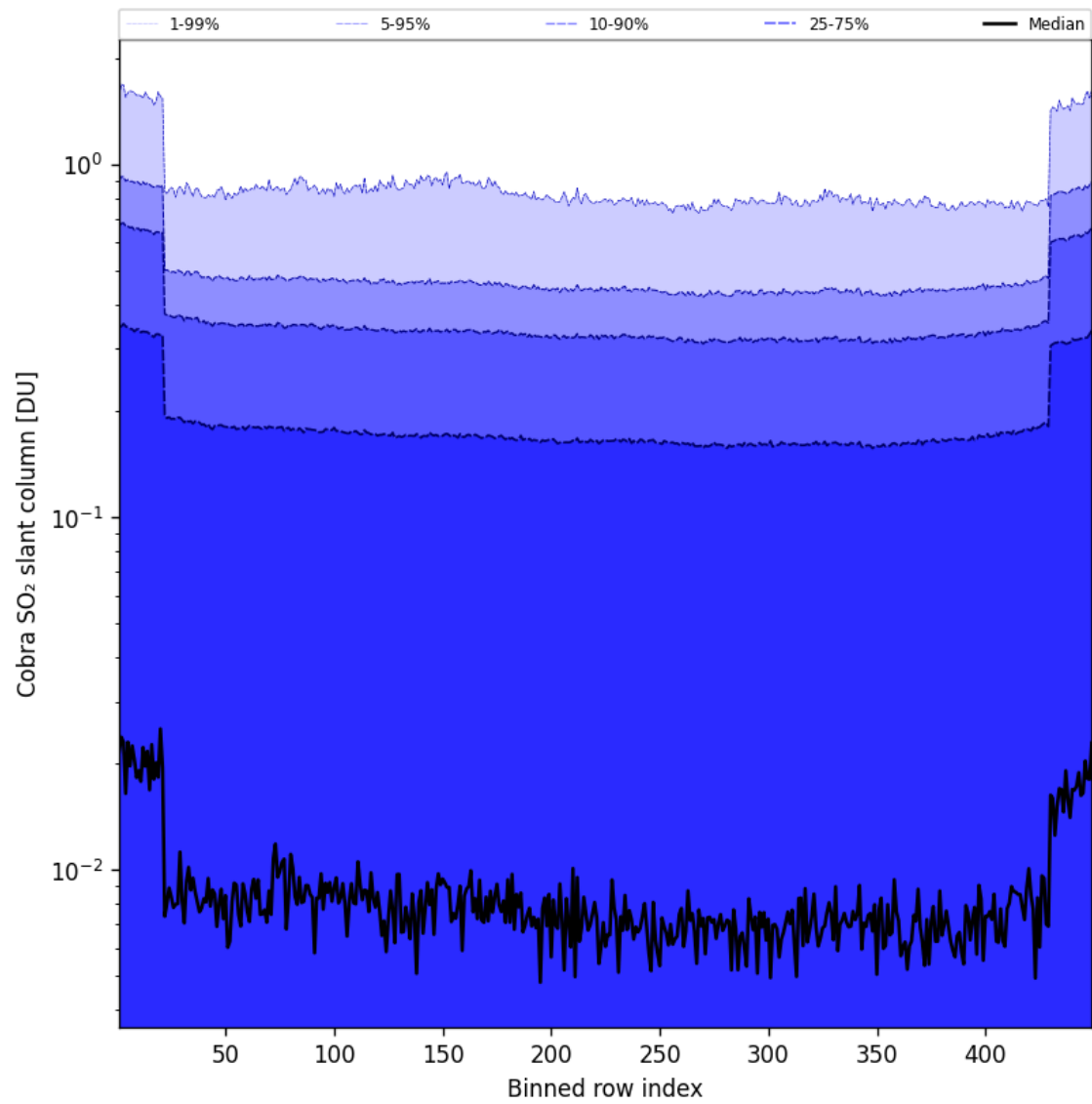
Figure 88: Along track statistics of “Cobra SO 2 slant column” for 2025-01-10 to 2025-01-10
