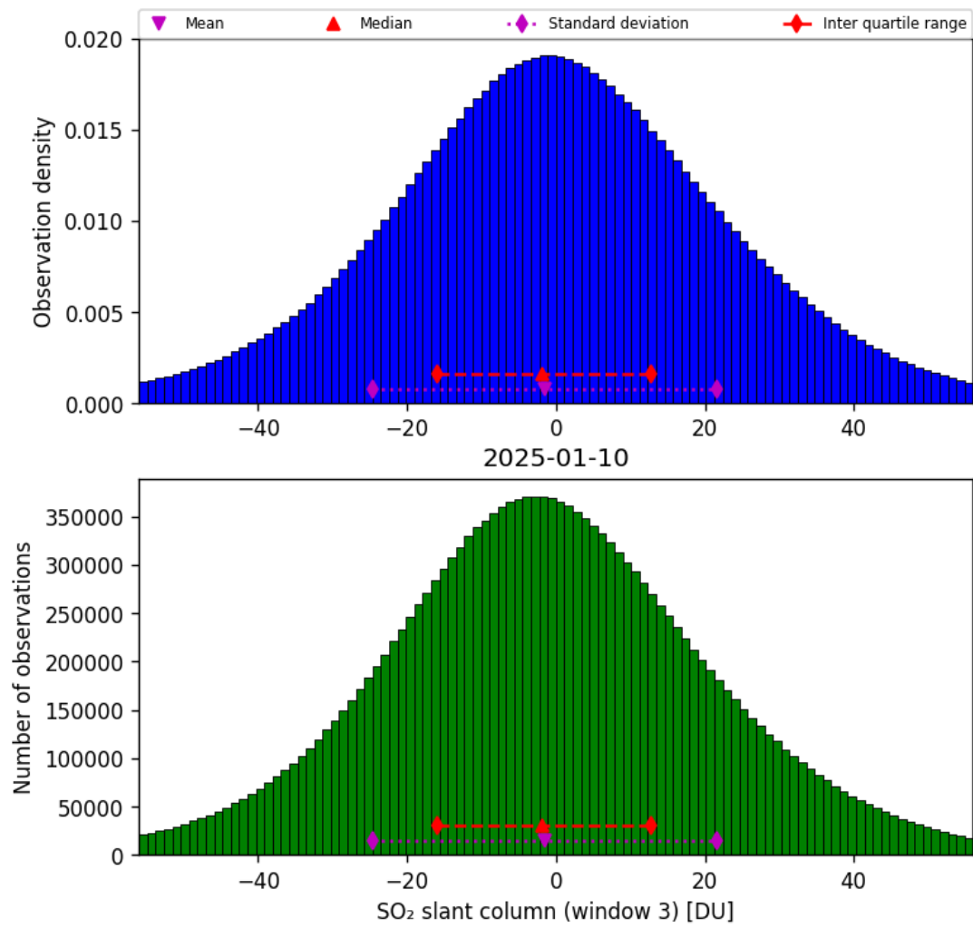
Figure 71: Histogram of “SO 2 slant column (window 3)” for 2025-01-10 to 2025-01-10
