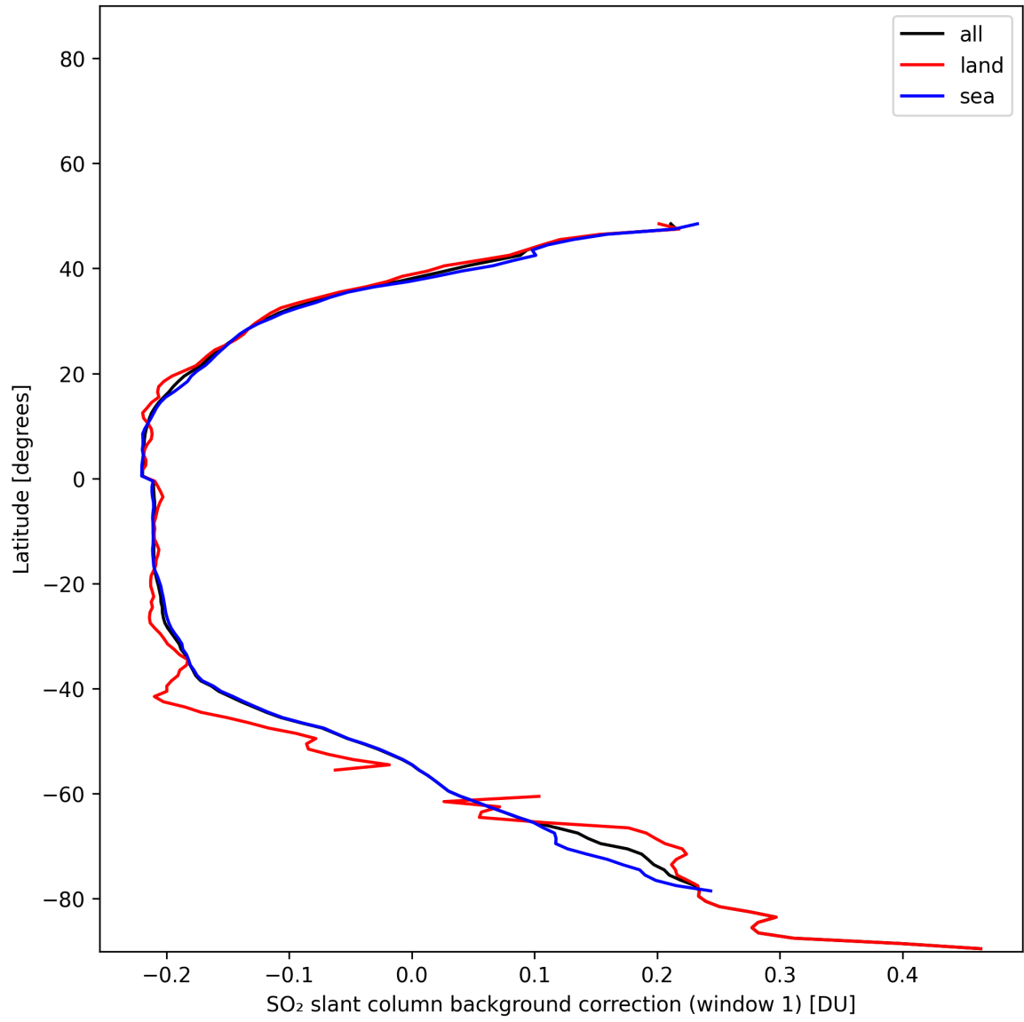
Figure 39: Zonal average of “SO 2 slant column background correction (window 1)” for 2025-01-10 to 2025-01-10.
