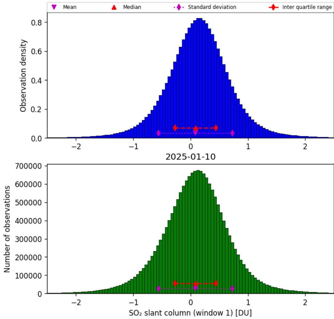
Figure 63: Histogram of “SO 2 slant column (window 1)” for 2025-01-10 to 2025-01-10
