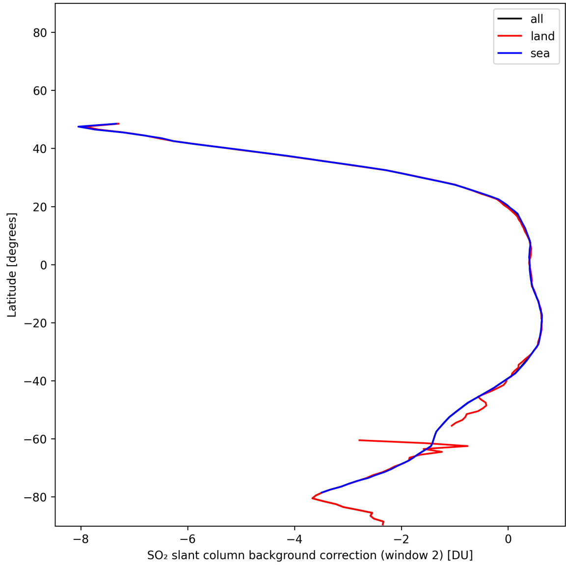
Figure 43: Zonal average of “SO 2 slant column background correction (window 2)” for 2025-01-10 to 2025-01-10.
