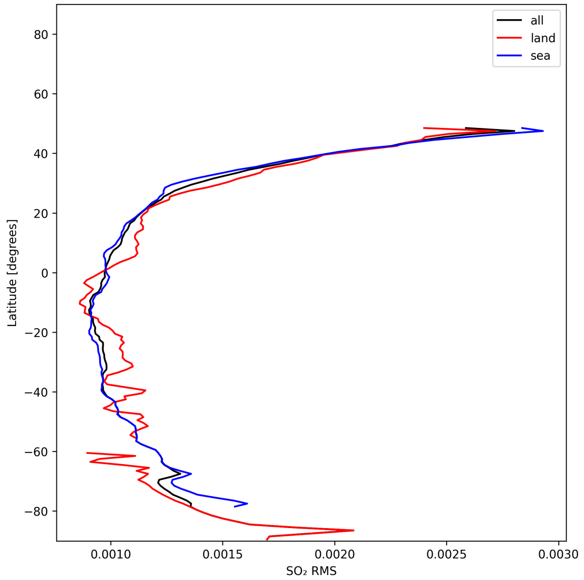
Figure 52: Zonal average of “SO 2 RMS” for 2025-01-10 to 2025-01-10.
