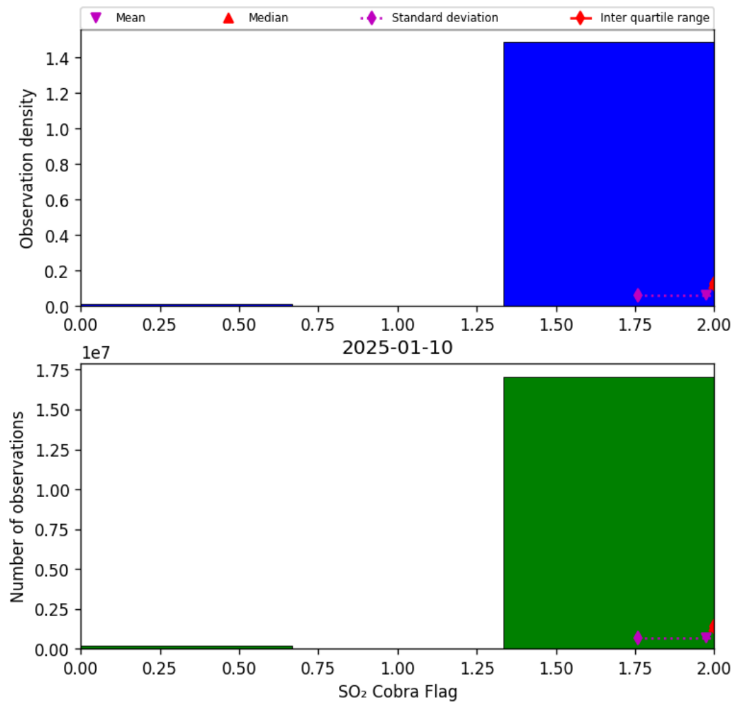
Figure 75: Histogram of “SO 2 Cobra Flag” for 2025-01-10 to 2025-01-10
