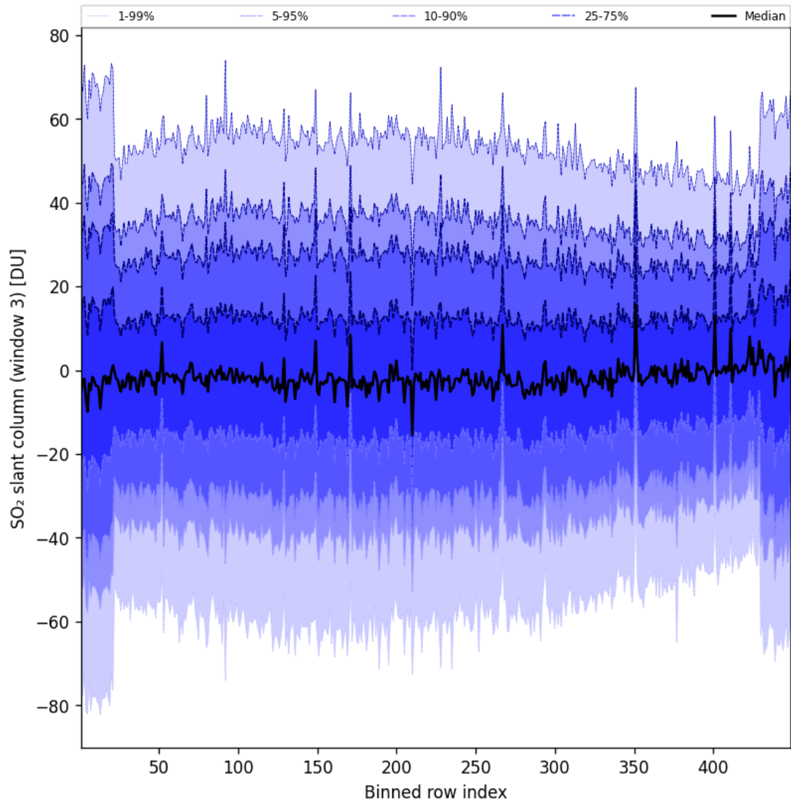
Figure 98: Along track statistics of “SO 2 slant column (window 3)” for 2025-01-10 to 2025-01-10
