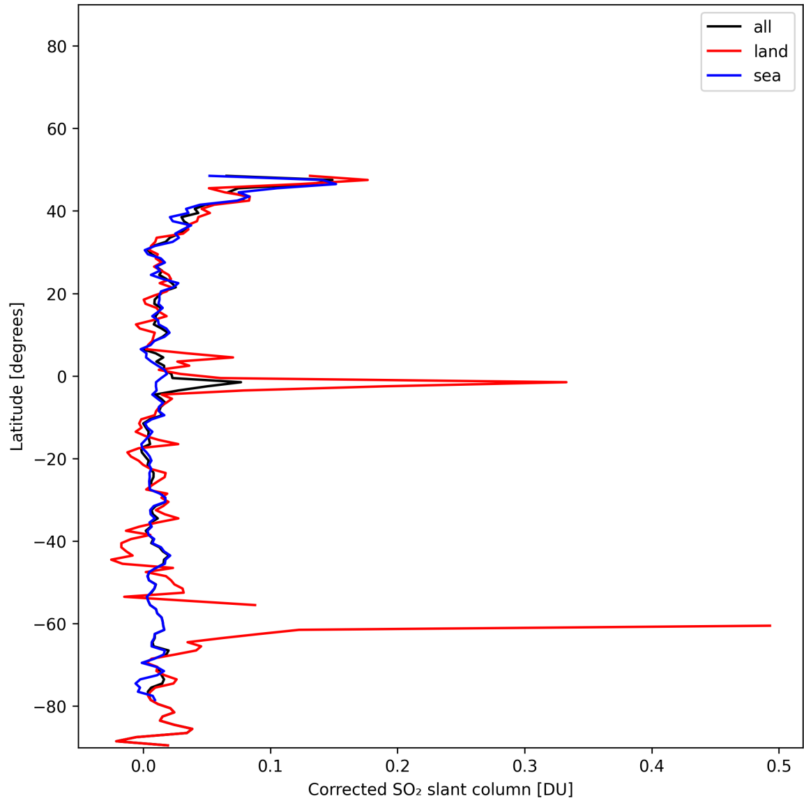
Figure 33: Zonal average of “Corrected SO 2 slant column” for 2025-01-10 to 2025-01-10.
