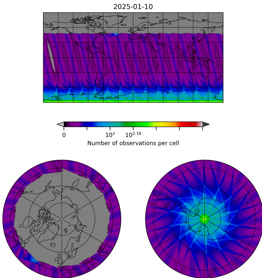
Figure 29: Map of the number of observations for 2025-01-10 to 2025-01-10
