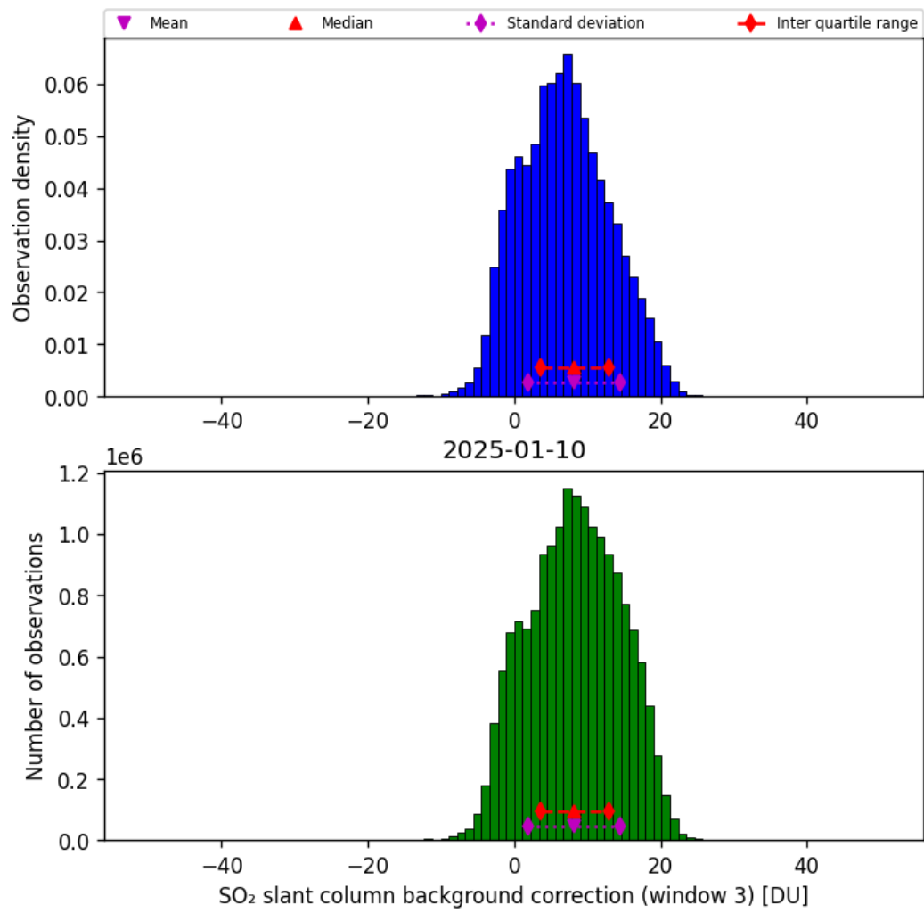
Figure 74: Histogram of “SO 2 slant column background correction (window 3)” for 2025-01-10 to 2025-01-10
