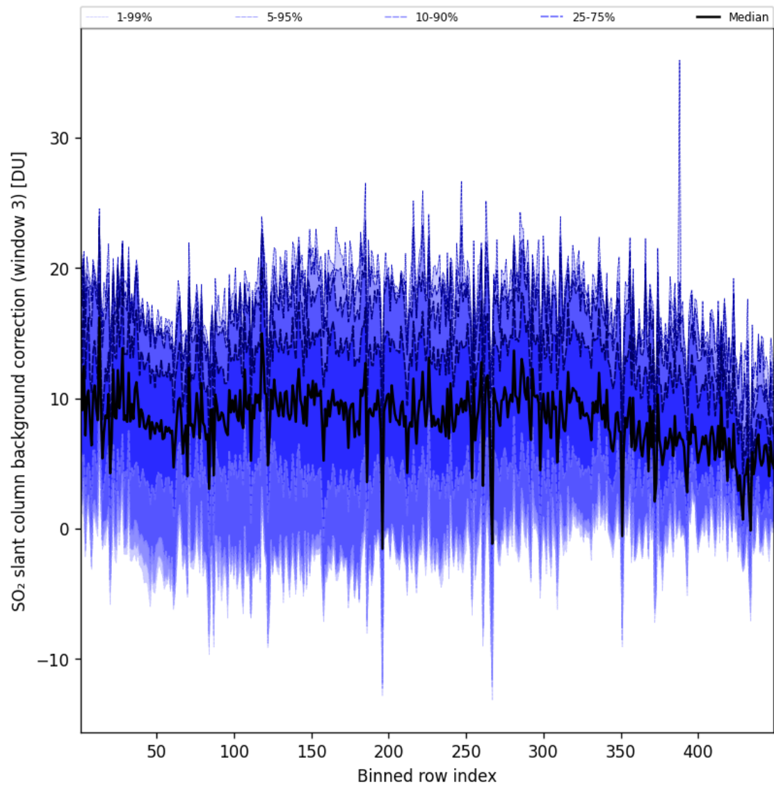
Figure 101: Along track statistics of "SO 2 slant column background correction (window 3)" for 2025-01-10 to 2025-01-10
