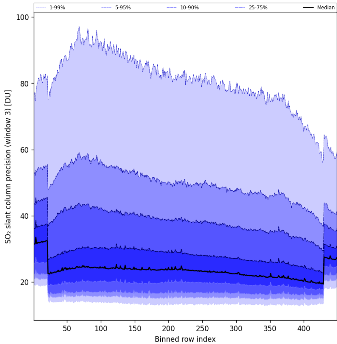
Figure 99: Along track statistics of “SO 2 slant column precision (window 3)” for 2025-01-10 to 2025-01-10
