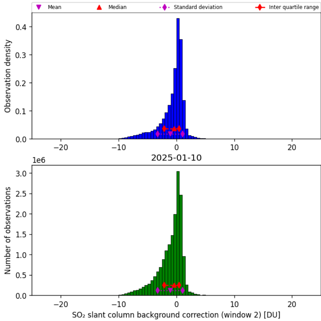
Figure 70: Histogram of “SO 2 slant column background correction (window 2)” for 2025-01-10 to 2025-01-10
