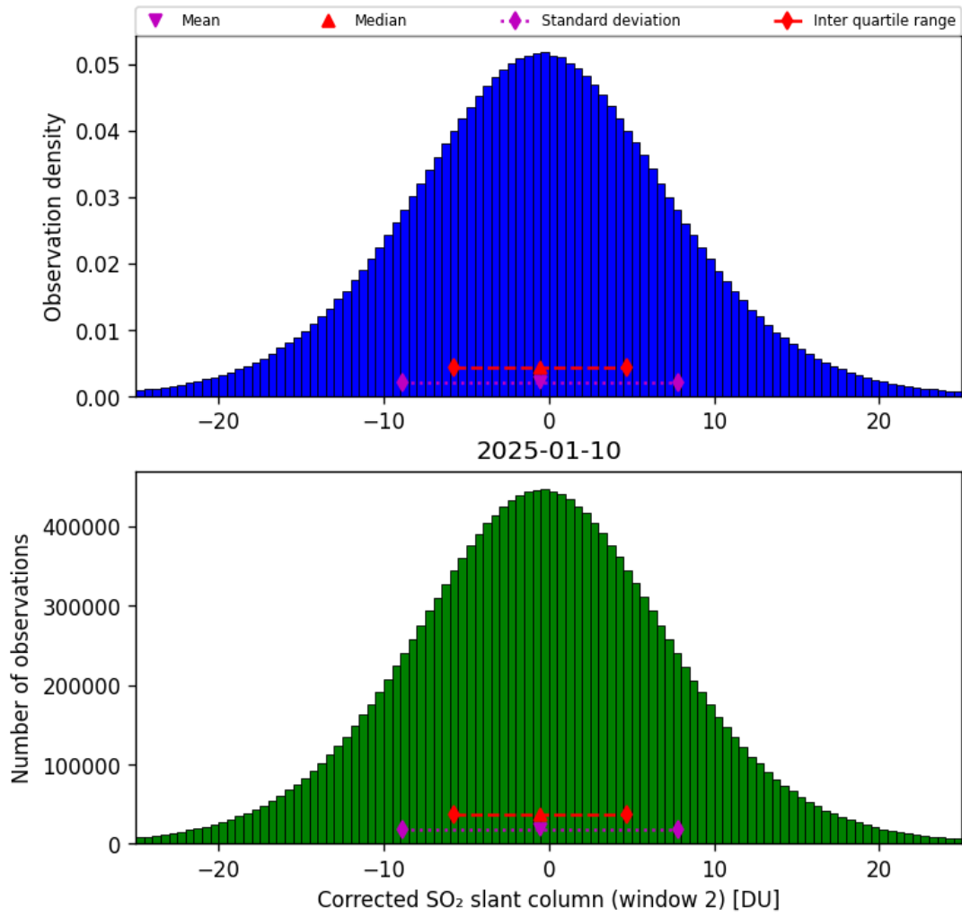
Figure 69: Histogram of “Corrected SO 2 slant column (window 2)” for 2025-01-10 to 2025-01-10
