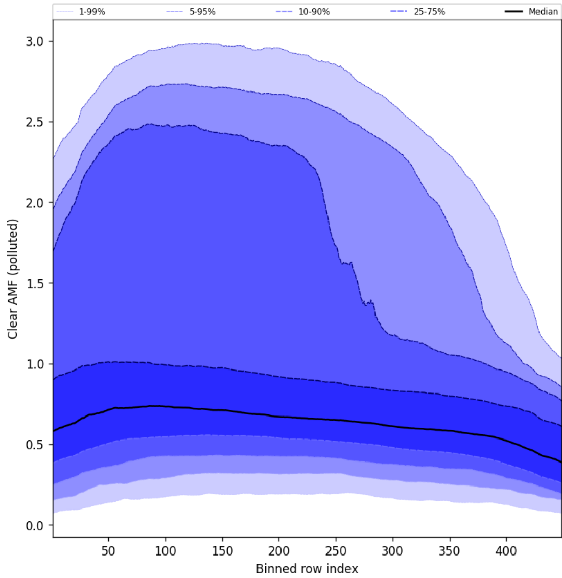
Figure 109: Along track statistics of “Clear AMF (polluted)” for 2025-01-10 to 2025-01-10
