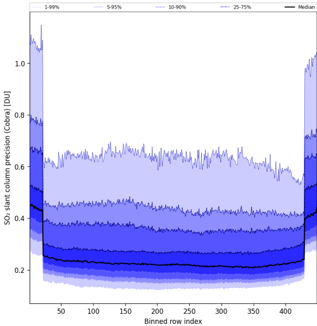
Figure 89: Along track statistics of “SO 2 slant column precision (Cobra)” for 2025-01-10 to 2025-01-10
