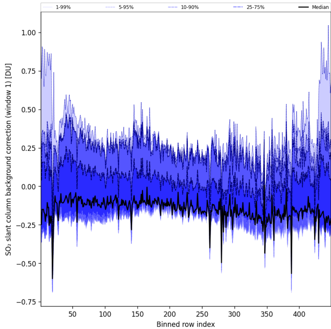
Figure 93: Along track statistics of “SO 2 slant column background correction (window 1)” for 2025-01-10 to 2025-01-10
