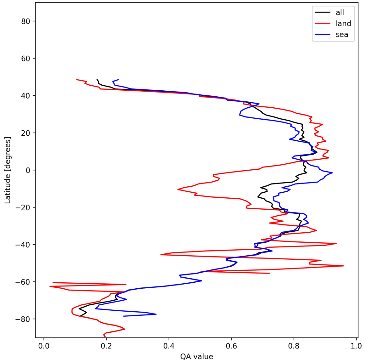
Figure 30: Zonal average of “QA value” for 2025-01-10 to 2025-01-10.
