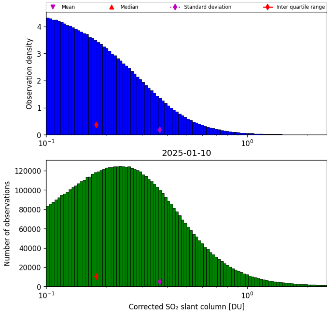
Figure 60: Histogram of “Corrected SO 2 slant column” for 2025-01-10 to 2025-01-10
