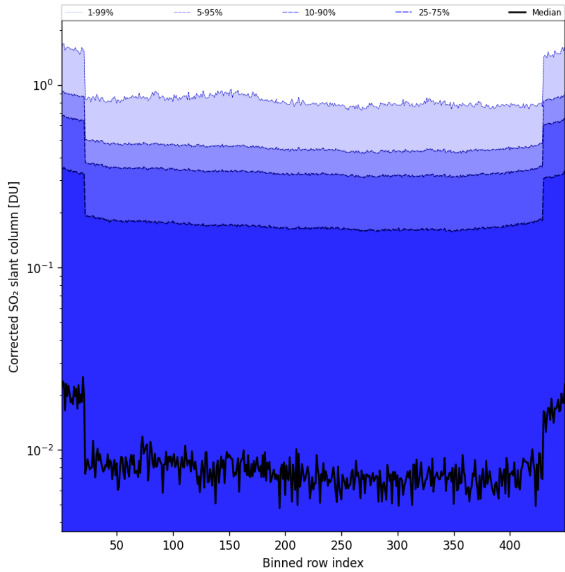
Figure 87: Along track statistics of “Corrected SO 2 slant column” for 2025-01-10 to 2025-01-10
