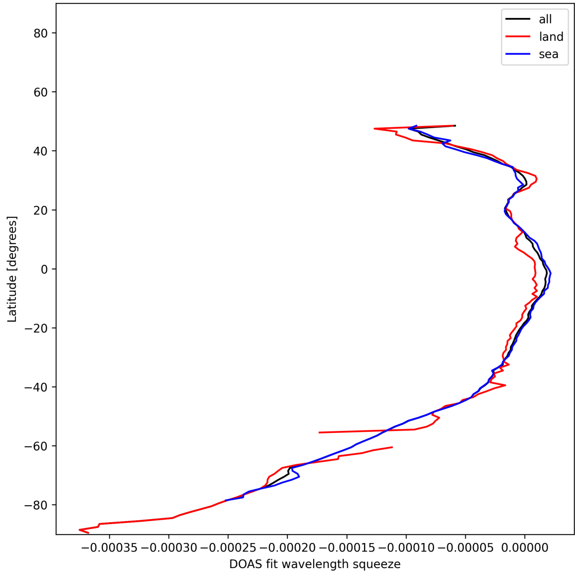
Figure 51: Zonal average of “DOAS fit wavelength squeeze” for 2025-01-10 to 2025-01-10.
