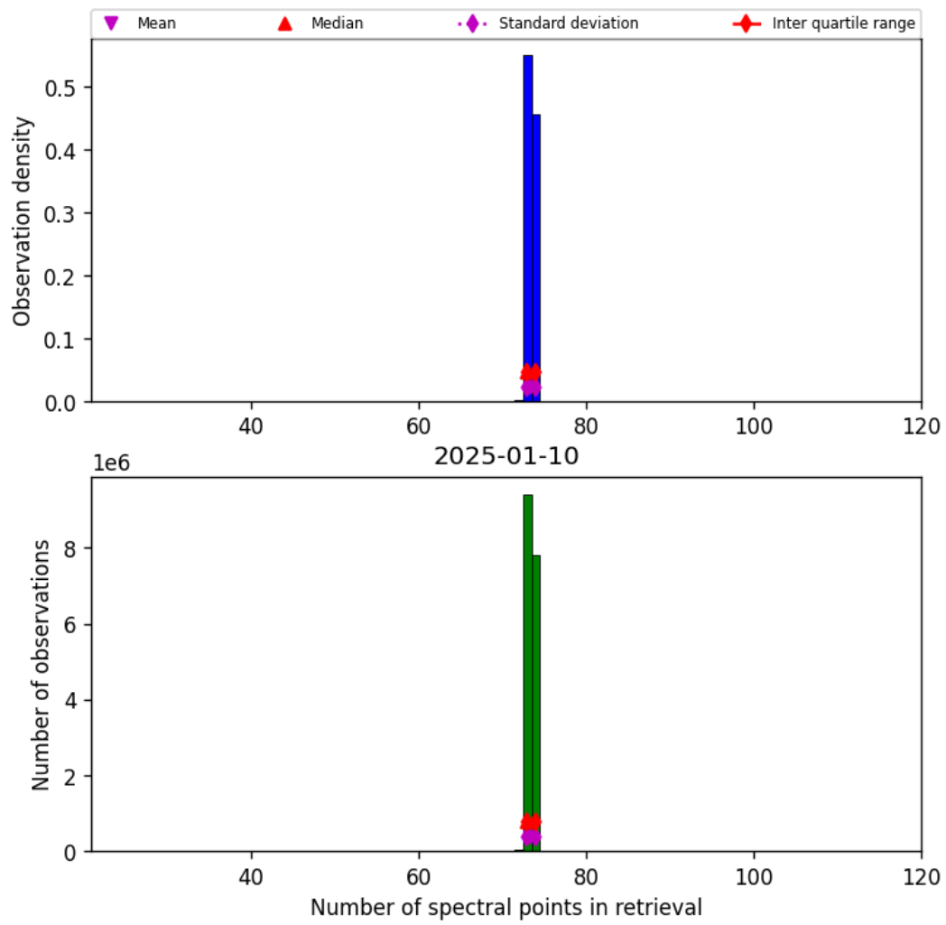
Figure 83: Histogram of “Number of spectral points in retrieval” for 2025-01-10 to 2025-01-10
