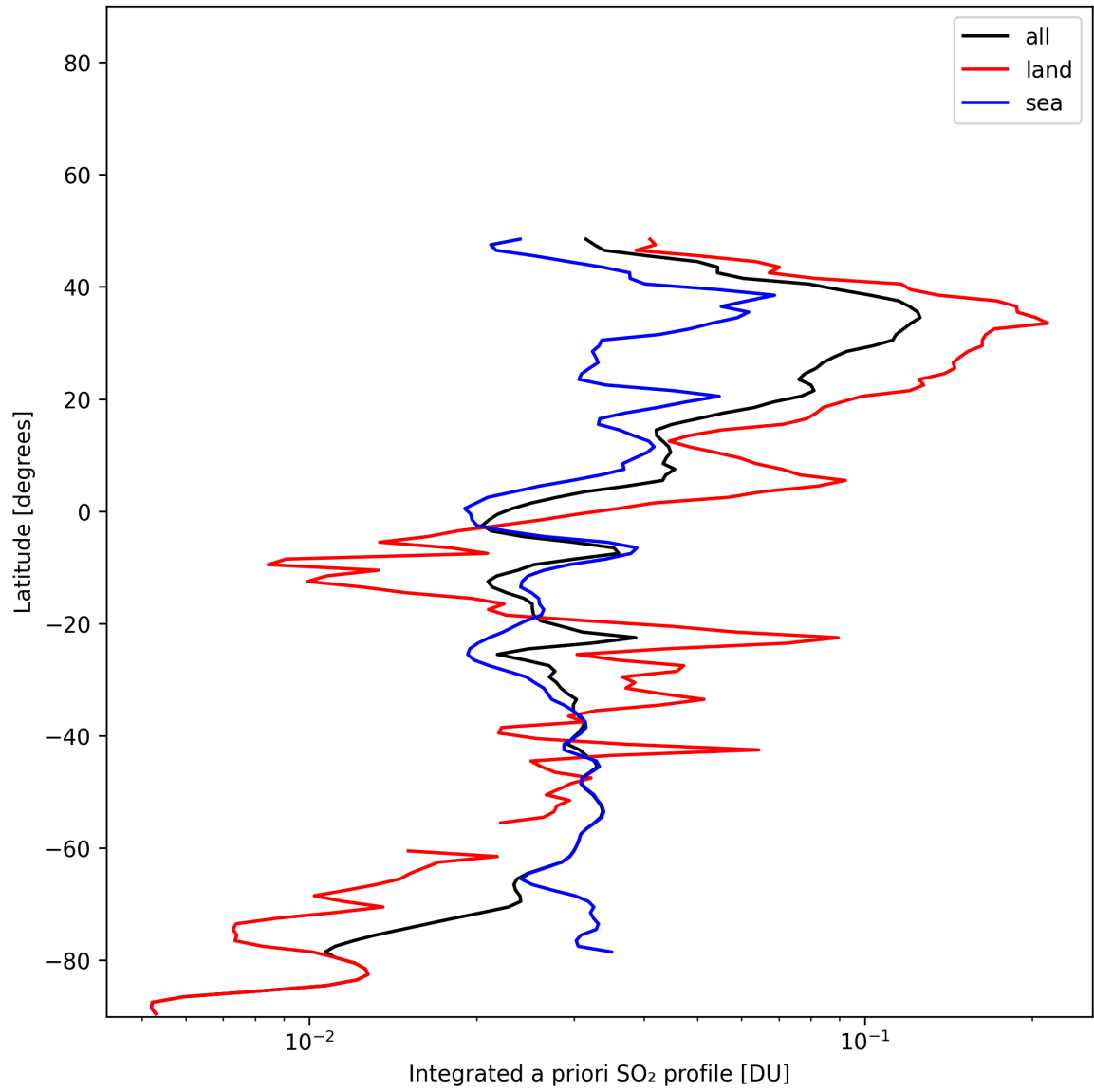
Figure 49: Zonal average of “Integrated a priori SO 2 profile” for 2025-01-10 to 2025-01-10.
