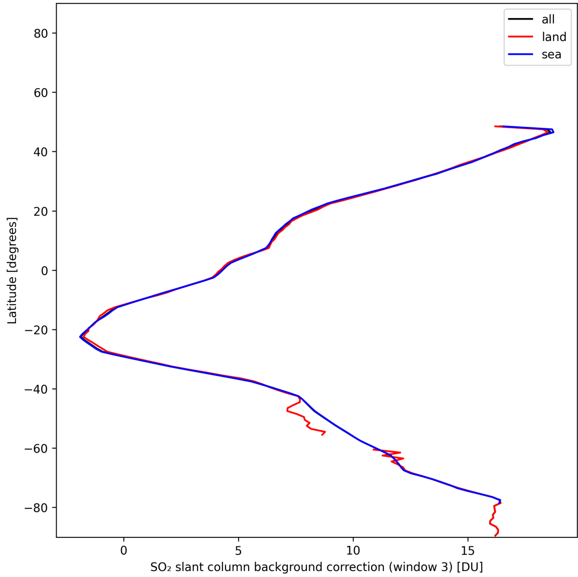
Figure 47: Zonal average of “SO 2 slant column background correction (window 3)” for 2025-01-10 to 2025-01-10.
