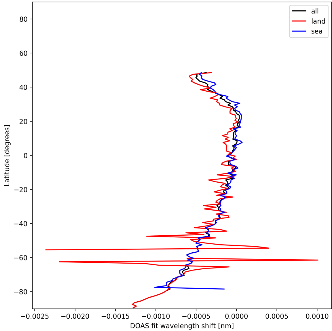
Figure 50: Zonal average of “DOAS fit wavelength shift” for 2025-01-10 to 2025-01-10.
