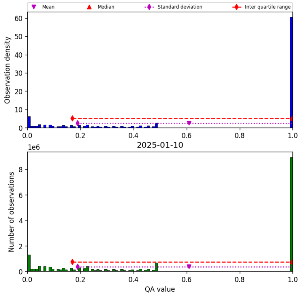
Figure 57: Histogram of “QA value” for 2025-01-10 to 2025-01-10
