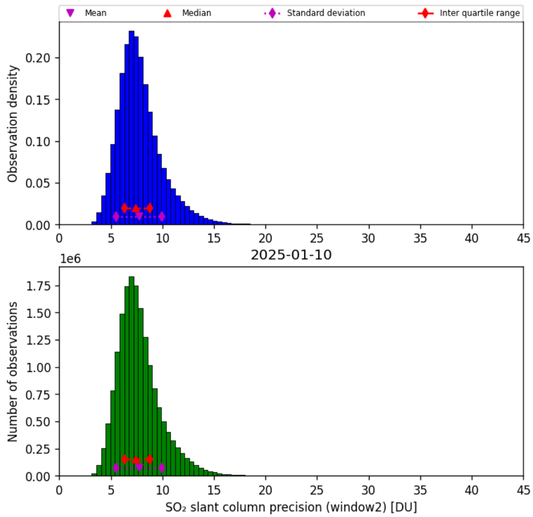
Figure 68: Histogram of “SO 2 slant column precision (window2)” for 2025-01-10 to 2025-01-10
