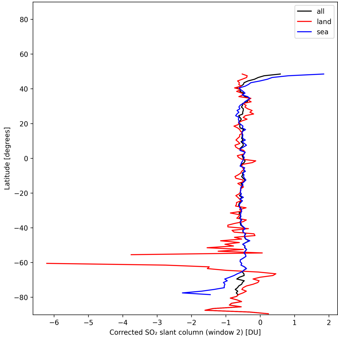
Figure 42: Zonal average of “Corrected SO 2 slant column (window 2)” for 2025-01-10 to 2025-01-10.
