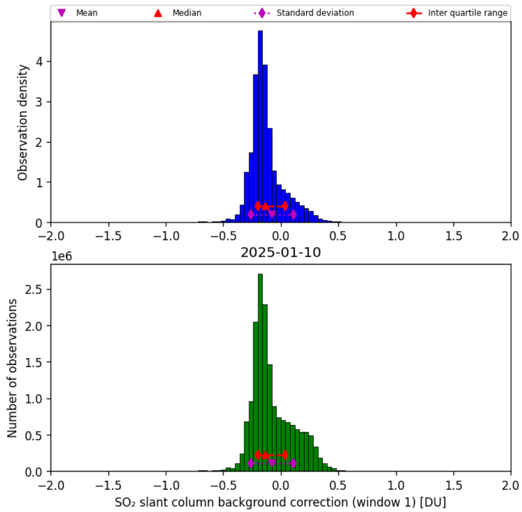
Figure 66: Histogram of “SO 2 slant column background correction (window 1)” for 2025-01-10 to 2025-01-10
