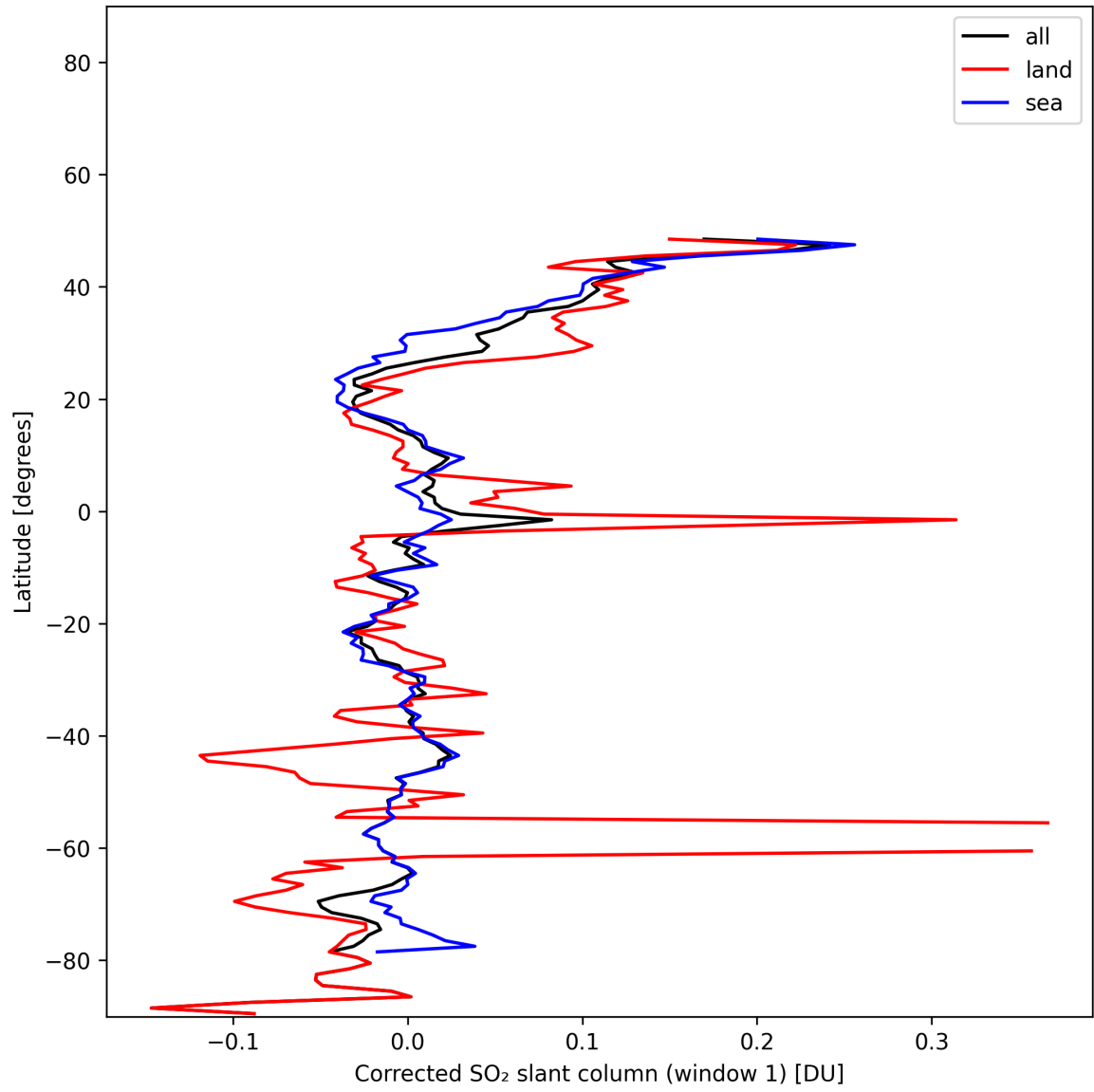
Figure 38: Zonal average of “Corrected SO 2 slant column (window 1)” for 2025-01-10 to 2025-01-10.
