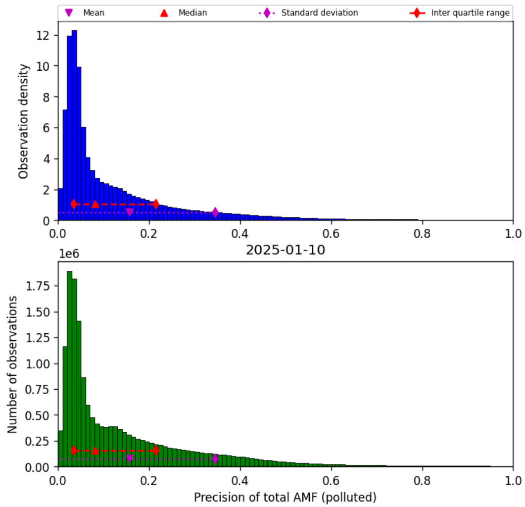
Figure 81: Histogram of “Precision of total AMF (polluted)” for 2025-01-10 to 2025-01-10
