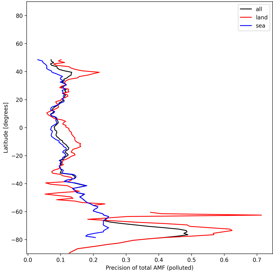
Figure 54: Zonal average of “Precision of total AMF (polluted)” for 2025-01-10 to 2025-01-10.
