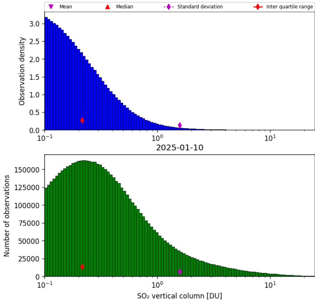
Figure 58: Histogram of “SO 2 vertical column” for 2025-01-10 to 2025-01-10
