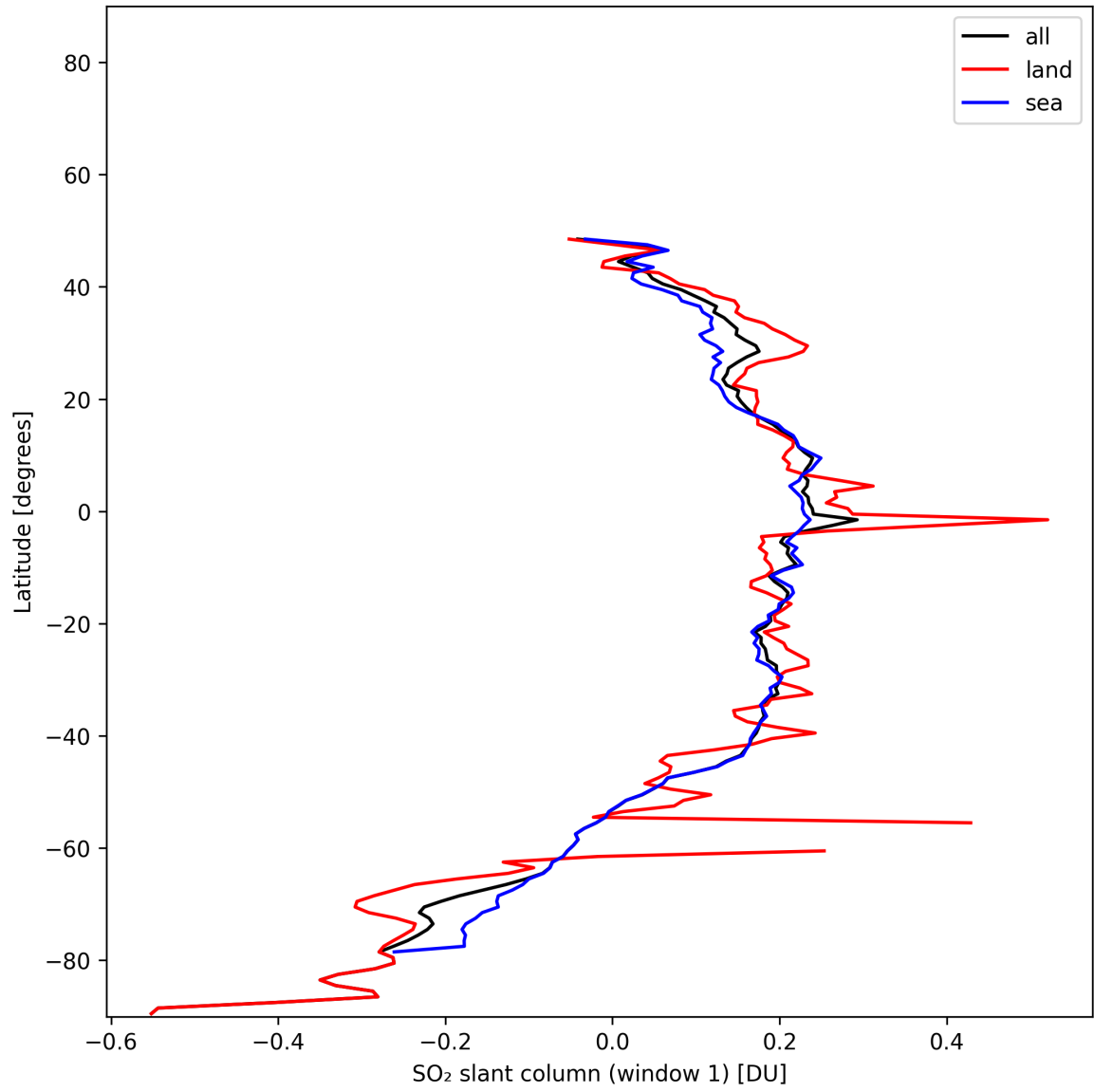
Figure 36: Zonal average of “SO 2 slant column (window 1)” for 2025-01-10 to 2025-01-10.
