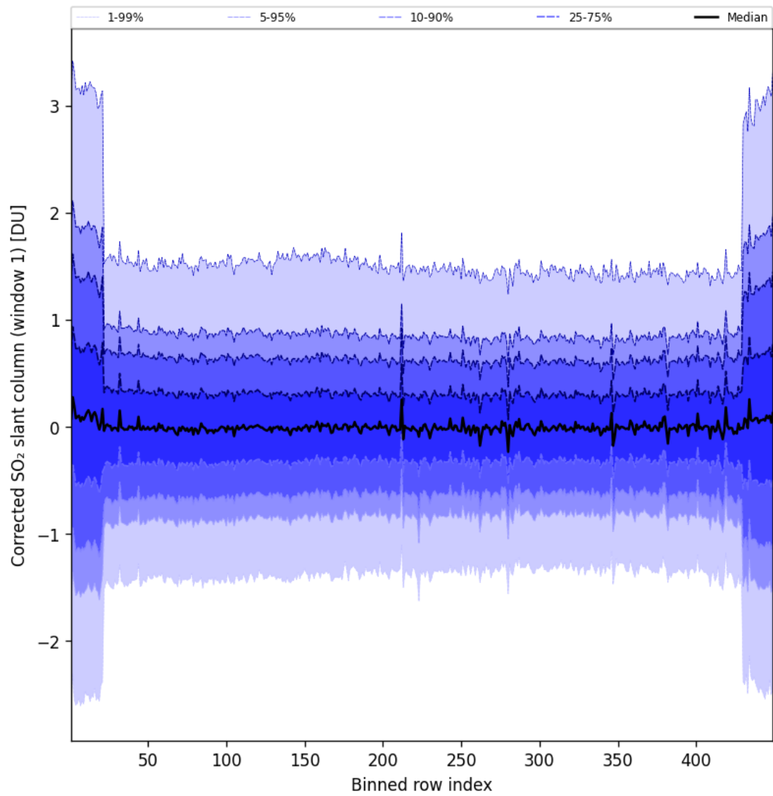
Figure 92: Along track statistics of “Corrected SO 2 slant column (window 1)” for 2025-01-10 to 2025-01-10
