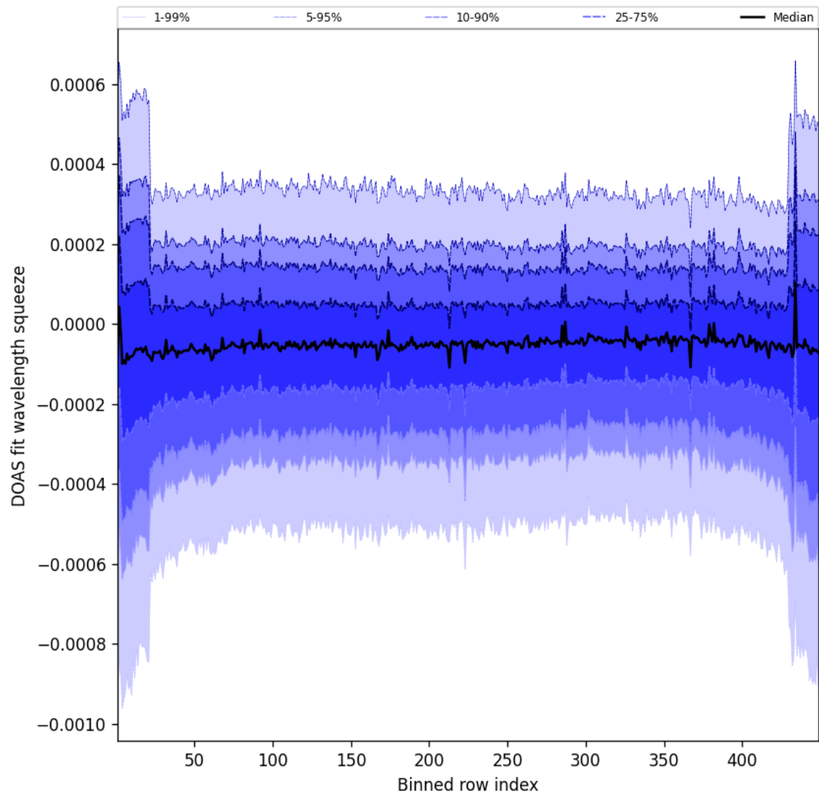
Figure 105: Along track statistics of “DOAS fit wavelength squeeze” for 2025-01-10 to 2025-01-10
