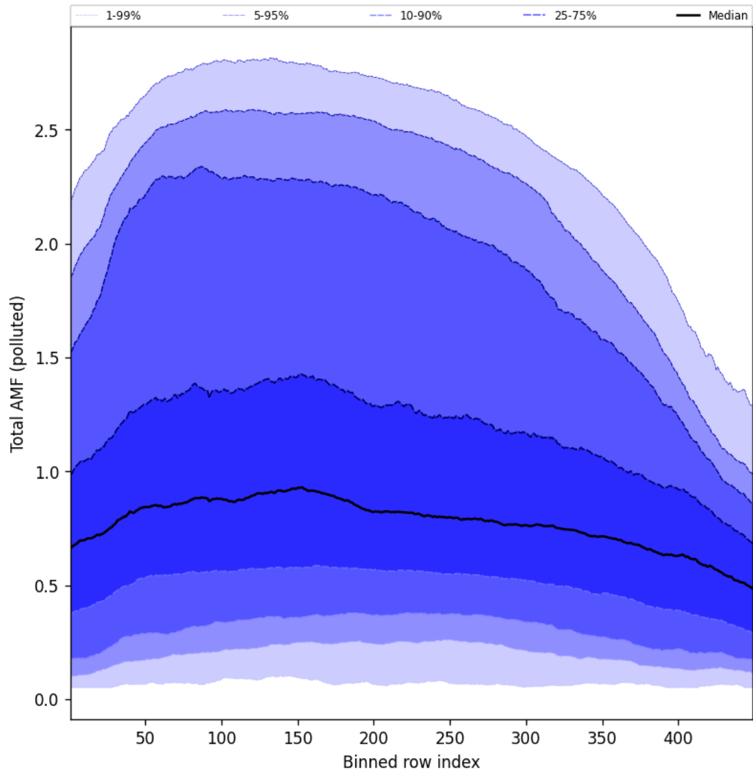
Figure 107: Along track statistics of “Total AMF (polluted)” for 2025-01-10 to 2025-01-10
