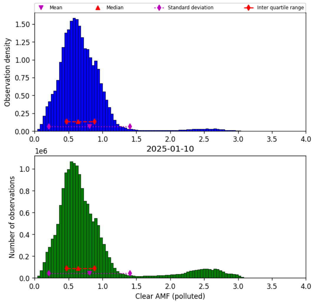
Figure 82: Histogram of “Clear AMF (polluted)” for 2025-01-10 to 2025-01-10
