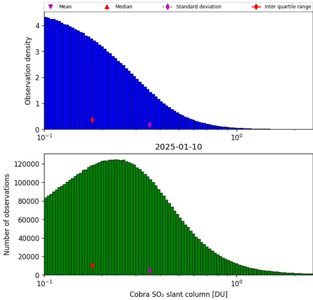
Figure 61: Histogram of “Cobra SO 2 slant column” for 2025-01-10 to 2025-01-10
