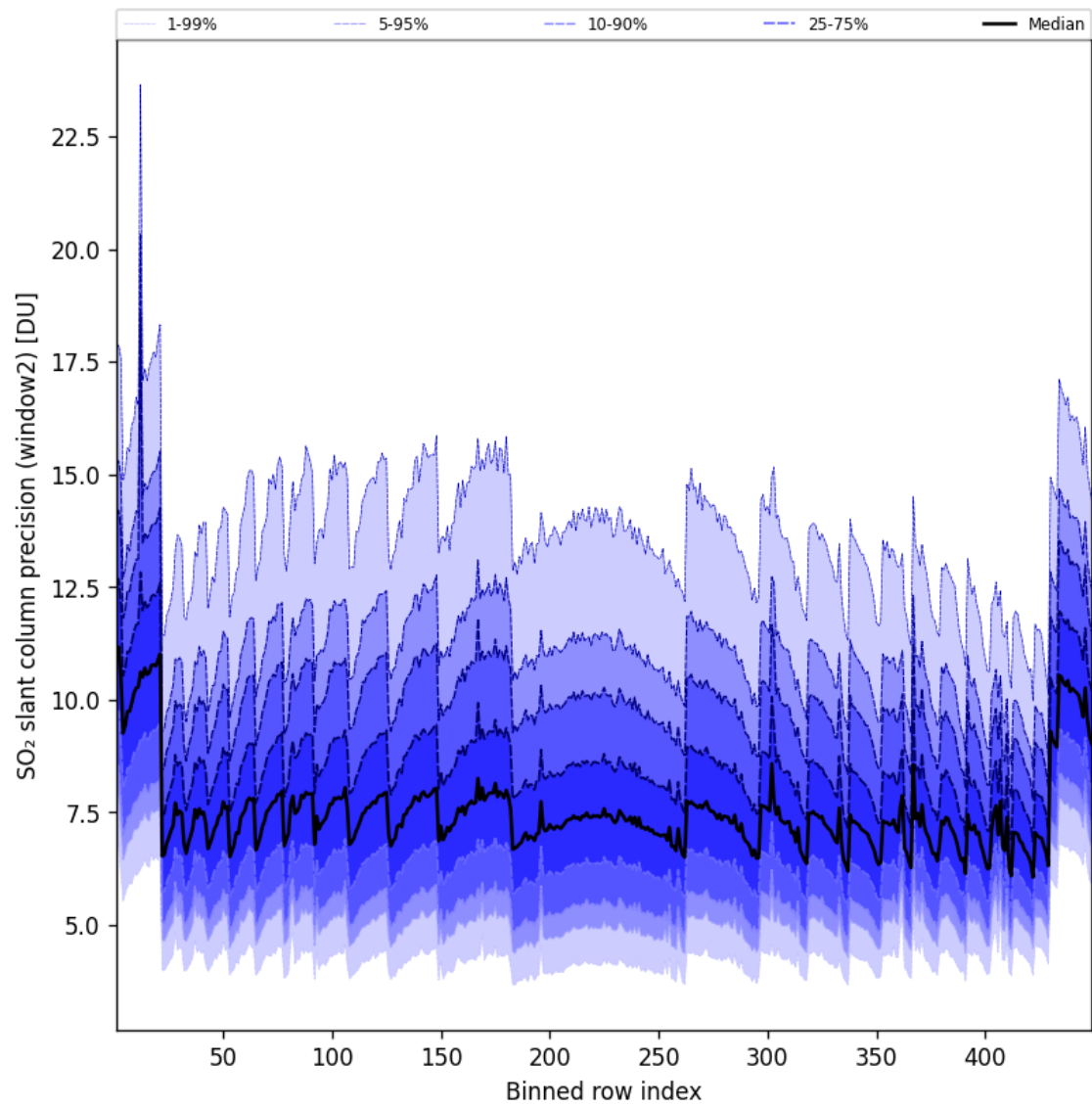
Figure 95: Along track statistics of “SO 2 slant column precision (window2)” for 2025-01-10 to 2025-01-10
